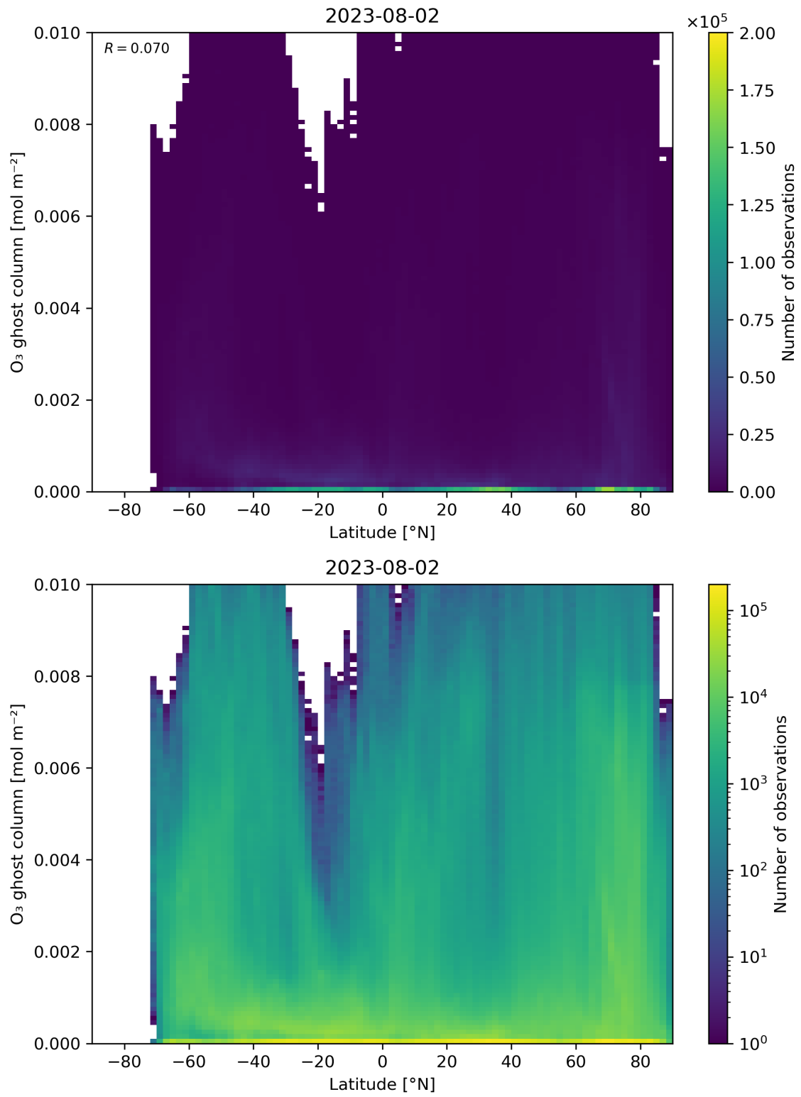
Figure 35: Scatter density plot of “Latitude” against “O 3 ghost column” for 2023-08-01 to 2023-08-03.
