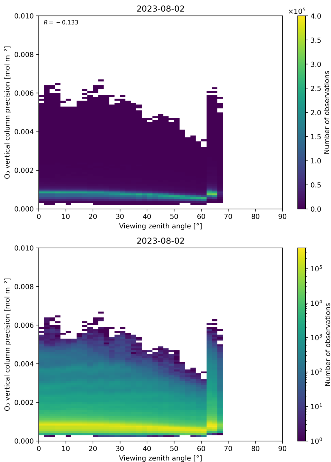
Figure 53: Scatter density plot of “Viewing zenith angle” against “O 3 vertical column precision” for 2023-08-01 to 2023-08-03.
