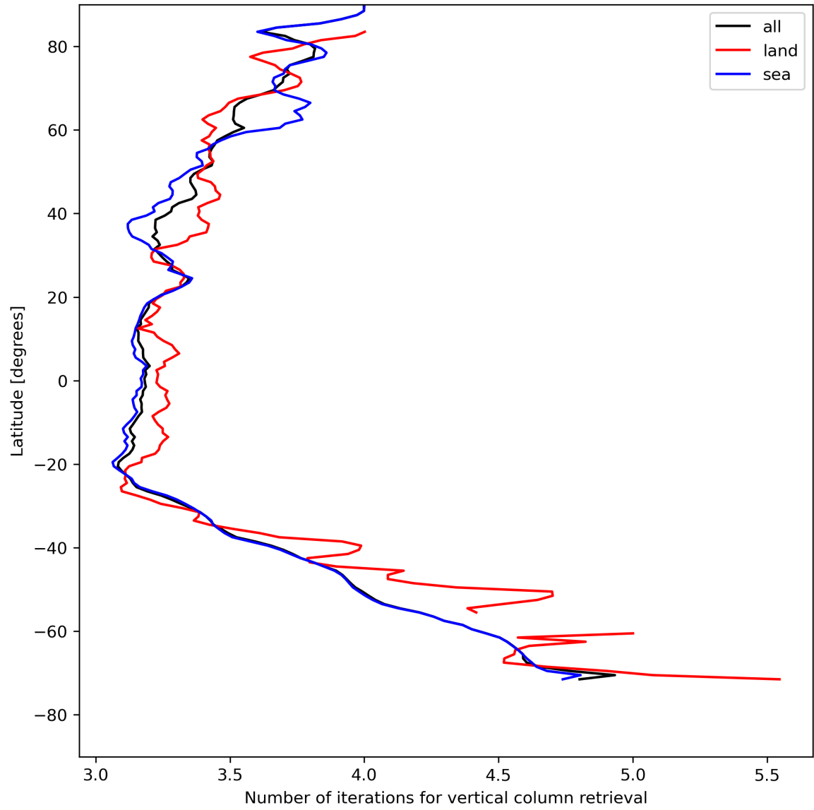
Figure 19: Zonal average of “Number of iterations for vertical column retrieval” for 2023-08-01 to 2023-08-03.
