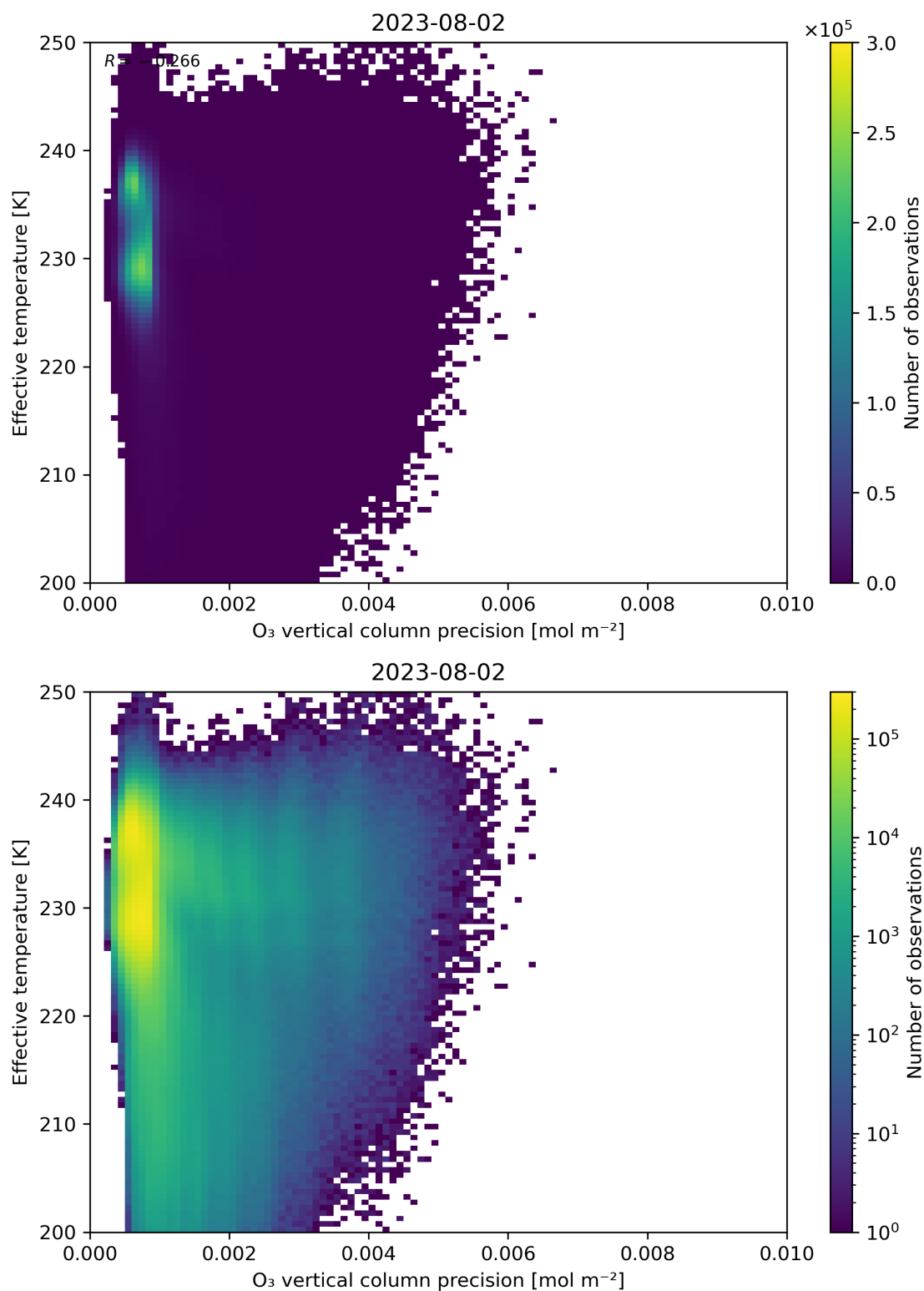
Figure 42: Scatter density plot of “O 3 vertical column precision” against “Effective temperature” for 2023-08-01 to 2023-08-03.
