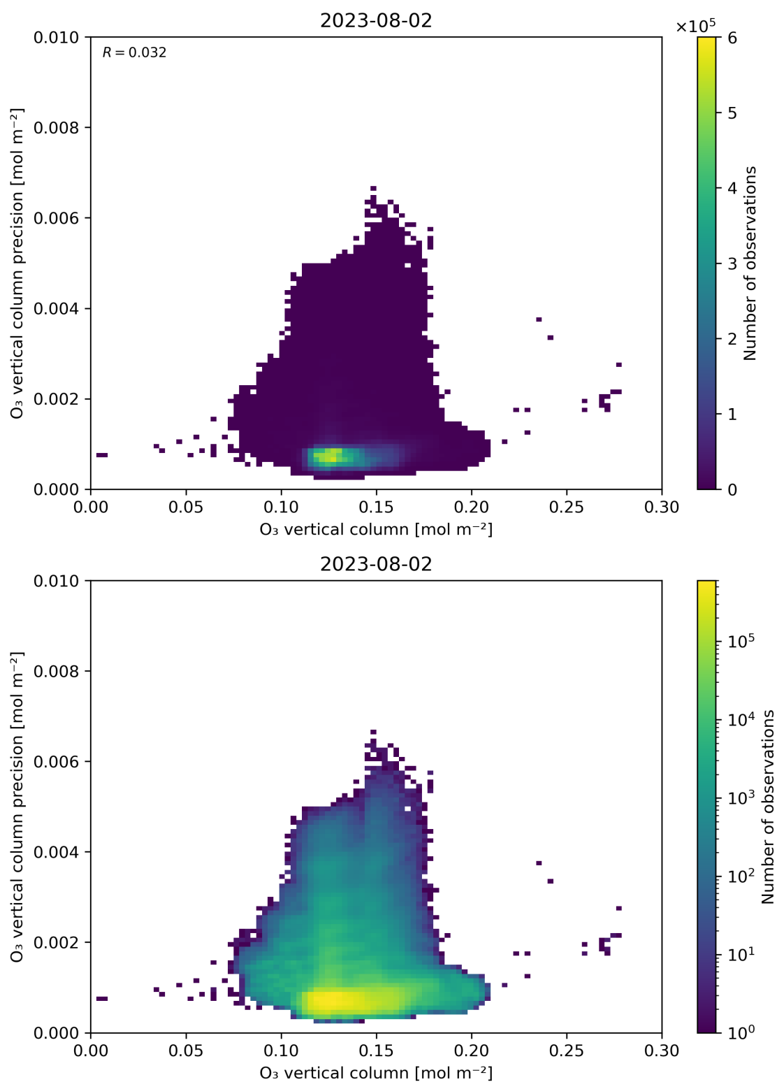
Figure 41: Scatter density plot of “O 3 vertical column” against “O 3 vertical column precision” for 2023-08-01 to 2023-08-03.
