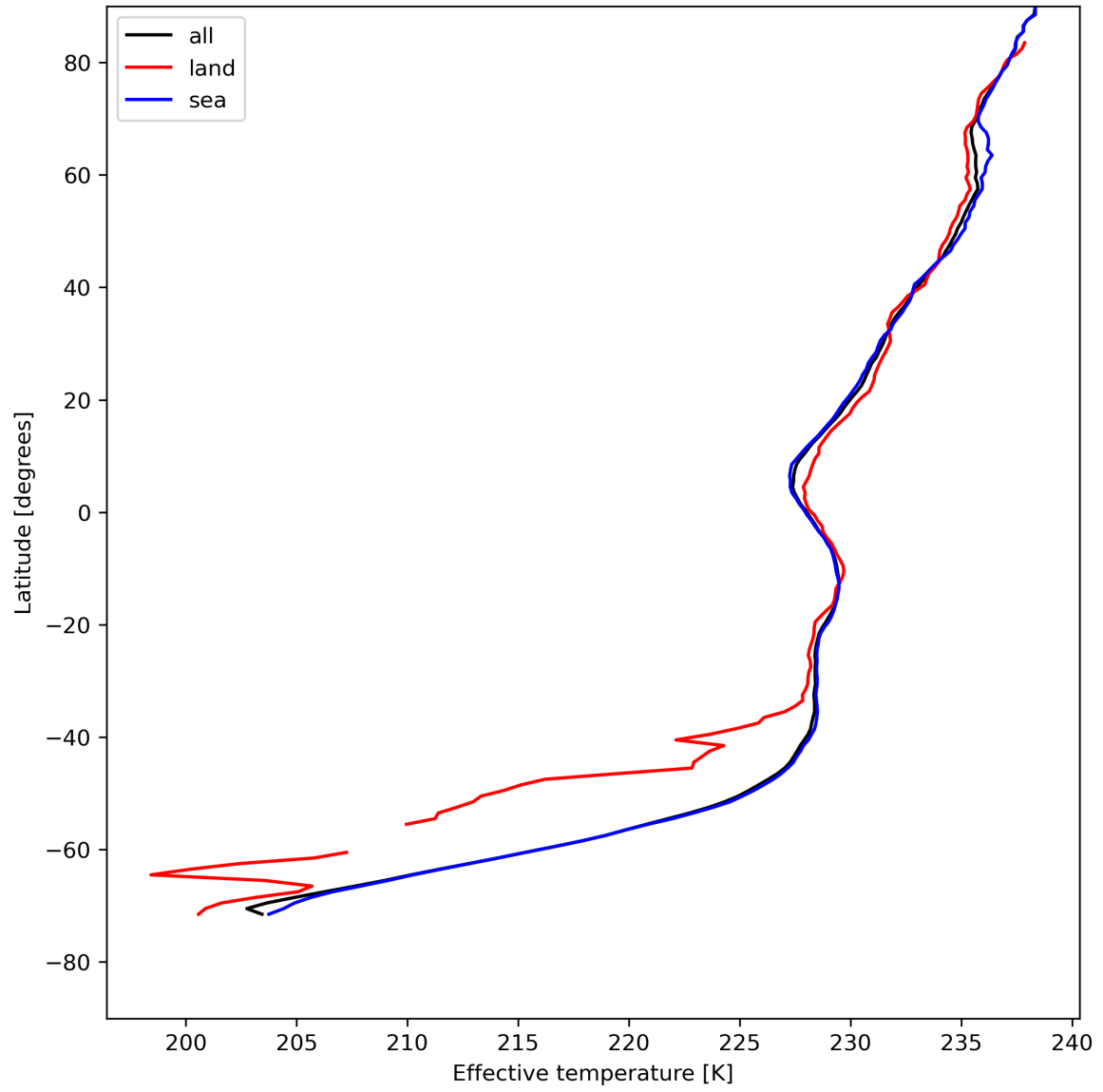
Figure 17: Zonal average of “Effective temperature” for 2023-08-01 to 2023-08-03.
