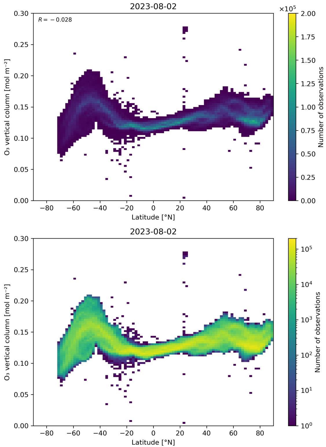
Figure 36: Scatter density plot of “Latitude” against “O 3 vertical column” for 2023-08-01 to 2023-08-03.
