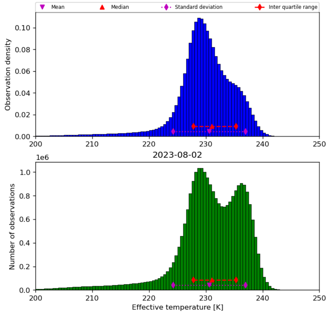
Figure 24: Histogram of “Effective temperature” for 2023-08-01 to 2023-08-03
