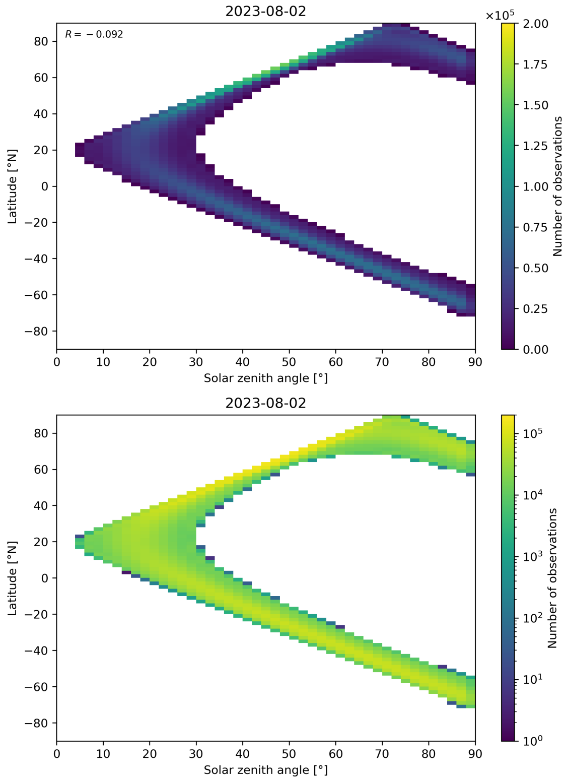
Figure 44: Scatter density plot of “Solar zenith angle” against “Latitude” for 2023-08-01 to 2023-08-03.
