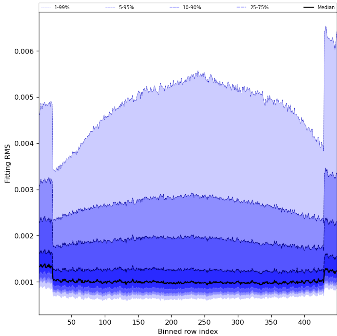
Figure 30: Along track statistics of “Fitting RMS” for 2023-08-01 to 2023-08-03
