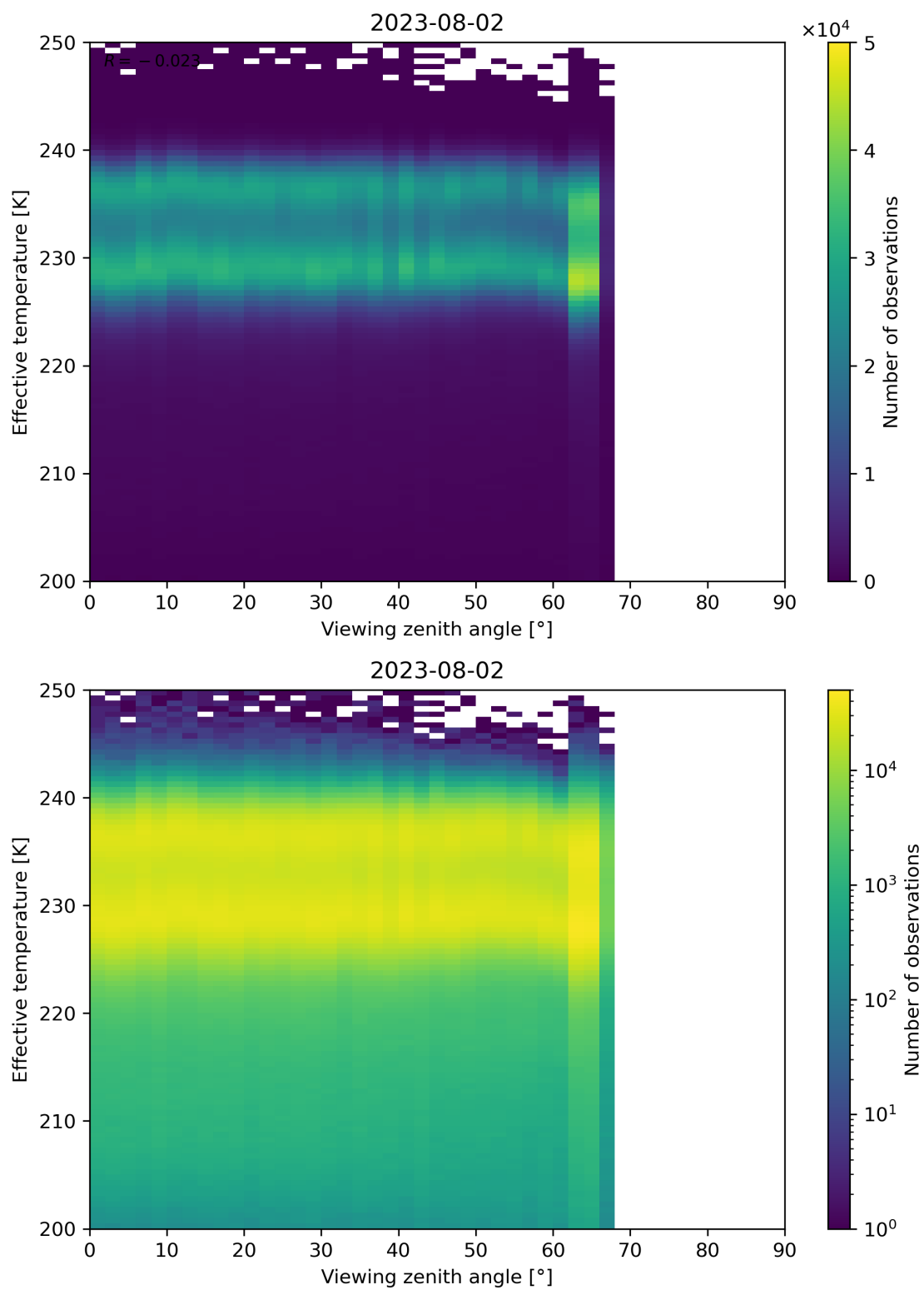
Figure 50: Scatter density plot of “Viewing zenith angle” against “Effective temperature” for 2023-08-01 to 2023-08-03.
