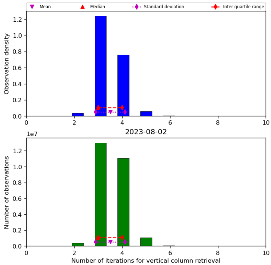
Figure 26: Histogram of “Number of iterations for vertical column retrieval” for 2023-08-01 to 2023-08-03
