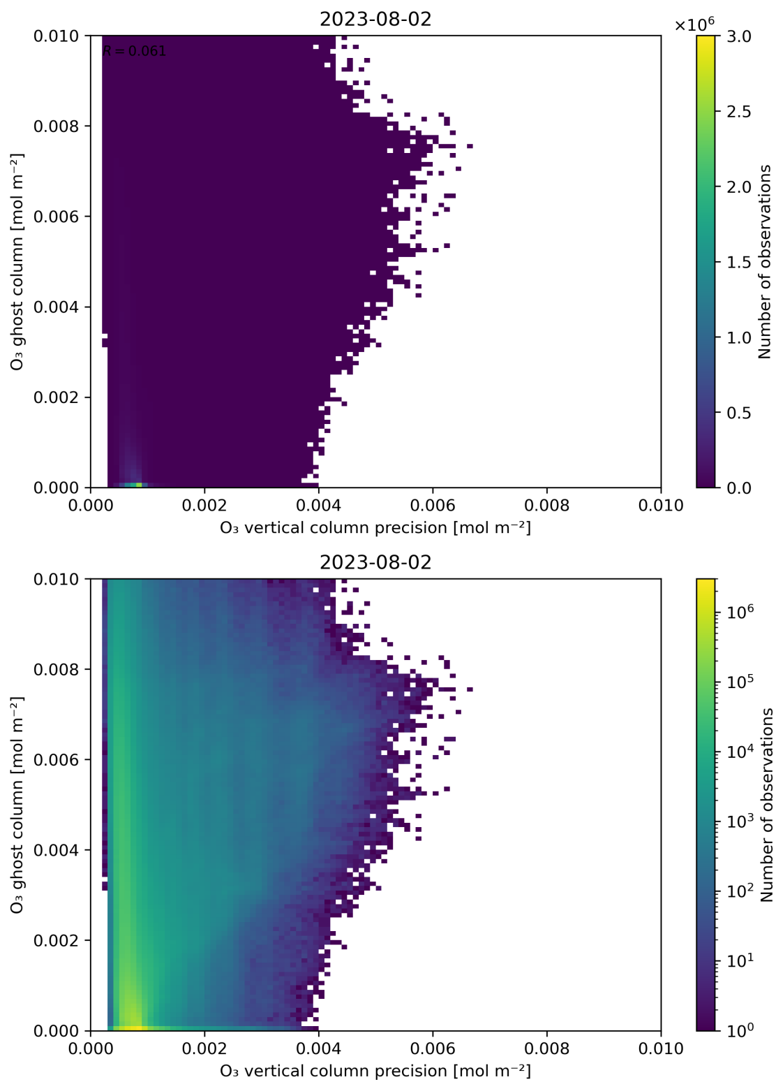
Figure 43: Scatter density plot of “O 3 vertical column precision” against “O 3 ghost column” for 2023-08-01 to 2023-08-03.
