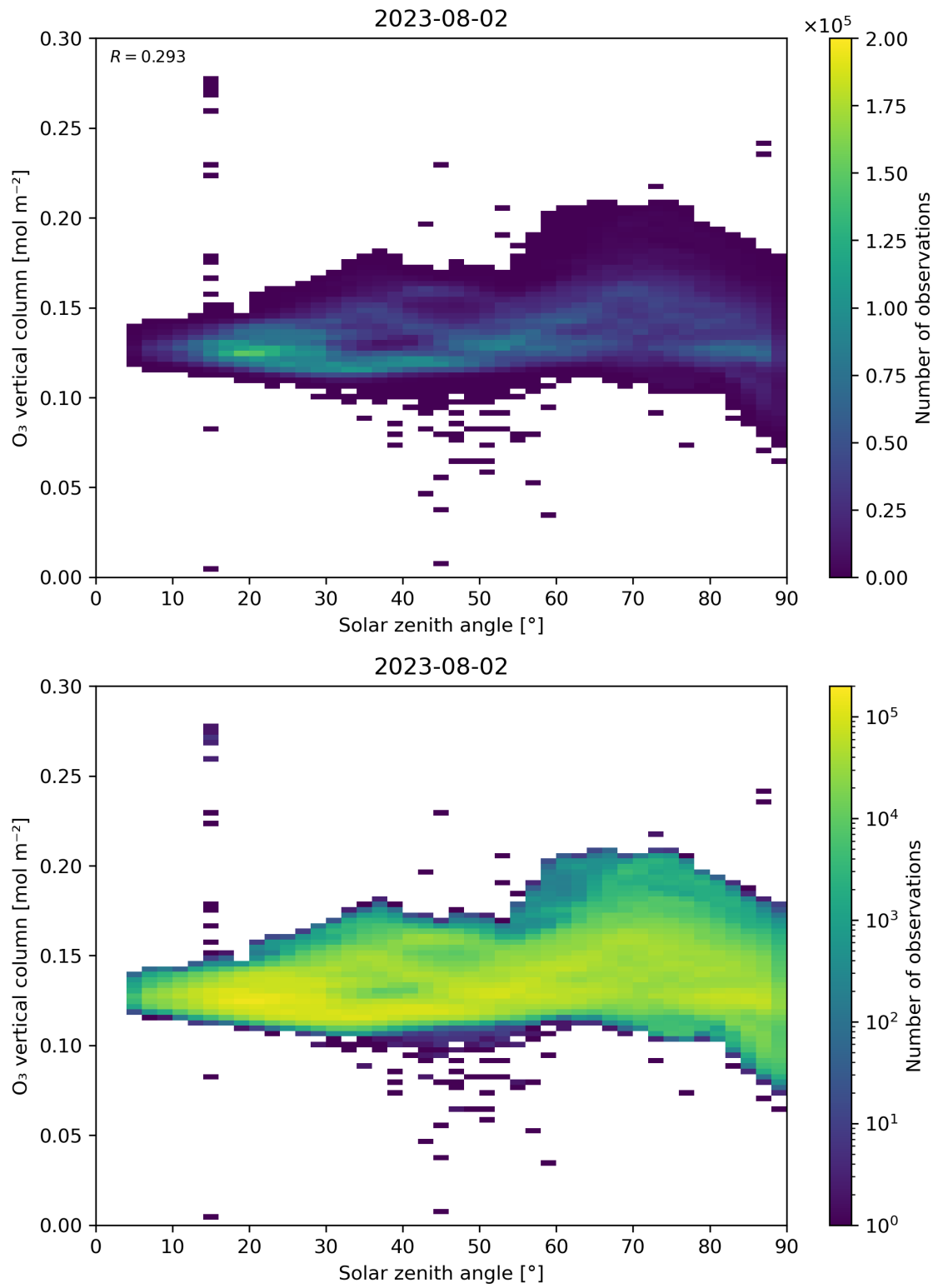
Figure 47: Scatter density plot of “Solar zenith angle” against “O 3 vertical column” for 2023-08-01 to 2023-08-03.
