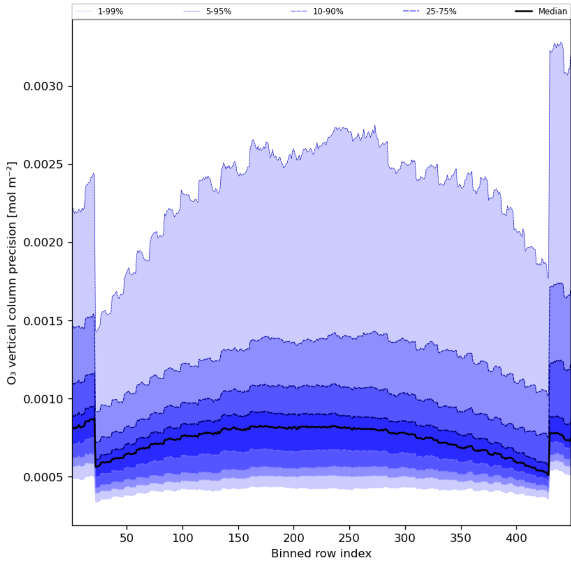
Figure 29: Along track statistics of “O 3 vertical column precision” for 2023-08-01 to 2023-08-03
