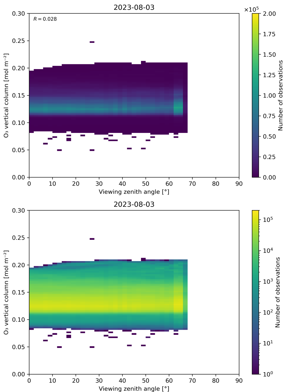
Figure 52: Scatter density plot of “Viewing zenith angle” against “O 3 vertical column” for 2023-08-02 to 2023-08-04.
