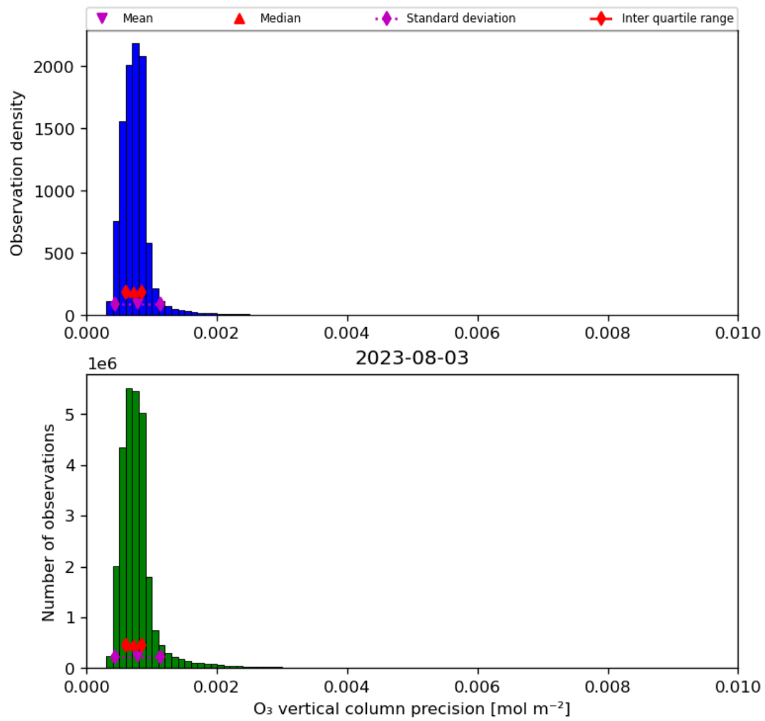
Figure 22: Histogram of “O 3 vertical column precision” for 2023-08-02 to 2023-08-04
