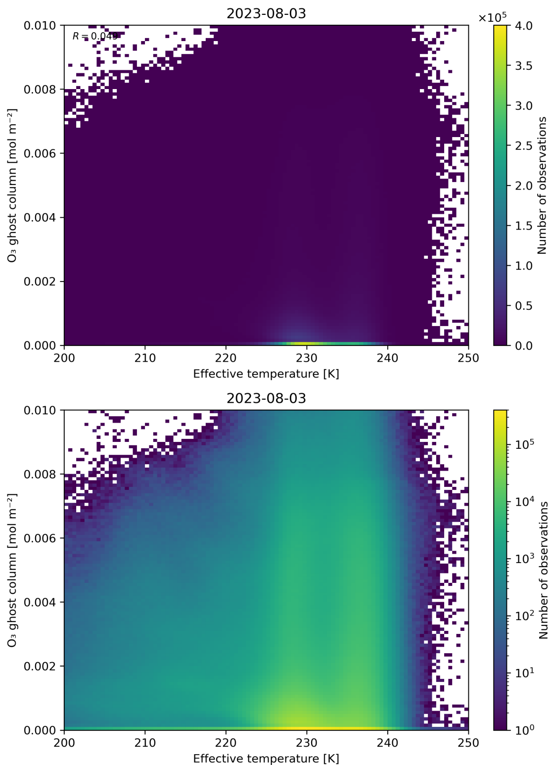
Figure 38: Scatter density plot of “Effective temperature” against “O 3 ghost column” for 2023-08-02 to 2023-08-04.
