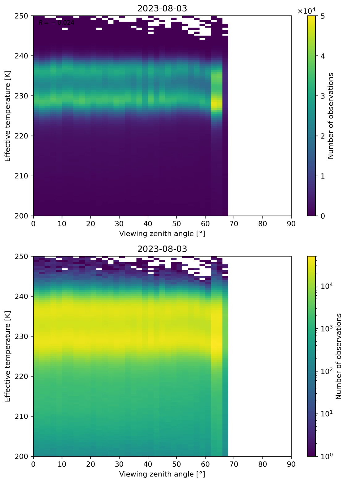
Figure 50: Scatter density plot of “Viewing zenith angle” against “Effective temperature” for 2023-08-02 to 2023-08-04.
