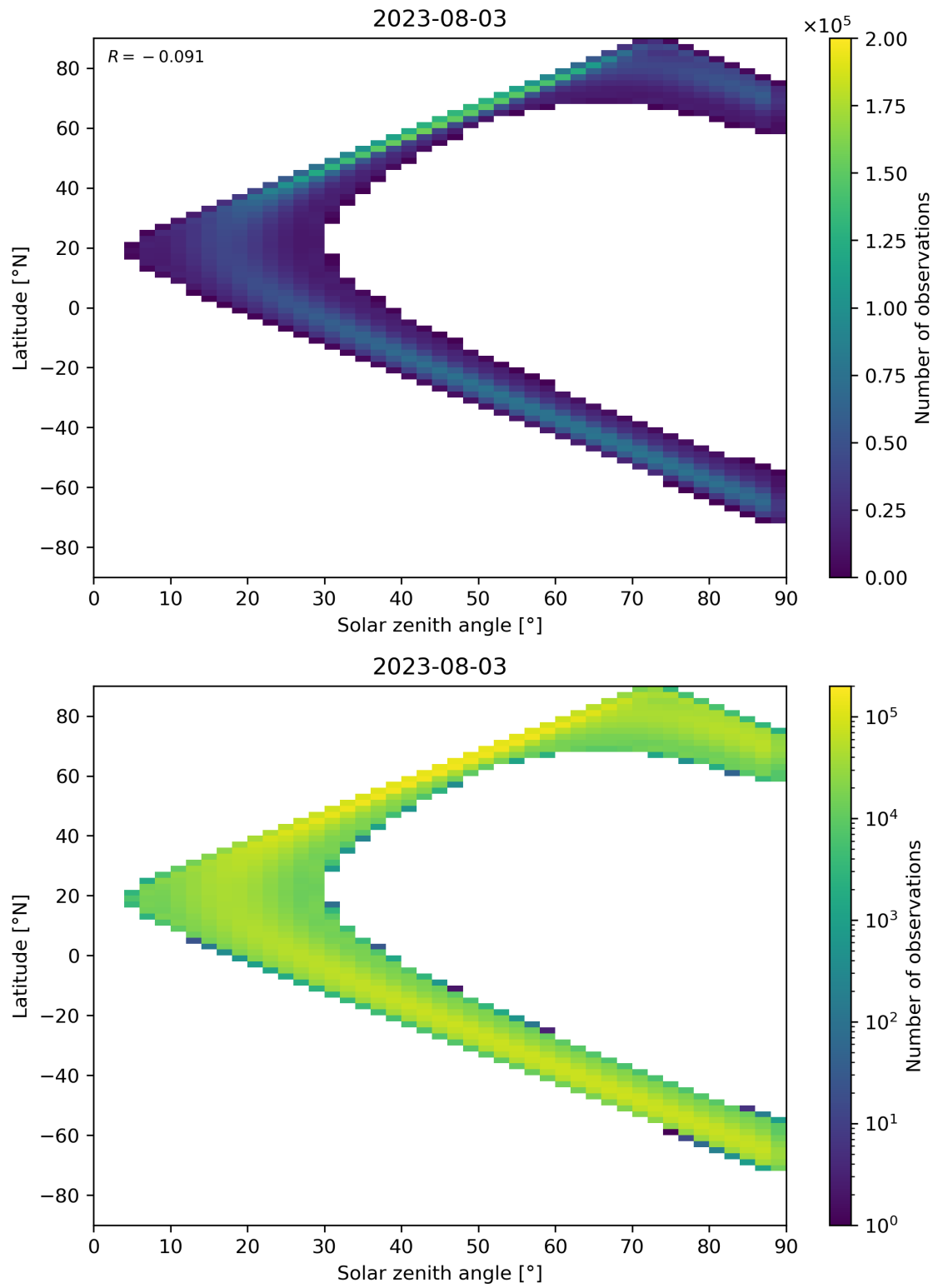
Figure 44: Scatter density plot of “Solar zenith angle” against “Latitude” for 2023-08-02 to 2023-08-04.
