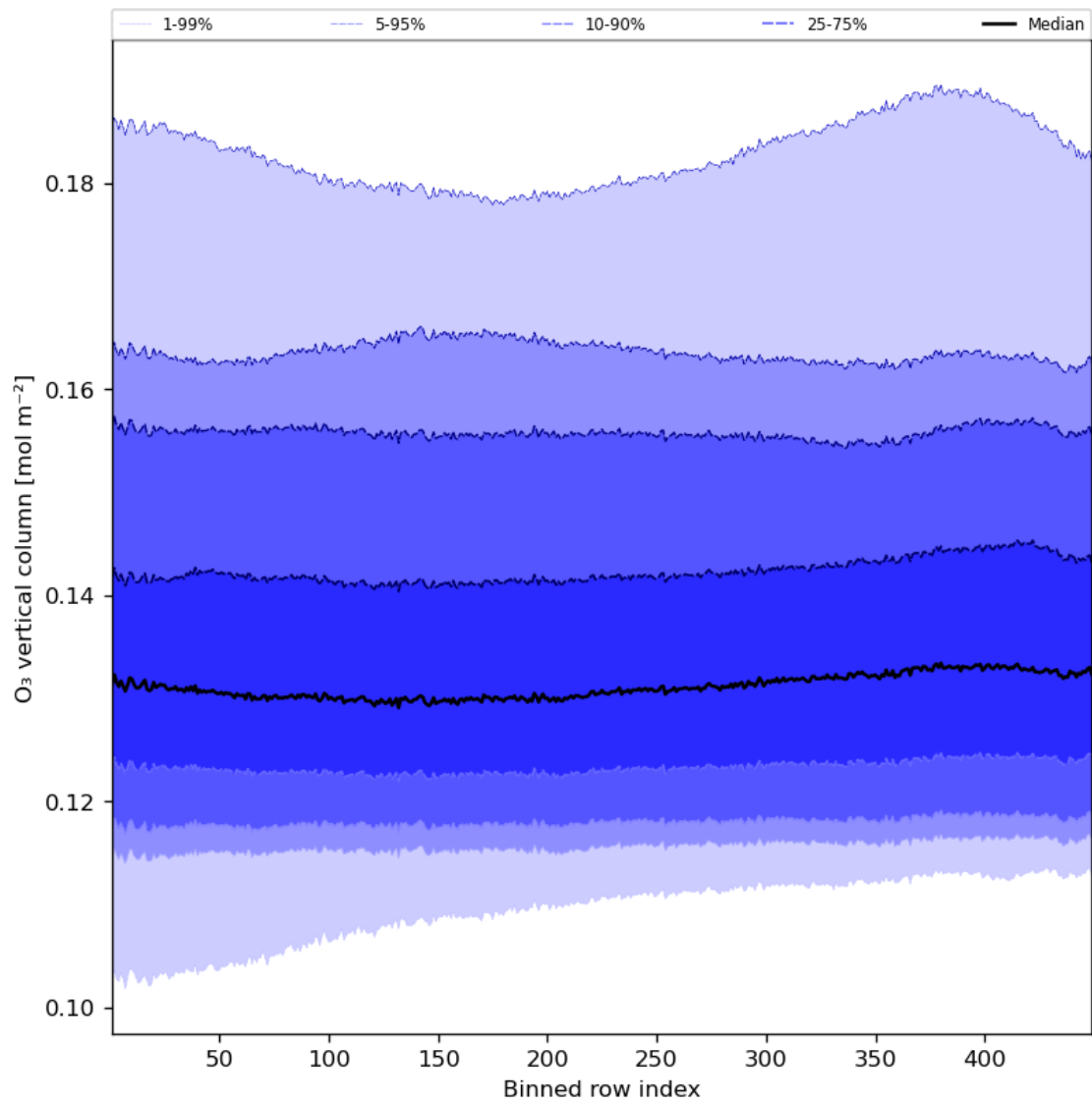
Figure 28: Along track statistics of “O 3 vertical column” for 2023-08-02 to 2023-08-04
