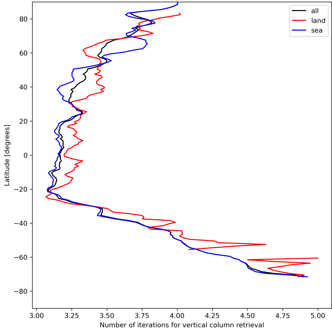
Figure 19: Zonal average of “Number of iterations for vertical column retrieval” for 2023-08-02 to 2023-08-04.
