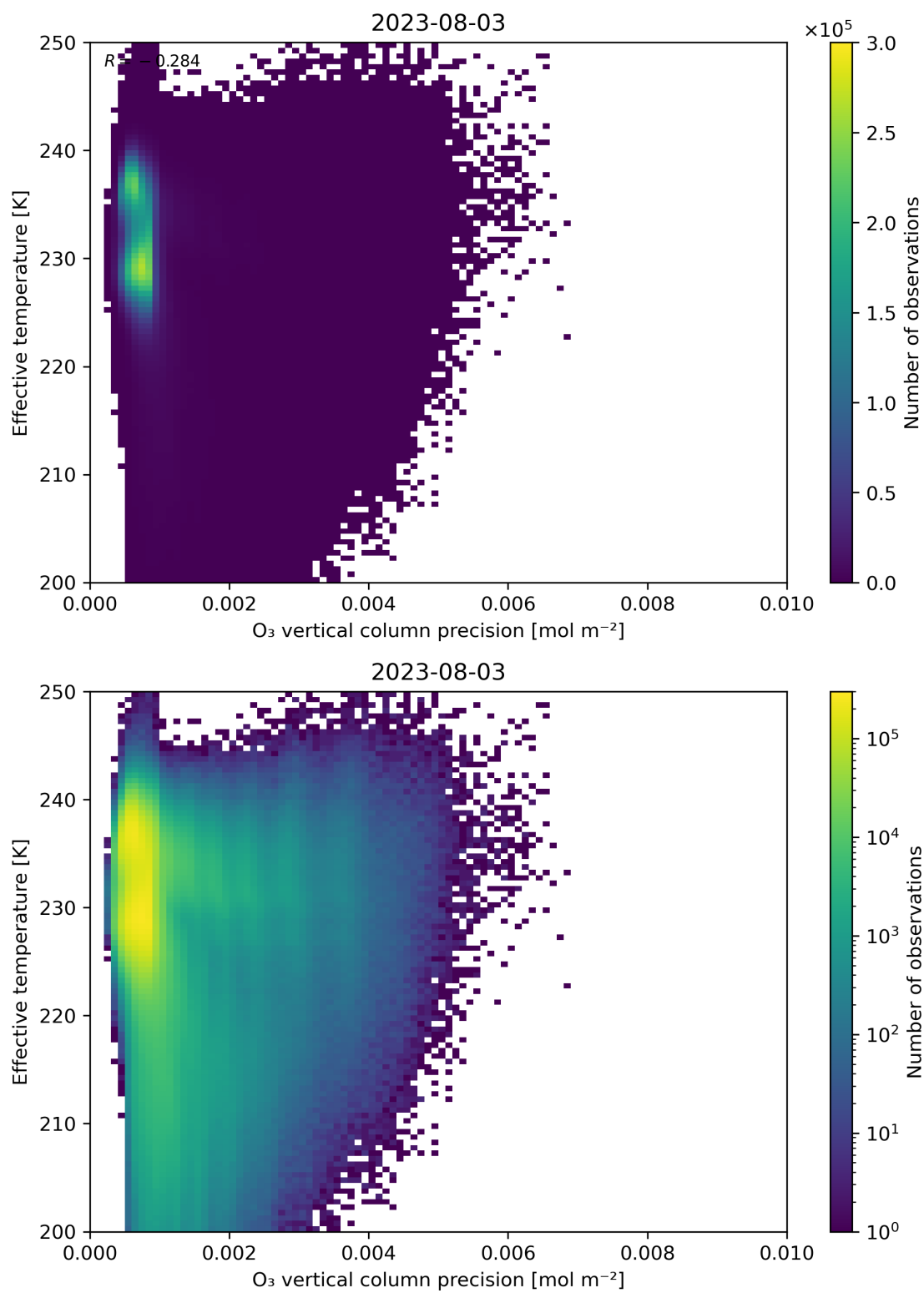
Figure 42: Scatter density plot of “O 3 vertical column precision” against “Effective temperature” for 2023-08-02 to 2023-08-04.
