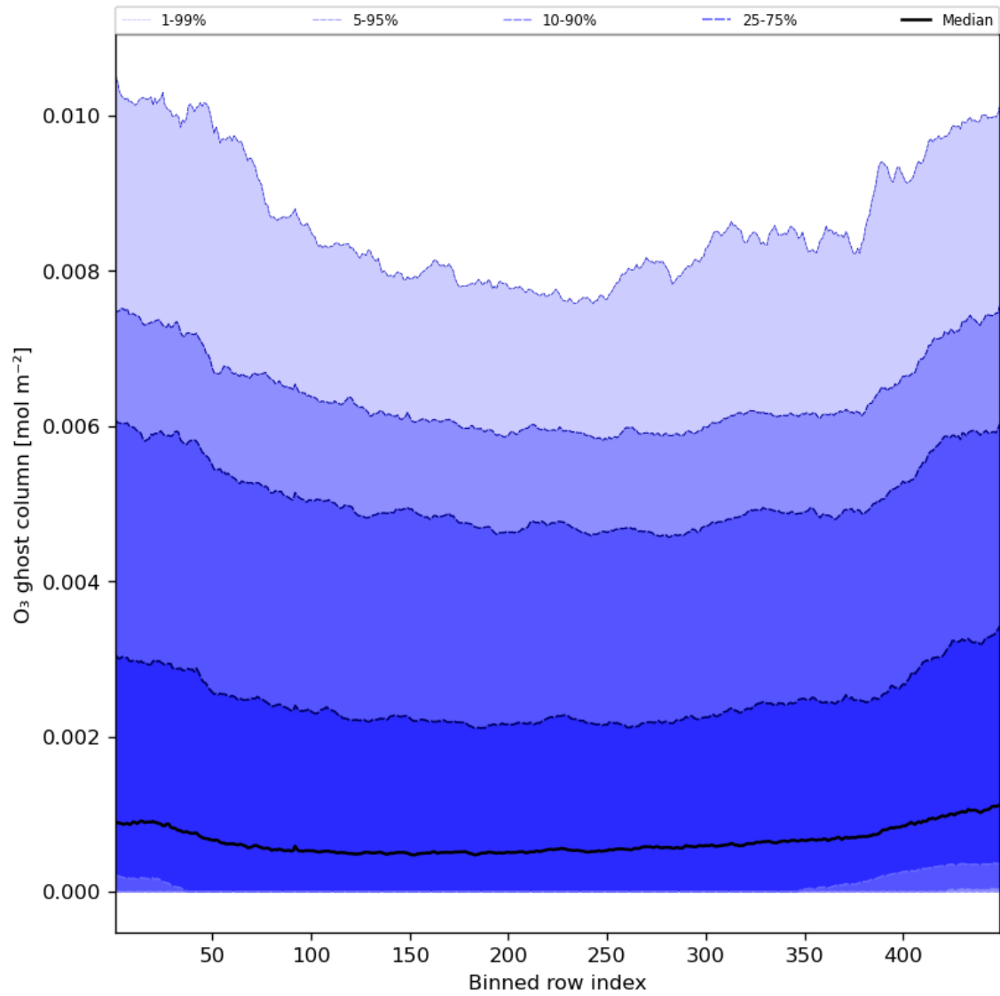
Figure 32: Along track statistics of “O 3 ghost column” for 2023-08-02 to 2023-08-04
