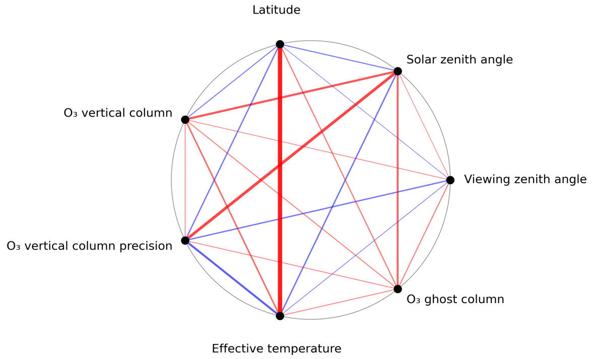
Figure 1: Map of correlation graph for 2023-08-02 to 2023-08-04.
