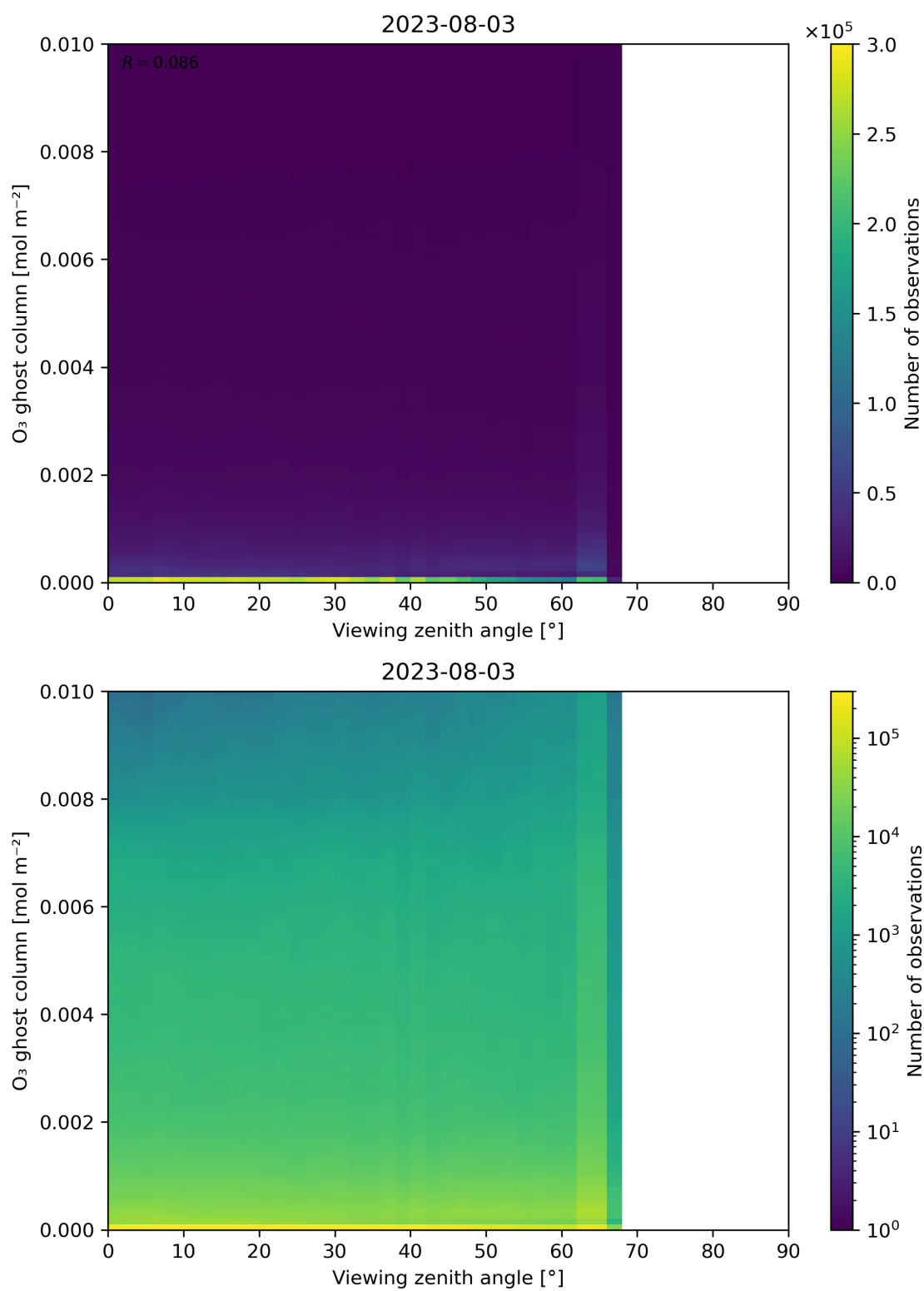
Figure 51: Scatter density plot of “Viewing zenith angle” against “O 3 ghost column” for 2023-08-02 to 2023-08-04.
