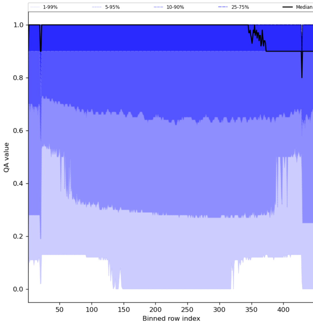
Figure 27: Along track statistics of “QA value” for 2023-08-02 to 2023-08-04
