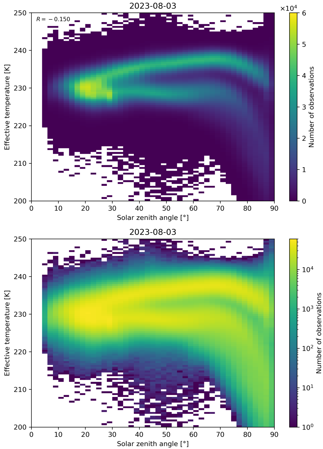
Figure 45: Scatter density plot of “Solar zenith angle” against “Effective temperature” for 2023-08-02 to 2023-08-04.
