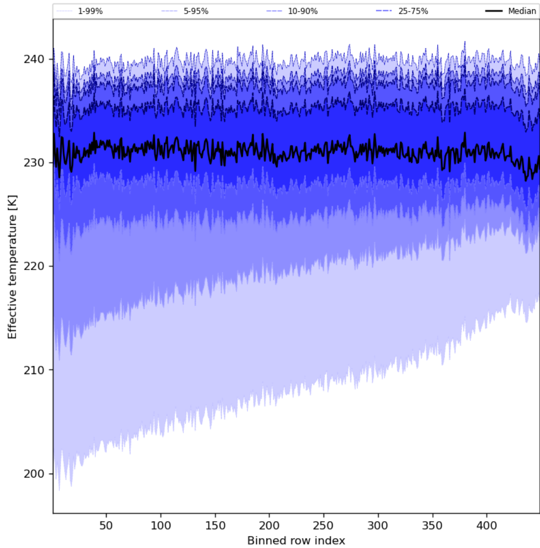
Figure 31: Along track statistics of “Effective temperature” for 2023-08-02 to 2023-08-04
