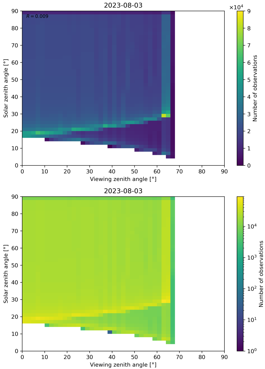
Figure 54: Scatter density plot of “Viewing zenith angle” against “Solar zenith angle” for 2023-08-02 to 2023-08-04.
