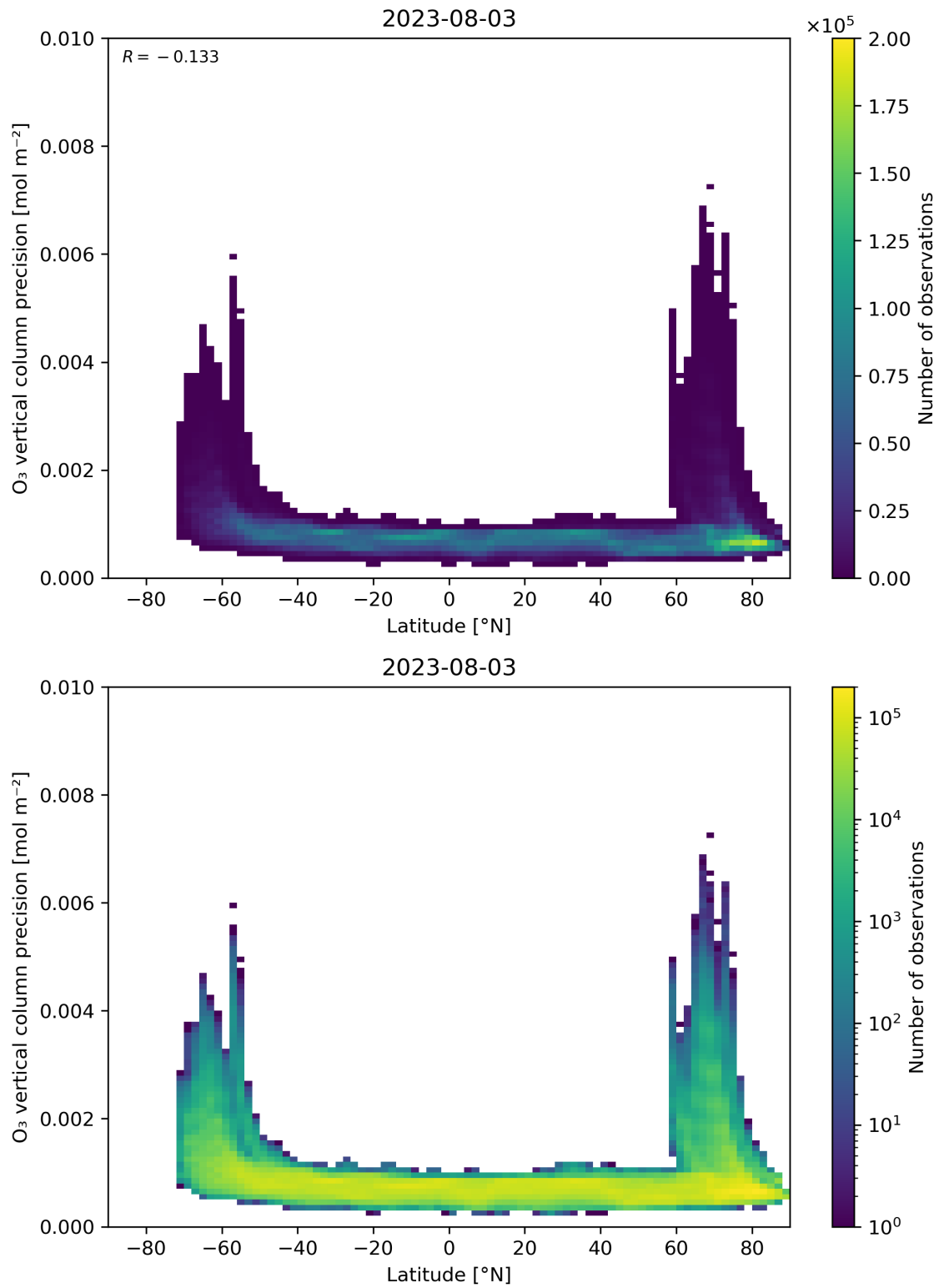
Figure 37: Scatter density plot of “Latitude” against “O 3 vertical column precision” for 2023-08-02 to 2023-08-04.
