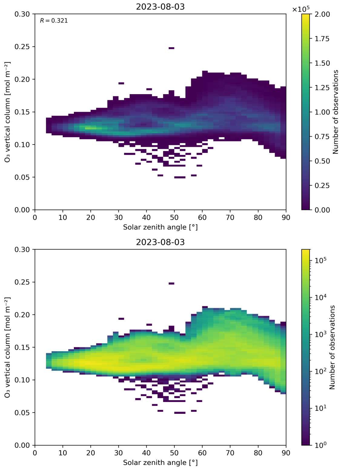
Figure 47: Scatter density plot of “Solar zenith angle” against “O 3 vertical column” for 2023-08-02 to 2023-08-04.
