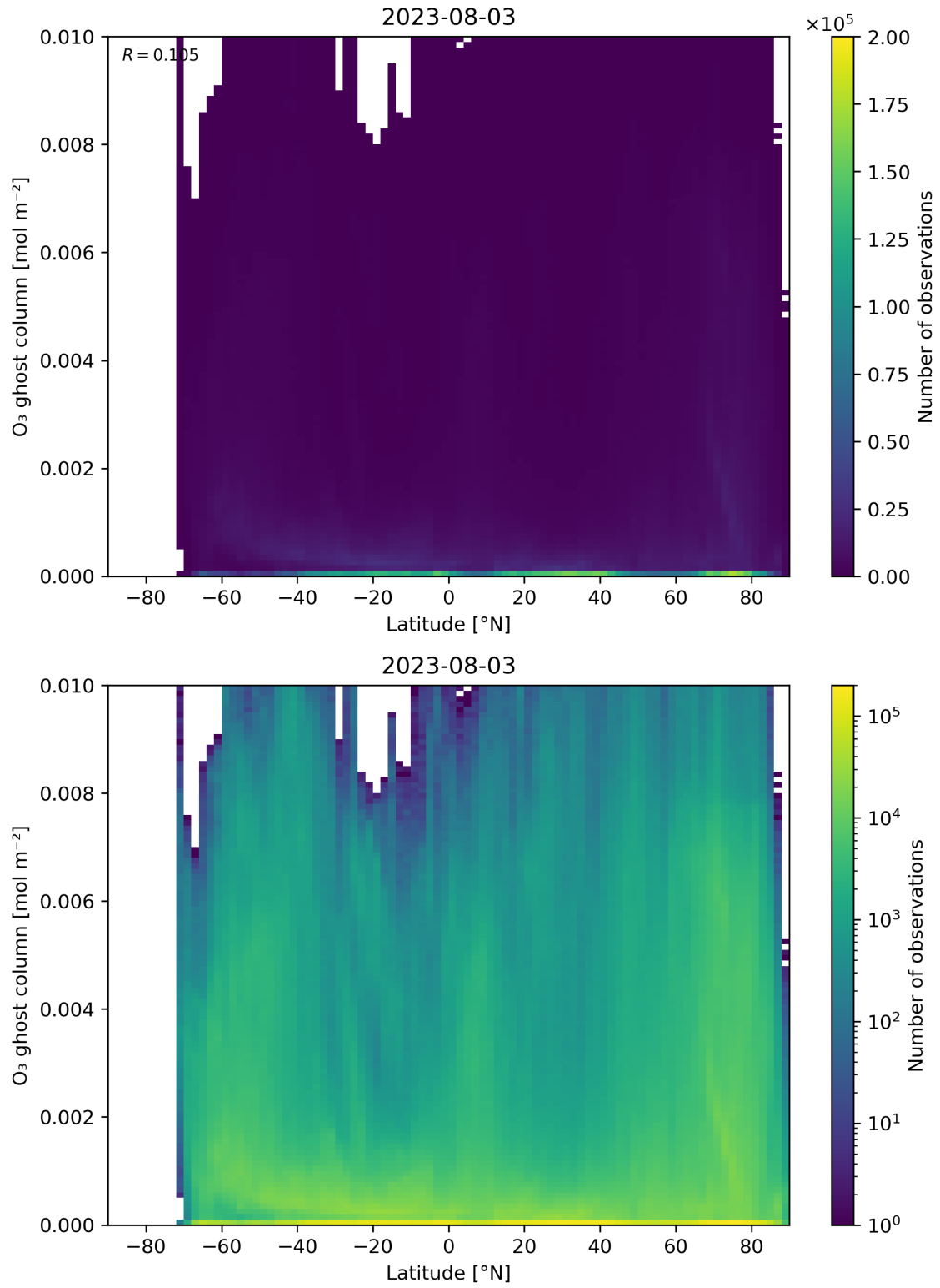
Figure 35: Scatter density plot of “Latitude” against “O 3 ghost column” for 2023-08-02 to 2023-08-04.
