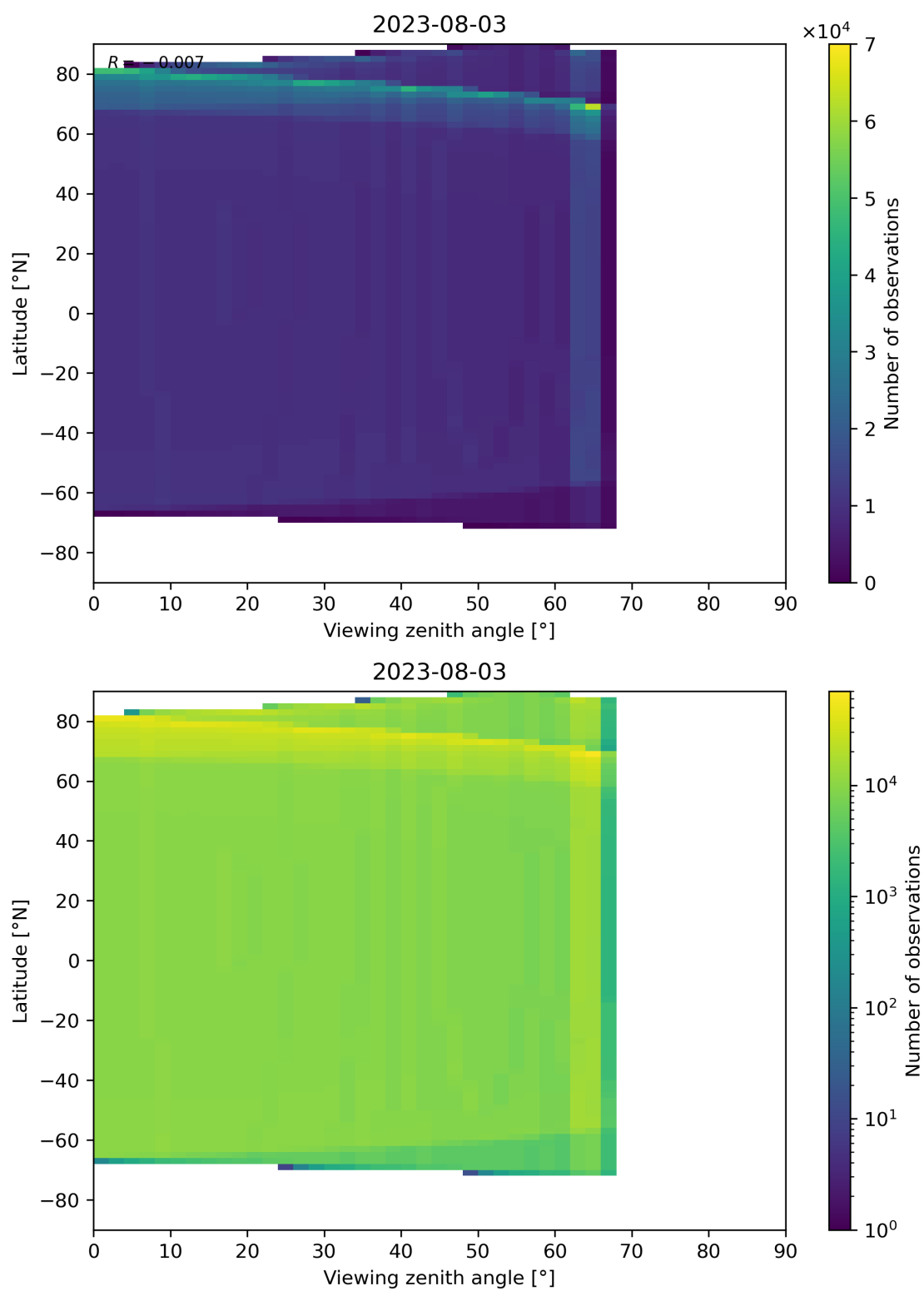
Figure 49: Scatter density plot of “Viewing zenith angle” against “Latitude” for 2023-08-02 to 2023-08-04.
