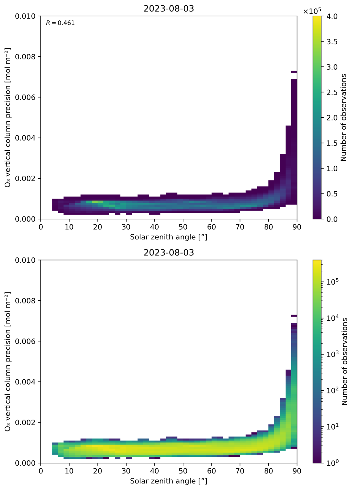
Figure 48: Scatter density plot of “Solar zenith angle” against “O 3 vertical column precision” for 2023-08-02 to 2023-08-04.
