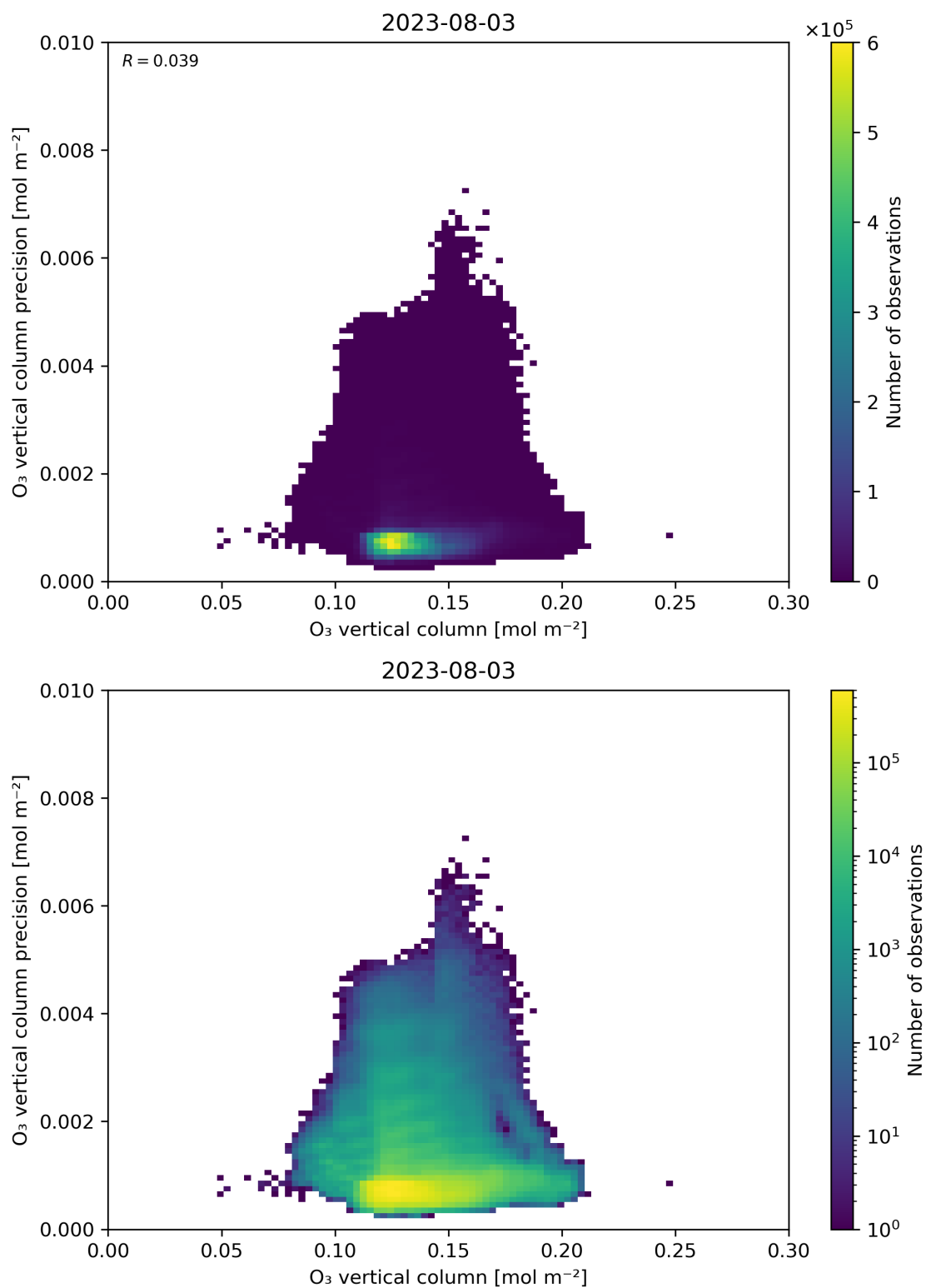
Figure 41: Scatter density plot of “O 3 vertical column” against “O 3 vertical column precision” for 2023-08-02 to 2023-08-04.
