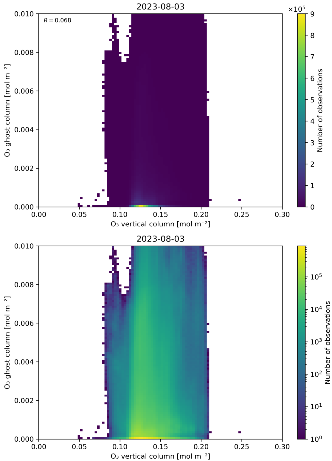
Figure 40: Scatter density plot of “O 3 vertical column” against “O 3 ghost column” for 2023-08-02 to 2023-08-04.
