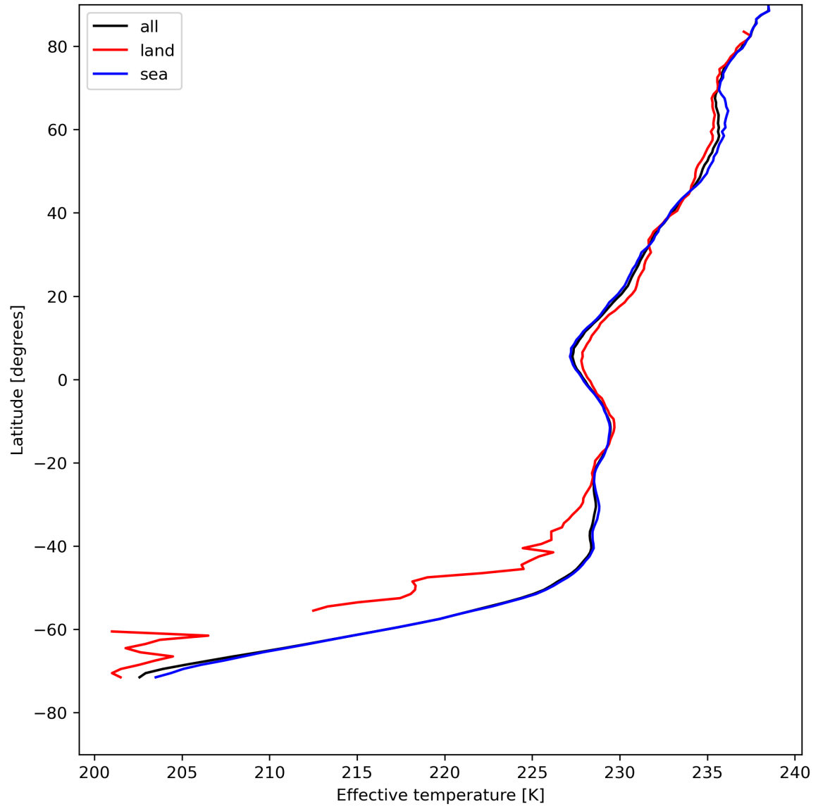
Figure 17: Zonal average of "Effective temperature" for 2023-08-02 to 2023-08-04.
