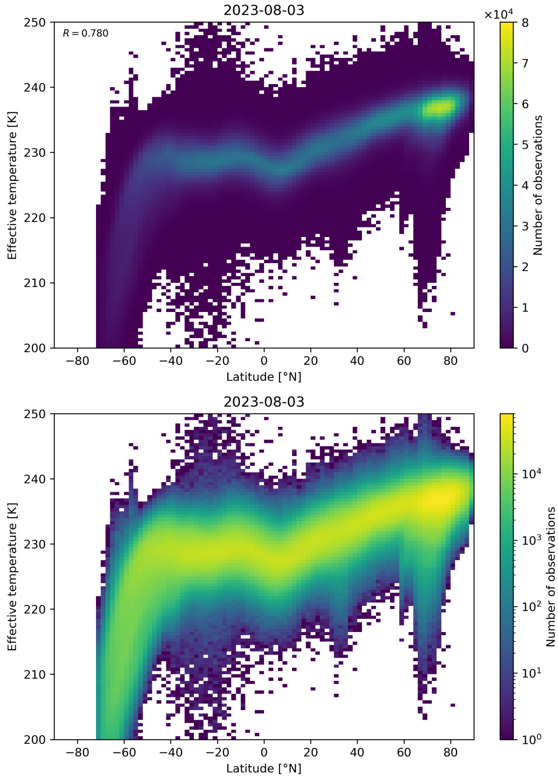
Figure 34: Scatter density plot of “Latitude” against “Effective temperature” for 2023-08-02 to 2023-08-04.
