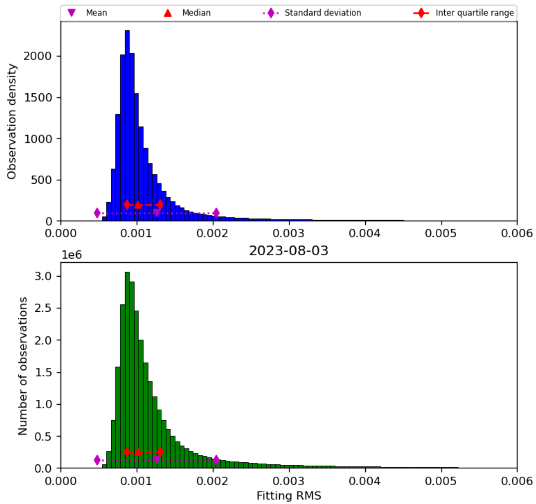
Figure 23: Histogram of “Fitting RMS” for 2023-08-02 to 2023-08-04
