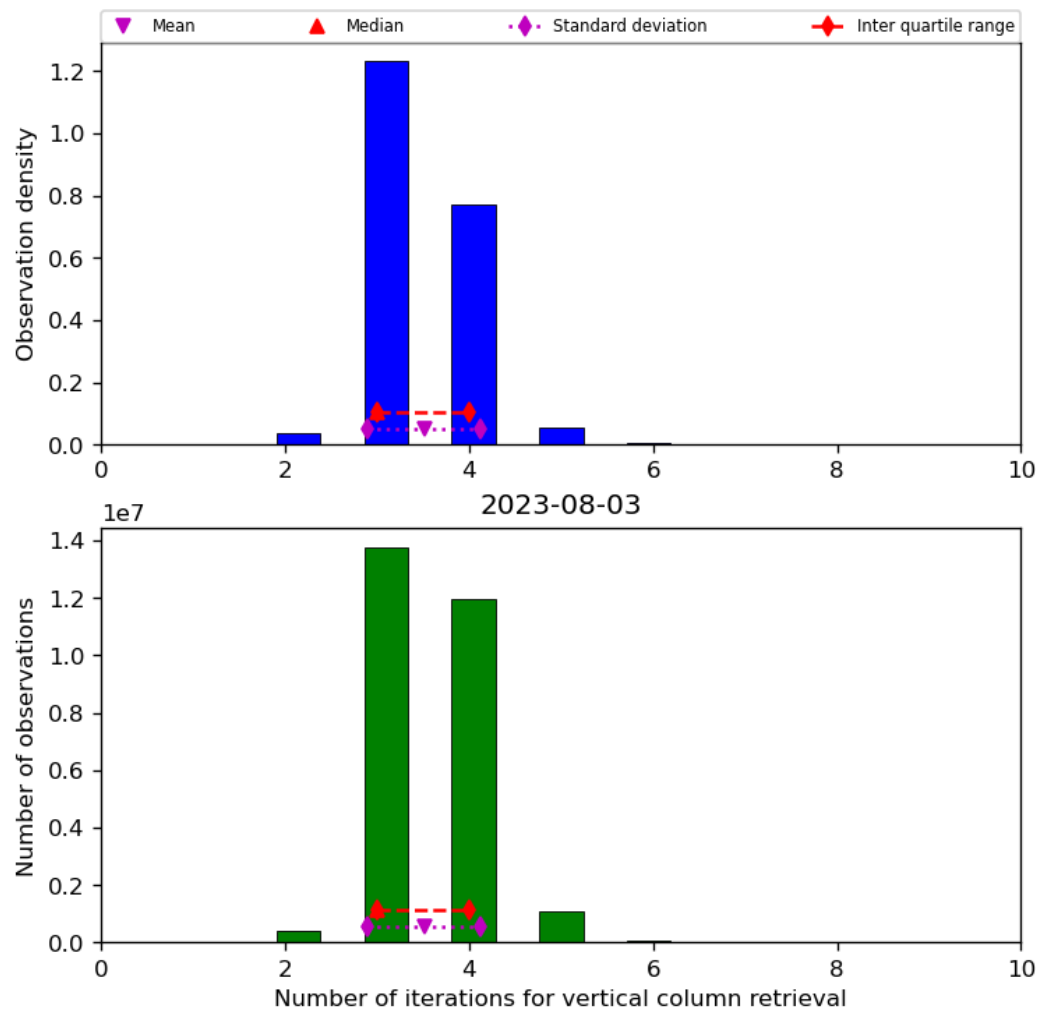
Figure 26: Histogram of “Number of iterations for vertical column retrieval” for 2023-08-02 to 2023-08-04
