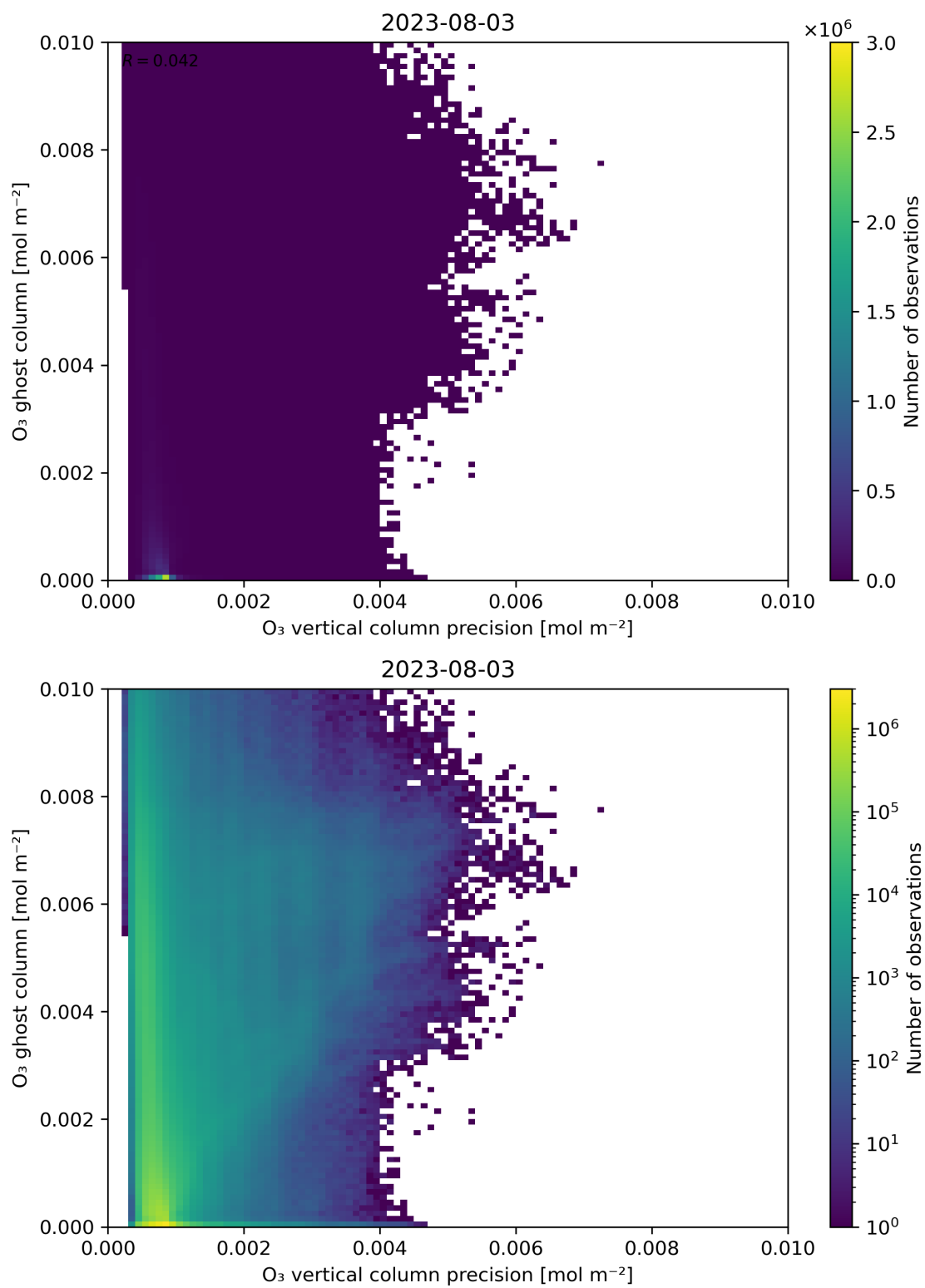
Figure 43: Scatter density plot of “ O_3 vertical column precision” against “ O_3 ghost column” for 2023-08-02 to 2023-08-04.
