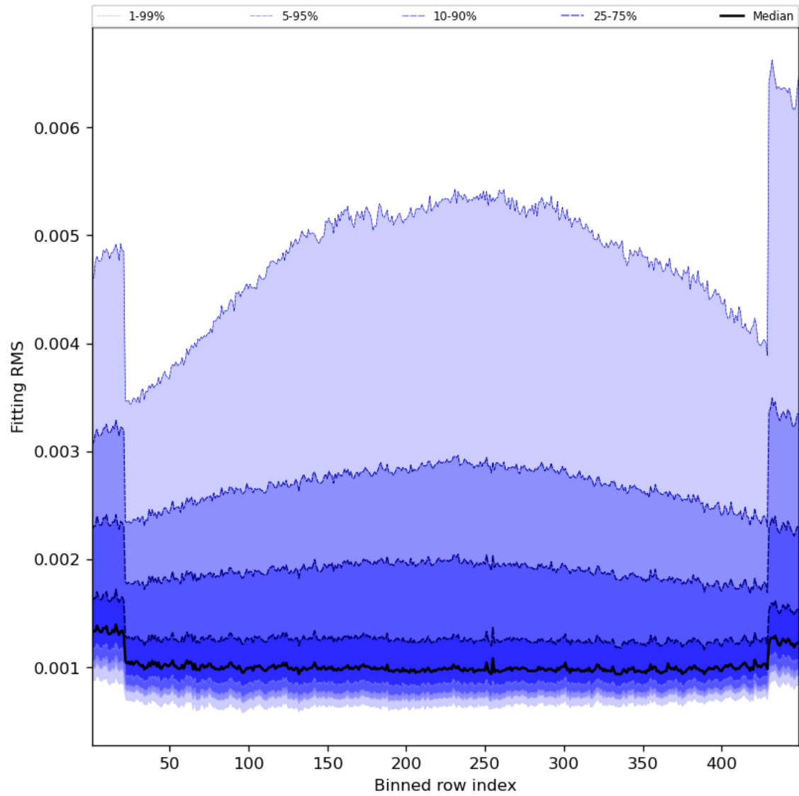
Figure 30: Along track statistics of “Fitting RMS” for 2023-08-02 to 2023-08-04
