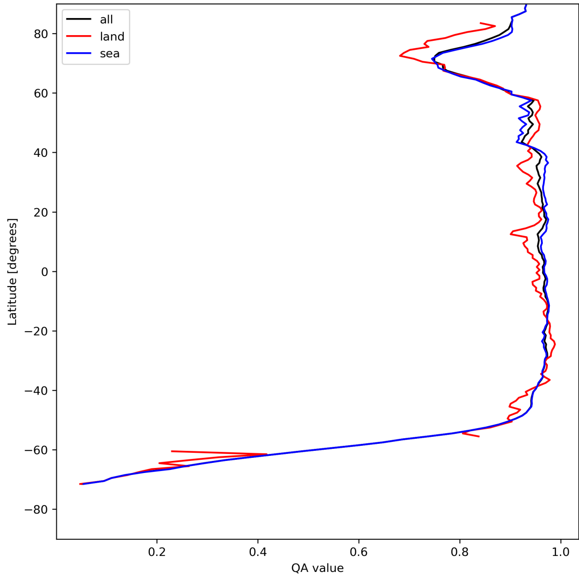
Figure 13: Zonal average of “QA value” for 2023-08-02 to 2023-08-04.
