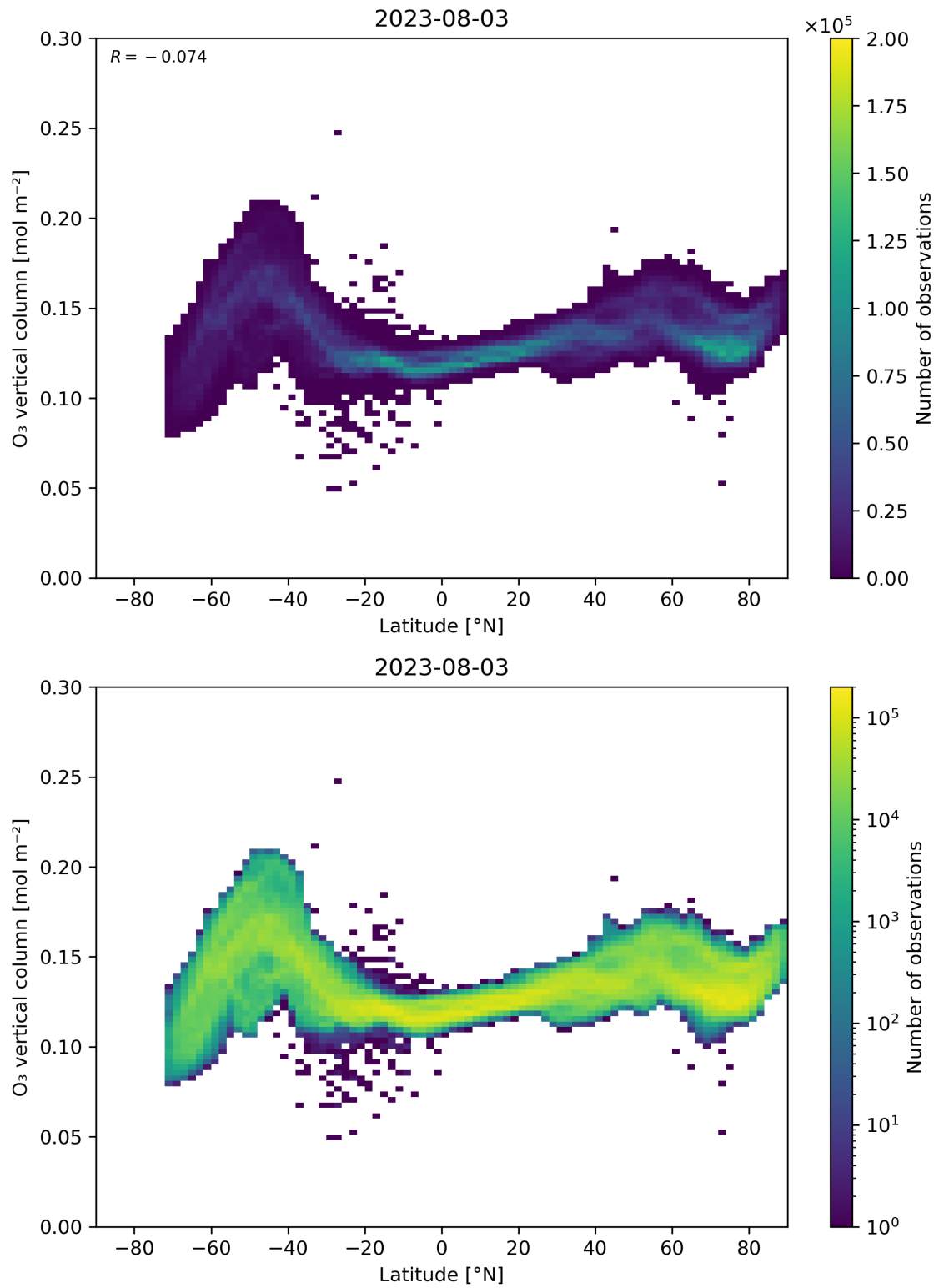
Figure 36: Scatter density plot of “Latitude” against “O 3 vertical column” for 2023-08-02 to 2023-08-04.
