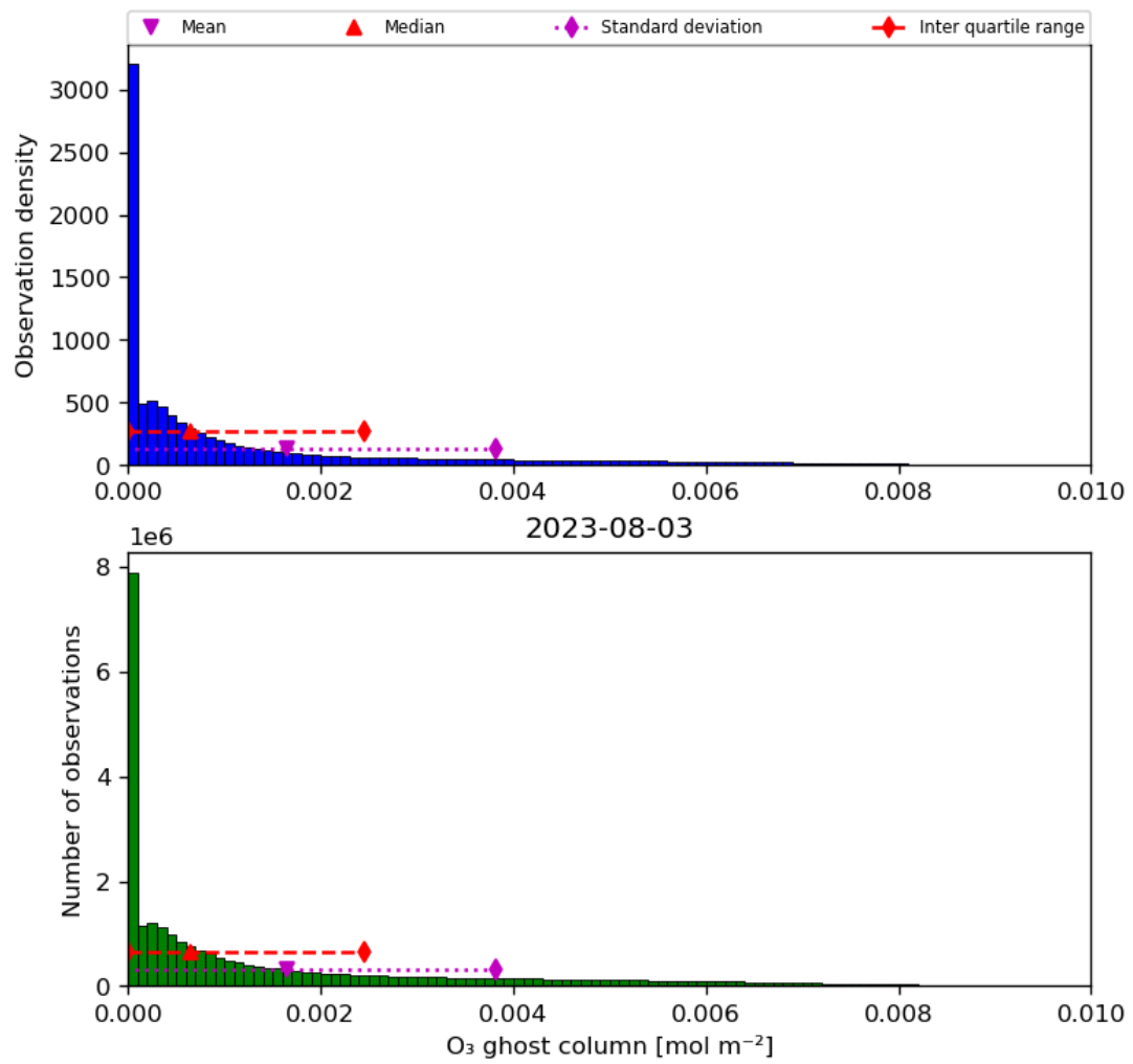
Figure 25: Histogram of “O 3 ghost column” for 2023-08-02 to 2023-08-04
