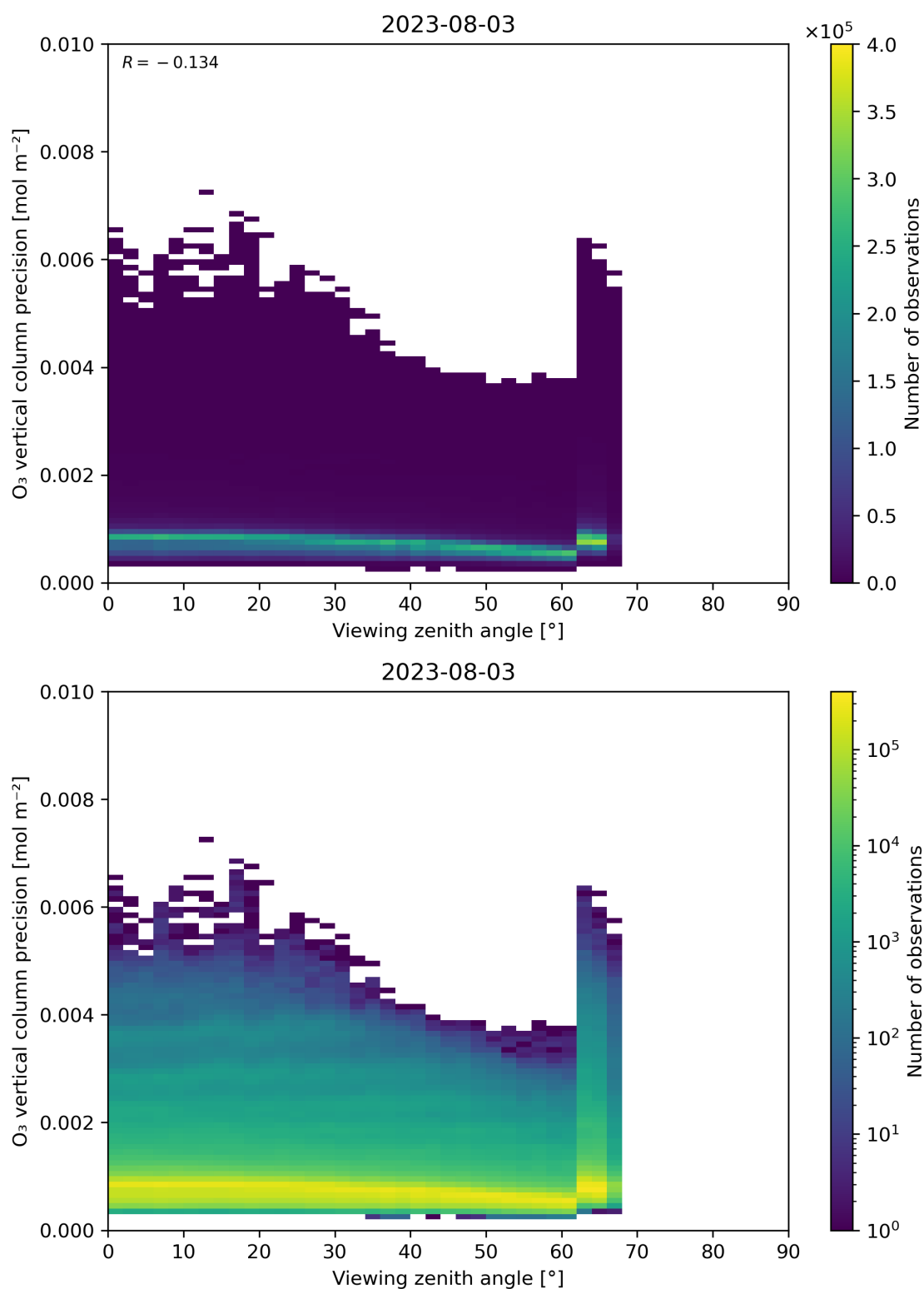
Figure 53: Scatter density plot of “Viewing zenith angle” against “O 3 vertical column precision” for 2023-08-02 to 2023-08-04.
