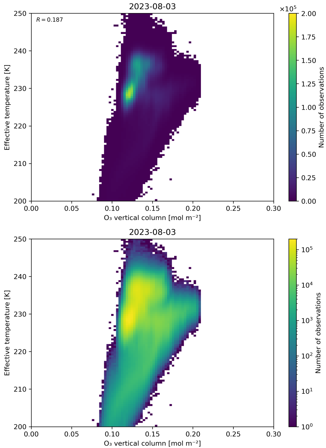
Figure 39: Scatter density plot of “O 3 vertical column” against “Effective temperature” for 2023-08-02 to 2023-08-04.
