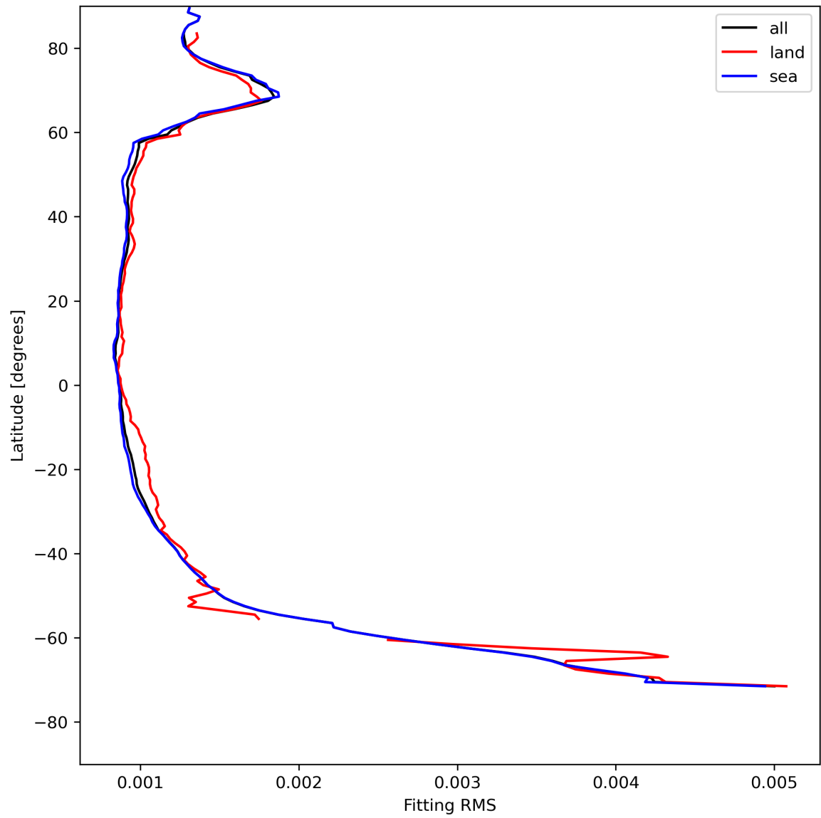
Figure 16: Zonal average of “Fitting RMS” for 2023-08-02 to 2023-08-04.
