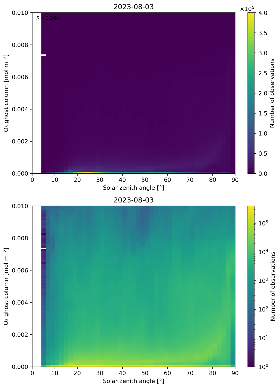
Figure 46: Scatter density plot of “Solar zenith angle” against “O 3 ghost column” for 2023-08-02 to 2023-08-04.
