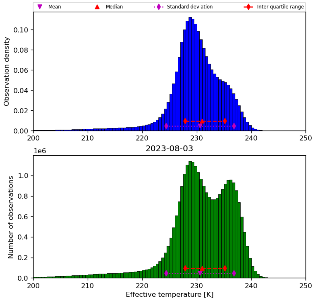
Figure 24: Histogram of “Effective temperature” for 2023-08-02 to 2023-08-04
