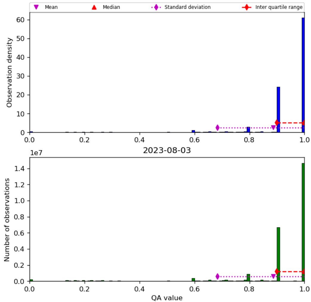
Figure 20: Histogram of “QA value” for 2023-08-02 to 2023-08-04
