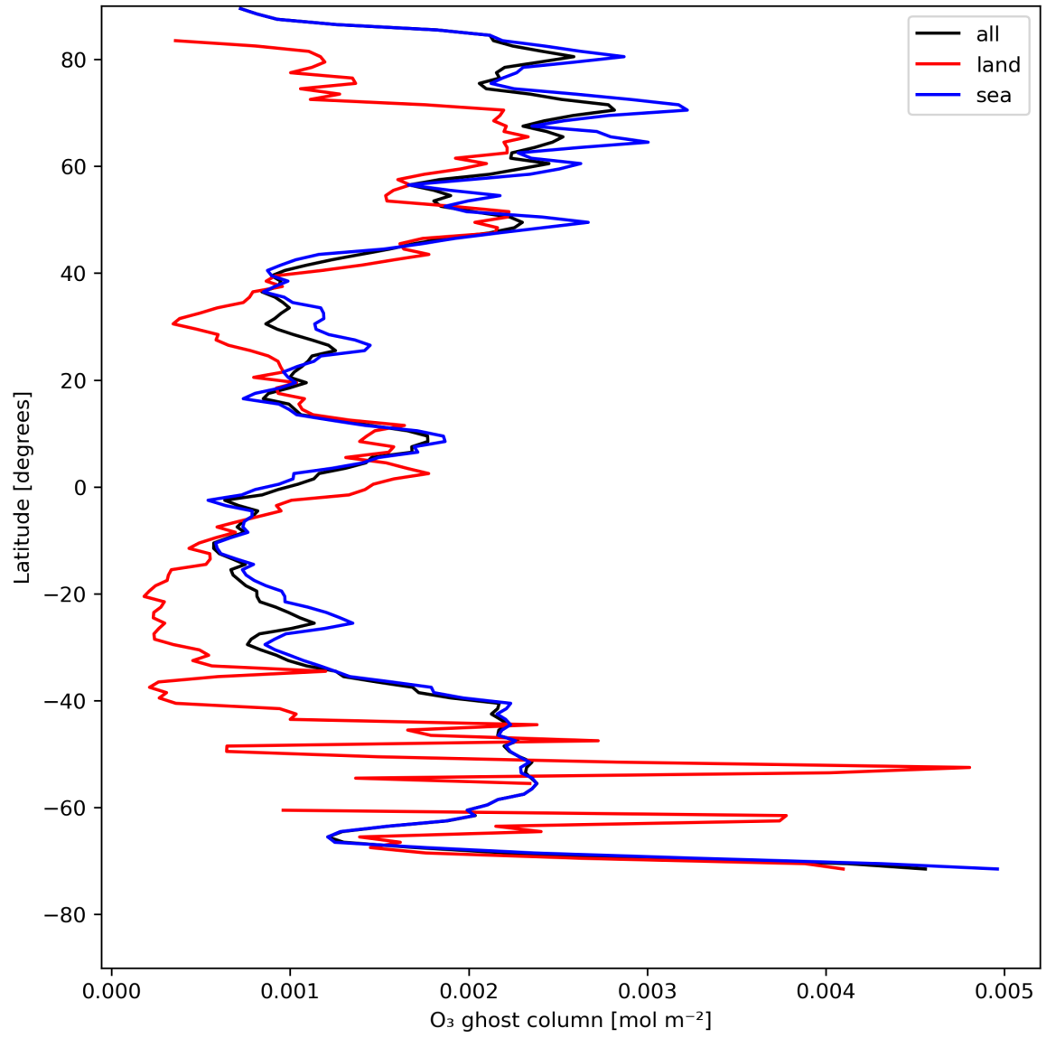
Figure 18: Zonal average of “O 3 ghost column” for 2023-08-02 to 2023-08-04.
