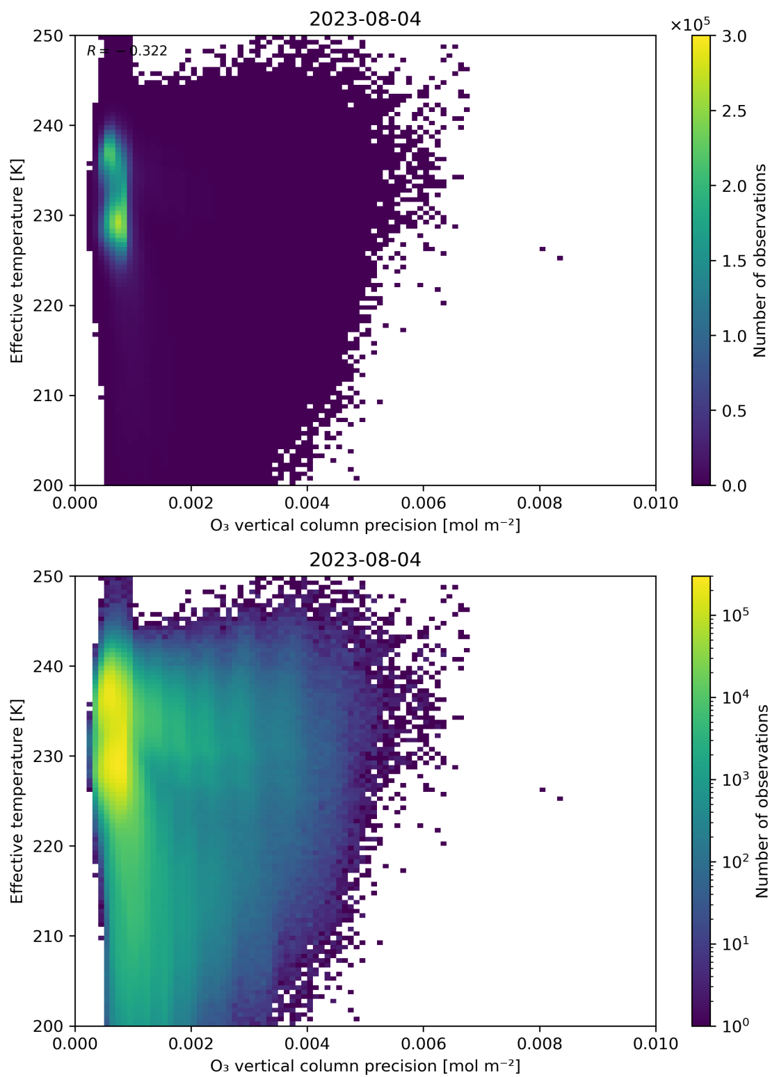
Figure 42: Scatter density plot of “O 3 vertical column precision” against “Effective temperature” for 2023-08-04 to 2023-08-05.
