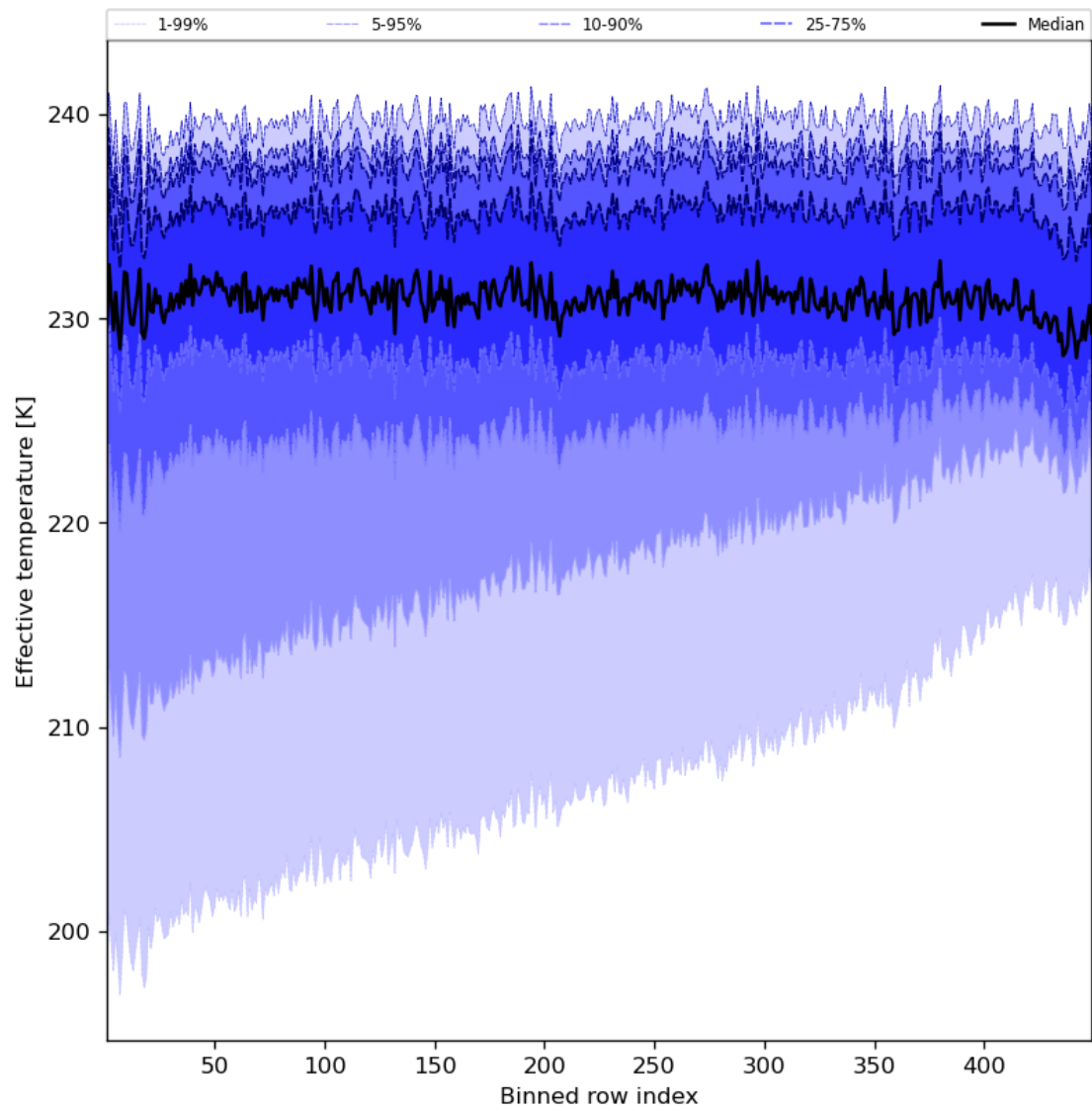
Figure 31: Along track statistics of “Effective temperature” for 2023-08-04 to 2023-08-05
