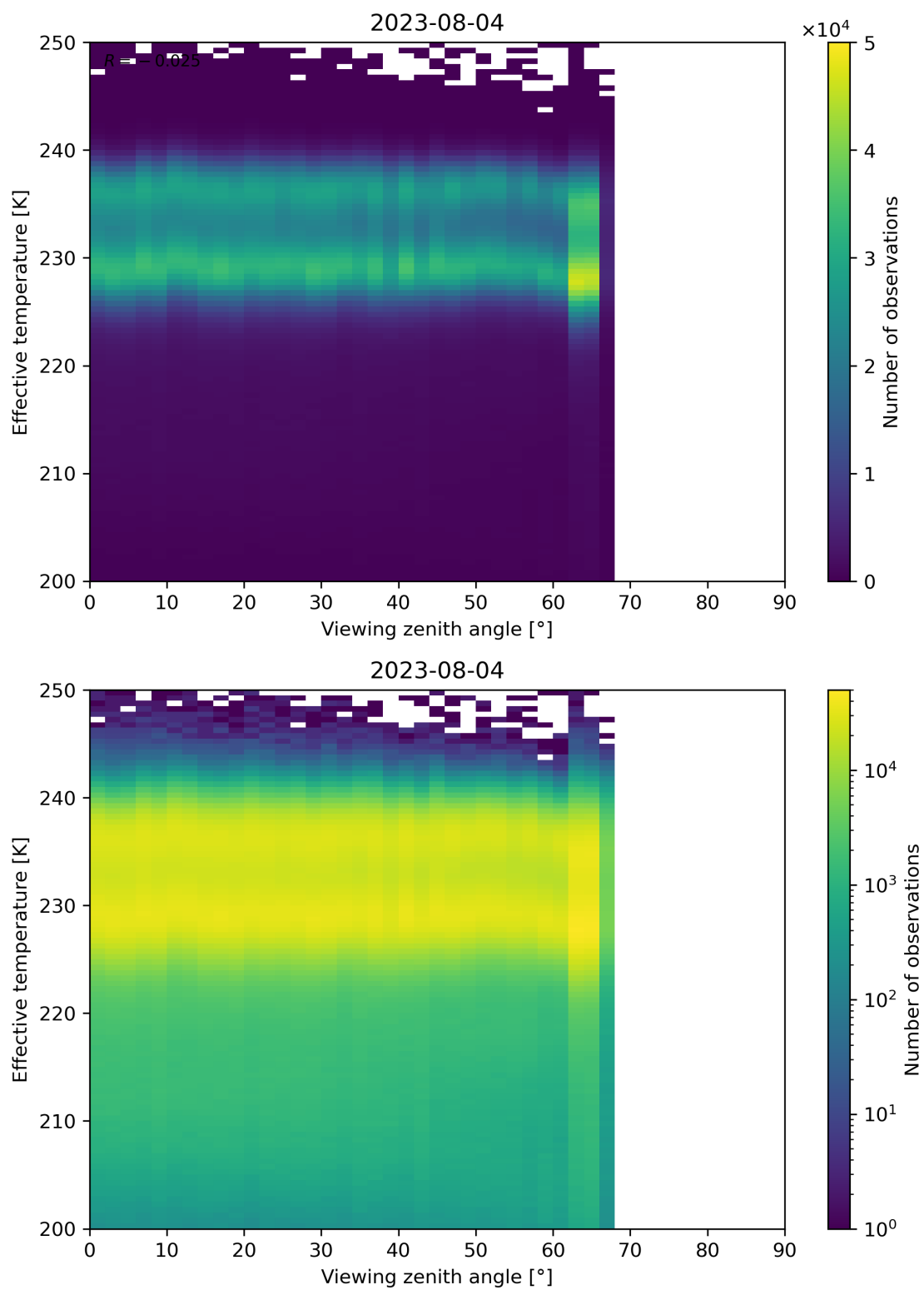
Figure 50: Scatter density plot of “Viewing zenith angle” against “Effective temperature” for 2023-08-04 to 2023-08-05.
