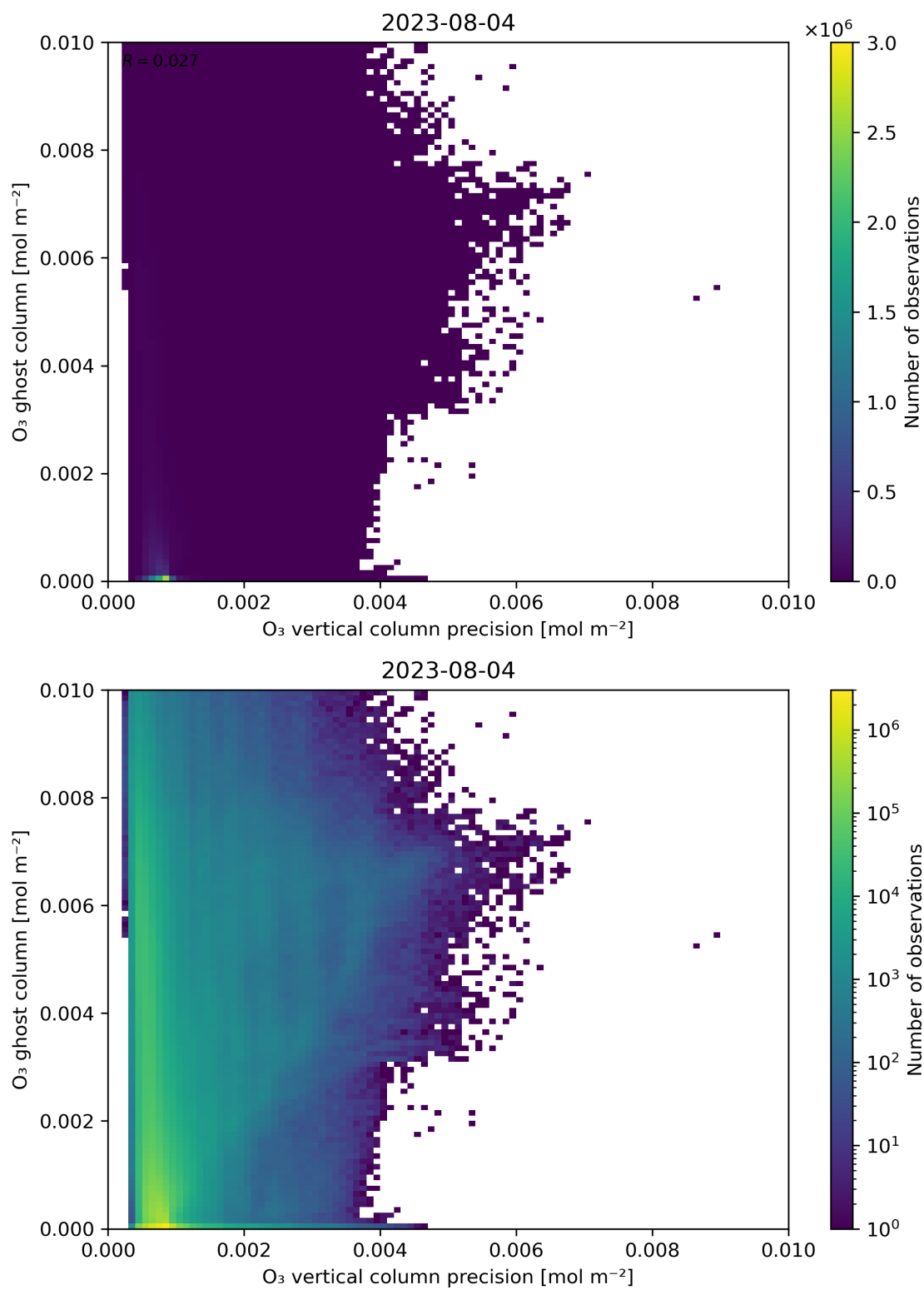
Figure 43: Scatter density plot of “O 3 vertical column precision” against “O 3 ghost column” for 2023-08-04 to 2023-08-05.
