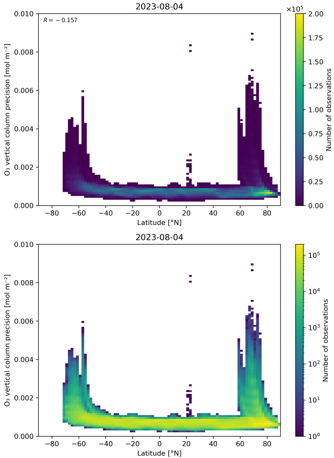
Figure 37: Scatter density plot of “Latitude” against “O 3 vertical column precision” for 2023-08-04 to 2023-08-05.
