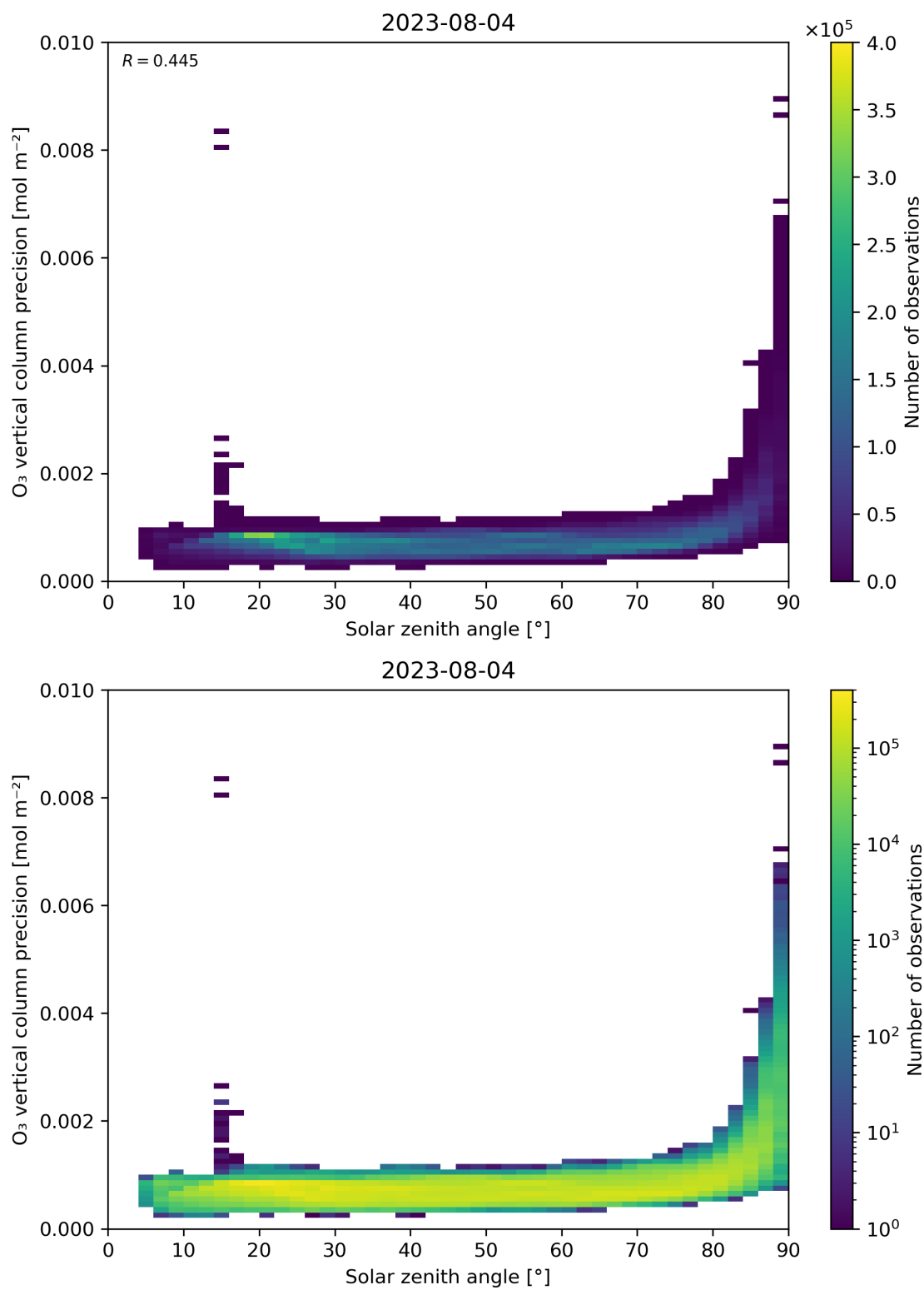
Figure 48: Scatter density plot of “Solar zenith angle” against “O 3 vertical column precision” for 2023-08-04 to 2023-08-05.
