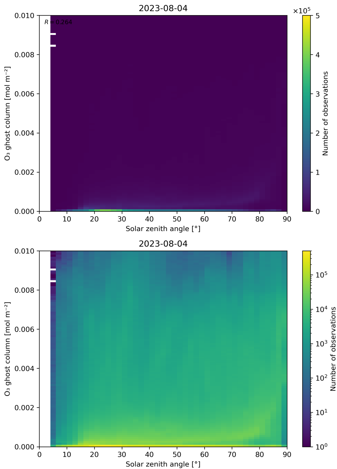
Figure 46: Scatter density plot of “Solar zenith angle” against “O 3 ghost column” for 2023-08-04 to 2023-08-05.
