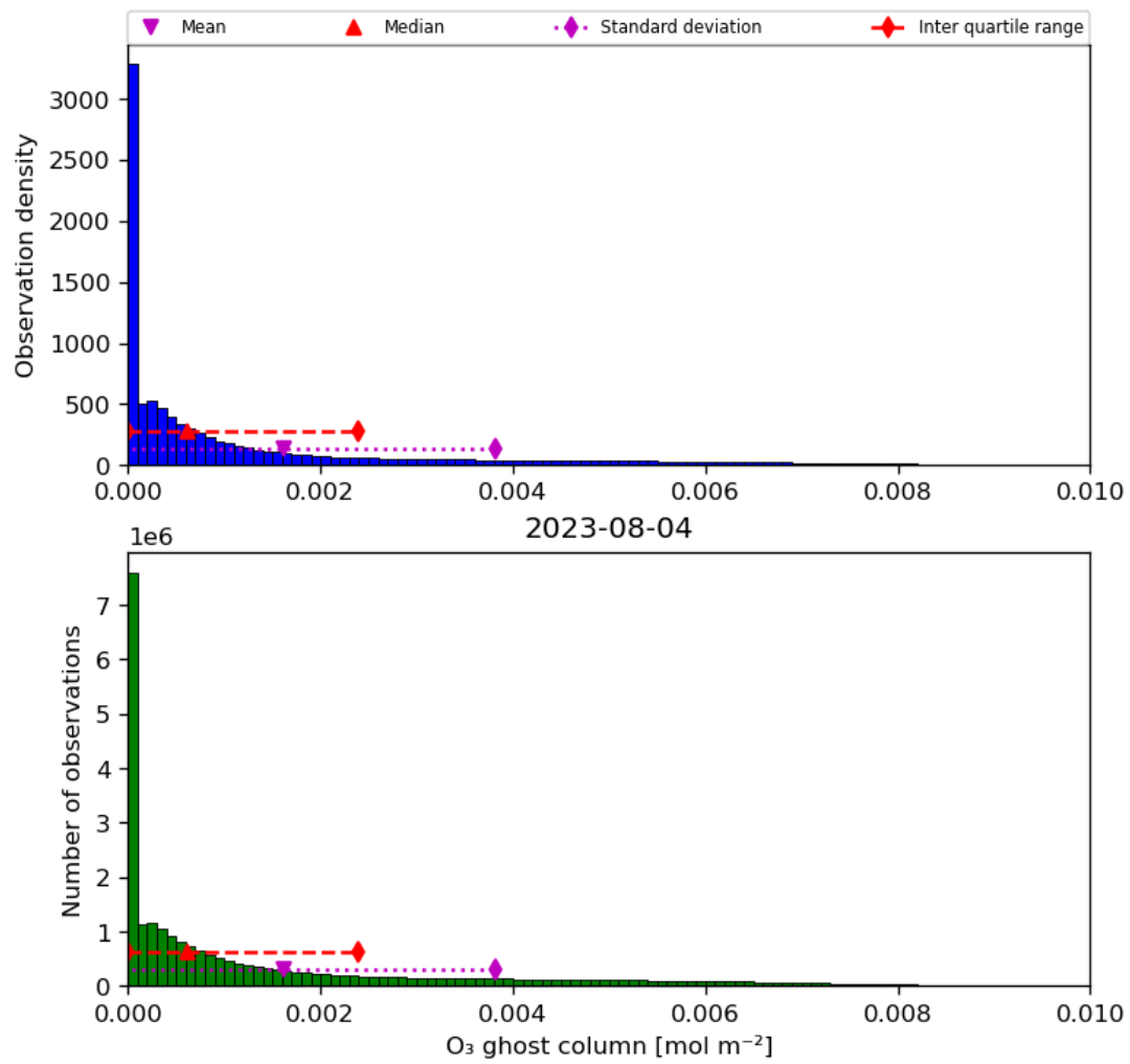
Figure 25: Histogram of “O 3 ghost column” for 2023-08-04 to 2023-08-05
