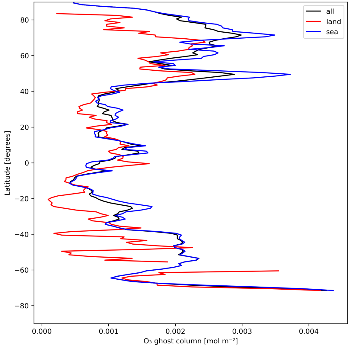
Figure 18: Zonal average of "O 3 ghost column" for 2023-08-04 to 2023-08-05.
