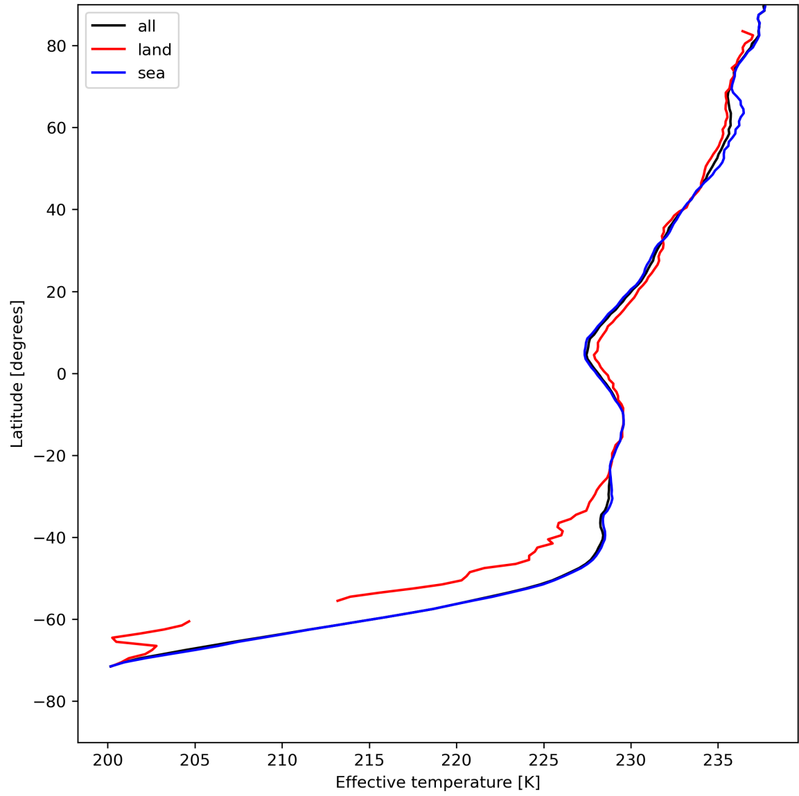
Figure 17: Zonal average of "Effective temperature" for 2023-08-04 to 2023-08-05.
