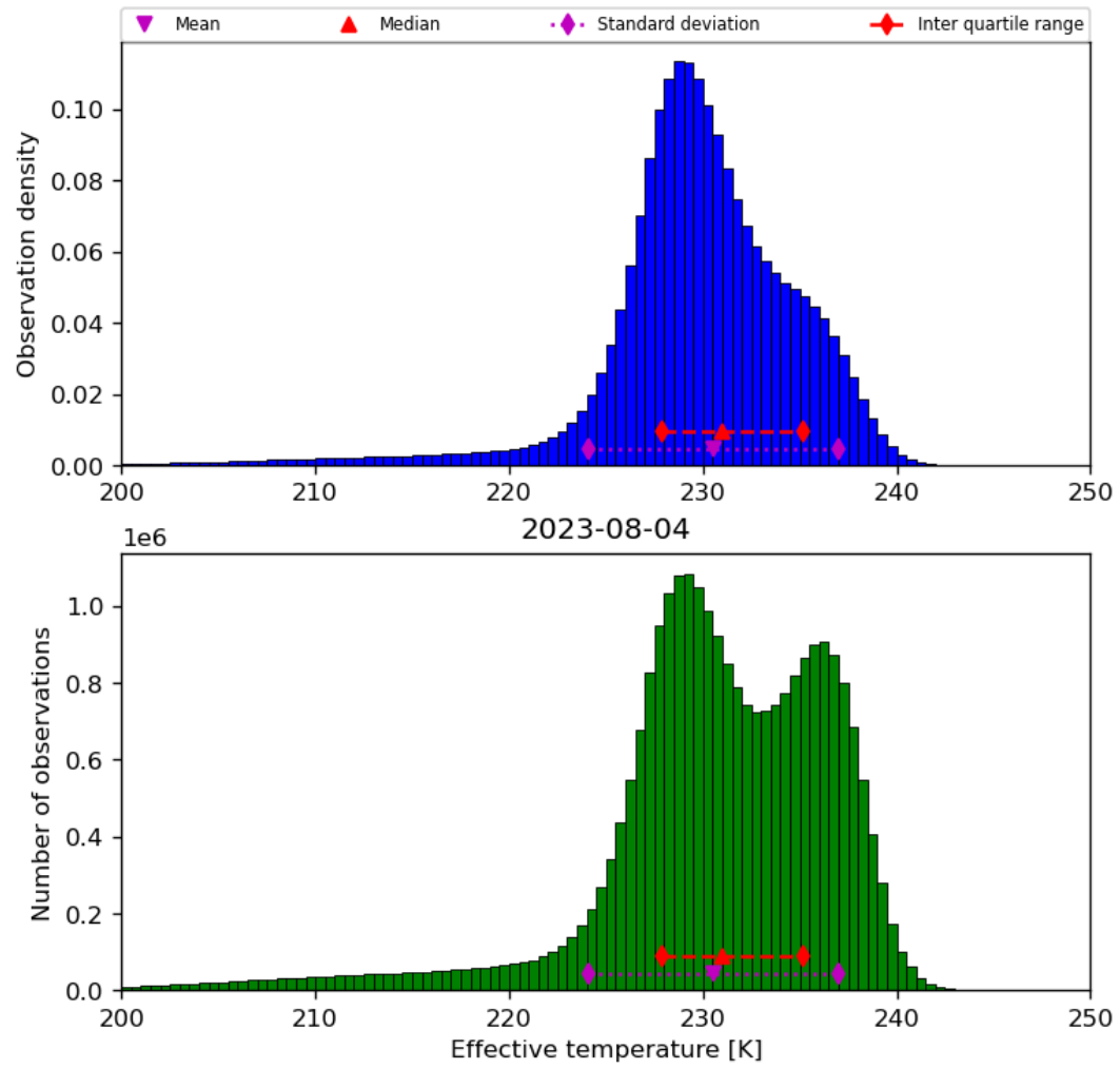
Figure 24: Histogram of “Effective temperature” for 2023-08-04 to 2023-08-05
