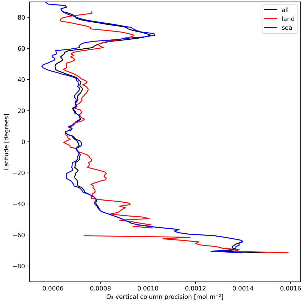
Figure 15: Zonal average of "O 3 vertical column precision" for 2023-08-04 to 2023-08-05.
