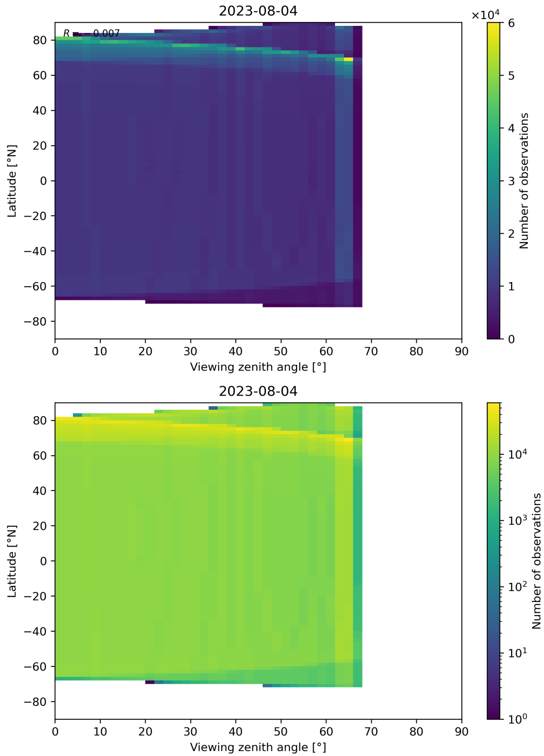
Figure 49: Scatter density plot of “Viewing zenith angle” against “Latitude” for 2023-08-04 to 2023-08-05.
