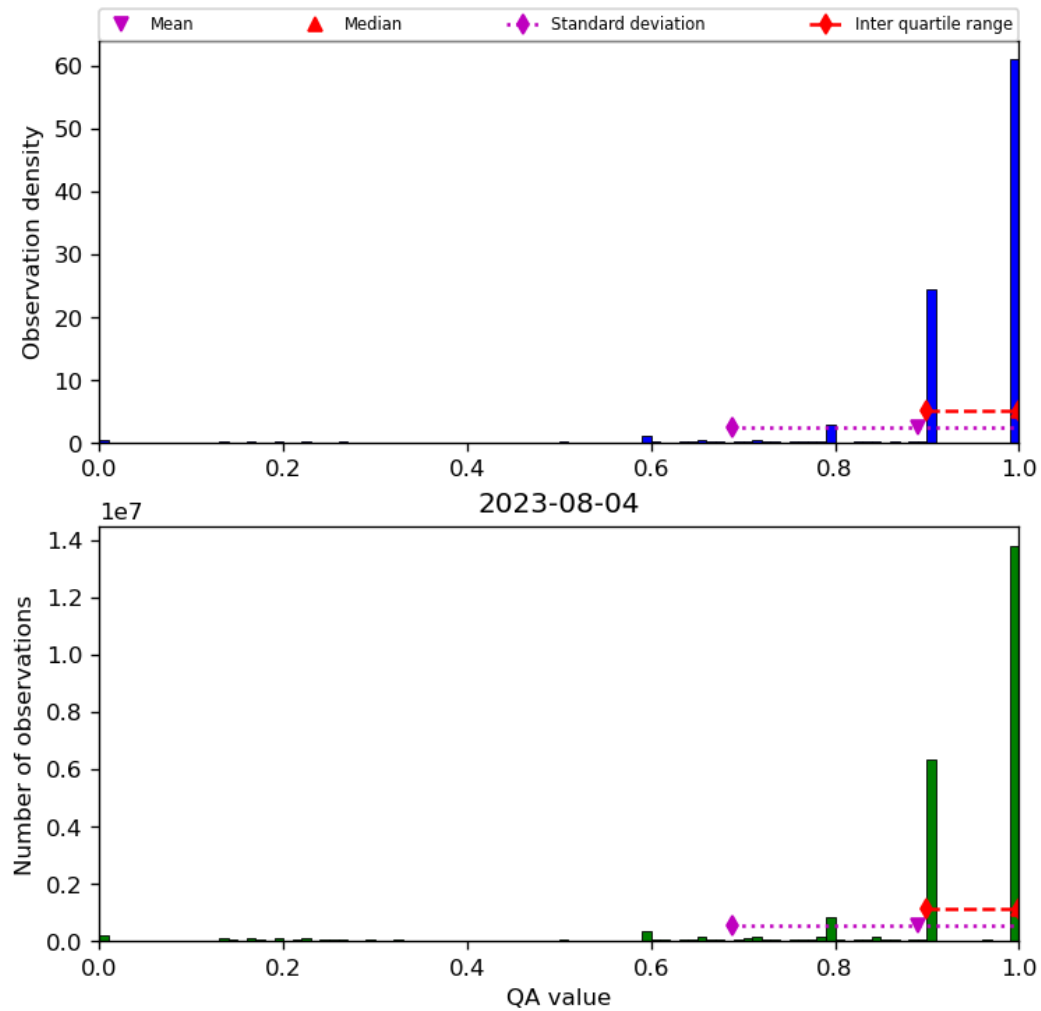
Figure 20: Histogram of “QA value” for 2023-08-04 to 2023-08-05
