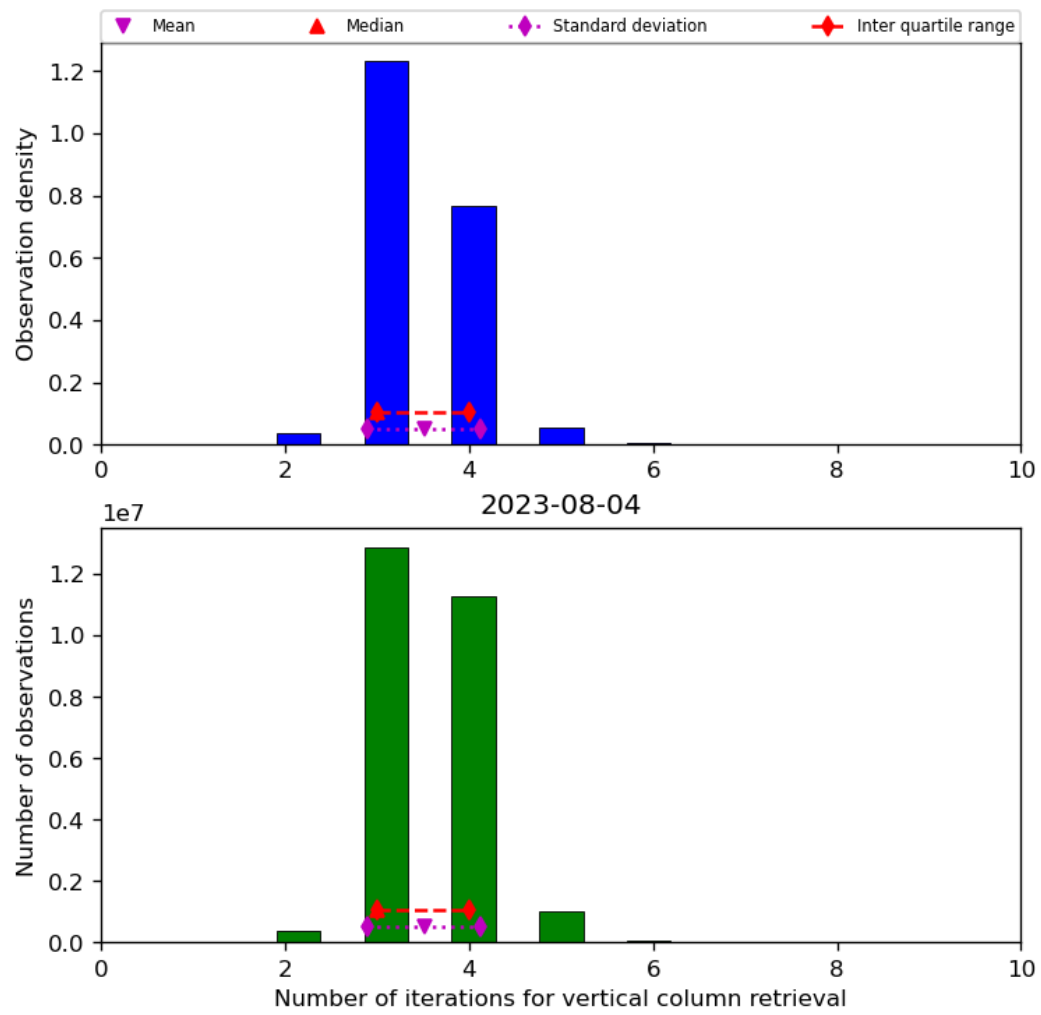
Figure 26: Histogram of “Number of iterations for vertical column retrieval” for 2023-08-04 to 2023-08-05
