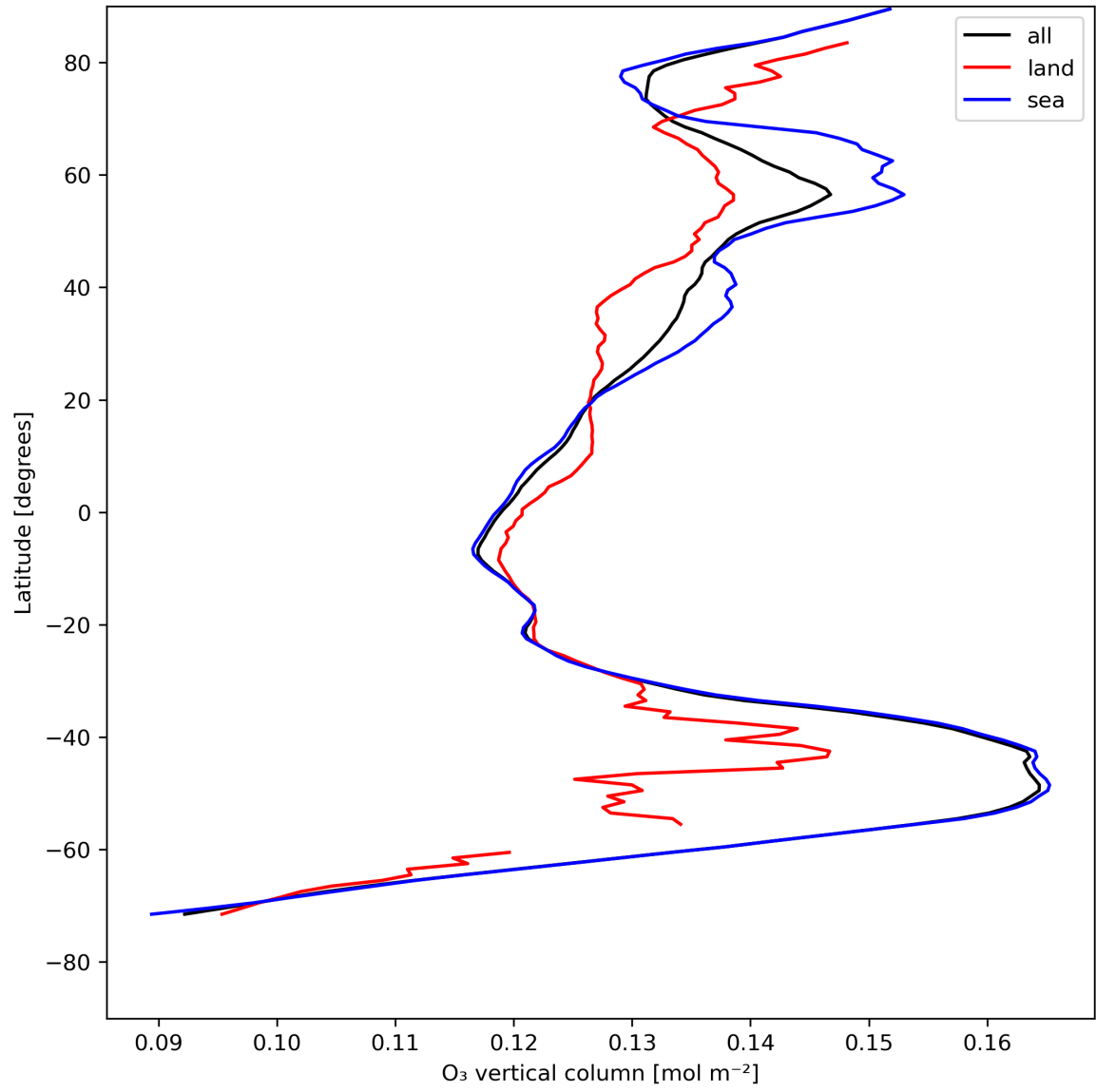
Figure 14: Zonal average of “O 3 vertical column” for 2023-08-04 to 2023-08-05.
