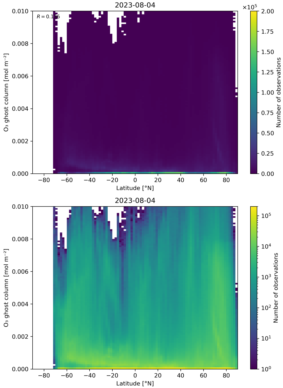
Figure 35: Scatter density plot of “Latitude” against “O 3 ghost column” for 2023-08-04 to 2023-08-05.
