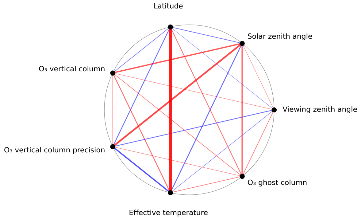
Figure 1: Map of correlation graph for 2023-08-04 to 2023-08-05.
