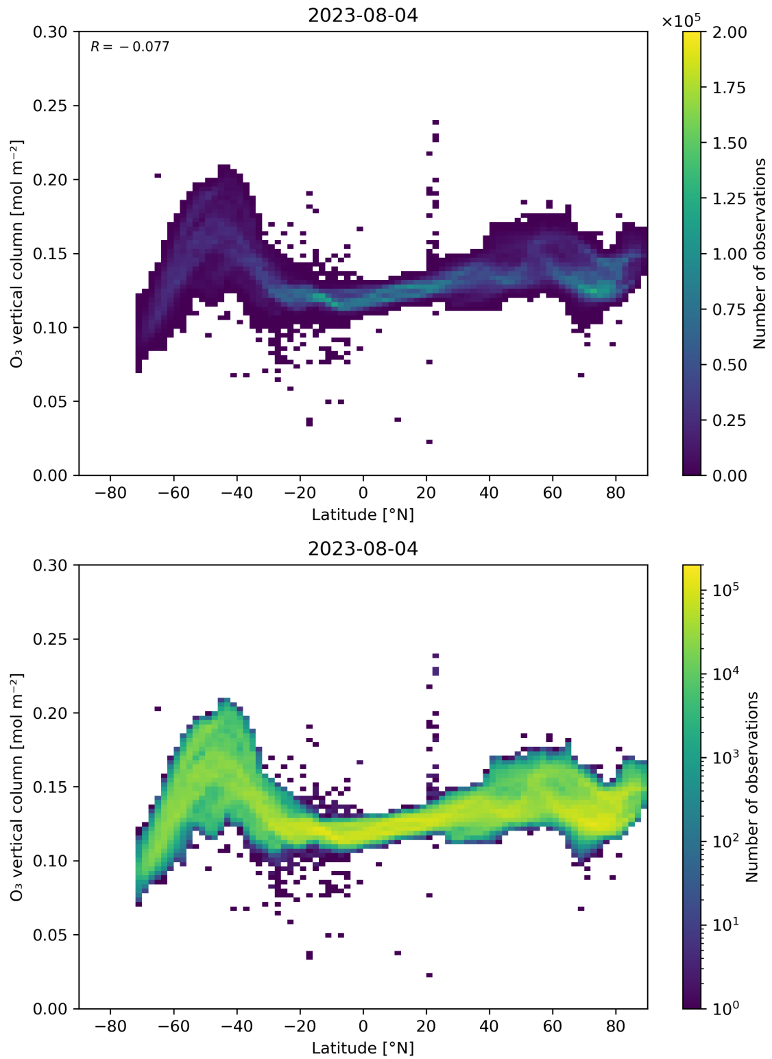
Figure 36: Scatter density plot of “Latitude” against “O 3 vertical column” for 2023-08-04 to 2023-08-05.
