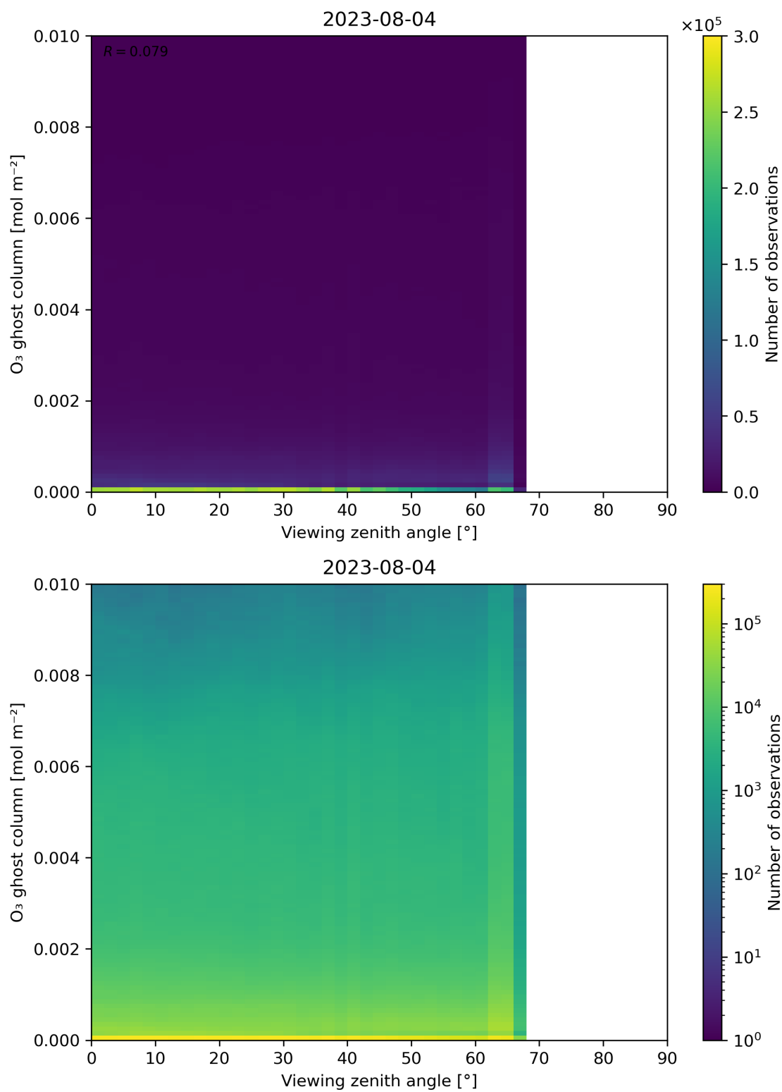
Figure 51: Scatter density plot of “Viewing zenith angle” against “O 3 ghost column” for 2023-08-04 to 2023-08-05.
