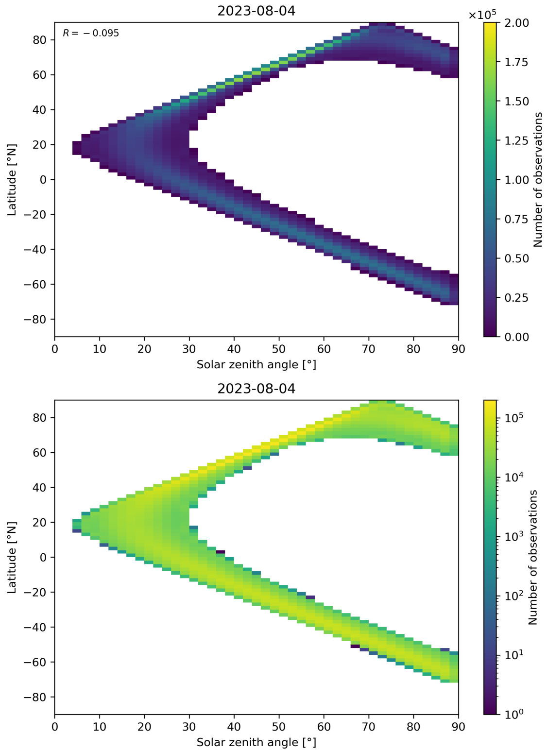
Figure 44: Scatter density plot of “Solar zenith angle” against “Latitude” for 2023-08-04 to 2023-08-05.
