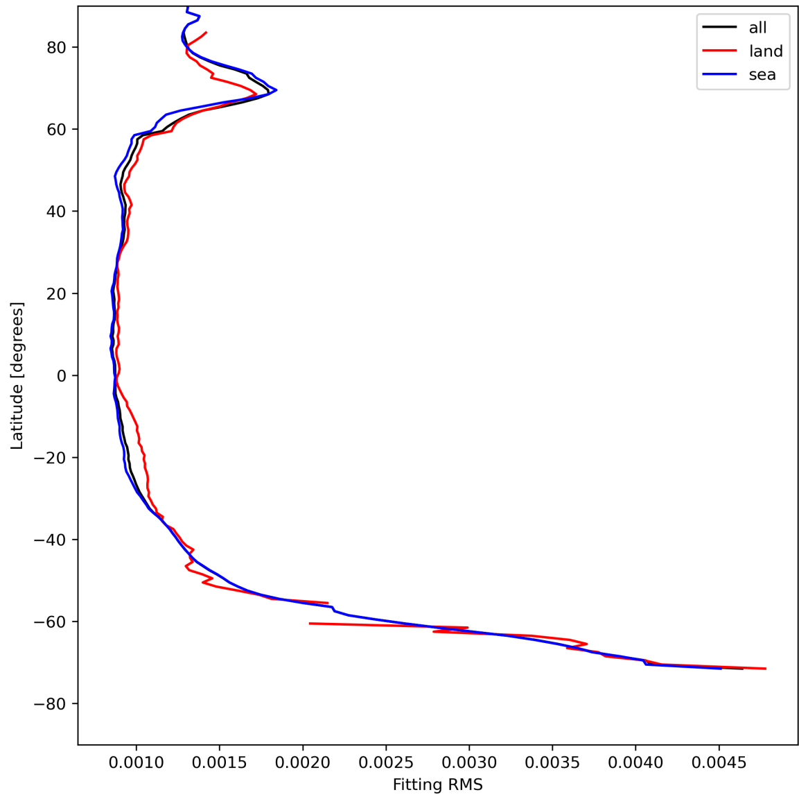
Figure 16: Zonal average of “Fitting RMS” for 2023-08-04 to 2023-08-05.
