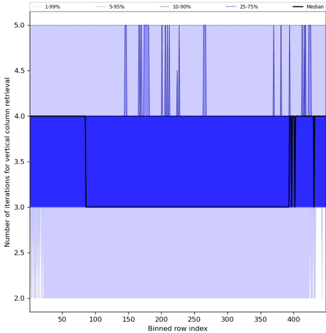
Figure 33: Along track statistics of “Number of iterations for vertical column retrieval” for 2023-08-04 to 2023-08-05
