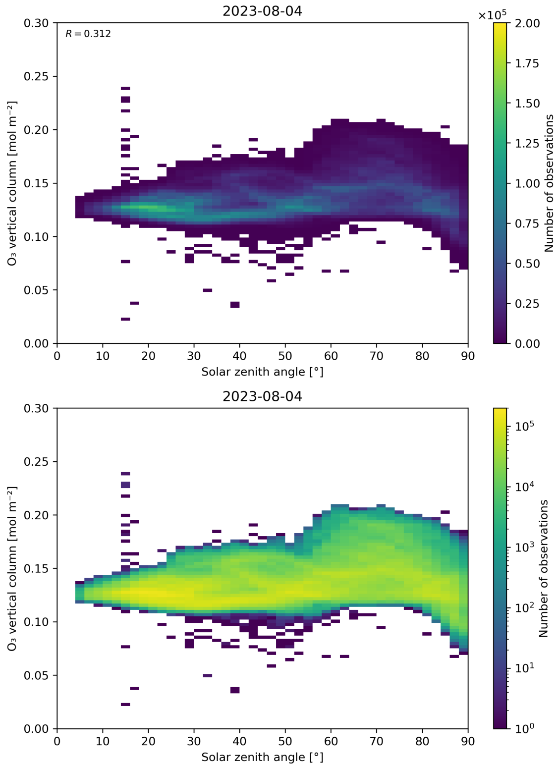
Figure 47: Scatter density plot of “Solar zenith angle” against “O 3 vertical column” for 2023-08-04 to 2023-08-05.
