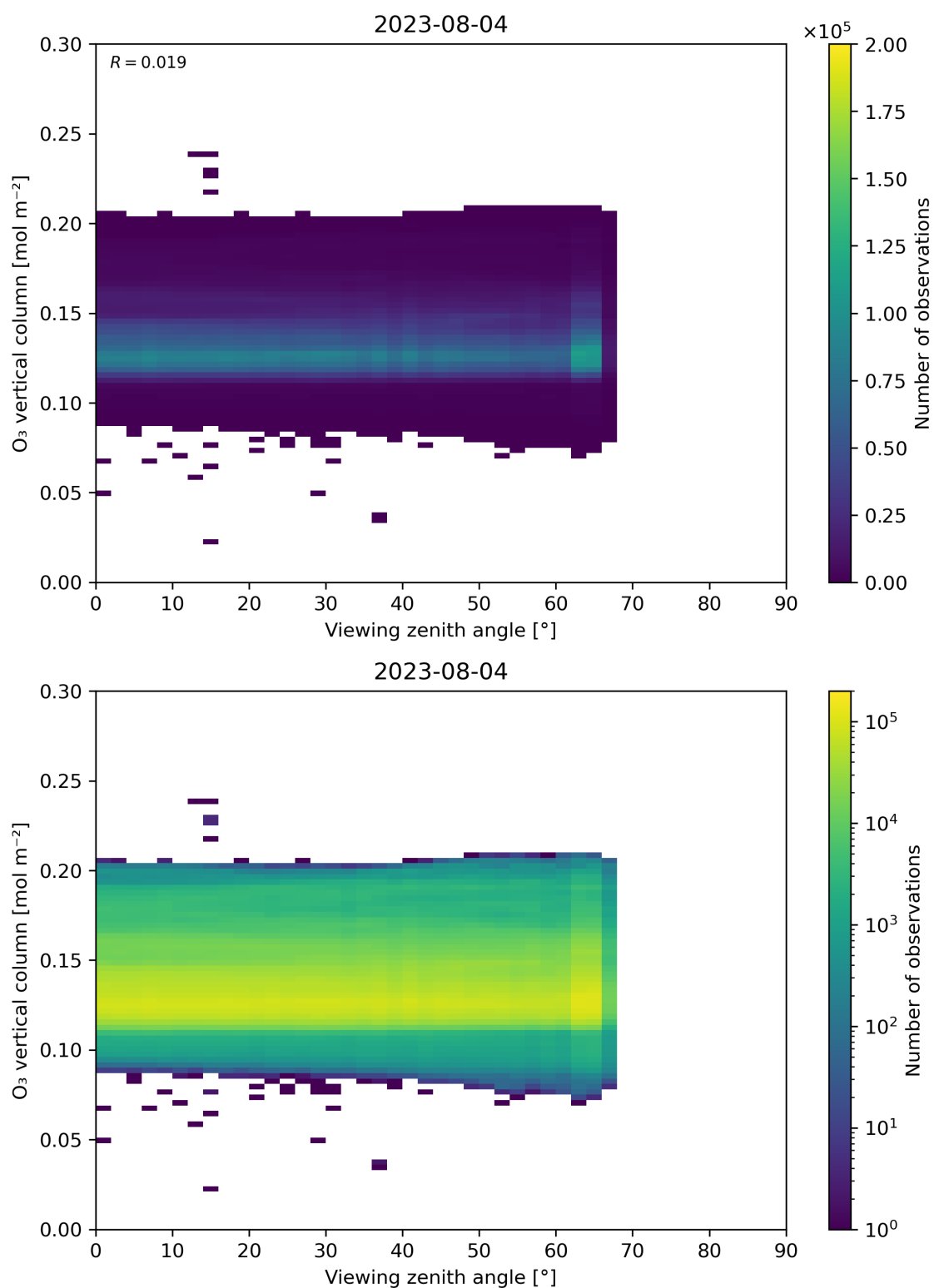
Figure 52: Scatter density plot of “Viewing zenith angle” against “O 3 vertical column” for 2023-08-04 to 2023-08-05.
