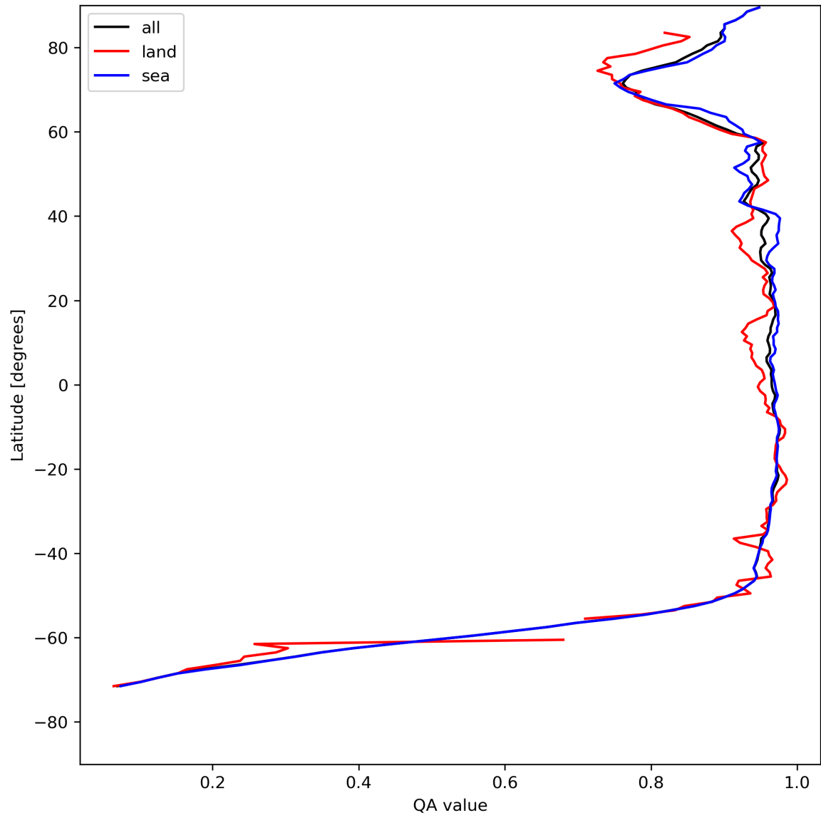
Figure 13: Zonal average of “QA value” for 2023-08-04 to 2023-08-05.
