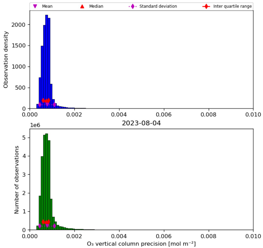
Figure 22: Histogram of “O 3 vertical column precision” for 2023-08-04 to 2023-08-05
