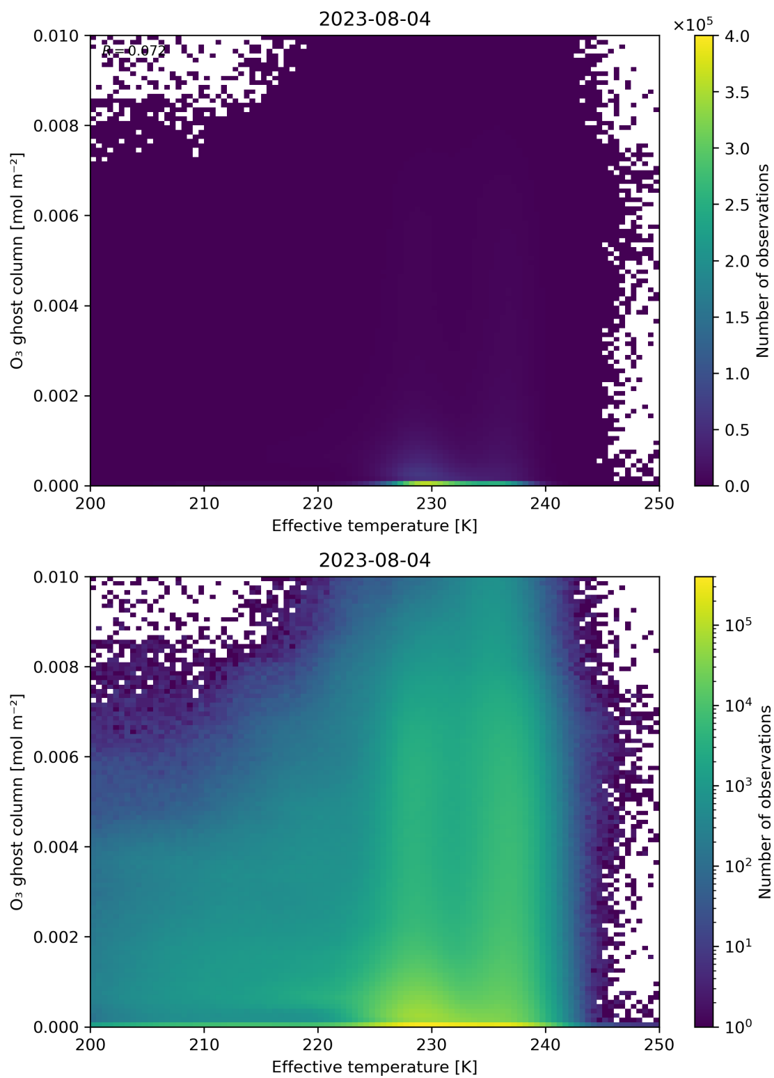
Figure 38: Scatter density plot of “Effective temperature” against “O 3 ghost column” for 2023-08-04 to 2023-08-05.
