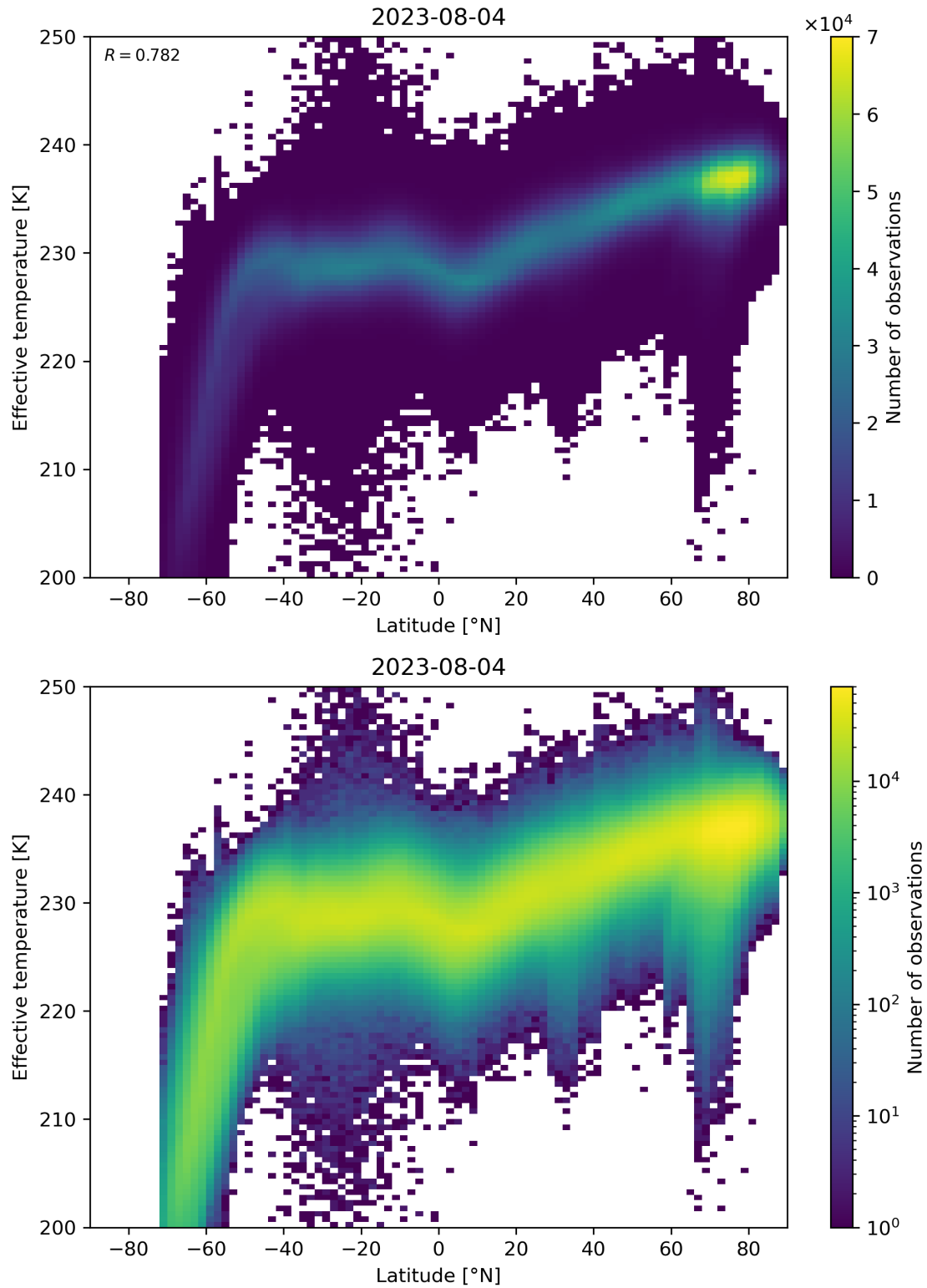
Figure 34: Scatter density plot of “Latitude” against “Effective temperature” for 2023-08-04 to 2023-08-05.
