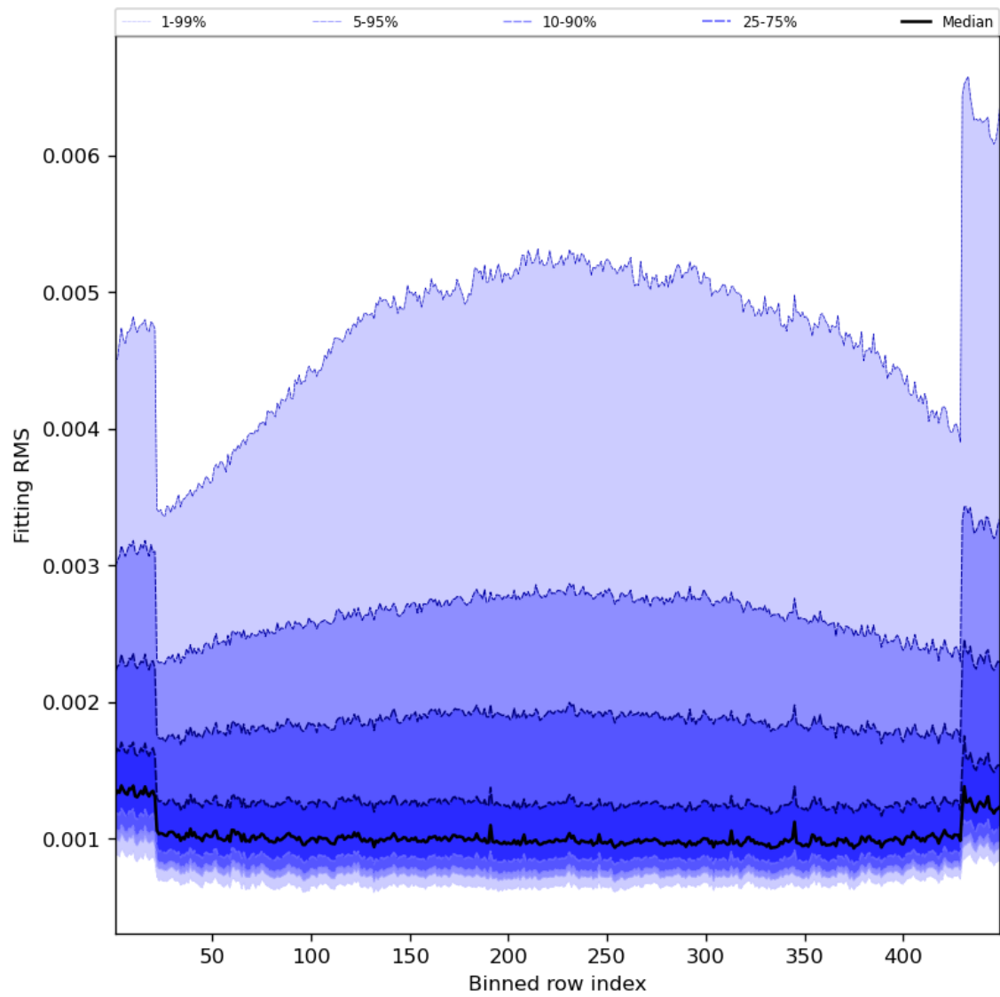
Figure 30: Along track statistics of “Fitting RMS” for 2023-08-04 to 2023-08-05
