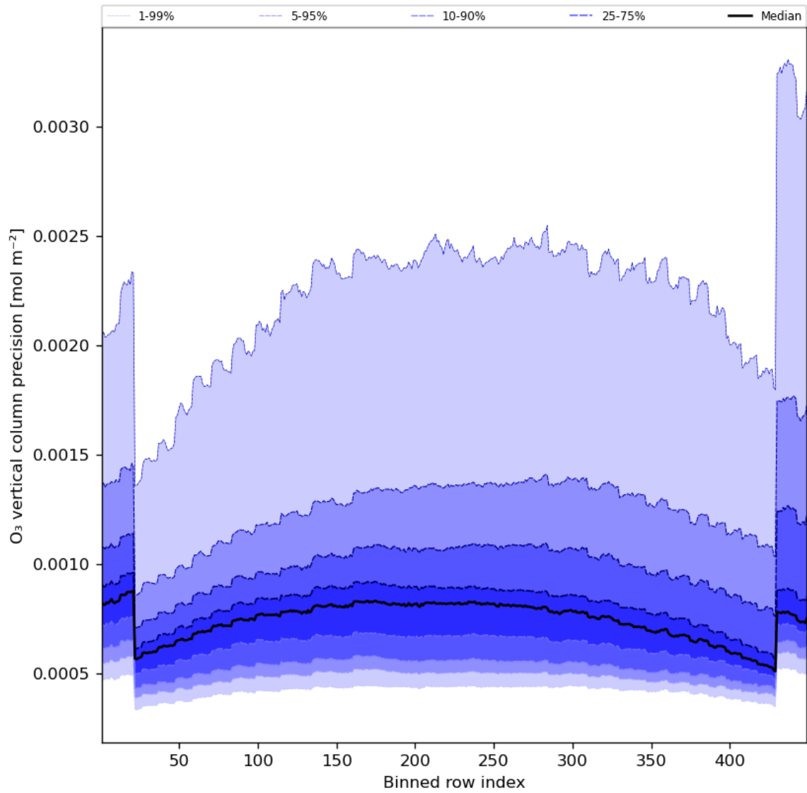
Figure 29: Along track statistics of “O 3 vertical column precision” for 2023-08-04 to 2023-08-05
