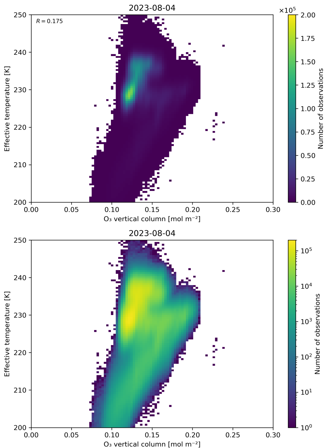
Figure 39: Scatter density plot of “O 3 vertical column” against “Effective temperature” for 2023-08-04 to 2023-08-05.
