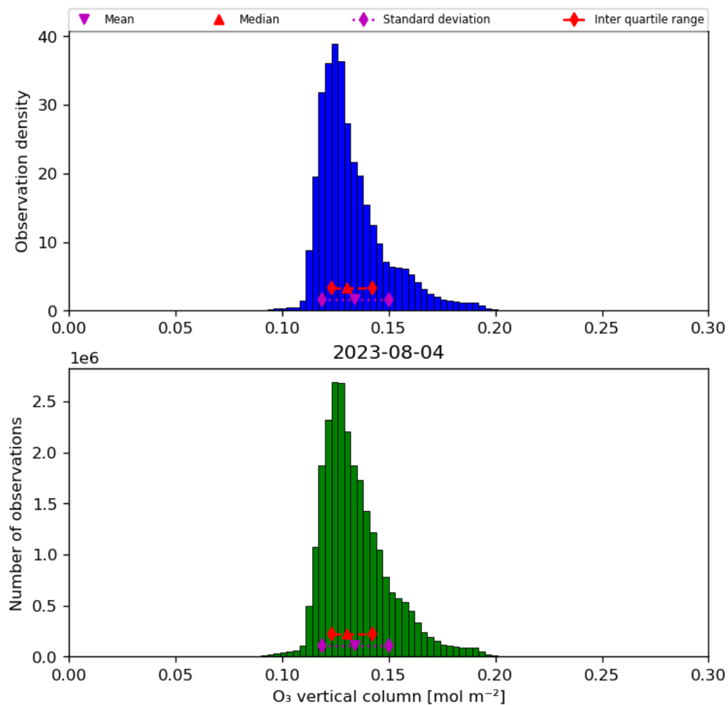
Figure 21: Histogram of “O 3 vertical column” for 2023-08-04 to 2023-08-05
