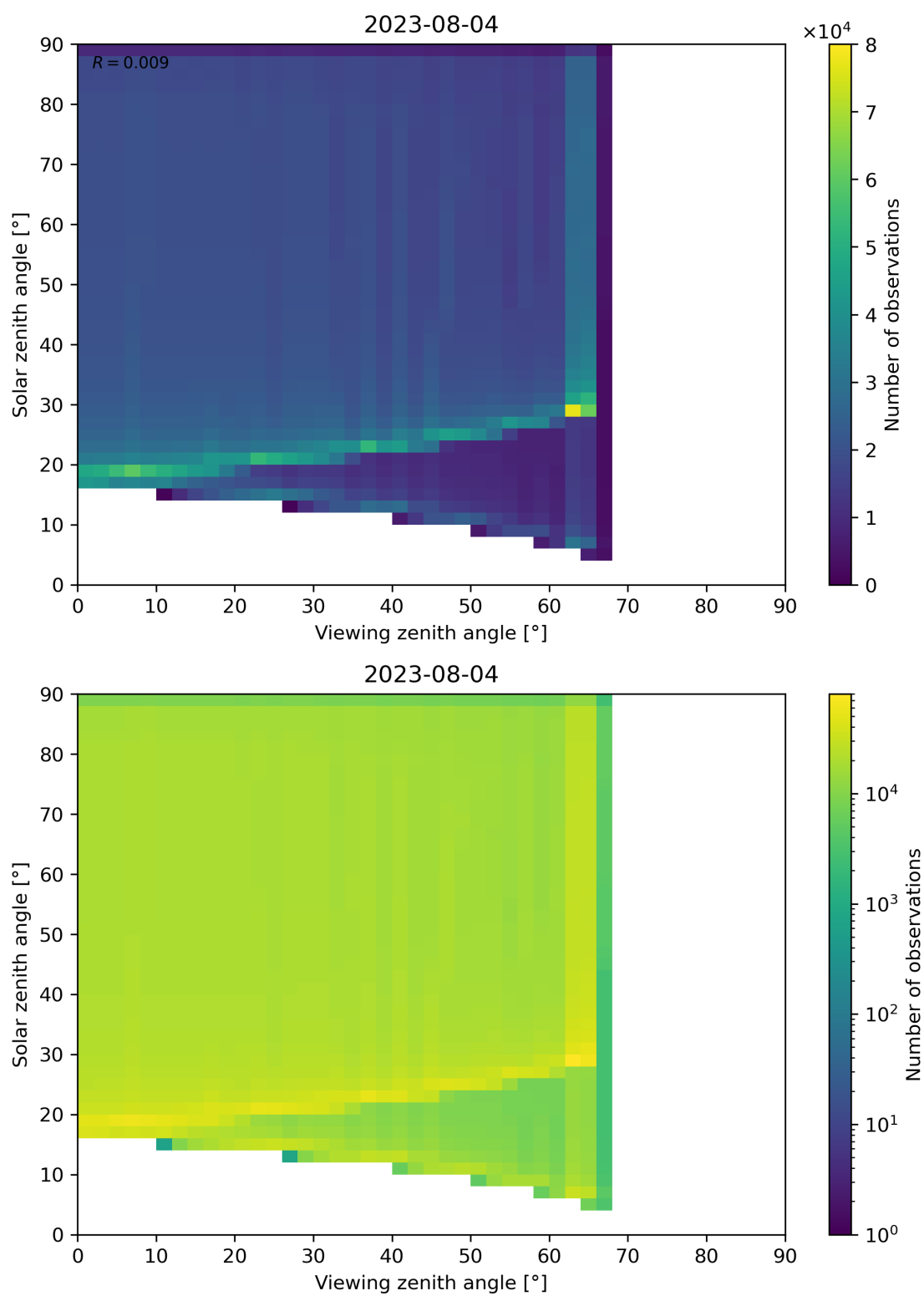
Figure 54: Scatter density plot of “Viewing zenith angle” against “Solar zenith angle” for 2023-08-04 to 2023-08-05.
