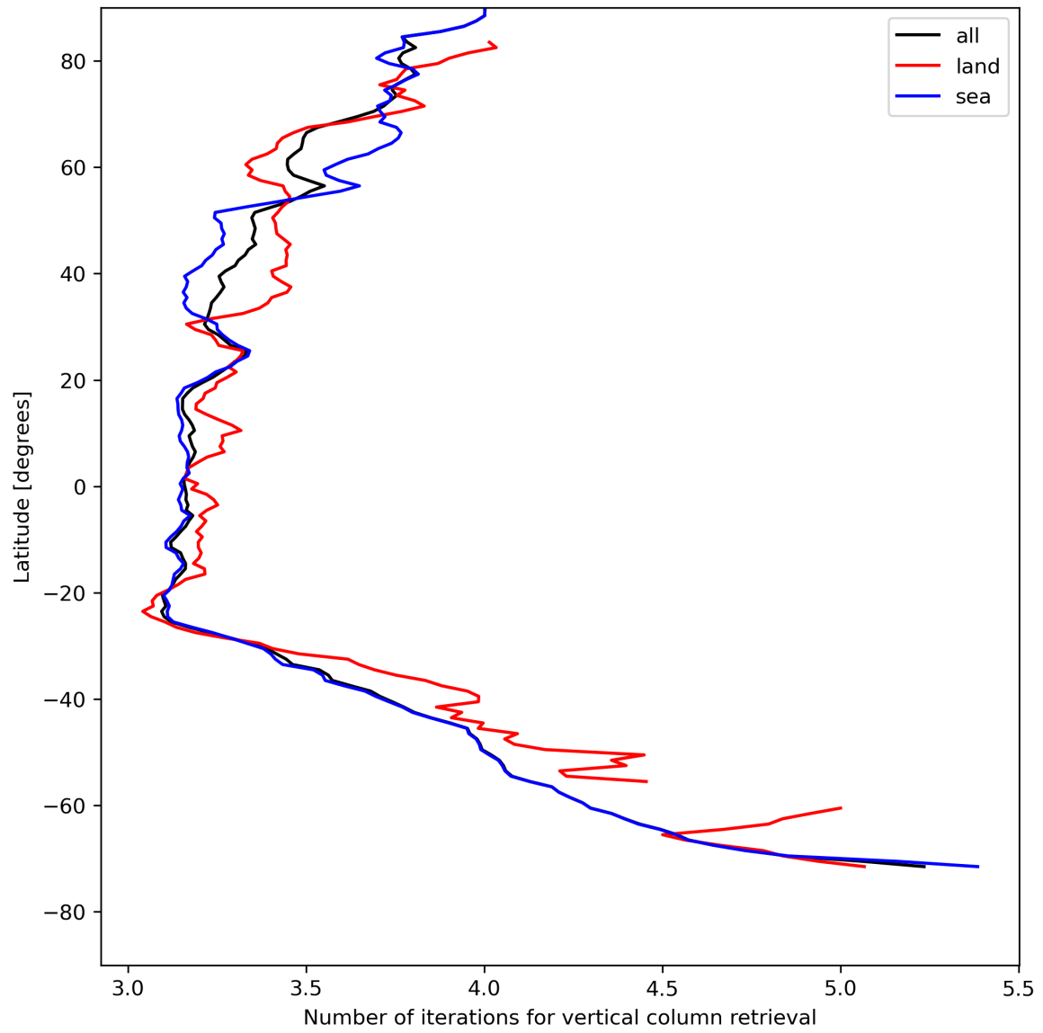
Figure 19: Zonal average of “Number of iterations for vertical column retrieval” for 2023-08-04 to 2023-08-05.
