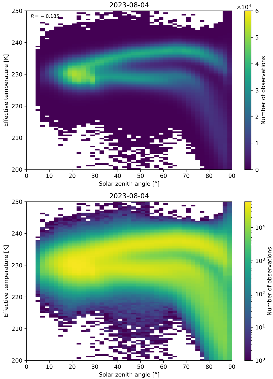
Figure 45: Scatter density plot of “Solar zenith angle” against “Effective temperature” for 2023-08-04 to 2023-08-05.
