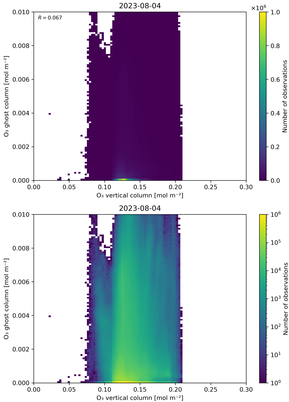
Figure 40: Scatter density plot of “O 3 vertical column” against “O 3 ghost column” for 2023-08-04 to 2023-08-05.
