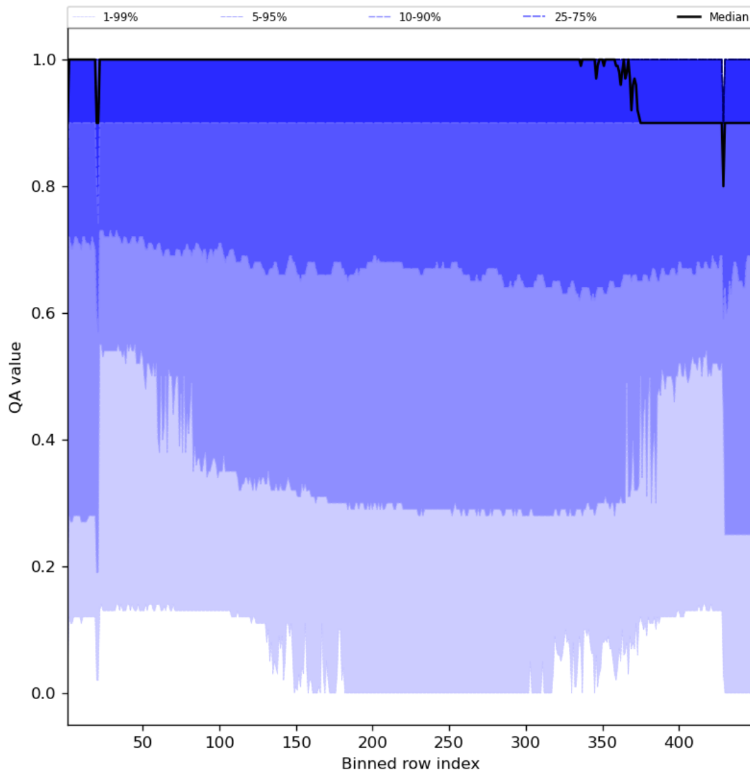
Figure 27: Along track statistics of “QA value” for 2023-08-04 to 2023-08-05
