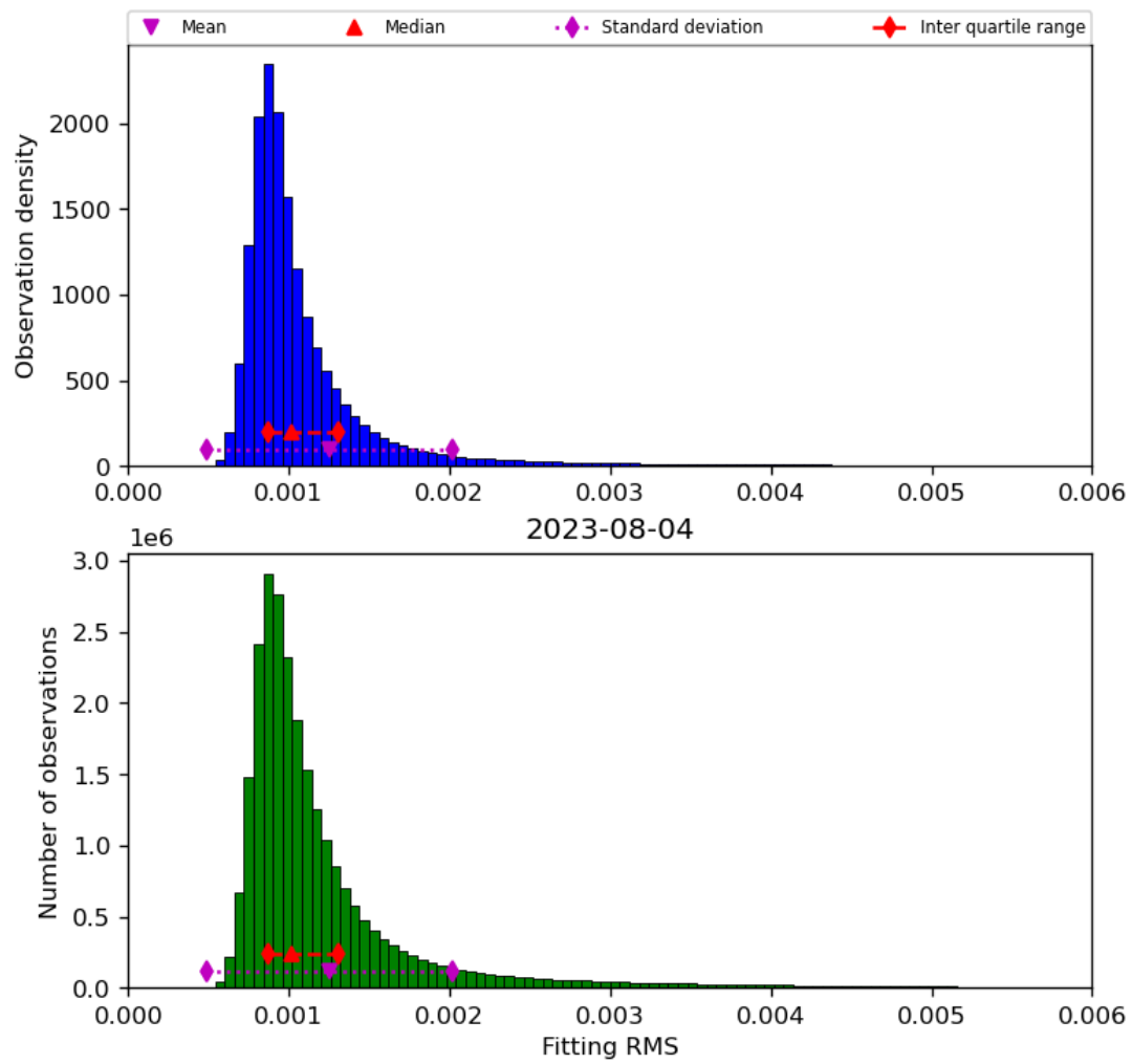
Figure 23: Histogram of “Fitting RMS” for 2023-08-04 to 2023-08-05
