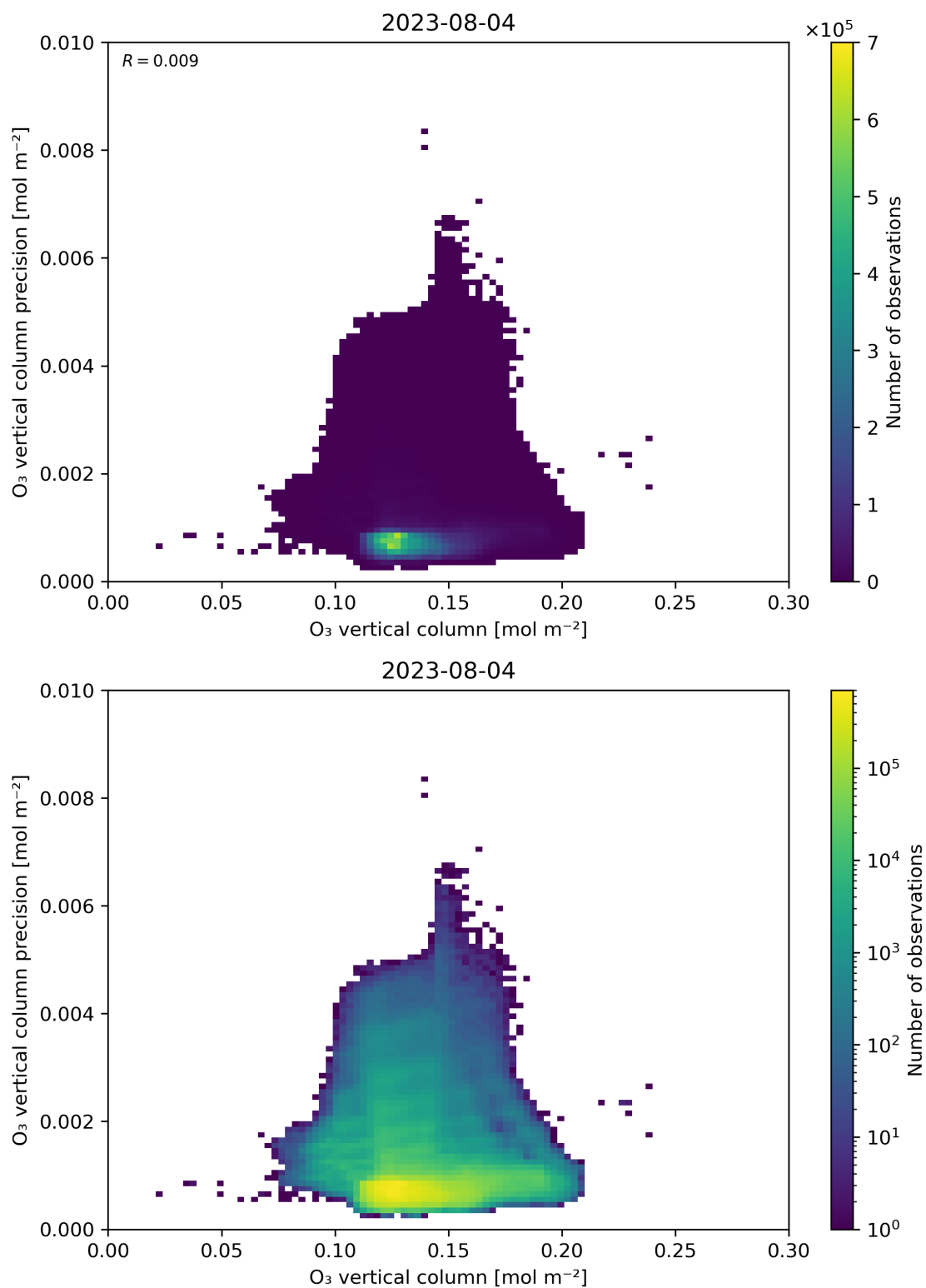
Figure 41: Scatter density plot of “O 3 vertical column” against “O 3 vertical column precision” for 2023-08-04 to 2023-08-05.
