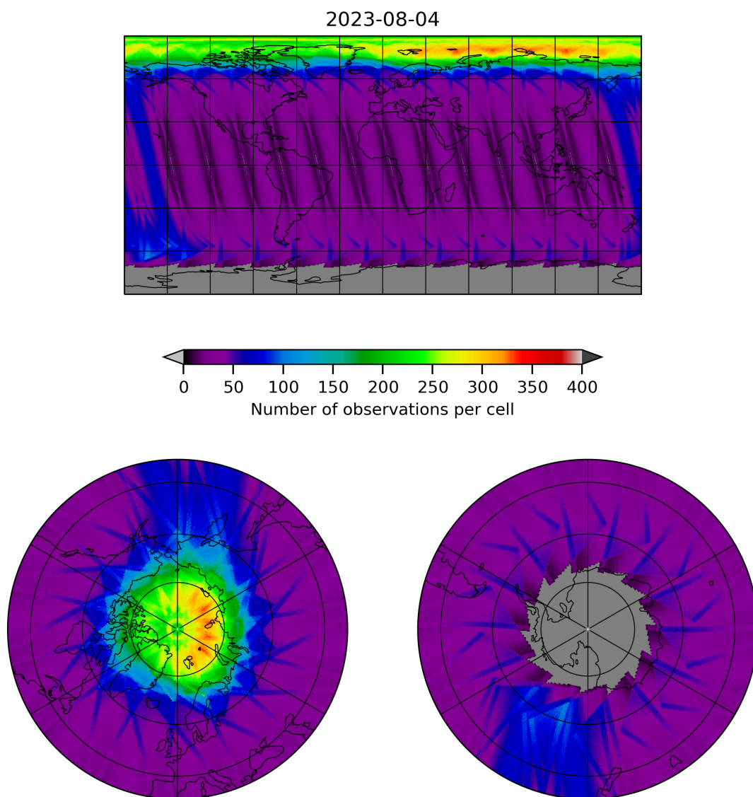
Figure 12: Map of the number of observations for 2023-08-04 to 2023-08-05
