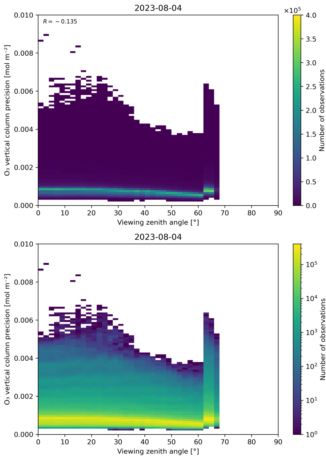
Figure 53: Scatter density plot of “Viewing zenith angle” against “O 3 vertical column precision” for 2023-08-04 to 2023-08-05.
