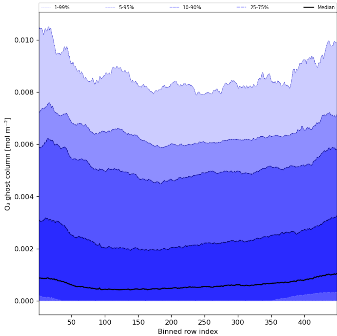
Figure 32: Along track statistics of “O 3 ghost column” for 2023-08-04 to 2023-08-05
