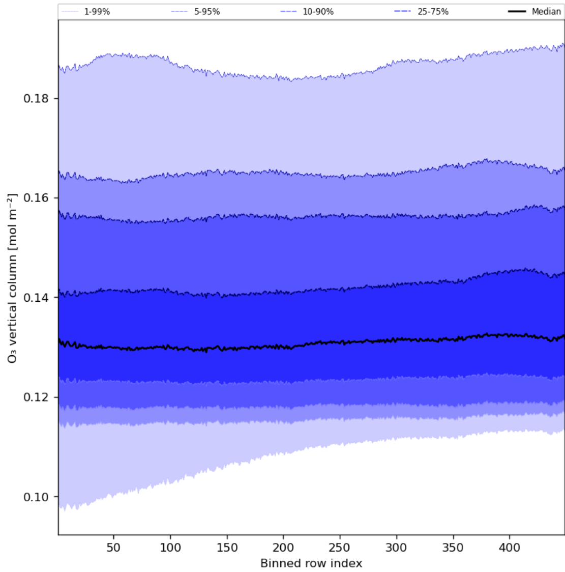
Figure 28: Along track statistics of “O 3 vertical column” for 2023-08-04 to 2023-08-05
