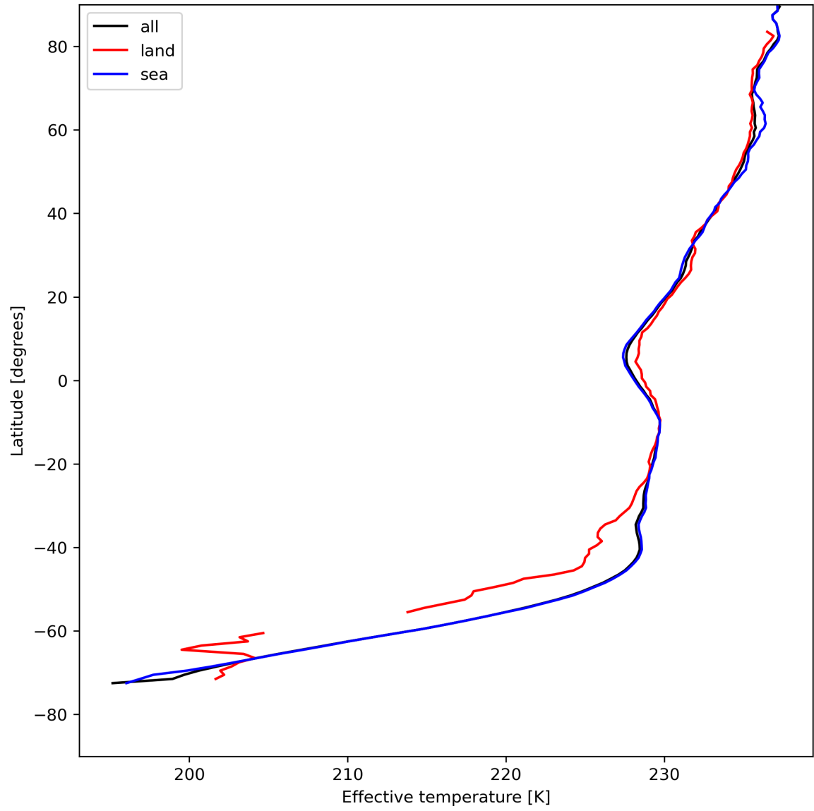
Figure 17: Zonal average of "Effective temperature" for 2023-08-04 to 2023-08-06.
