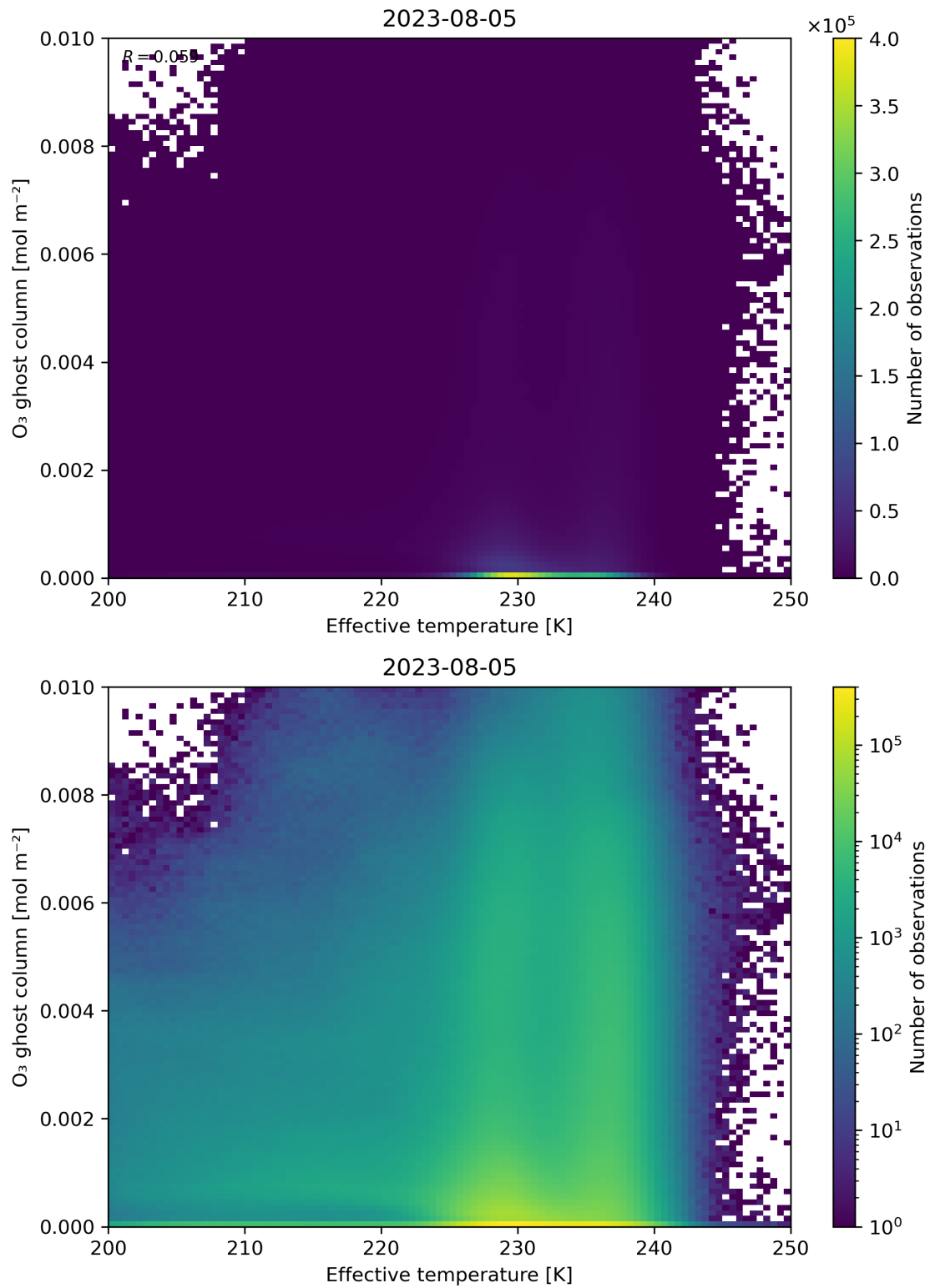
Figure 38: Scatter density plot of “Effective temperature” against “O 3 ghost column” for 2023-08-04 to 2023-08-06.
