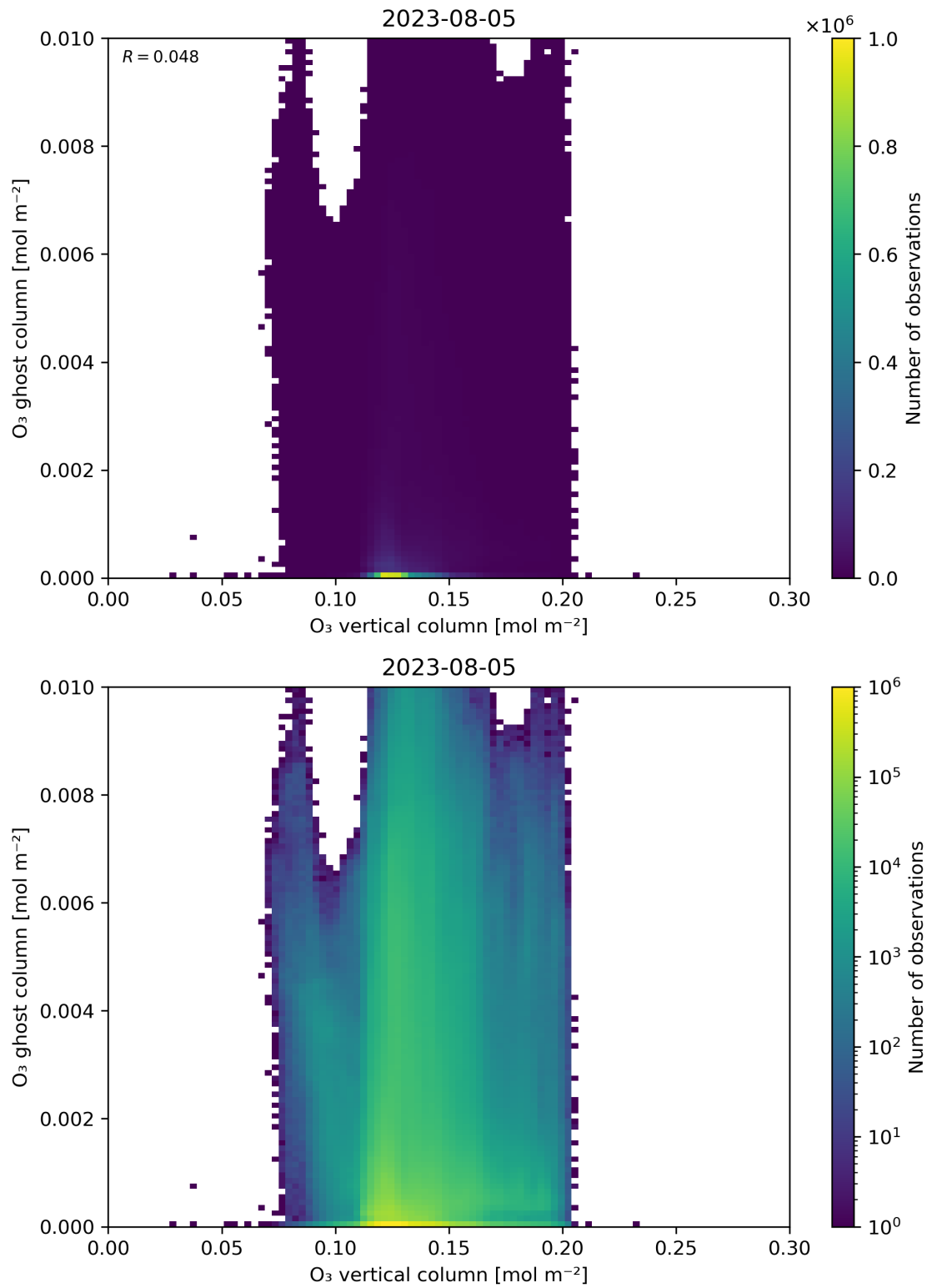
Figure 40: Scatter density plot of “O 3 vertical column” against “O 3 ghost column” for 2023-08-04 to 2023-08-06.
