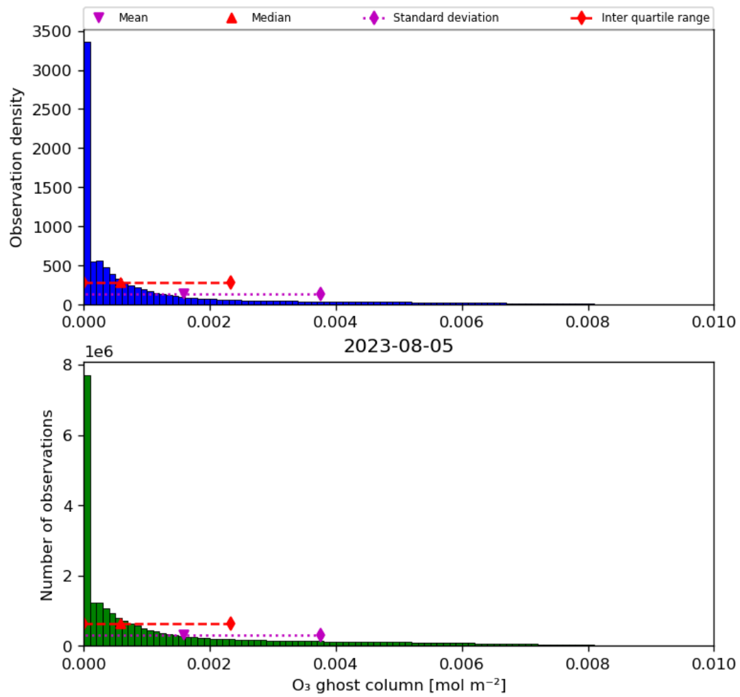
Figure 25: Histogram of “O 3 ghost column” for 2023-08-04 to 2023-08-06
