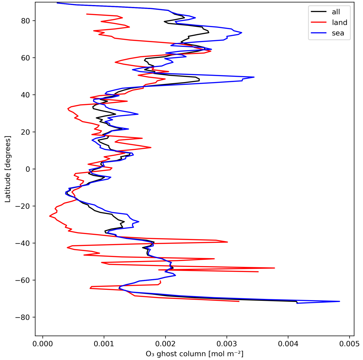
Figure 18: Zonal average of "O 3 ghost column" for 2023-08-04 to 2023-08-06.
