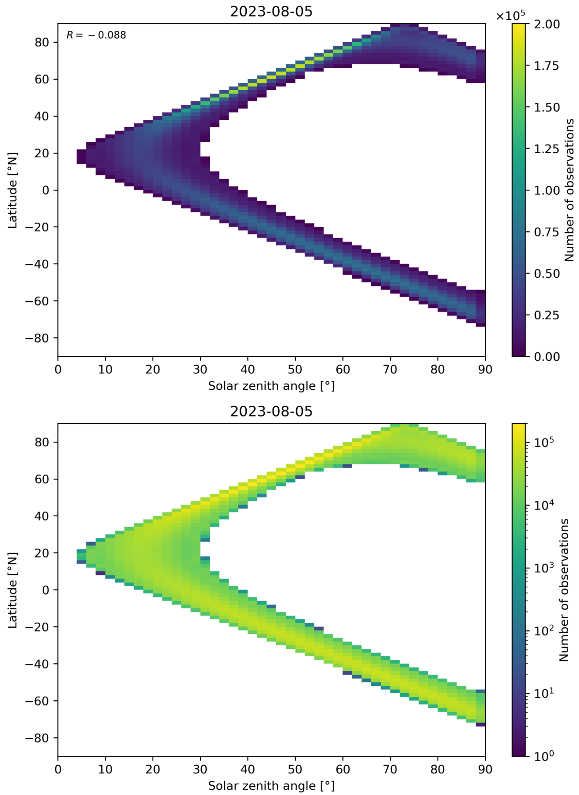
Figure 44: Scatter density plot of “Solar zenith angle” against “Latitude” for 2023-08-04 to 2023-08-06.
