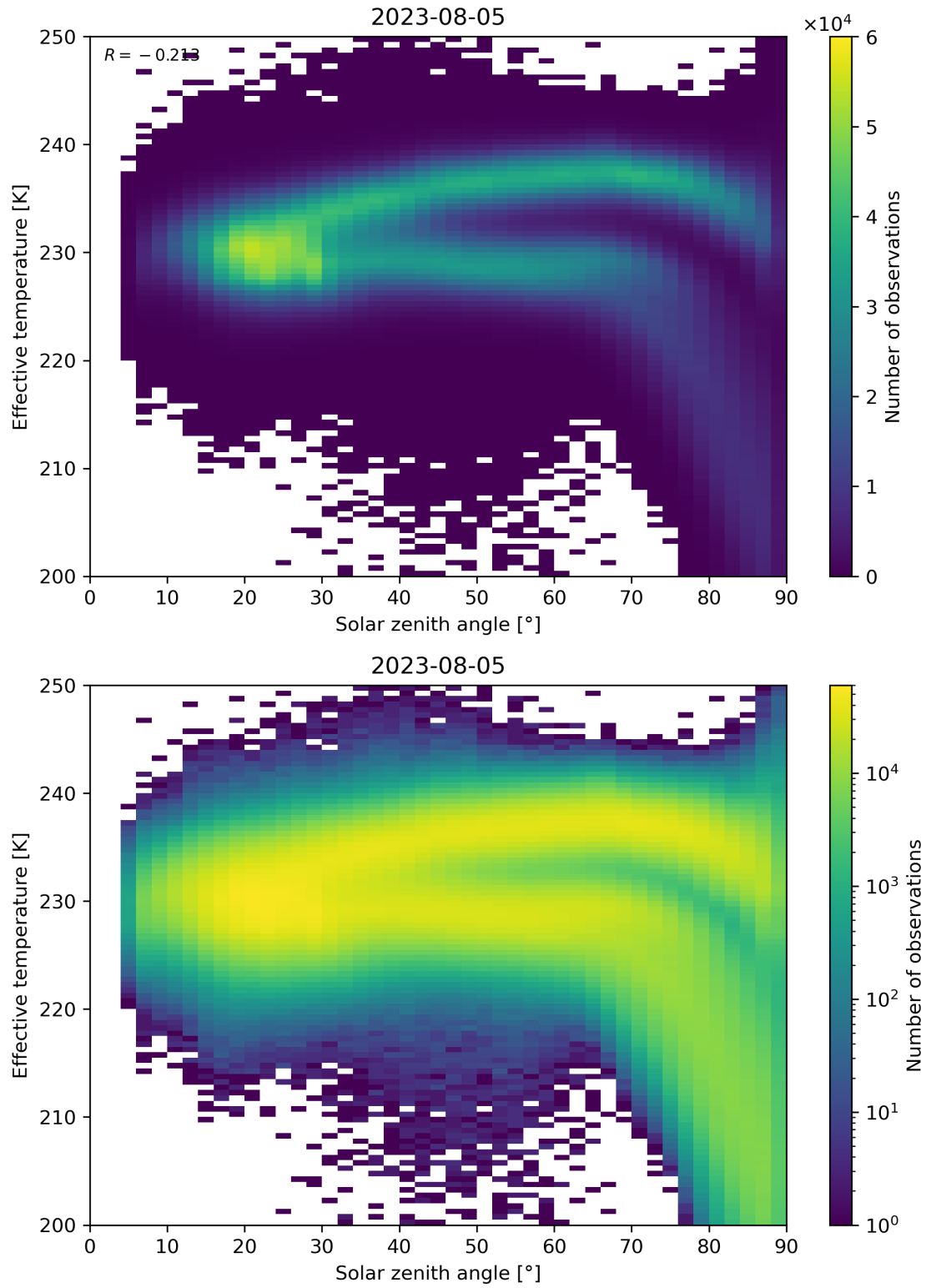
Figure 45: Scatter density plot of “Solar zenith angle” against “Effective temperature” for 2023-08-04 to 2023-08-06.
