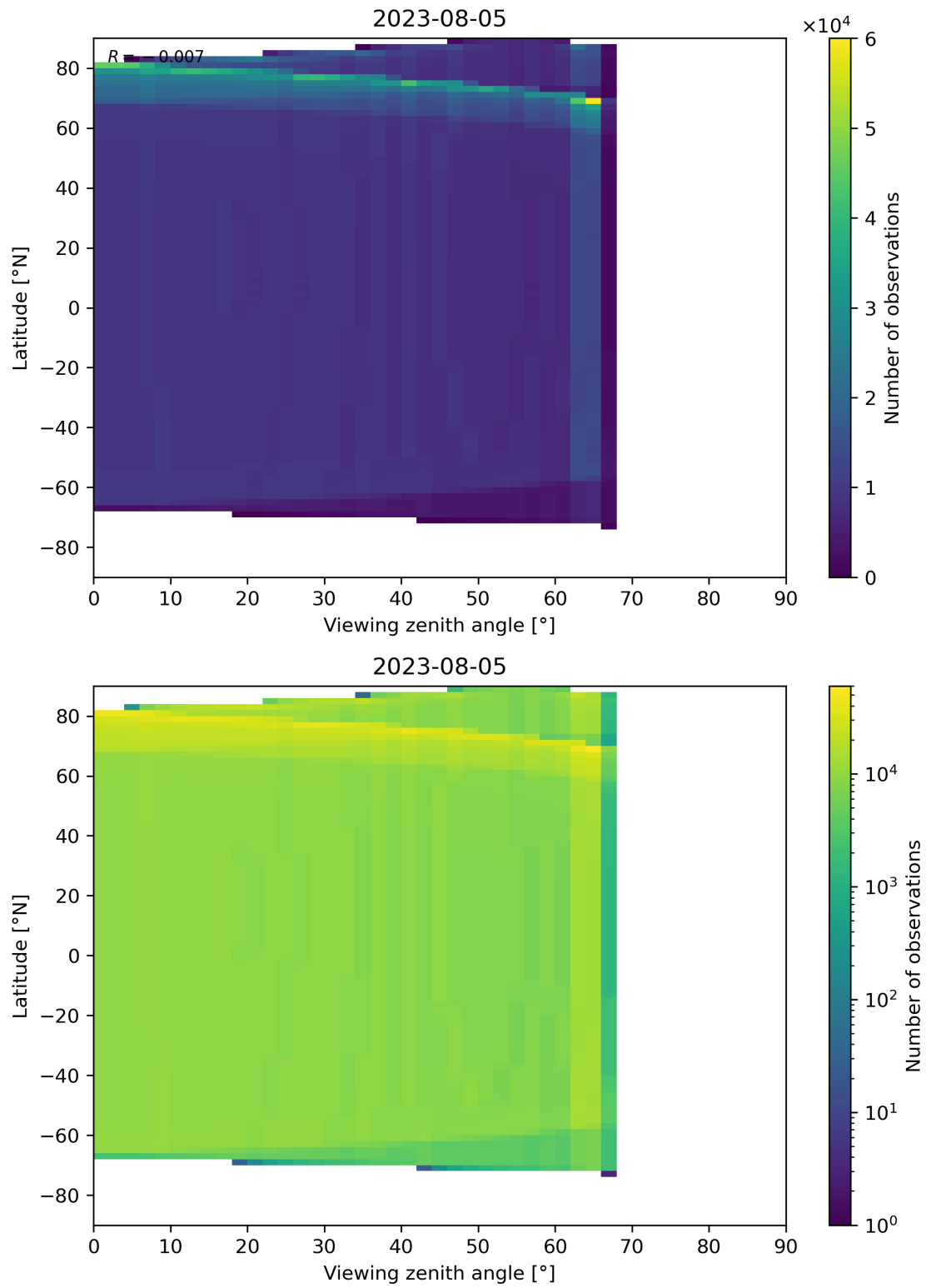
Figure 49: Scatter density plot of “Viewing zenith angle” against “Latitude” for 2023-08-04 to 2023-08-06.
