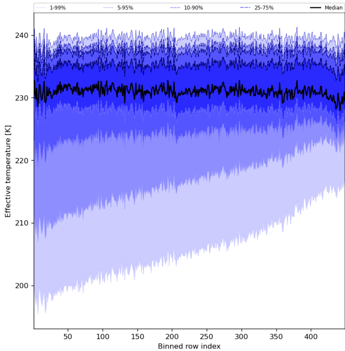
Figure 31: Along track statistics of “Effective temperature” for 2023-08-04 to 2023-08-06
