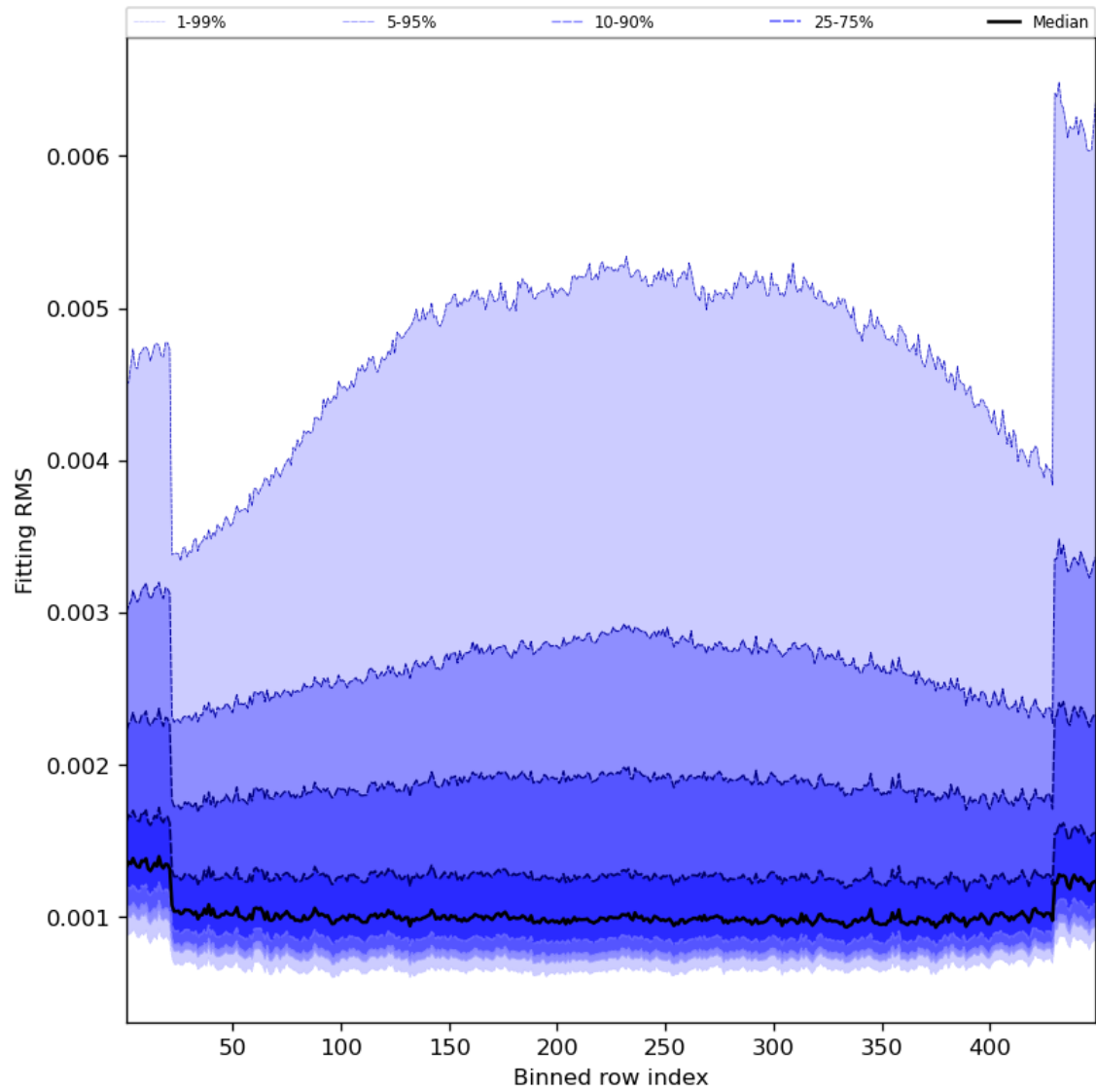
Figure 30: Along track statistics of “Fitting RMS” for 2023-08-04 to 2023-08-06
