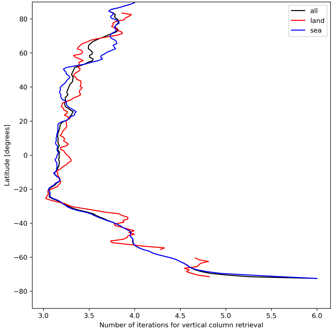
Figure 19: Zonal average of “Number of iterations for vertical column retrieval” for 2023-08-04 to 2023-08-06.
