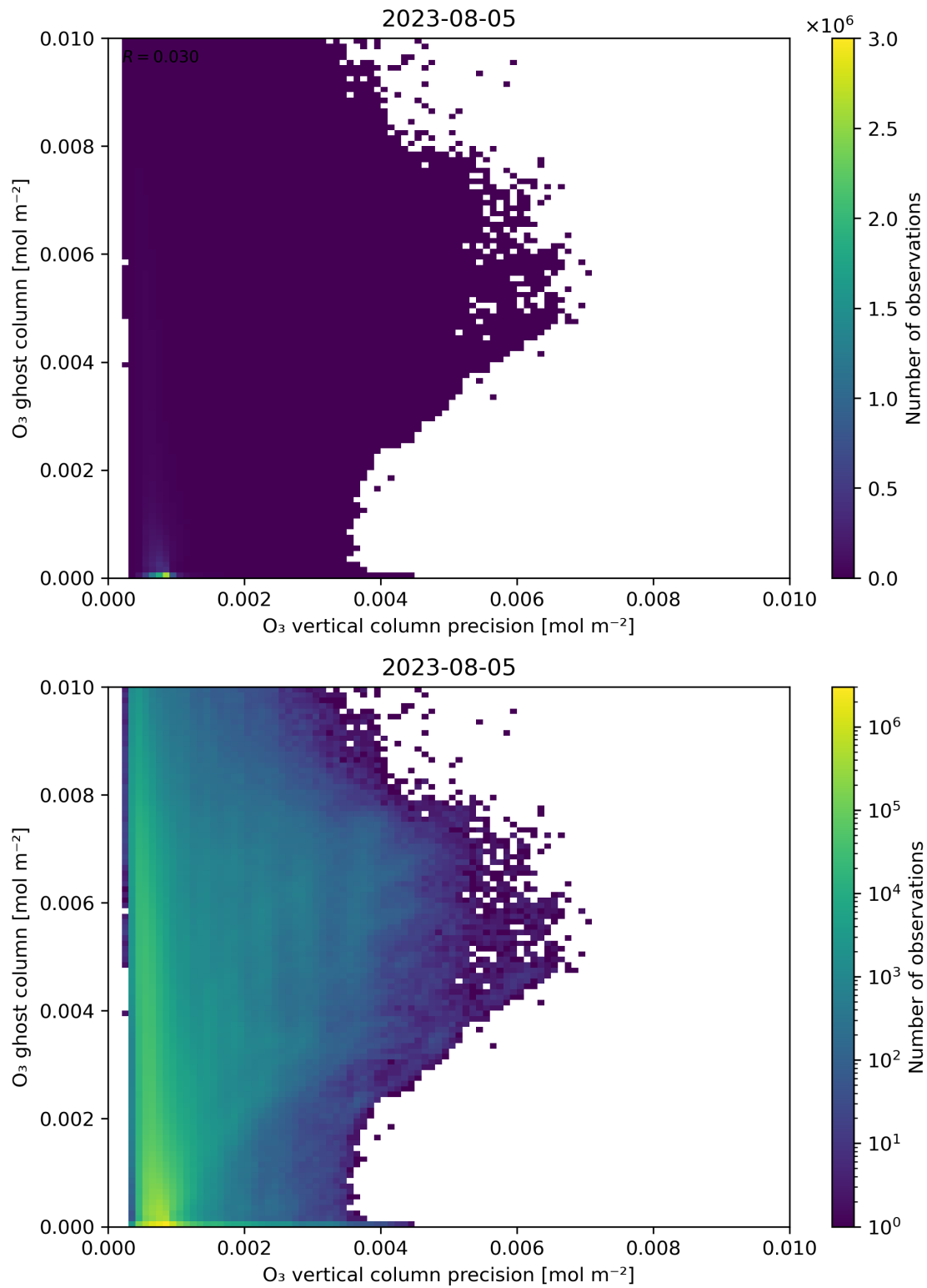
Figure 43: Scatter density plot of “ \text{O}_3 vertical column precision” against “ \text{O}_3 ghost column” for 2023-08-04 to 2023-08-06.
