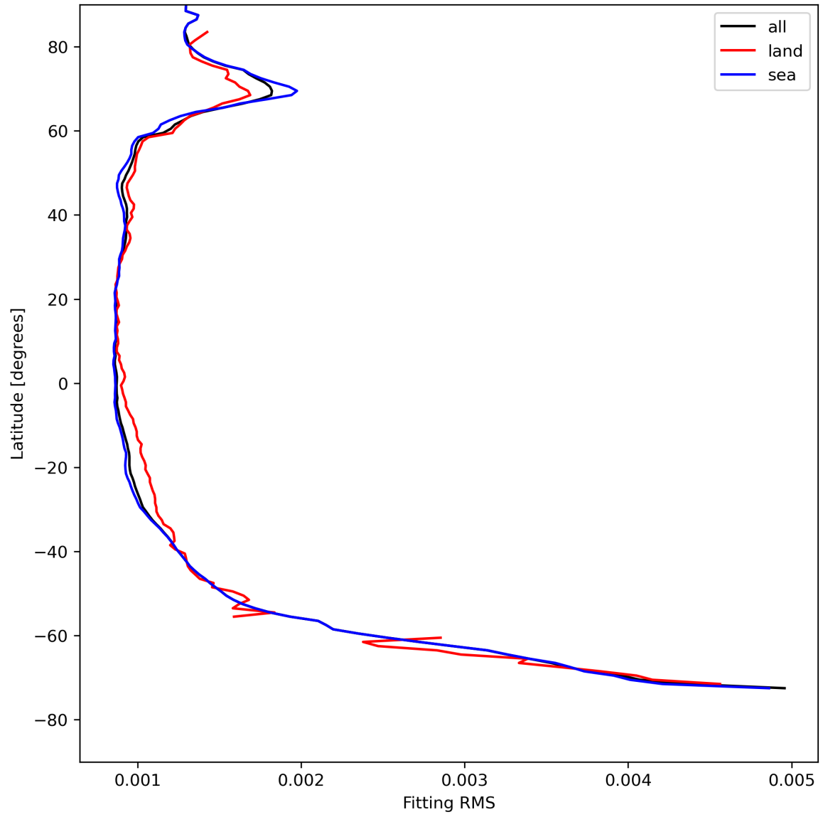
Figure 16: Zonal average of “Fitting RMS” for 2023-08-04 to 2023-08-06.
