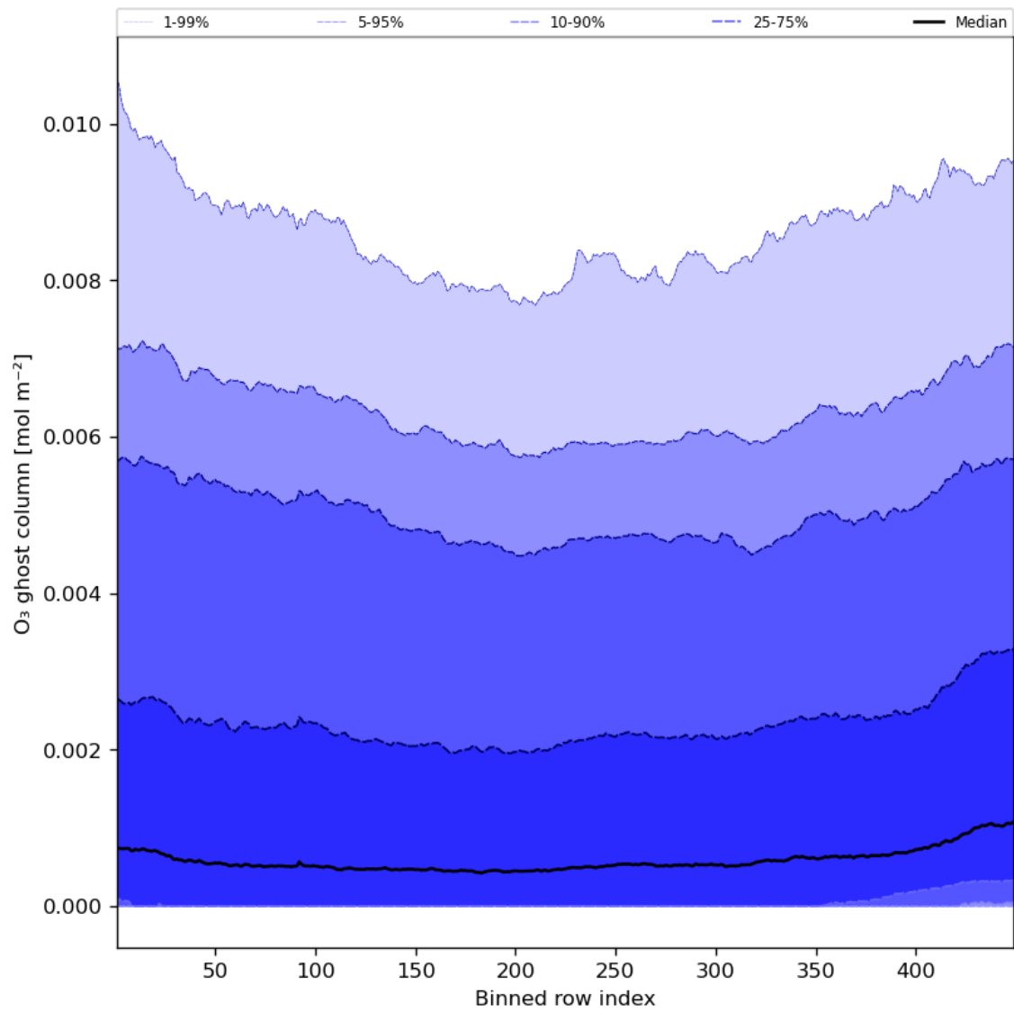
Figure 32: Along track statistics of “O 3 ghost column” for 2023-08-04 to 2023-08-06
