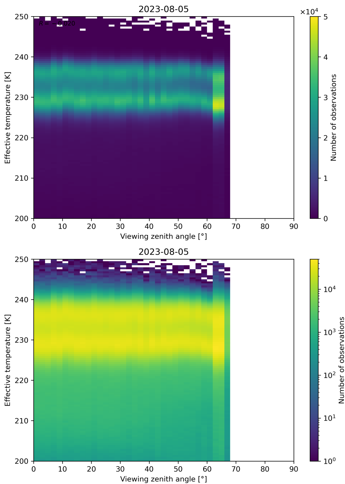
Figure 50: Scatter density plot of “Viewing zenith angle” against “Effective temperature” for 2023-08-04 to 2023-08-06.
