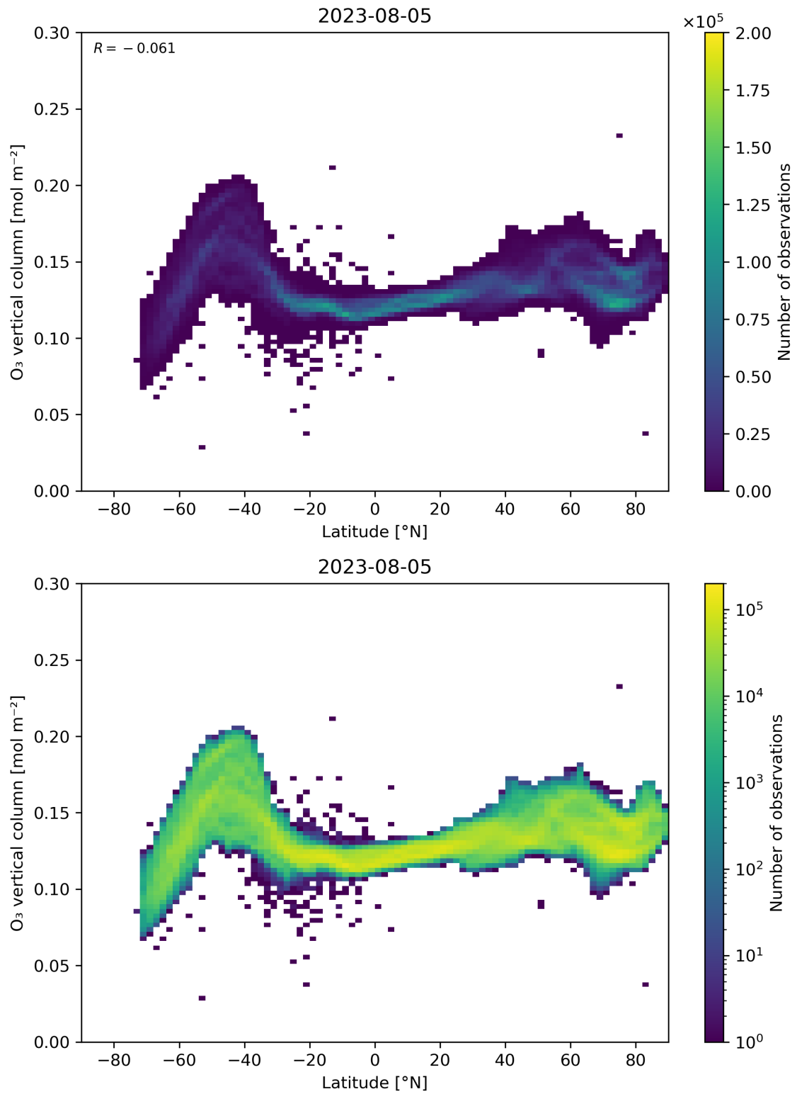
Figure 36: Scatter density plot of “Latitude” against “O 3 vertical column” for 2023-08-04 to 2023-08-06.
