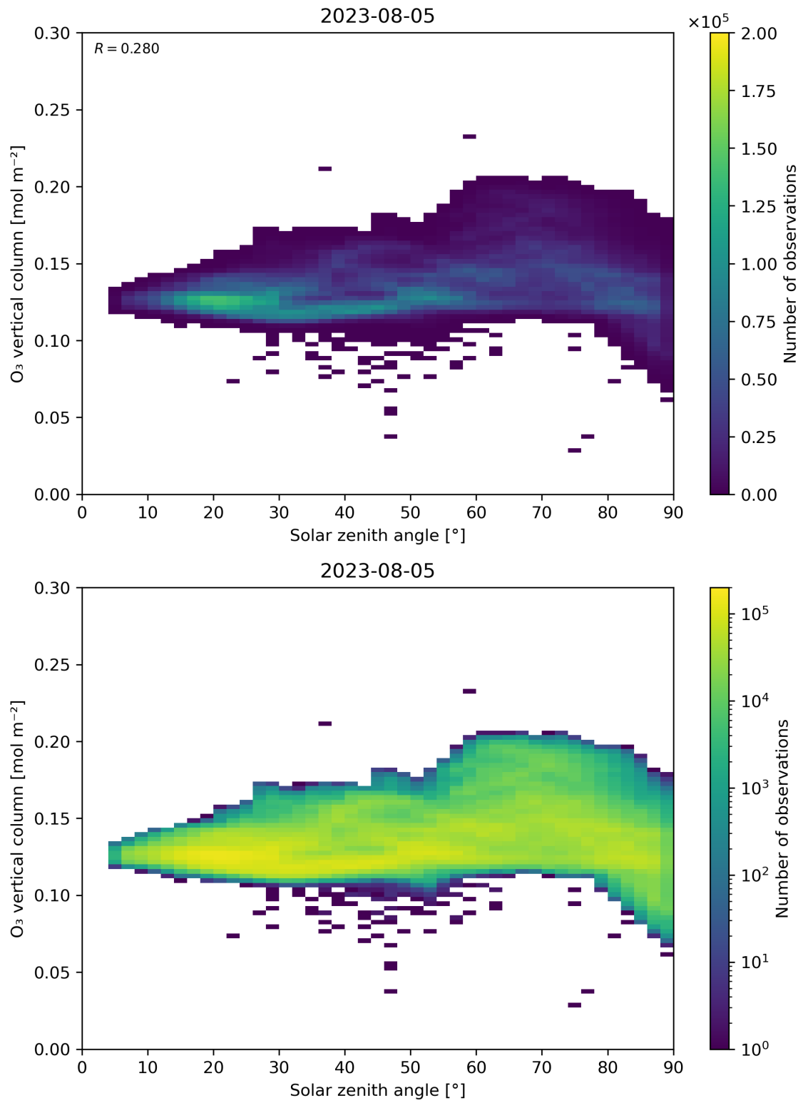
Figure 47: Scatter density plot of “Solar zenith angle” against “O 3 vertical column” for 2023-08-04 to 2023-08-06.
