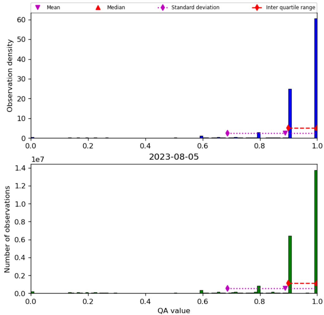
Figure 20: Histogram of “QA value” for 2023-08-04 to 2023-08-06
