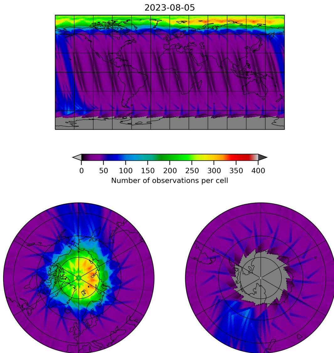
Figure 12: Map of the number of observations for 2023-08-04 to 2023-08-06
