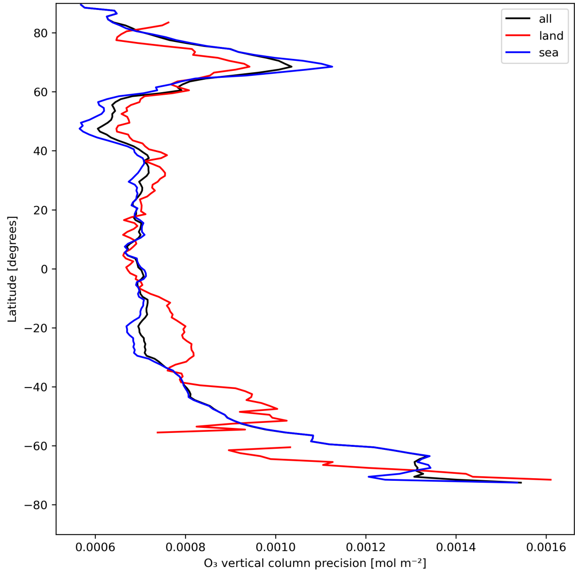
Figure 15: Zonal average of “O 3 vertical column precision” for 2023-08-04 to 2023-08-06.
