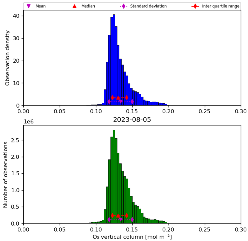
Figure 21: Histogram of “O 3 vertical column” for 2023-08-04 to 2023-08-06
