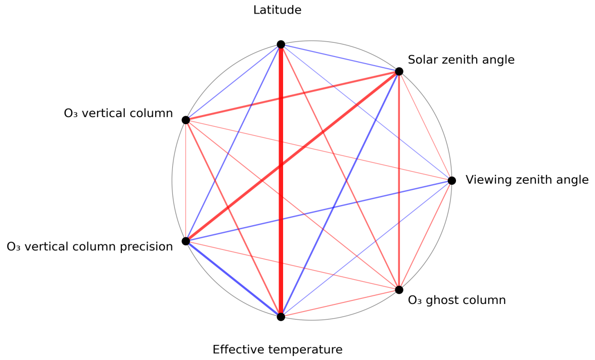
Figure 1: Map of correlation graph for 2023-08-04 to 2023-08-06.
