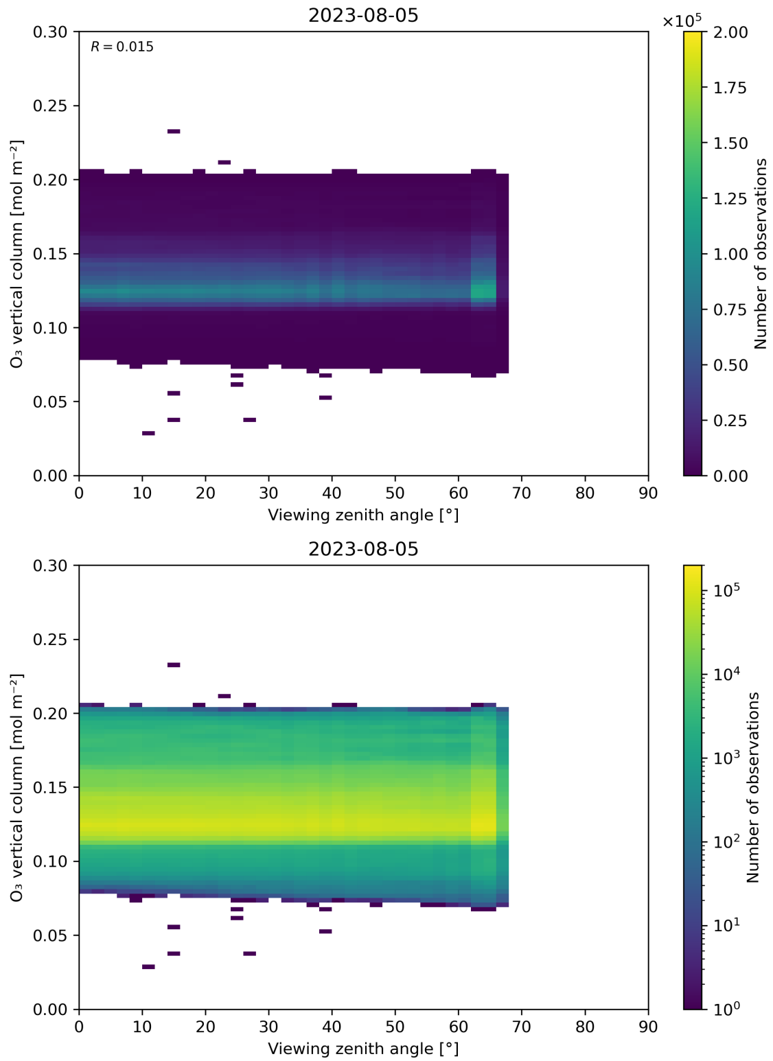
Figure 52: Scatter density plot of “Viewing zenith angle” against “O 3 vertical column” for 2023-08-04 to 2023-08-06.
