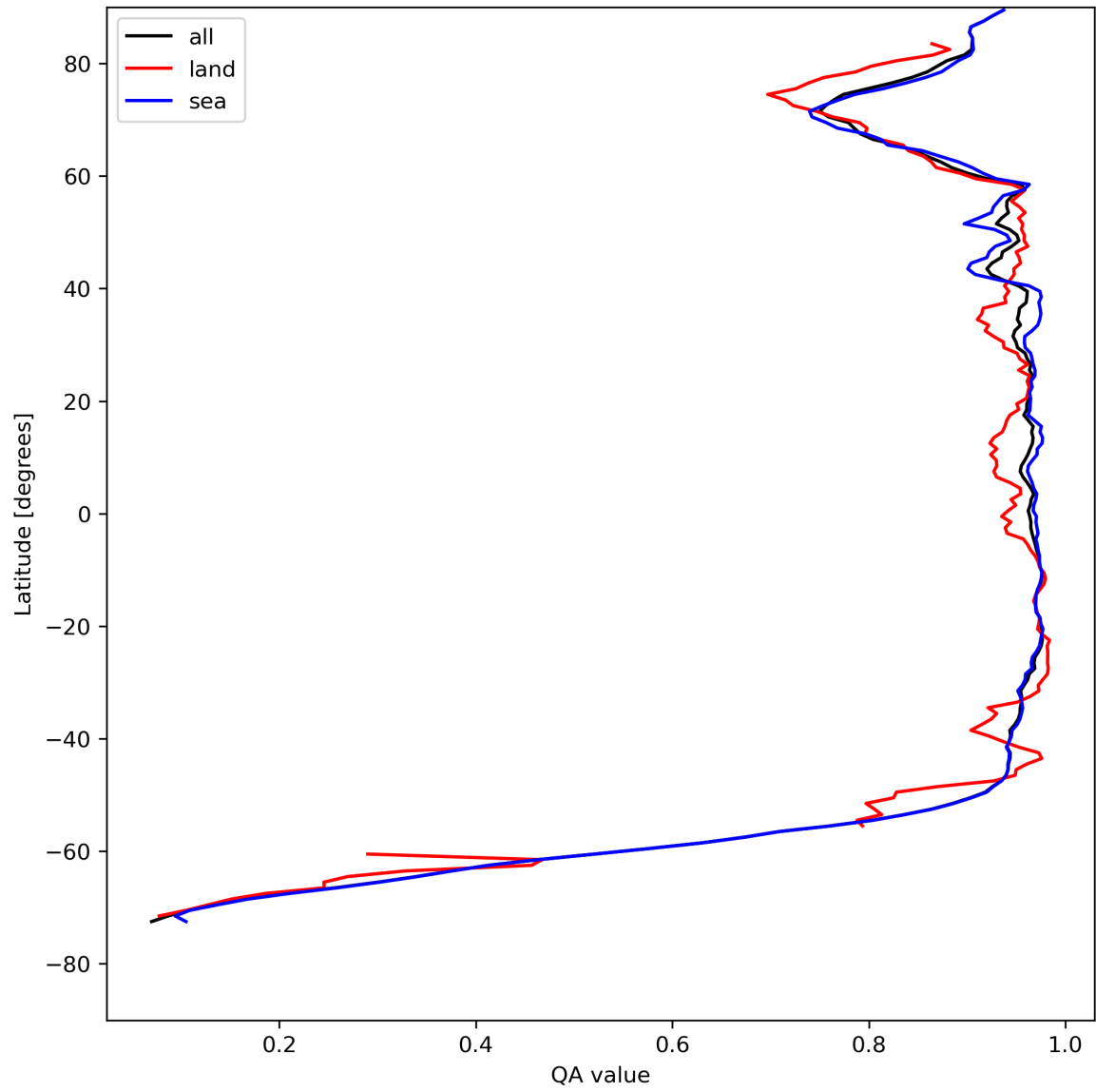
Figure 13: Zonal average of “QA value” for 2023-08-04 to 2023-08-06.
