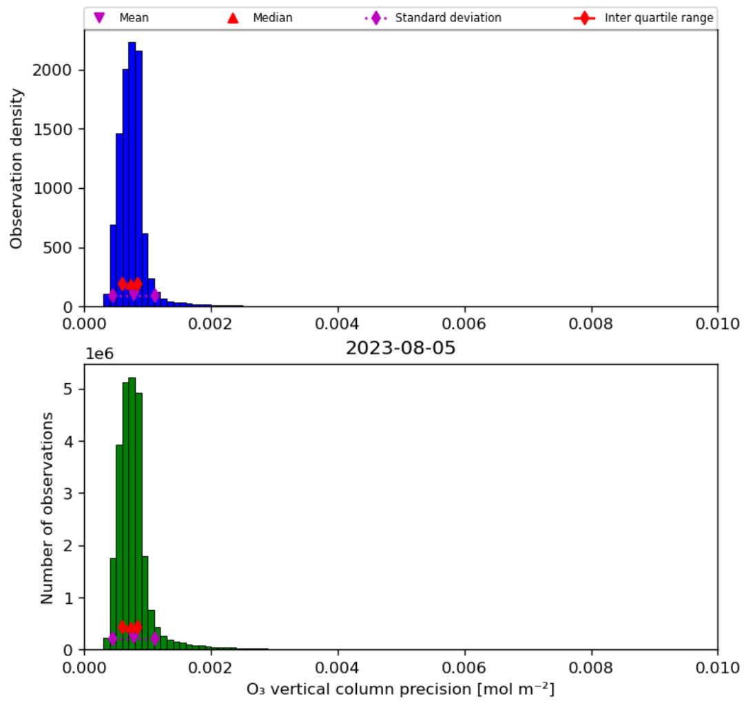
Figure 22: Histogram of “O 3 vertical column precision” for 2023-08-04 to 2023-08-06
