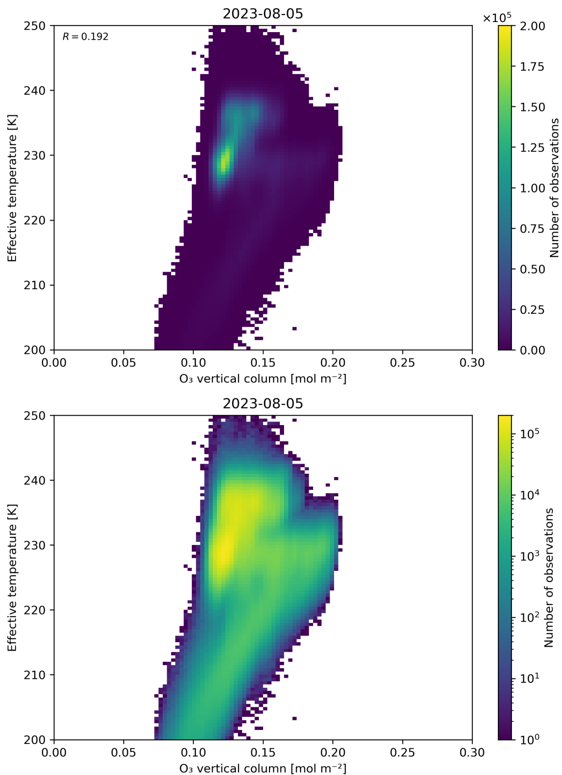
Figure 39: Scatter density plot of “O 3 vertical column” against “Effective temperature” for 2023-08-04 to 2023-08-06.
