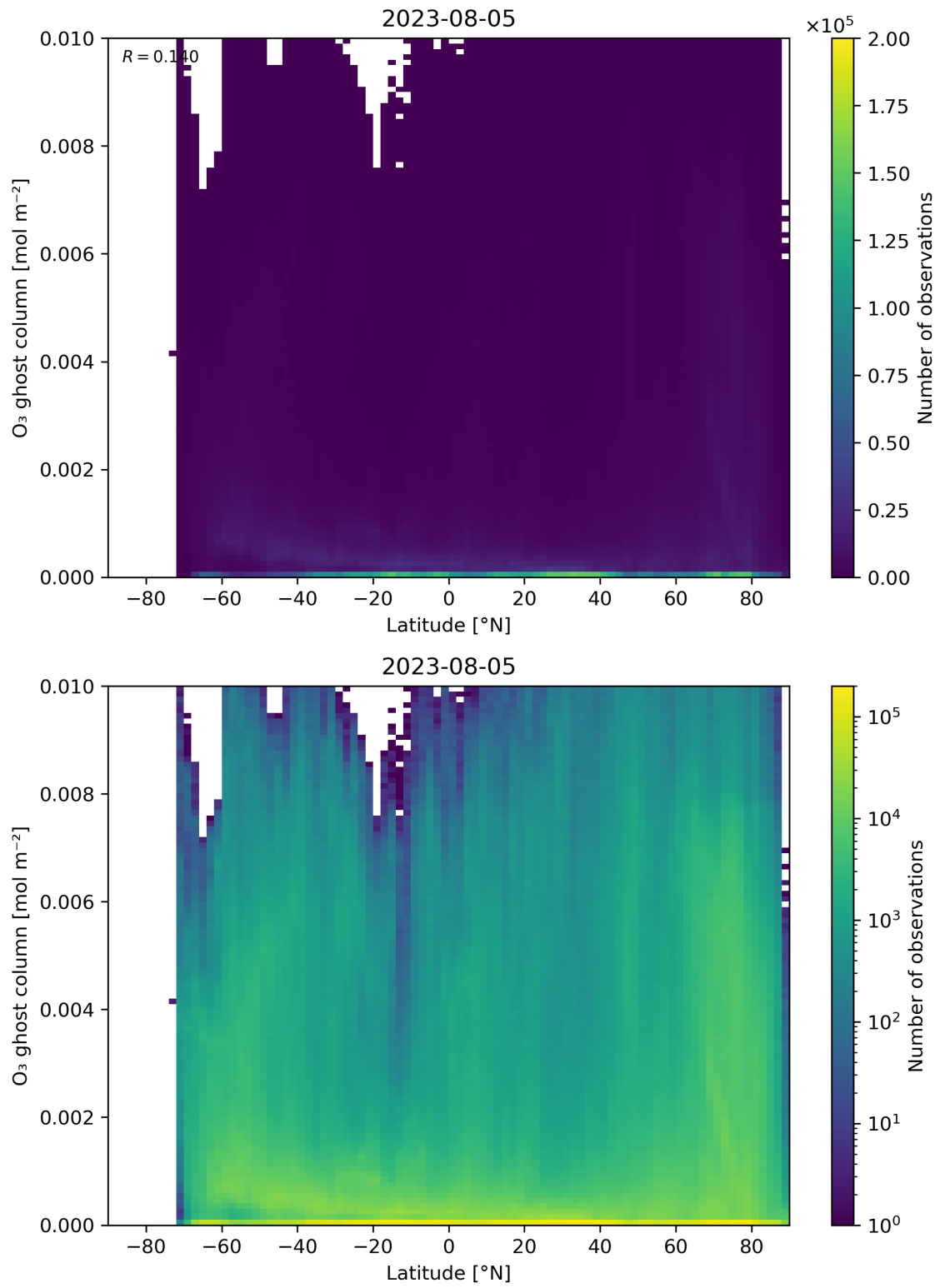
Figure 35: Scatter density plot of “Latitude” against “O 3 ghost column” for 2023-08-04 to 2023-08-06.
