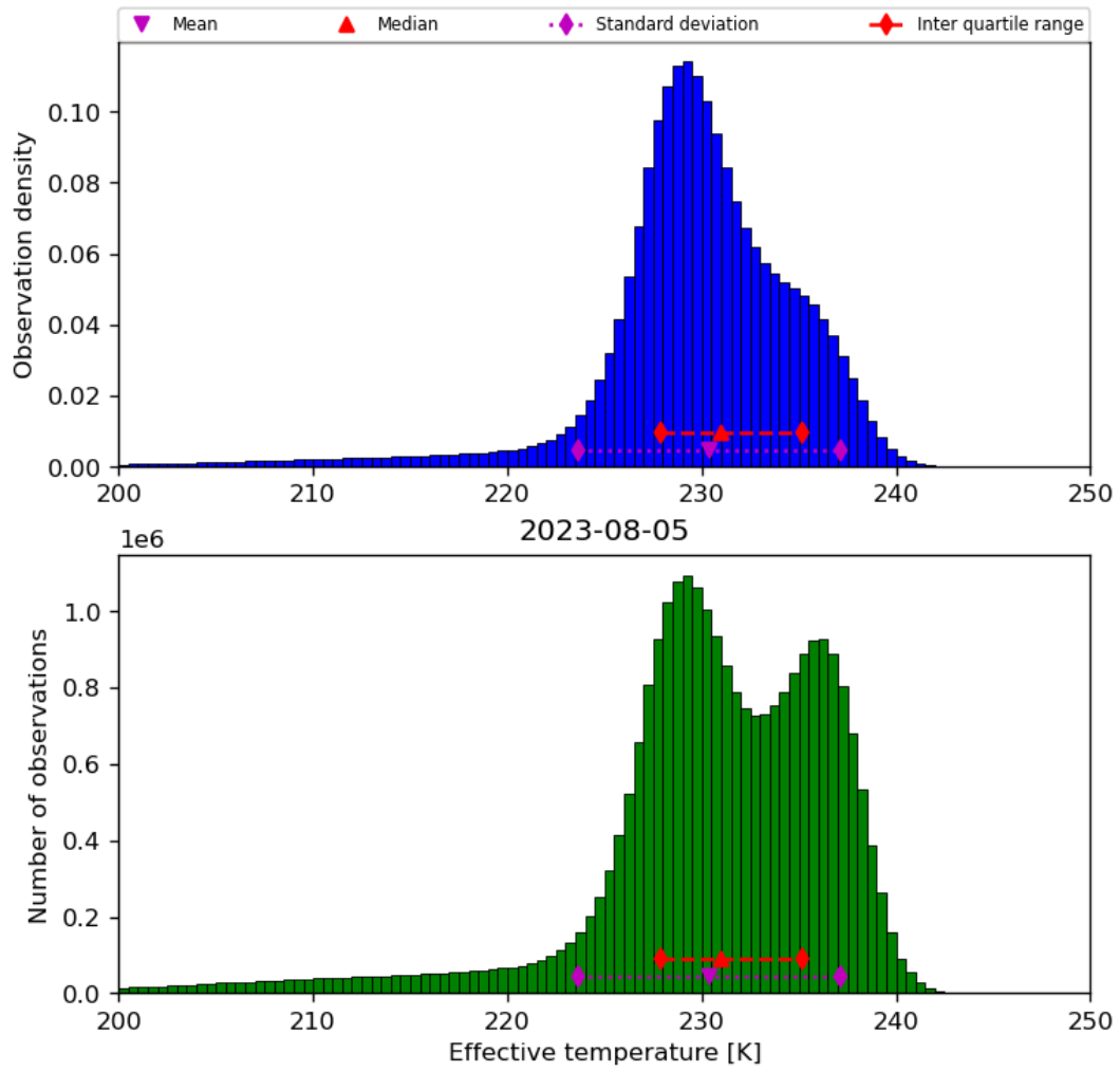
Figure 24: Histogram of “Effective temperature” for 2023-08-04 to 2023-08-06
