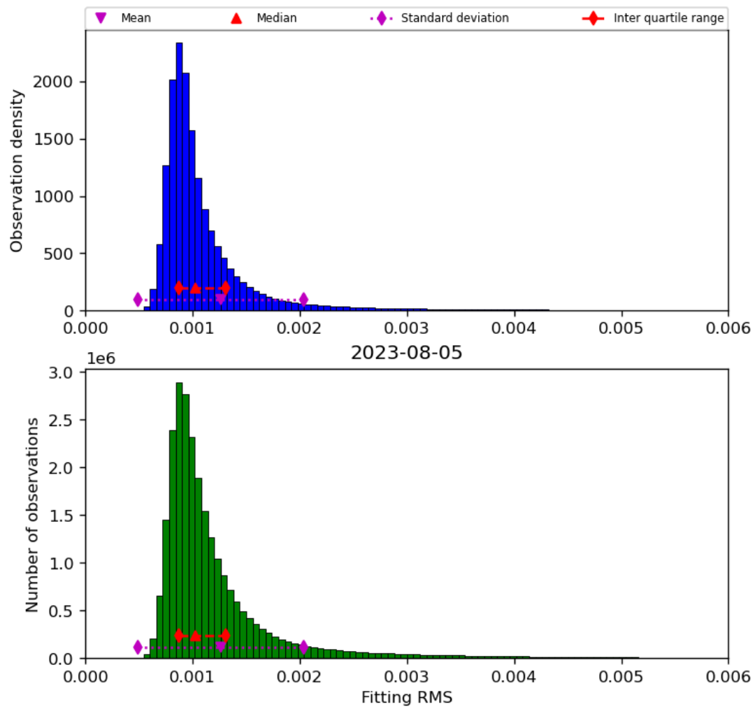
Figure 23: Histogram of “Fitting RMS” for 2023-08-04 to 2023-08-06
