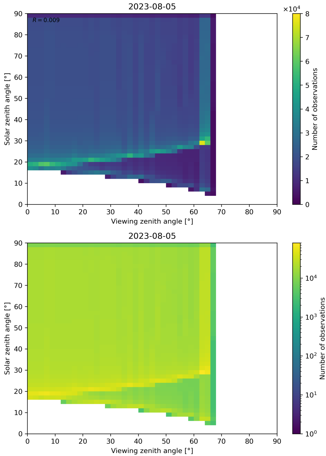
Figure 54: Scatter density plot of “Viewing zenith angle” against “Solar zenith angle” for 2023-08-04 to 2023-08-06.
