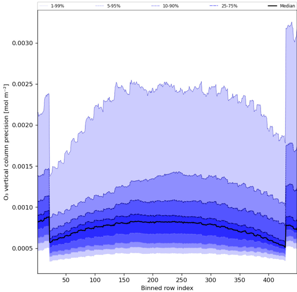
Figure 29: Along track statistics of “O 3 vertical column precision” for 2023-08-04 to 2023-08-06
