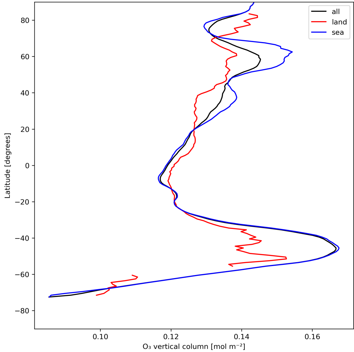
Figure 14: Zonal average of “O 3 vertical column” for 2023-08-04 to 2023-08-06.
