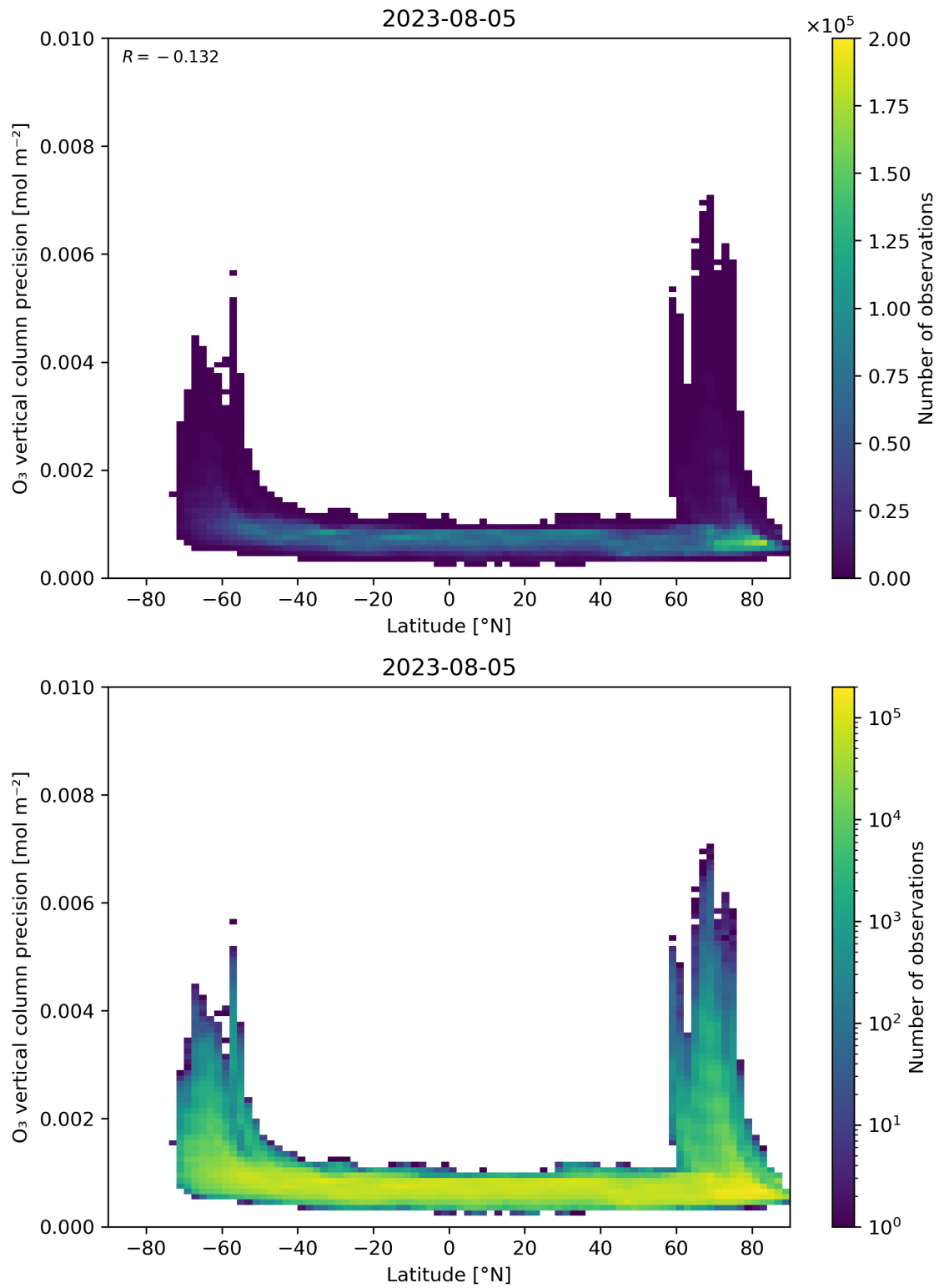
Figure 37: Scatter density plot of “Latitude” against “O 3 vertical column precision” for 2023-08-04 to 2023-08-06.
