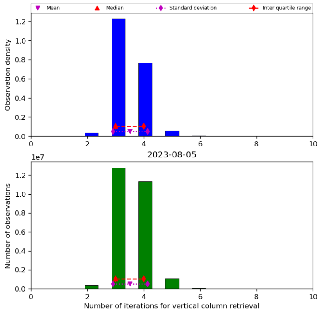
Figure 26: Histogram of “Number of iterations for vertical column retrieval” for 2023-08-04 to 2023-08-06
