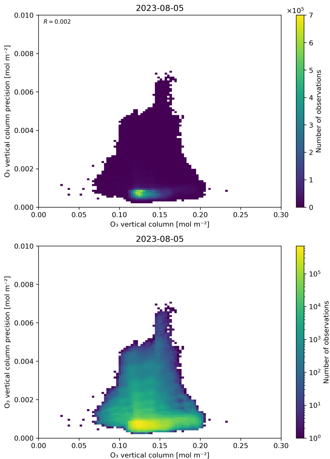
Figure 41: Scatter density plot of “O 3 vertical column” against “O 3 vertical column precision” for 2023-08-04 to 2023-08-06.
