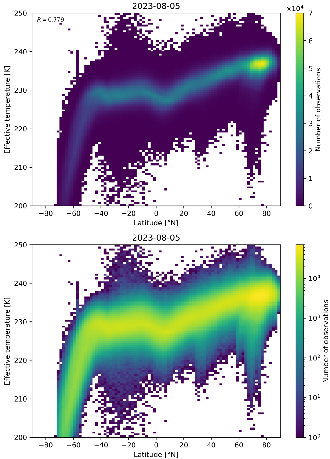
Figure 34: Scatter density plot of “Latitude” against “Effective temperature” for 2023-08-04 to 2023-08-06.
