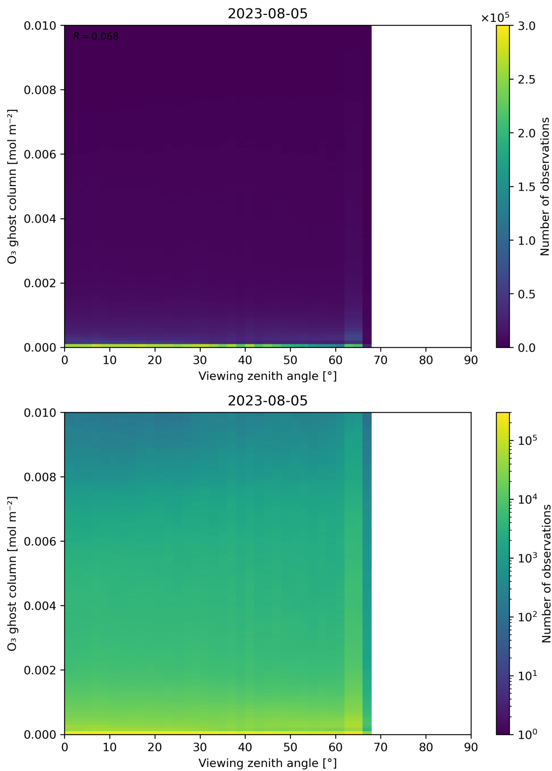
Figure 51: Scatter density plot of “Viewing zenith angle” against “O 3 ghost column” for 2023-08-04 to 2023-08-06.
