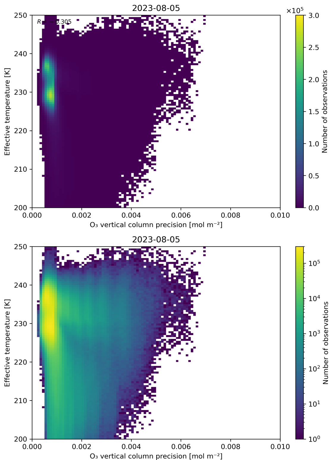
Figure 42: Scatter density plot of “O 3 vertical column precision” against “Effective temperature” for 2023-08-04 to 2023-08-06.
