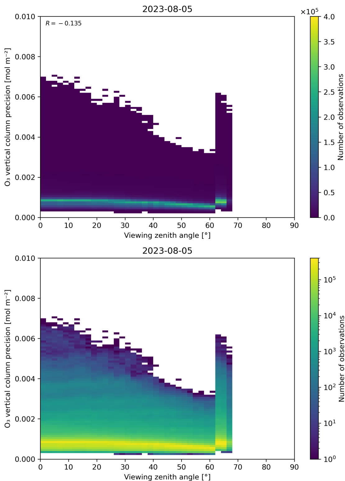
Figure 53: Scatter density plot of “Viewing zenith angle” against “O 3 vertical column precision” for 2023-08-04 to 2023-08-06.
