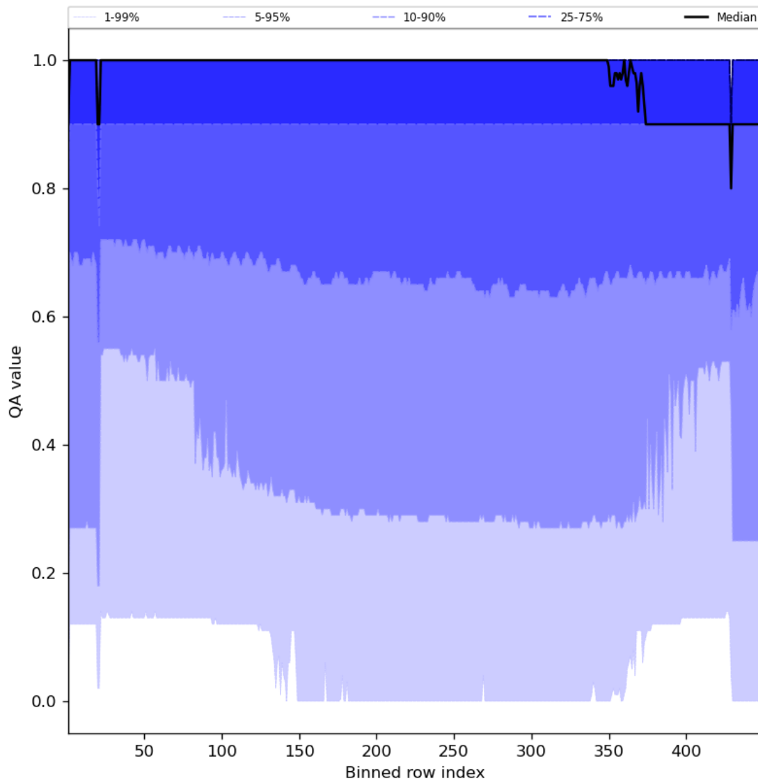
Figure 27: Along track statistics of “QA value” for 2023-08-04 to 2023-08-06
