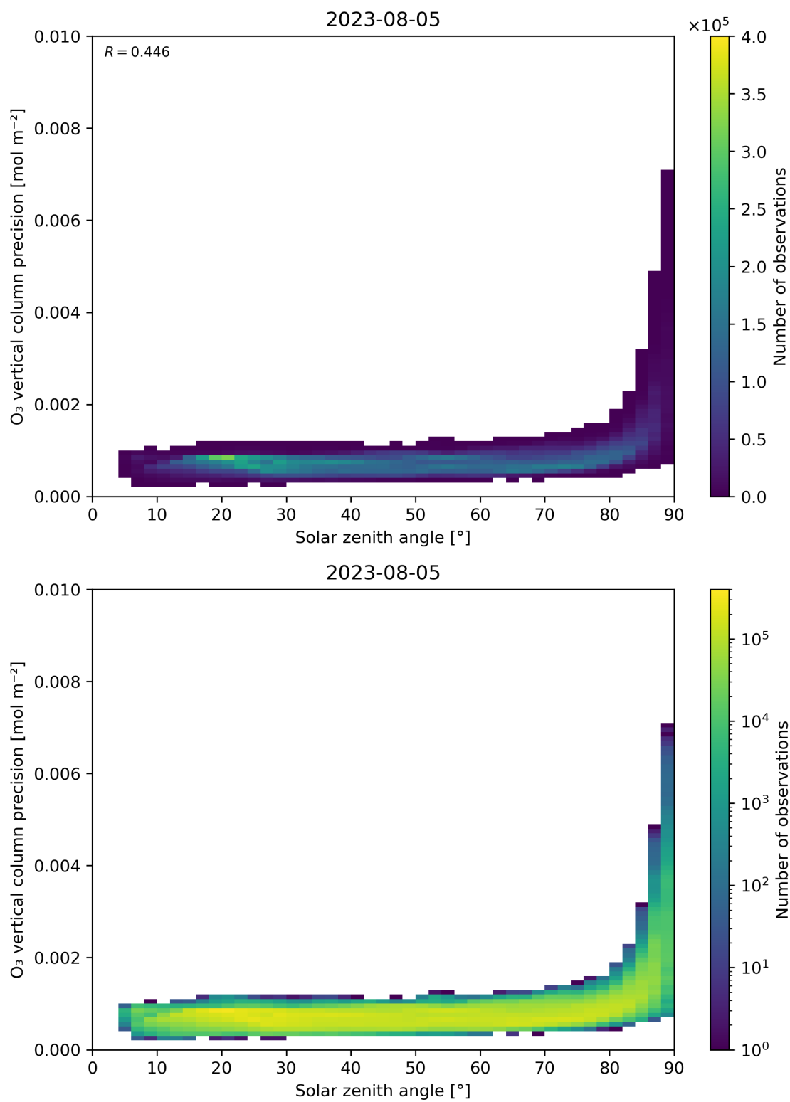
Figure 48: Scatter density plot of “Solar zenith angle” against “O 3 vertical column precision” for 2023-08-04 to 2023-08-06.
