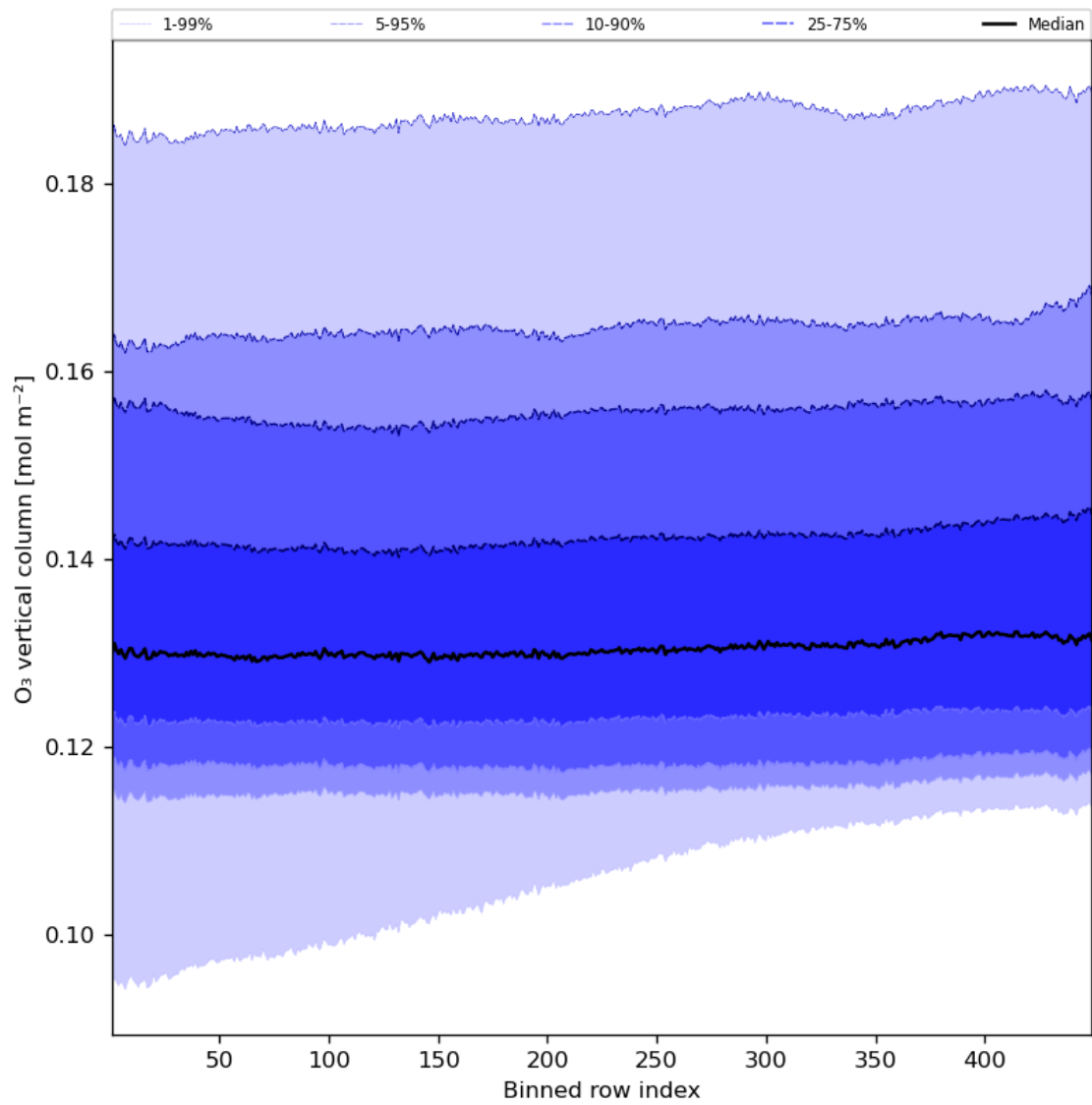
Figure 28: Along track statistics of “O 3 vertical column” for 2023-08-04 to 2023-08-06
