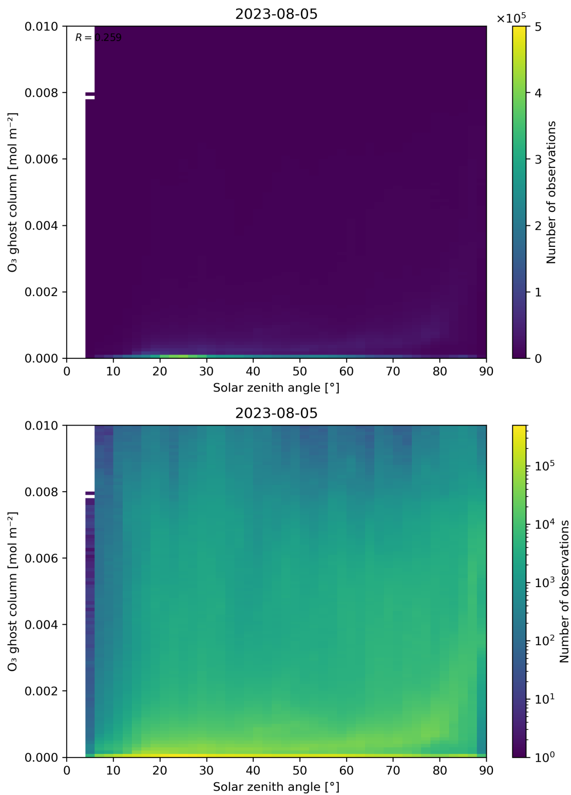
Figure 46: Scatter density plot of “Solar zenith angle” against “O 3 ghost column” for 2023-08-04 to 2023-08-06.
