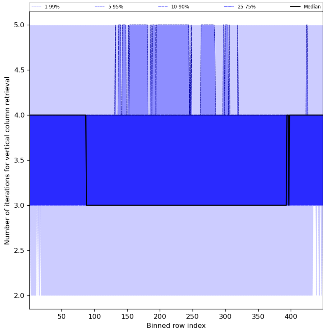
Figure 33: Along track statistics of “Number of iterations for vertical column retrieval” for 2023-08-04 to 2023-08-06
