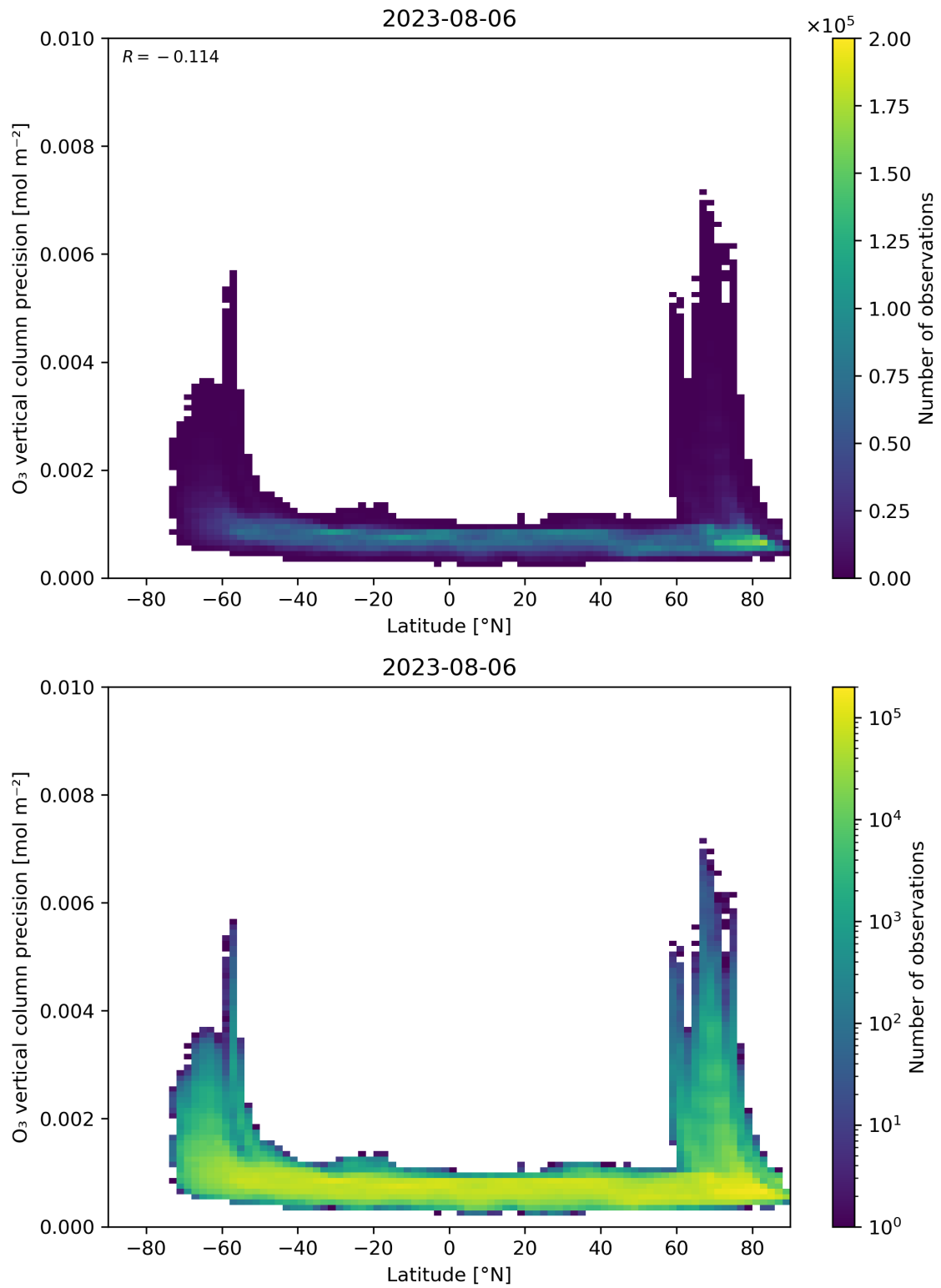
Figure 37: Scatter density plot of “Latitude” against “O 3 vertical column precision” for 2023-08-05 to 2023-08-07.
