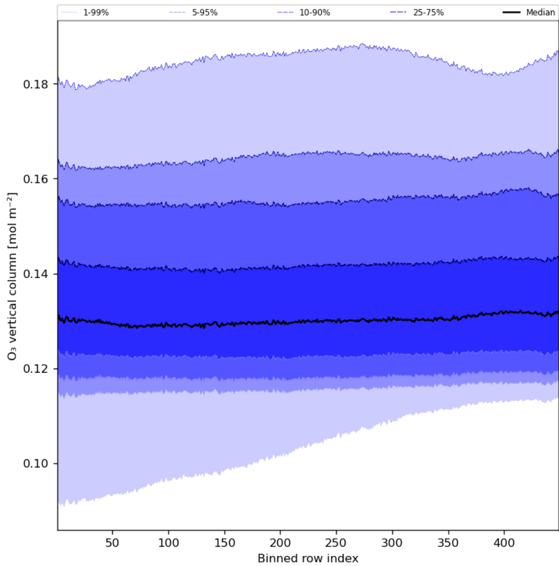
Figure 28: Along track statistics of “O 3 vertical column” for 2023-08-05 to 2023-08-07
