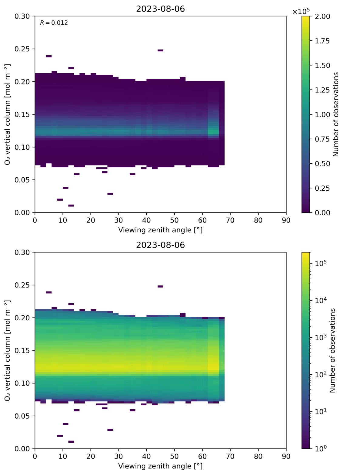
Figure 52: Scatter density plot of “Viewing zenith angle” against “O 3 vertical column” for 2023-08-05 to 2023-08-07.
