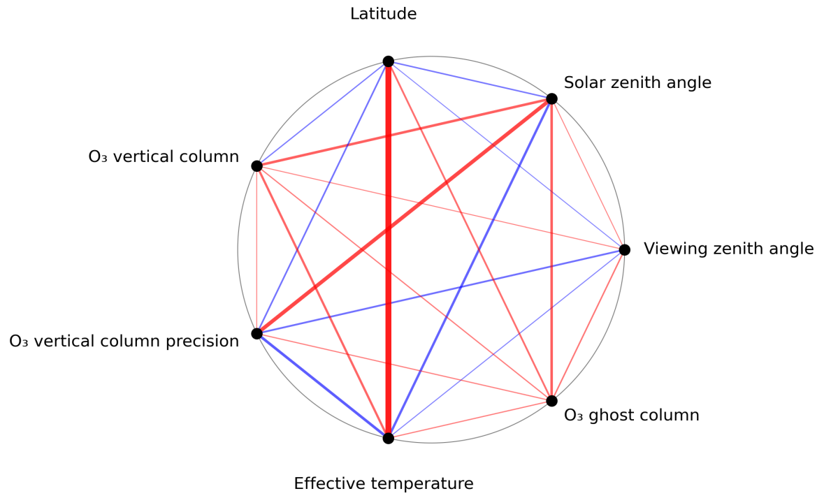
Figure 1: Map of correlation graph for 2023-08-05 to 2023-08-07.
