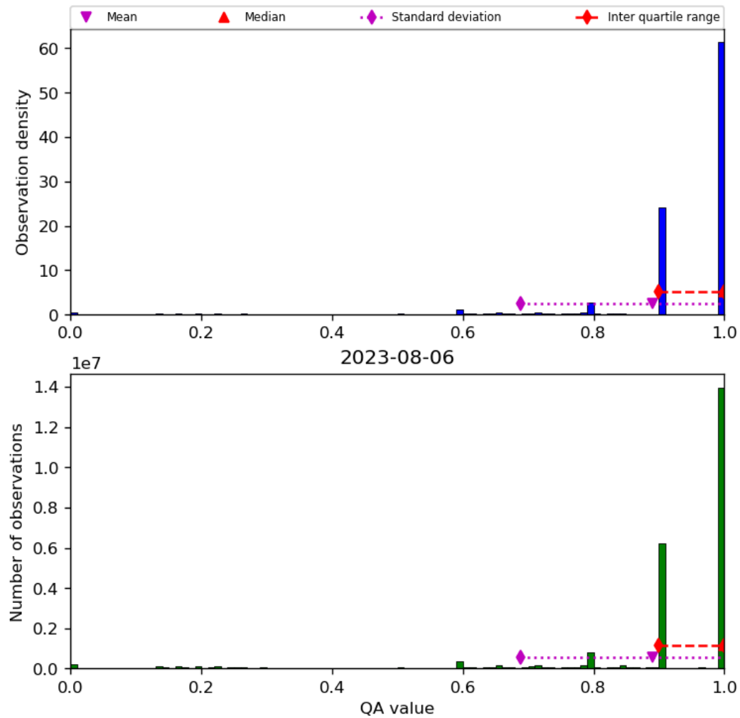
Figure 20: Histogram of “QA value” for 2023-08-05 to 2023-08-07
