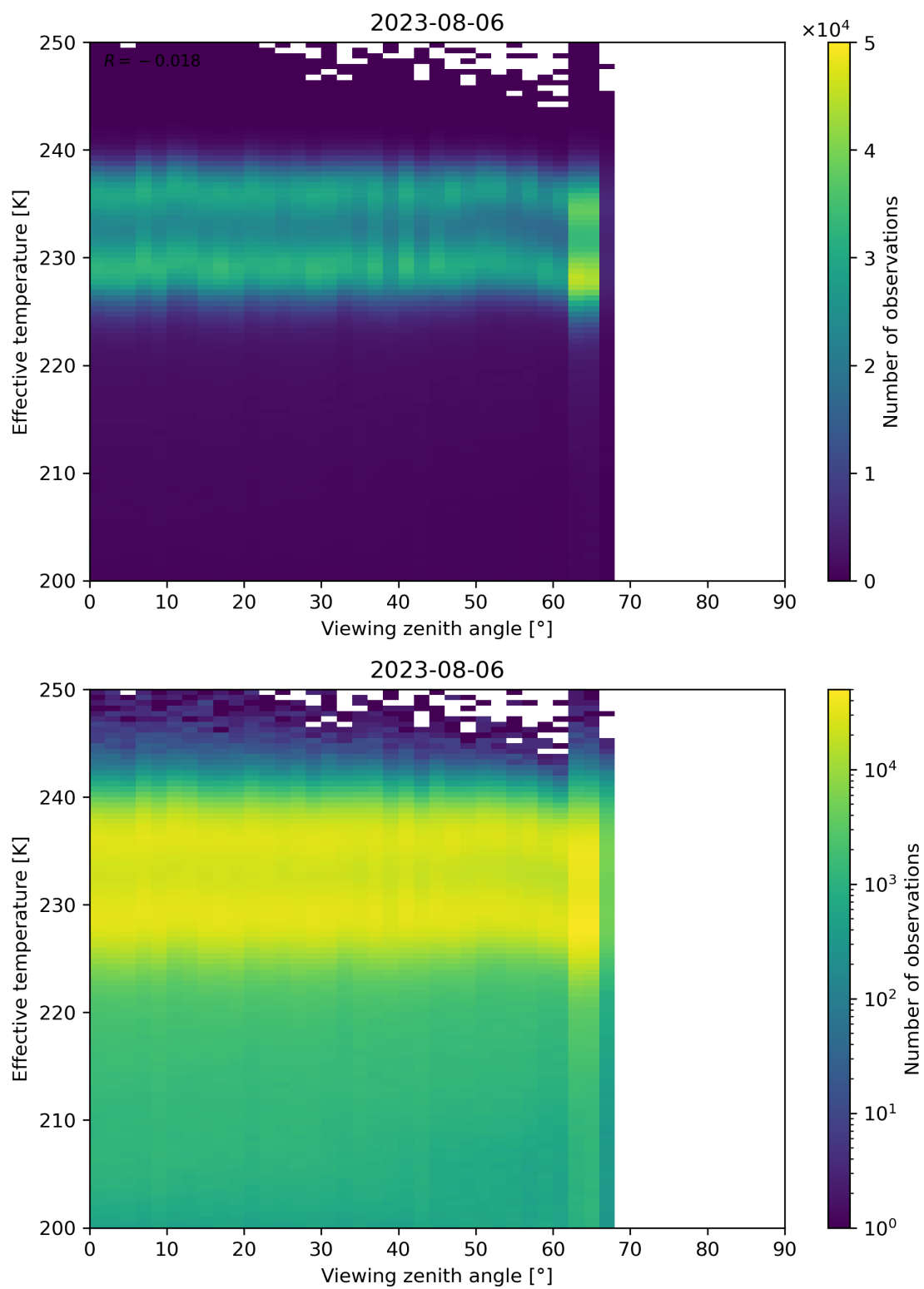
Figure 50: Scatter density plot of “Viewing zenith angle” against “Effective temperature” for 2023-08-05 to 2023-08-07.
