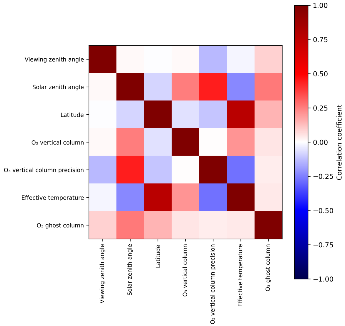
Figure 2: Map of correlation matrix for 2023-08-05 to 2023-08-07.
