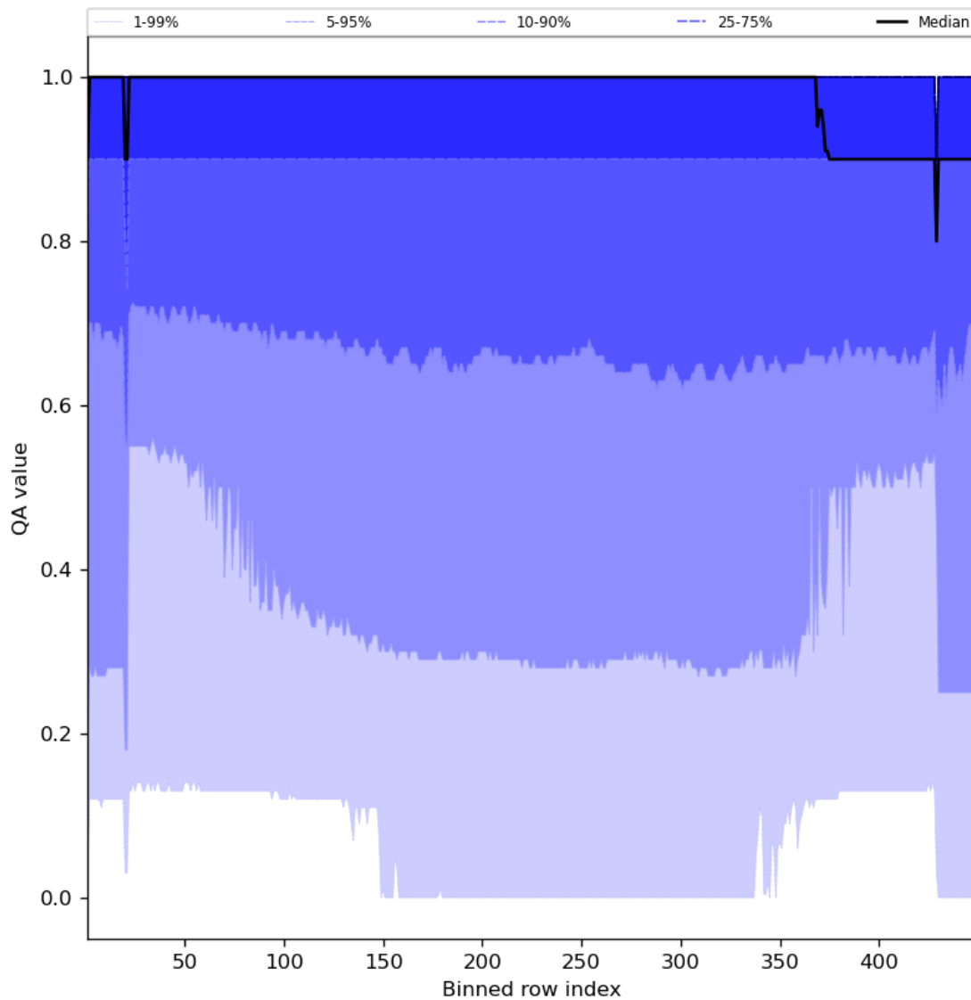
Figure 27: Along track statistics of “QA value” for 2023-08-05 to 2023-08-07
