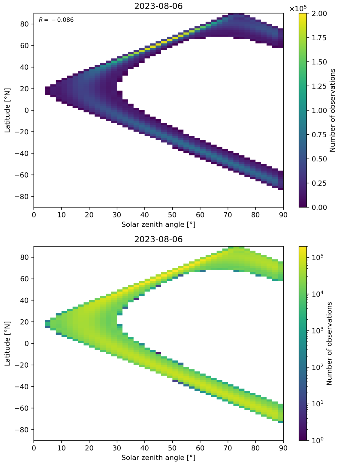
Figure 44: Scatter density plot of “Solar zenith angle” against “Latitude” for 2023-08-05 to 2023-08-07.
