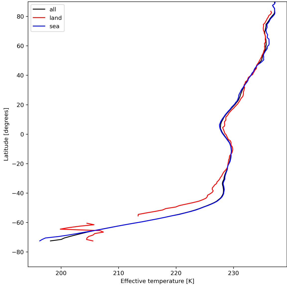
Figure 17: Zonal average of “Effective temperature” for 2023-08-05 to 2023-08-07.
