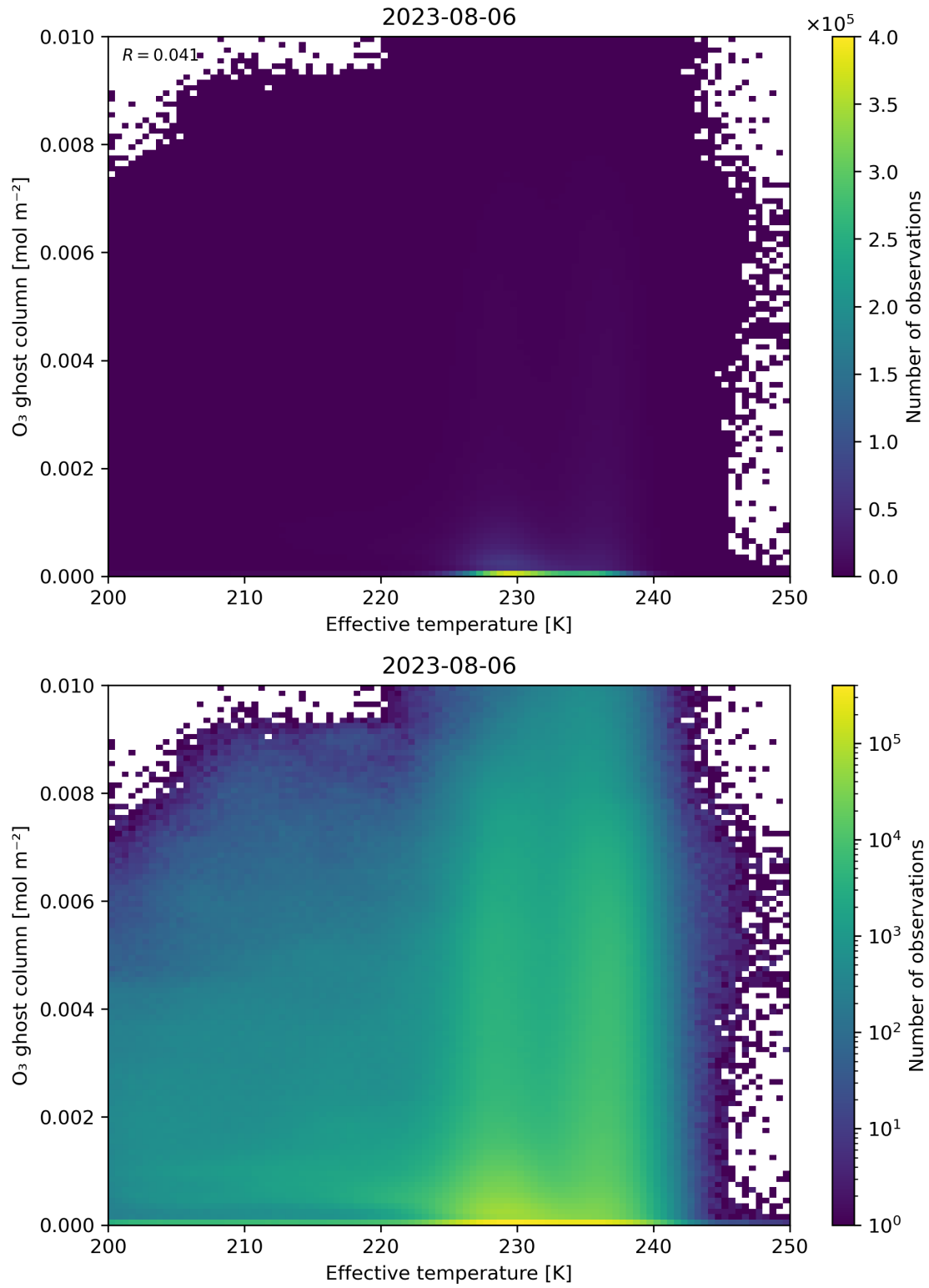
Figure 38: Scatter density plot of “Effective temperature” against “O 3 ghost column” for 2023-08-05 to 2023-08-07.
