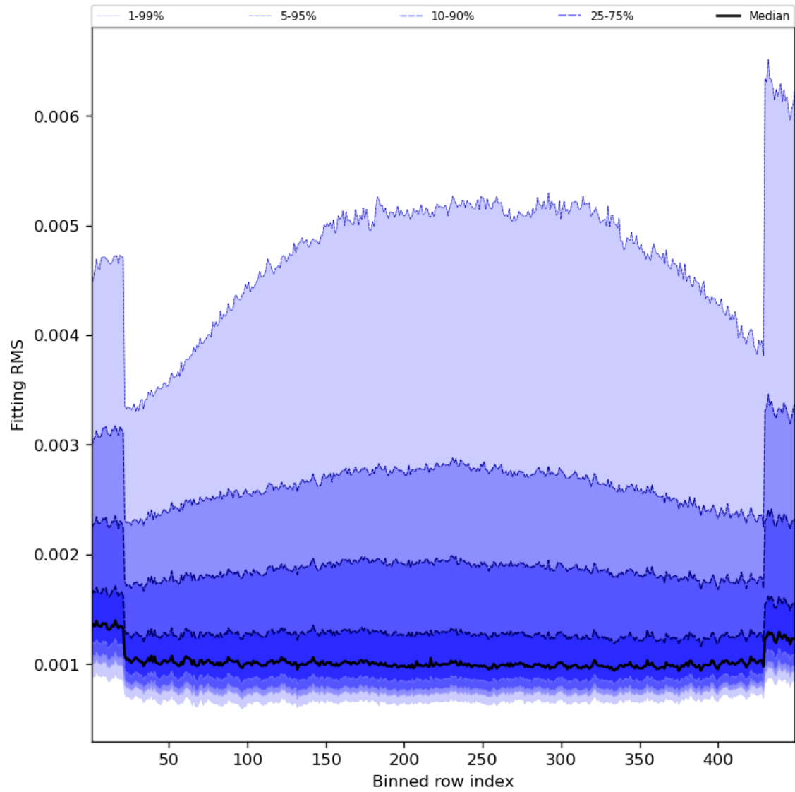
Figure 30: Along track statistics of “Fitting RMS” for 2023-08-05 to 2023-08-07
