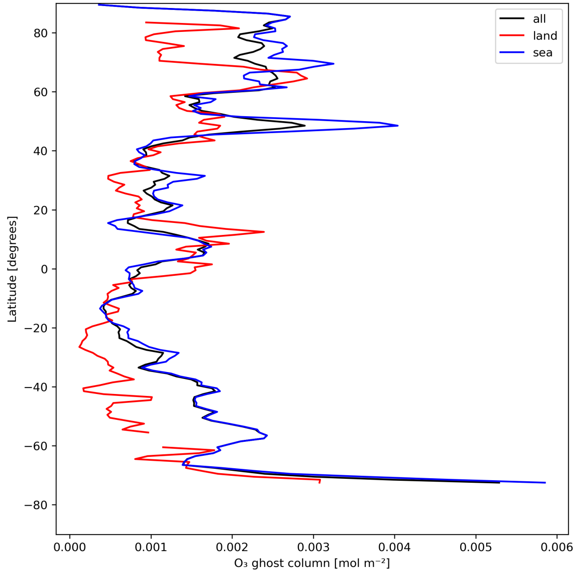
Figure 18: Zonal average of "O 3 ghost column" for 2023-08-05 to 2023-08-07.
