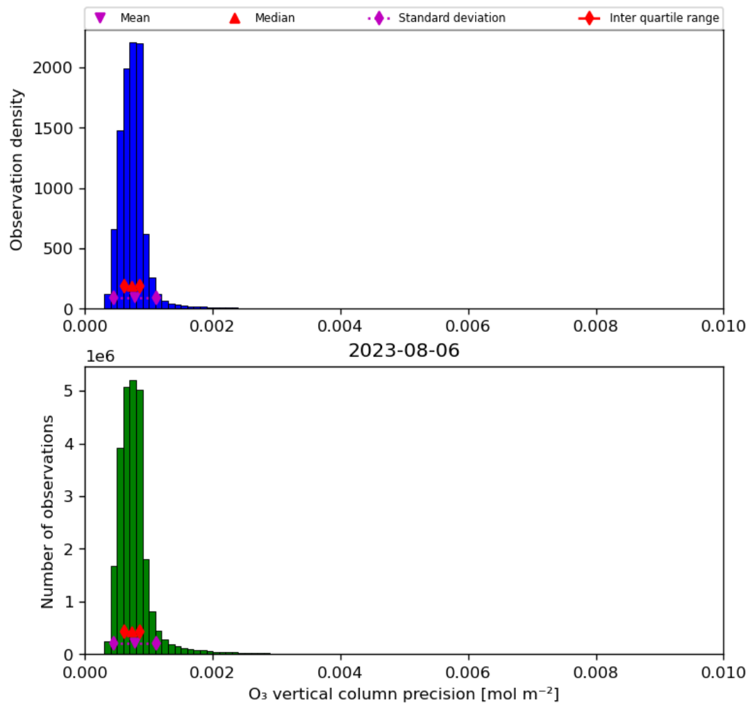
Figure 22: Histogram of “O 3 vertical column precision” for 2023-08-05 to 2023-08-07
