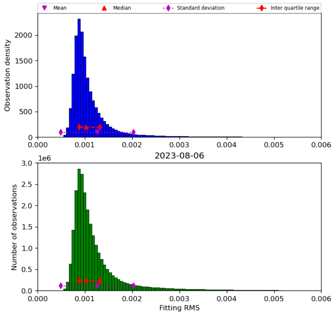
Figure 23: Histogram of “Fitting RMS” for 2023-08-05 to 2023-08-07
