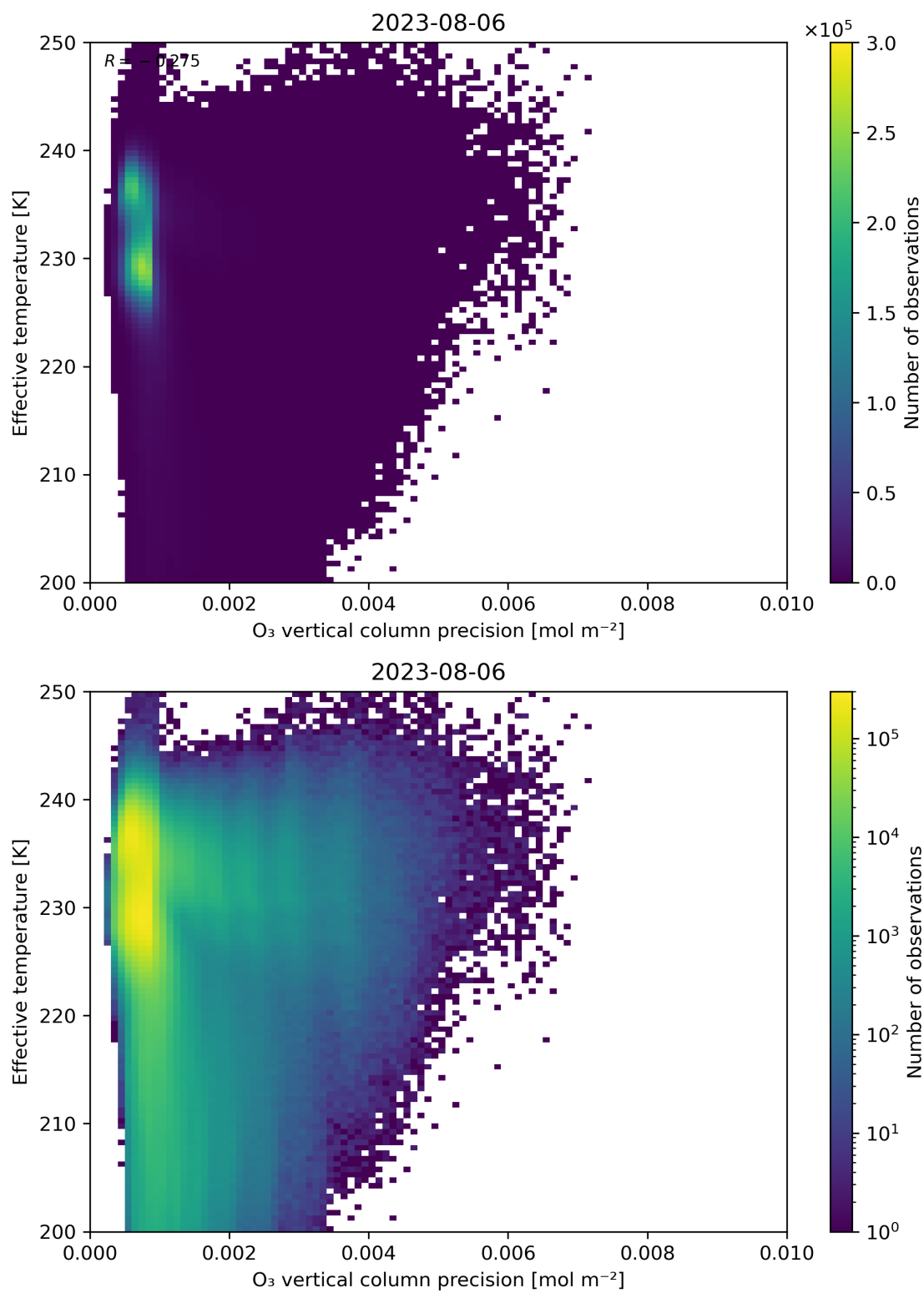
Figure 42: Scatter density plot of “O 3 vertical column precision” against “Effective temperature” for 2023-08-05 to 2023-08-07.
