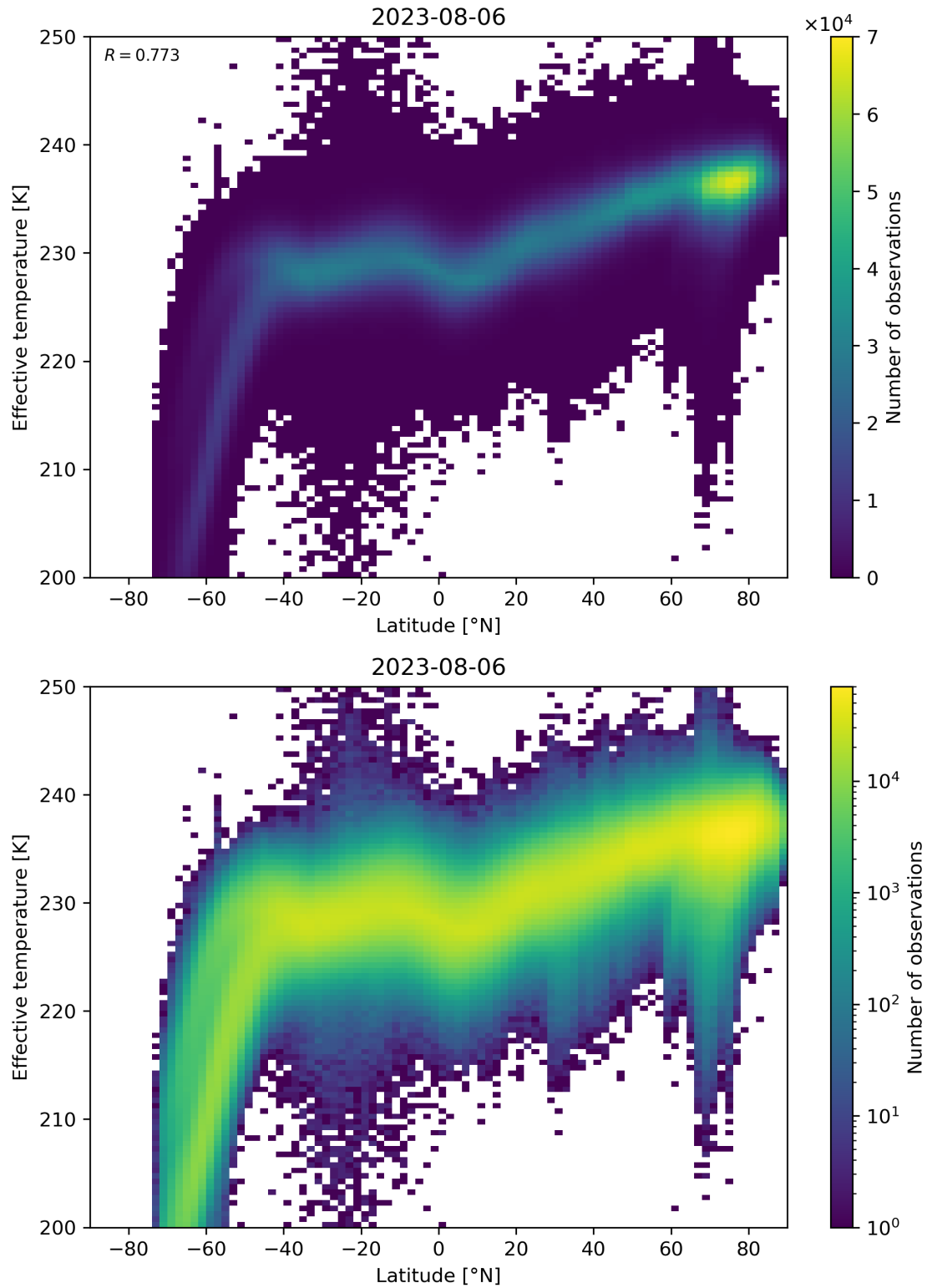
Figure 34: Scatter density plot of “Latitude” against “Effective temperature” for 2023-08-05 to 2023-08-07.
