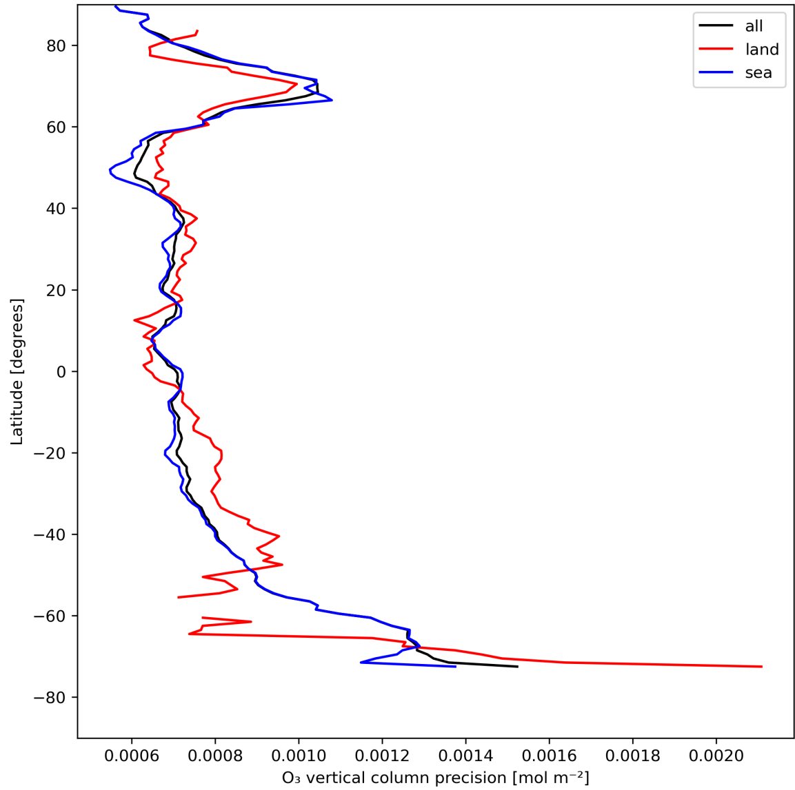
Figure 15: Zonal average of “O 3 vertical column precision” for 2023-08-05 to 2023-08-07.
