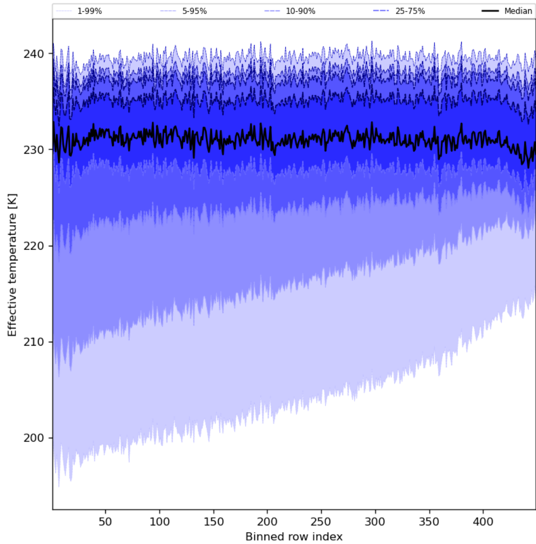
Figure 31: Along track statistics of “Effective temperature” for 2023-08-05 to 2023-08-07
