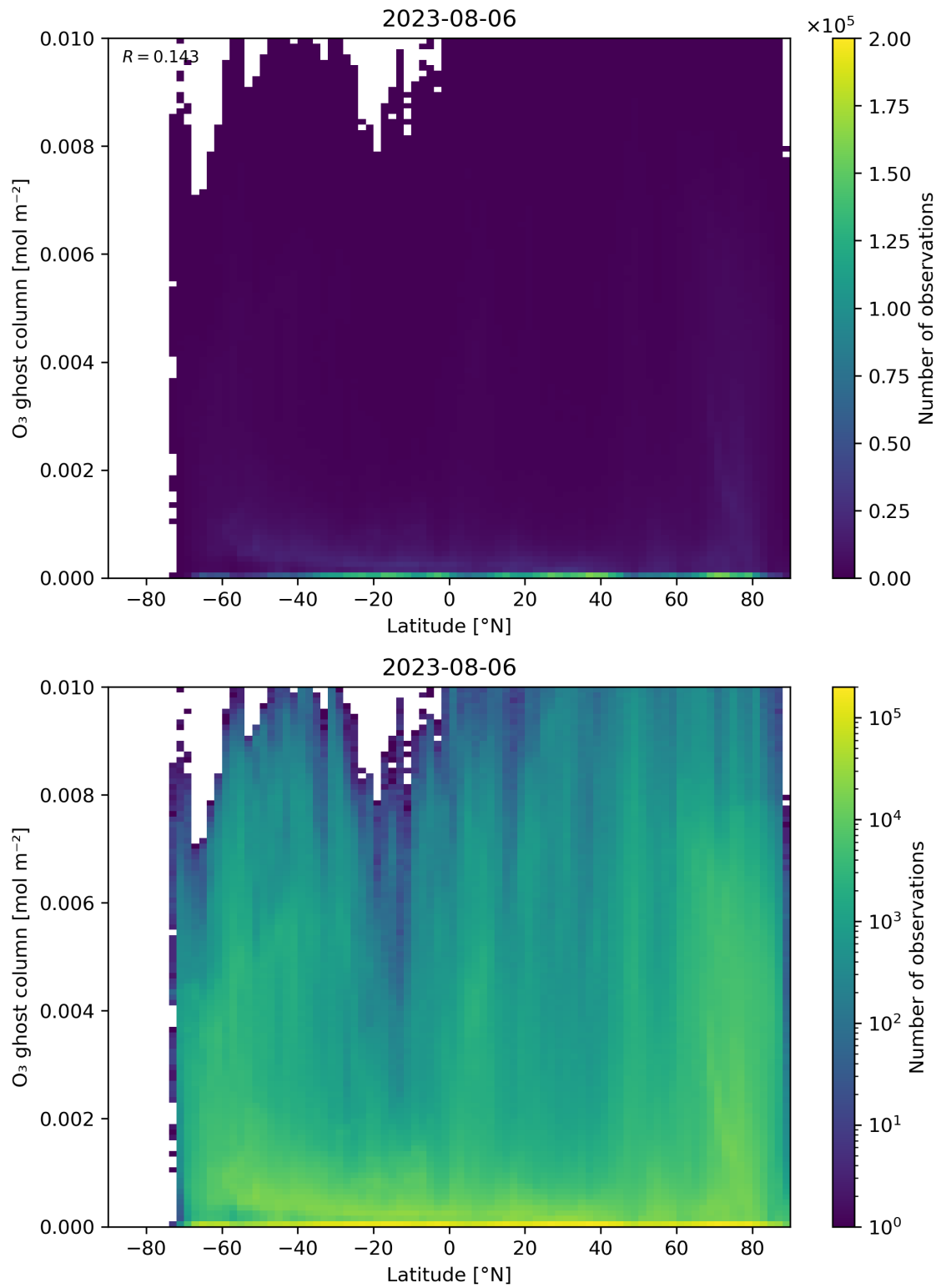
Figure 35: Scatter density plot of “Latitude” against “O 3 ghost column” for 2023-08-05 to 2023-08-07.
