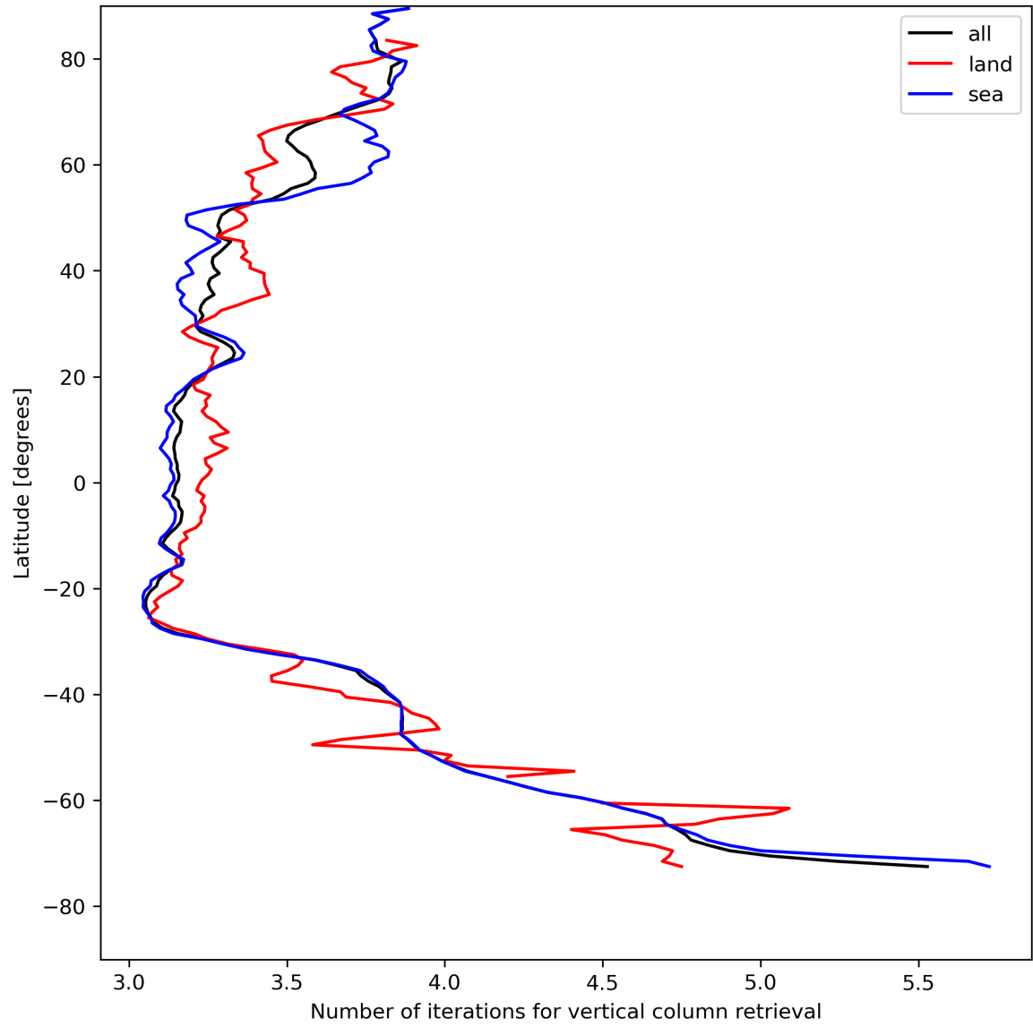
Figure 19: Zonal average of “Number of iterations for vertical column retrieval” for 2023-08-05 to 2023-08-07.
