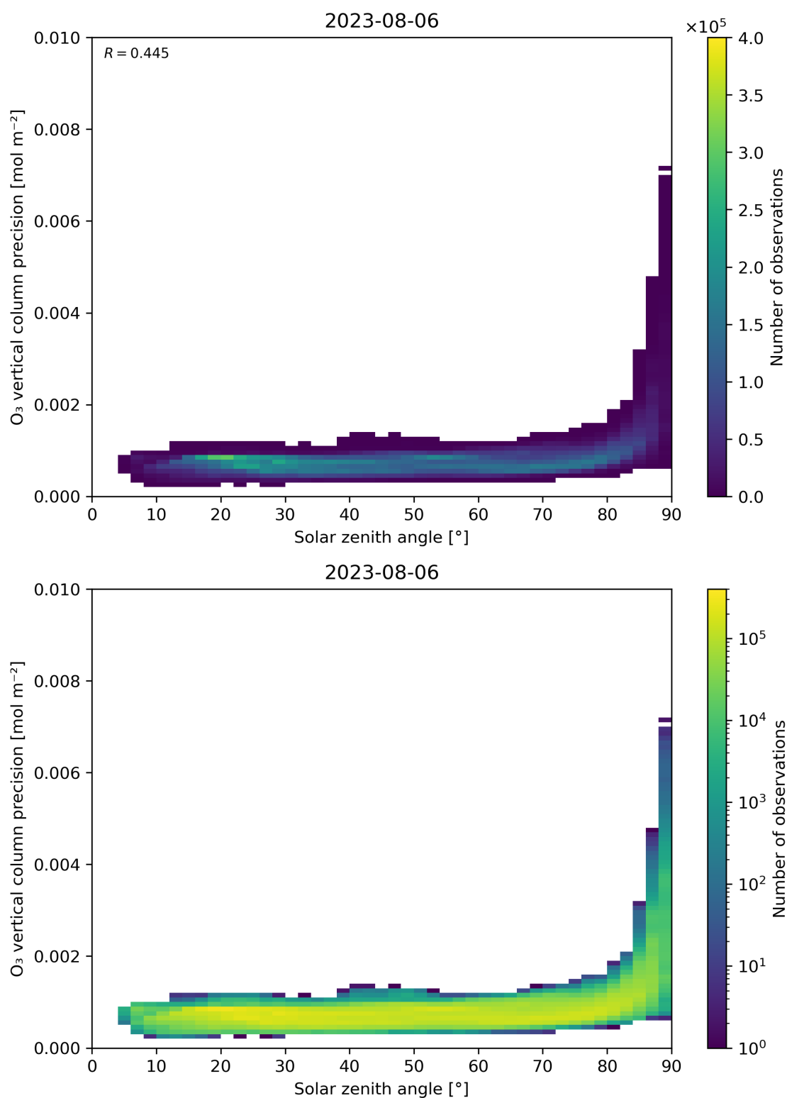
Figure 48: Scatter density plot of “Solar zenith angle” against “O 3 vertical column precision” for 2023-08-05 to 2023-08-07.
