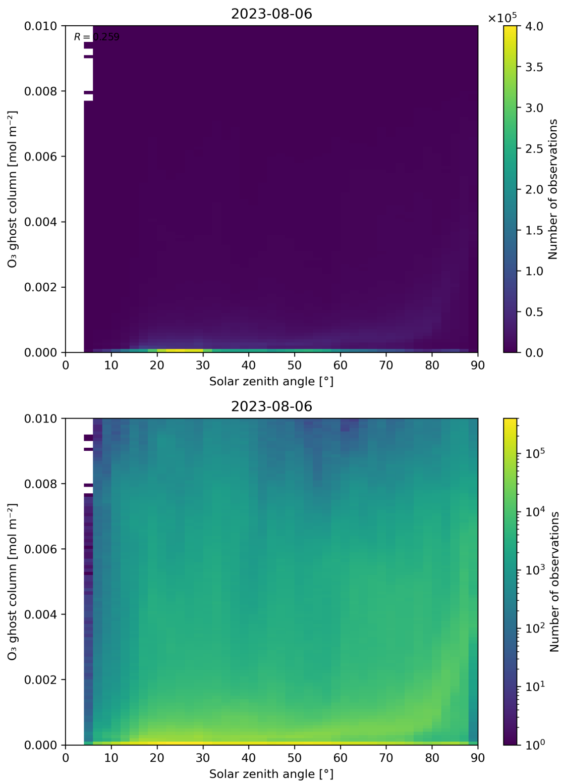
Figure 46: Scatter density plot of “Solar zenith angle” against “O 3 ghost column” for 2023-08-05 to 2023-08-07.
