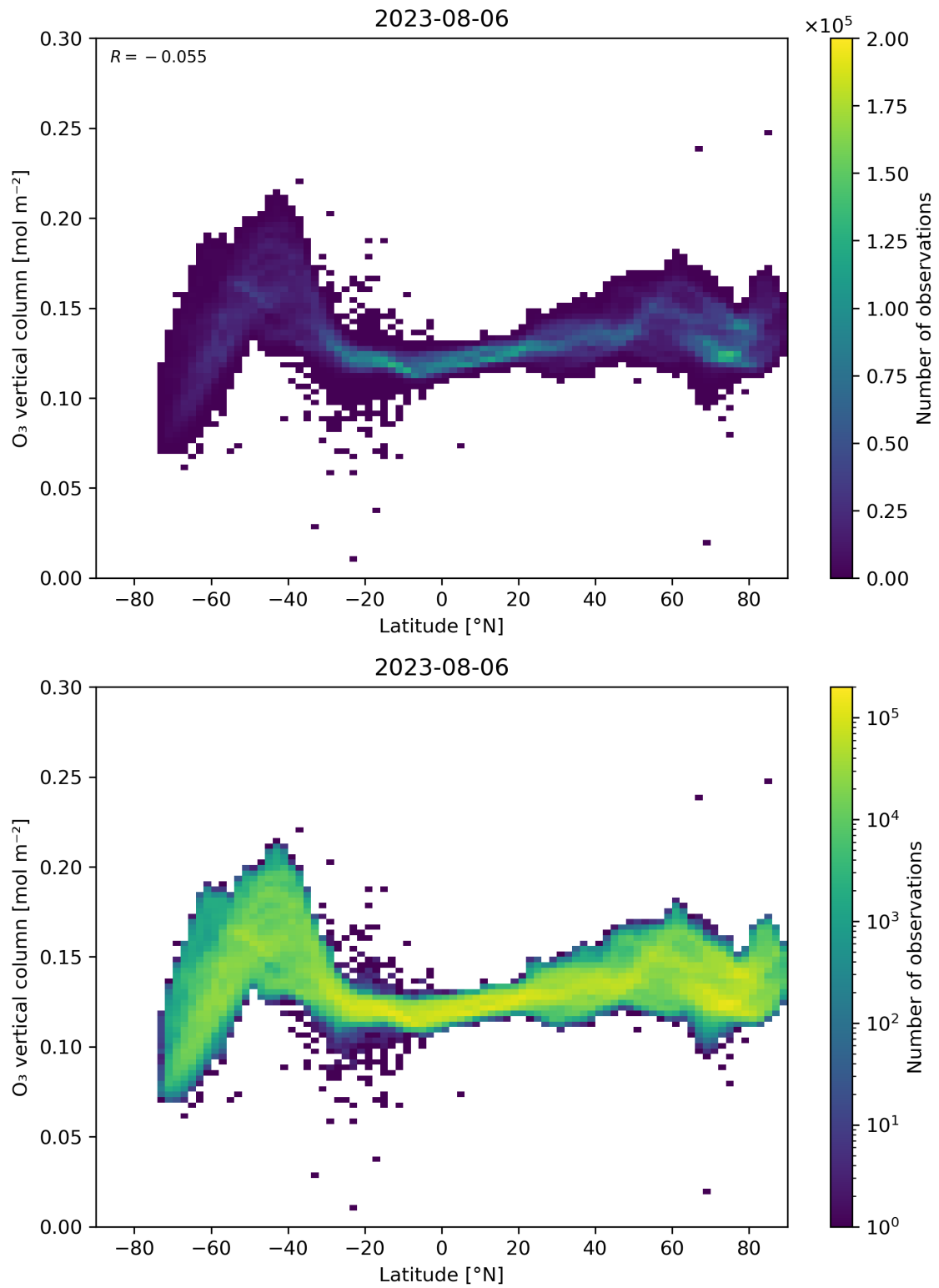
Figure 36: Scatter density plot of “Latitude” against “O 3 vertical column” for 2023-08-05 to 2023-08-07.
