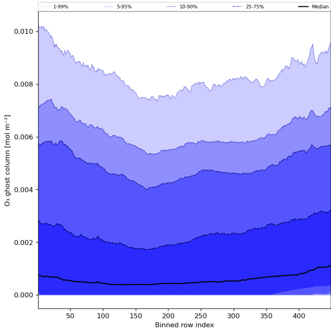
Figure 32: Along track statistics of “O 3 ghost column” for 2023-08-05 to 2023-08-07
