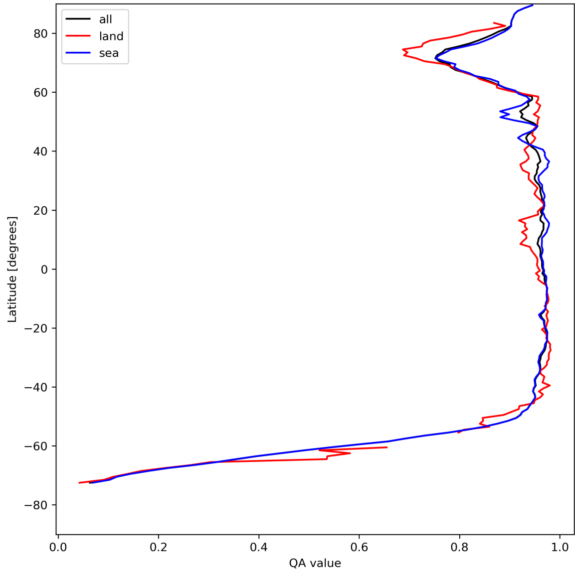
Figure 13: Zonal average of “QA value” for 2023-08-05 to 2023-08-07.
