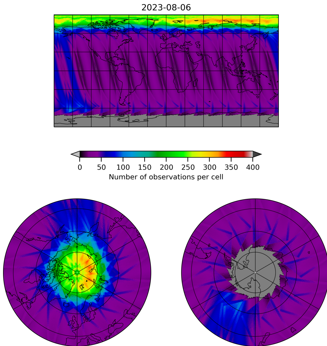
Figure 12: Map of the number of observations for 2023-08-05 to 2023-08-07
