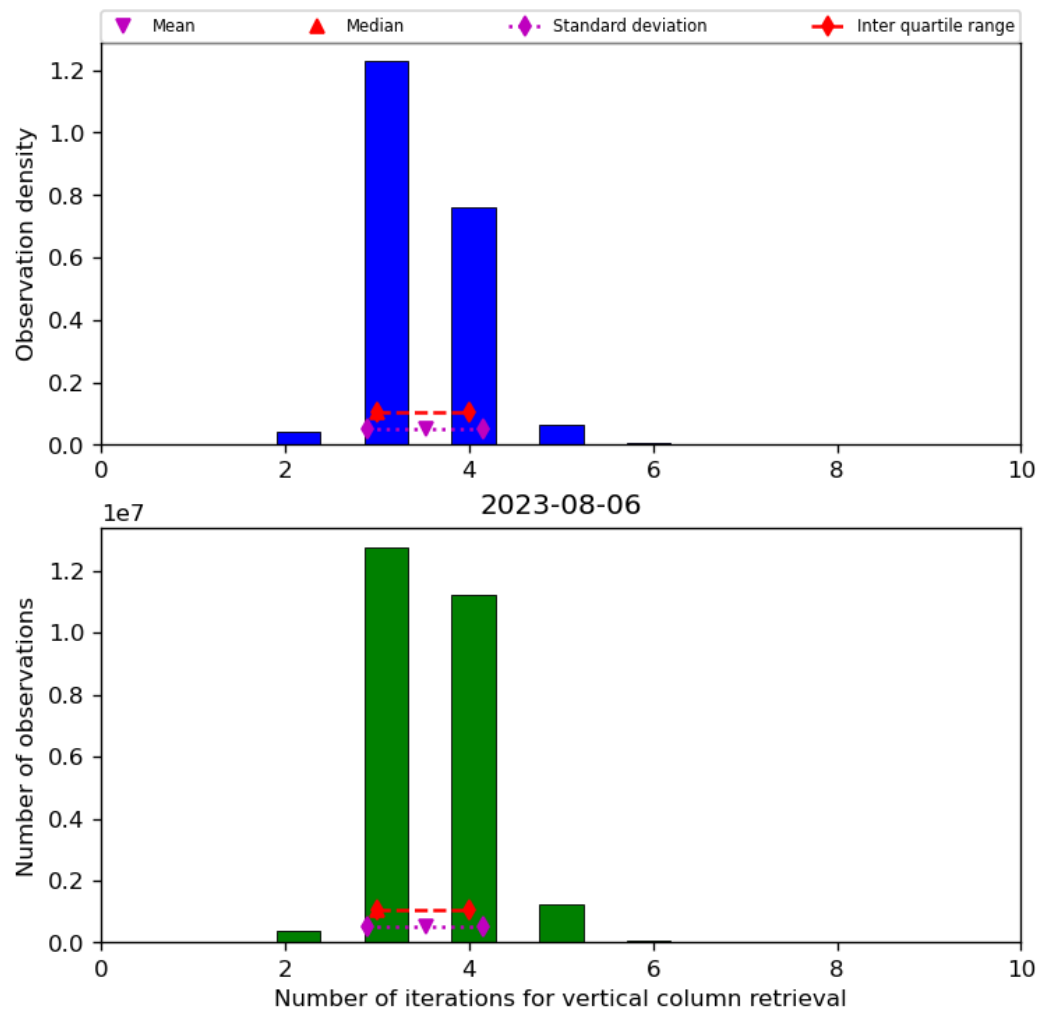
Figure 26: Histogram of “Number of iterations for vertical column retrieval” for 2023-08-05 to 2023-08-07
