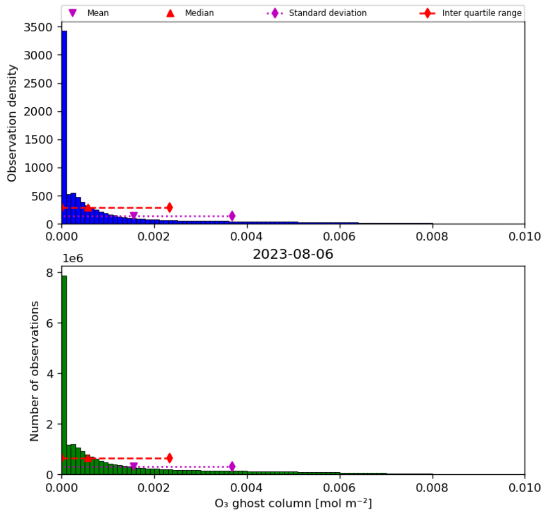
Figure 25: Histogram of “O 3 ghost column” for 2023-08-05 to 2023-08-07
