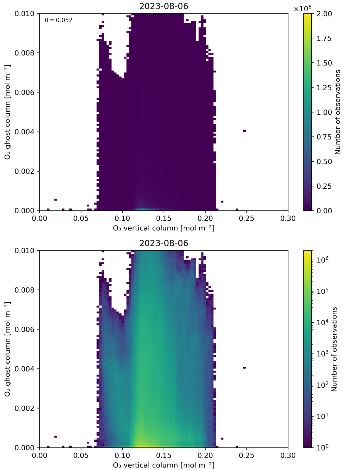
Figure 40: Scatter density plot of “O 3 vertical column” against “O 3 ghost column” for 2023-08-05 to 2023-08-07.
