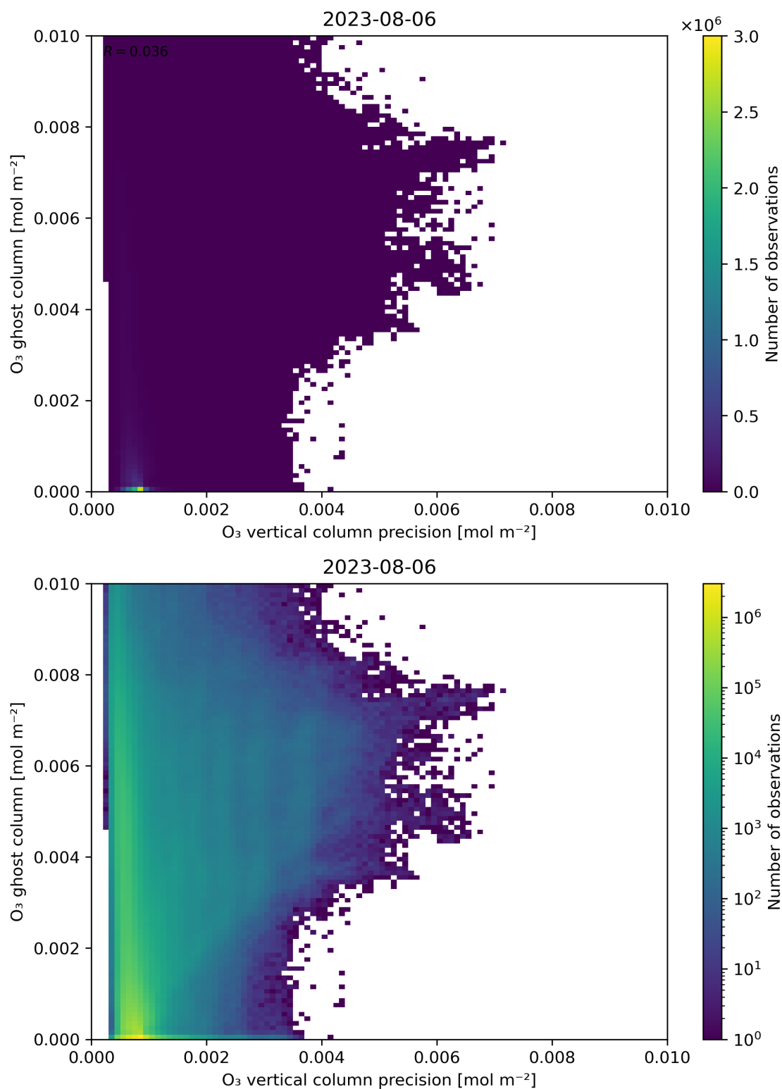
Figure 43: Scatter density plot of “ O_3 vertical column precision” against “ O_3 ghost column” for 2023-08-05 to 2023-08-07.
