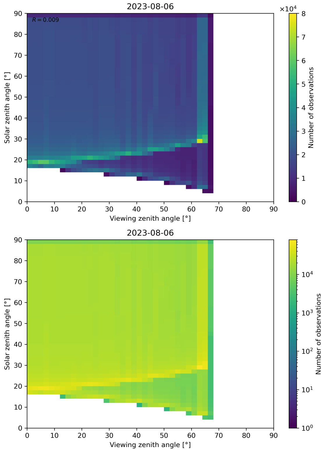
Figure 54: Scatter density plot of “Viewing zenith angle” against “Solar zenith angle” for 2023-08-05 to 2023-08-07.
