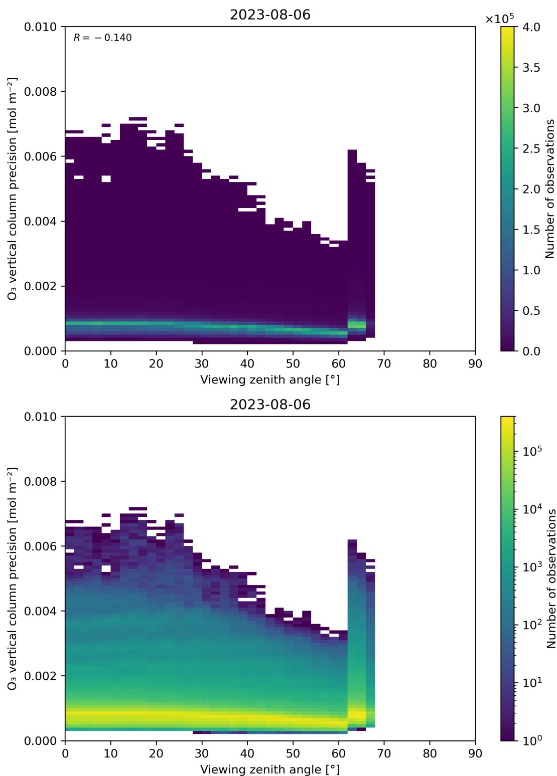
Figure 53: Scatter density plot of “Viewing zenith angle” against “O 3 vertical column precision” for 2023-08-05 to 2023-08-07.
