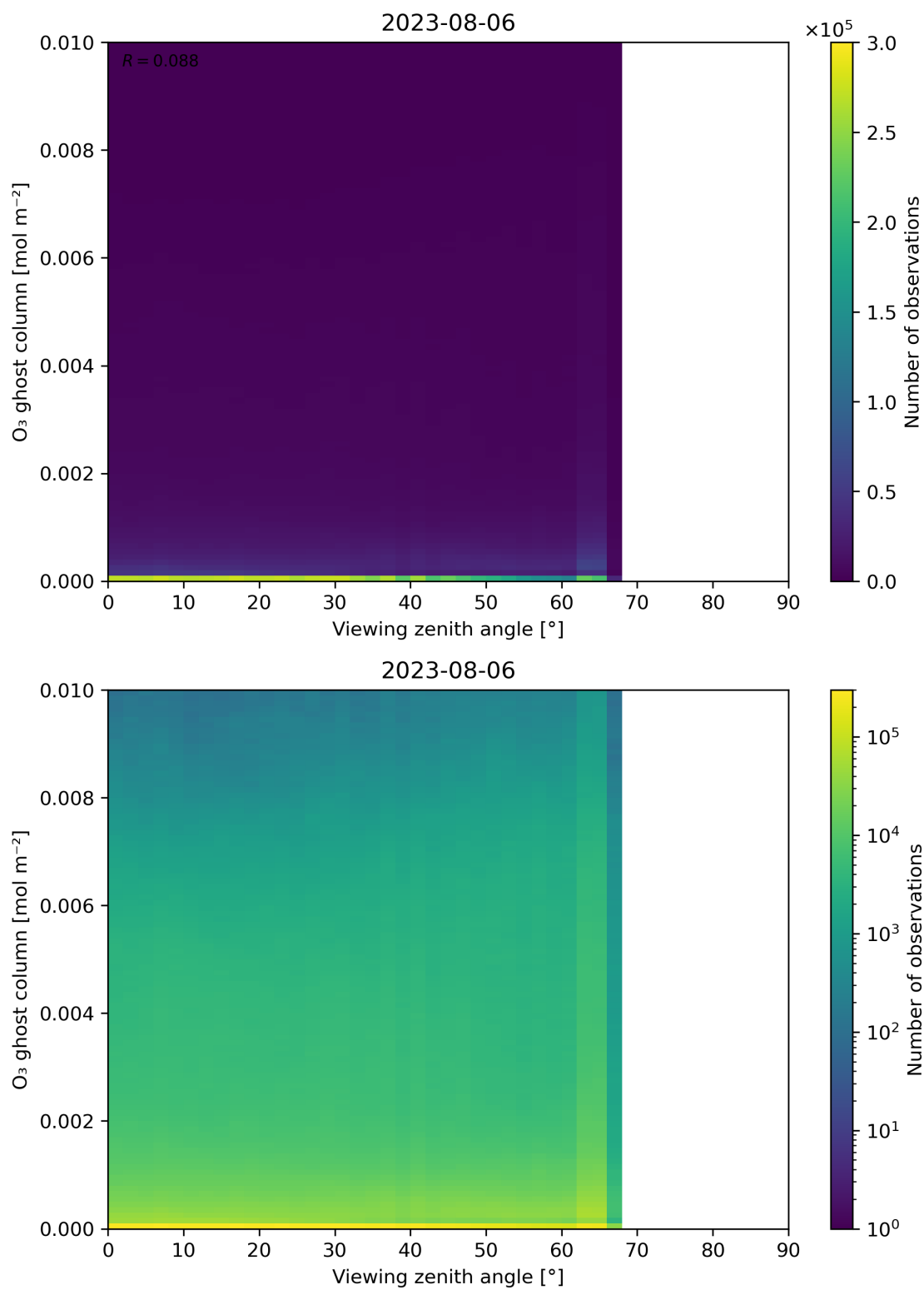
Figure 51: Scatter density plot of “Viewing zenith angle” against “O 3 ghost column” for 2023-08-05 to 2023-08-07.
