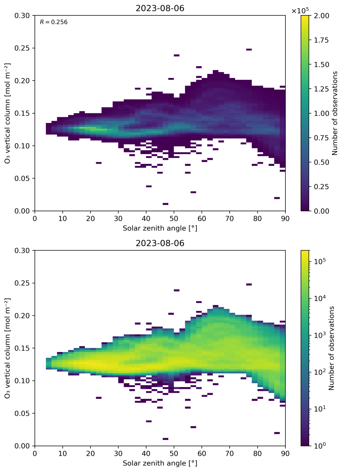
Figure 47: Scatter density plot of “Solar zenith angle” against “O 3 vertical column” for 2023-08-05 to 2023-08-07.
