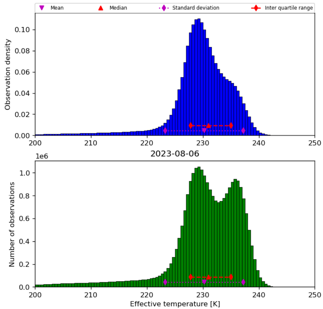
Figure 24: Histogram of “Effective temperature” for 2023-08-05 to 2023-08-07
