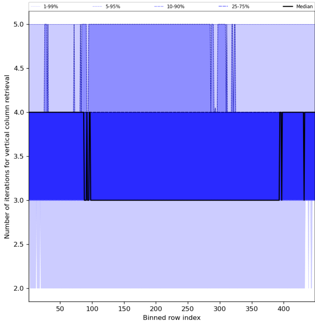
Figure 33: Along track statistics of “Number of iterations for vertical column retrieval” for 2023-08-05 to 2023-08-07
