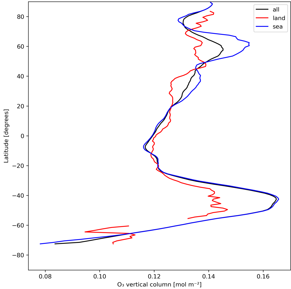
Figure 14: Zonal average of “O 3 vertical column” for 2023-08-05 to 2023-08-07.
