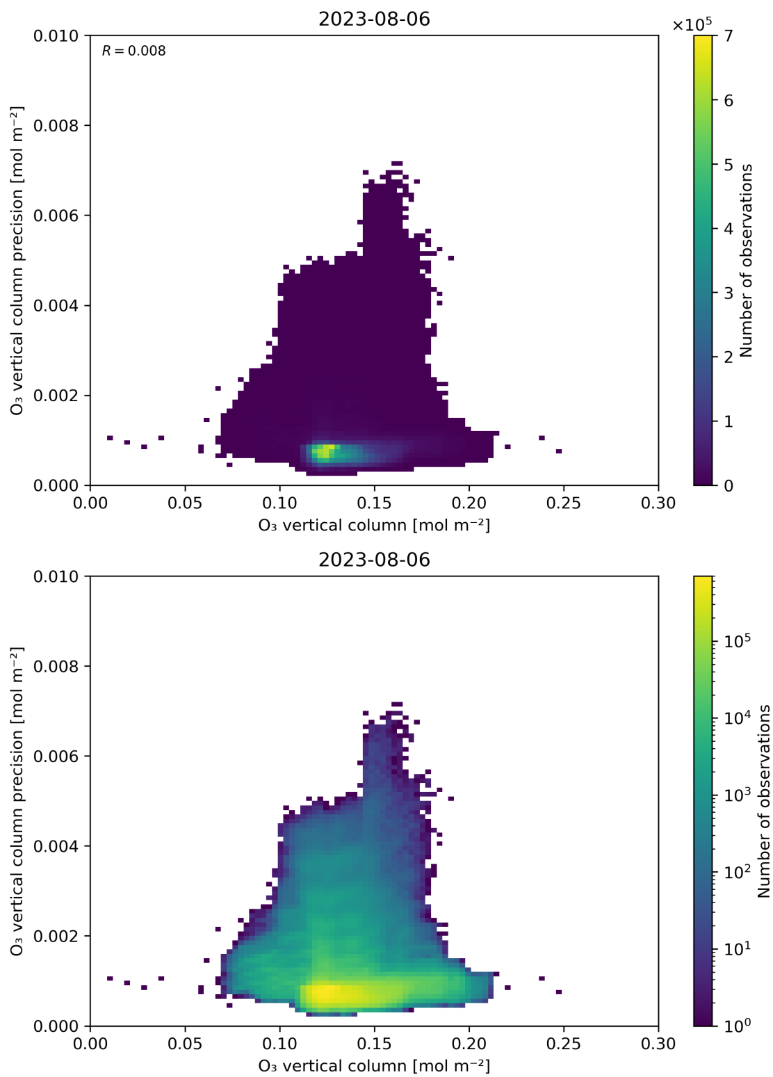
Figure 41: Scatter density plot of “O 3 vertical column” against “O 3 vertical column precision” for 2023-08-05 to 2023-08-07.
