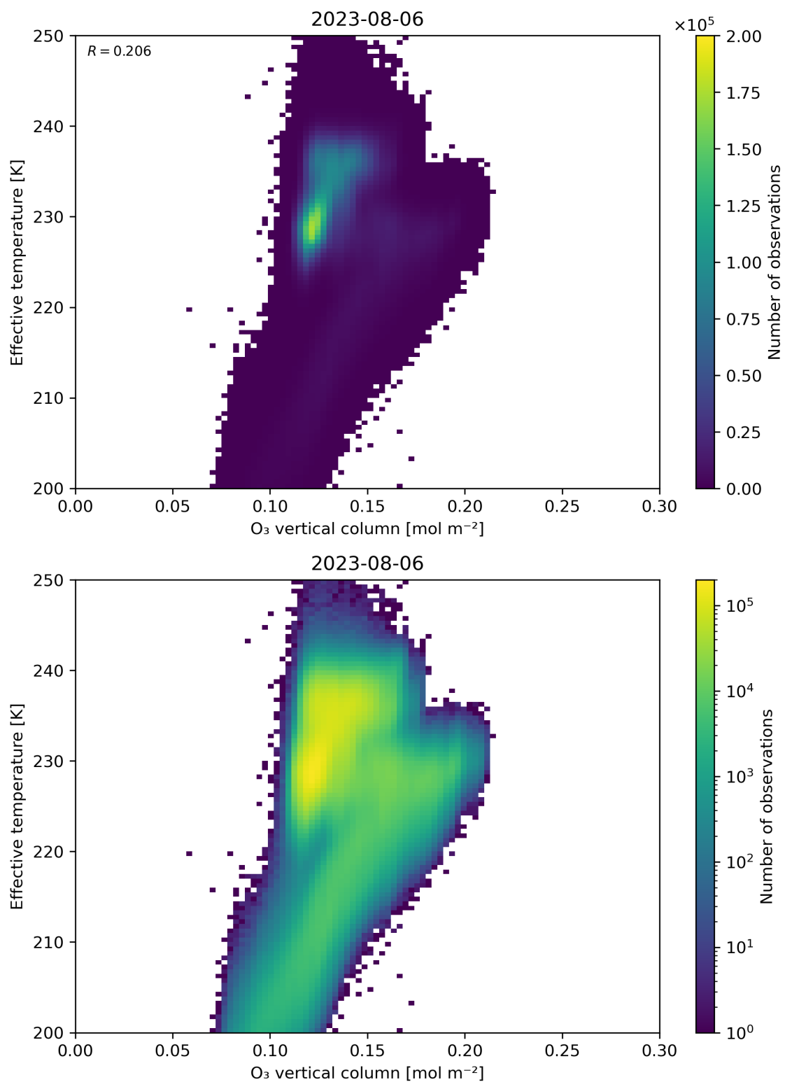
Figure 39: Scatter density plot of “O 3 vertical column” against “Effective temperature” for 2023-08-05 to 2023-08-07.
