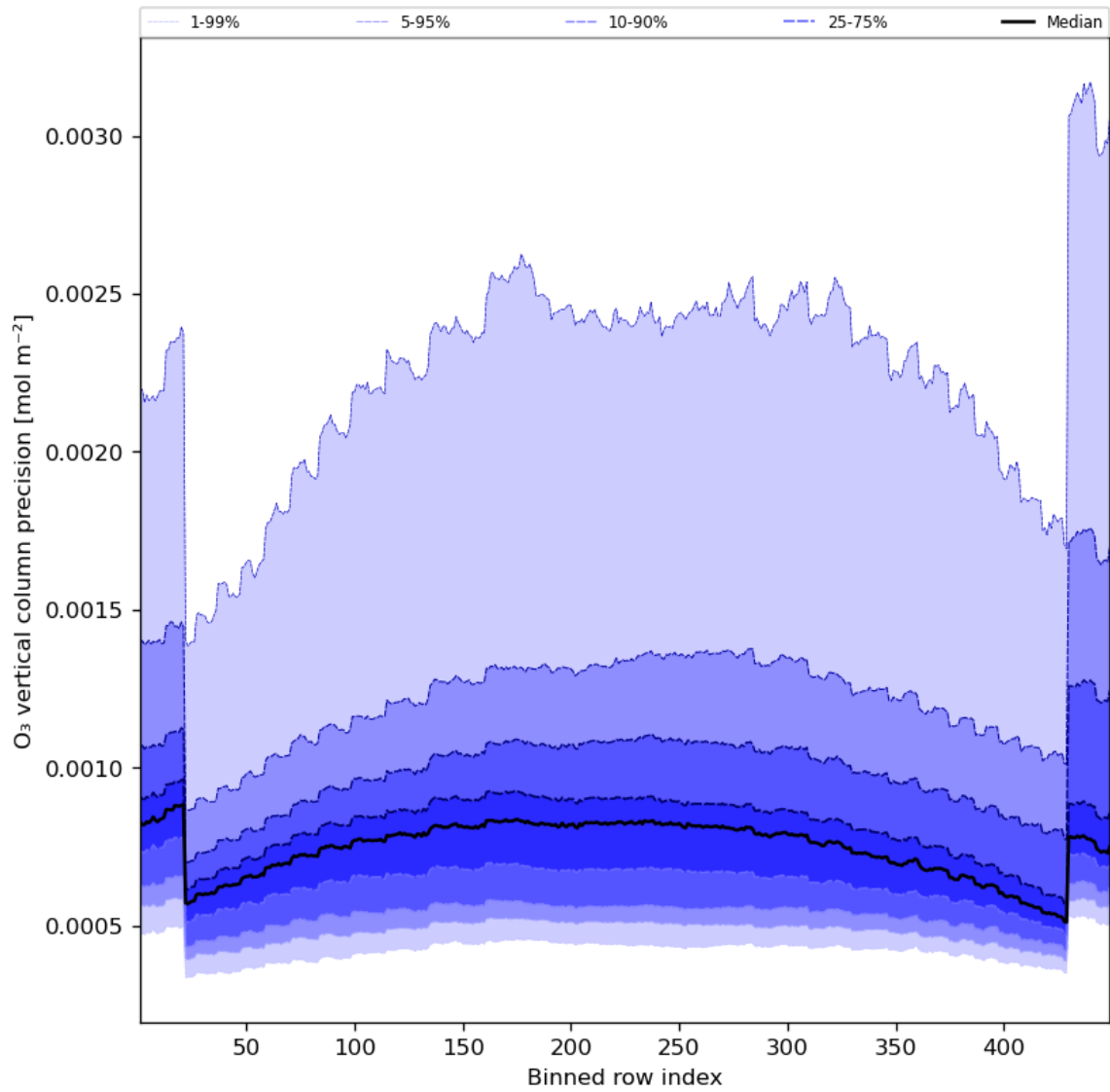
Figure 29: Along track statistics of “O 3 vertical column precision” for 2023-08-05 to 2023-08-07
