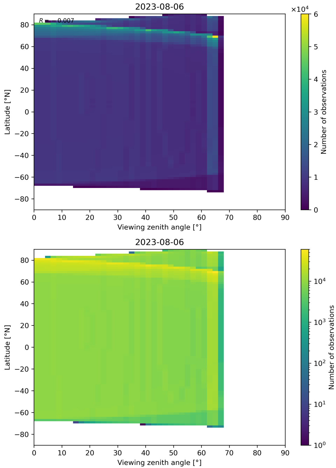
Figure 49: Scatter density plot of “Viewing zenith angle” against “Latitude” for 2023-08-05 to 2023-08-07.
