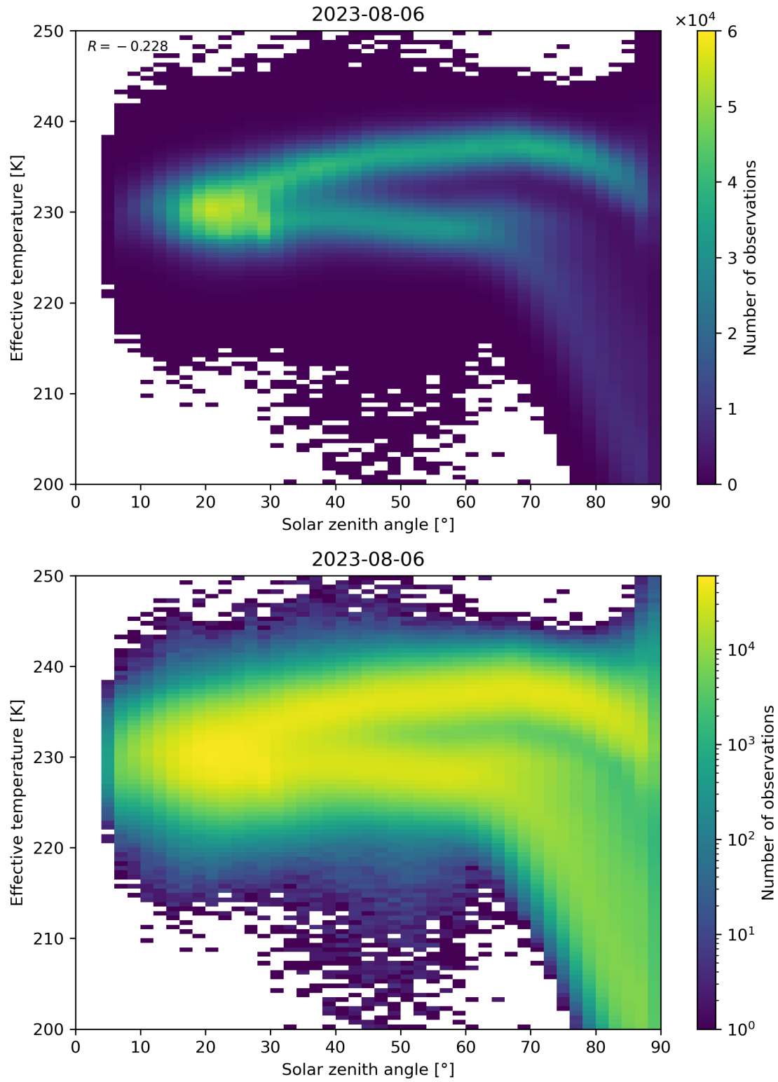
Figure 45: Scatter density plot of “Solar zenith angle” against “Effective temperature” for 2023-08-05 to 2023-08-07.
