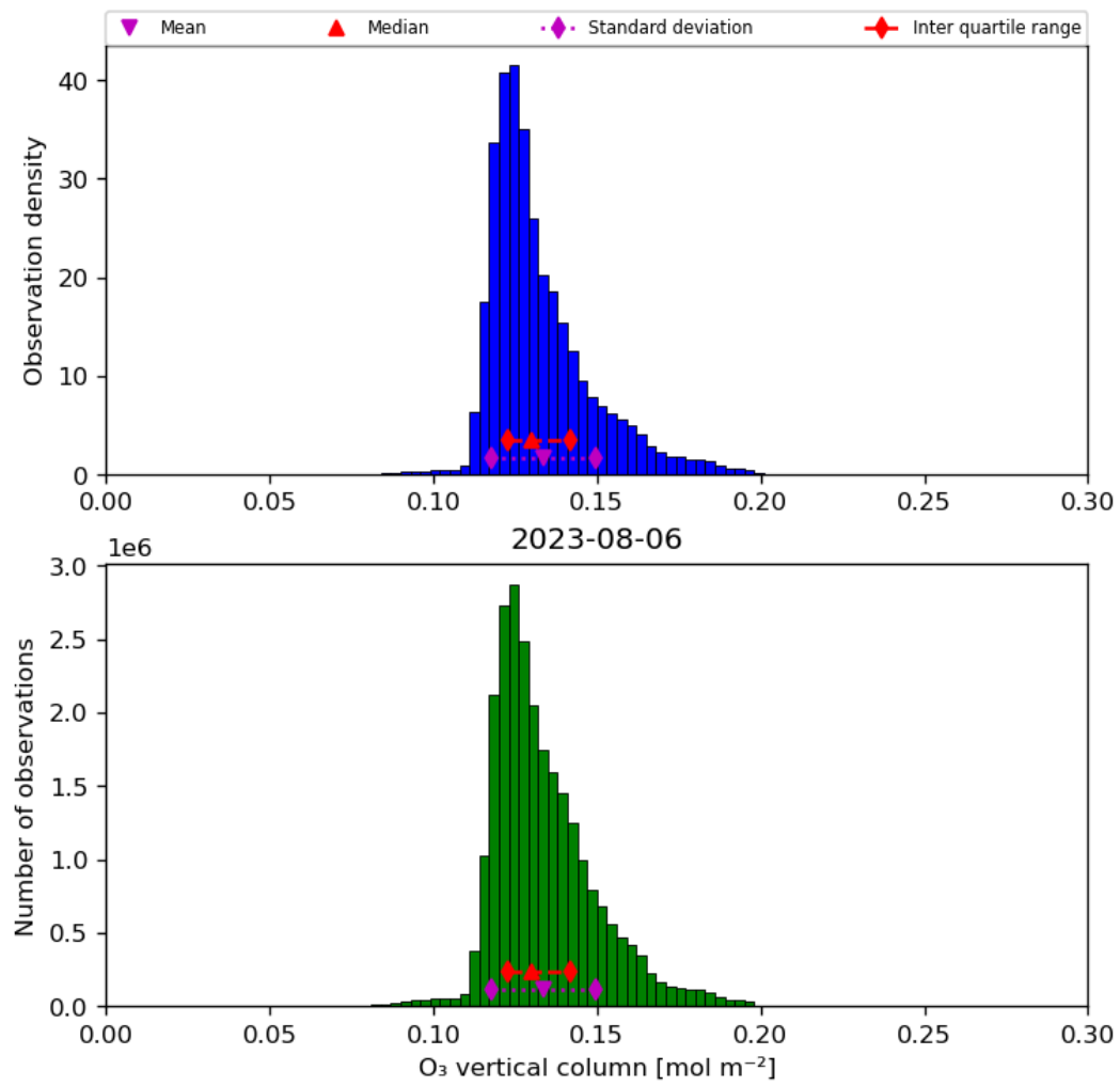
Figure 21: Histogram of “O 3 vertical column” for 2023-08-05 to 2023-08-07
