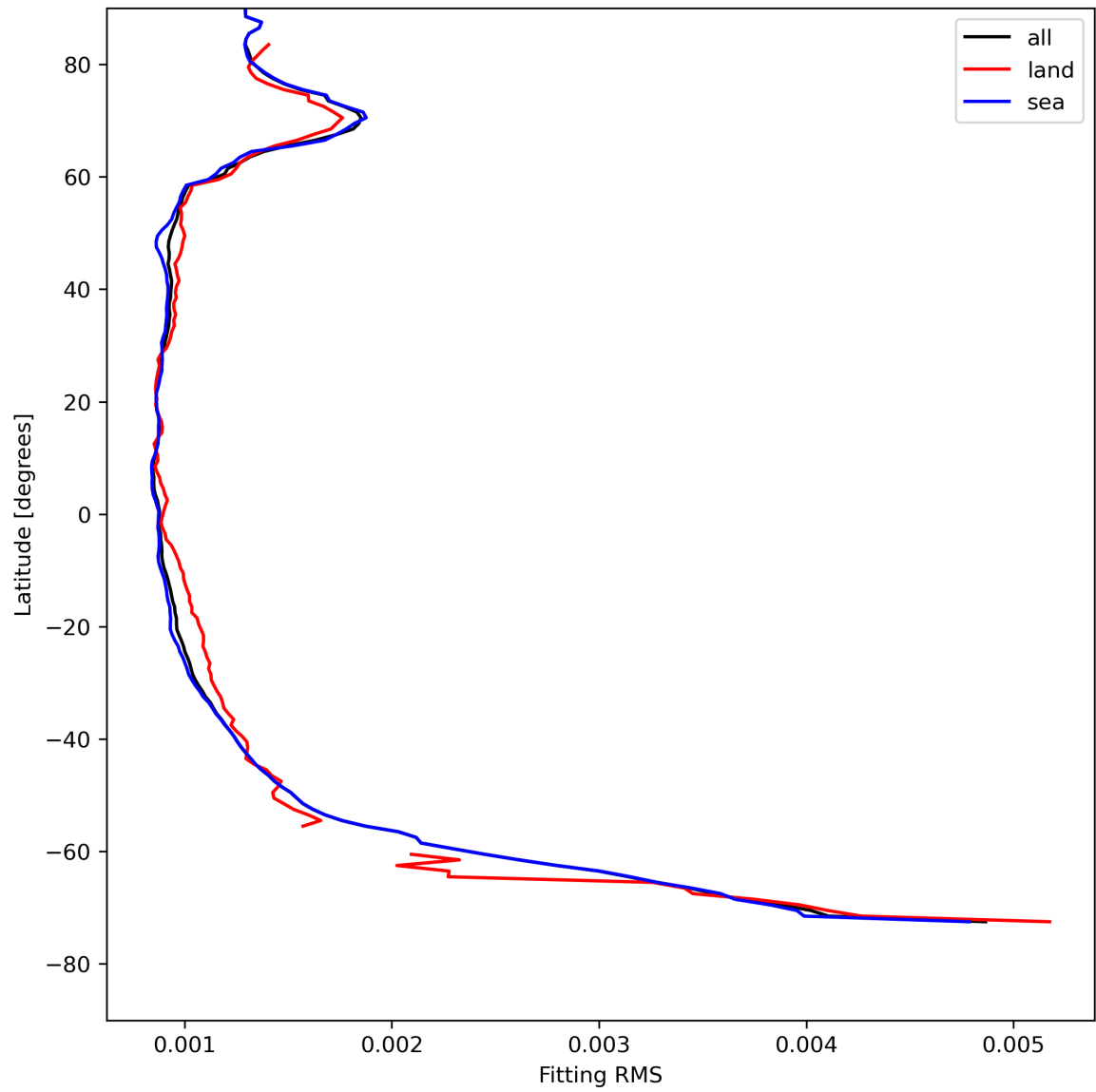
Figure 16: Zonal average of “Fitting RMS” for 2023-08-05 to 2023-08-07.
