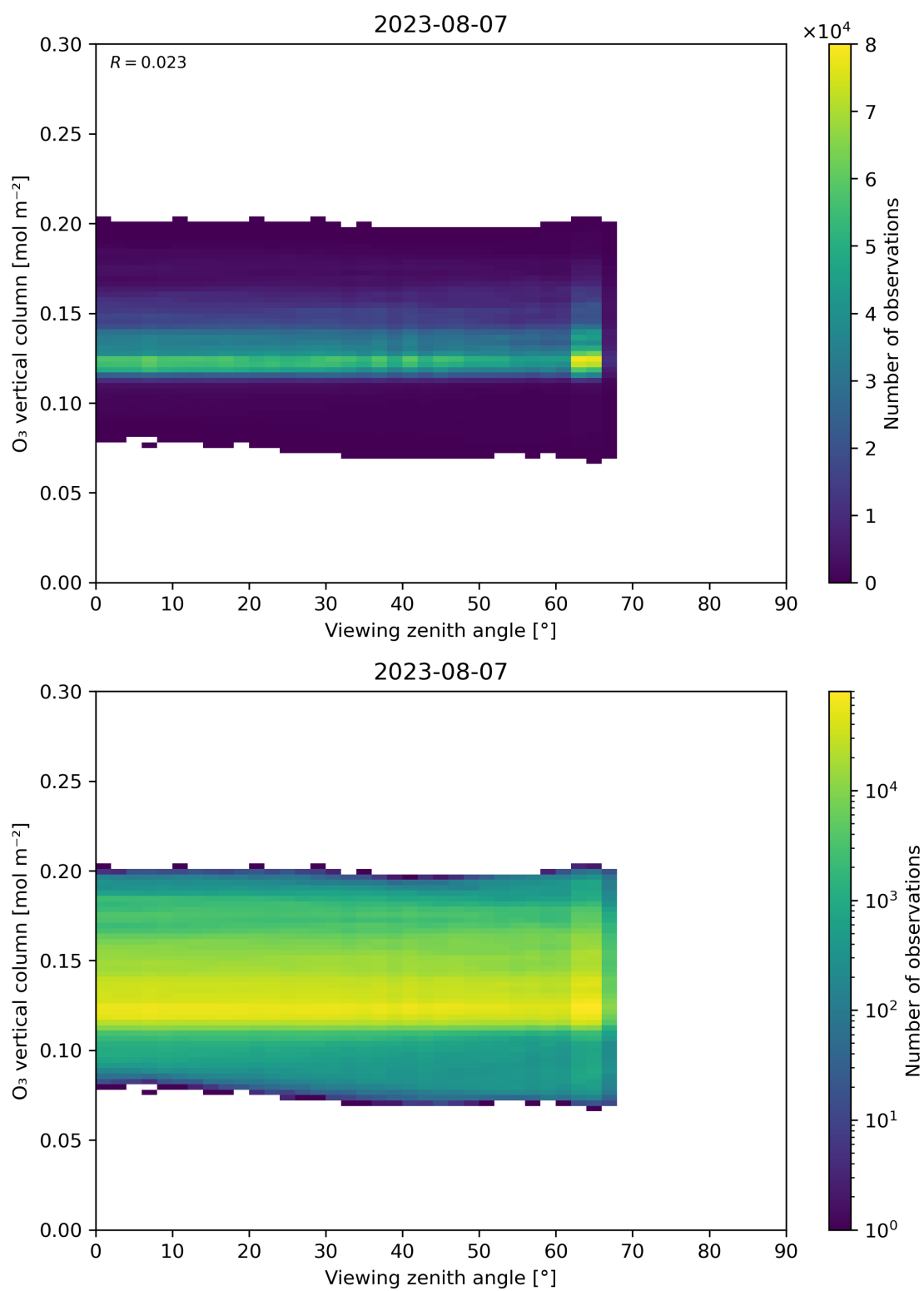
Figure 52: Scatter density plot of “Viewing zenith angle” against “O 3 vertical column” for 2023-08-06 to 2023-08-08.
