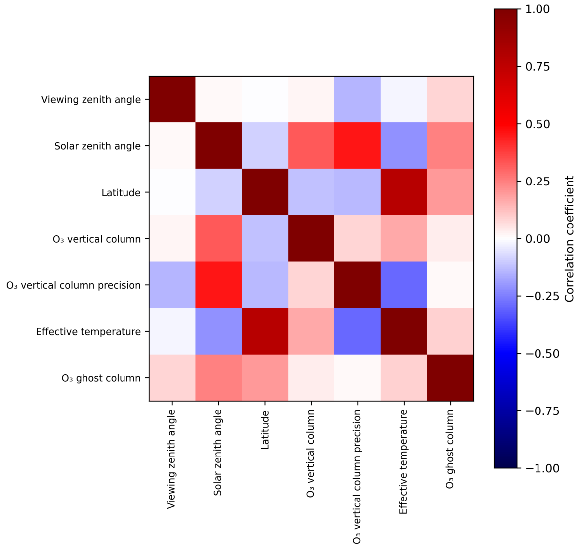
Figure 2: Map of correlation matrix for 2023-08-06 to 2023-08-08.
