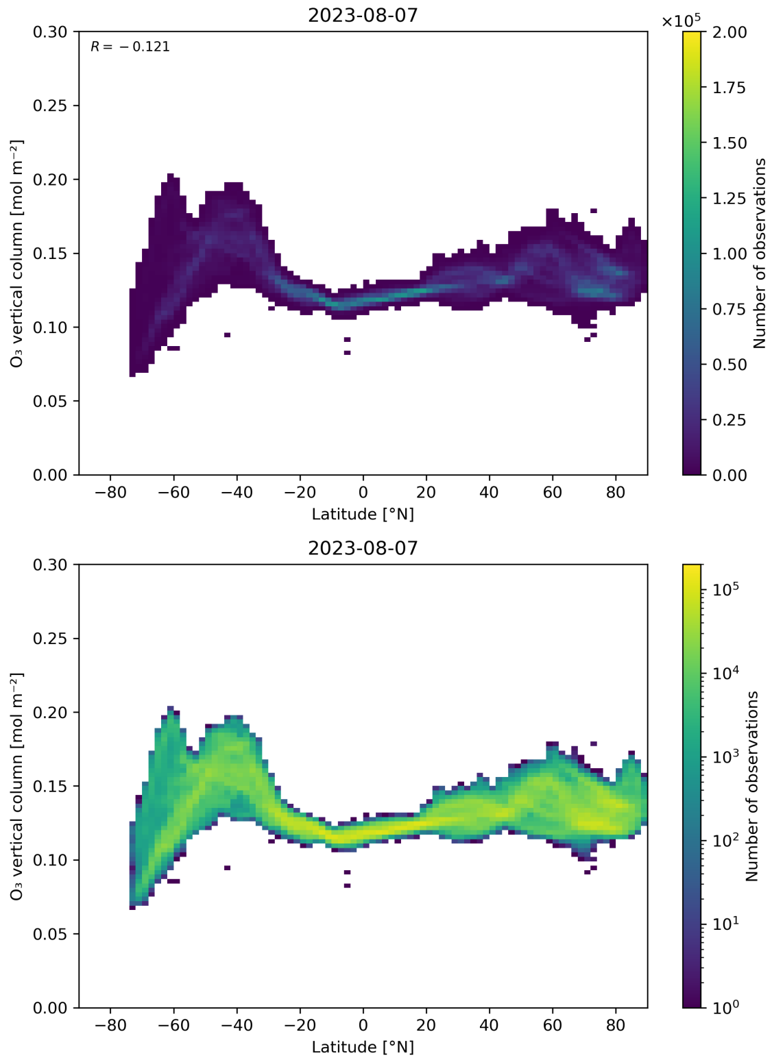
Figure 36: Scatter density plot of “Latitude” against “O 3 vertical column” for 2023-08-06 to 2023-08-08.
