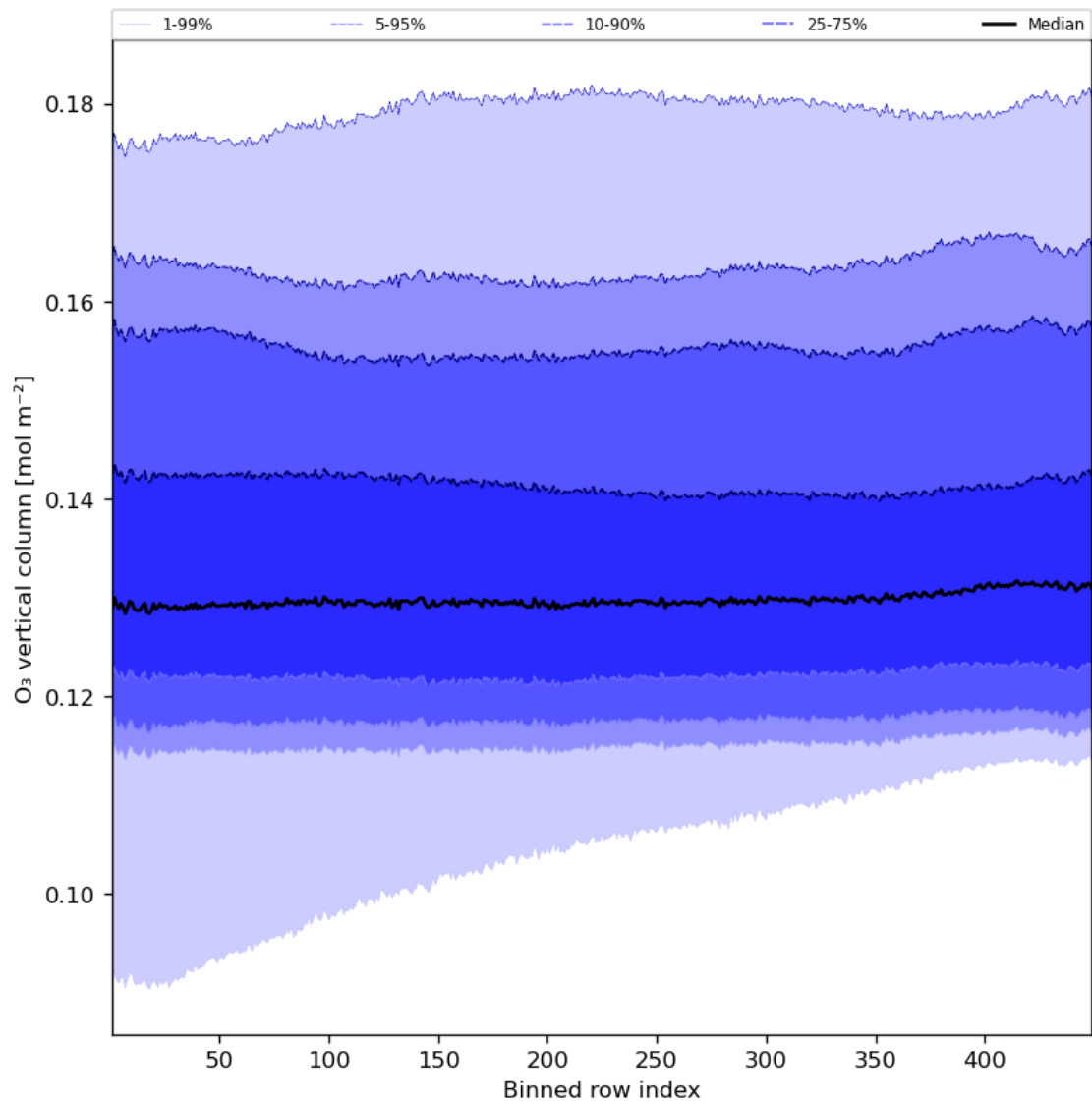
Figure 28: Along track statistics of “O 3 vertical column” for 2023-08-06 to 2023-08-08
