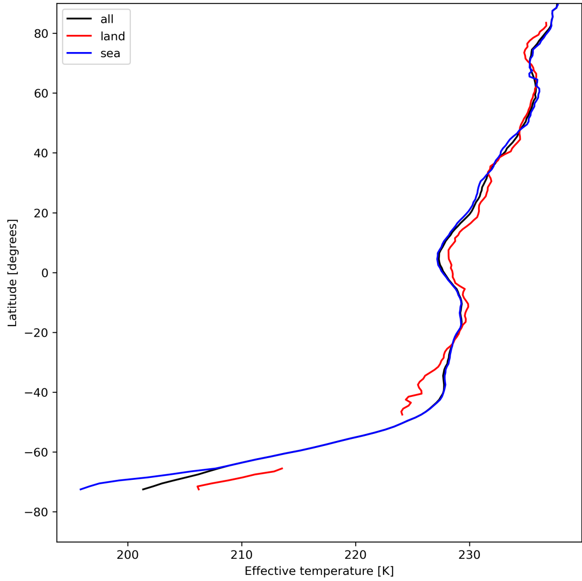
Figure 17: Zonal average of "Effective temperature" for 2023-08-06 to 2023-08-08.
