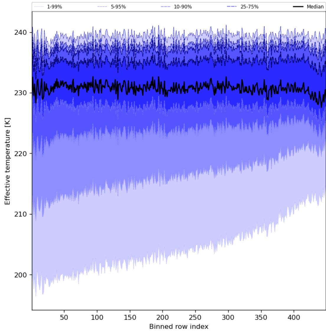
Figure 31: Along track statistics of “Effective temperature” for 2023-08-06 to 2023-08-08
