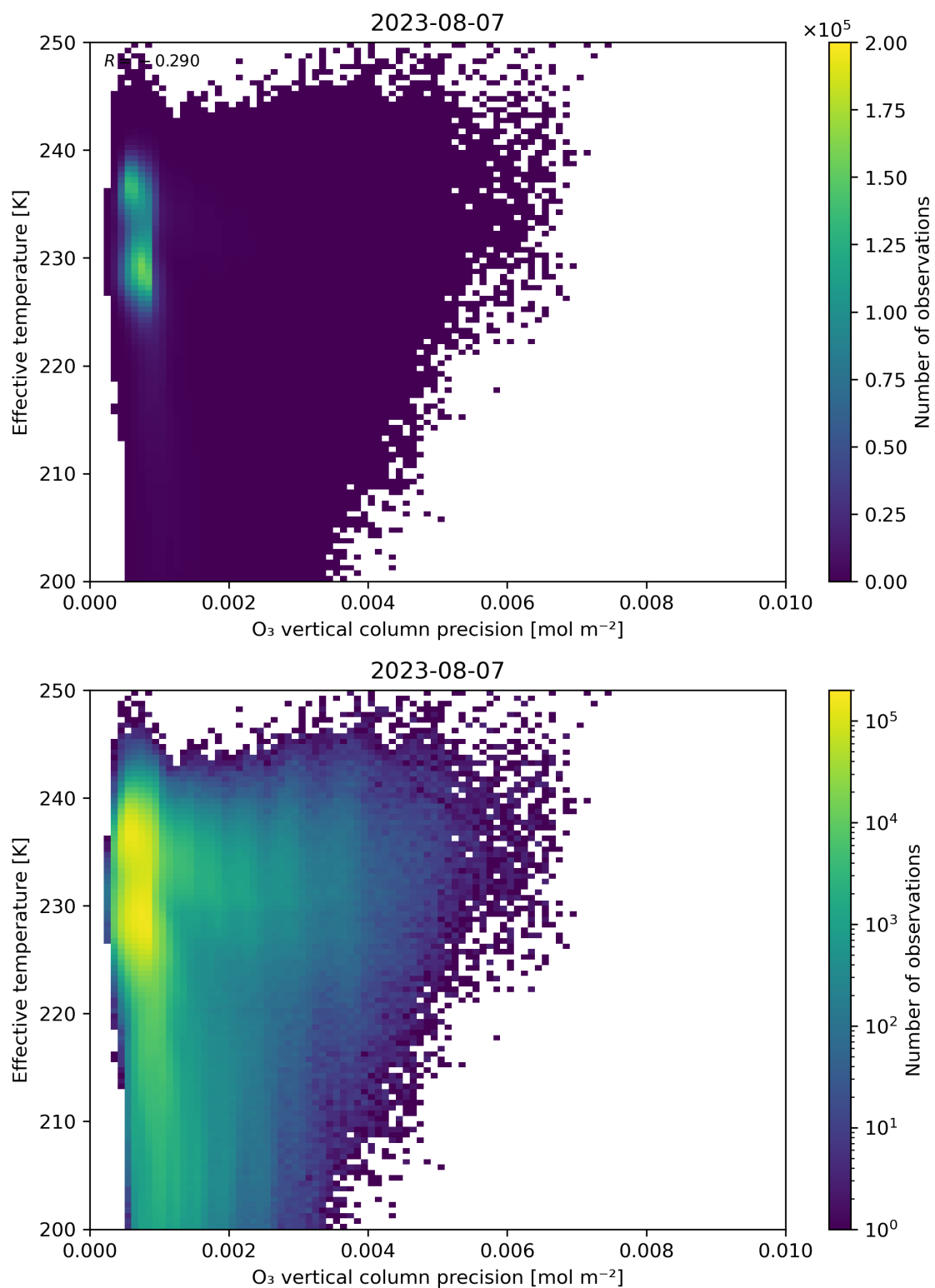
Figure 42: Scatter density plot of “O 3 vertical column precision” against “Effective temperature” for 2023-08-06 to 2023-08-08.
