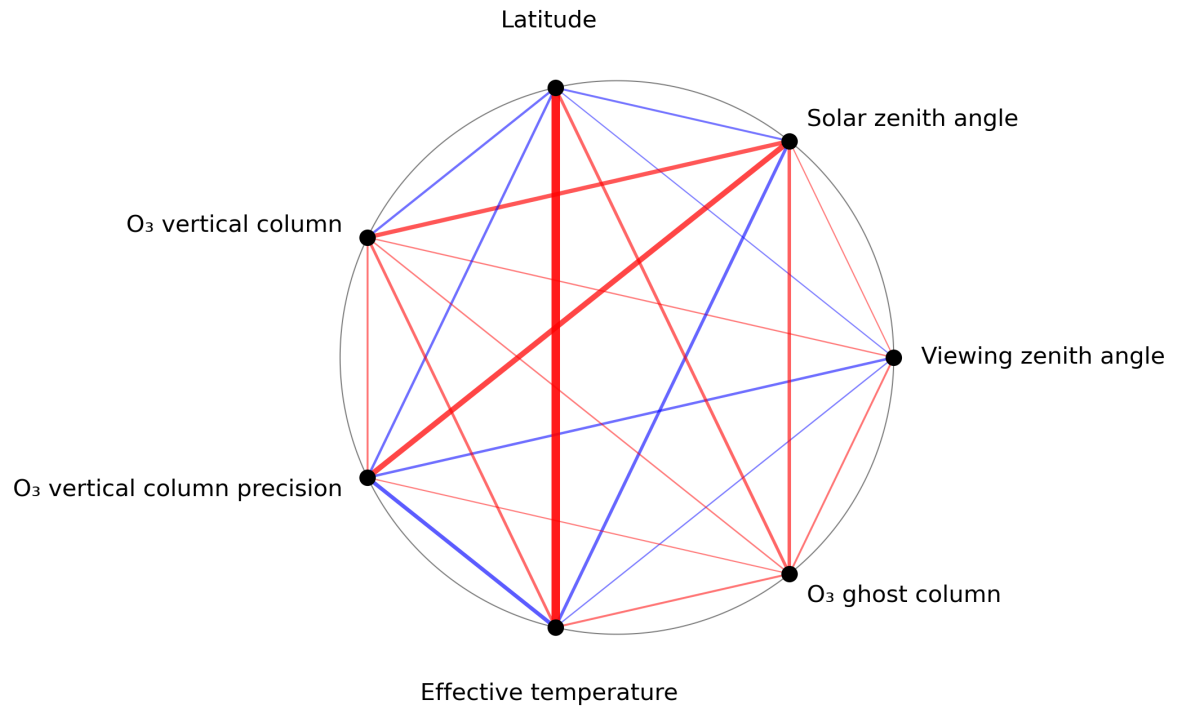
Figure 1: Map of correlation graph for 2023-08-06 to 2023-08-08.
