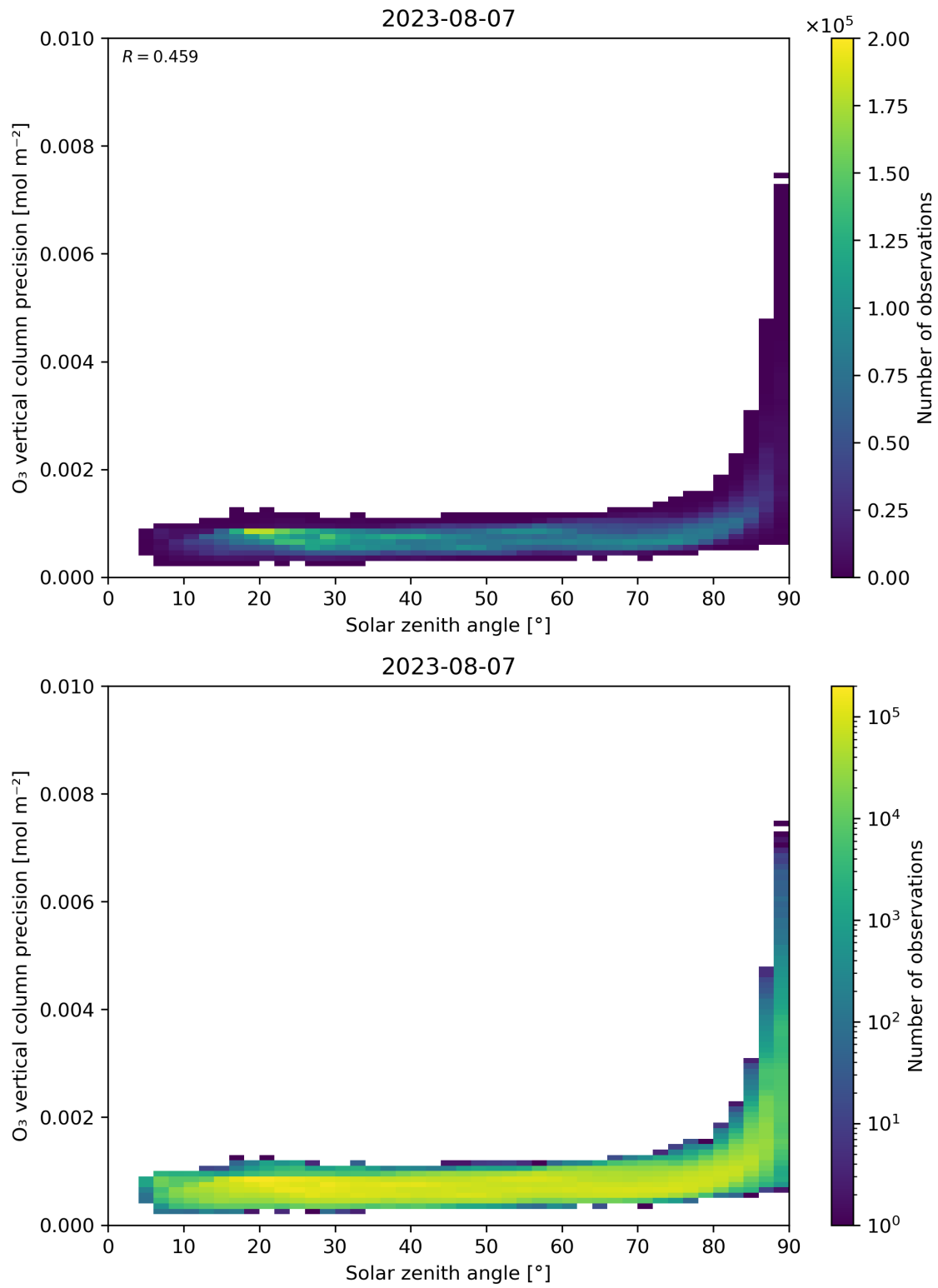
Figure 48: Scatter density plot of “Solar zenith angle” against “O 3 vertical column precision” for 2023-08-06 to 2023-08-08.
