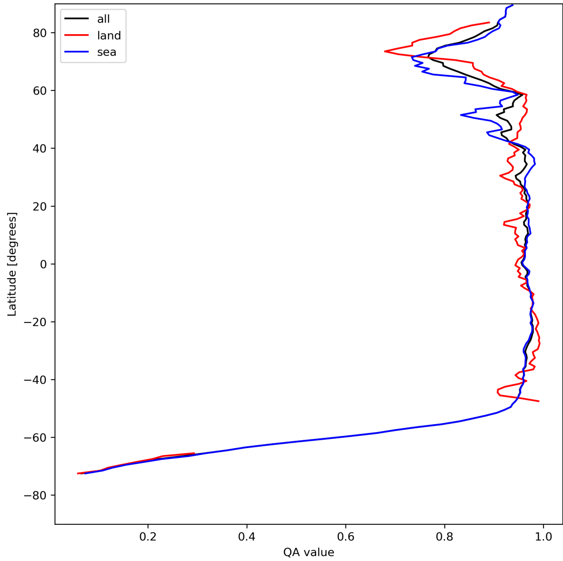
Figure 13: Zonal average of “QA value” for 2023-08-06 to 2023-08-08.
