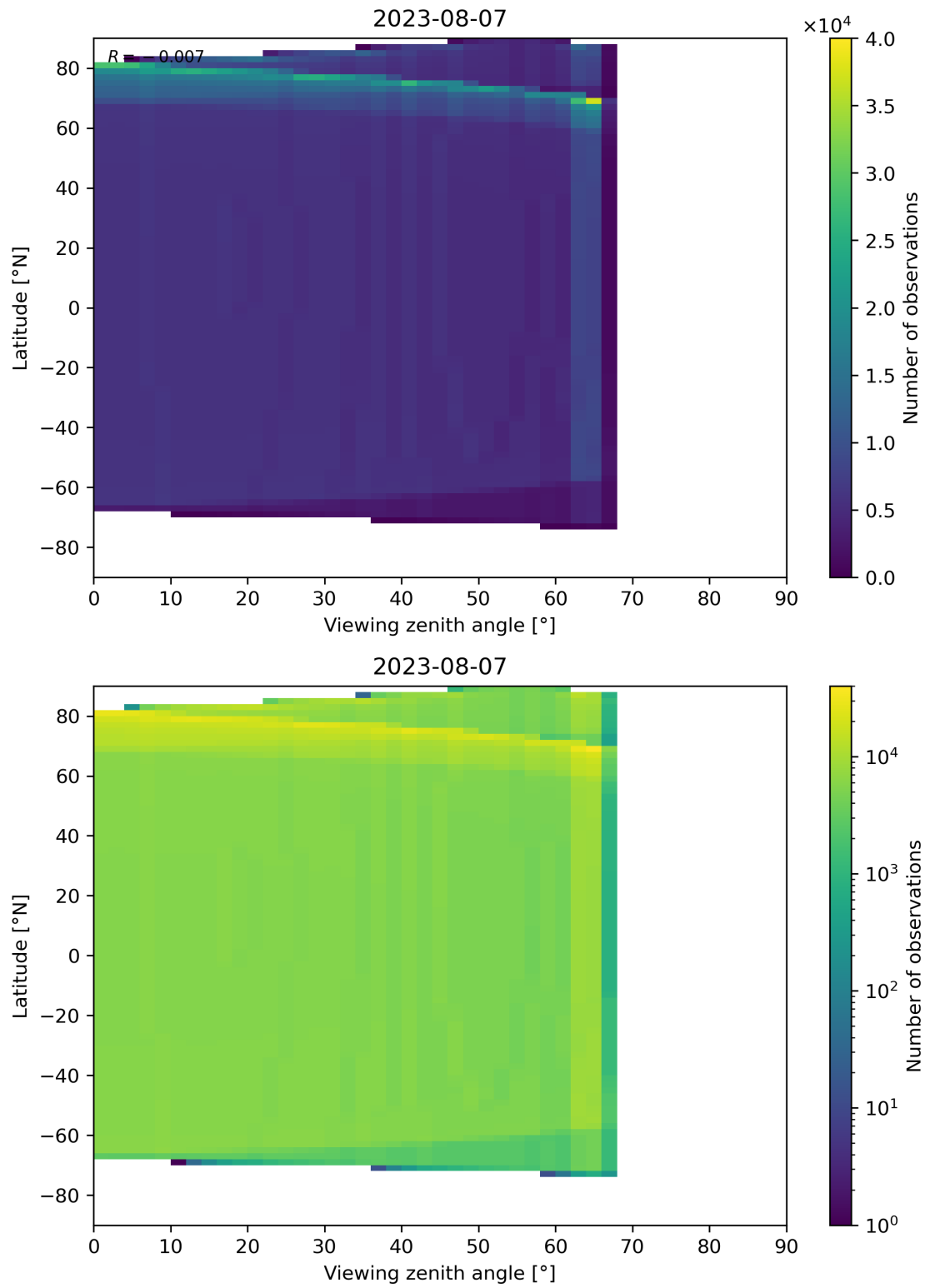
Figure 49: Scatter density plot of “Viewing zenith angle” against “Latitude” for 2023-08-06 to 2023-08-08.
