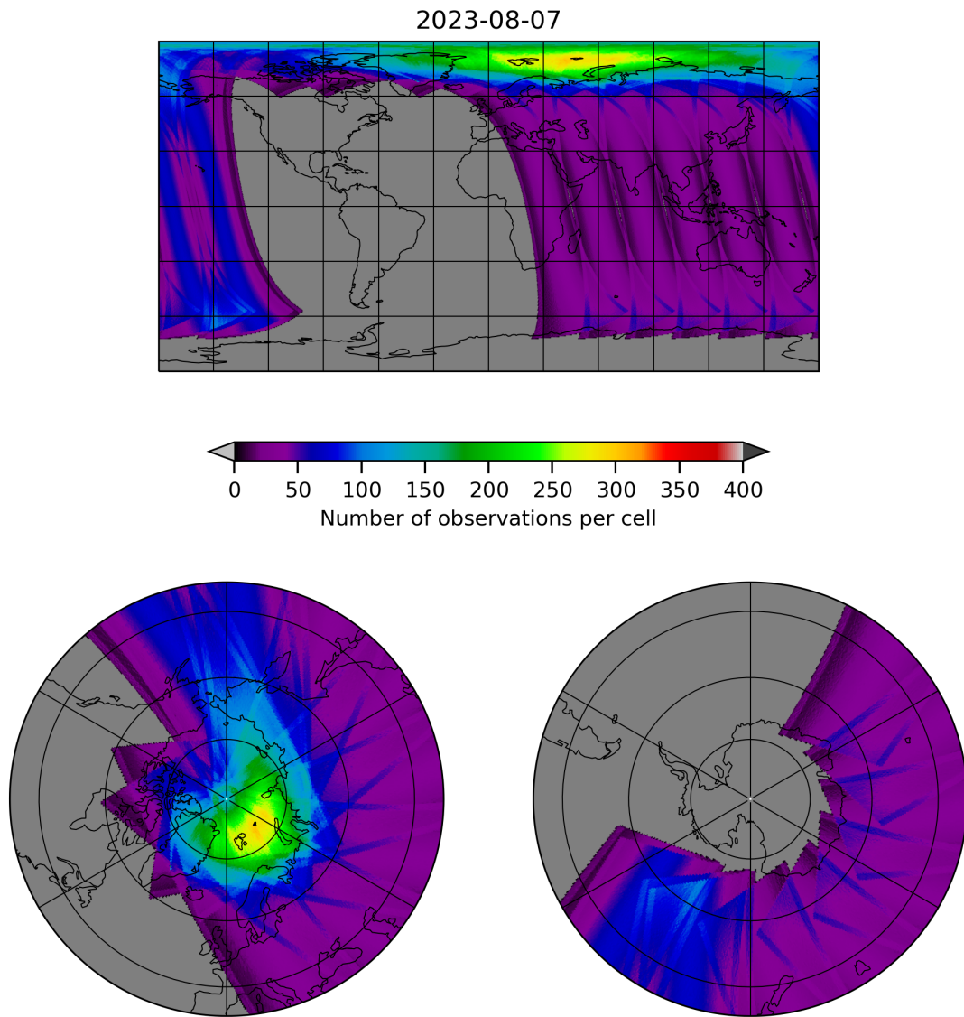
Figure 12: Map of the number of observations for 2023-08-06 to 2023-08-08
