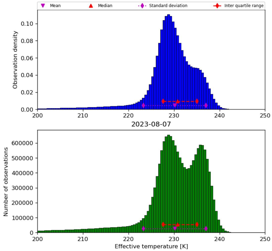
Figure 24: Histogram of “Effective temperature” for 2023-08-06 to 2023-08-08
