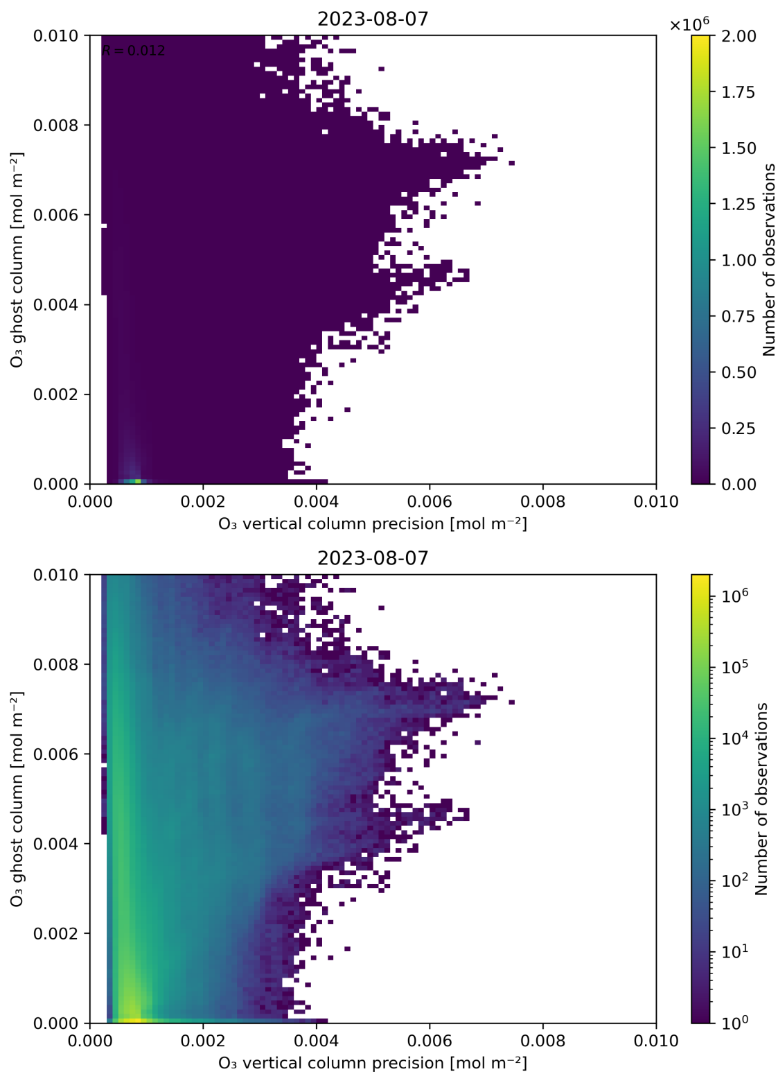
Figure 43: Scatter density plot of “O 3 vertical column precision” against “O 3 ghost column” for 2023-08-06 to 2023-08-08.
