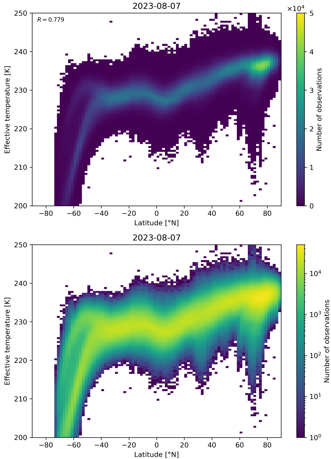
Figure 34: Scatter density plot of “Latitude” against “Effective temperature” for 2023-08-06 to 2023-08-08.
