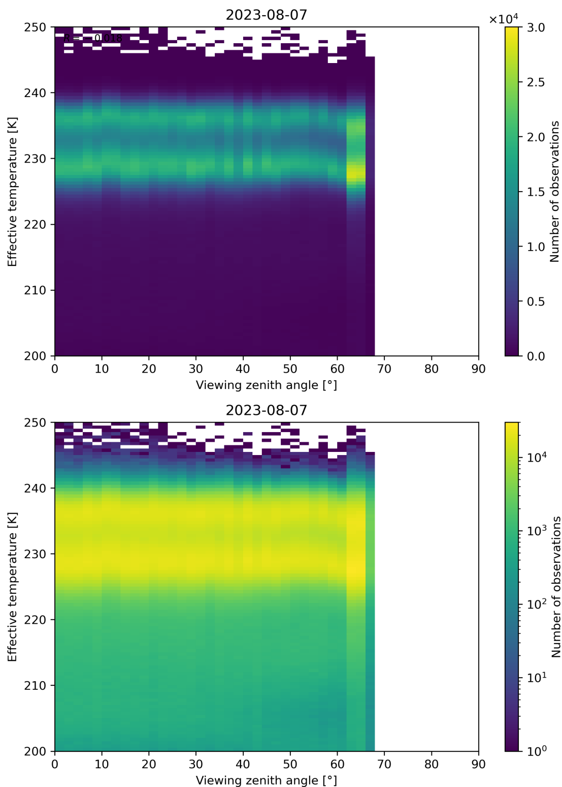
Figure 50: Scatter density plot of “Viewing zenith angle” against “Effective temperature” for 2023-08-06 to 2023-08-08.
