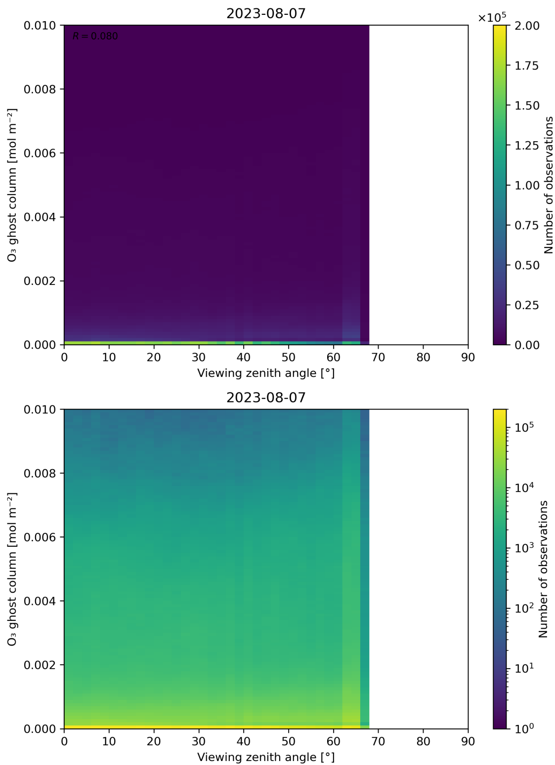
Figure 51: Scatter density plot of “Viewing zenith angle” against “O 3 ghost column” for 2023-08-06 to 2023-08-08.
