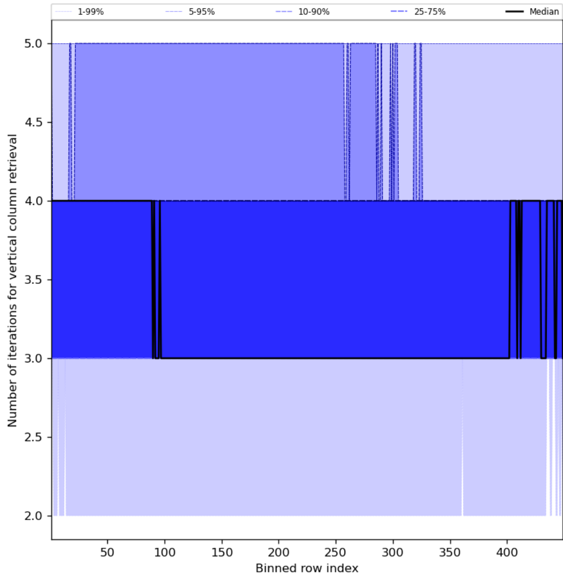
Figure 33: Along track statistics of “Number of iterations for vertical column retrieval” for 2023-08-06 to 2023-08-08
