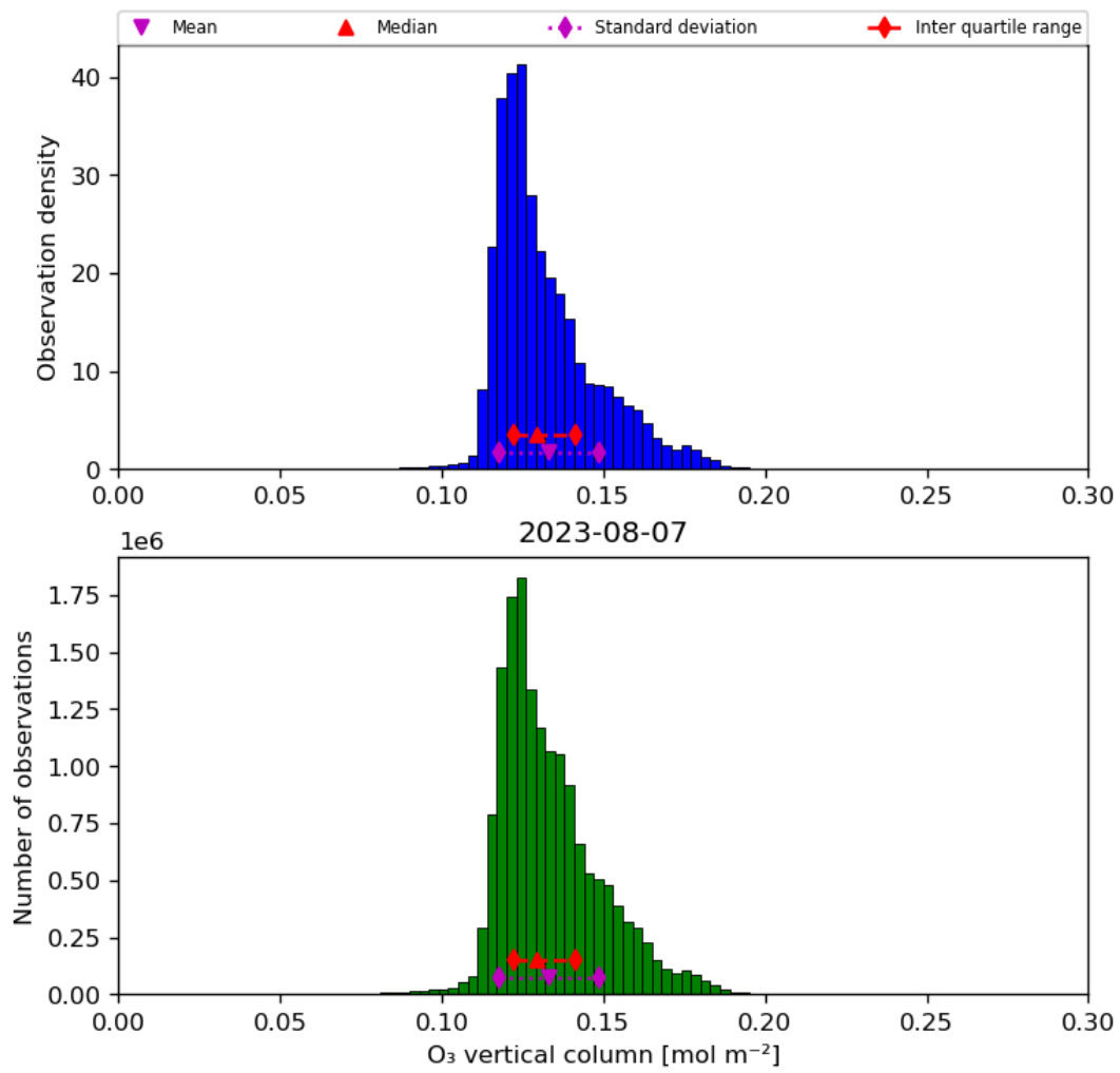
Figure 21: Histogram of “O 3 vertical column” for 2023-08-06 to 2023-08-08
