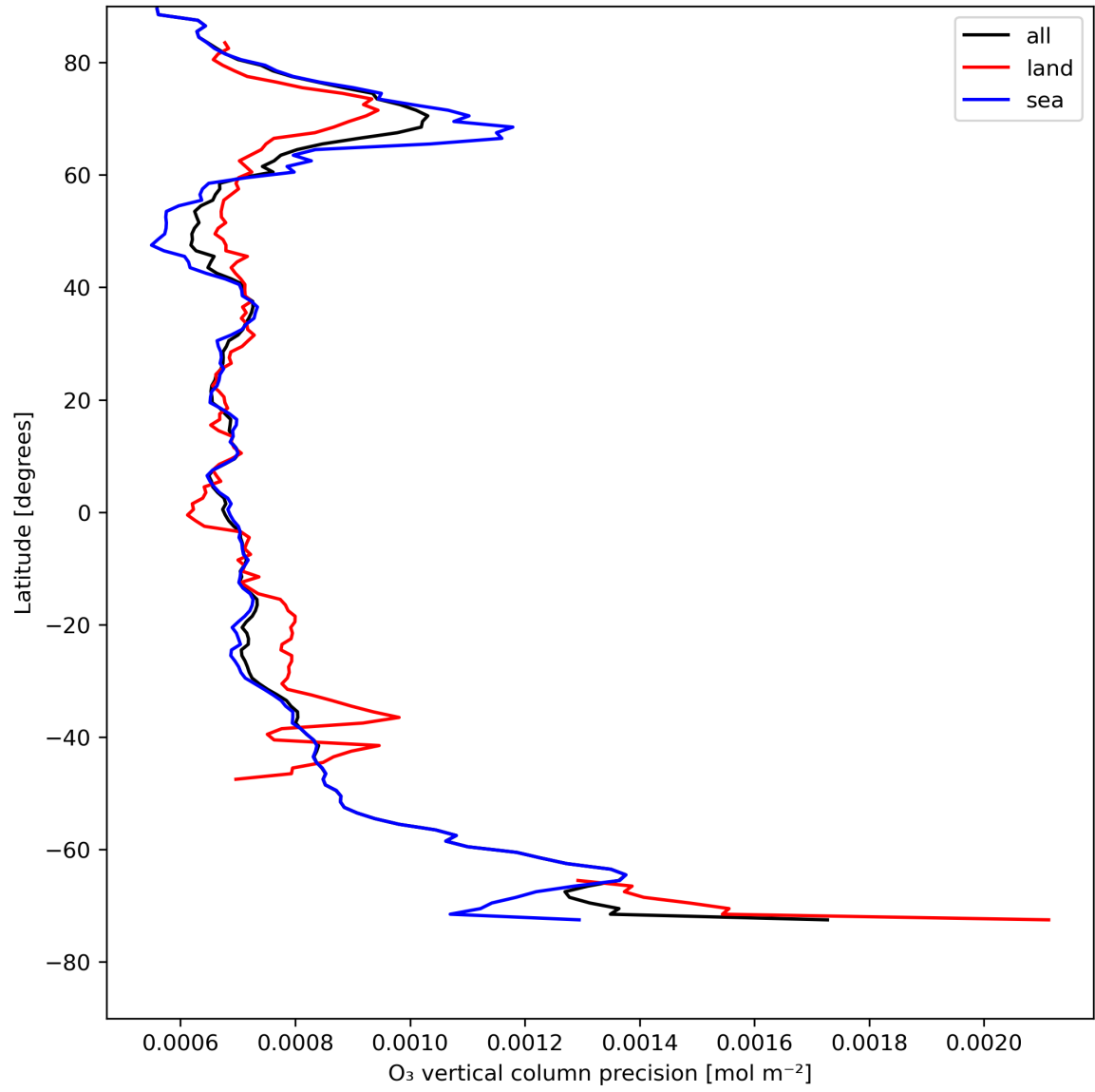
Figure 15: Zonal average of “O 3 vertical column precision” for 2023-08-06 to 2023-08-08.
