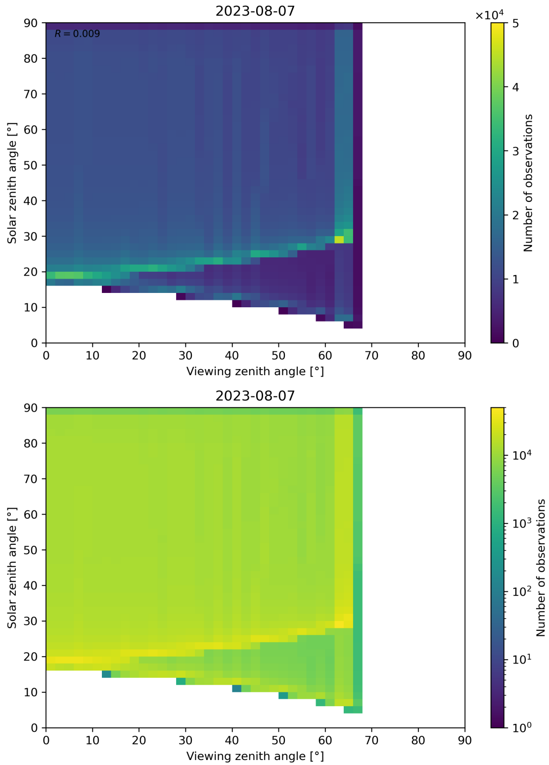
Figure 54: Scatter density plot of “Viewing zenith angle” against “Solar zenith angle” for 2023-08-06 to 2023-08-08.
