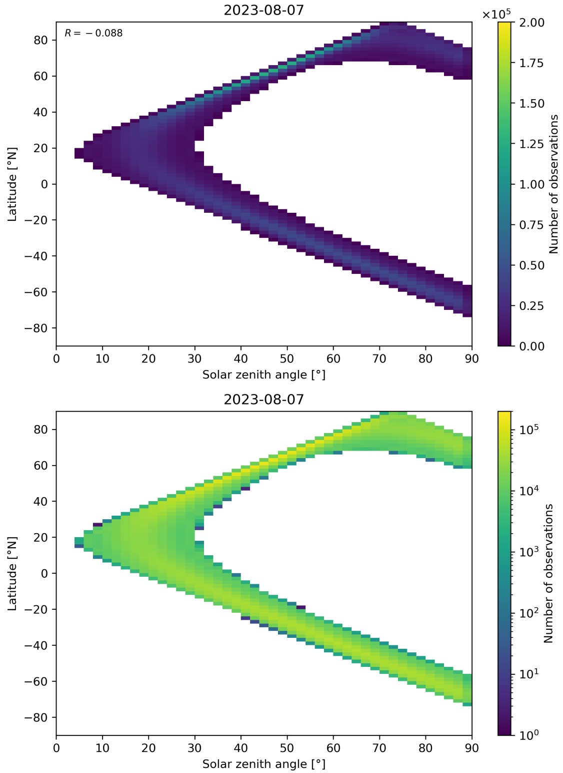
Figure 44: Scatter density plot of “Solar zenith angle” against “Latitude” for 2023-08-06 to 2023-08-08.
