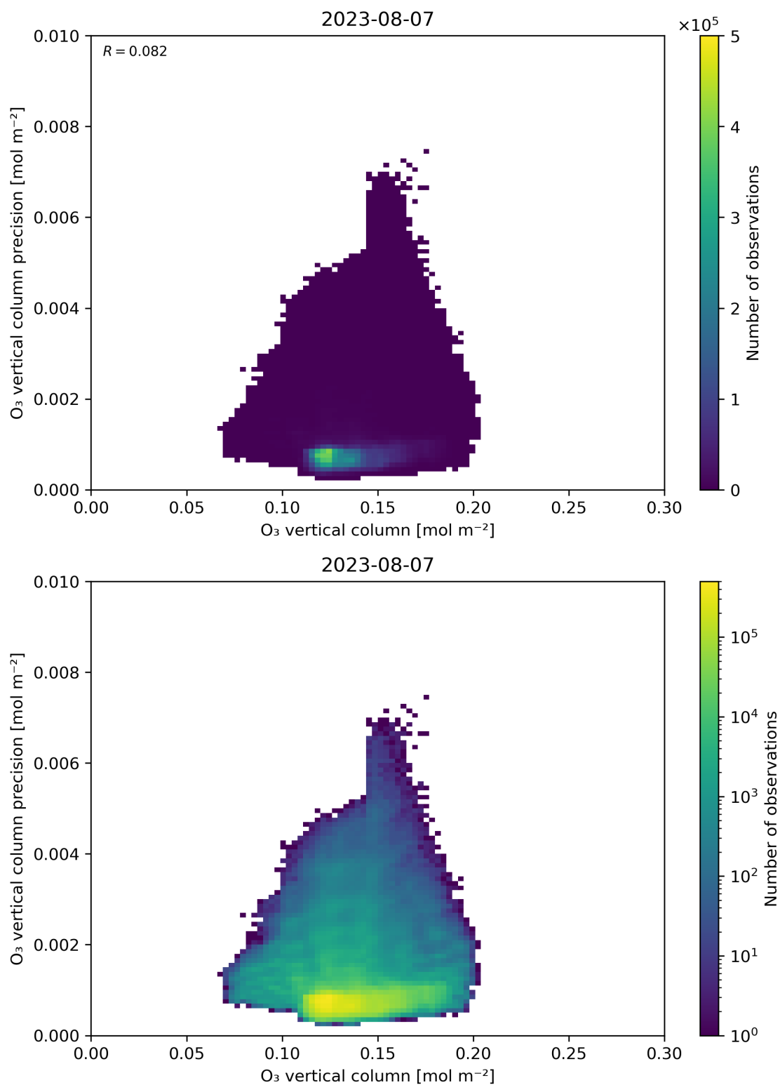
Figure 41: Scatter density plot of “O 3 vertical column” against “O 3 vertical column precision” for 2023-08-06 to 2023-08-08.
