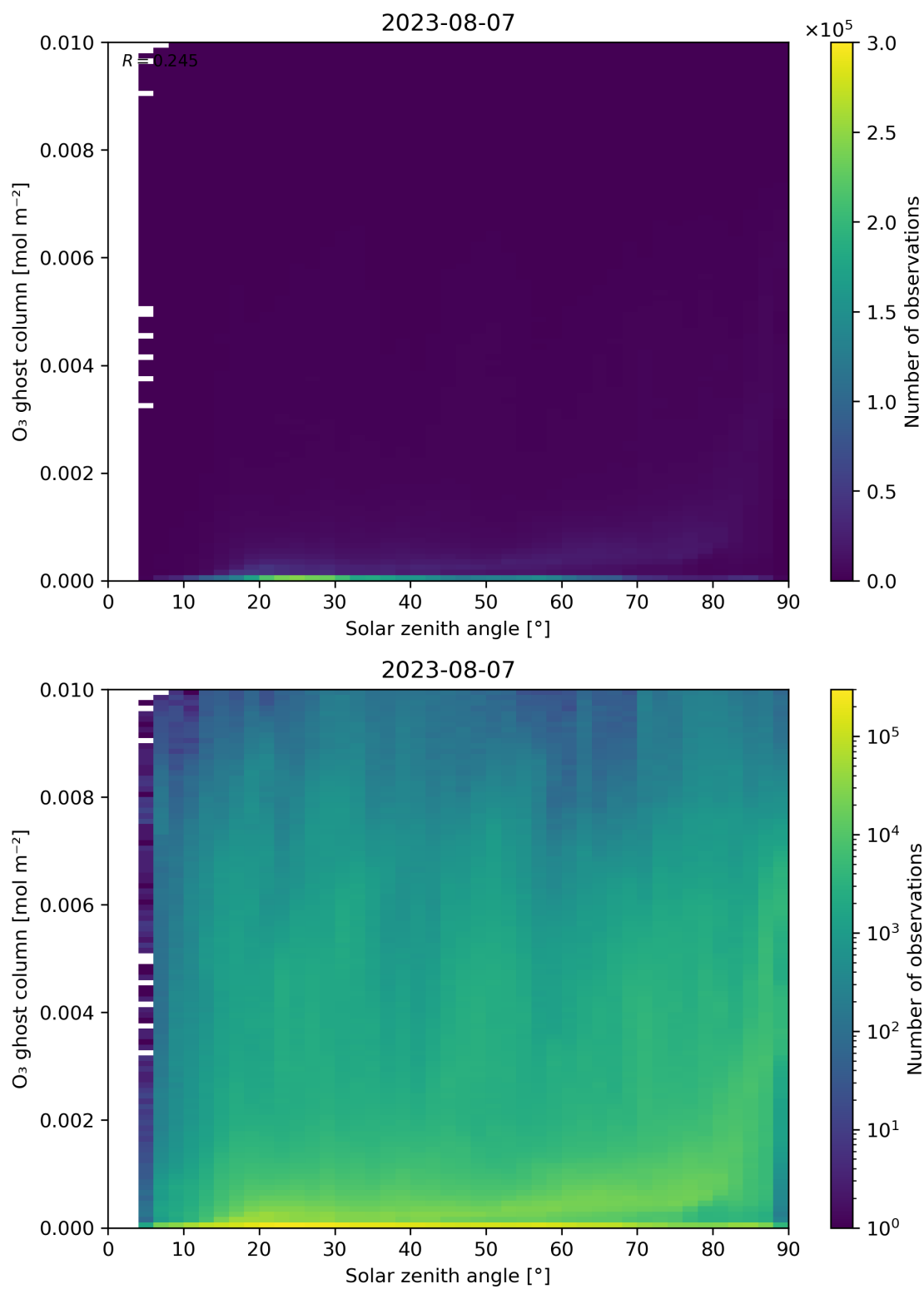
Figure 46: Scatter density plot of “Solar zenith angle” against “O 3 ghost column” for 2023-08-06 to 2023-08-08.
