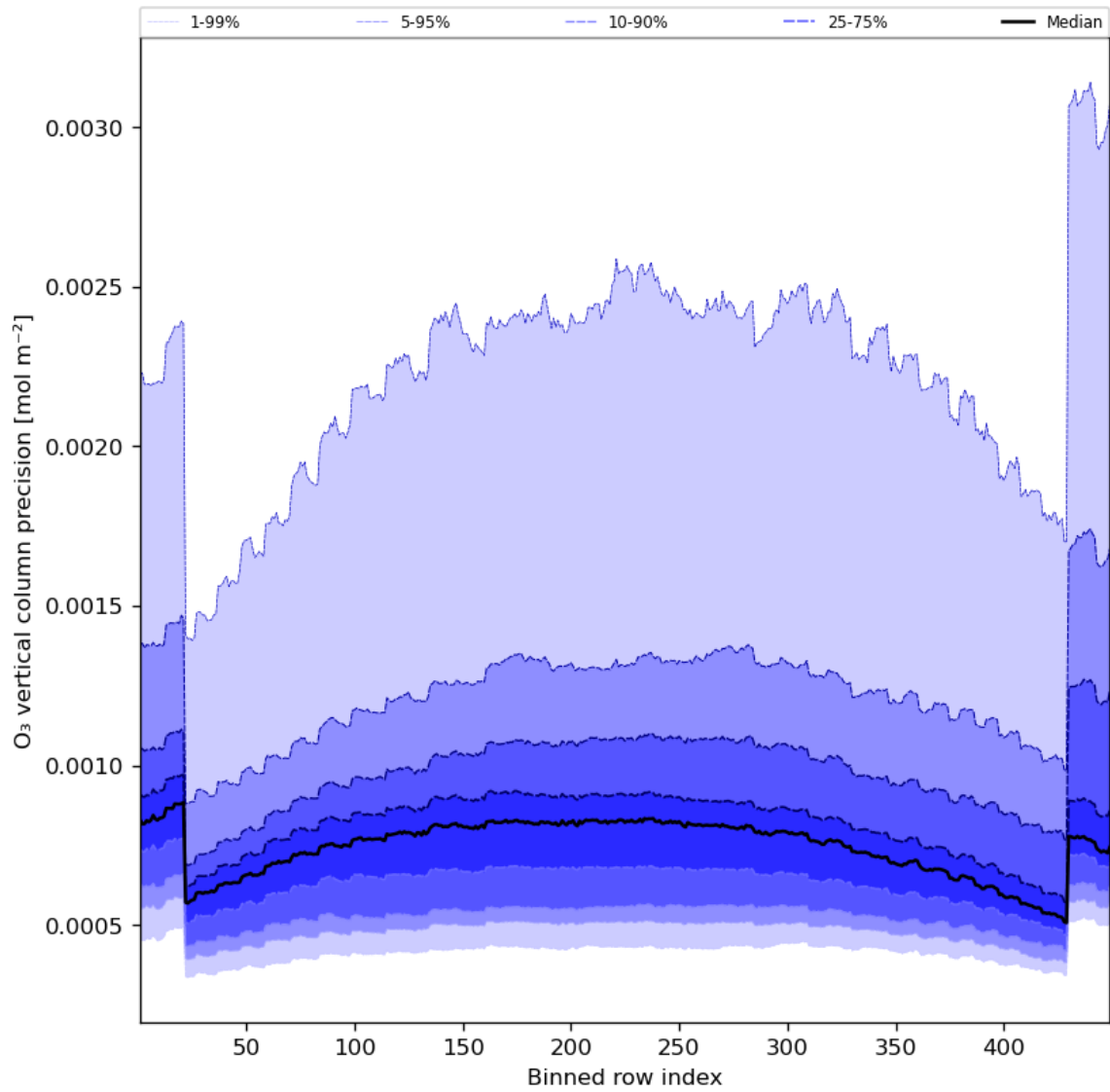
Figure 29: Along track statistics of “O 3 vertical column precision” for 2023-08-06 to 2023-08-08
