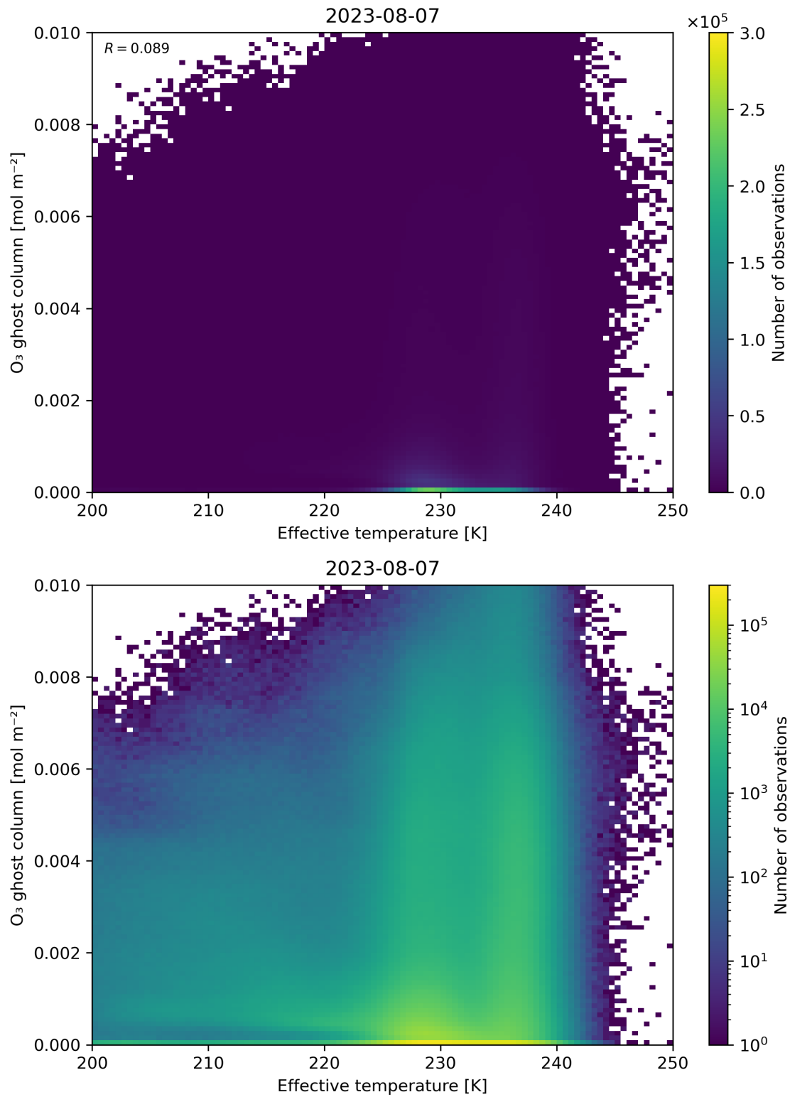
Figure 38: Scatter density plot of “Effective temperature” against “O 3 ghost column” for 2023-08-06 to 2023-08-08.
