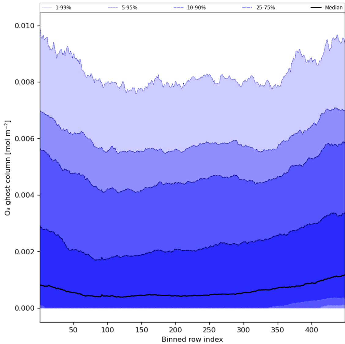
Figure 32: Along track statistics of “O 3 ghost column” for 2023-08-06 to 2023-08-08
