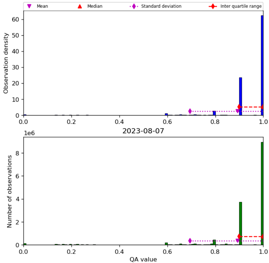
Figure 20: Histogram of “QA value” for 2023-08-06 to 2023-08-08
