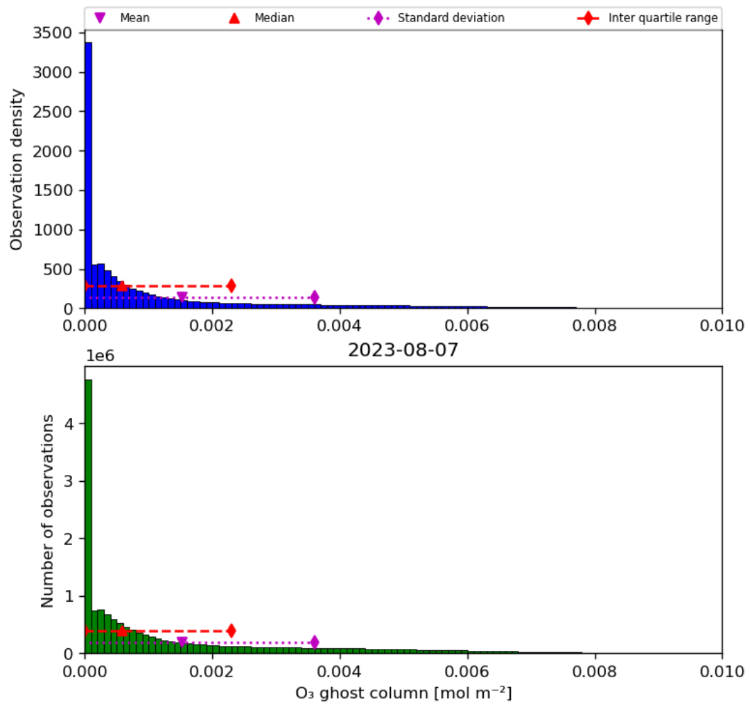
Figure 25: Histogram of "O 3 ghost column" for 2023-08-06 to 2023-08-08
