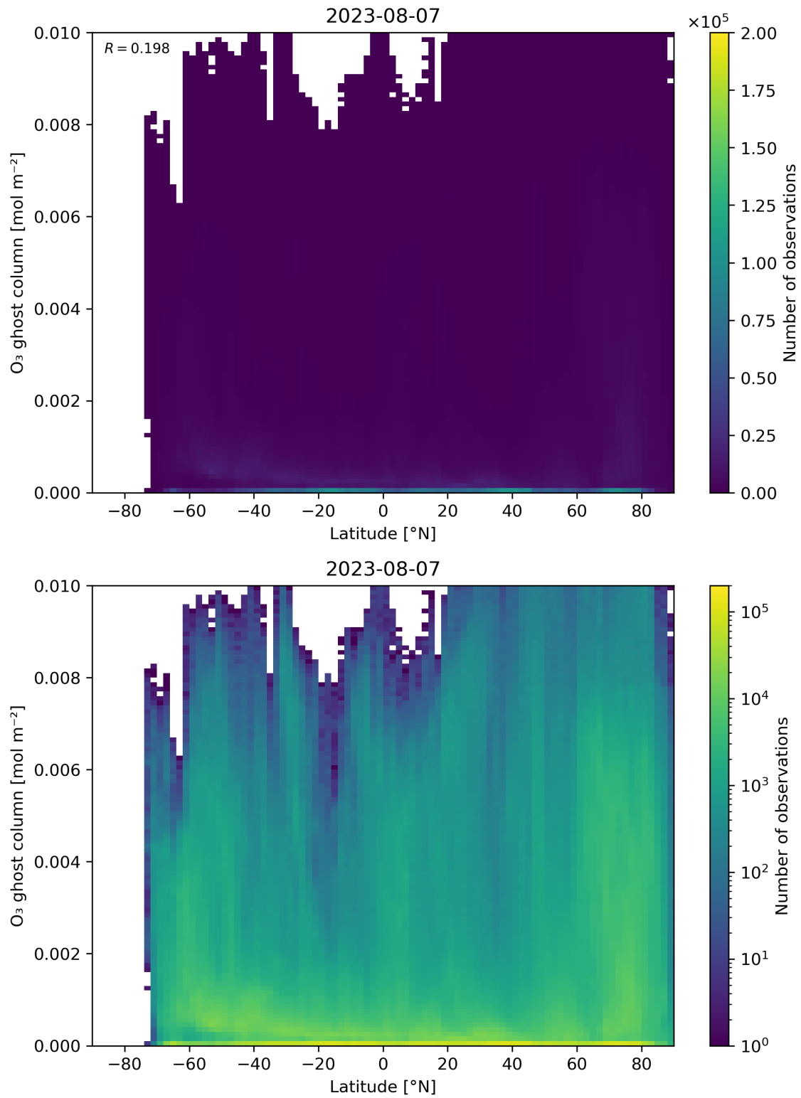
Figure 35: Scatter density plot of “Latitude” against “O 3 ghost column” for 2023-08-06 to 2023-08-08.
