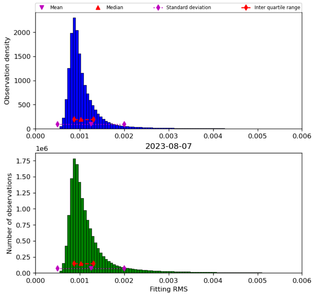
Figure 23: Histogram of “Fitting RMS” for 2023-08-06 to 2023-08-08
