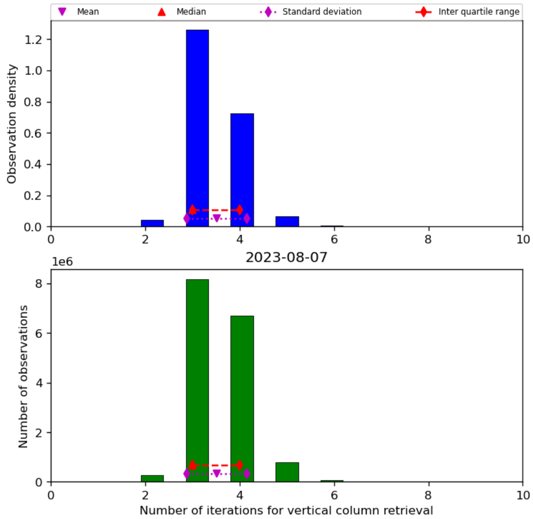
Figure 26: Histogram of “Number of iterations for vertical column retrieval” for 2023-08-06 to 2023-08-08
