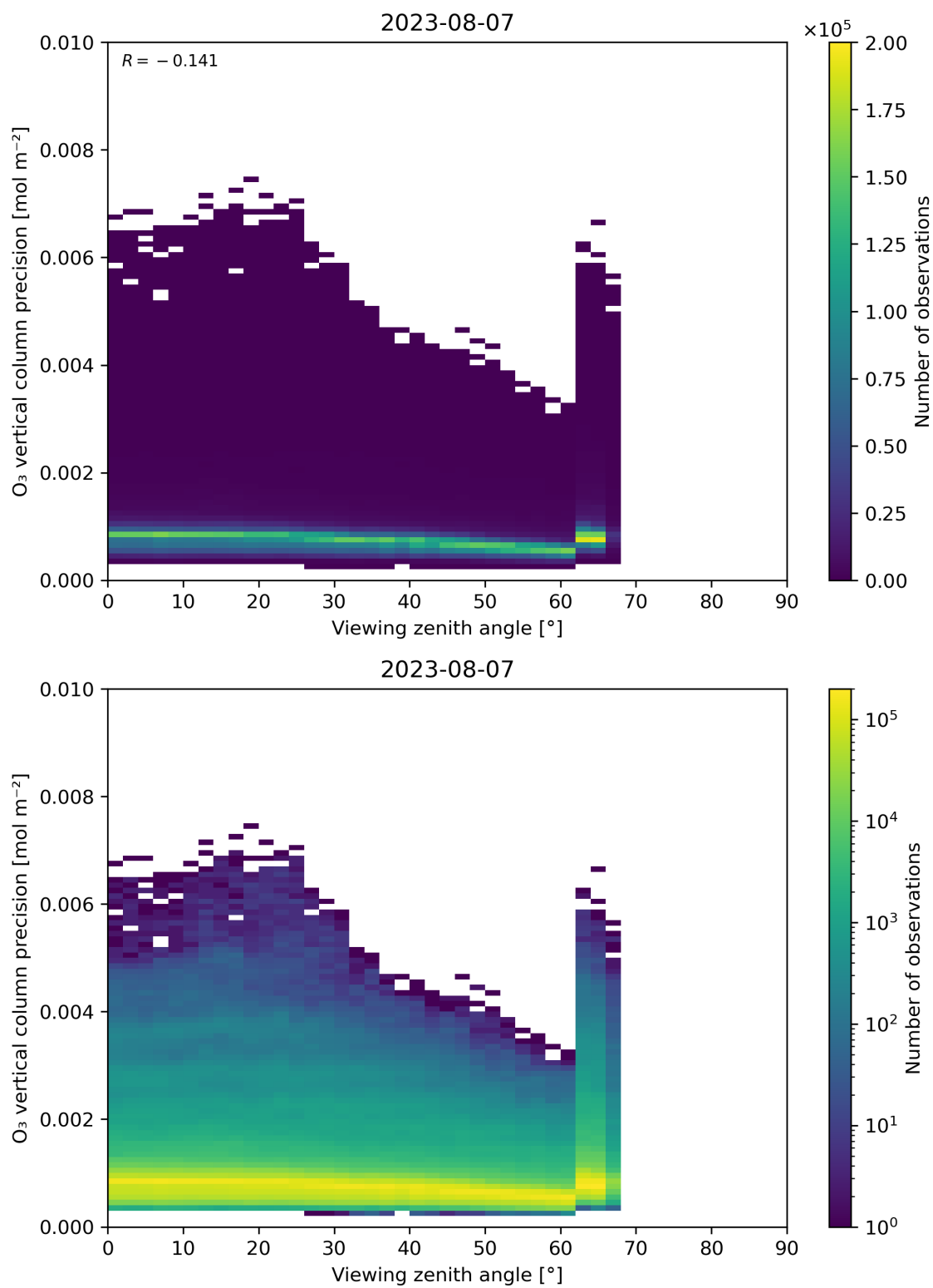
Figure 53: Scatter density plot of “Viewing zenith angle” against “O 3 vertical column precision” for 2023-08-06 to 2023-08-08.
