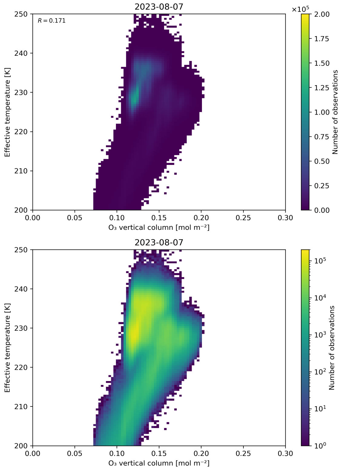
Figure 39: Scatter density plot of “O 3 vertical column” against “Effective temperature” for 2023-08-06 to 2023-08-08.
