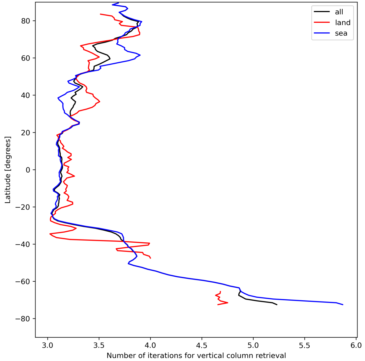
Figure 19: Zonal average of “Number of iterations for vertical column retrieval” for 2023-08-06 to 2023-08-08.
