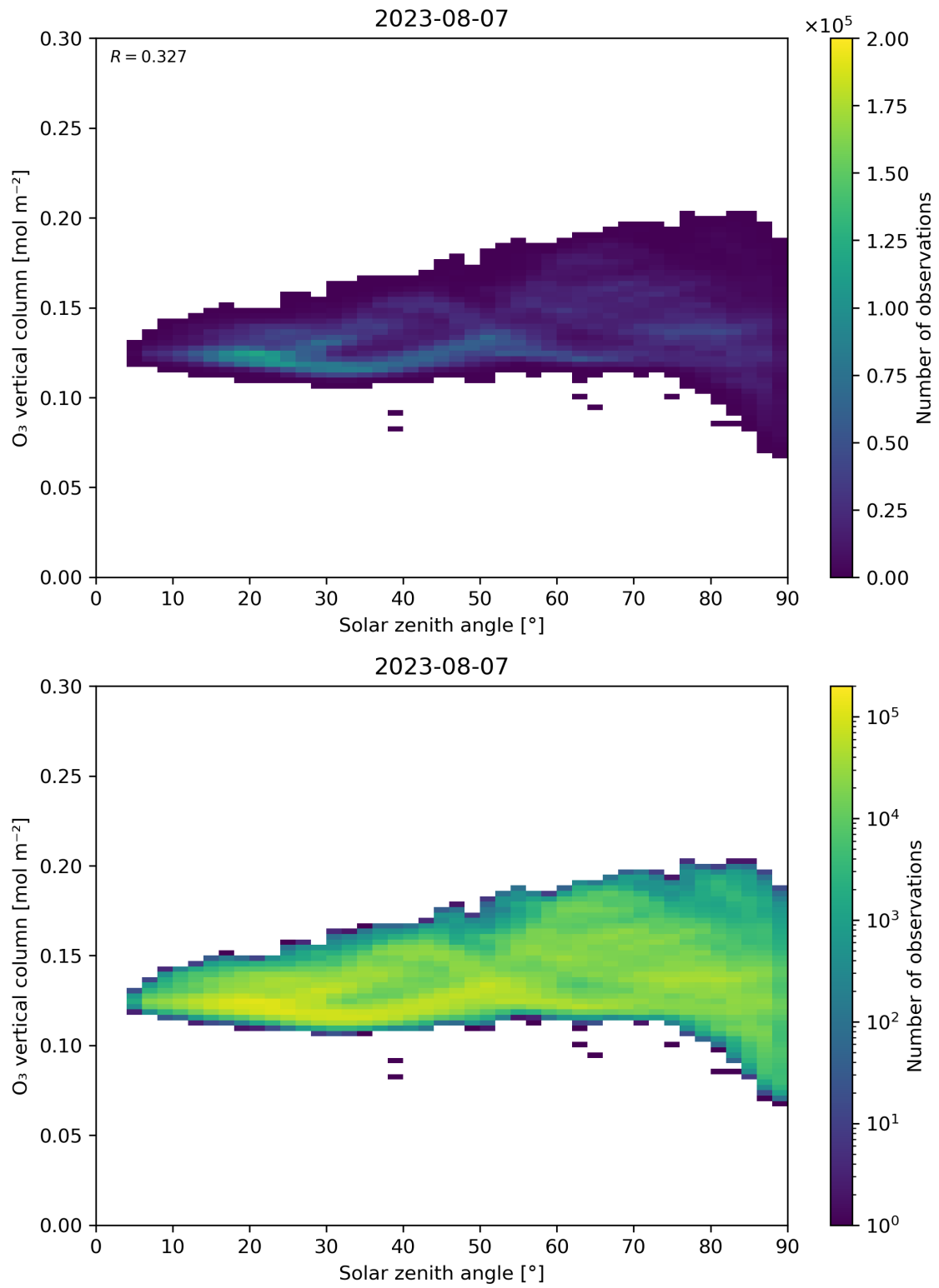
Figure 47: Scatter density plot of “Solar zenith angle” against “O 3 vertical column” for 2023-08-06 to 2023-08-08.
