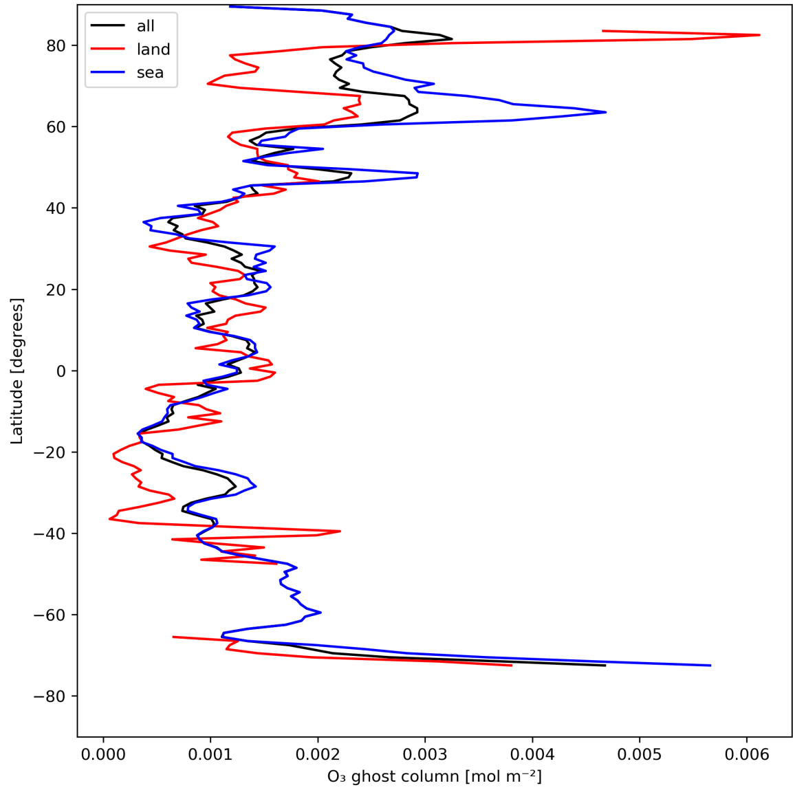
Figure 18: Zonal average of “O 3 ghost column” for 2023-08-06 to 2023-08-08.
