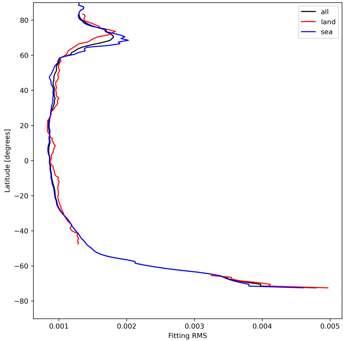
Figure 16: Zonal average of “Fitting RMS” for 2023-08-06 to 2023-08-08.
