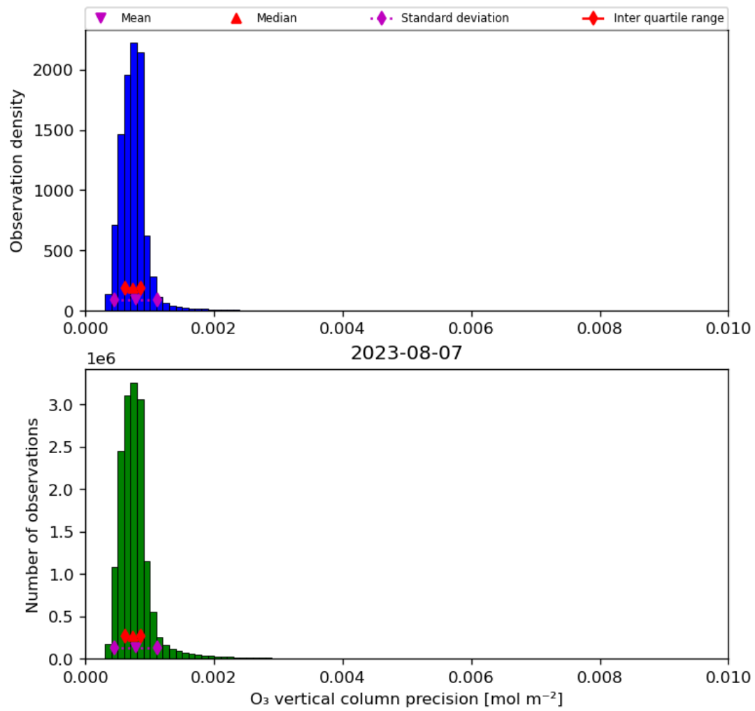
Figure 22: Histogram of “O 3 vertical column precision” for 2023-08-06 to 2023-08-08
