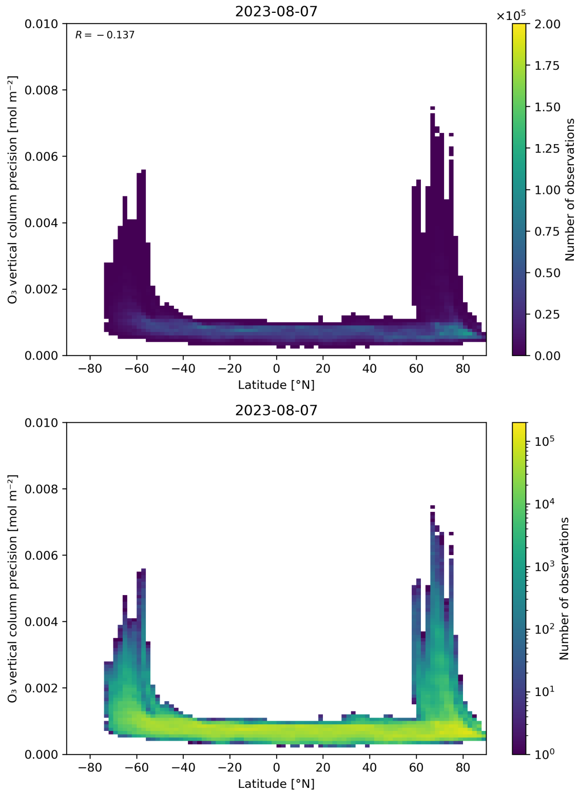
Figure 37: Scatter density plot of “Latitude” against “O 3 vertical column precision” for 2023-08-06 to 2023-08-08.
