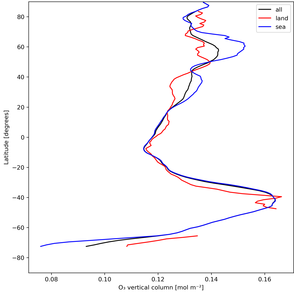
Figure 14: Zonal average of “O 3 vertical column” for 2023-08-06 to 2023-08-08.
