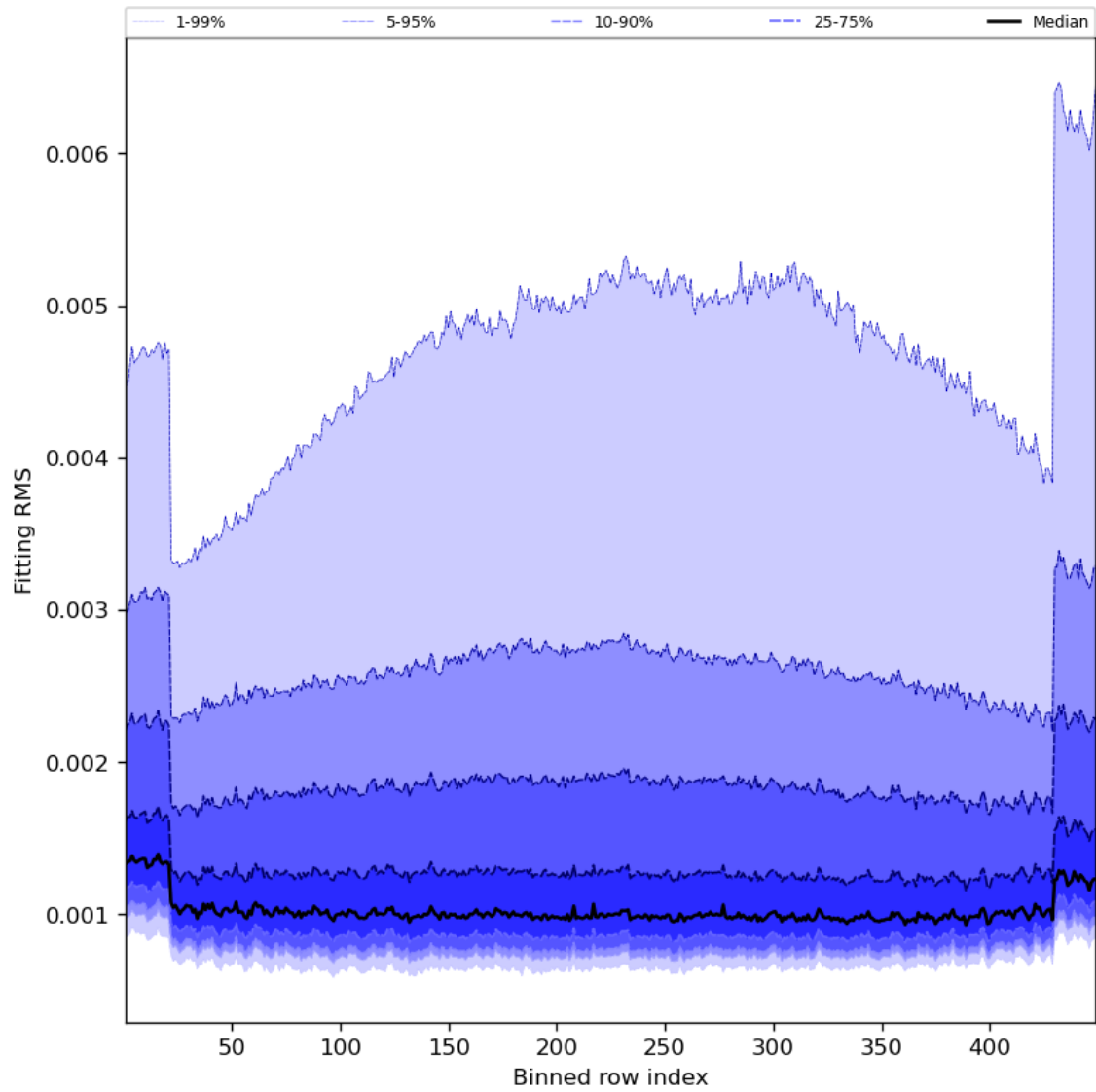
Figure 30: Along track statistics of “Fitting RMS” for 2023-08-06 to 2023-08-08
