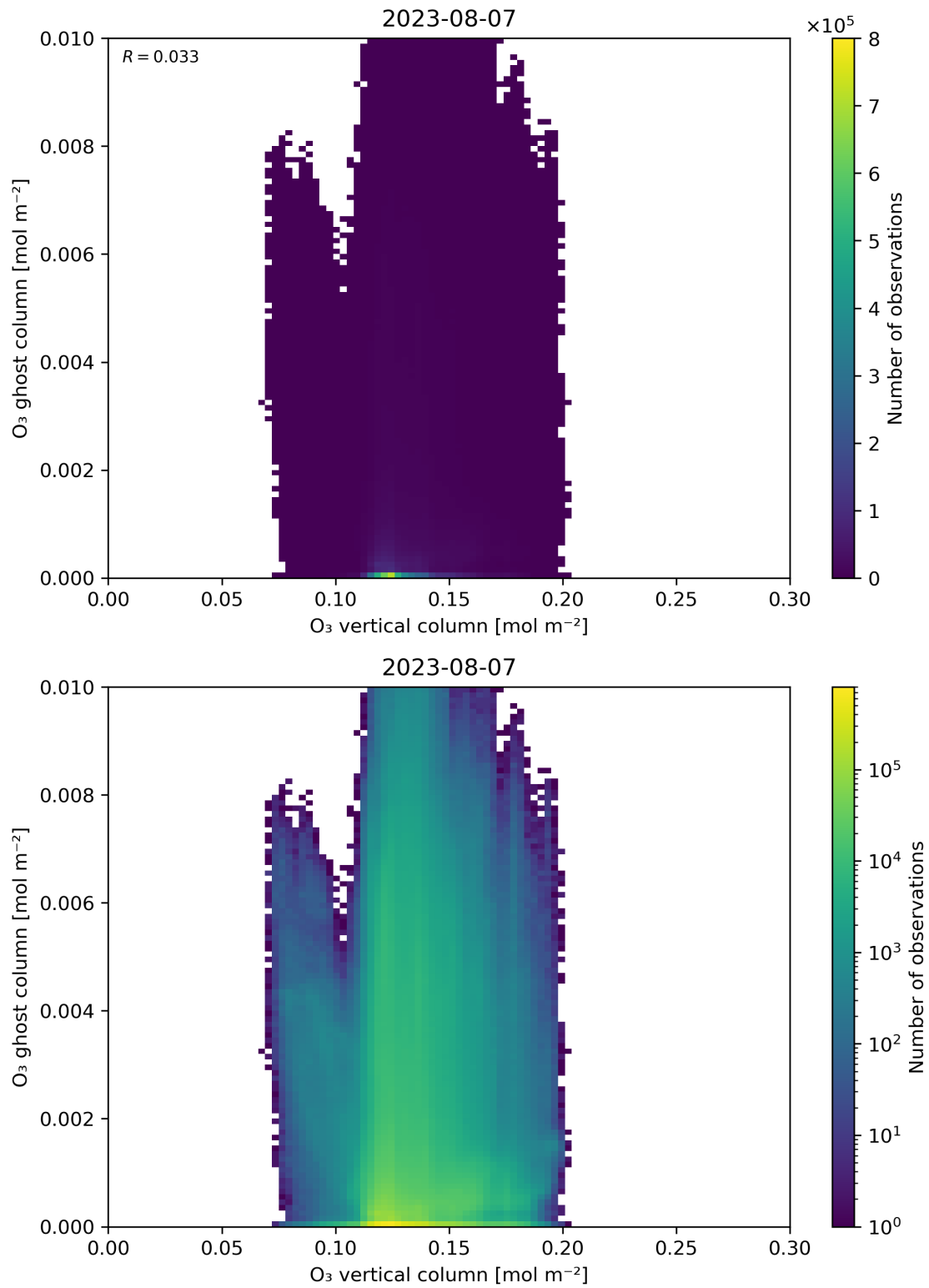
Figure 40: Scatter density plot of “O 3 vertical column” against “O 3 ghost column” for 2023-08-06 to 2023-08-08.
