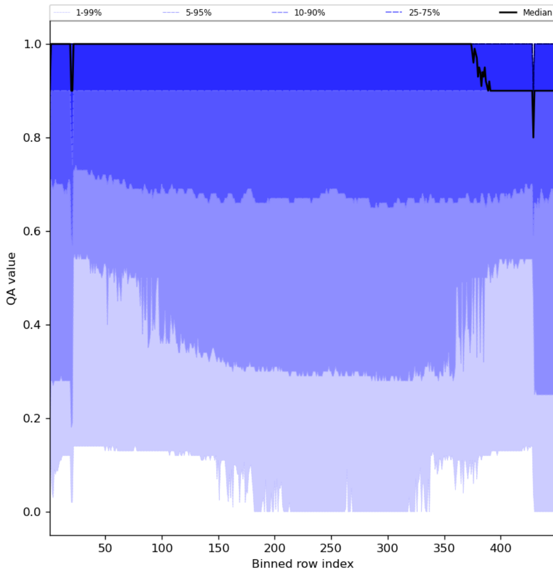
Figure 27: Along track statistics of “QA value” for 2023-08-06 to 2023-08-08
