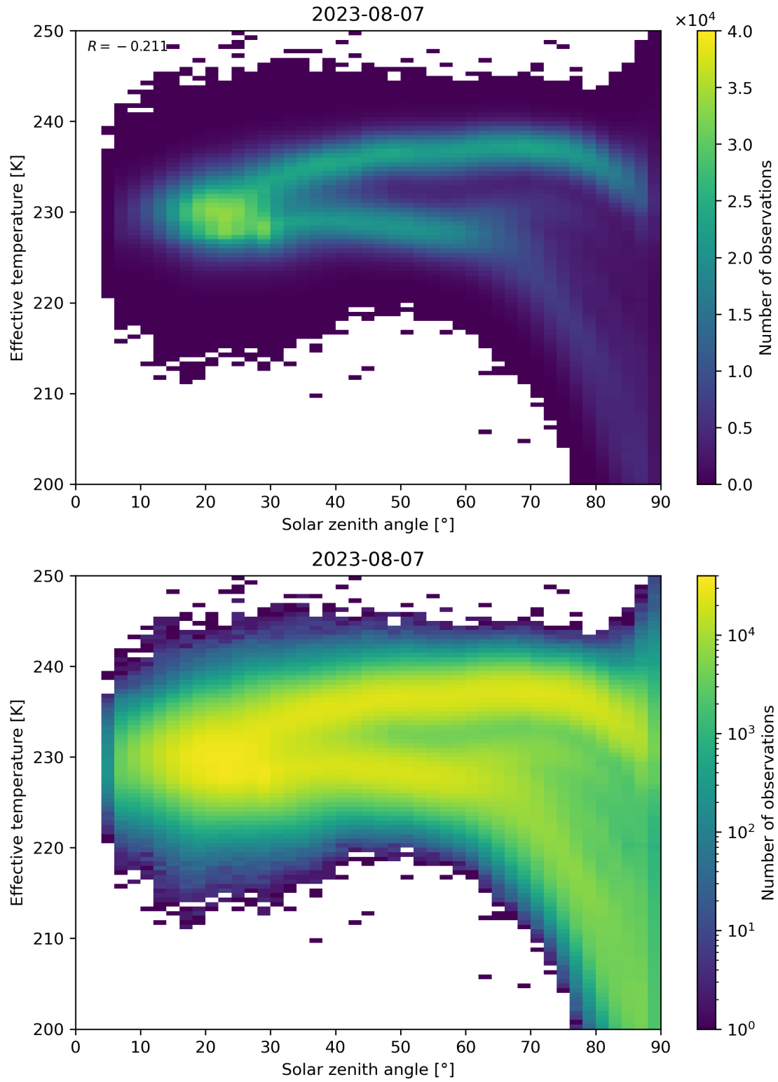
Figure 45: Scatter density plot of “Solar zenith angle” against “Effective temperature” for 2023-08-06 to 2023-08-08.
