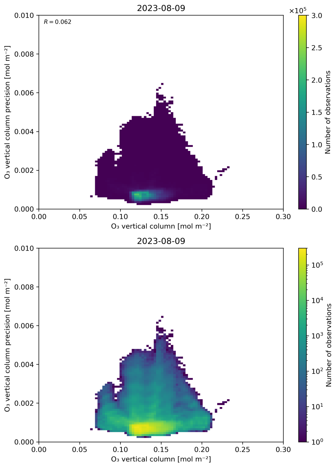
Figure 41: Scatter density plot of “O 3 vertical column” against “O 3 vertical column precision” for 2023-08-09 to 2023-08-10.
