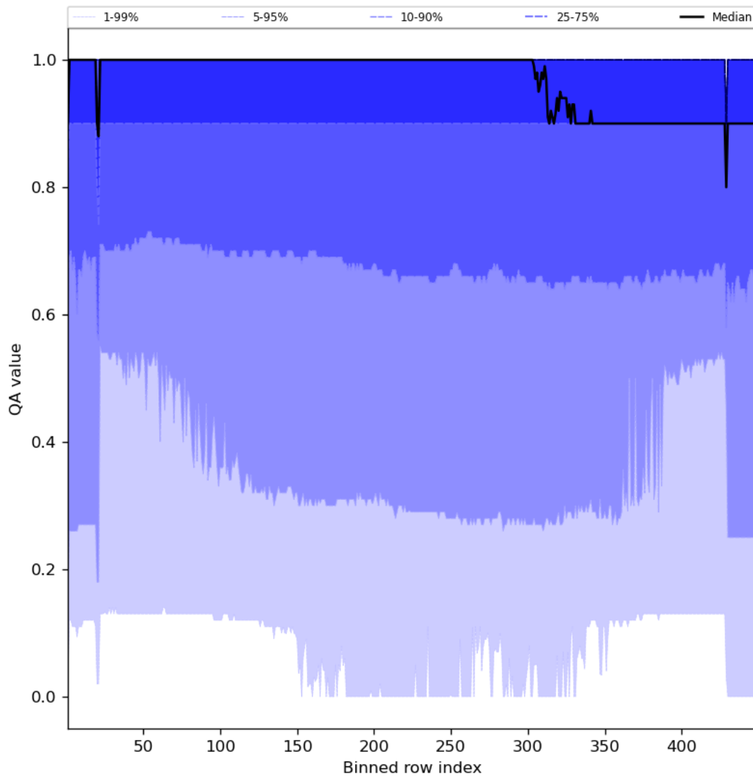
Figure 27: Along track statistics of “QA value” for 2023-08-09 to 2023-08-10
