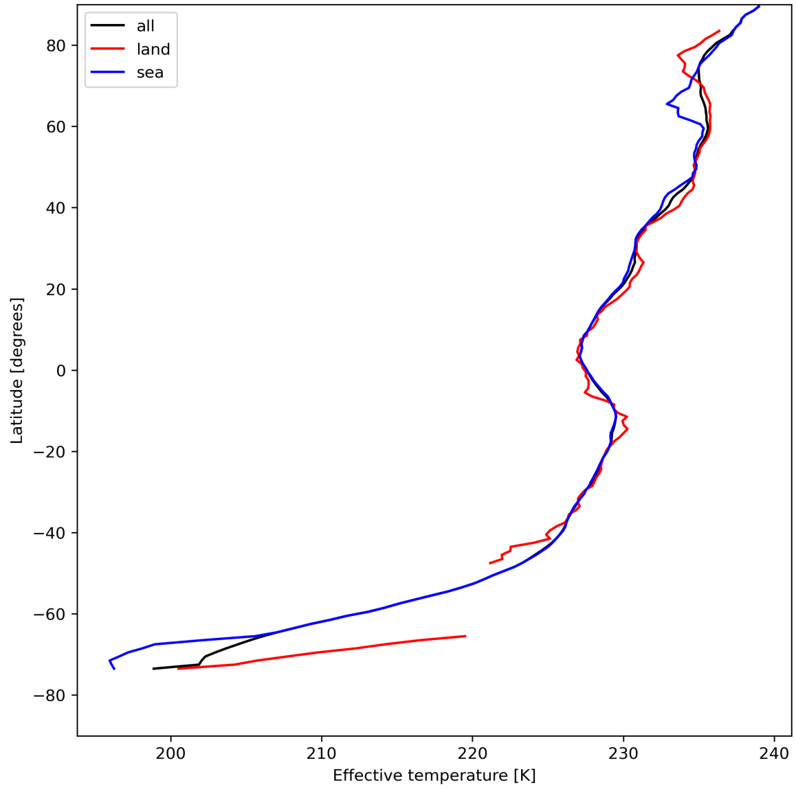
Figure 17: Zonal average of "Effective temperature" for 2023-08-09 to 2023-08-10.
