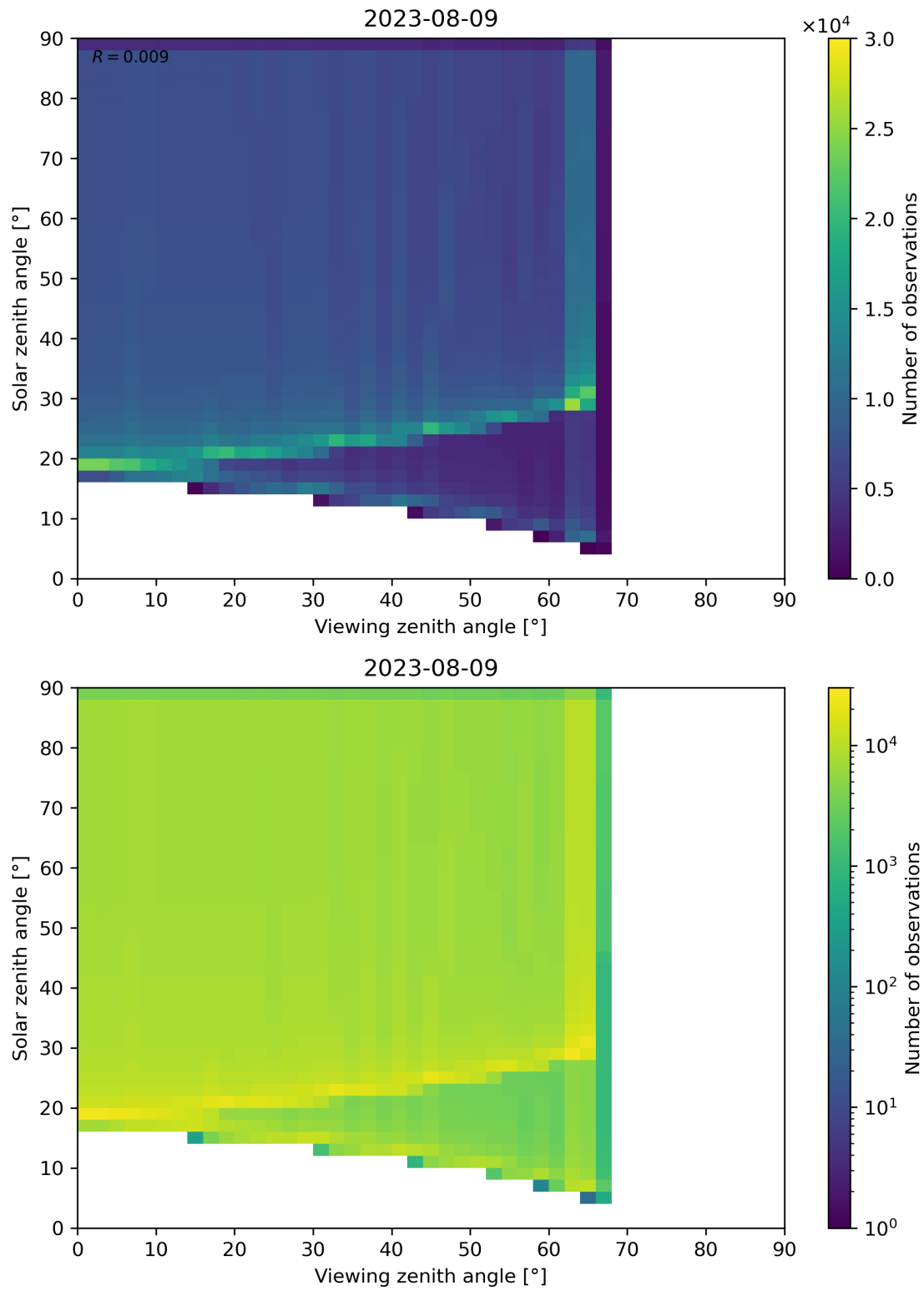
Figure 54: Scatter density plot of “Viewing zenith angle” against “Solar zenith angle” for 2023-08-09 to 2023-08-10.
