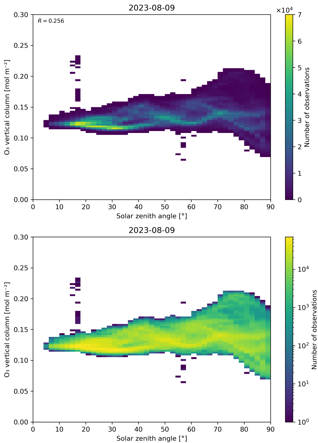
Figure 47: Scatter density plot of “Solar zenith angle” against “O 3 vertical column” for 2023-08-09 to 2023-08-10.
