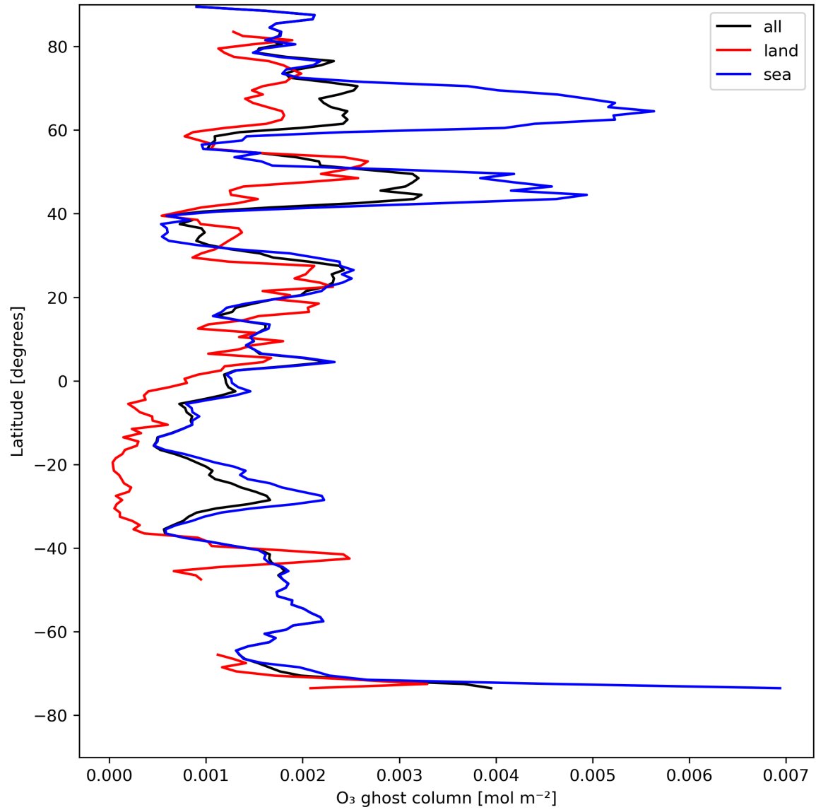
Figure 18: Zonal average of “O 3 ghost column” for 2023-08-09 to 2023-08-10.
