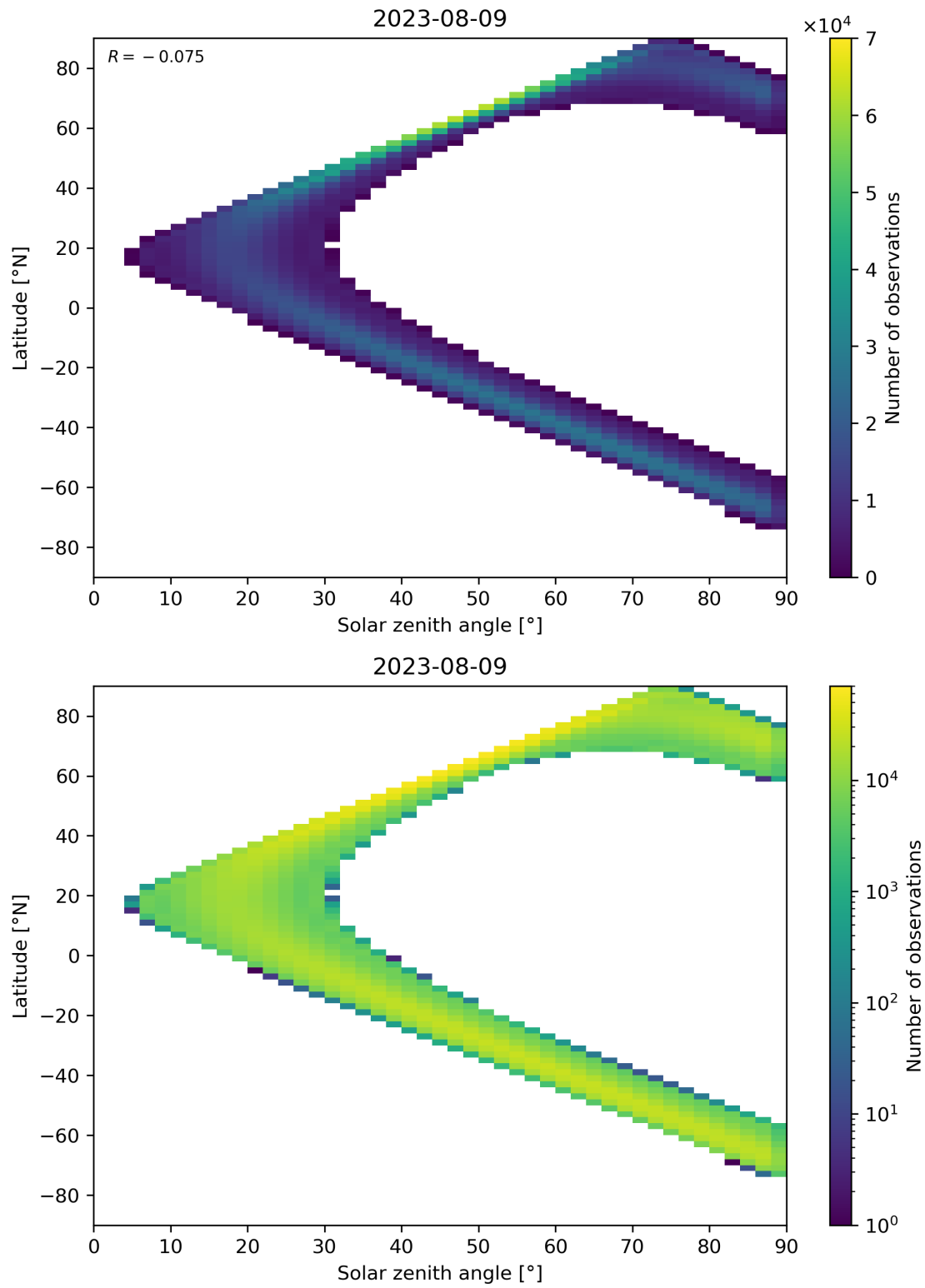
Figure 44: Scatter density plot of “Solar zenith angle” against “Latitude” for 2023-08-09 to 2023-08-10.
