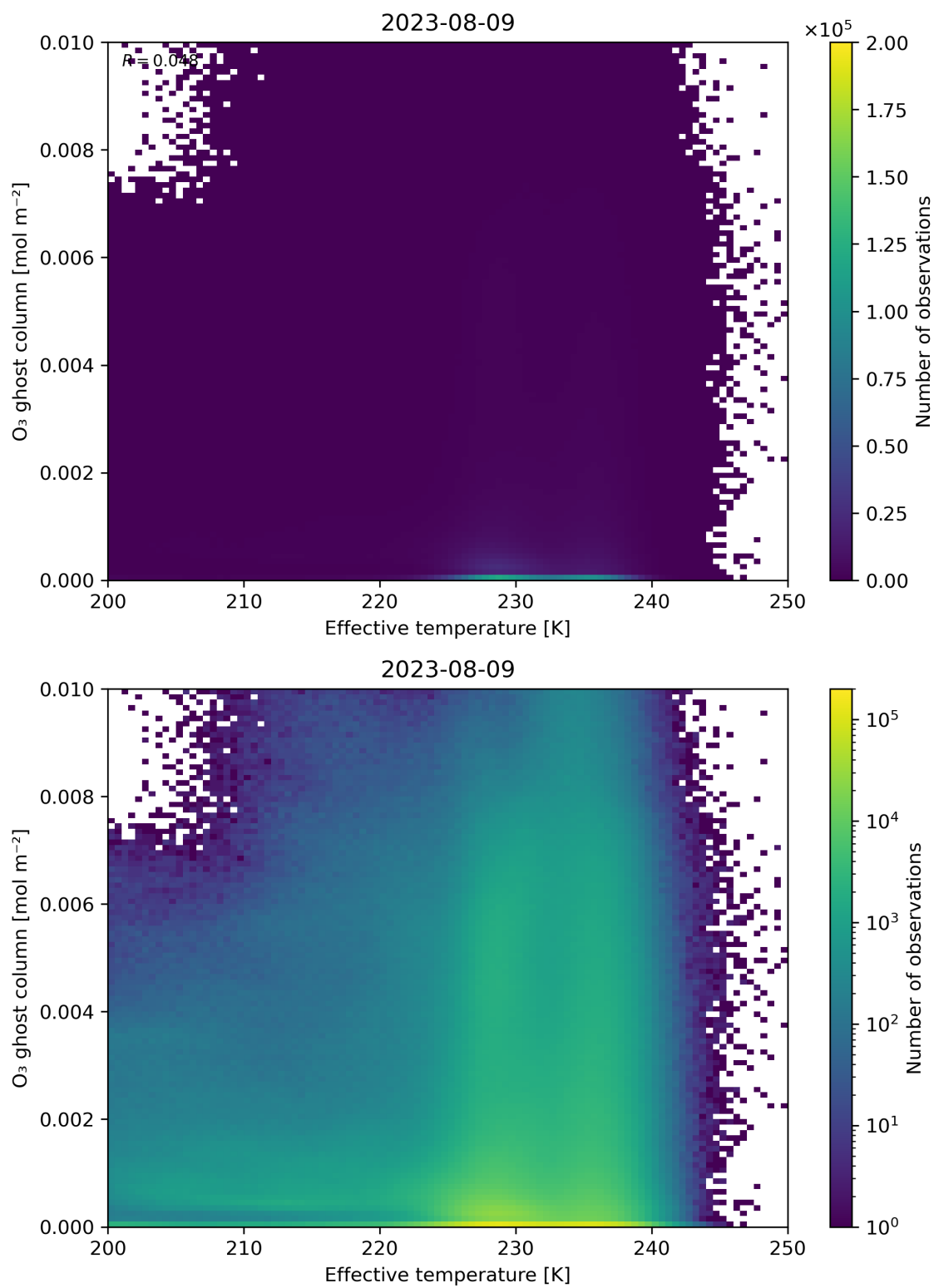
Figure 38: Scatter density plot of “Effective temperature” against “O 3 ghost column” for 2023-08-09 to 2023-08-10.
