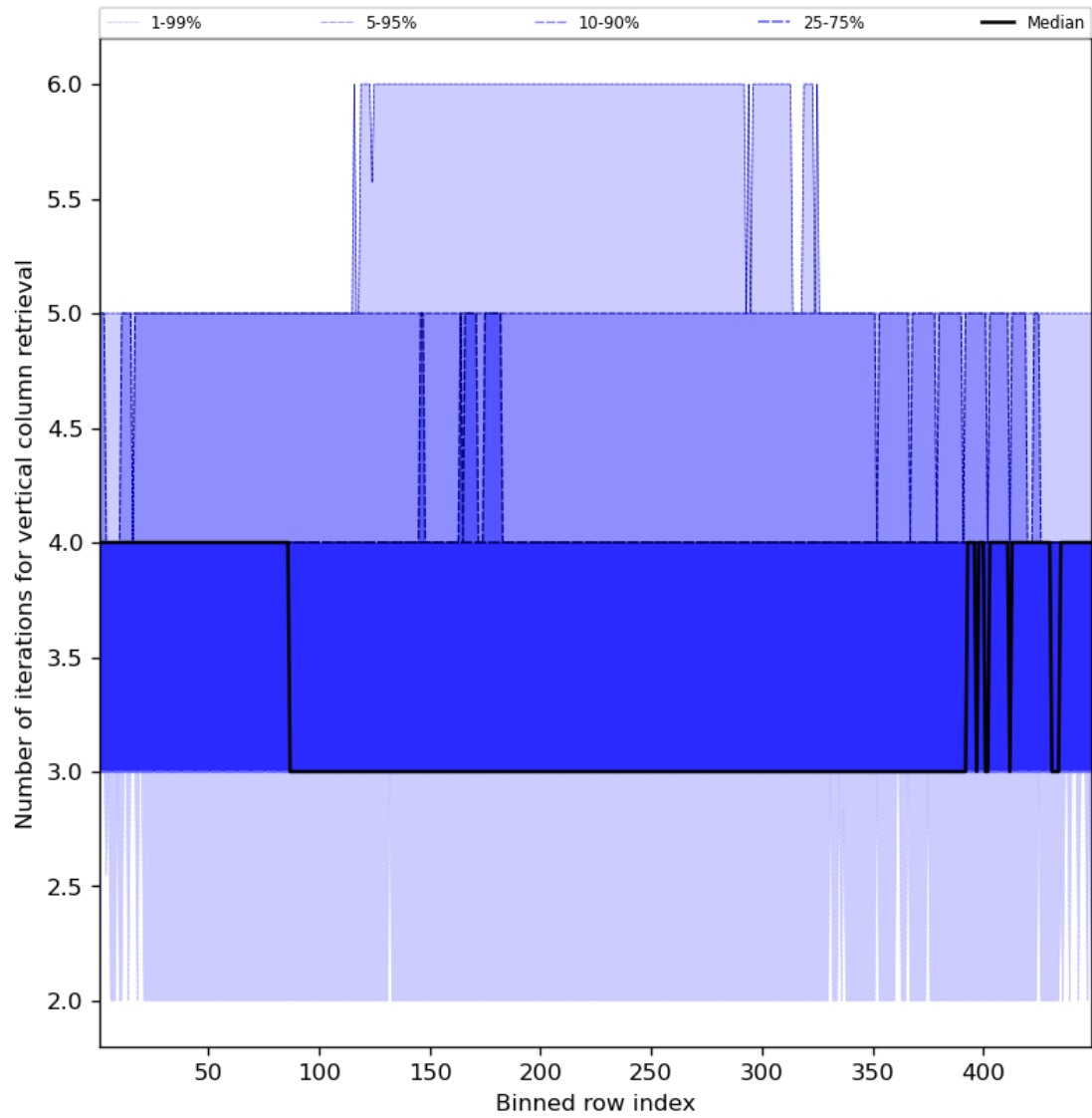
Figure 33: Along track statistics of “Number of iterations for vertical column retrieval” for 2023-08-09 to 2023-08-10
