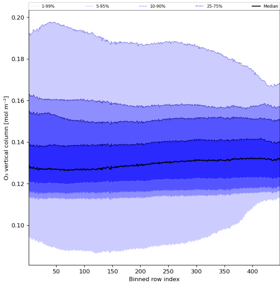
Figure 28: Along track statistics of “O 3 vertical column” for 2023-08-09 to 2023-08-10
