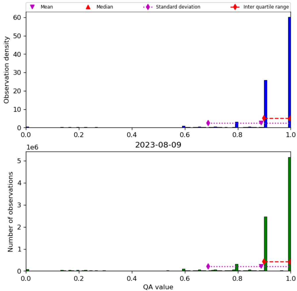
Figure 20: Histogram of “QA value” for 2023-08-09 to 2023-08-10
