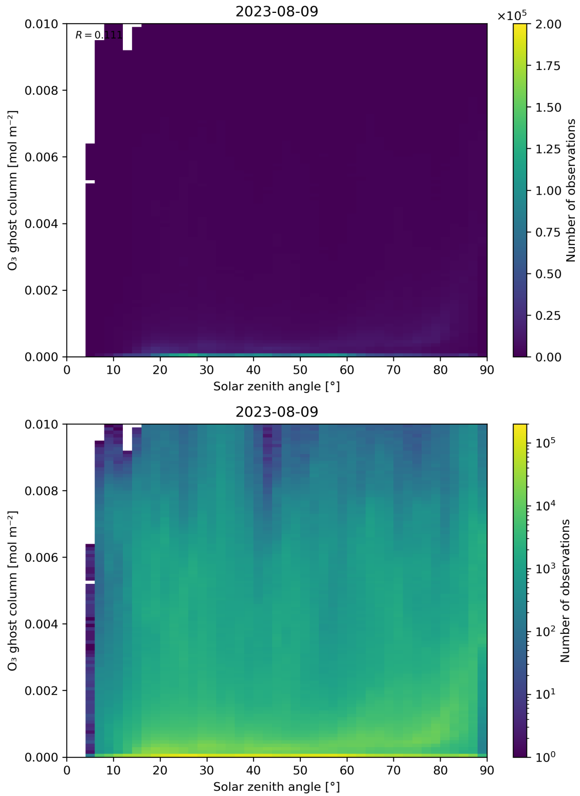
Figure 46: Scatter density plot of “Solar zenith angle” against “O 3 ghost column” for 2023-08-09 to 2023-08-10.
