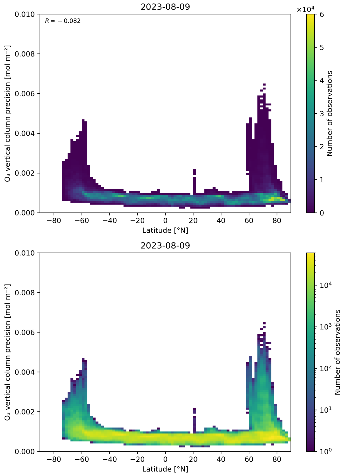
Figure 37: Scatter density plot of “Latitude” against “O 3 vertical column precision” for 2023-08-09 to 2023-08-10.
