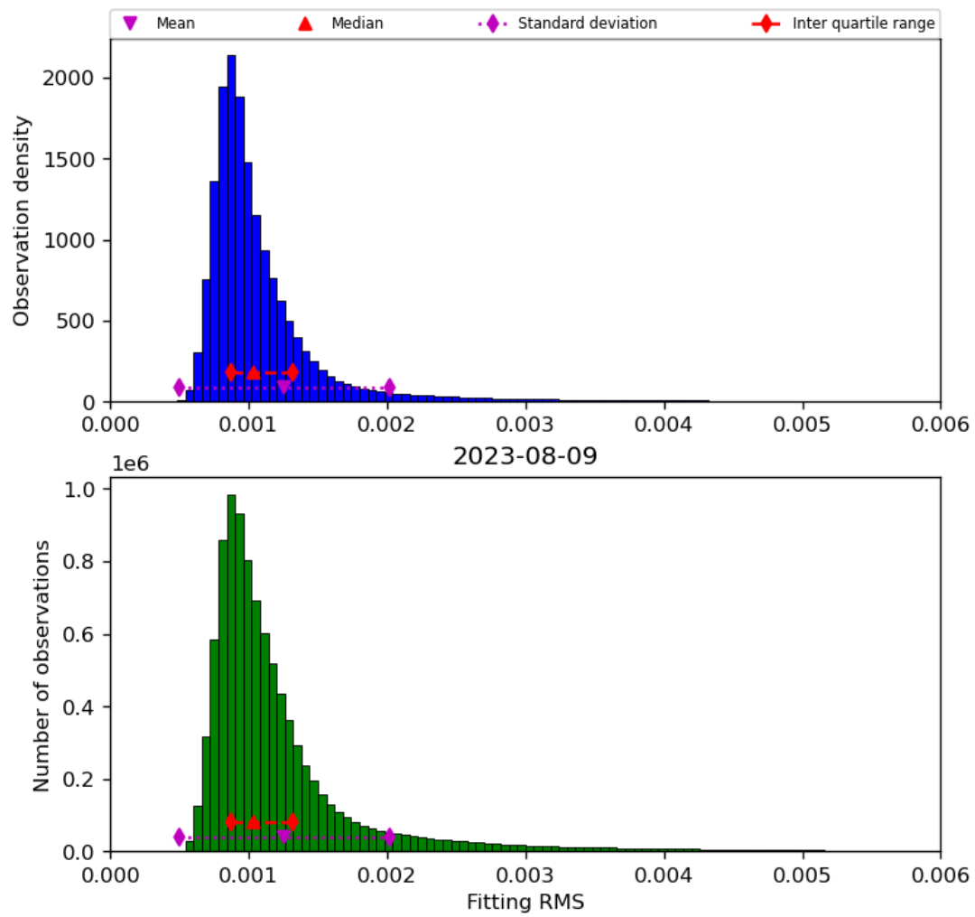
Figure 23: Histogram of “Fitting RMS” for 2023-08-09 to 2023-08-10
