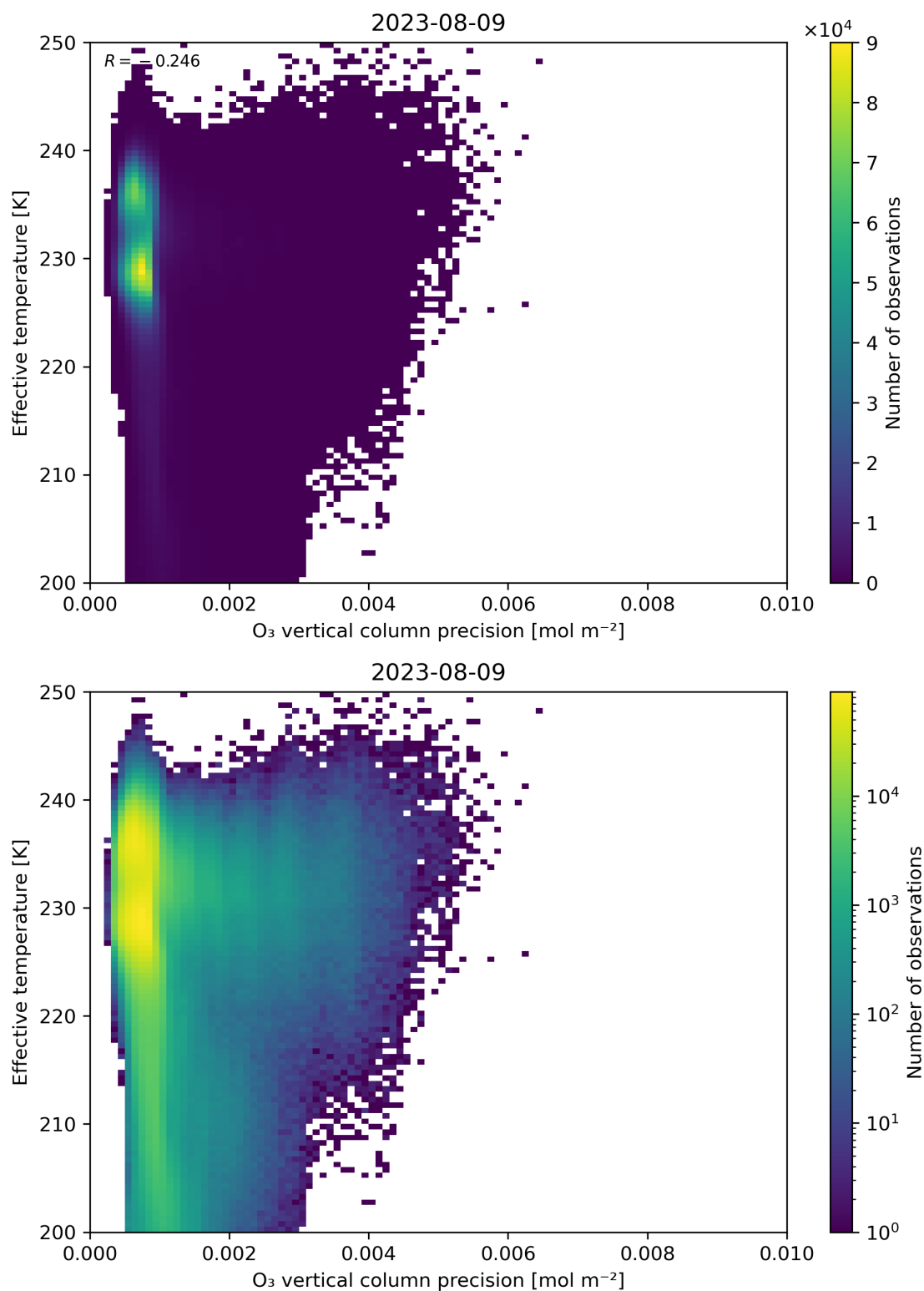
Figure 42: Scatter density plot of “O 3 vertical column precision” against “Effective temperature” for 2023-08-09 to 2023-08-10.
