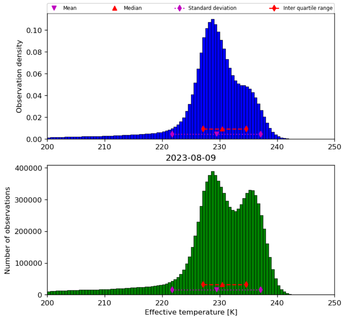
Figure 24: Histogram of “Effective temperature” for 2023-08-09 to 2023-08-10
