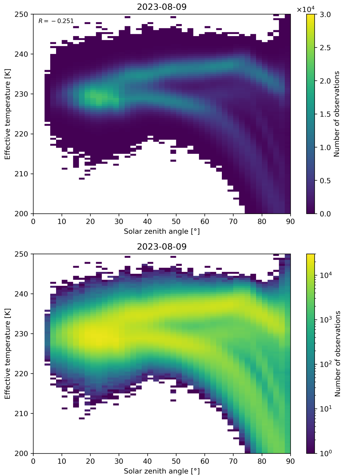
Figure 45: Scatter density plot of “Solar zenith angle” against “Effective temperature” for 2023-08-09 to 2023-08-10.
