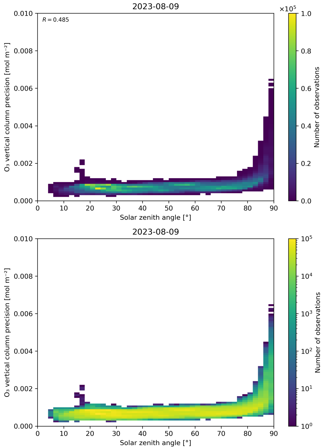
Figure 48: Scatter density plot of “Solar zenith angle” against “O 3 vertical column precision” for 2023-08-09 to 2023-08-10.
