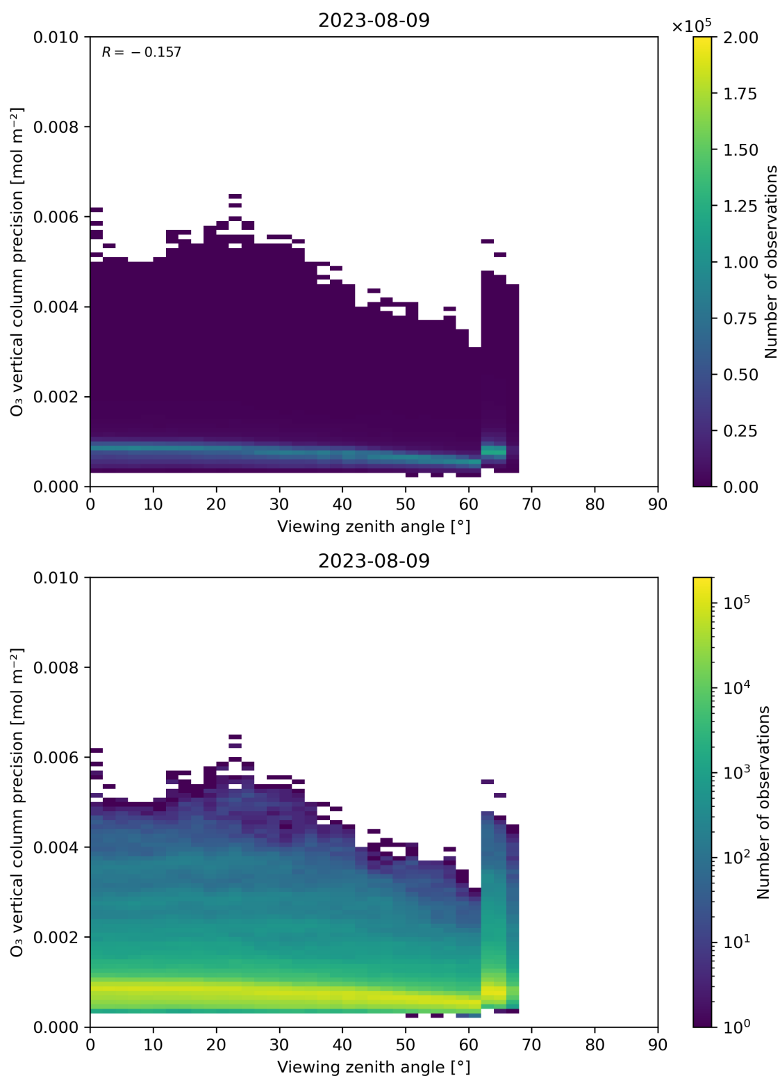
Figure 53: Scatter density plot of “Viewing zenith angle” against “O 3 vertical column precision” for 2023-08-09 to 2023-08-10.
