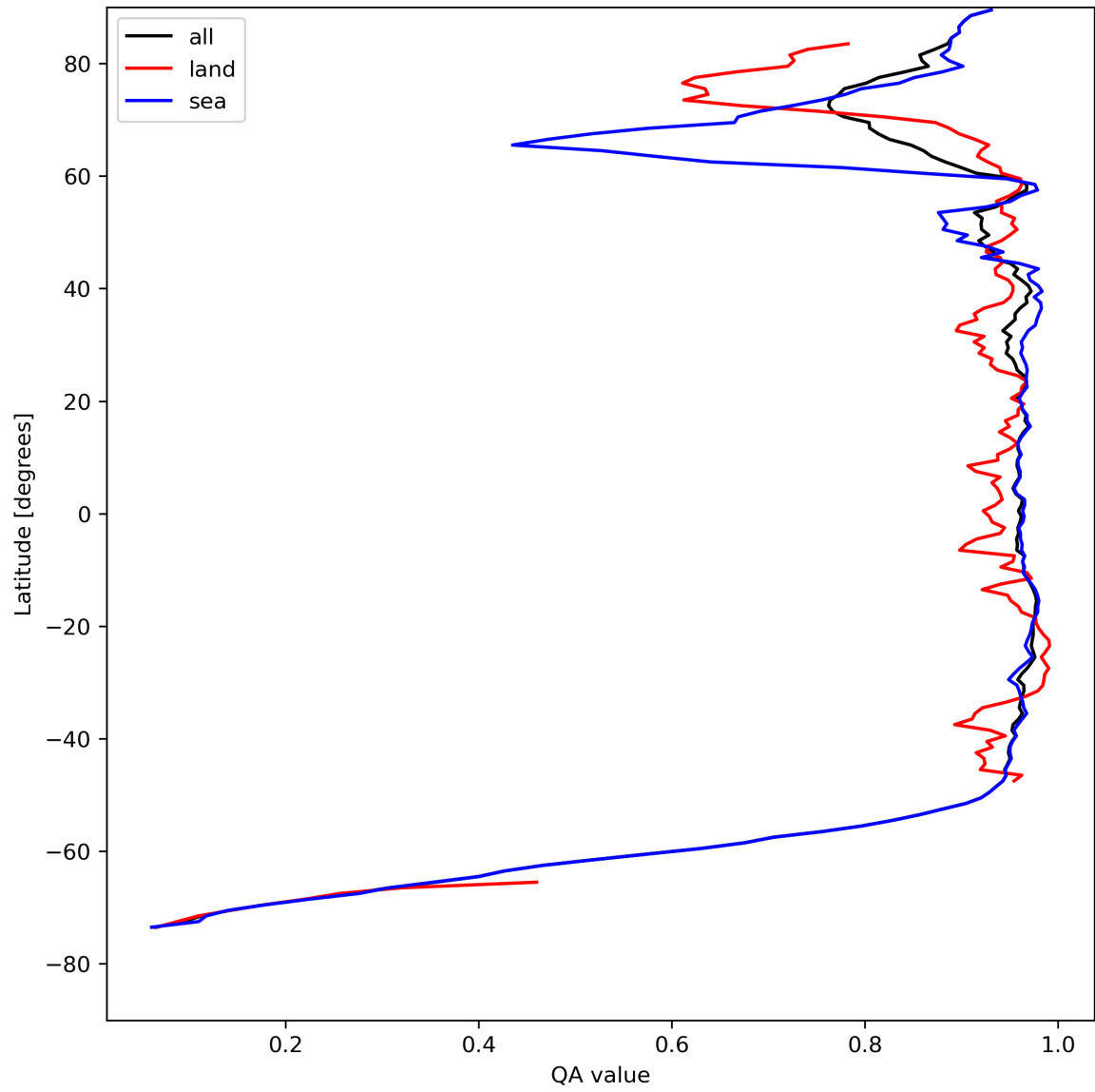
Figure 13: Zonal average of “QA value” for 2023-08-09 to 2023-08-10.
