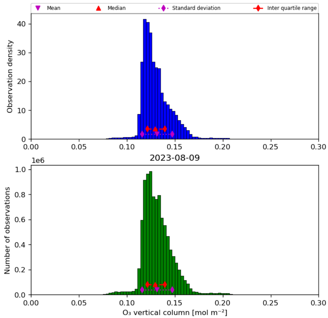
Figure 21: Histogram of “O 3 vertical column” for 2023-08-09 to 2023-08-10
