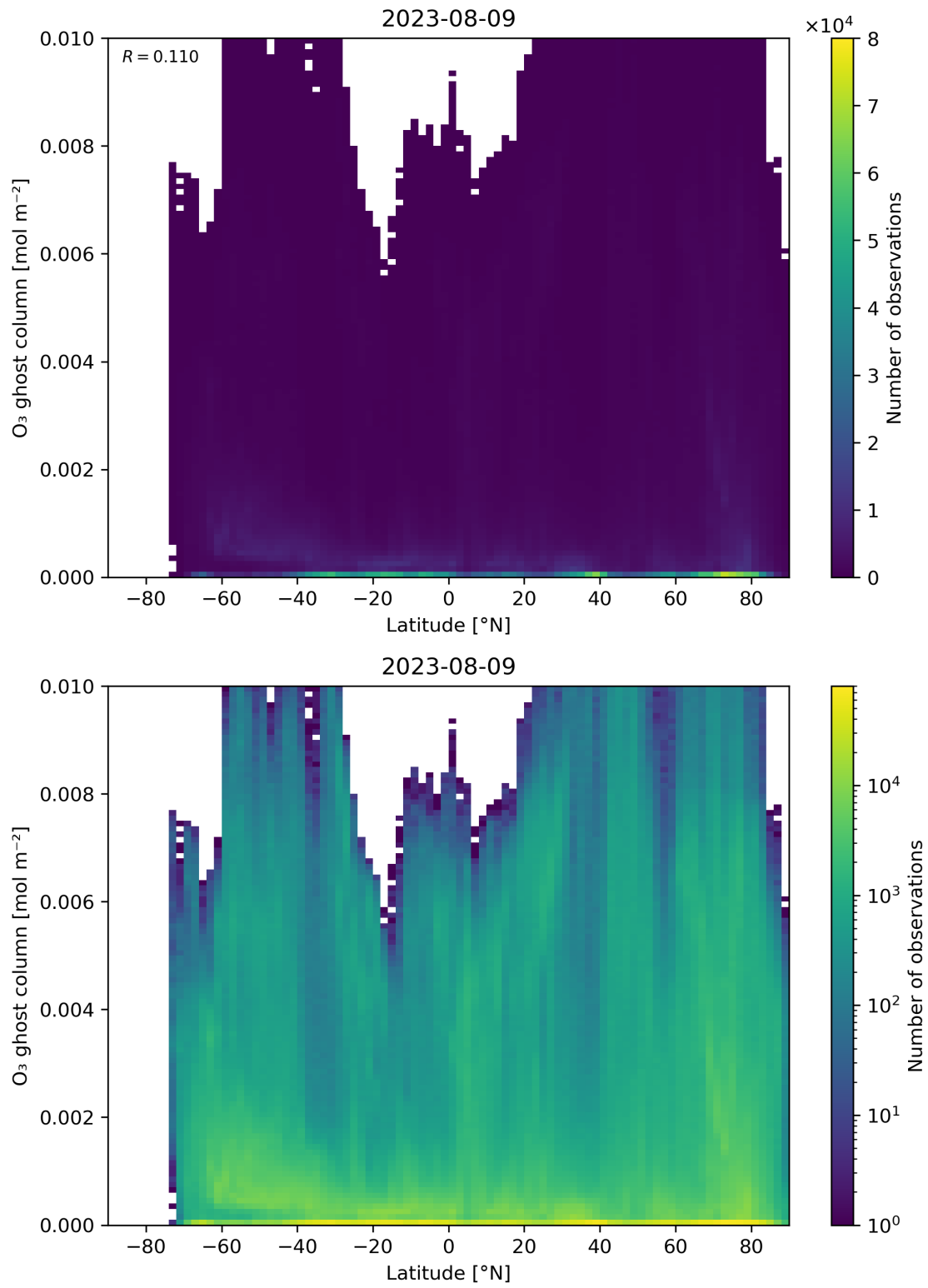
Figure 35: Scatter density plot of “Latitude” against “O 3 ghost column” for 2023-08-09 to 2023-08-10.
