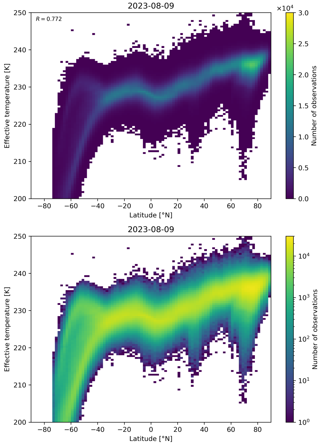
Figure 34: Scatter density plot of “Latitude” against “Effective temperature” for 2023-08-09 to 2023-08-10.
