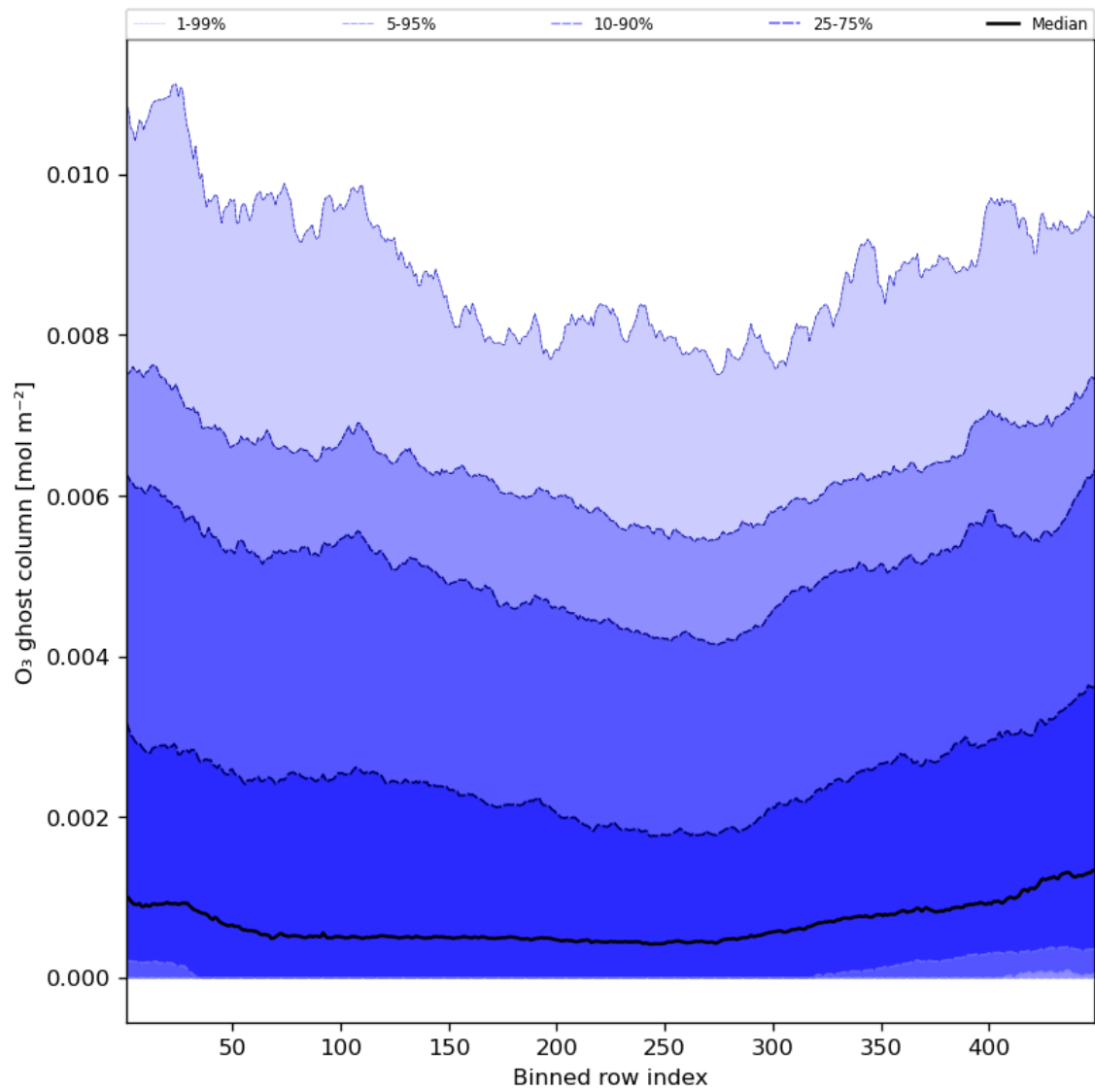
Figure 32: Along track statistics of “O 3 ghost column” for 2023-08-09 to 2023-08-10
