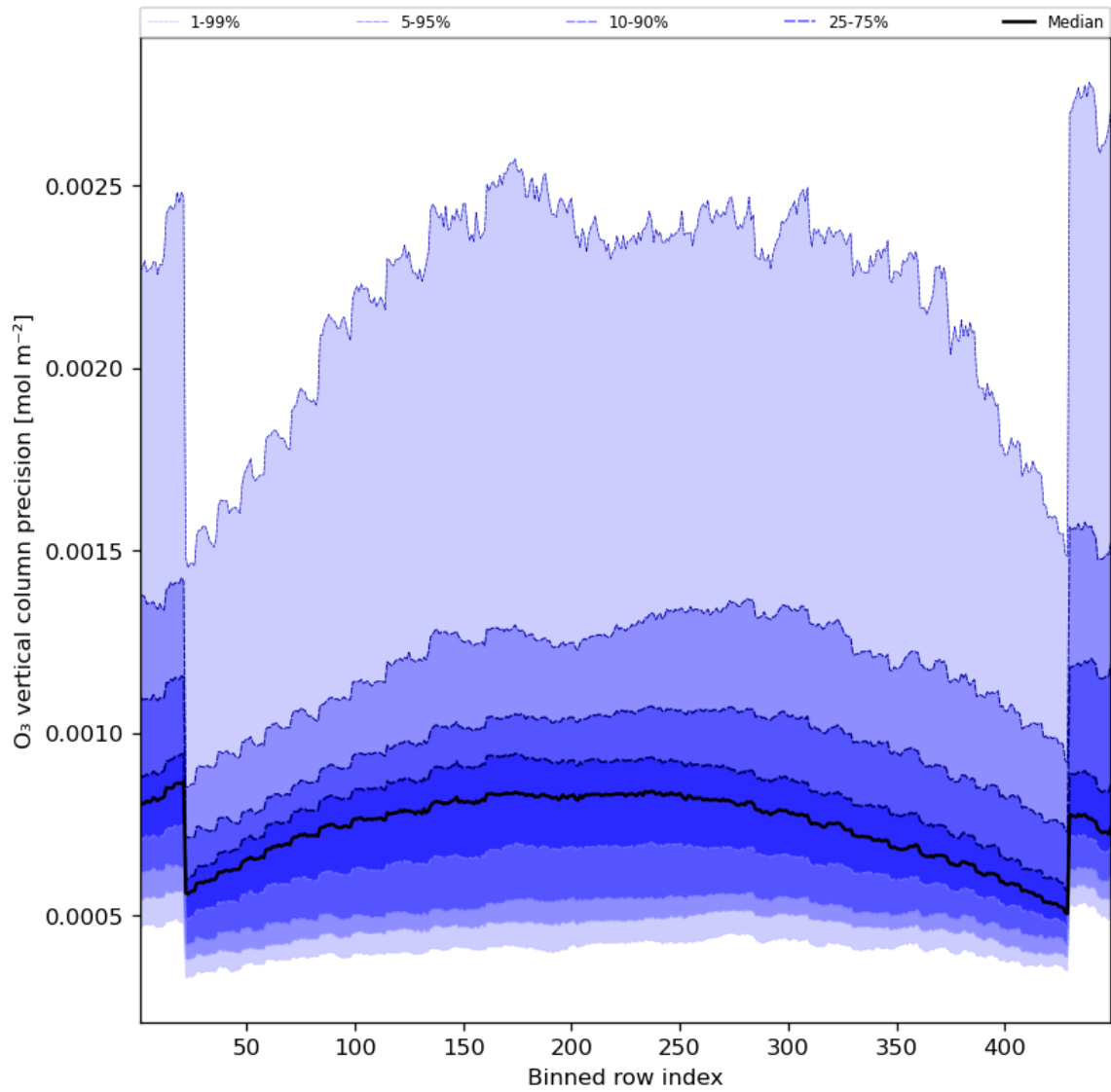
Figure 29: Along track statistics of “O 3 vertical column precision” for 2023-08-09 to 2023-08-10
