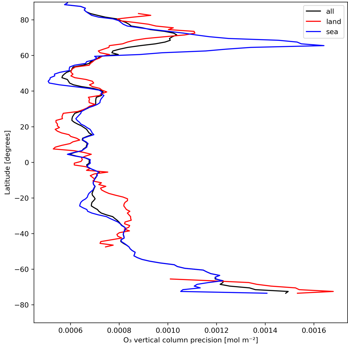
Figure 15: Zonal average of “O 3 vertical column precision” for 2023-08-09 to 2023-08-10.
