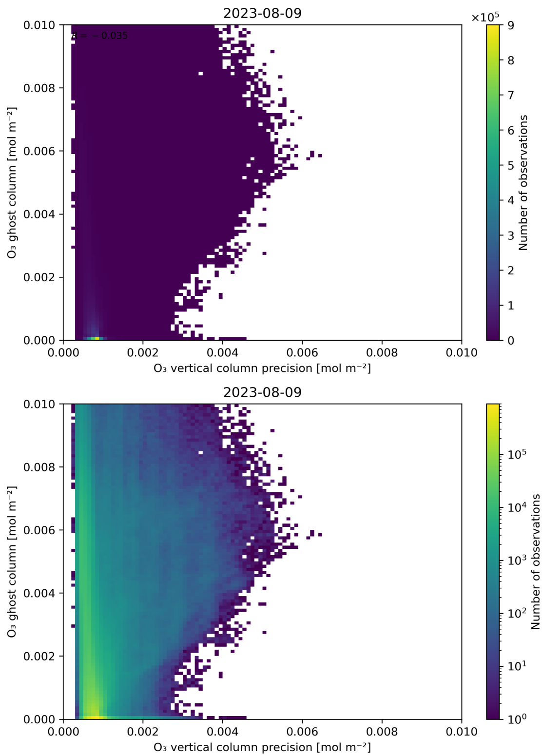
Figure 43: Scatter density plot of “O 3 vertical column precision” against “O 3 ghost column” for 2023-08-09 to 2023-08-10.
