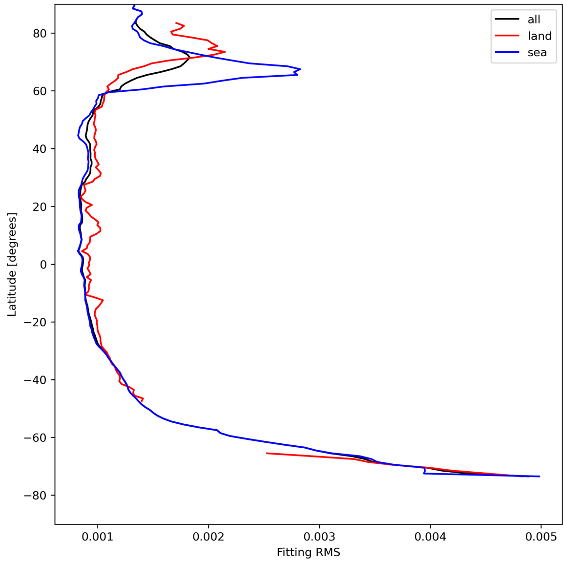
Figure 16: Zonal average of “Fitting RMS” for 2023-08-09 to 2023-08-10.
