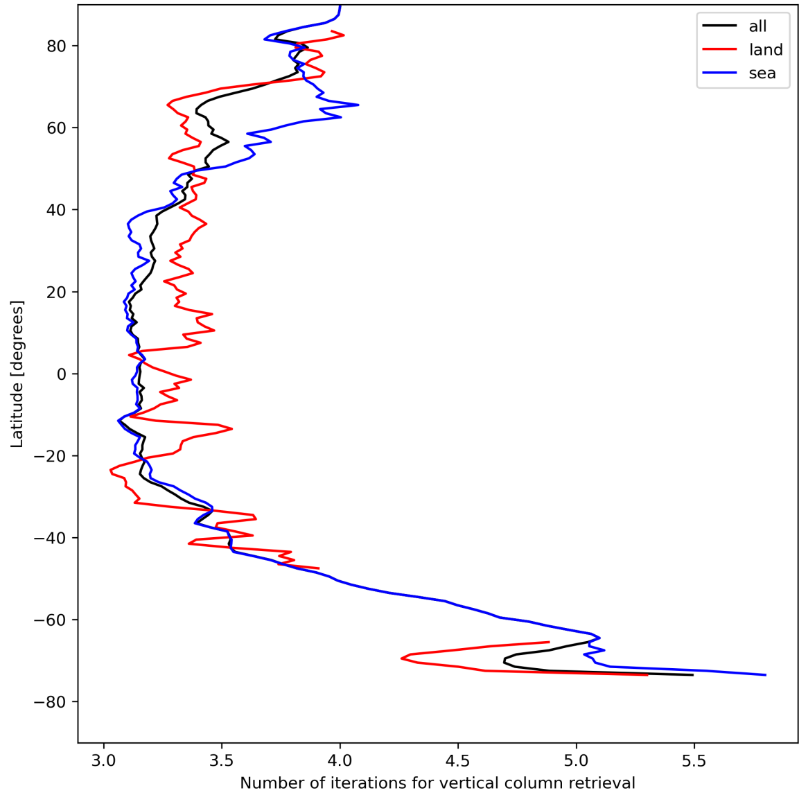
Figure 19: Zonal average of “Number of iterations for vertical column retrieval” for 2023-08-09 to 2023-08-10.
