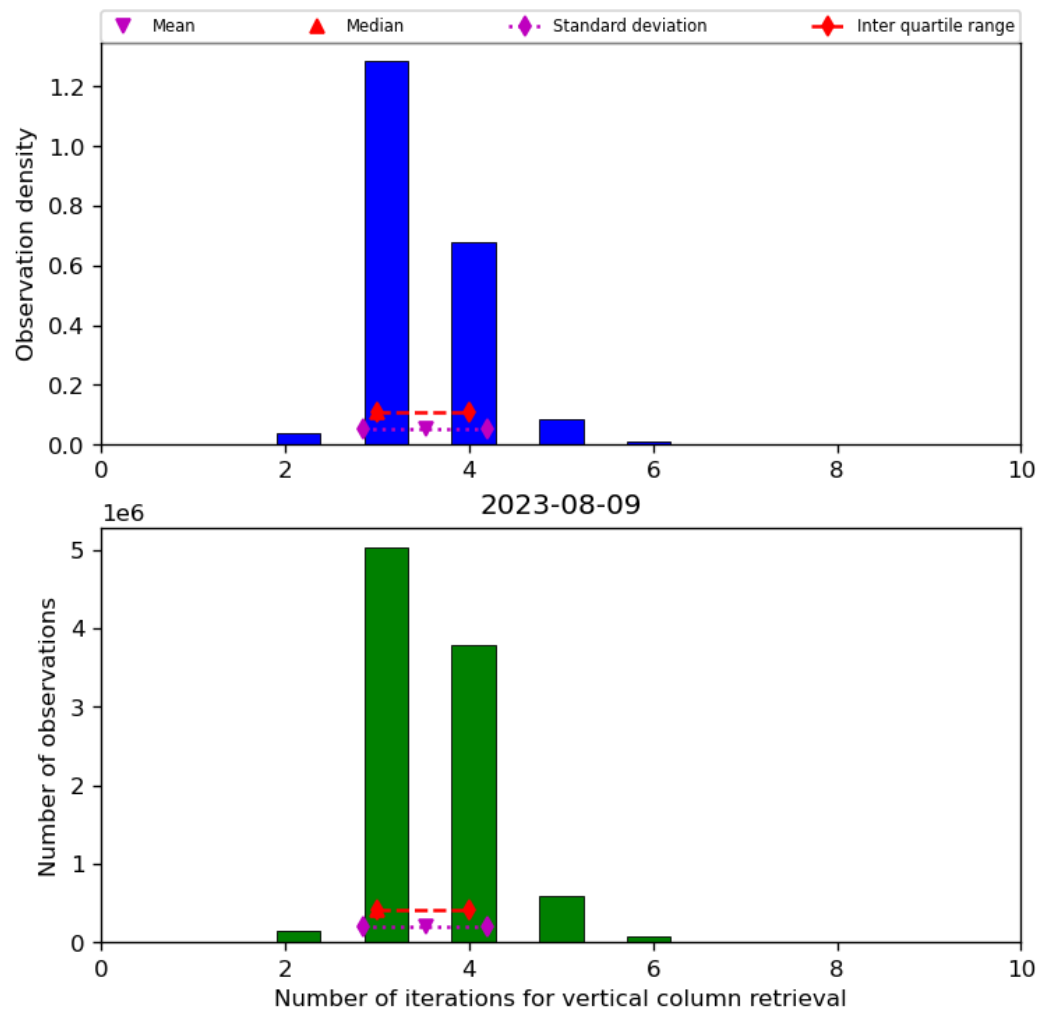
Figure 26: Histogram of “Number of iterations for vertical column retrieval” for 2023-08-09 to 2023-08-10
