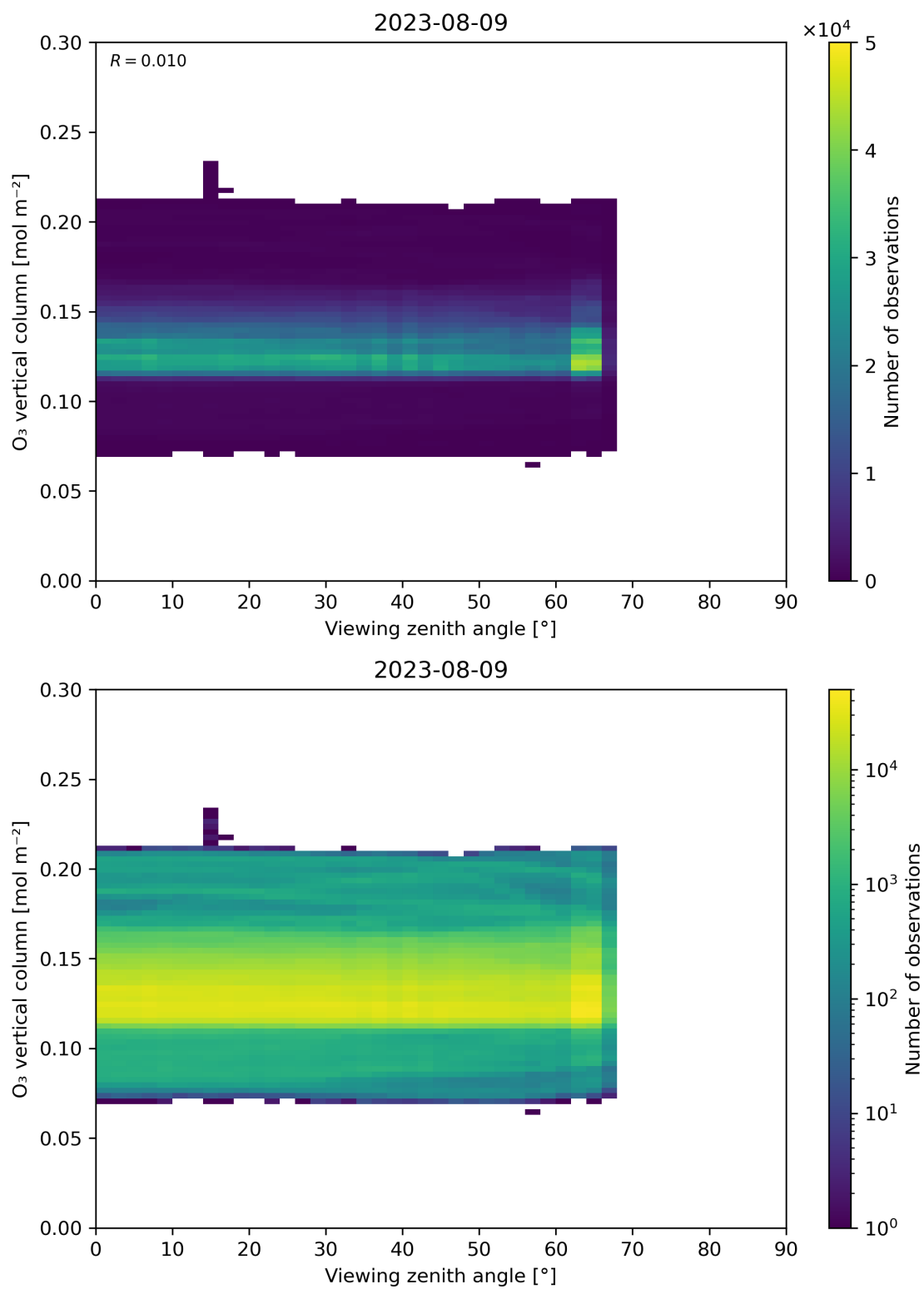
Figure 52: Scatter density plot of “Viewing zenith angle” against “O 3 vertical column” for 2023-08-09 to 2023-08-10.
