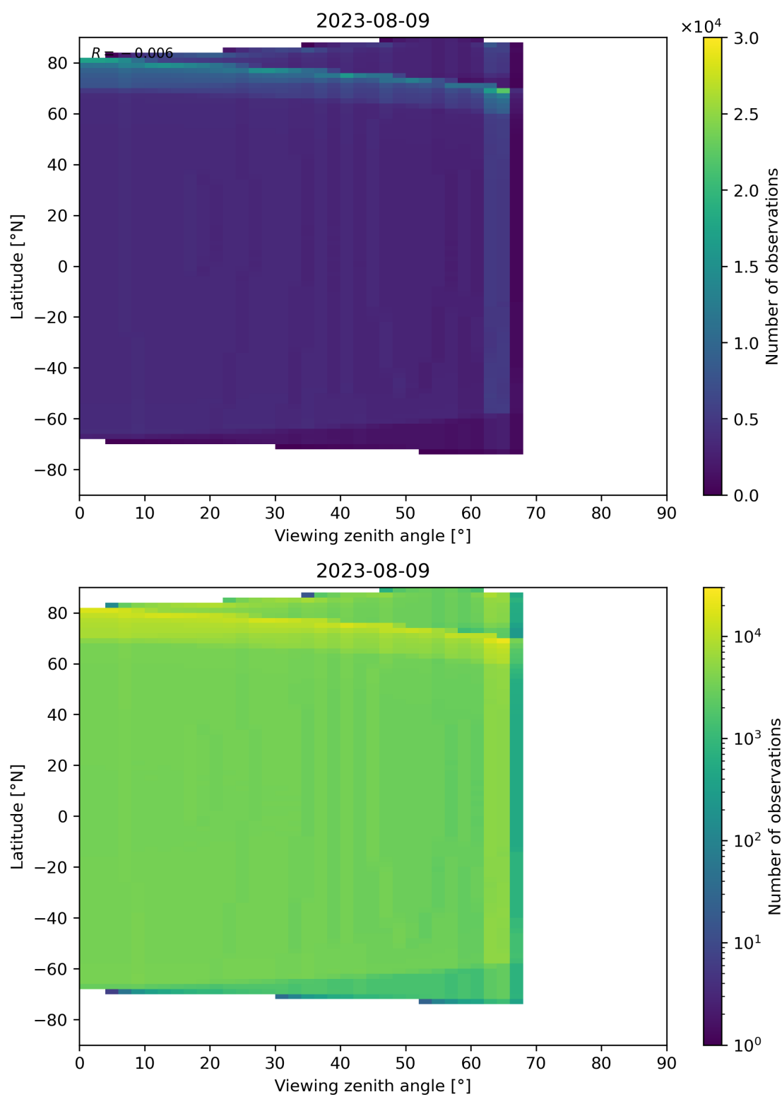
Figure 49: Scatter density plot of “Viewing zenith angle” against “Latitude” for 2023-08-09 to 2023-08-10.
