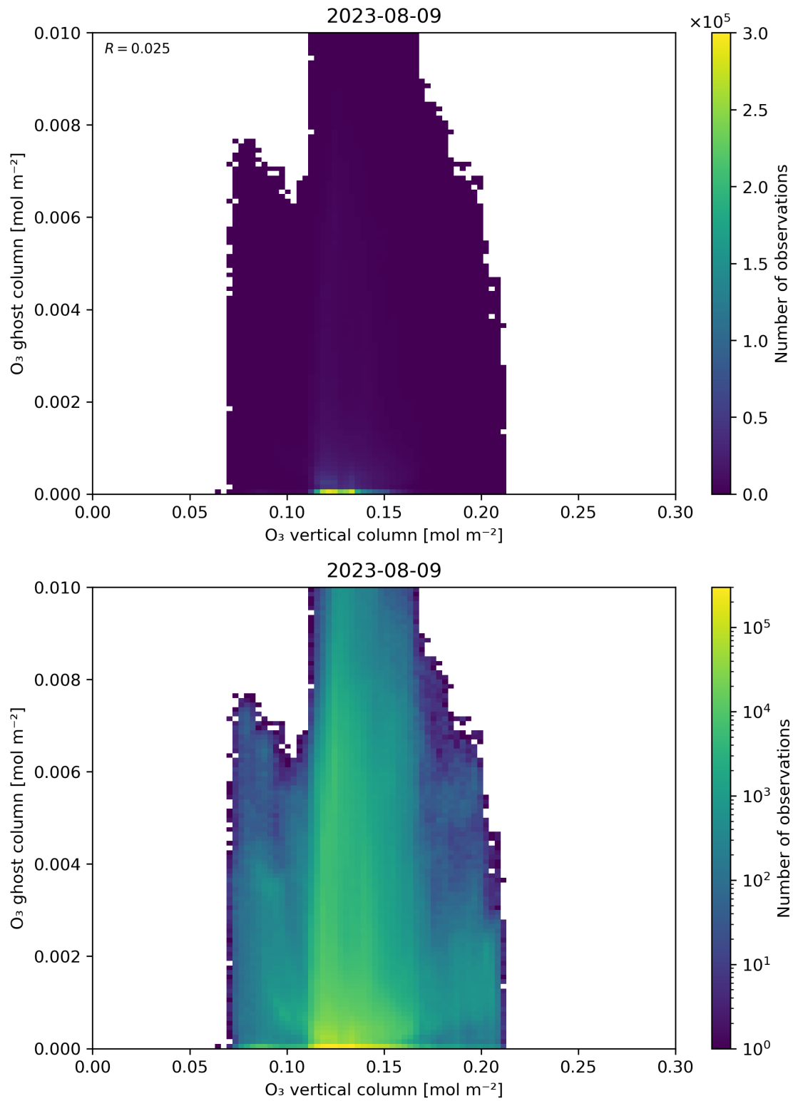
Figure 40: Scatter density plot of “O 3 vertical column” against “O 3 ghost column” for 2023-08-09 to 2023-08-10.
