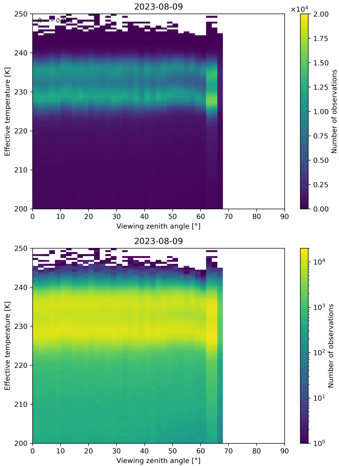
Figure 50: Scatter density plot of “Viewing zenith angle” against “Effective temperature” for 2023-08-09 to 2023-08-10.
