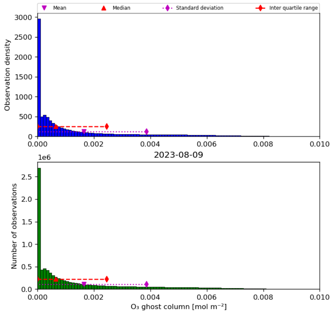
Figure 25: Histogram of “O 3 ghost column” for 2023-08-09 to 2023-08-10
