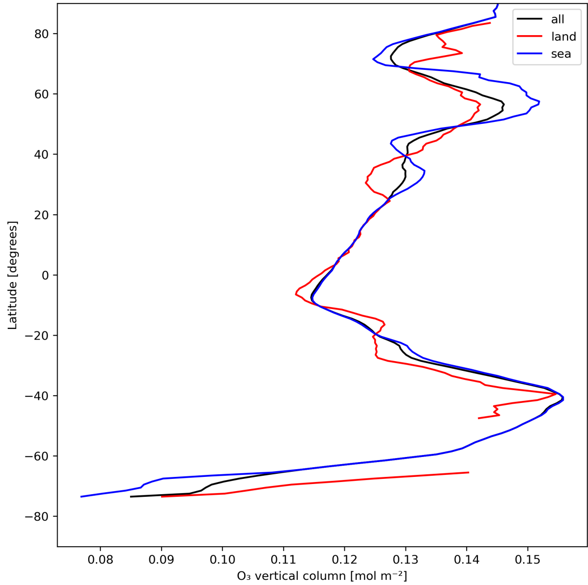
Figure 14: Zonal average of “O 3 vertical column” for 2023-08-09 to 2023-08-10.
