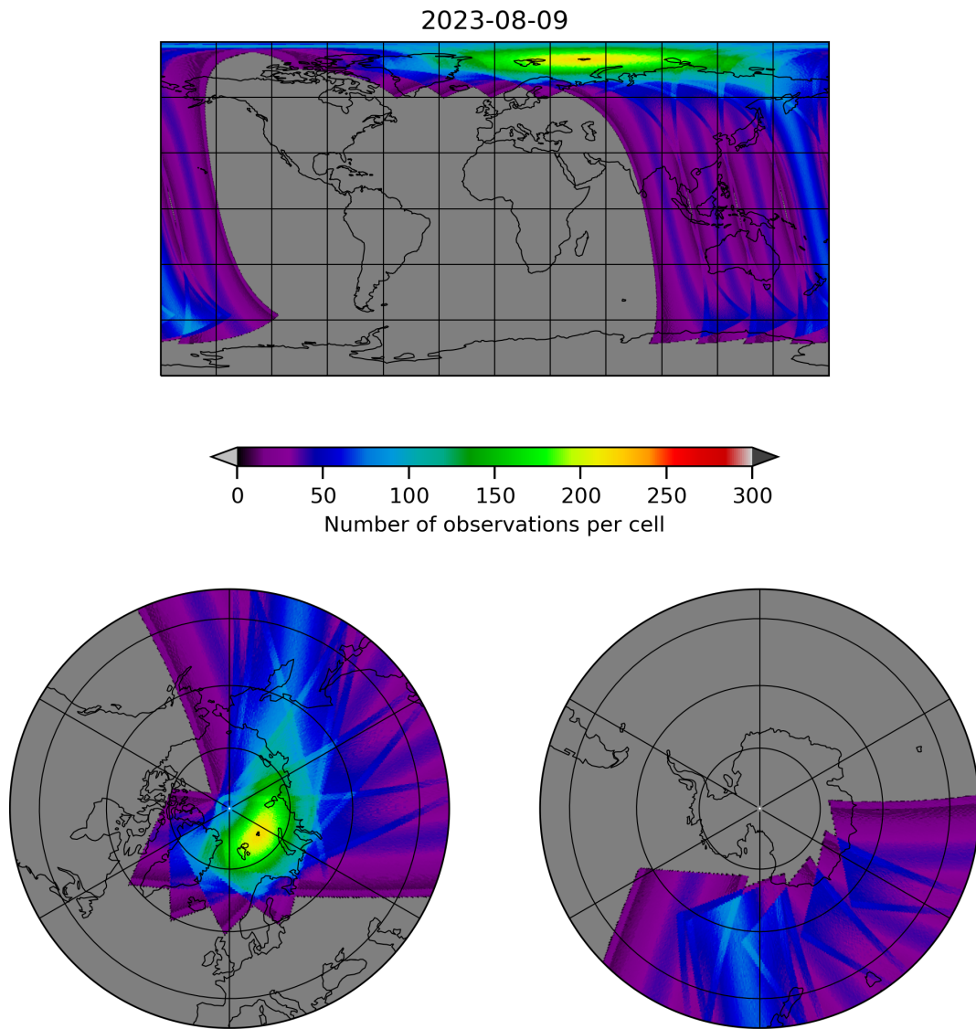
Figure 12: Map of the number of observations for 2023-08-09 to 2023-08-10
