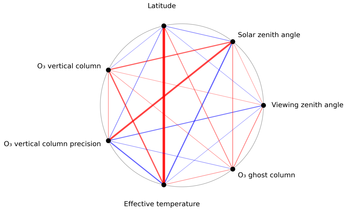
Figure 1: Map of correlation graph for 2023-08-09 to 2023-08-10.
