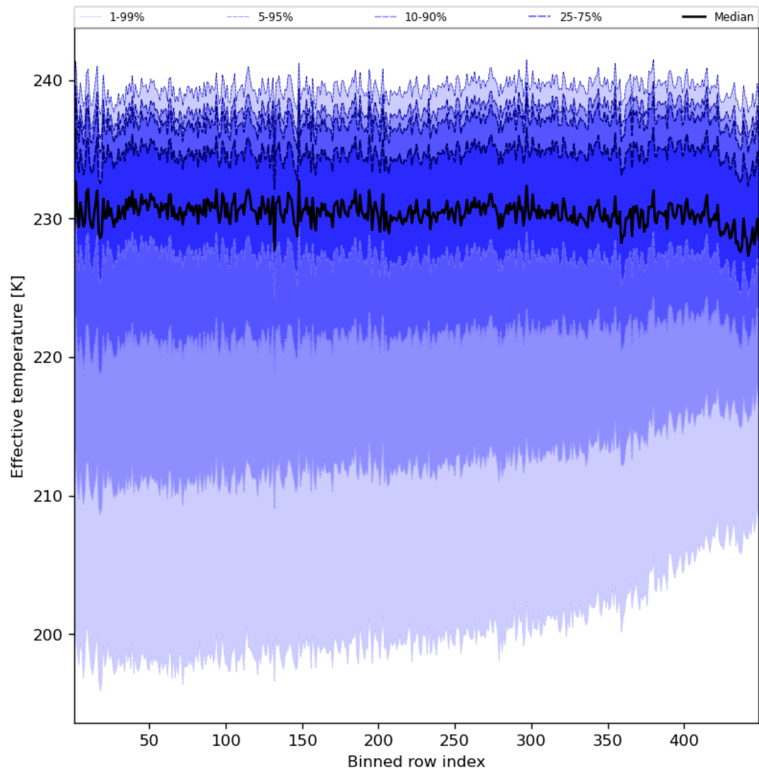
Figure 31: Along track statistics of “Effective temperature” for 2023-08-09 to 2023-08-10
