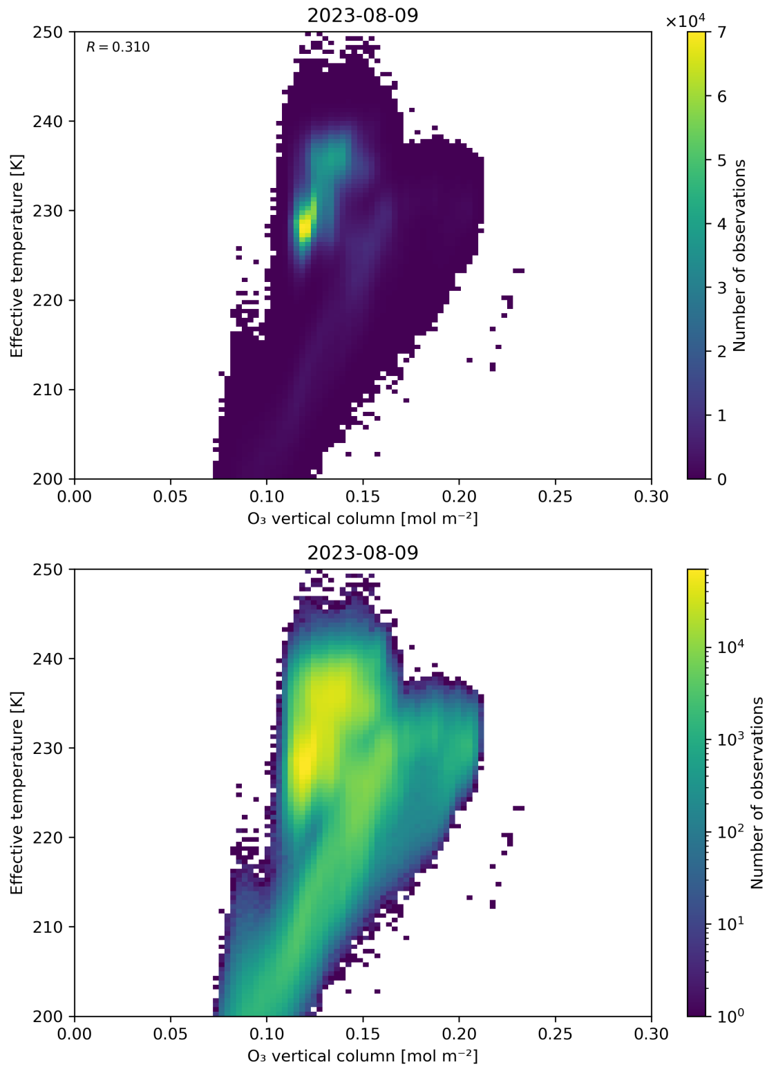
Figure 39: Scatter density plot of “O 3 vertical column” against “Effective temperature” for 2023-08-09 to 2023-08-10.
