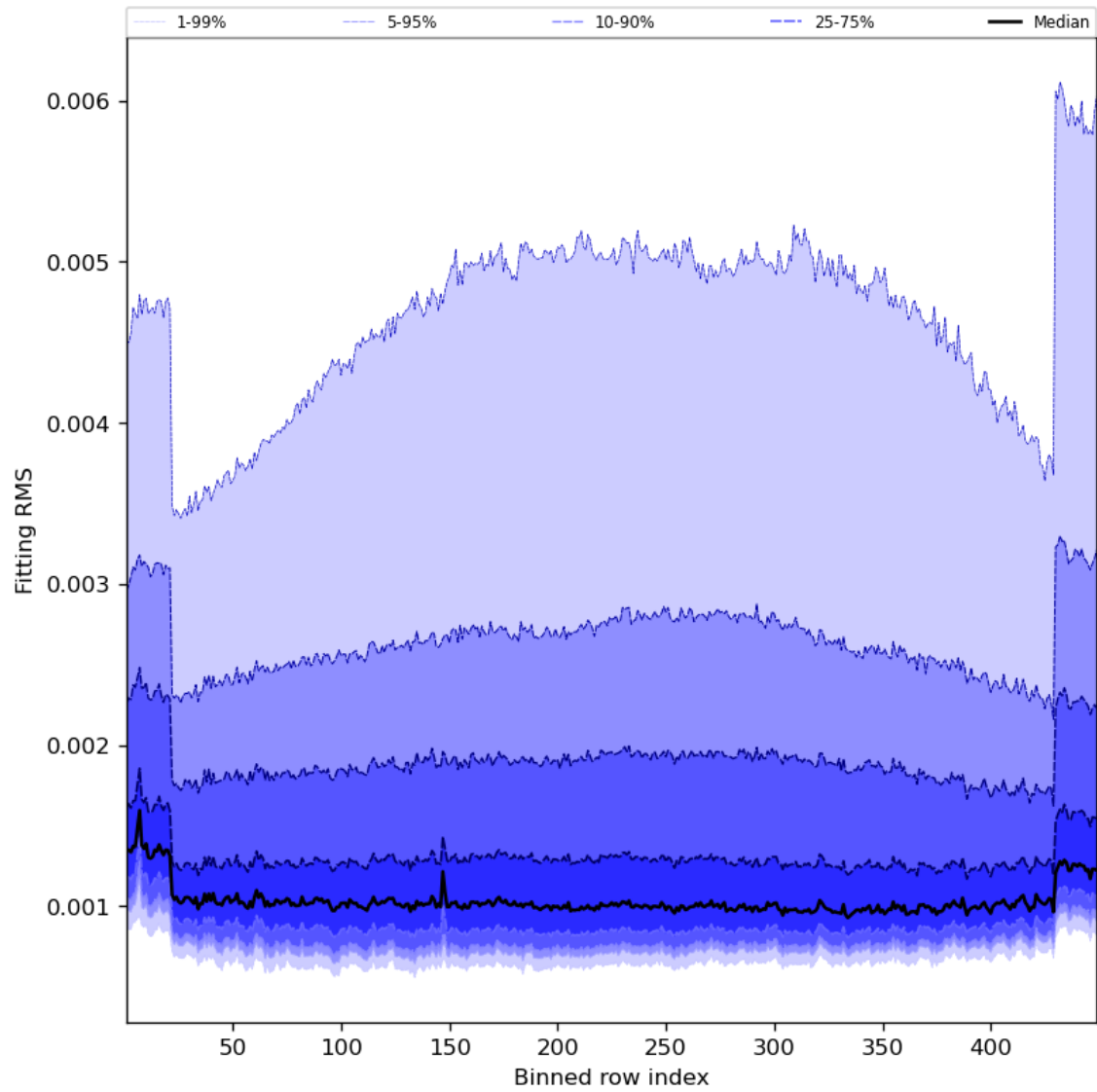
Figure 30: Along track statistics of “Fitting RMS” for 2023-08-09 to 2023-08-10
