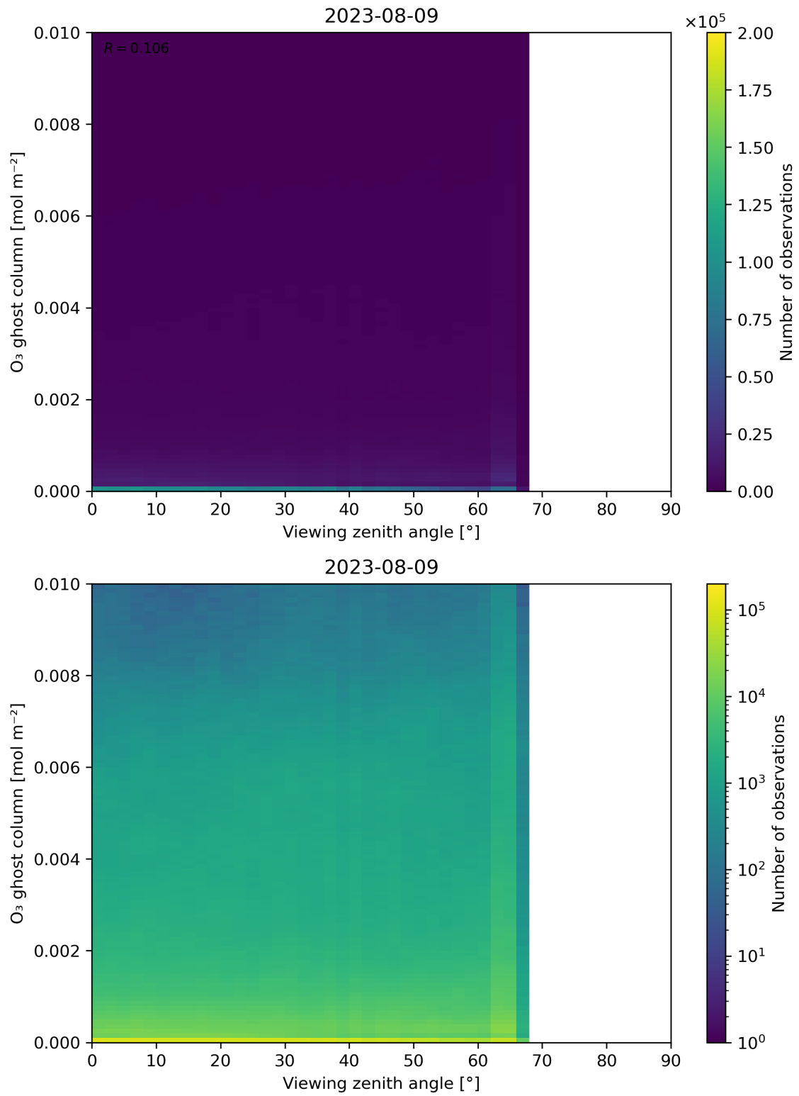
Figure 51: Scatter density plot of “Viewing zenith angle” against “O 3 ghost column” for 2023-08-09 to 2023-08-10.
