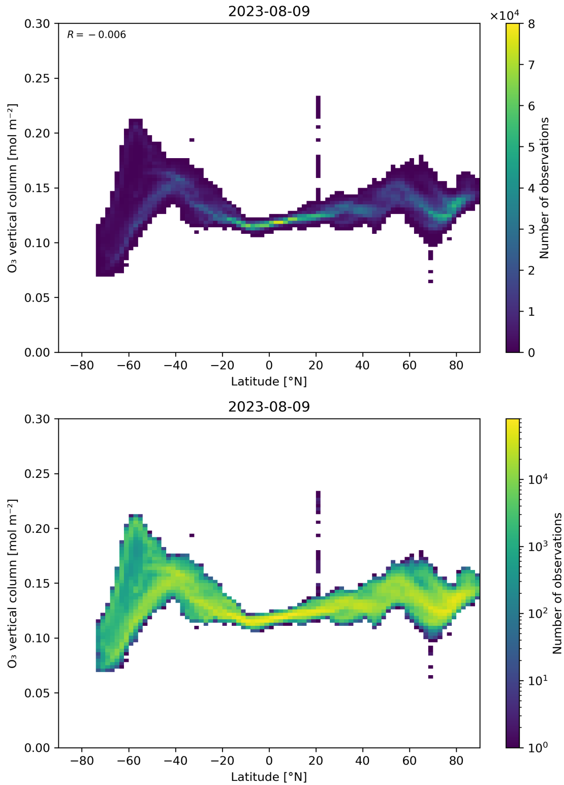
Figure 36: Scatter density plot of “Latitude” against “O 3 vertical column” for 2023-08-09 to 2023-08-10.
