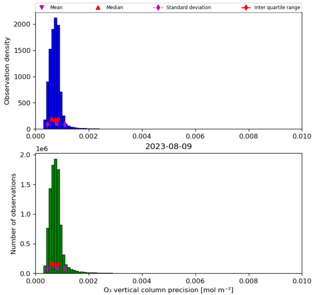
Figure 22: Histogram of “O 3 vertical column precision” for 2023-08-09 to 2023-08-10
