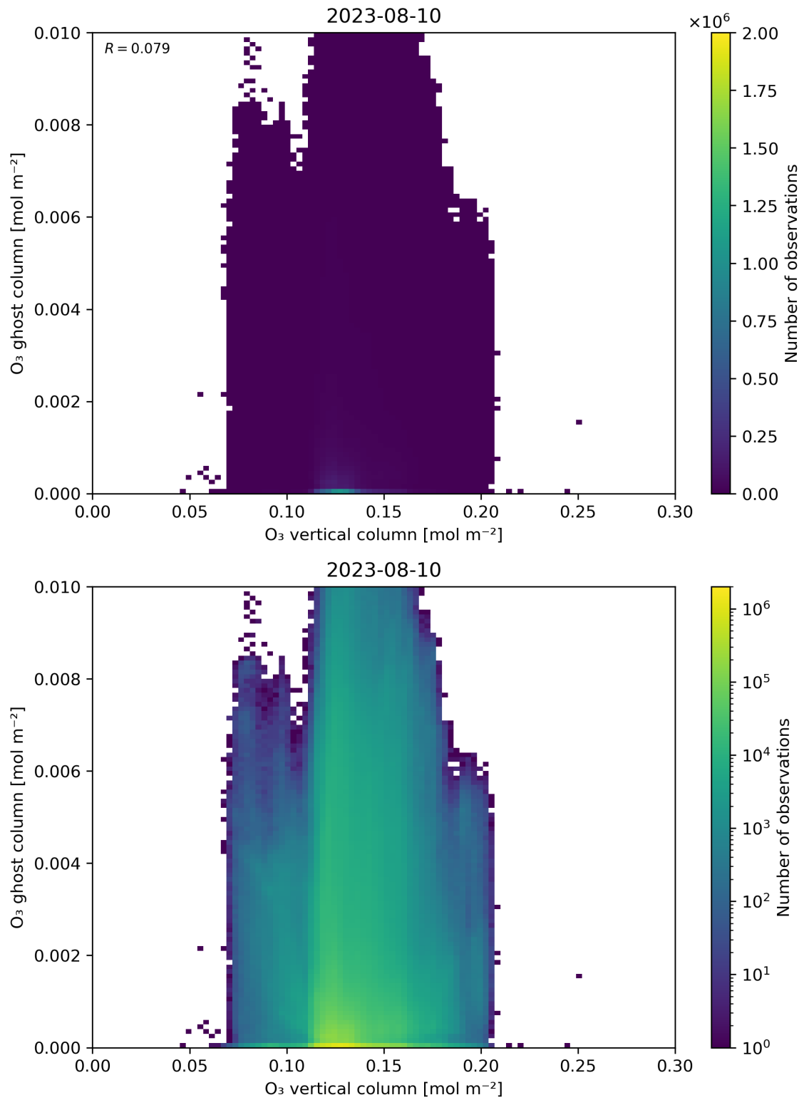
Figure 40: Scatter density plot of “O 3 vertical column” against “O 3 ghost column” for 2023-08-09 to 2023-08-11.
