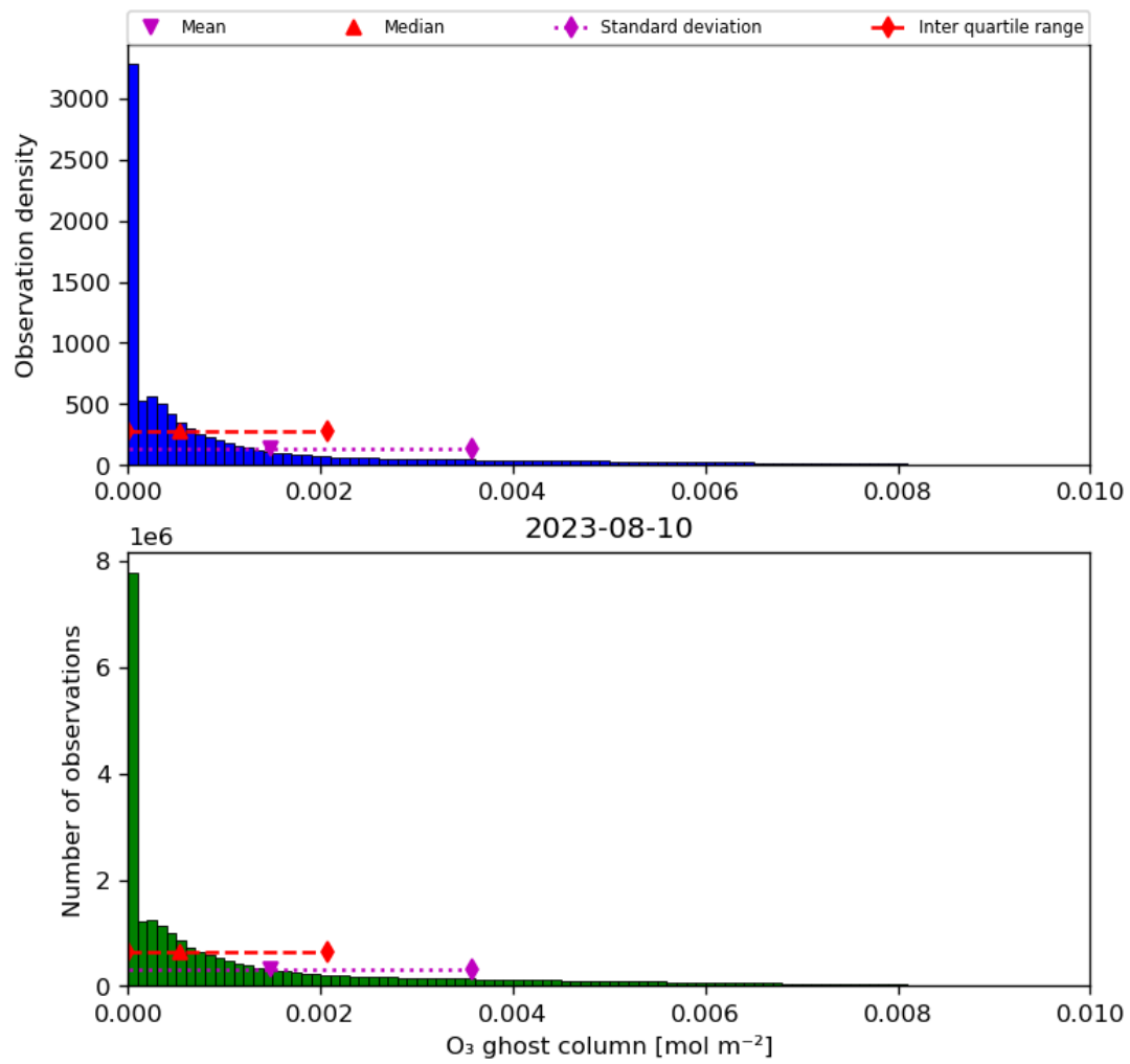
Figure 25: Histogram of “O 3 ghost column” for 2023-08-09 to 2023-08-11
