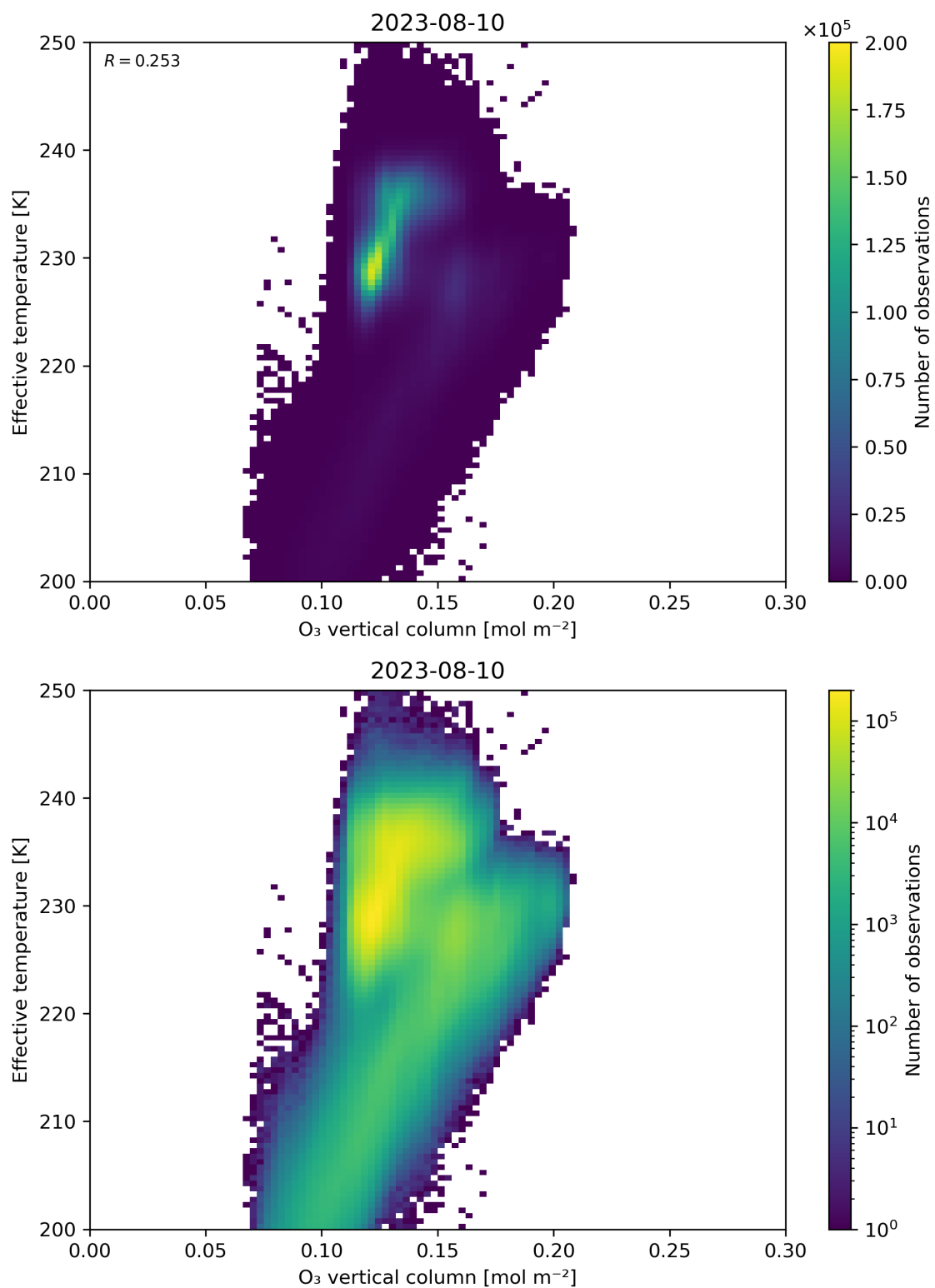
Figure 39: Scatter density plot of “O 3 vertical column” against “Effective temperature” for 2023-08-09 to 2023-08-11.
