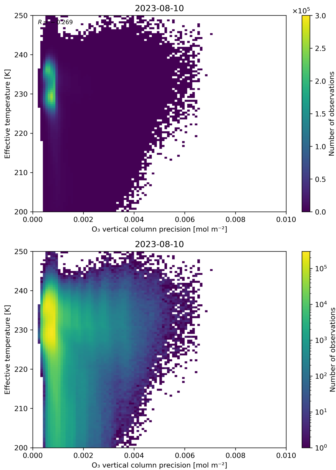
Figure 42: Scatter density plot of “O 3 vertical column precision” against “Effective temperature” for 2023-08-09 to 2023-08-11.
