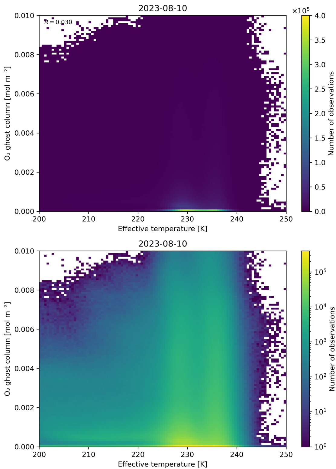
Figure 38: Scatter density plot of “Effective temperature” against “O 3 ghost column” for 2023-08-09 to 2023-08-11.
