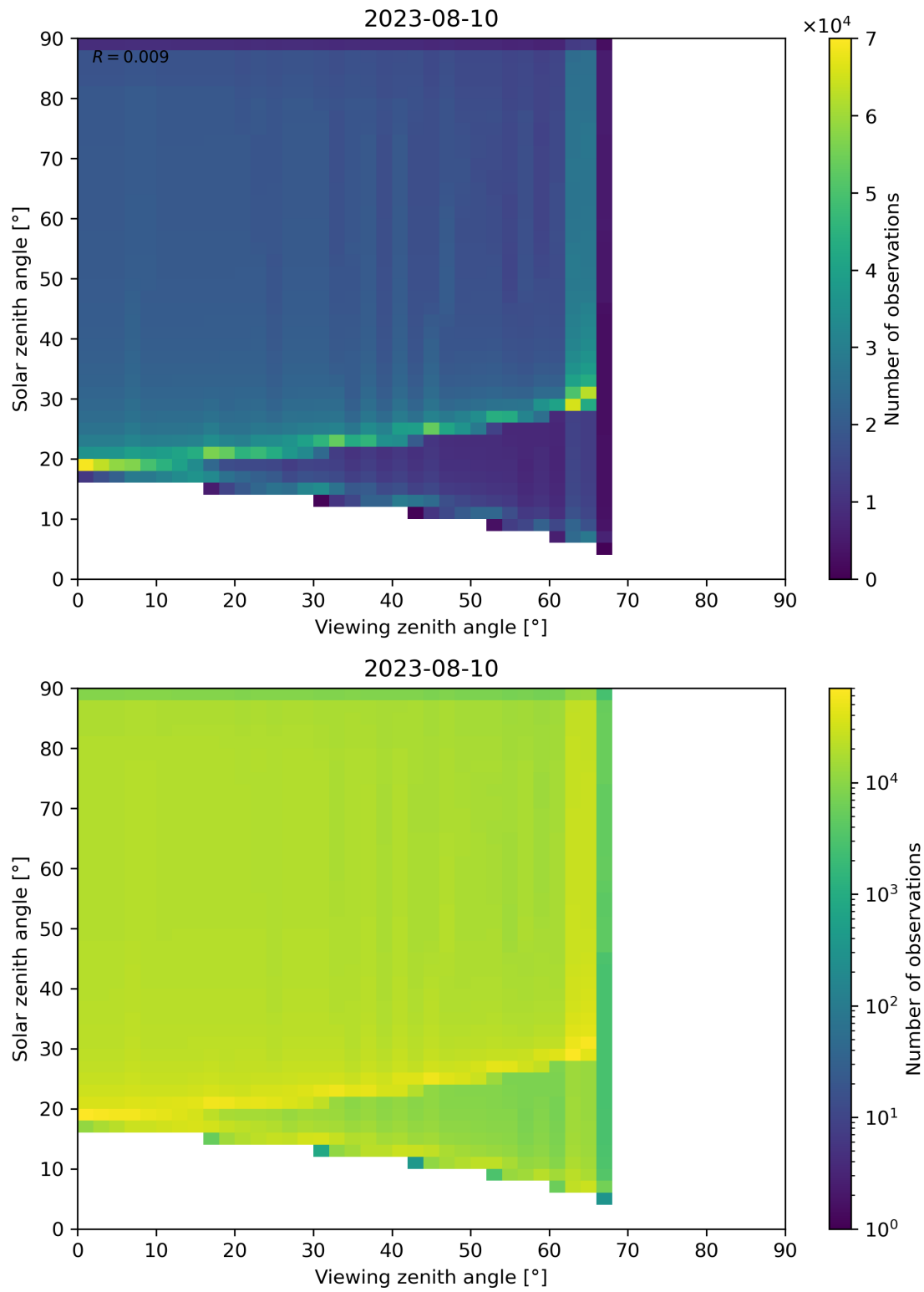
Figure 54: Scatter density plot of “Viewing zenith angle” against “Solar zenith angle” for 2023-08-09 to 2023-08-11.
