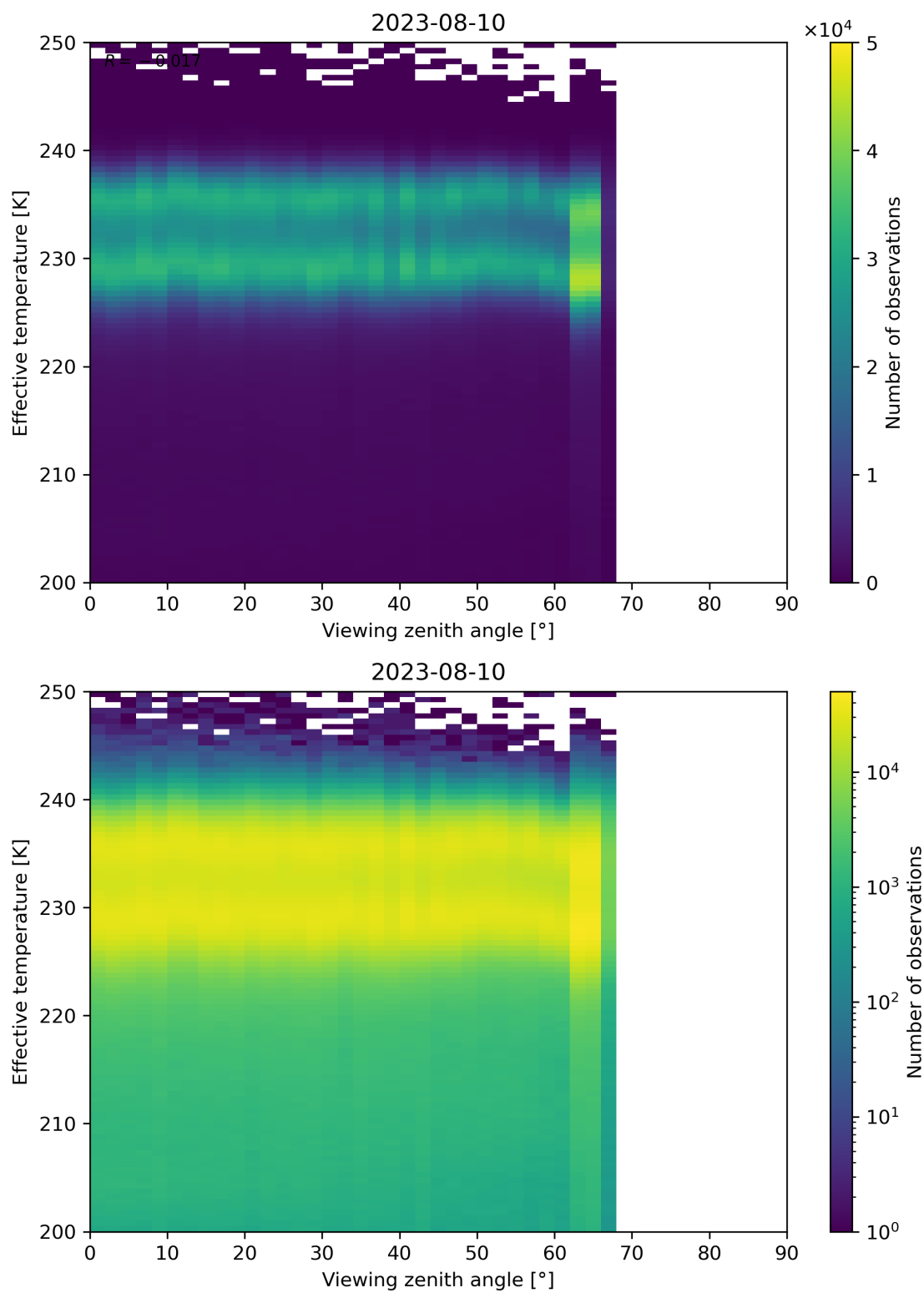
Figure 50: Scatter density plot of “Viewing zenith angle” against “Effective temperature” for 2023-08-09 to 2023-08-11.
