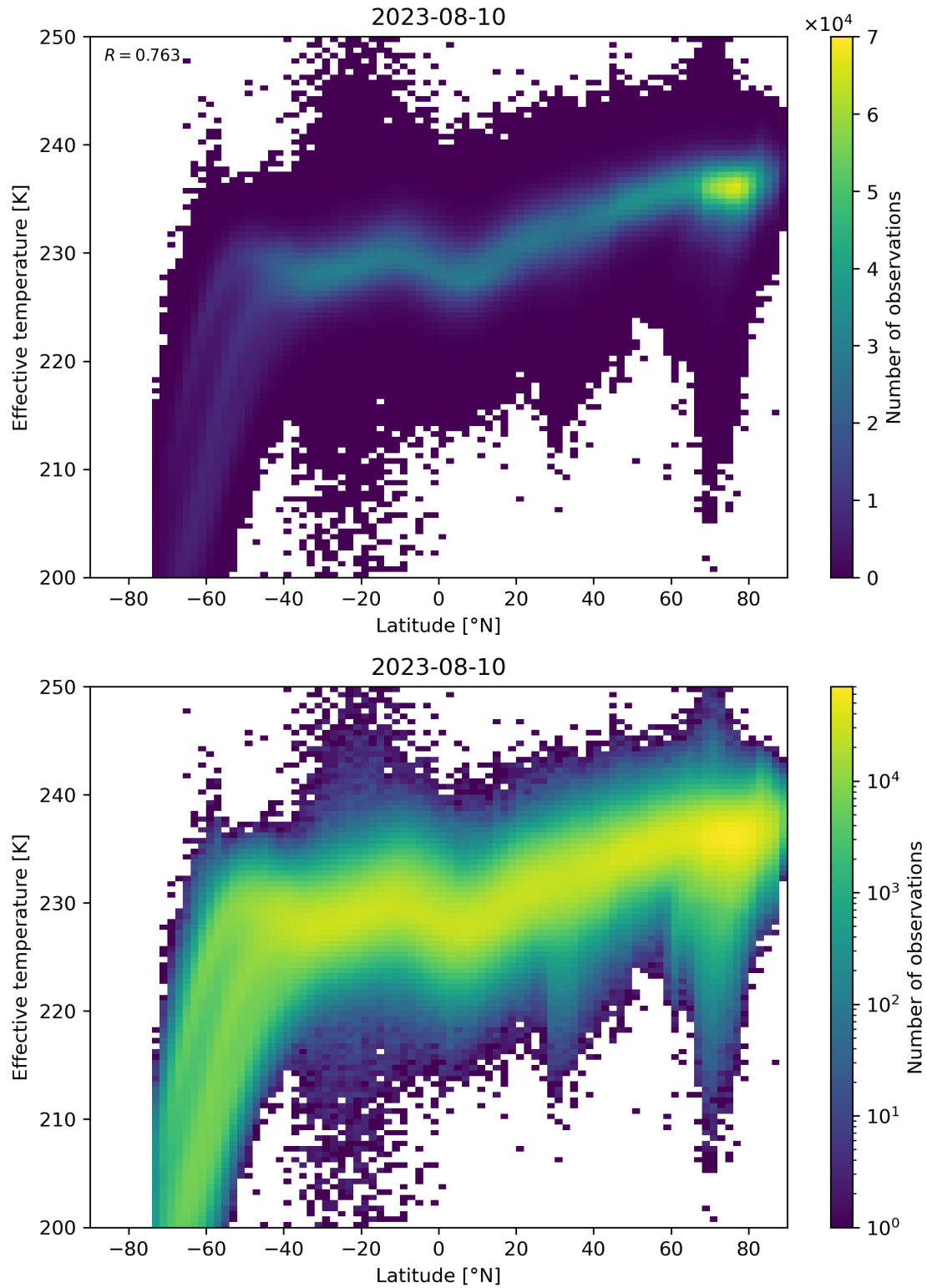
Figure 34: Scatter density plot of “Latitude” against “Effective temperature” for 2023-08-09 to 2023-08-11.
