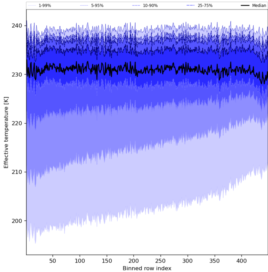
Figure 31: Along track statistics of “Effective temperature” for 2023-08-09 to 2023-08-11
