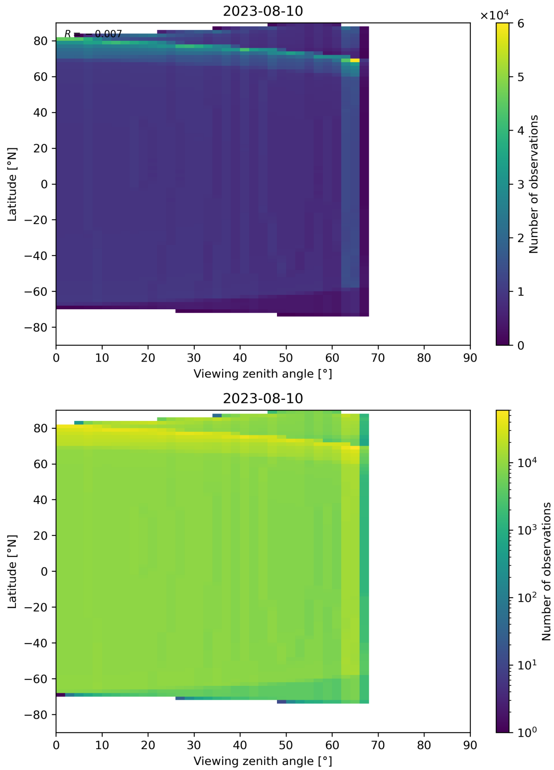
Figure 49: Scatter density plot of “Viewing zenith angle” against “Latitude” for 2023-08-09 to 2023-08-11.
