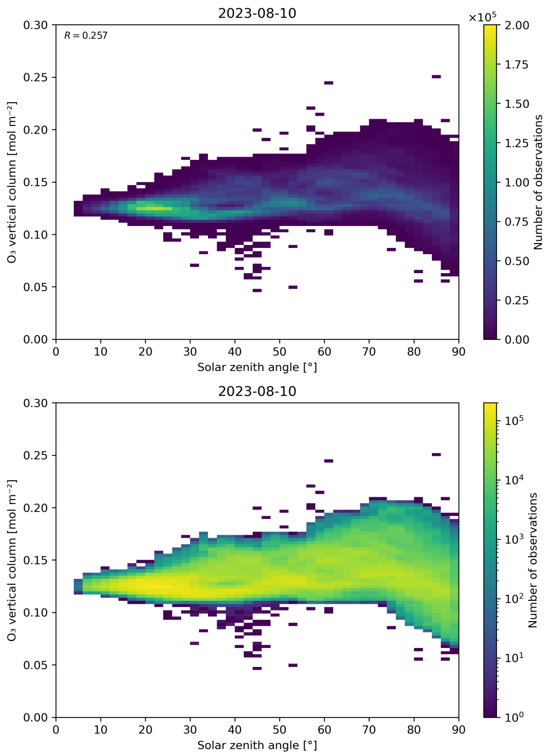
Figure 47: Scatter density plot of “Solar zenith angle” against “O 3 vertical column” for 2023-08-09 to 2023-08-11.
