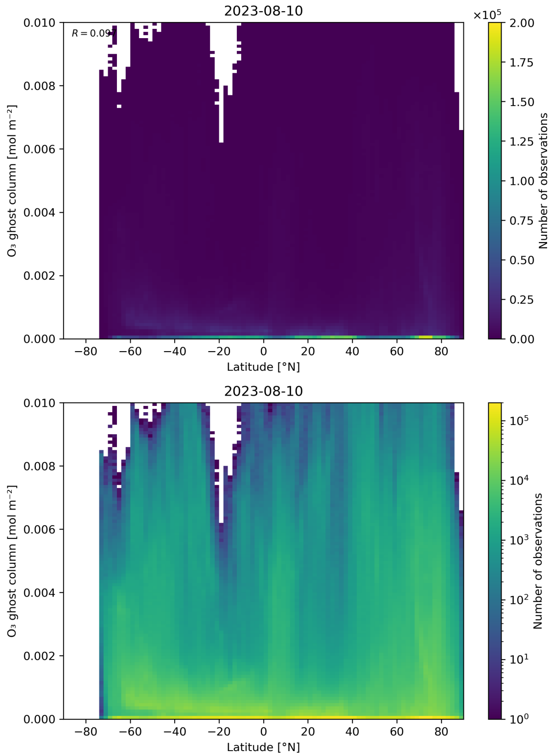
Figure 35: Scatter density plot of “Latitude” against “O 3 ghost column” for 2023-08-09 to 2023-08-11.
