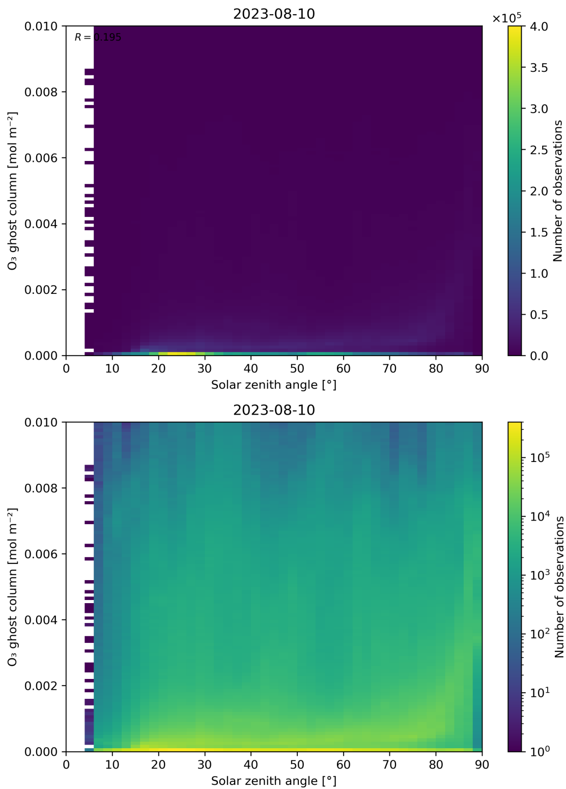
Figure 46: Scatter density plot of “Solar zenith angle” against “O 3 ghost column” for 2023-08-09 to 2023-08-11.
