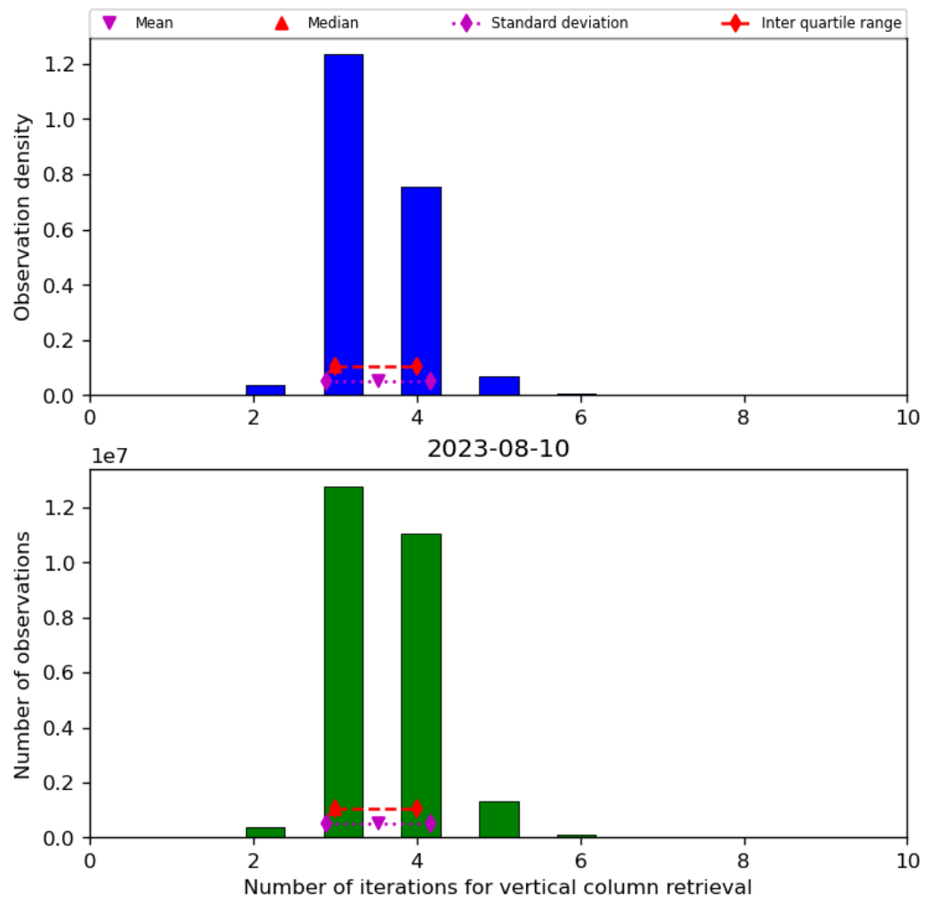
Figure 26: Histogram of “Number of iterations for vertical column retrieval” for 2023-08-09 to 2023-08-11
