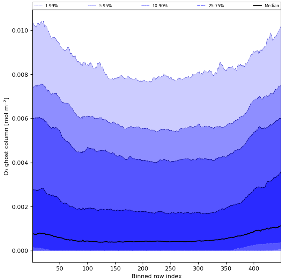
Figure 32: Along track statistics of “O 3 ghost column” for 2023-08-09 to 2023-08-11
