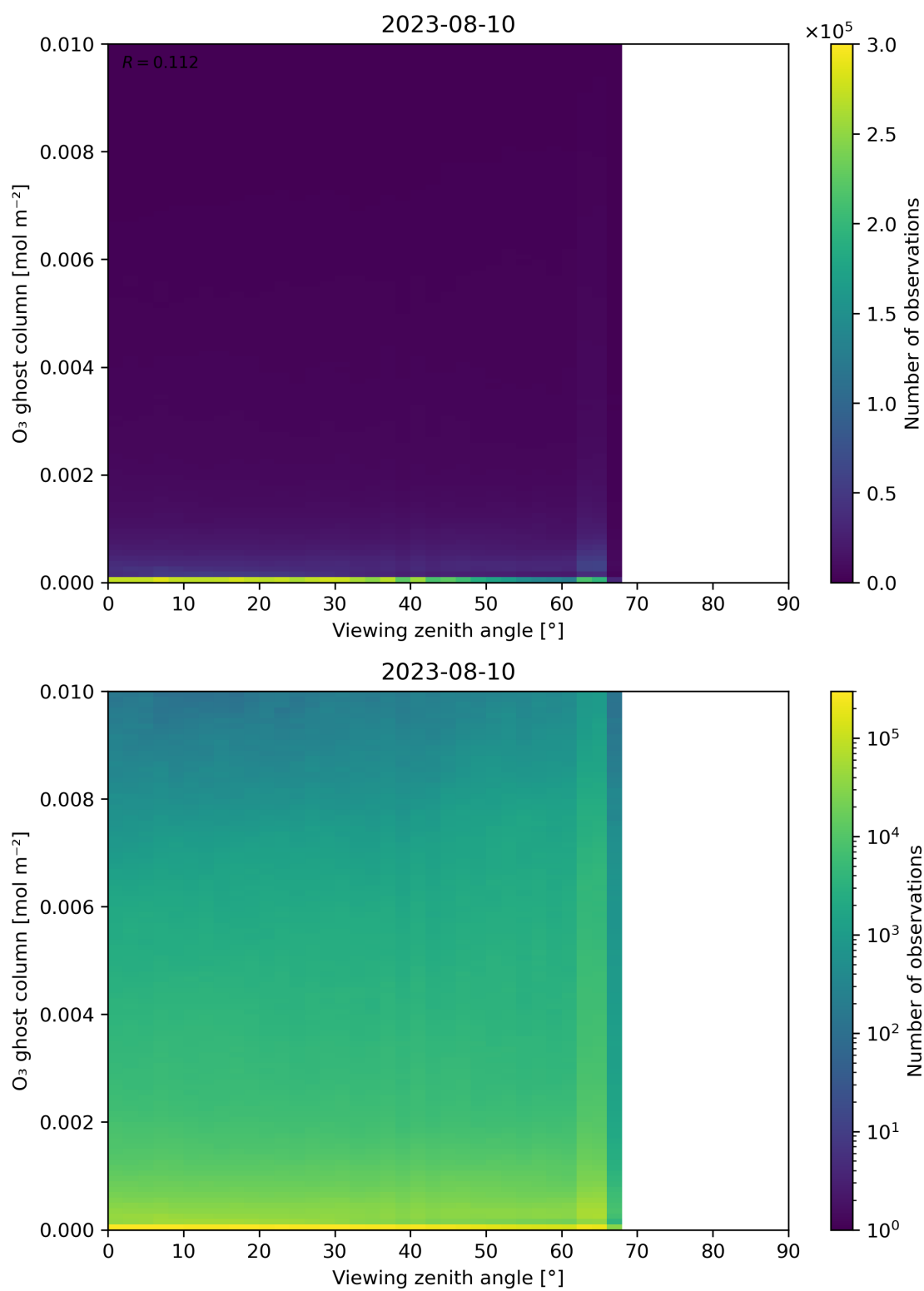
Figure 51: Scatter density plot of “Viewing zenith angle” against “O 3 ghost column” for 2023-08-09 to 2023-08-11.
