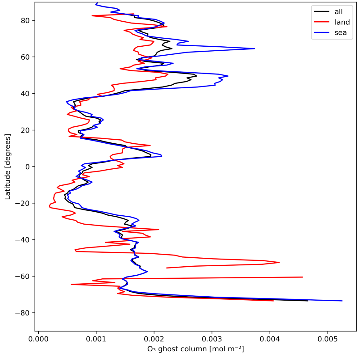
Figure 18: Zonal average of "O 3 ghost column" for 2023-08-09 to 2023-08-11.
