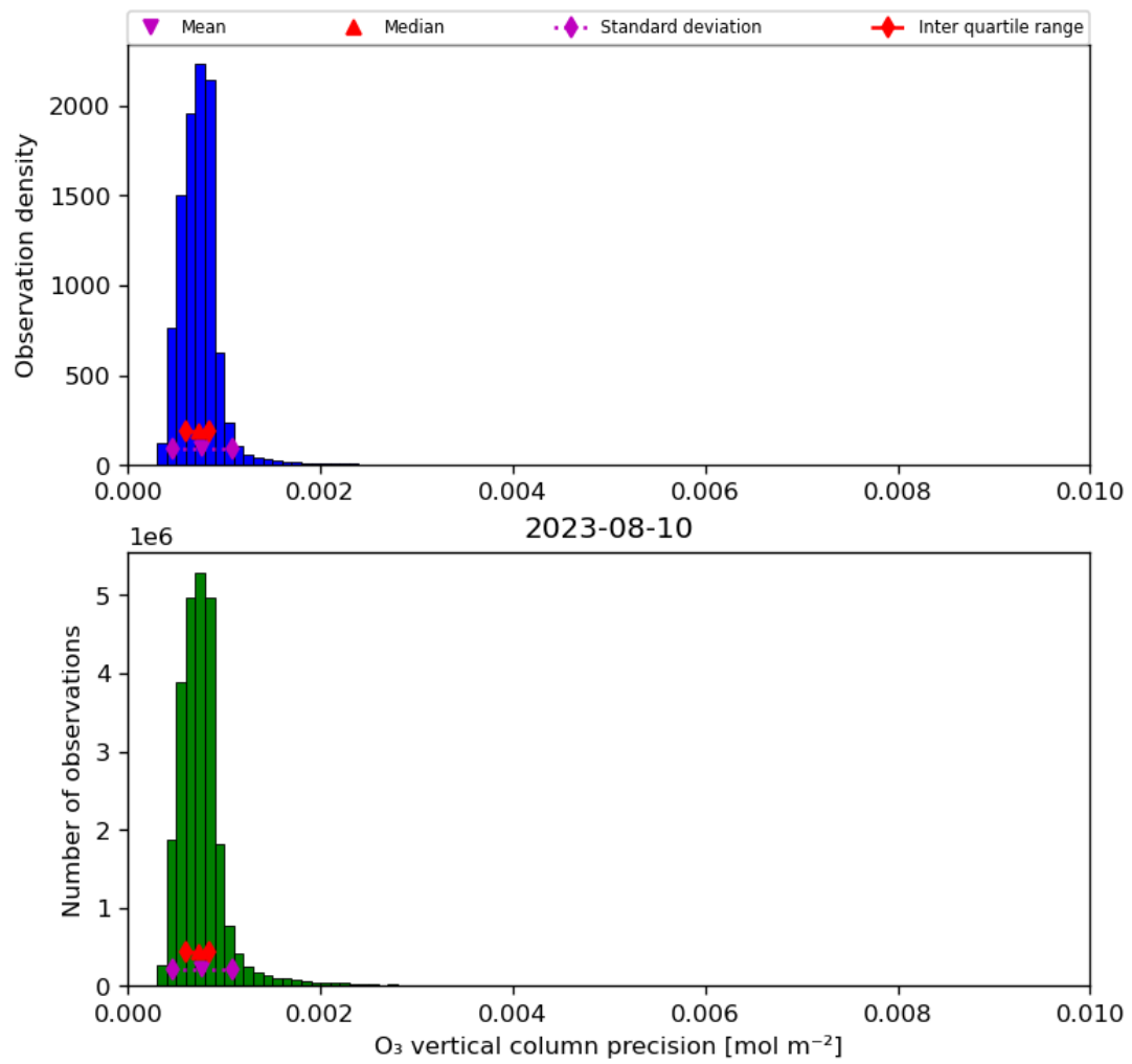
Figure 22: Histogram of “O 3 vertical column precision” for 2023-08-09 to 2023-08-11
