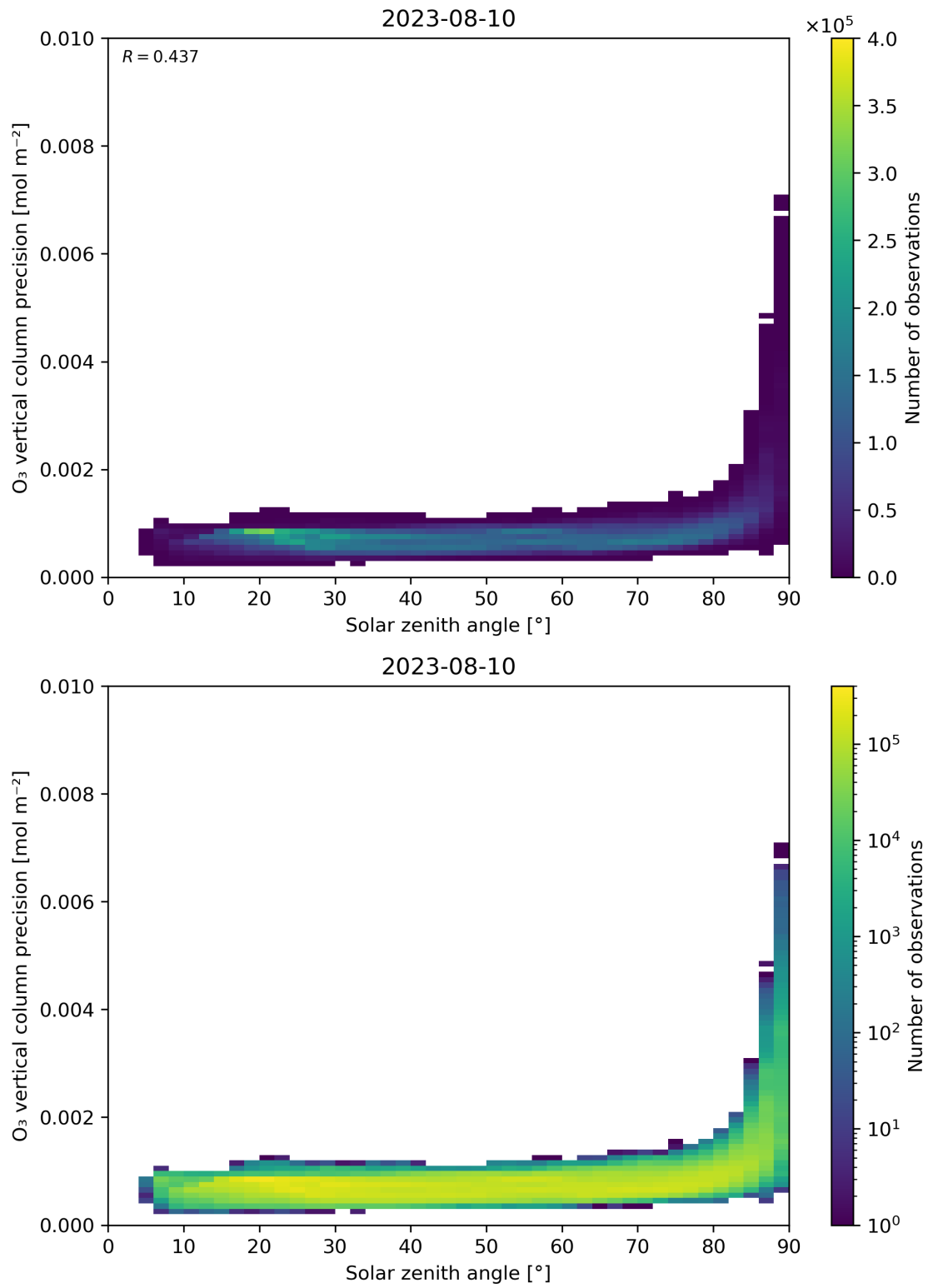
Figure 48: Scatter density plot of “Solar zenith angle” against “O 3 vertical column precision” for 2023-08-09 to 2023-08-11.
