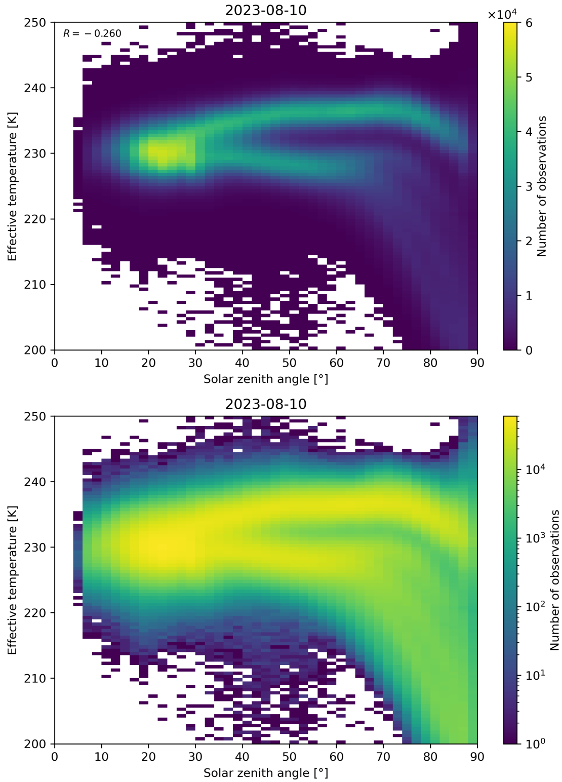
Figure 45: Scatter density plot of “Solar zenith angle” against “Effective temperature” for 2023-08-09 to 2023-08-11.
