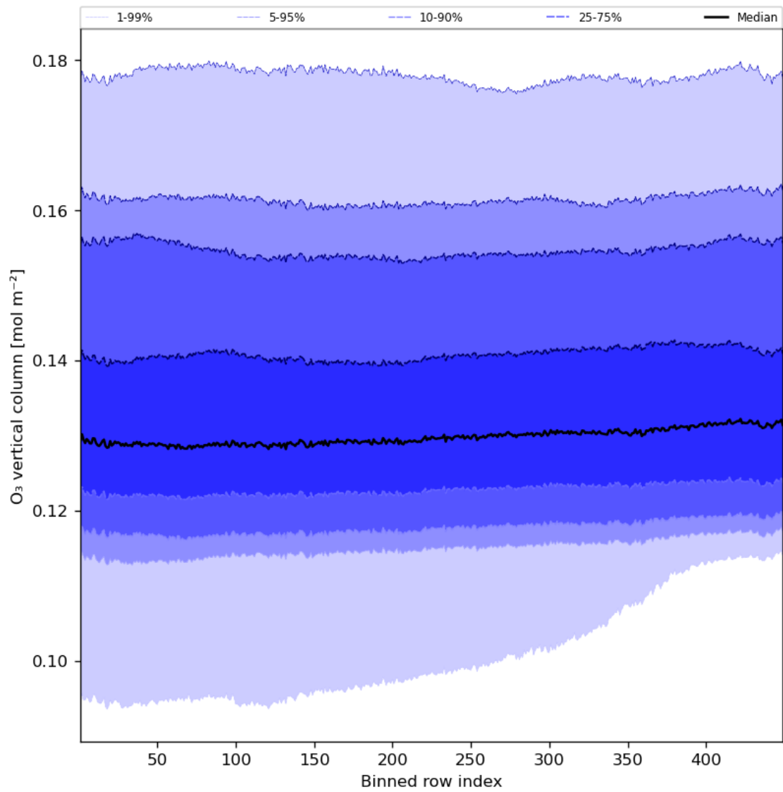
Figure 28: Along track statistics of “O 3 vertical column” for 2023-08-09 to 2023-08-11
