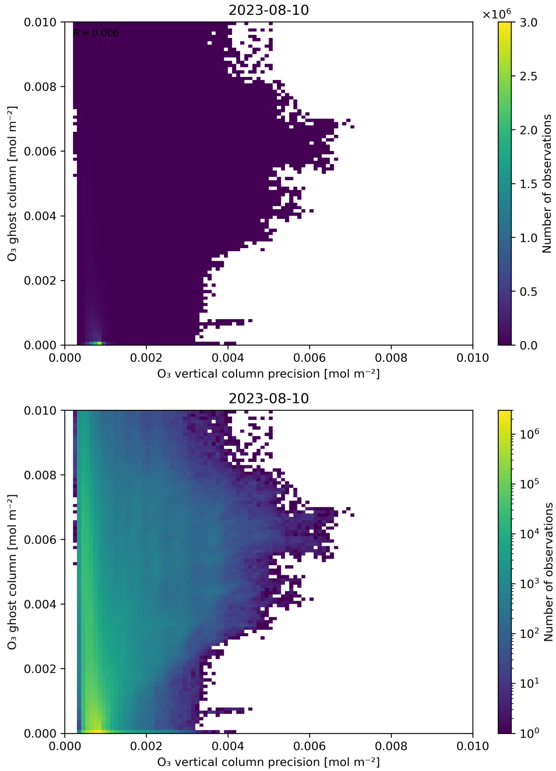
Figure 43: Scatter density plot of “ \text{O}_3 vertical column precision” against “ \text{O}_3 ghost column” for 2023-08-09 to 2023-08-11.
