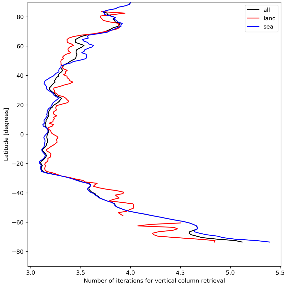
Figure 19: Zonal average of “Number of iterations for vertical column retrieval” for 2023-08-09 to 2023-08-11.
