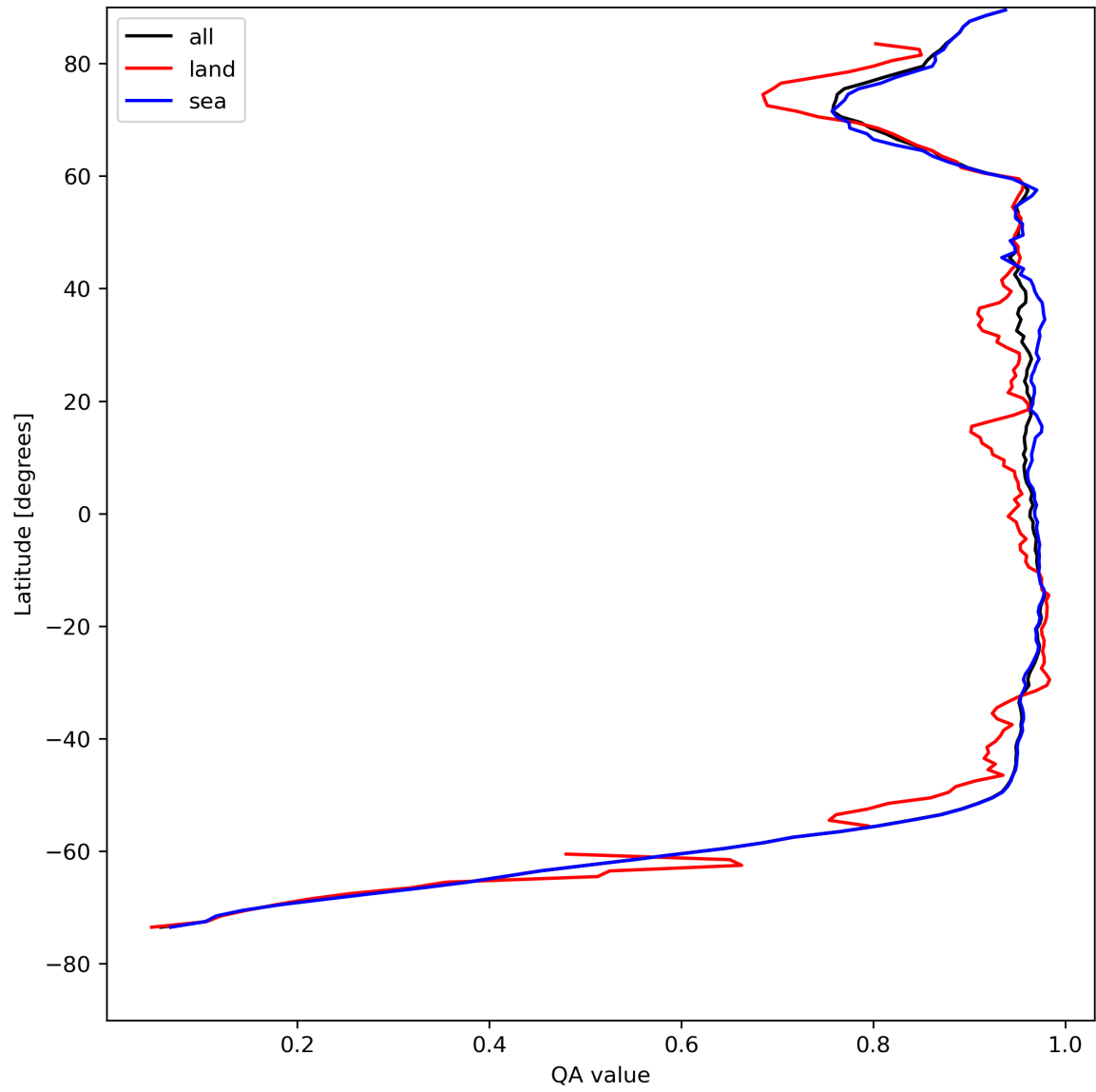
Figure 13: Zonal average of “QA value” for 2023-08-09 to 2023-08-11.
