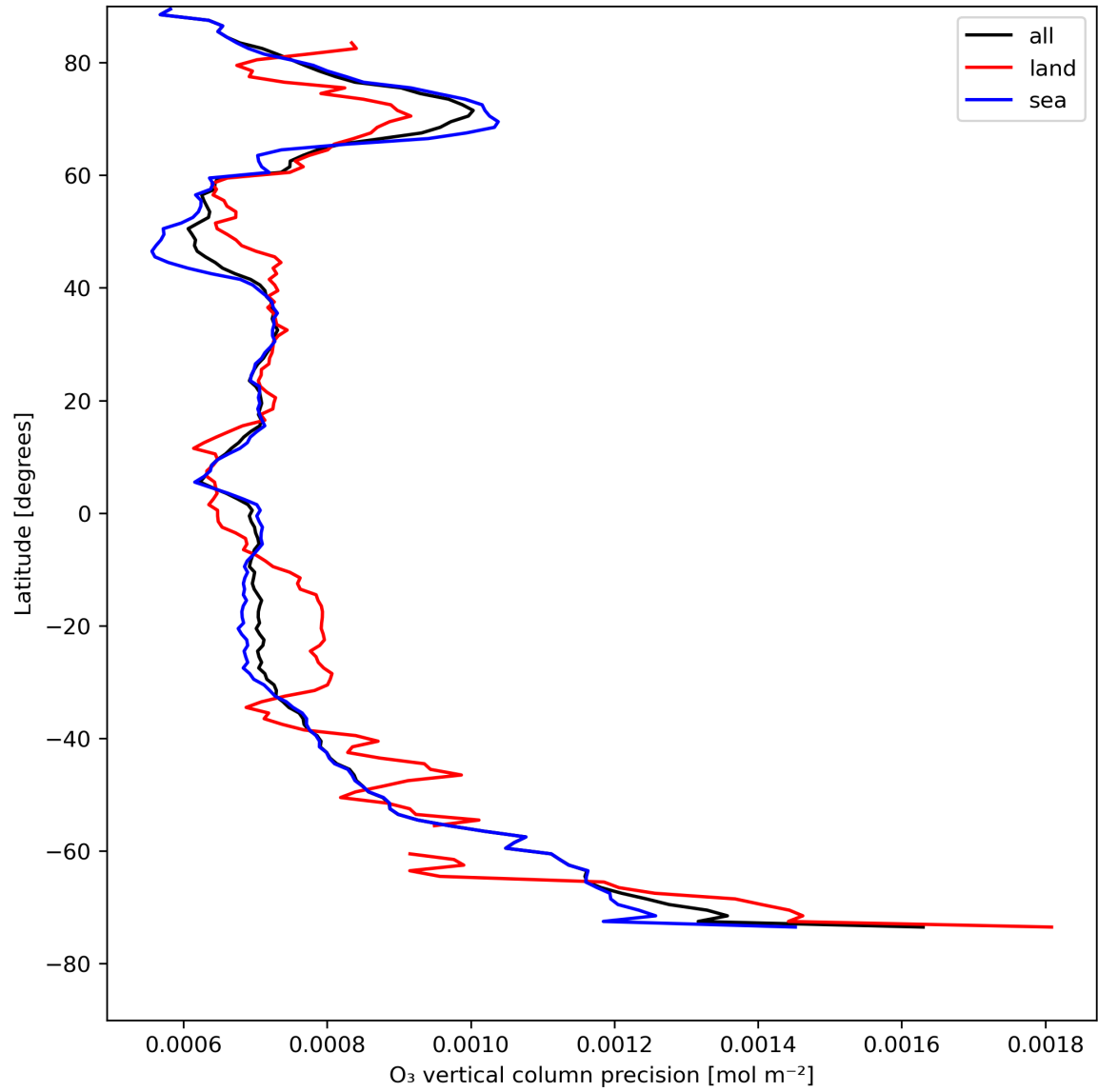
Figure 15: Zonal average of “O 3 vertical column precision” for 2023-08-09 to 2023-08-11.
