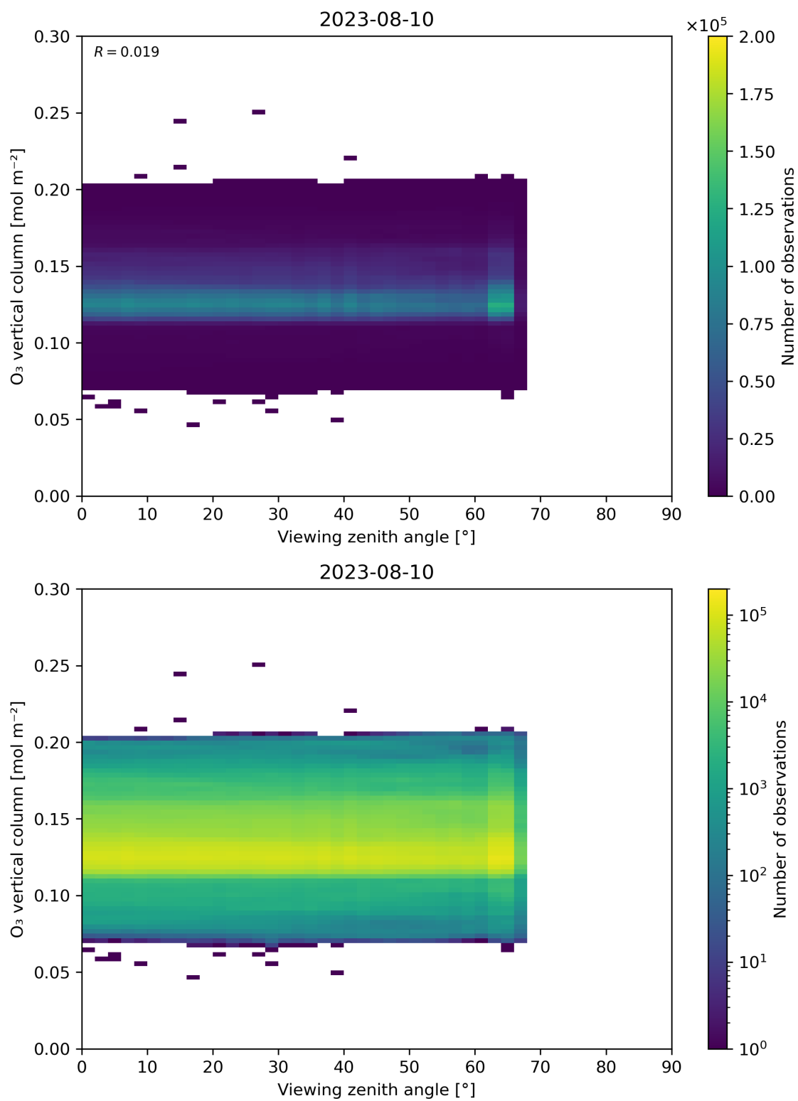
Figure 52: Scatter density plot of “Viewing zenith angle” against “O 3 vertical column” for 2023-08-09 to 2023-08-11.
