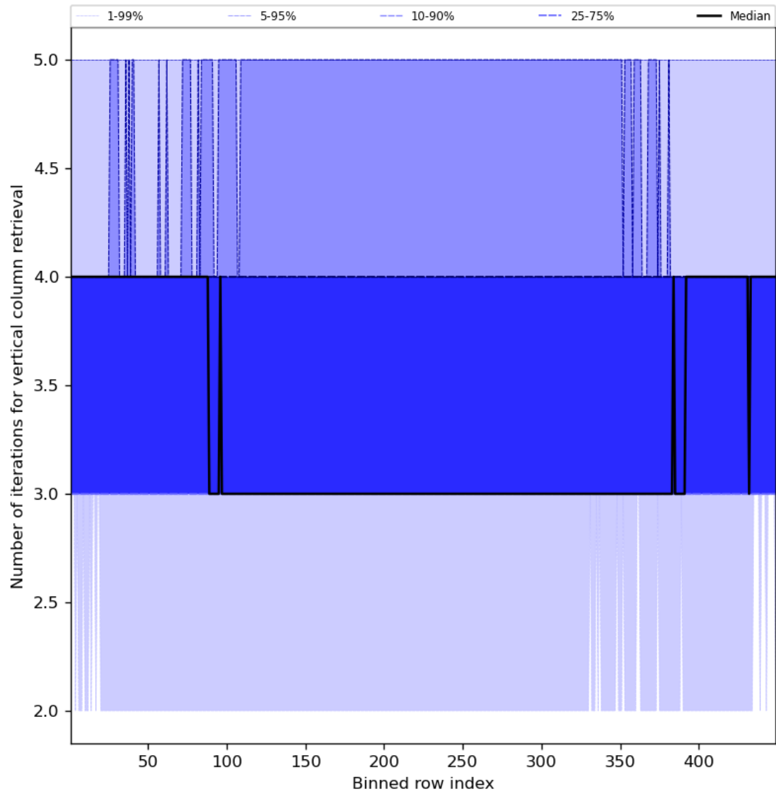
Figure 33: Along track statistics of “Number of iterations for vertical column retrieval” for 2023-08-09 to 2023-08-11
