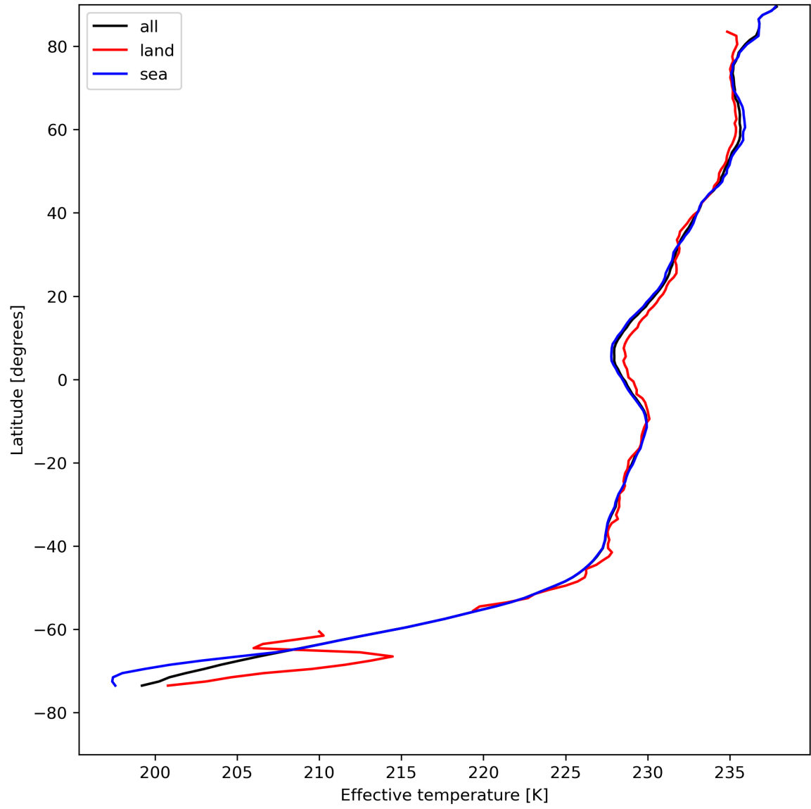
Figure 17: Zonal average of "Effective temperature" for 2023-08-09 to 2023-08-11.
