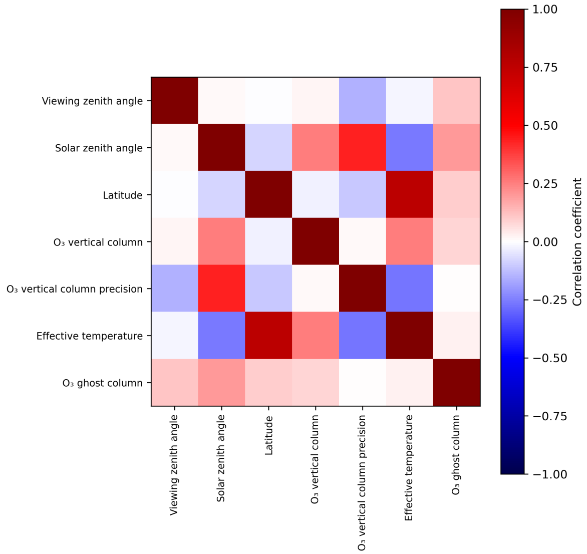
Figure 2: Map of correlation matrix for 2023-08-09 to 2023-08-11.
