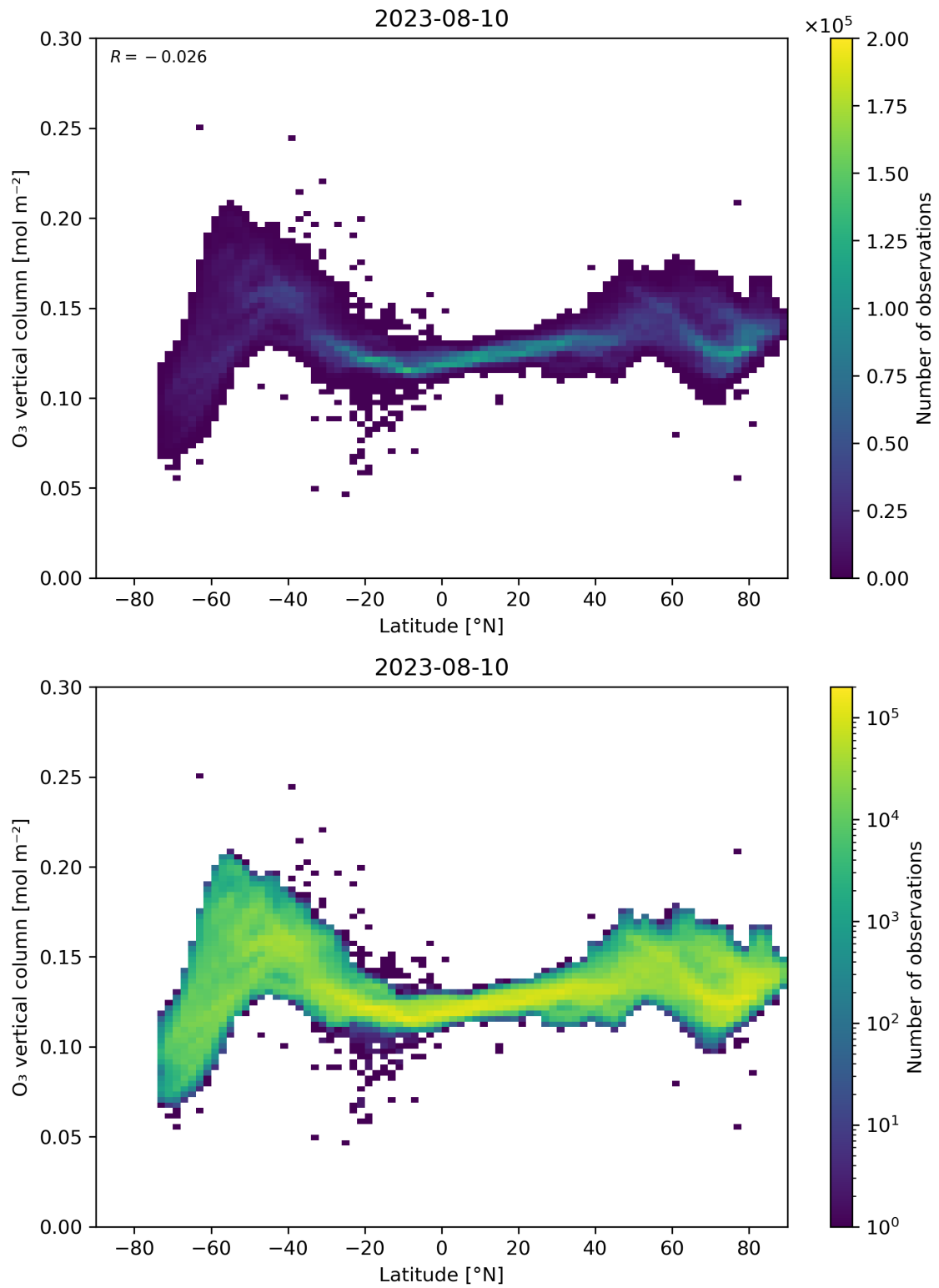
Figure 36: Scatter density plot of “Latitude” against “O 3 vertical column” for 2023-08-09 to 2023-08-11.
