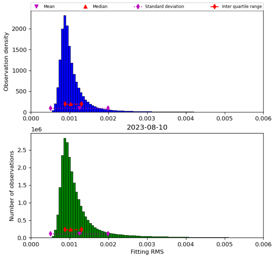
Figure 23: Histogram of “Fitting RMS” for 2023-08-09 to 2023-08-11
