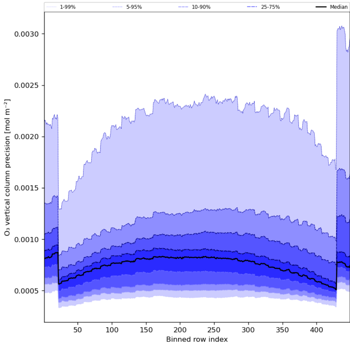
Figure 29: Along track statistics of “O 3 vertical column precision” for 2023-08-09 to 2023-08-11
