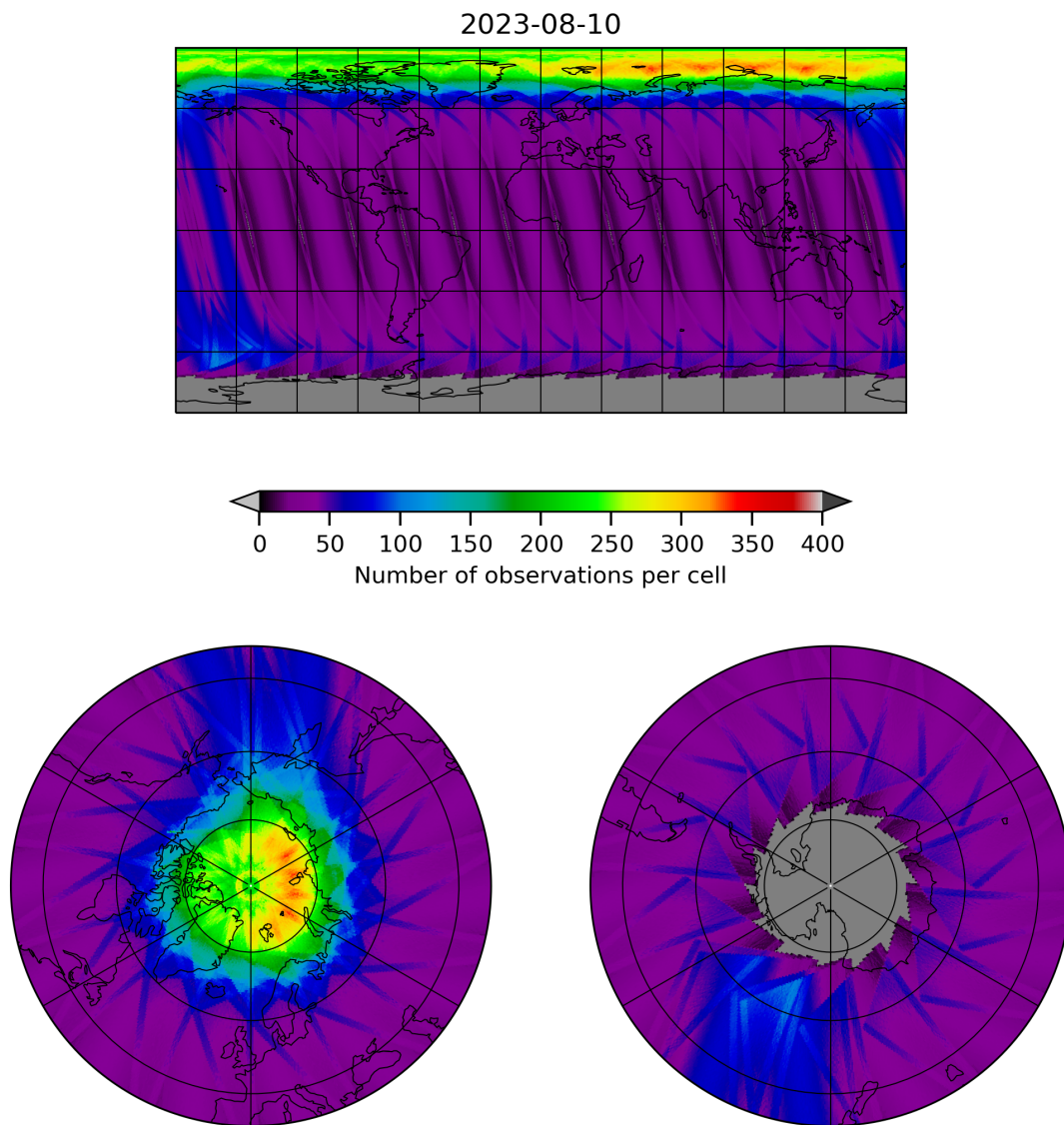
Figure 12: Map of the number of observations for 2023-08-09 to 2023-08-11
