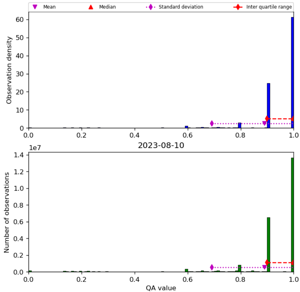
Figure 20: Histogram of “QA value” for 2023-08-09 to 2023-08-11
