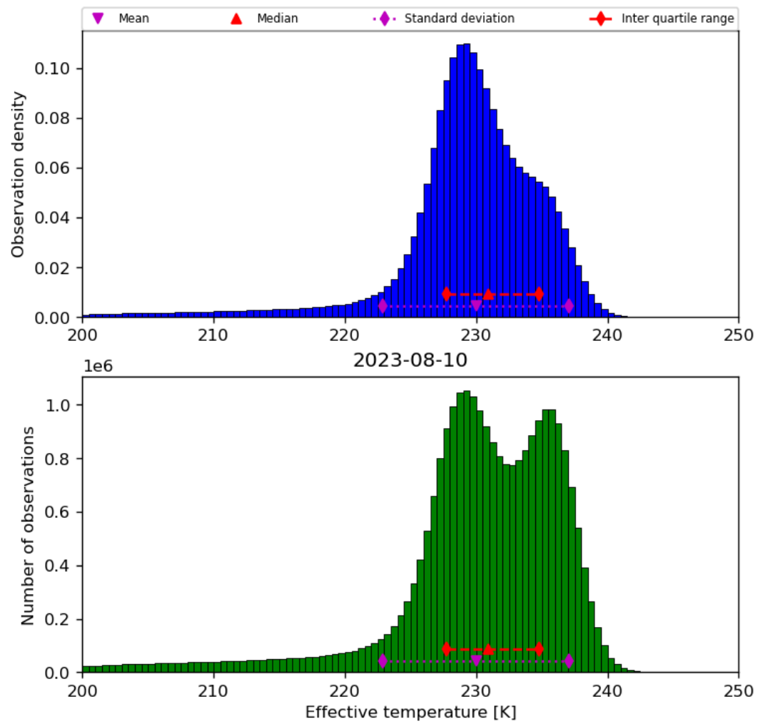
Figure 24: Histogram of “Effective temperature” for 2023-08-09 to 2023-08-11
