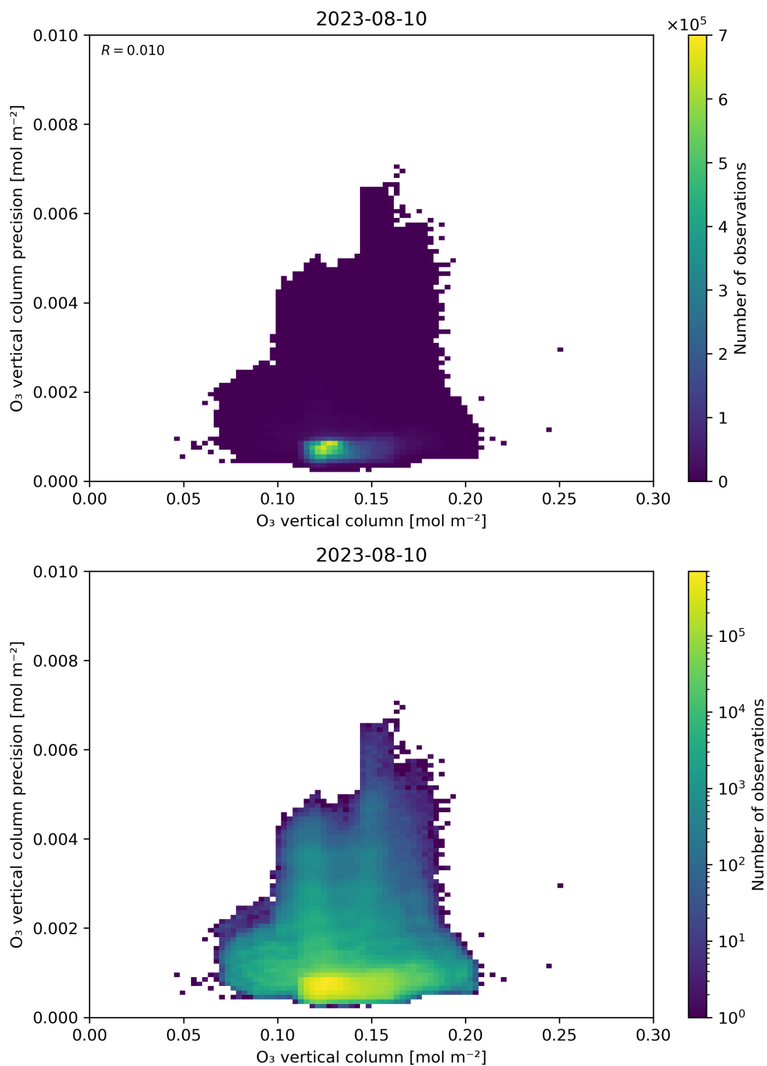
Figure 41: Scatter density plot of “O 3 vertical column” against “O 3 vertical column precision” for 2023-08-09 to 2023-08-11.
