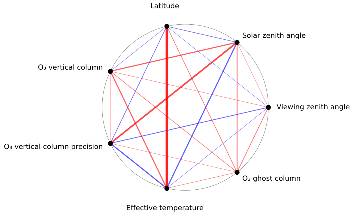
Figure 1: Map of correlation graph for 2023-08-09 to 2023-08-11.
