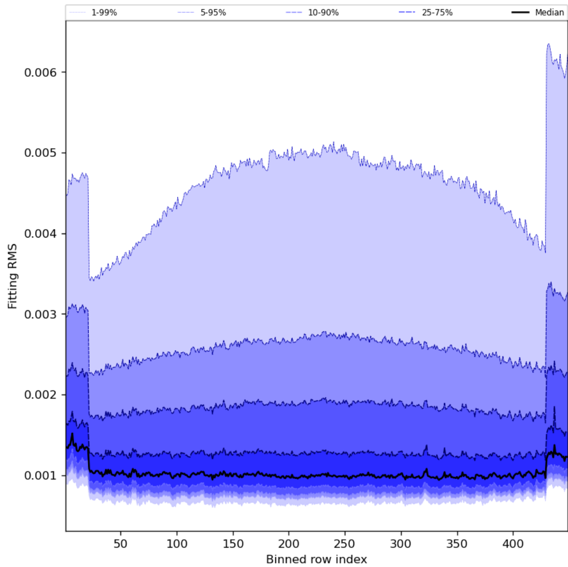
Figure 30: Along track statistics of “Fitting RMS” for 2023-08-09 to 2023-08-11
