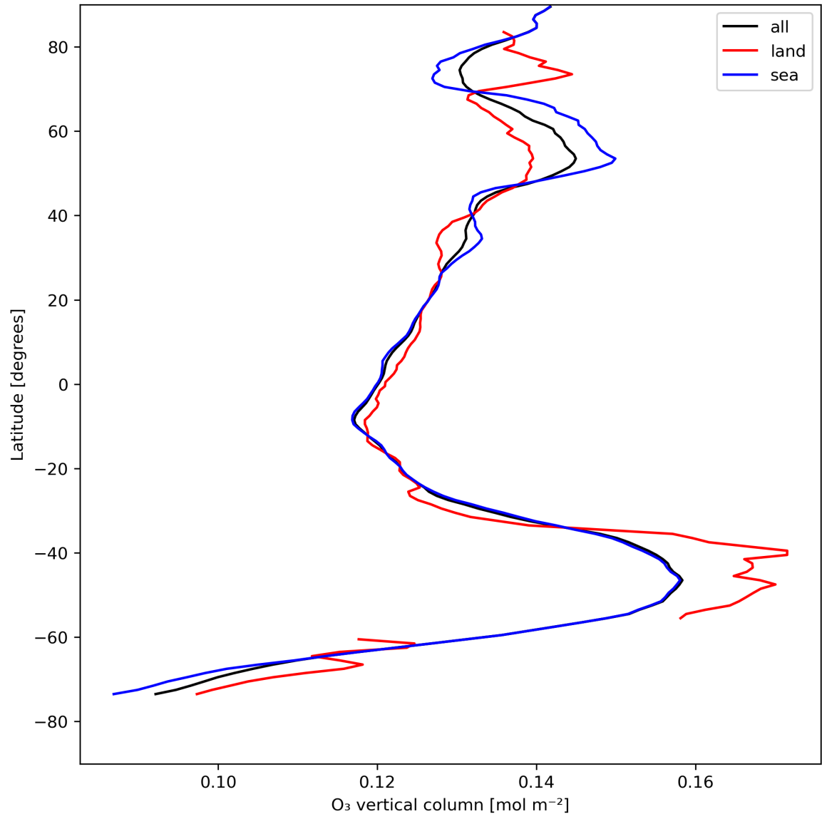
Figure 14: Zonal average of “O 3 vertical column” for 2023-08-09 to 2023-08-11.
