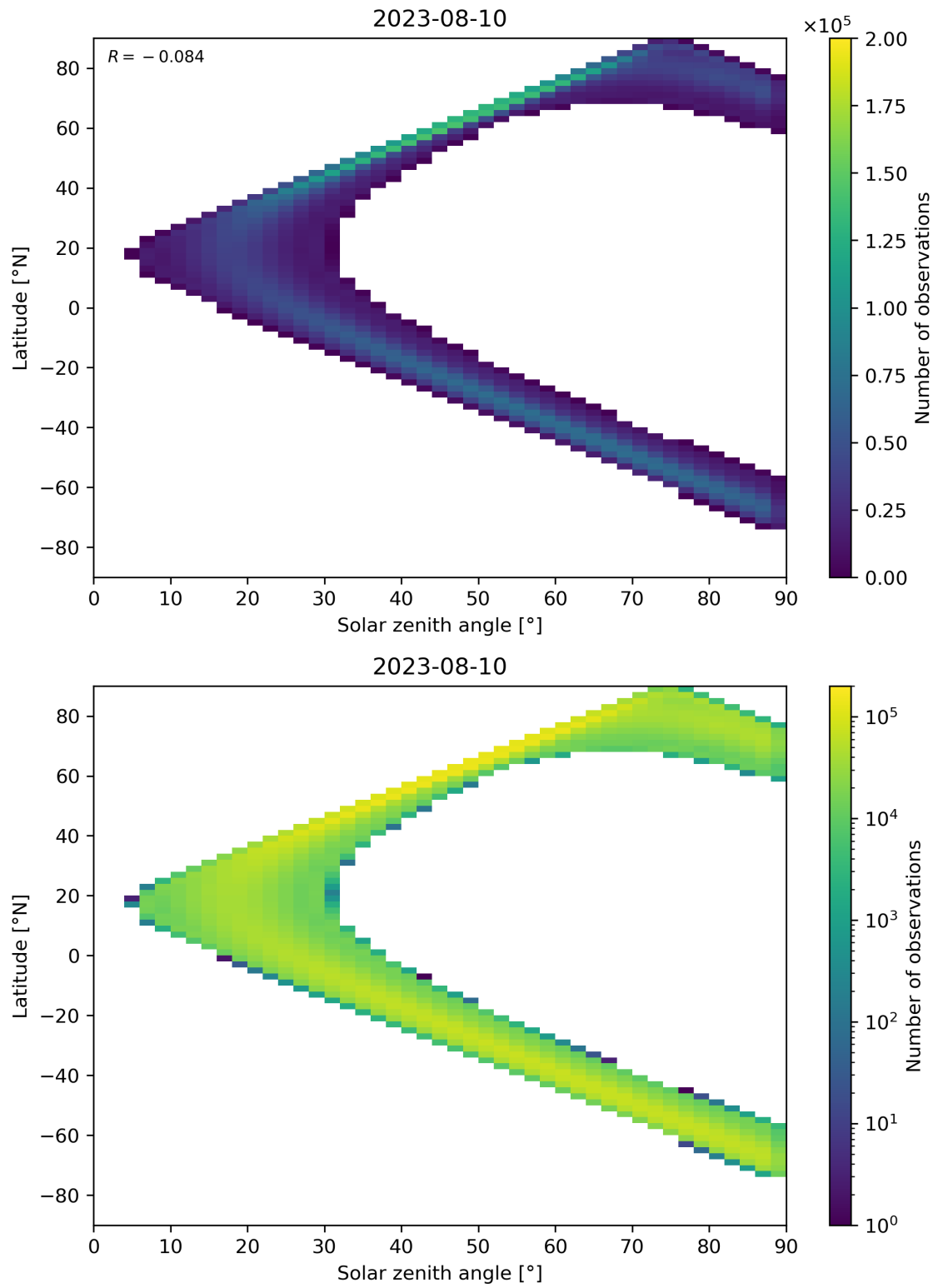
Figure 44: Scatter density plot of “Solar zenith angle” against “Latitude” for 2023-08-09 to 2023-08-11.
