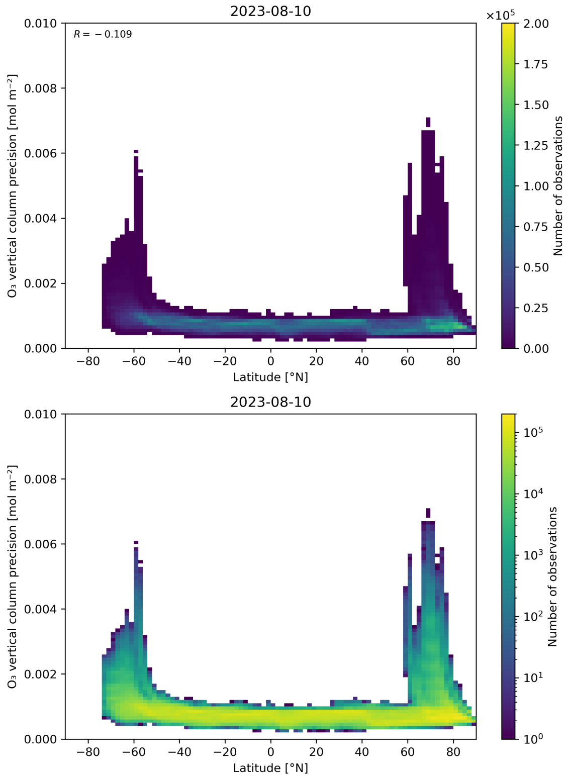
Figure 37: Scatter density plot of “Latitude” against “O 3 vertical column precision” for 2023-08-09 to 2023-08-11.
