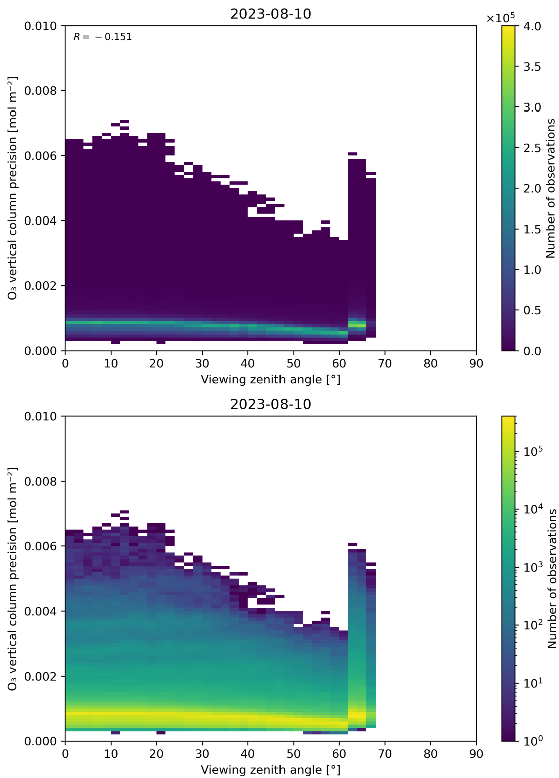
Figure 53: Scatter density plot of “Viewing zenith angle” against “O 3 vertical column precision” for 2023-08-09 to 2023-08-11.
