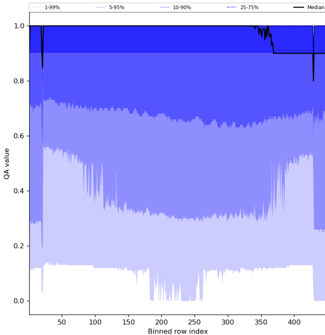
Figure 27: Along track statistics of “QA value” for 2023-08-09 to 2023-08-11
