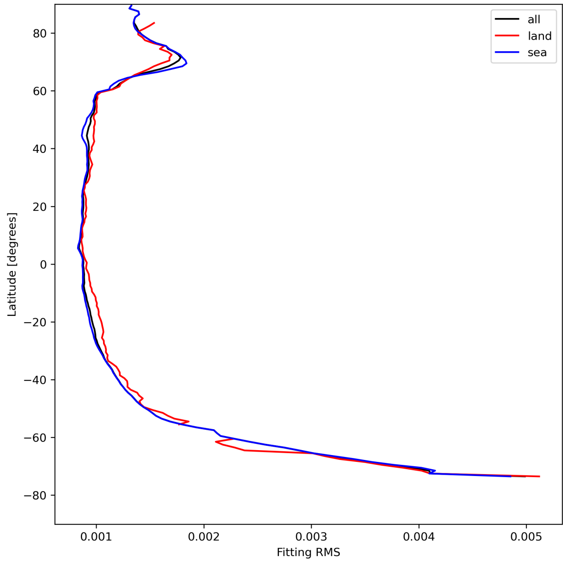
Figure 16: Zonal average of “Fitting RMS” for 2023-08-09 to 2023-08-11.
