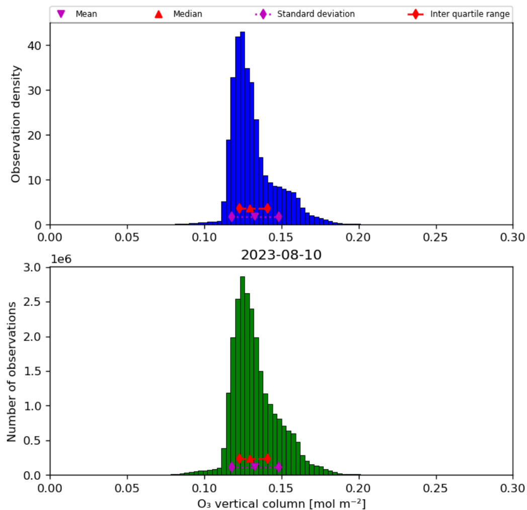
Figure 21: Histogram of “O 3 vertical column” for 2023-08-09 to 2023-08-11
