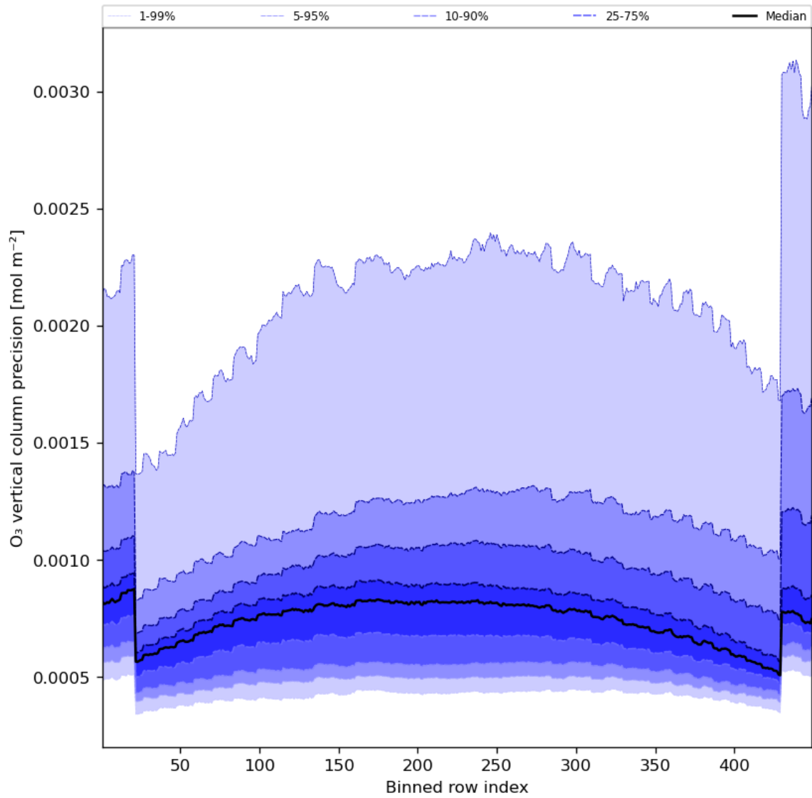
Figure 29: Along track statistics of “O 3 vertical column precision” for 2023-08-10 to 2023-08-12
