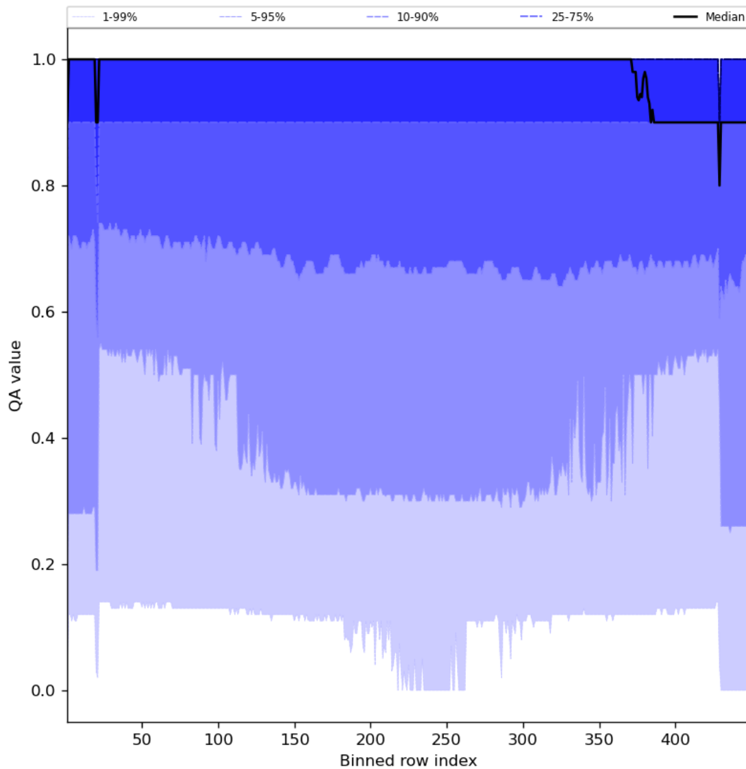
Figure 27: Along track statistics of “QA value” for 2023-08-10 to 2023-08-12
