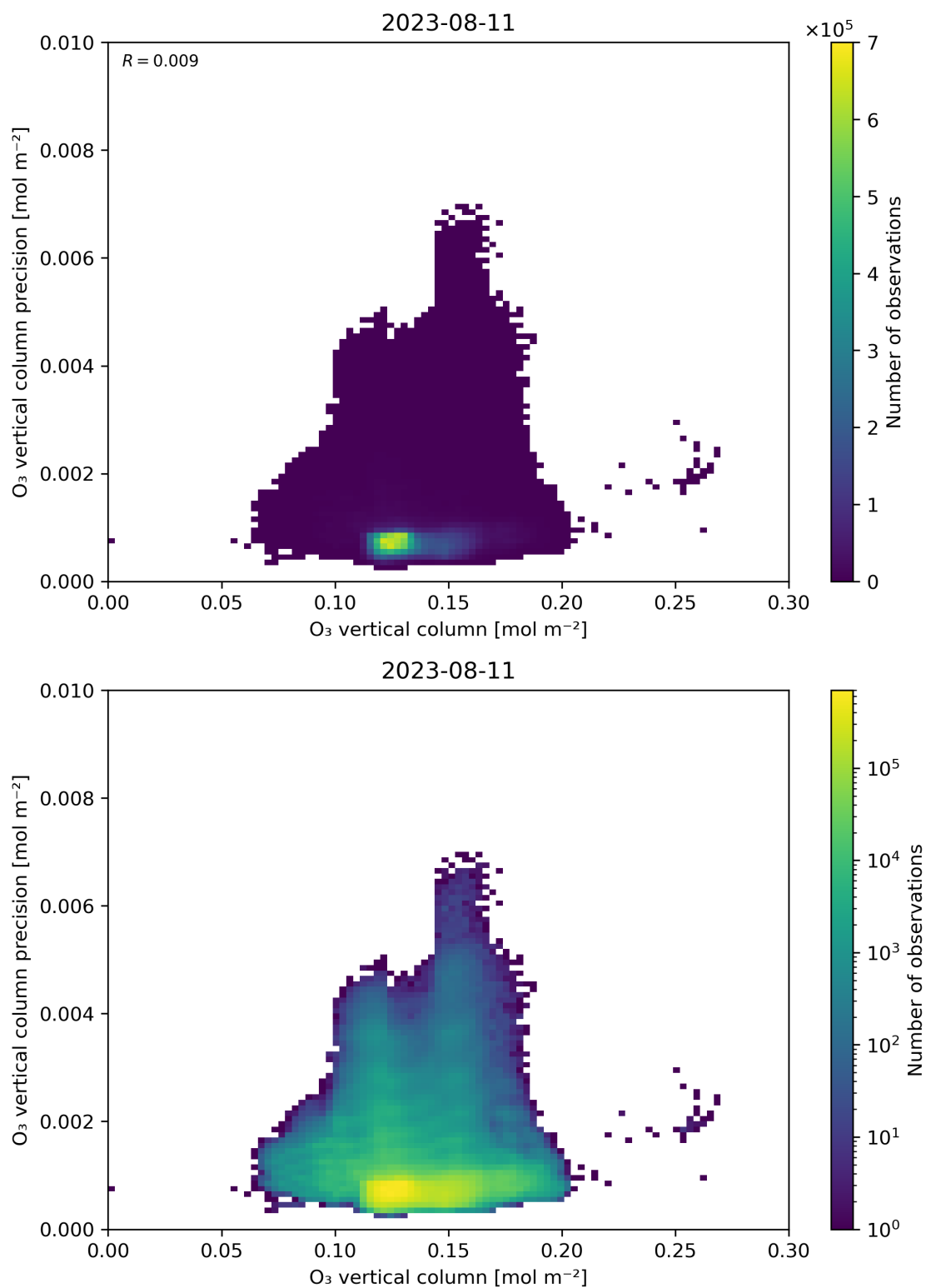
Figure 41: Scatter density plot of “O 3 vertical column” against “O 3 vertical column precision” for 2023-08-10 to 2023-08-12.
