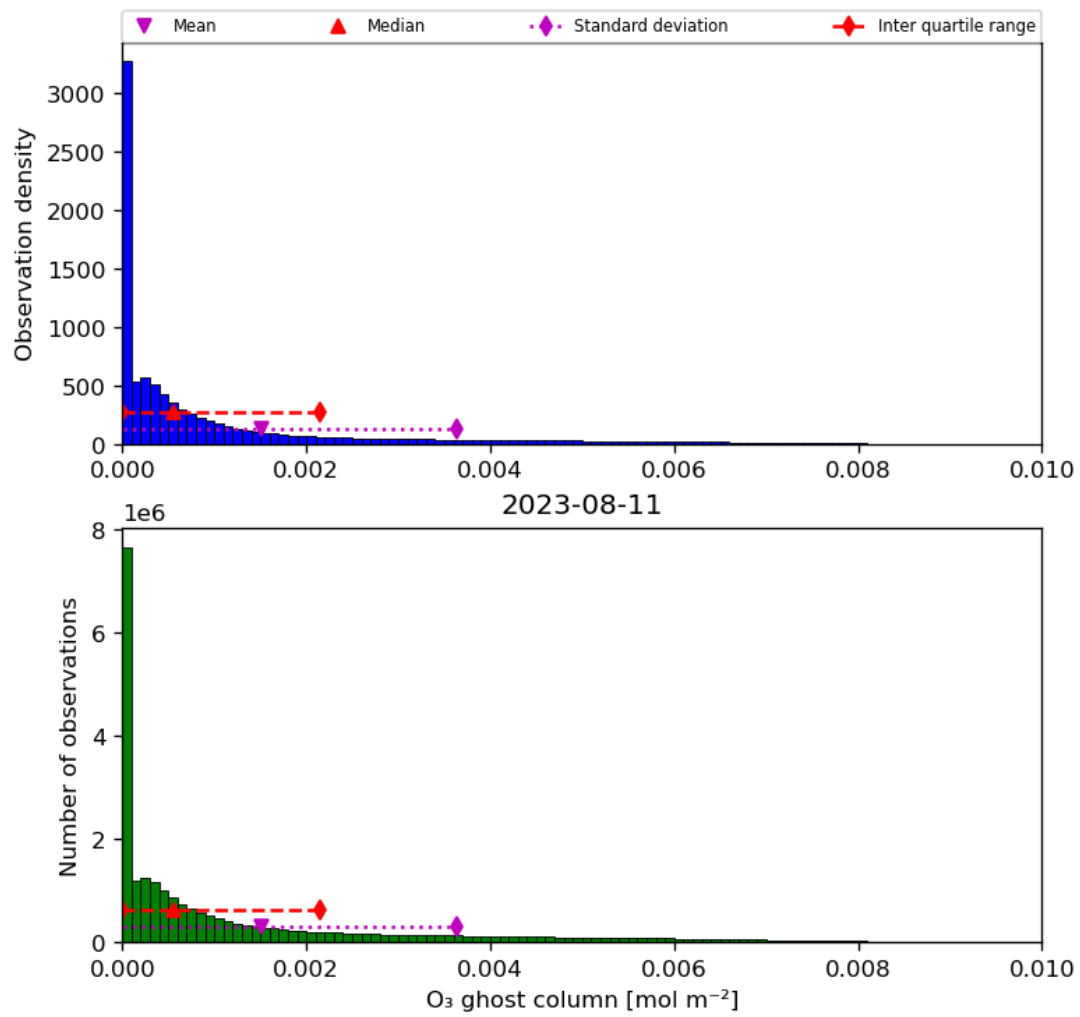
Figure 25: Histogram of “O 3 ghost column” for 2023-08-10 to 2023-08-12
