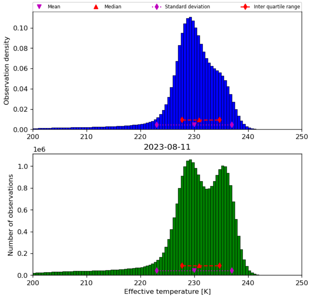
Figure 24: Histogram of “Effective temperature” for 2023-08-10 to 2023-08-12
