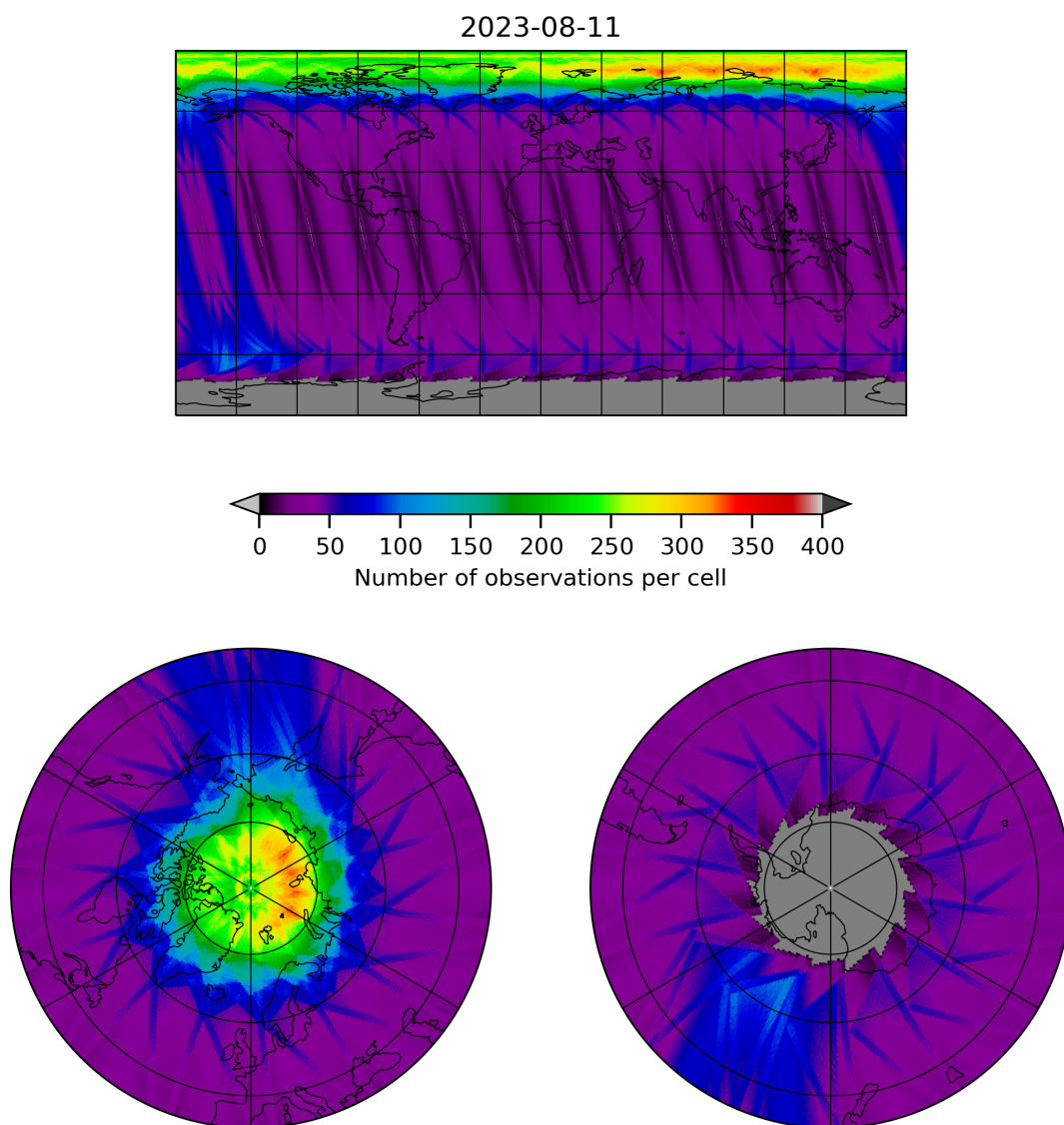
Figure 12: Map of the number of observations for 2023-08-10 to 2023-08-12
