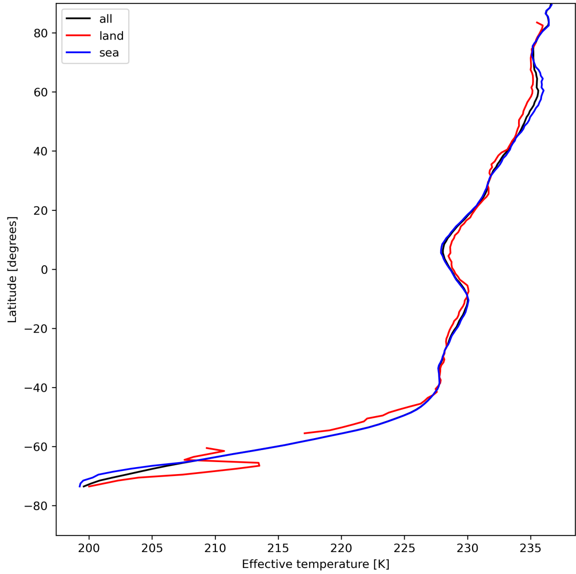
Figure 17: Zonal average of "Effective temperature" for 2023-08-10 to 2023-08-12.
