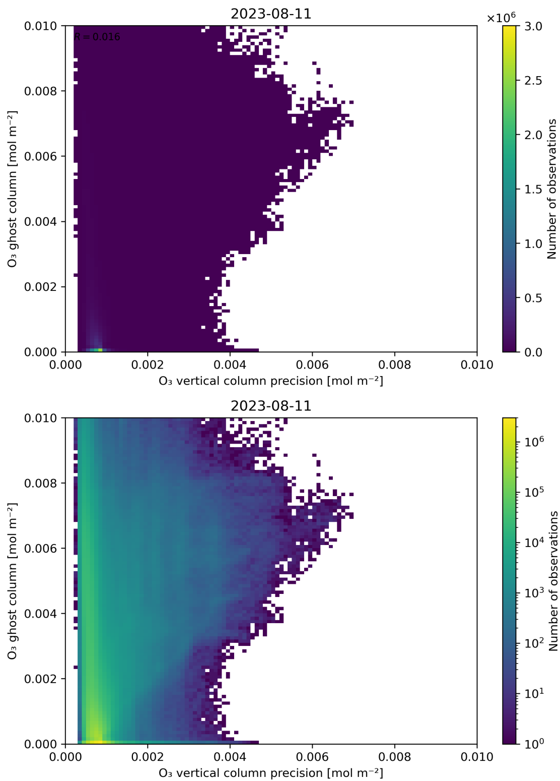
Figure 43: Scatter density plot of “O 3 vertical column precision” against “O 3 ghost column” for 2023-08-10 to 2023-08-12.
