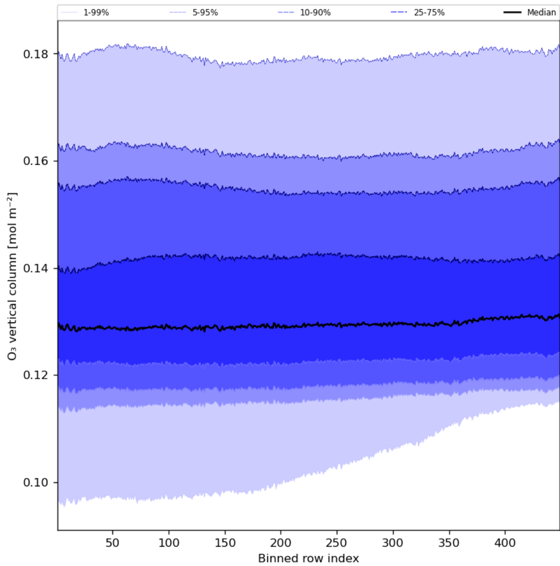
Figure 28: Along track statistics of “O 3 vertical column” for 2023-08-10 to 2023-08-12
