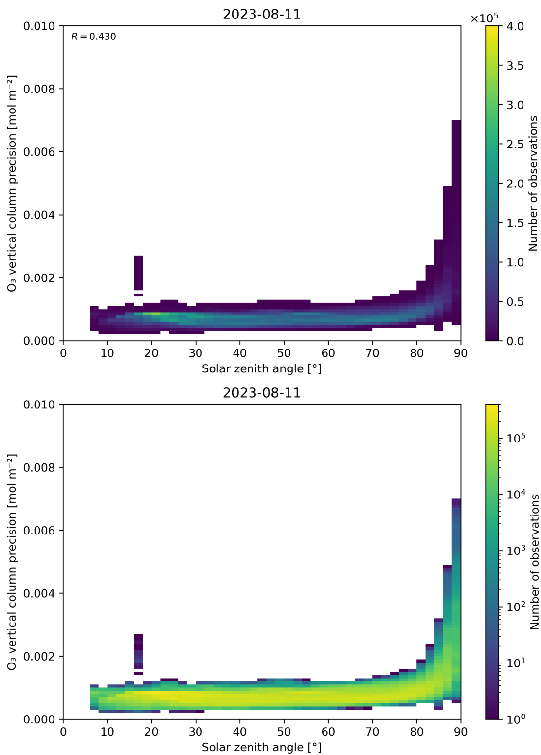
Figure 48: Scatter density plot of “Solar zenith angle” against “O 3 vertical column precision” for 2023-08-10 to 2023-08-12.
