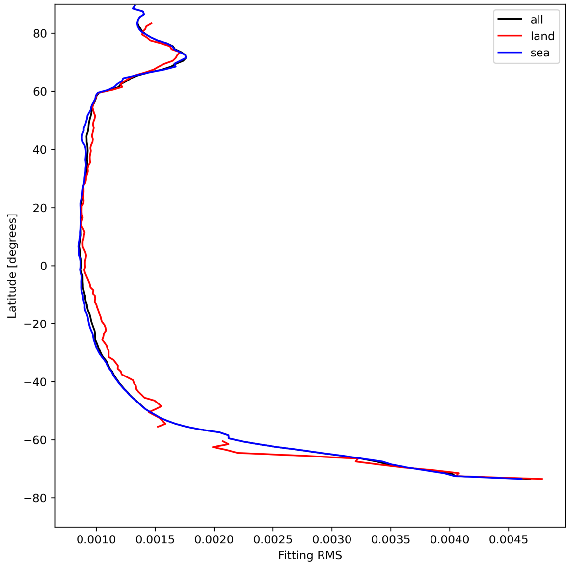
Figure 16: Zonal average of “Fitting RMS” for 2023-08-10 to 2023-08-12.
