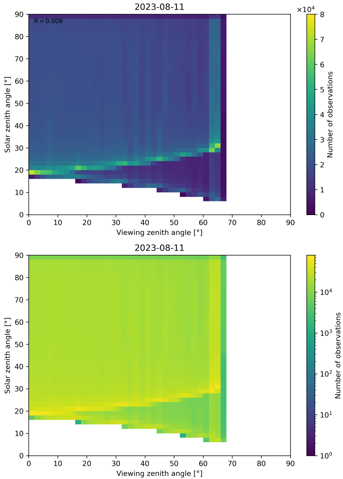
Figure 54: Scatter density plot of “Viewing zenith angle” against “Solar zenith angle” for 2023-08-10 to 2023-08-12.
