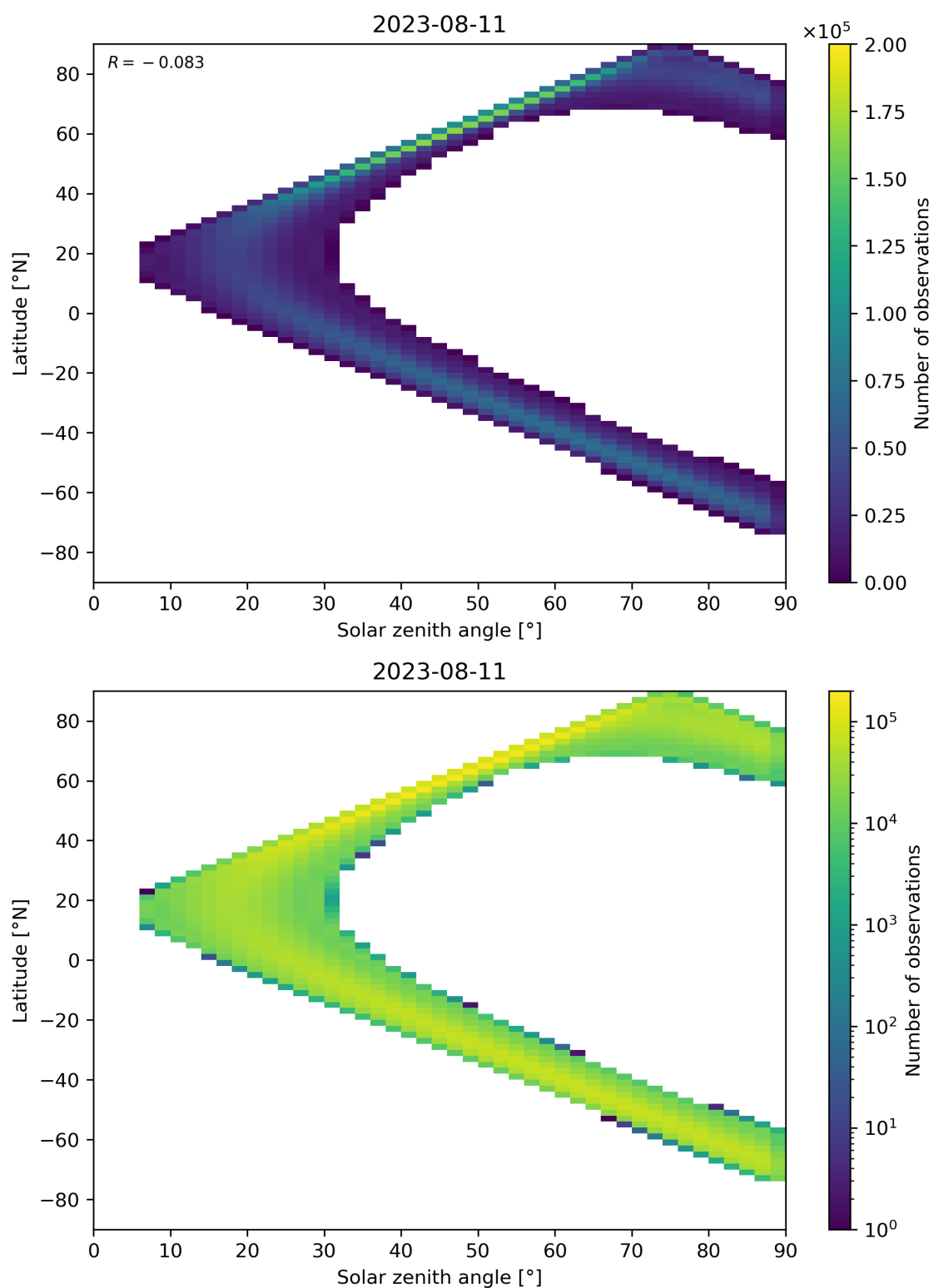
Figure 44: Scatter density plot of “Solar zenith angle” against “Latitude” for 2023-08-10 to 2023-08-12.
