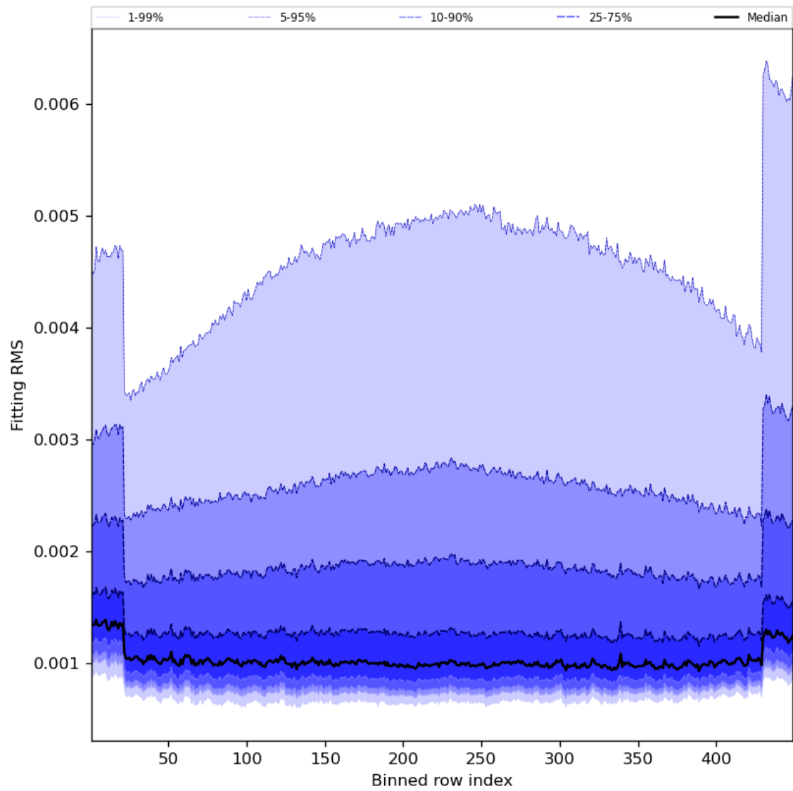
Figure 30: Along track statistics of “Fitting RMS” for 2023-08-10 to 2023-08-12
