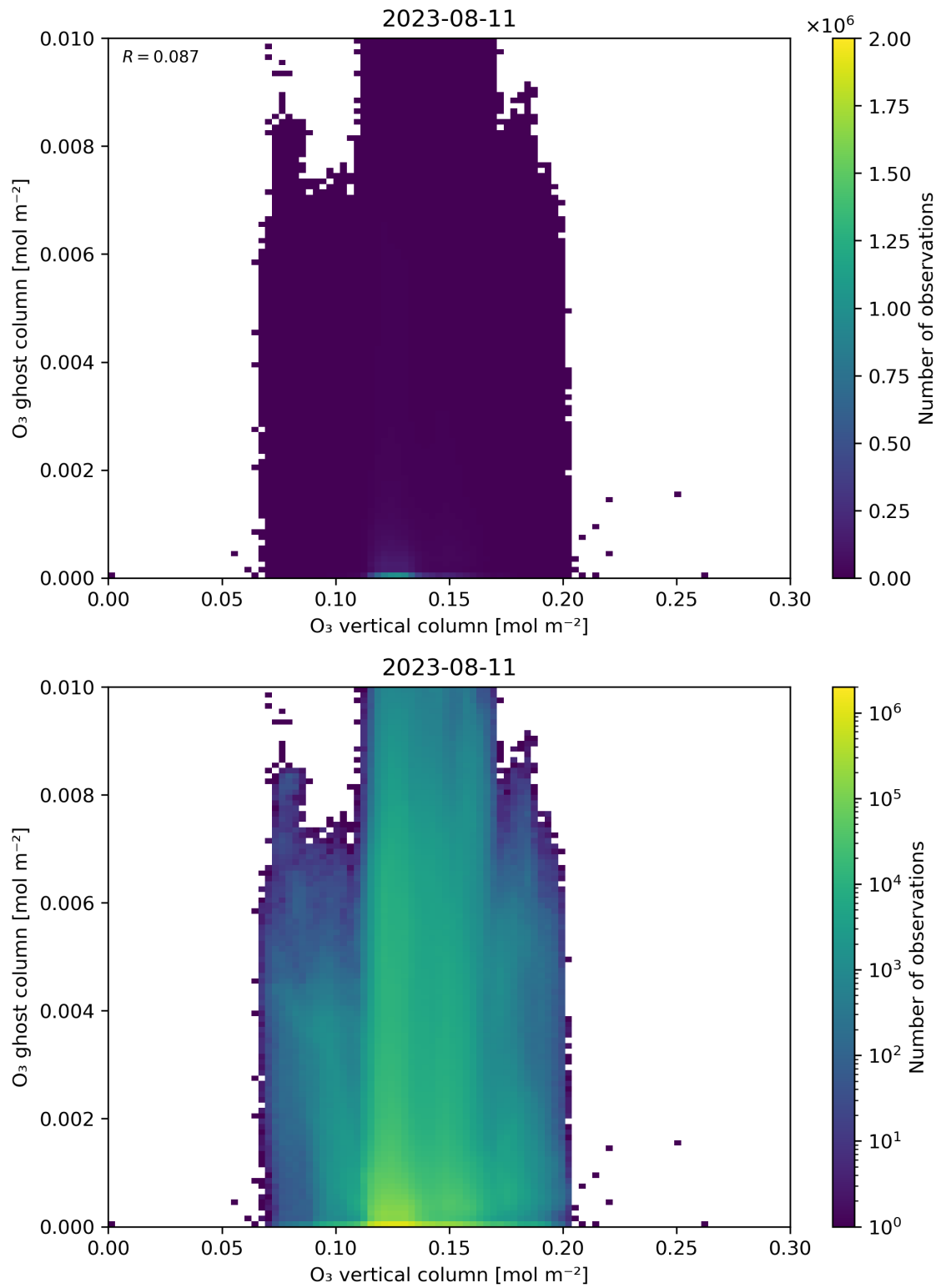
Figure 40: Scatter density plot of “O 3 vertical column” against “O 3 ghost column” for 2023-08-10 to 2023-08-12.
