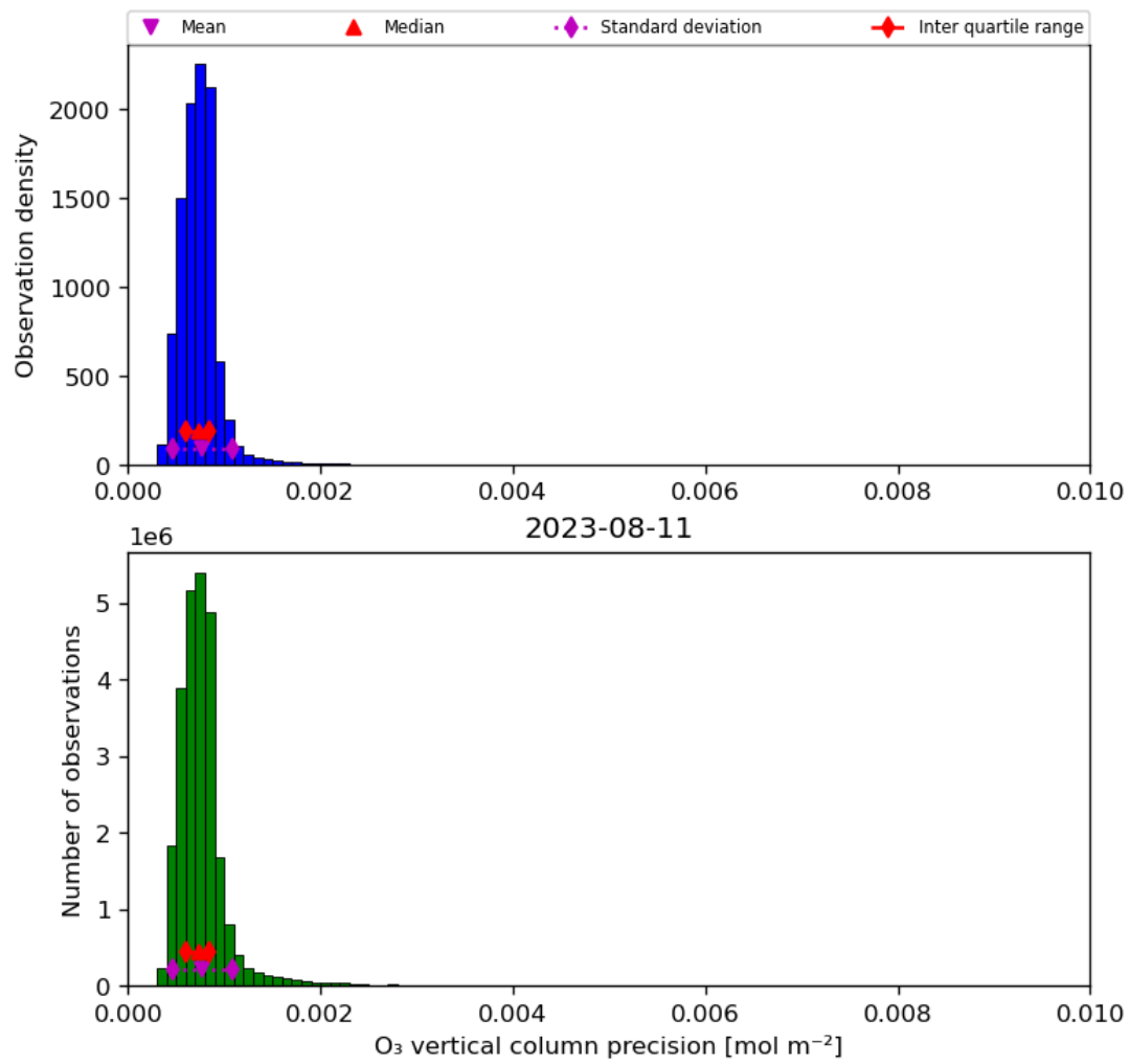
Figure 22: Histogram of “O 3 vertical column precision” for 2023-08-10 to 2023-08-12
