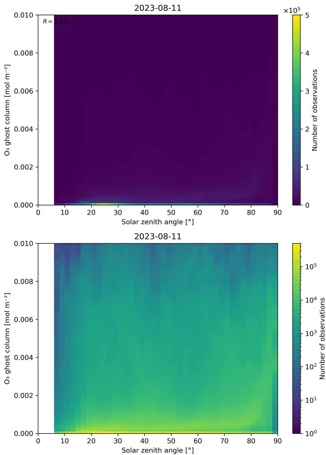
Figure 46: Scatter density plot of “Solar zenith angle” against “O 3 ghost column” for 2023-08-10 to 2023-08-12.
