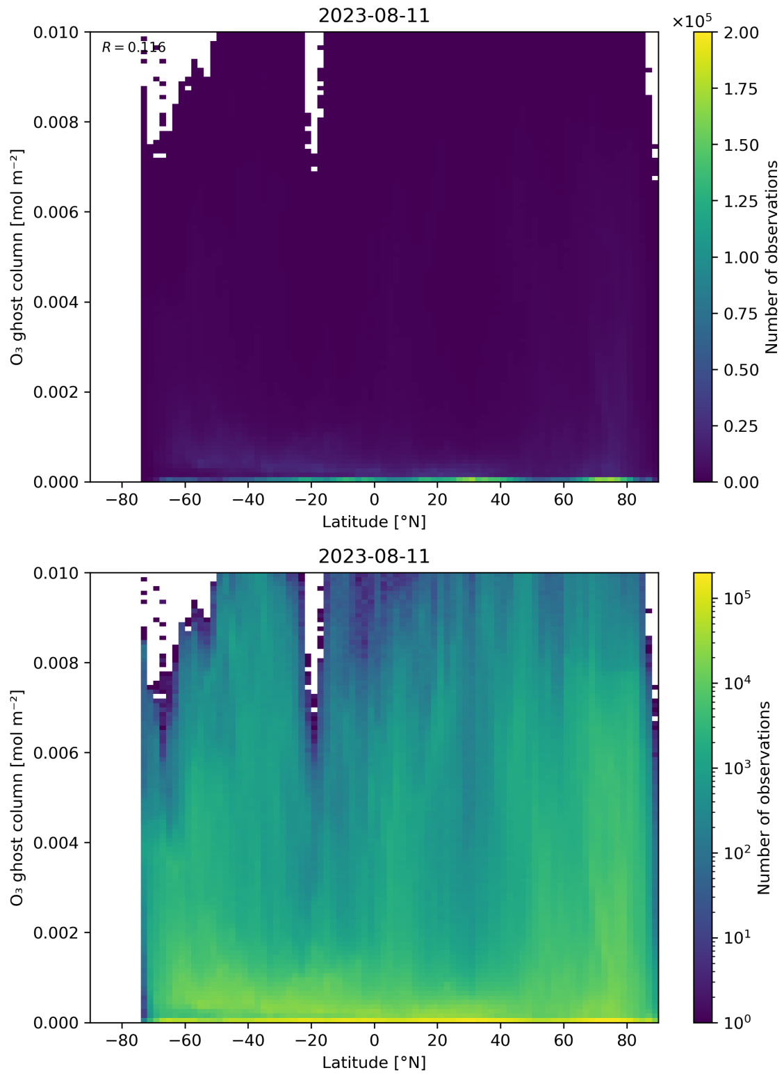
Figure 35: Scatter density plot of “Latitude” against “O 3 ghost column” for 2023-08-10 to 2023-08-12.
