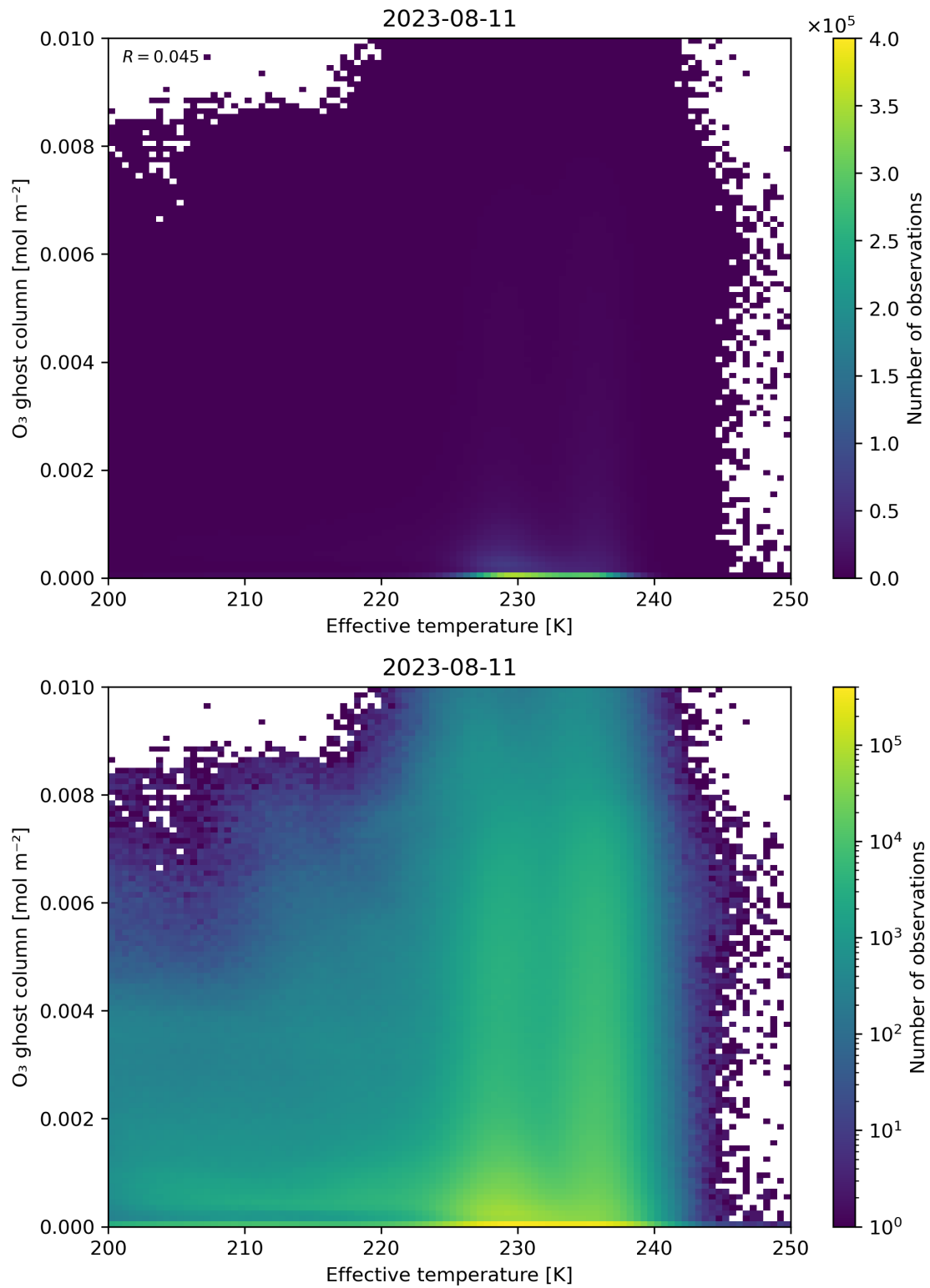
Figure 38: Scatter density plot of “Effective temperature” against “O 3 ghost column” for 2023-08-10 to 2023-08-12.
