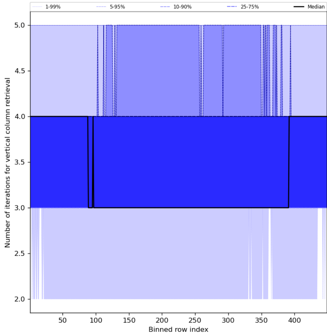
Figure 33: Along track statistics of “Number of iterations for vertical column retrieval” for 2023-08-10 to 2023-08-12
