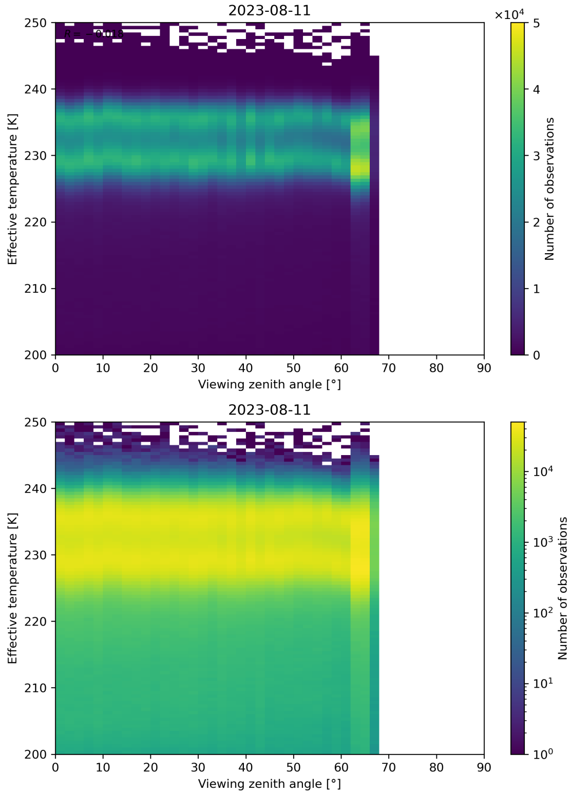
Figure 50: Scatter density plot of “Viewing zenith angle” against “Effective temperature” for 2023-08-10 to 2023-08-12.
