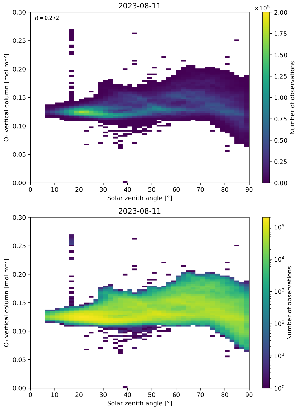
Figure 47: Scatter density plot of “Solar zenith angle” against “O 3 vertical column” for 2023-08-10 to 2023-08-12.
