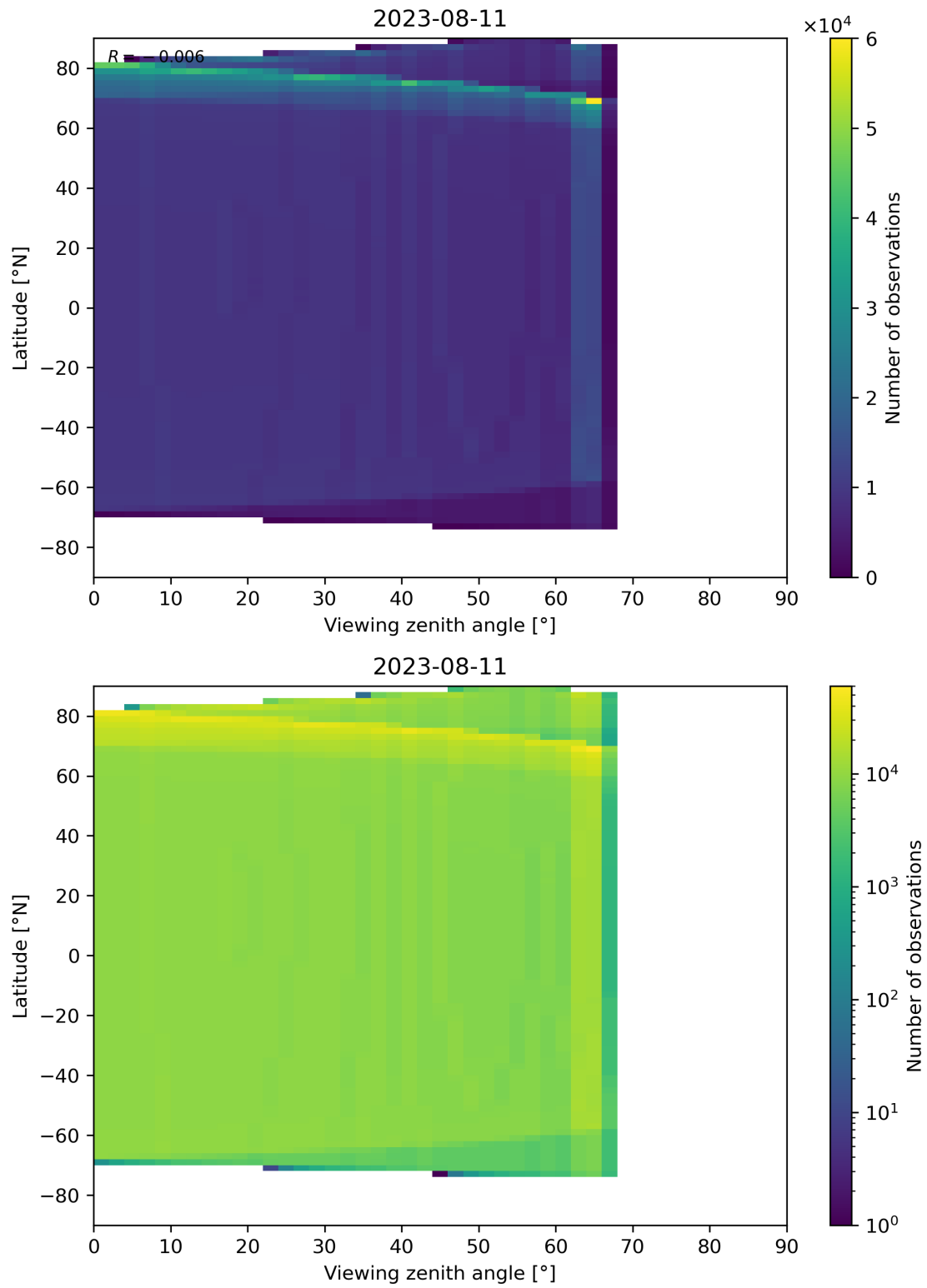
Figure 49: Scatter density plot of “Viewing zenith angle” against “Latitude” for 2023-08-10 to 2023-08-12.
