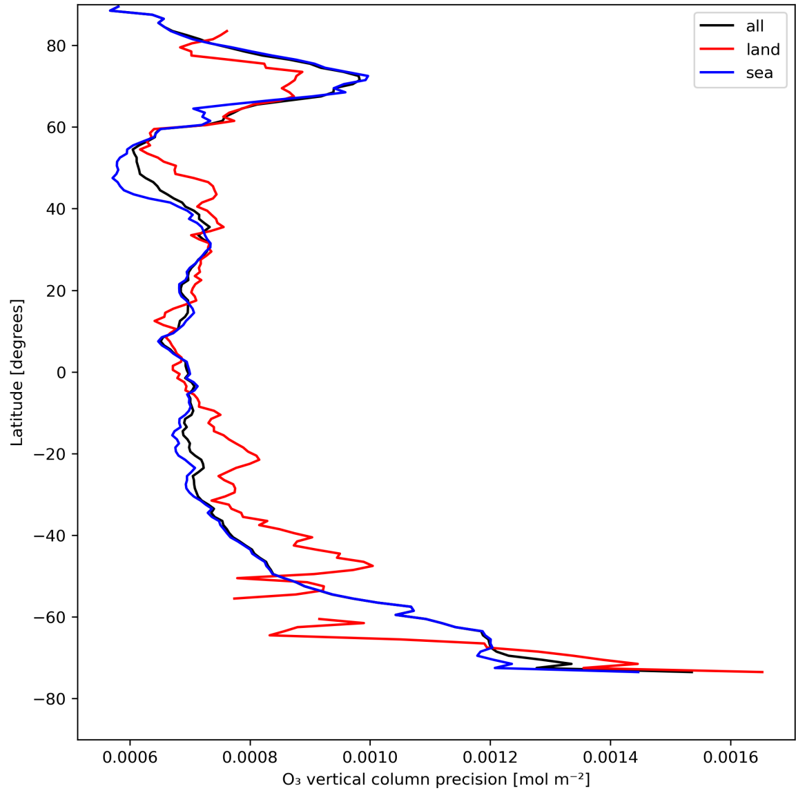
Figure 15: Zonal average of “O 3 vertical column precision” for 2023-08-10 to 2023-08-12.
