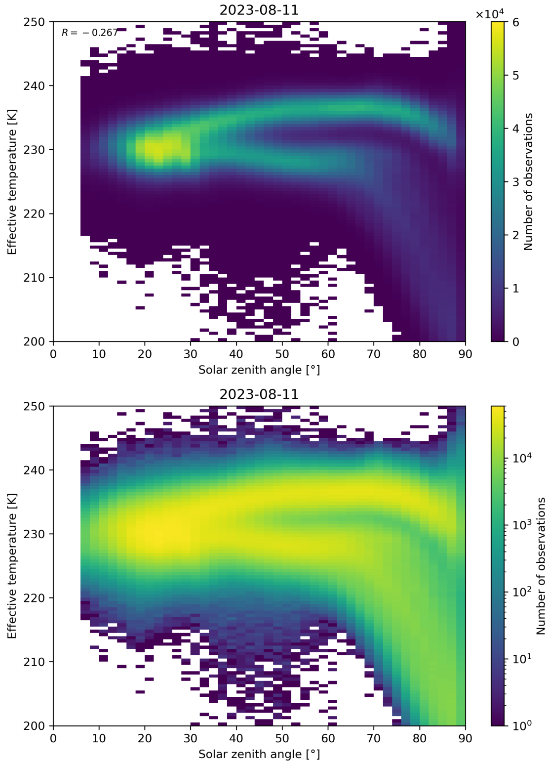
Figure 45: Scatter density plot of “Solar zenith angle” against “Effective temperature” for 2023-08-10 to 2023-08-12.
