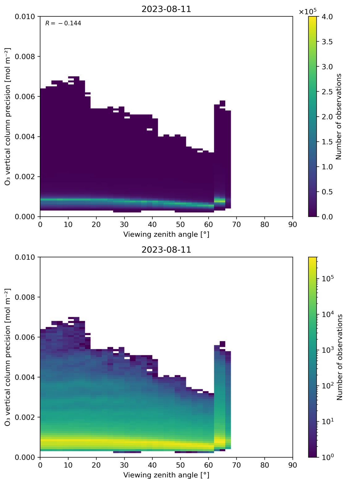
Figure 53: Scatter density plot of “Viewing zenith angle” against “O 3 vertical column precision” for 2023-08-10 to 2023-08-12.
