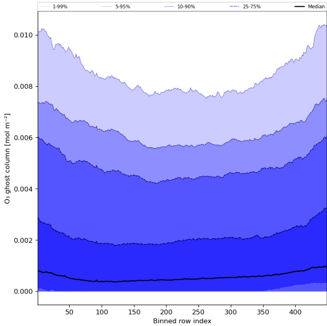
Figure 32: Along track statistics of "O 3 ghost column" for 2023-08-10 to 2023-08-12
