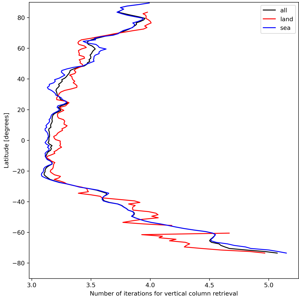
Figure 19: Zonal average of “Number of iterations for vertical column retrieval” for 2023-08-10 to 2023-08-12.
