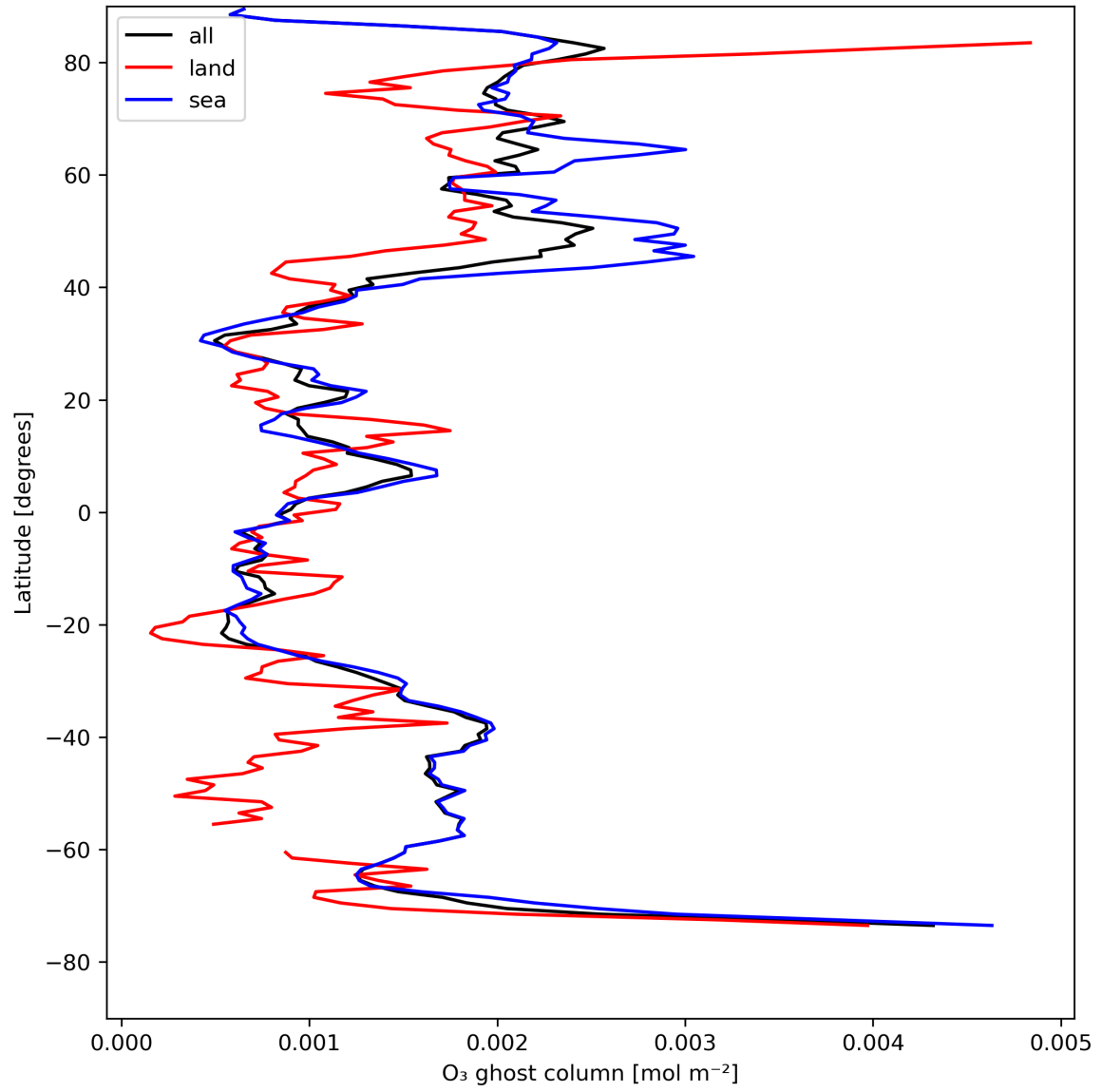
Figure 18: Zonal average of “O 3 ghost column” for 2023-08-10 to 2023-08-12.
