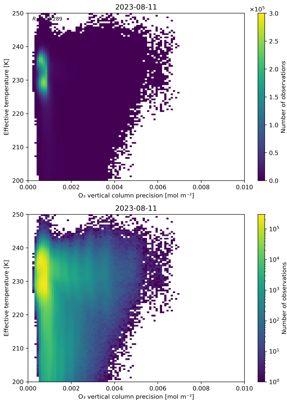
Figure 42: Scatter density plot of “O 3 vertical column precision” against “Effective temperature” for 2023-08-10 to 2023-08-12.
