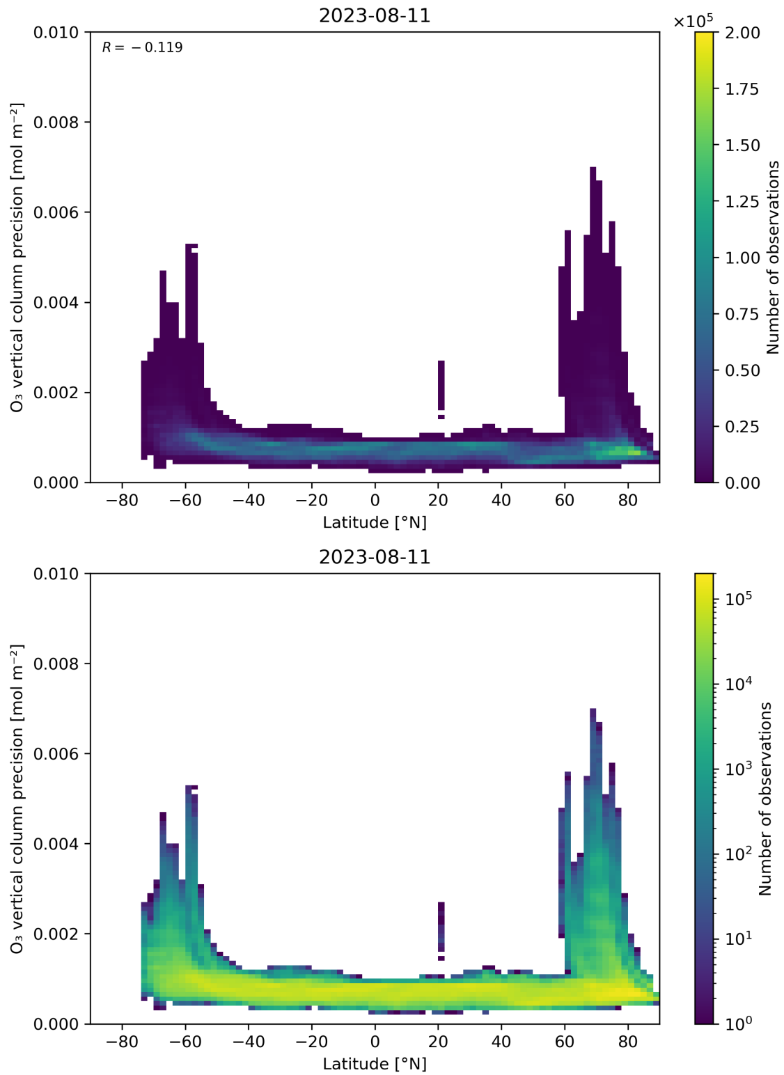
Figure 37: Scatter density plot of “Latitude” against “O 3 vertical column precision” for 2023-08-10 to 2023-08-12.
