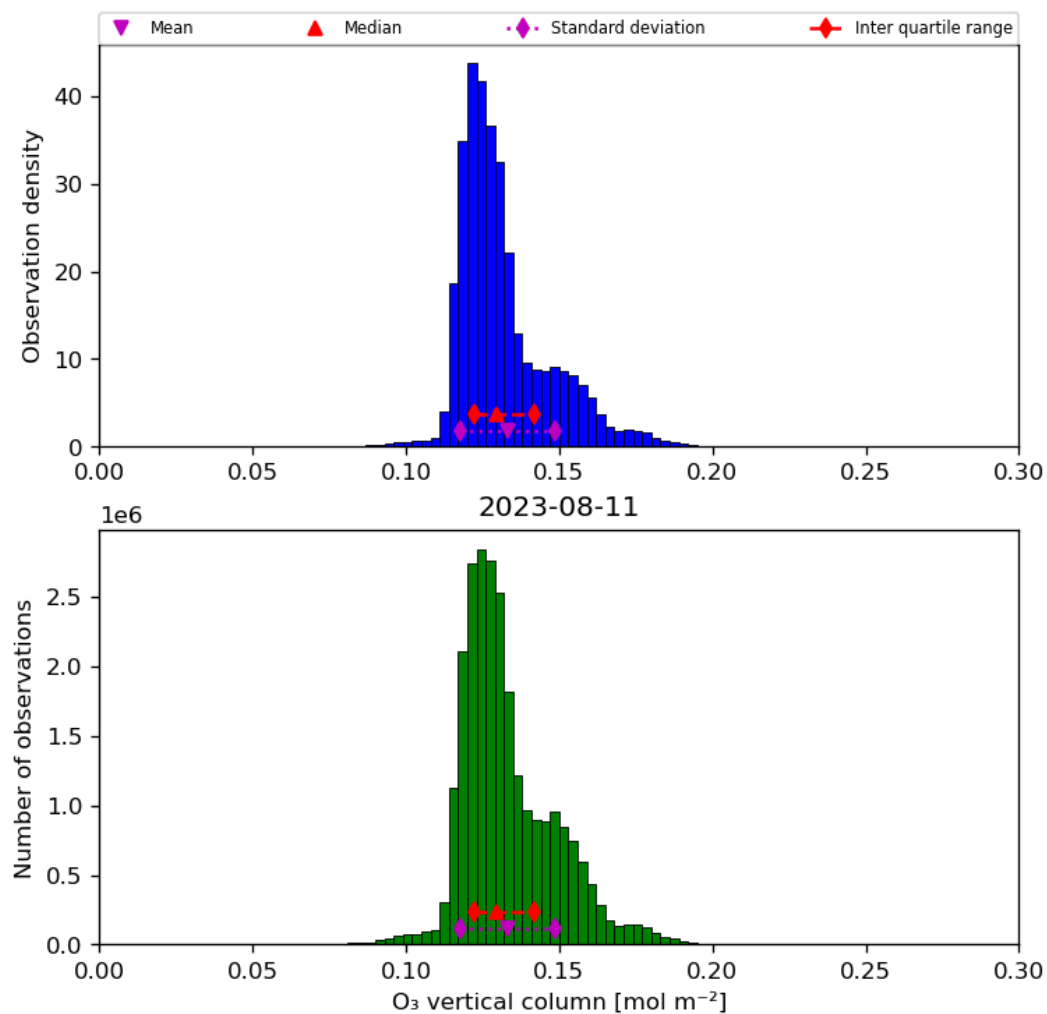
Figure 21: Histogram of “O 3 vertical column” for 2023-08-10 to 2023-08-12
