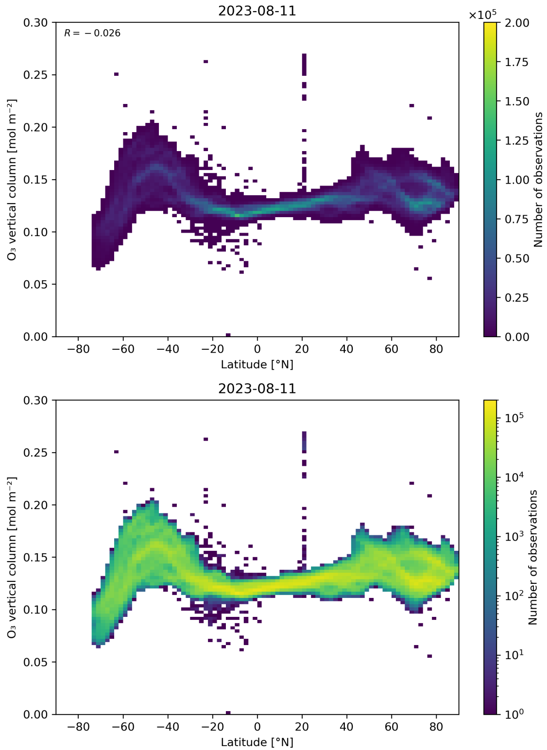
Figure 36: Scatter density plot of “Latitude” against “O 3 vertical column” for 2023-08-10 to 2023-08-12.
