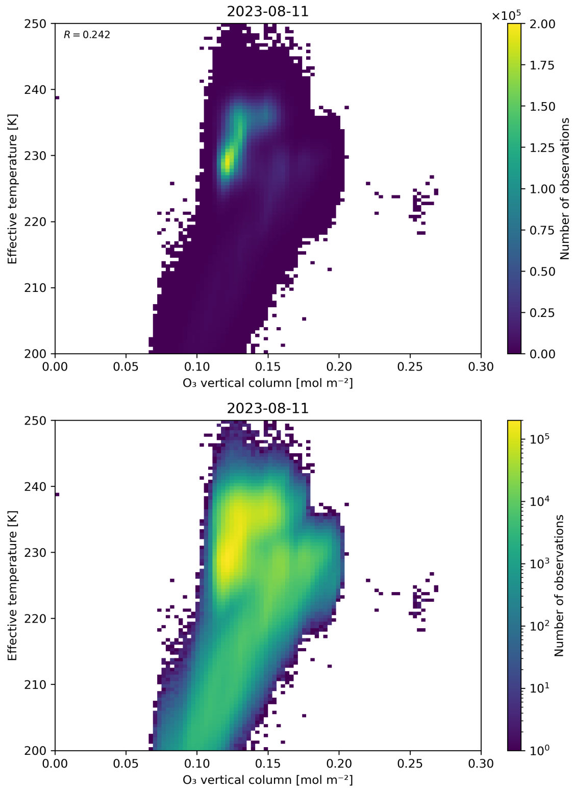
Figure 39: Scatter density plot of “O 3 vertical column” against “Effective temperature” for 2023-08-10 to 2023-08-12.
