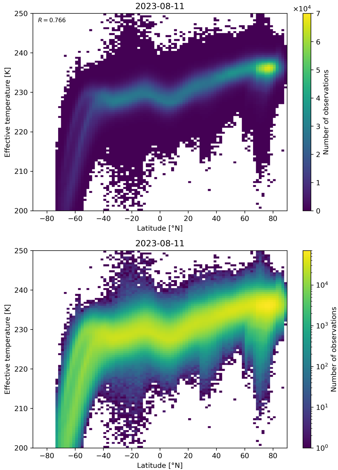
Figure 34: Scatter density plot of “Latitude” against “Effective temperature” for 2023-08-10 to 2023-08-12.
