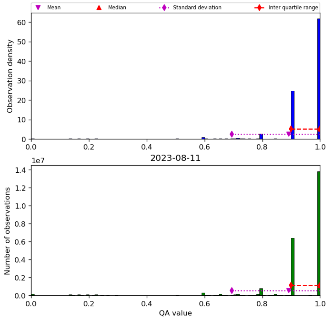
Figure 20: Histogram of “QA value” for 2023-08-10 to 2023-08-12
