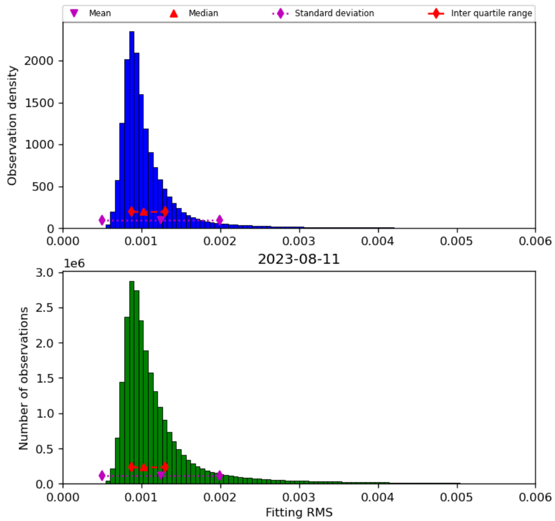
Figure 23: Histogram of “Fitting RMS” for 2023-08-10 to 2023-08-12
