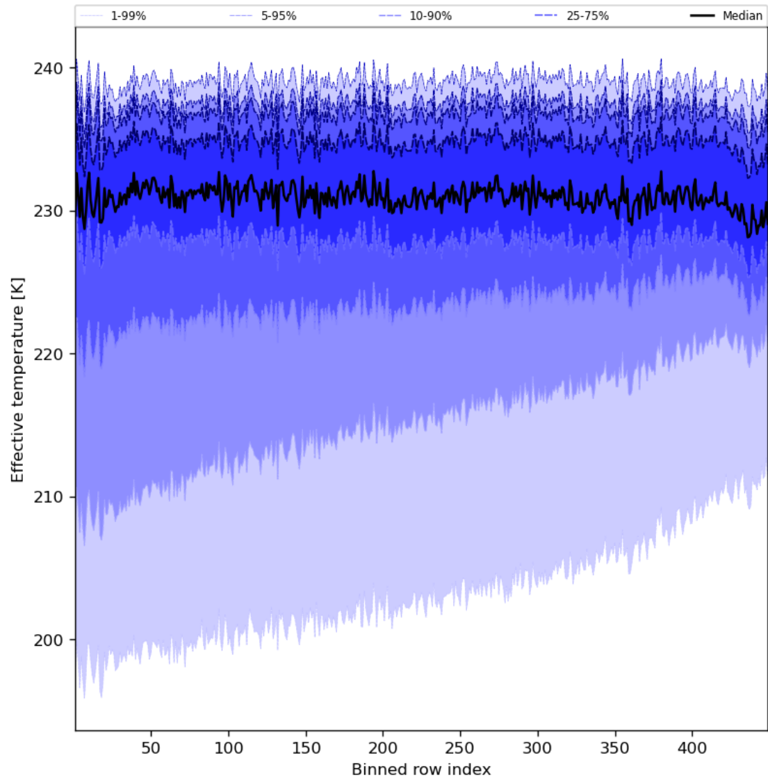
Figure 31: Along track statistics of “Effective temperature” for 2023-08-10 to 2023-08-12
