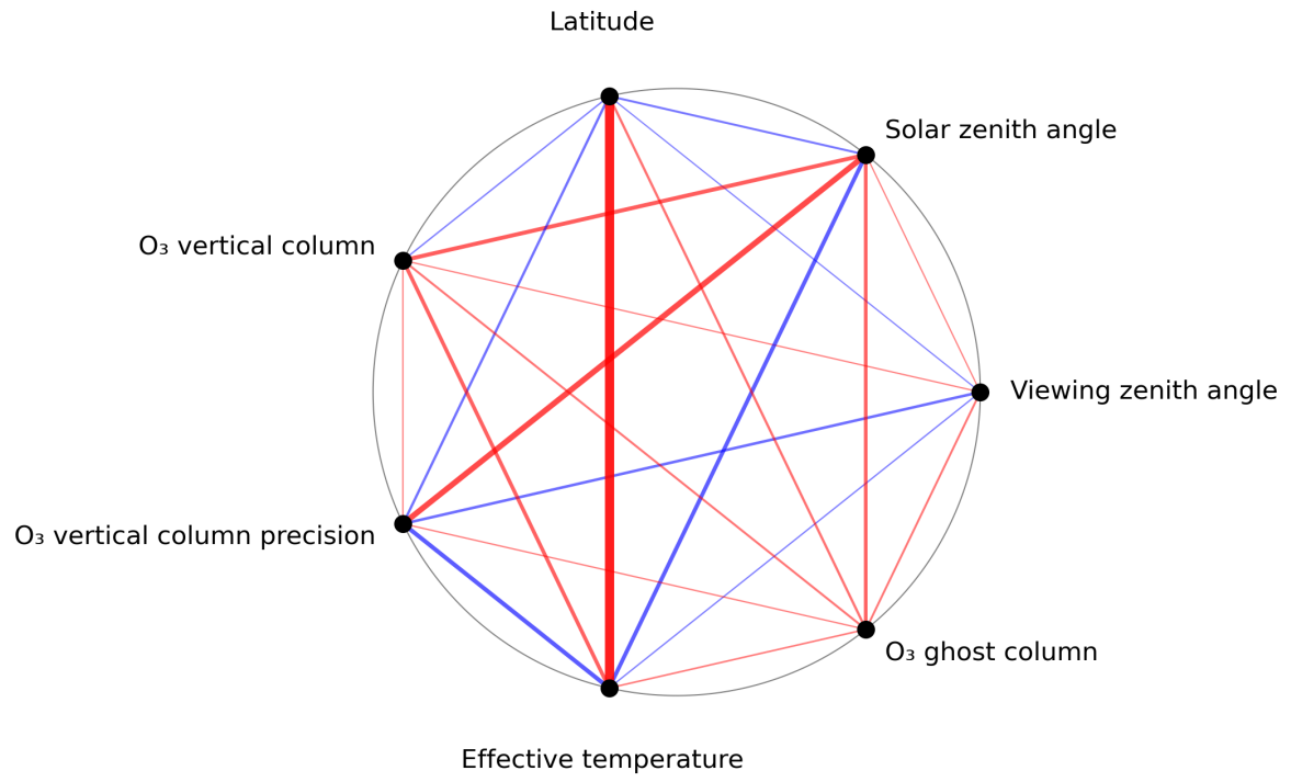
Figure 1: Map of correlation graph for 2023-08-10 to 2023-08-12.
