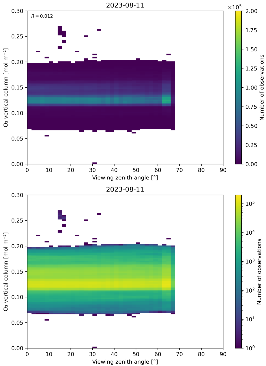
Figure 52: Scatter density plot of “Viewing zenith angle” against “O 3 vertical column” for 2023-08-10 to 2023-08-12.
