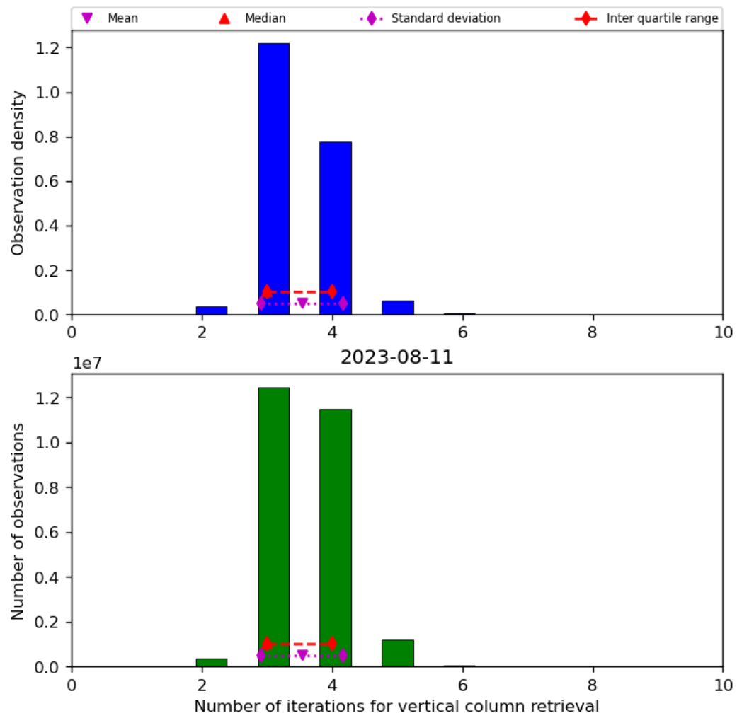
Figure 26: Histogram of “Number of iterations for vertical column retrieval” for 2023-08-10 to 2023-08-12
