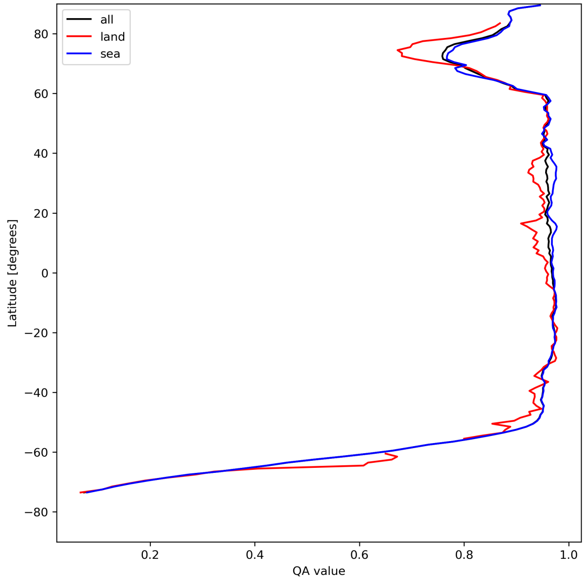
Figure 13: Zonal average of “QA value” for 2023-08-10 to 2023-08-12.
