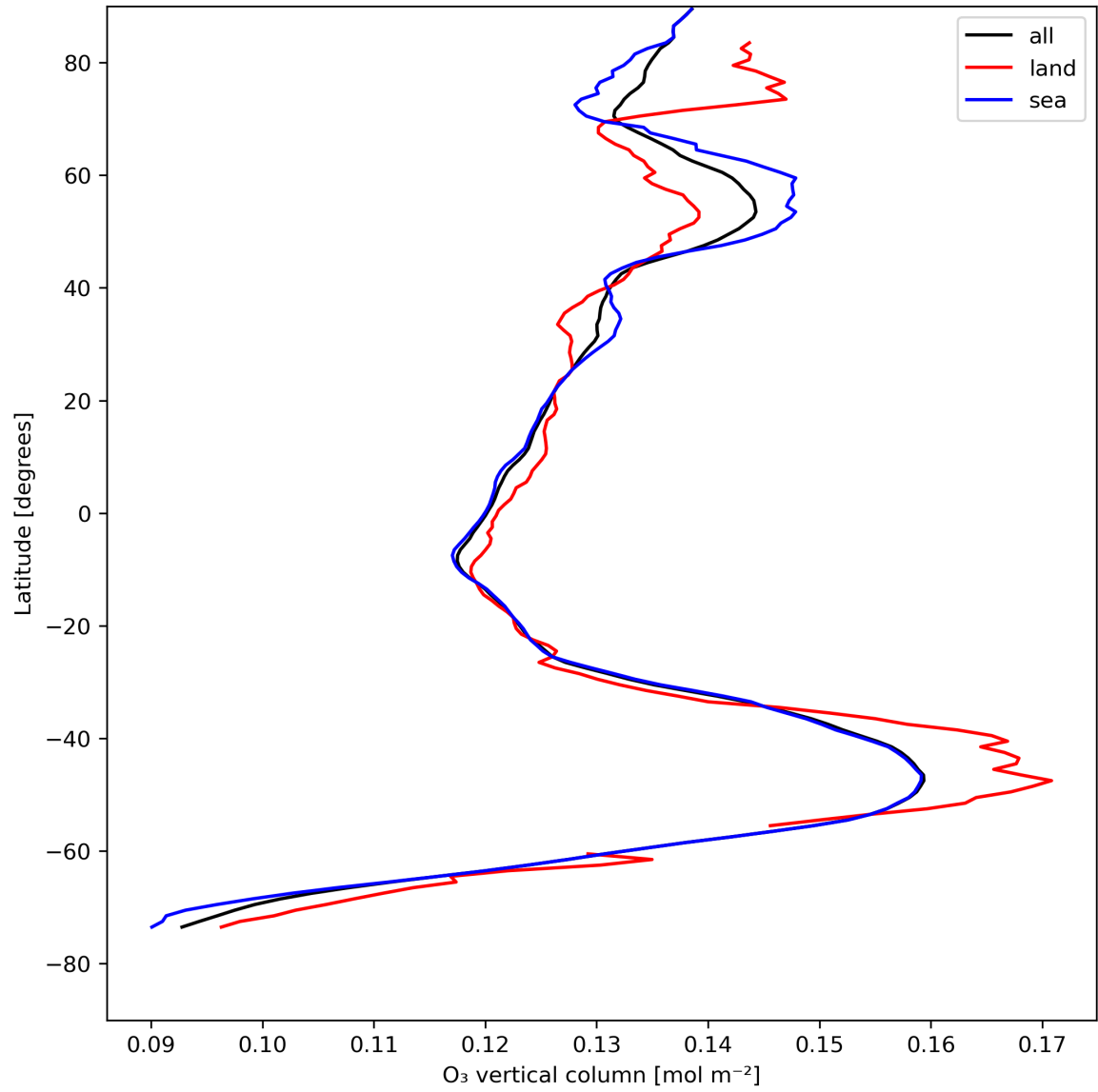
Figure 14: Zonal average of “O 3 vertical column” for 2023-08-10 to 2023-08-12.
