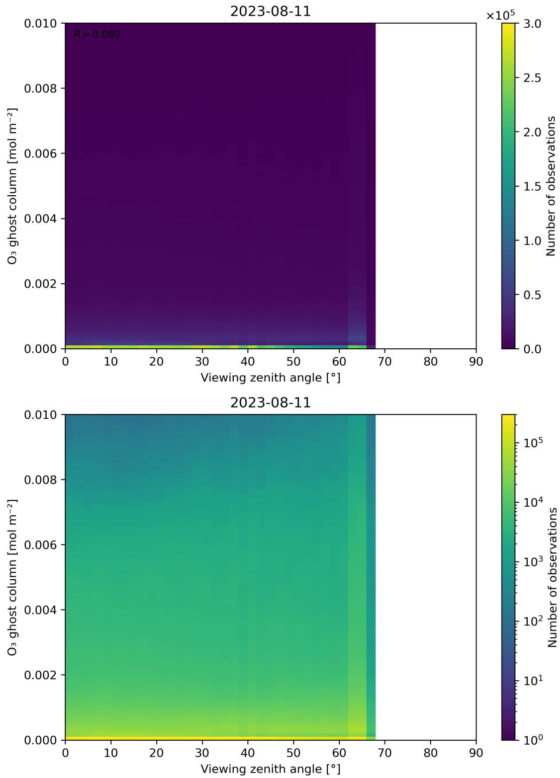
Figure 51: Scatter density plot of “Viewing zenith angle” against “O 3 ghost column” for 2023-08-10 to 2023-08-12.
