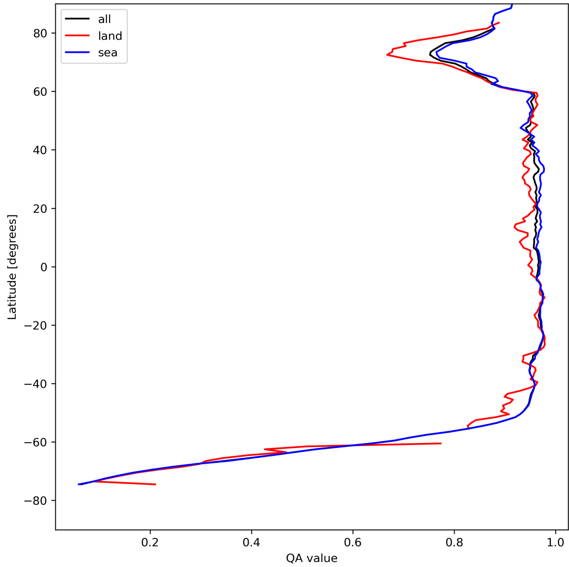
Figure 13: Zonal average of “QA value” for 2023-08-11 to 2023-08-13.
