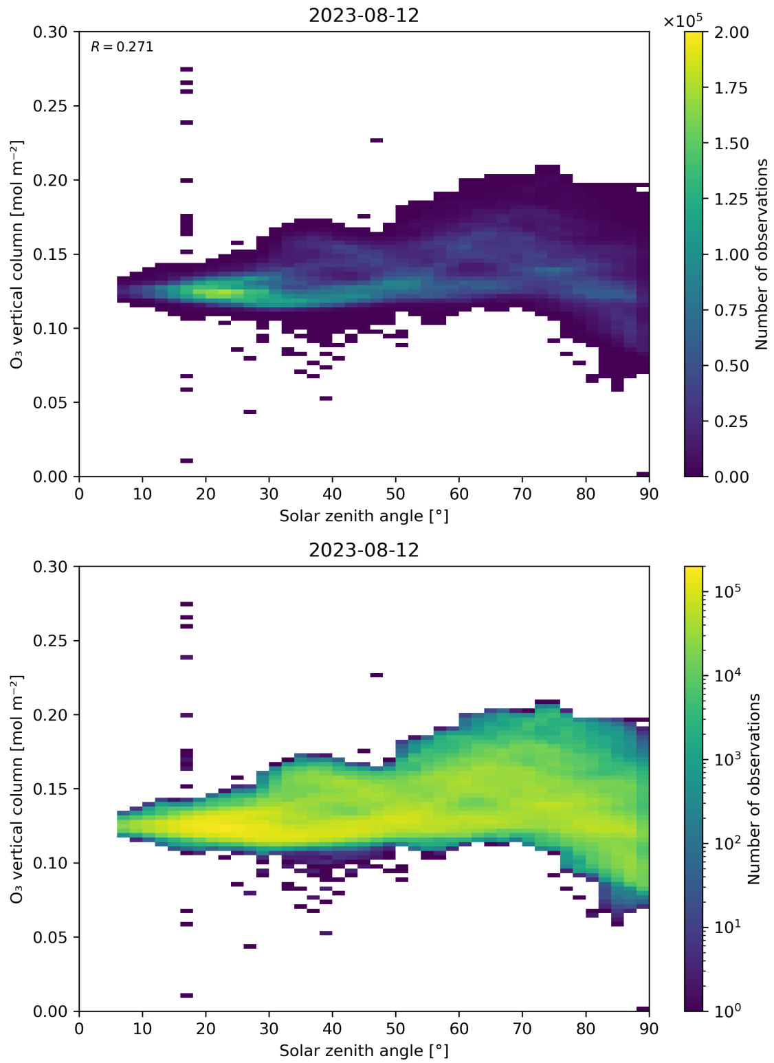
Figure 47: Scatter density plot of “Solar zenith angle” against “O 3 vertical column” for 2023-08-11 to 2023-08-13.
