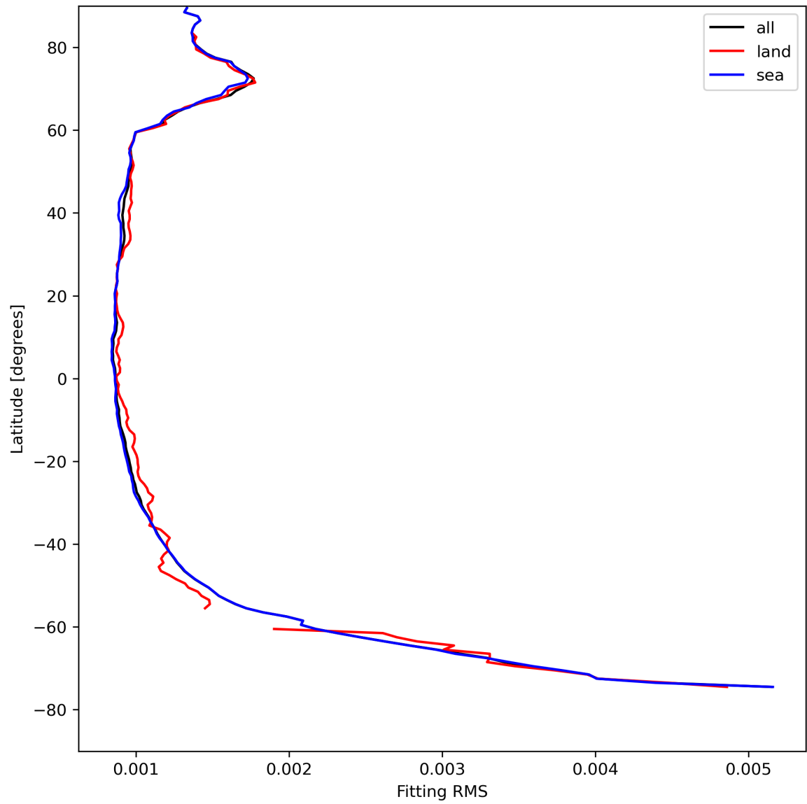
Figure 16: Zonal average of “Fitting RMS” for 2023-08-11 to 2023-08-13.
