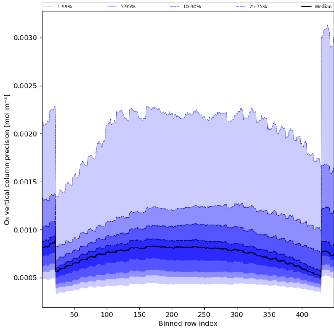
Figure 29: Along track statistics of “O 3 vertical column precision” for 2023-08-11 to 2023-08-13
