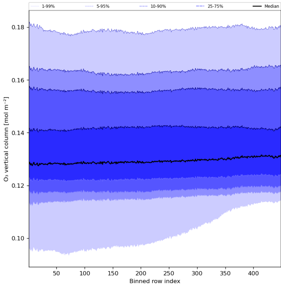
Figure 28: Along track statistics of “O 3 vertical column” for 2023-08-11 to 2023-08-13
