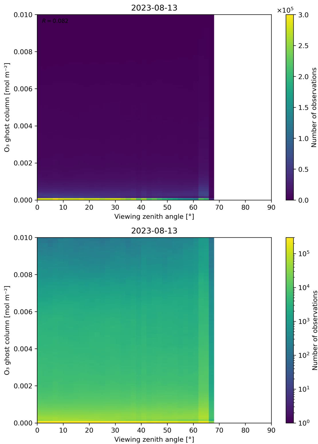
Figure 51: Scatter density plot of “Viewing zenith angle” against “O 3 ghost column” for 2023-08-12 to 2023-08-14.
