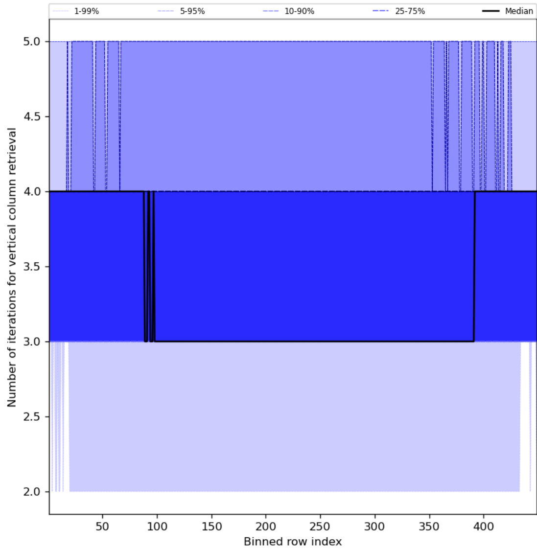
Figure 33: Along track statistics of “Number of iterations for vertical column retrieval” for 2023-08-12 to 2023-08-14
