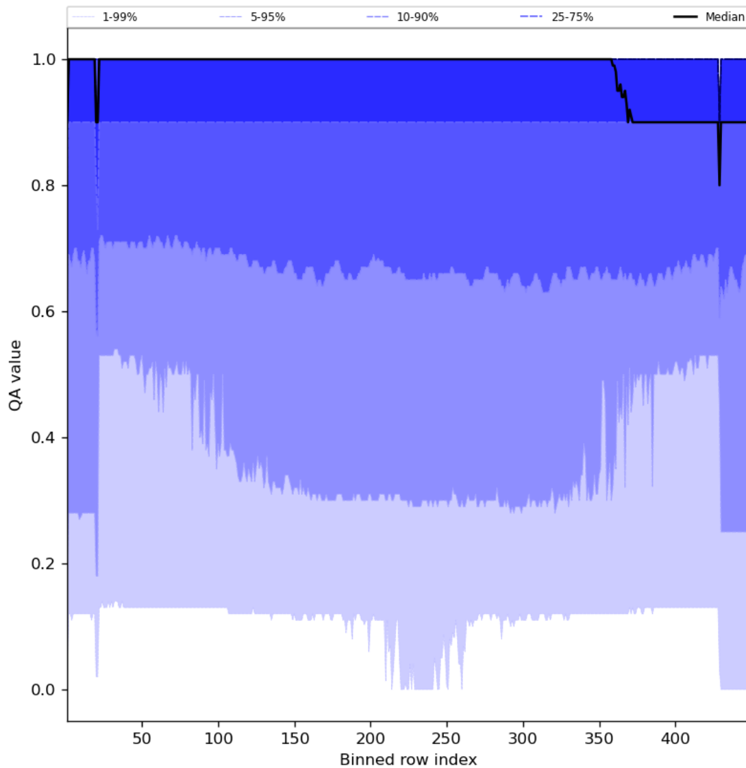
Figure 27: Along track statistics of “QA value” for 2023-08-12 to 2023-08-14
