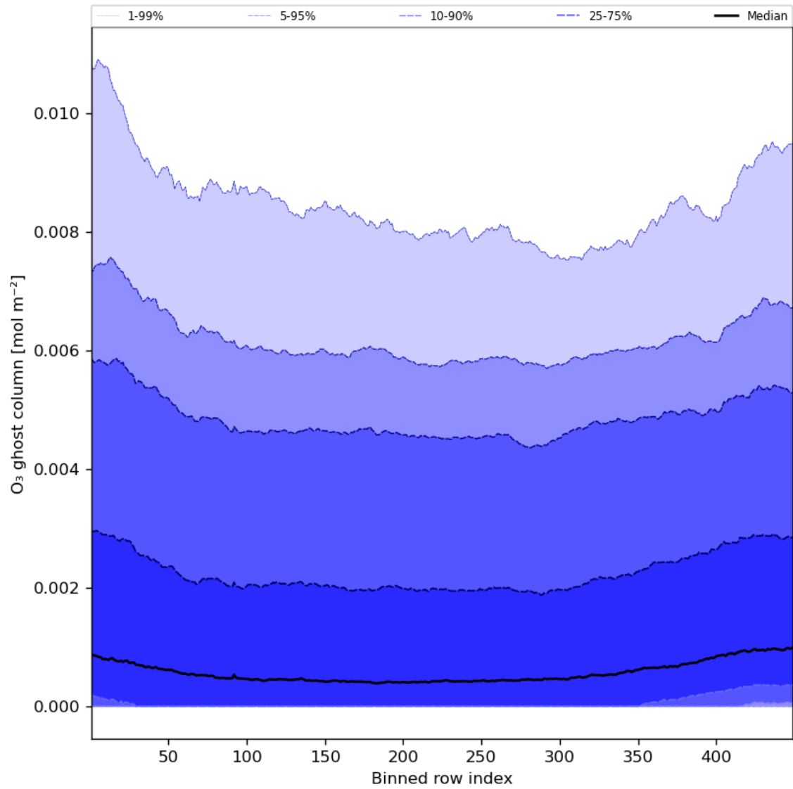
Figure 32: Along track statistics of “O 3 ghost column” for 2023-08-12 to 2023-08-14
