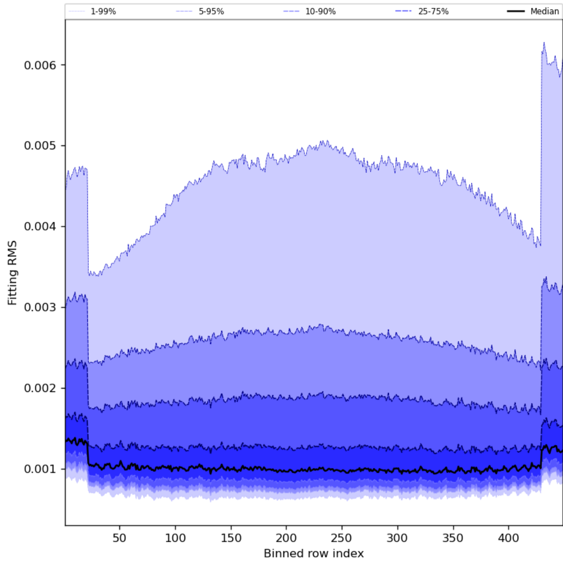
Figure 30: Along track statistics of “Fitting RMS” for 2023-08-12 to 2023-08-14
