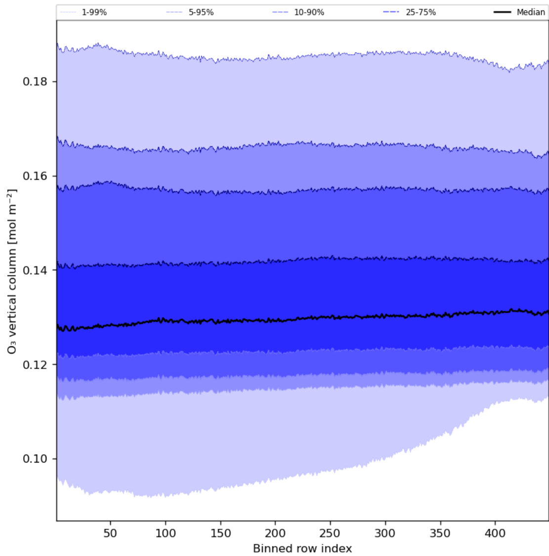
Figure 28: Along track statistics of “O 3 vertical column” for 2023-08-12 to 2023-08-14
