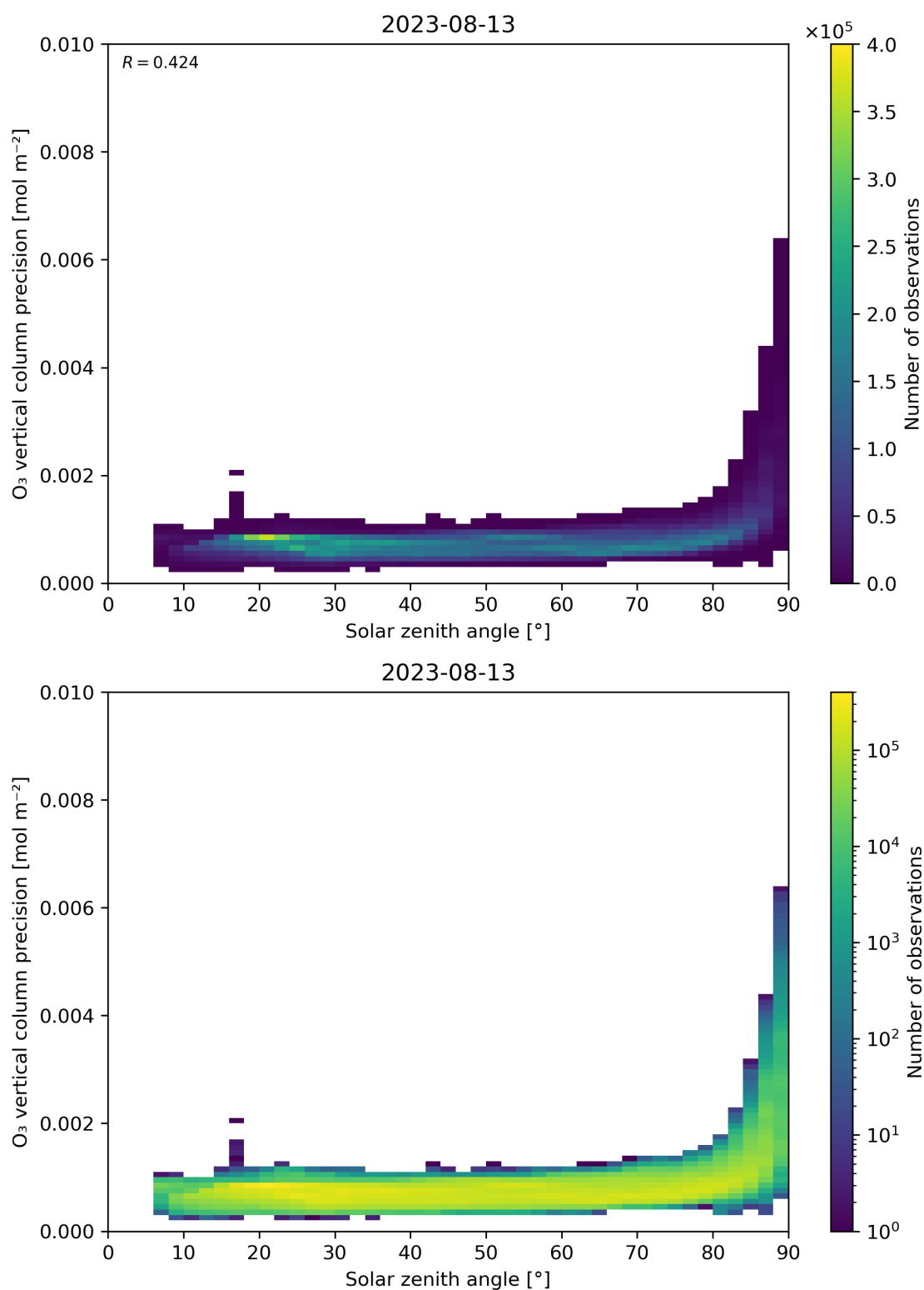
Figure 48: Scatter density plot of “Solar zenith angle” against “O 3 vertical column precision” for 2023-08-12 to 2023-08-14.
