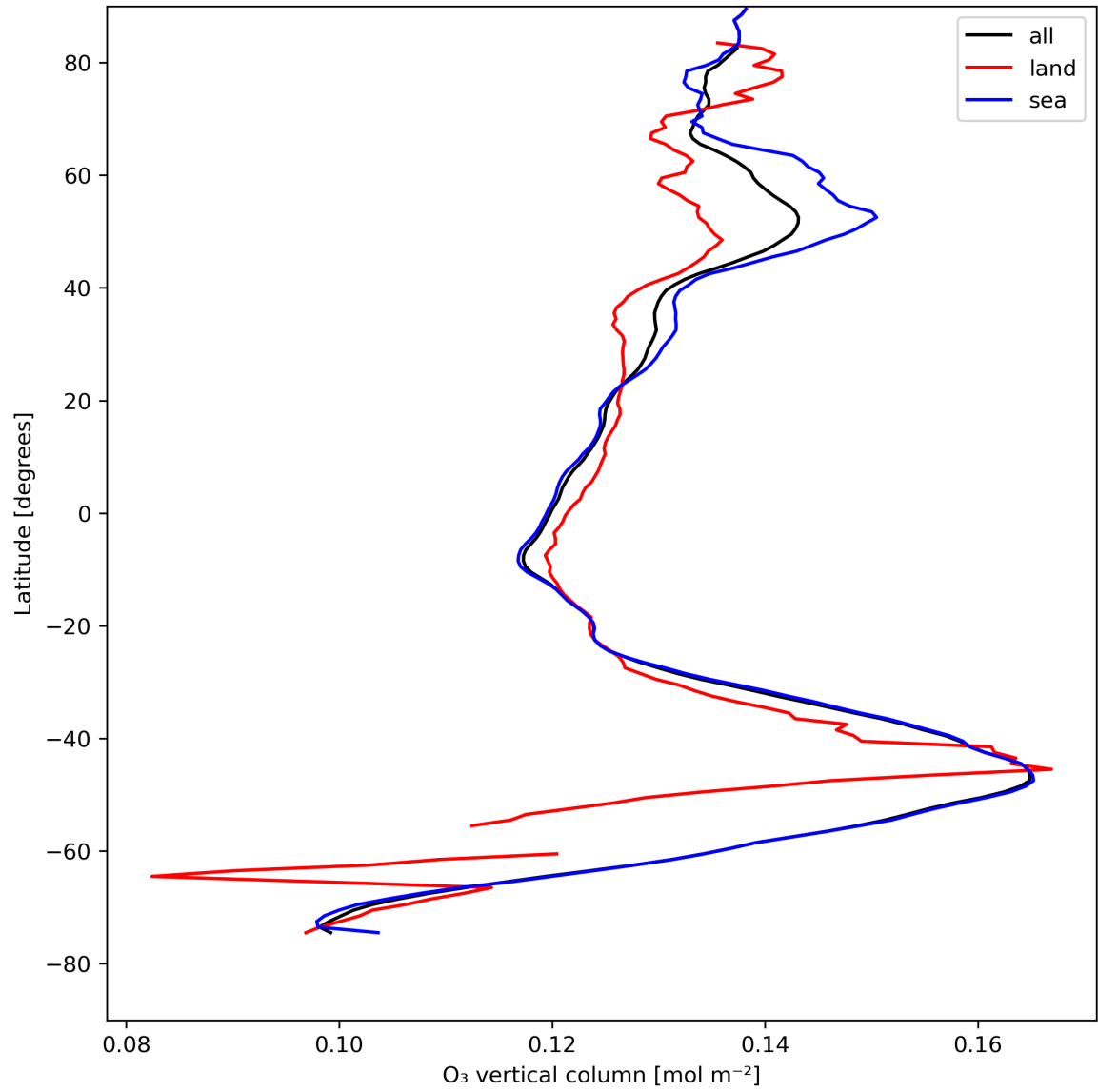
Figure 14: Zonal average of “O 3 vertical column” for 2023-08-12 to 2023-08-14.
