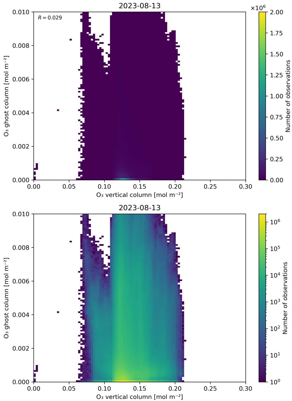
Figure 40: Scatter density plot of “O 3 vertical column” against “O 3 ghost column” for 2023-08-12 to 2023-08-14.
