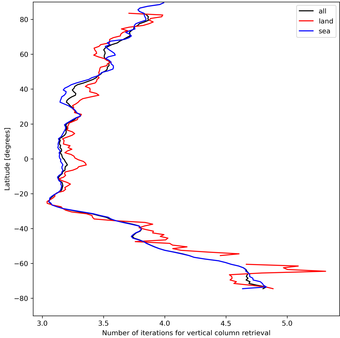
Figure 19: Zonal average of “Number of iterations for vertical column retrieval” for 2023-08-12 to 2023-08-14.
