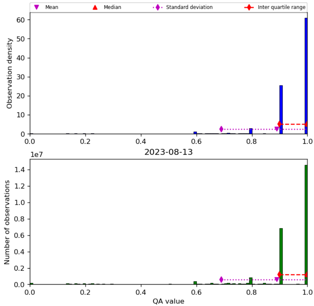
Figure 20: Histogram of “QA value” for 2023-08-12 to 2023-08-14
