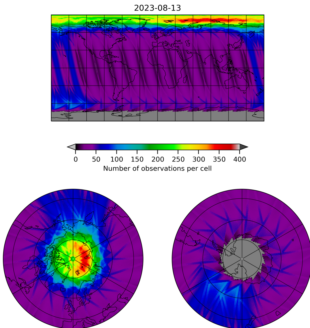
Figure 12: Map of the number of observations for 2023-08-12 to 2023-08-14
