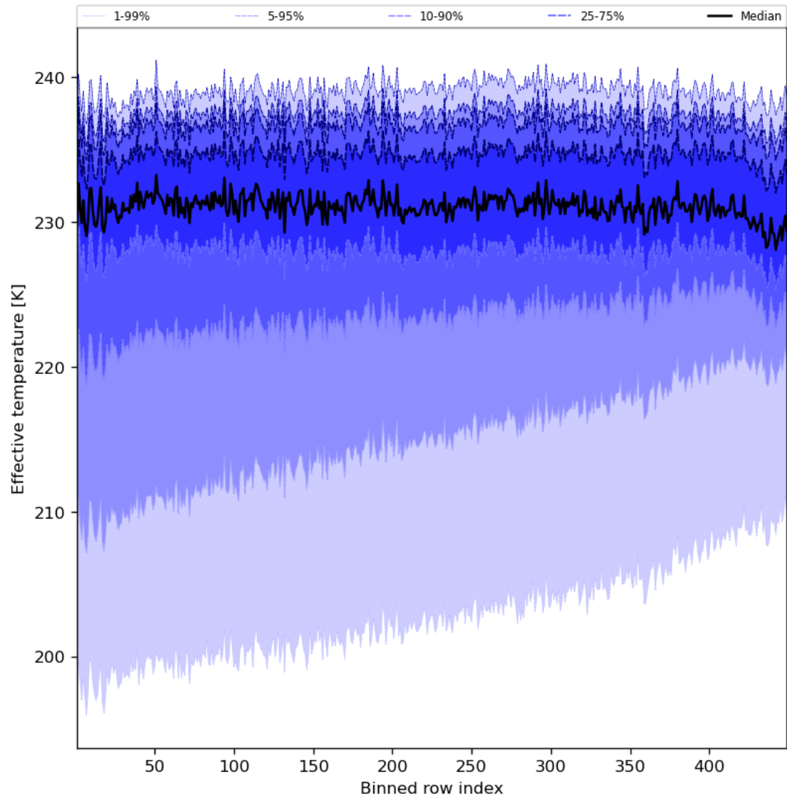
Figure 31: Along track statistics of “Effective temperature” for 2023-08-12 to 2023-08-14
