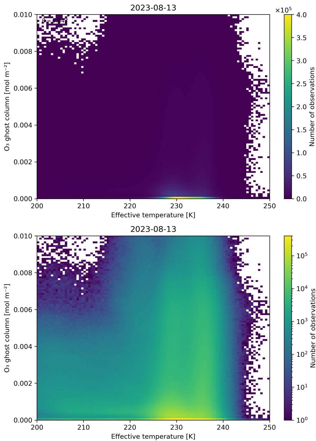
Figure 38: Scatter density plot of “Effective temperature” against “O 3 ghost column” for 2023-08-12 to 2023-08-14.
