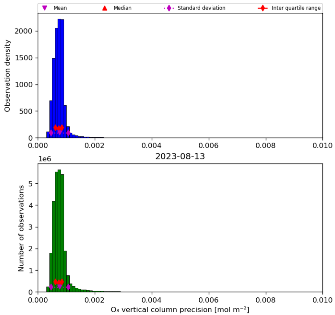
Figure 22: Histogram of “O 3 vertical column precision” for 2023-08-12 to 2023-08-14
