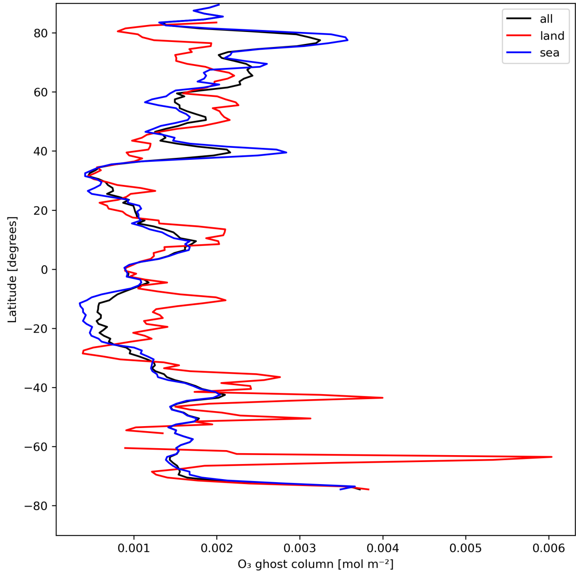
Figure 18: Zonal average of "O 3 ghost column" for 2023-08-12 to 2023-08-14.
