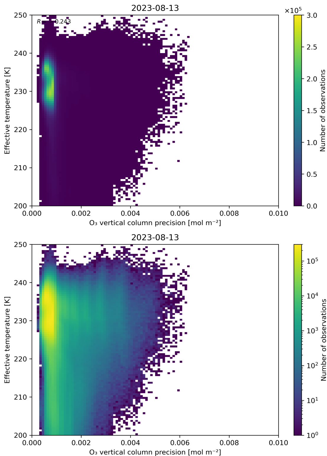
Figure 42: Scatter density plot of “O 3 vertical column precision” against “Effective temperature” for 2023-08-12 to 2023-08-14.
