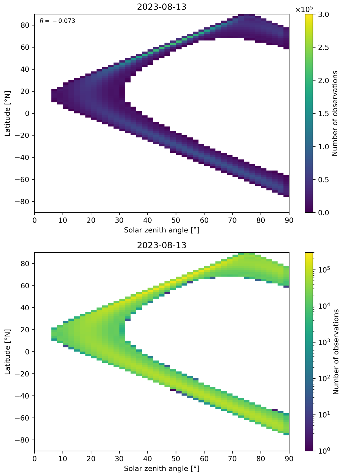
Figure 44: Scatter density plot of “Solar zenith angle” against “Latitude” for 2023-08-12 to 2023-08-14.
