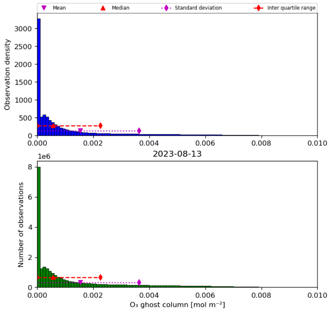
Figure 25: Histogram of “O 3 ghost column” for 2023-08-12 to 2023-08-14
