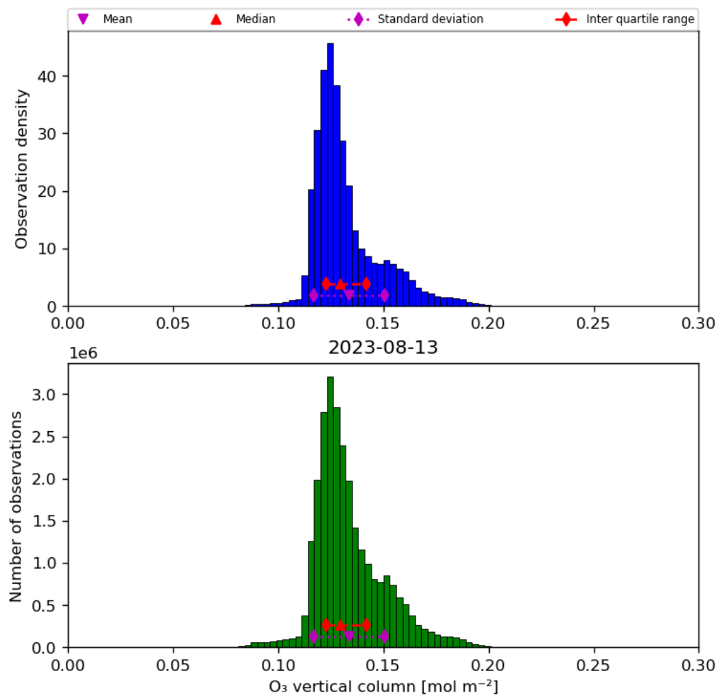
Figure 21: Histogram of “O 3 vertical column” for 2023-08-12 to 2023-08-14
