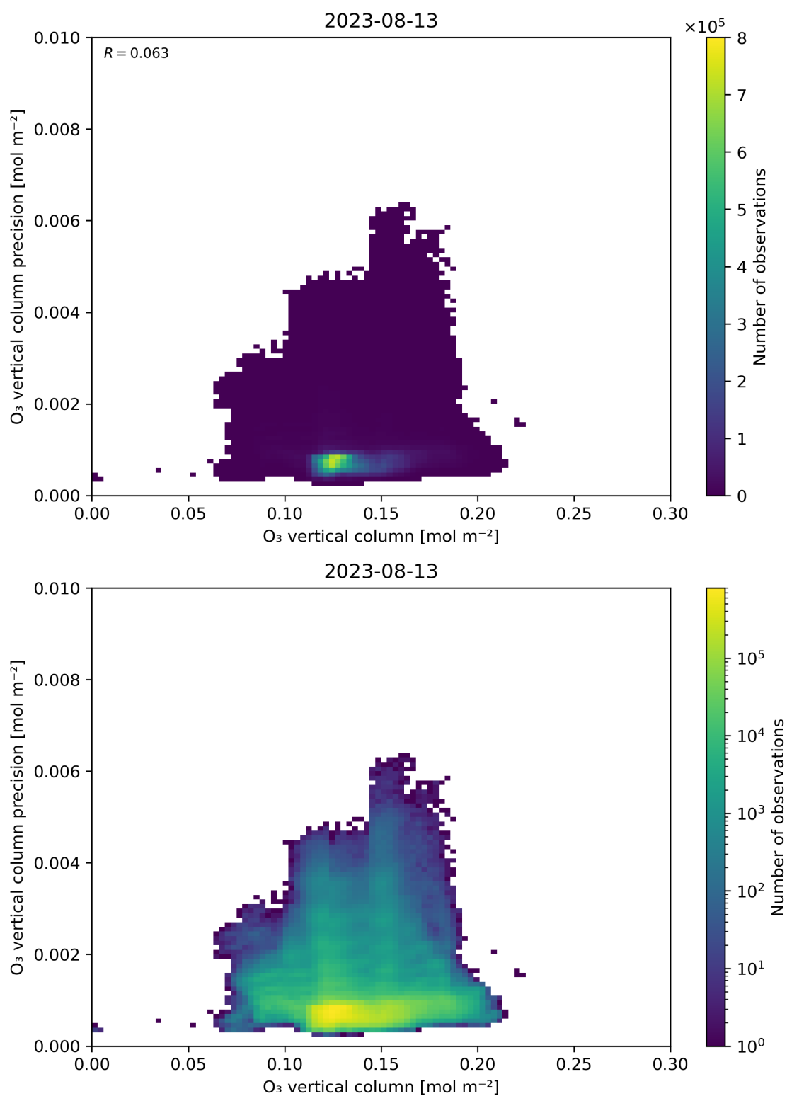
Figure 41: Scatter density plot of “O 3 vertical column” against “O 3 vertical column precision” for 2023-08-12 to 2023-08-14.
