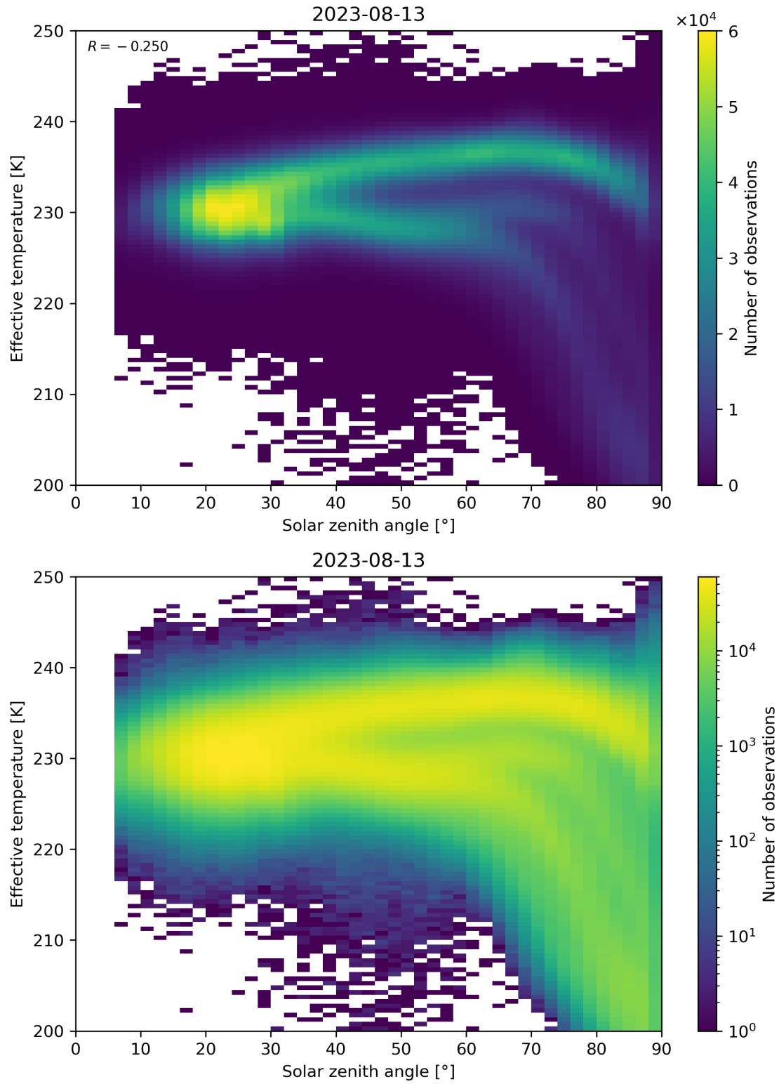
Figure 45: Scatter density plot of “Solar zenith angle” against “Effective temperature” for 2023-08-12 to 2023-08-14.
