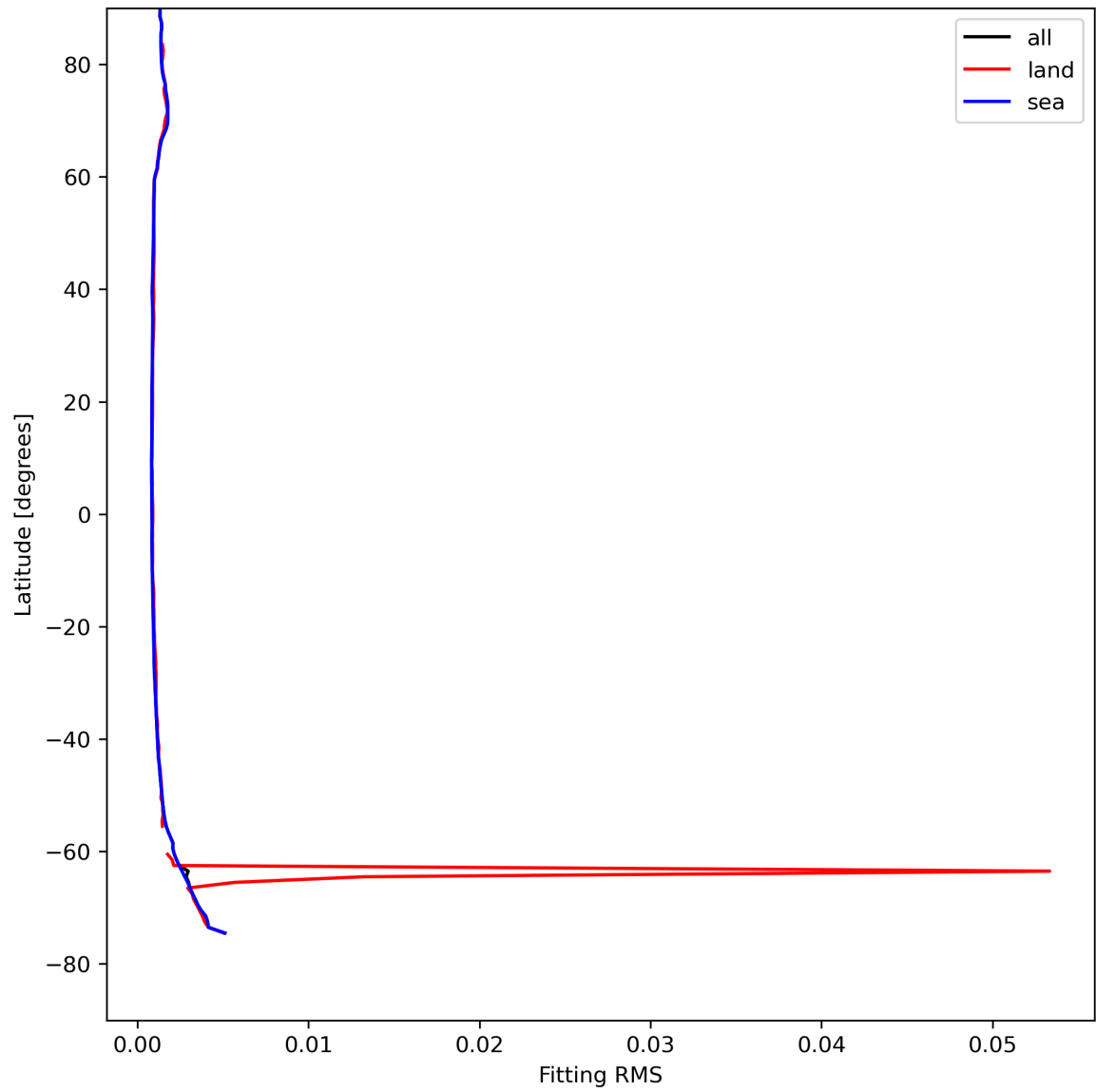
Figure 16: Zonal average of “Fitting RMS” for 2023-08-12 to 2023-08-14.
