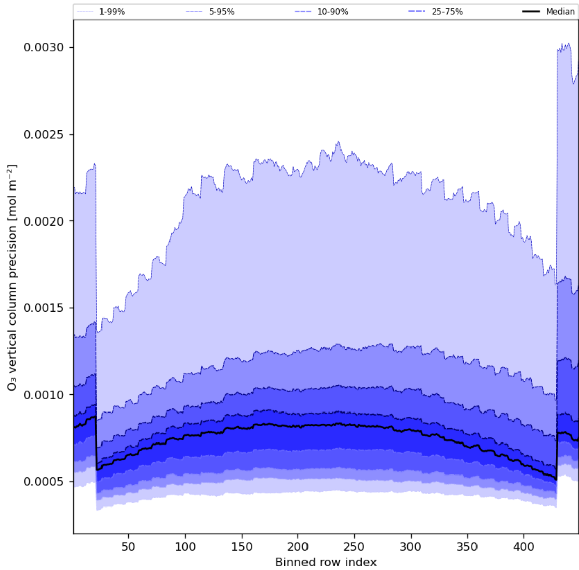
Figure 29: Along track statistics of “O 3 vertical column precision” for 2023-08-12 to 2023-08-14
