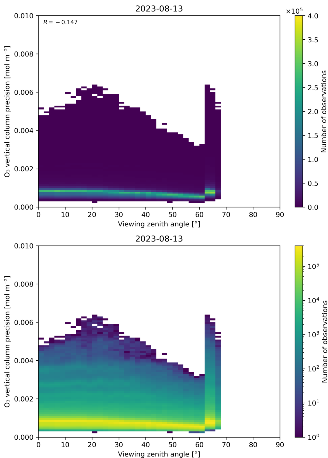
Figure 53: Scatter density plot of “Viewing zenith angle” against “O 3 vertical column precision” for 2023-08-12 to 2023-08-14.
