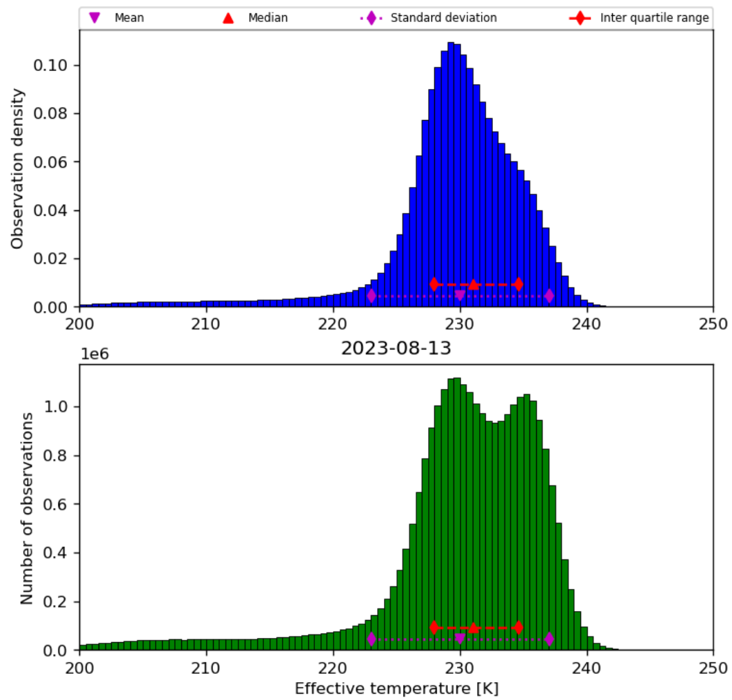
Figure 24: Histogram of “Effective temperature” for 2023-08-12 to 2023-08-14
