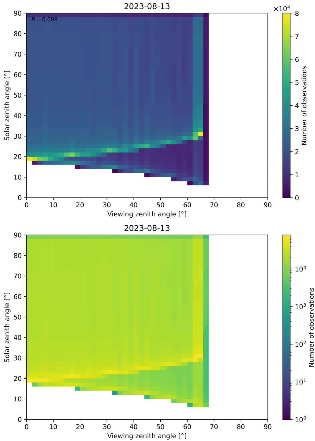
Figure 54: Scatter density plot of “Viewing zenith angle” against “Solar zenith angle” for 2023-08-12 to 2023-08-14.
