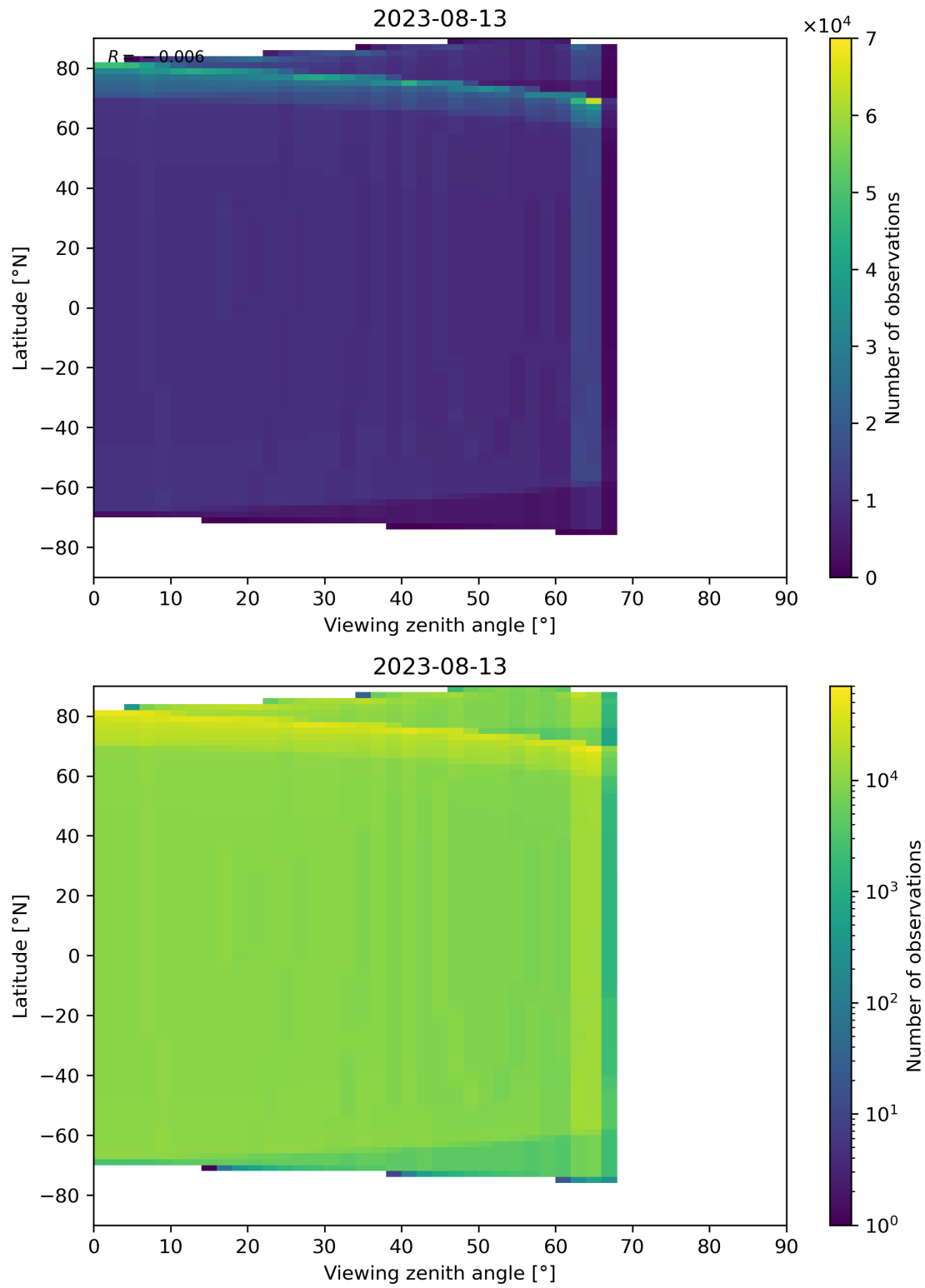
Figure 49: Scatter density plot of “Viewing zenith angle” against “Latitude” for 2023-08-12 to 2023-08-14.
