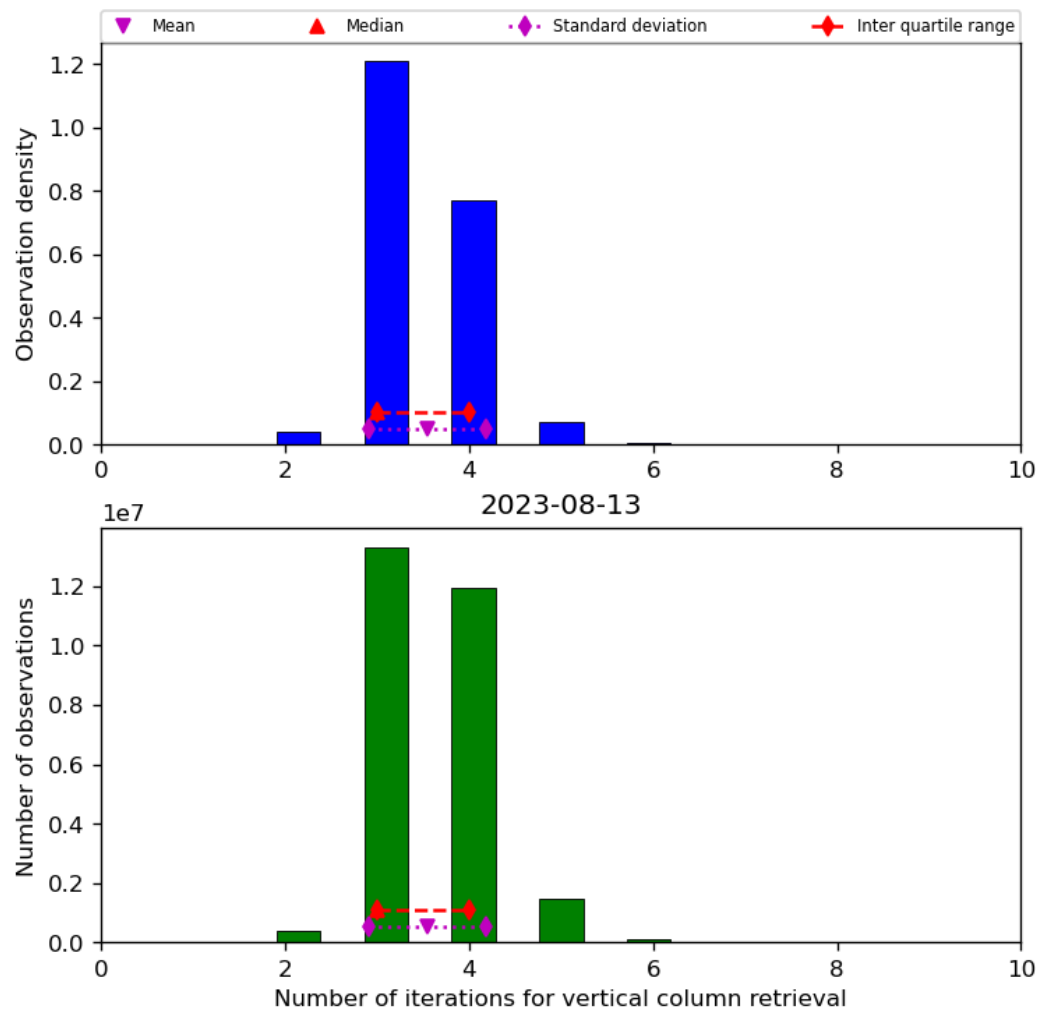
Figure 26: Histogram of “Number of iterations for vertical column retrieval” for 2023-08-12 to 2023-08-14
