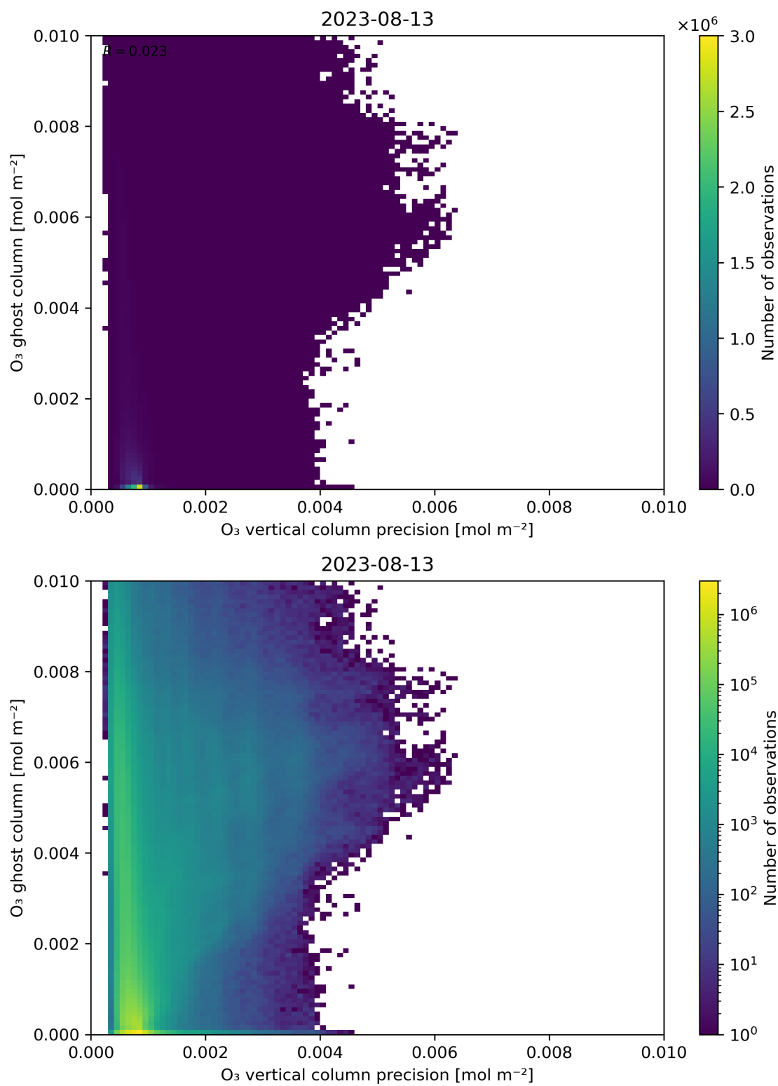
Figure 43: Scatter density plot of “O 3 vertical column precision” against “O 3 ghost column” for 2023-08-12 to 2023-08-14.
