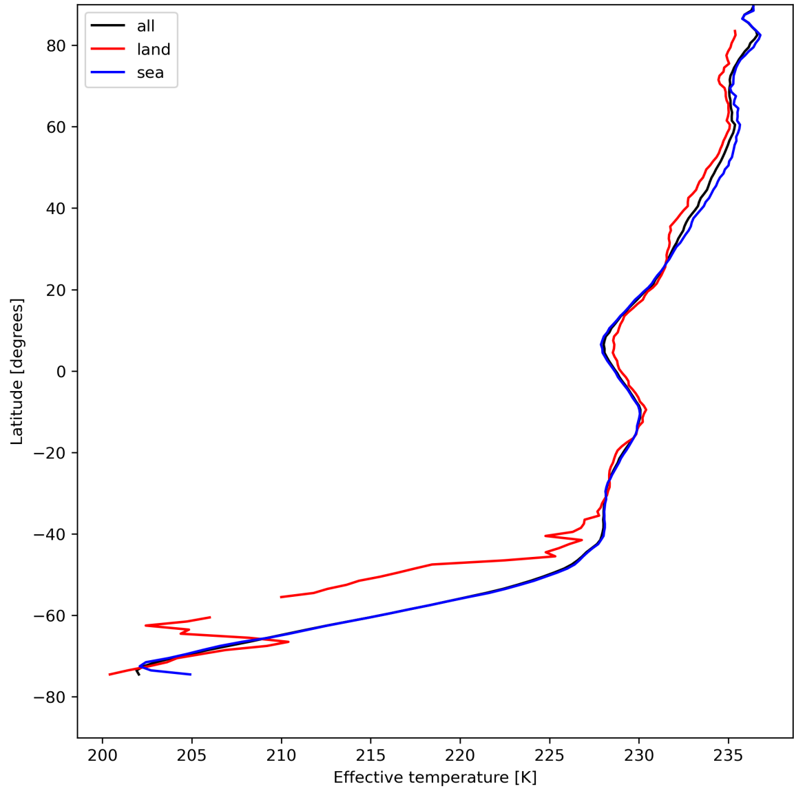
Figure 17: Zonal average of “Effective temperature” for 2023-08-12 to 2023-08-14.
