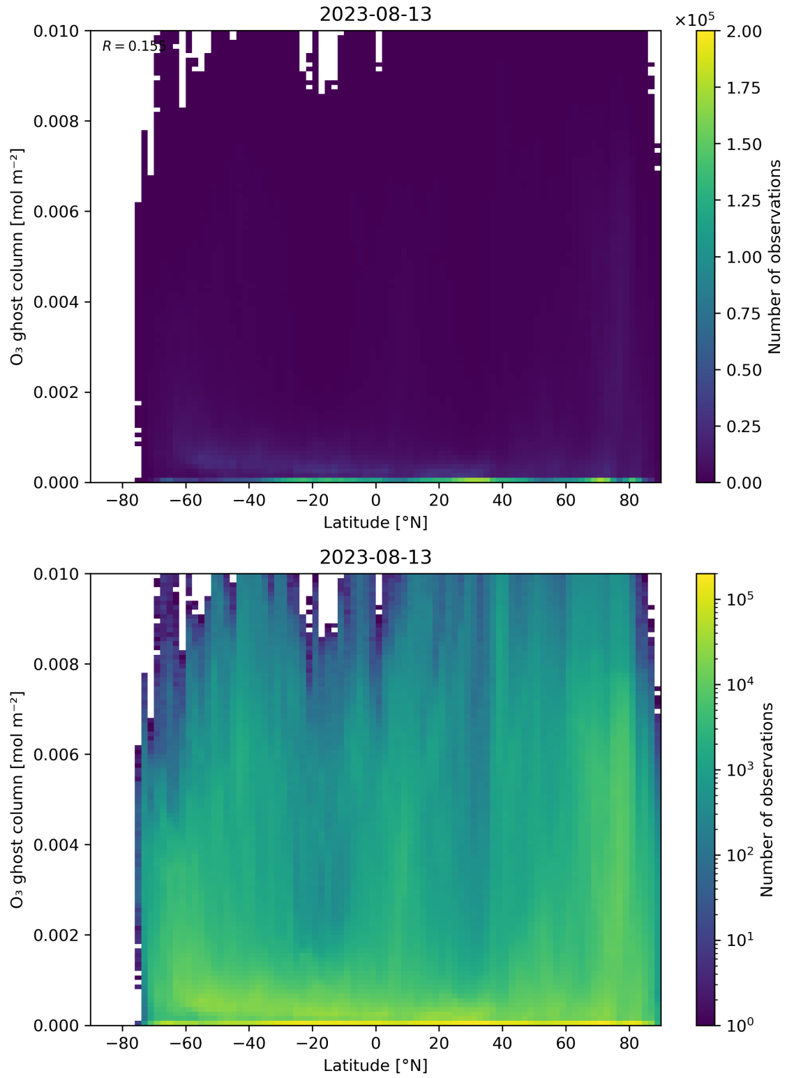
Figure 35: Scatter density plot of “Latitude” against “O 3 ghost column” for 2023-08-12 to 2023-08-14.
