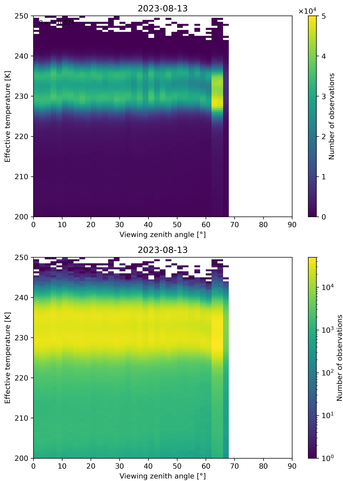
Figure 50: Scatter density plot of “Viewing zenith angle” against “Effective temperature” for 2023-08-12 to 2023-08-14.
