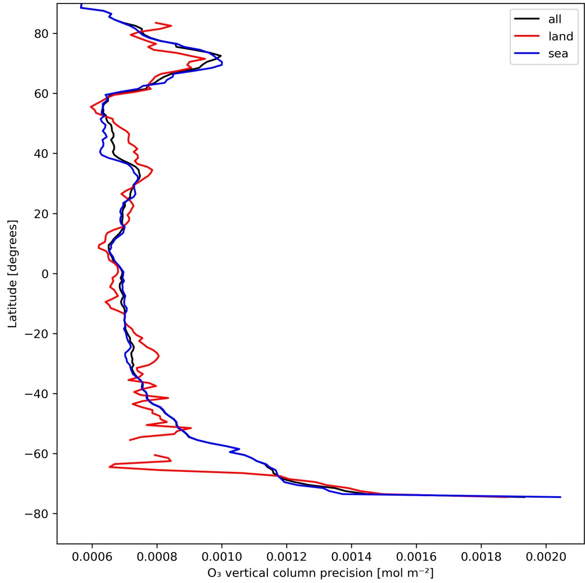
Figure 15: Zonal average of "O 3 vertical column precision" for 2023-08-12 to 2023-08-14.
