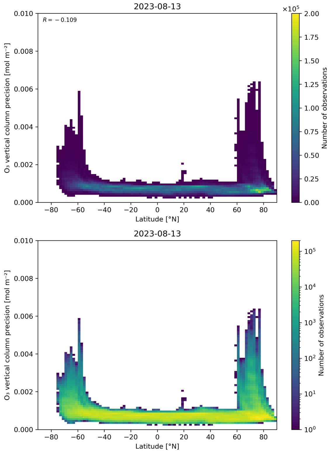
Figure 37: Scatter density plot of “Latitude” against “O 3 vertical column precision” for 2023-08-12 to 2023-08-14.
