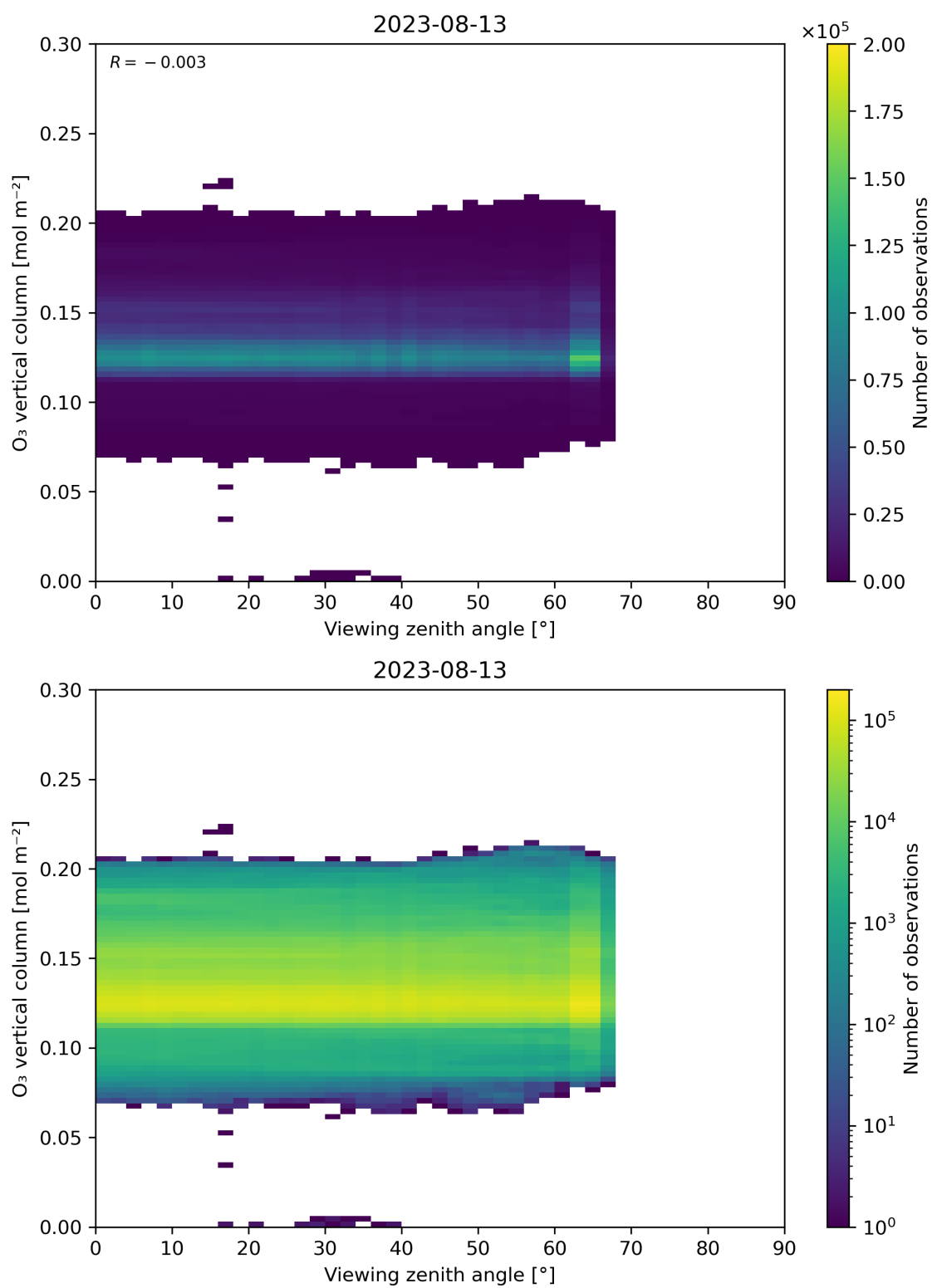
Figure 52: Scatter density plot of “Viewing zenith angle” against “O 3 vertical column” for 2023-08-12 to 2023-08-14.
