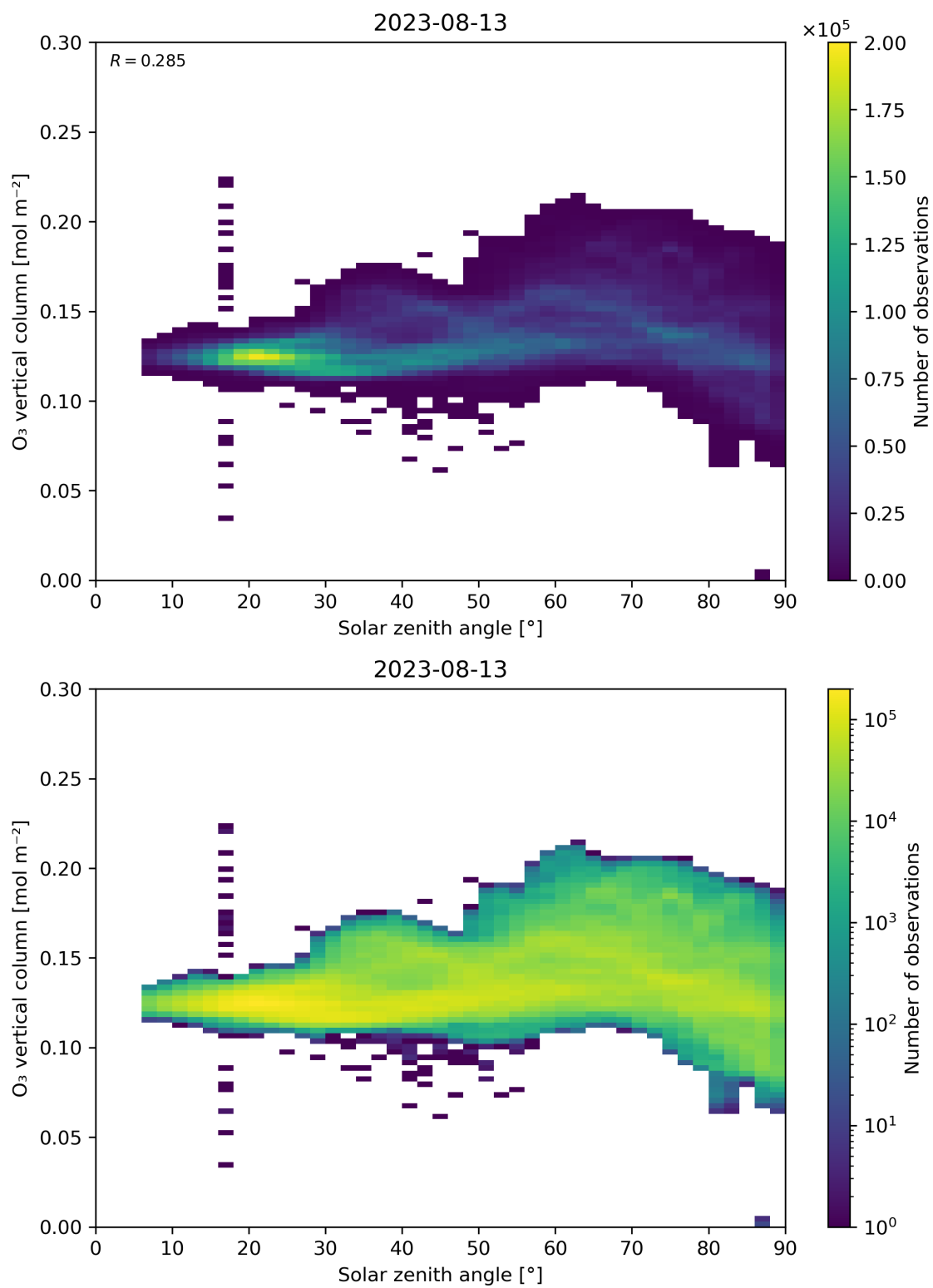
Figure 47: Scatter density plot of “Solar zenith angle” against “O 3 vertical column” for 2023-08-12 to 2023-08-14.
