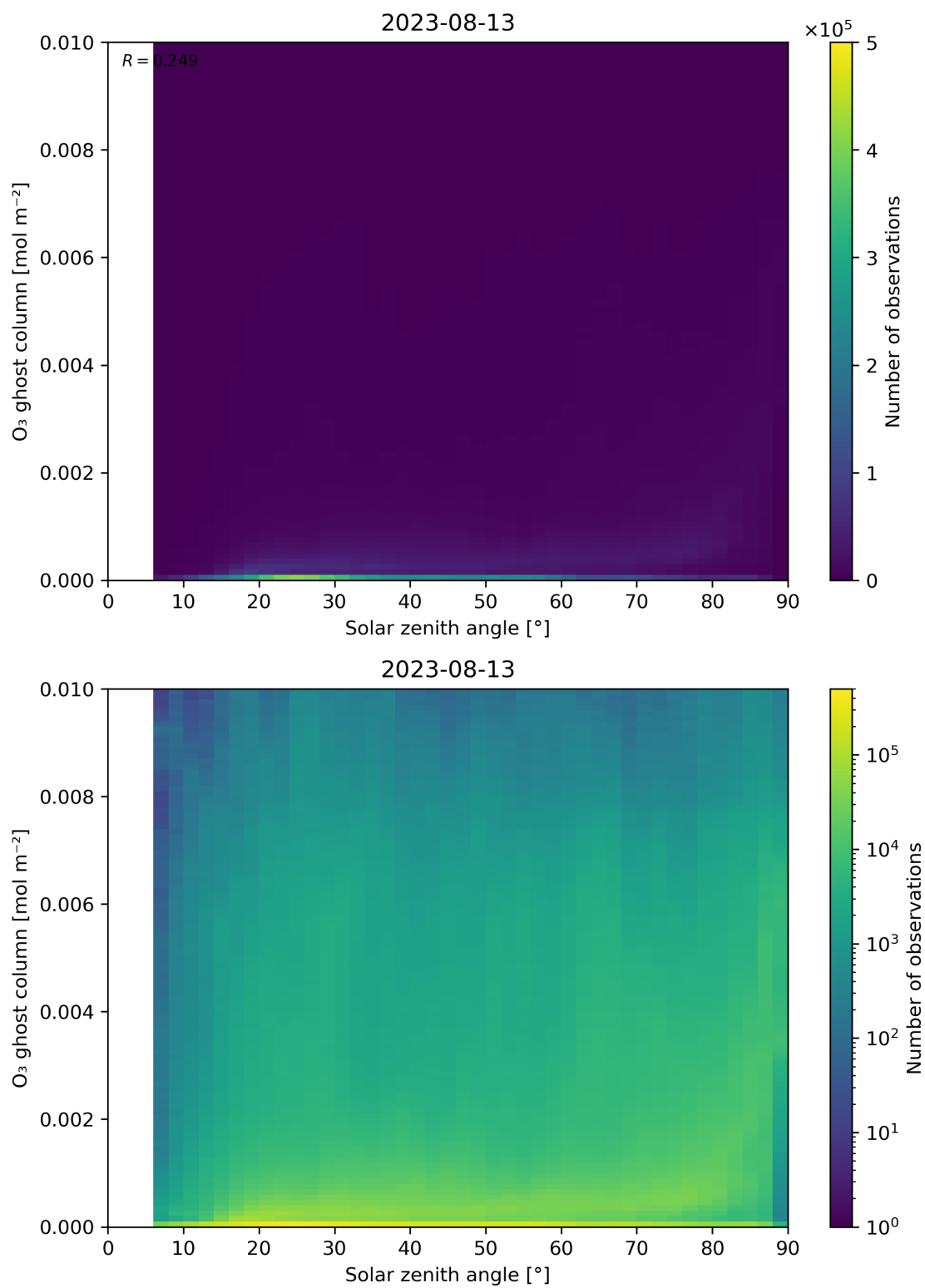
Figure 46: Scatter density plot of “Solar zenith angle” against “O 3 ghost column” for 2023-08-12 to 2023-08-14.
