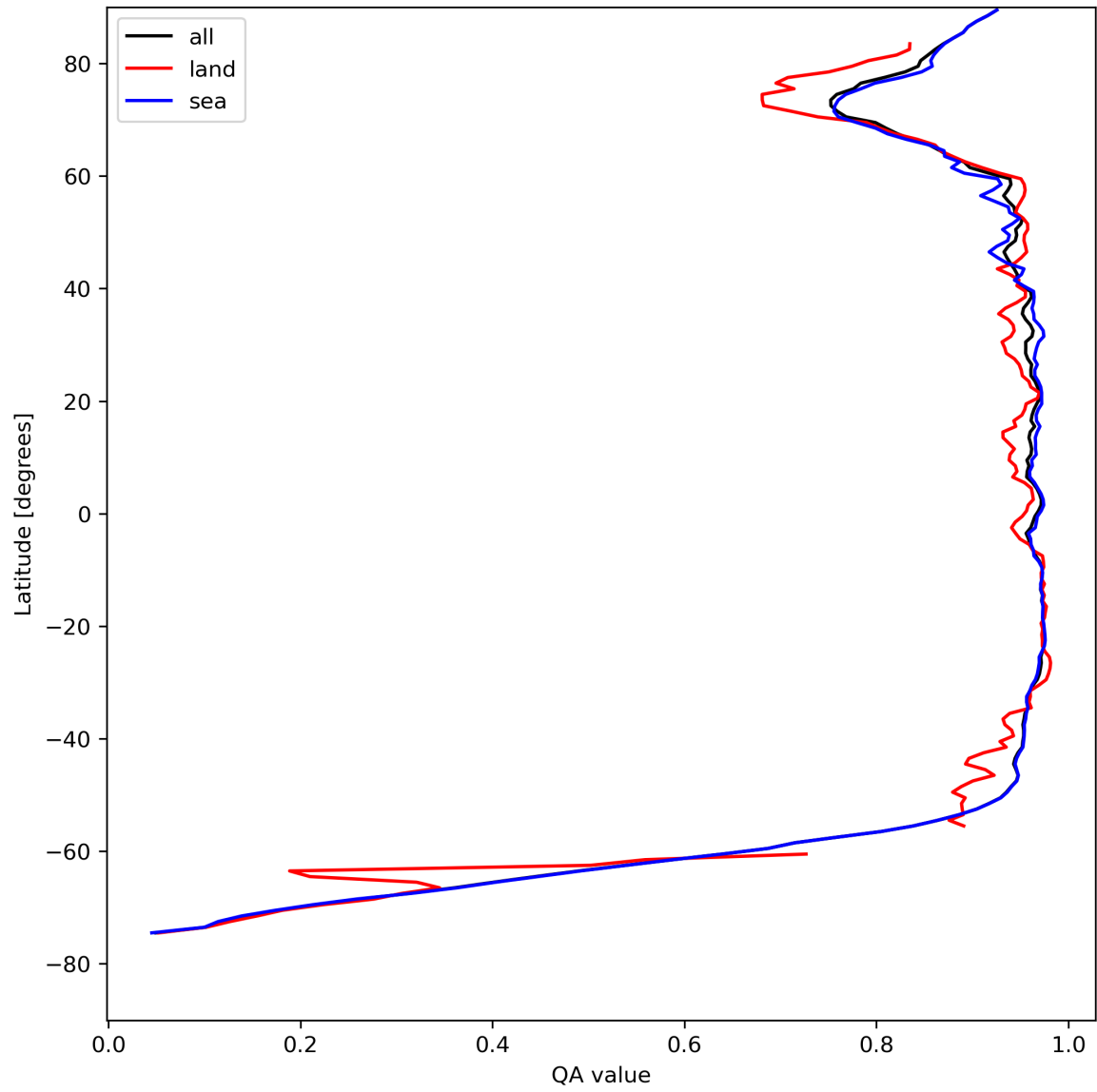
Figure 13: Zonal average of “QA value” for 2023-08-12 to 2023-08-14.
