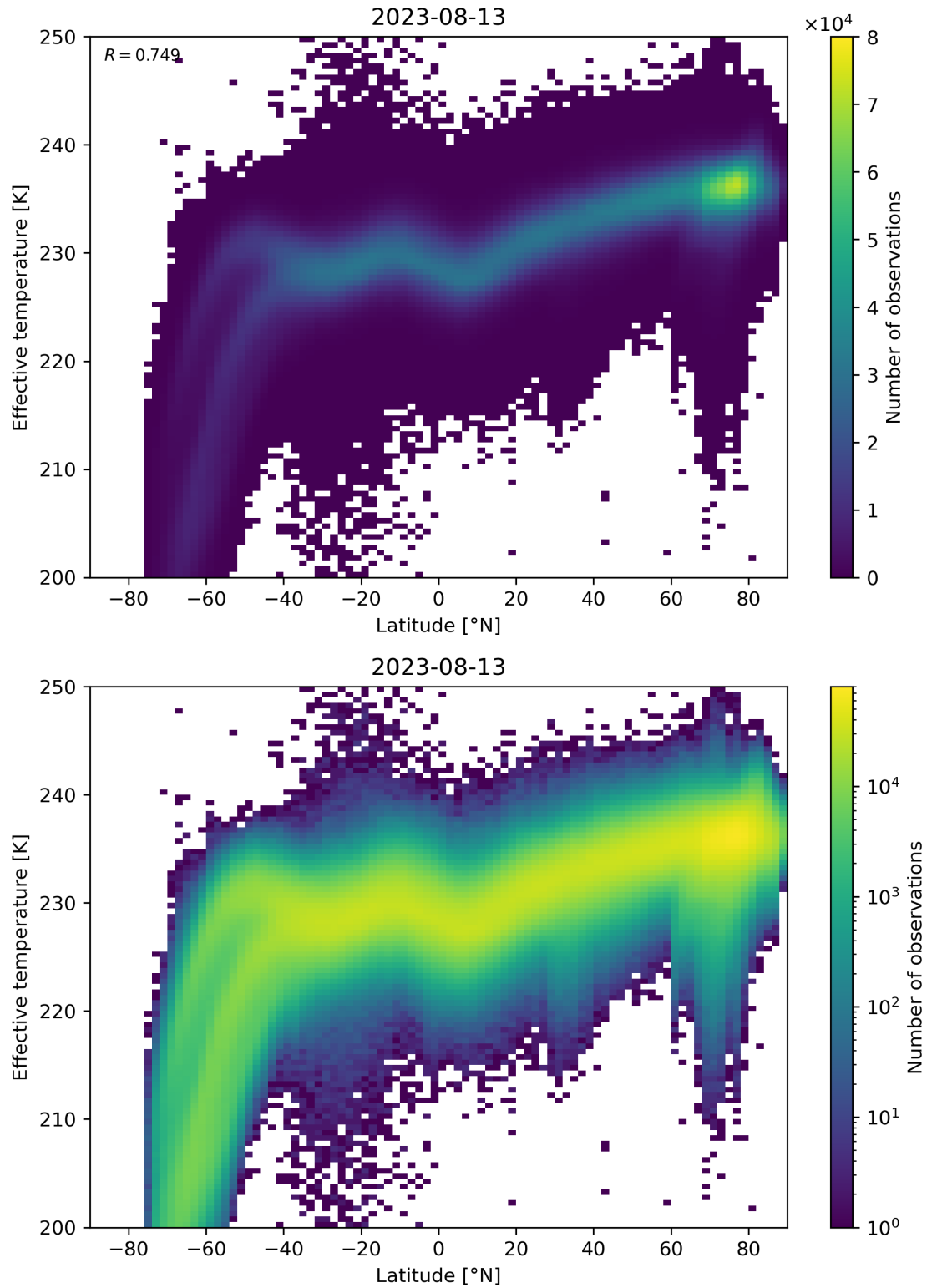
Figure 34: Scatter density plot of “Latitude” against “Effective temperature” for 2023-08-12 to 2023-08-14.
