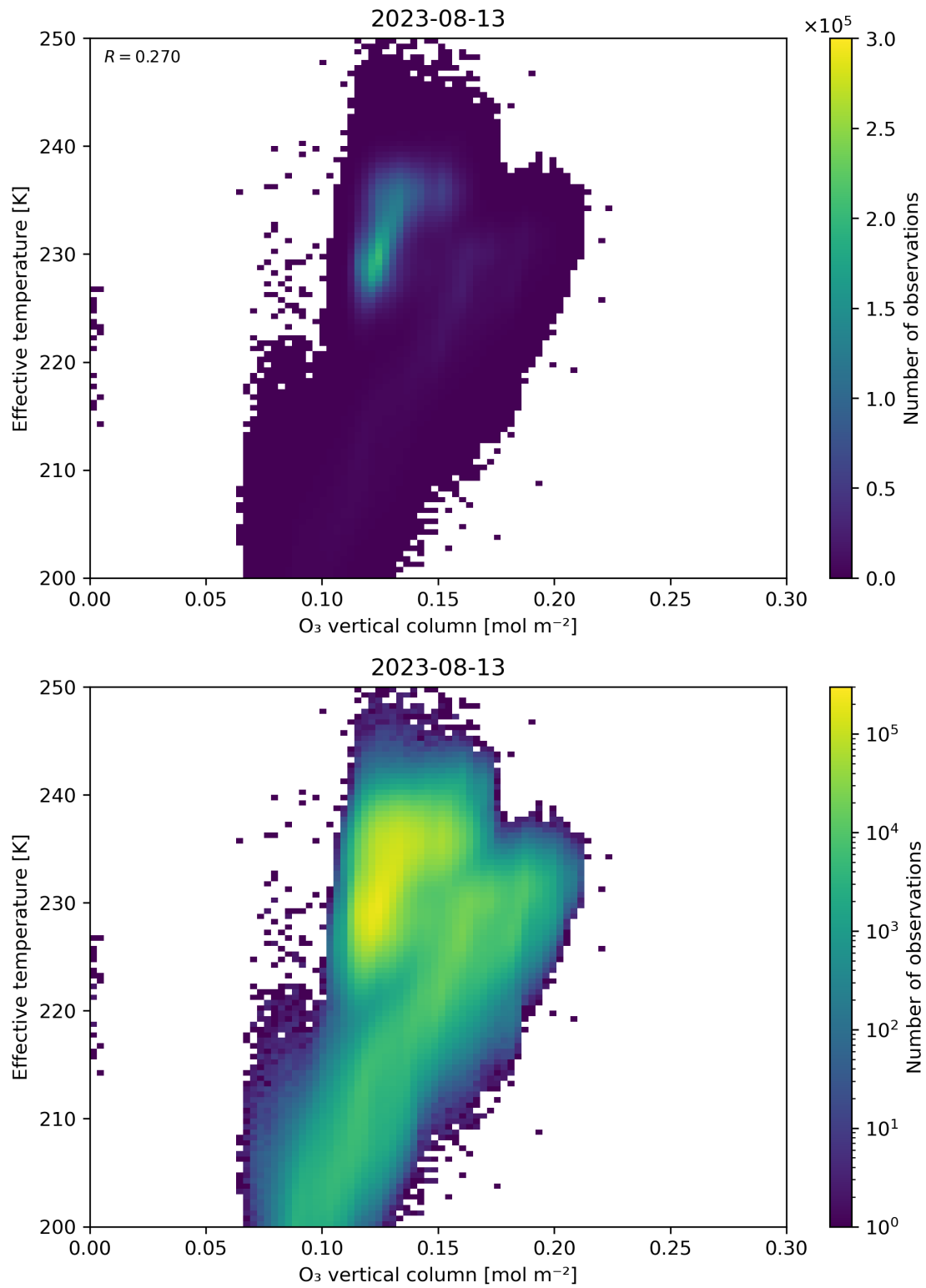
Figure 39: Scatter density plot of “O 3 vertical column” against “Effective temperature” for 2023-08-12 to 2023-08-14.
