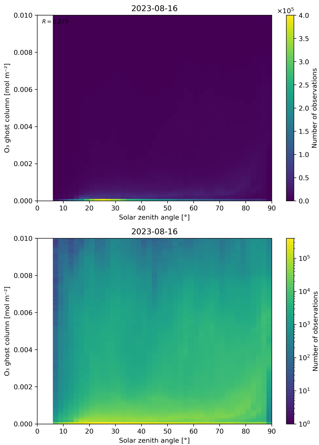
Figure 46: Scatter density plot of “Solar zenith angle” against “O 3 ghost column” for 2023-08-15 to 2023-08-17.
