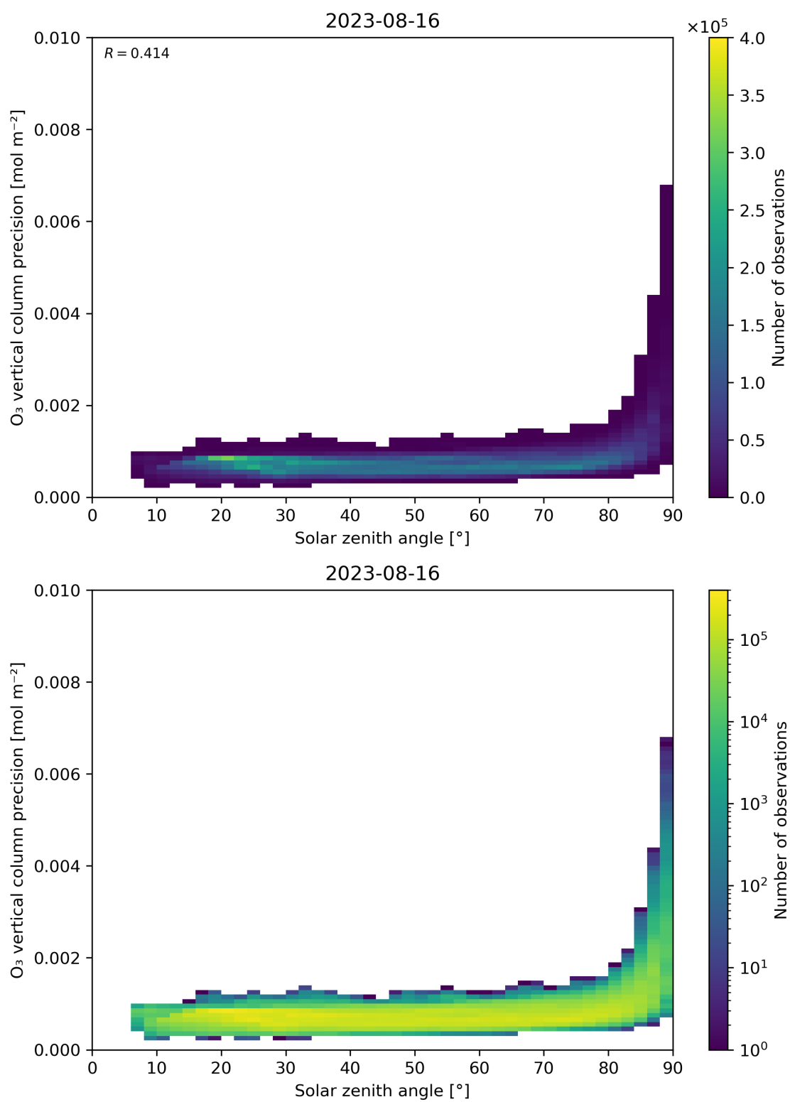
Figure 48: Scatter density plot of “Solar zenith angle” against “O 3 vertical column precision” for 2023-08-15 to 2023-08-17.
