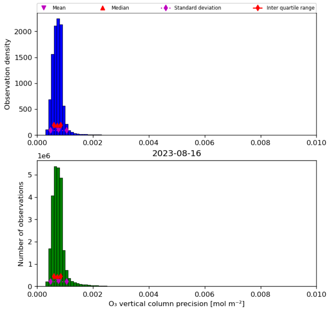
Figure 22: Histogram of “O 3 vertical column precision” for 2023-08-15 to 2023-08-17
