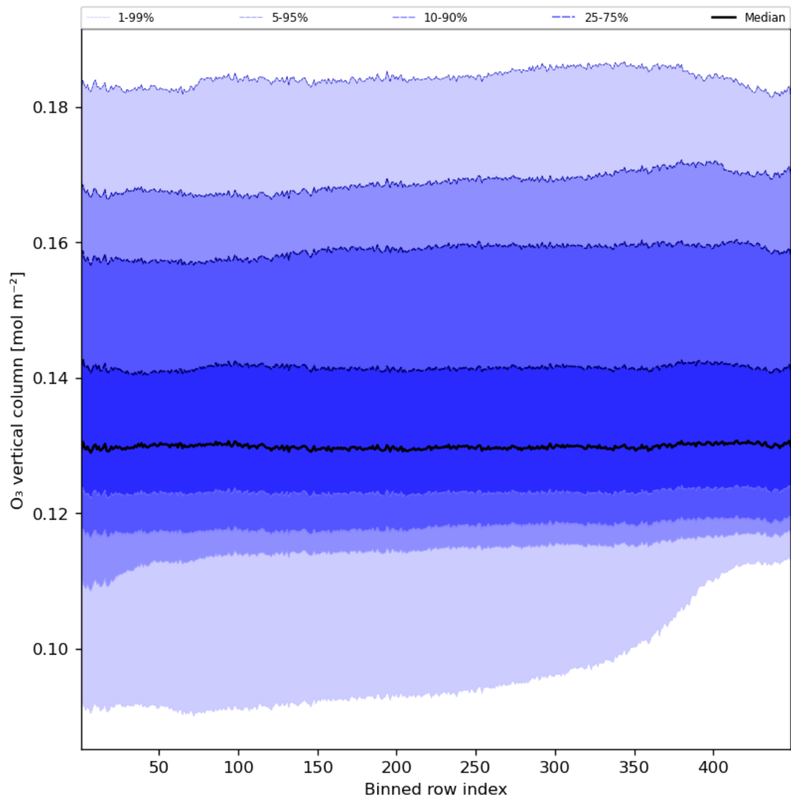
Figure 28: Along track statistics of “O 3 vertical column” for 2023-08-15 to 2023-08-17
