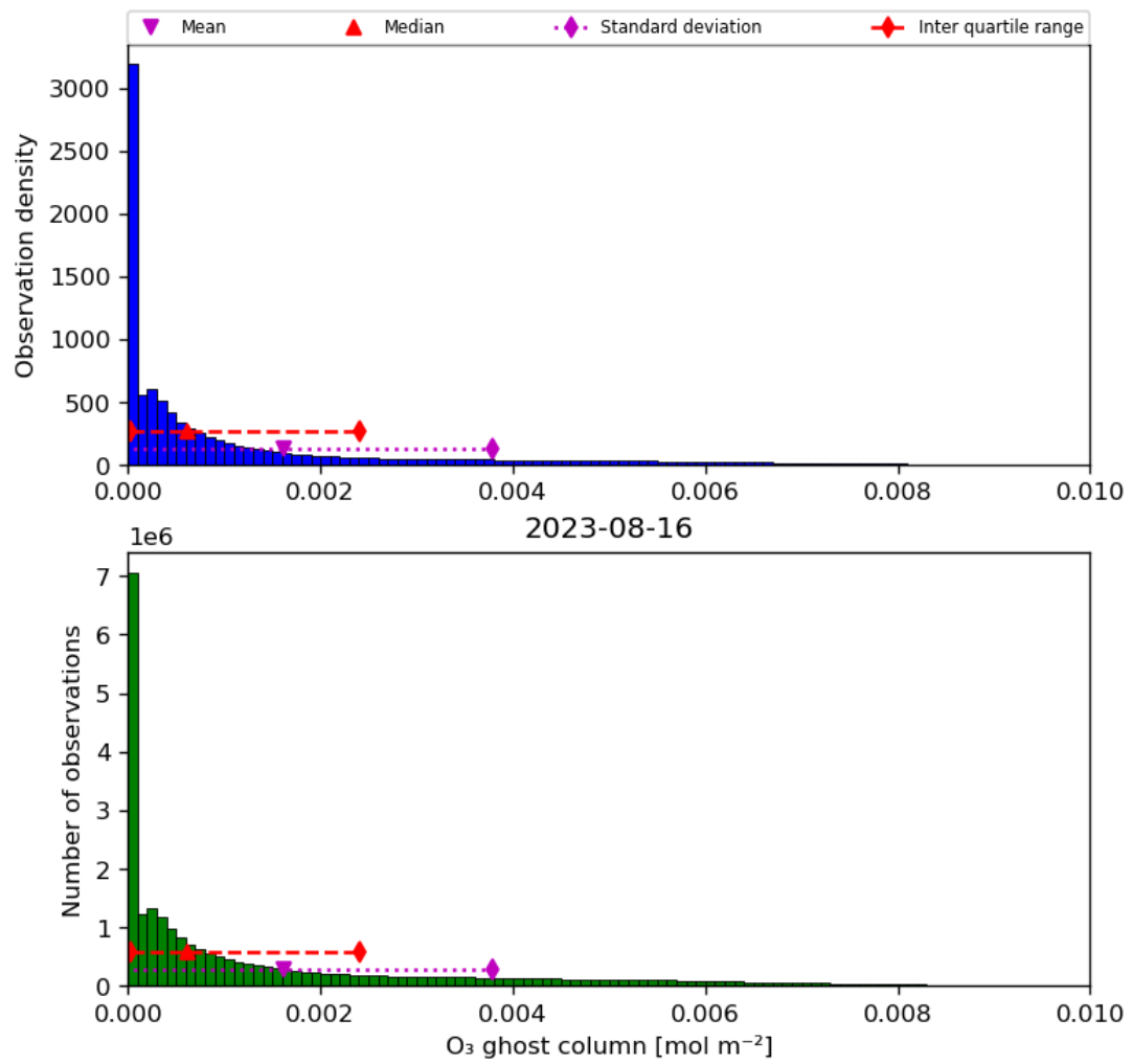
Figure 25: Histogram of “O 3 ghost column” for 2023-08-15 to 2023-08-17
