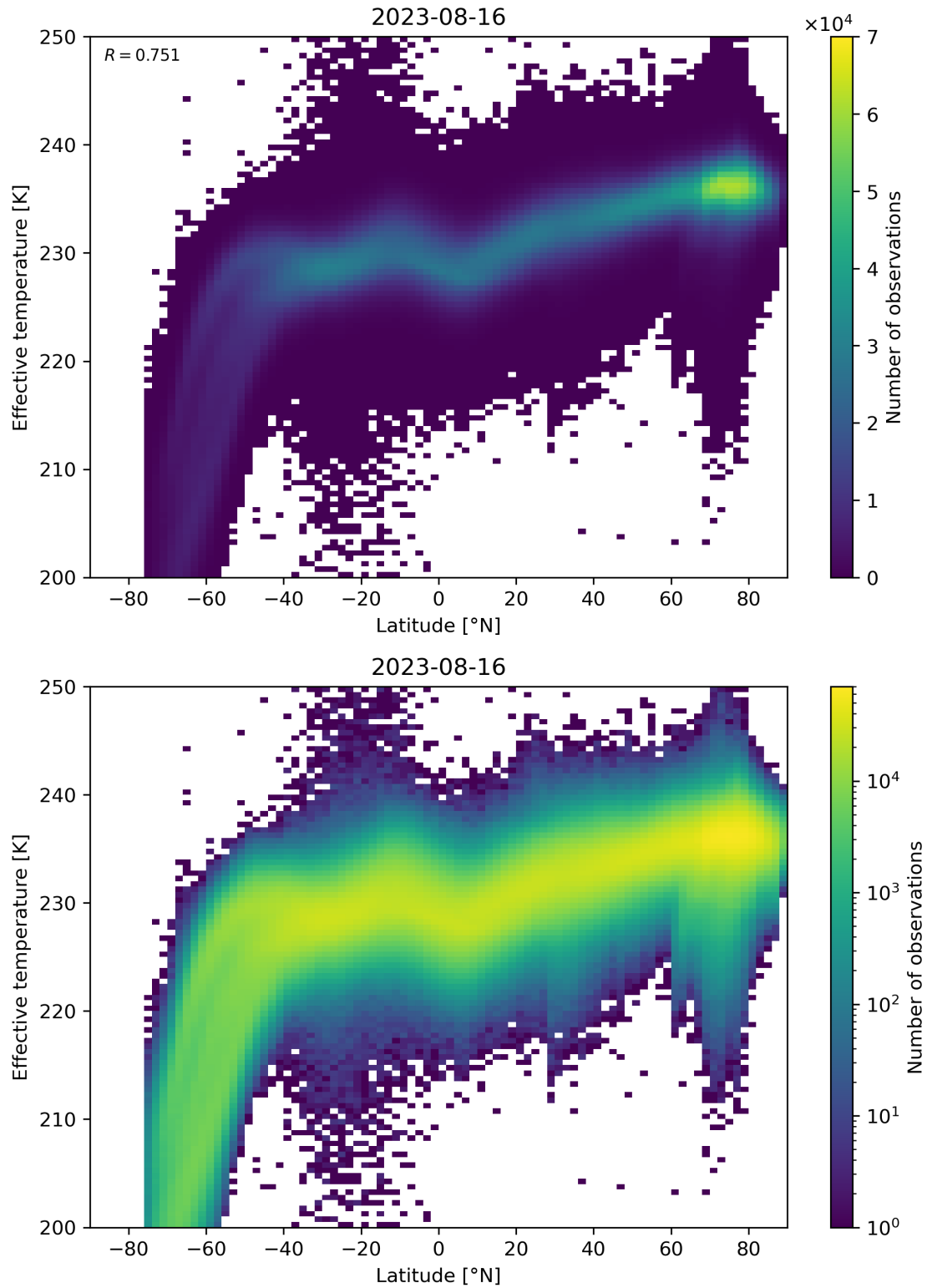
Figure 34: Scatter density plot of “Latitude” against “Effective temperature” for 2023-08-15 to 2023-08-17.
