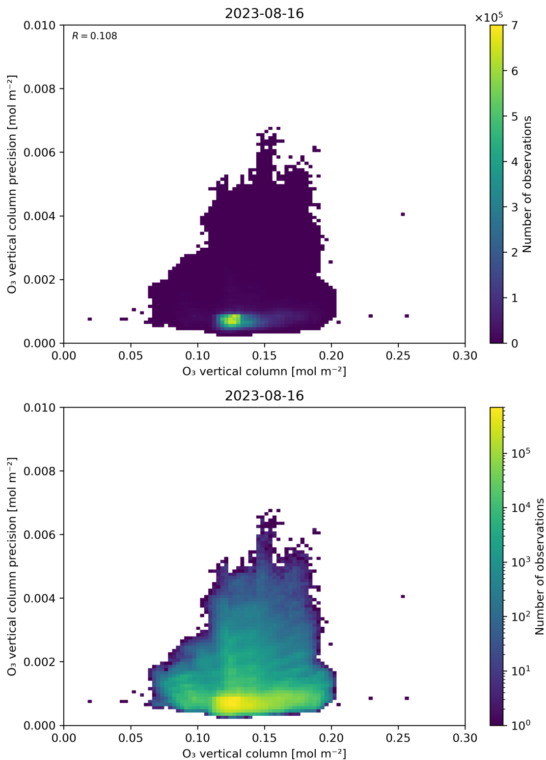
Figure 41: Scatter density plot of “O 3 vertical column” against “O 3 vertical column precision” for 2023-08-15 to 2023-08-17.
