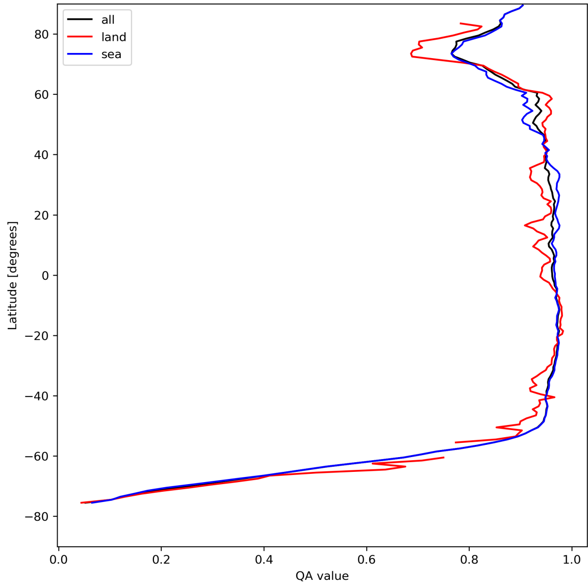
Figure 13: Zonal average of “QA value” for 2023-08-15 to 2023-08-17.
