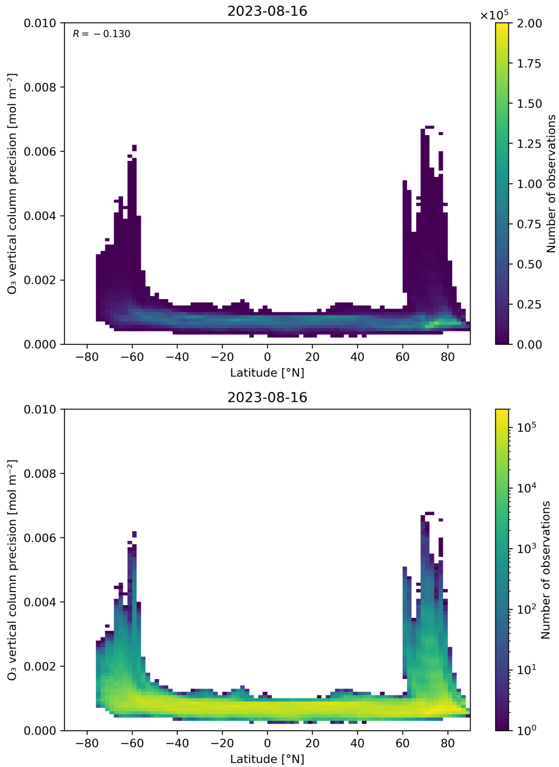
Figure 37: Scatter density plot of “Latitude” against “O 3 vertical column precision” for 2023-08-15 to 2023-08-17.
