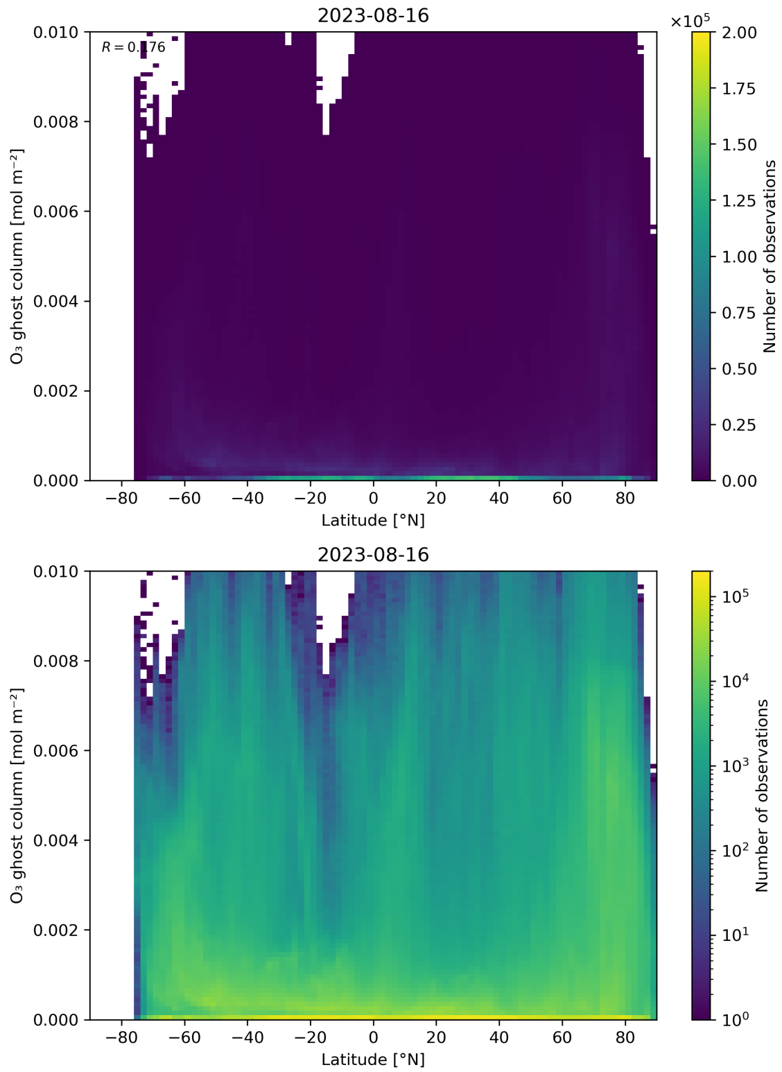
Figure 35: Scatter density plot of “Latitude” against “O 3 ghost column” for 2023-08-15 to 2023-08-17.
