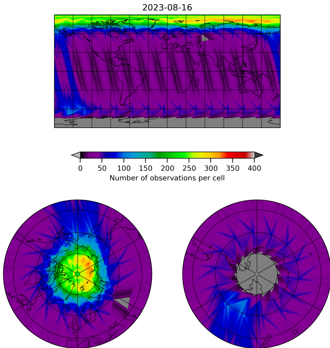
Figure 12: Map of the number of observations for 2023-08-15 to 2023-08-17
