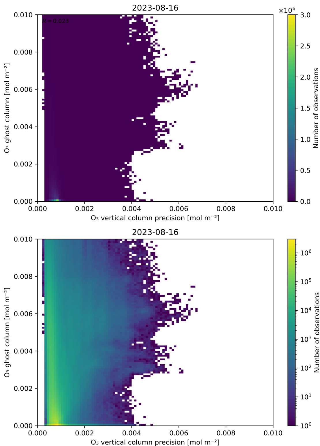
Figure 43: Scatter density plot of “O 3 vertical column precision” against “O 3 ghost column” for 2023-08-15 to 2023-08-17.
