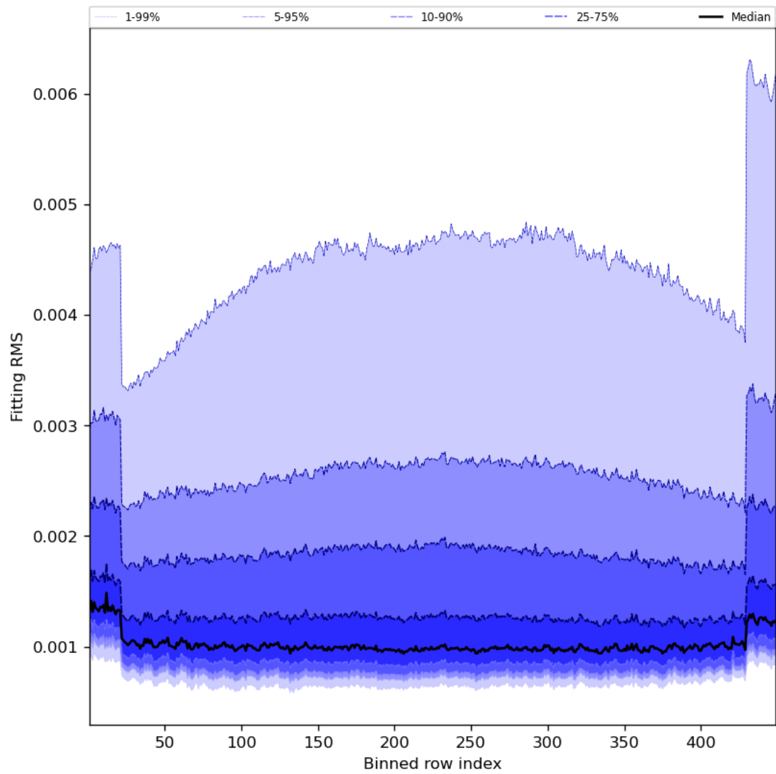
Figure 30: Along track statistics of “Fitting RMS” for 2023-08-15 to 2023-08-17
