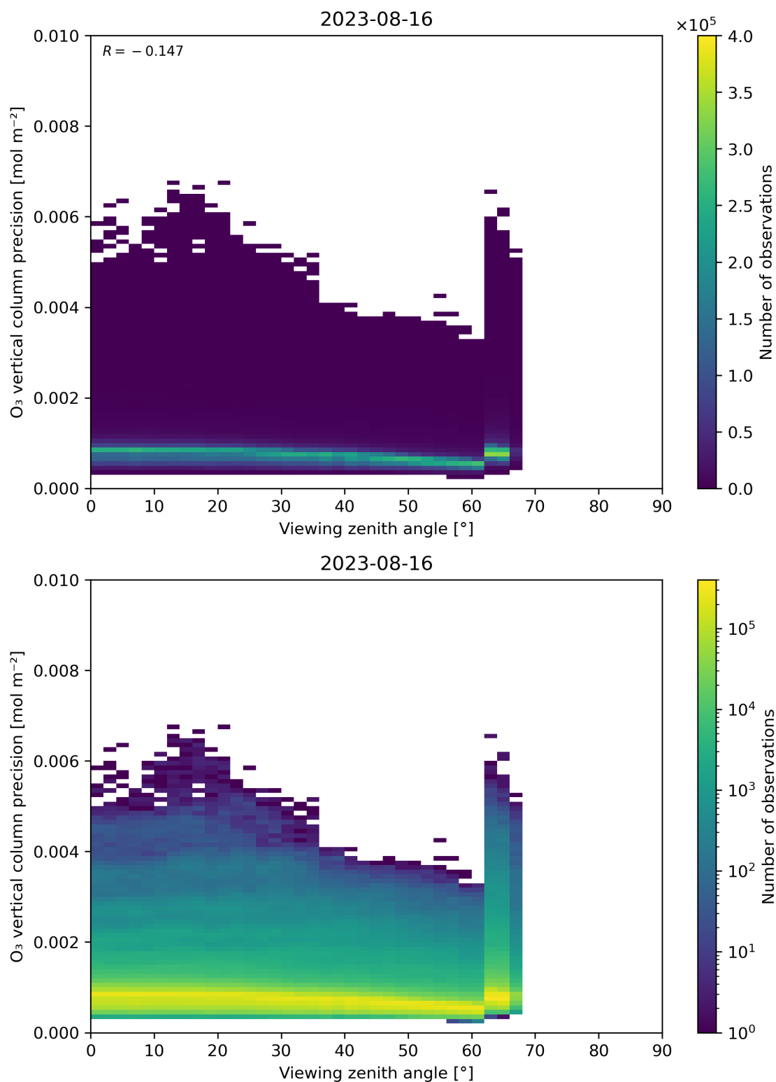
Figure 53: Scatter density plot of “Viewing zenith angle” against “O 3 vertical column precision” for 2023-08-15 to 2023-08-17.
