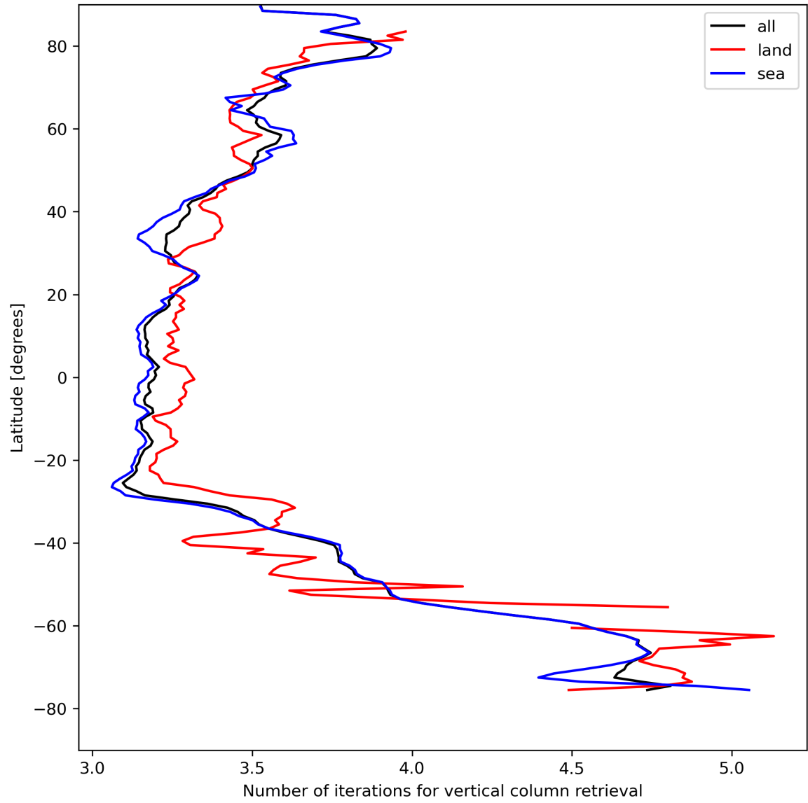
Figure 19: Zonal average of “Number of iterations for vertical column retrieval” for 2023-08-15 to 2023-08-17.
