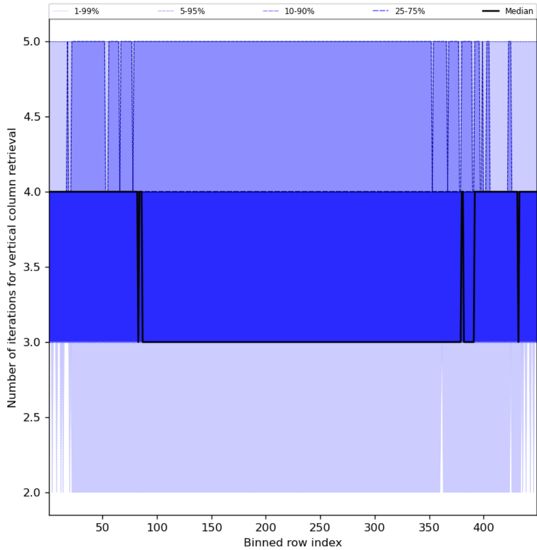
Figure 33: Along track statistics of “Number of iterations for vertical column retrieval” for 2023-08-15 to 2023-08-17
