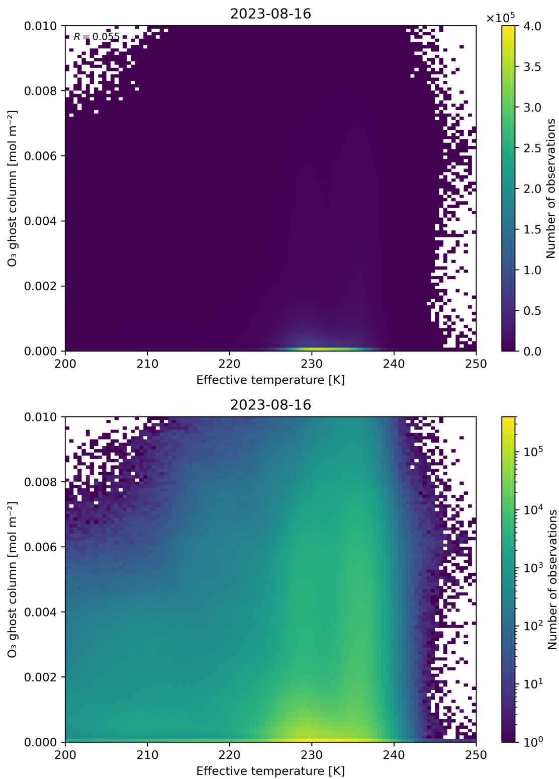
Figure 38: Scatter density plot of “Effective temperature” against “O 3 ghost column” for 2023-08-15 to 2023-08-17.
