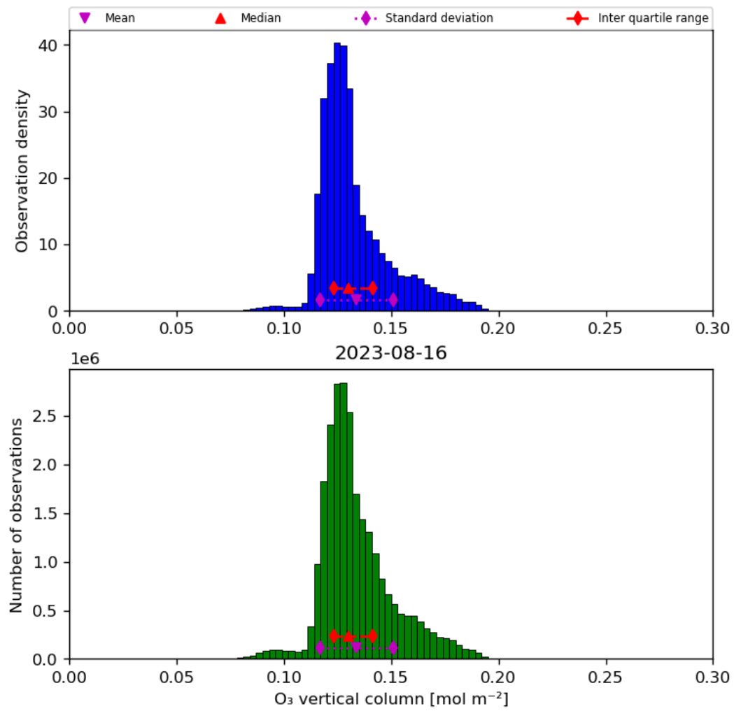
Figure 21: Histogram of “O 3 vertical column” for 2023-08-15 to 2023-08-17
