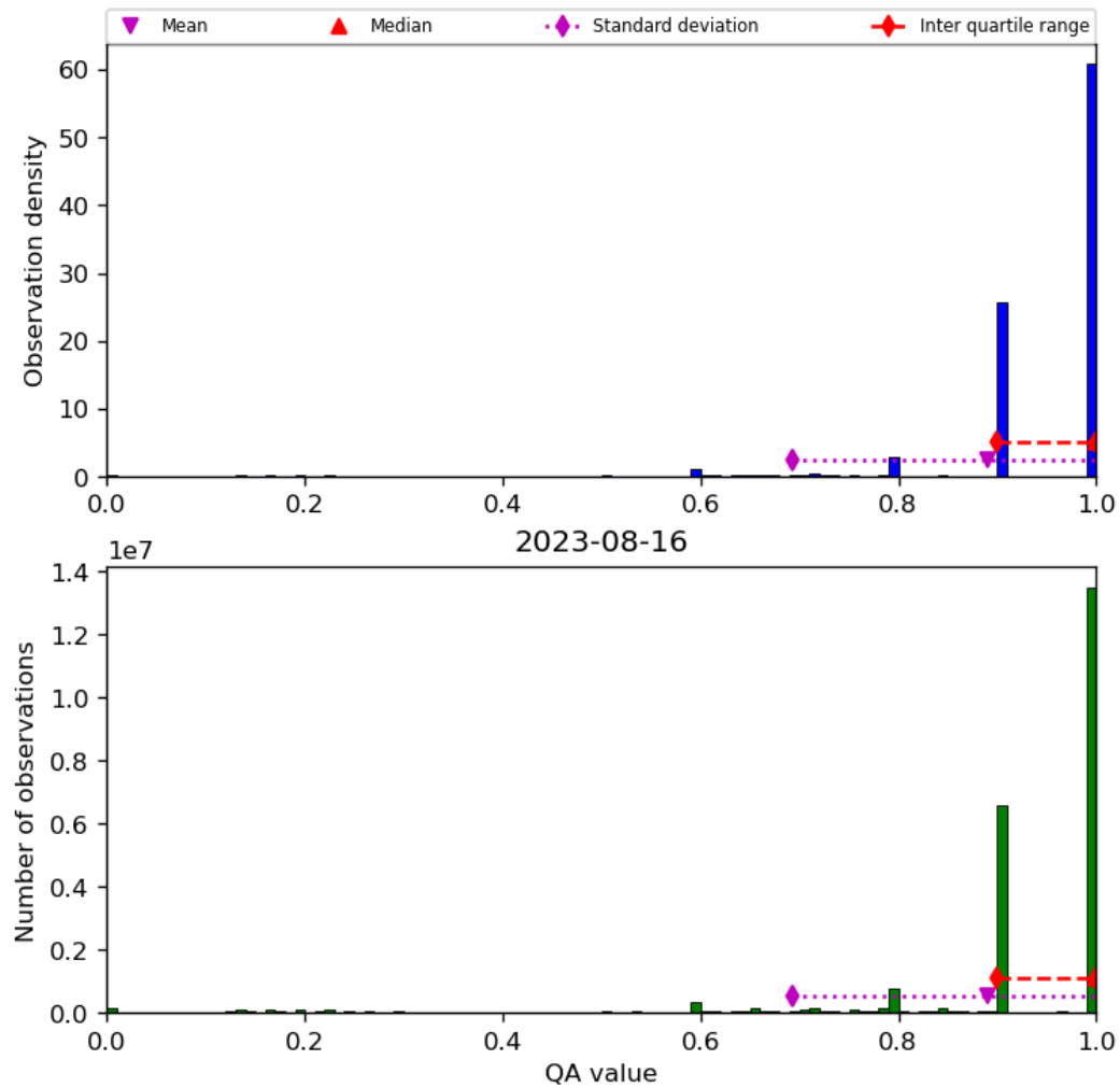
Figure 20: Histogram of “QA value” for 2023-08-15 to 2023-08-17
