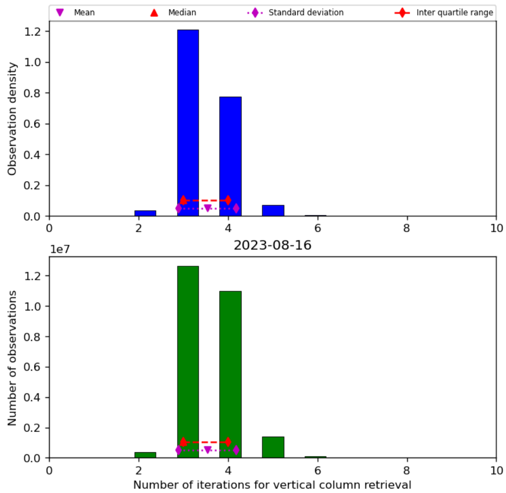
Figure 26: Histogram of “Number of iterations for vertical column retrieval” for 2023-08-15 to 2023-08-17
