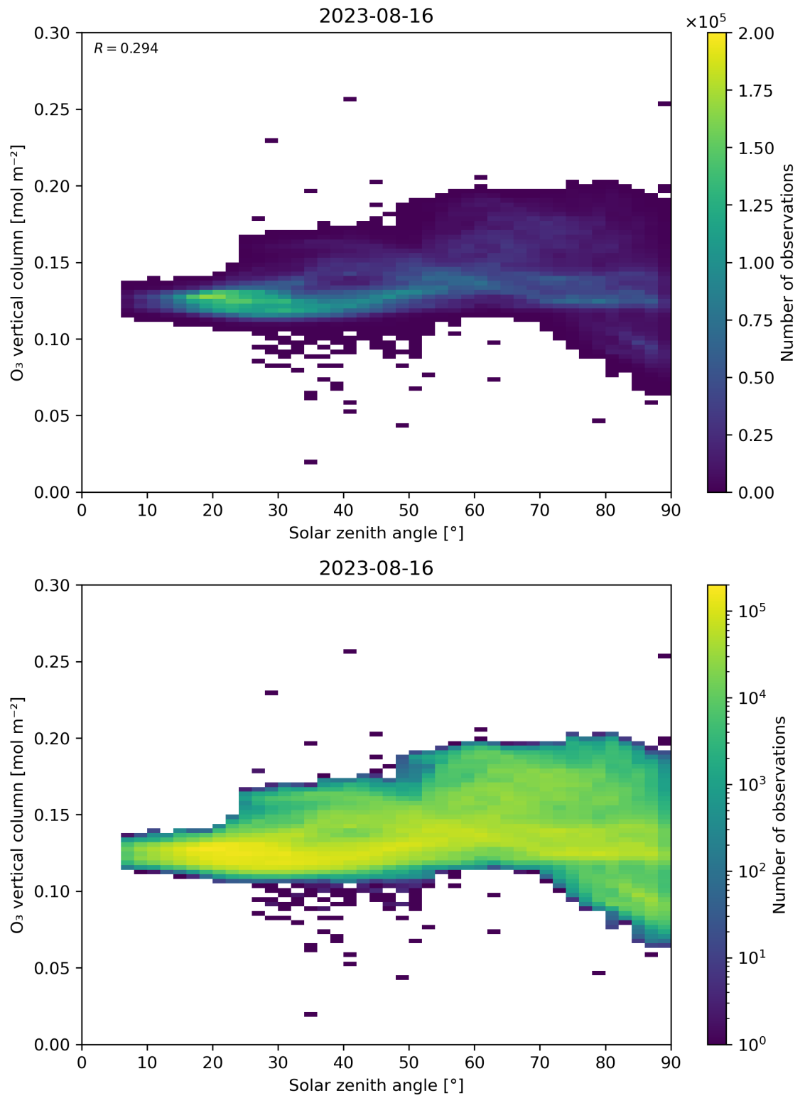
Figure 47: Scatter density plot of “Solar zenith angle” against “O 3 vertical column” for 2023-08-15 to 2023-08-17.
