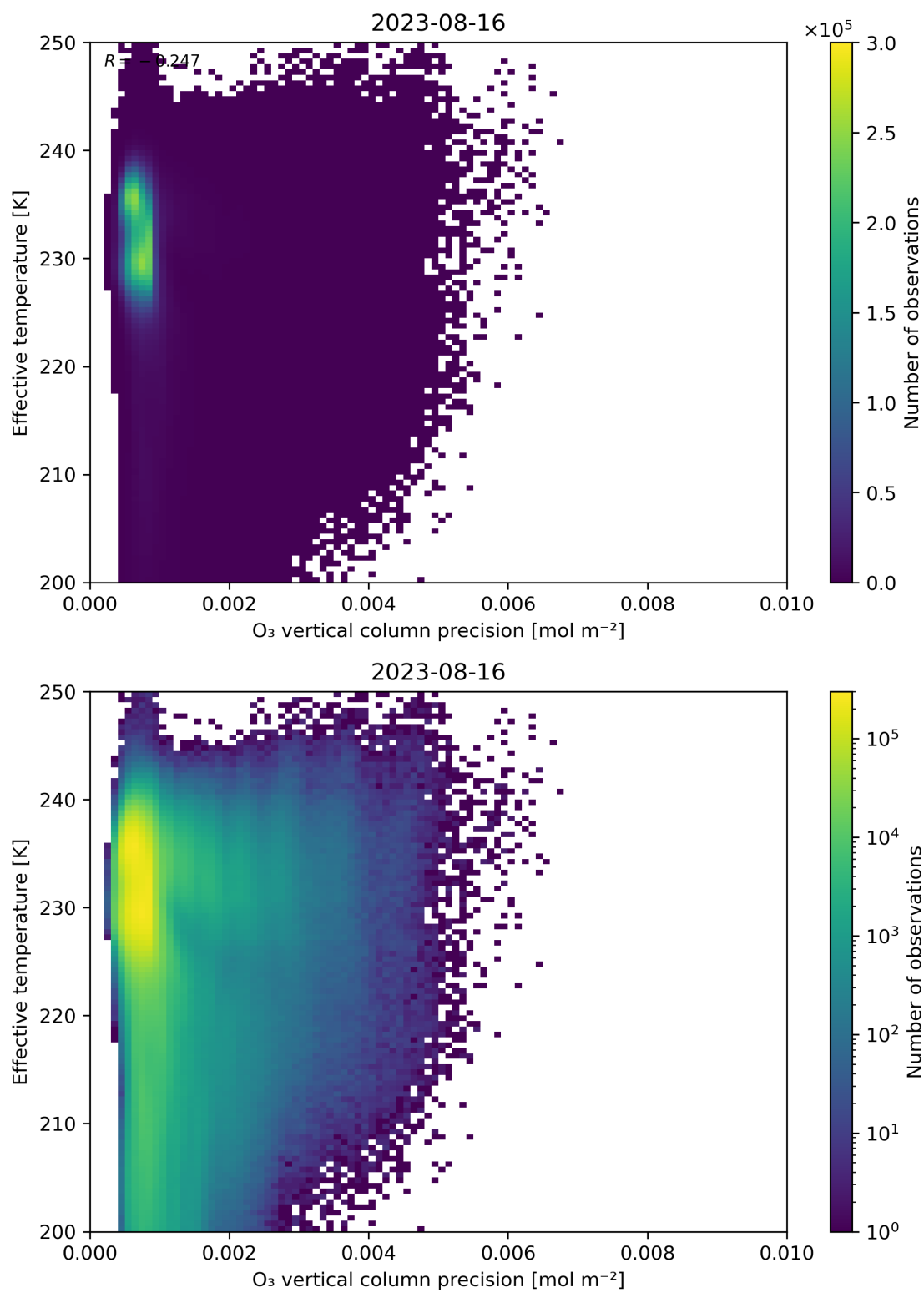
Figure 42: Scatter density plot of “O 3 vertical column precision” against “Effective temperature” for 2023-08-15 to 2023-08-17.
