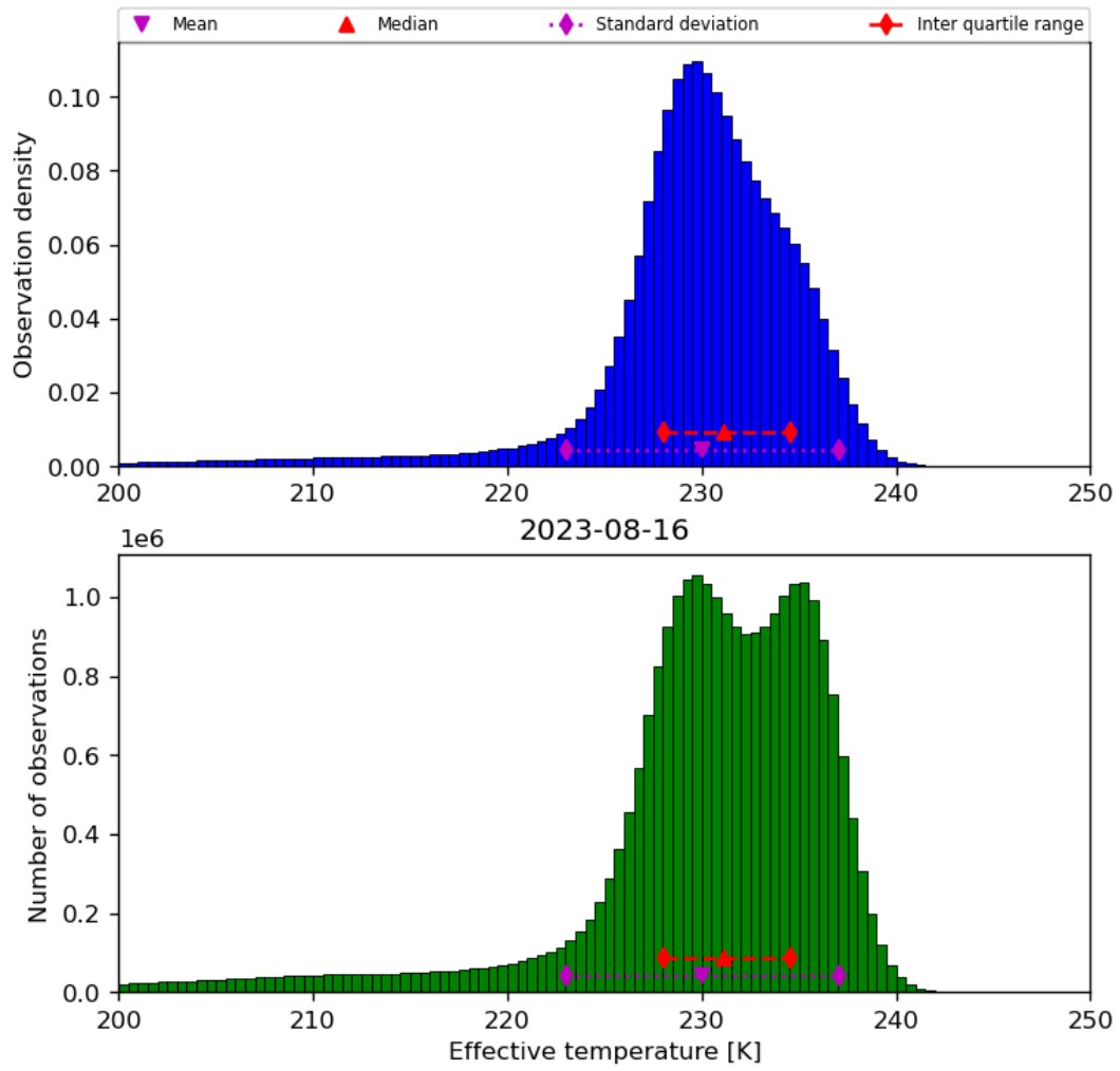
Figure 24: Histogram of “Effective temperature” for 2023-08-15 to 2023-08-17
