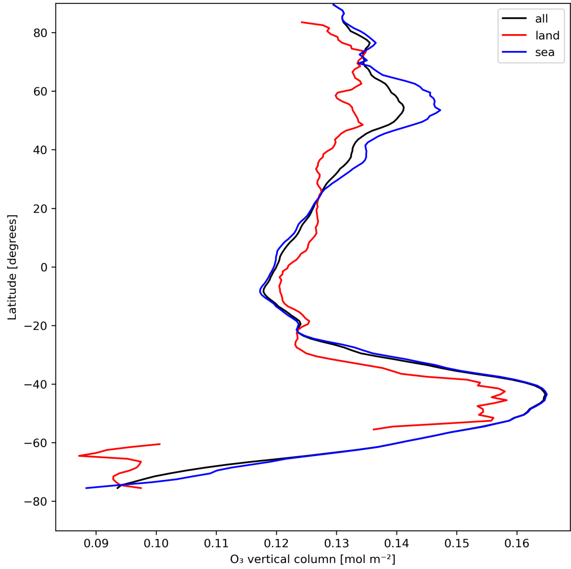
Figure 14: Zonal average of “O 3 vertical column” for 2023-08-15 to 2023-08-17.
