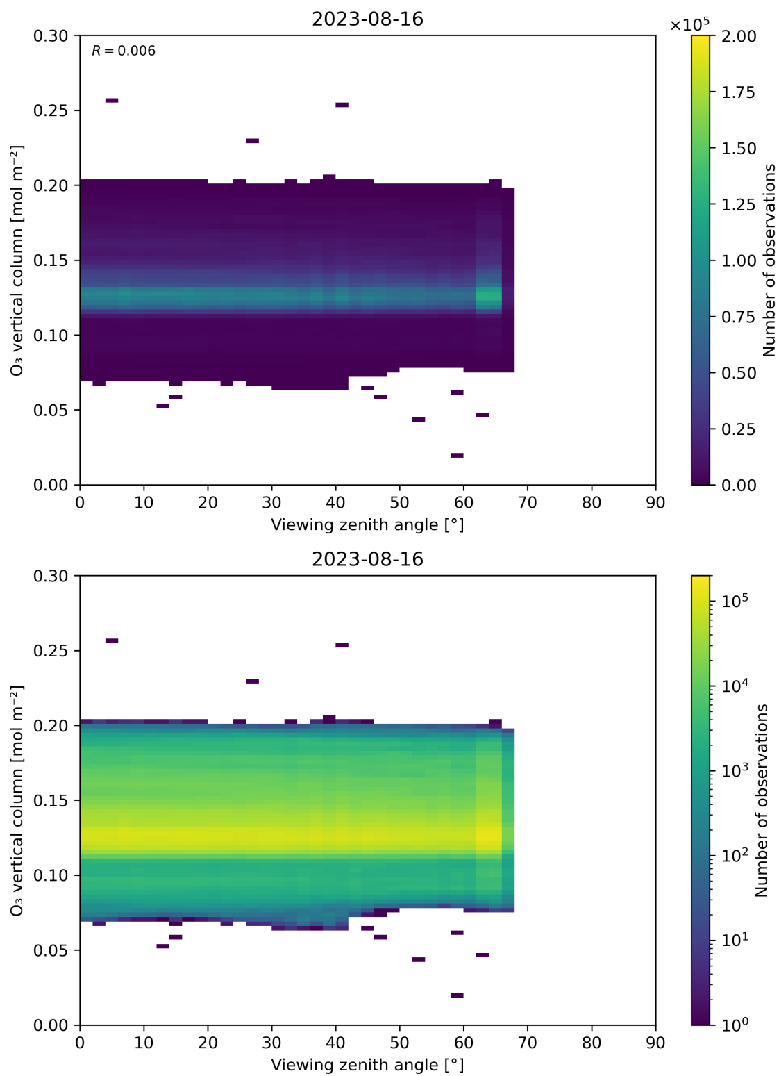
Figure 52: Scatter density plot of “Viewing zenith angle” against “O 3 vertical column” for 2023-08-15 to 2023-08-17.
