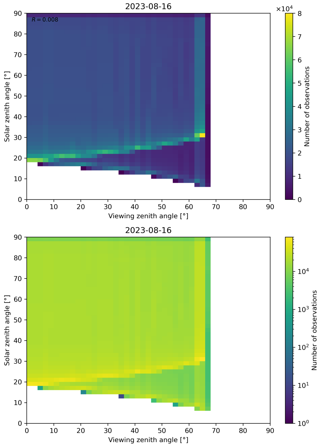
Figure 54: Scatter density plot of “Viewing zenith angle” against “Solar zenith angle” for 2023-08-15 to 2023-08-17.
