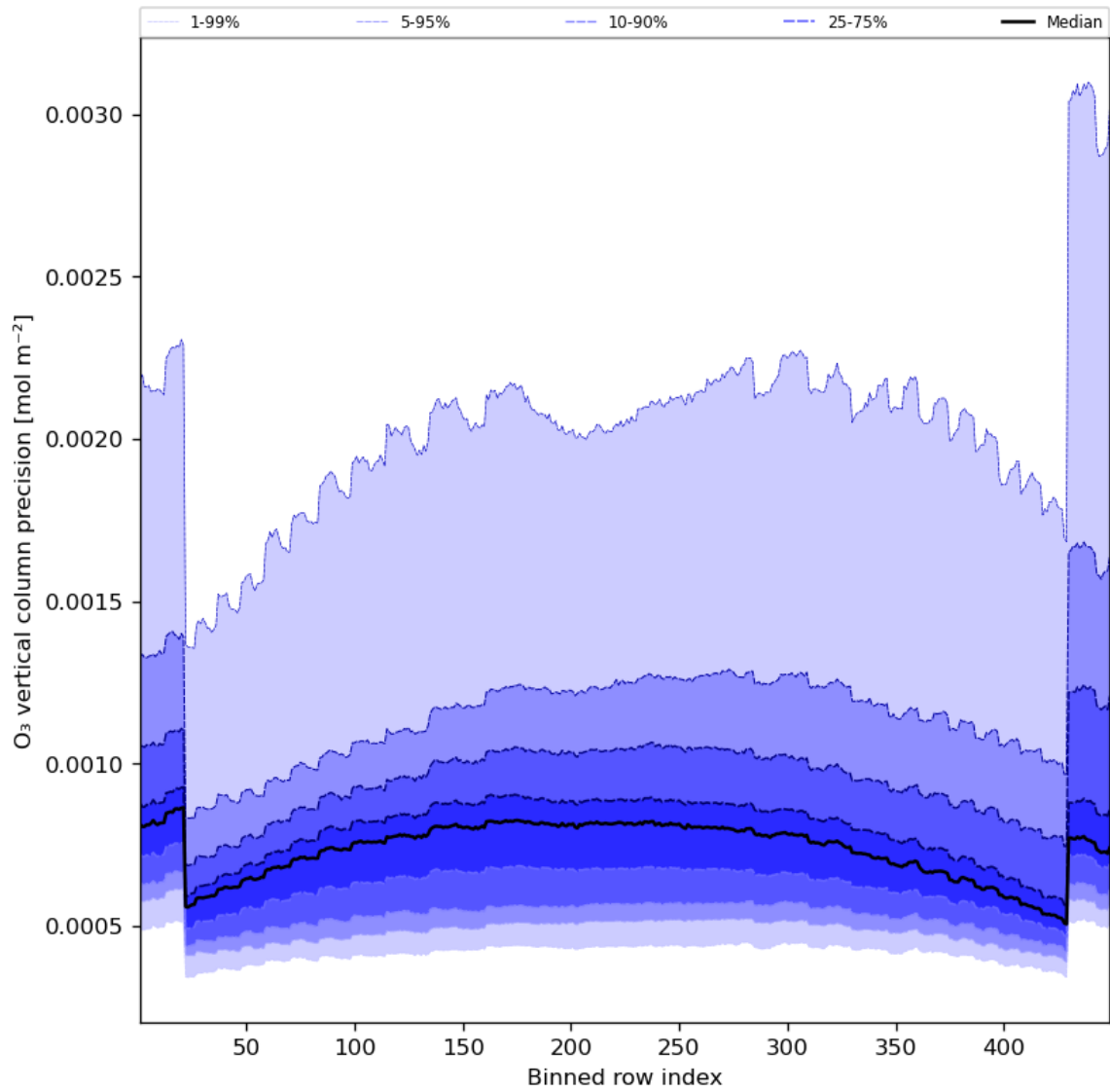
Figure 29: Along track statistics of “O 3 vertical column precision” for 2023-08-15 to 2023-08-17
