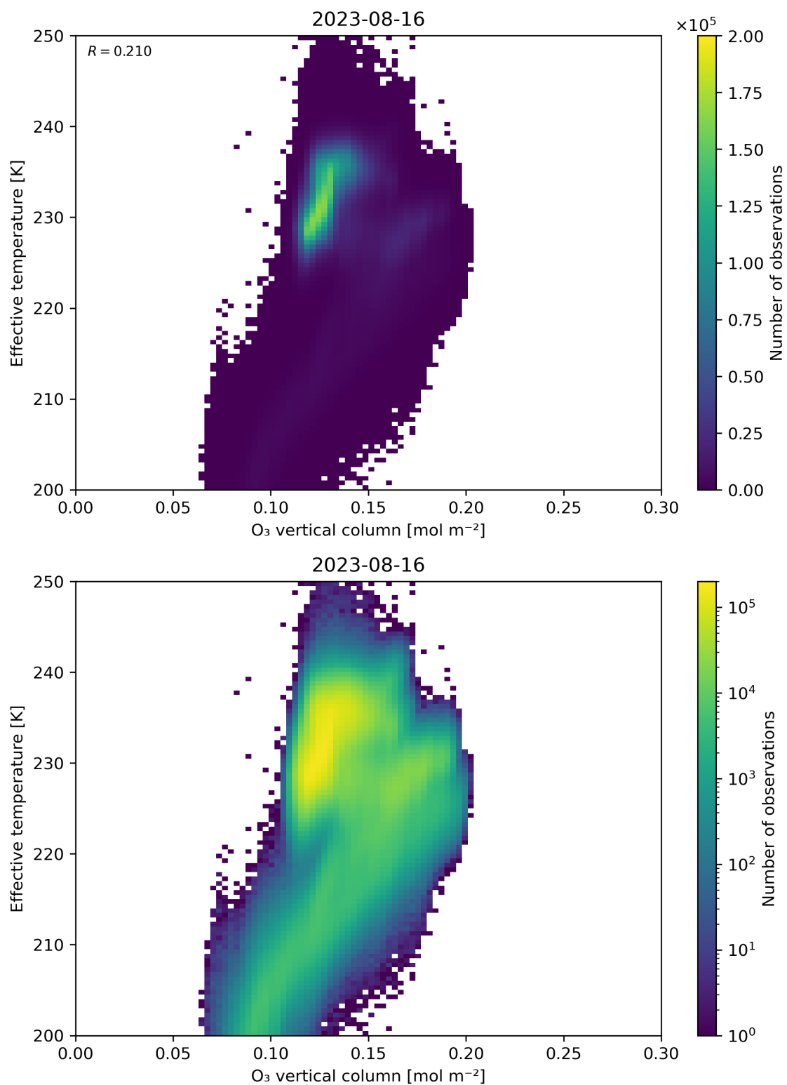
Figure 39: Scatter density plot of “O 3 vertical column” against “Effective temperature” for 2023-08-15 to 2023-08-17.
