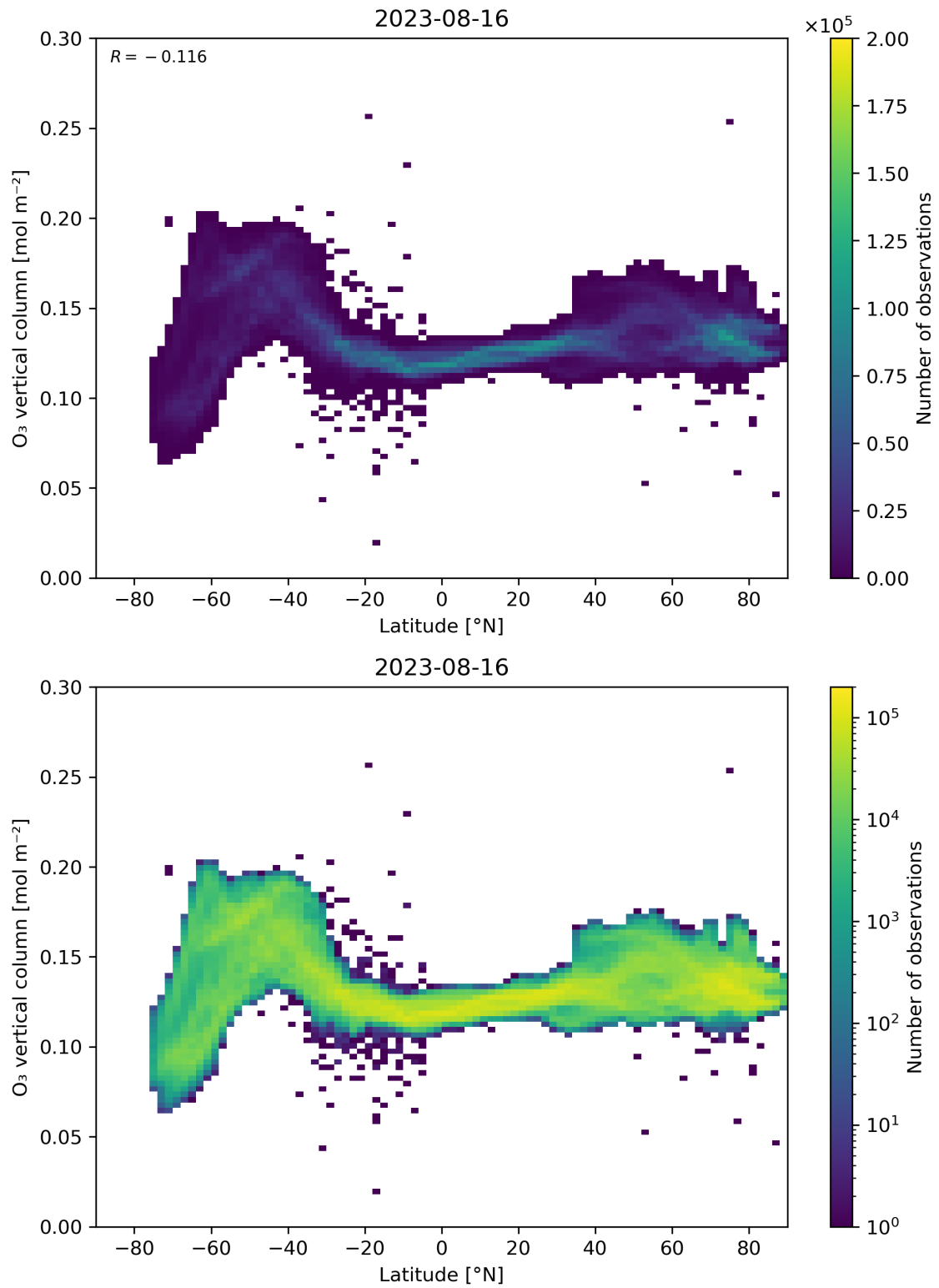
Figure 36: Scatter density plot of “Latitude” against “O 3 vertical column” for 2023-08-15 to 2023-08-17.
