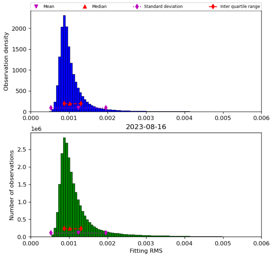
Figure 23: Histogram of “Fitting RMS” for 2023-08-15 to 2023-08-17
