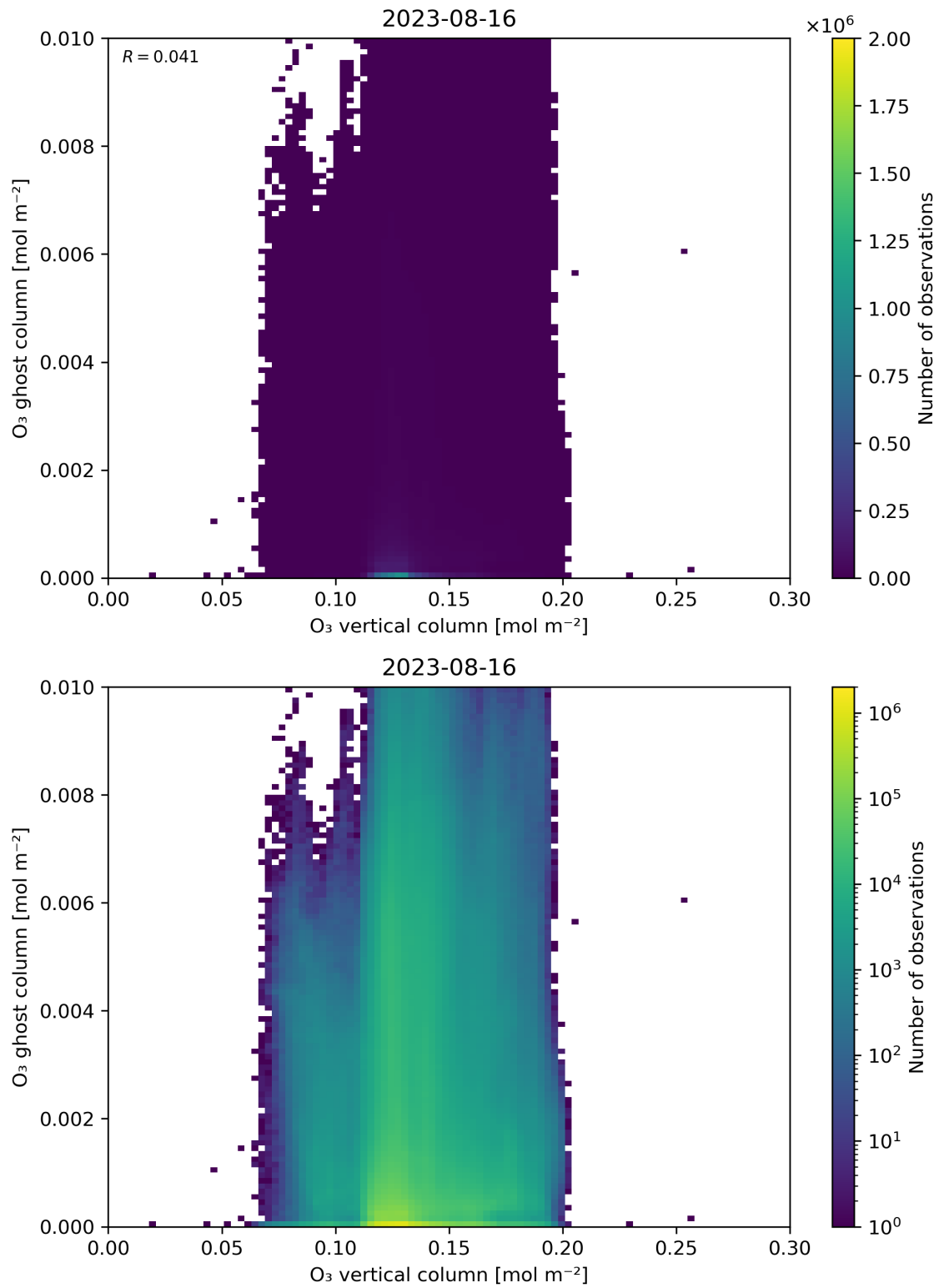
Figure 40: Scatter density plot of “O 3 vertical column” against “O 3 ghost column” for 2023-08-15 to 2023-08-17.
