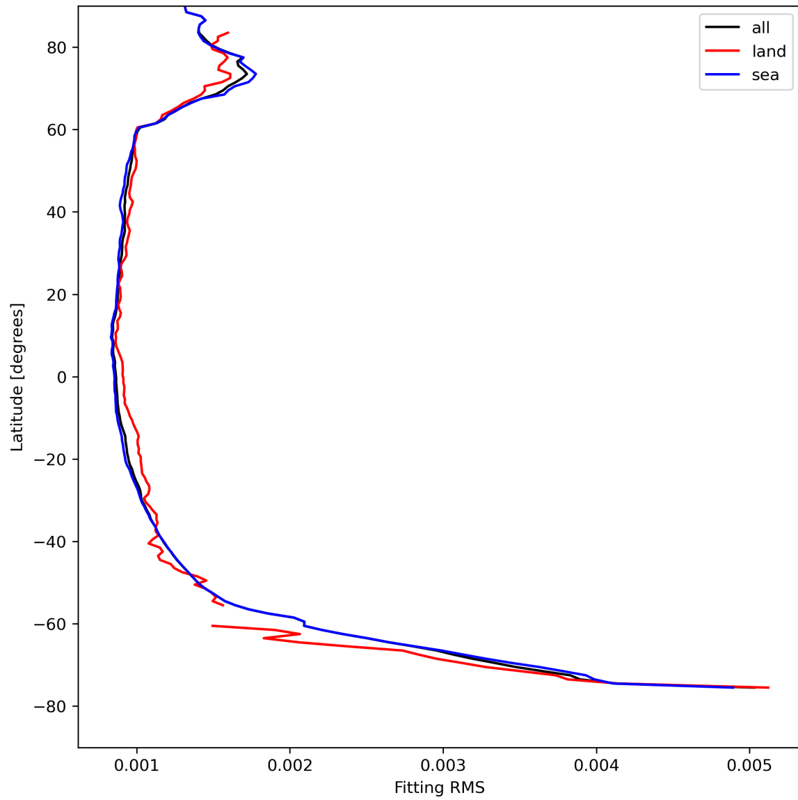
Figure 16: Zonal average of “Fitting RMS” for 2023-08-15 to 2023-08-17.
