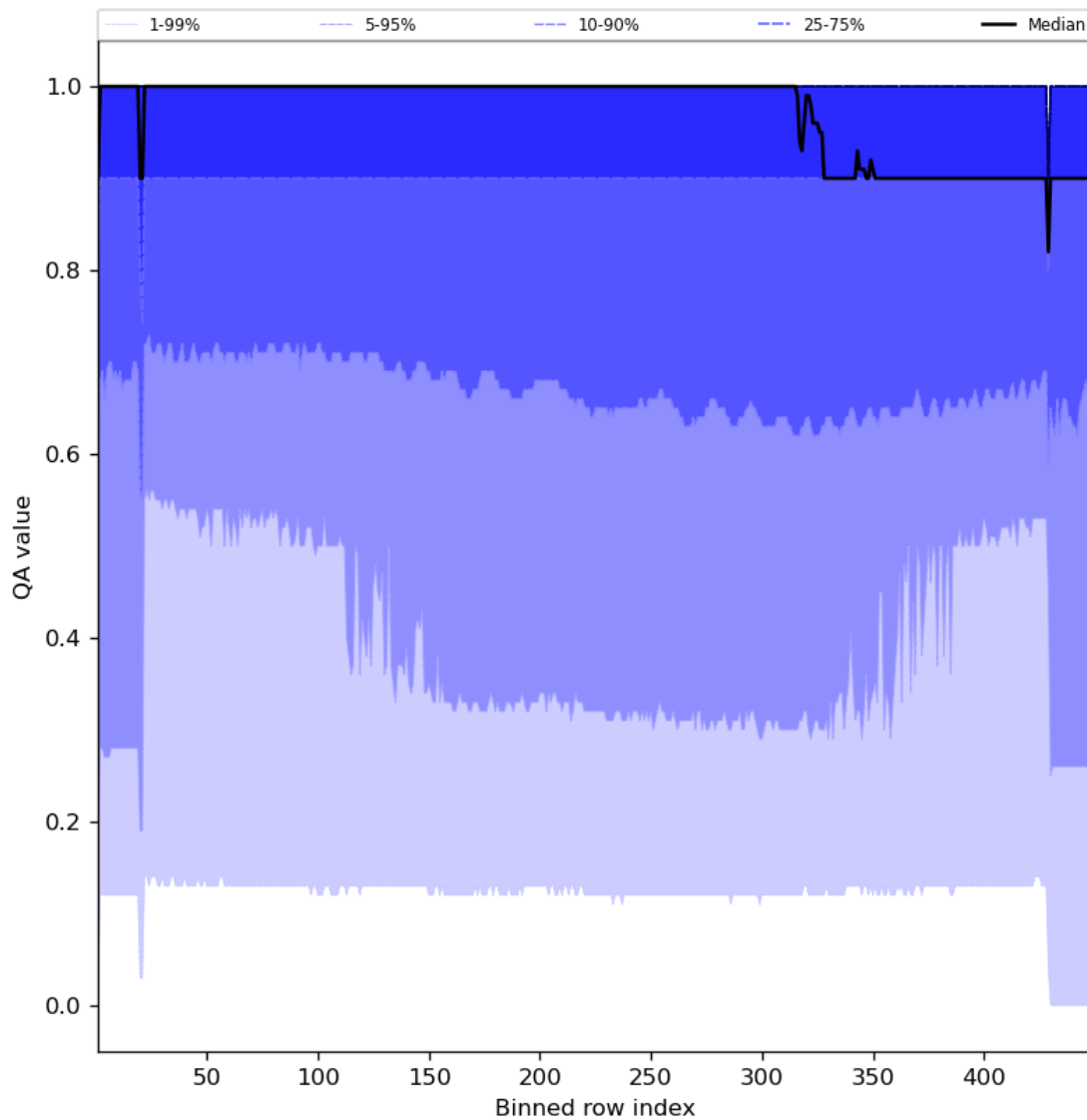
Figure 27: Along track statistics of “QA value” for 2023-08-15 to 2023-08-17
