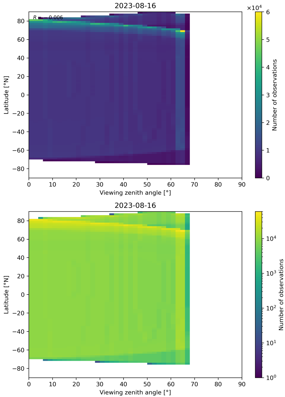
Figure 49: Scatter density plot of “Viewing zenith angle” against “Latitude” for 2023-08-15 to 2023-08-17.
