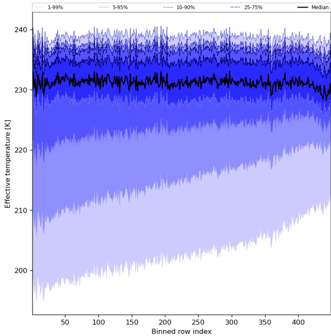
Figure 31: Along track statistics of “Effective temperature” for 2023-08-15 to 2023-08-17
