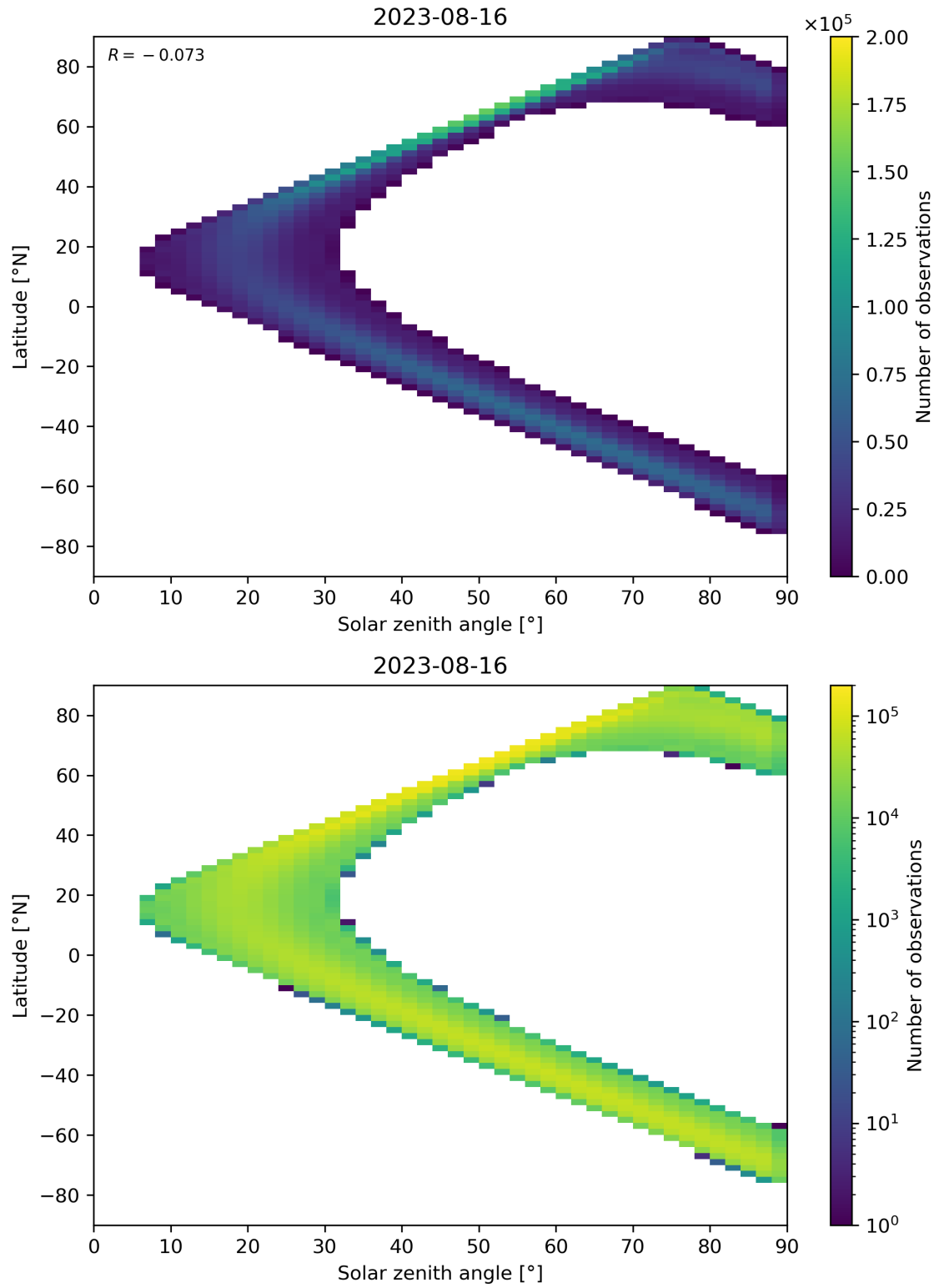
Figure 44: Scatter density plot of “Solar zenith angle” against “Latitude” for 2023-08-15 to 2023-08-17.
