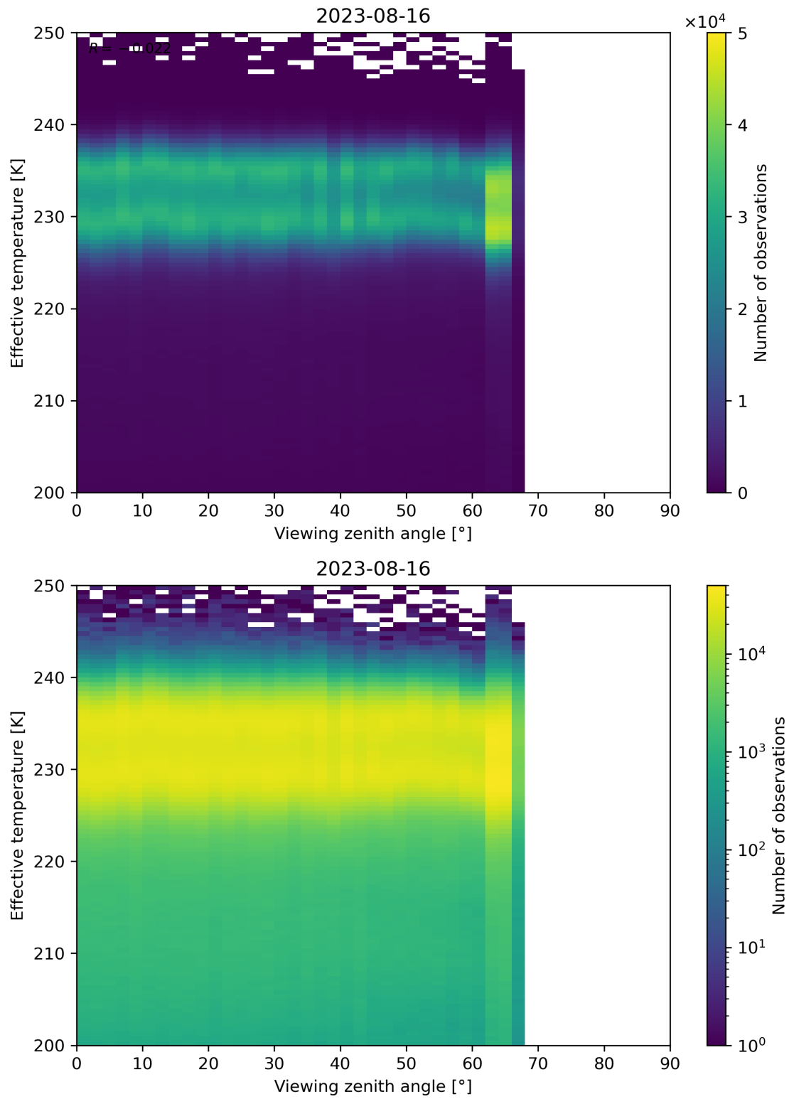
Figure 50: Scatter density plot of “Viewing zenith angle” against “Effective temperature” for 2023-08-15 to 2023-08-17.
