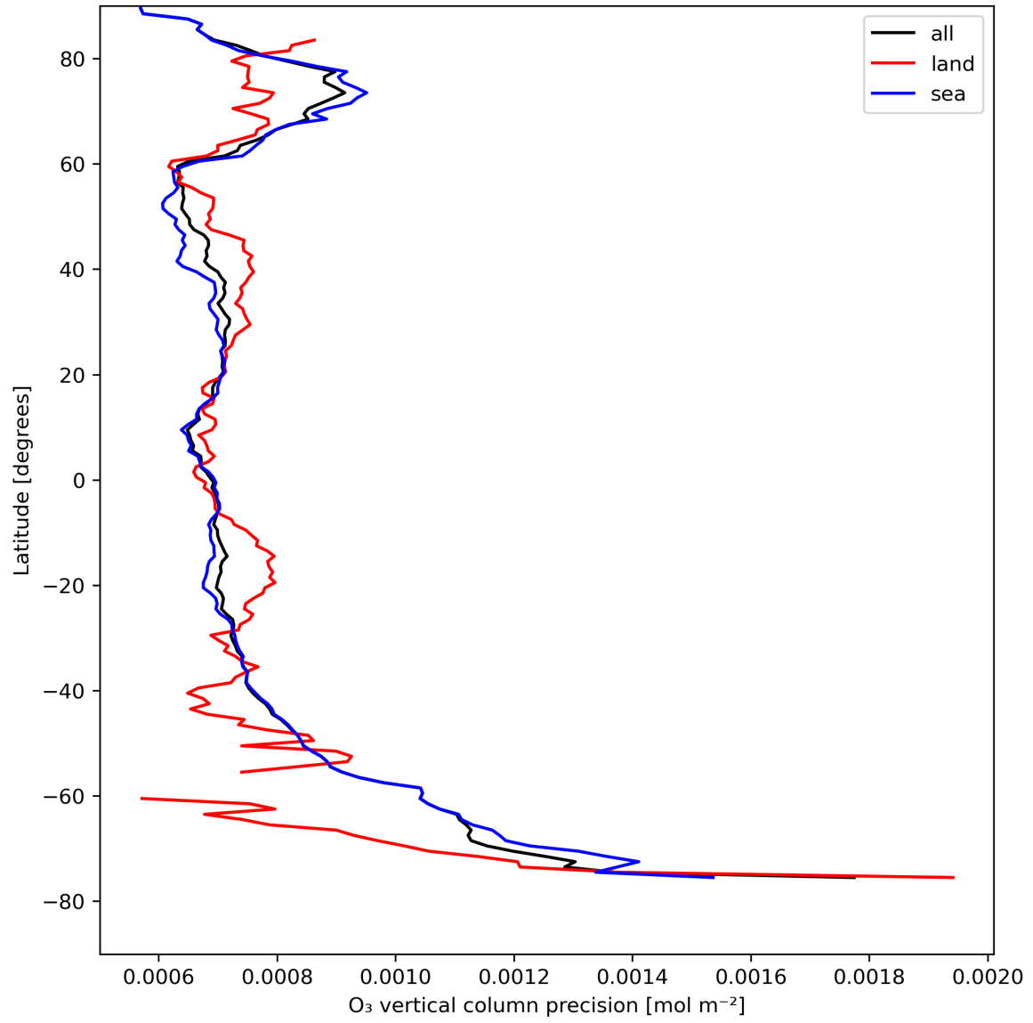
Figure 15: Zonal average of "O 3 vertical column precision" for 2023-08-15 to 2023-08-17.
