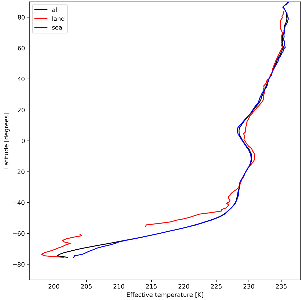
Figure 17: Zonal average of "Effective temperature" for 2023-08-15 to 2023-08-17.
