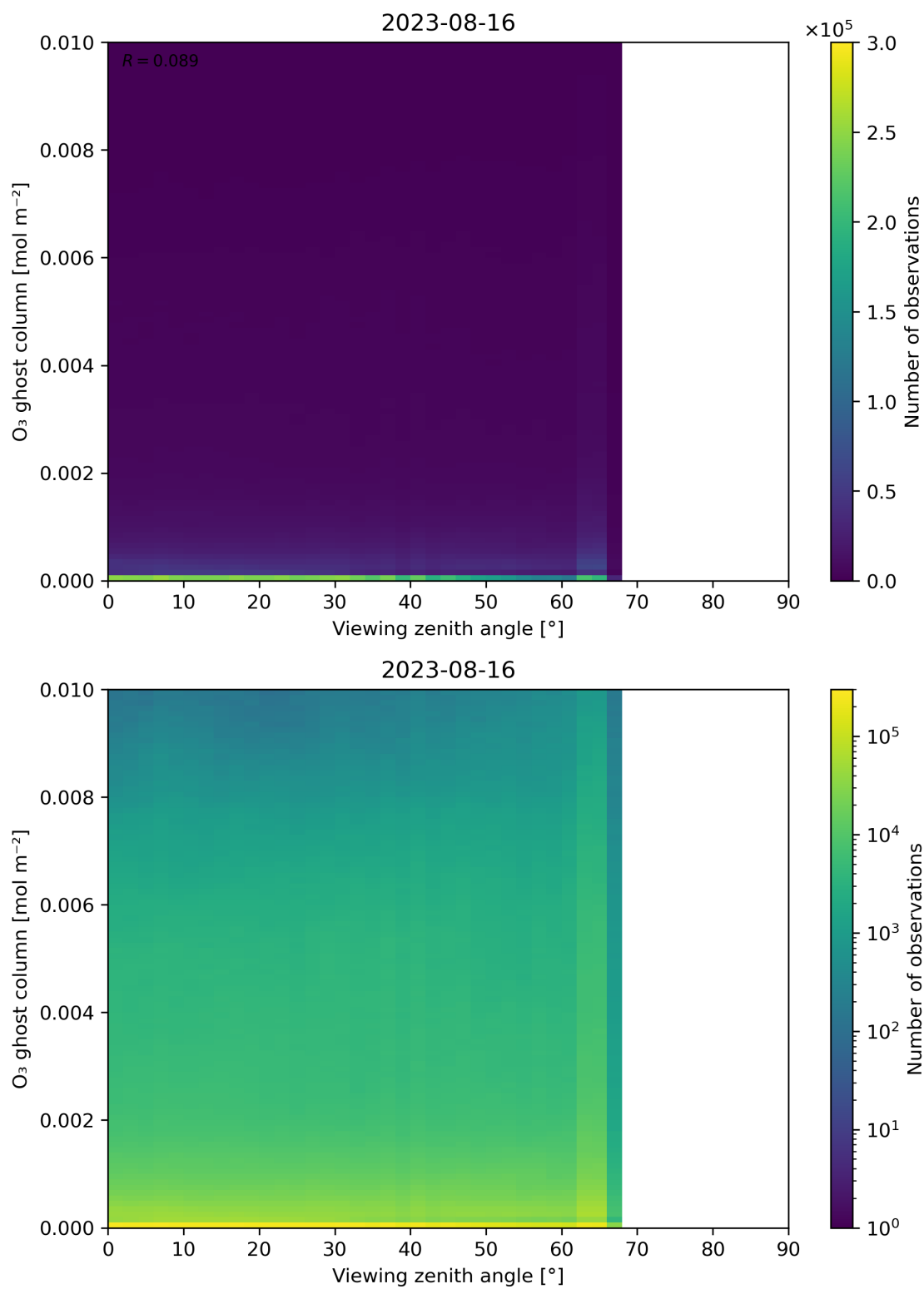
Figure 51: Scatter density plot of “Viewing zenith angle” against “O 3 ghost column” for 2023-08-15 to 2023-08-17.
