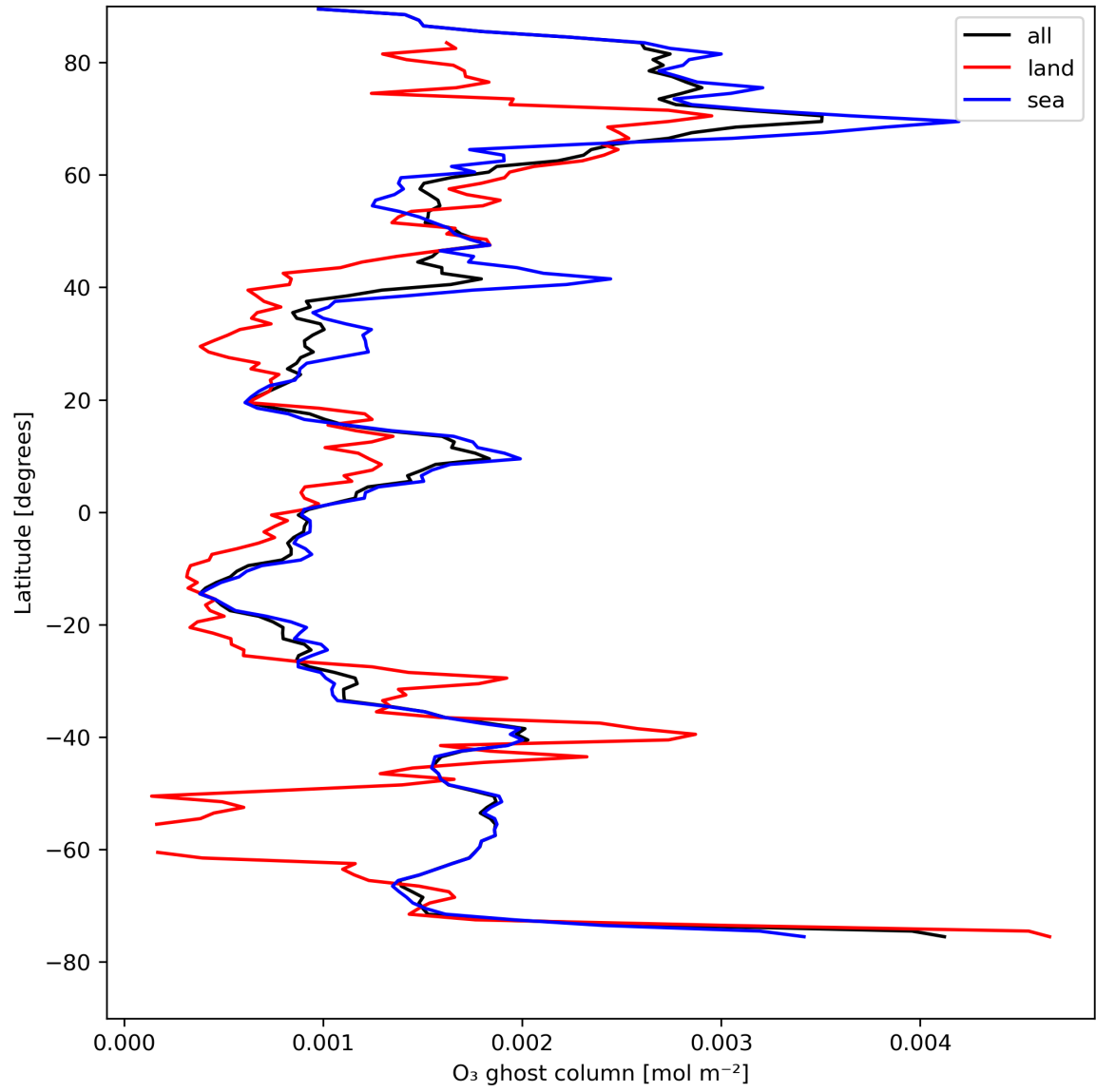
Figure 18: Zonal average of “O 3 ghost column” for 2023-08-15 to 2023-08-17.
