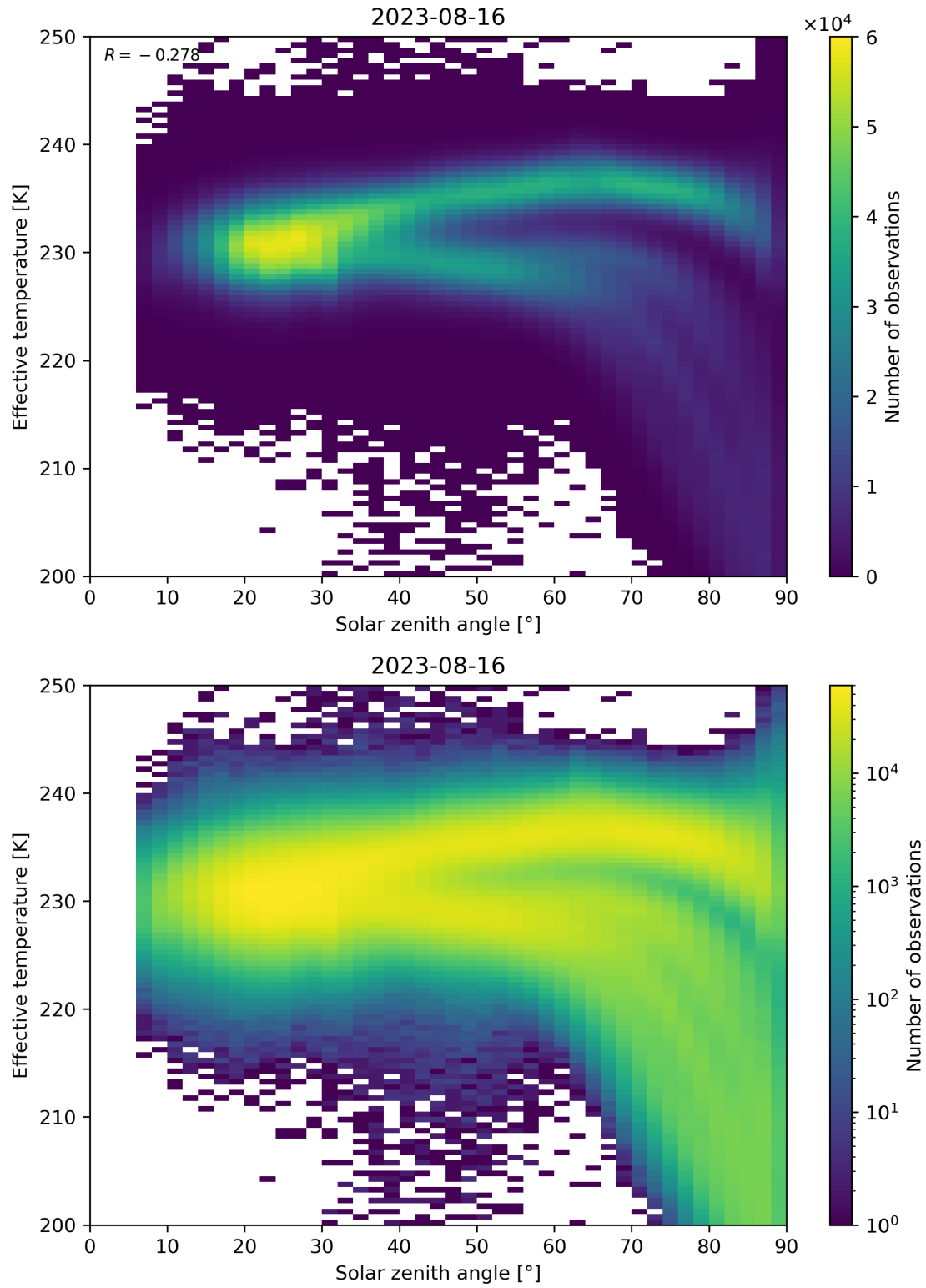
Figure 45: Scatter density plot of “Solar zenith angle” against “Effective temperature” for 2023-08-15 to 2023-08-17.
