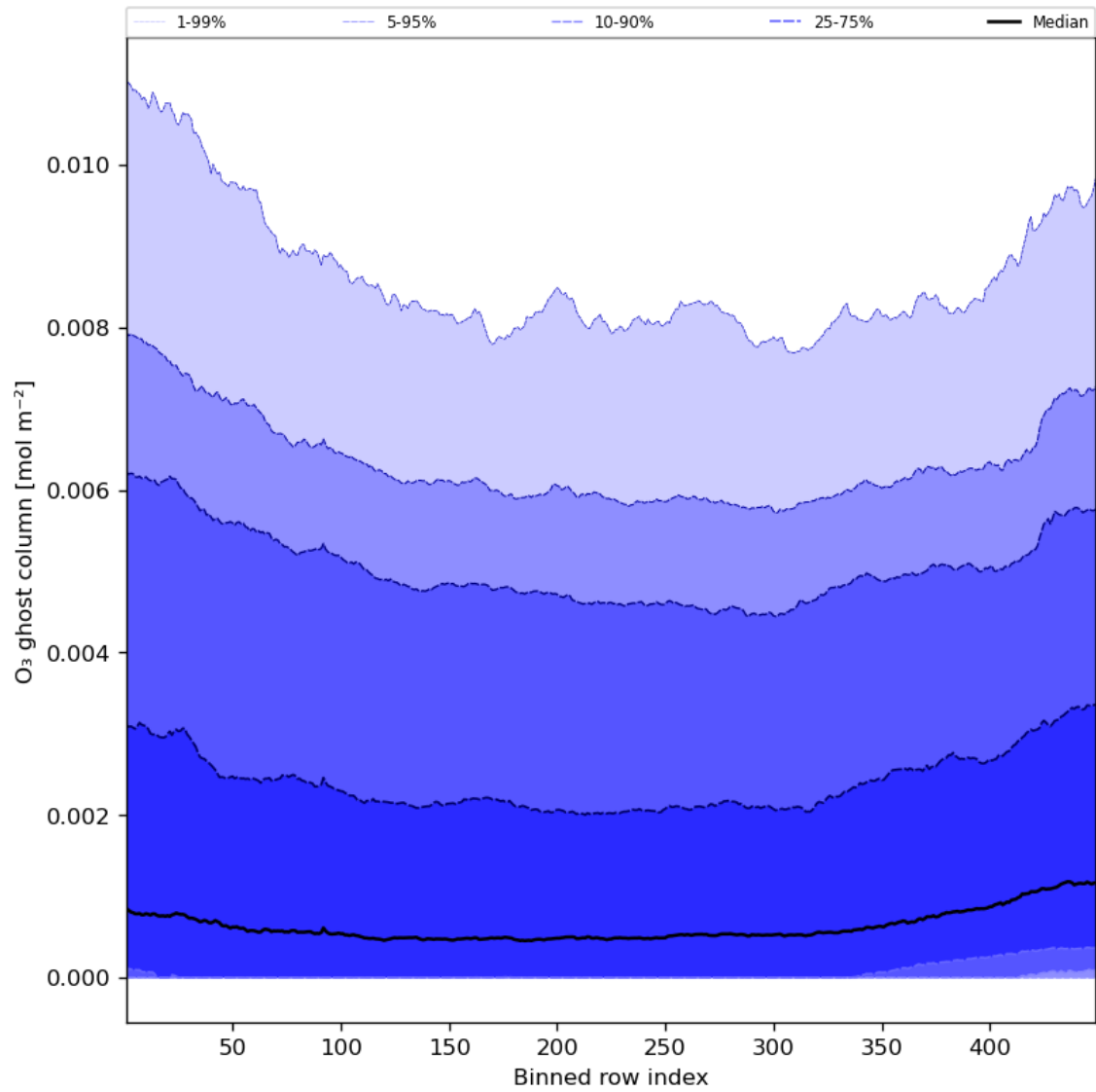
Figure 32: Along track statistics of “O 3 ghost column” for 2023-08-15 to 2023-08-17
