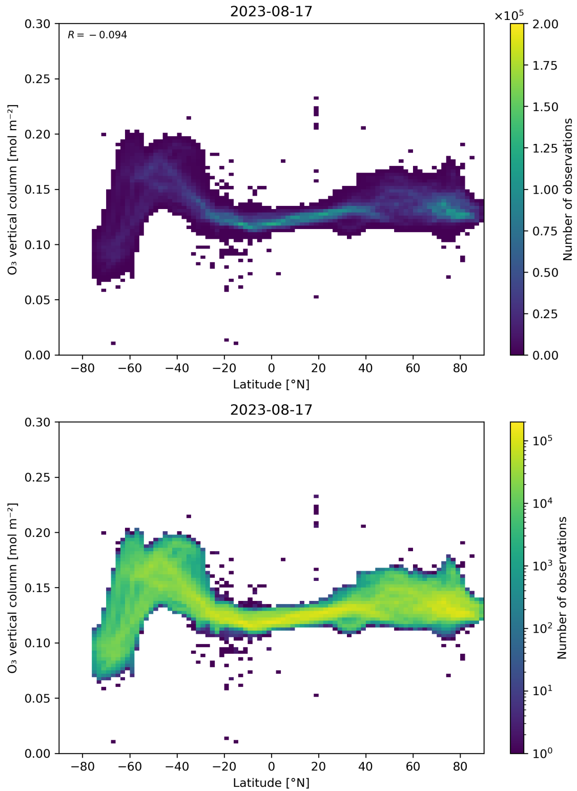
Figure 36: Scatter density plot of “Latitude” against “O 3 vertical column” for 2023-08-16 to 2023-08-18.
