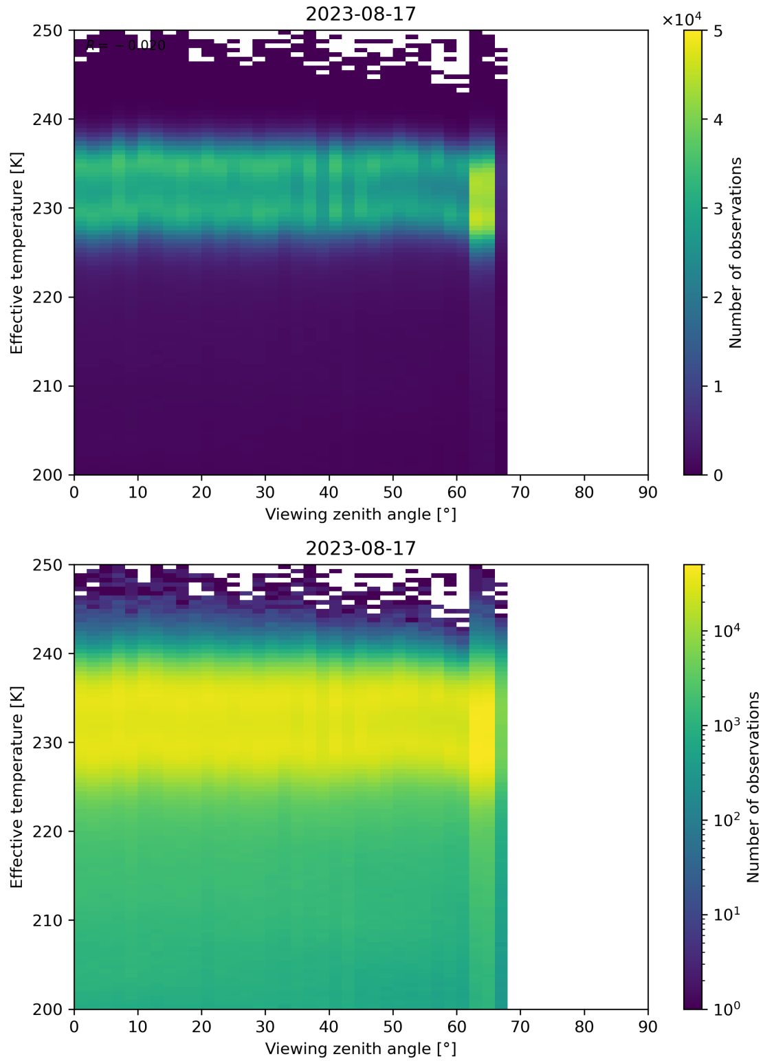
Figure 50: Scatter density plot of “Viewing zenith angle” against “Effective temperature” for 2023-08-16 to 2023-08-18.
