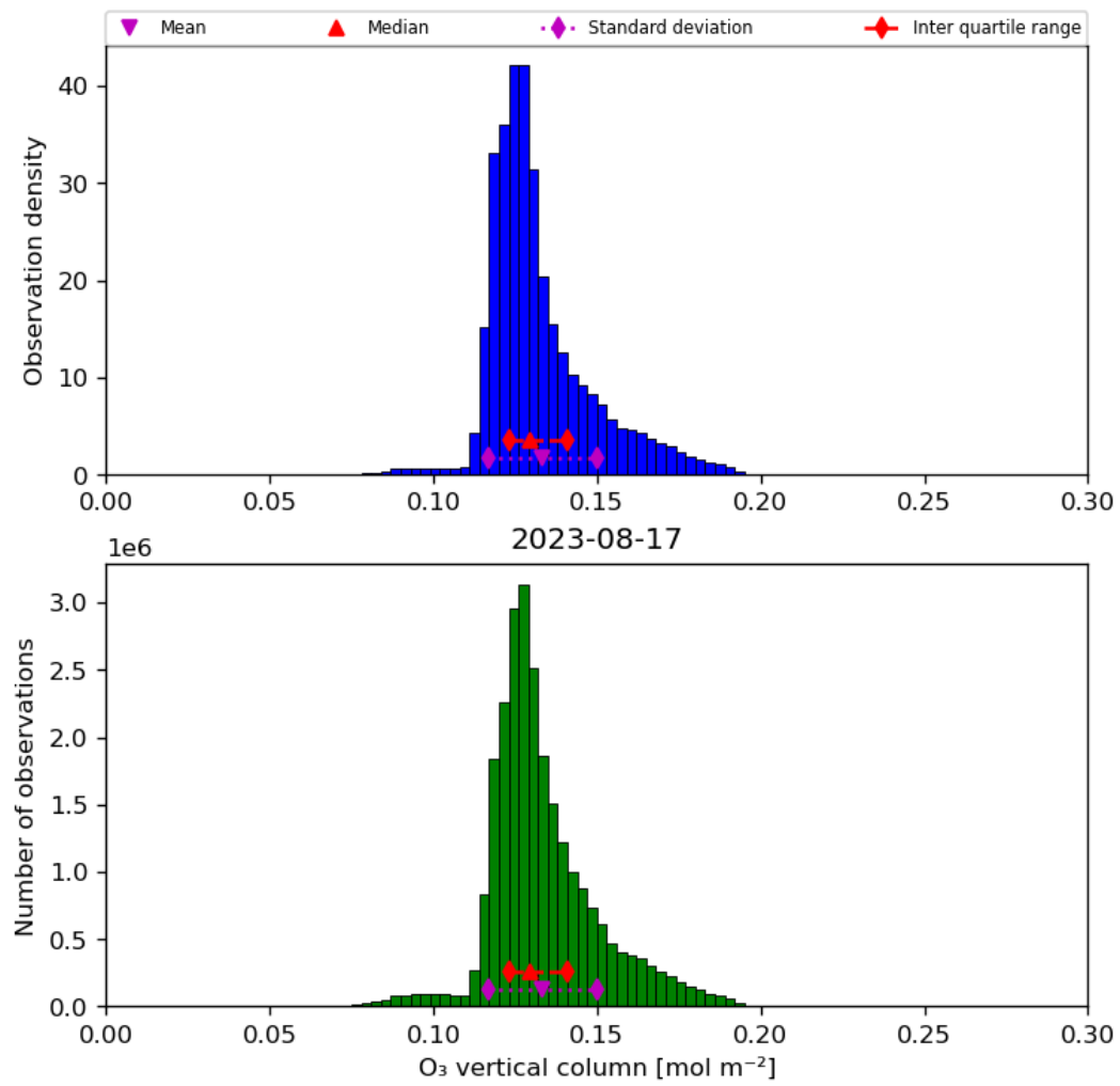
Figure 21: Histogram of “O 3 vertical column” for 2023-08-16 to 2023-08-18
