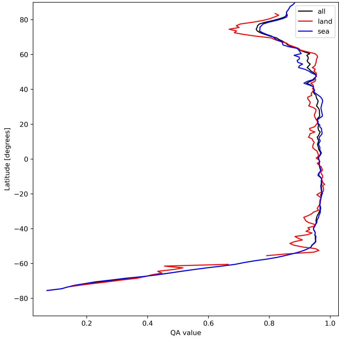
Figure 13: Zonal average of “QA value” for 2023-08-16 to 2023-08-18.
