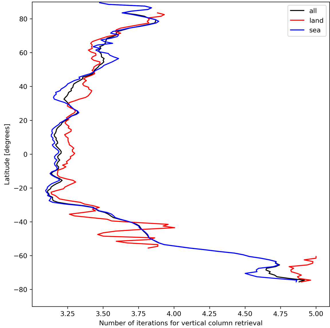
Figure 19: Zonal average of “Number of iterations for vertical column retrieval” for 2023-08-16 to 2023-08-18.
