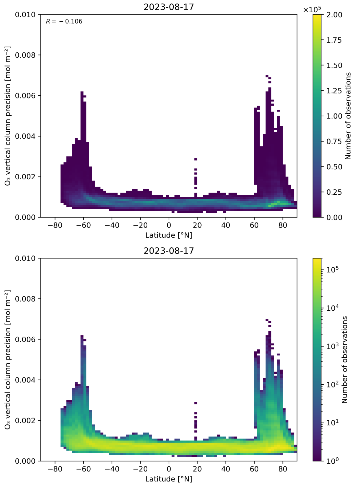
Figure 37: Scatter density plot of “Latitude” against “O 3 vertical column precision” for 2023-08-16 to 2023-08-18.
