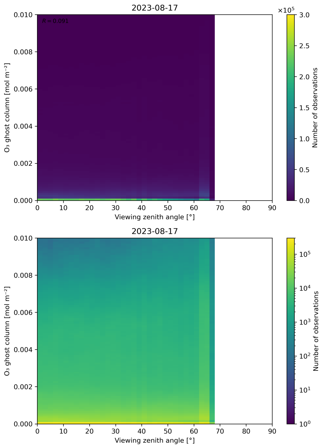
Figure 51: Scatter density plot of “Viewing zenith angle” against “O 3 ghost column” for 2023-08-16 to 2023-08-18.
