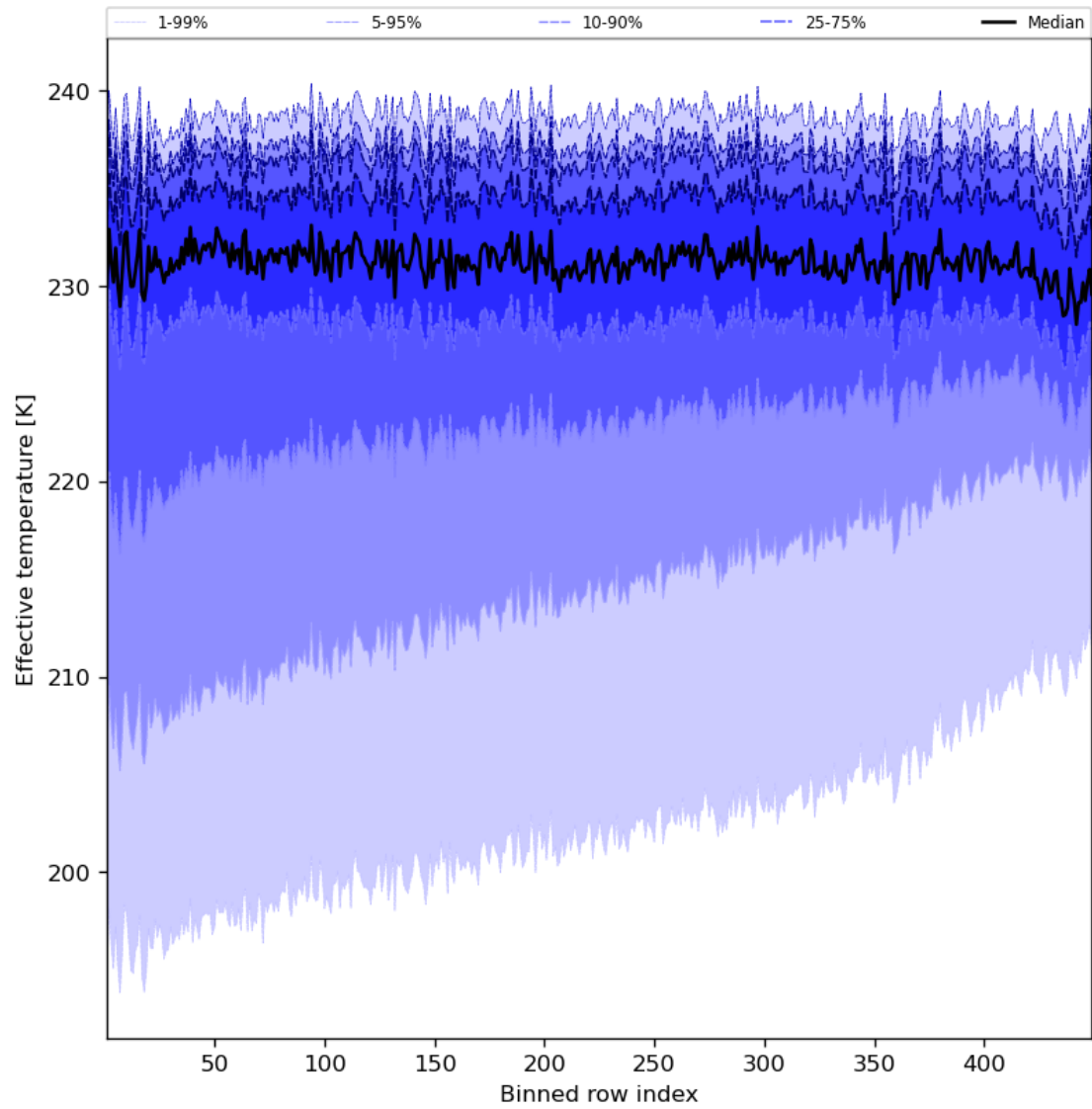
Figure 31: Along track statistics of “Effective temperature” for 2023-08-16 to 2023-08-18
