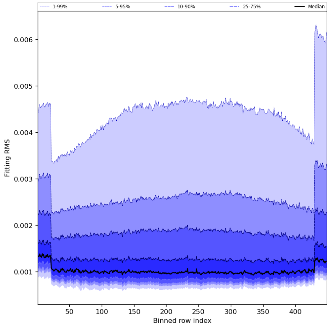
Figure 30: Along track statistics of “Fitting RMS” for 2023-08-16 to 2023-08-18
