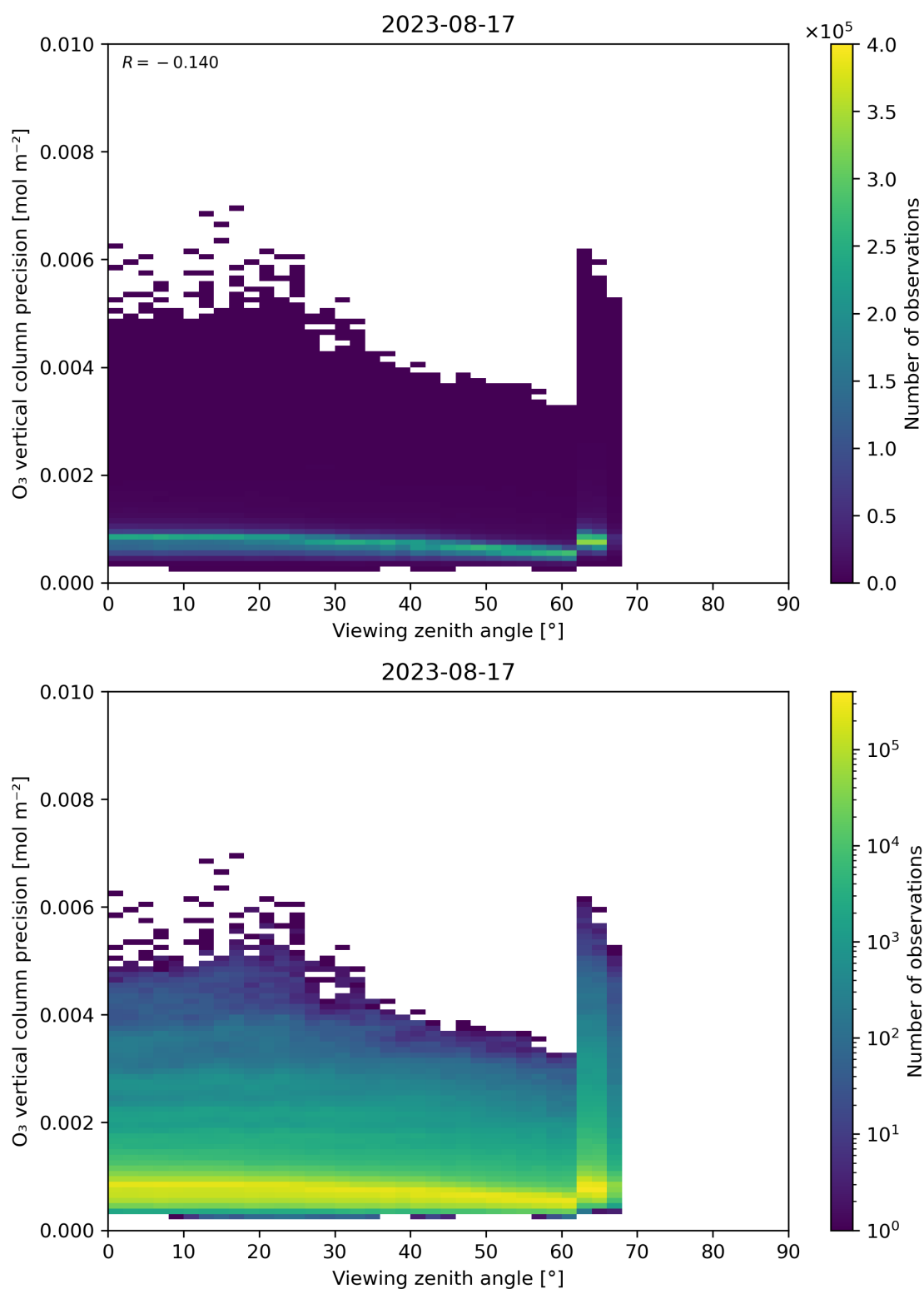
Figure 53: Scatter density plot of “Viewing zenith angle” against “O 3 vertical column precision” for 2023-08-16 to 2023-08-18.
