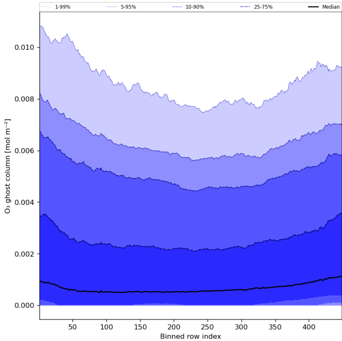
Figure 32: Along track statistics of “O 3 ghost column” for 2023-08-16 to 2023-08-18
