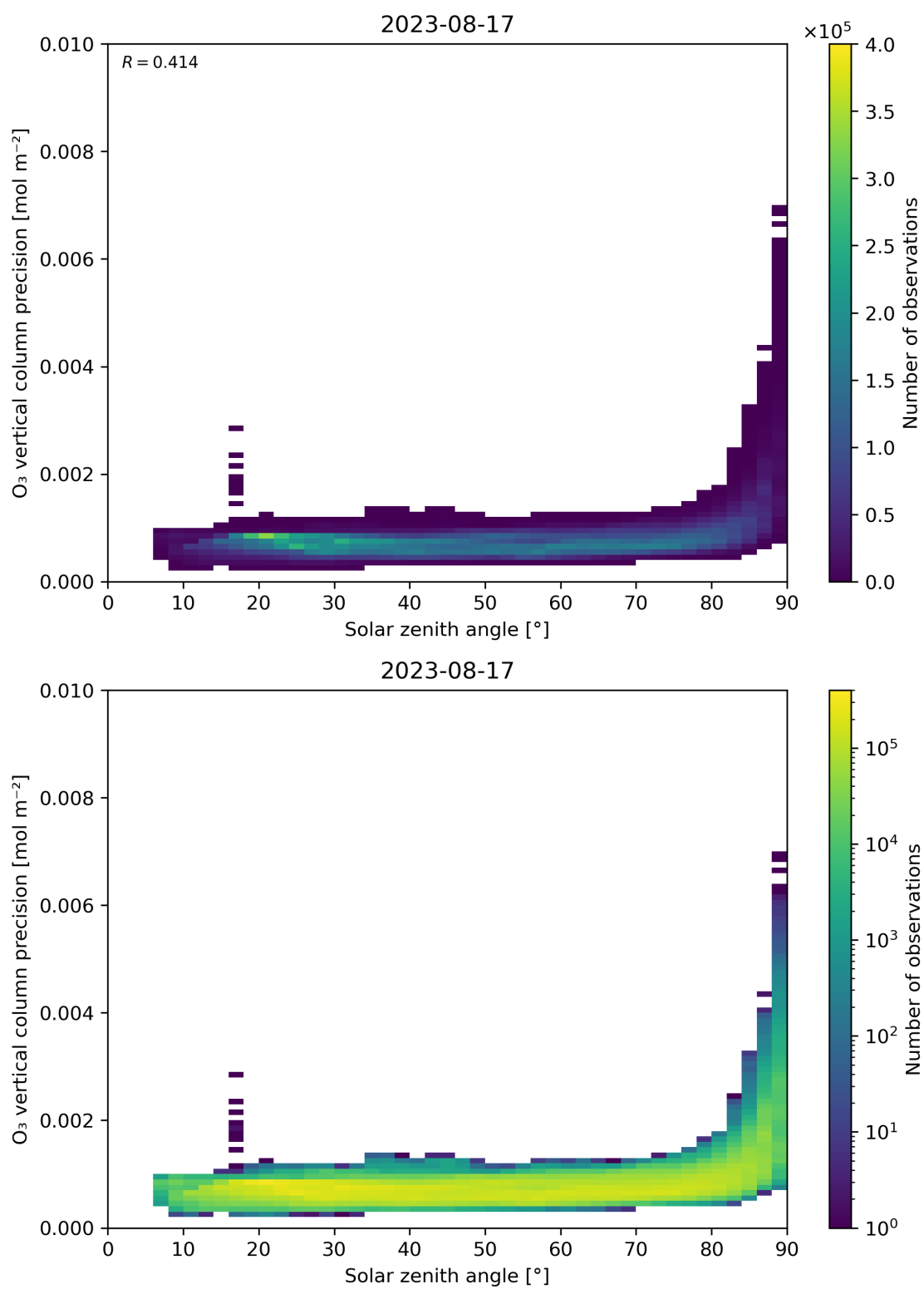
Figure 48: Scatter density plot of “Solar zenith angle” against “O 3 vertical column precision” for 2023-08-16 to 2023-08-18.
