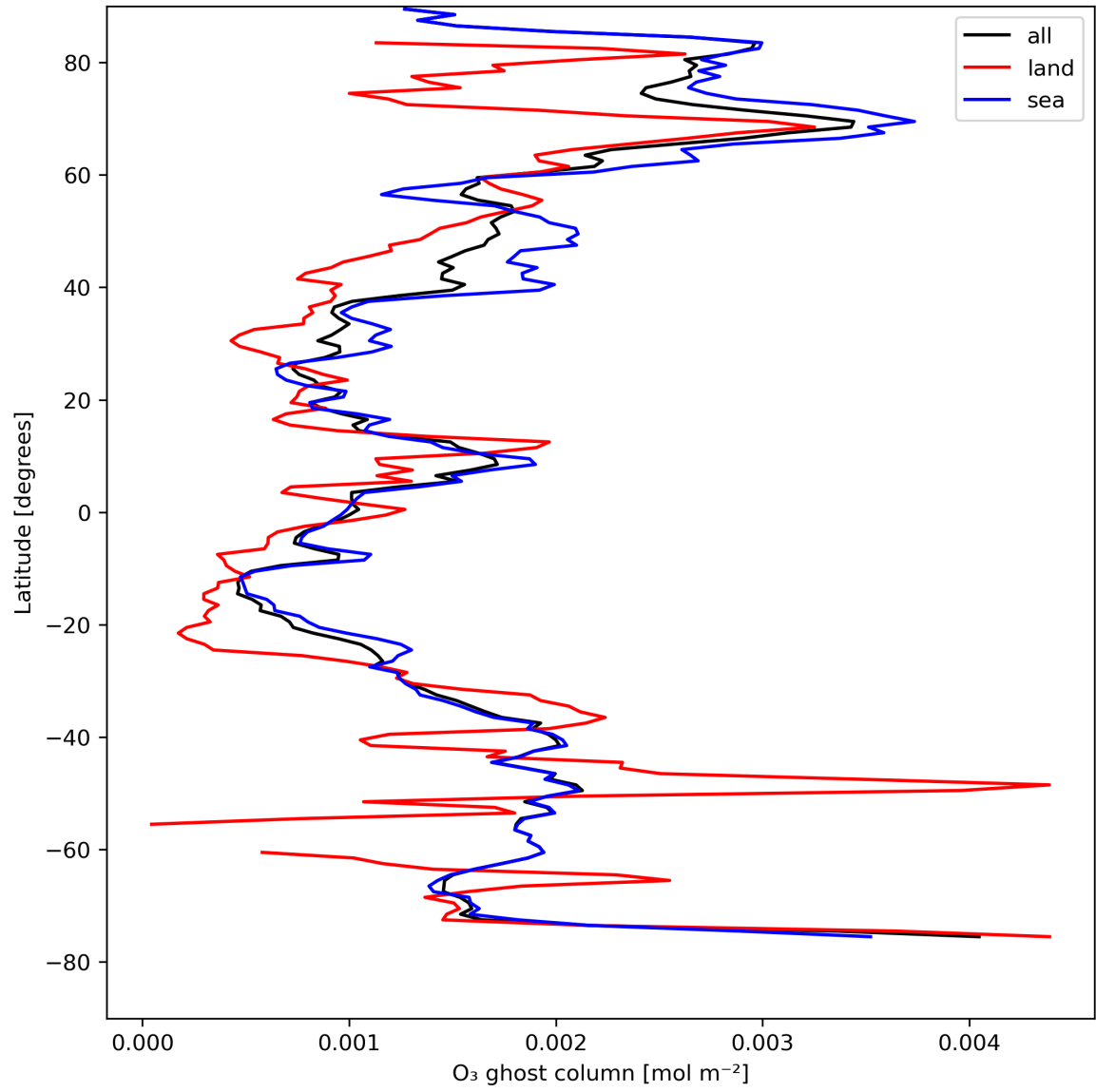
Figure 18: Zonal average of "O 3 ghost column" for 2023-08-16 to 2023-08-18.
