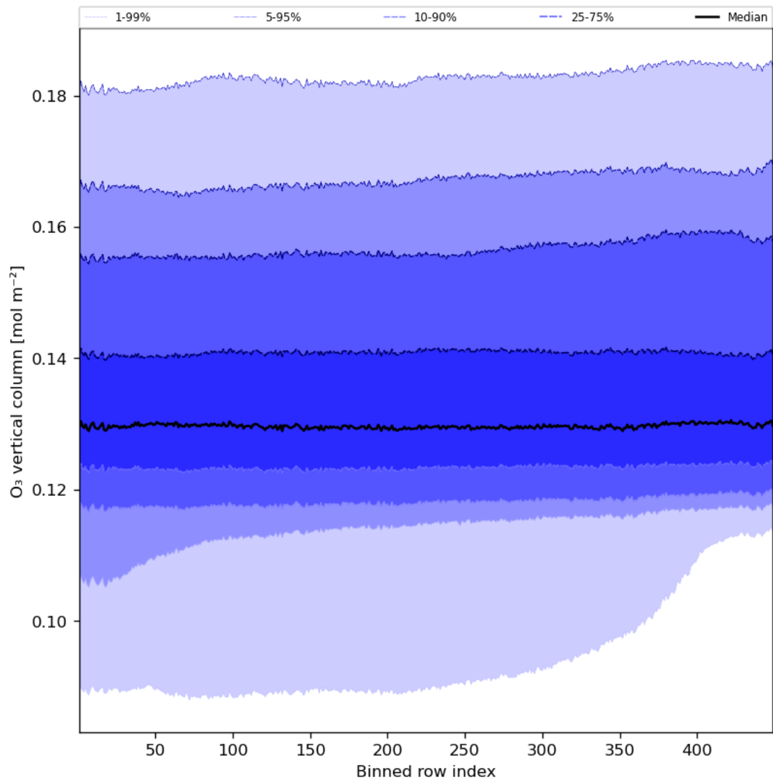
Figure 28: Along track statistics of “O 3 vertical column” for 2023-08-16 to 2023-08-18
