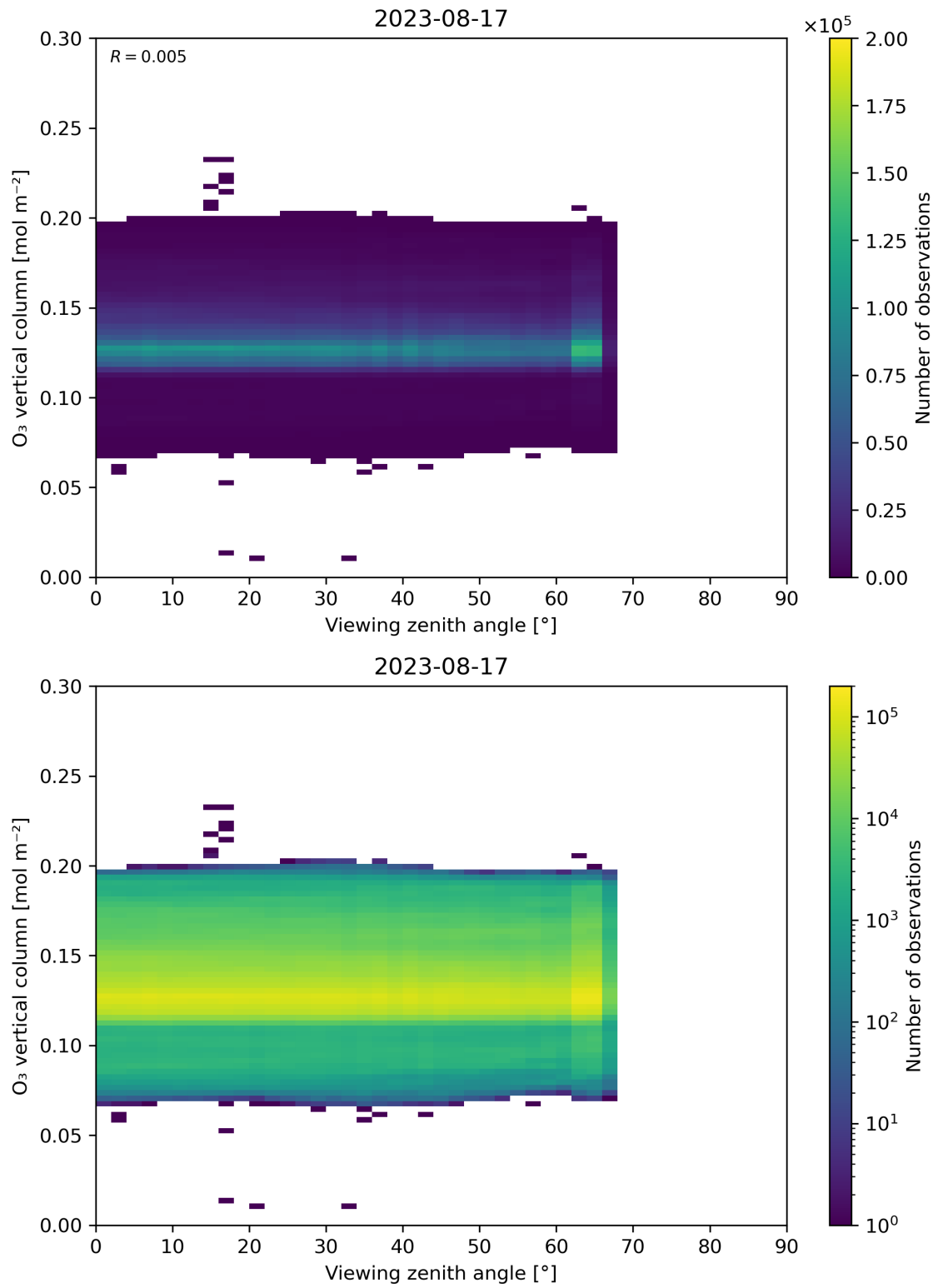
Figure 52: Scatter density plot of “Viewing zenith angle” against “O 3 vertical column” for 2023-08-16 to 2023-08-18.
