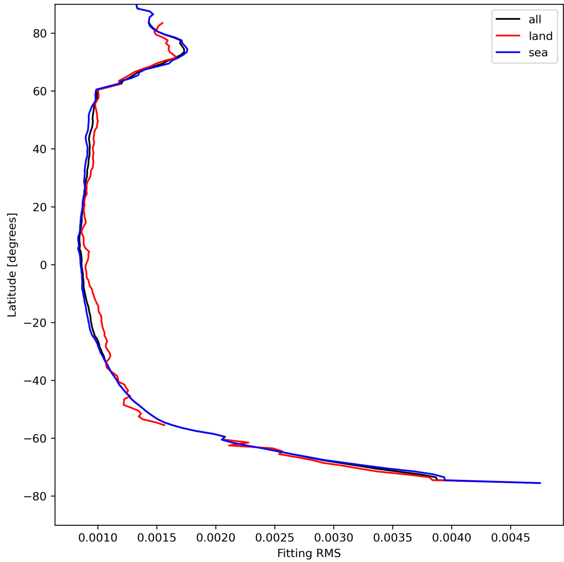
Figure 16: Zonal average of “Fitting RMS” for 2023-08-16 to 2023-08-18.
