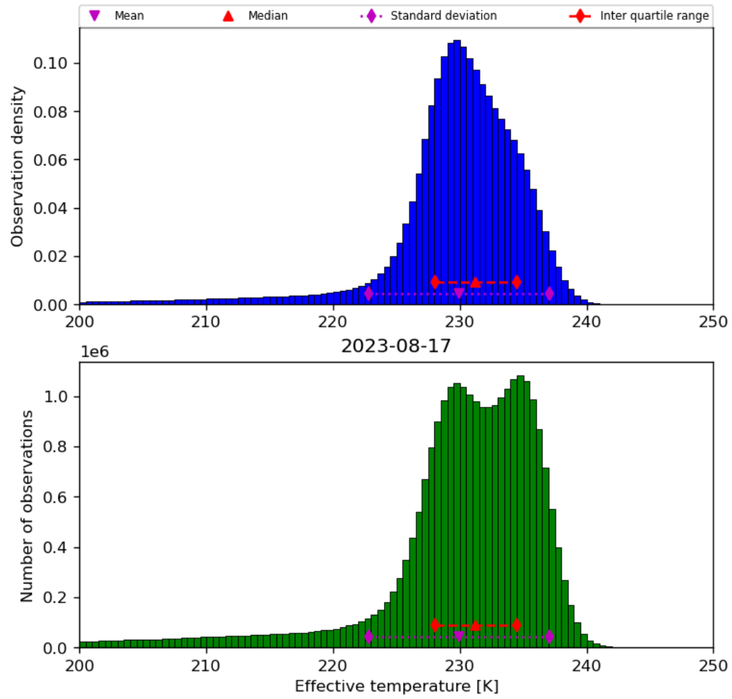
Figure 24: Histogram of “Effective temperature” for 2023-08-16 to 2023-08-18
