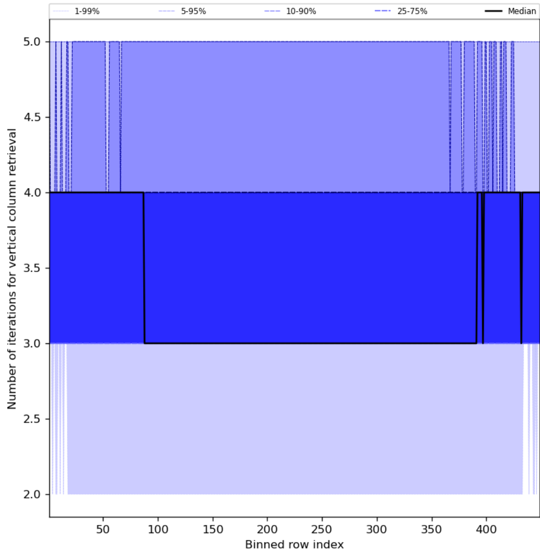
Figure 33: Along track statistics of “Number of iterations for vertical column retrieval” for 2023-08-16 to 2023-08-18
