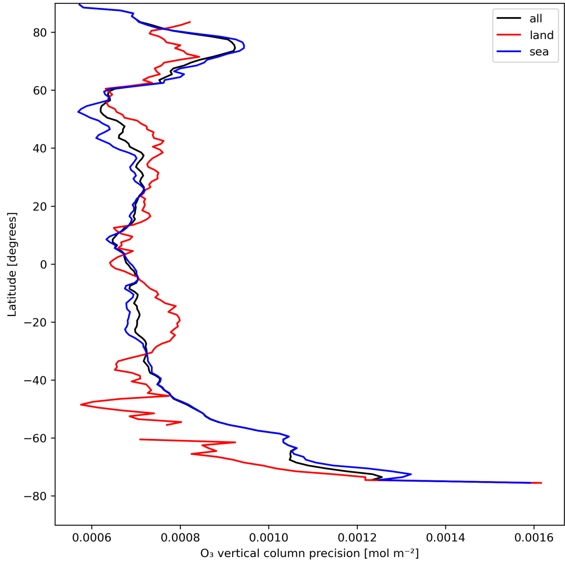
Figure 15: Zonal average of “O 3 vertical column precision” for 2023-08-16 to 2023-08-18.
