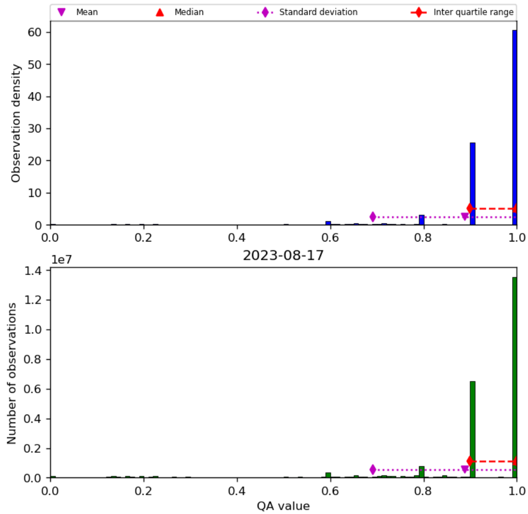
Figure 20: Histogram of “QA value” for 2023-08-16 to 2023-08-18
