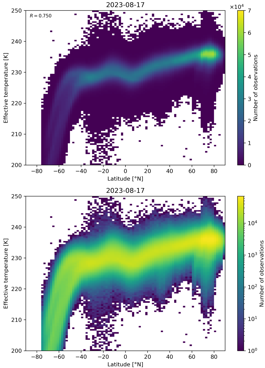
Figure 34: Scatter density plot of “Latitude” against “Effective temperature” for 2023-08-16 to 2023-08-18.
