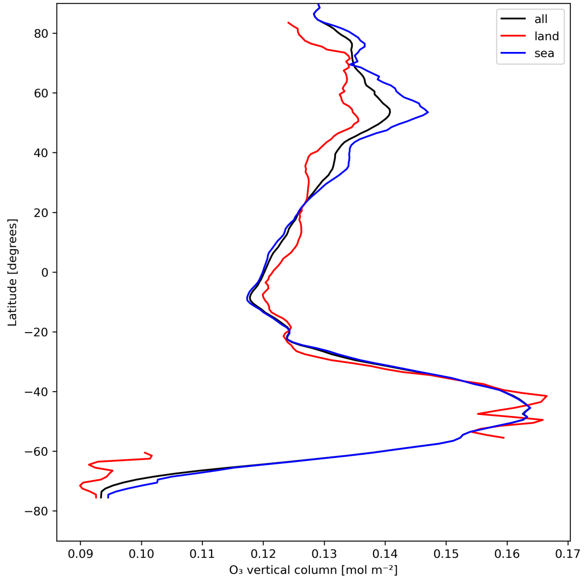
Figure 14: Zonal average of “O 3 vertical column” for 2023-08-16 to 2023-08-18.
