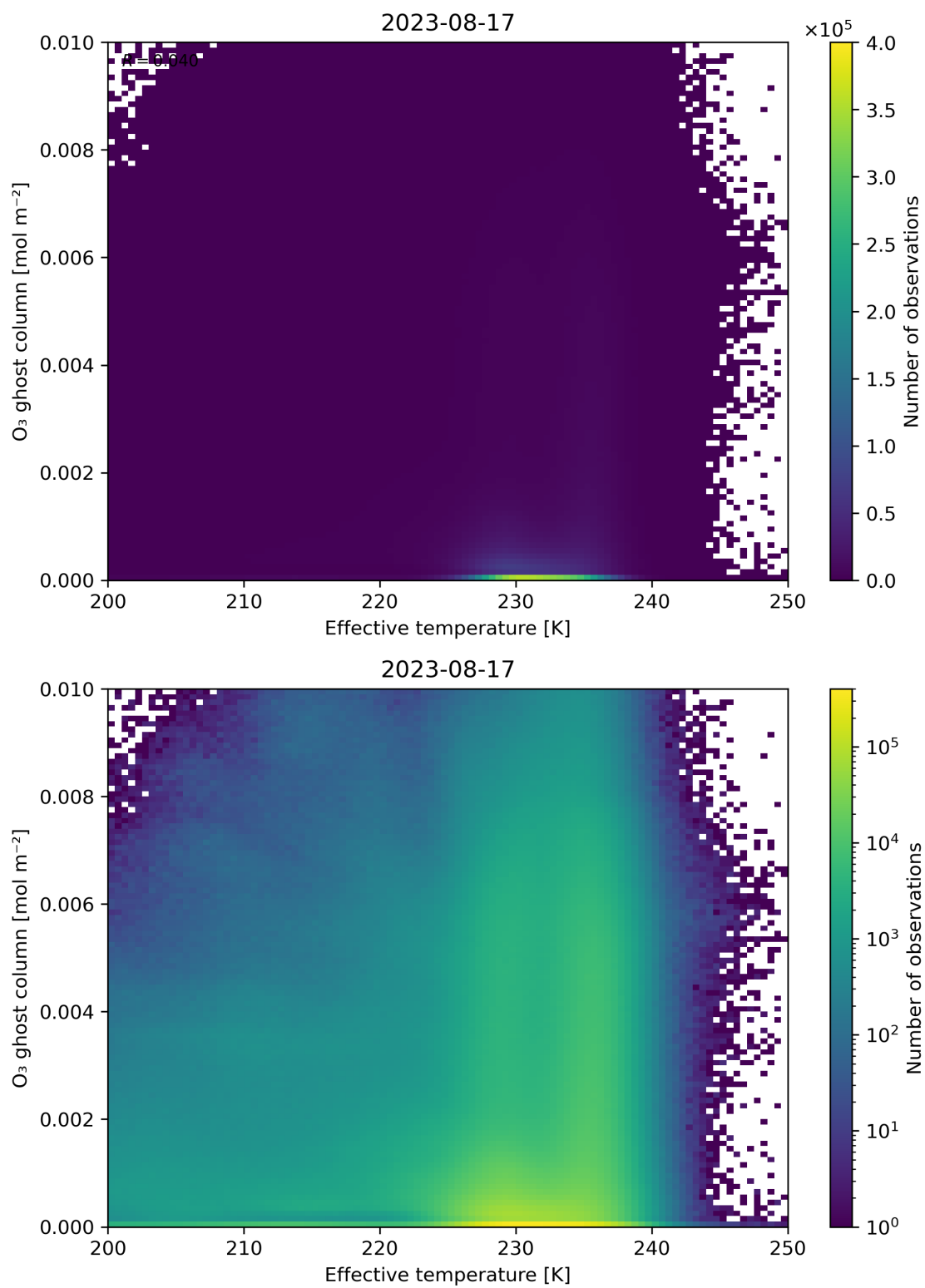
Figure 38: Scatter density plot of “Effective temperature” against “O 3 ghost column” for 2023-08-16 to 2023-08-18.
