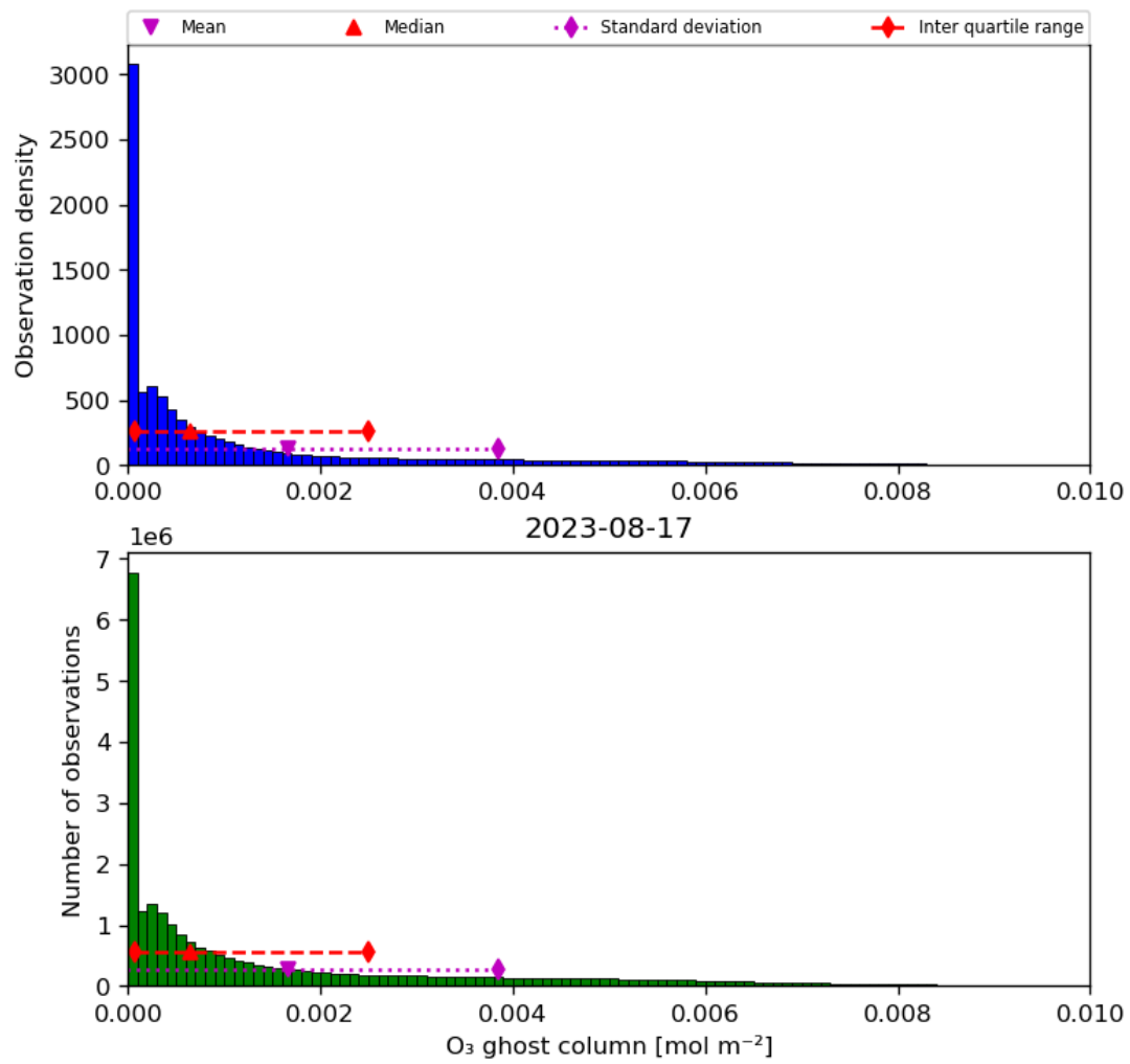
Figure 25: Histogram of “O 3 ghost column” for 2023-08-16 to 2023-08-18
