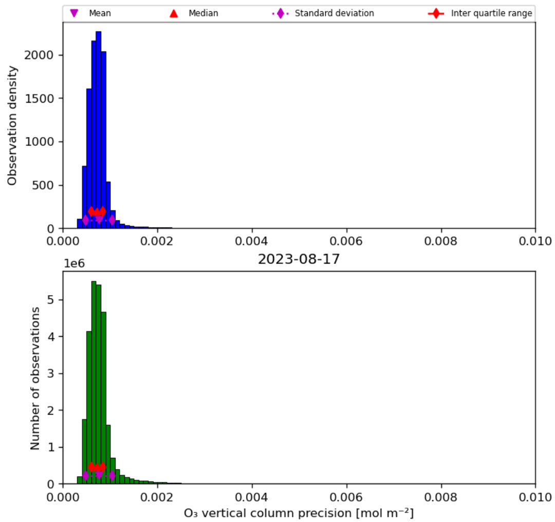
Figure 22: Histogram of “O 3 vertical column precision” for 2023-08-16 to 2023-08-18
