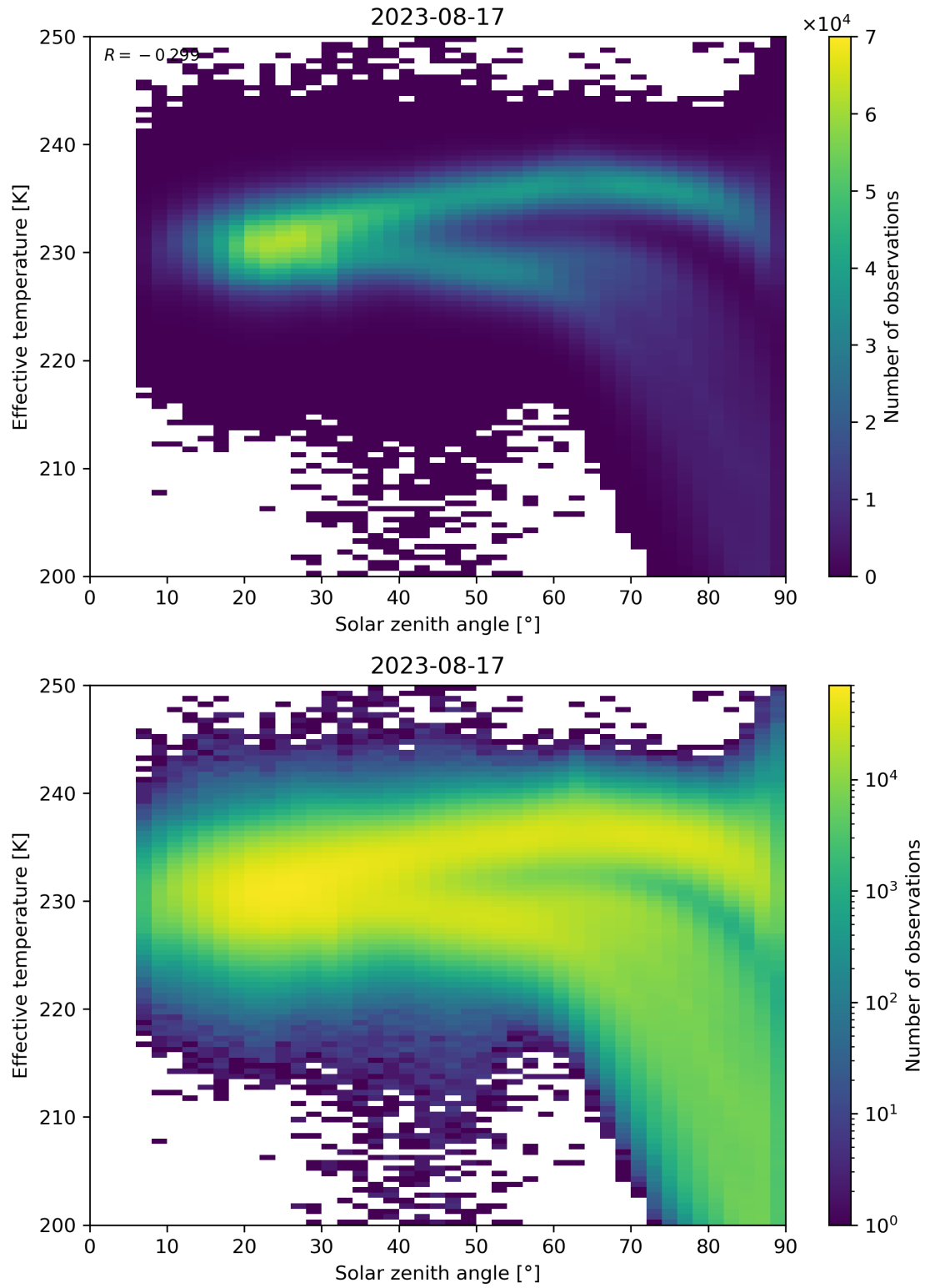
Figure 45: Scatter density plot of “Solar zenith angle” against “Effective temperature” for 2023-08-16 to 2023-08-18.
