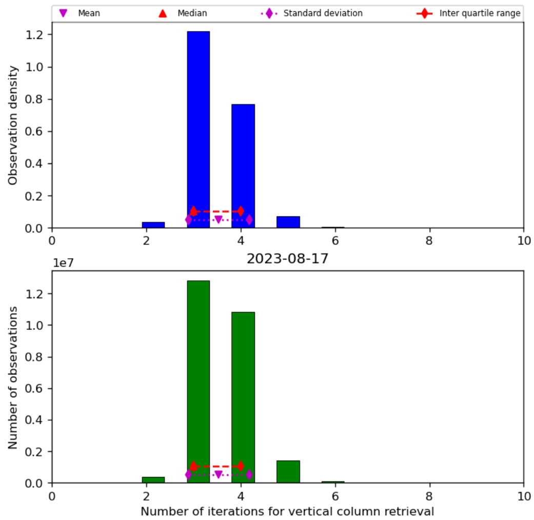
Figure 26: Histogram of “Number of iterations for vertical column retrieval” for 2023-08-16 to 2023-08-18
