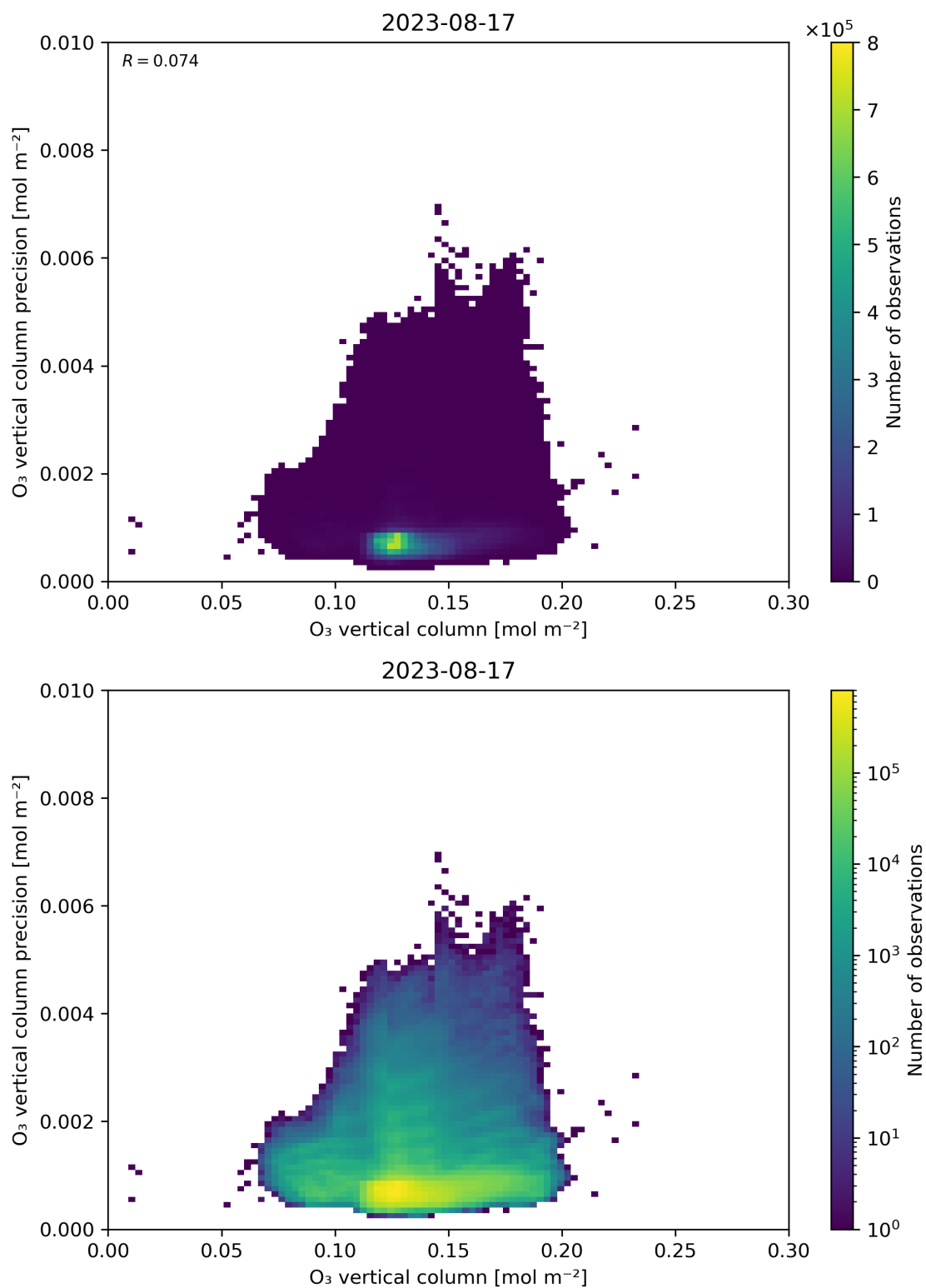
Figure 41: Scatter density plot of “O 3 vertical column” against “O 3 vertical column precision” for 2023-08-16 to 2023-08-18.
