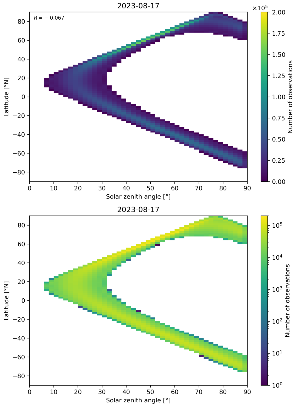
Figure 44: Scatter density plot of “Solar zenith angle” against “Latitude” for 2023-08-16 to 2023-08-18.
