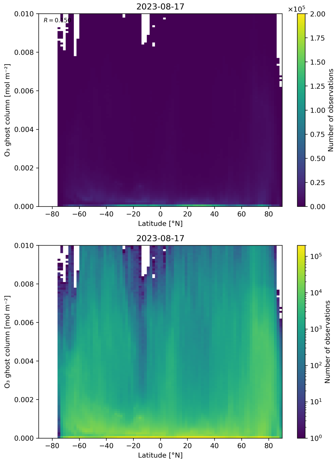
Figure 35: Scatter density plot of “Latitude” against “O 3 ghost column” for 2023-08-16 to 2023-08-18.
