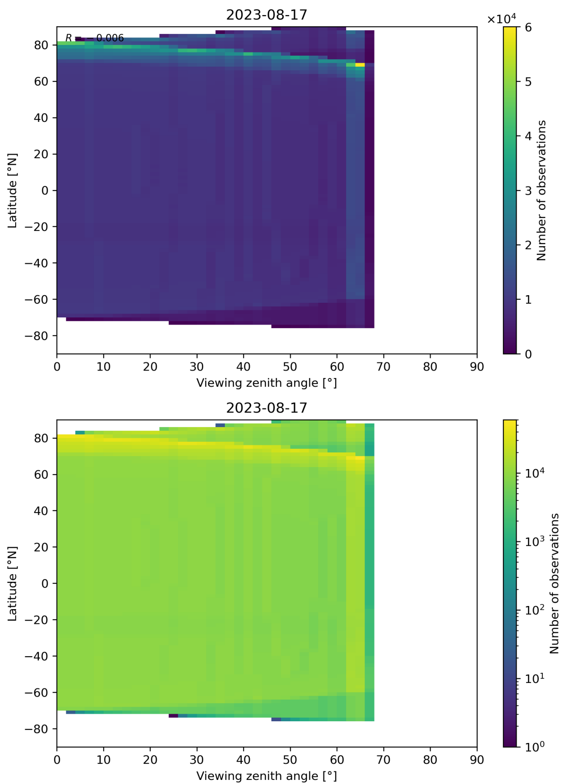
Figure 49: Scatter density plot of “Viewing zenith angle” against “Latitude” for 2023-08-16 to 2023-08-18.
