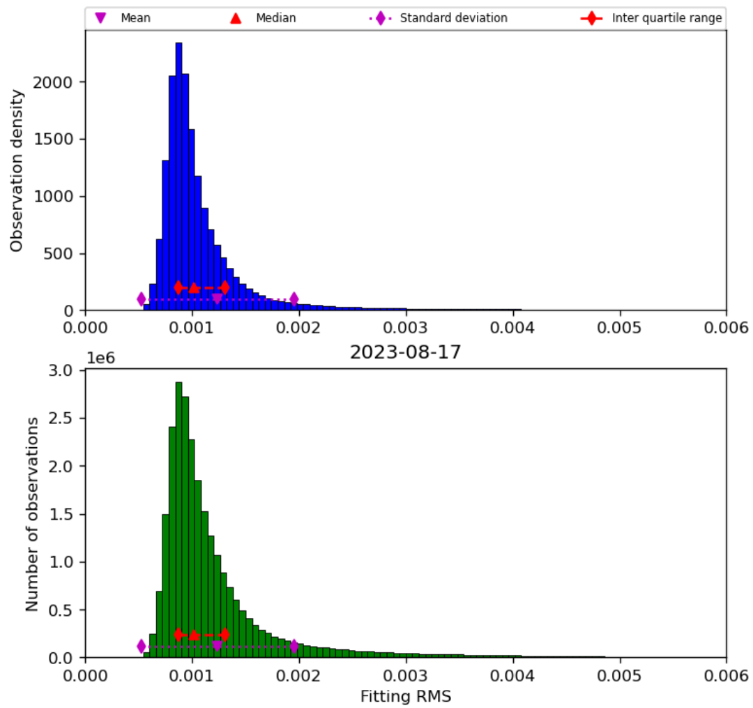
Figure 23: Histogram of “Fitting RMS” for 2023-08-16 to 2023-08-18
