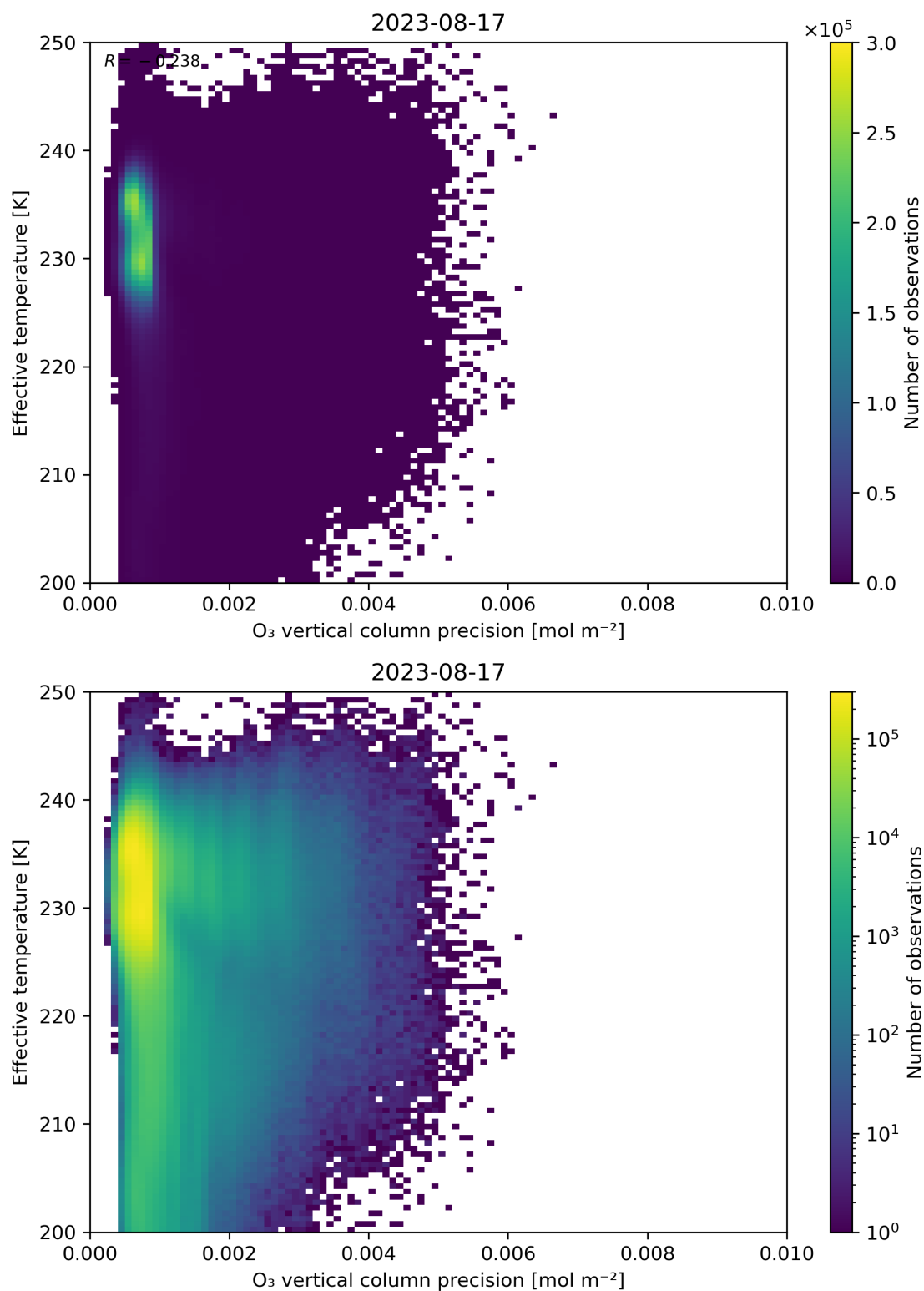
Figure 42: Scatter density plot of “O 3 vertical column precision” against “Effective temperature” for 2023-08-16 to 2023-08-18.
