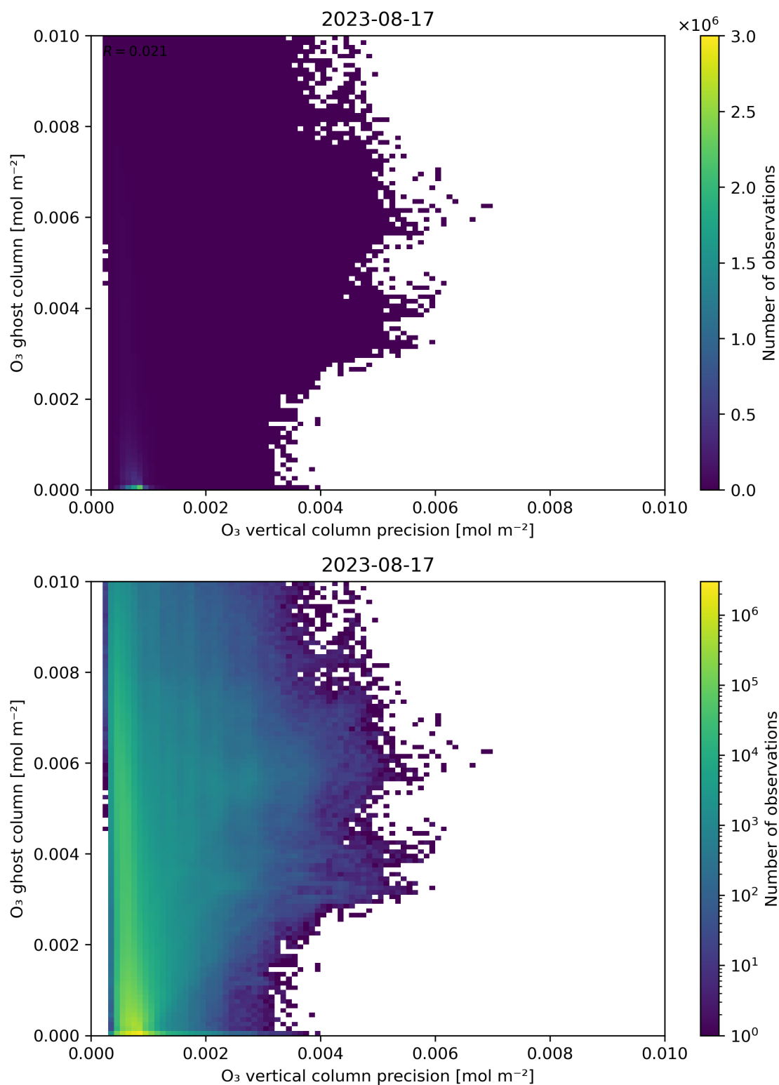
Figure 43: Scatter density plot of “ \text{O}_3 vertical column precision” against “ \text{O}_3 ghost column” for 2023-08-16 to 2023-08-18.
