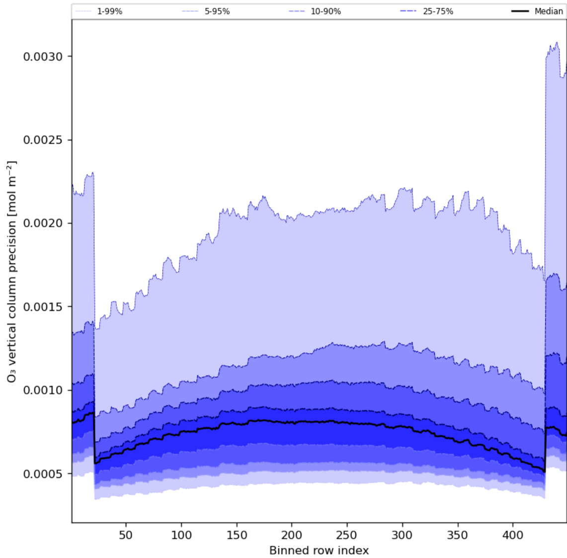
Figure 29: Along track statistics of “O 3 vertical column precision” for 2023-08-16 to 2023-08-18
