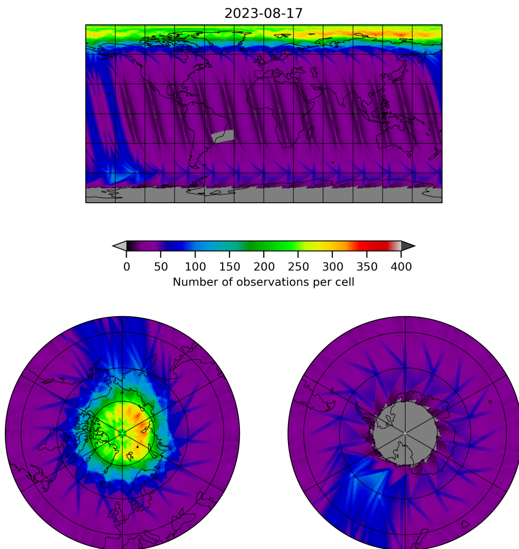
Figure 12: Map of the number of observations for 2023-08-16 to 2023-08-18
