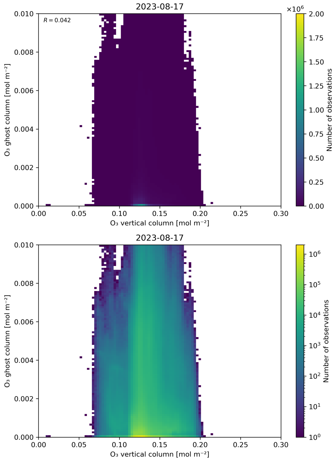
Figure 40: Scatter density plot of “O 3 vertical column” against “O 3 ghost column” for 2023-08-16 to 2023-08-18.
