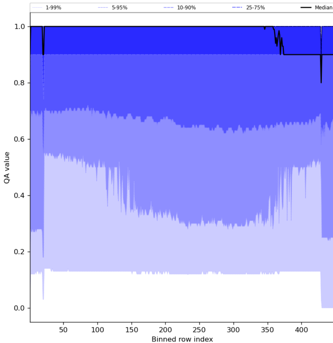
Figure 27: Along track statistics of “QA value” for 2023-08-16 to 2023-08-18
