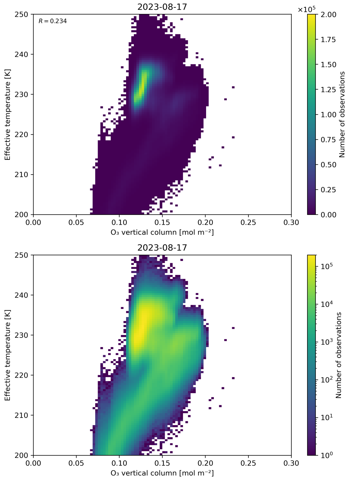
Figure 39: Scatter density plot of “O 3 vertical column” against “Effective temperature” for 2023-08-16 to 2023-08-18.
