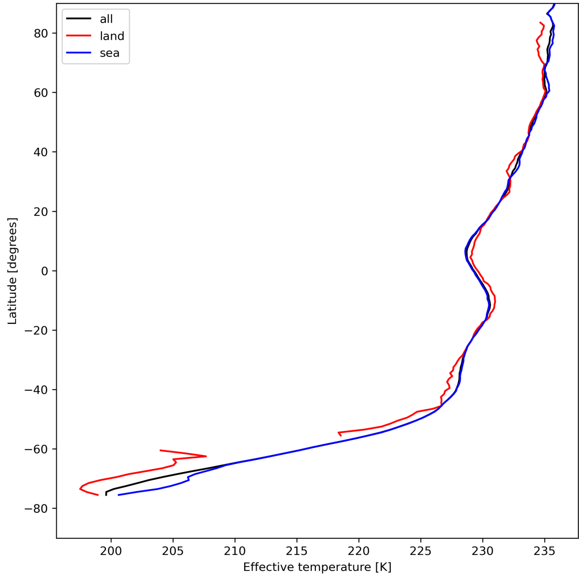
Figure 17: Zonal average of “Effective temperature” for 2023-08-16 to 2023-08-18.
