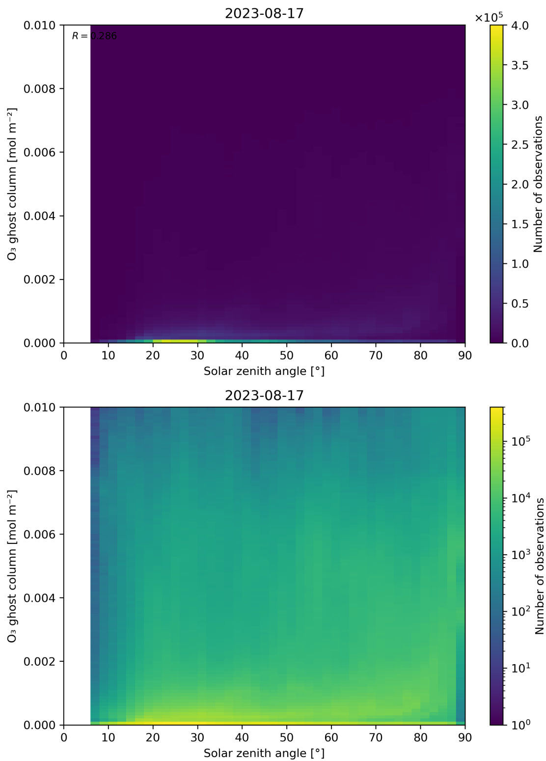
Figure 46: Scatter density plot of “Solar zenith angle” against “O 3 ghost column” for 2023-08-16 to 2023-08-18.
