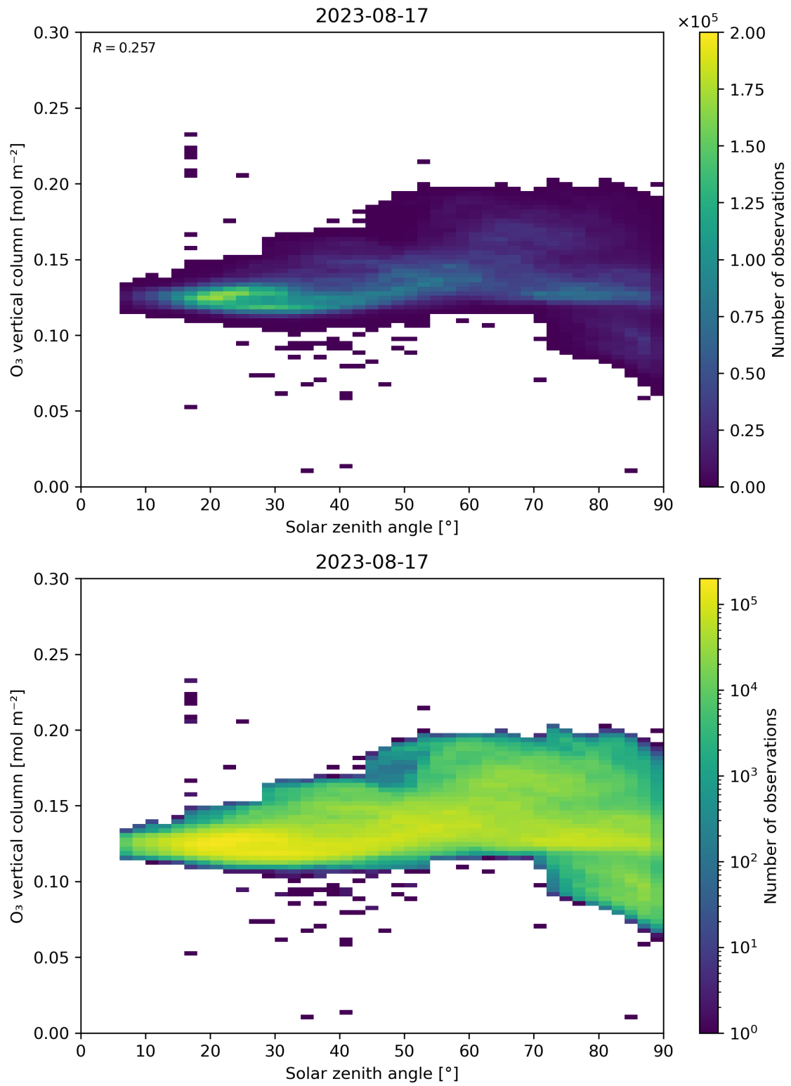
Figure 47: Scatter density plot of “Solar zenith angle” against “O 3 vertical column” for 2023-08-16 to 2023-08-18.
