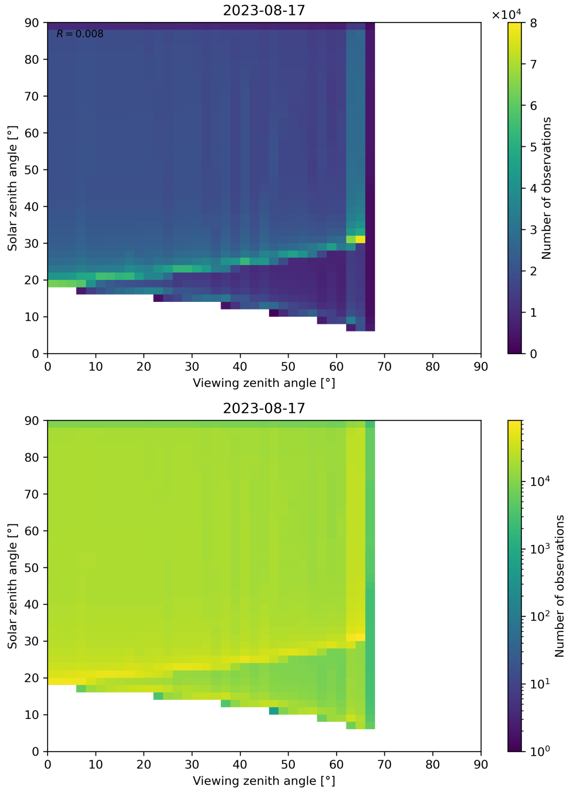
Figure 54: Scatter density plot of “Viewing zenith angle” against “Solar zenith angle” for 2023-08-16 to 2023-08-18.
