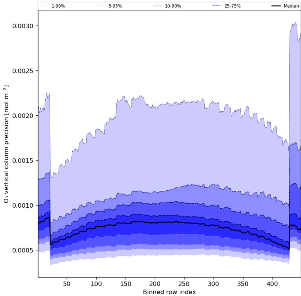
Figure 29: Along track statistics of “O 3 vertical column precision” for 2023-08-17 to 2023-08-19
