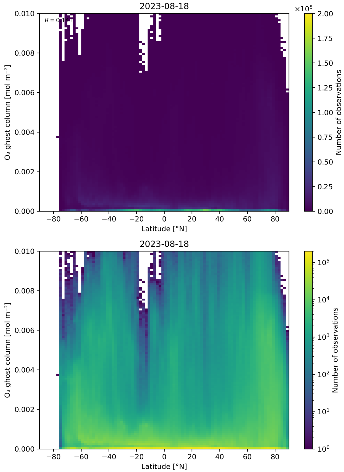
Figure 35: Scatter density plot of “Latitude” against “O 3 ghost column” for 2023-08-17 to 2023-08-19.
