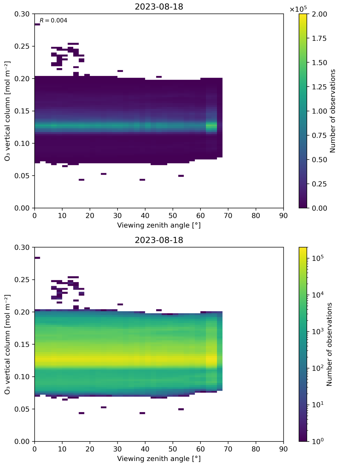
Figure 52: Scatter density plot of “Viewing zenith angle” against “O 3 vertical column” for 2023-08-17 to 2023-08-19.
