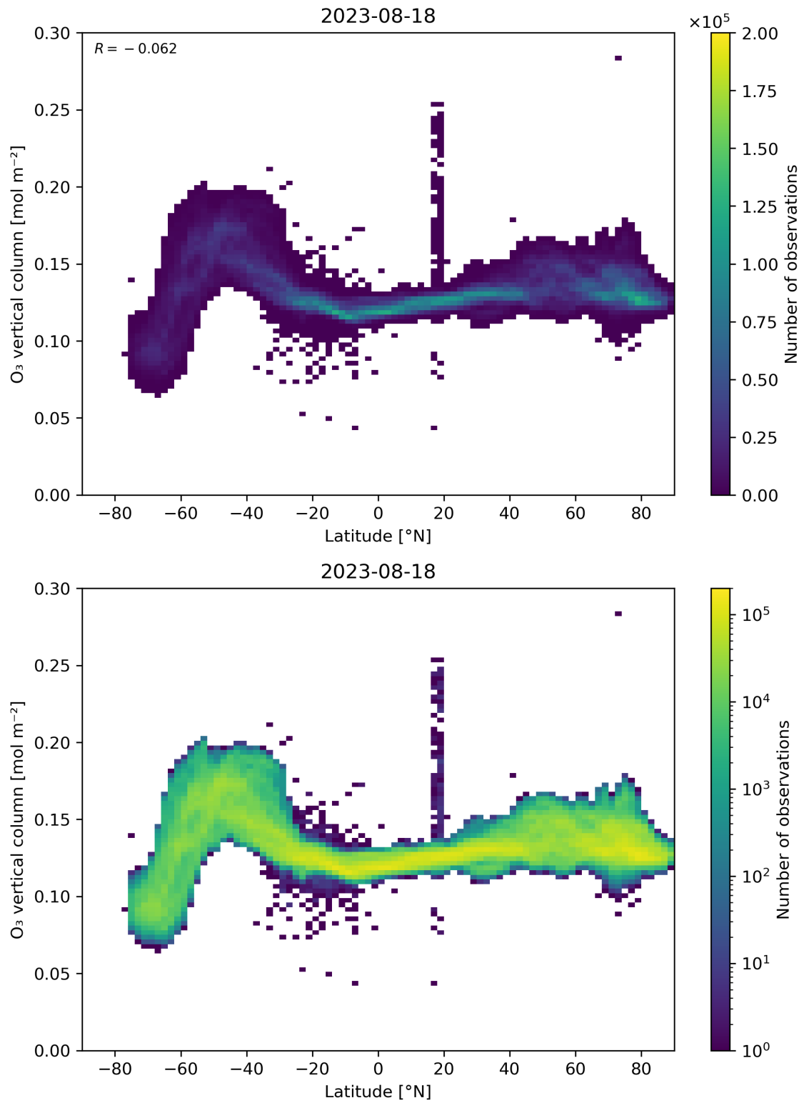
Figure 36: Scatter density plot of “Latitude” against “O 3 vertical column” for 2023-08-17 to 2023-08-19.
