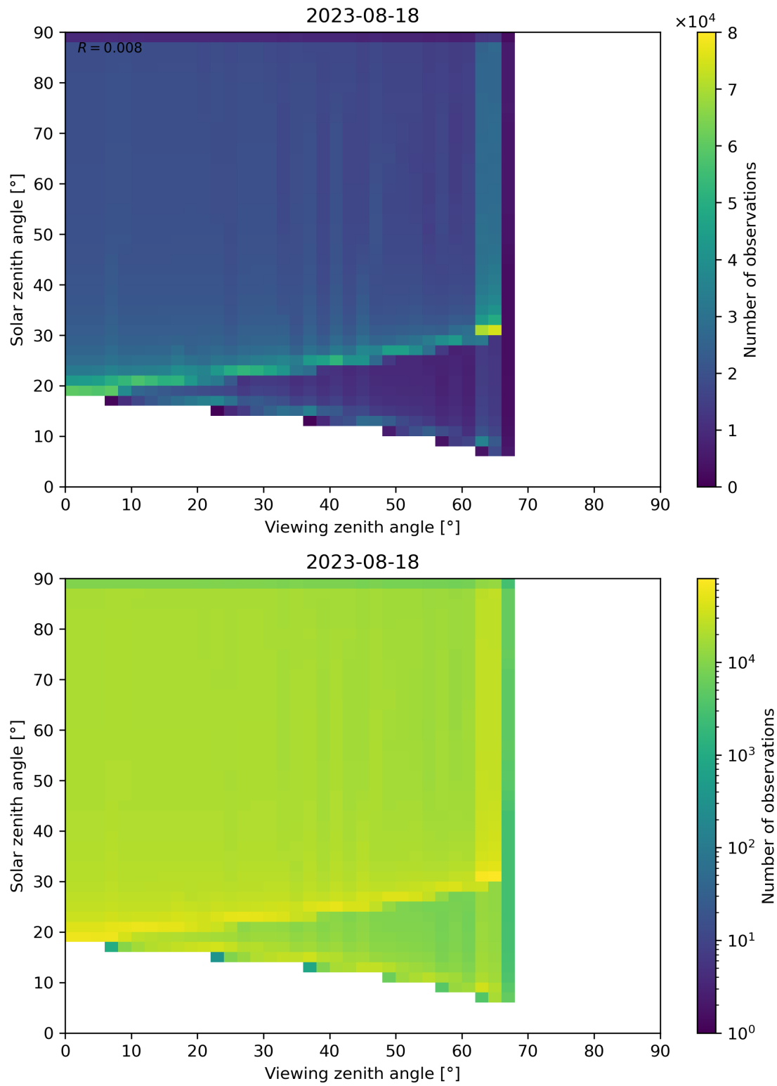
Figure 54: Scatter density plot of “Viewing zenith angle” against “Solar zenith angle” for 2023-08-17 to 2023-08-19.
