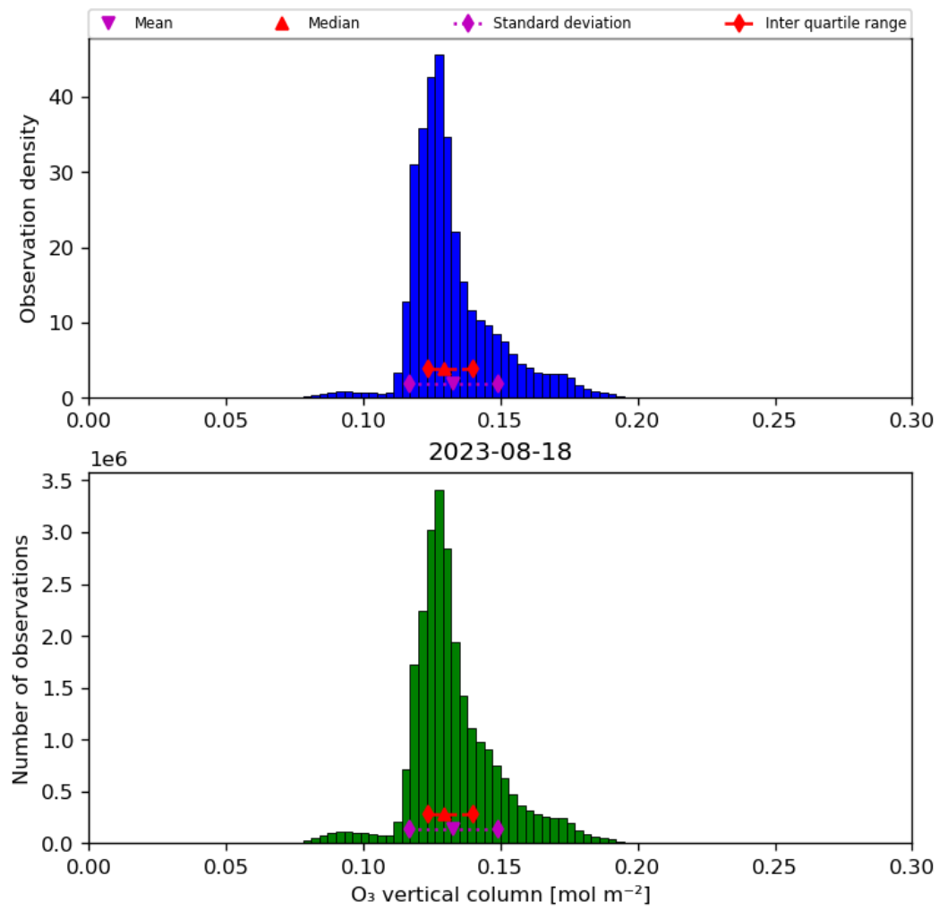
Figure 21: Histogram of “O 3 vertical column” for 2023-08-17 to 2023-08-19
