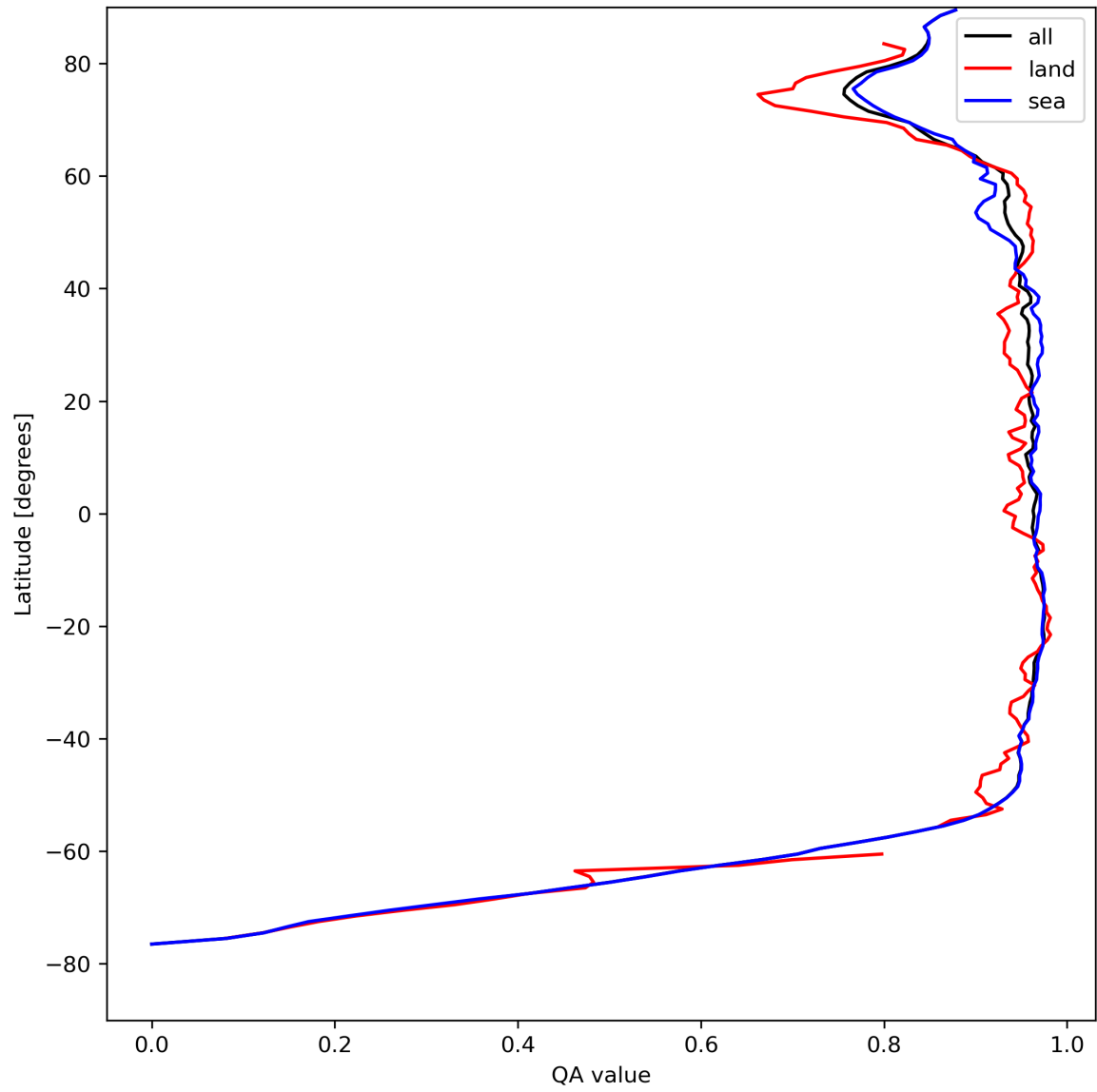
Figure 13: Zonal average of “QA value” for 2023-08-17 to 2023-08-19.
