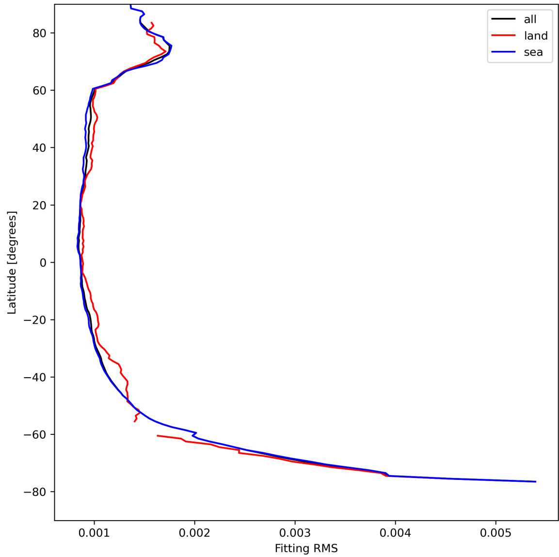
Figure 16: Zonal average of “Fitting RMS” for 2023-08-17 to 2023-08-19.
