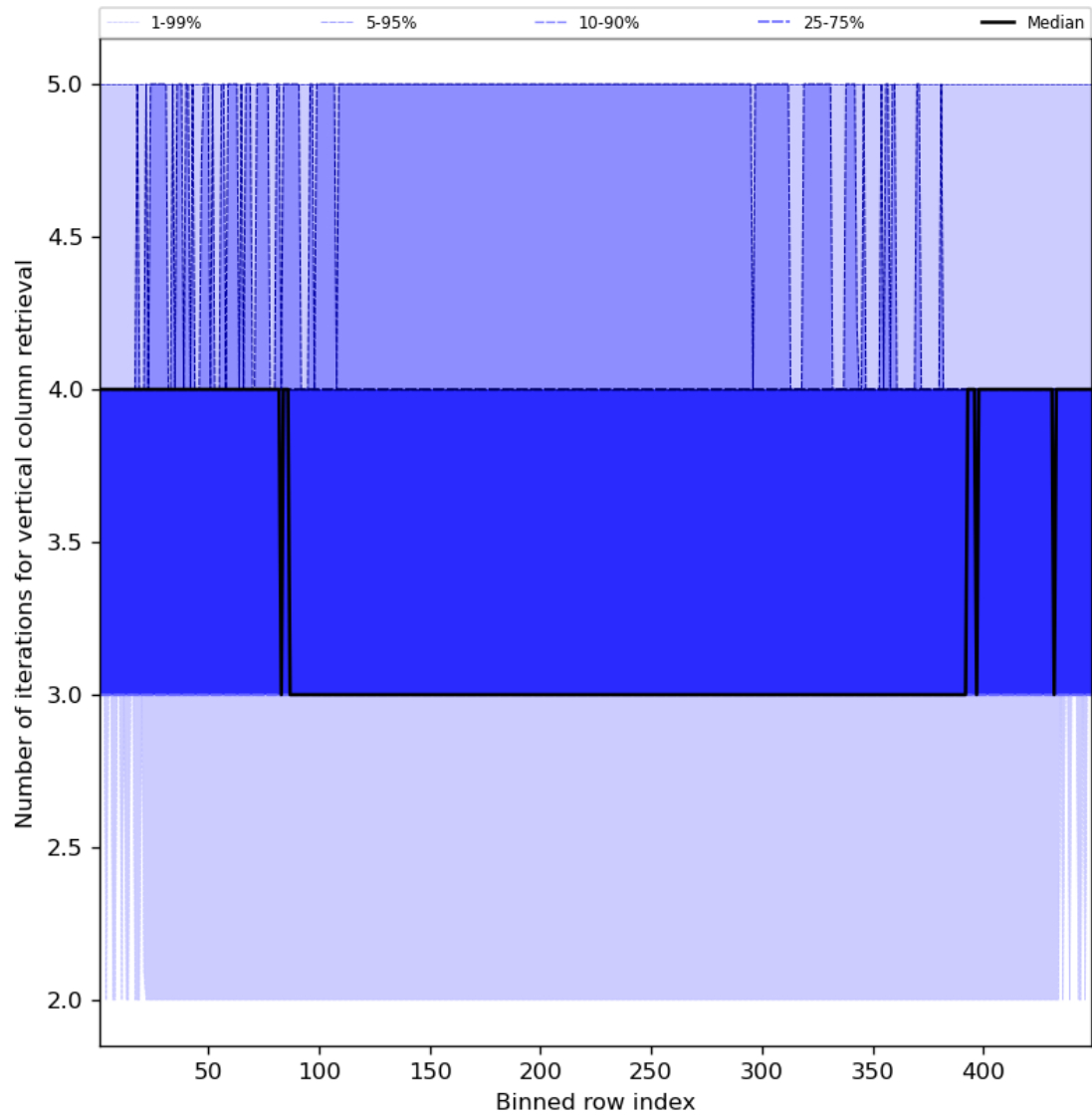
Figure 33: Along track statistics of “Number of iterations for vertical column retrieval” for 2023-08-17 to 2023-08-19
