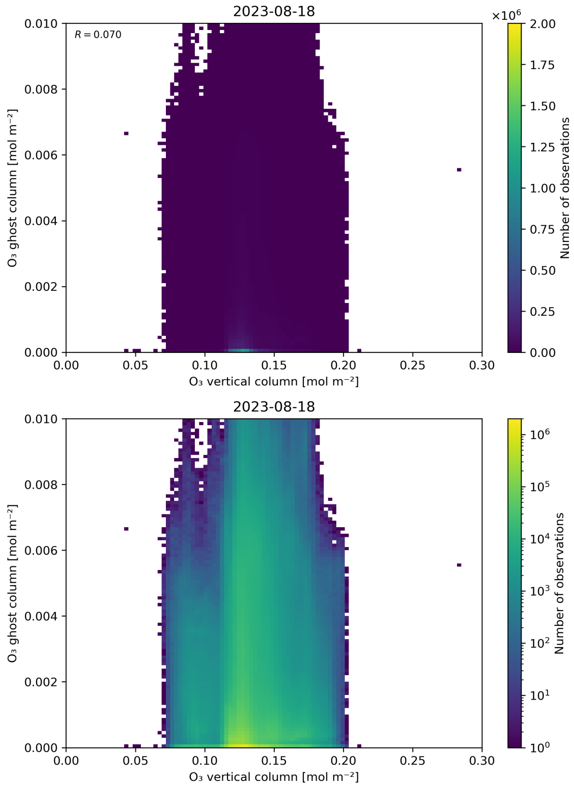
Figure 40: Scatter density plot of “O 3 vertical column” against “O 3 ghost column” for 2023-08-17 to 2023-08-19.
