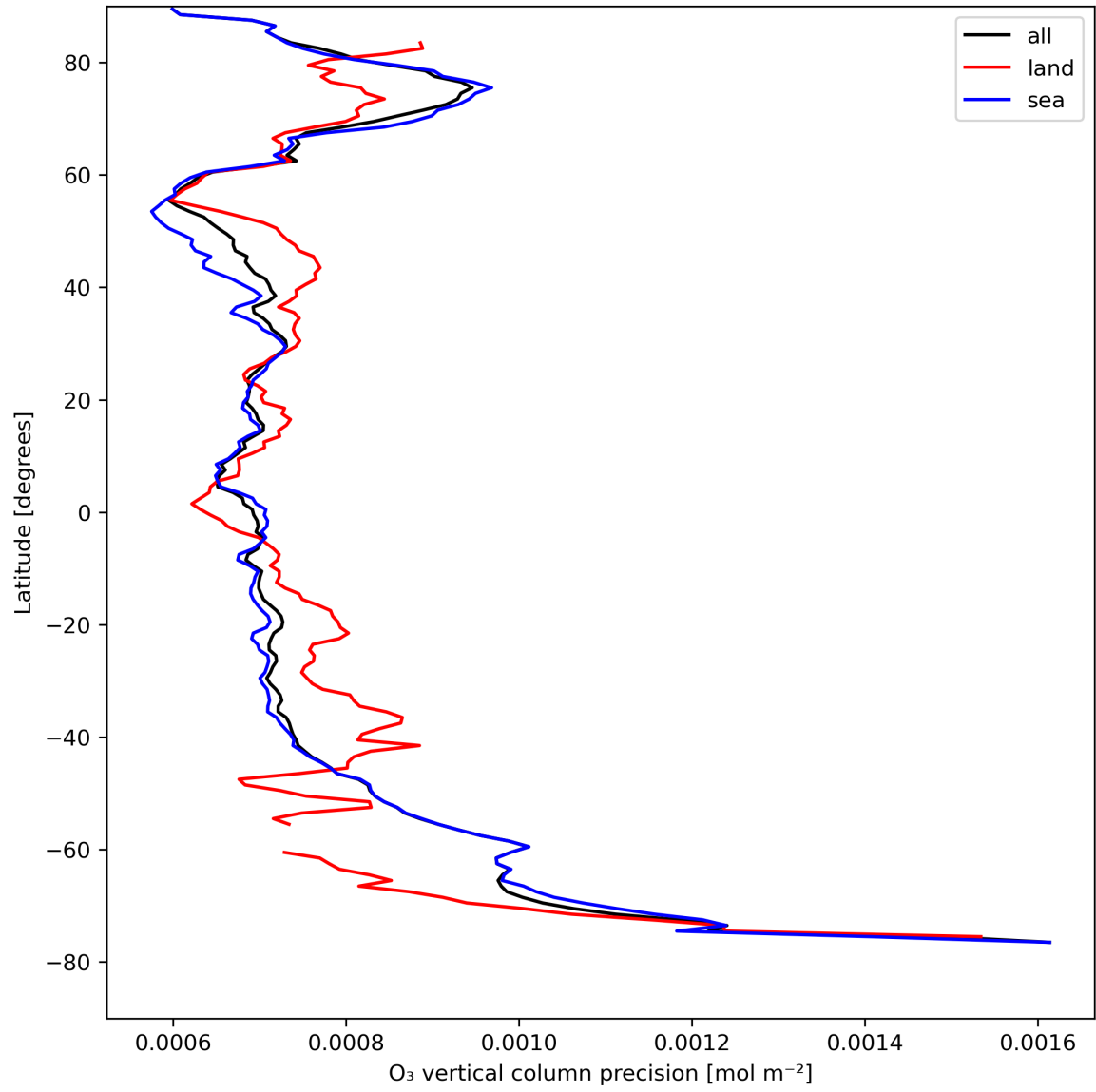
Figure 15: Zonal average of “O 3 vertical column precision” for 2023-08-17 to 2023-08-19.
