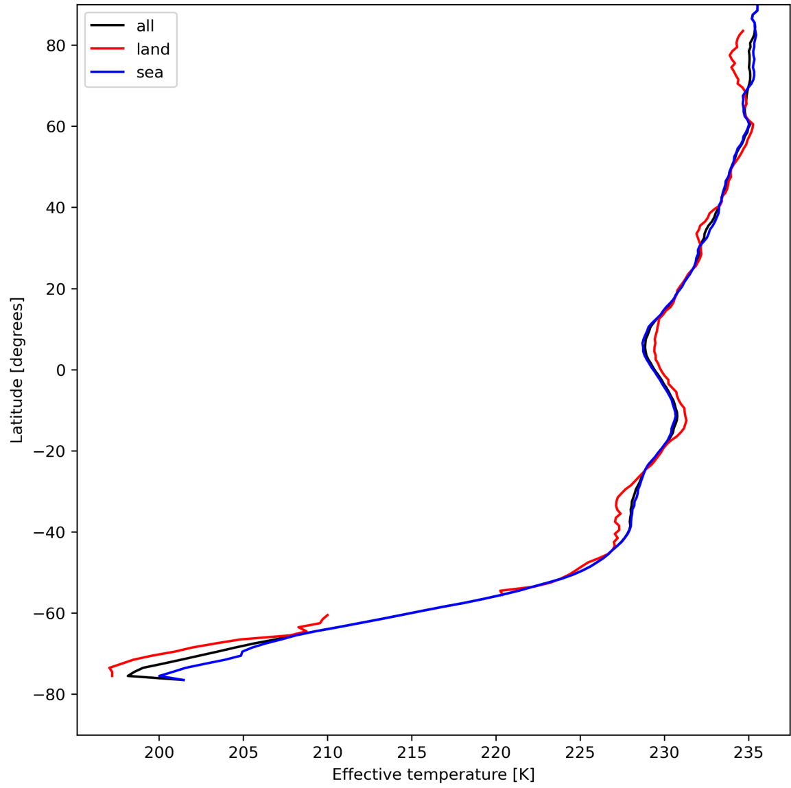
Figure 17: Zonal average of "Effective temperature" for 2023-08-17 to 2023-08-19.
