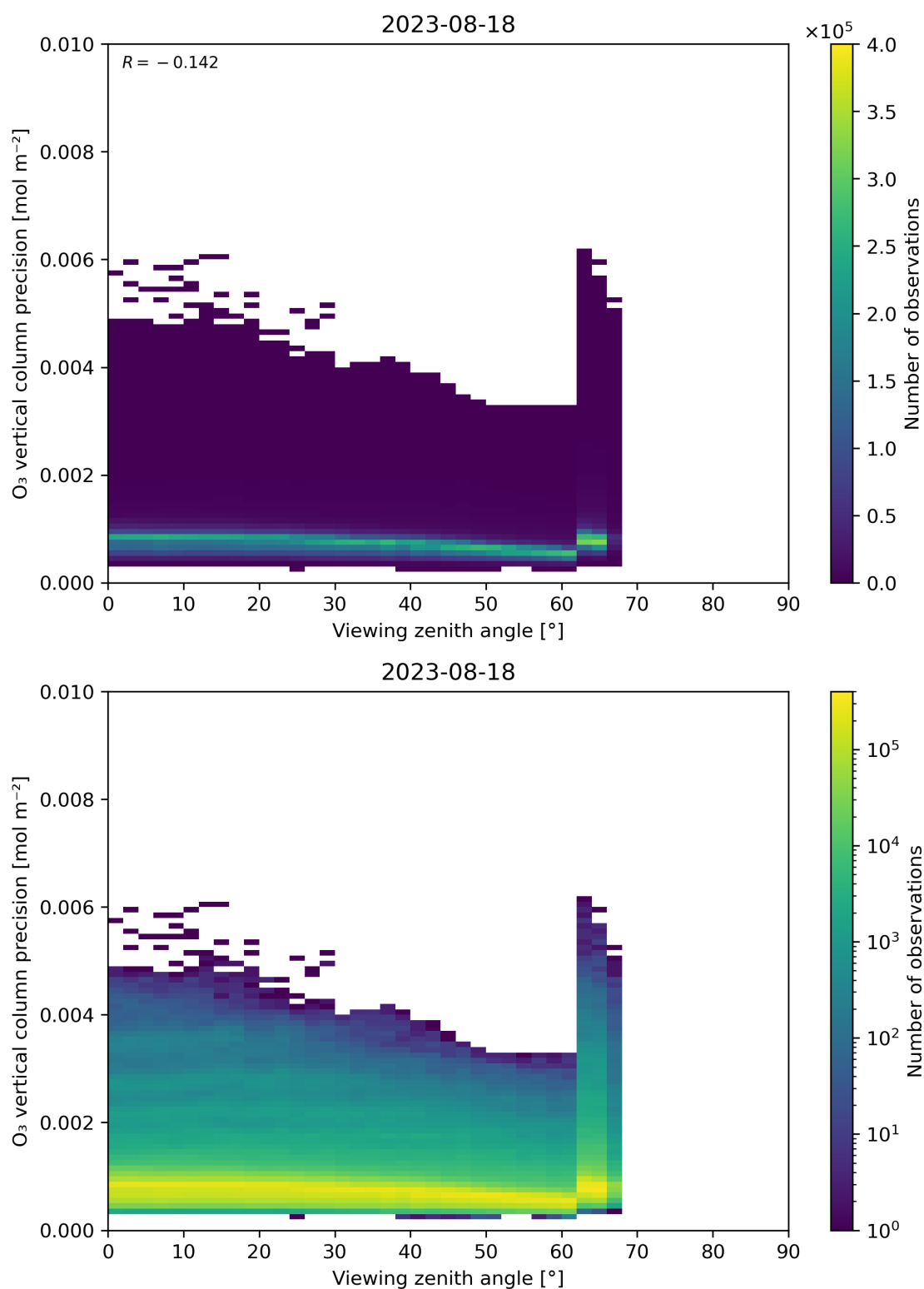
Figure 53: Scatter density plot of “Viewing zenith angle” against “O 3 vertical column precision” for 2023-08-17 to 2023-08-19.
