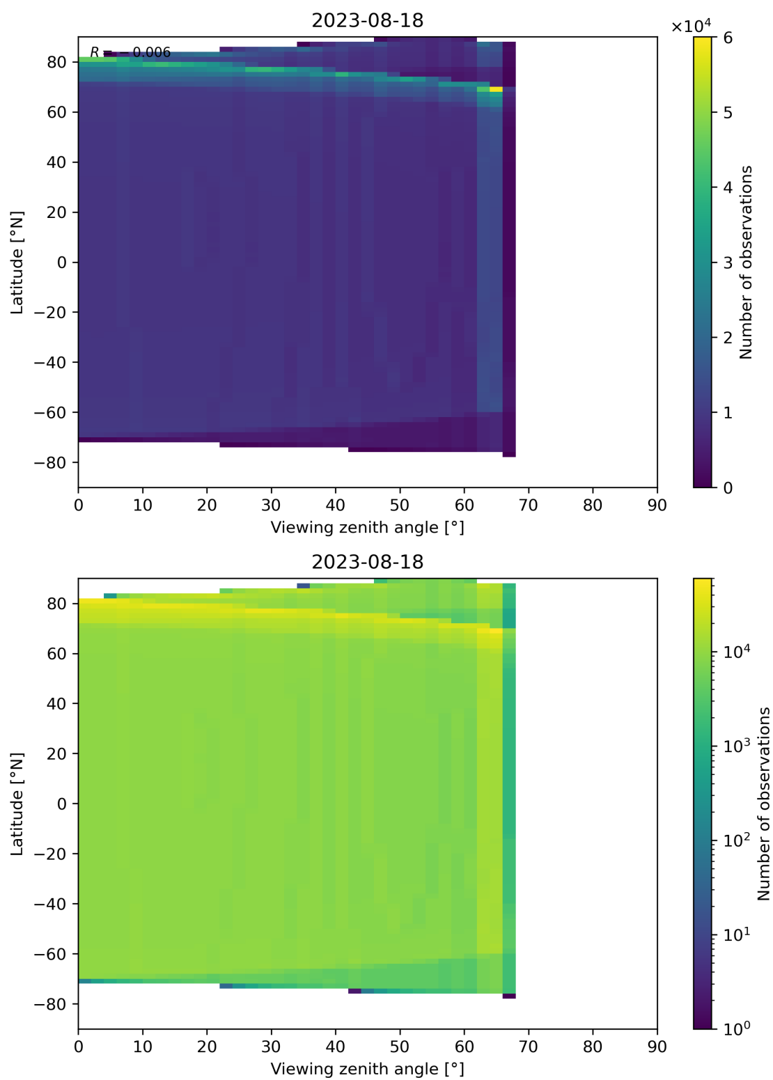
Figure 49: Scatter density plot of “Viewing zenith angle” against “Latitude” for 2023-08-17 to 2023-08-19.
