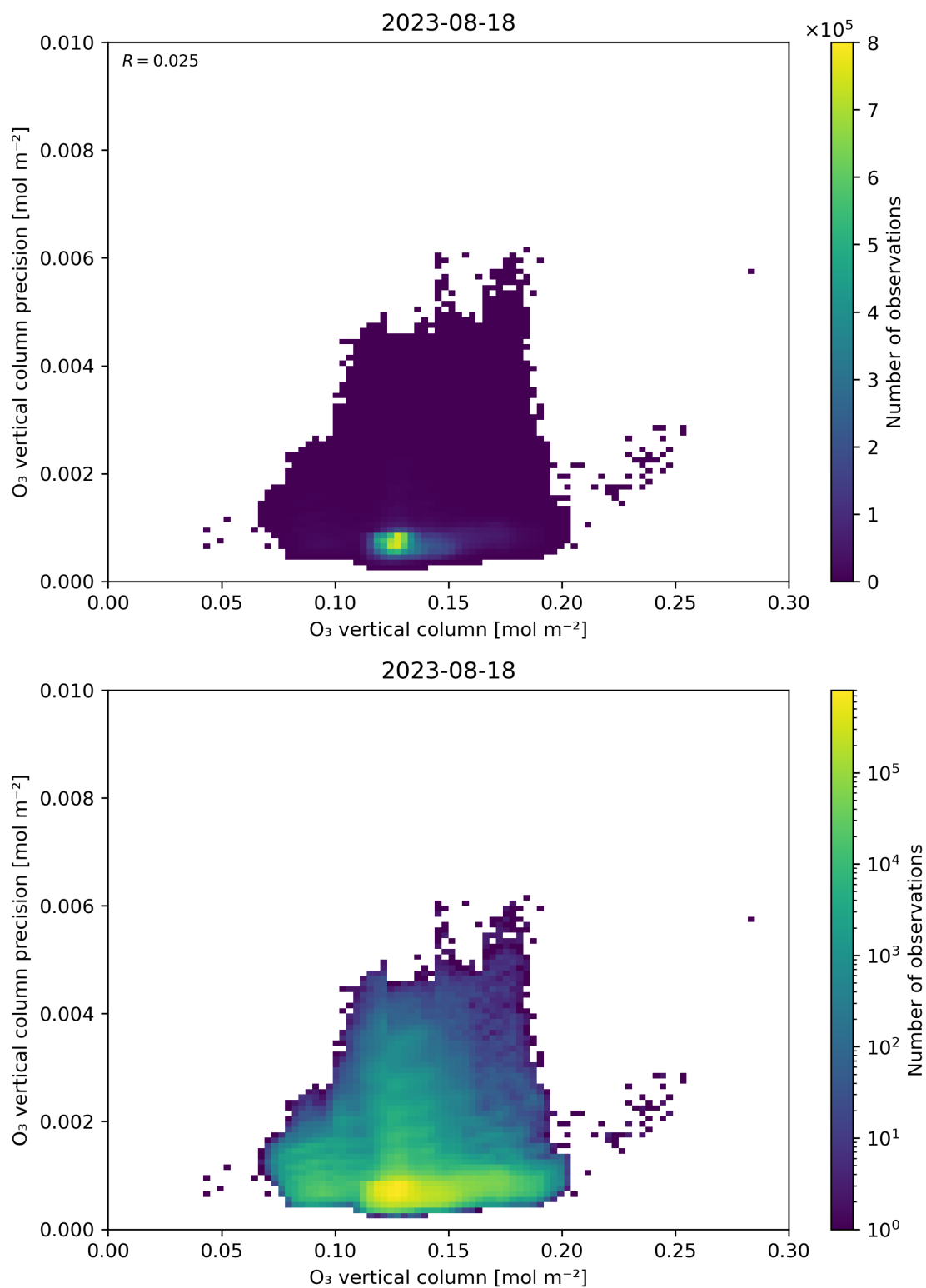
Figure 41: Scatter density plot of “O 3 vertical column” against “O 3 vertical column precision” for 2023-08-17 to 2023-08-19.
