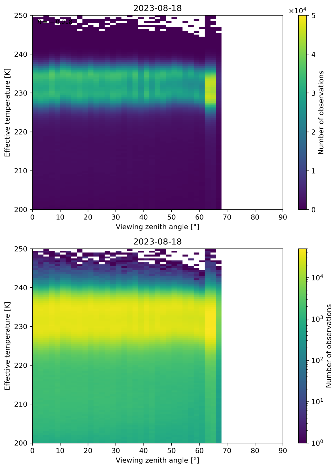
Figure 50: Scatter density plot of “Viewing zenith angle” against “Effective temperature” for 2023-08-17 to 2023-08-19.
