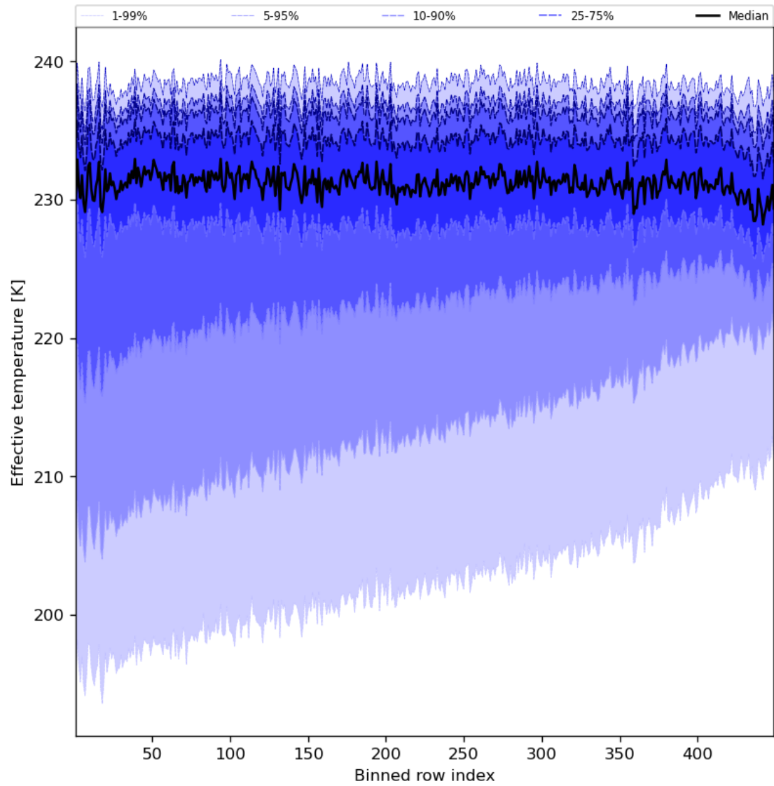
Figure 31: Along track statistics of “Effective temperature” for 2023-08-17 to 2023-08-19
