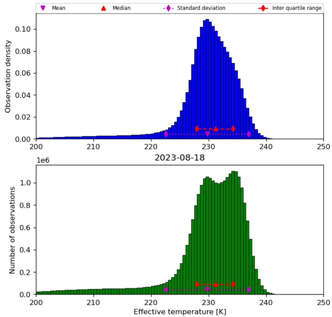
Figure 24: Histogram of “Effective temperature” for 2023-08-17 to 2023-08-19
