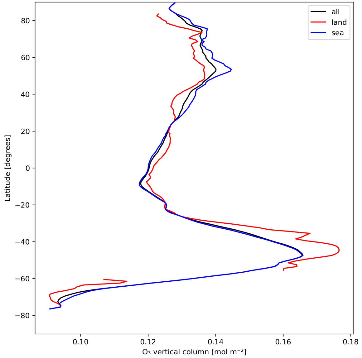
Figure 14: Zonal average of “O 3 vertical column” for 2023-08-17 to 2023-08-19.
