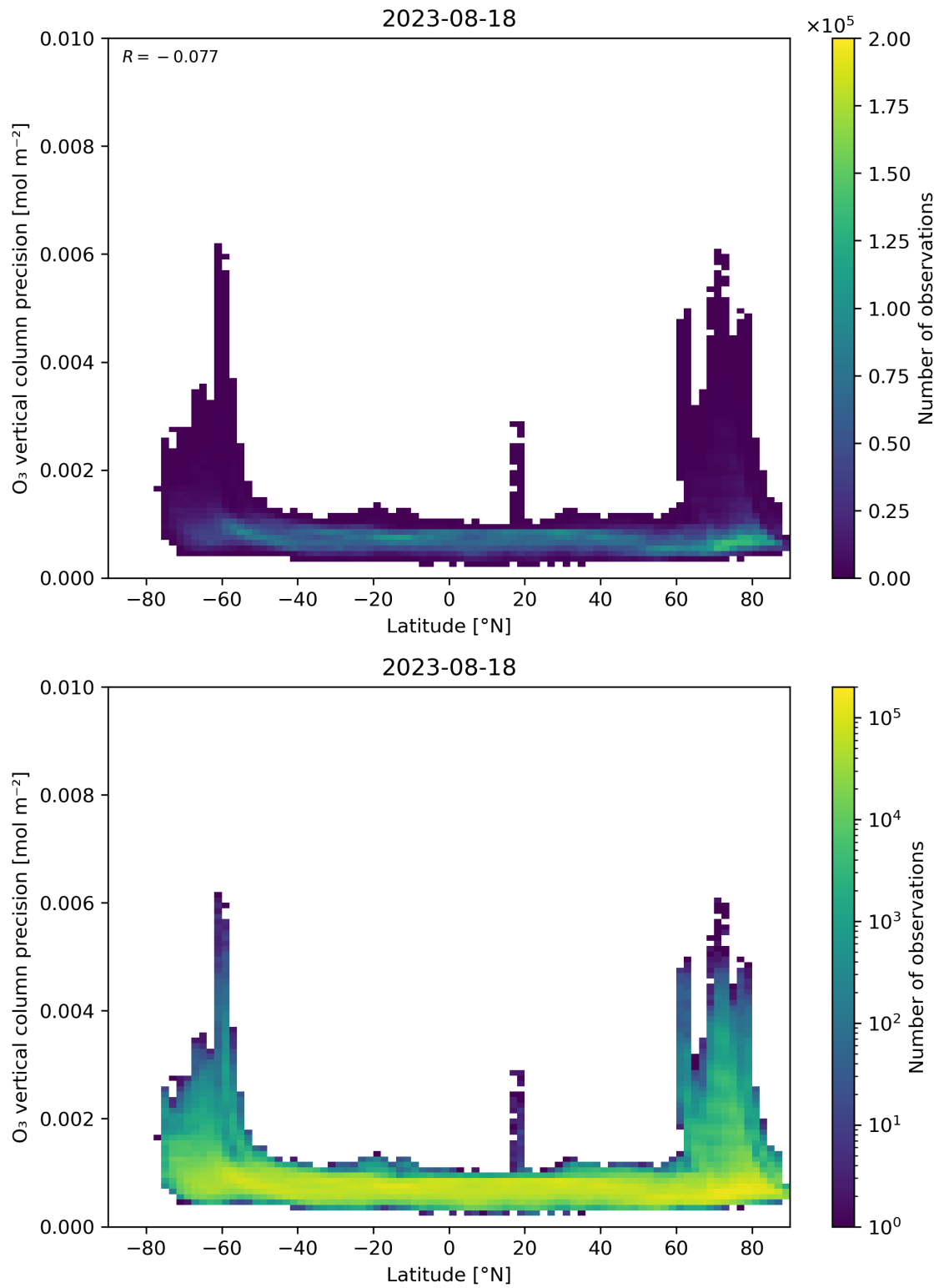
Figure 37: Scatter density plot of “Latitude” against “O 3 vertical column precision” for 2023-08-17 to 2023-08-19.
