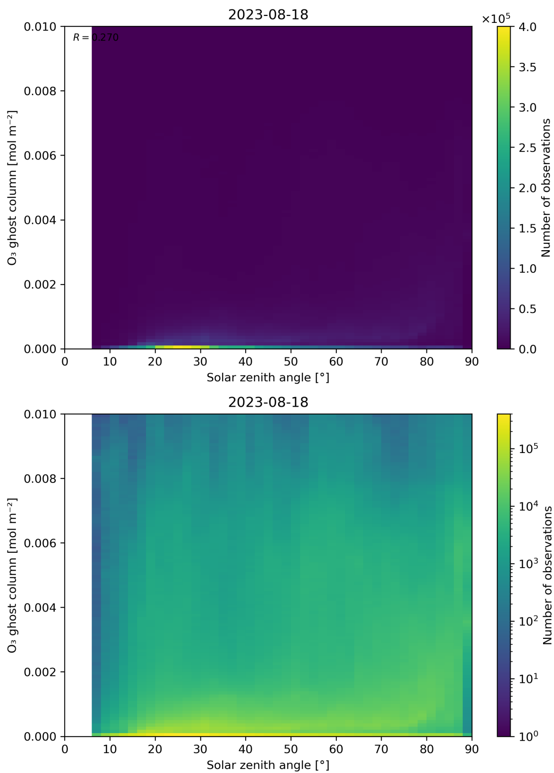
Figure 46: Scatter density plot of “Solar zenith angle” against “O 3 ghost column” for 2023-08-17 to 2023-08-19.
