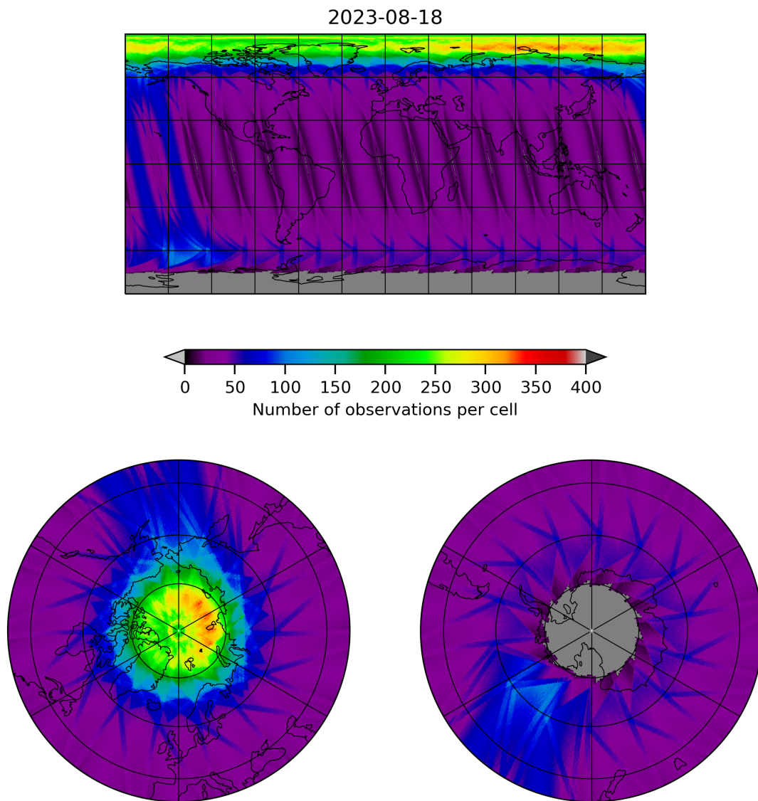
Figure 12: Map of the number of observations for 2023-08-17 to 2023-08-19
