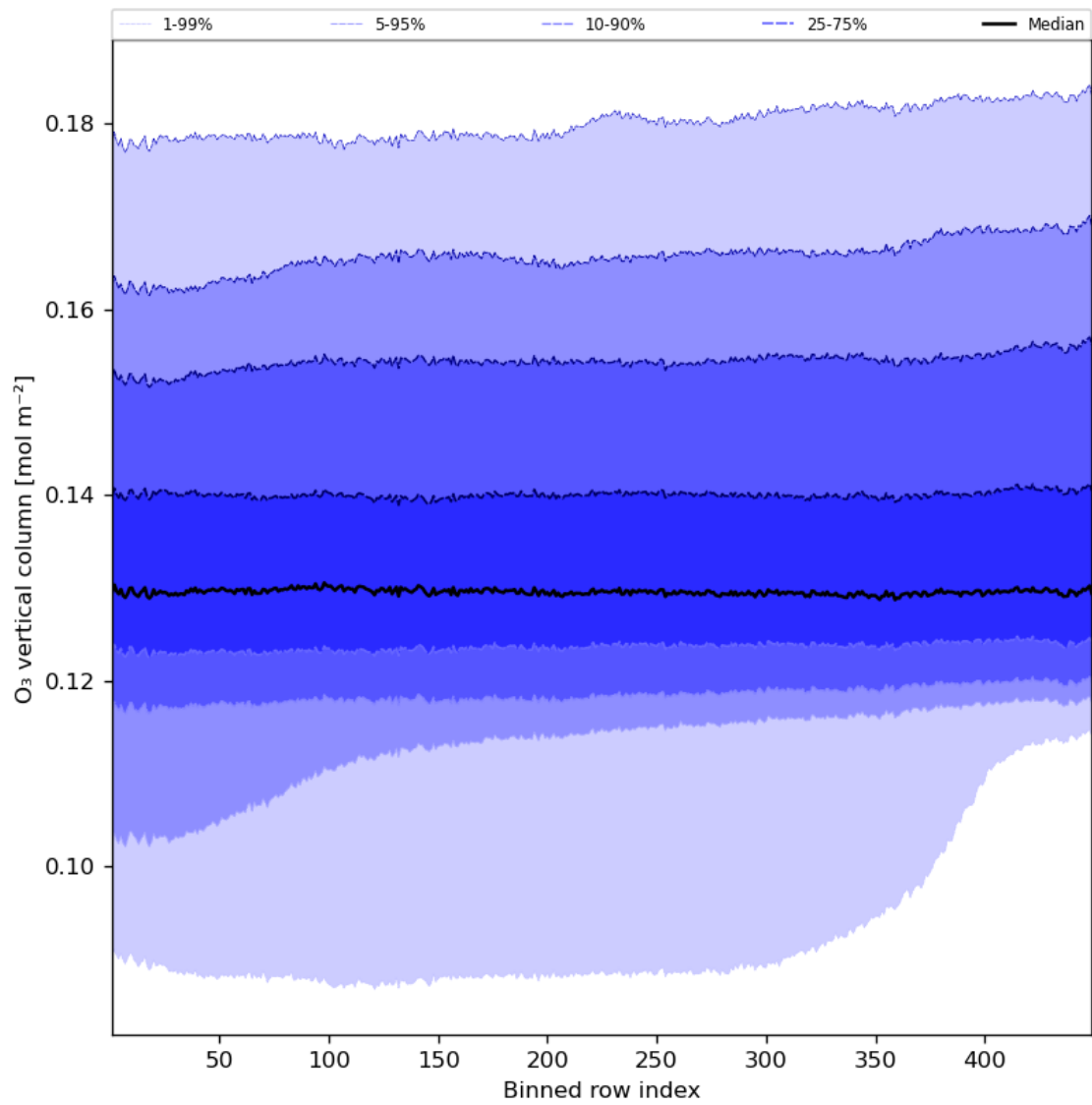
Figure 28: Along track statistics of “O 3 vertical column” for 2023-08-17 to 2023-08-19
