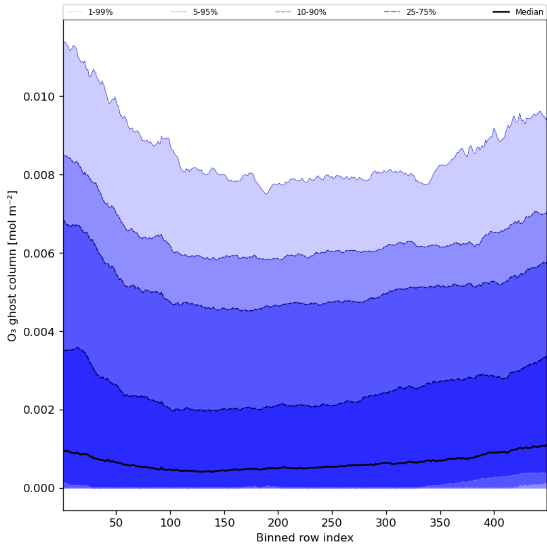
Figure 32: Along track statistics of “O 3 ghost column” for 2023-08-17 to 2023-08-19
