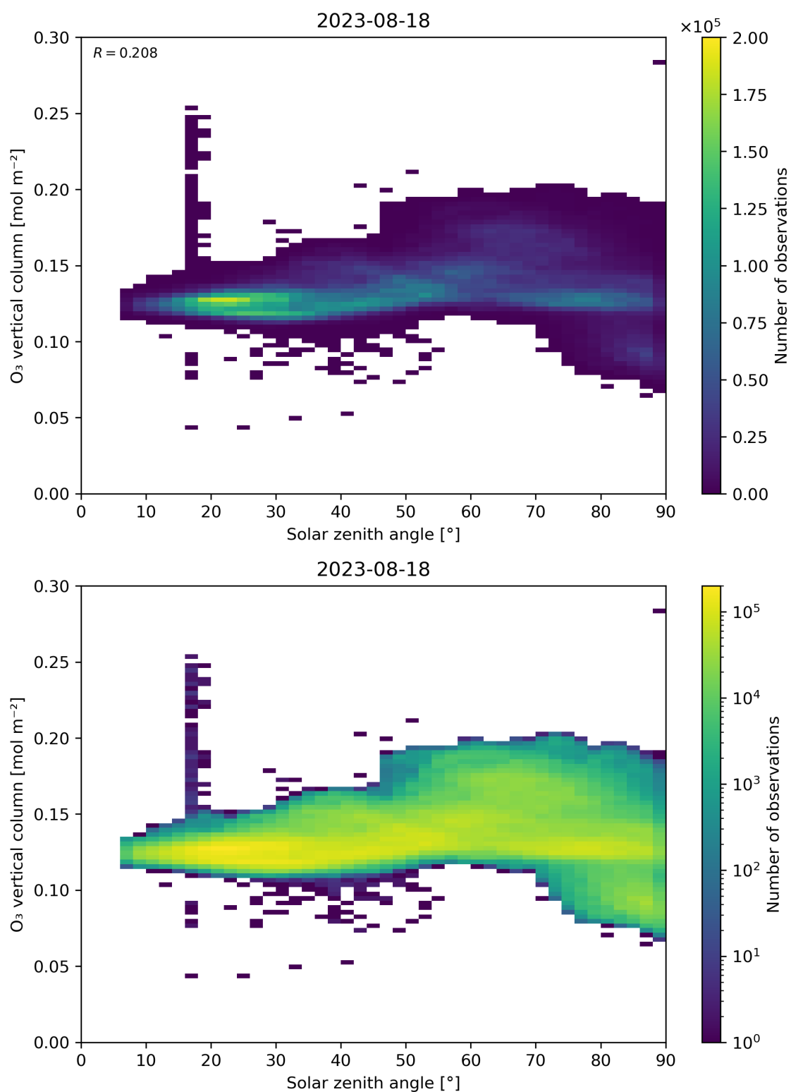
Figure 47: Scatter density plot of “Solar zenith angle” against “O 3 vertical column” for 2023-08-17 to 2023-08-19.
