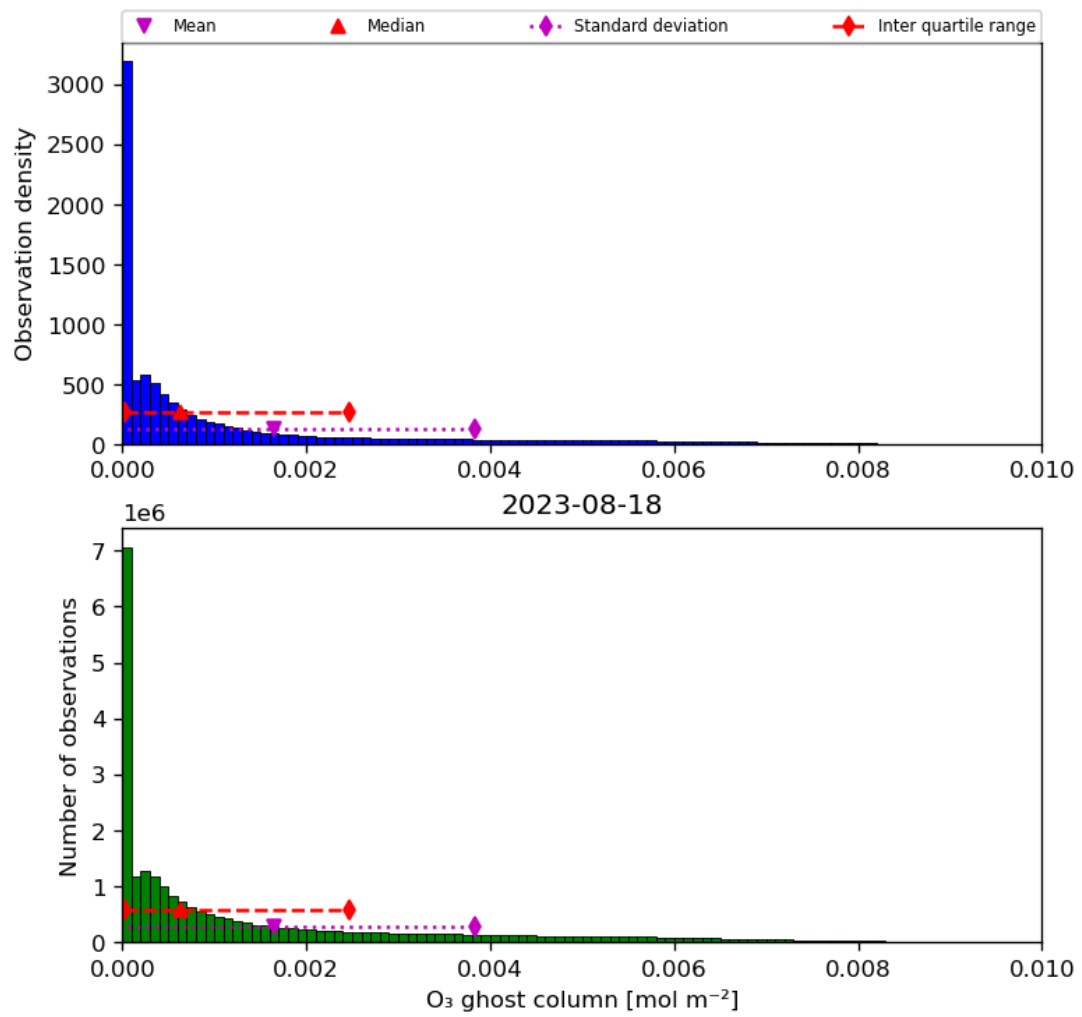
Figure 25: Histogram of “O 3 ghost column” for 2023-08-17 to 2023-08-19
