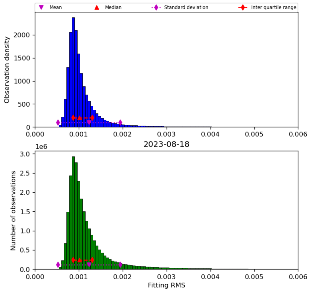
Figure 23: Histogram of “Fitting RMS” for 2023-08-17 to 2023-08-19
