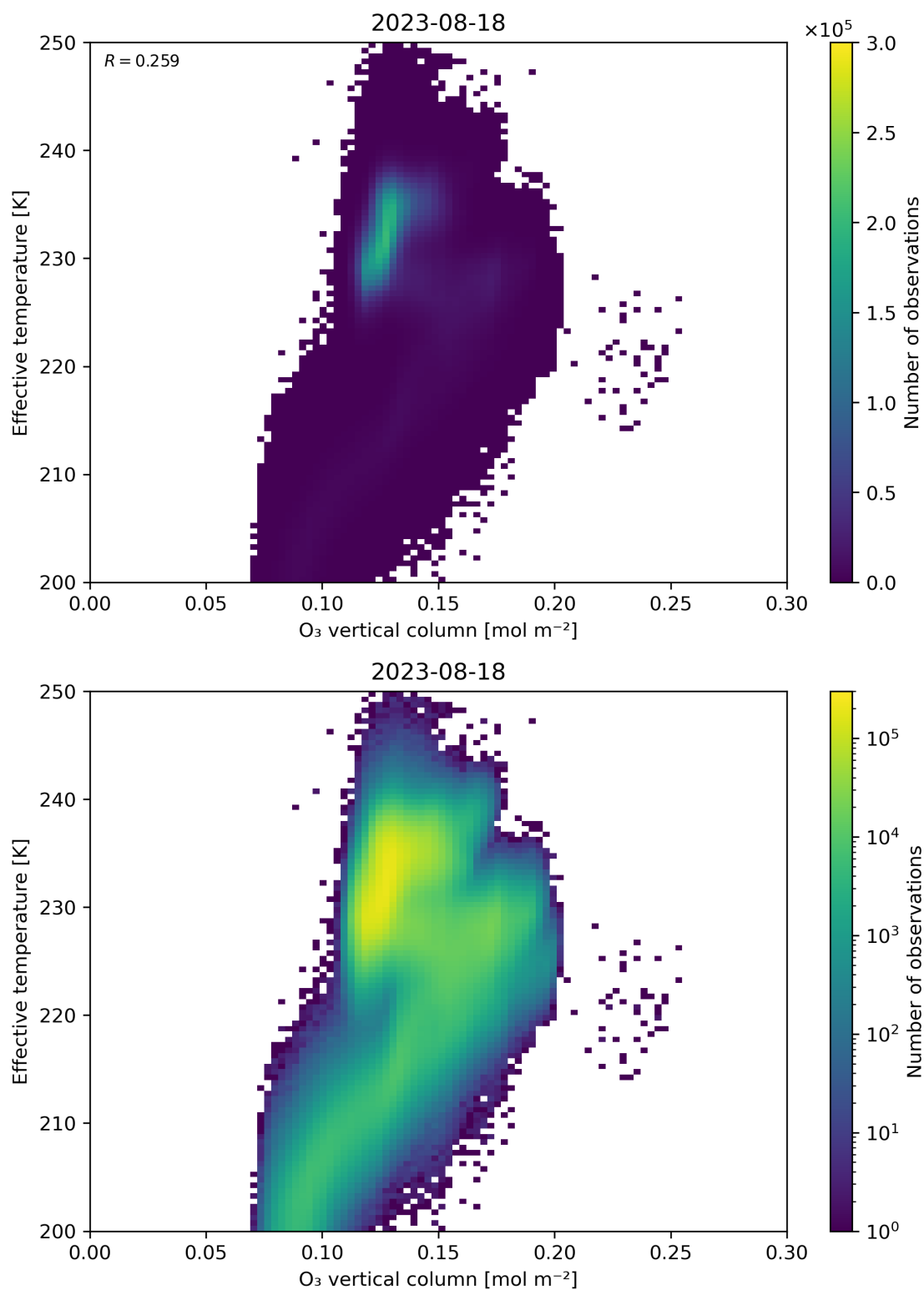
Figure 39: Scatter density plot of “O 3 vertical column” against “Effective temperature” for 2023-08-17 to 2023-08-19.
