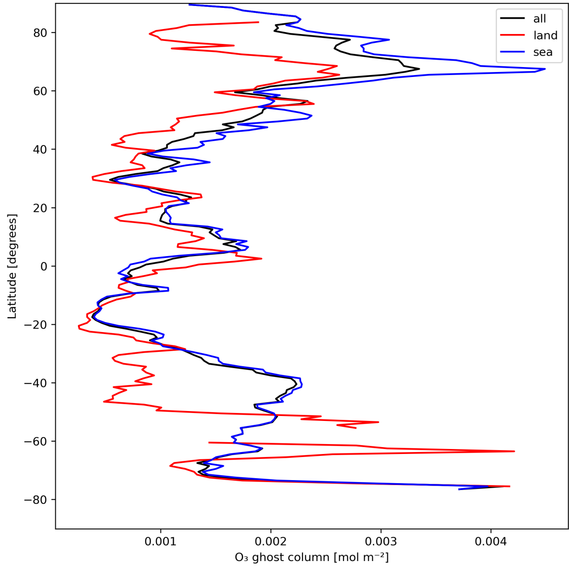
Figure 18: Zonal average of "O 3 ghost column" for 2023-08-17 to 2023-08-19.
