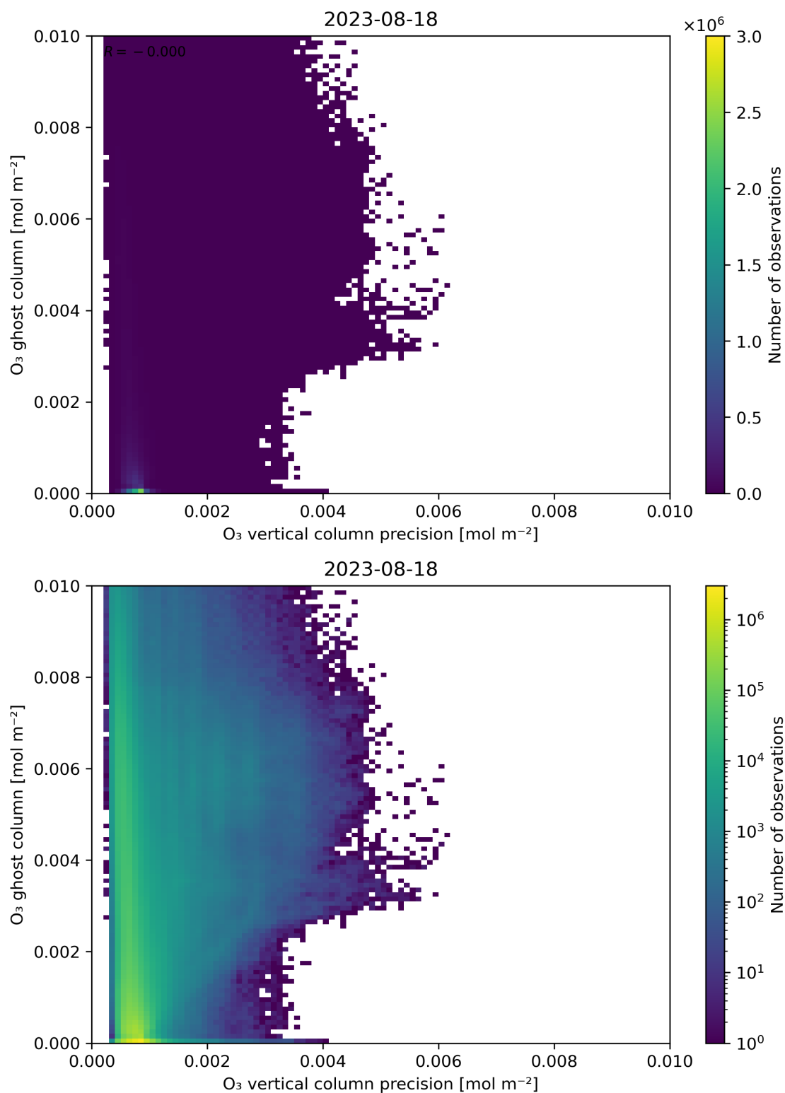
Figure 43: Scatter density plot of “ \text{O}_3 vertical column precision” against “ \text{O}_3 ghost column” for 2023-08-17 to 2023-08-19.
