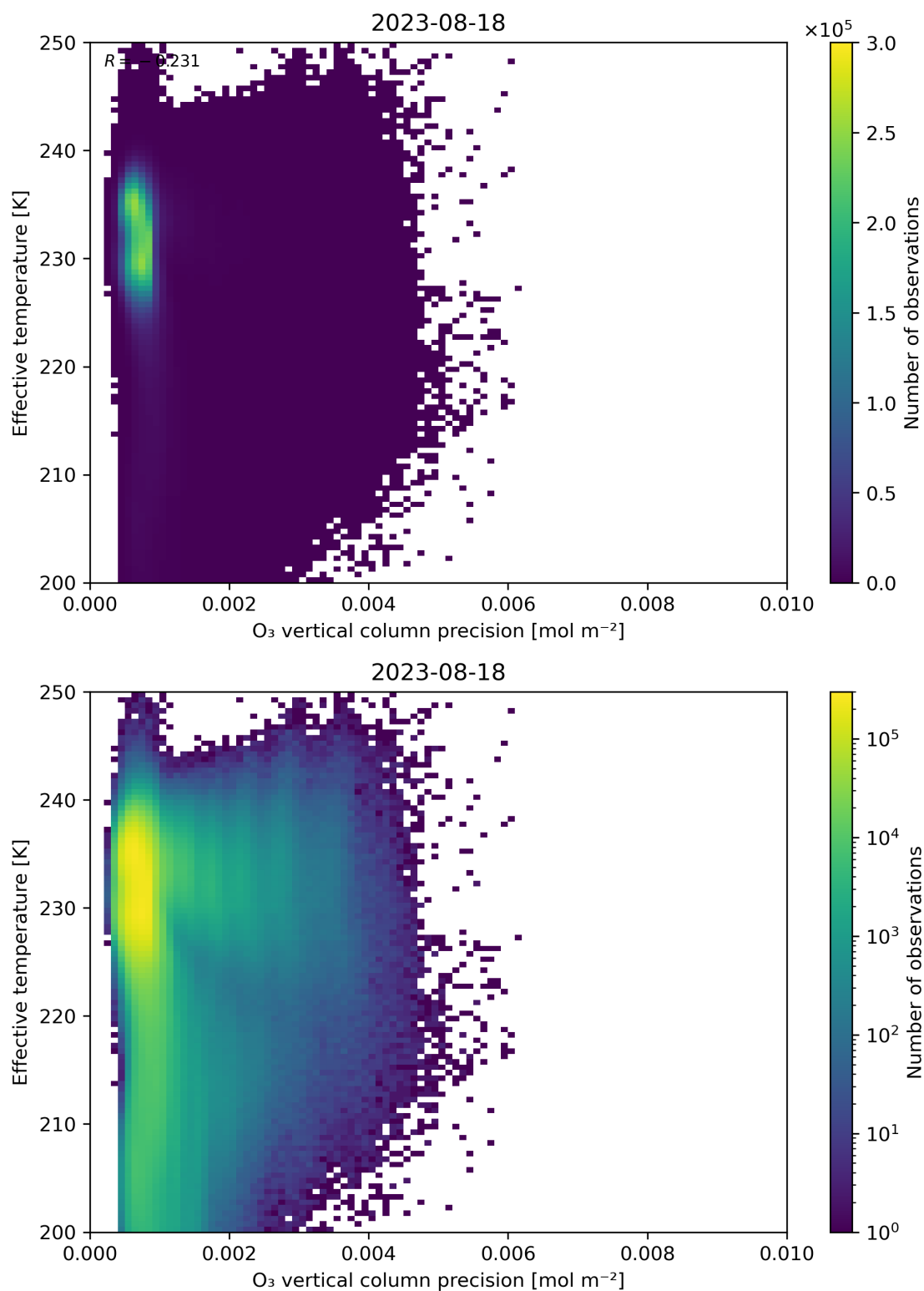
Figure 42: Scatter density plot of “O 3 vertical column precision” against “Effective temperature” for 2023-08-17 to 2023-08-19.
