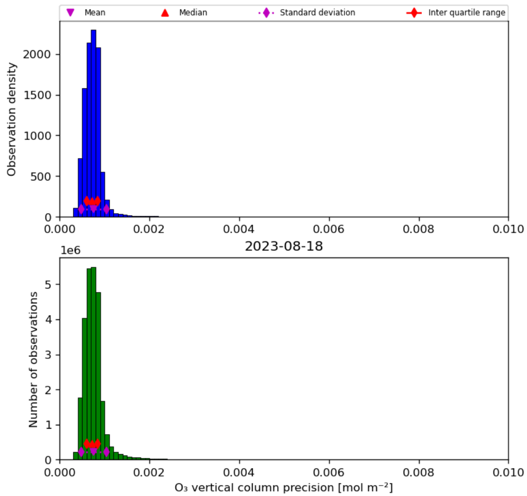
Figure 22: Histogram of “O 3 vertical column precision” for 2023-08-17 to 2023-08-19
