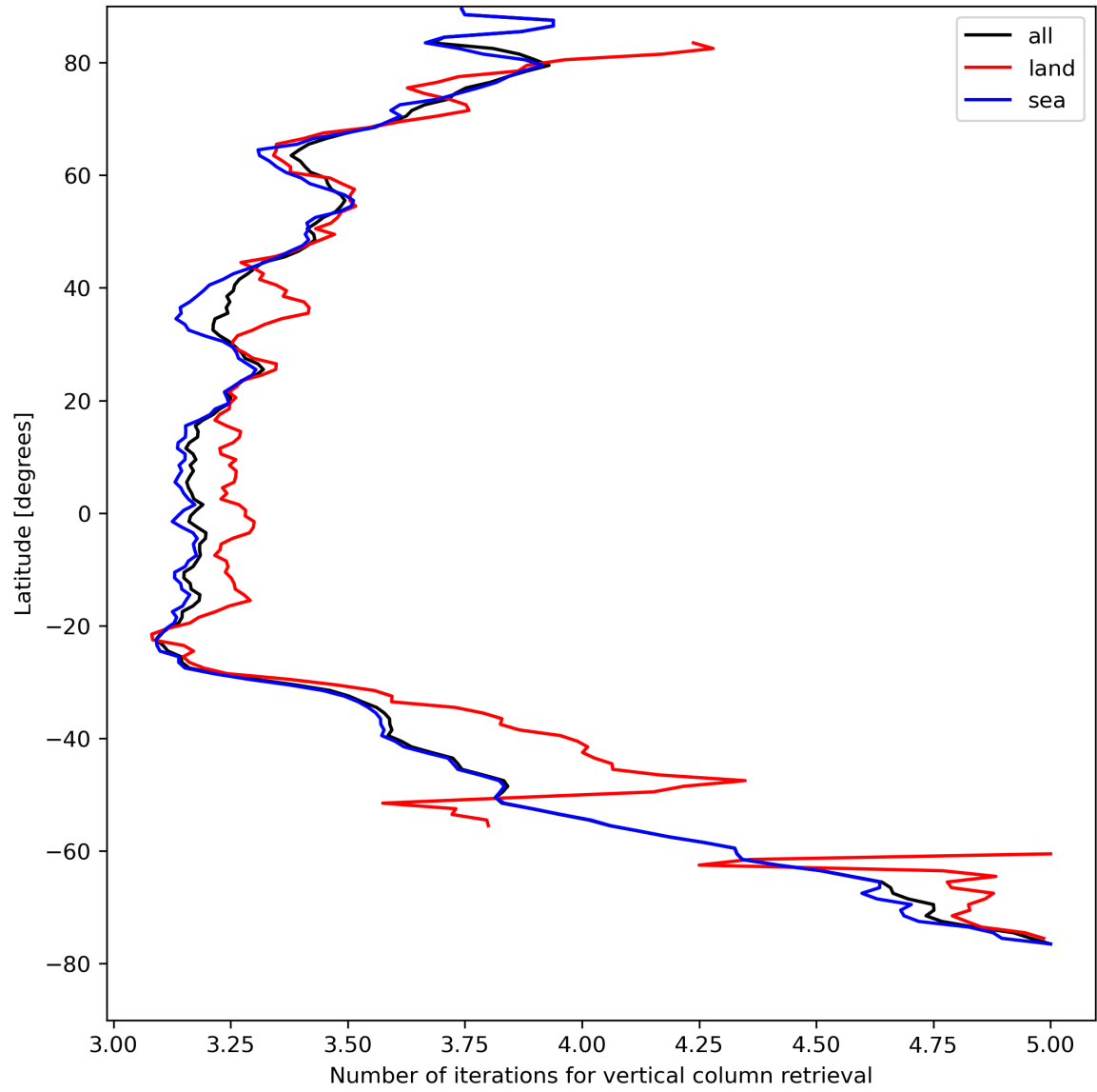
Figure 19: Zonal average of “Number of iterations for vertical column retrieval” for 2023-08-17 to 2023-08-19.
