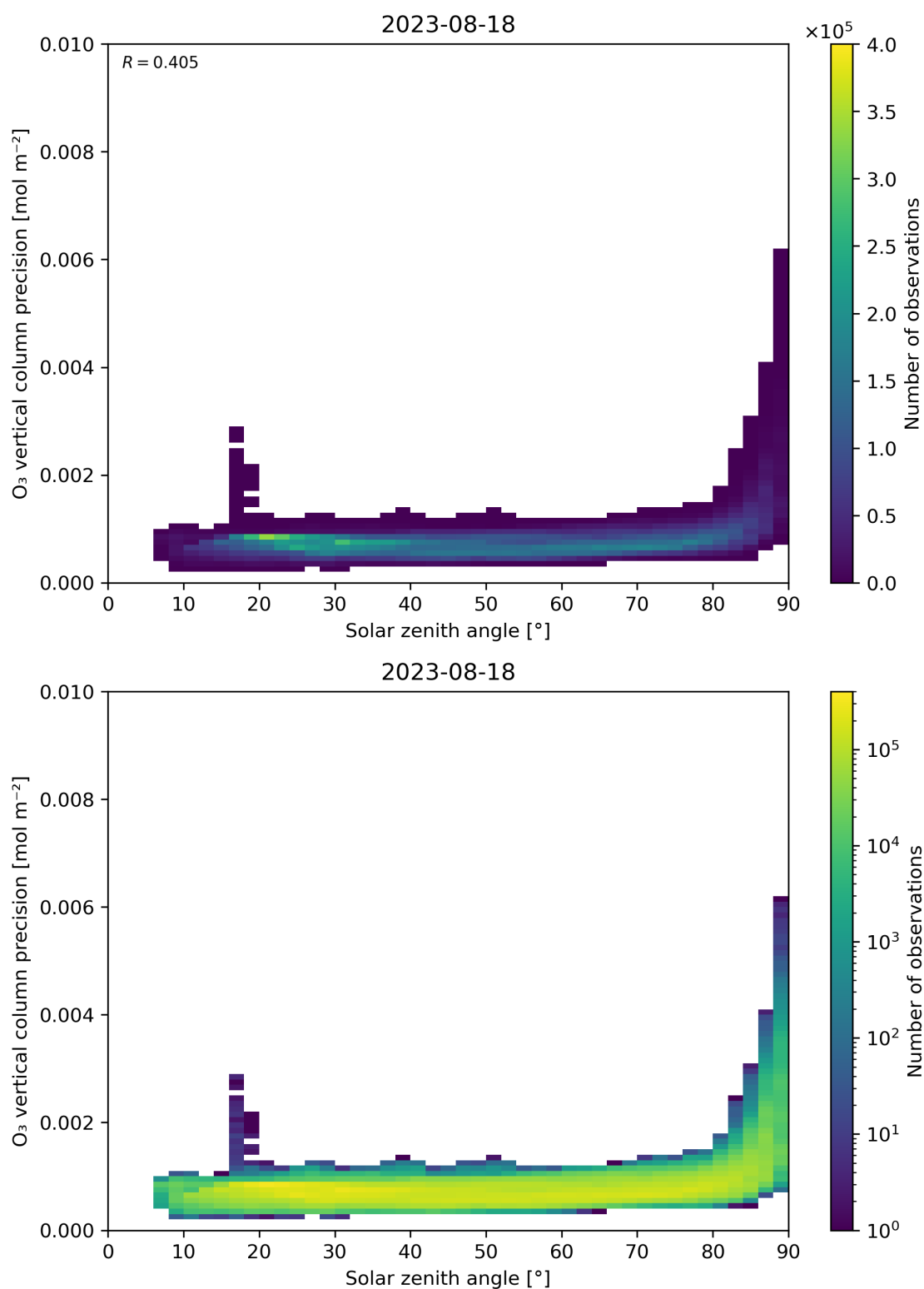
Figure 48: Scatter density plot of “Solar zenith angle” against “O 3 vertical column precision” for 2023-08-17 to 2023-08-19.
