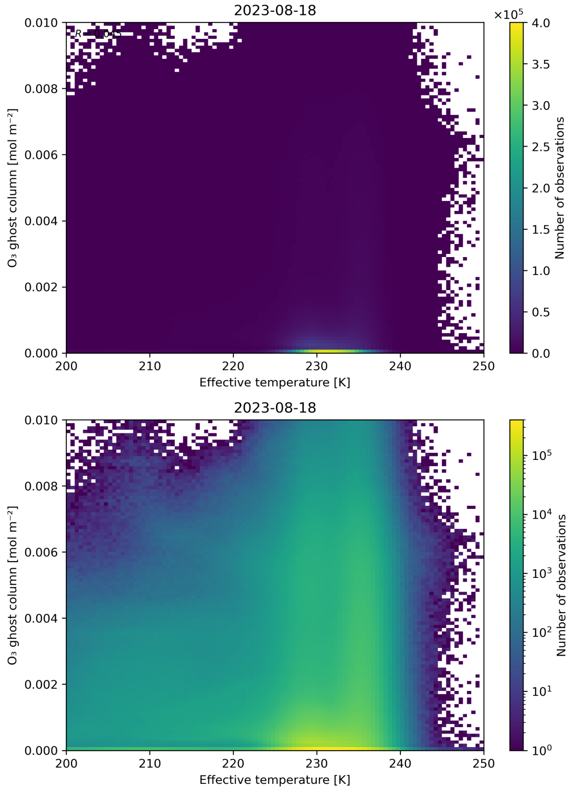
Figure 38: Scatter density plot of “Effective temperature” against “O 3 ghost column” for 2023-08-17 to 2023-08-19.
