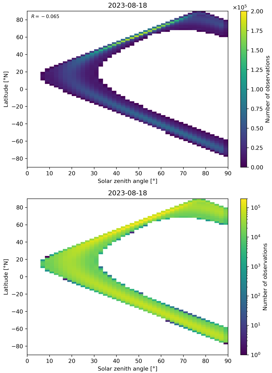
Figure 44: Scatter density plot of “Solar zenith angle” against “Latitude” for 2023-08-17 to 2023-08-19.
