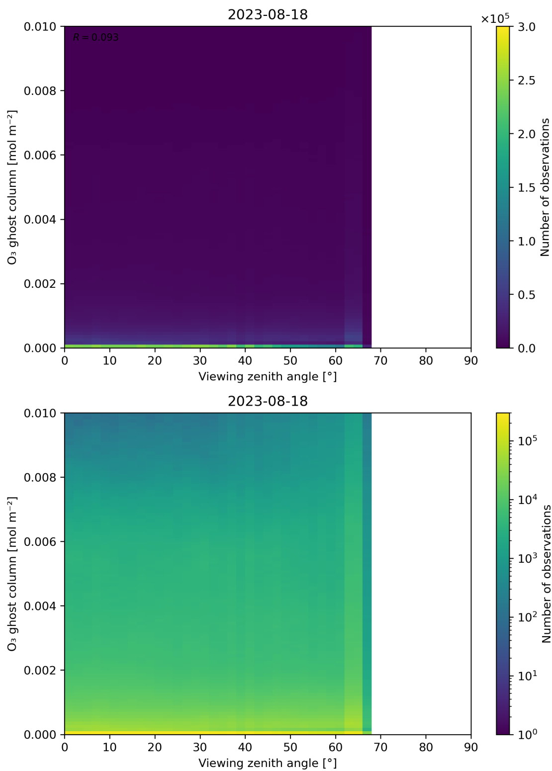
Figure 51: Scatter density plot of “Viewing zenith angle” against “O 3 ghost column” for 2023-08-17 to 2023-08-19.
