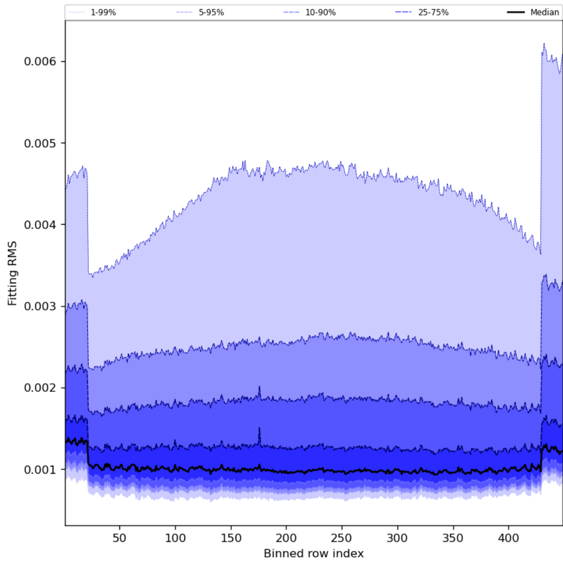
Figure 30: Along track statistics of “Fitting RMS” for 2023-08-17 to 2023-08-19
