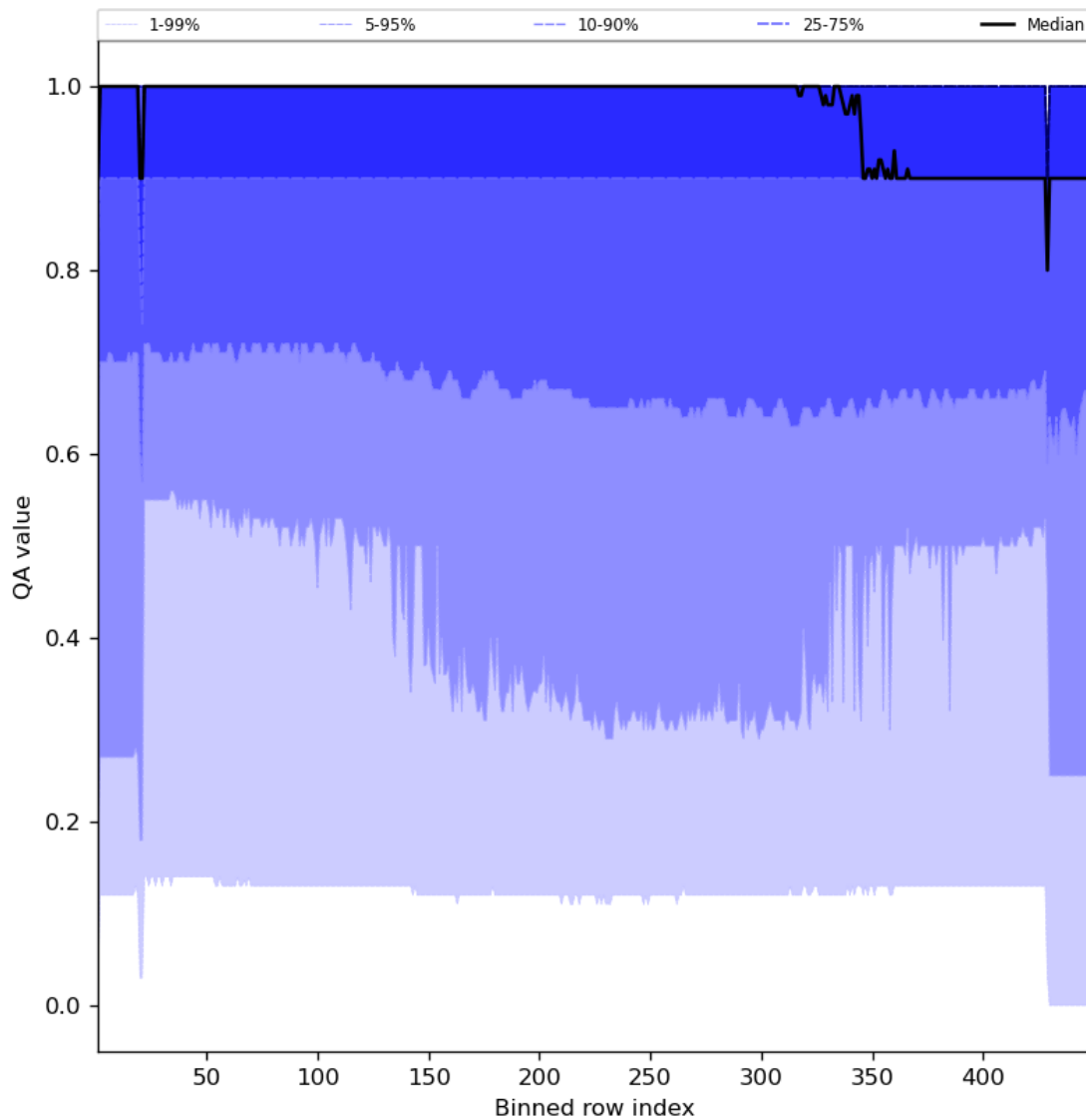
Figure 27: Along track statistics of “QA value” for 2023-08-17 to 2023-08-19
