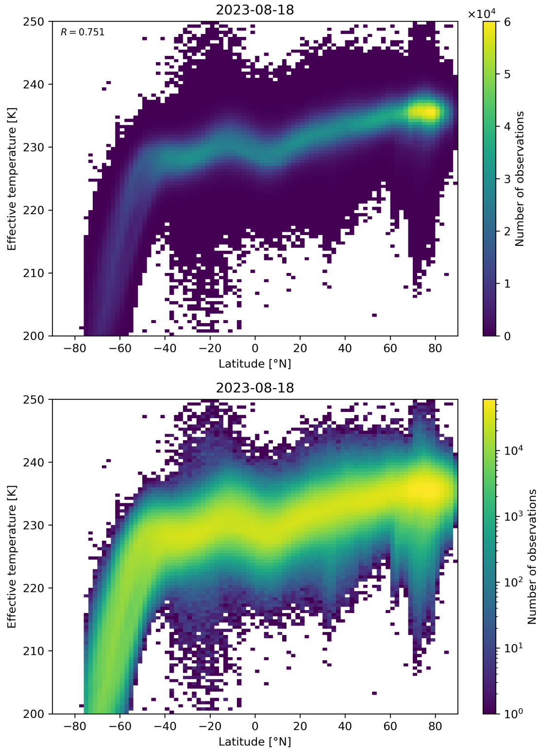
Figure 34: Scatter density plot of “Latitude” against “Effective temperature” for 2023-08-17 to 2023-08-19.
