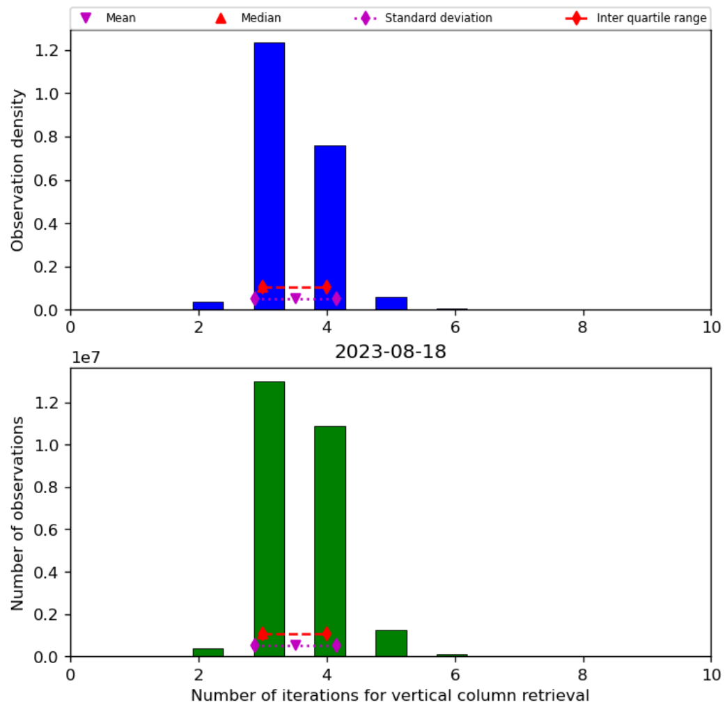
Figure 26: Histogram of “Number of iterations for vertical column retrieval” for 2023-08-17 to 2023-08-19
