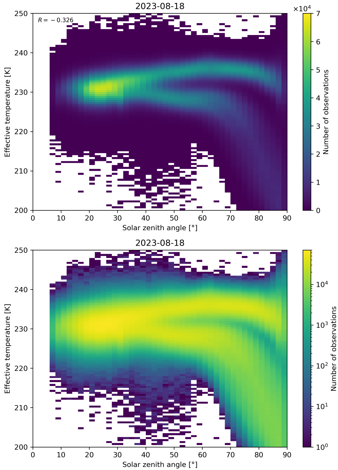
Figure 45: Scatter density plot of “Solar zenith angle” against “Effective temperature” for 2023-08-17 to 2023-08-19.
