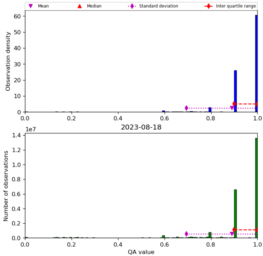
Figure 20: Histogram of “QA value” for 2023-08-17 to 2023-08-19
