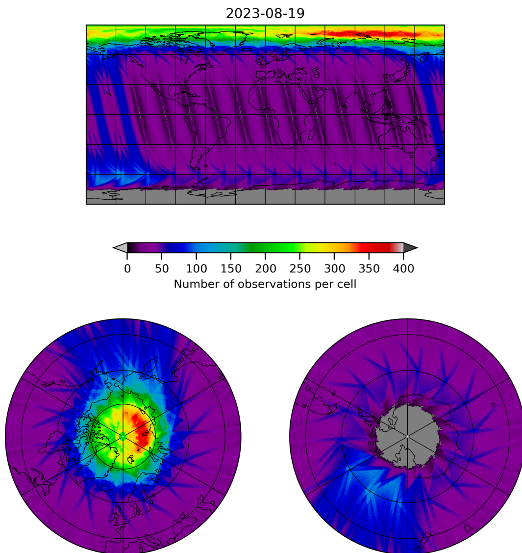
Figure 12: Map of the number of observations for 2023-08-18 to 2023-08-20
