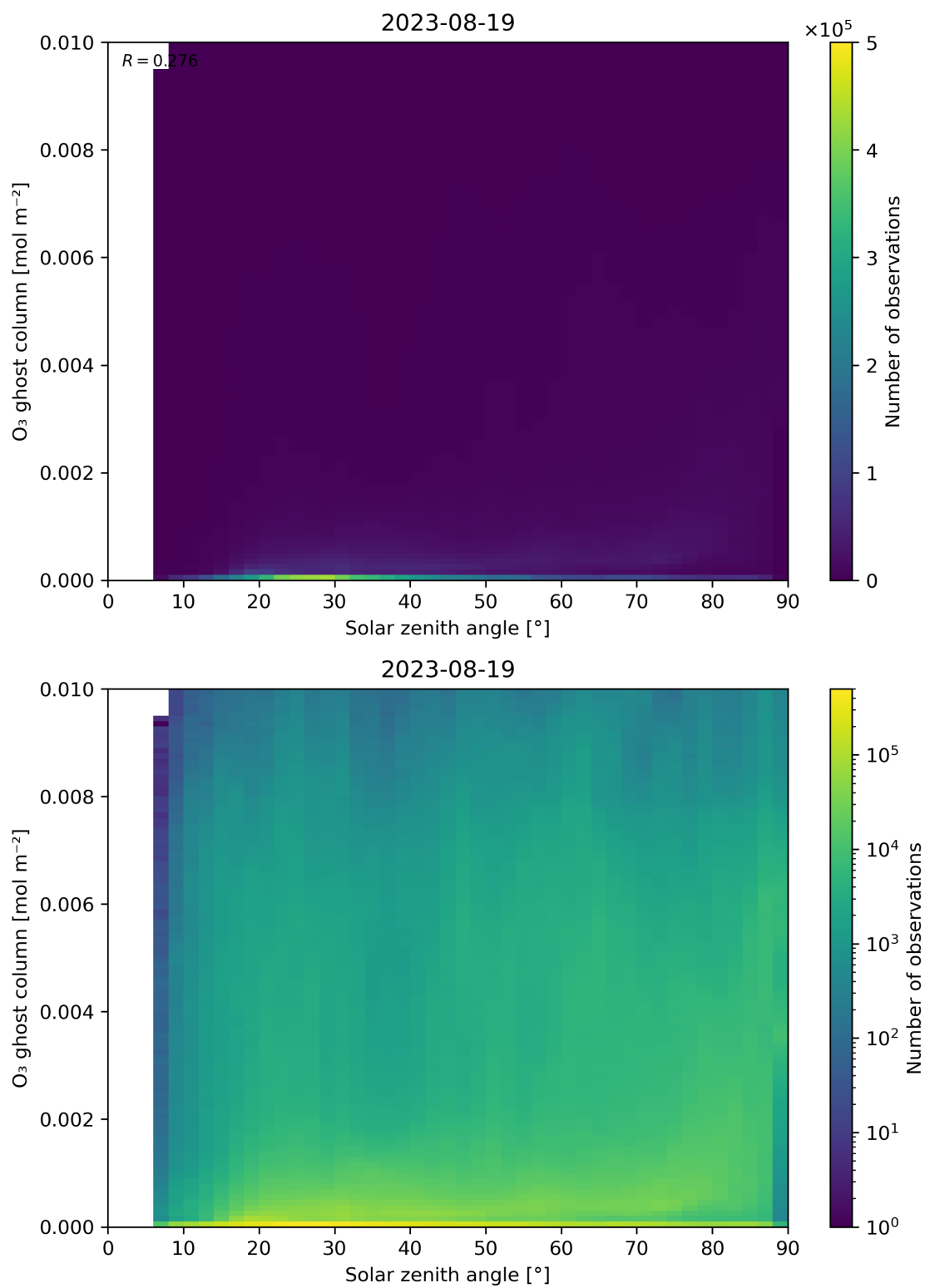
Figure 46: Scatter density plot of “Solar zenith angle” against “O 3 ghost column” for 2023-08-18 to 2023-08-20.
