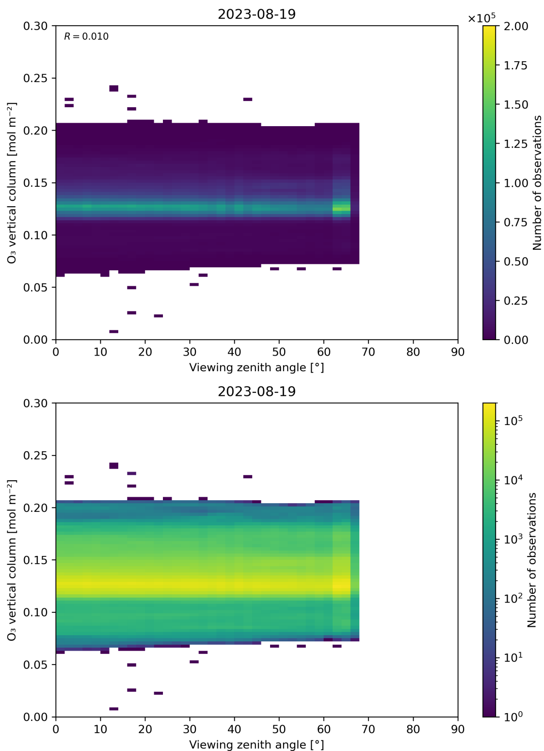
Figure 52: Scatter density plot of “Viewing zenith angle” against “O 3 vertical column” for 2023-08-18 to 2023-08-20.
