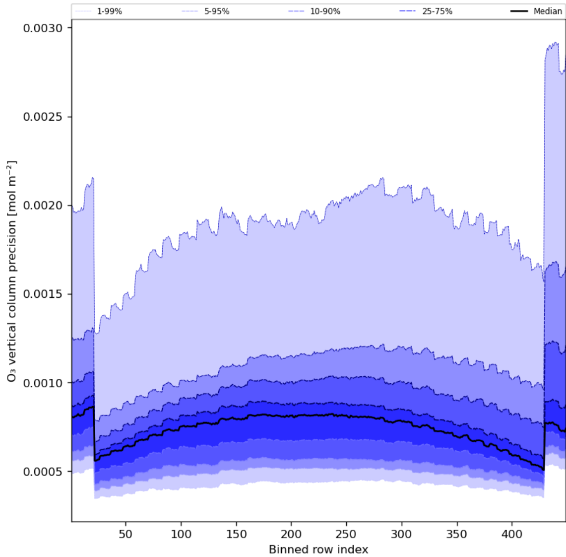
Figure 29: Along track statistics of “O 3 vertical column precision” for 2023-08-18 to 2023-08-20
