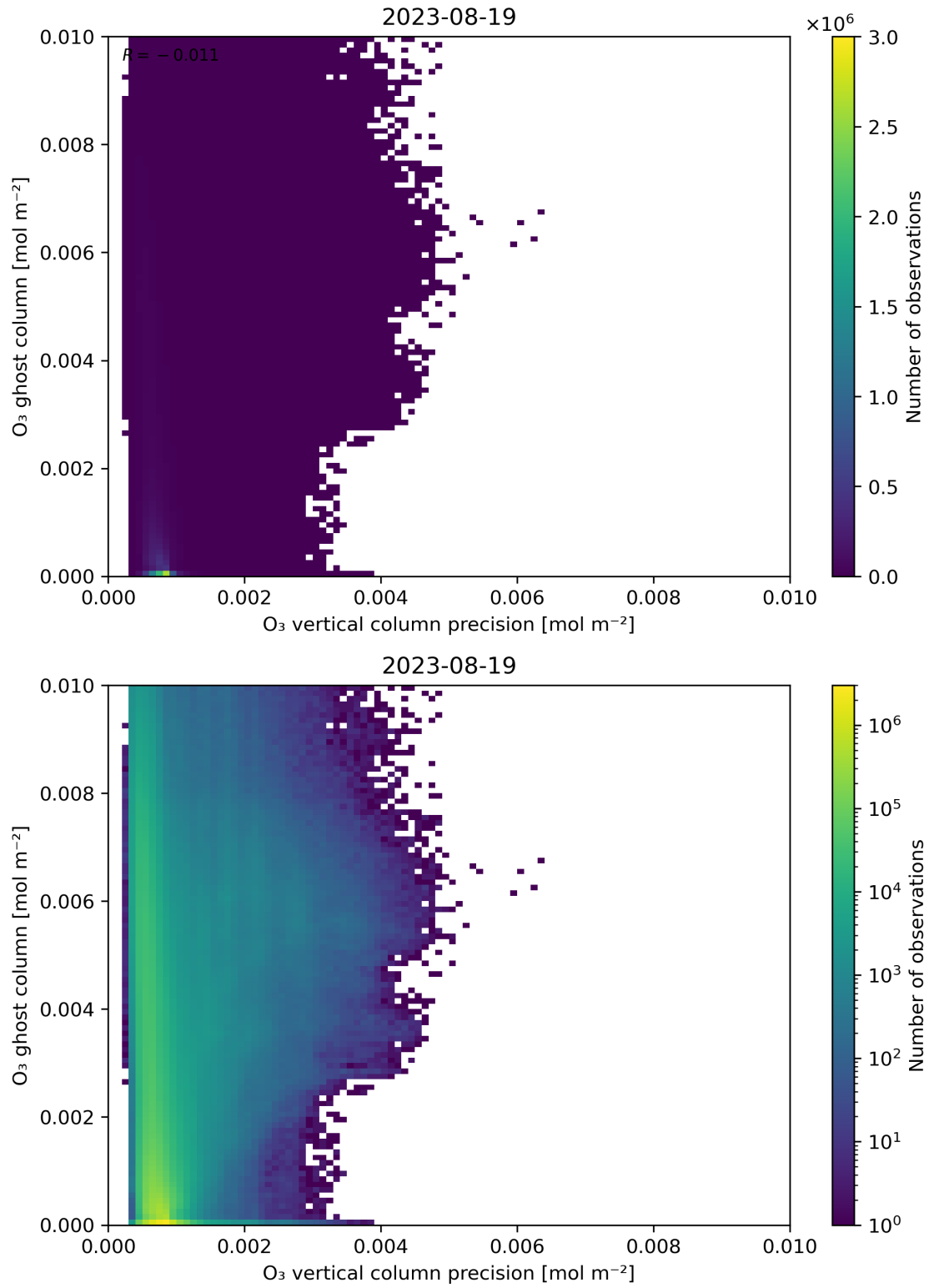
Figure 43: Scatter density plot of “ \text{O}_3 vertical column precision” against “ \text{O}_3 ghost column” for 2023-08-18 to 2023-08-20.
