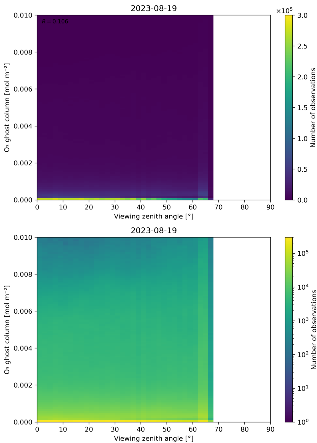
Figure 51: Scatter density plot of “Viewing zenith angle” against “O 3 ghost column” for 2023-08-18 to 2023-08-20.
