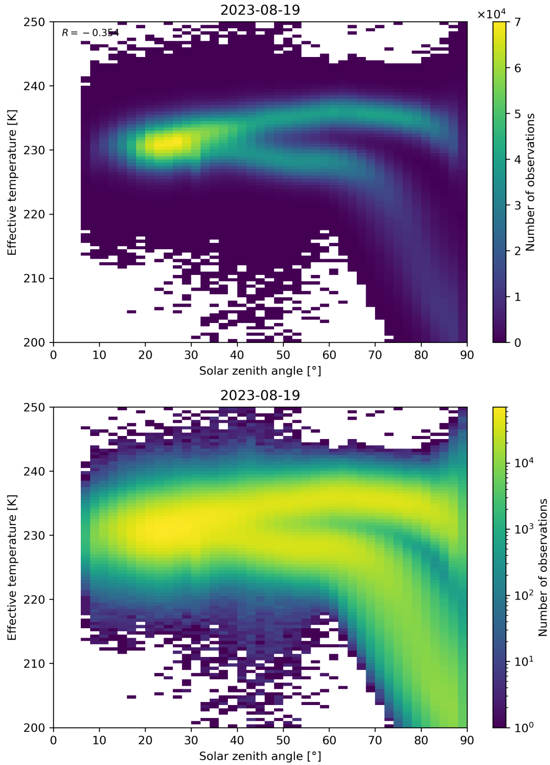
Figure 45: Scatter density plot of “Solar zenith angle” against “Effective temperature” for 2023-08-18 to 2023-08-20.
