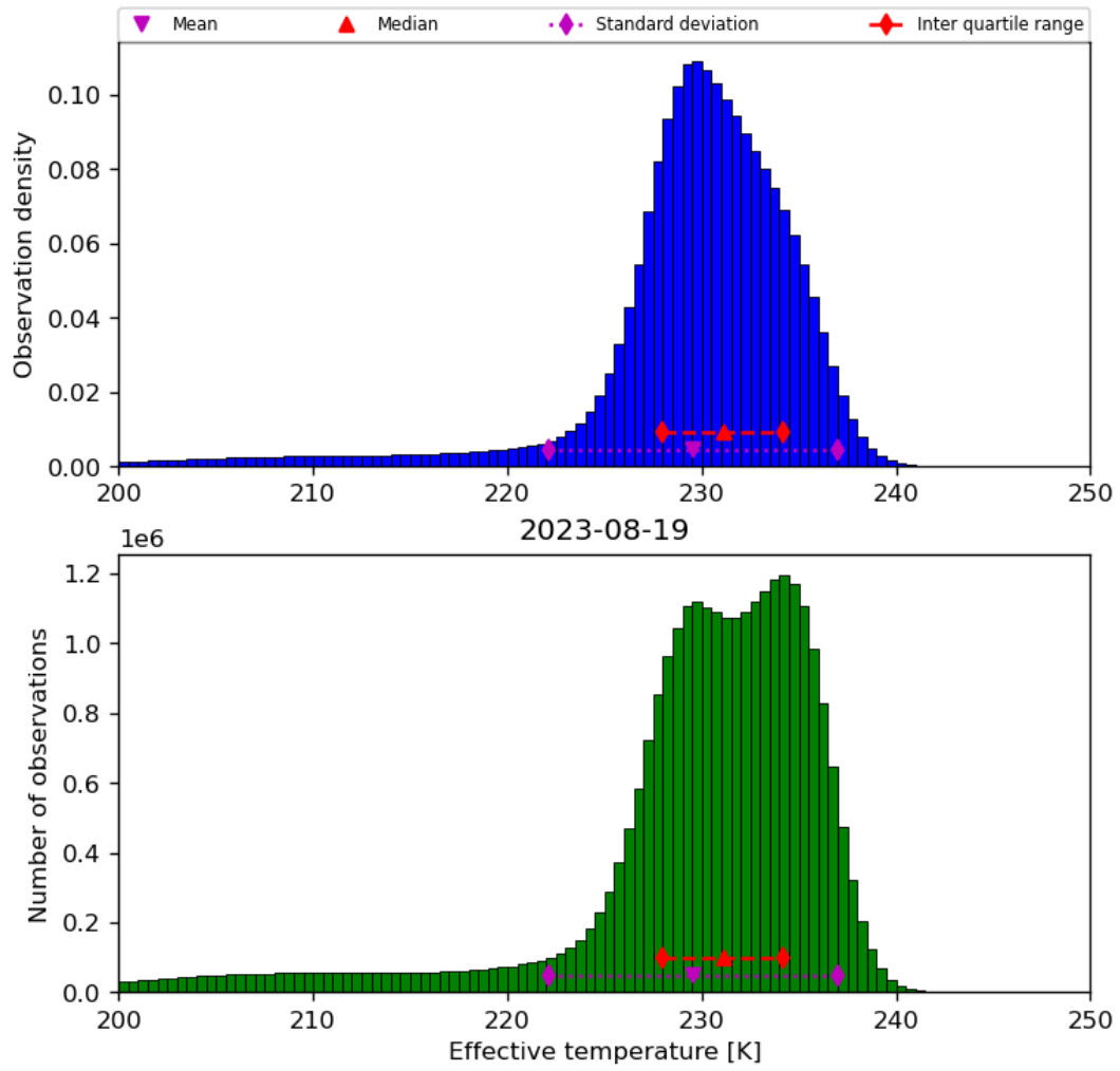
Figure 24: Histogram of “Effective temperature” for 2023-08-18 to 2023-08-20
