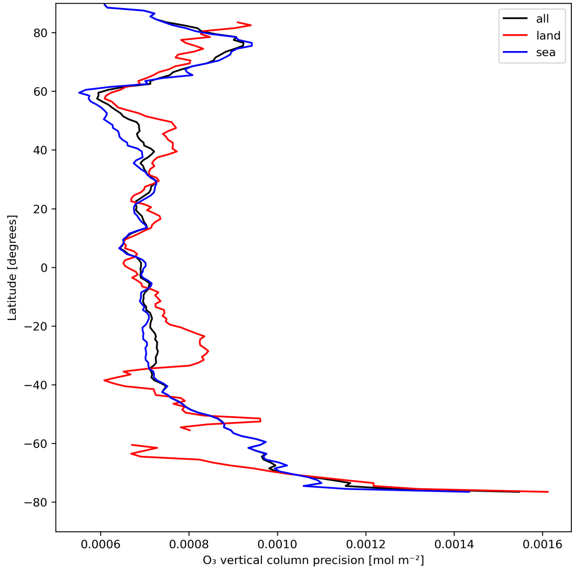
Figure 15: Zonal average of “O 3 vertical column precision” for 2023-08-18 to 2023-08-20.
