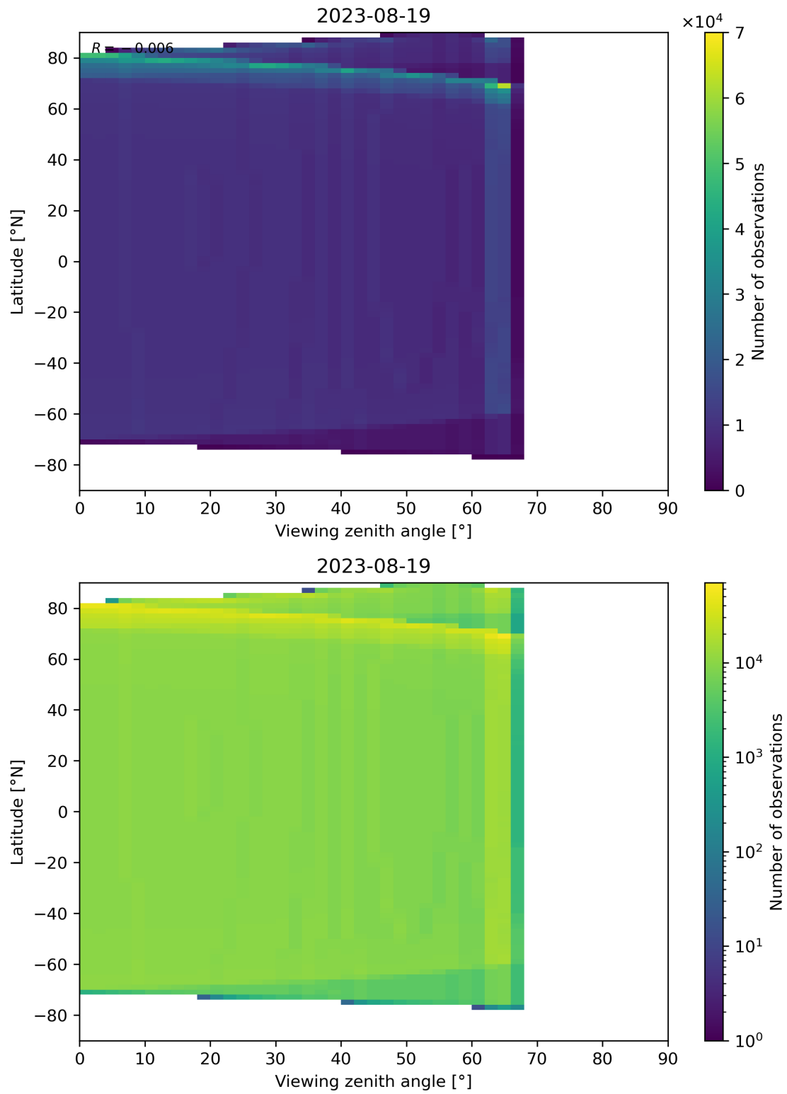
Figure 49: Scatter density plot of “Viewing zenith angle” against “Latitude” for 2023-08-18 to 2023-08-20.
