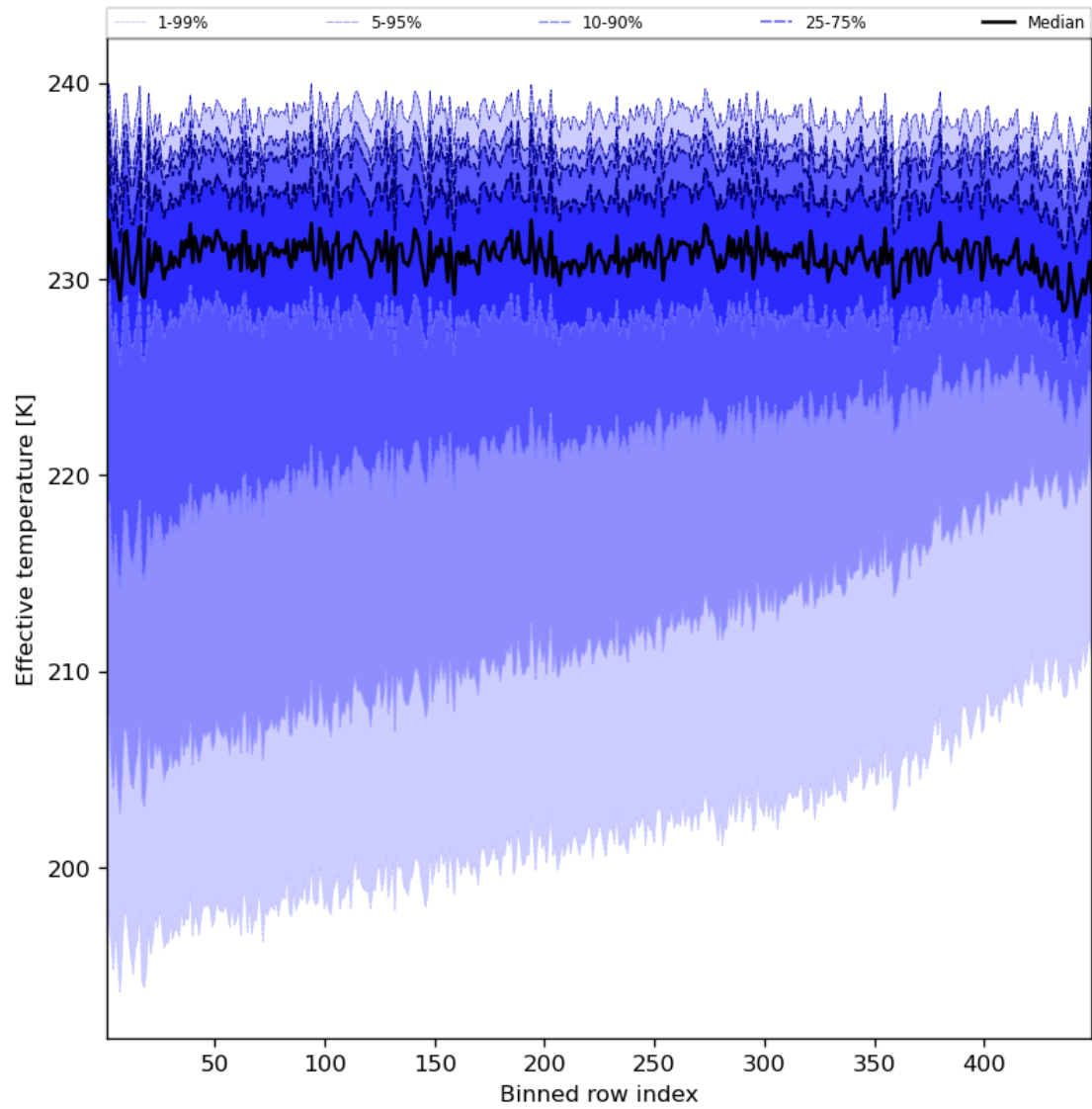
Figure 31: Along track statistics of “Effective temperature” for 2023-08-18 to 2023-08-20
