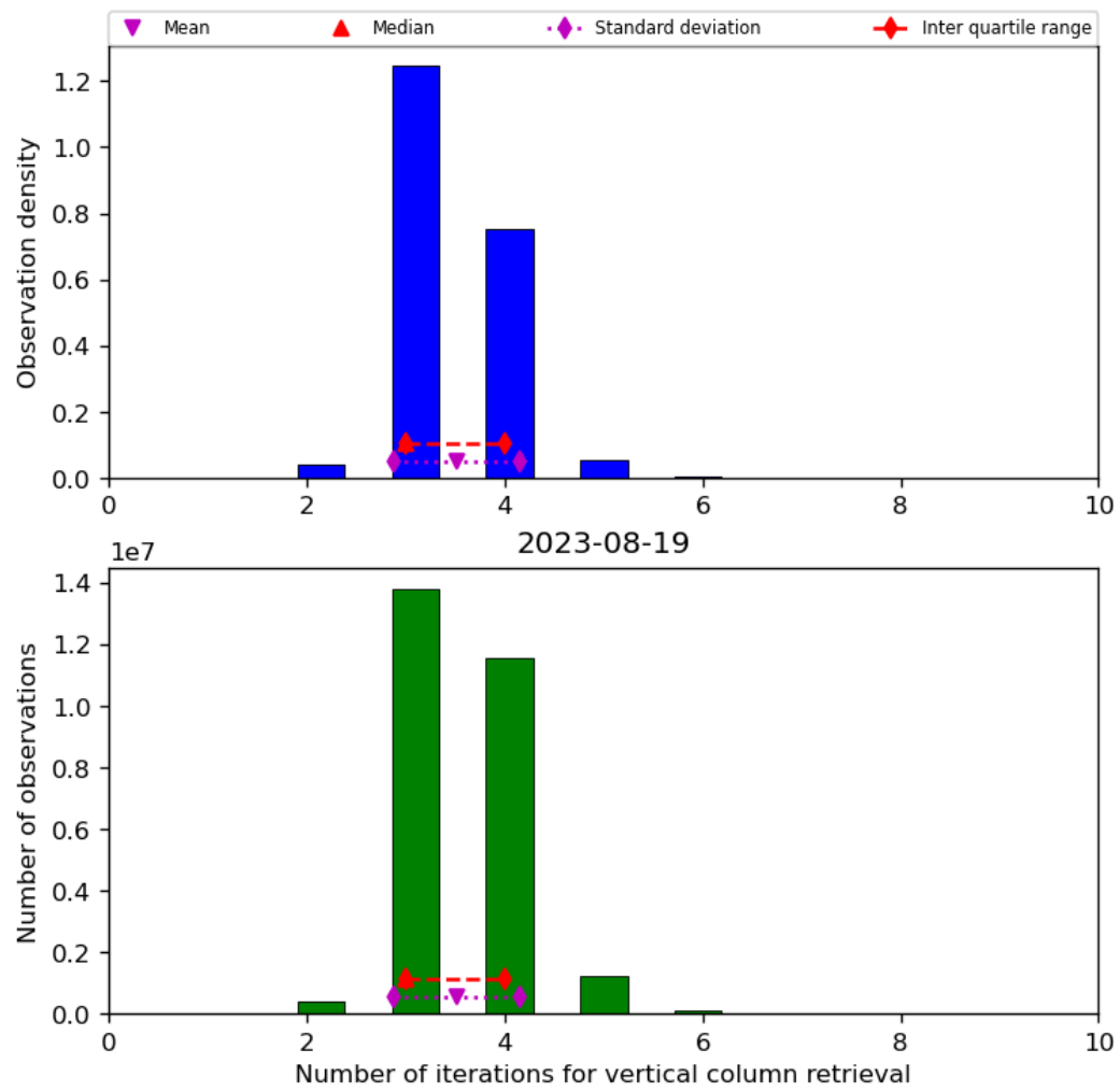
Figure 26: Histogram of “Number of iterations for vertical column retrieval” for 2023-08-18 to 2023-08-20
