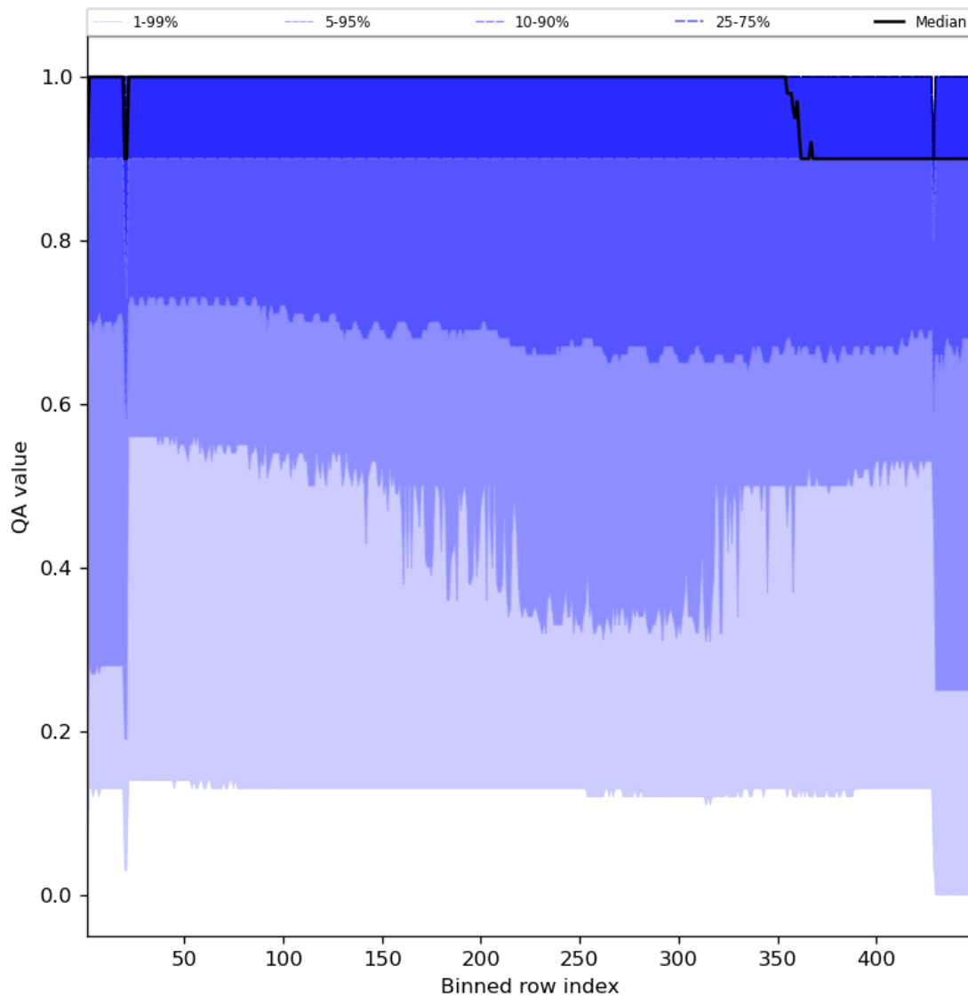
Figure 27: Along track statistics of “QA value” for 2023-08-18 to 2023-08-20
