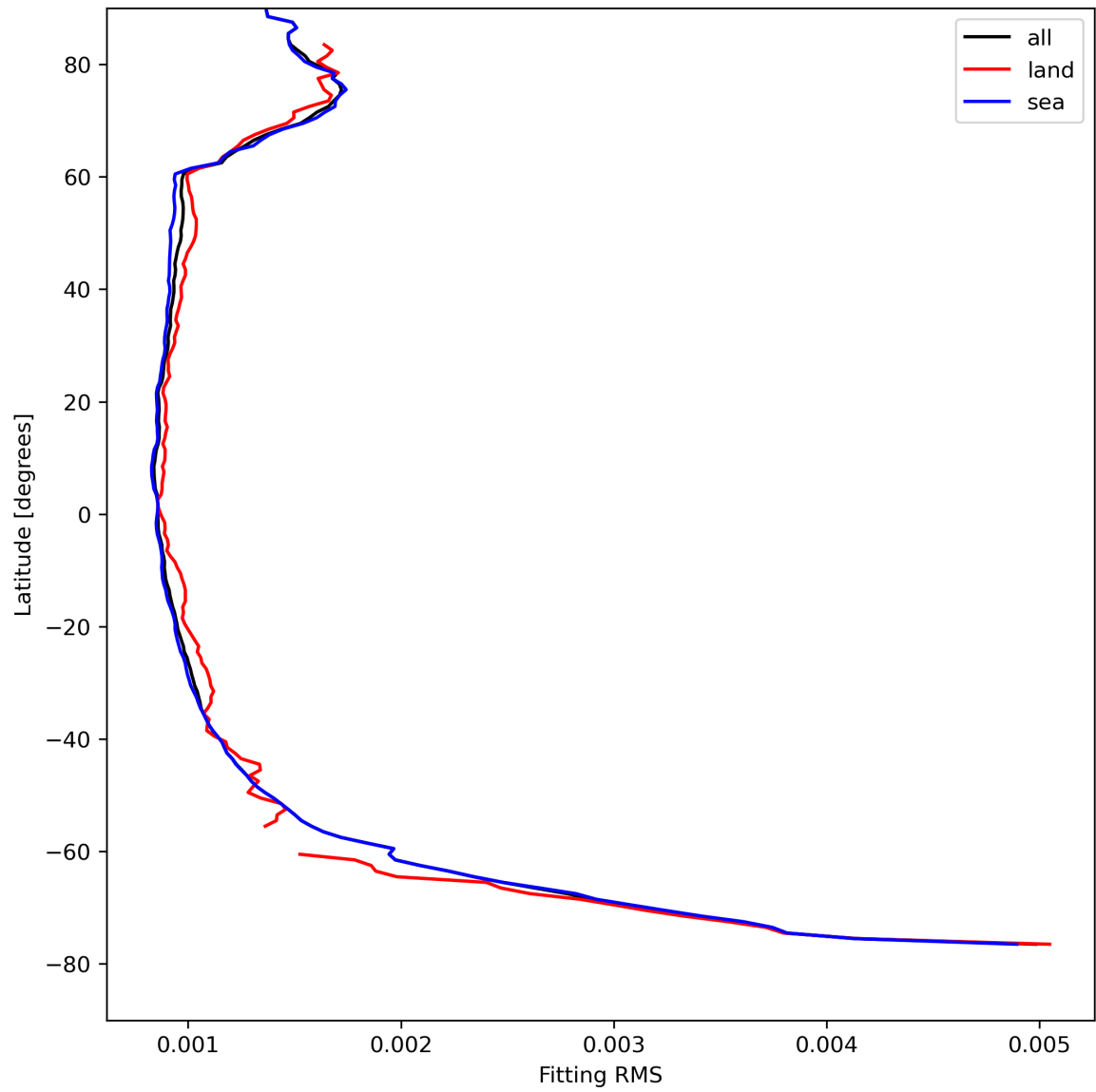
Figure 16: Zonal average of “Fitting RMS” for 2023-08-18 to 2023-08-20.
