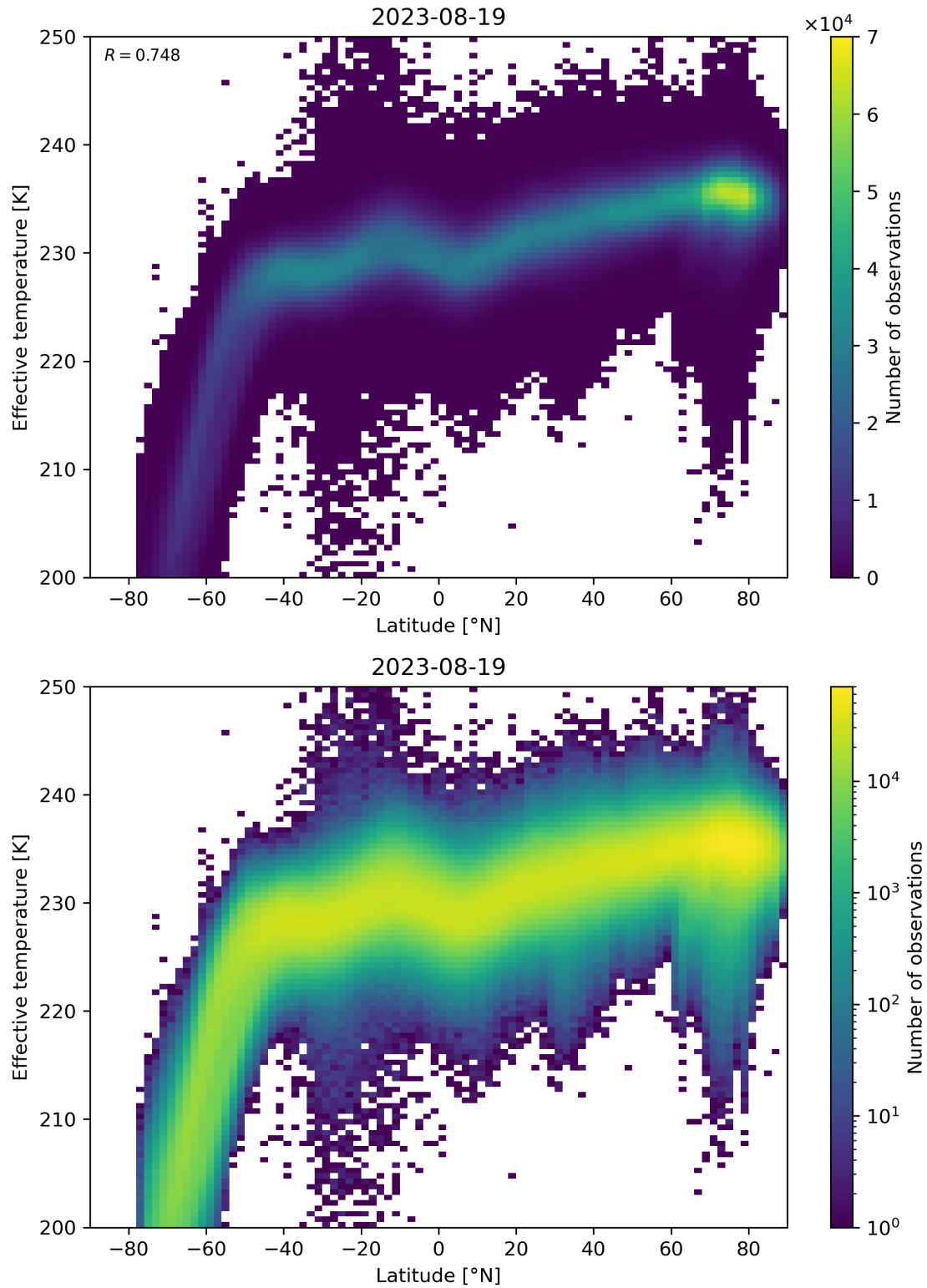
Figure 34: Scatter density plot of “Latitude” against “Effective temperature” for 2023-08-18 to 2023-08-20.
