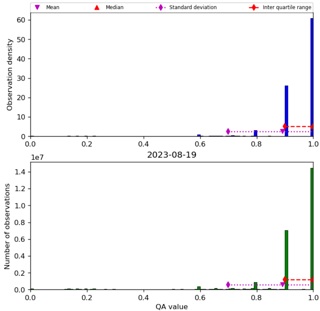
Figure 20: Histogram of “QA value” for 2023-08-18 to 2023-08-20
