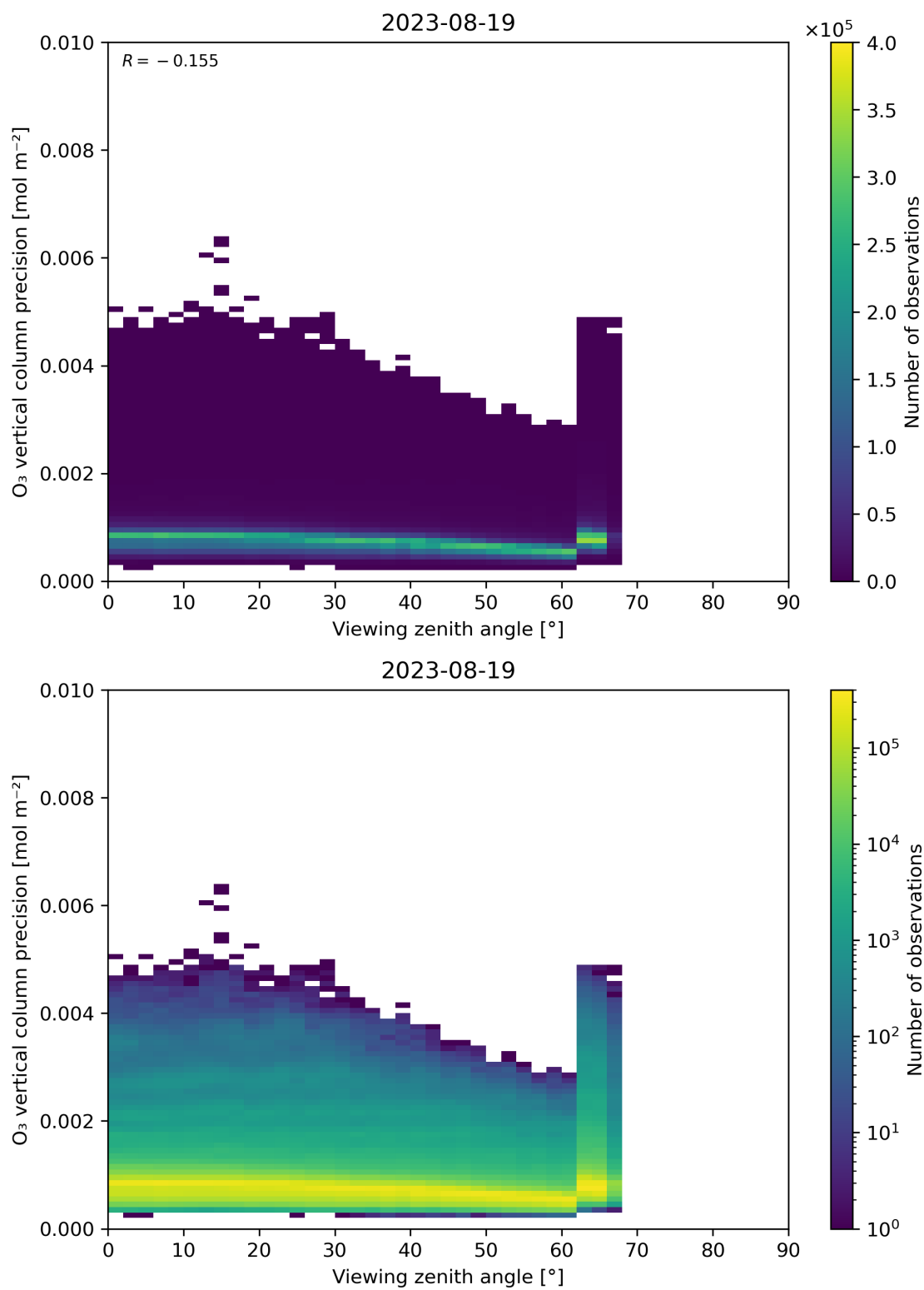
Figure 53: Scatter density plot of “Viewing zenith angle” against “O 3 vertical column precision” for 2023-08-18 to 2023-08-20.
