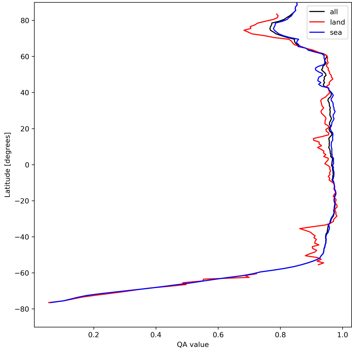
Figure 13: Zonal average of “QA value” for 2023-08-18 to 2023-08-20.
