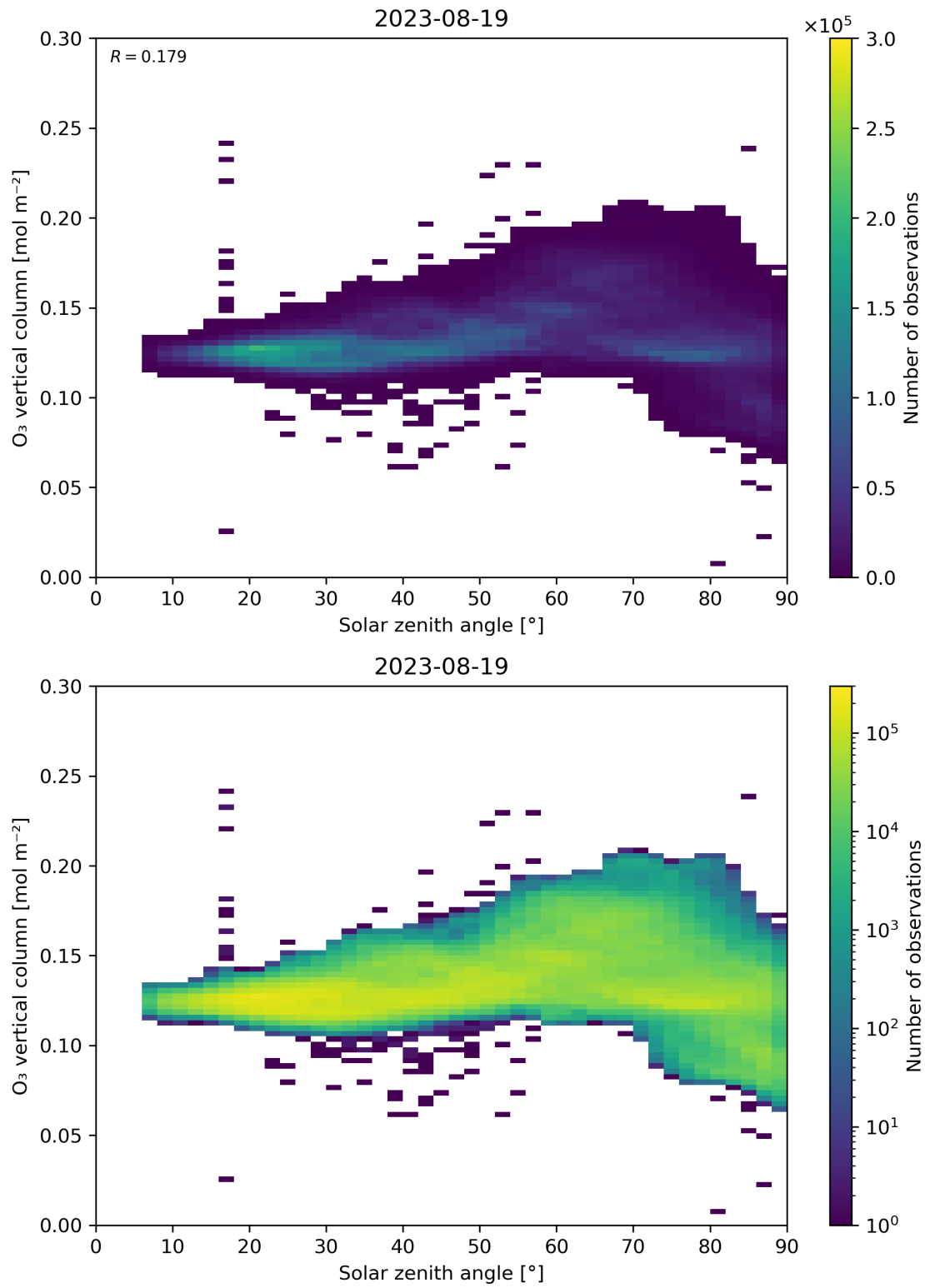
Figure 47: Scatter density plot of “Solar zenith angle” against “O 3 vertical column” for 2023-08-18 to 2023-08-20.
