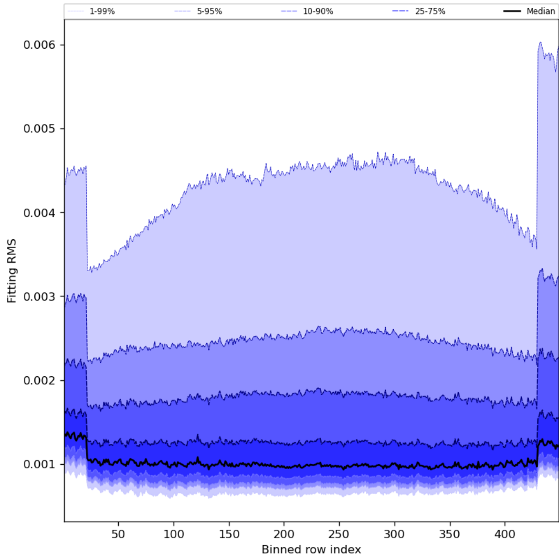
Figure 30: Along track statistics of “Fitting RMS” for 2023-08-18 to 2023-08-20
