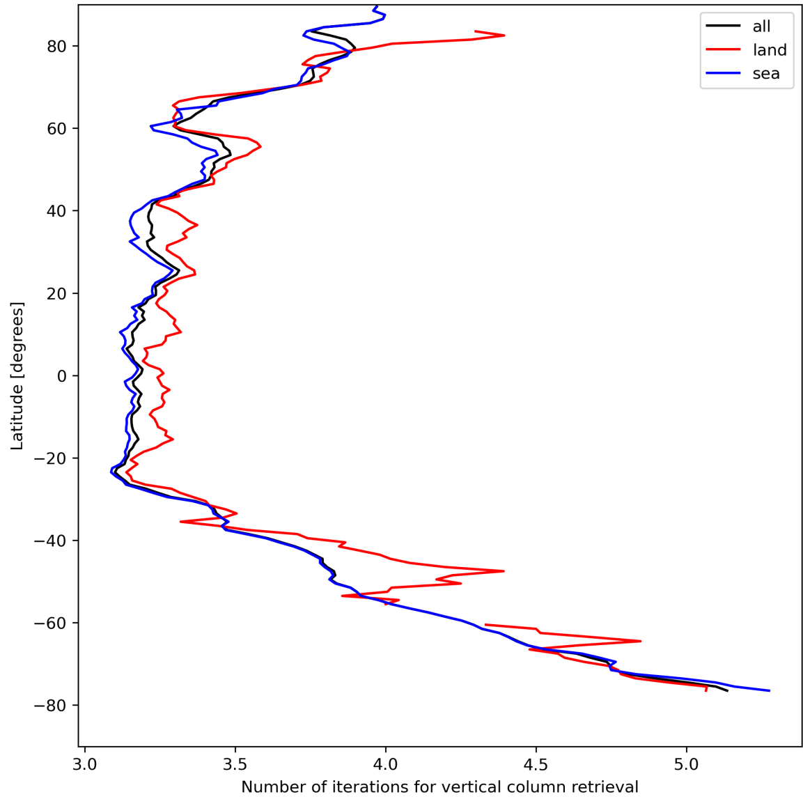
Figure 19: Zonal average of “Number of iterations for vertical column retrieval” for 2023-08-18 to 2023-08-20.
