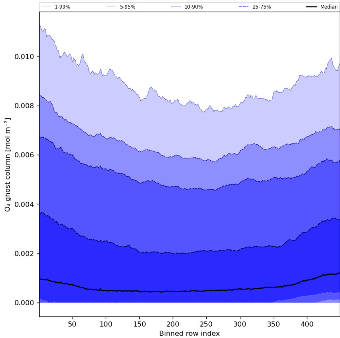
Figure 32: Along track statistics of “O 3 ghost column” for 2023-08-18 to 2023-08-20
