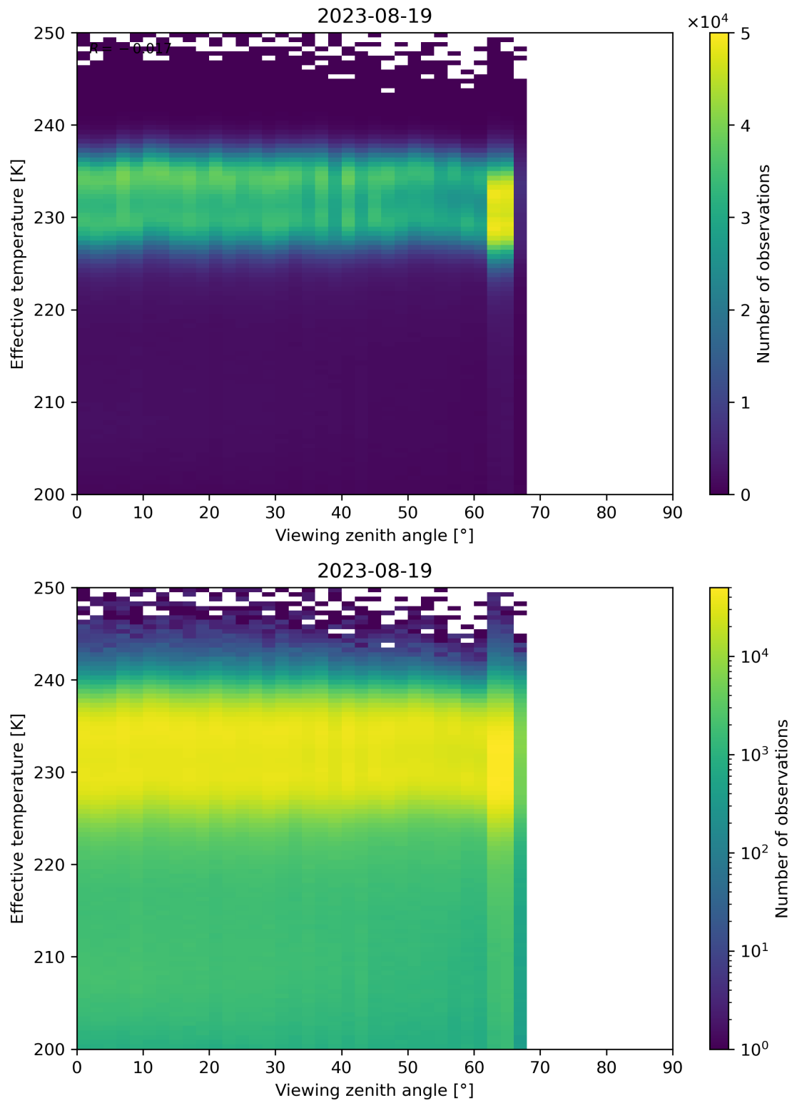
Figure 50: Scatter density plot of “Viewing zenith angle” against “Effective temperature” for 2023-08-18 to 2023-08-20.
