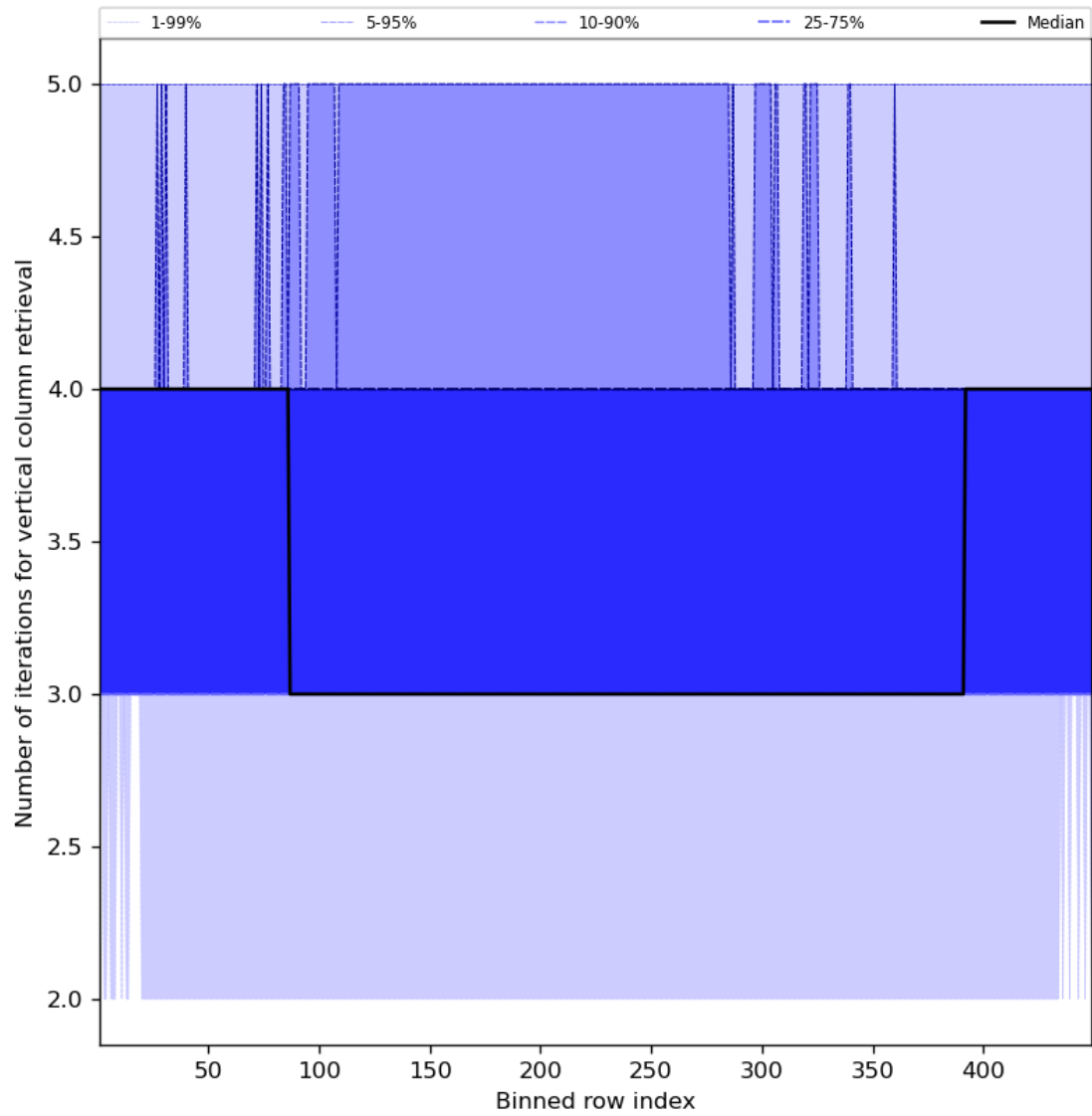
Figure 33: Along track statistics of “Number of iterations for vertical column retrieval” for 2023-08-18 to 2023-08-20
