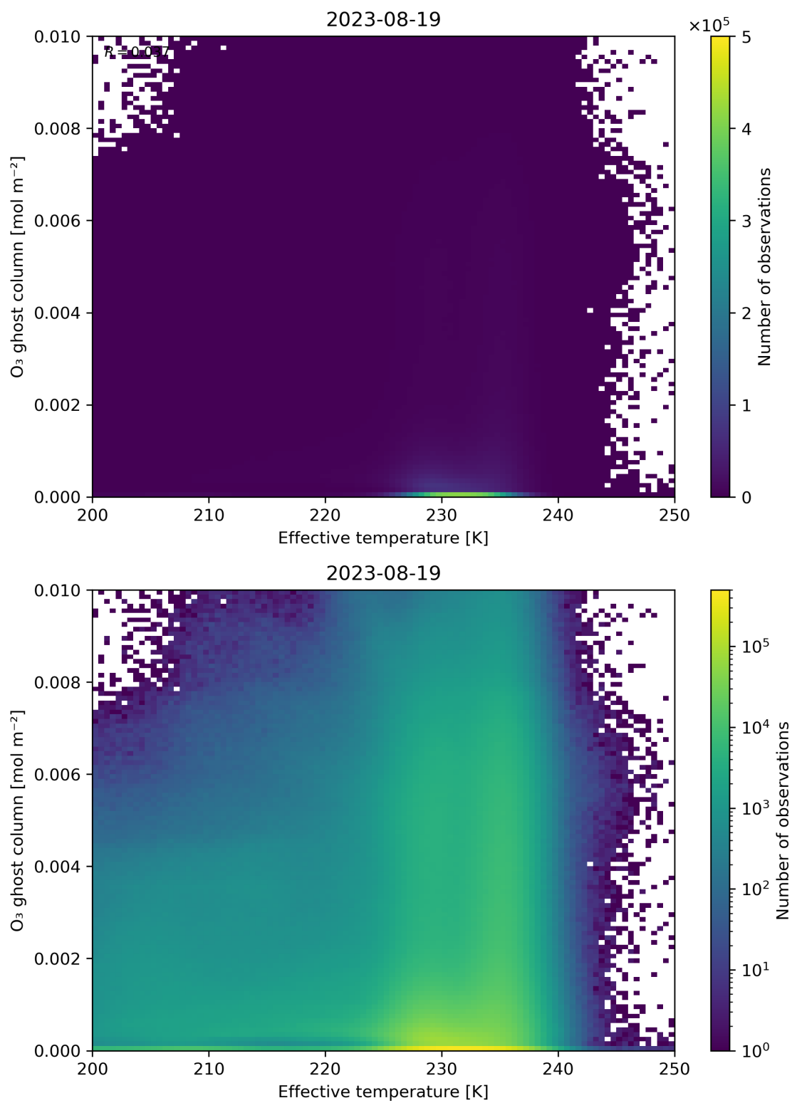
Figure 38: Scatter density plot of “Effective temperature” against “O 3 ghost column” for 2023-08-18 to 2023-08-20.
