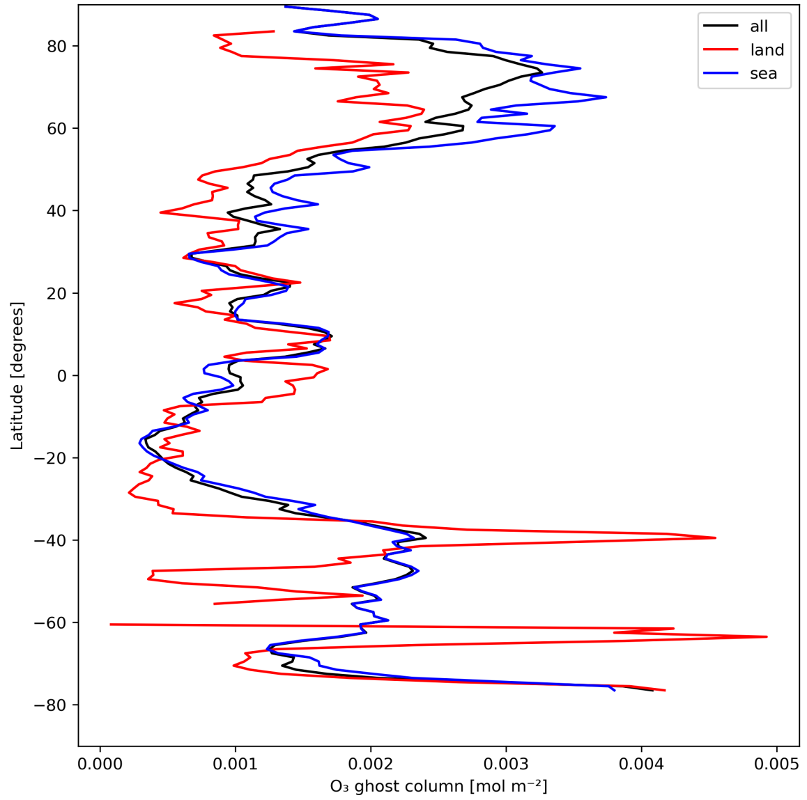
Figure 18: Zonal average of "O 3 ghost column" for 2023-08-18 to 2023-08-20.
