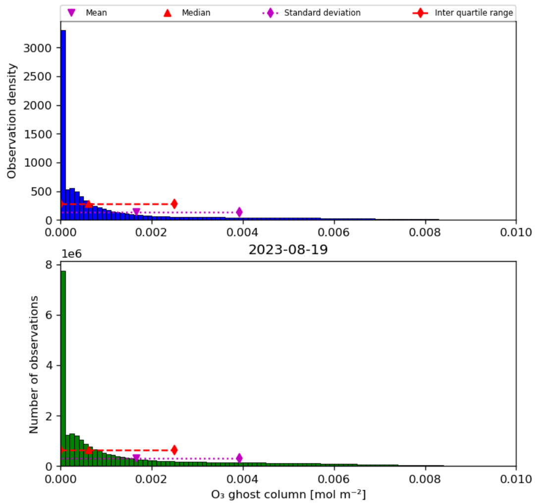
Figure 25: Histogram of “O 3 ghost column” for 2023-08-18 to 2023-08-20
