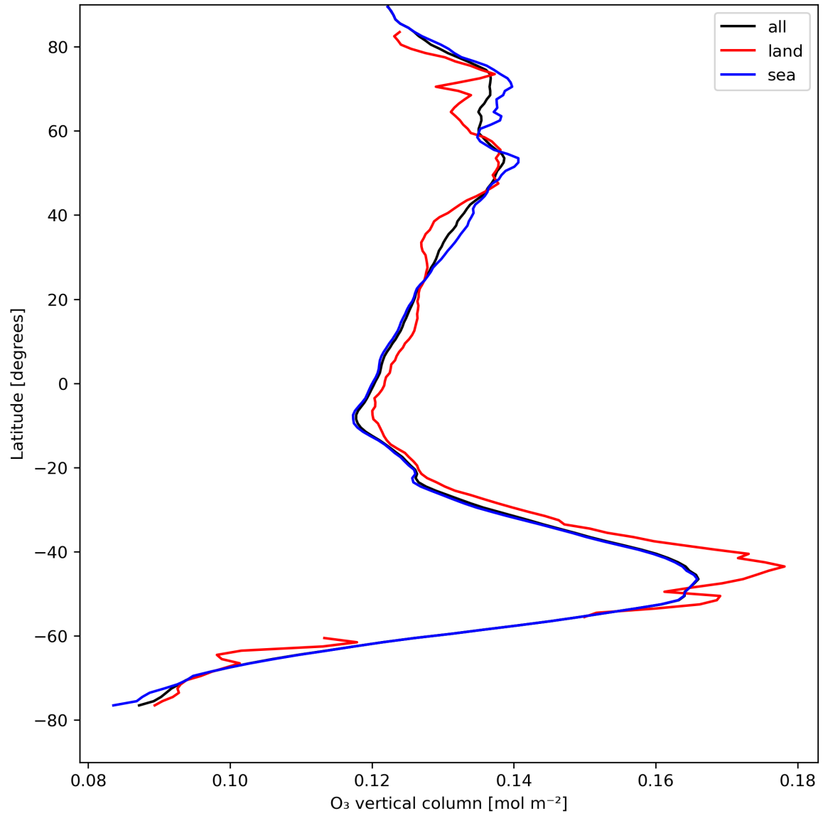
Figure 14: Zonal average of “O 3 vertical column” for 2023-08-18 to 2023-08-20.
