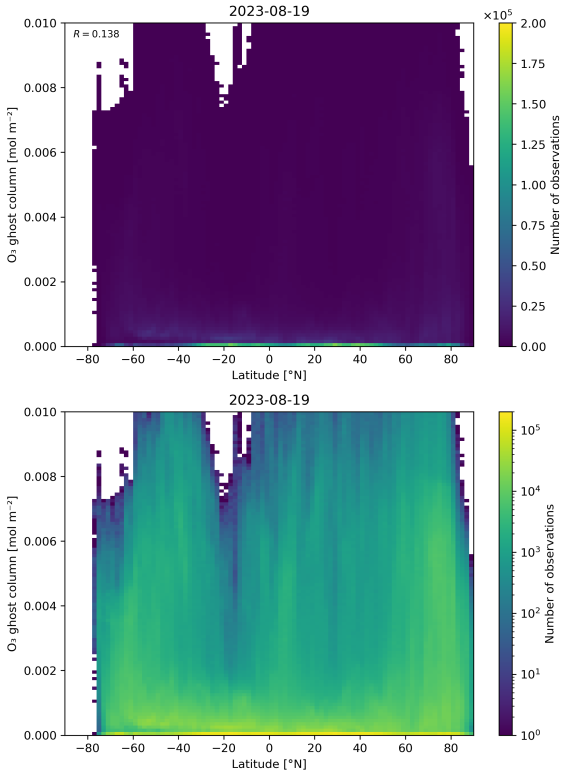
Figure 35: Scatter density plot of “Latitude” against “O 3 ghost column” for 2023-08-18 to 2023-08-20.
