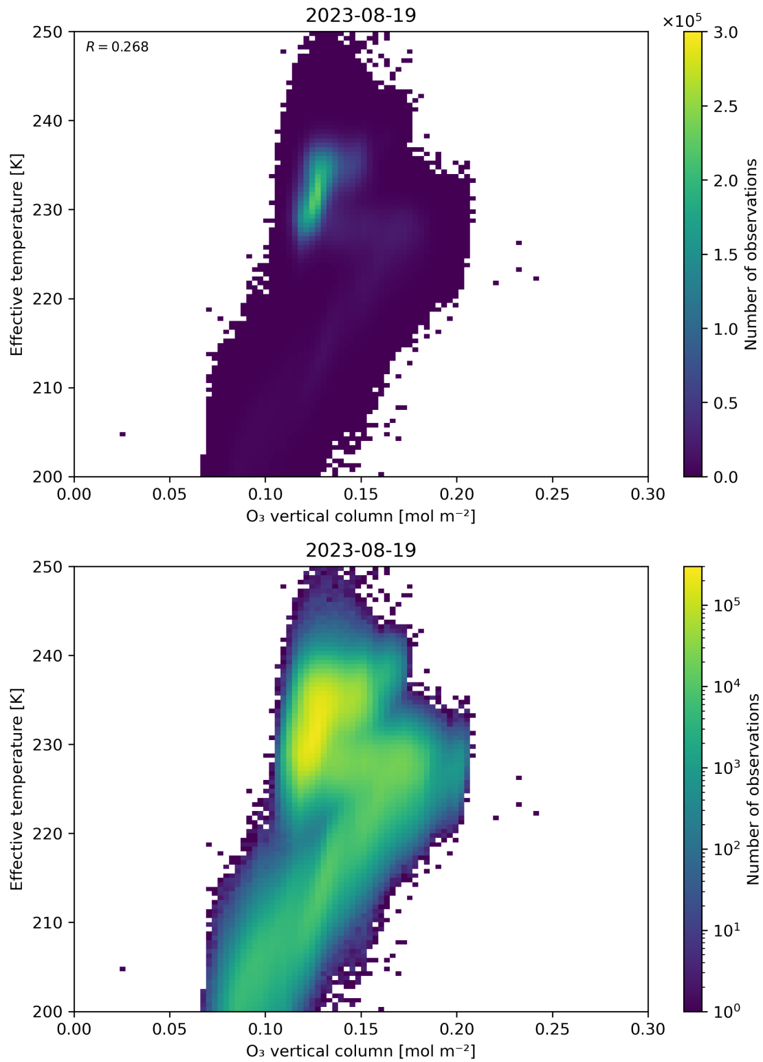
Figure 39: Scatter density plot of “O 3 vertical column” against “Effective temperature” for 2023-08-18 to 2023-08-20.
