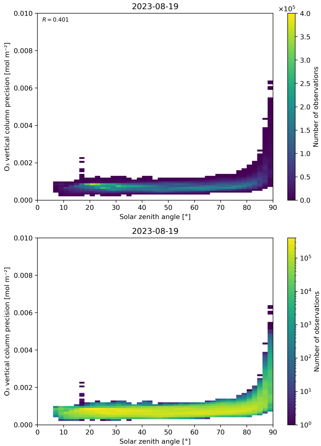
Figure 48: Scatter density plot of “Solar zenith angle” against “O 3 vertical column precision” for 2023-08-18 to 2023-08-20.
