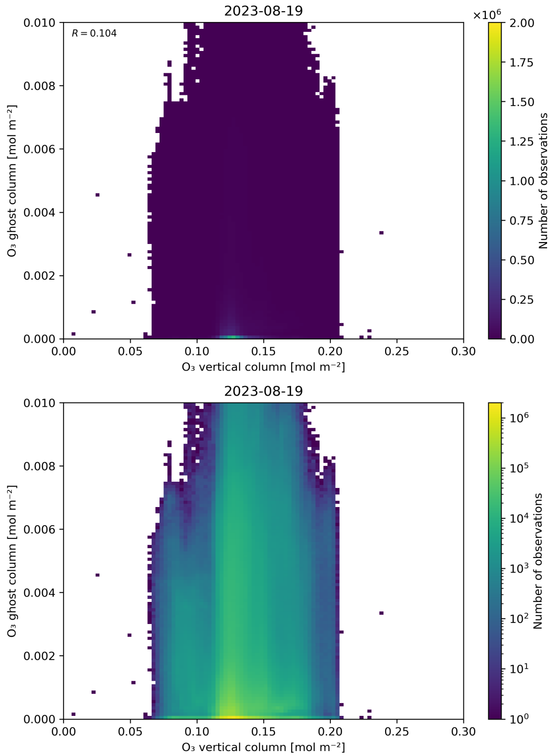
Figure 40: Scatter density plot of “O 3 vertical column” against “O 3 ghost column” for 2023-08-18 to 2023-08-20.
