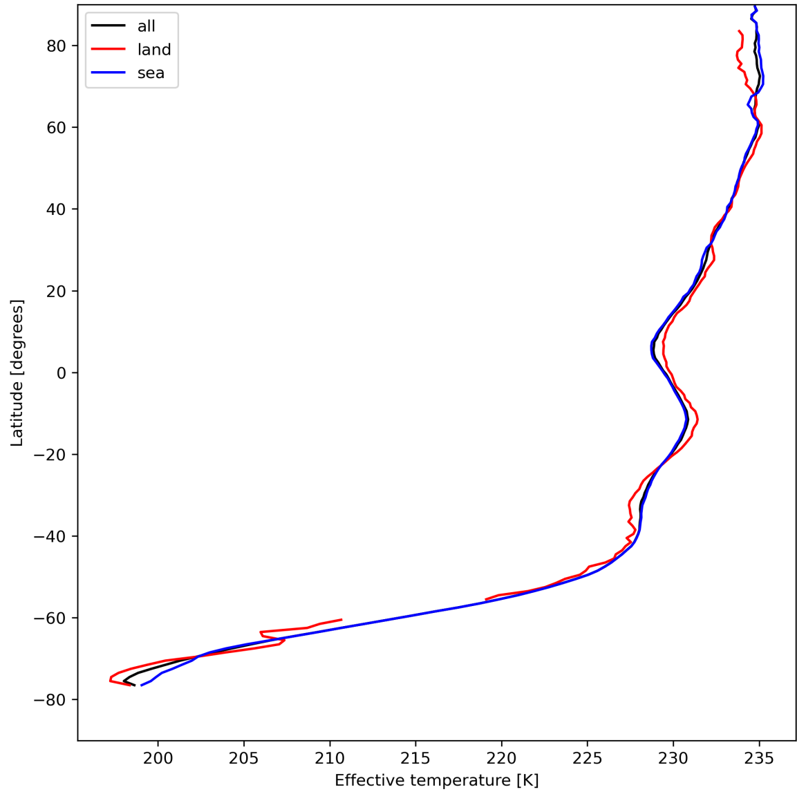
Figure 17: Zonal average of “Effective temperature” for 2023-08-18 to 2023-08-20.
