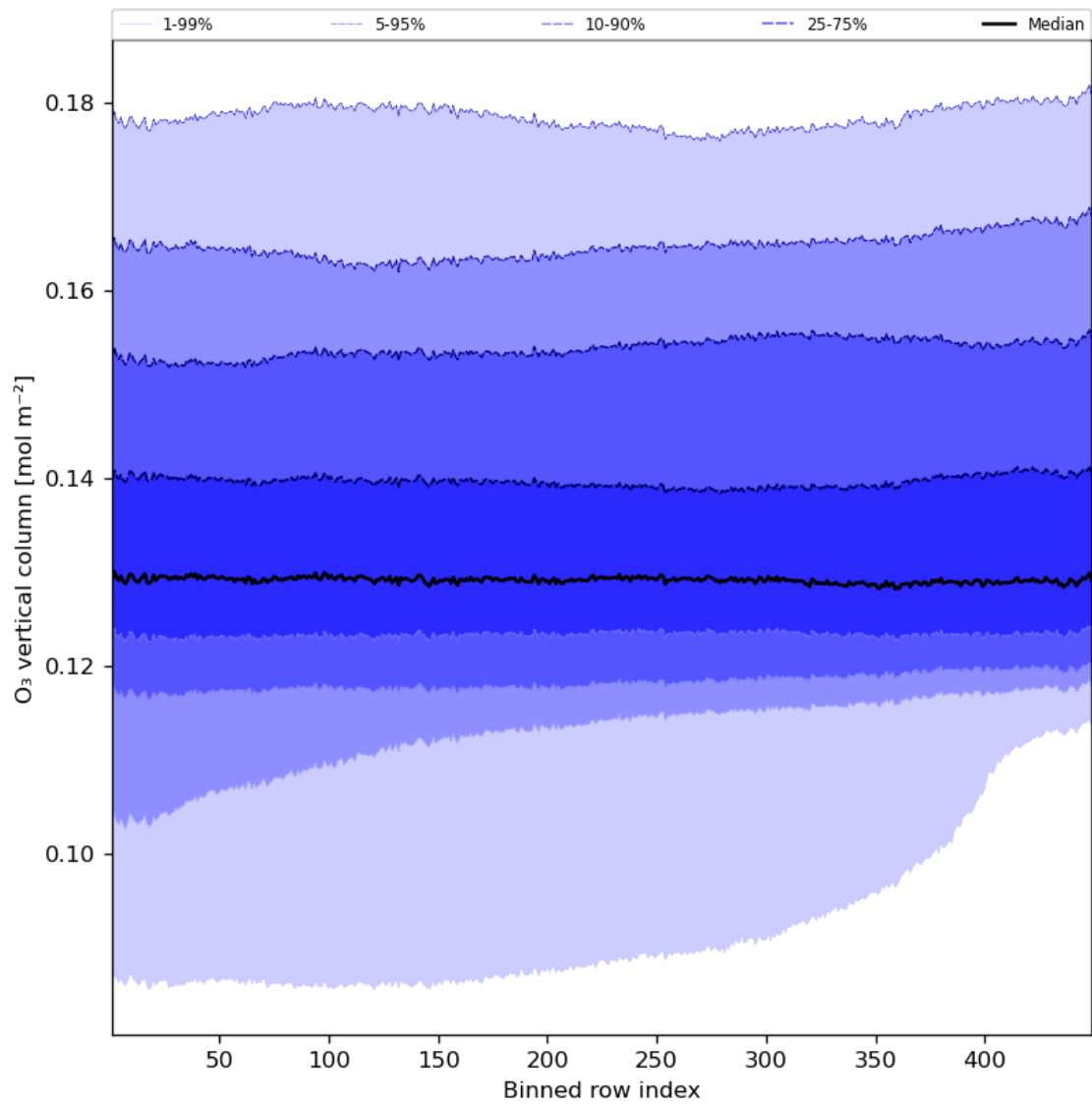
Figure 28: Along track statistics of “O 3 vertical column” for 2023-08-18 to 2023-08-20
