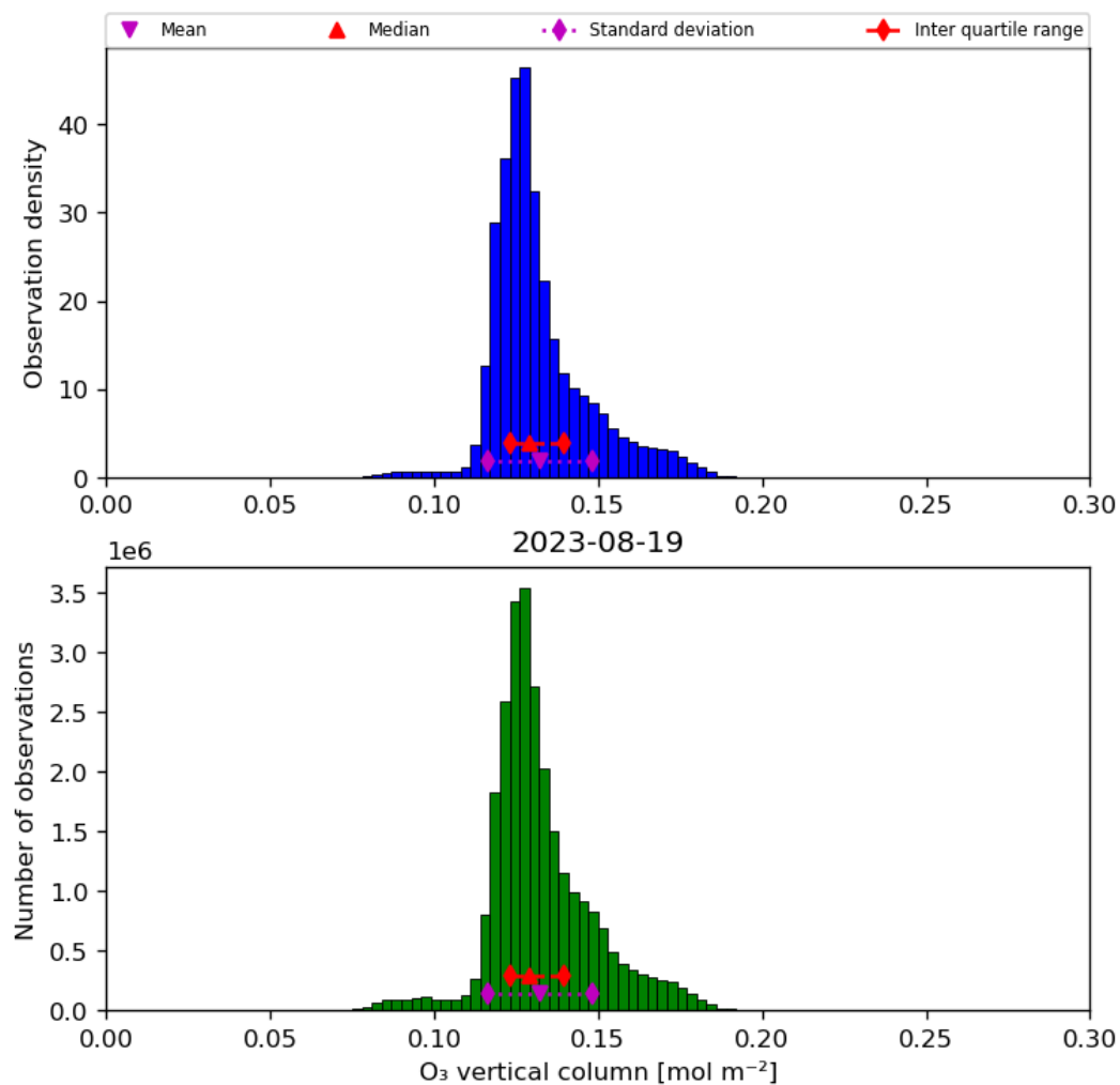
Figure 21: Histogram of “O 3 vertical column” for 2023-08-18 to 2023-08-20
