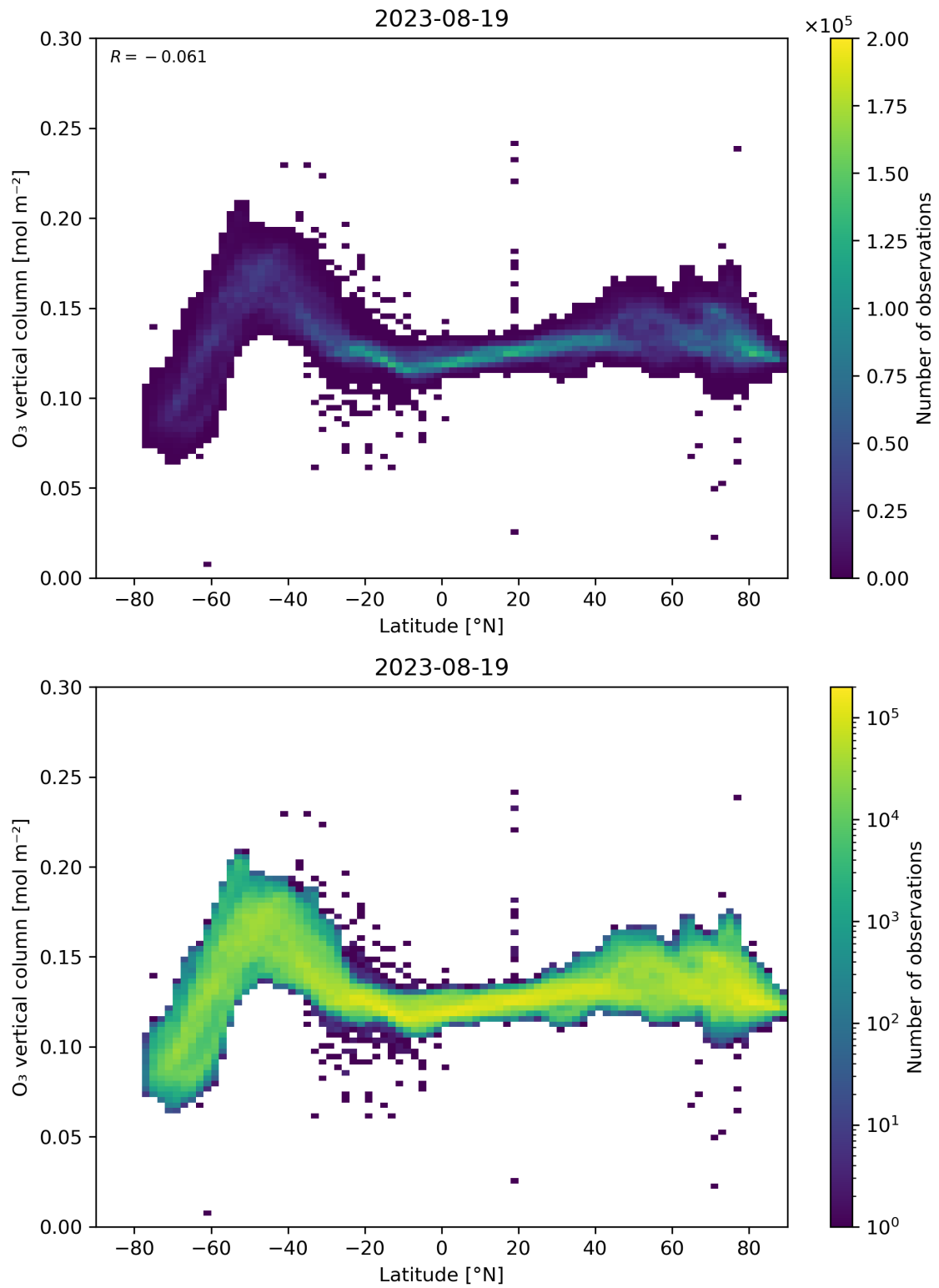
Figure 36: Scatter density plot of “Latitude” against “O 3 vertical column” for 2023-08-18 to 2023-08-20.
