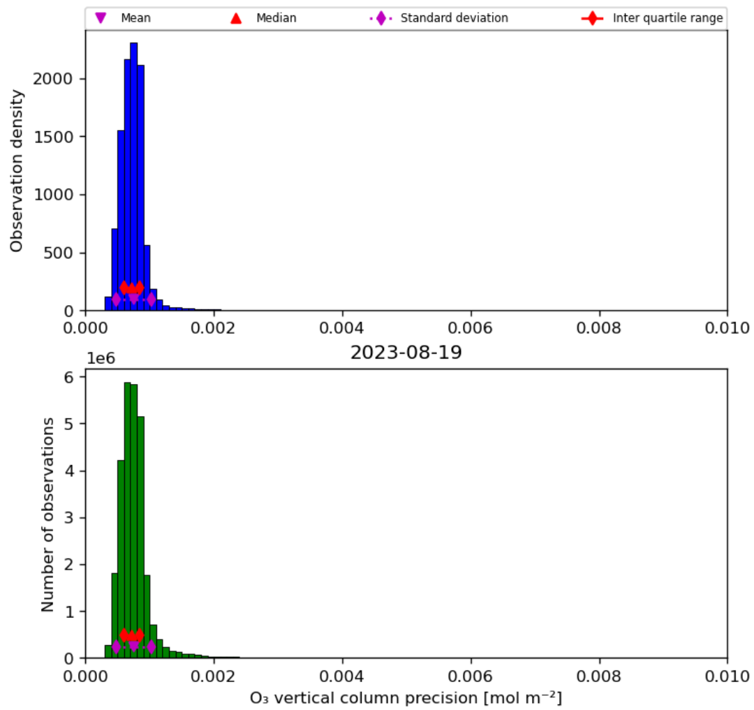
Figure 22: Histogram of “O 3 vertical column precision” for 2023-08-18 to 2023-08-20
