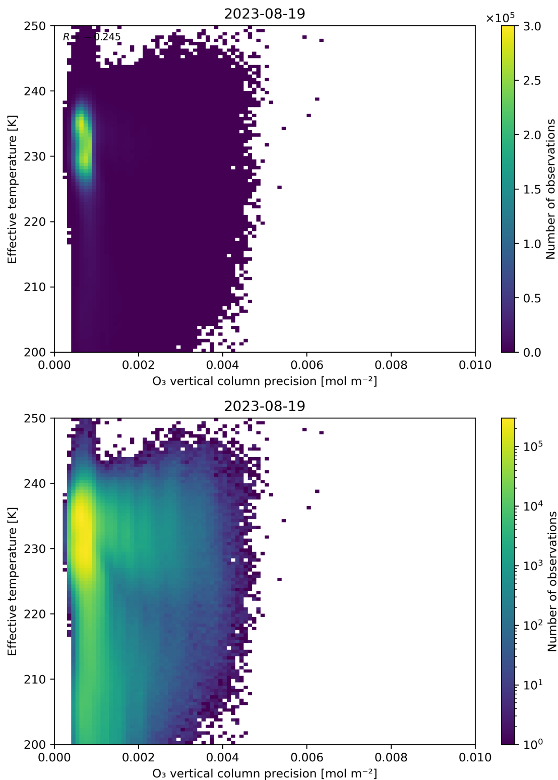
Figure 42: Scatter density plot of “O 3 vertical column precision” against “Effective temperature” for 2023-08-18 to 2023-08-20.
