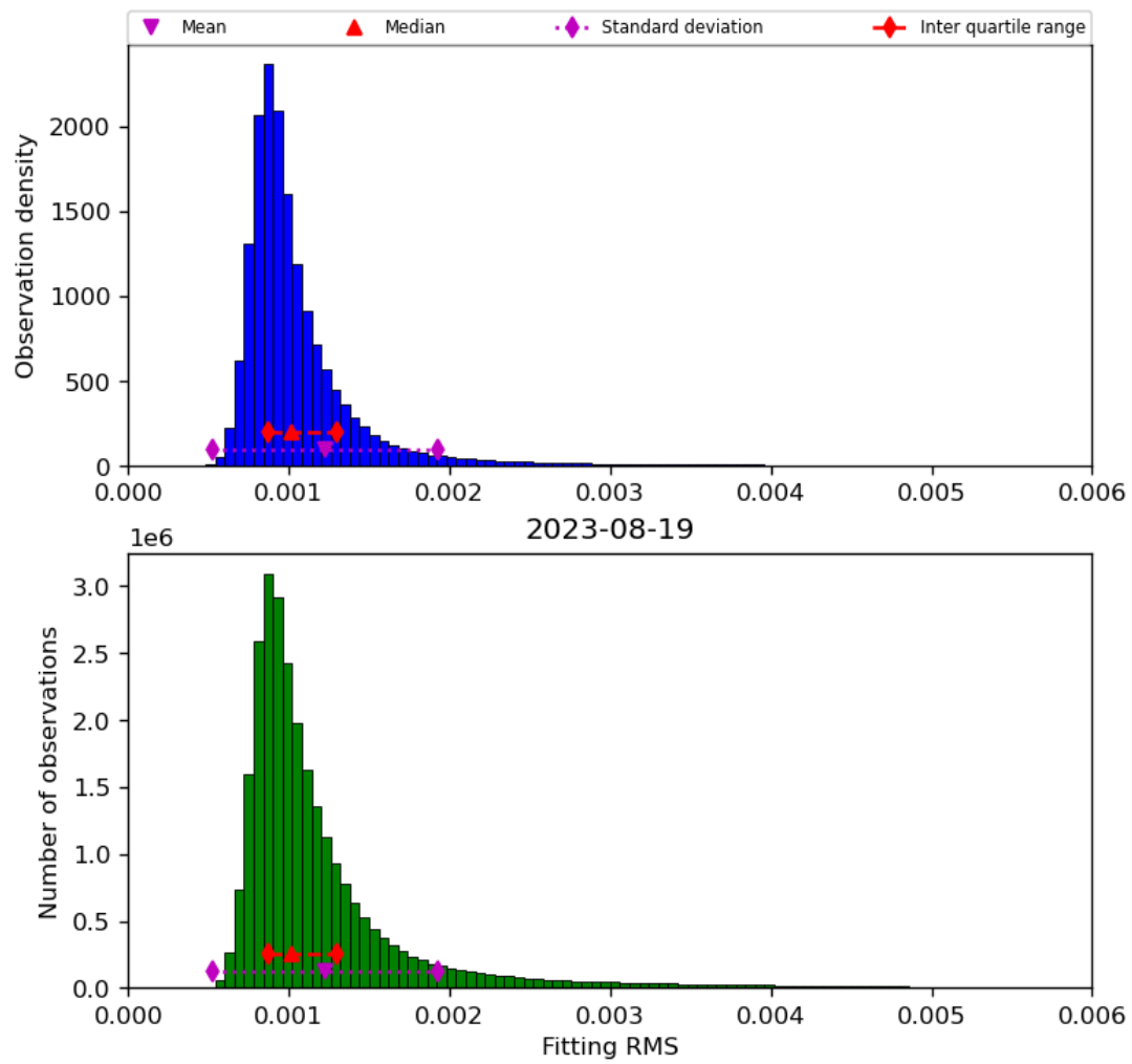
Figure 23: Histogram of “Fitting RMS” for 2023-08-18 to 2023-08-20
