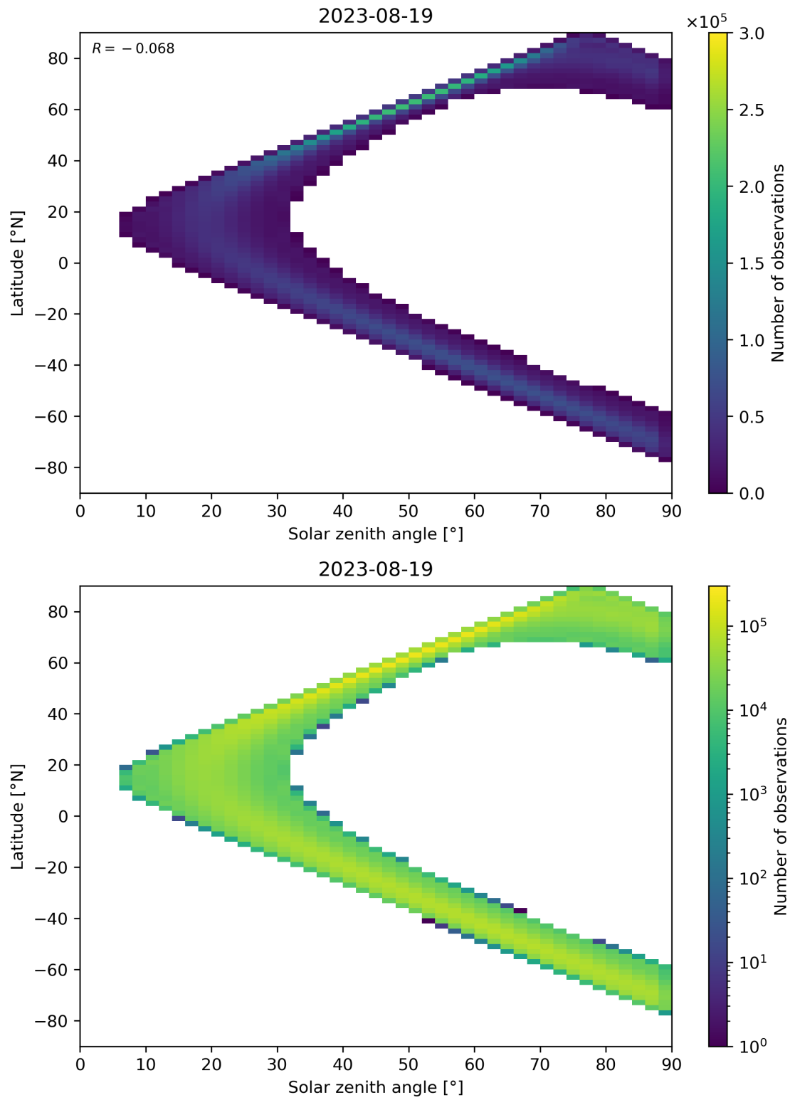
Figure 44: Scatter density plot of “Solar zenith angle” against “Latitude” for 2023-08-18 to 2023-08-20.
