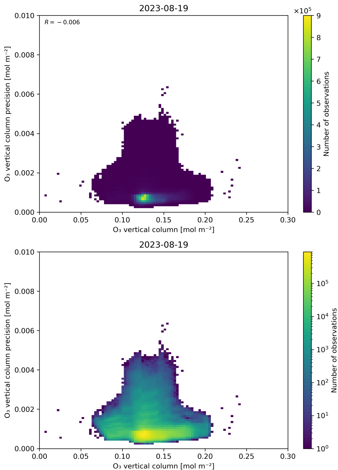
Figure 41: Scatter density plot of “O 3 vertical column” against “O 3 vertical column precision” for 2023-08-18 to 2023-08-20.
