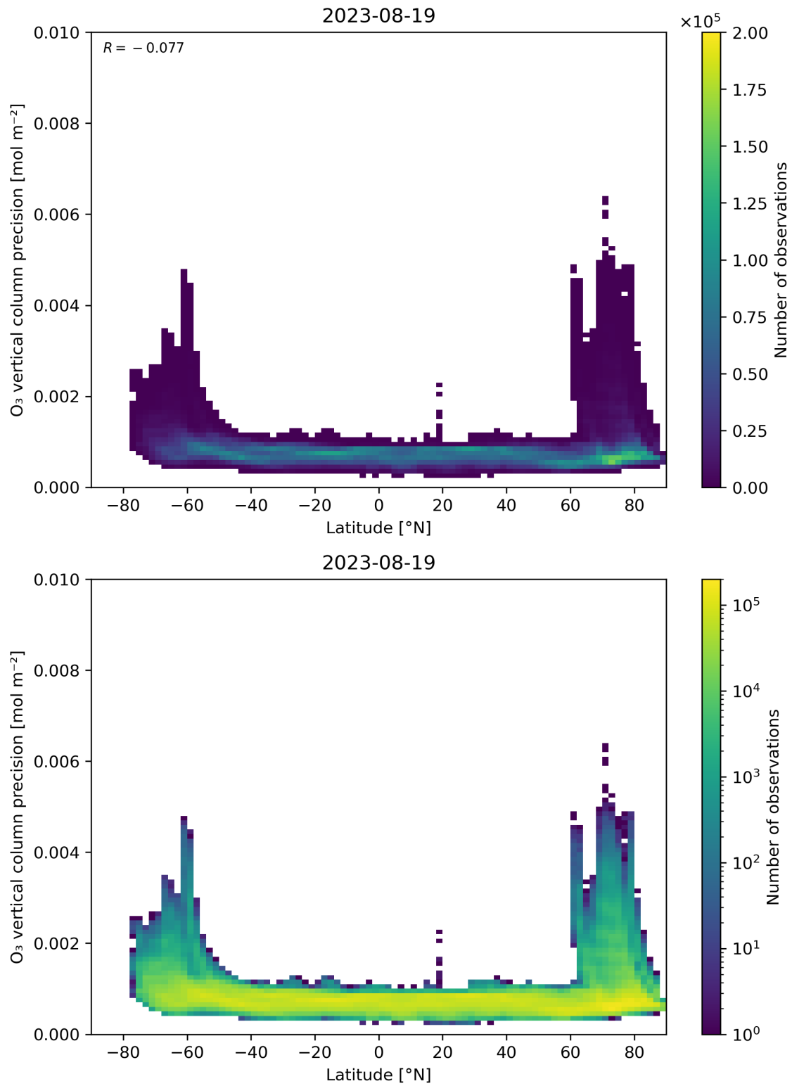
Figure 37: Scatter density plot of “Latitude” against “O 3 vertical column precision” for 2023-08-18 to 2023-08-20.
