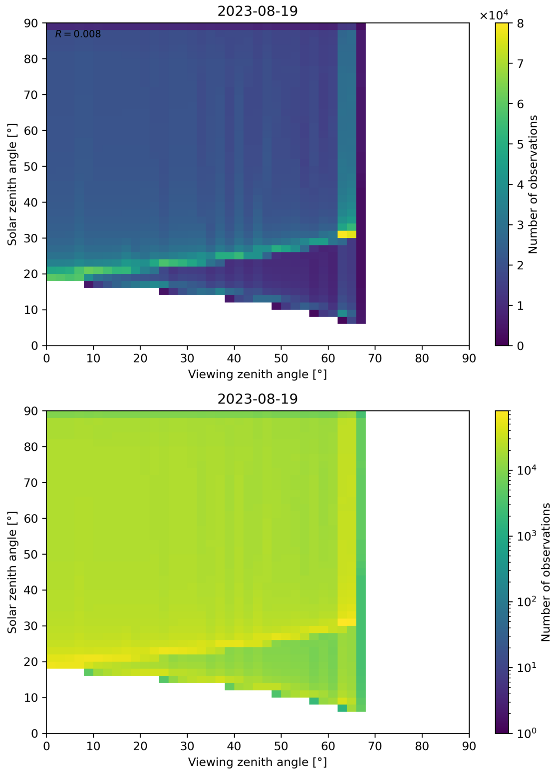
Figure 54: Scatter density plot of “Viewing zenith angle” against “Solar zenith angle” for 2023-08-18 to 2023-08-20.
