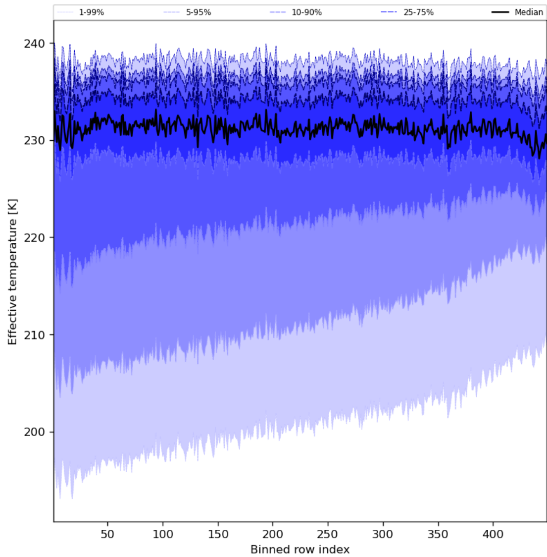
Figure 31: Along track statistics of “Effective temperature” for 2023-08-20 to 2023-08-21
