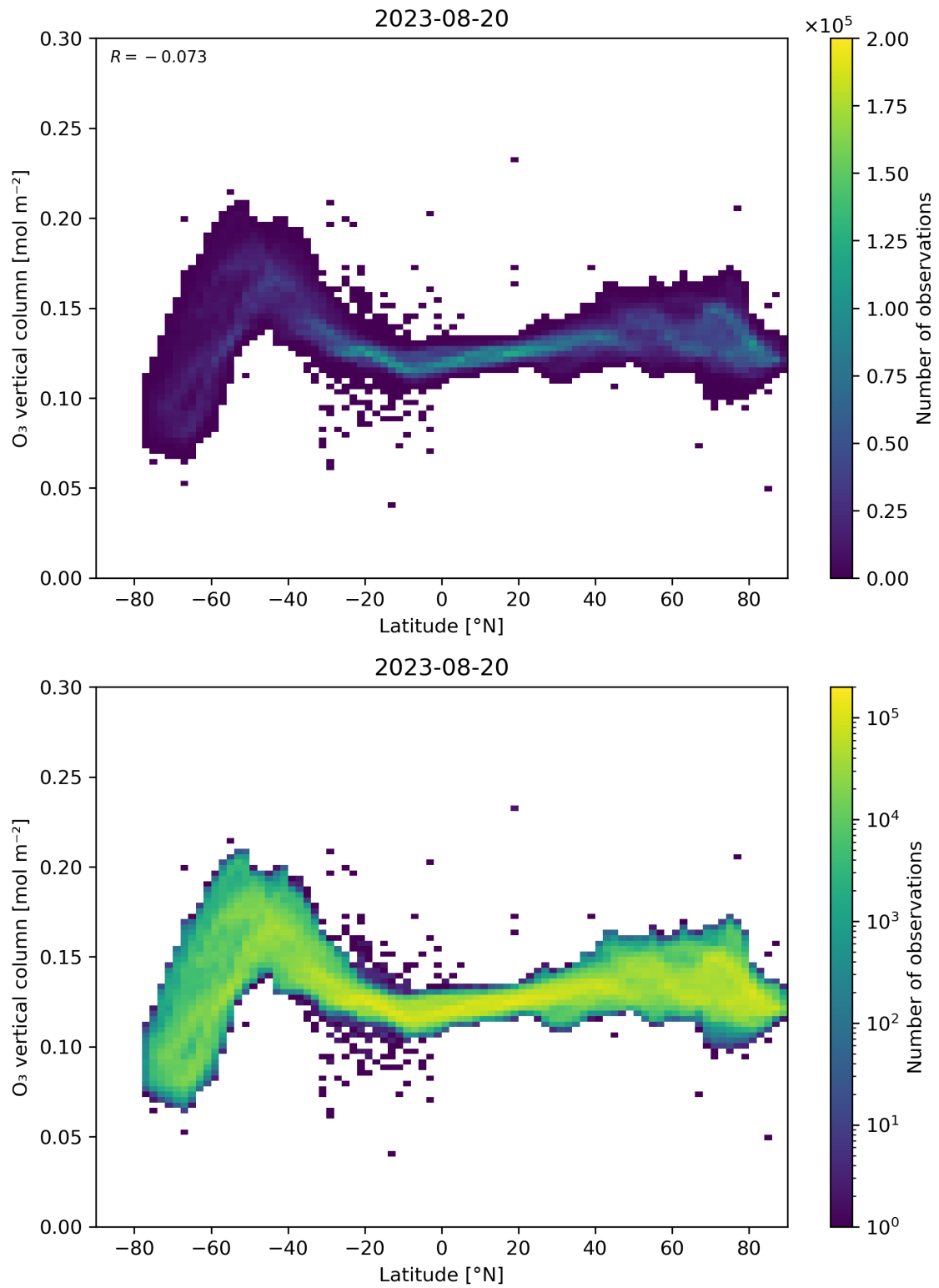
Figure 36: Scatter density plot of “Latitude” against “O 3 vertical column” for 2023-08-20 to 2023-08-21.
