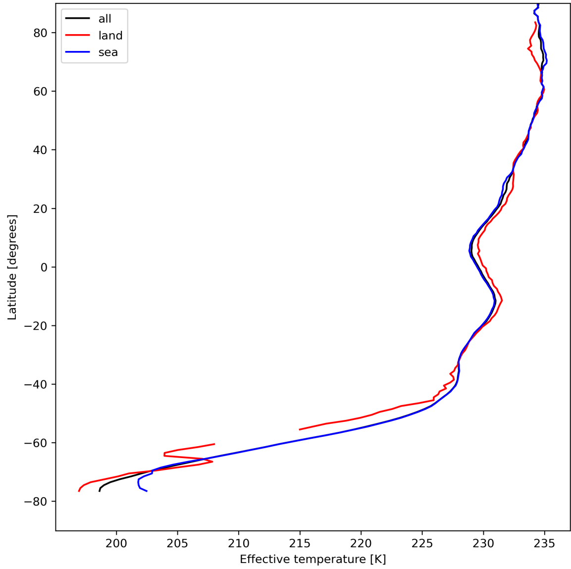
Figure 17: Zonal average of "Effective temperature" for 2023-08-20 to 2023-08-21.
