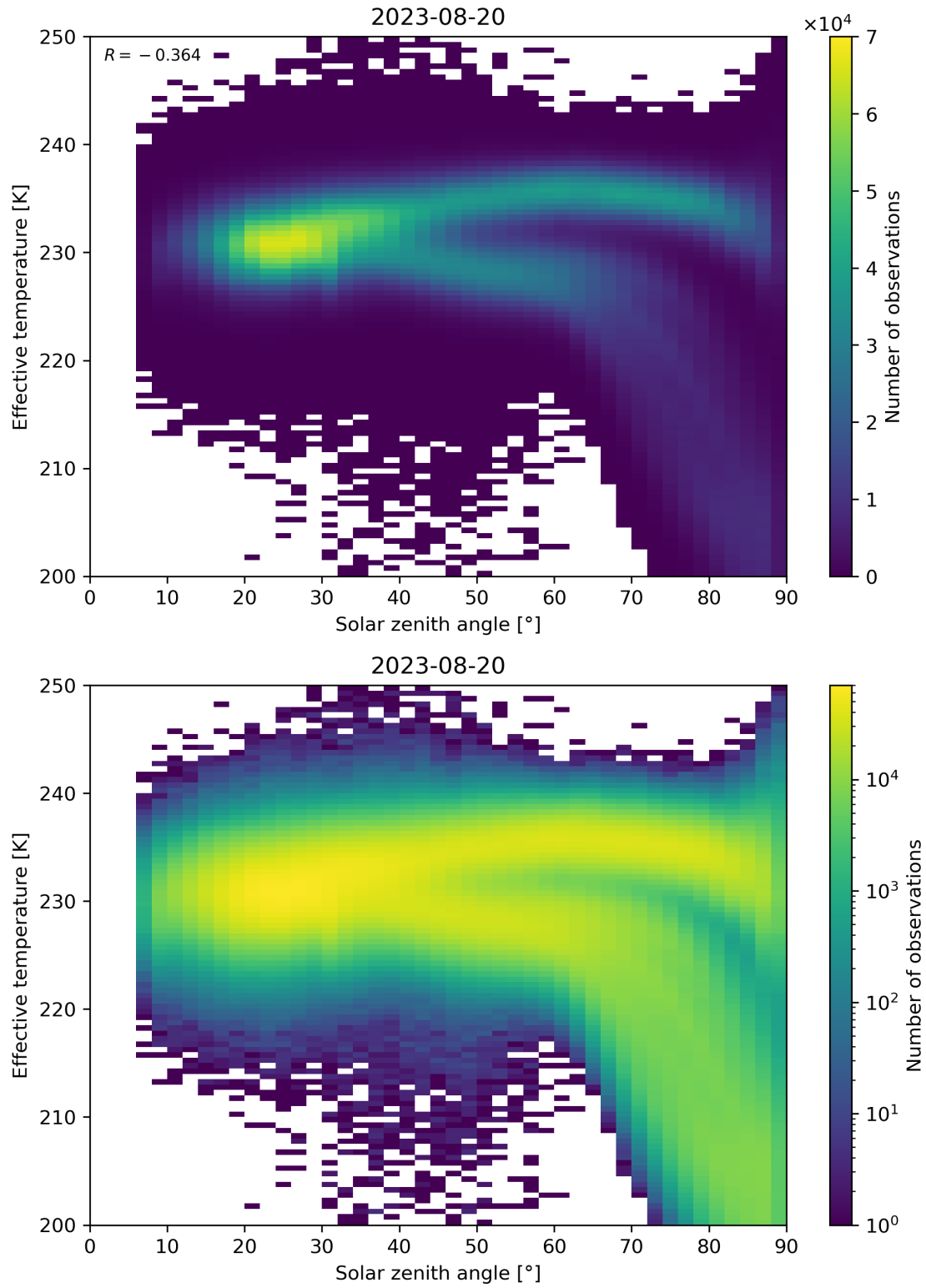
Figure 45: Scatter density plot of “Solar zenith angle” against “Effective temperature” for 2023-08-20 to 2023-08-21.
