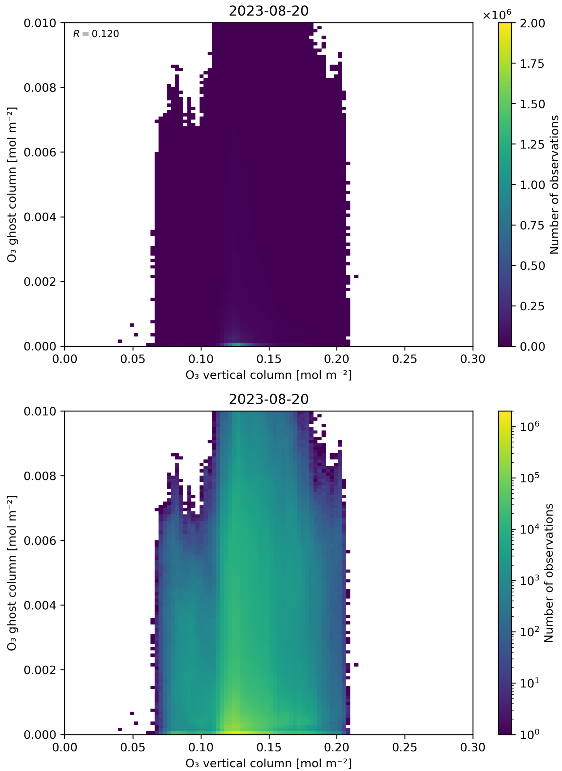
Figure 40: Scatter density plot of “O 3 vertical column” against “O 3 ghost column” for 2023-08-20 to 2023-08-21.
