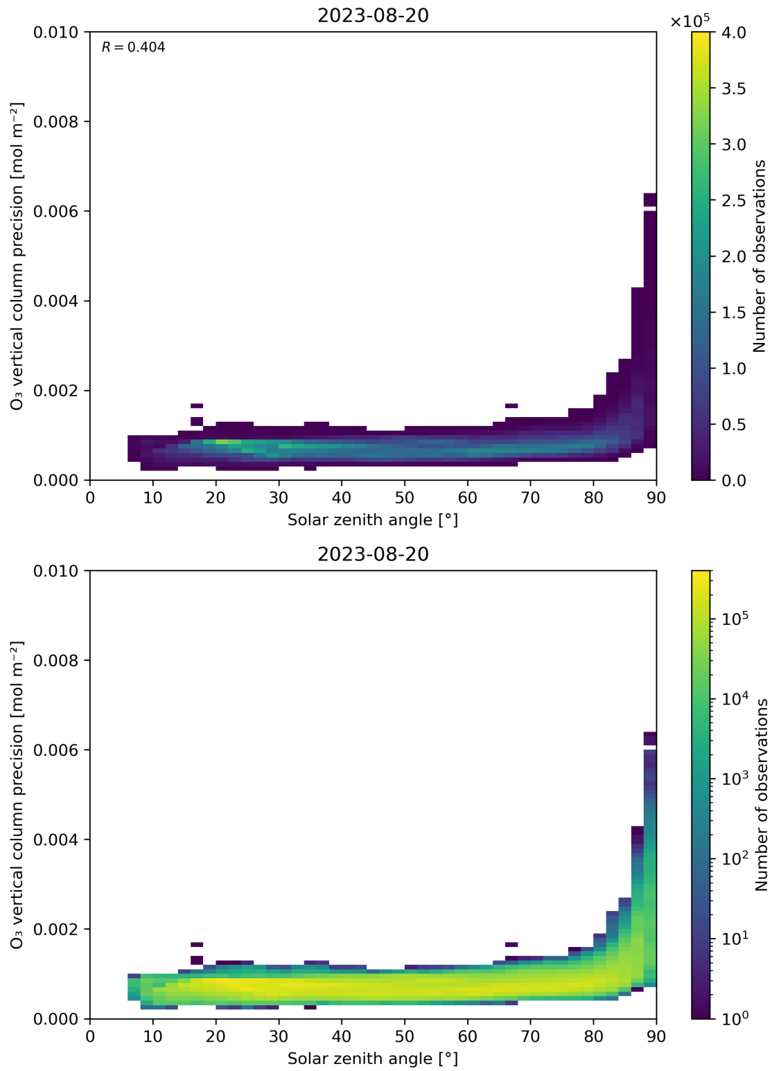
Figure 48: Scatter density plot of “Solar zenith angle” against “O 3 vertical column precision” for 2023-08-20 to 2023-08-21.
