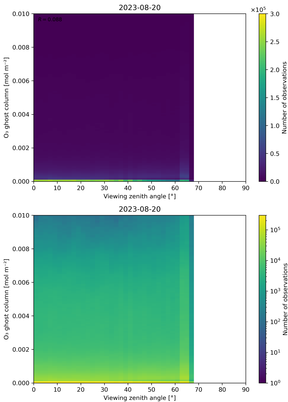
Figure 51: Scatter density plot of “Viewing zenith angle” against “O 3 ghost column” for 2023-08-20 to 2023-08-21.
