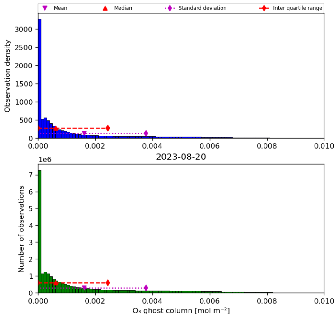
Figure 25: Histogram of “O 3 ghost column” for 2023-08-20 to 2023-08-21
