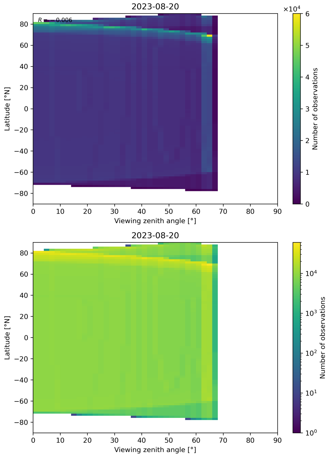
Figure 49: Scatter density plot of “Viewing zenith angle” against “Latitude” for 2023-08-20 to 2023-08-21.
