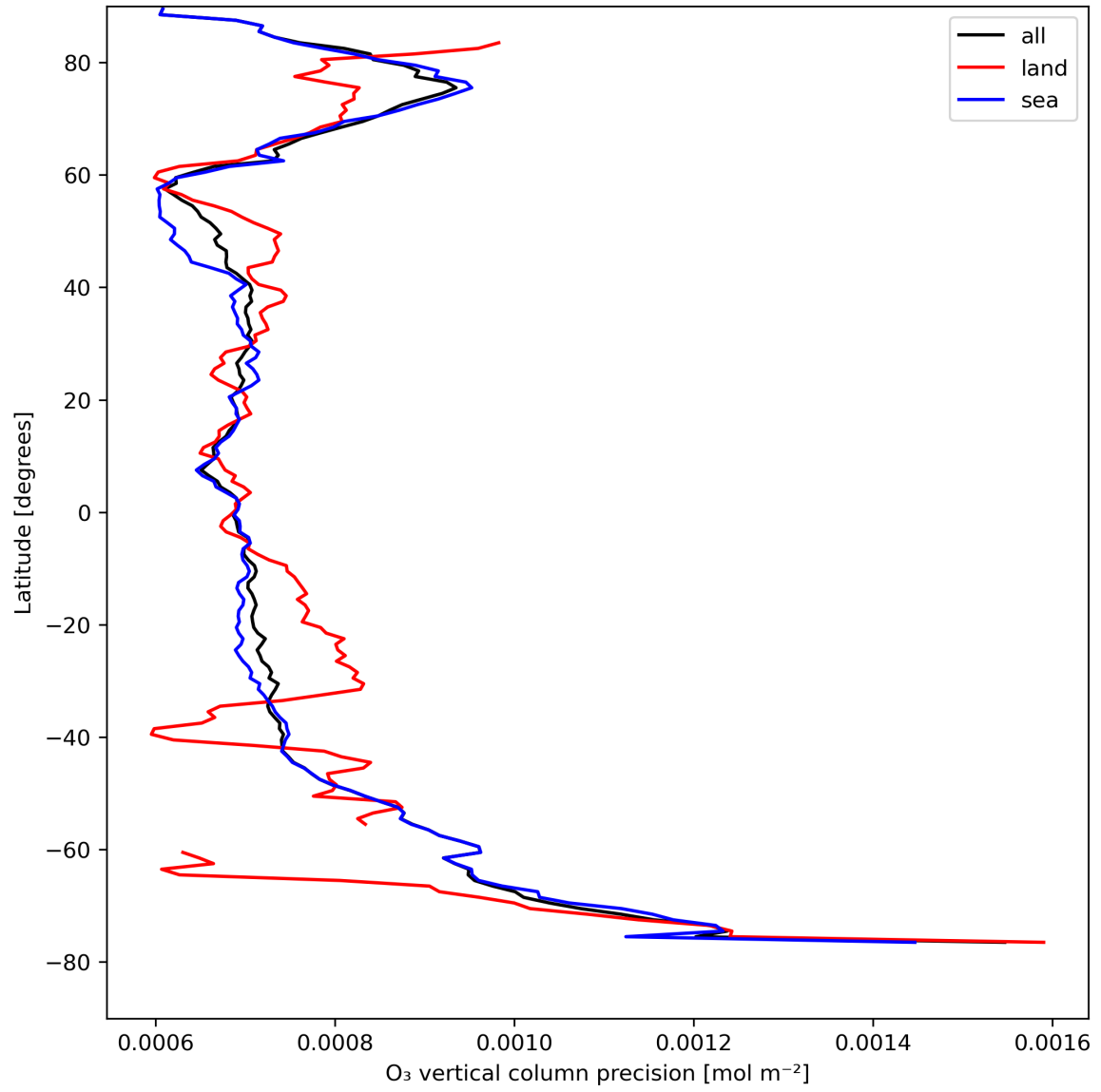
Figure 15: Zonal average of “O 3 vertical column precision” for 2023-08-20 to 2023-08-21.
