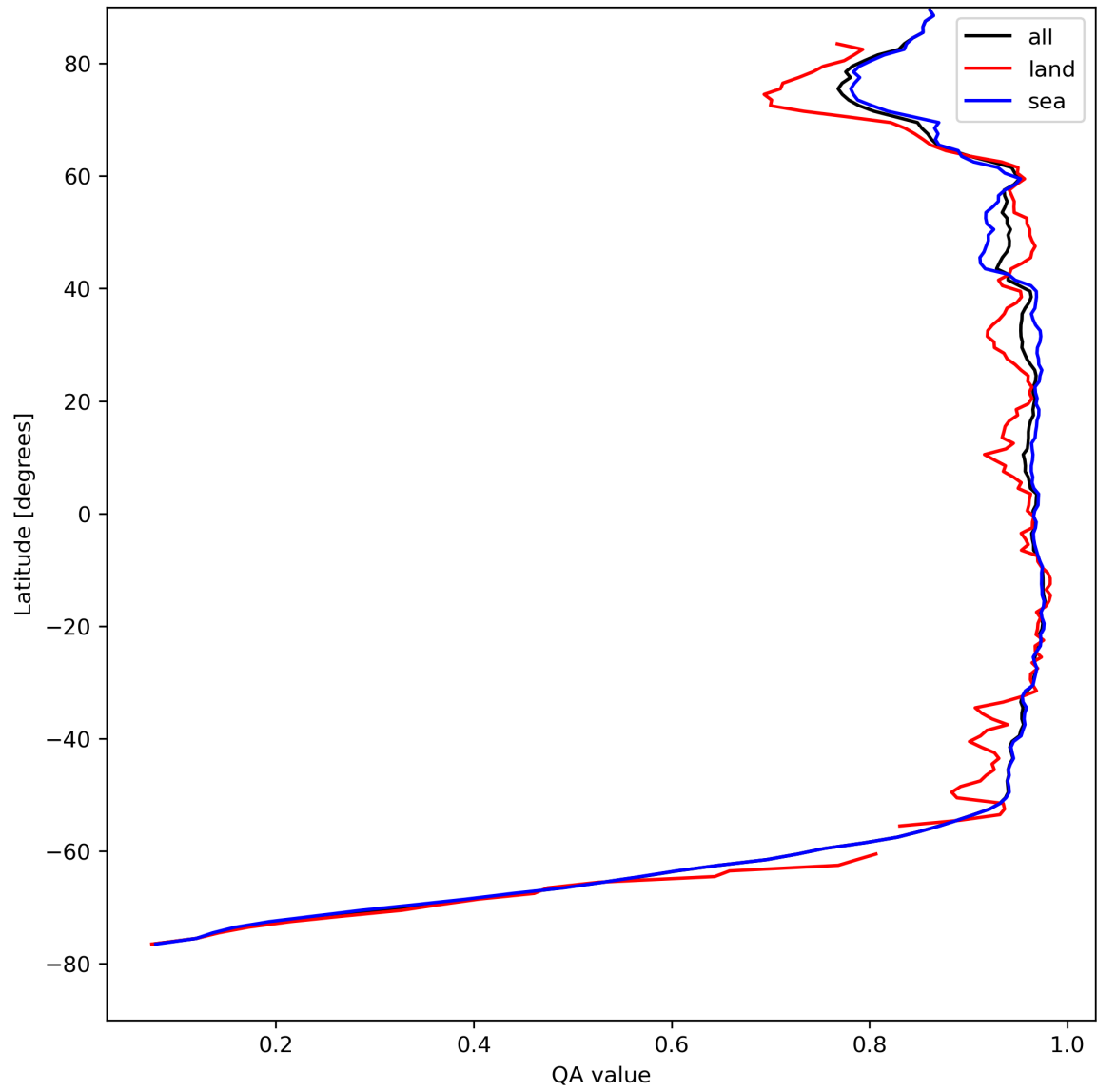
Figure 13: Zonal average of “QA value” for 2023-08-20 to 2023-08-21.
