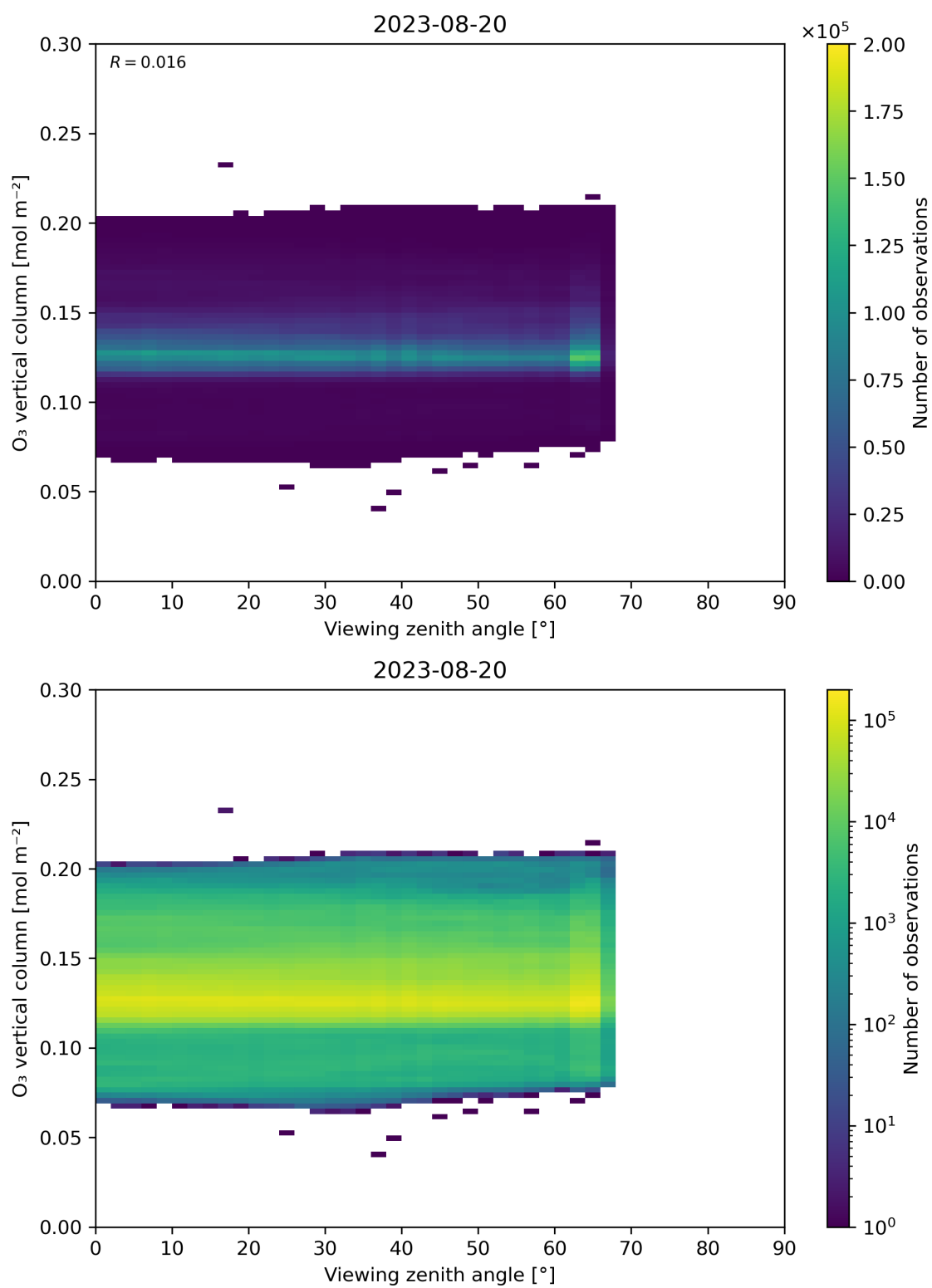
Figure 52: Scatter density plot of “Viewing zenith angle” against “O 3 vertical column” for 2023-08-20 to 2023-08-21.
