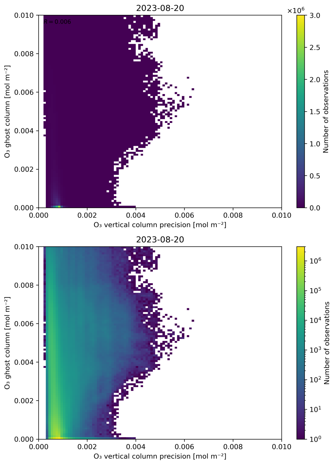
Figure 43: Scatter density plot of “ \text{O}_3 vertical column precision” against “ \text{O}_3 ghost column” for 2023-08-20 to 2023-08-21.
