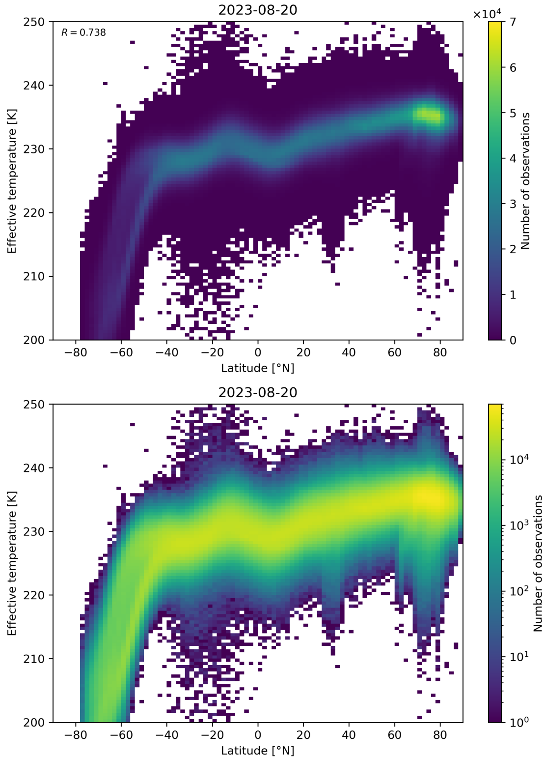
Figure 34: Scatter density plot of “Latitude” against “Effective temperature” for 2023-08-20 to 2023-08-21.
