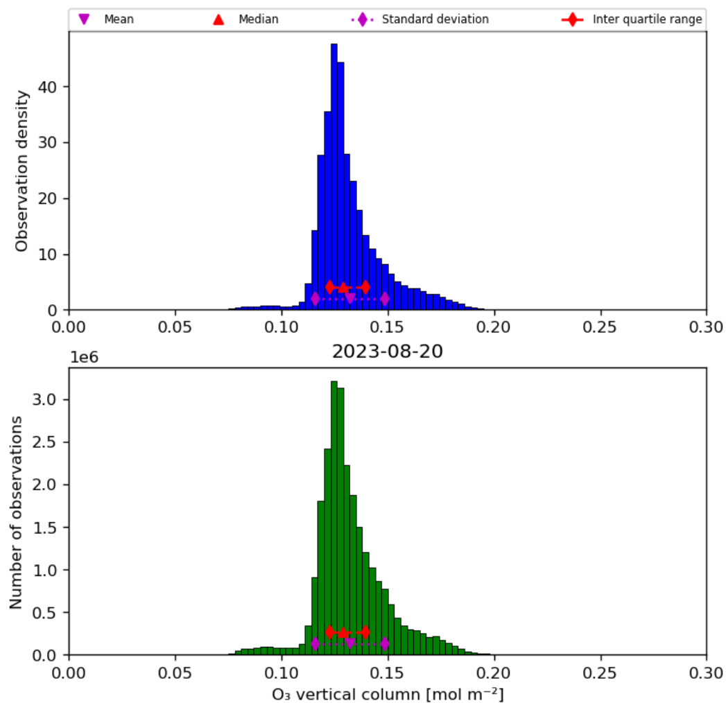
Figure 21: Histogram of “O 3 vertical column” for 2023-08-20 to 2023-08-21
