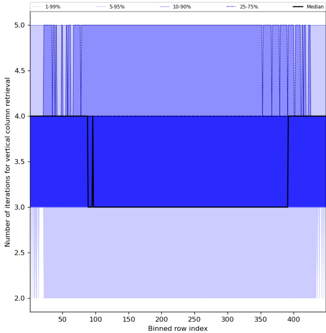
Figure 33: Along track statistics of “Number of iterations for vertical column retrieval” for 2023-08-20 to 2023-08-21
