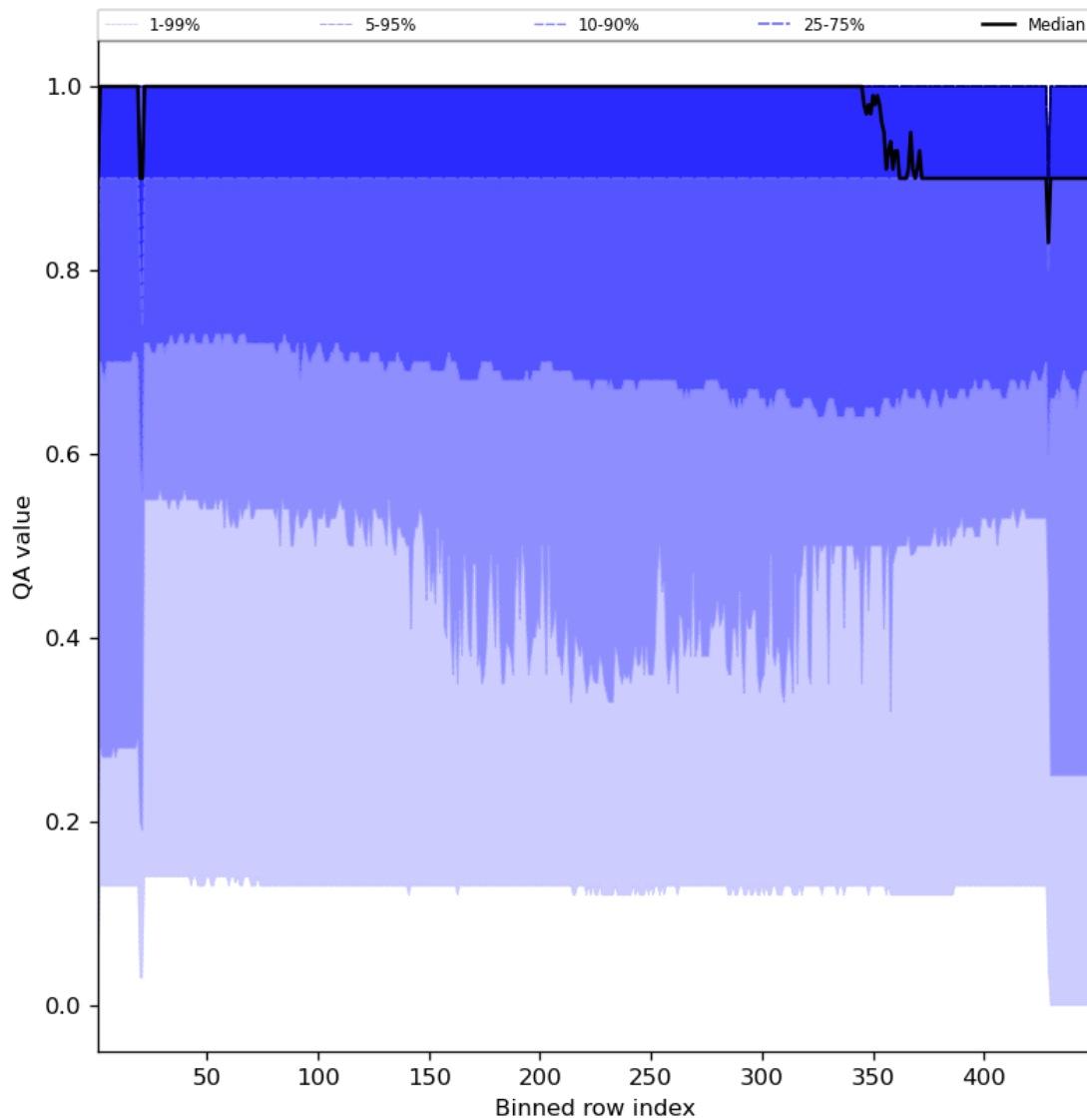
Figure 27: Along track statistics of “QA value” for 2023-08-20 to 2023-08-21
