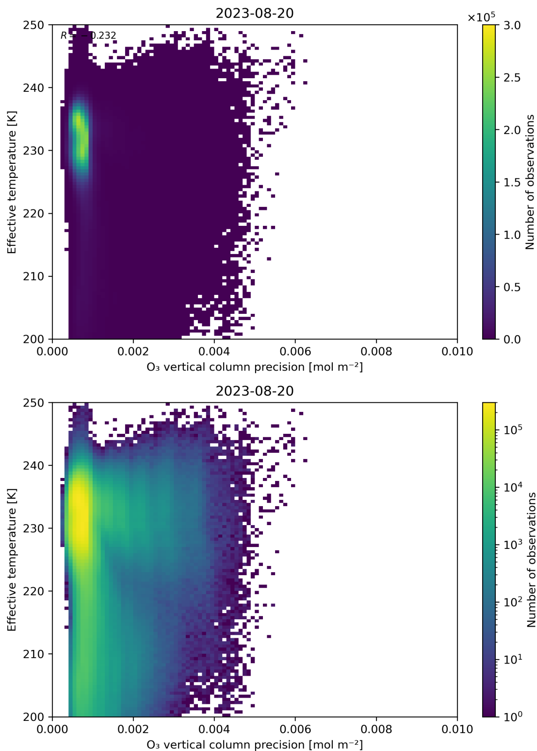
Figure 42: Scatter density plot of “O 3 vertical column precision” against “Effective temperature” for 2023-08-20 to 2023-08-21.
