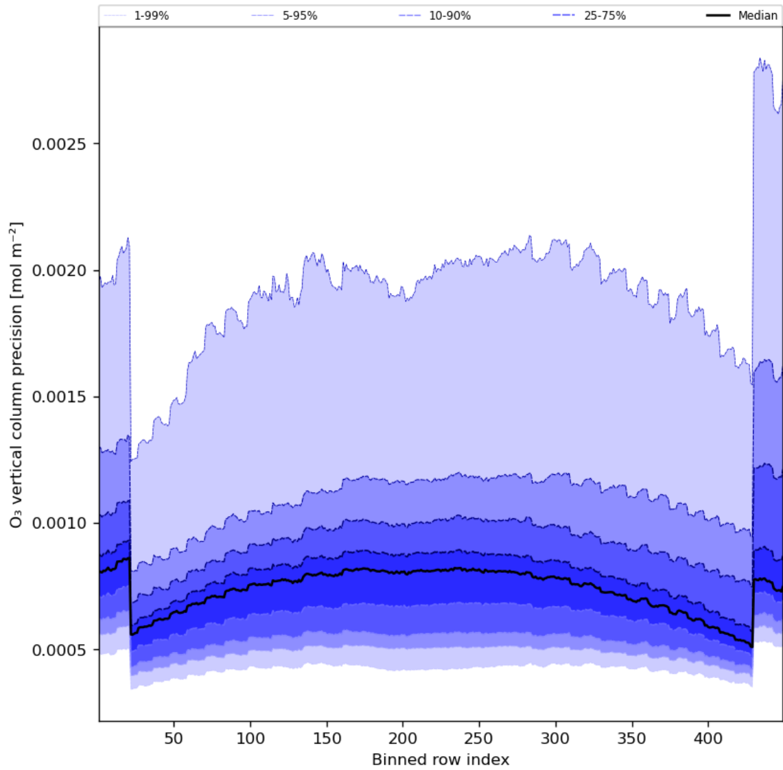
Figure 29: Along track statistics of “O 3 vertical column precision” for 2023-08-20 to 2023-08-21
