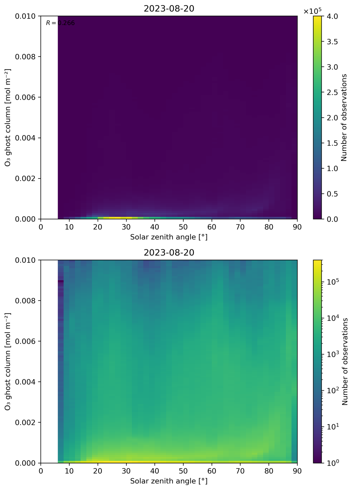
Figure 46: Scatter density plot of “Solar zenith angle” against “O 3 ghost column” for 2023-08-20 to 2023-08-21.
