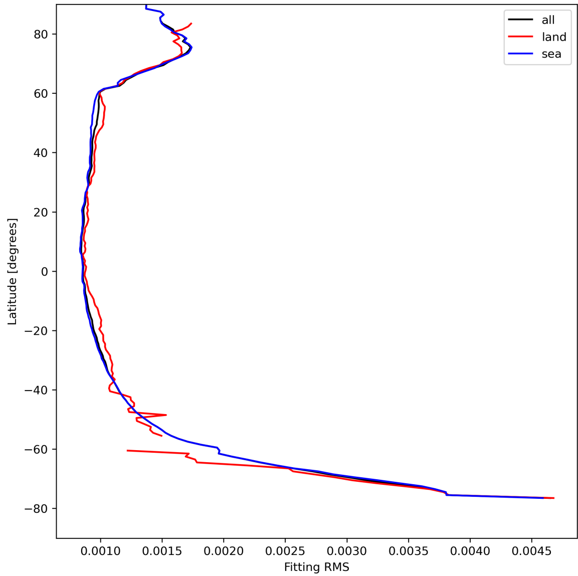
Figure 16: Zonal average of “Fitting RMS” for 2023-08-20 to 2023-08-21.
