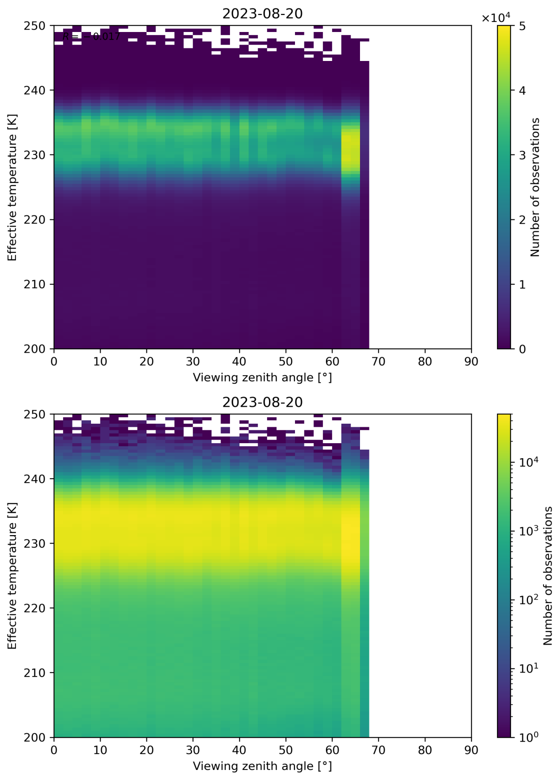
Figure 50: Scatter density plot of “Viewing zenith angle” against “Effective temperature” for 2023-08-20 to 2023-08-21.
