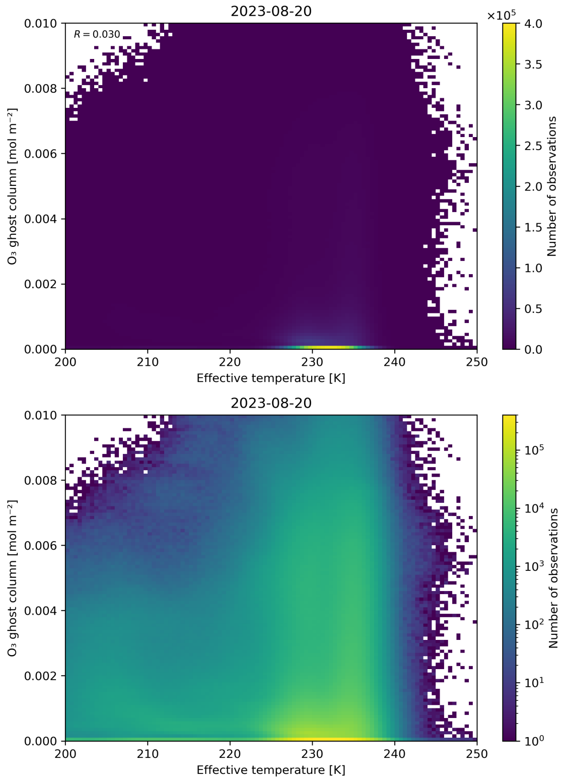
Figure 38: Scatter density plot of “Effective temperature” against “O 3 ghost column” for 2023-08-20 to 2023-08-21.
