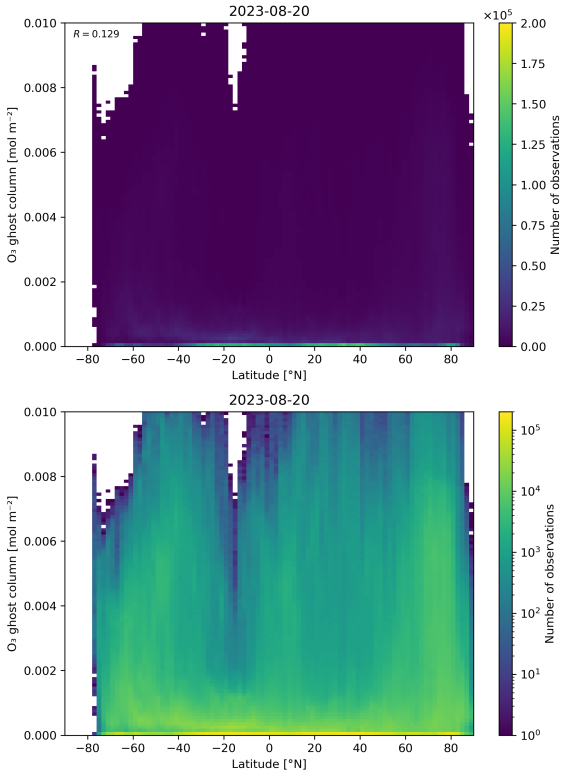
Figure 35: Scatter density plot of “Latitude” against “O 3 ghost column” for 2023-08-20 to 2023-08-21.
