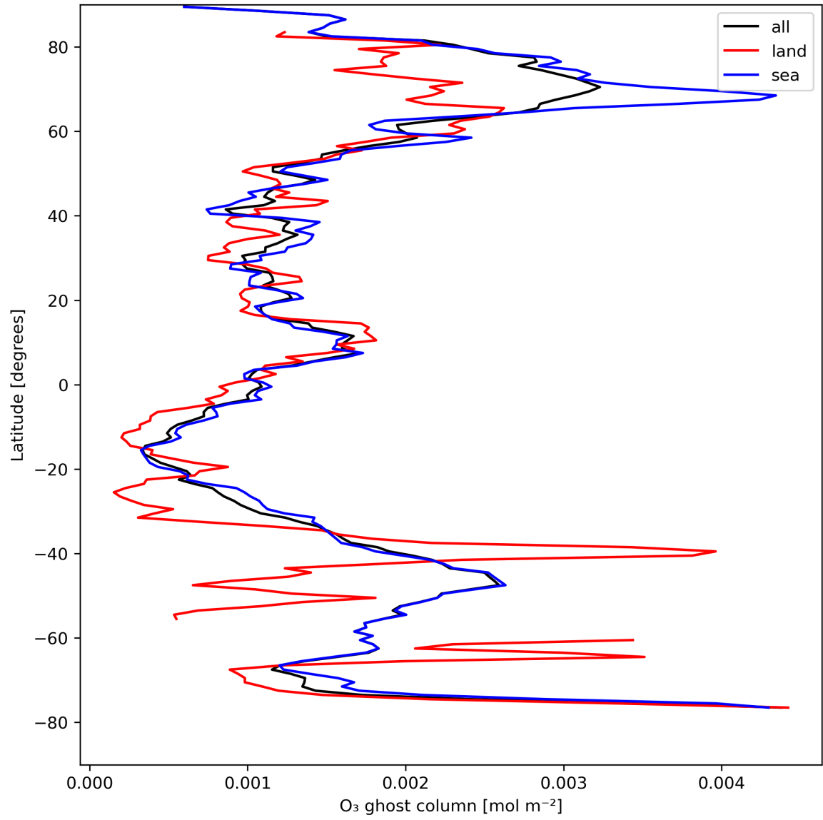
Figure 18: Zonal average of “O 3 ghost column” for 2023-08-20 to 2023-08-21.
