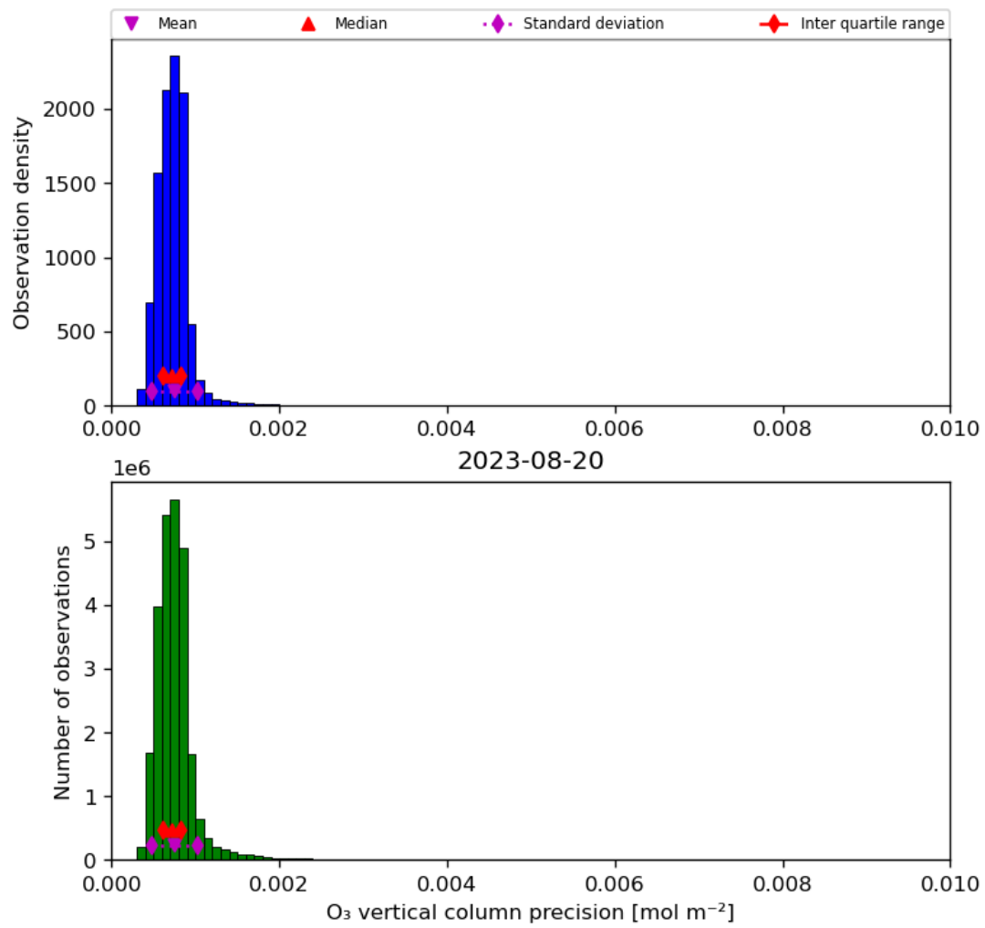
Figure 22: Histogram of “O 3 vertical column precision” for 2023-08-20 to 2023-08-21
