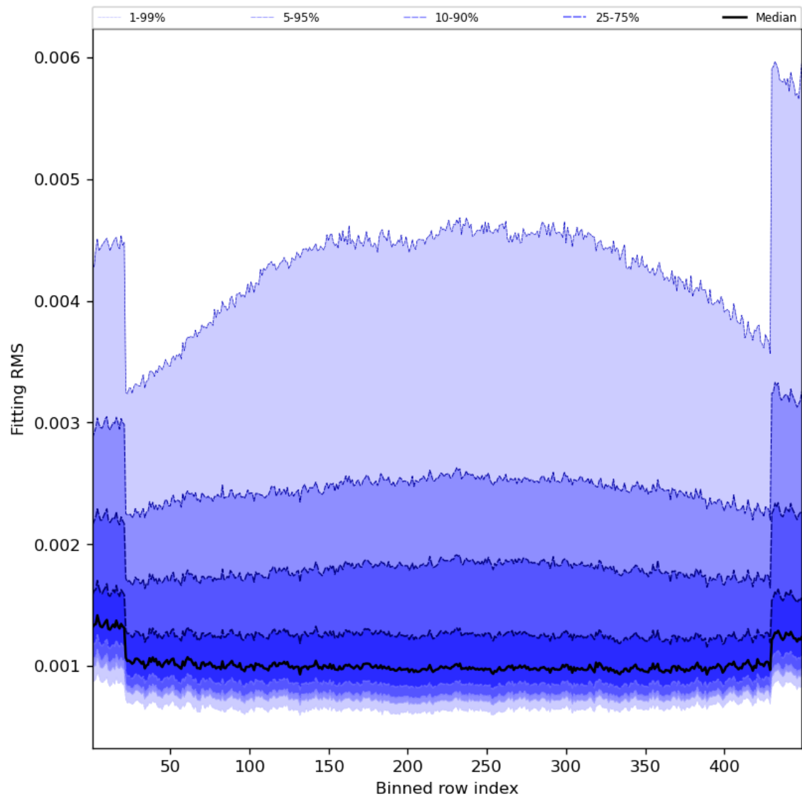
Figure 30: Along track statistics of “Fitting RMS” for 2023-08-20 to 2023-08-21
