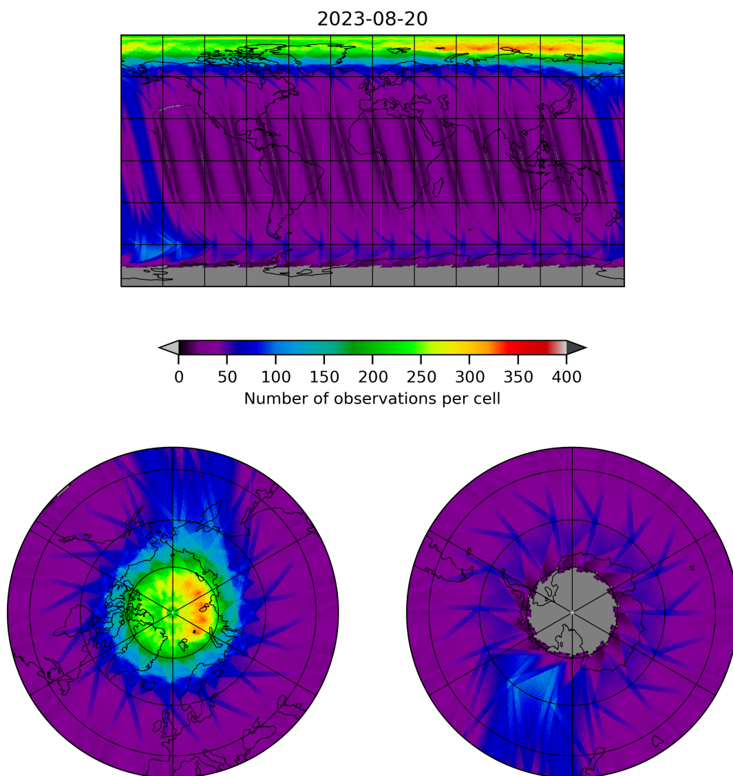
Figure 12: Map of the number of observations for 2023-08-20 to 2023-08-21
