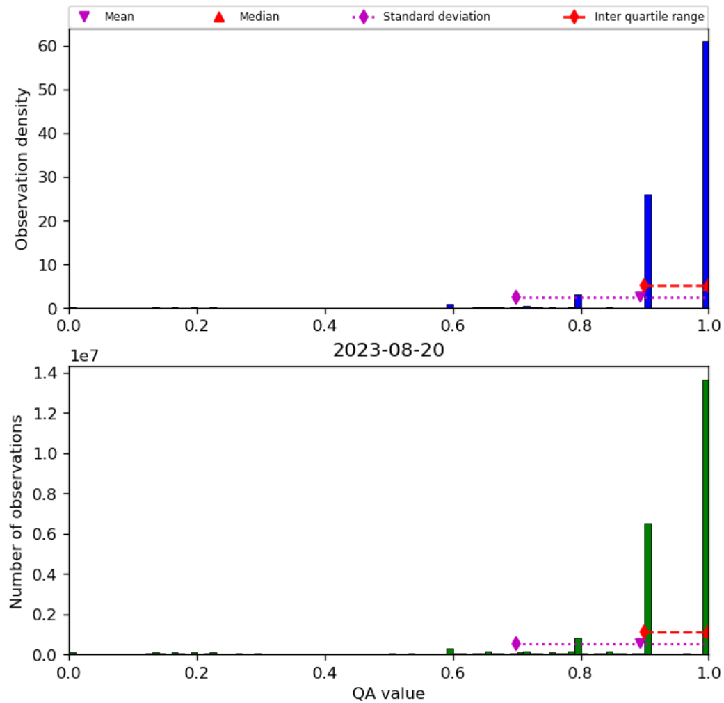
Figure 20: Histogram of “QA value” for 2023-08-20 to 2023-08-21
