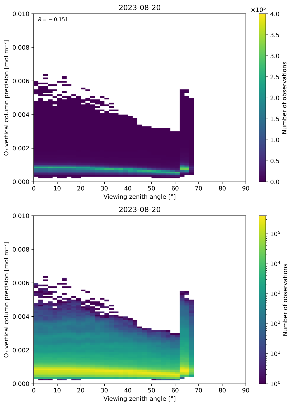
Figure 53: Scatter density plot of “Viewing zenith angle” against “O 3 vertical column precision” for 2023-08-20 to 2023-08-21.
