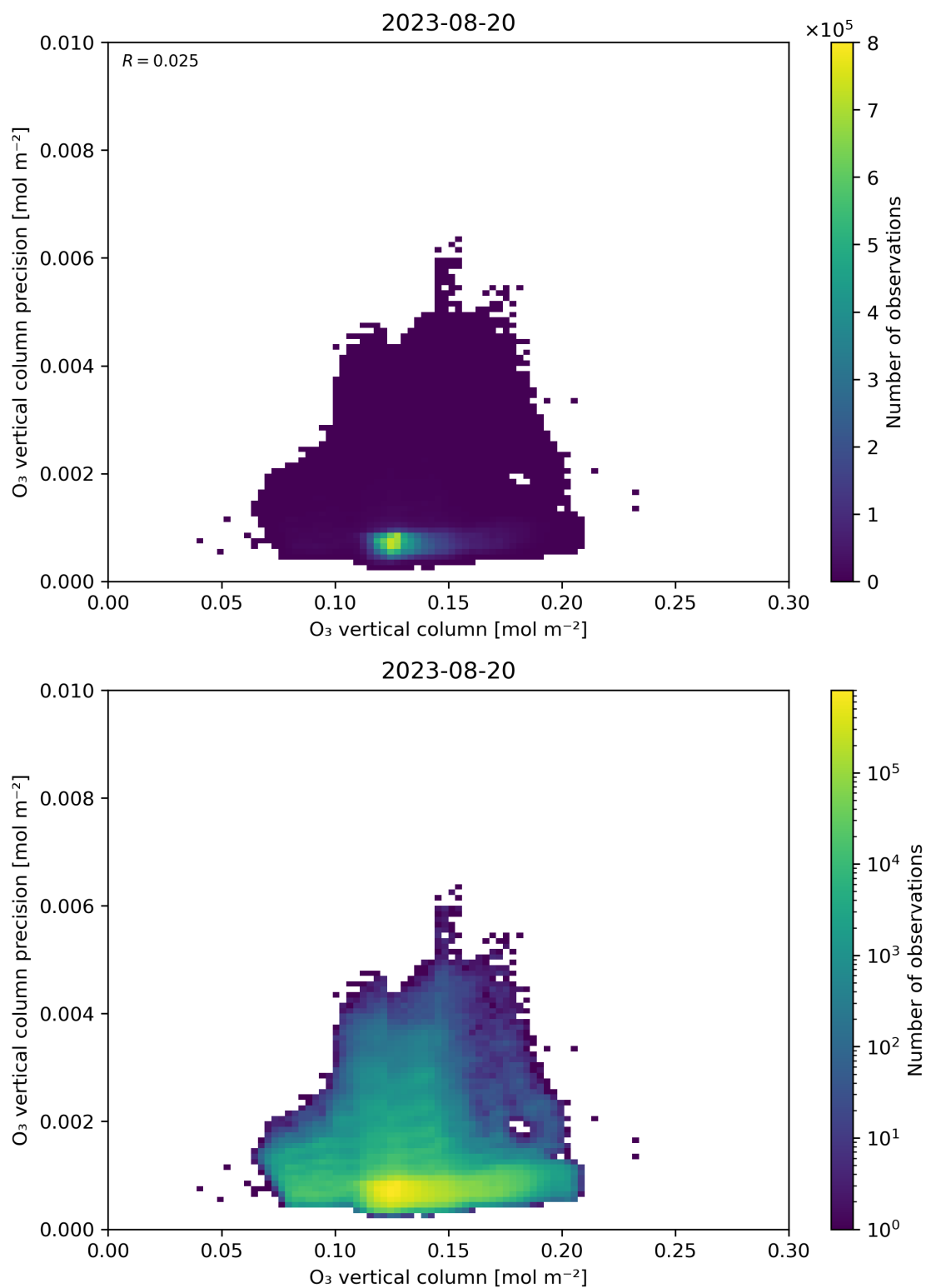
Figure 41: Scatter density plot of “O 3 vertical column” against “O 3 vertical column precision” for 2023-08-20 to 2023-08-21.
