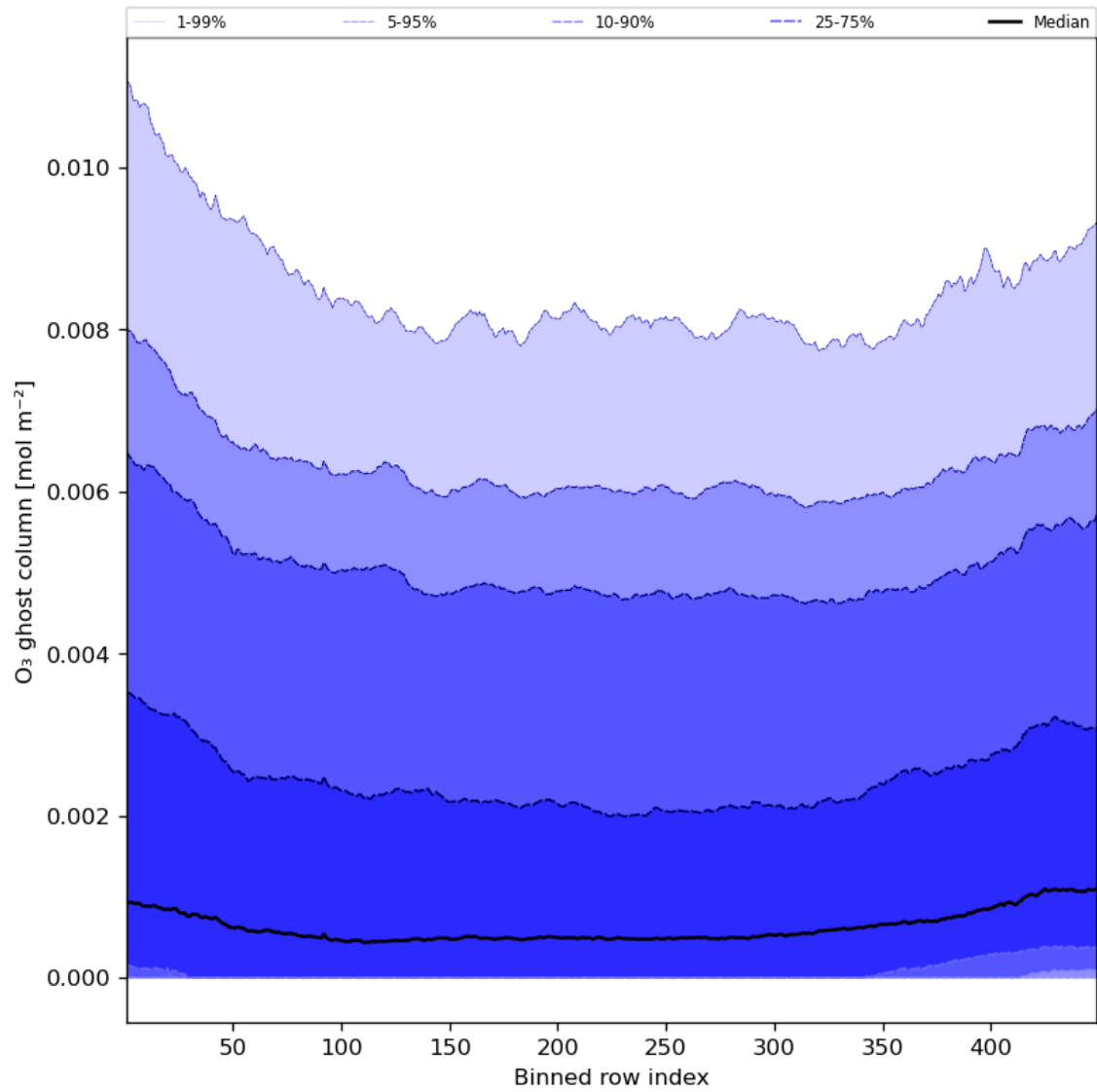
Figure 32: Along track statistics of “O 3 ghost column” for 2023-08-20 to 2023-08-21
