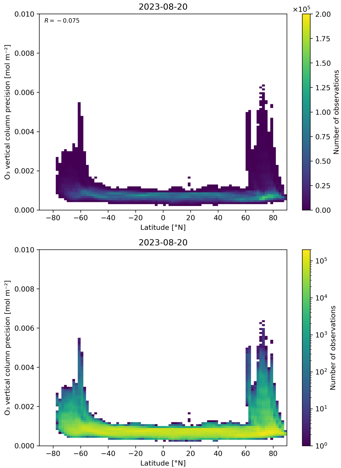
Figure 37: Scatter density plot of “Latitude” against “O 3 vertical column precision” for 2023-08-20 to 2023-08-21.
