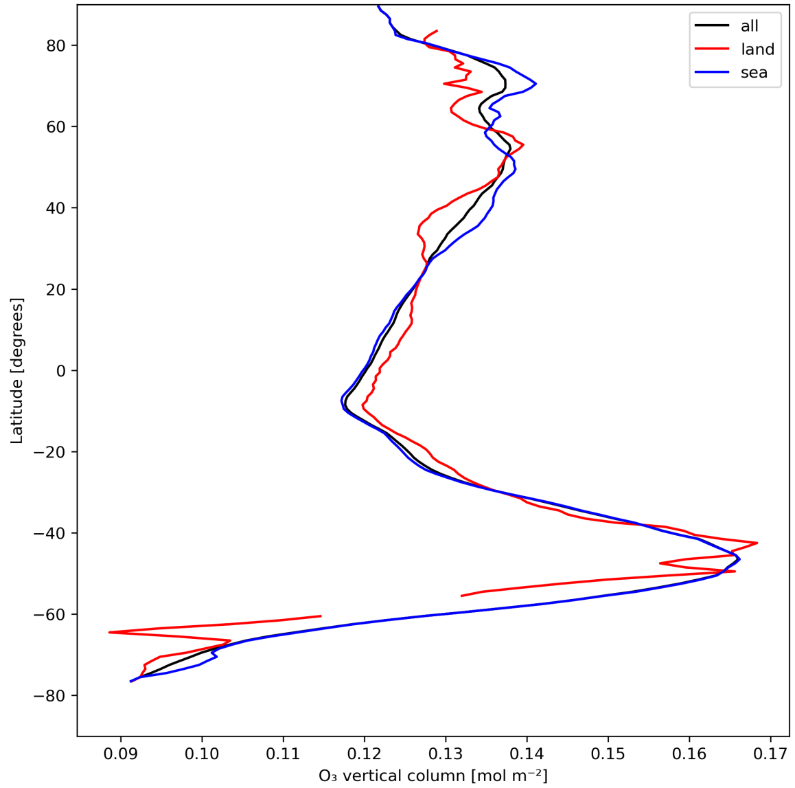
Figure 14: Zonal average of “O 3 vertical column” for 2023-08-20 to 2023-08-21.
