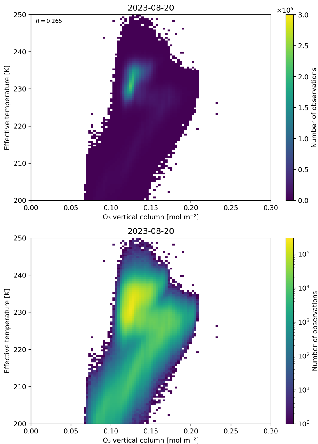
Figure 39: Scatter density plot of “O 3 vertical column” against “Effective temperature” for 2023-08-20 to 2023-08-21.
