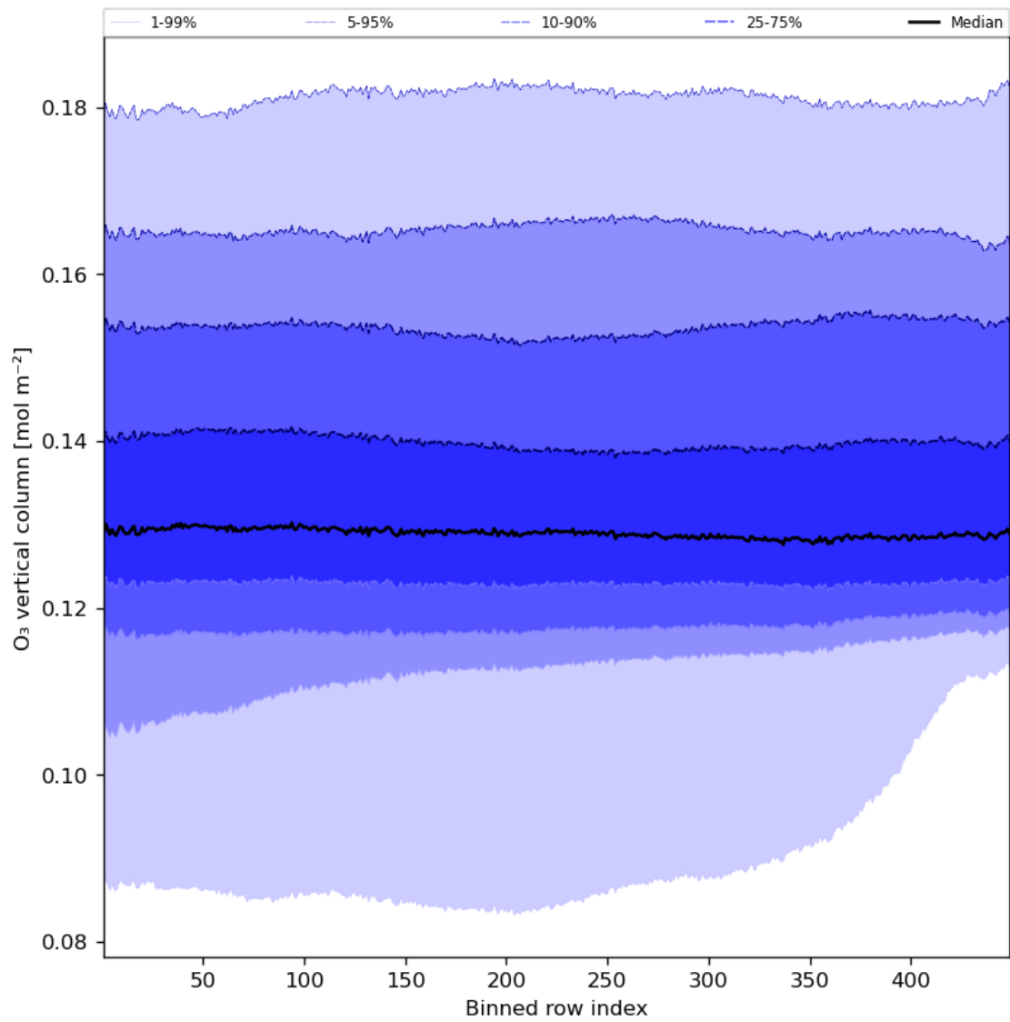
Figure 28: Along track statistics of “O 3 vertical column” for 2023-08-20 to 2023-08-21
