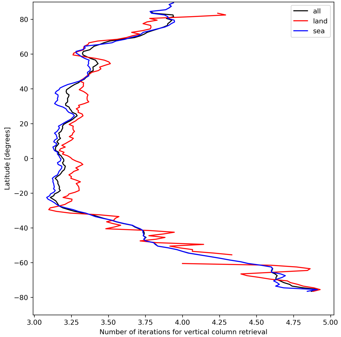
Figure 19: Zonal average of “Number of iterations for vertical column retrieval” for 2023-08-20 to 2023-08-21.
