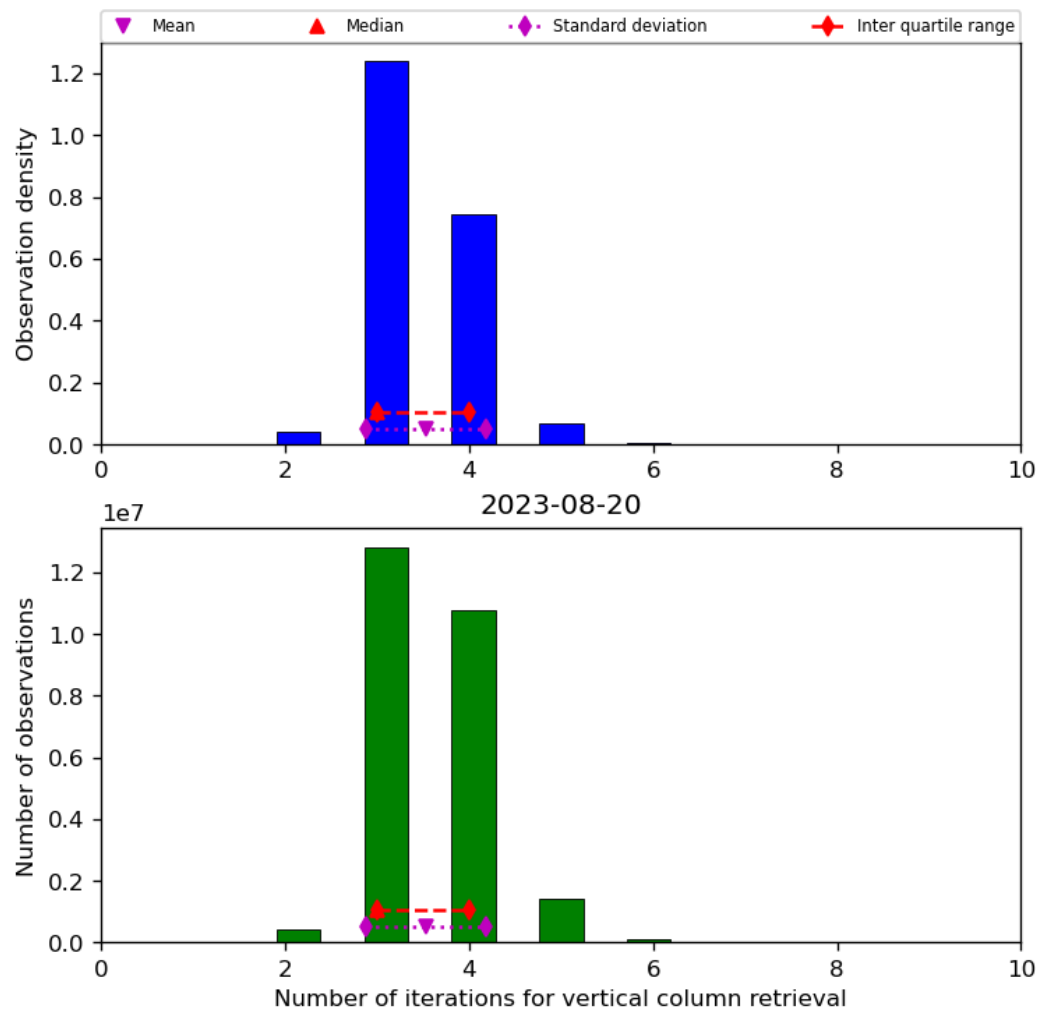
Figure 26: Histogram of “Number of iterations for vertical column retrieval” for 2023-08-20 to 2023-08-21
