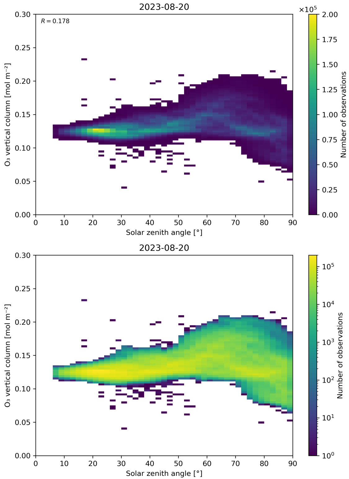
Figure 47: Scatter density plot of “Solar zenith angle” against “O 3 vertical column” for 2023-08-20 to 2023-08-21.
