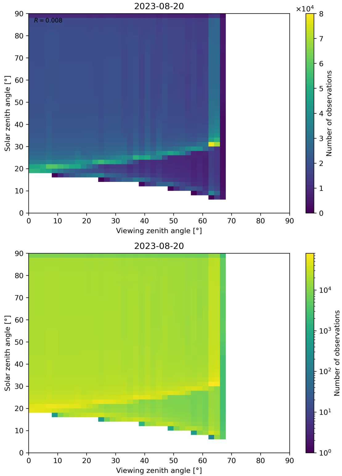
Figure 54: Scatter density plot of “Viewing zenith angle” against “Solar zenith angle” for 2023-08-20 to 2023-08-21.
