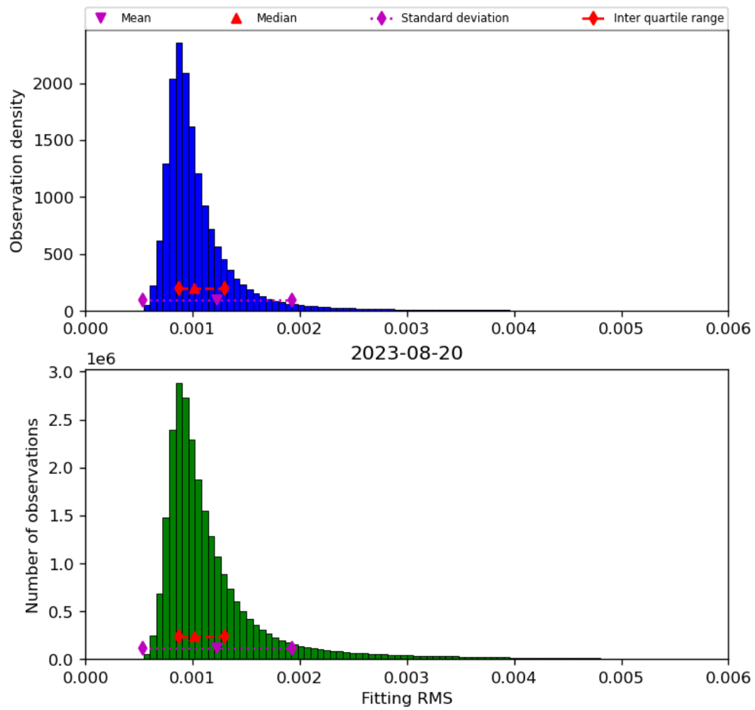
Figure 23: Histogram of “Fitting RMS” for 2023-08-20 to 2023-08-21
