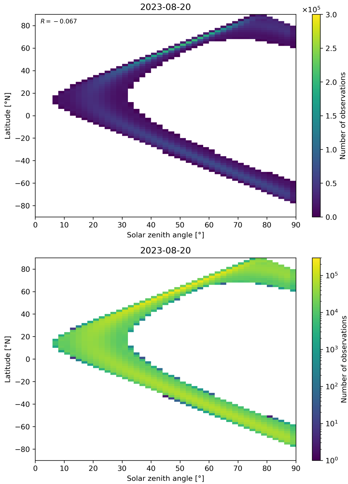
Figure 44: Scatter density plot of “Solar zenith angle” against “Latitude” for 2023-08-20 to 2023-08-21.
