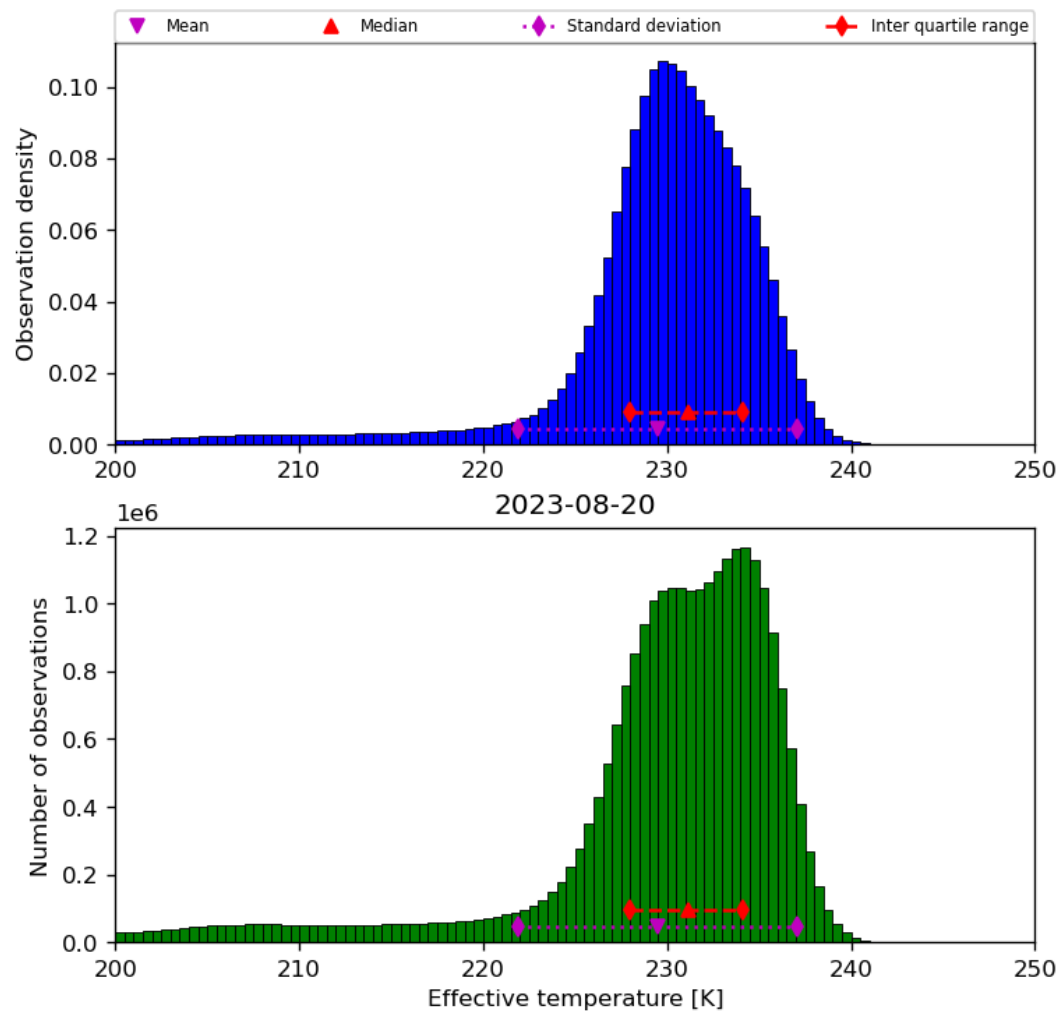
Figure 24: Histogram of “Effective temperature” for 2023-08-20 to 2023-08-21
