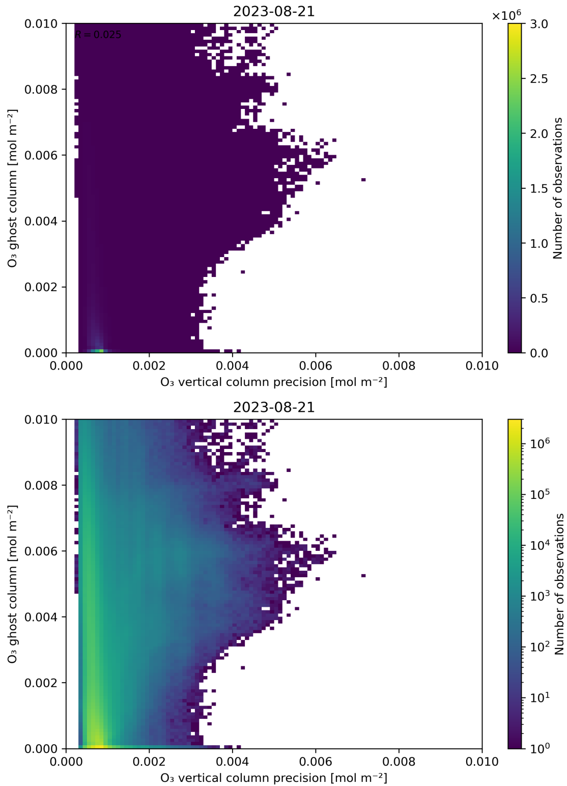
Figure 43: Scatter density plot of “O 3 vertical column precision” against “O 3 ghost column” for 2023-08-20 to 2023-08-22.
