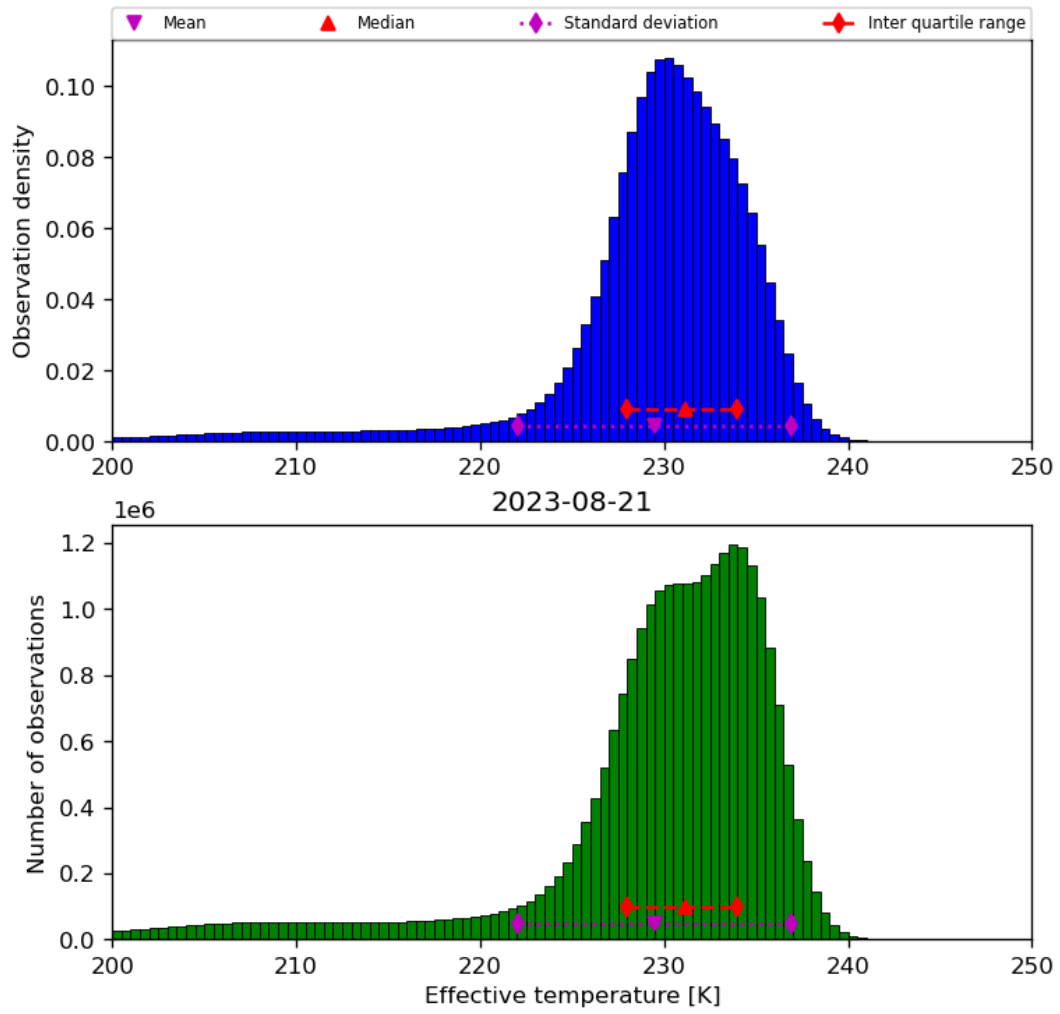
Figure 24: Histogram of “Effective temperature” for 2023-08-20 to 2023-08-22
