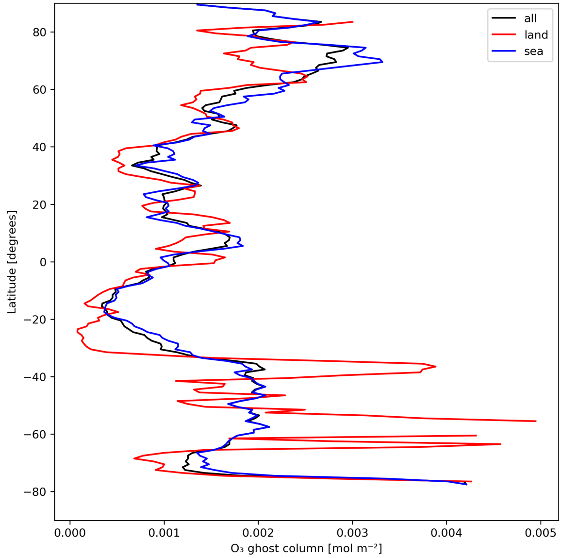
Figure 18: Zonal average of "O 3 ghost column" for 2023-08-20 to 2023-08-22.
