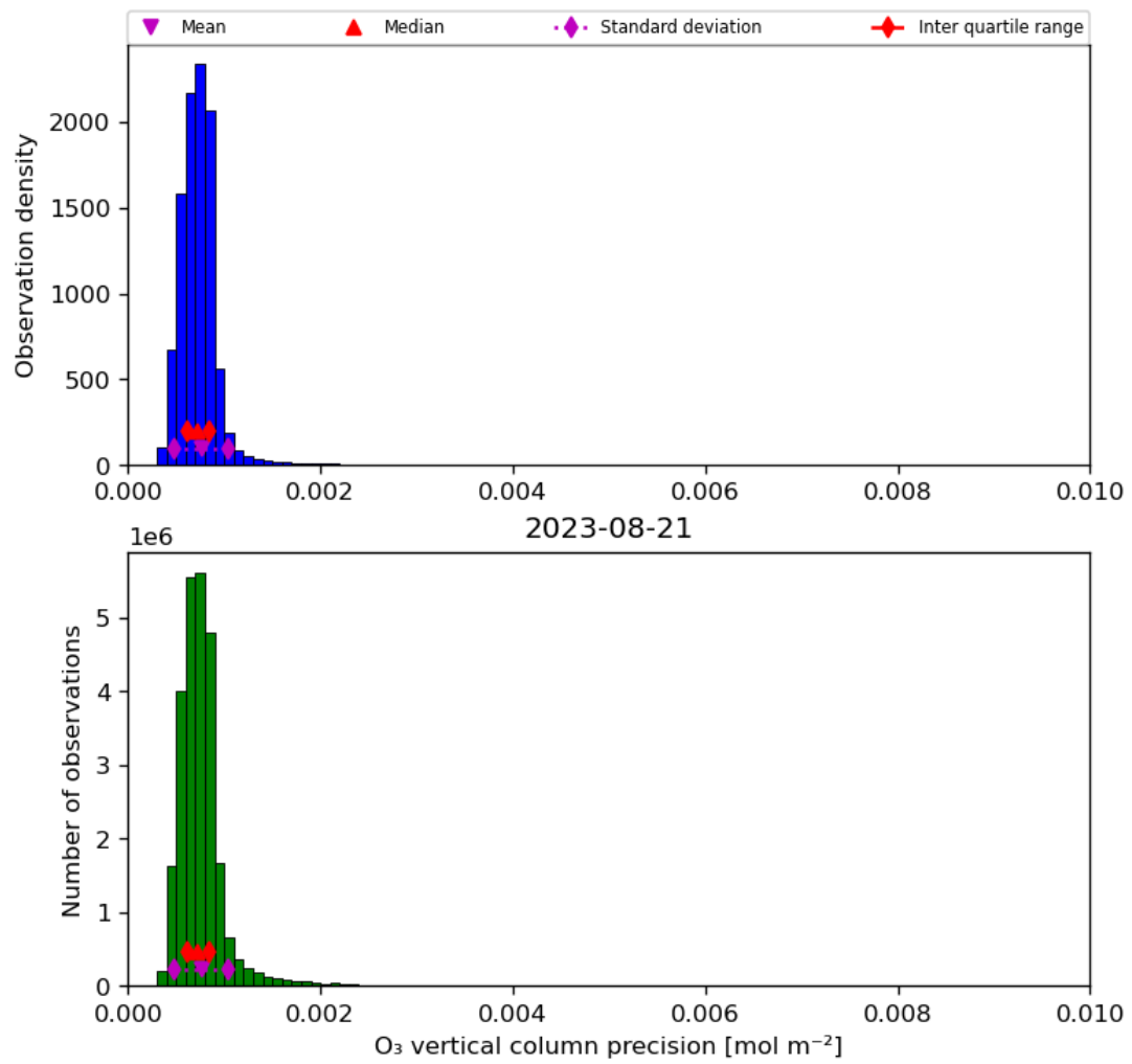
Figure 22: Histogram of “O 3 vertical column precision” for 2023-08-20 to 2023-08-22
