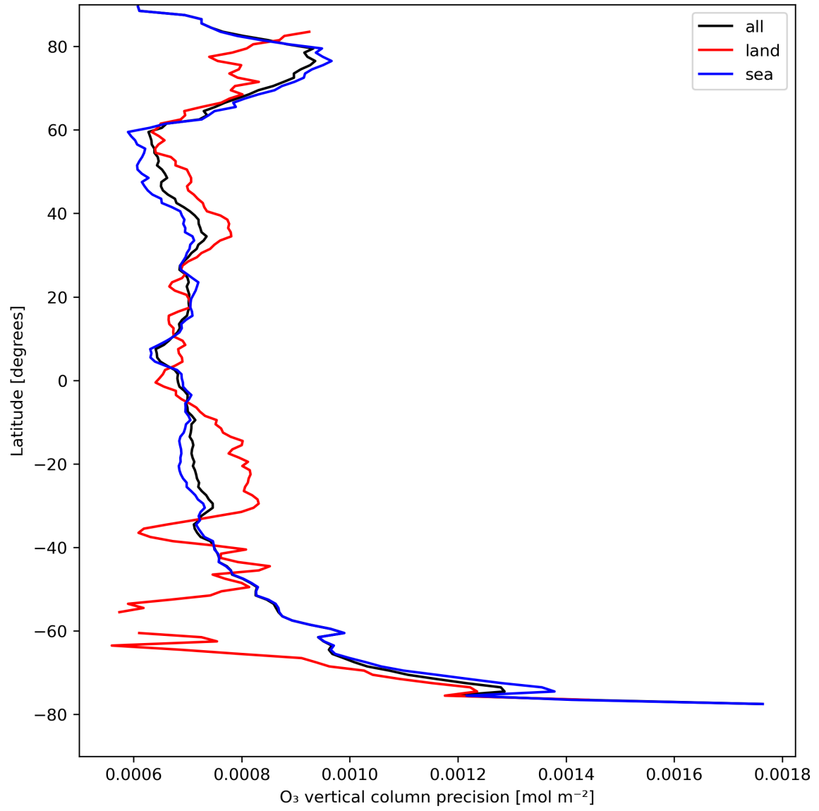
Figure 15: Zonal average of “O 3 vertical column precision” for 2023-08-20 to 2023-08-22.
