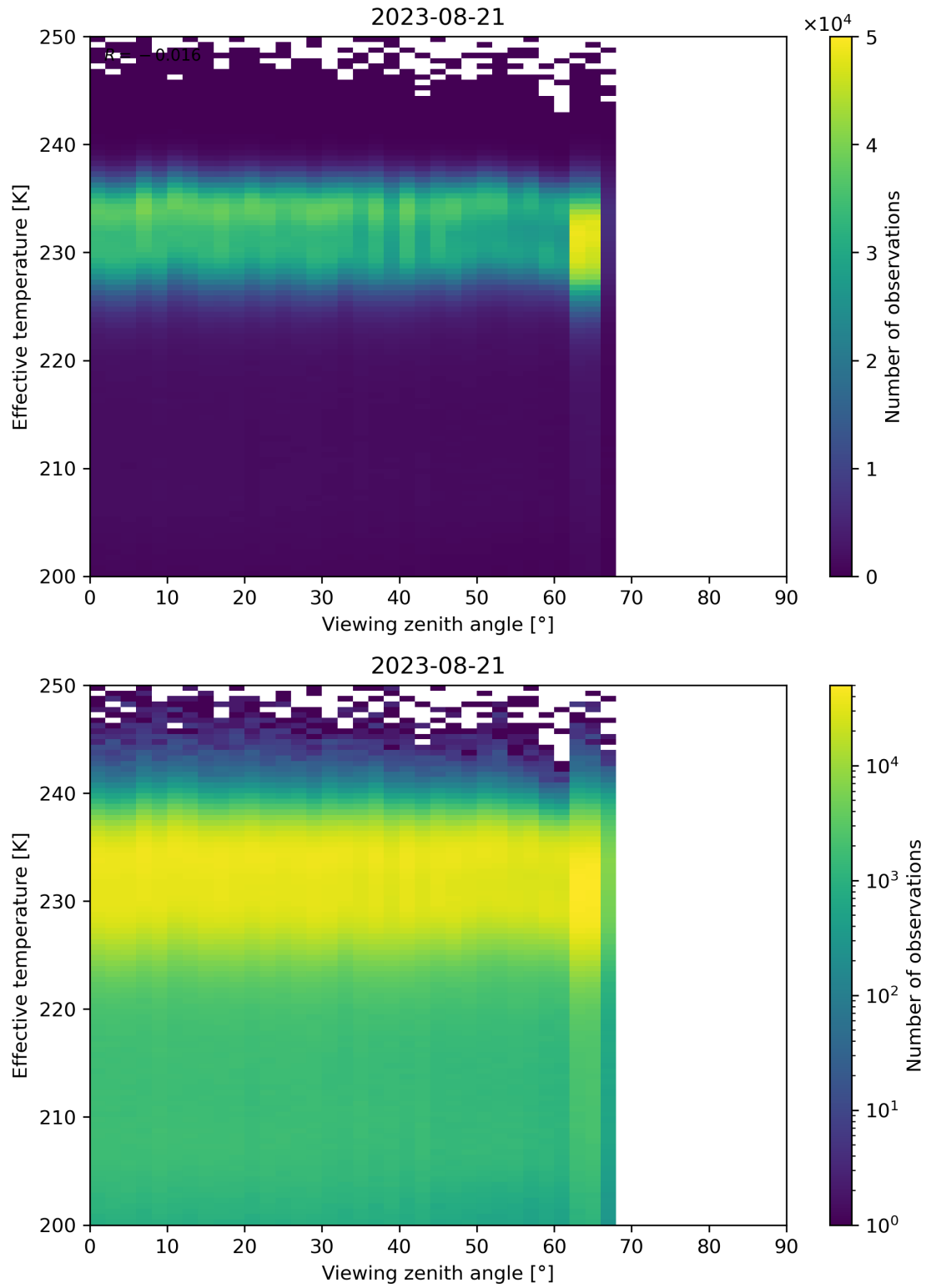
Figure 50: Scatter density plot of “Viewing zenith angle” against “Effective temperature” for 2023-08-20 to 2023-08-22.
