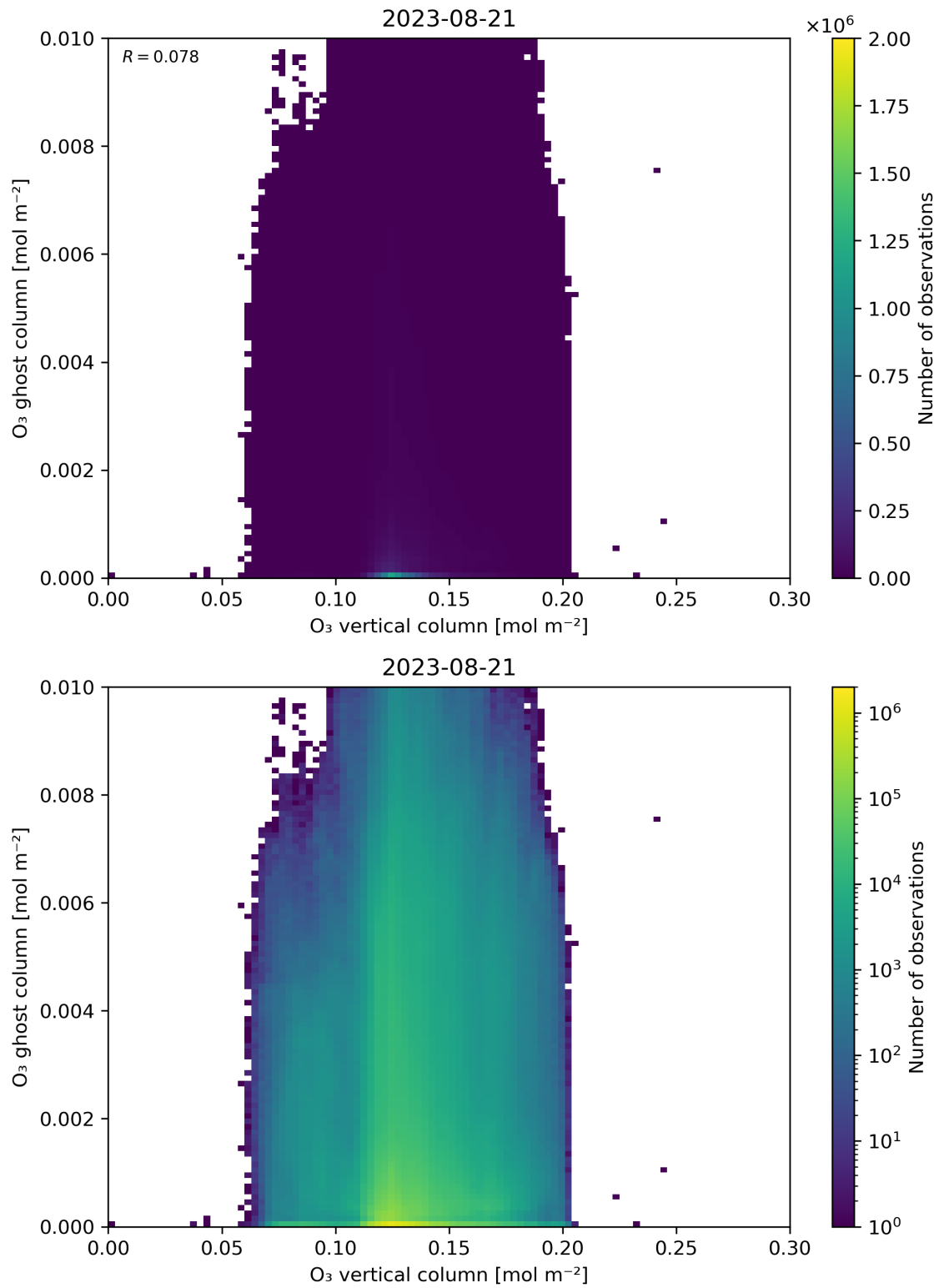
Figure 40: Scatter density plot of “O 3 vertical column” against “O 3 ghost column” for 2023-08-20 to 2023-08-22.
