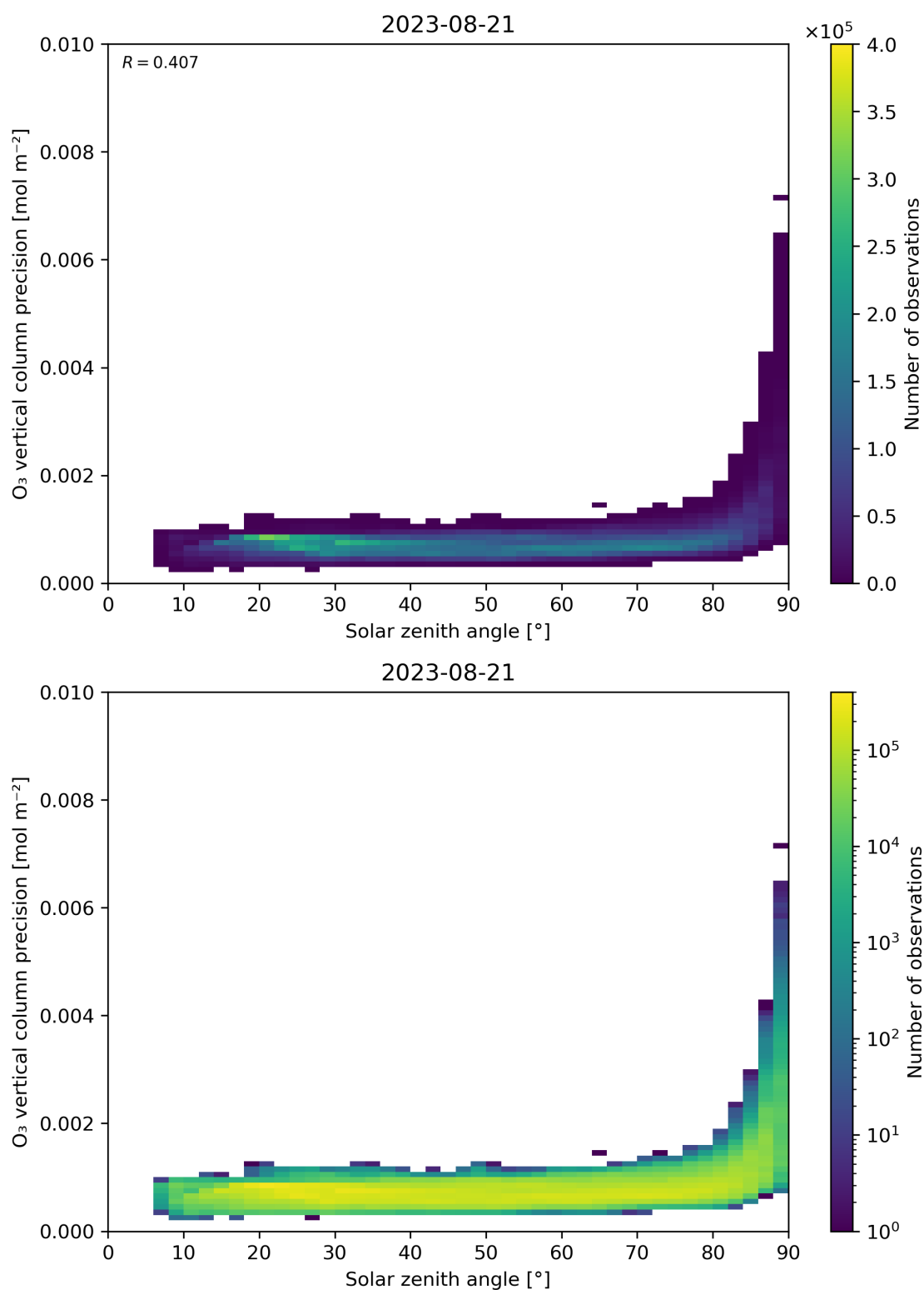
Figure 48: Scatter density plot of “Solar zenith angle” against “O 3 vertical column precision” for 2023-08-20 to 2023-08-22.
