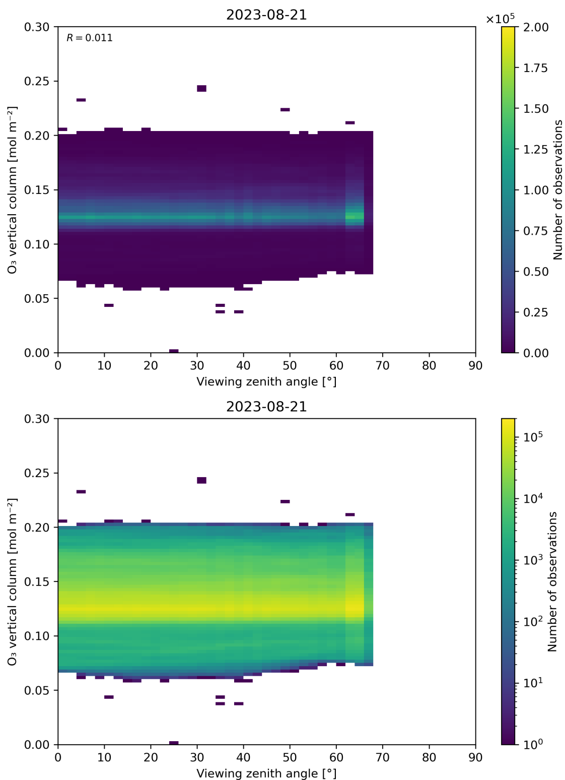
Figure 52: Scatter density plot of “Viewing zenith angle” against “O 3 vertical column” for 2023-08-20 to 2023-08-22.
