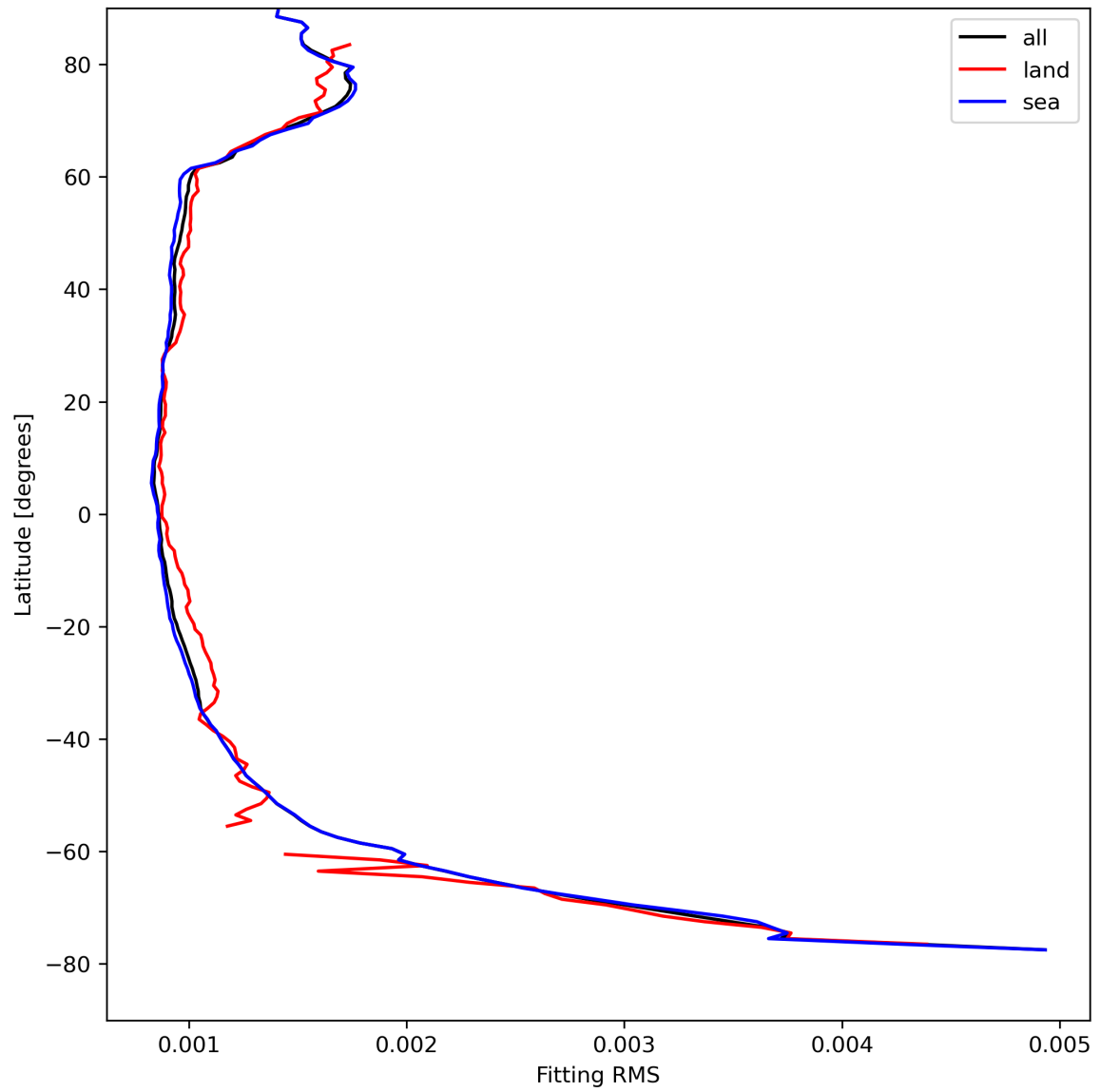
Figure 16: Zonal average of “Fitting RMS” for 2023-08-20 to 2023-08-22.
