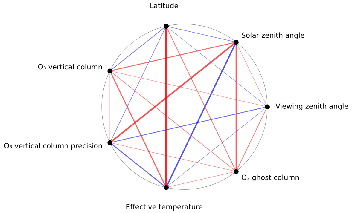
Figure 1: Map of correlation graph for 2023-08-20 to 2023-08-22.
