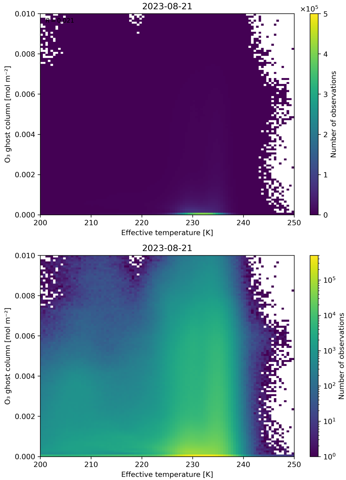
Figure 38: Scatter density plot of “Effective temperature” against “O 3 ghost column” for 2023-08-20 to 2023-08-22.
