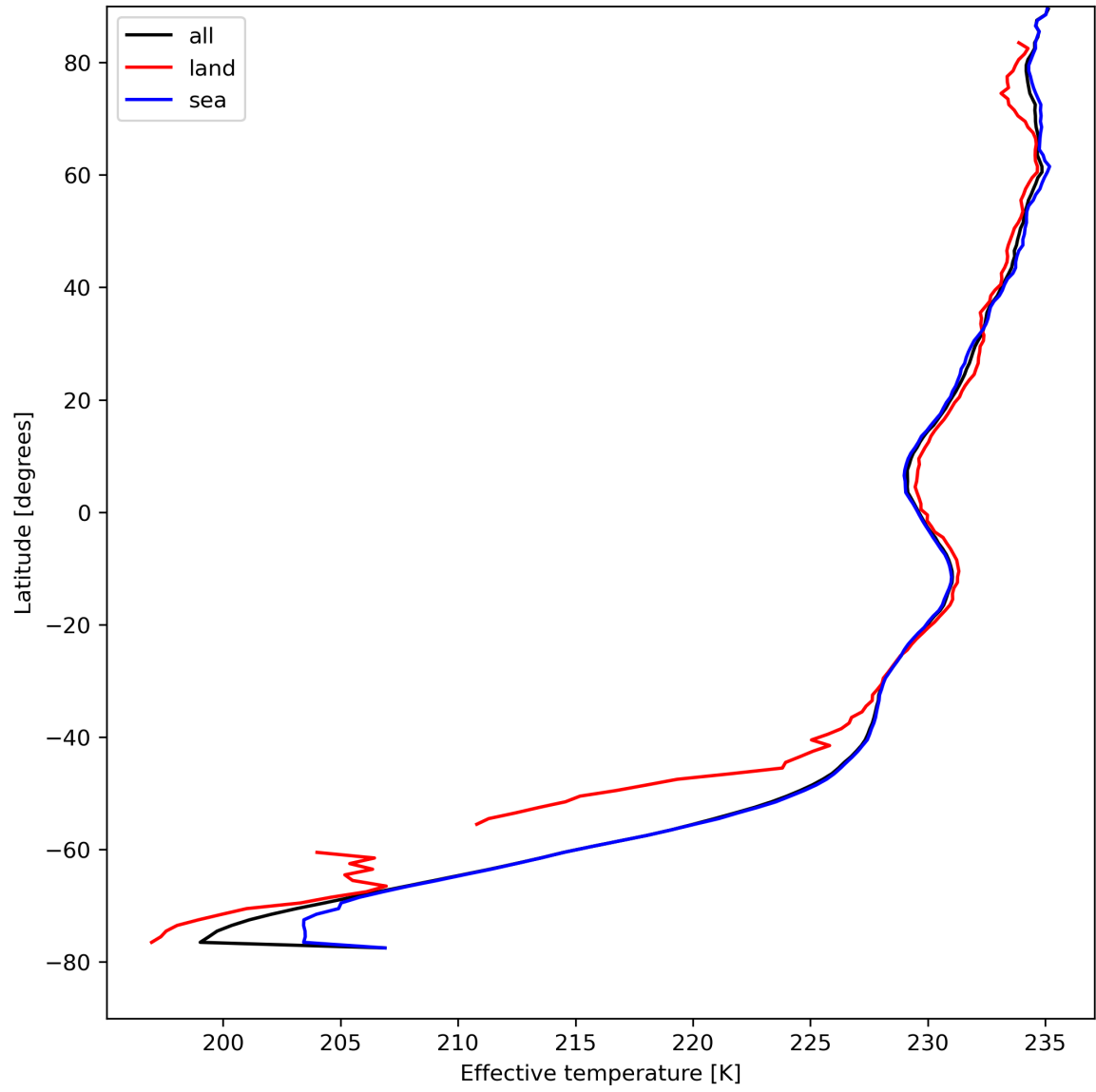
Figure 17: Zonal average of "Effective temperature" for 2023-08-20 to 2023-08-22.
