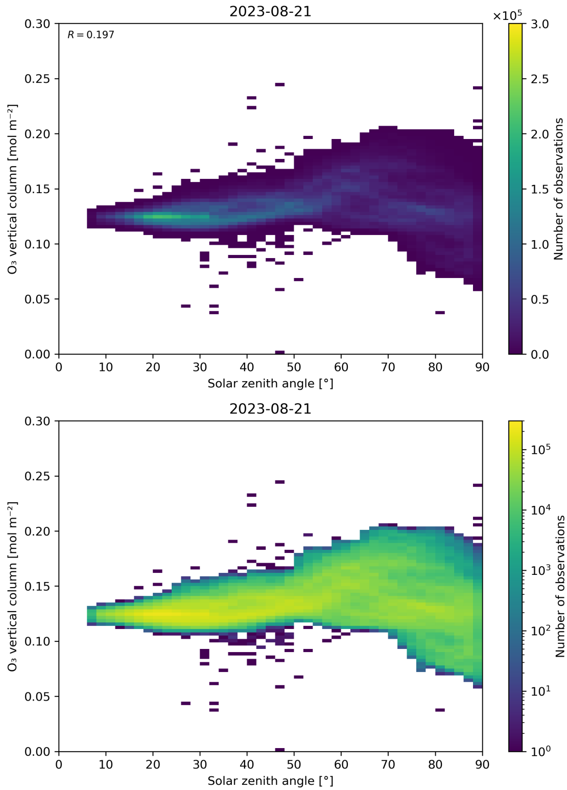
Figure 47: Scatter density plot of “Solar zenith angle” against “O 3 vertical column” for 2023-08-20 to 2023-08-22.
