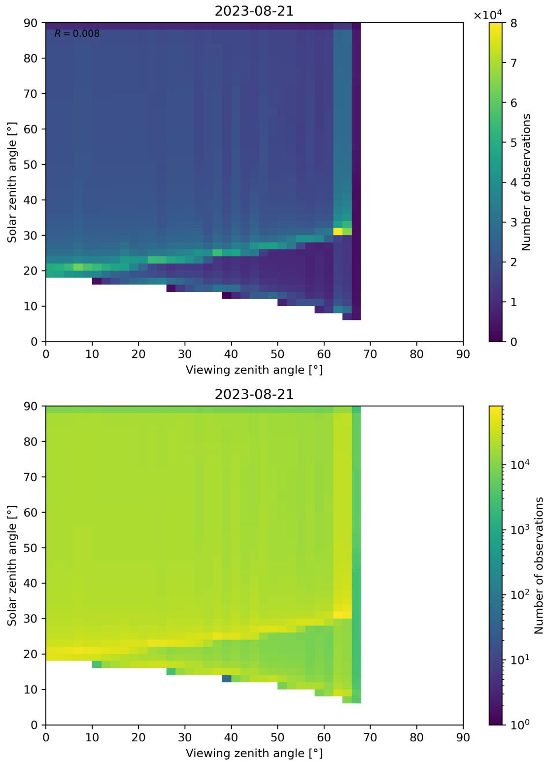
Figure 54: Scatter density plot of “Viewing zenith angle” against “Solar zenith angle” for 2023-08-20 to 2023-08-22.
