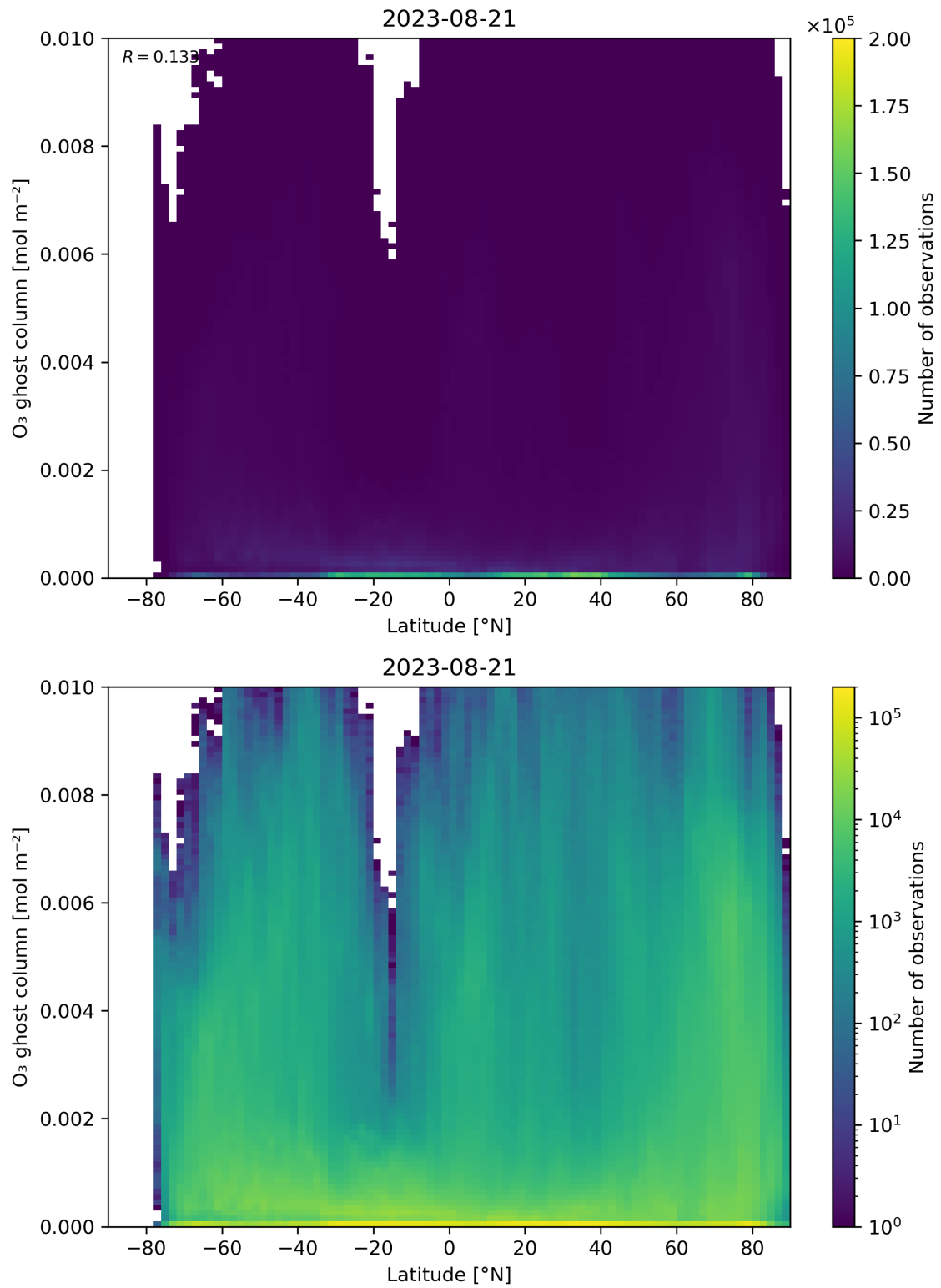
Figure 35: Scatter density plot of “Latitude” against “O 3 ghost column” for 2023-08-20 to 2023-08-22.
