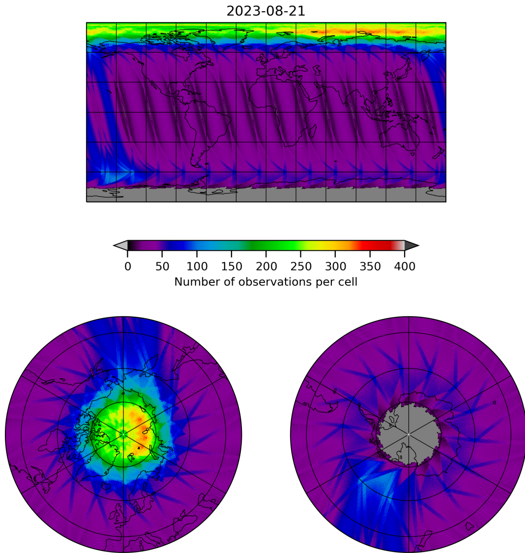
Figure 12: Map of the number of observations for 2023-08-20 to 2023-08-22
