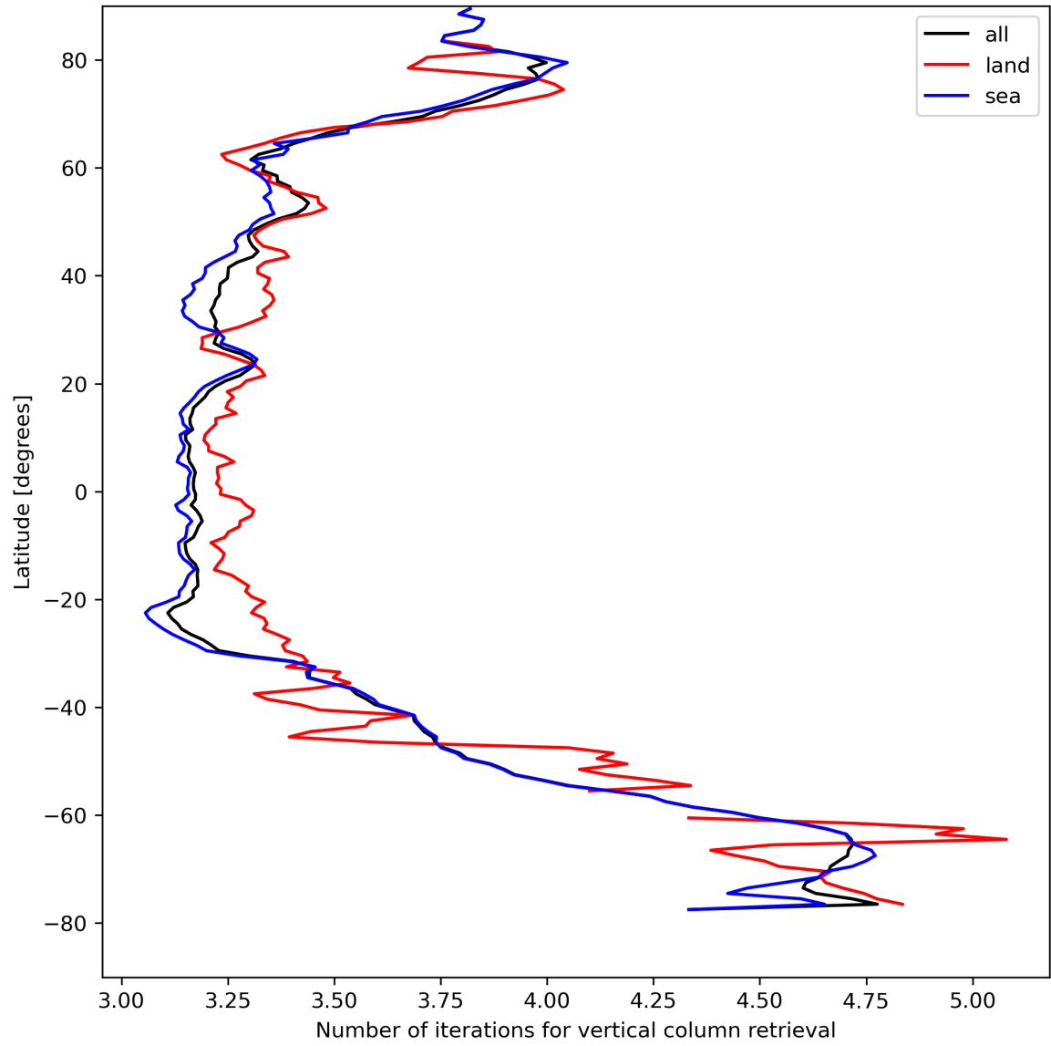
Figure 19: Zonal average of “Number of iterations for vertical column retrieval” for 2023-08-20 to 2023-08-22.
