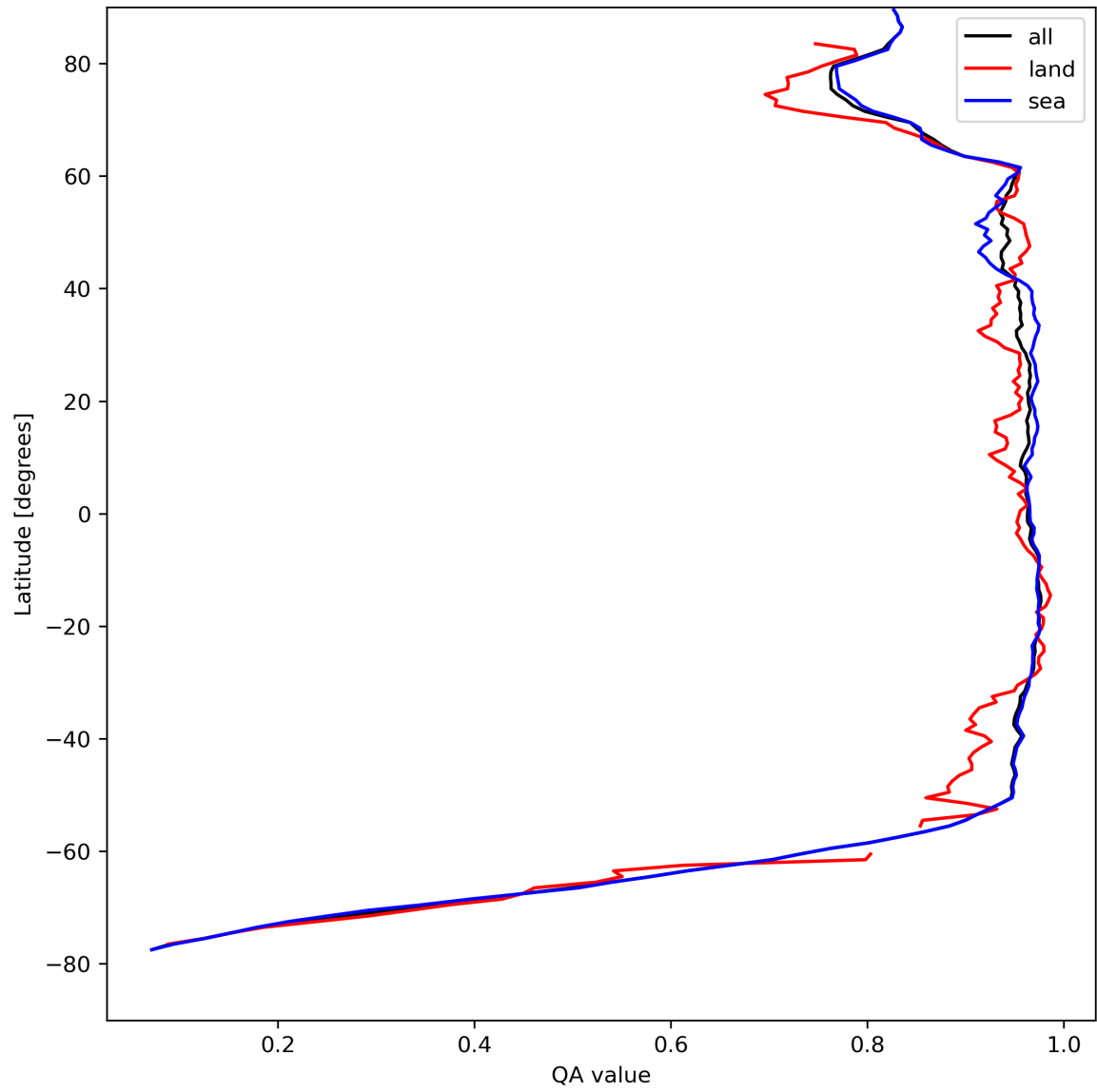
Figure 13: Zonal average of “QA value” for 2023-08-20 to 2023-08-22.
