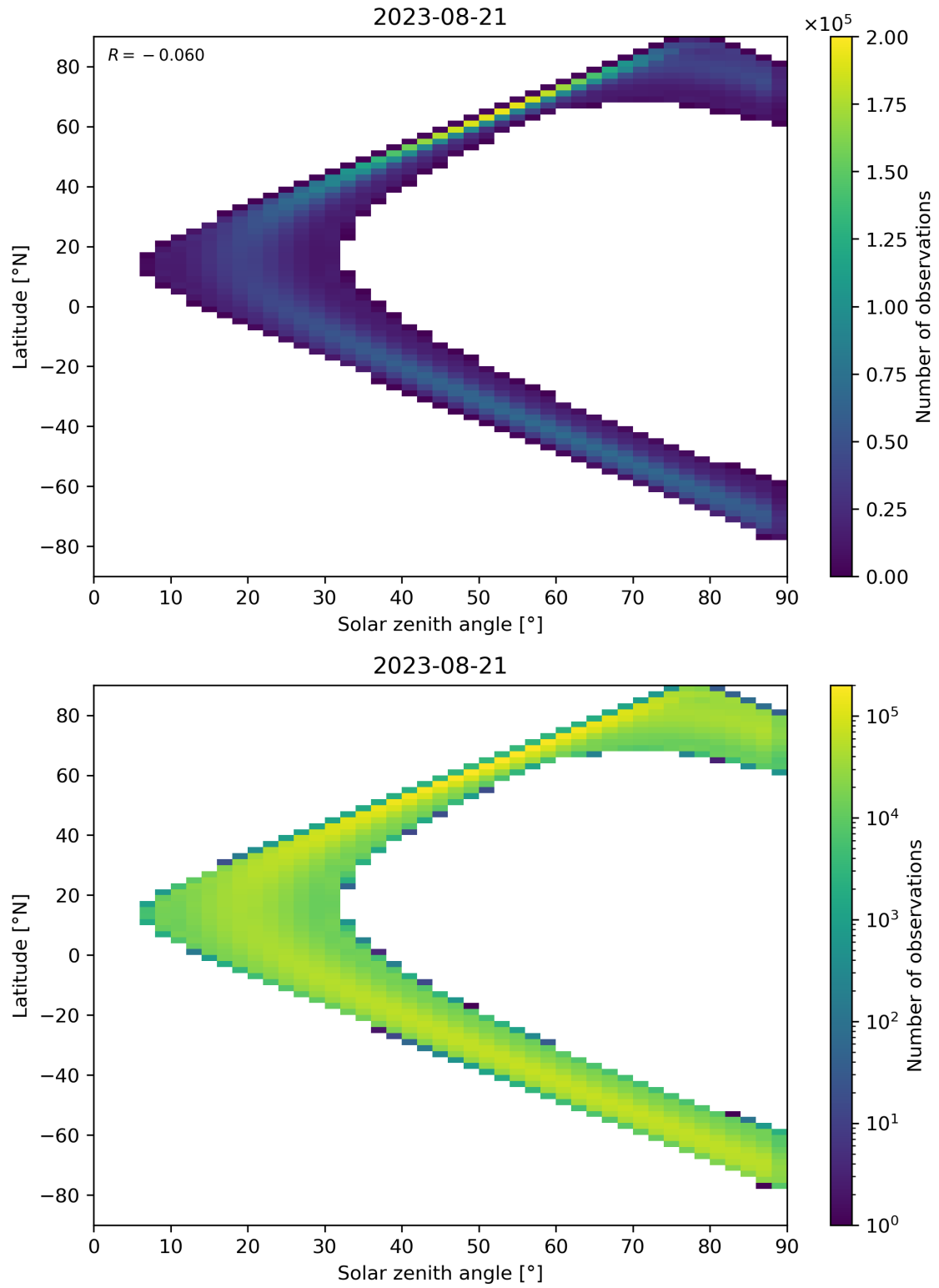
Figure 44: Scatter density plot of “Solar zenith angle” against “Latitude” for 2023-08-20 to 2023-08-22.
