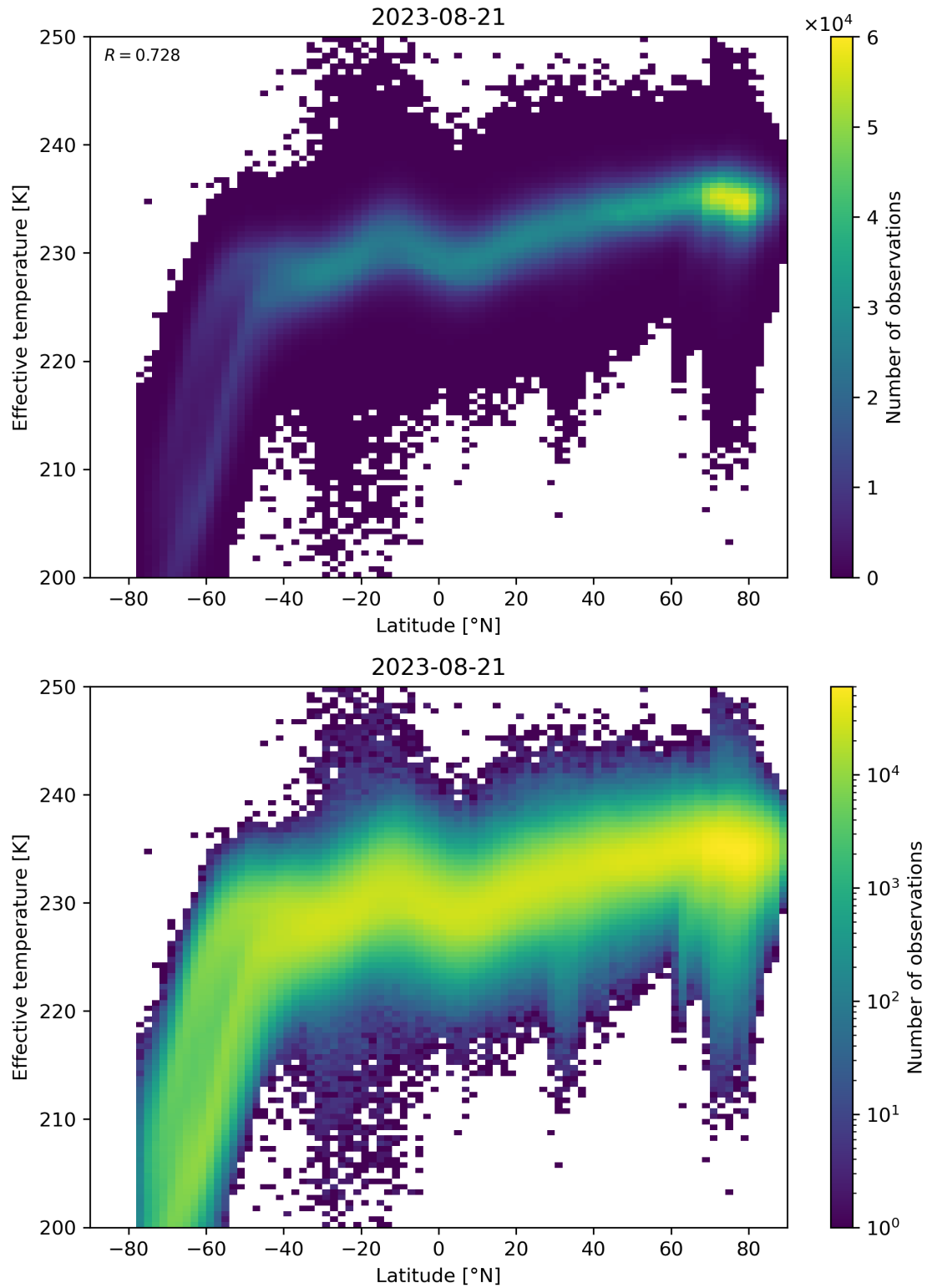
Figure 34: Scatter density plot of “Latitude” against “Effective temperature” for 2023-08-20 to 2023-08-22.
