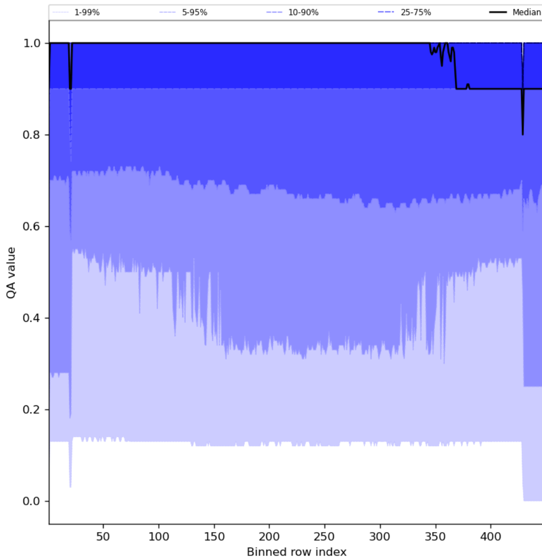
Figure 27: Along track statistics of “QA value” for 2023-08-20 to 2023-08-22
