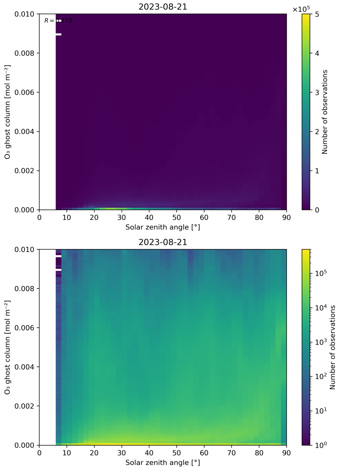
Figure 46: Scatter density plot of “Solar zenith angle” against “O 3 ghost column” for 2023-08-20 to 2023-08-22.
