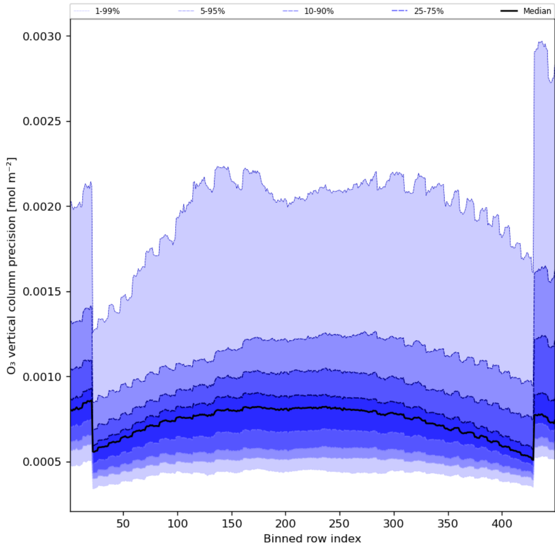
Figure 29: Along track statistics of “O 3 vertical column precision” for 2023-08-20 to 2023-08-22
