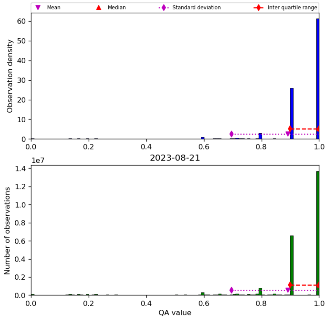
Figure 20: Histogram of “QA value” for 2023-08-20 to 2023-08-22
