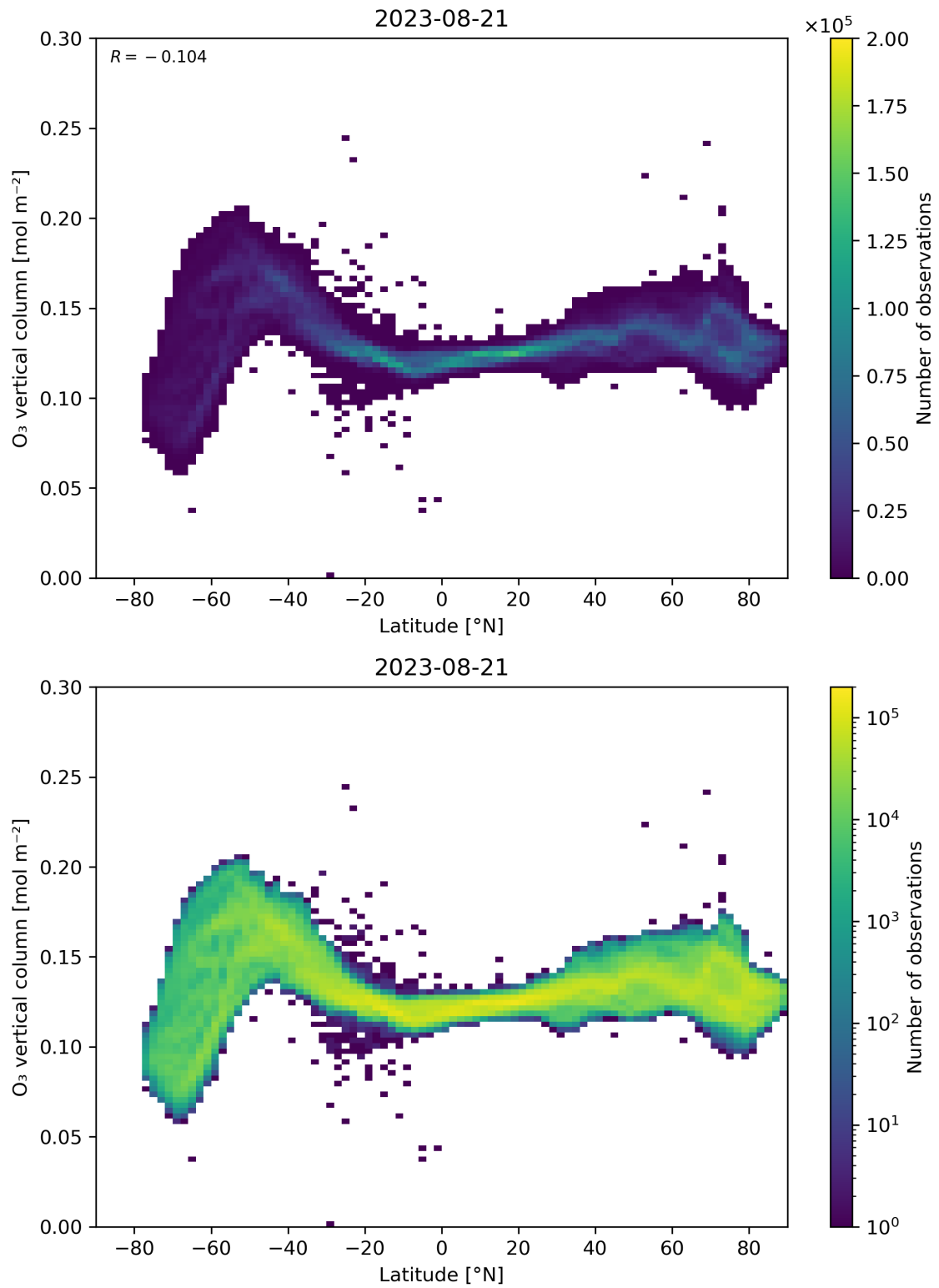
Figure 36: Scatter density plot of “Latitude” against “O 3 vertical column” for 2023-08-20 to 2023-08-22.
