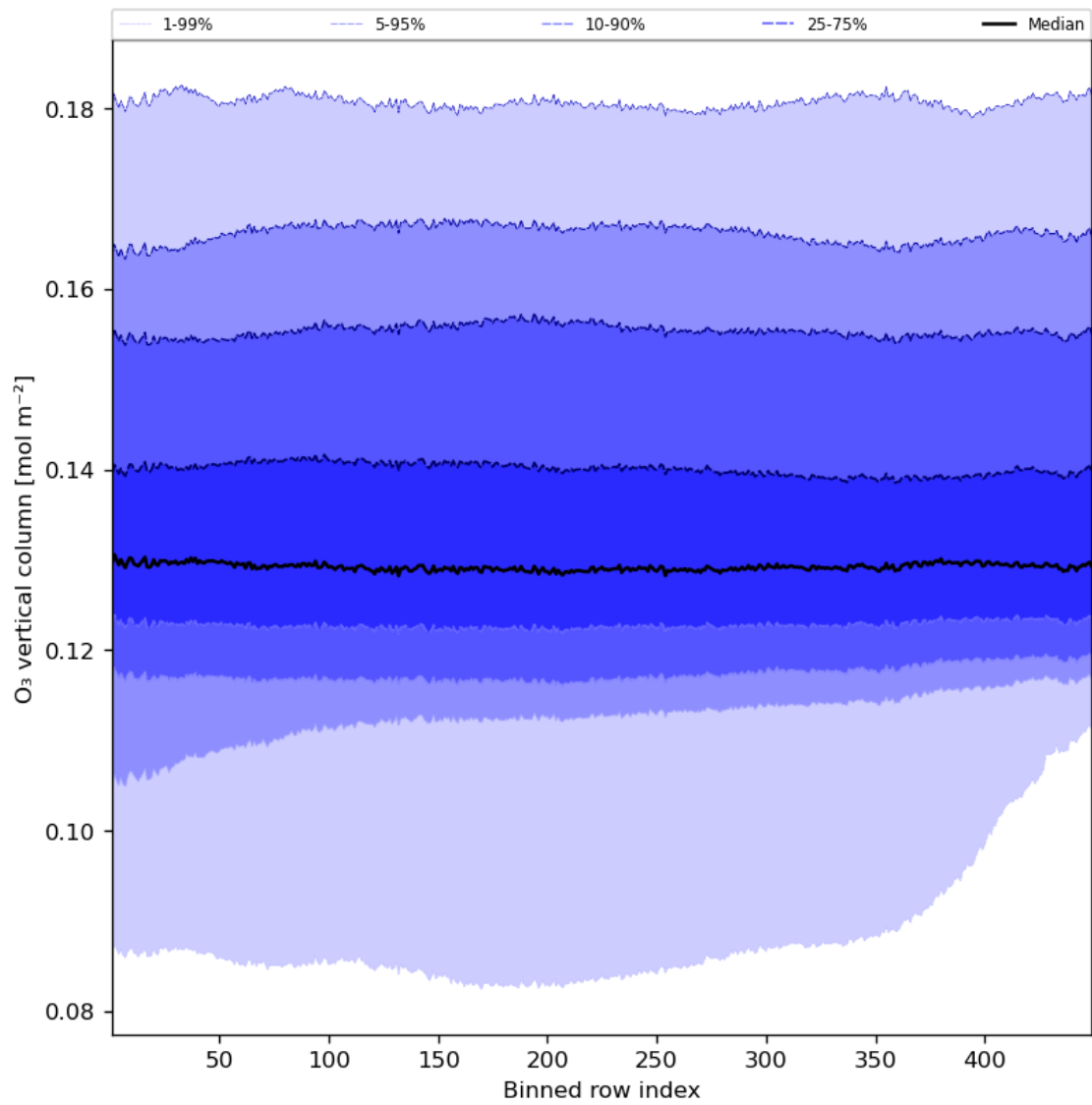
Figure 28: Along track statistics of “O 3 vertical column” for 2023-08-20 to 2023-08-22
