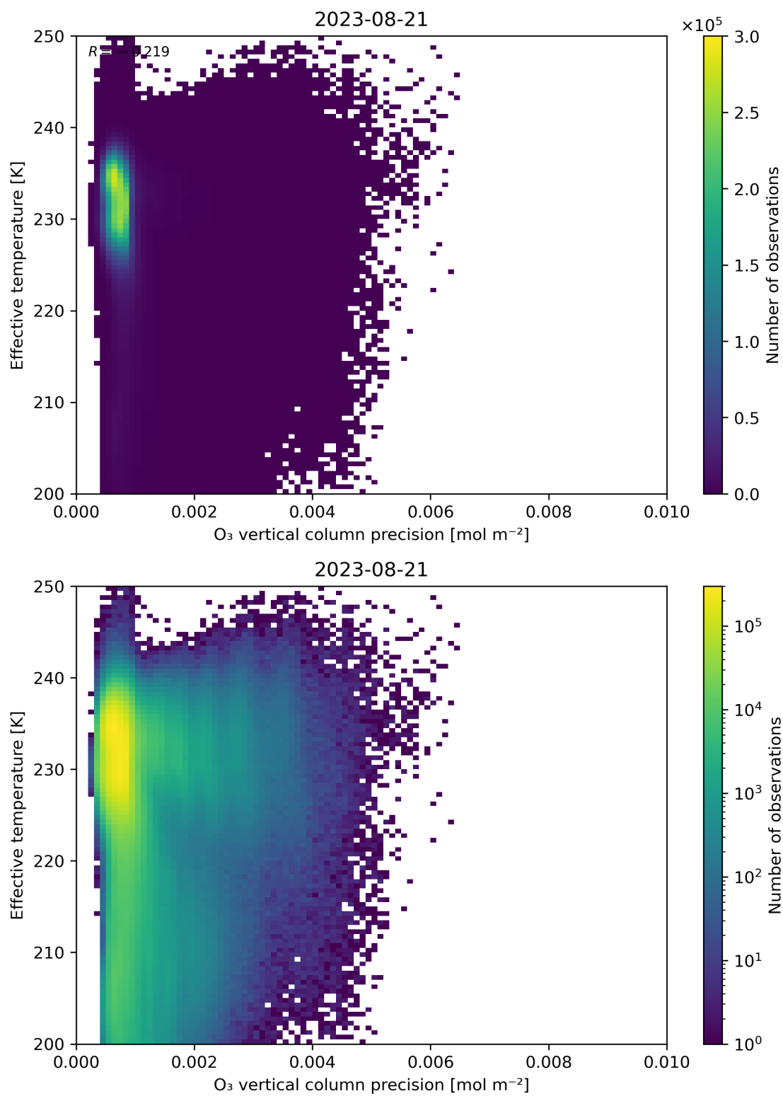
Figure 42: Scatter density plot of “O 3 vertical column precision” against “Effective temperature” for 2023-08-20 to 2023-08-22.
