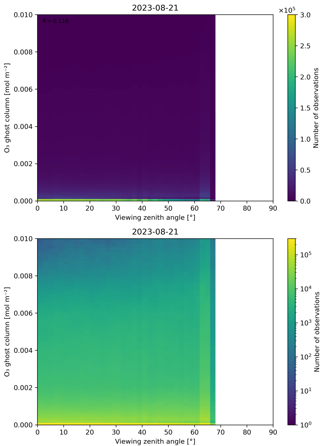
Figure 51: Scatter density plot of “Viewing zenith angle” against “O 3 ghost column” for 2023-08-20 to 2023-08-22.
