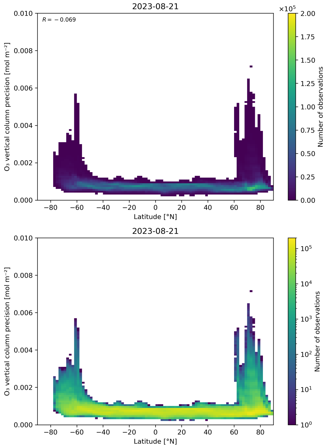
Figure 37: Scatter density plot of “Latitude” against “O 3 vertical column precision” for 2023-08-20 to 2023-08-22.
