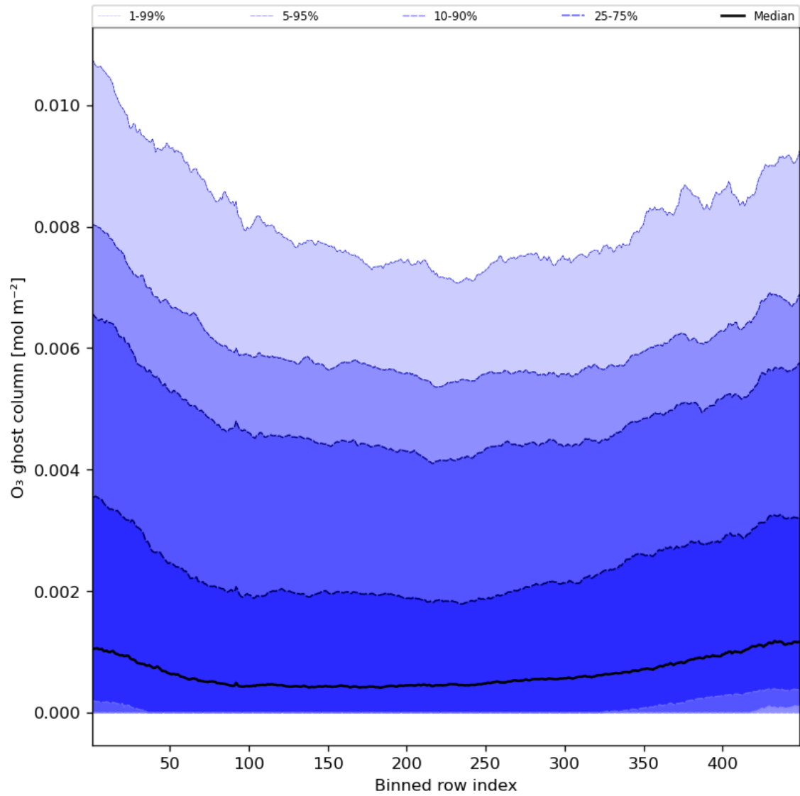
Figure 32: Along track statistics of “O 3 ghost column” for 2023-08-20 to 2023-08-22
