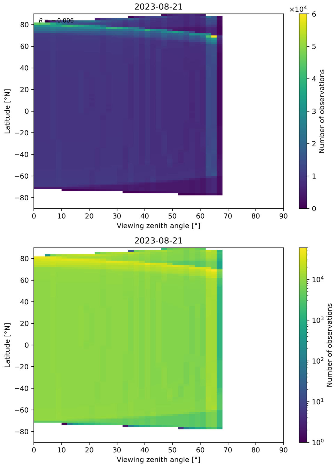
Figure 49: Scatter density plot of “Viewing zenith angle” against “Latitude” for 2023-08-20 to 2023-08-22.
