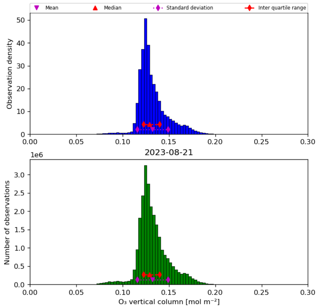
Figure 21: Histogram of “O 3 vertical column” for 2023-08-20 to 2023-08-22
