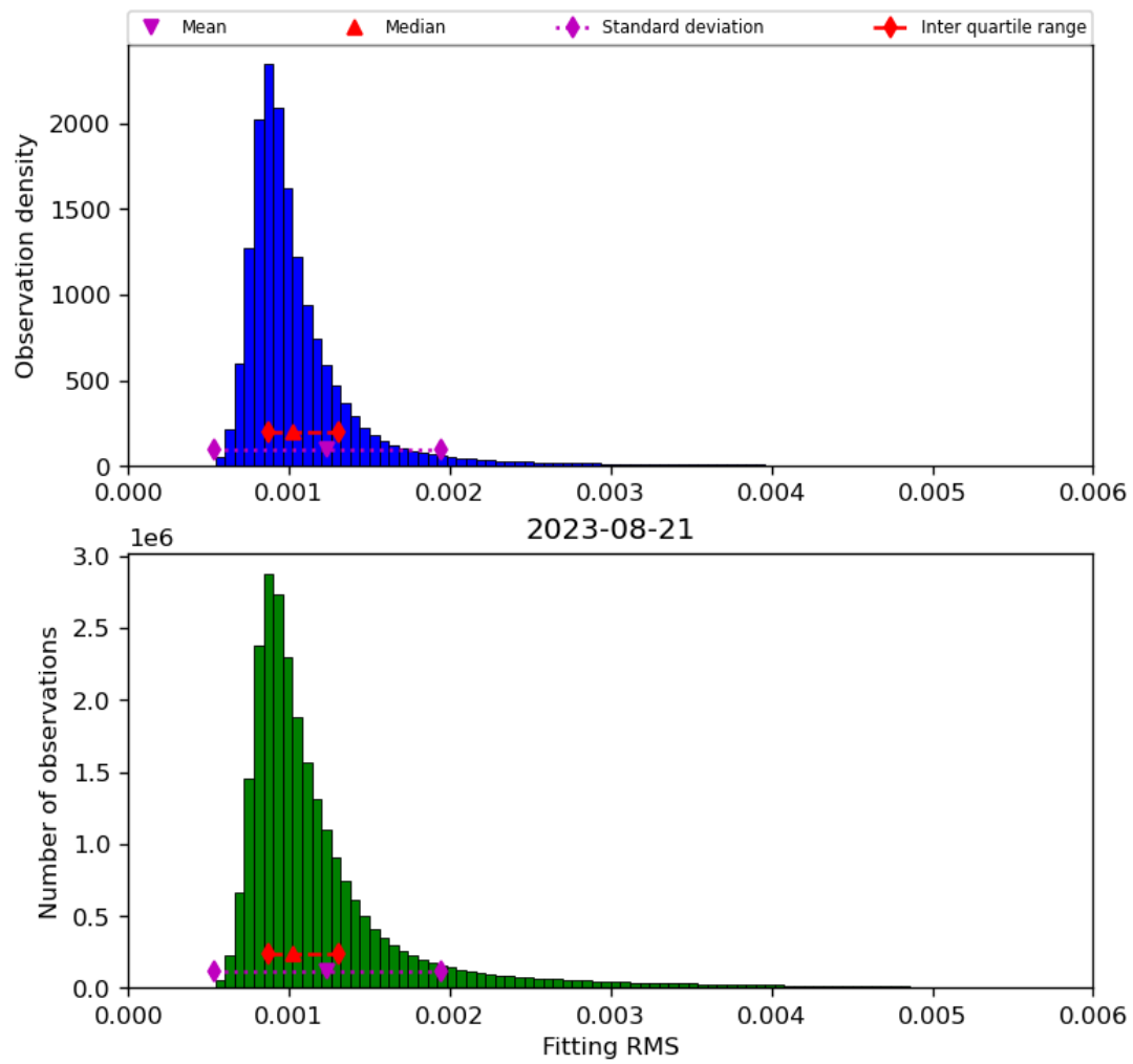
Figure 23: Histogram of “Fitting RMS” for 2023-08-20 to 2023-08-22
