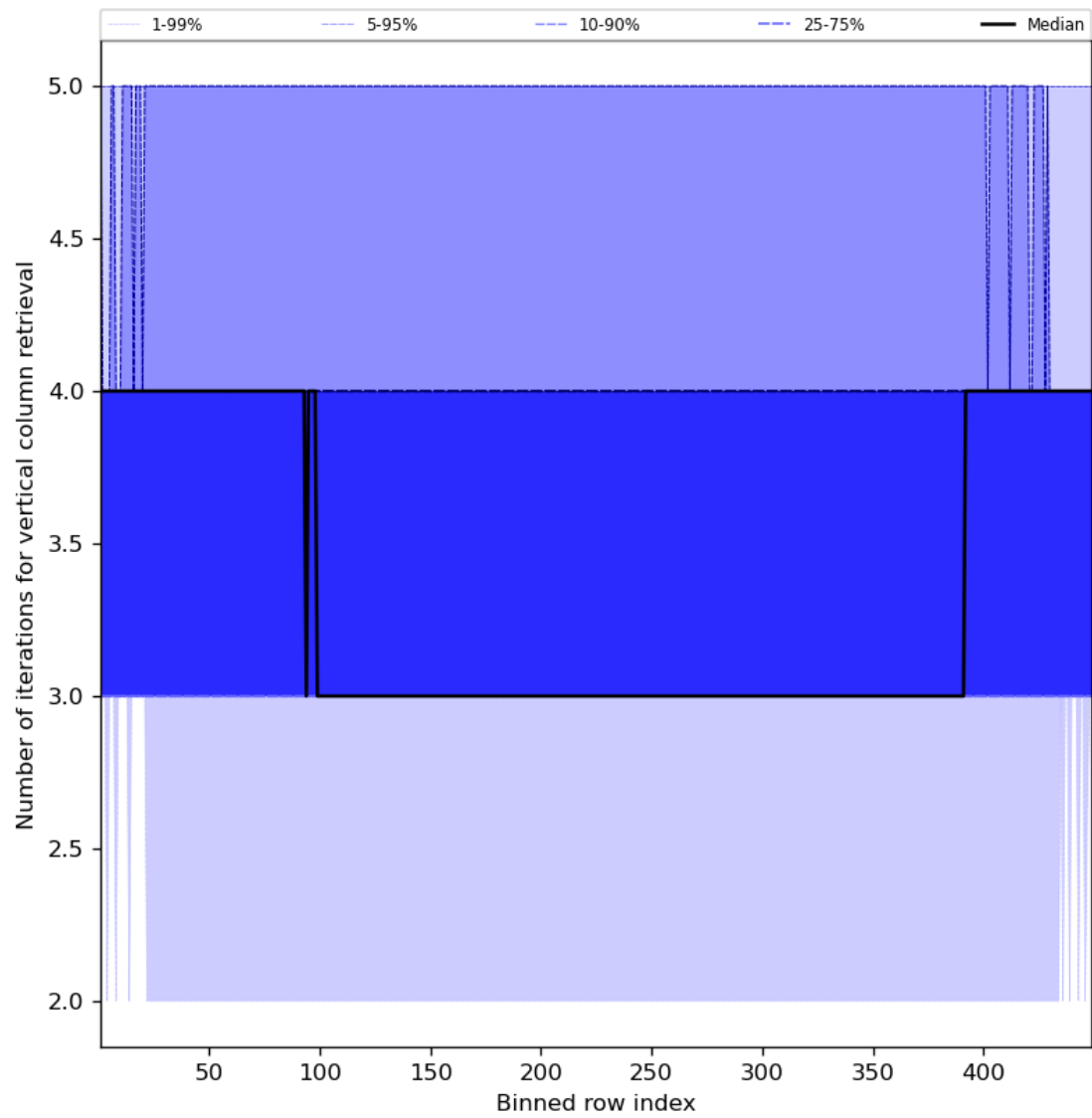
Figure 33: Along track statistics of “Number of iterations for vertical column retrieval” for 2023-08-20 to 2023-08-22
