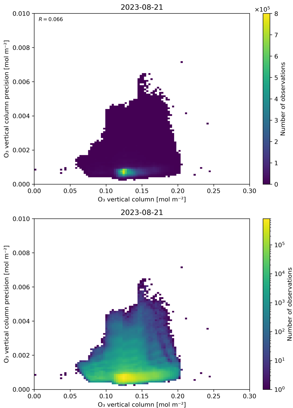
Figure 41: Scatter density plot of “O 3 vertical column” against “O 3 vertical column precision” for 2023-08-20 to 2023-08-22.
