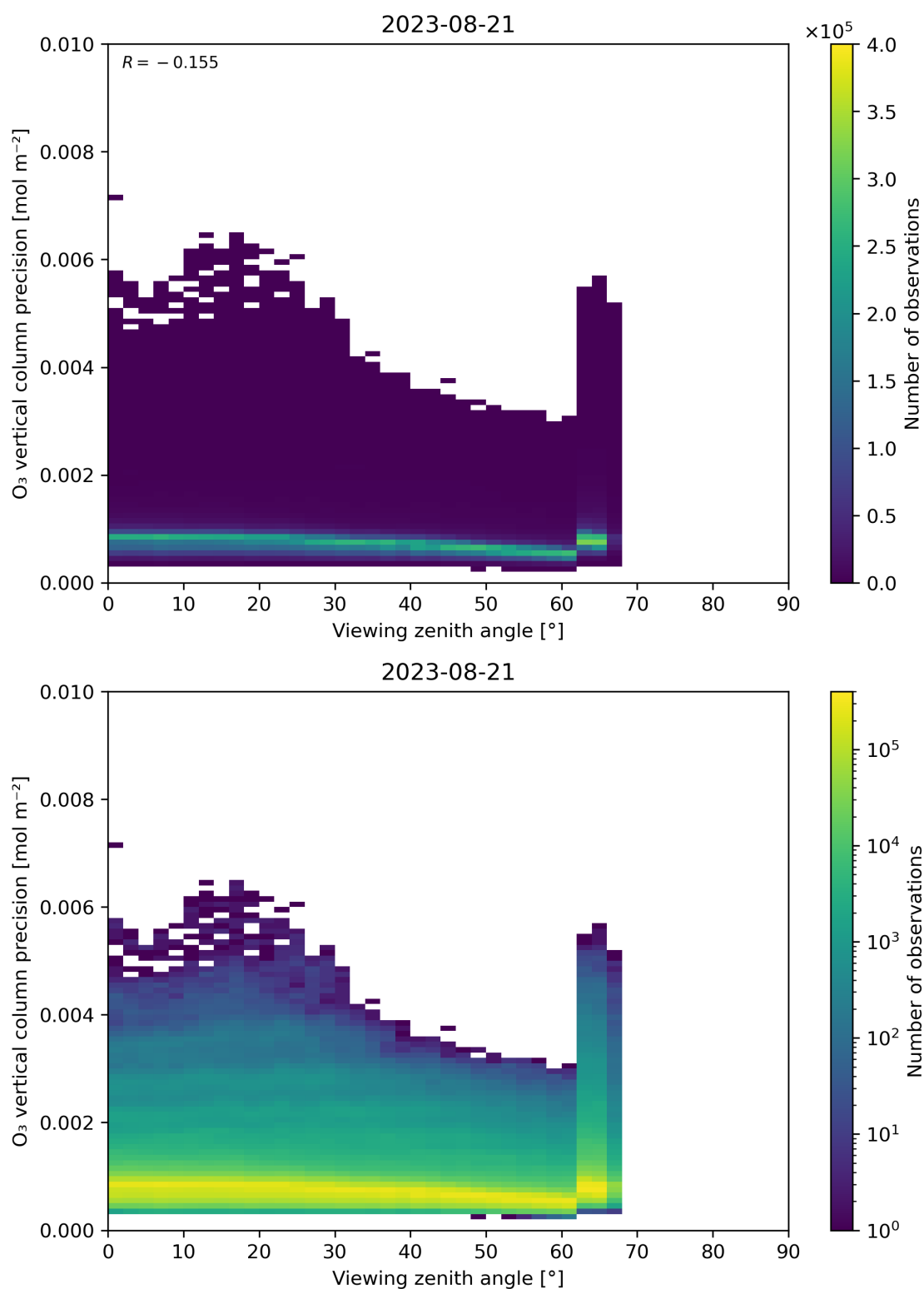
Figure 53: Scatter density plot of “Viewing zenith angle” against “O 3 vertical column precision” for 2023-08-20 to 2023-08-22.
