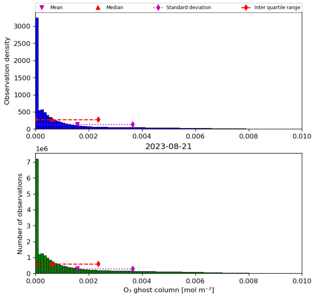
Figure 25: Histogram of “O 3 ghost column” for 2023-08-20 to 2023-08-22
