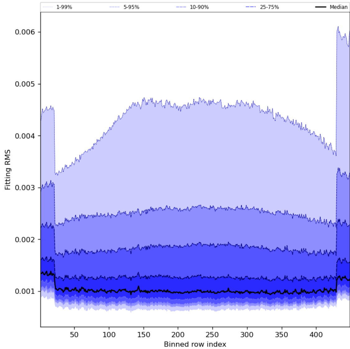
Figure 30: Along track statistics of “Fitting RMS” for 2023-08-20 to 2023-08-22
