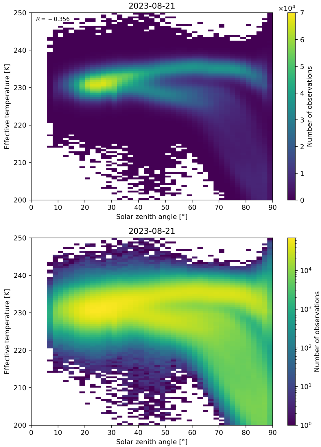
Figure 45: Scatter density plot of “Solar zenith angle” against “Effective temperature” for 2023-08-20 to 2023-08-22.
