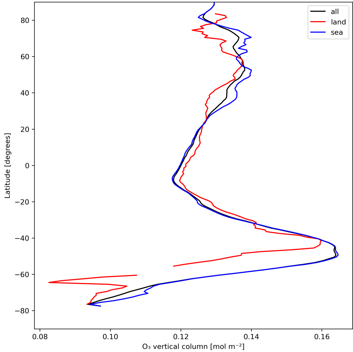
Figure 14: Zonal average of “O 3 vertical column” for 2023-08-20 to 2023-08-22.
