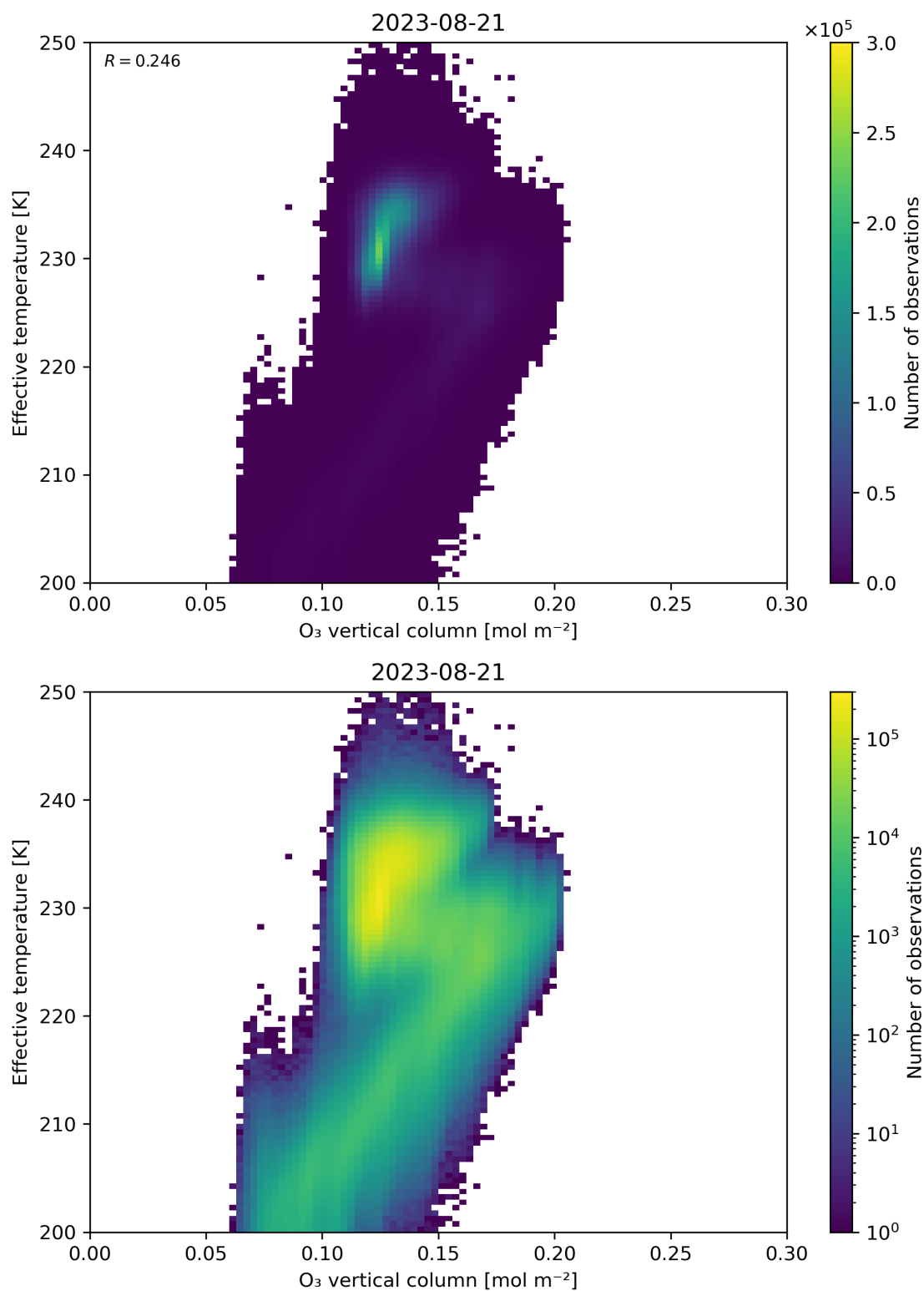
Figure 39: Scatter density plot of “O 3 vertical column” against “Effective temperature” for 2023-08-20 to 2023-08-22.
