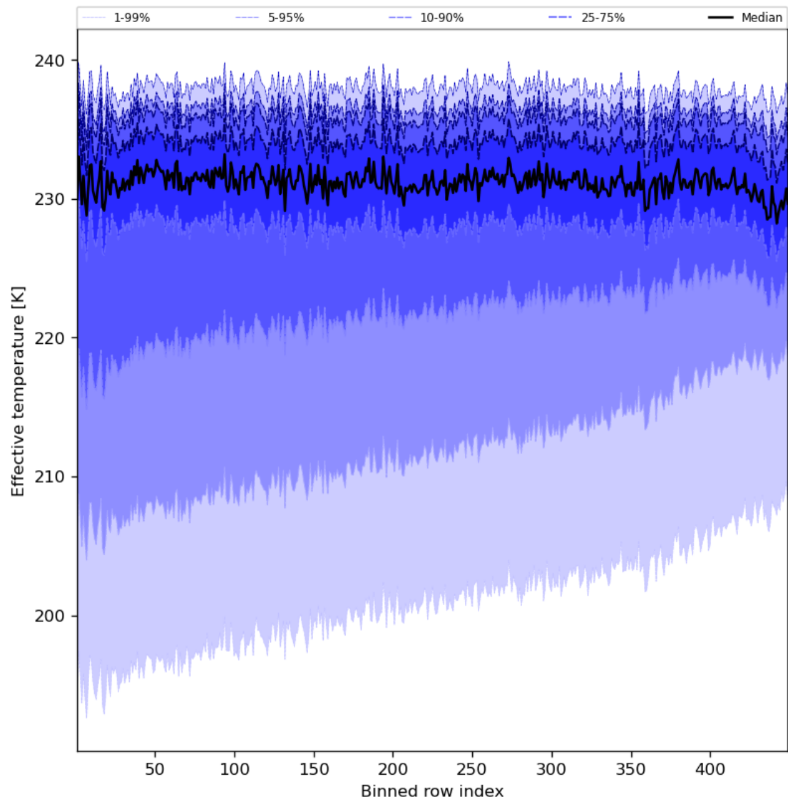
Figure 31: Along track statistics of “Effective temperature” for 2023-08-20 to 2023-08-22
