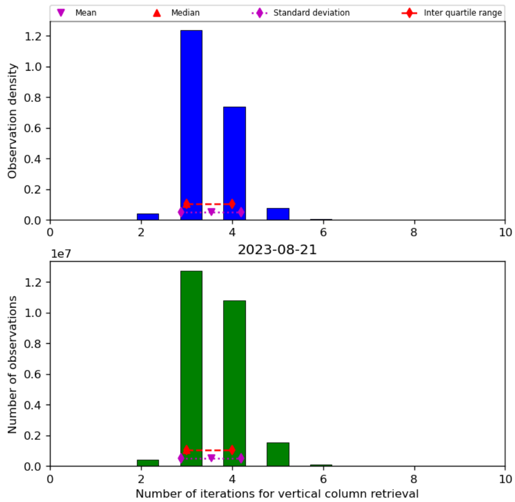
Figure 26: Histogram of “Number of iterations for vertical column retrieval” for 2023-08-20 to 2023-08-22
