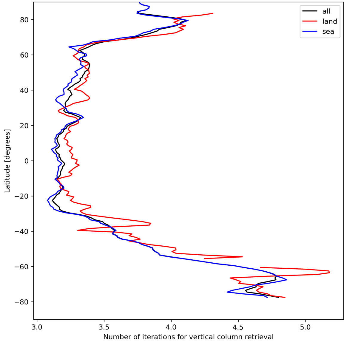
Figure 19: Zonal average of “Number of iterations for vertical column retrieval” for 2023-08-21 to 2023-08-23.
