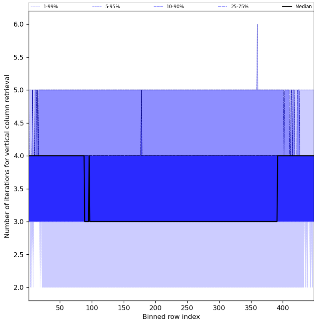
Figure 33: Along track statistics of “Number of iterations for vertical column retrieval” for 2023-08-21 to 2023-08-23
