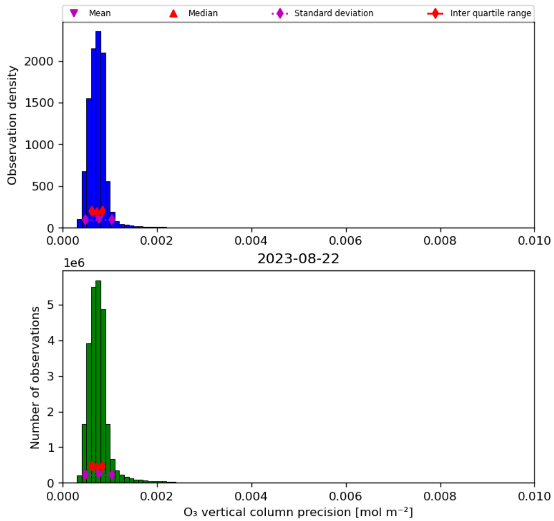
Figure 22: Histogram of “O 3 vertical column precision” for 2023-08-21 to 2023-08-23
