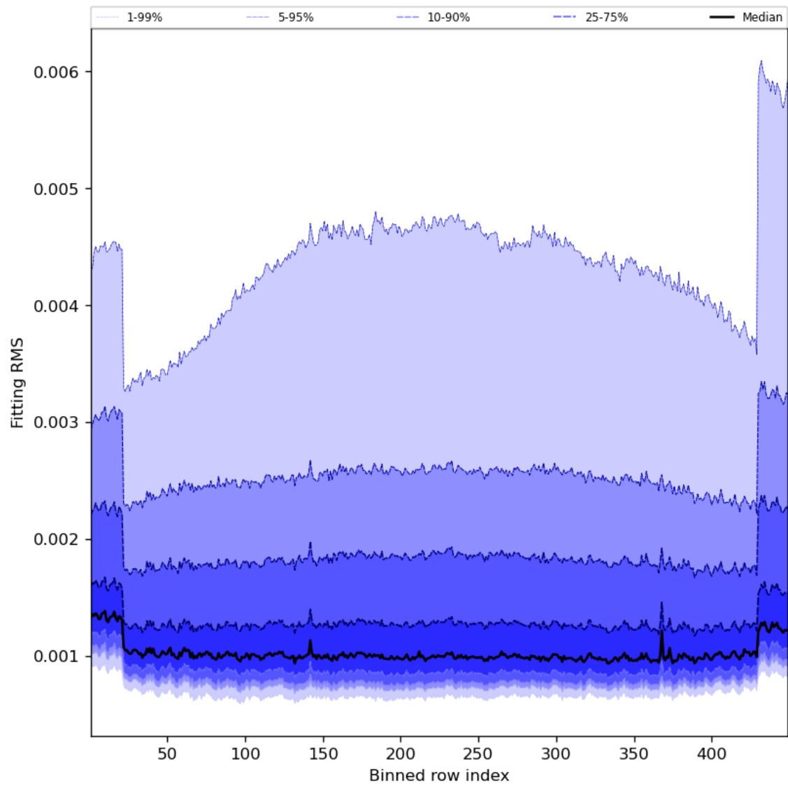
Figure 30: Along track statistics of “Fitting RMS” for 2023-08-21 to 2023-08-23
