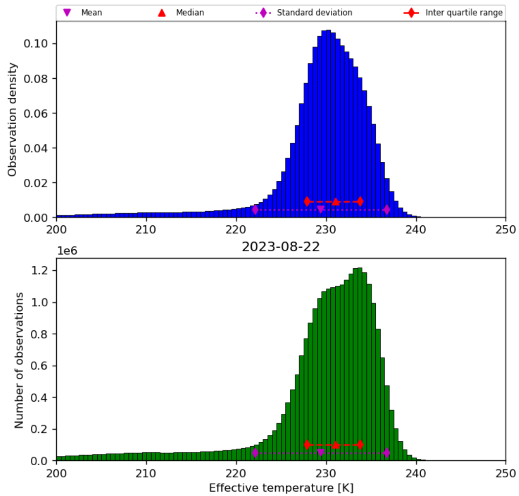
Figure 24: Histogram of “Effective temperature” for 2023-08-21 to 2023-08-23
