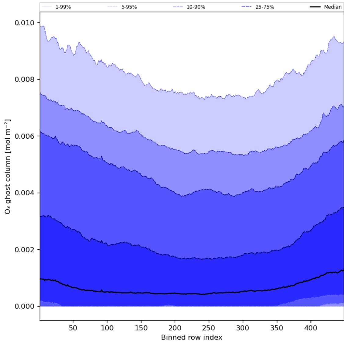
Figure 32: Along track statistics of "O 3 ghost column" for 2023-08-21 to 2023-08-23
