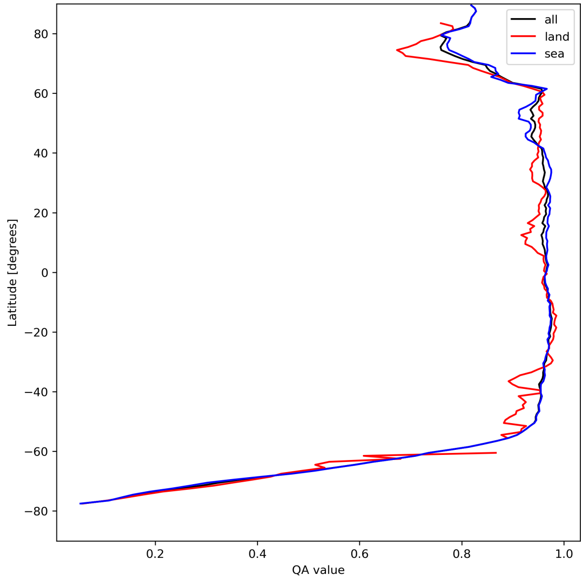
Figure 13: Zonal average of “QA value” for 2023-08-21 to 2023-08-23.
