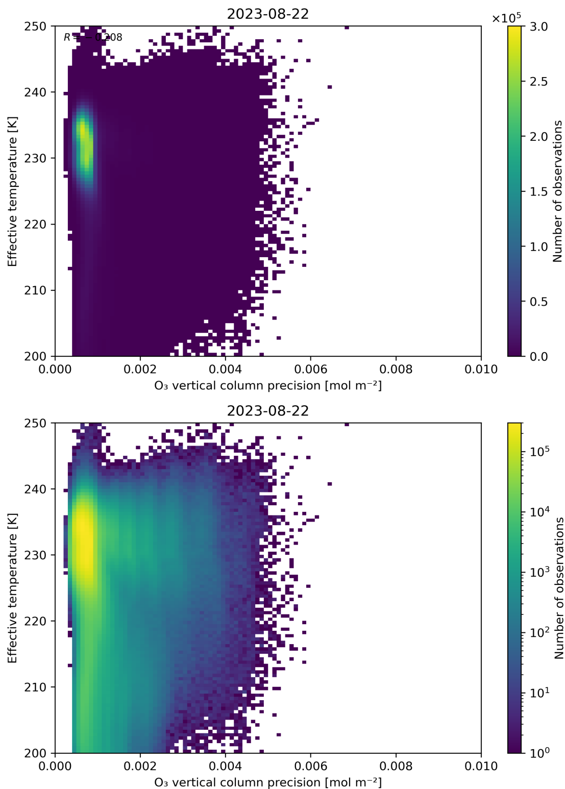
Figure 42: Scatter density plot of “O 3 vertical column precision” against “Effective temperature” for 2023-08-21 to 2023-08-23.
