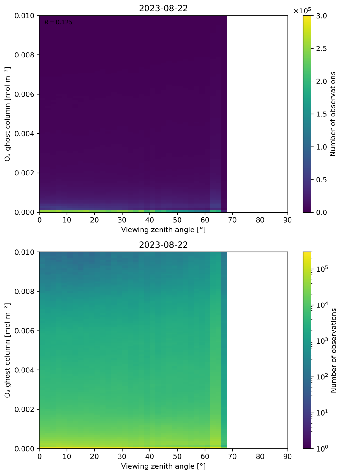
Figure 51: Scatter density plot of “Viewing zenith angle” against “O 3 ghost column” for 2023-08-21 to 2023-08-23.
