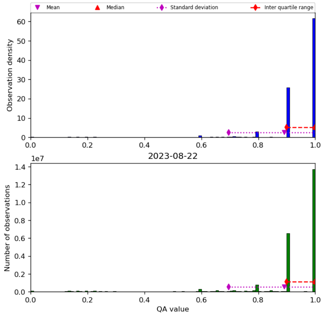
Figure 20: Histogram of “QA value” for 2023-08-21 to 2023-08-23
