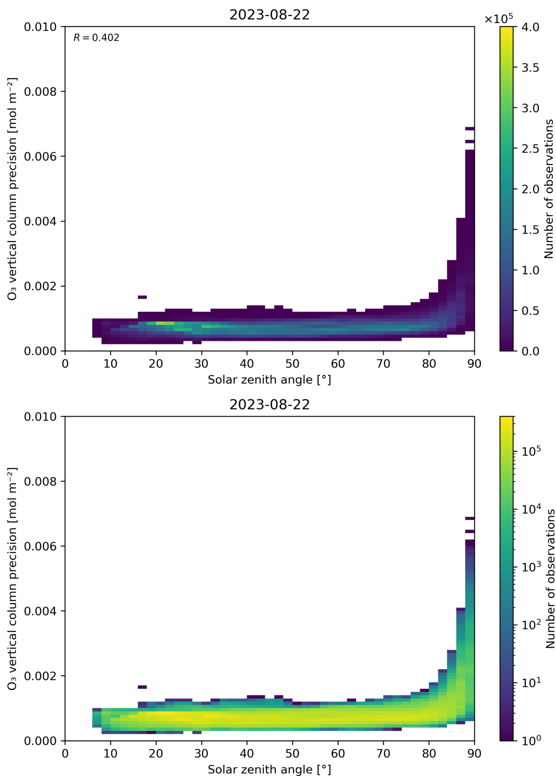
Figure 48: Scatter density plot of “Solar zenith angle” against “O 3 vertical column precision” for 2023-08-21 to 2023-08-23.
