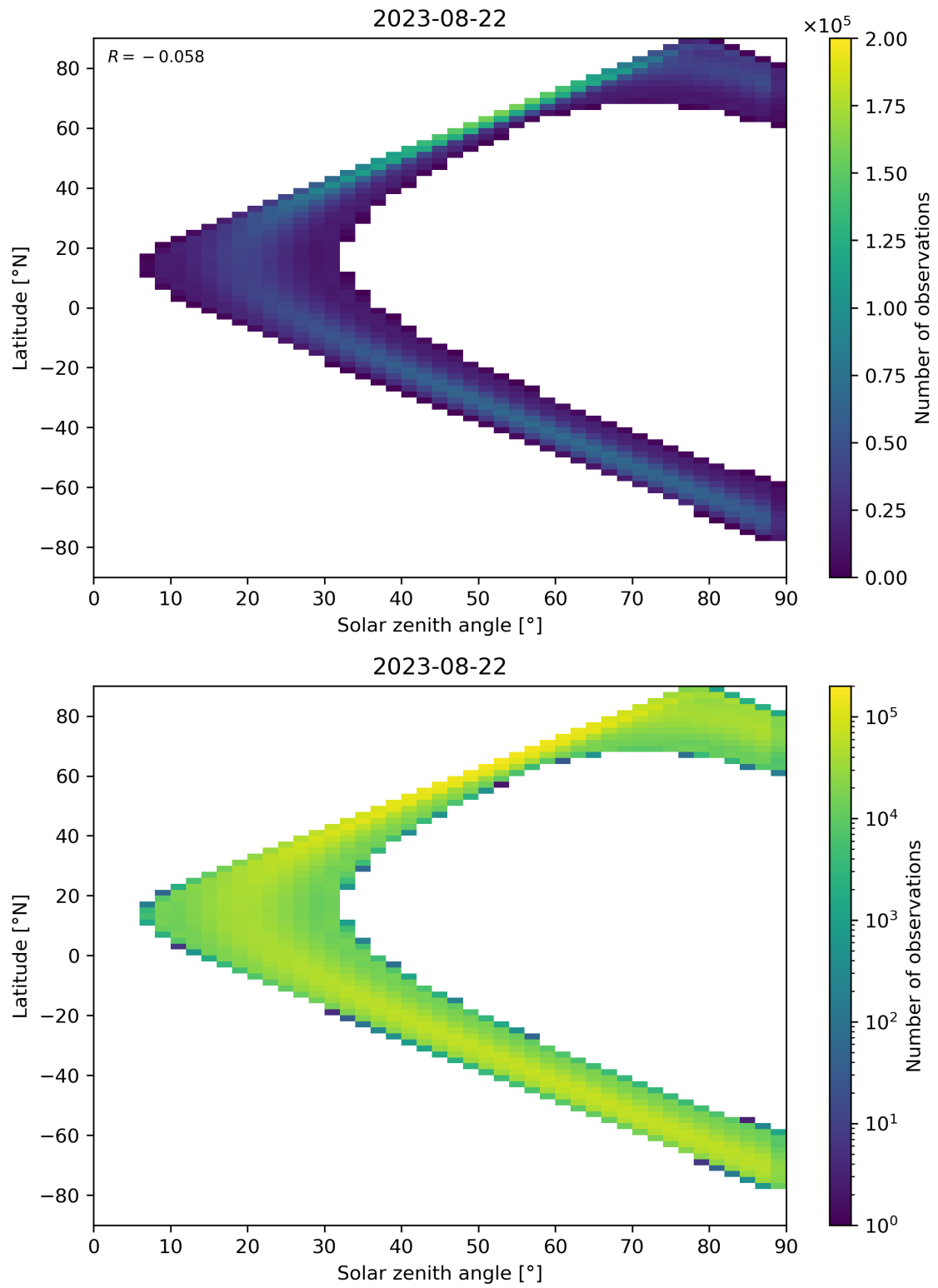
Figure 44: Scatter density plot of “Solar zenith angle” against “Latitude” for 2023-08-21 to 2023-08-23.
