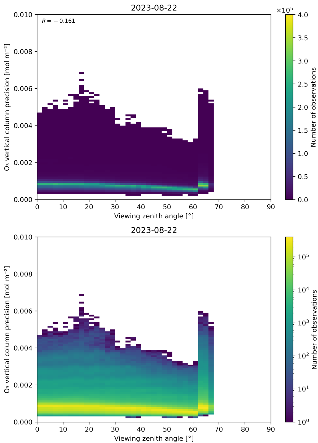
Figure 53: Scatter density plot of “Viewing zenith angle” against “O 3 vertical column precision” for 2023-08-21 to 2023-08-23.
