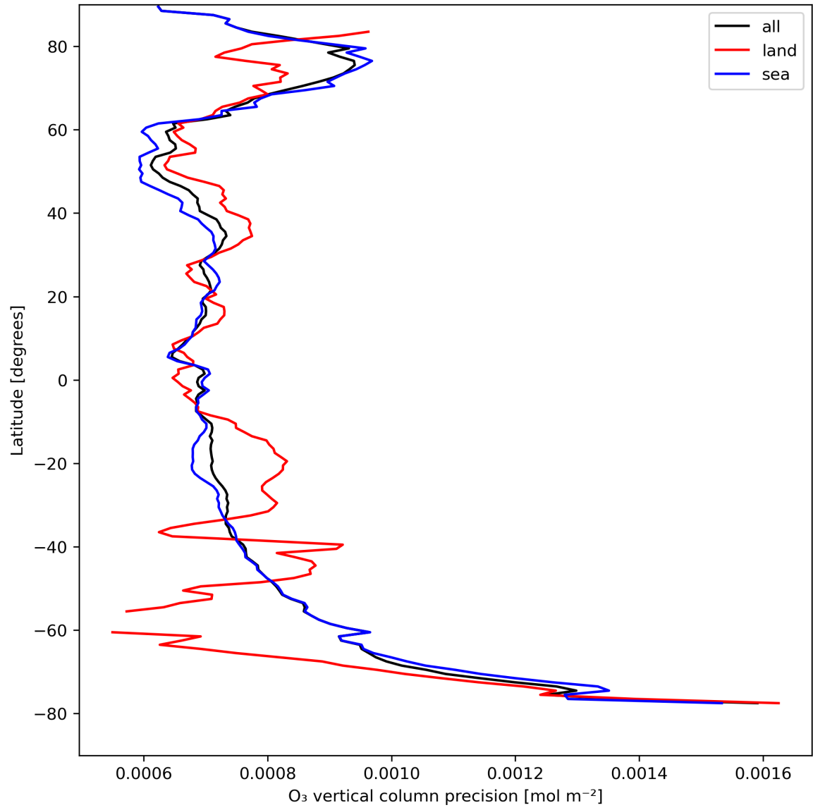
Figure 15: Zonal average of "O 3 vertical column precision" for 2023-08-21 to 2023-08-23.
