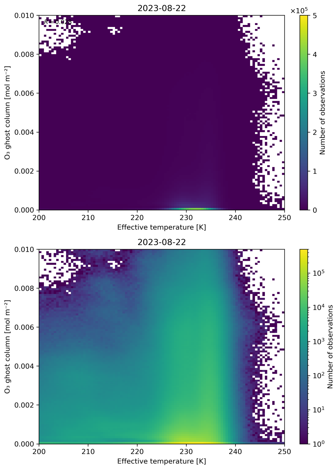
Figure 38: Scatter density plot of “Effective temperature” against “O 3 ghost column” for 2023-08-21 to 2023-08-23.
