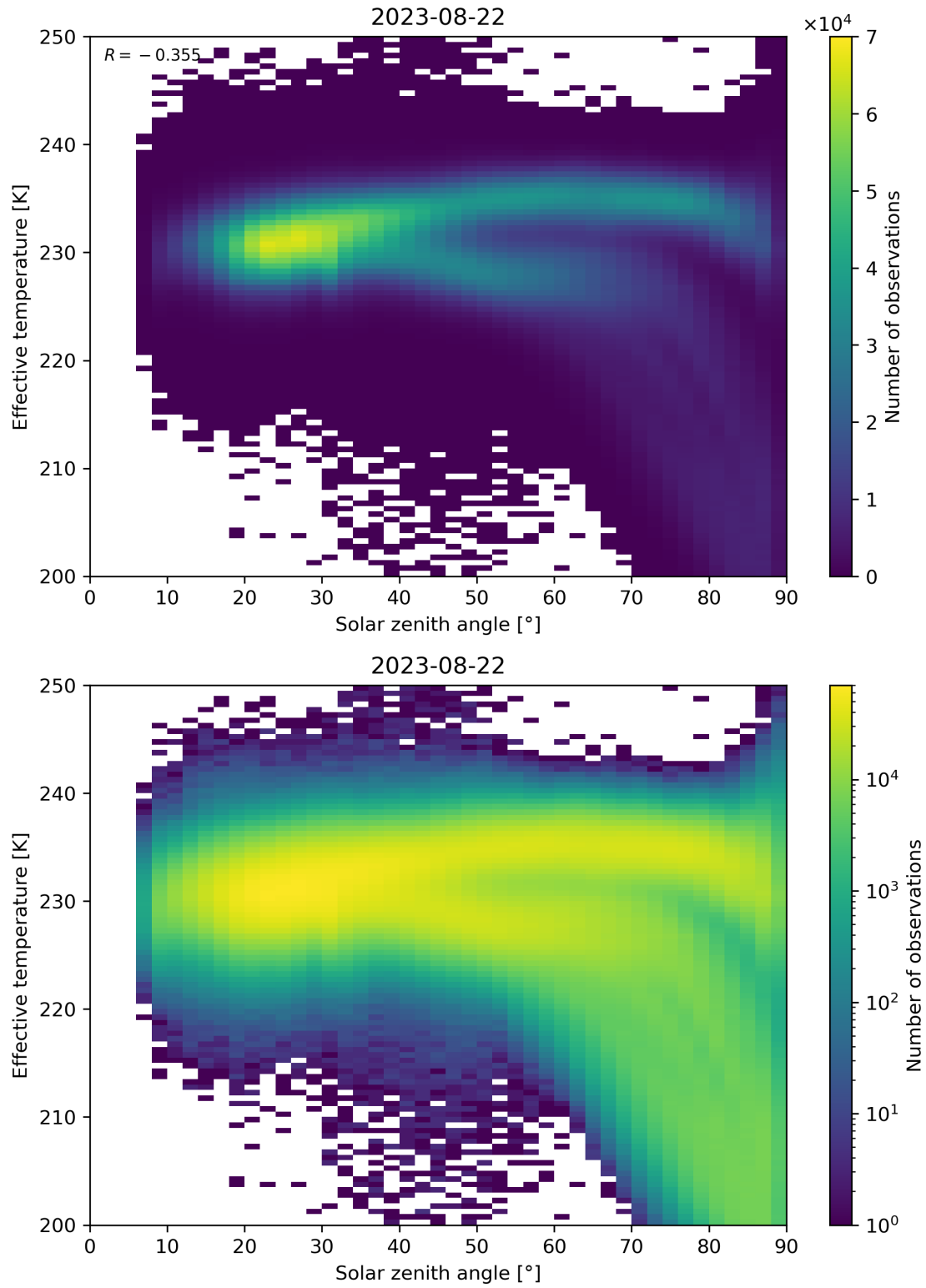
Figure 45: Scatter density plot of “Solar zenith angle” against “Effective temperature” for 2023-08-21 to 2023-08-23.
