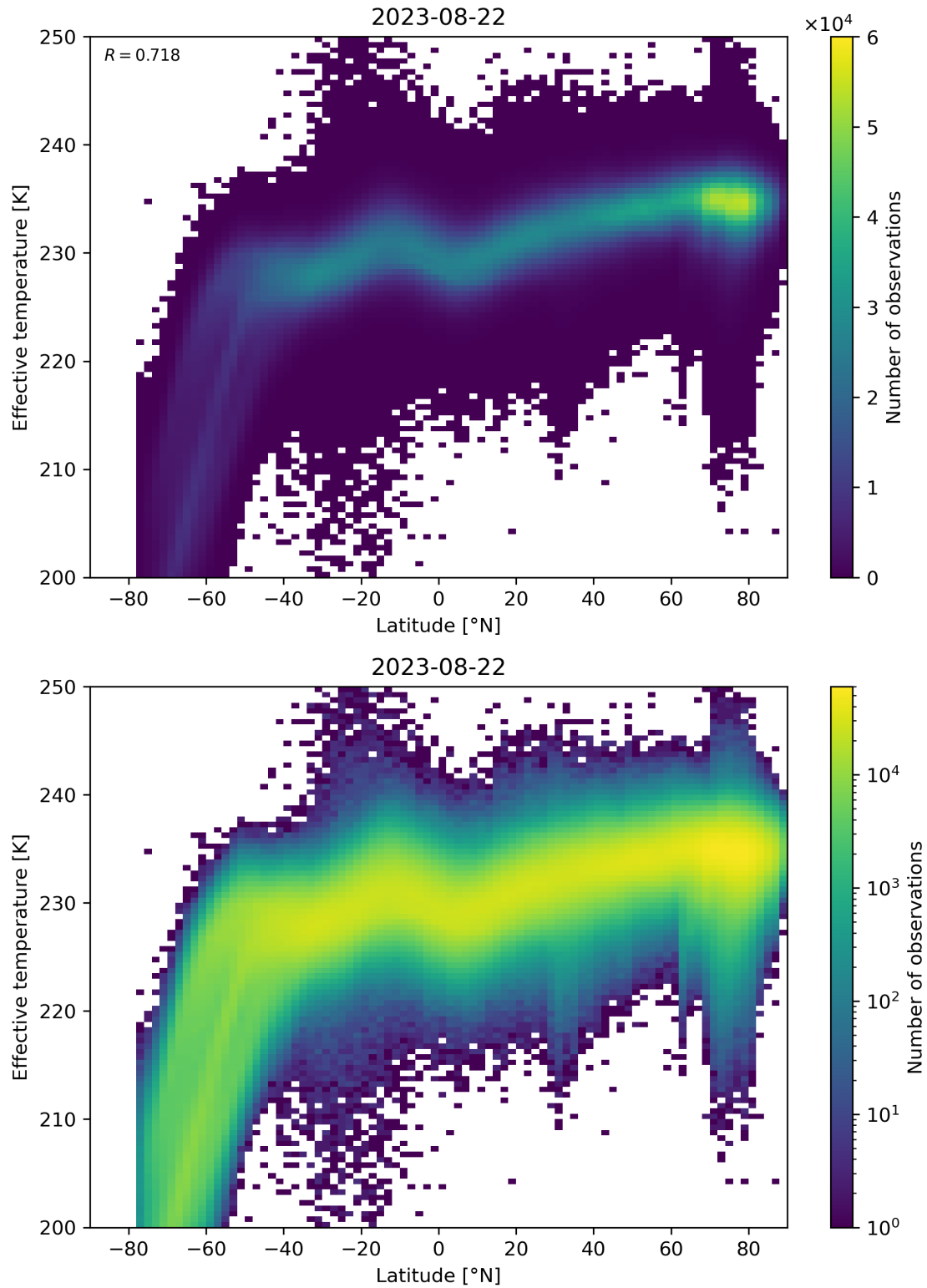
Figure 34: Scatter density plot of “Latitude” against “Effective temperature” for 2023-08-21 to 2023-08-23.
