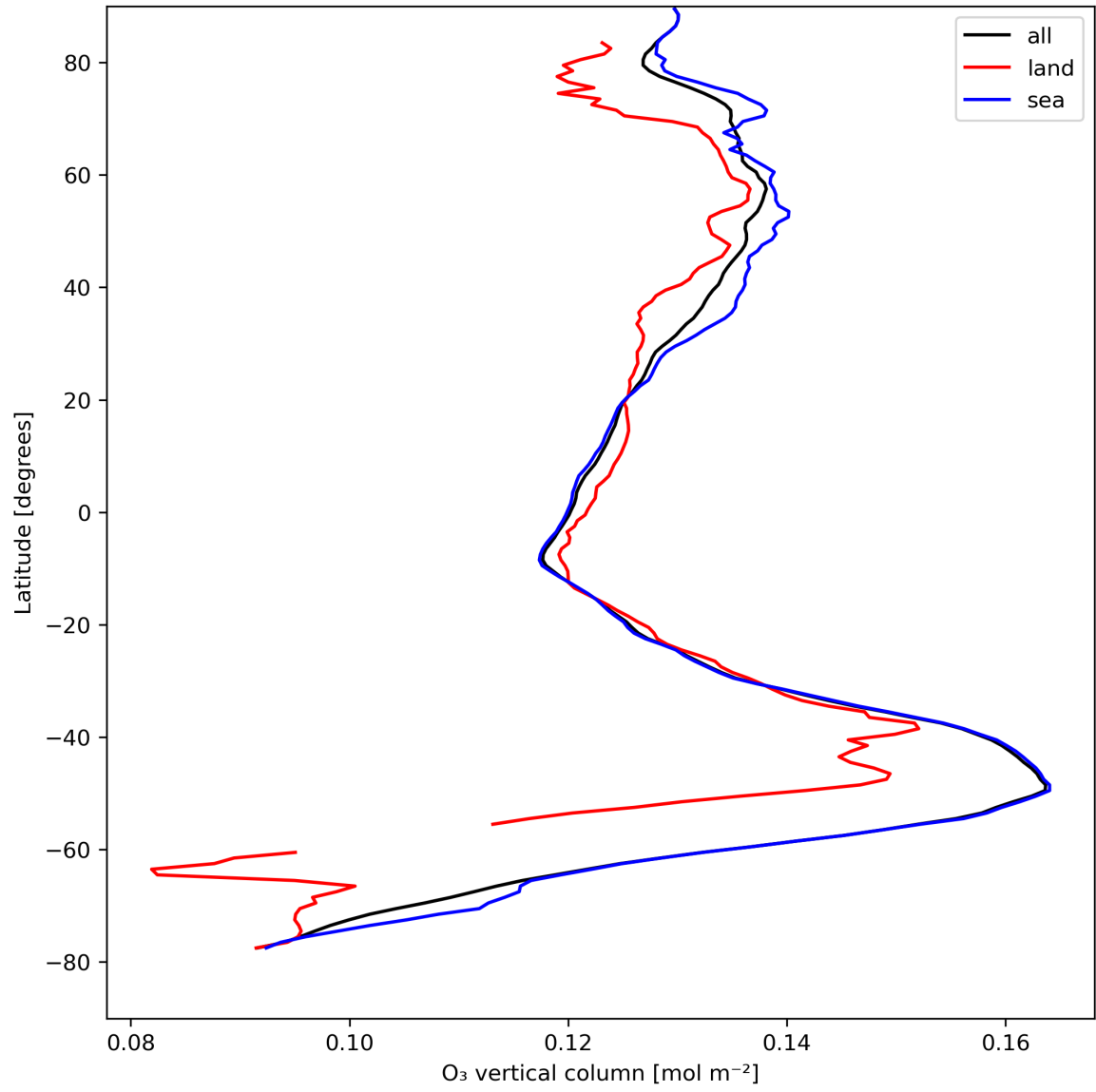
Figure 14: Zonal average of “O 3 vertical column” for 2023-08-21 to 2023-08-23.
