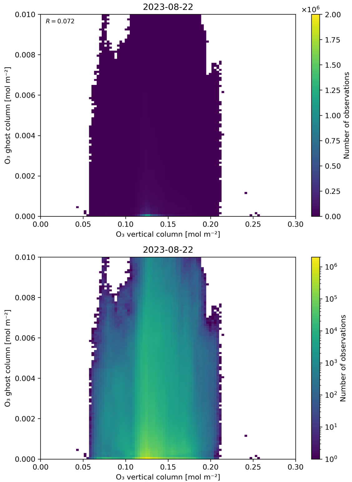
Figure 40: Scatter density plot of “O 3 vertical column” against “O 3 ghost column” for 2023-08-21 to 2023-08-23.
