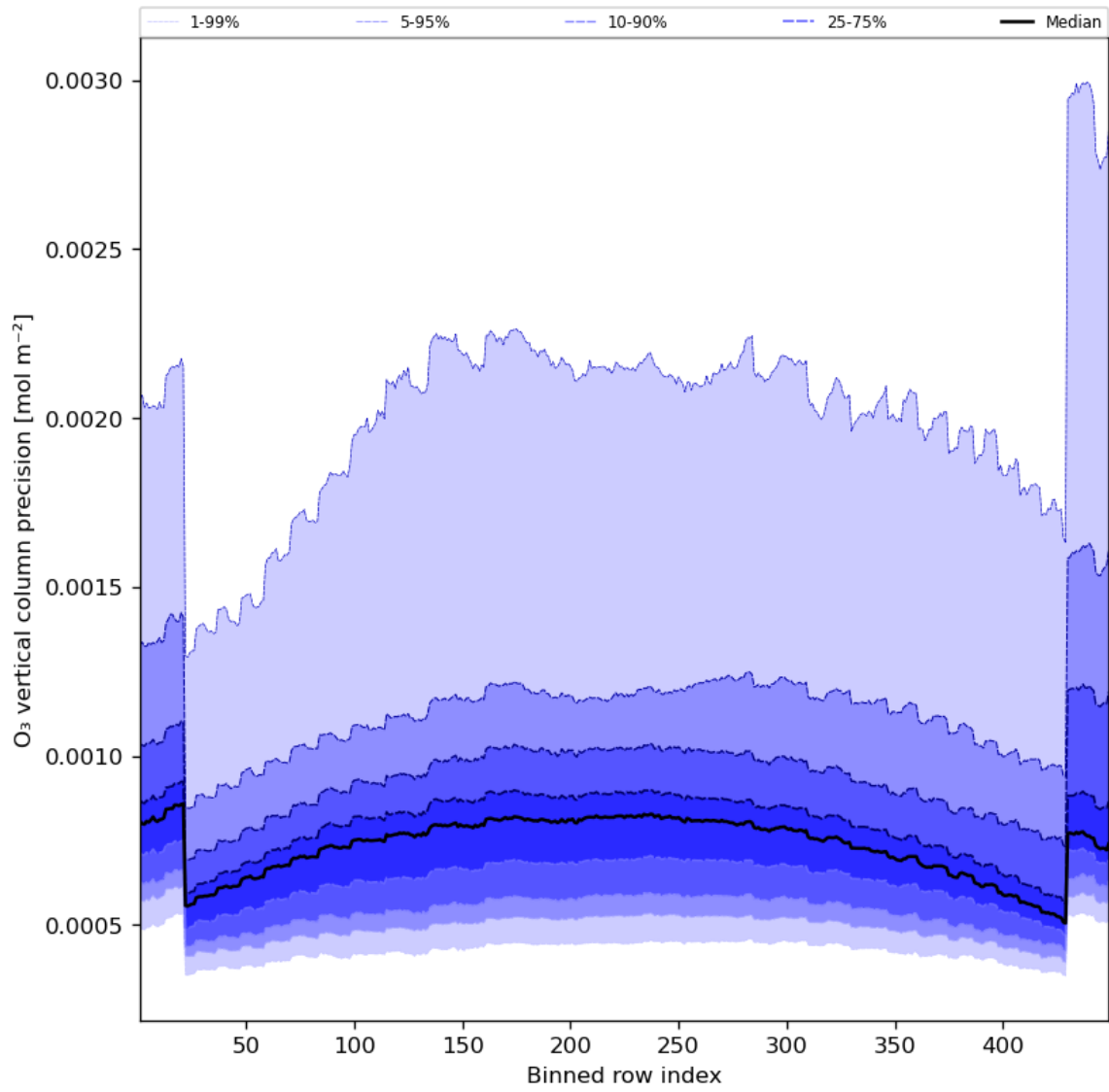
Figure 29: Along track statistics of “O 3 vertical column precision” for 2023-08-21 to 2023-08-23
