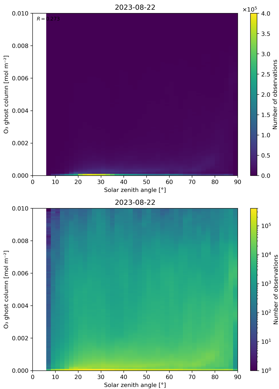
Figure 46: Scatter density plot of “Solar zenith angle” against “O 3 ghost column” for 2023-08-21 to 2023-08-23.
