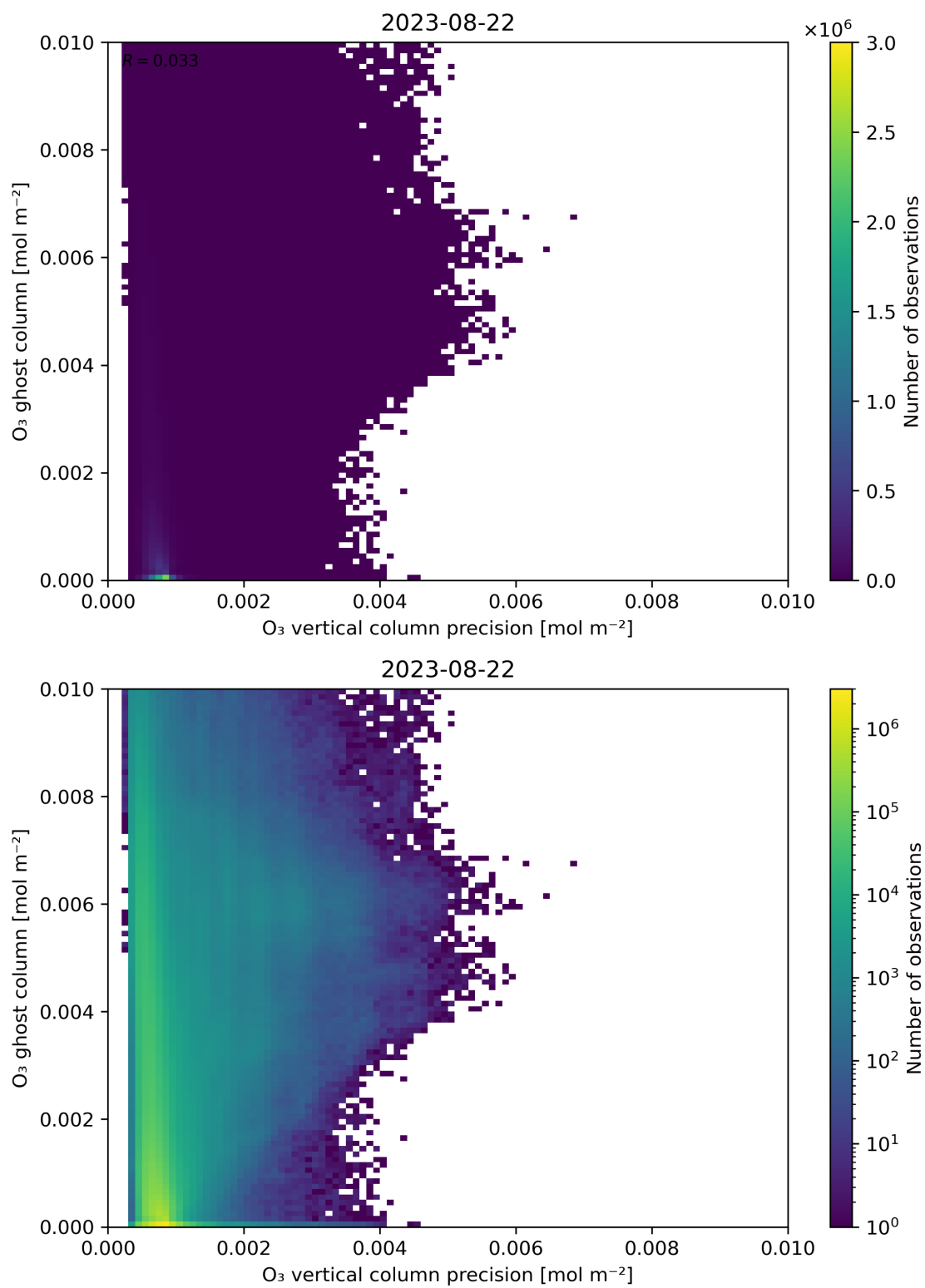
Figure 43: Scatter density plot of “ O_3 vertical column precision” against “ O_3 ghost column” for 2023-08-21 to 2023-08-23.
