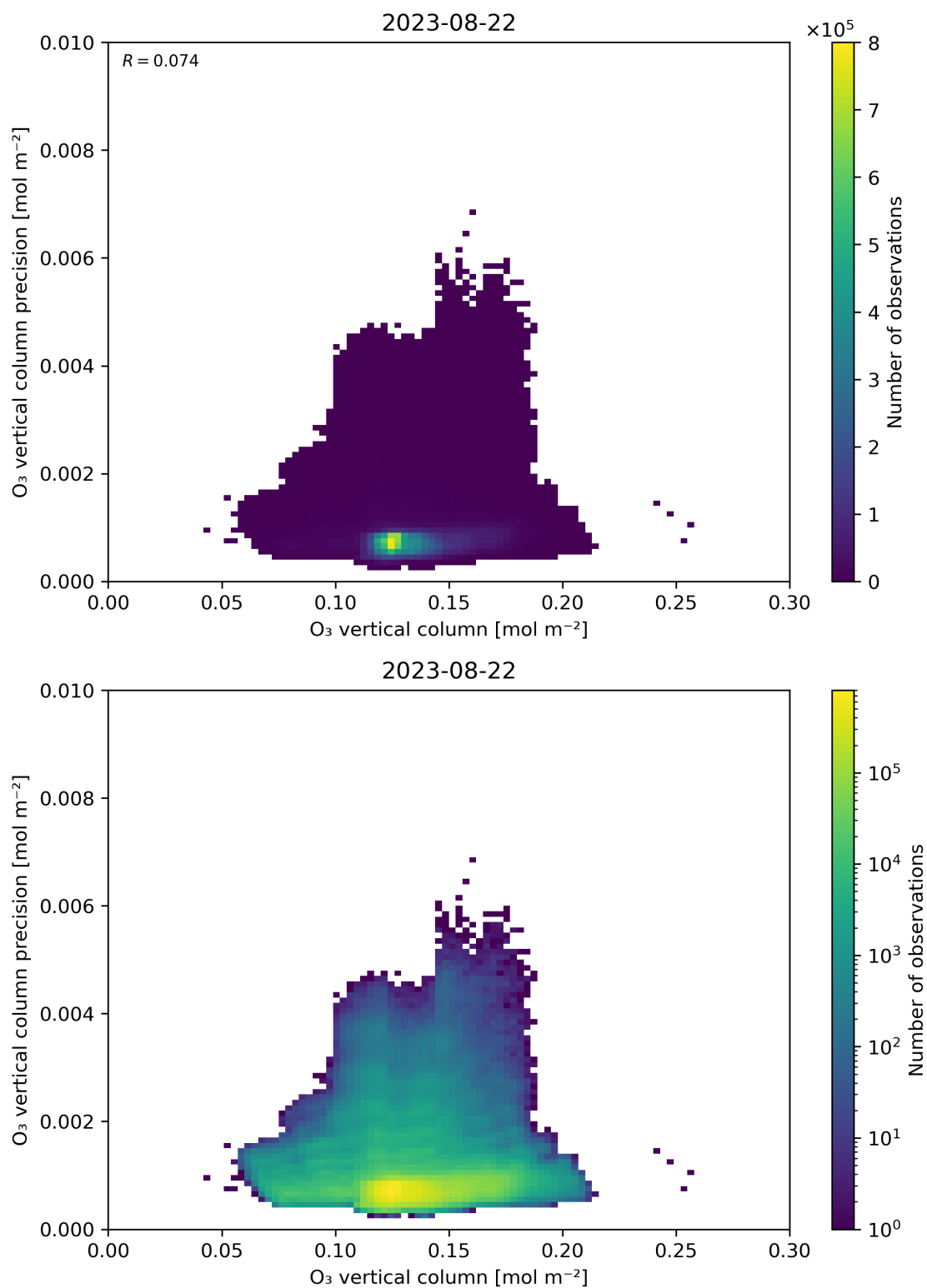
Figure 41: Scatter density plot of “O 3 vertical column” against “O 3 vertical column precision” for 2023-08-21 to 2023-08-23.
