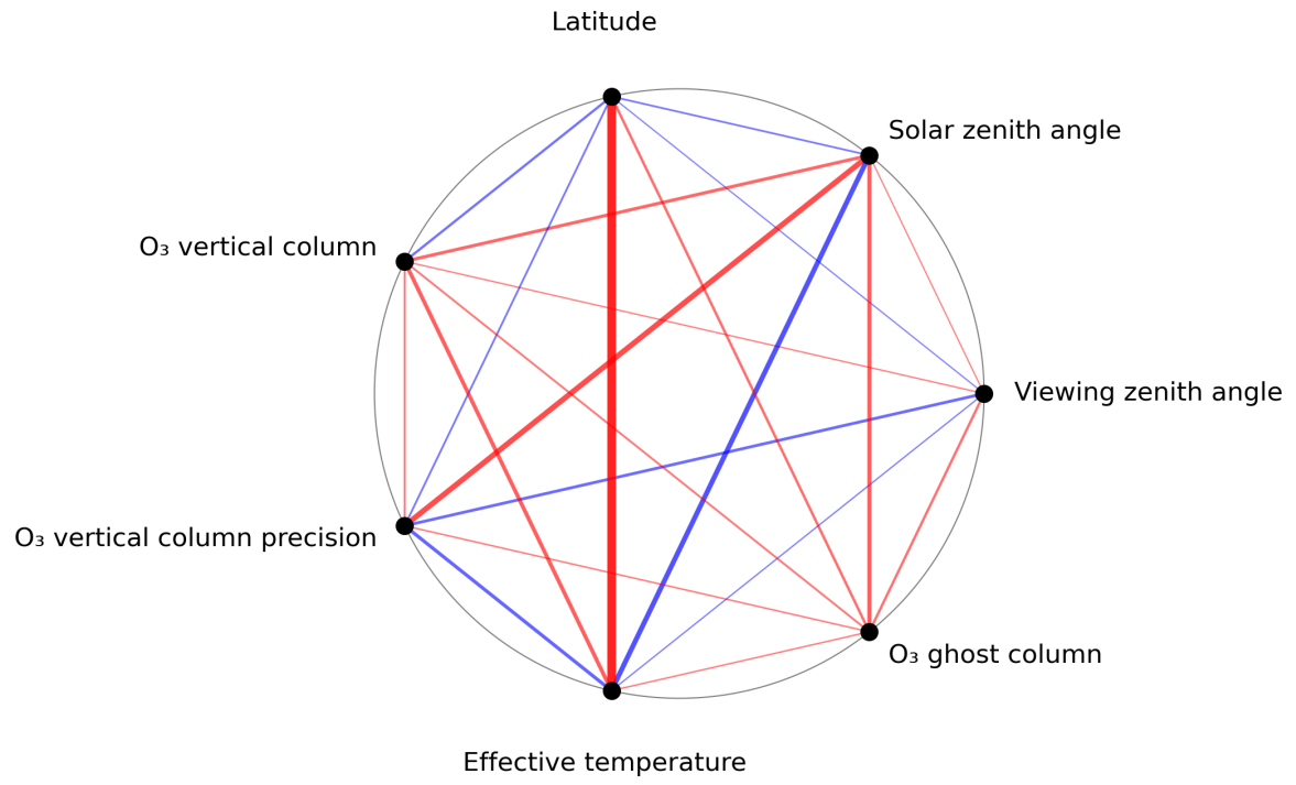
Figure 1: Map of correlation graph for 2023-08-21 to 2023-08-23.
