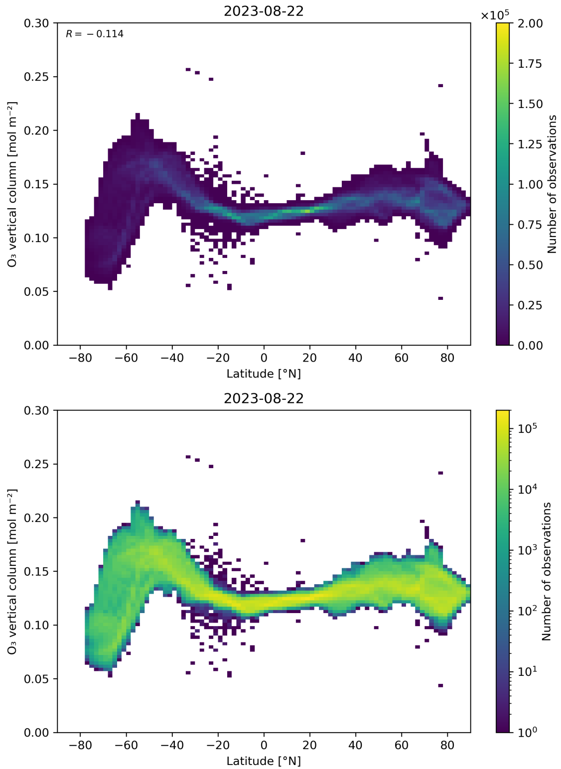
Figure 36: Scatter density plot of “Latitude” against “O 3 vertical column” for 2023-08-21 to 2023-08-23.
