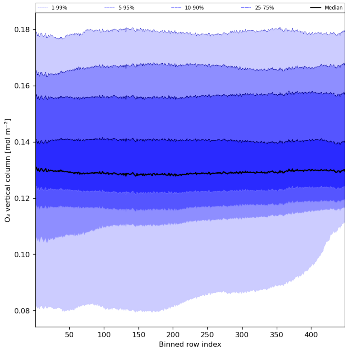
Figure 28: Along track statistics of “O 3 vertical column” for 2023-08-21 to 2023-08-23
