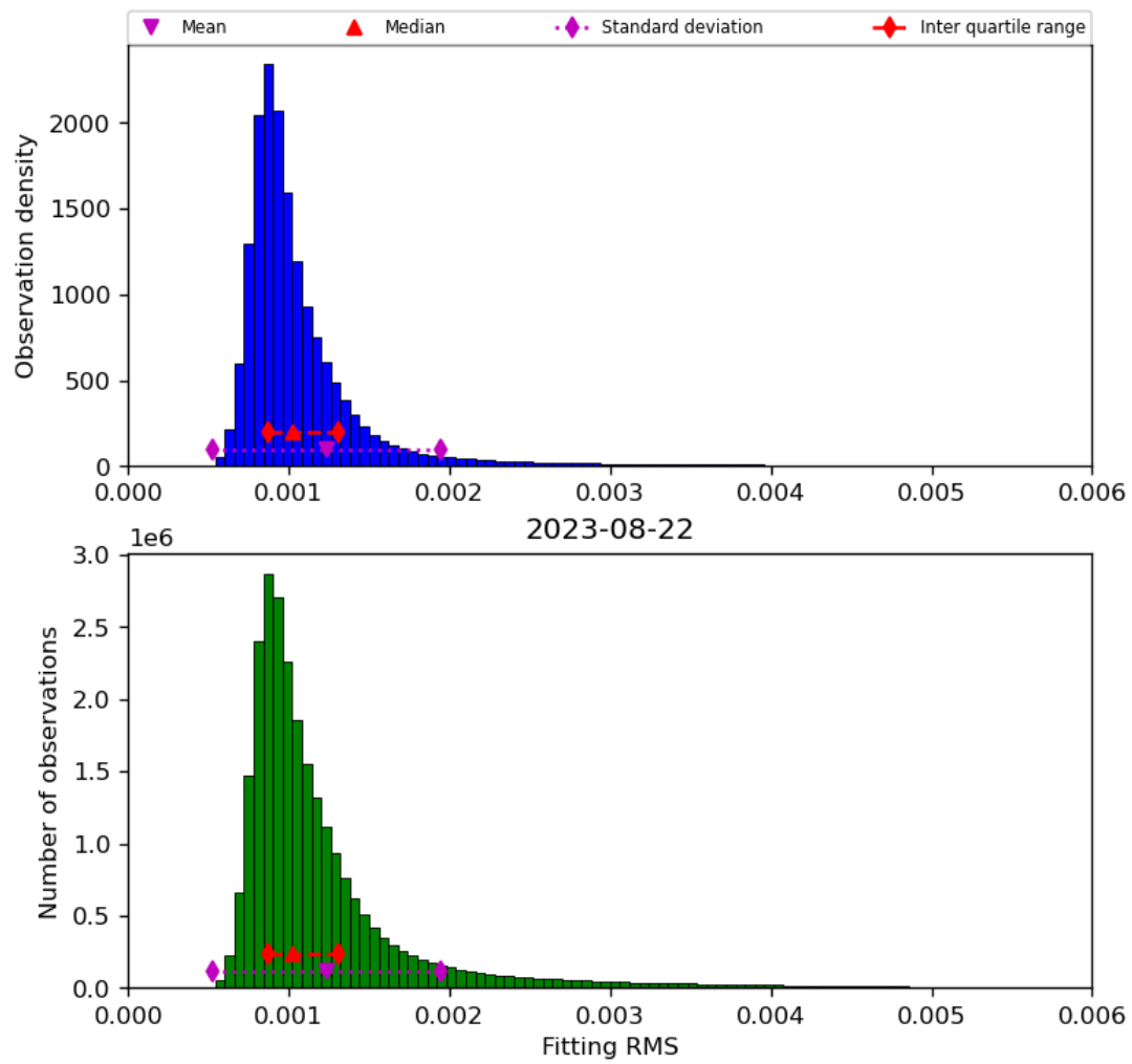
Figure 23: Histogram of “Fitting RMS” for 2023-08-21 to 2023-08-23
