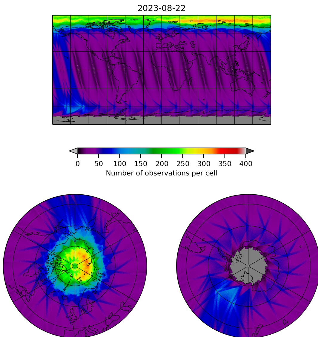
Figure 12: Map of the number of observations for 2023-08-21 to 2023-08-23
