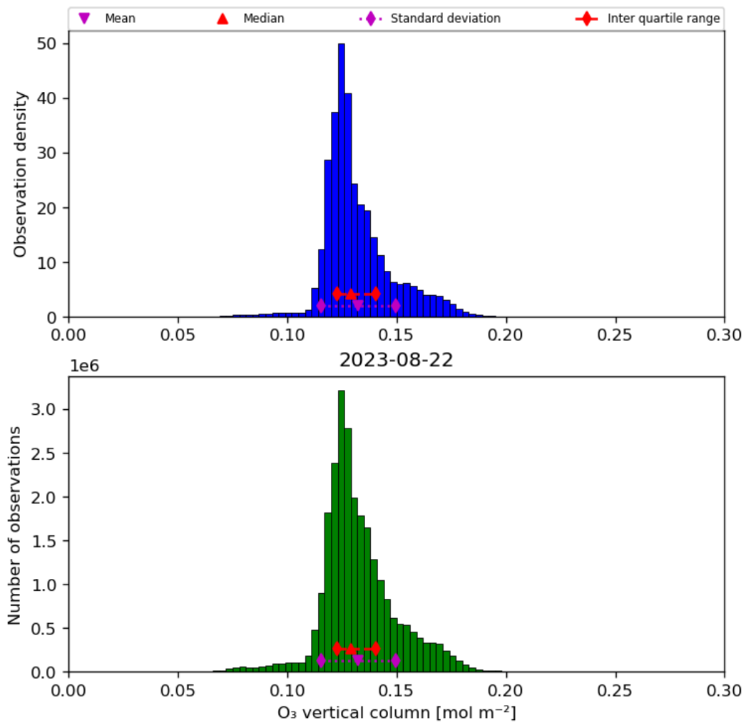
Figure 21: Histogram of “O 3 vertical column” for 2023-08-21 to 2023-08-23
