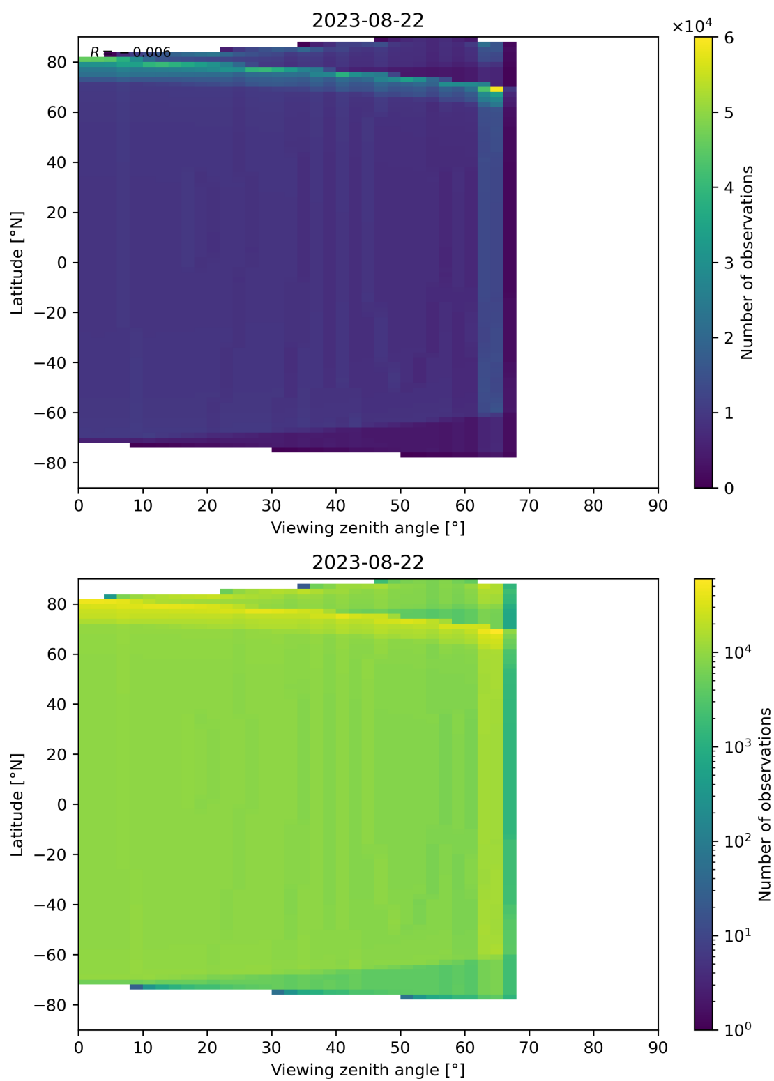
Figure 49: Scatter density plot of “Viewing zenith angle” against “Latitude” for 2023-08-21 to 2023-08-23.
