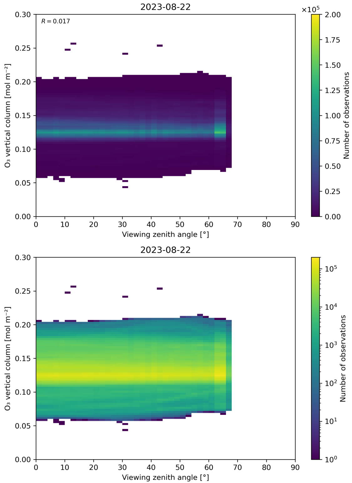
Figure 52: Scatter density plot of “Viewing zenith angle” against “O 3 vertical column” for 2023-08-21 to 2023-08-23.
