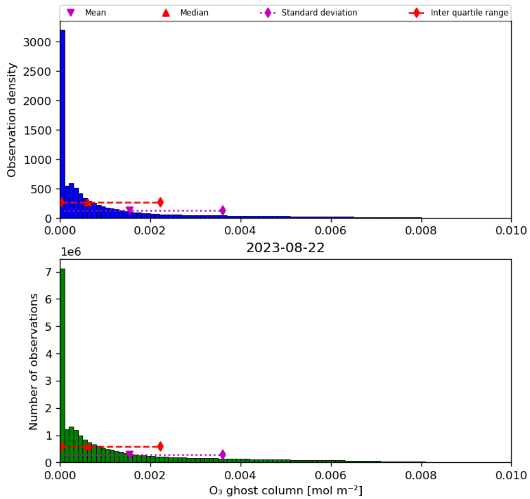
Figure 25: Histogram of “O 3 ghost column” for 2023-08-21 to 2023-08-23
