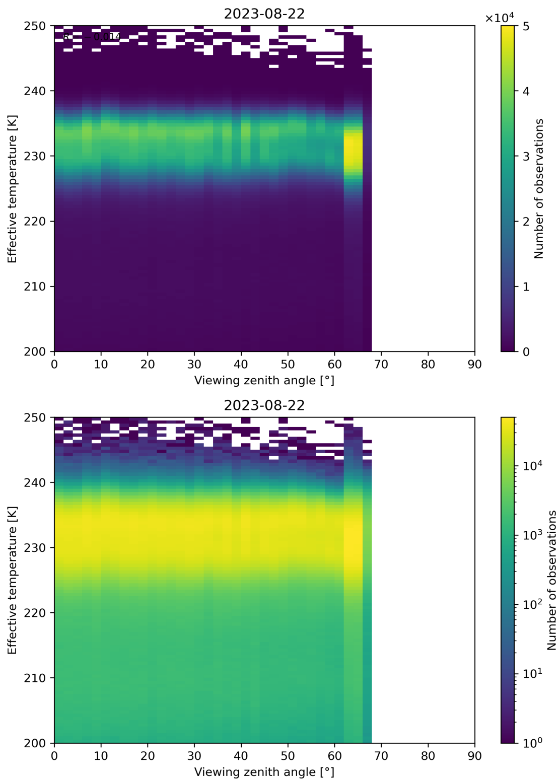
Figure 50: Scatter density plot of “Viewing zenith angle” against “Effective temperature” for 2023-08-21 to 2023-08-23.
