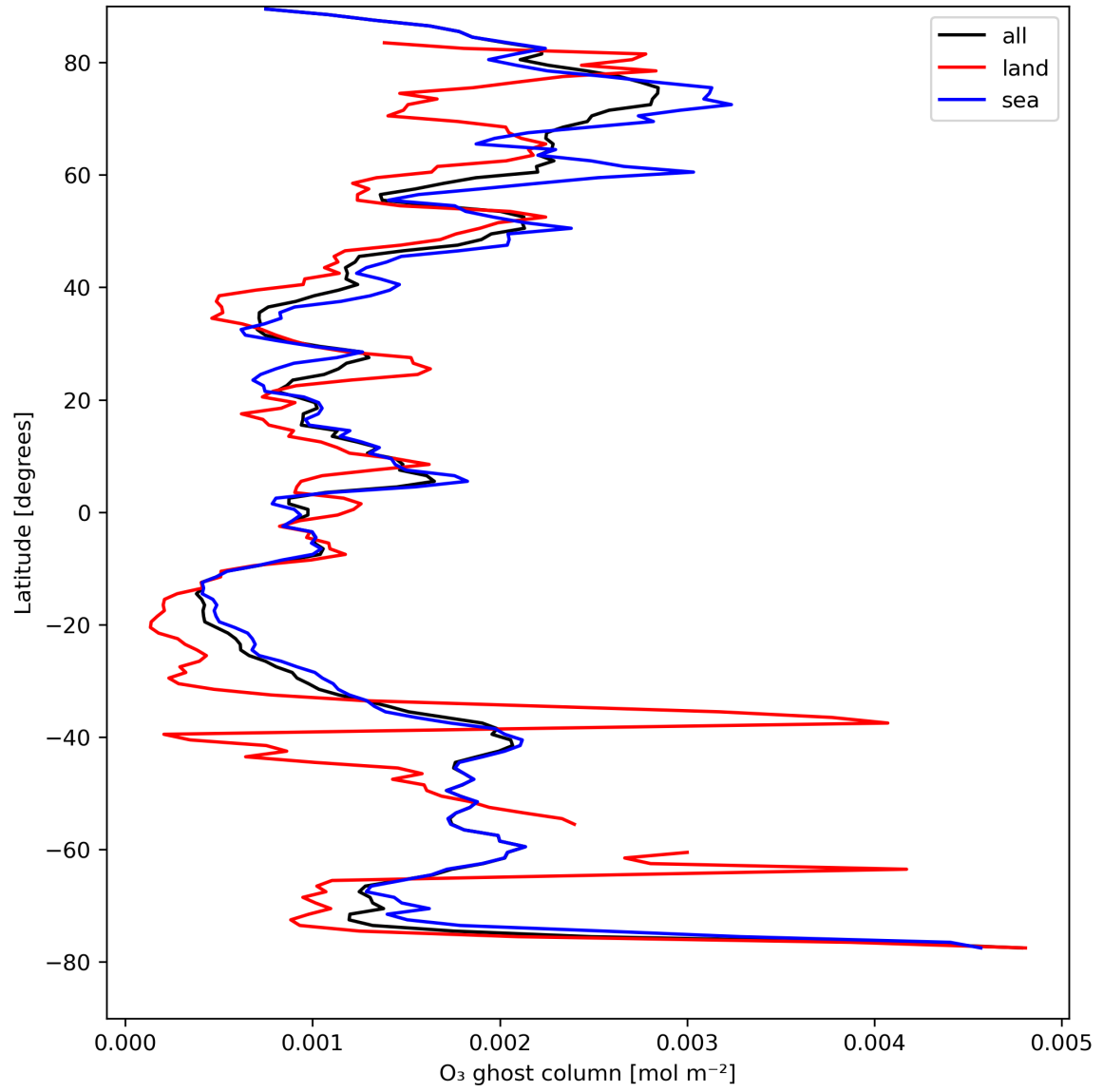
Figure 18: Zonal average of "O 3 ghost column" for 2023-08-21 to 2023-08-23.
