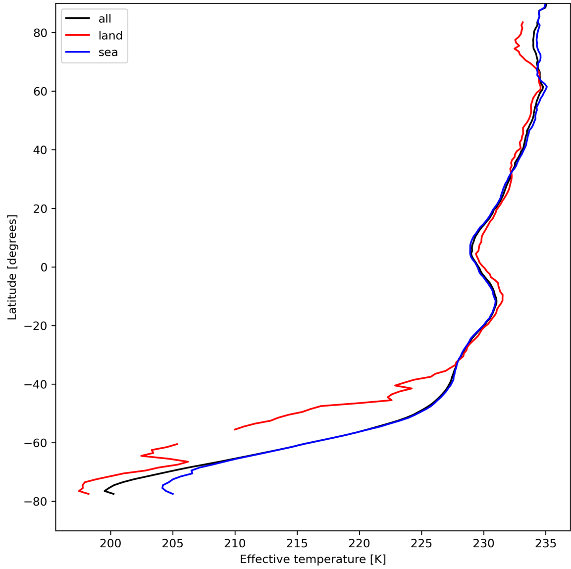
Figure 17: Zonal average of "Effective temperature" for 2023-08-21 to 2023-08-23.
