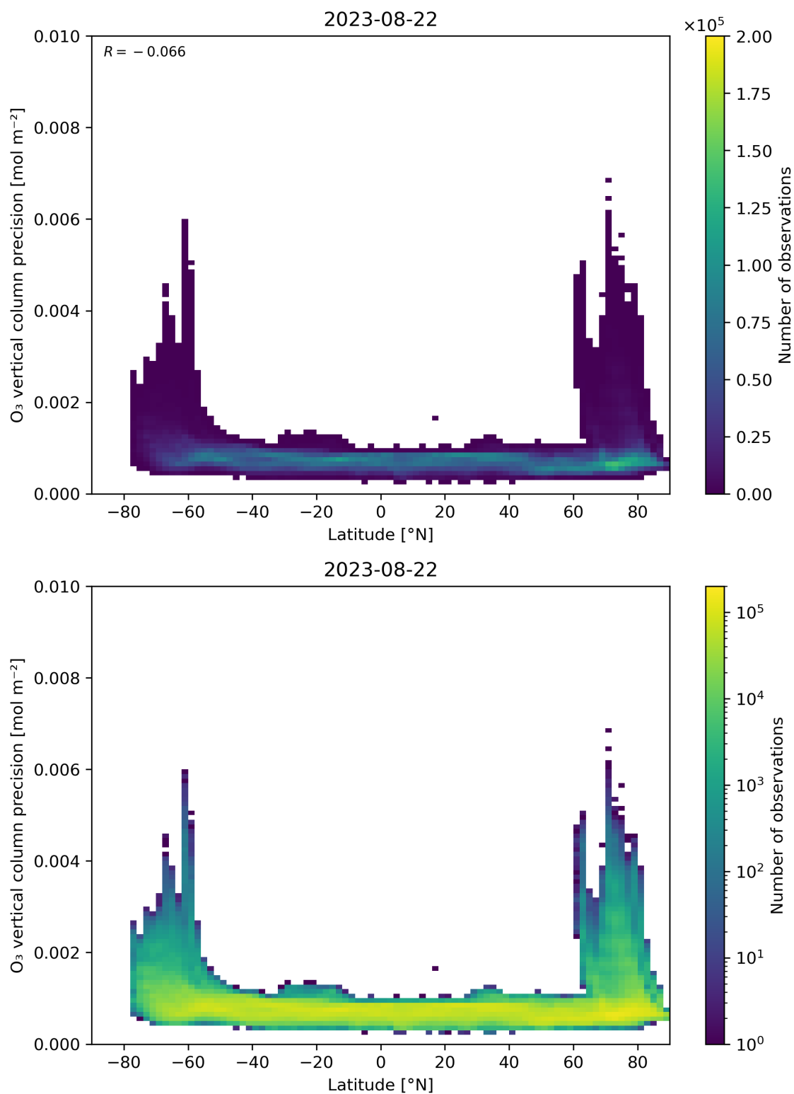
Figure 37: Scatter density plot of “Latitude” against “O 3 vertical column precision” for 2023-08-21 to 2023-08-23.
