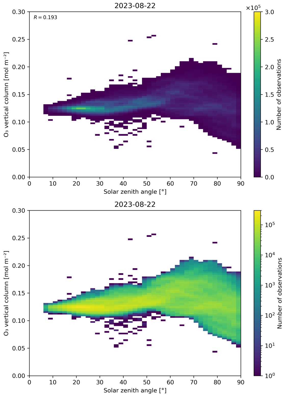
Figure 47: Scatter density plot of “Solar zenith angle” against “O 3 vertical column” for 2023-08-21 to 2023-08-23.
