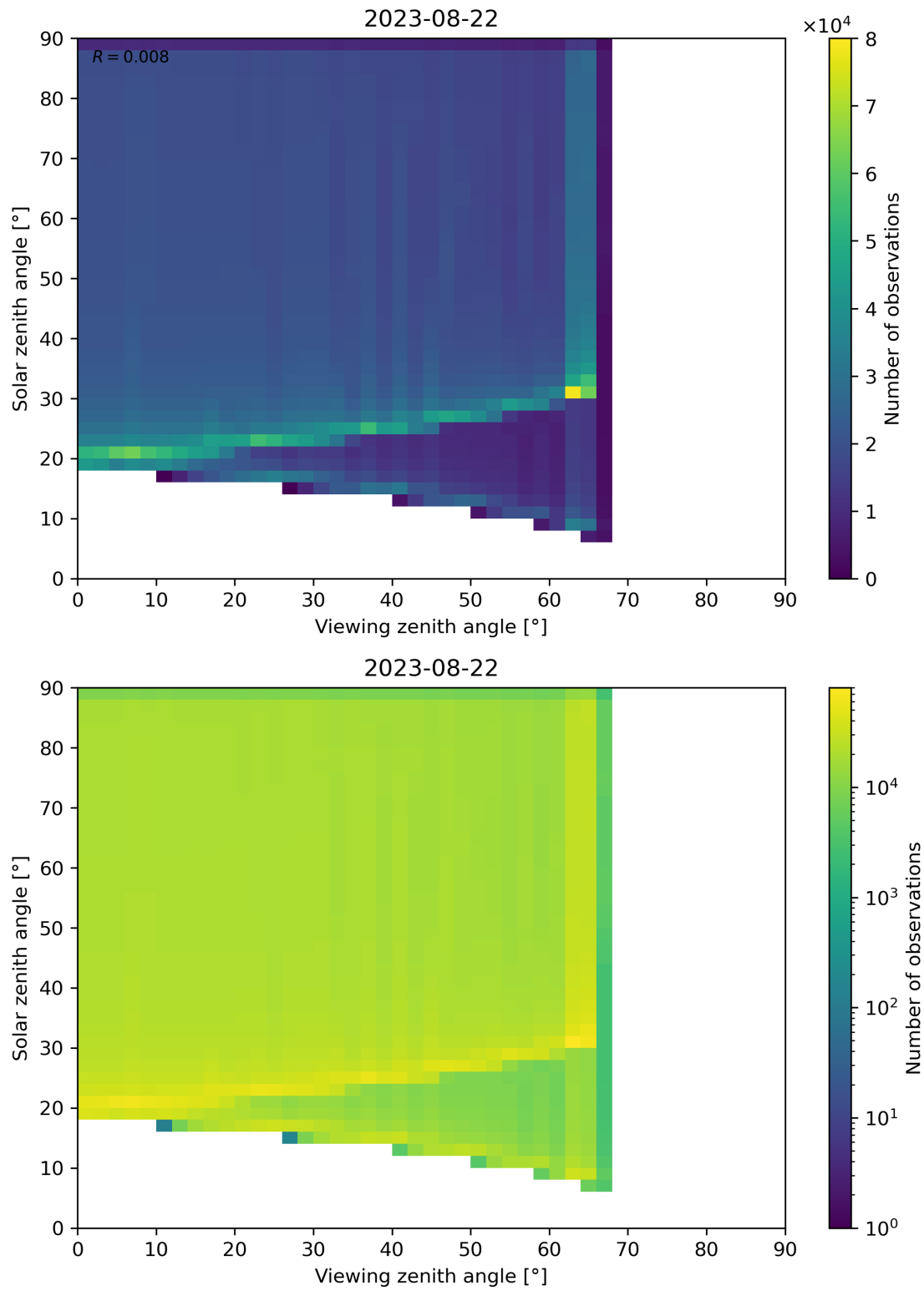
Figure 54: Scatter density plot of “Viewing zenith angle” against “Solar zenith angle” for 2023-08-21 to 2023-08-23.
