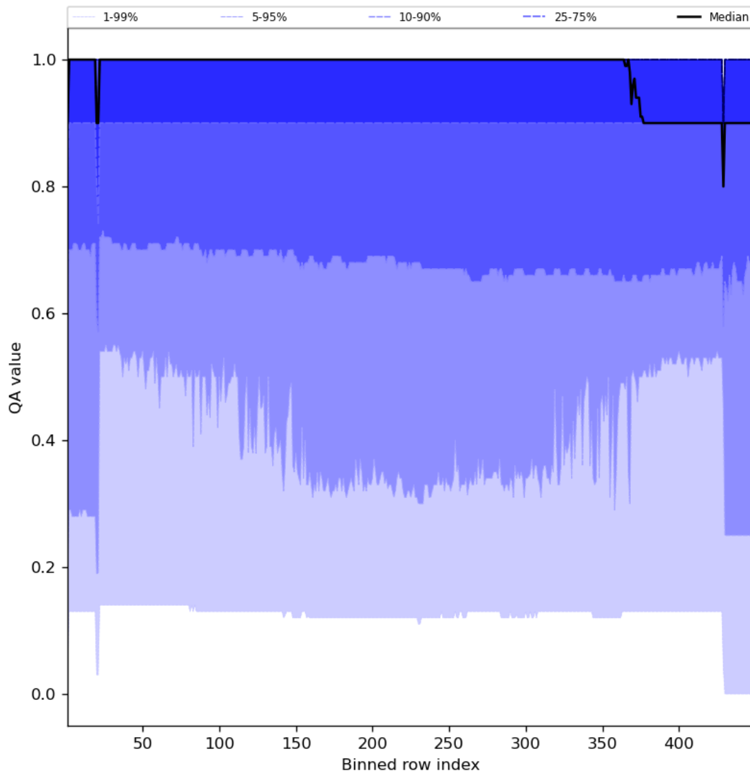
Figure 27: Along track statistics of “QA value” for 2023-08-21 to 2023-08-23
