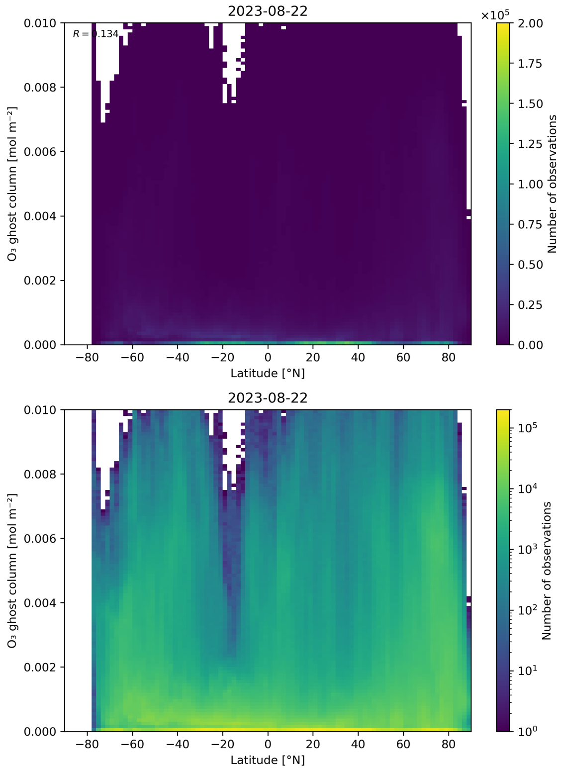
Figure 35: Scatter density plot of “Latitude” against “O 3 ghost column” for 2023-08-21 to 2023-08-23.
