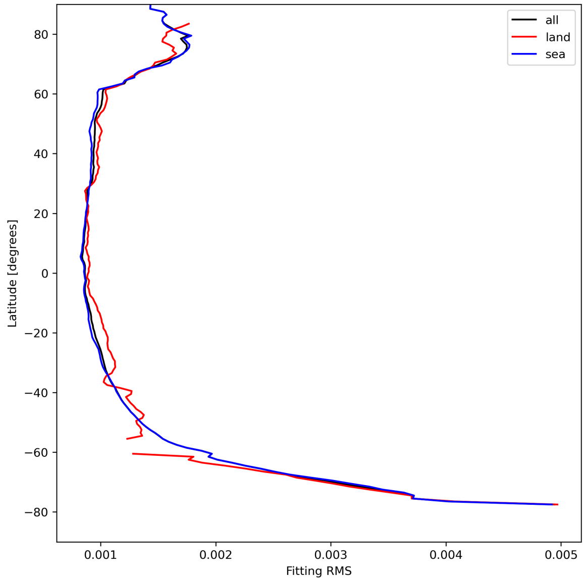
Figure 16: Zonal average of “Fitting RMS” for 2023-08-21 to 2023-08-23.
