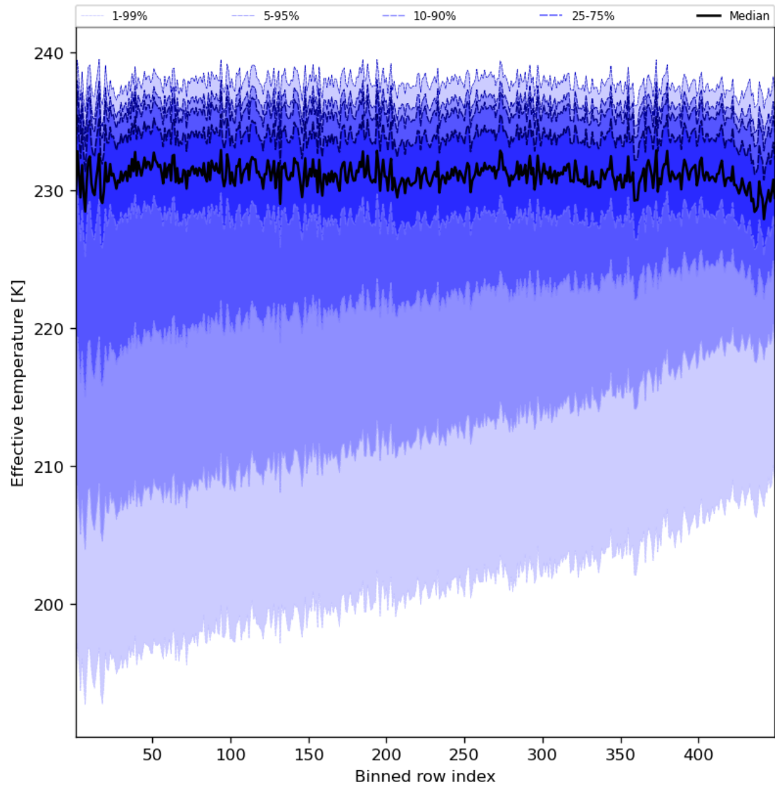
Figure 31: Along track statistics of “Effective temperature” for 2023-08-21 to 2023-08-23
