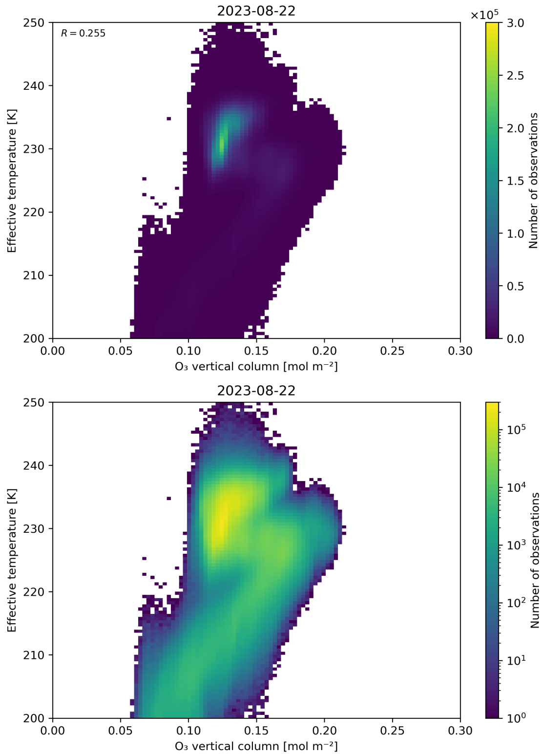
Figure 39: Scatter density plot of “O 3 vertical column” against “Effective temperature” for 2023-08-21 to 2023-08-23.
