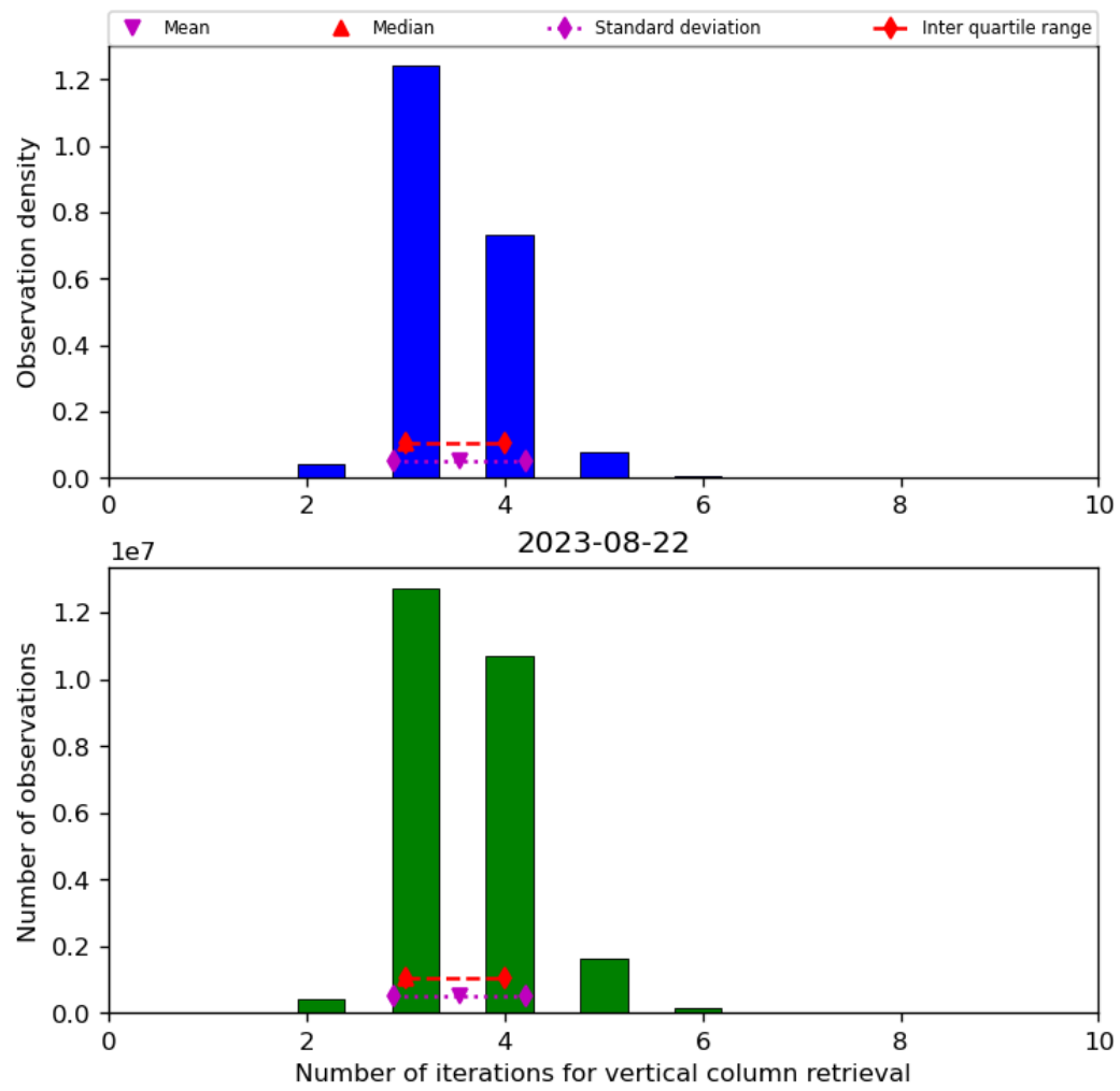
Figure 26: Histogram of “Number of iterations for vertical column retrieval” for 2023-08-21 to 2023-08-23
