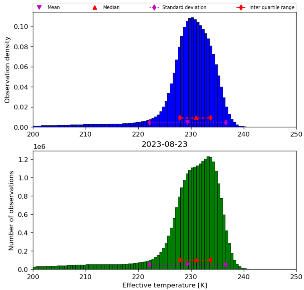
Figure 24: Histogram of “Effective temperature” for 2023-08-22 to 2023-08-24
