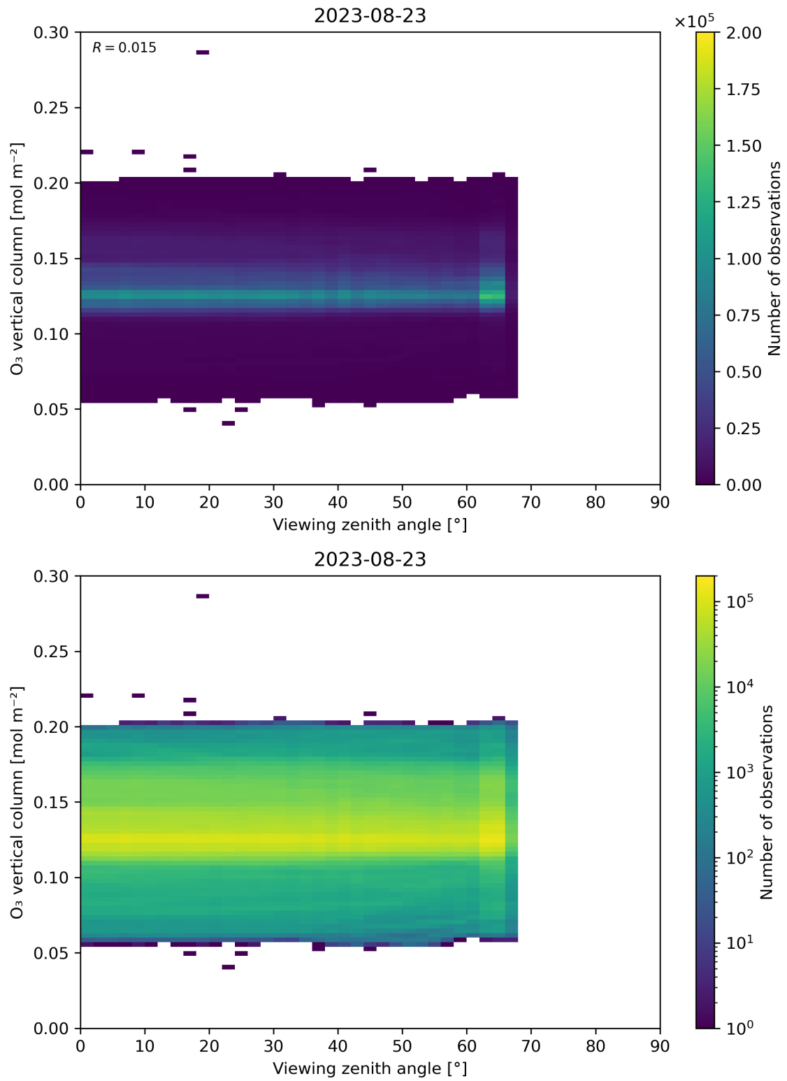
Figure 52: Scatter density plot of “Viewing zenith angle” against “O 3 vertical column” for 2023-08-22 to 2023-08-24.
