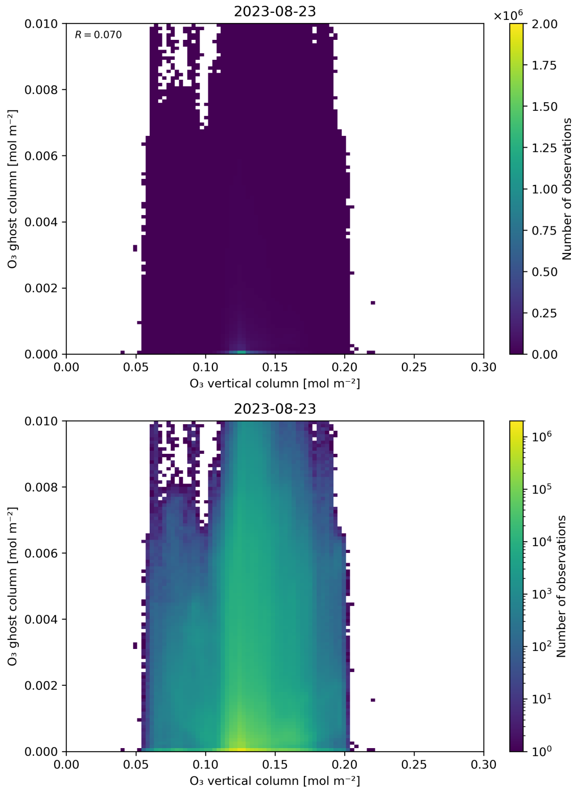
Figure 40: Scatter density plot of “O 3 vertical column” against “O 3 ghost column” for 2023-08-22 to 2023-08-24.
