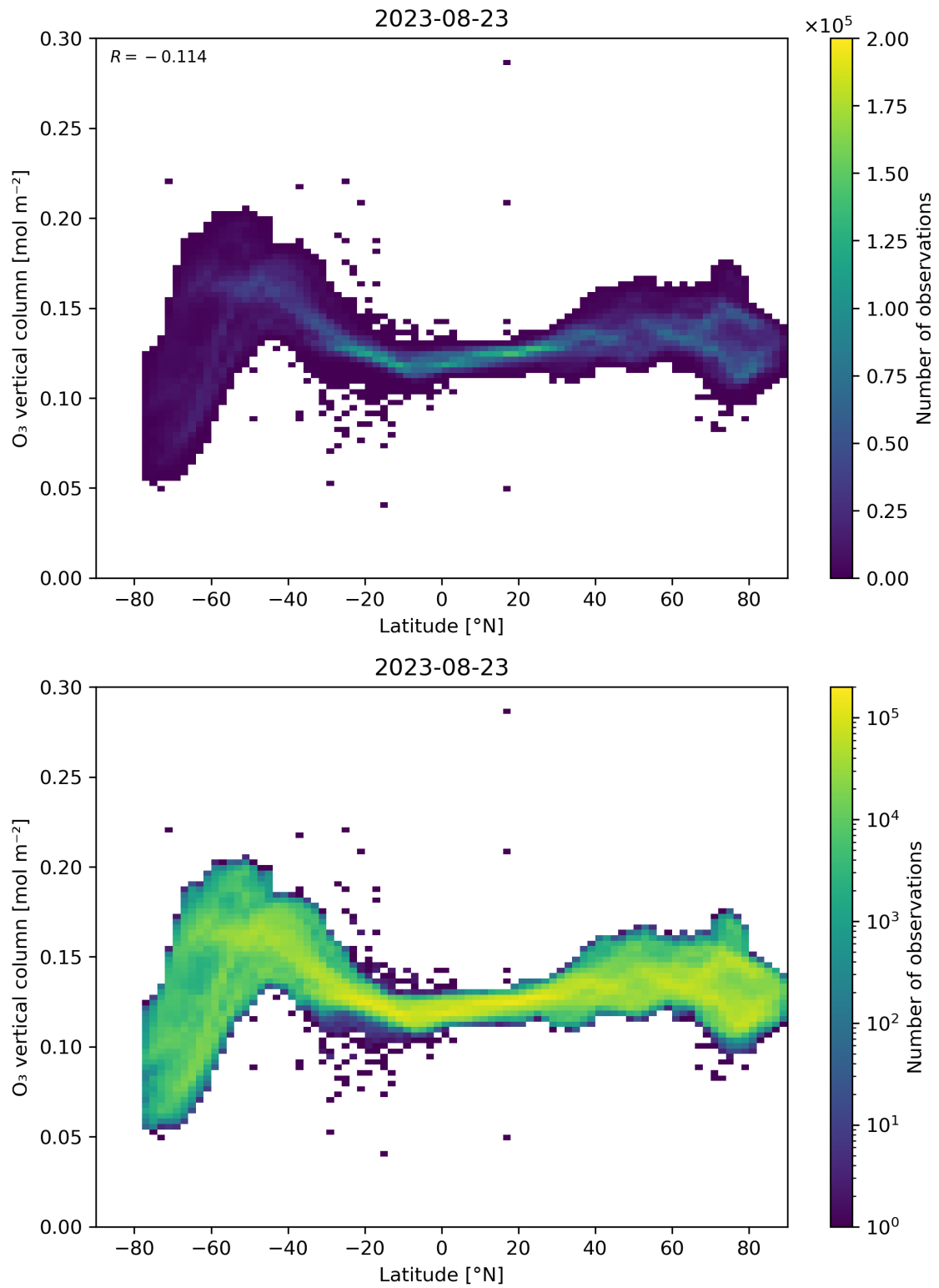
Figure 36: Scatter density plot of “Latitude” against “O 3 vertical column” for 2023-08-22 to 2023-08-24.
