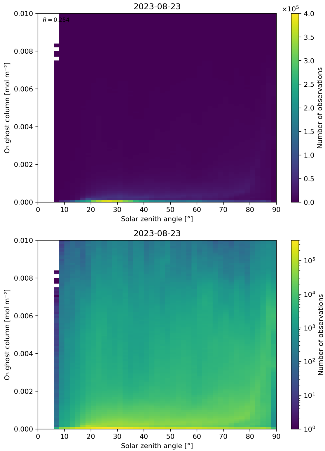
Figure 46: Scatter density plot of “Solar zenith angle” against “O 3 ghost column” for 2023-08-22 to 2023-08-24.
