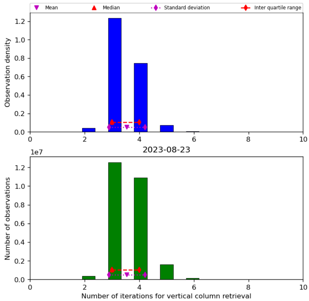
Figure 26: Histogram of “Number of iterations for vertical column retrieval” for 2023-08-22 to 2023-08-24
