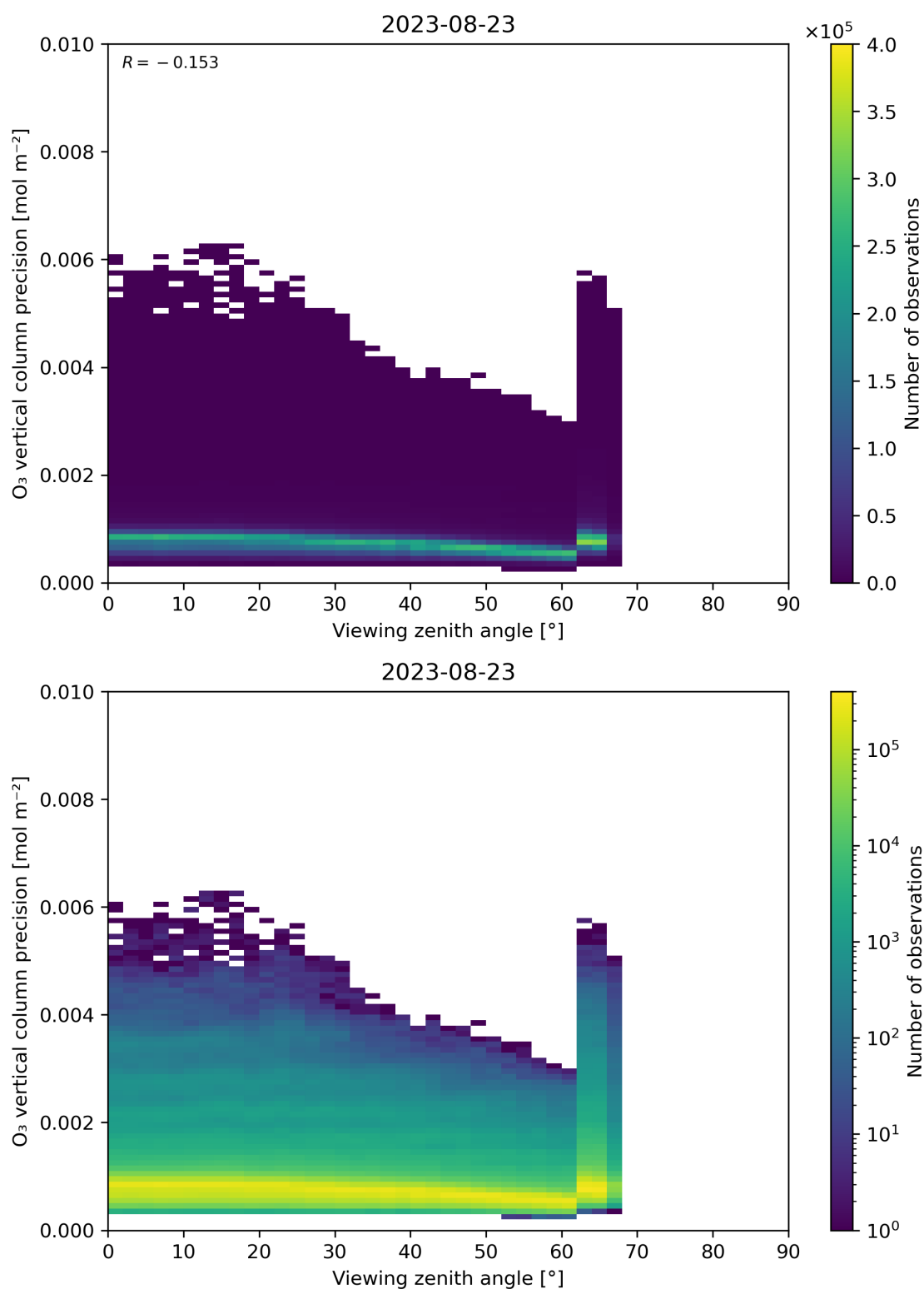
Figure 53: Scatter density plot of “Viewing zenith angle” against “O 3 vertical column precision” for 2023-08-22 to 2023-08-24.
