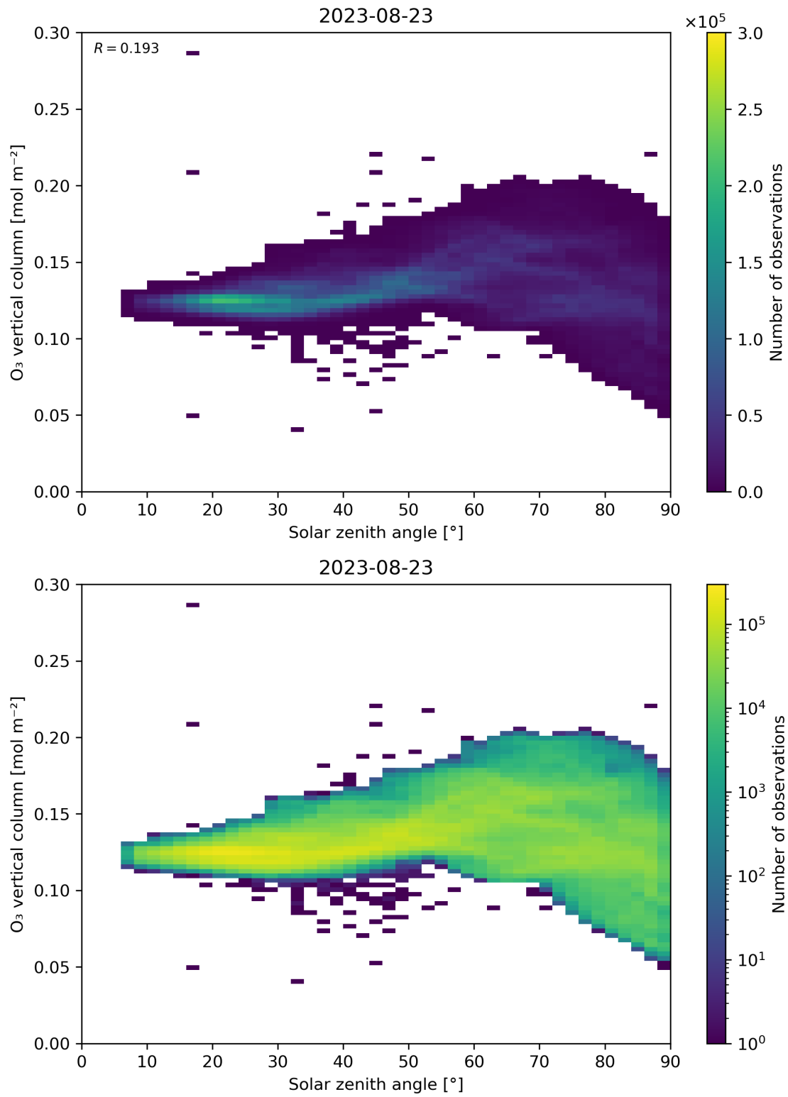
Figure 47: Scatter density plot of “Solar zenith angle” against “O 3 vertical column” for 2023-08-22 to 2023-08-24.
