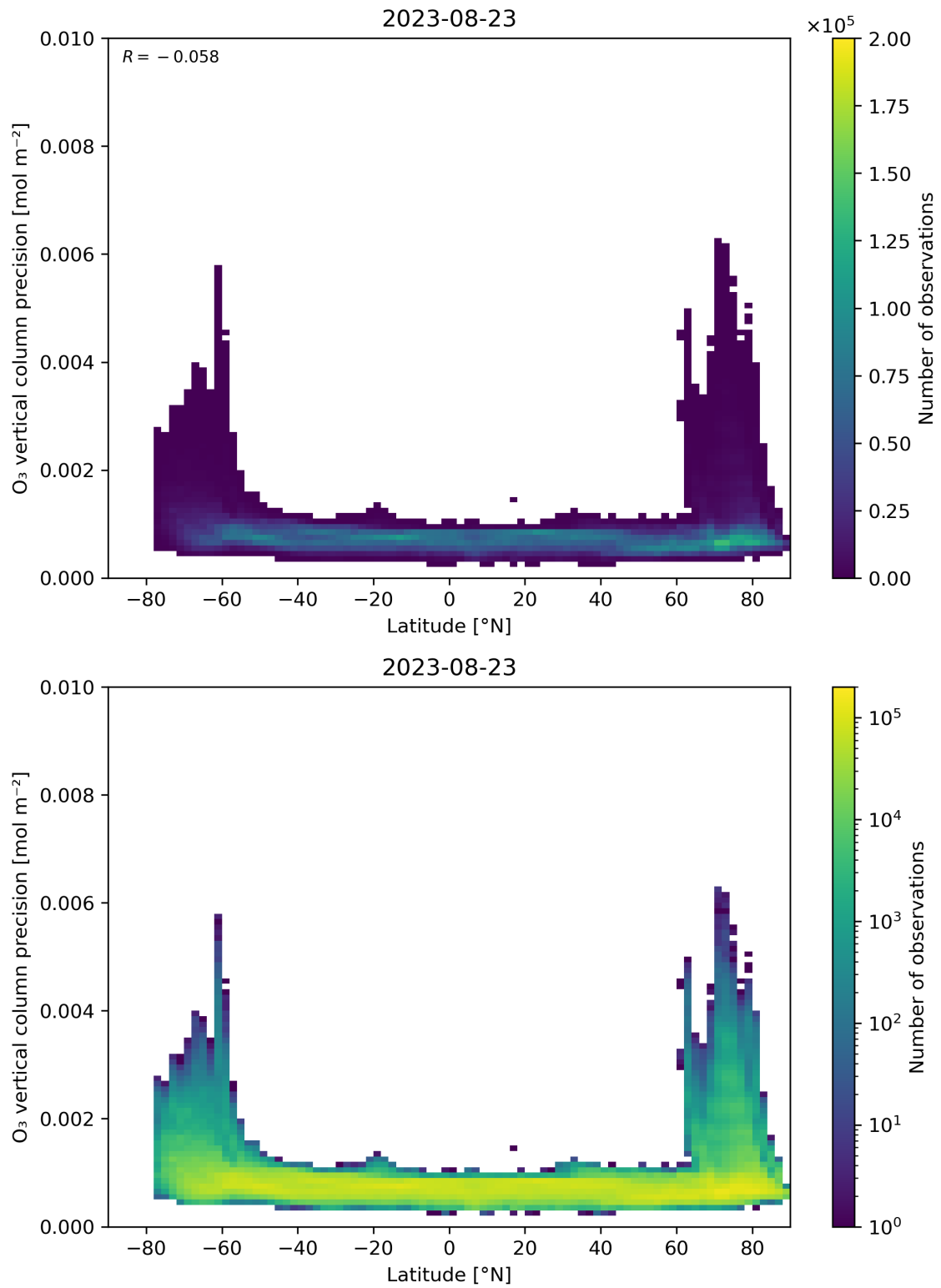
Figure 37: Scatter density plot of “Latitude” against “O 3 vertical column precision” for 2023-08-22 to 2023-08-24.
