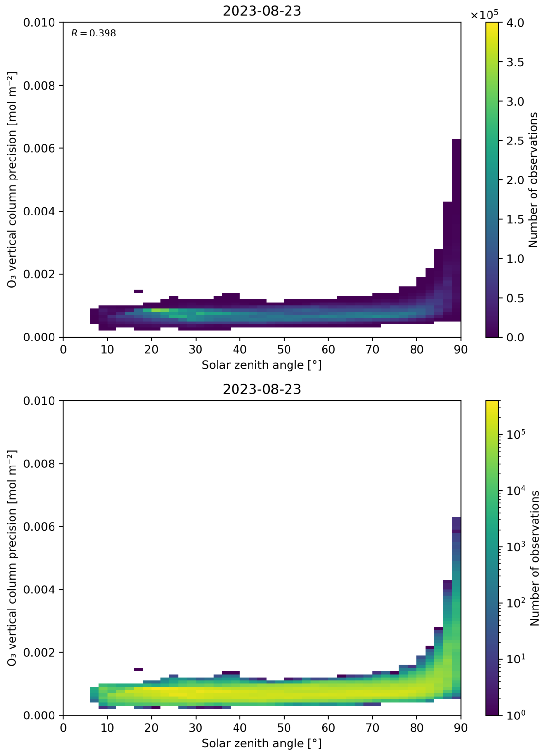
Figure 48: Scatter density plot of “Solar zenith angle” against “O 3 vertical column precision” for 2023-08-22 to 2023-08-24.
