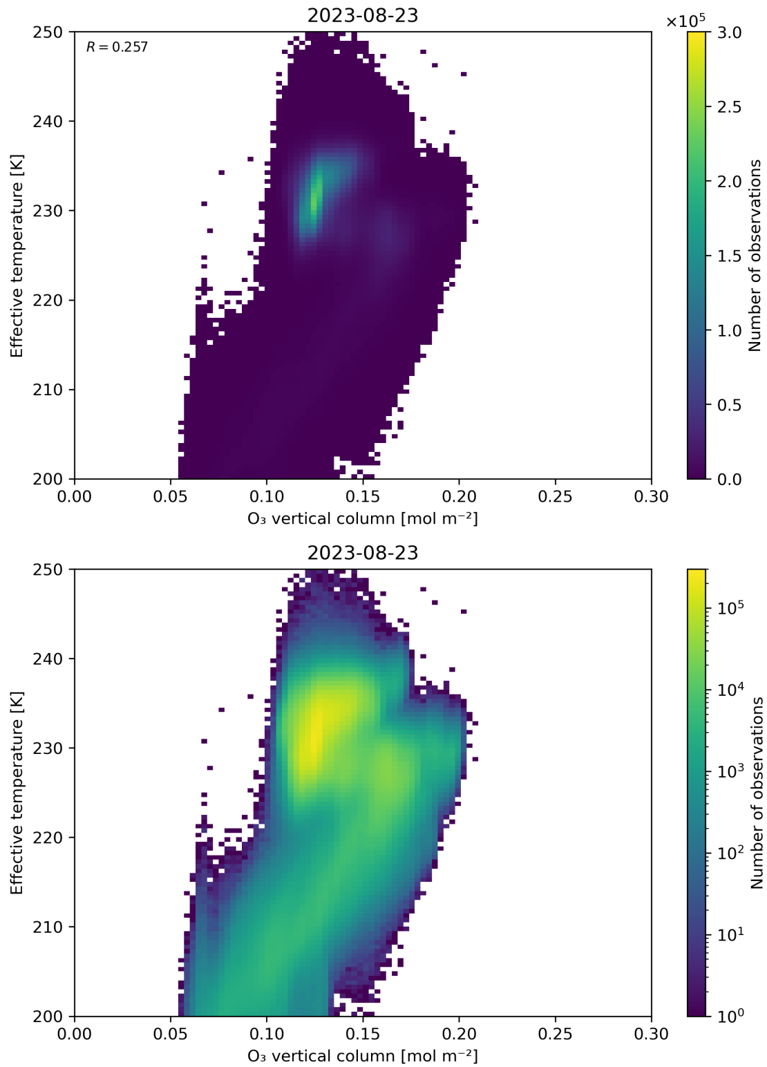
Figure 39: Scatter density plot of “O 3 vertical column” against “Effective temperature” for 2023-08-22 to 2023-08-24.
