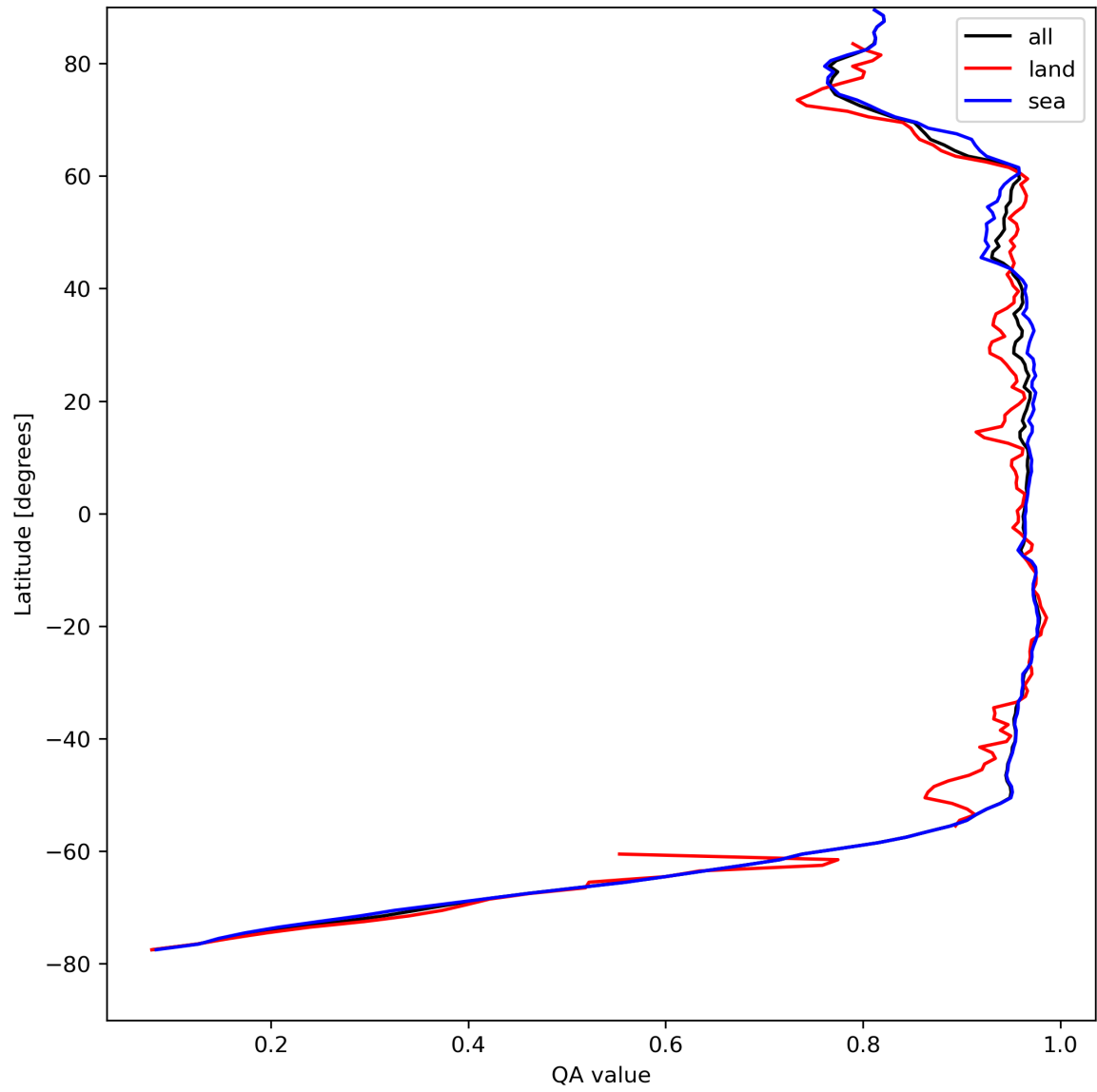
Figure 13: Zonal average of “QA value” for 2023-08-22 to 2023-08-24.
