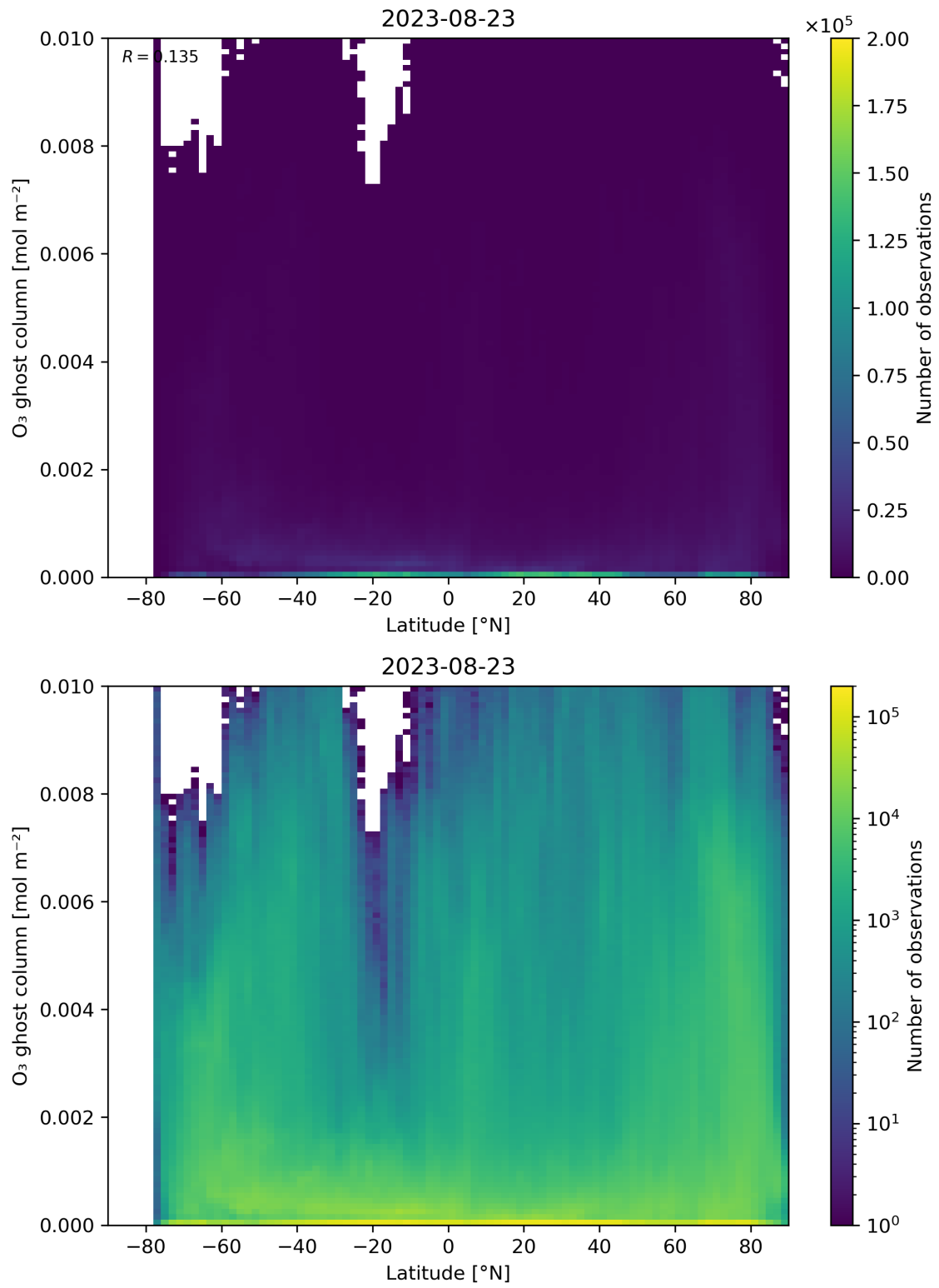
Figure 35: Scatter density plot of “Latitude” against “O 3 ghost column” for 2023-08-22 to 2023-08-24.
