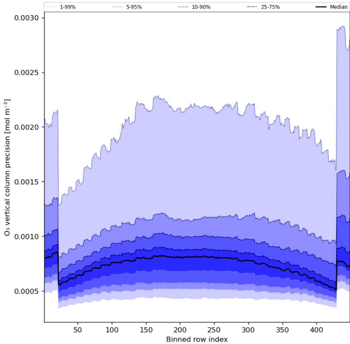
Figure 29: Along track statistics of “O 3 vertical column precision” for 2023-08-22 to 2023-08-24
