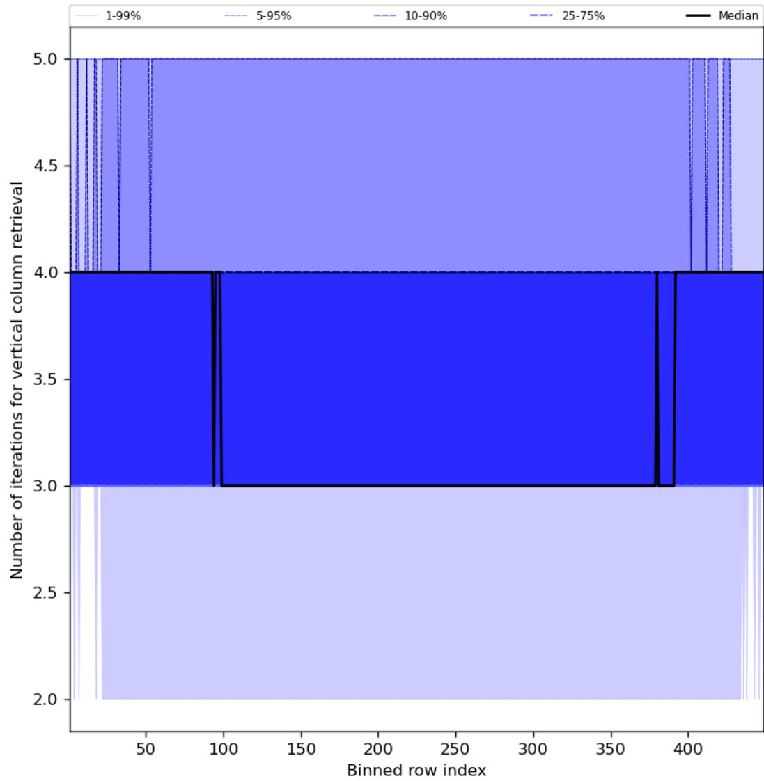
Figure 33: Along track statistics of “Number of iterations for vertical column retrieval” for 2023-08-22 to 2023-08-24
