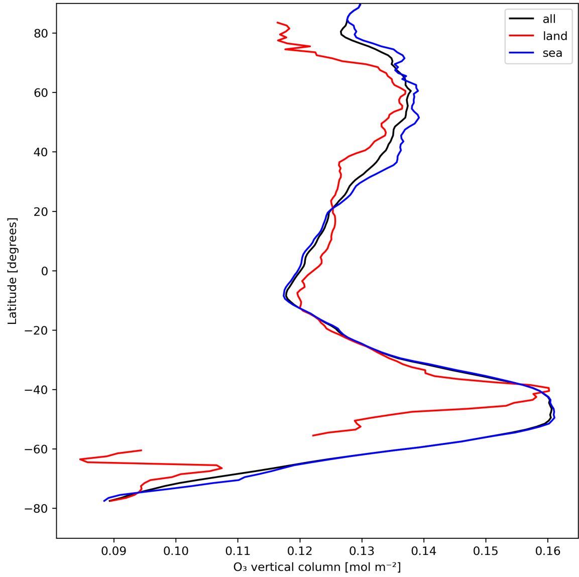
Figure 14: Zonal average of “O 3 vertical column” for 2023-08-22 to 2023-08-24.
