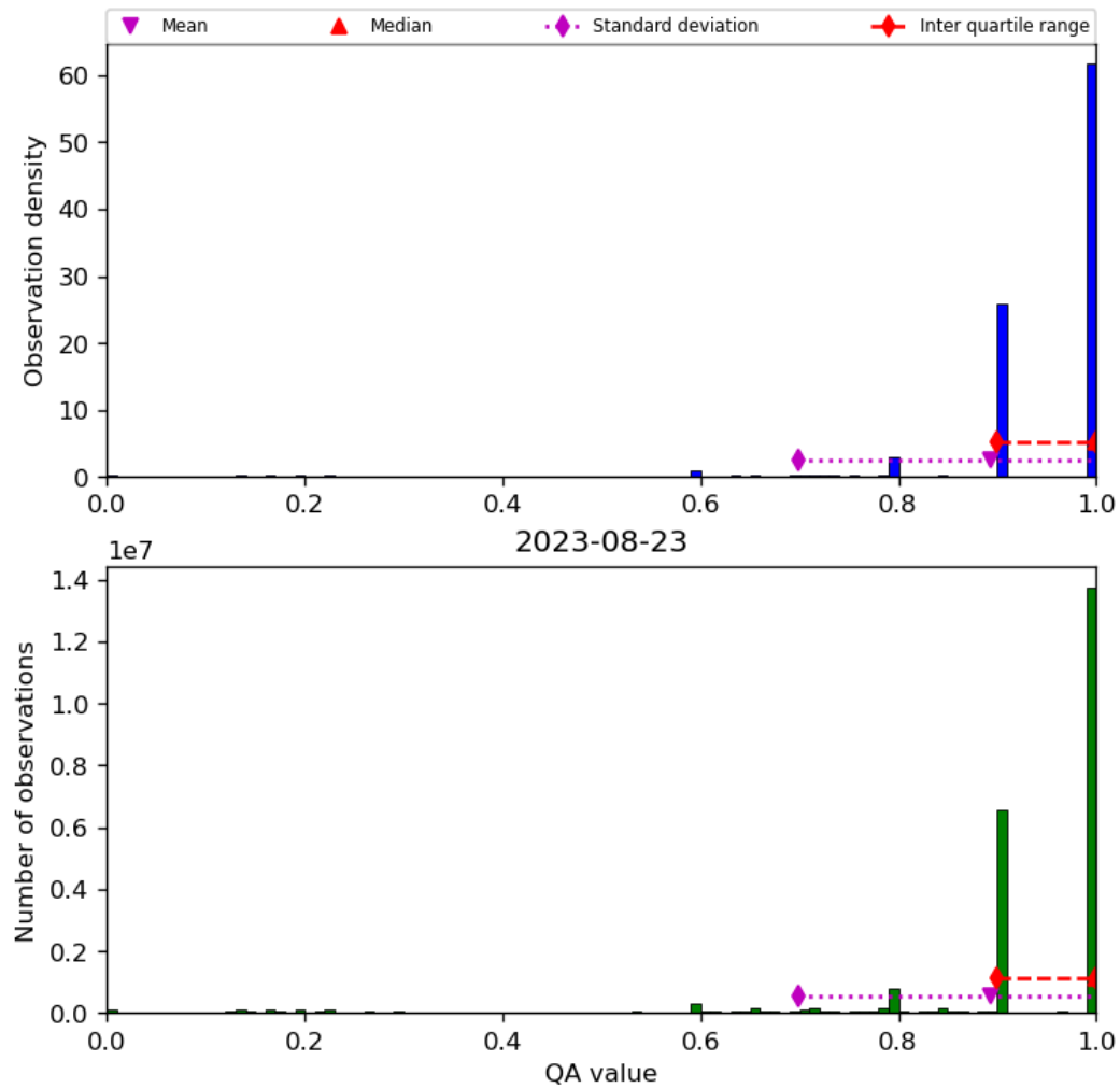
Figure 20: Histogram of “QA value” for 2023-08-22 to 2023-08-24
