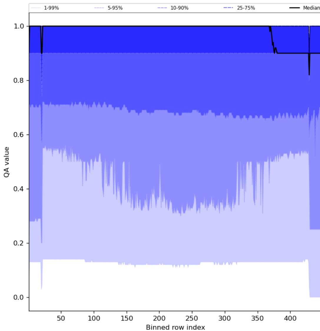
Figure 27: Along track statistics of “QA value” for 2023-08-22 to 2023-08-24
