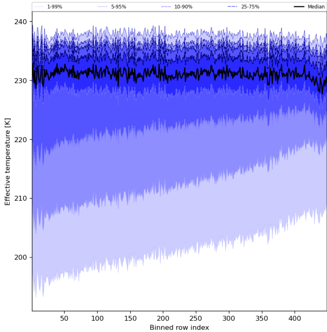
Figure 31: Along track statistics of “Effective temperature” for 2023-08-22 to 2023-08-24
