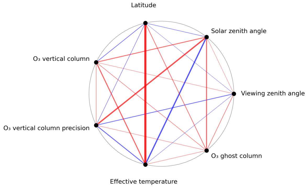
Figure 1: Map of correlation graph for 2023-08-22 to 2023-08-24.
