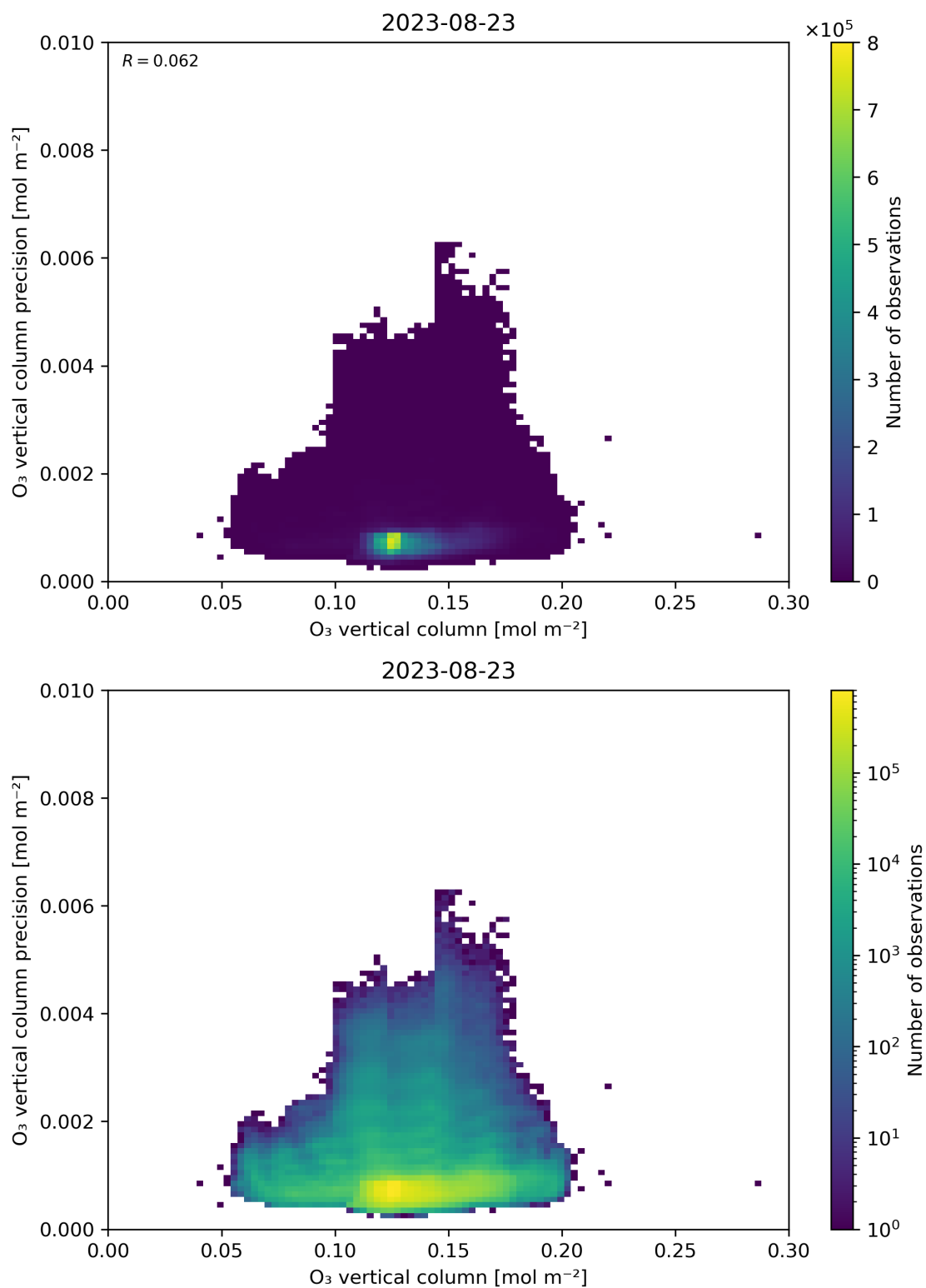
Figure 41: Scatter density plot of “O 3 vertical column” against “O 3 vertical column precision” for 2023-08-22 to 2023-08-24.
