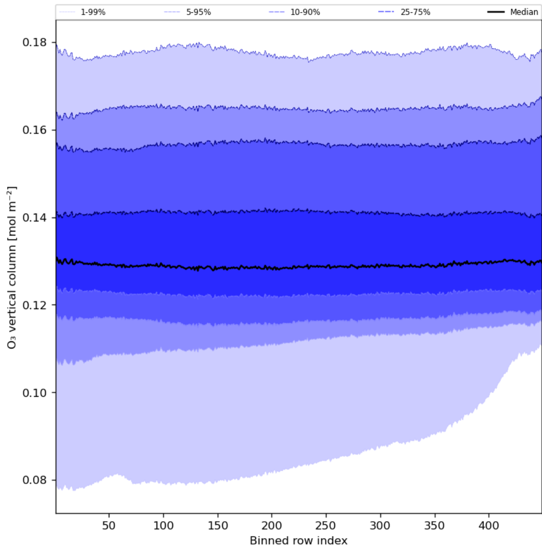
Figure 28: Along track statistics of “O 3 vertical column” for 2023-08-22 to 2023-08-24
