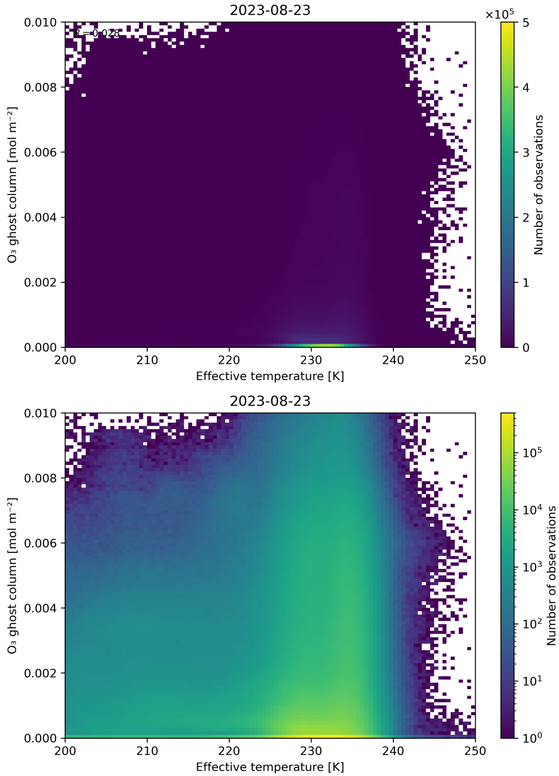
Figure 38: Scatter density plot of “Effective temperature” against “O 3 ghost column” for 2023-08-22 to 2023-08-24.
