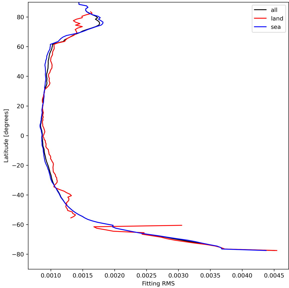
Figure 16: Zonal average of “Fitting RMS” for 2023-08-22 to 2023-08-24.
