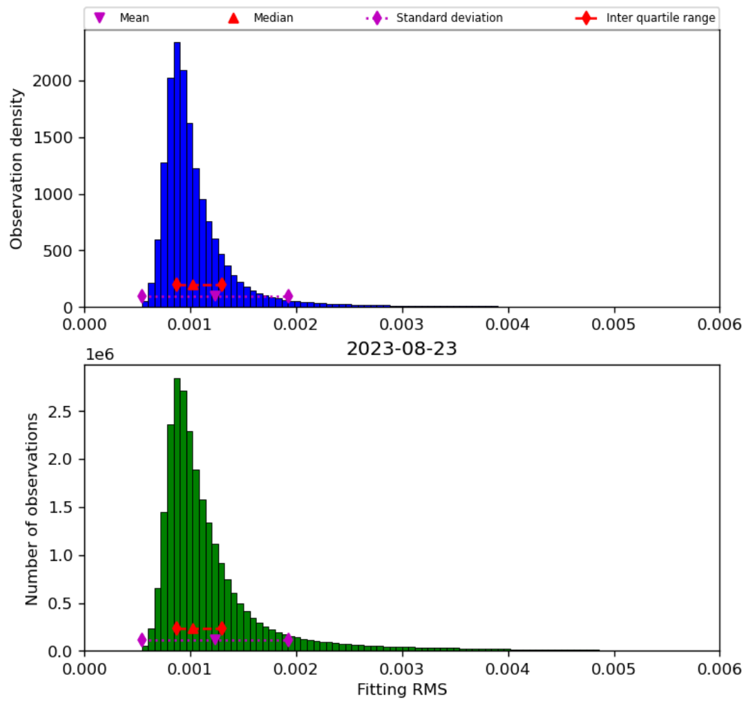
Figure 23: Histogram of “Fitting RMS” for 2023-08-22 to 2023-08-24
