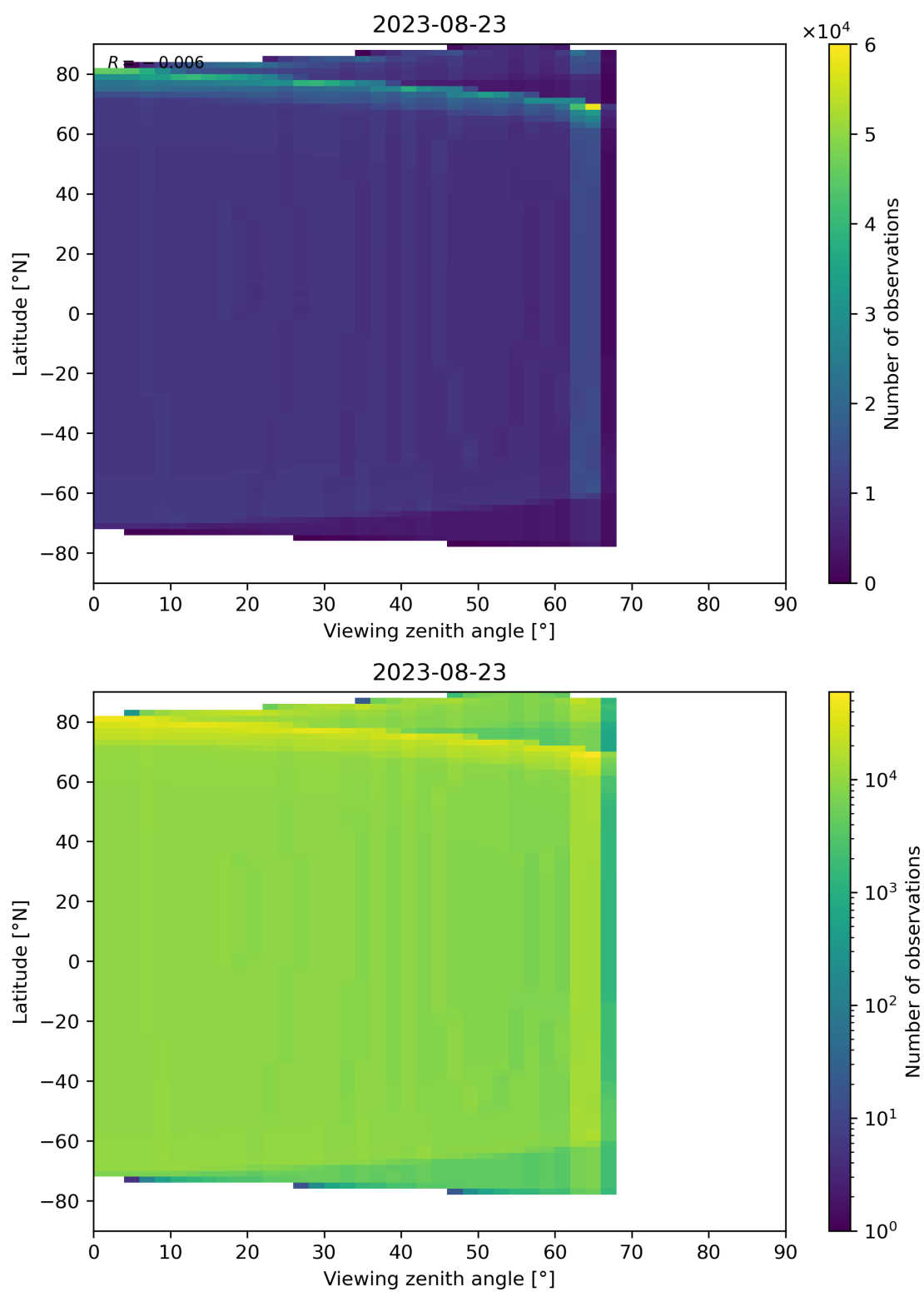
Figure 49: Scatter density plot of “Viewing zenith angle” against “Latitude” for 2023-08-22 to 2023-08-24.
