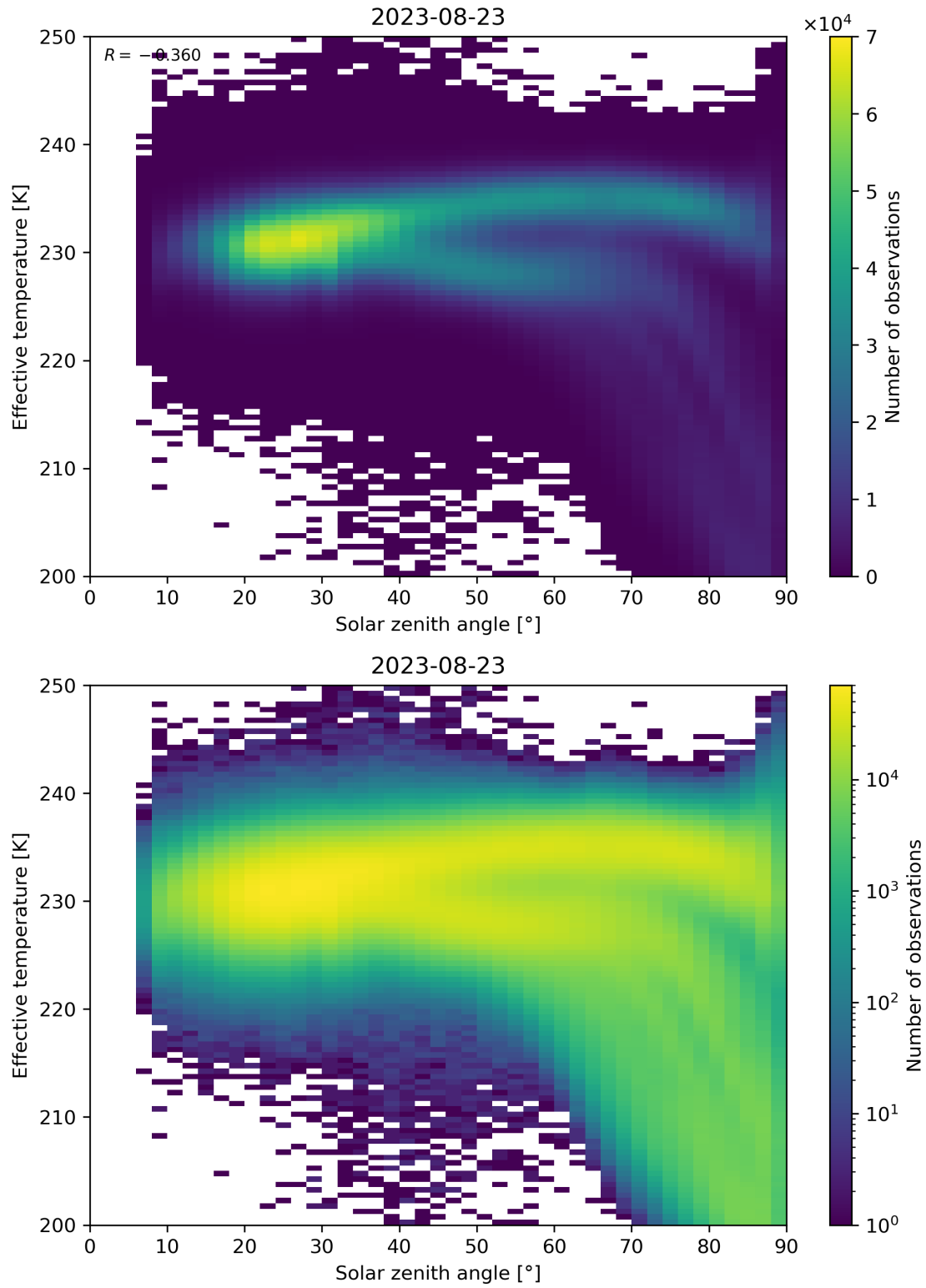
Figure 45: Scatter density plot of “Solar zenith angle” against “Effective temperature” for 2023-08-22 to 2023-08-24.
