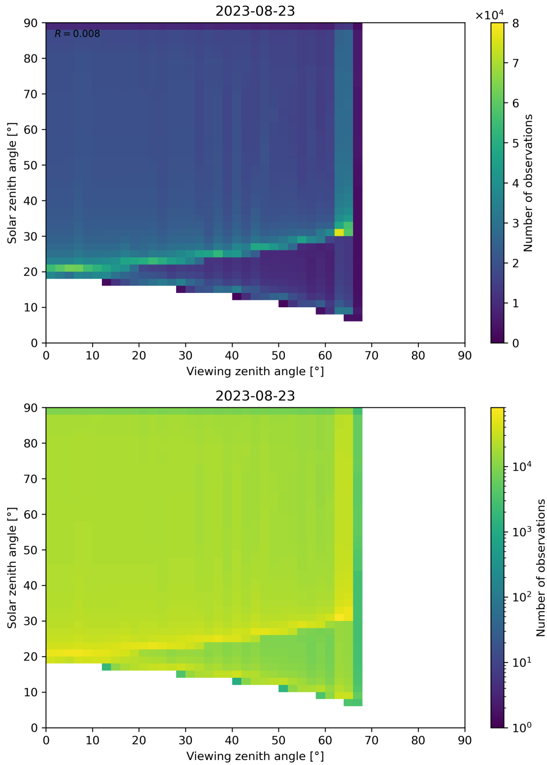
Figure 54: Scatter density plot of “Viewing zenith angle” against “Solar zenith angle” for 2023-08-22 to 2023-08-24.
