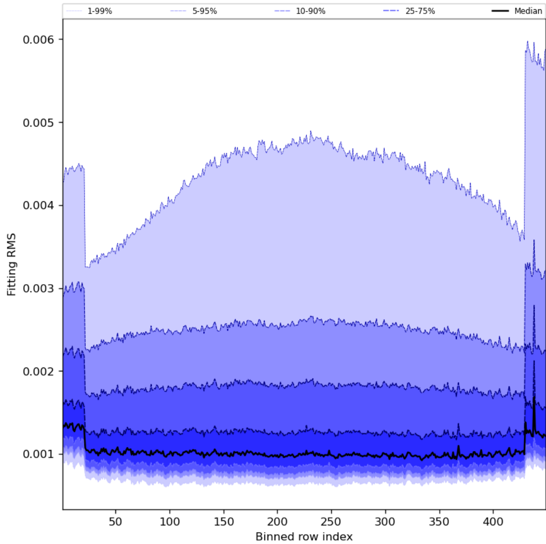
Figure 30: Along track statistics of “Fitting RMS” for 2023-08-22 to 2023-08-24
