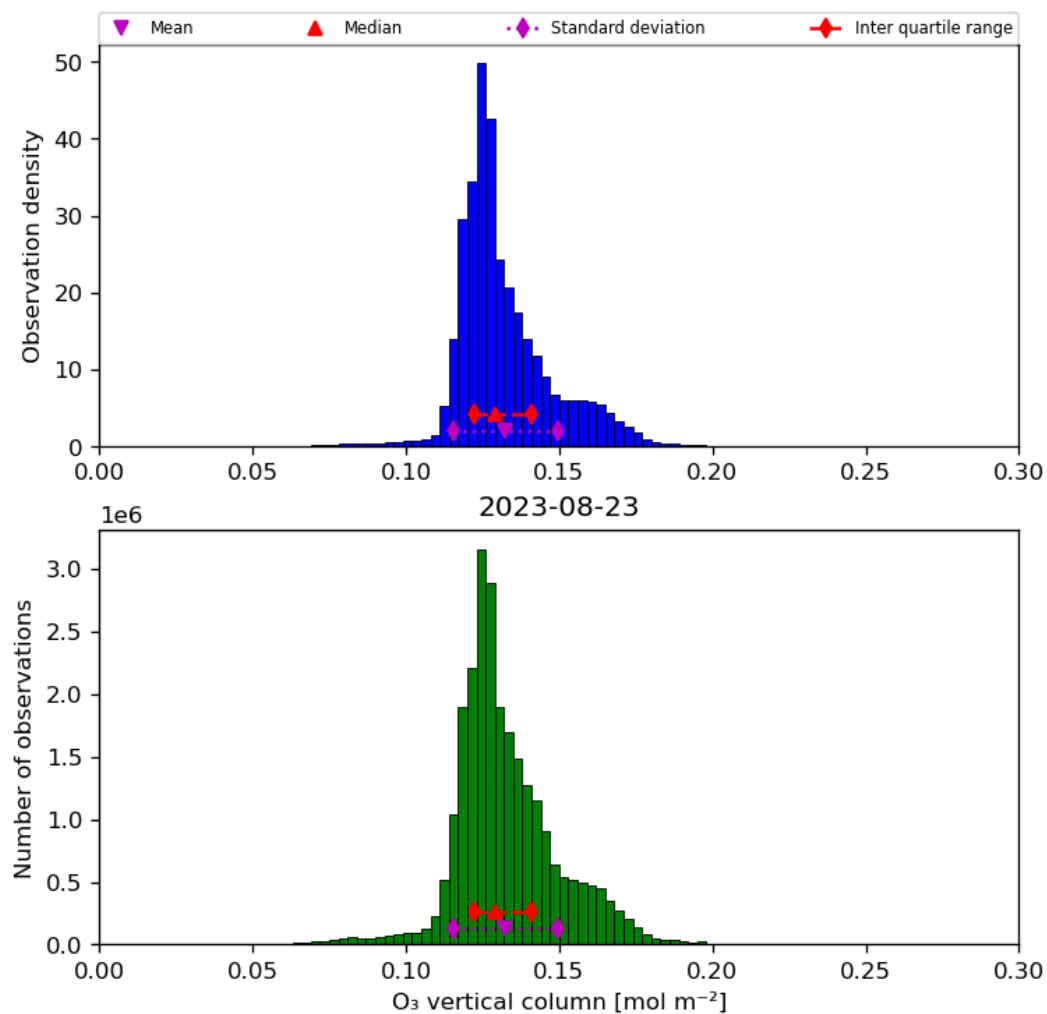
Figure 21: Histogram of “O 3 vertical column” for 2023-08-22 to 2023-08-24
