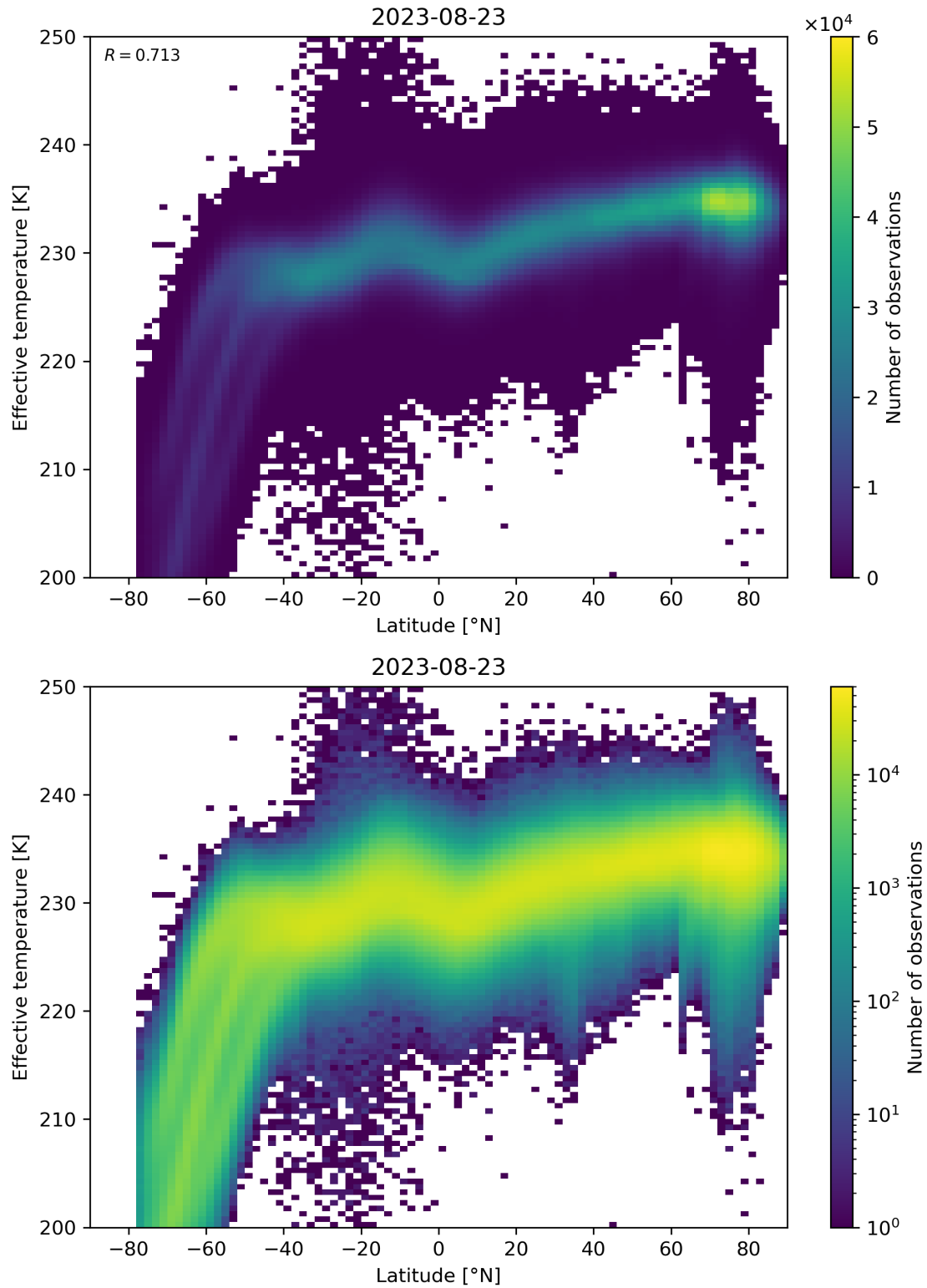
Figure 34: Scatter density plot of “Latitude” against “Effective temperature” for 2023-08-22 to 2023-08-24.
