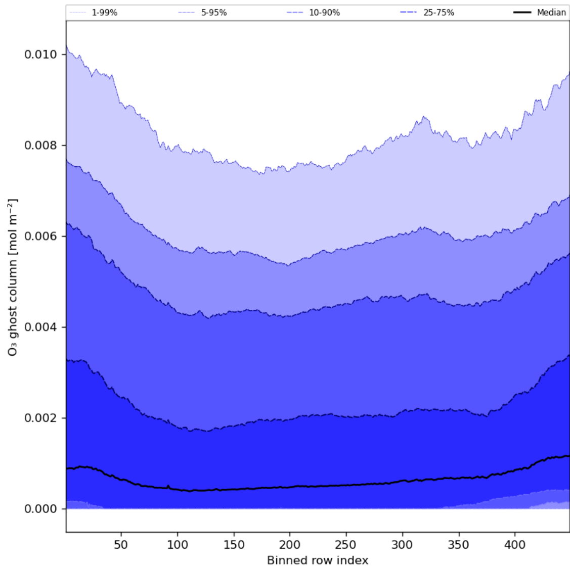
Figure 32: Along track statistics of “O 3 ghost column” for 2023-08-22 to 2023-08-24
