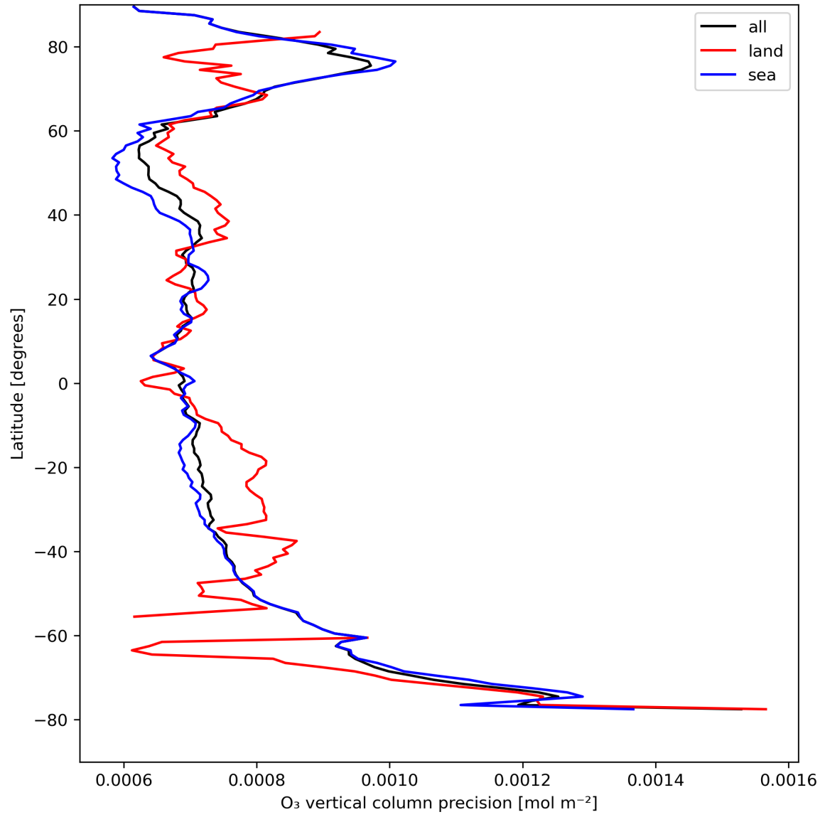
Figure 15: Zonal average of "O 3 vertical column precision" for 2023-08-22 to 2023-08-24.
