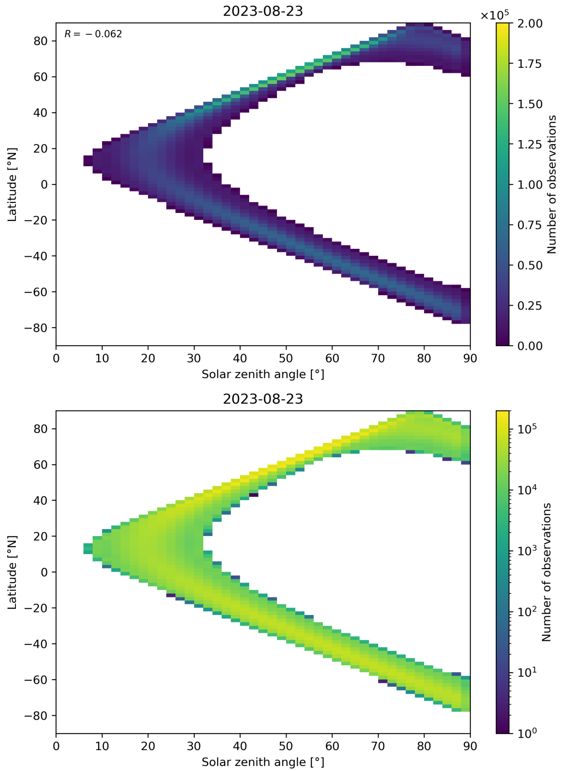
Figure 44: Scatter density plot of “Solar zenith angle” against “Latitude” for 2023-08-22 to 2023-08-24.
