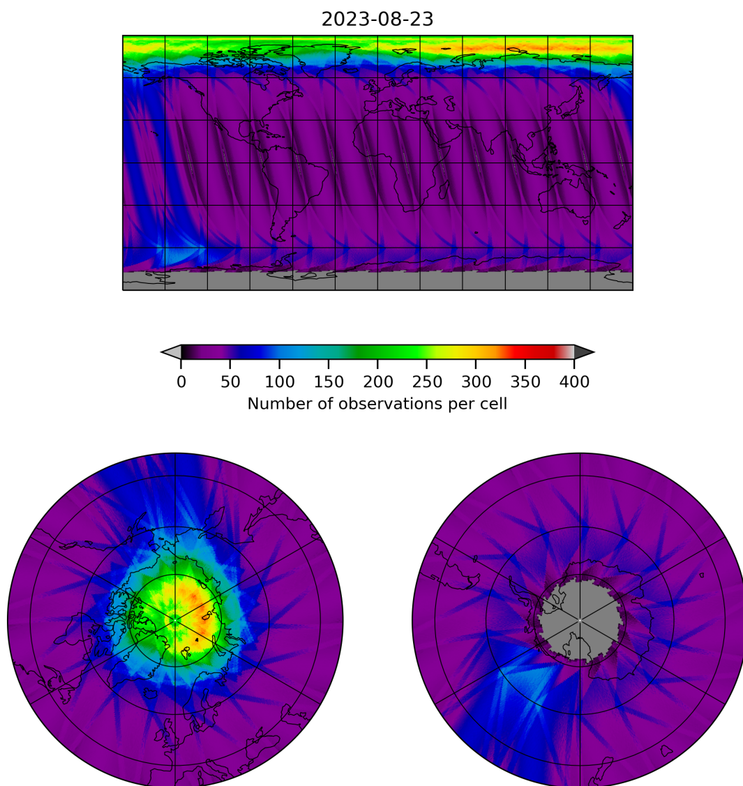
Figure 12: Map of the number of observations for 2023-08-22 to 2023-08-24
