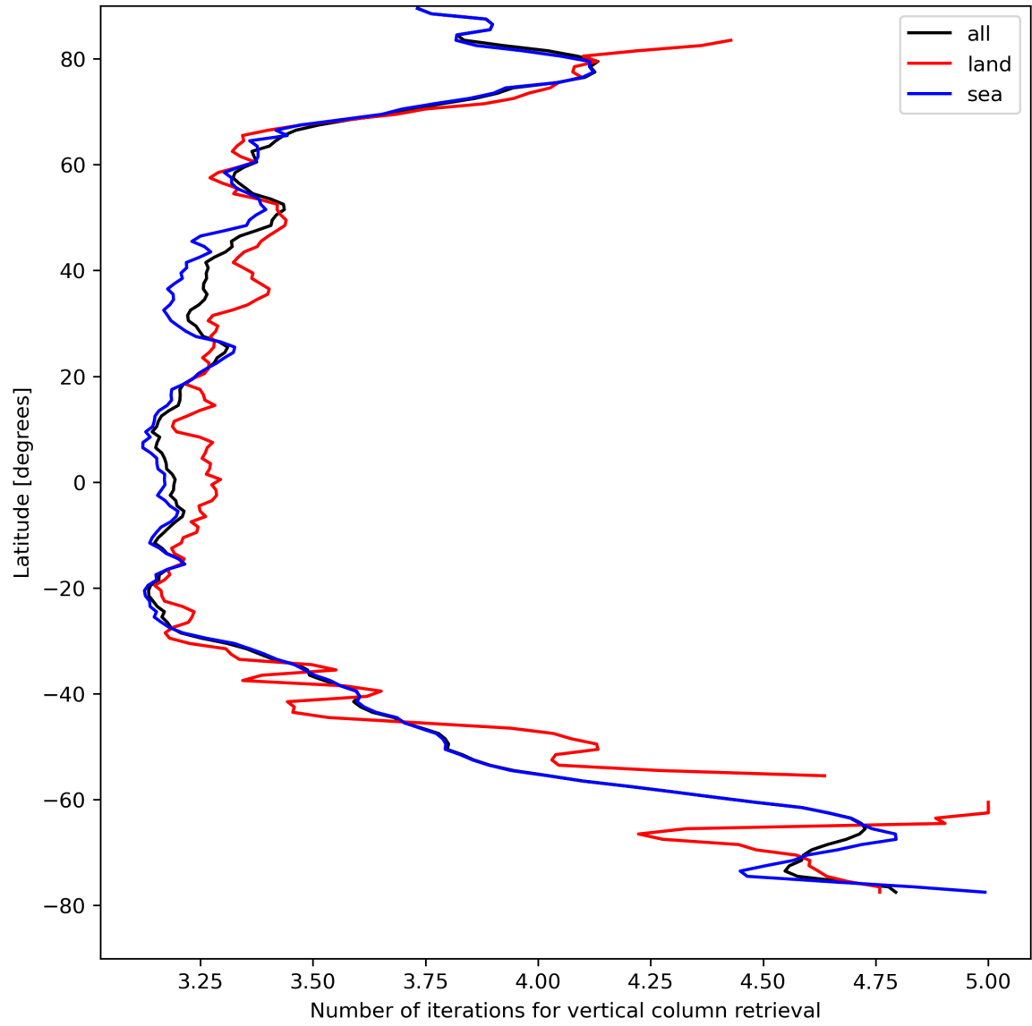
Figure 19: Zonal average of “Number of iterations for vertical column retrieval” for 2023-08-22 to 2023-08-24.
