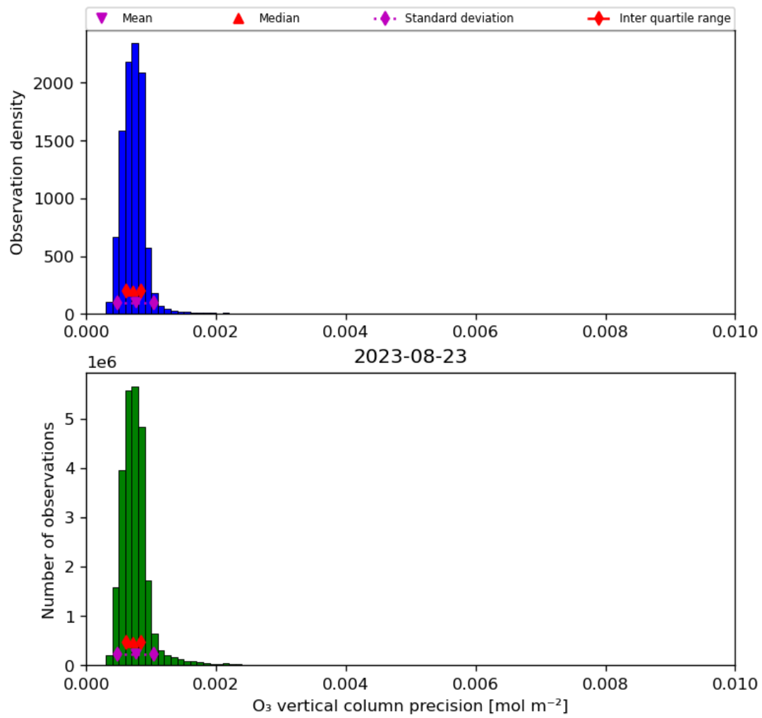
Figure 22: Histogram of “O 3 vertical column precision” for 2023-08-22 to 2023-08-24
