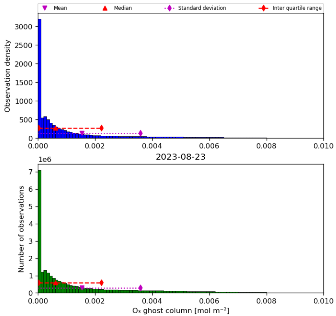
Figure 25: Histogram of “O 3 ghost column” for 2023-08-22 to 2023-08-24
