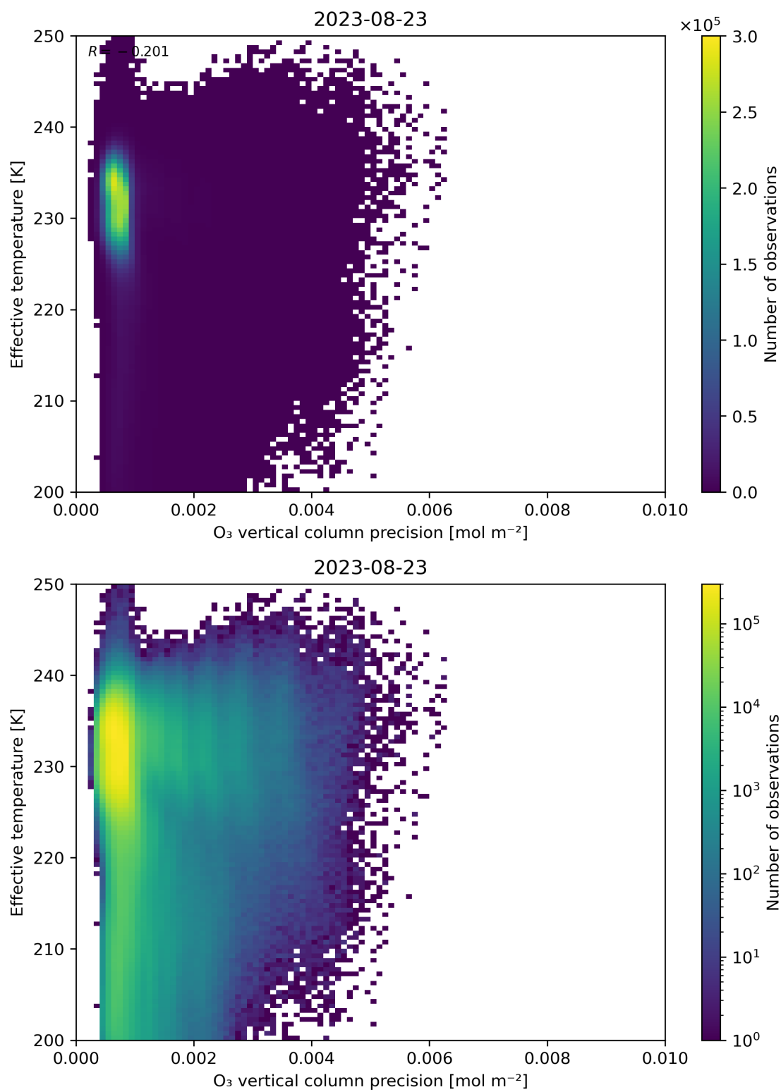
Figure 42: Scatter density plot of “O 3 vertical column precision” against “Effective temperature” for 2023-08-22 to 2023-08-24.
