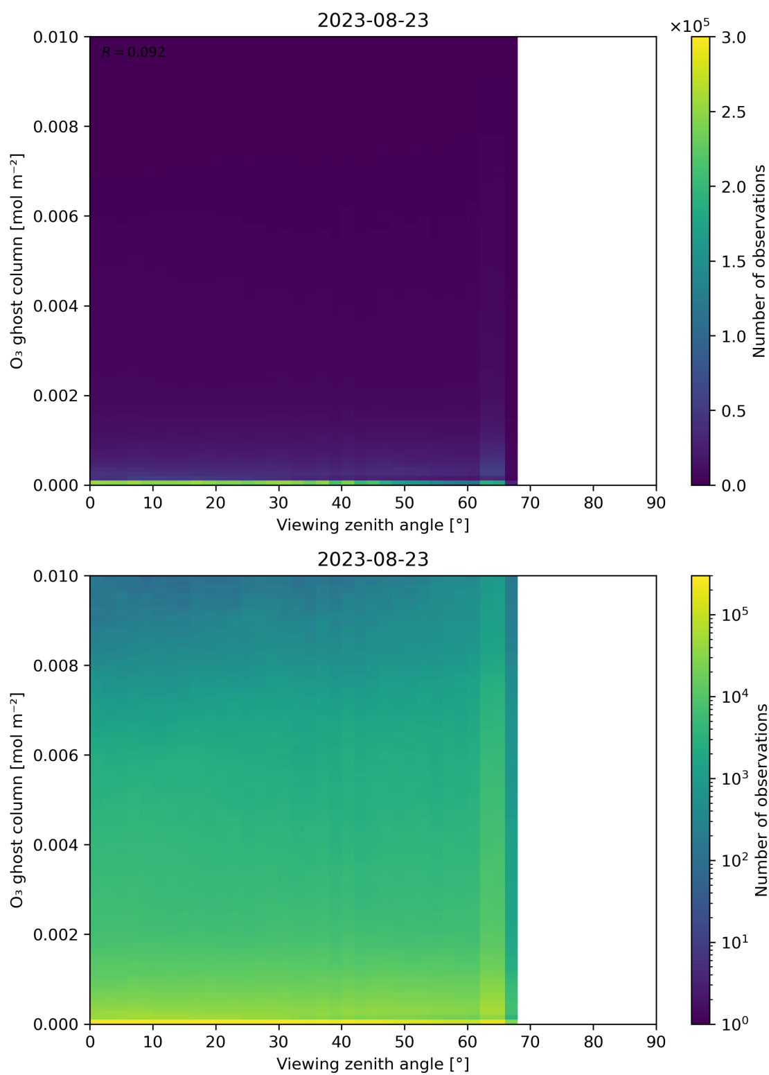
Figure 51: Scatter density plot of “Viewing zenith angle” against “O 3 ghost column” for 2023-08-22 to 2023-08-24.
