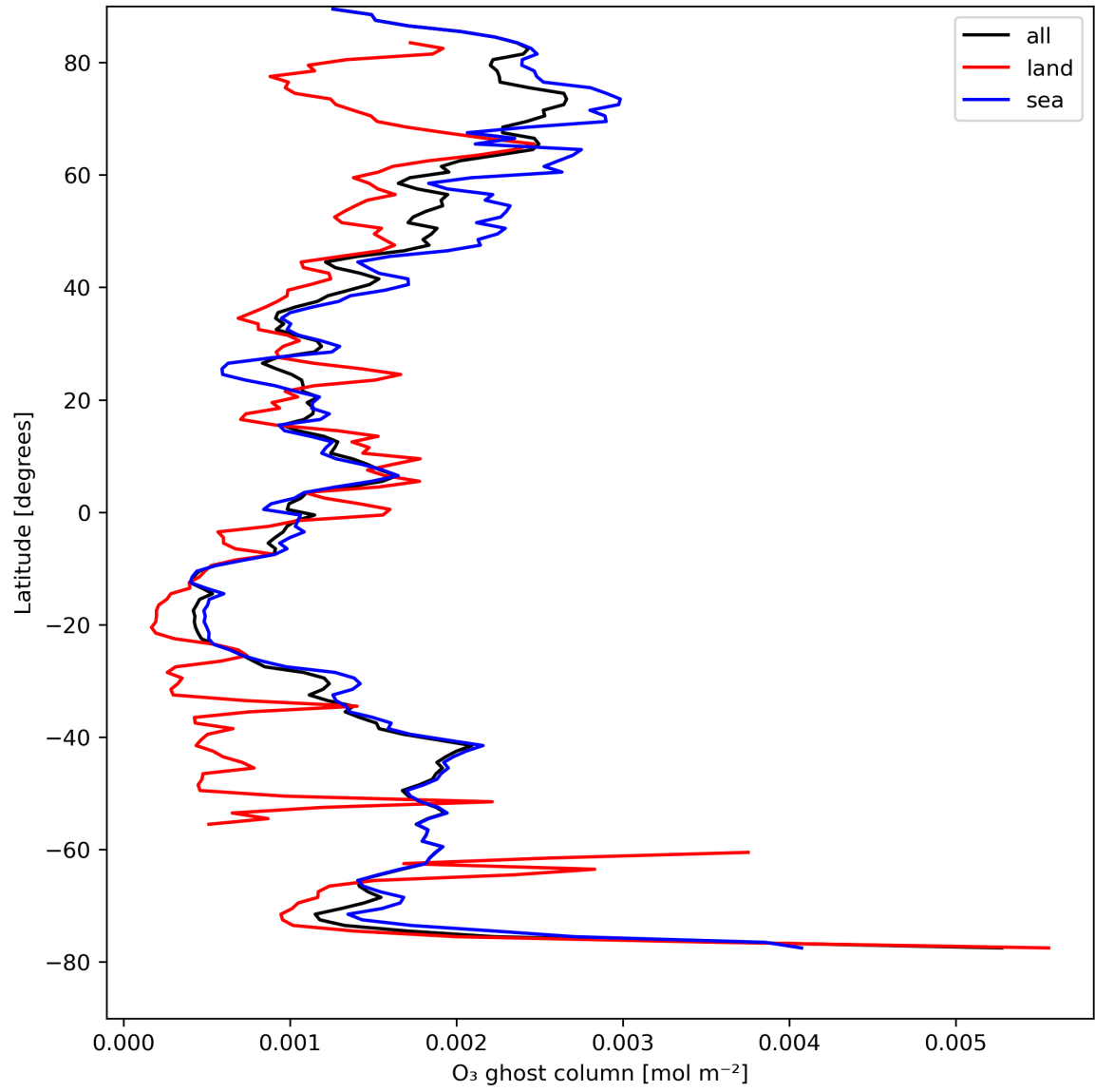
Figure 18: Zonal average of "O 3 ghost column" for 2023-08-22 to 2023-08-24.
