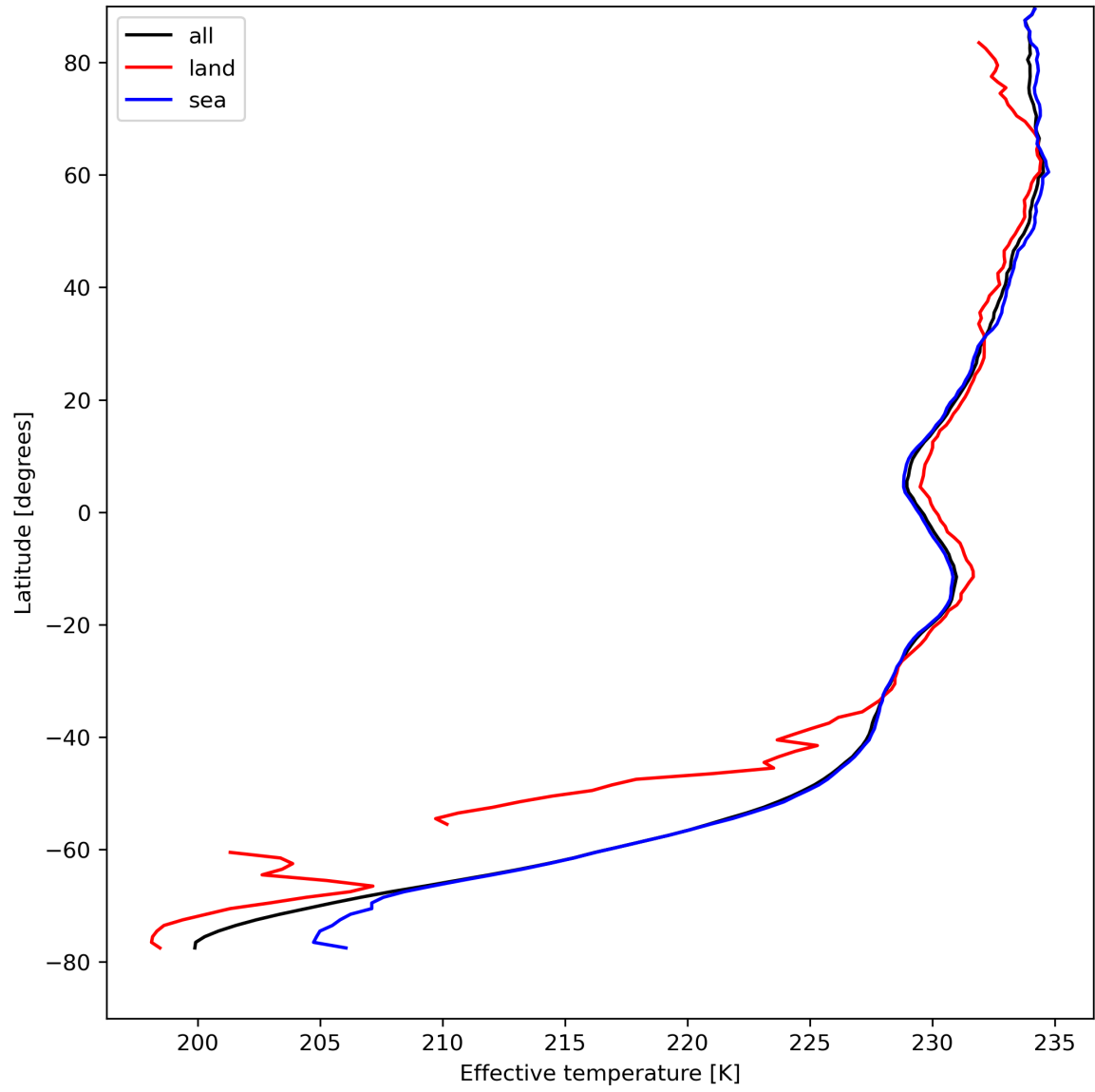
Figure 17: Zonal average of "Effective temperature" for 2023-08-22 to 2023-08-24.
