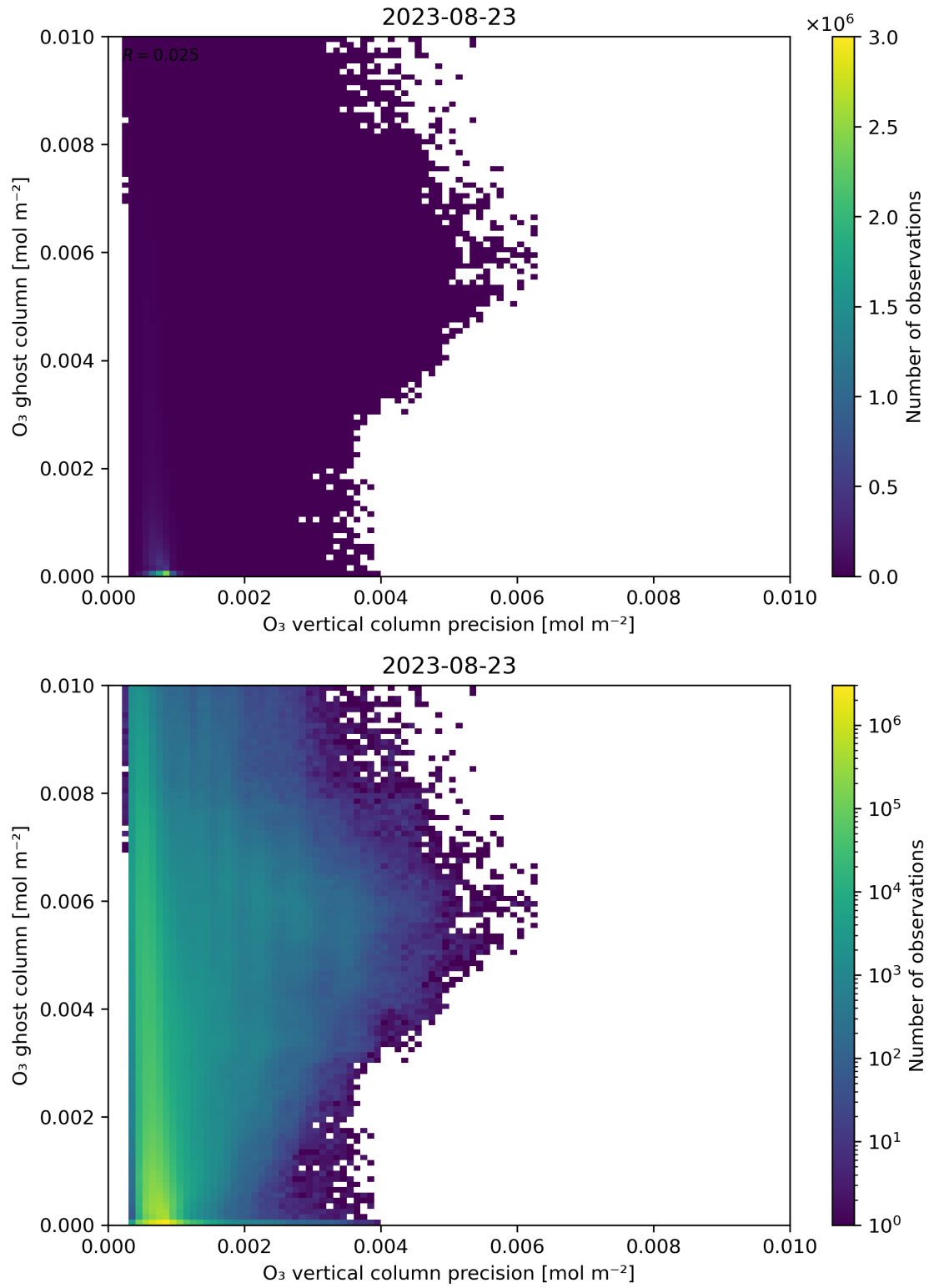
Figure 43: Scatter density plot of “ O_3 vertical column precision” against “ O_3 ghost column” for 2023-08-22 to 2023-08-24.
