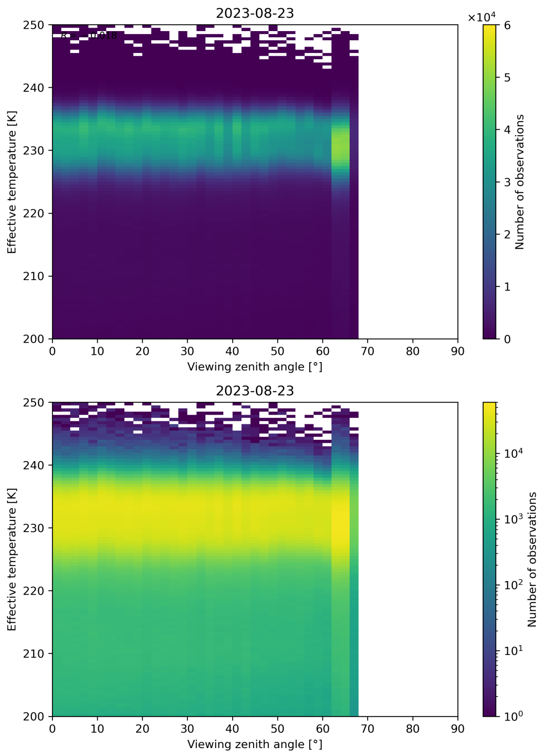
Figure 50: Scatter density plot of “Viewing zenith angle” against “Effective temperature” for 2023-08-22 to 2023-08-24.
