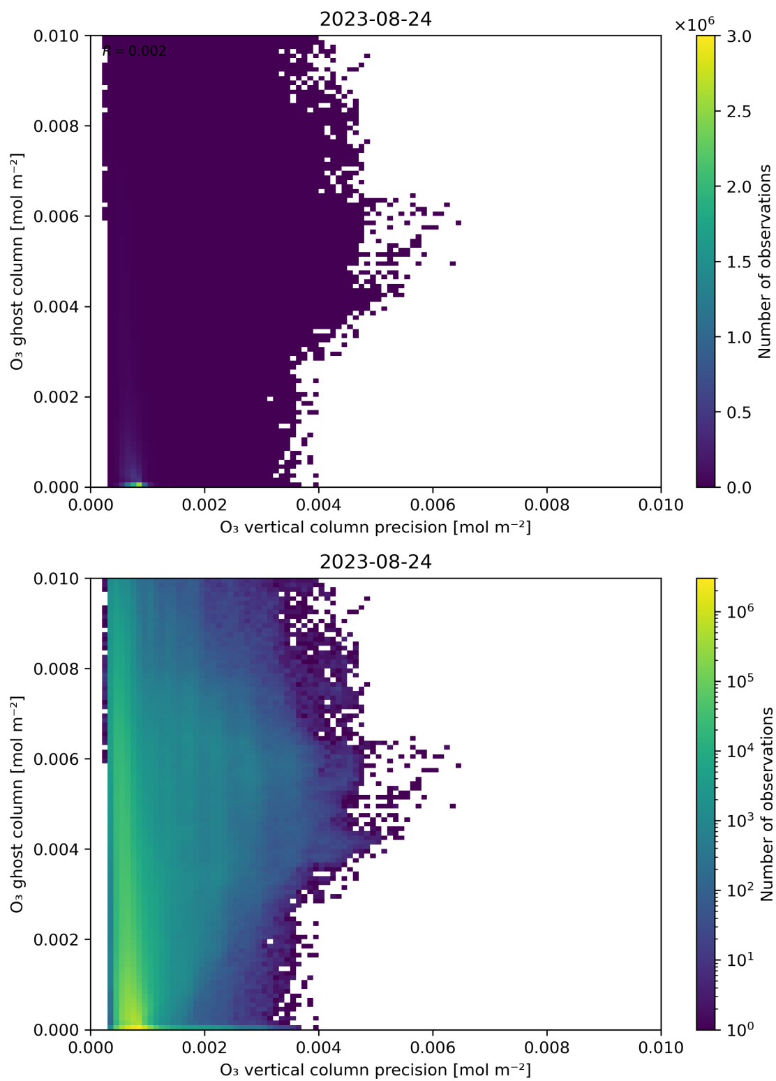
Figure 43: Scatter density plot of “O 3 vertical column precision” against “O 3 ghost column” for 2023-08-23 to 2023-08-25.
