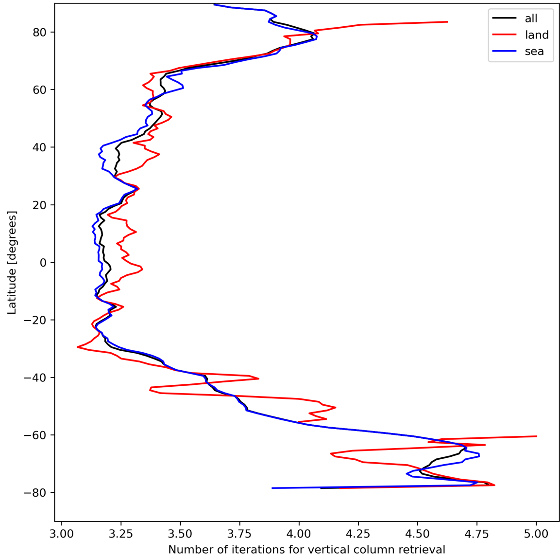
Figure 19: Zonal average of “Number of iterations for vertical column retrieval” for 2023-08-23 to 2023-08-25.
