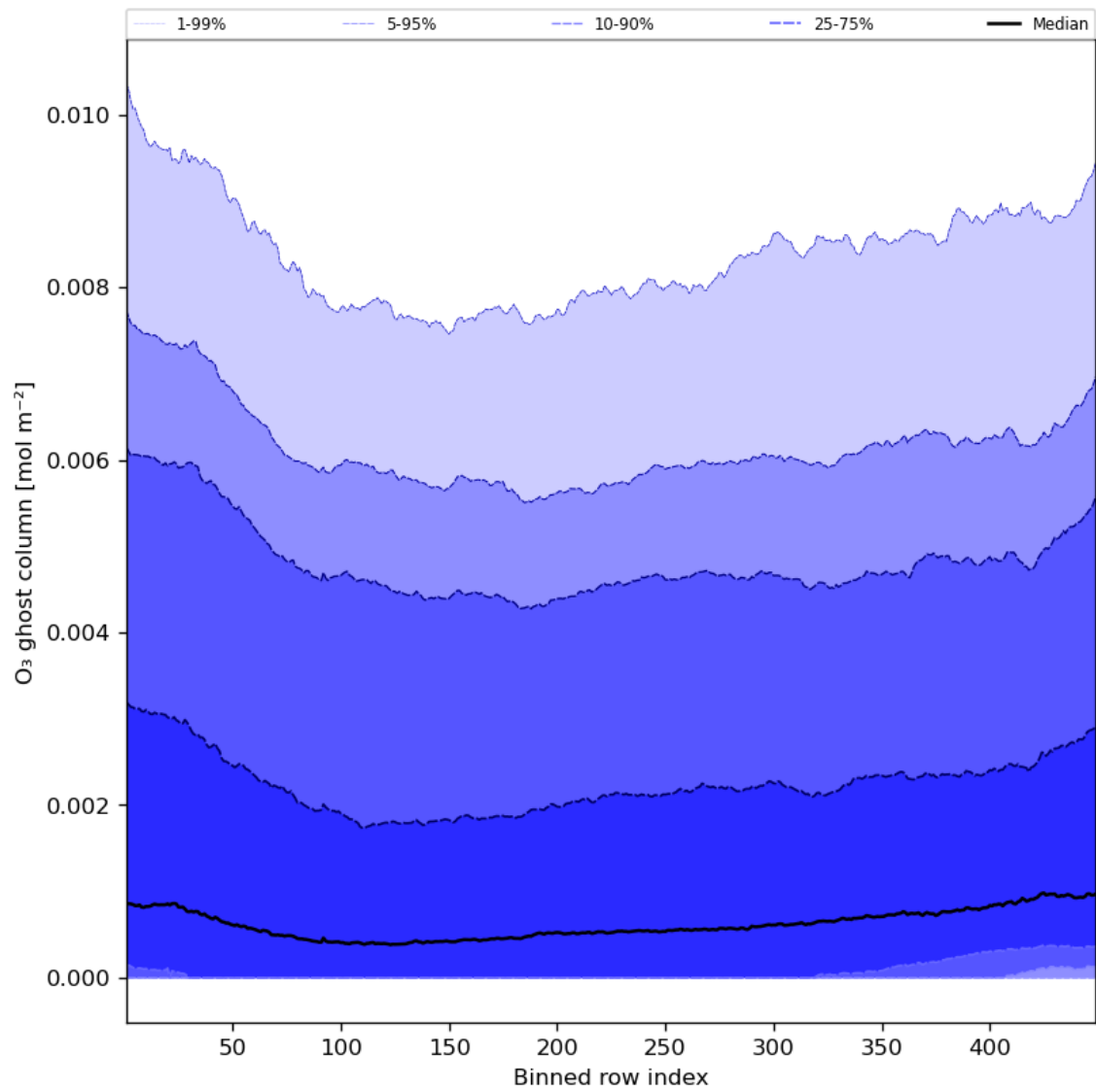
Figure 32: Along track statistics of “O 3 ghost column” for 2023-08-23 to 2023-08-25
