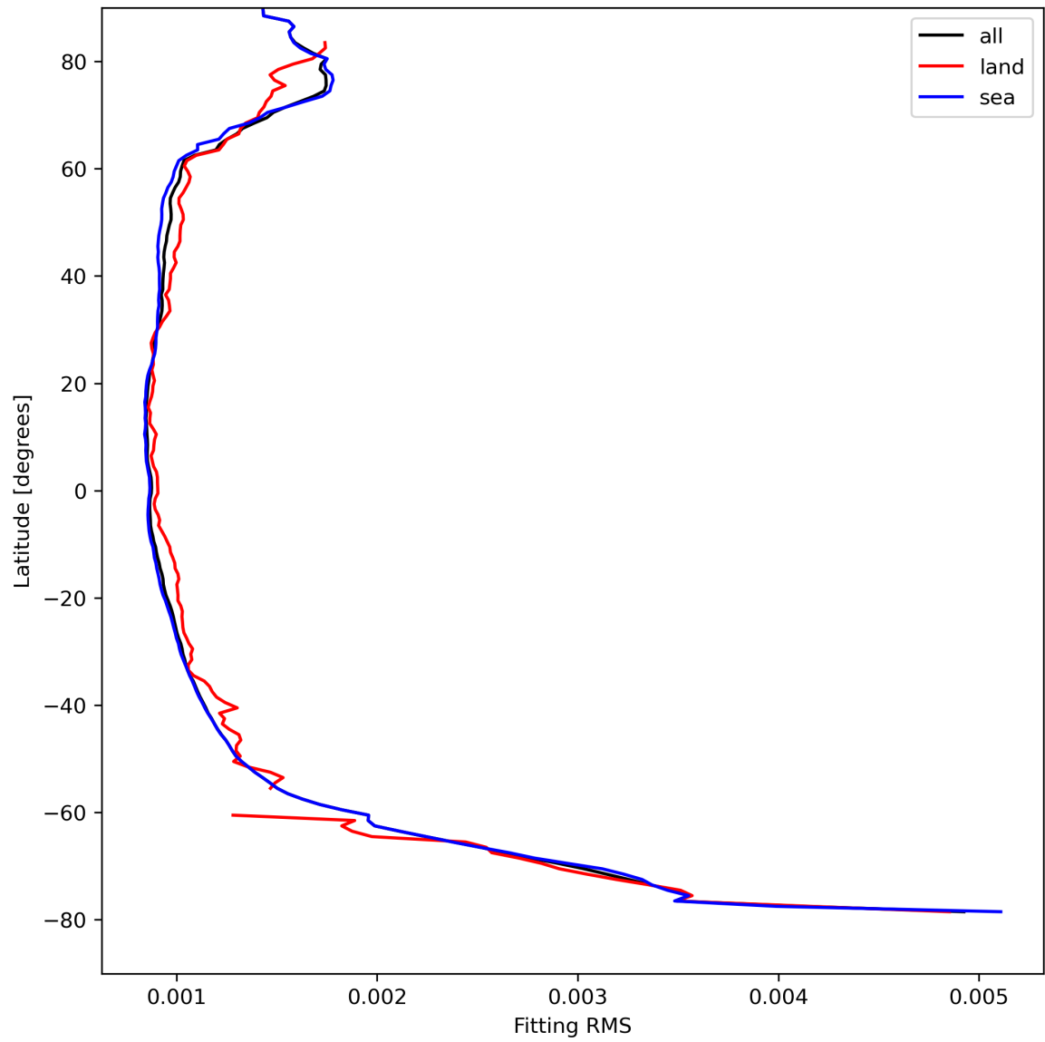
Figure 16: Zonal average of “Fitting RMS” for 2023-08-23 to 2023-08-25.
