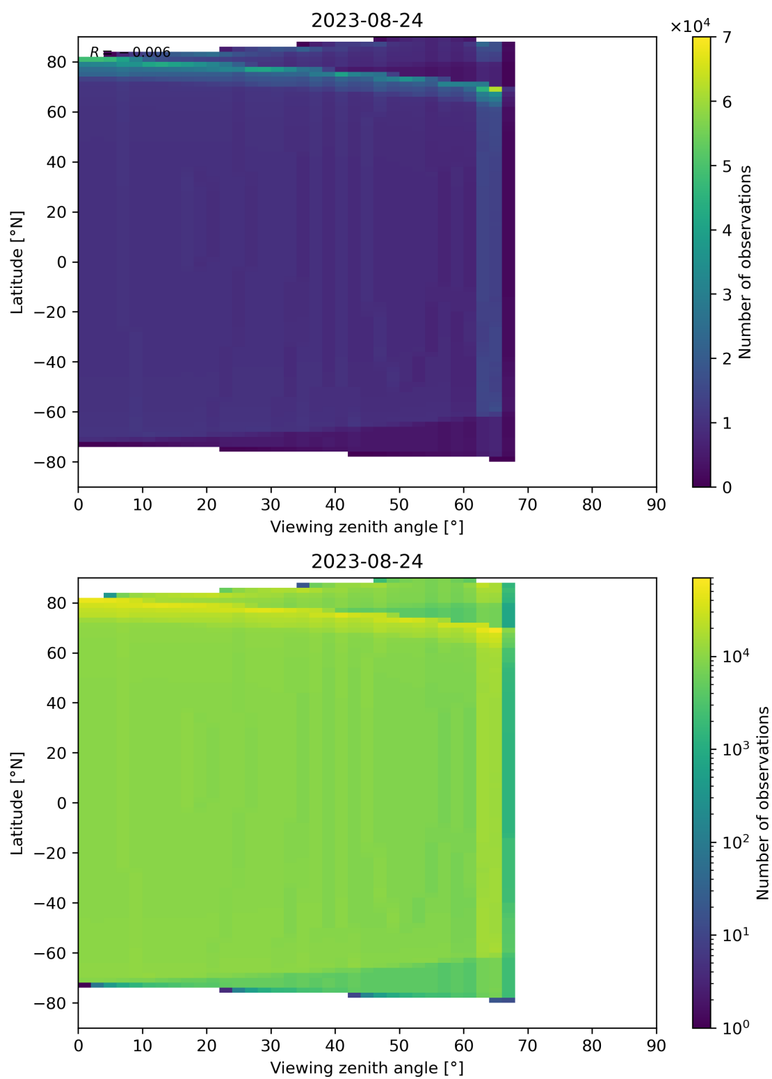
Figure 49: Scatter density plot of “Viewing zenith angle” against “Latitude” for 2023-08-23 to 2023-08-25.
