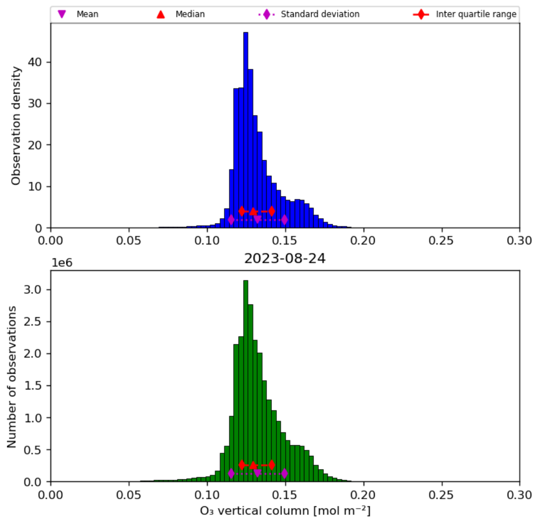
Figure 21: Histogram of “O 3 vertical column” for 2023-08-23 to 2023-08-25
