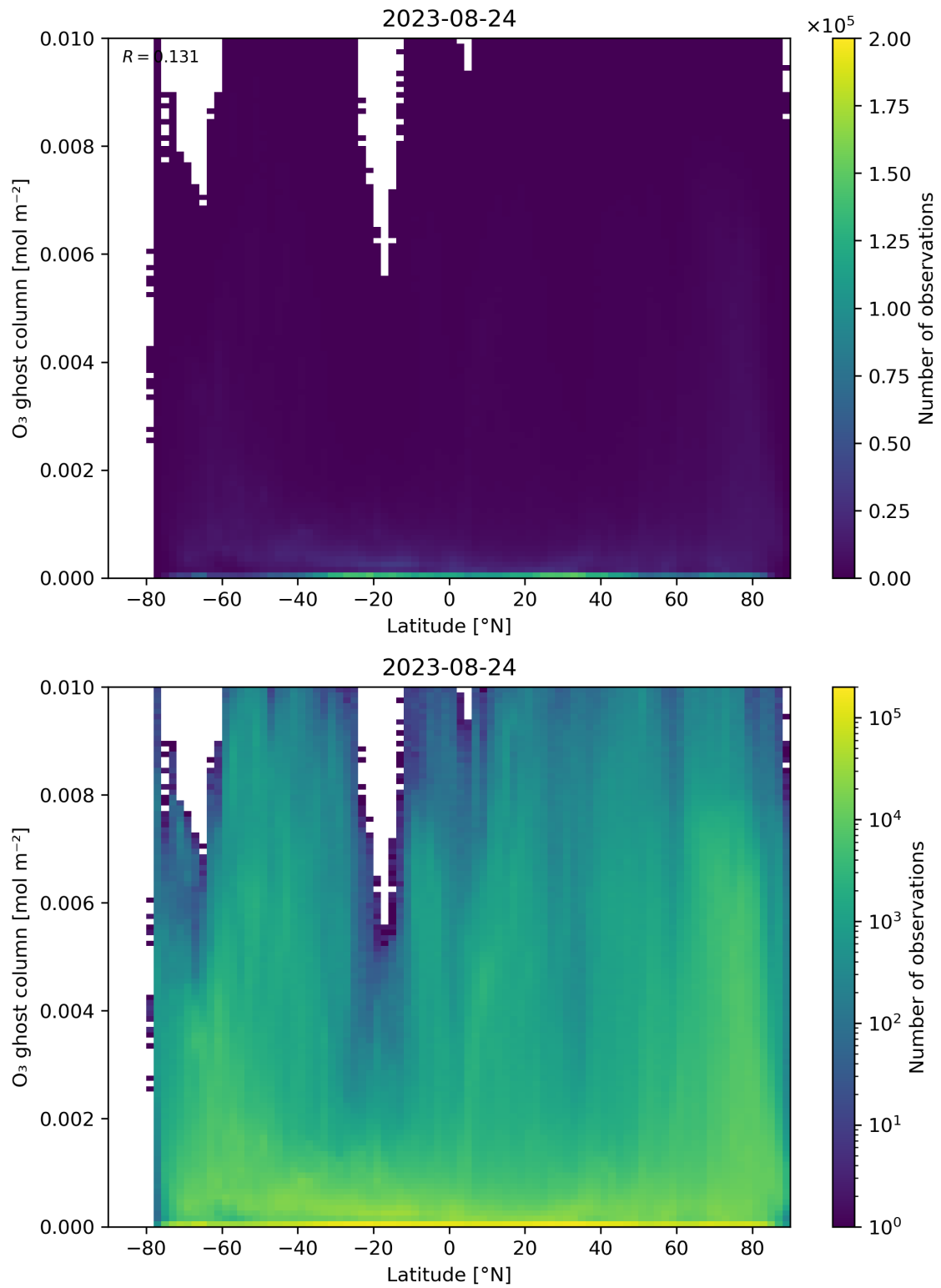
Figure 35: Scatter density plot of “Latitude” against “O 3 ghost column” for 2023-08-23 to 2023-08-25.
