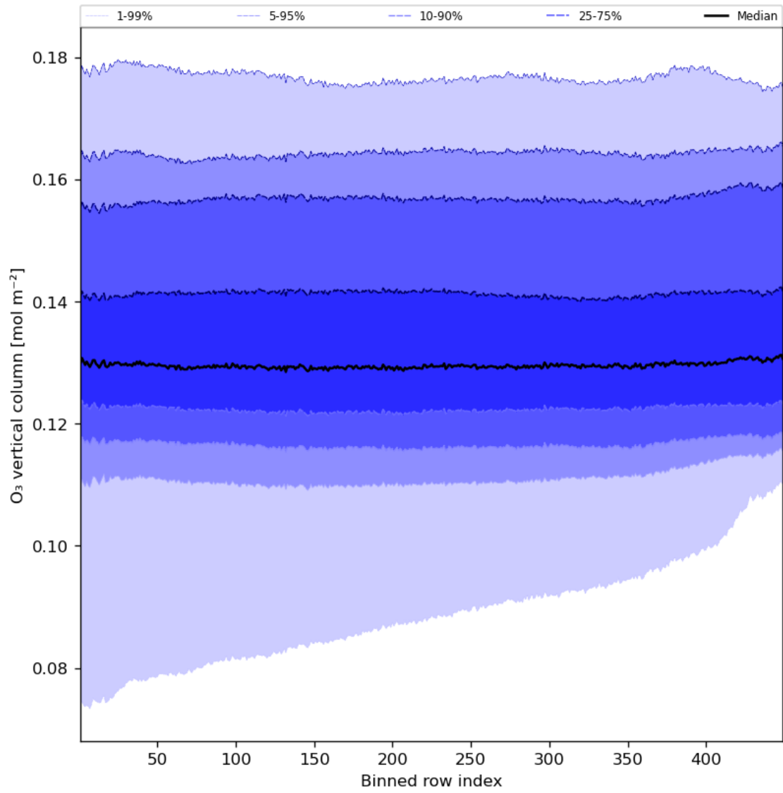
Figure 28: Along track statistics of “O 3 vertical column” for 2023-08-23 to 2023-08-25
