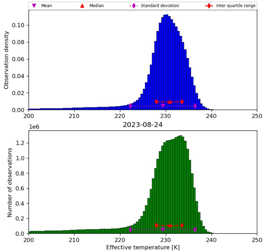
Figure 24: Histogram of “Effective temperature” for 2023-08-23 to 2023-08-25
