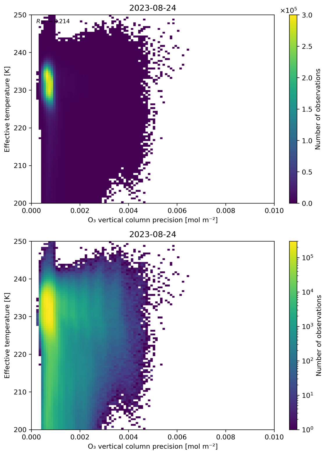
Figure 42: Scatter density plot of “O 3 vertical column precision” against “Effective temperature” for 2023-08-23 to 2023-08-25.
