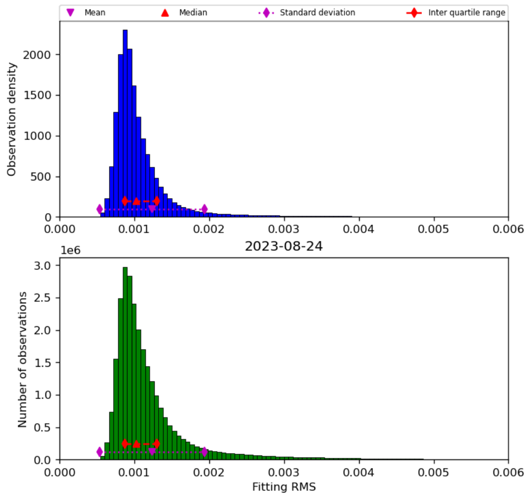
Figure 23: Histogram of “Fitting RMS” for 2023-08-23 to 2023-08-25
