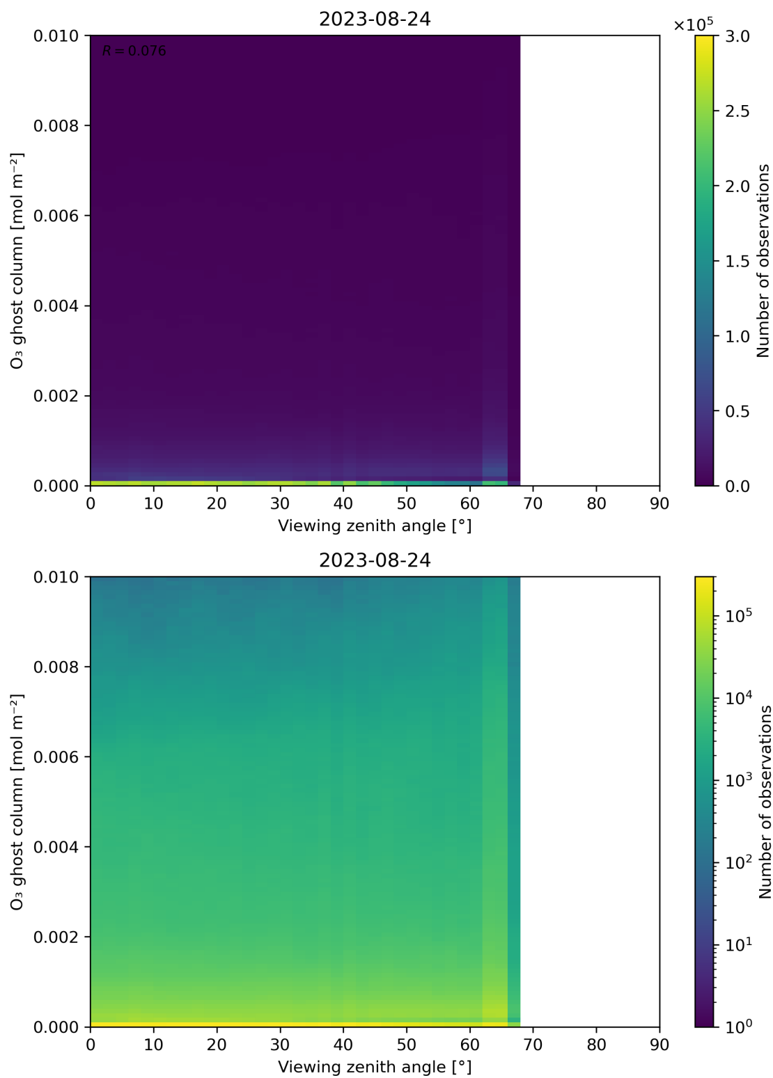
Figure 51: Scatter density plot of “Viewing zenith angle” against “O 3 ghost column” for 2023-08-23 to 2023-08-25.
