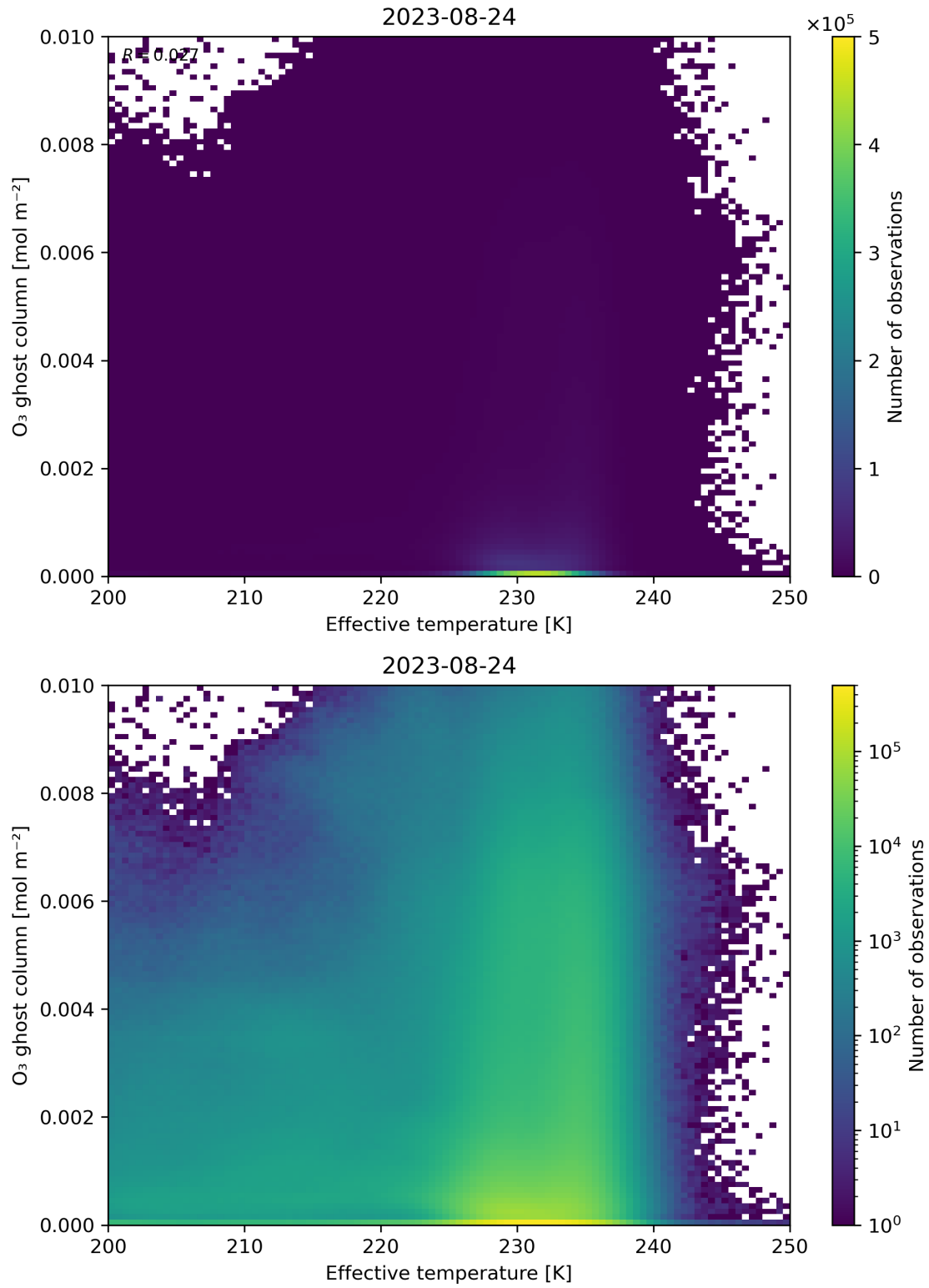
Figure 38: Scatter density plot of “Effective temperature” against “O 3 ghost column” for 2023-08-23 to 2023-08-25.
