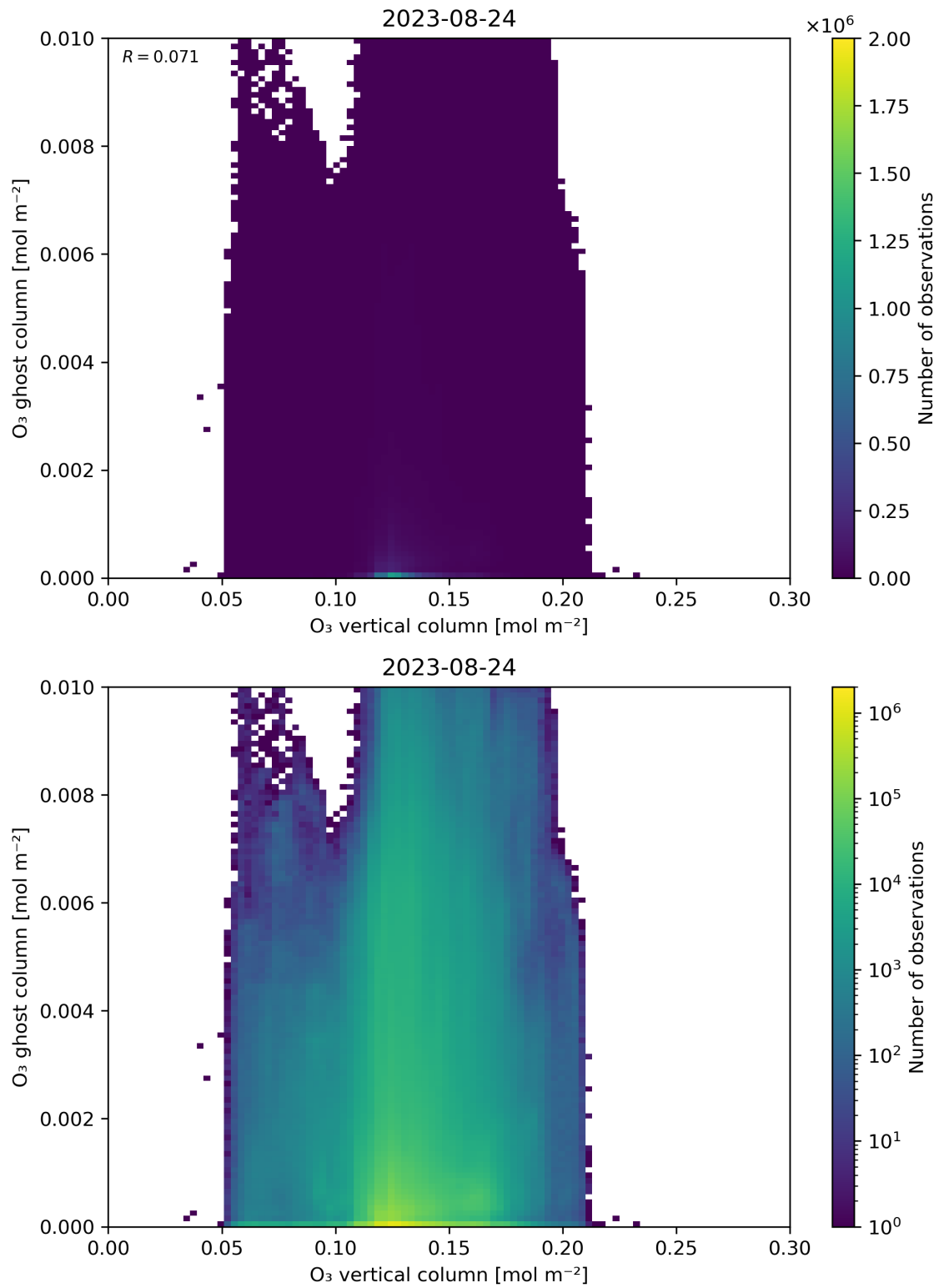
Figure 40: Scatter density plot of “O 3 vertical column” against “O 3 ghost column” for 2023-08-23 to 2023-08-25.
