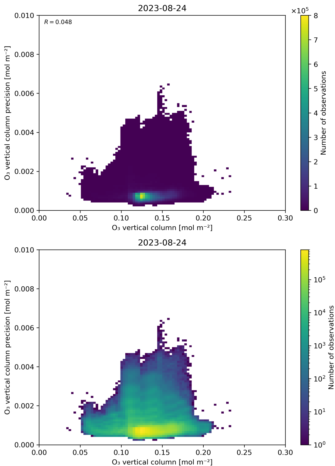
Figure 41: Scatter density plot of “O 3 vertical column” against “O 3 vertical column precision” for 2023-08-23 to 2023-08-25.
