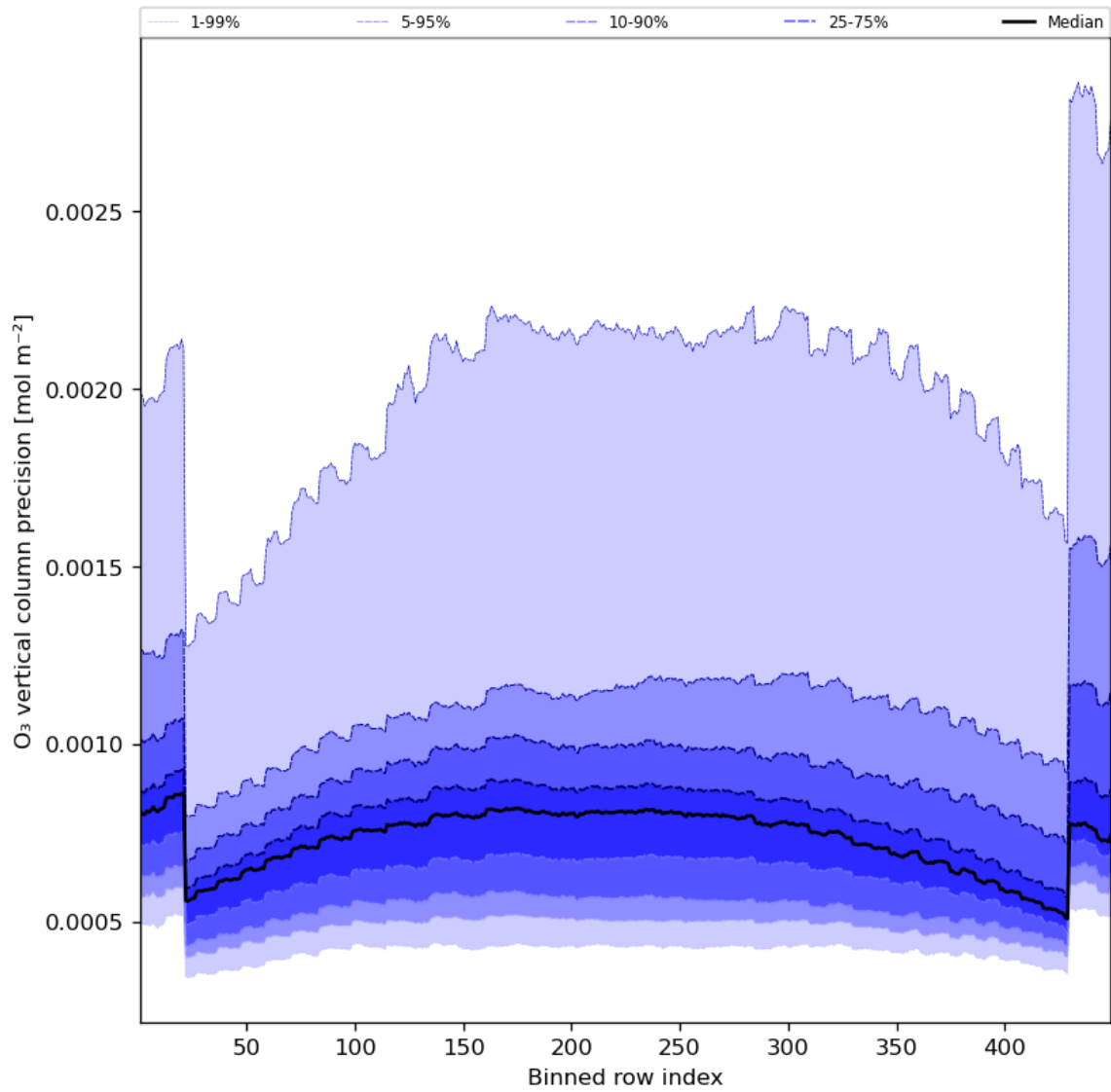
Figure 29: Along track statistics of “O 3 vertical column precision” for 2023-08-23 to 2023-08-25
