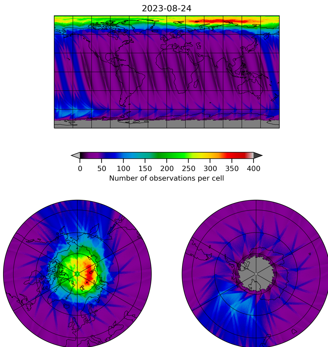
Figure 12: Map of the number of observations for 2023-08-23 to 2023-08-25
