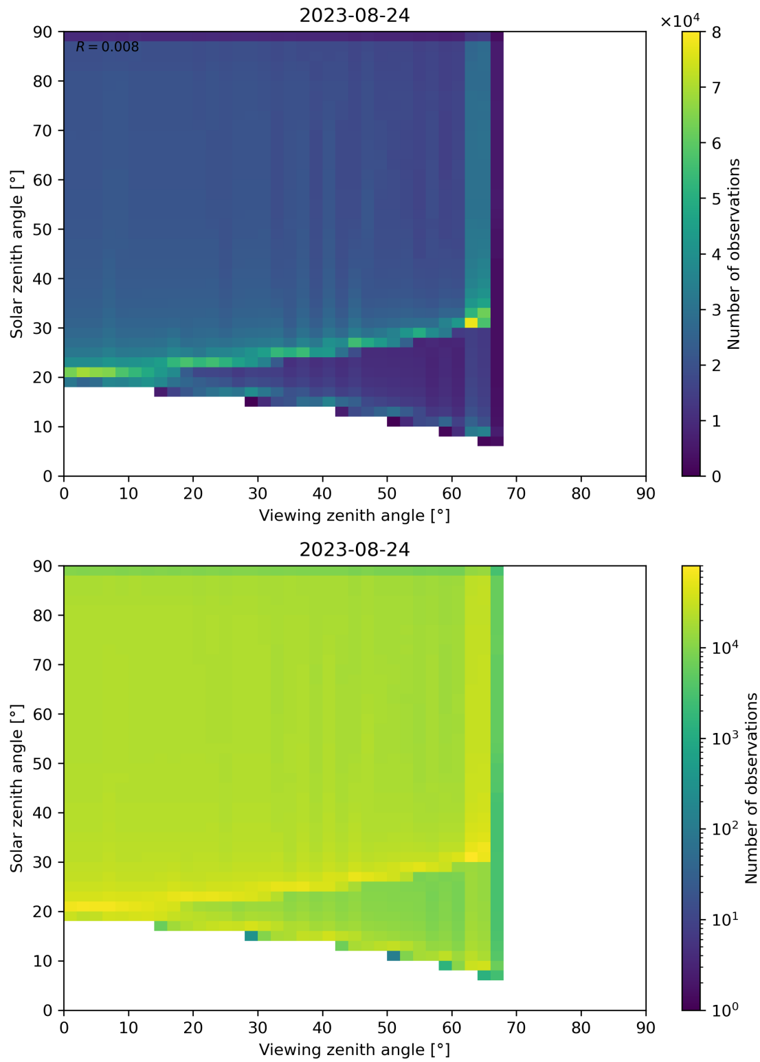
Figure 54: Scatter density plot of “Viewing zenith angle” against “Solar zenith angle” for 2023-08-23 to 2023-08-25.
