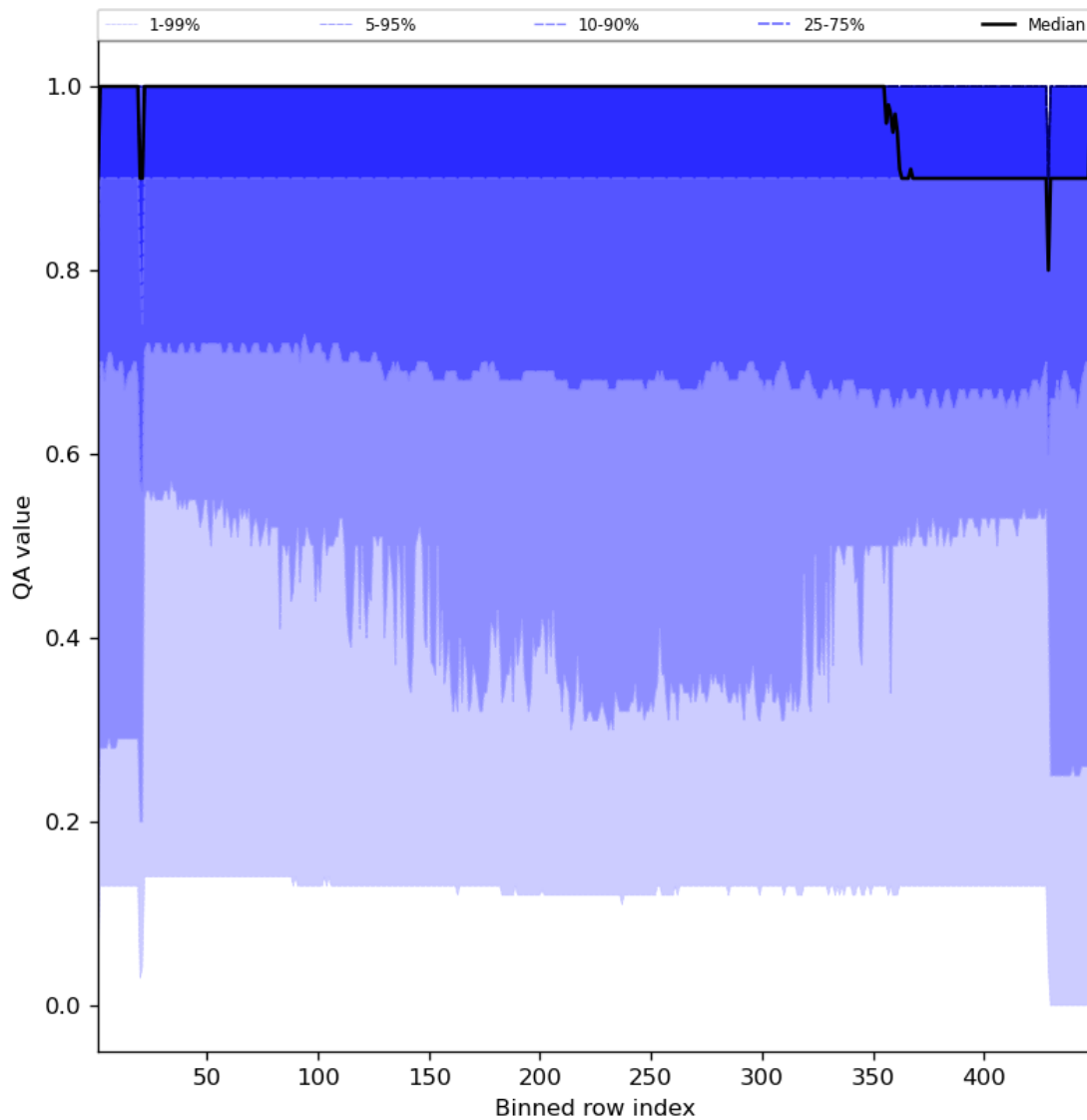
Figure 27: Along track statistics of “QA value” for 2023-08-23 to 2023-08-25
