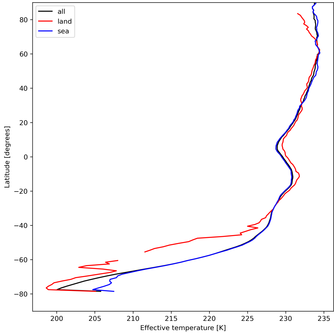
Figure 17: Zonal average of "Effective temperature" for 2023-08-23 to 2023-08-25.
