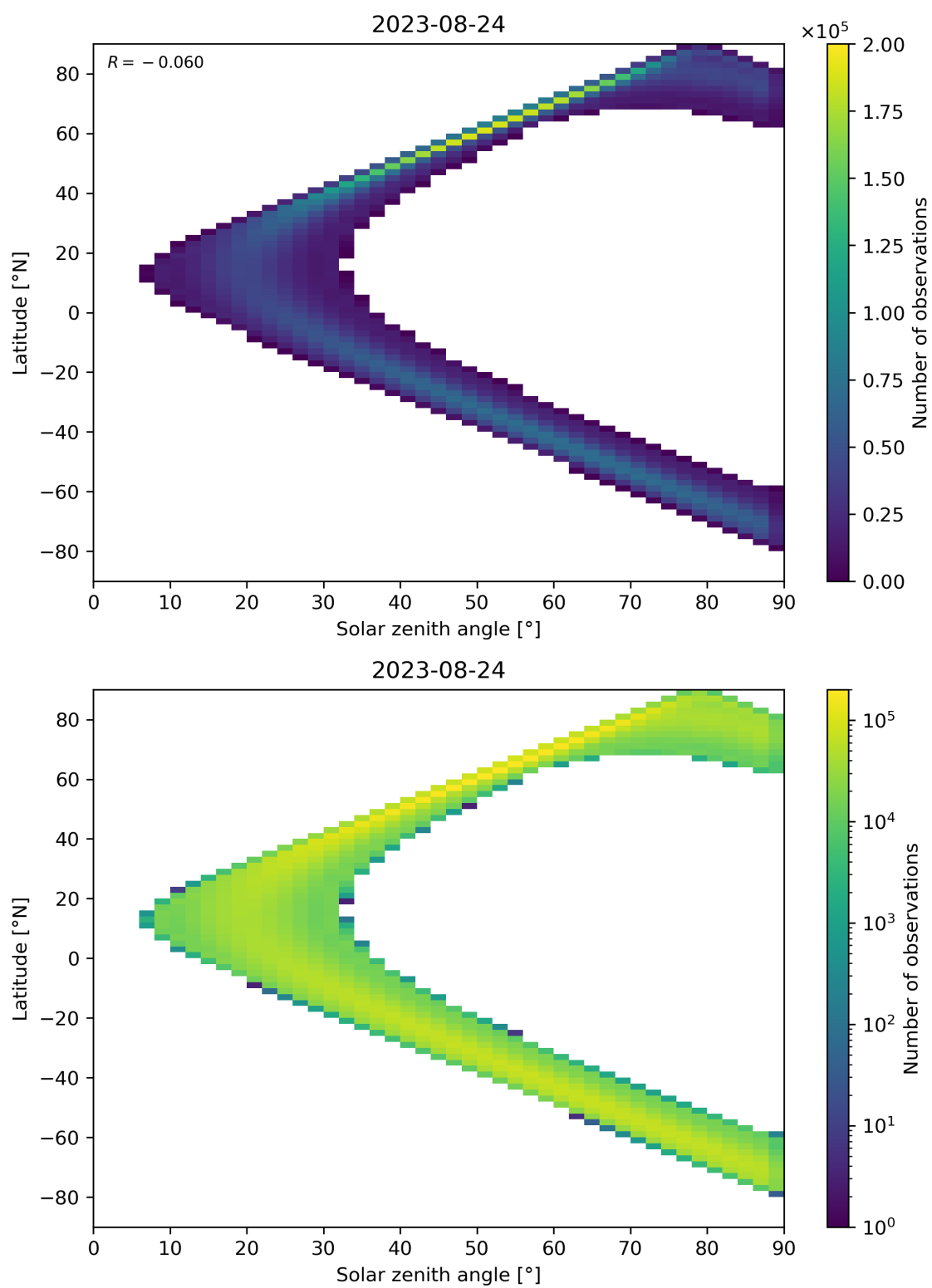
Figure 44: Scatter density plot of “Solar zenith angle” against “Latitude” for 2023-08-23 to 2023-08-25.
