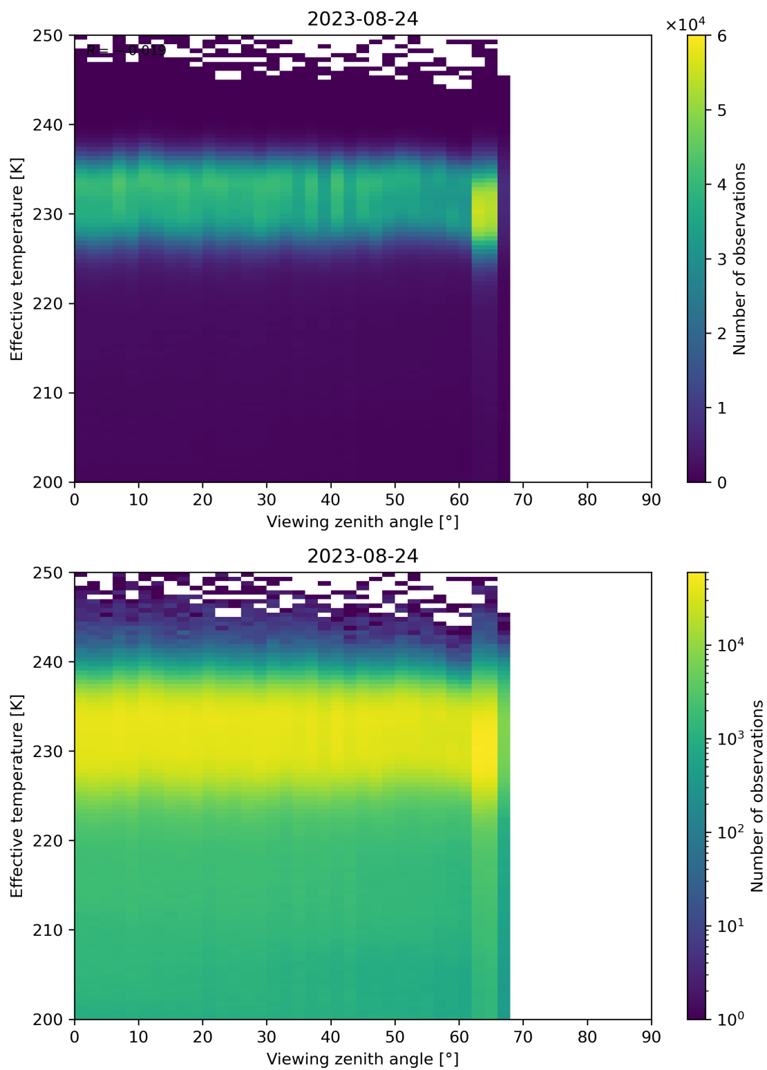
Figure 50: Scatter density plot of “Viewing zenith angle” against “Effective temperature” for 2023-08-23 to 2023-08-25.
