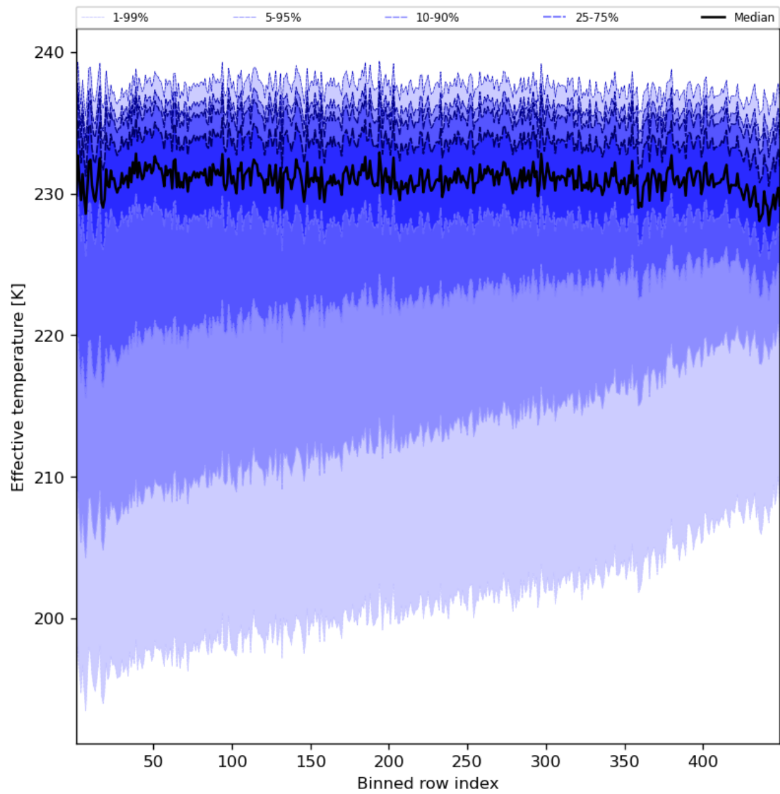
Figure 31: Along track statistics of “Effective temperature” for 2023-08-23 to 2023-08-25
