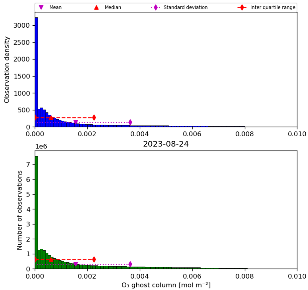
Figure 25: Histogram of “O 3 ghost column” for 2023-08-23 to 2023-08-25
