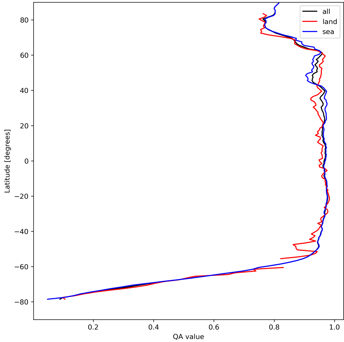
Figure 13: Zonal average of “QA value” for 2023-08-23 to 2023-08-25.
