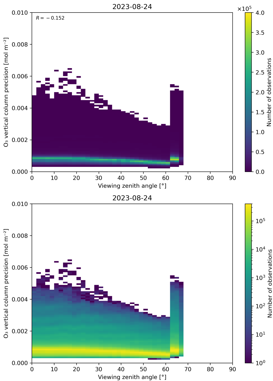
Figure 53: Scatter density plot of “Viewing zenith angle” against “O 3 vertical column precision” for 2023-08-23 to 2023-08-25.
