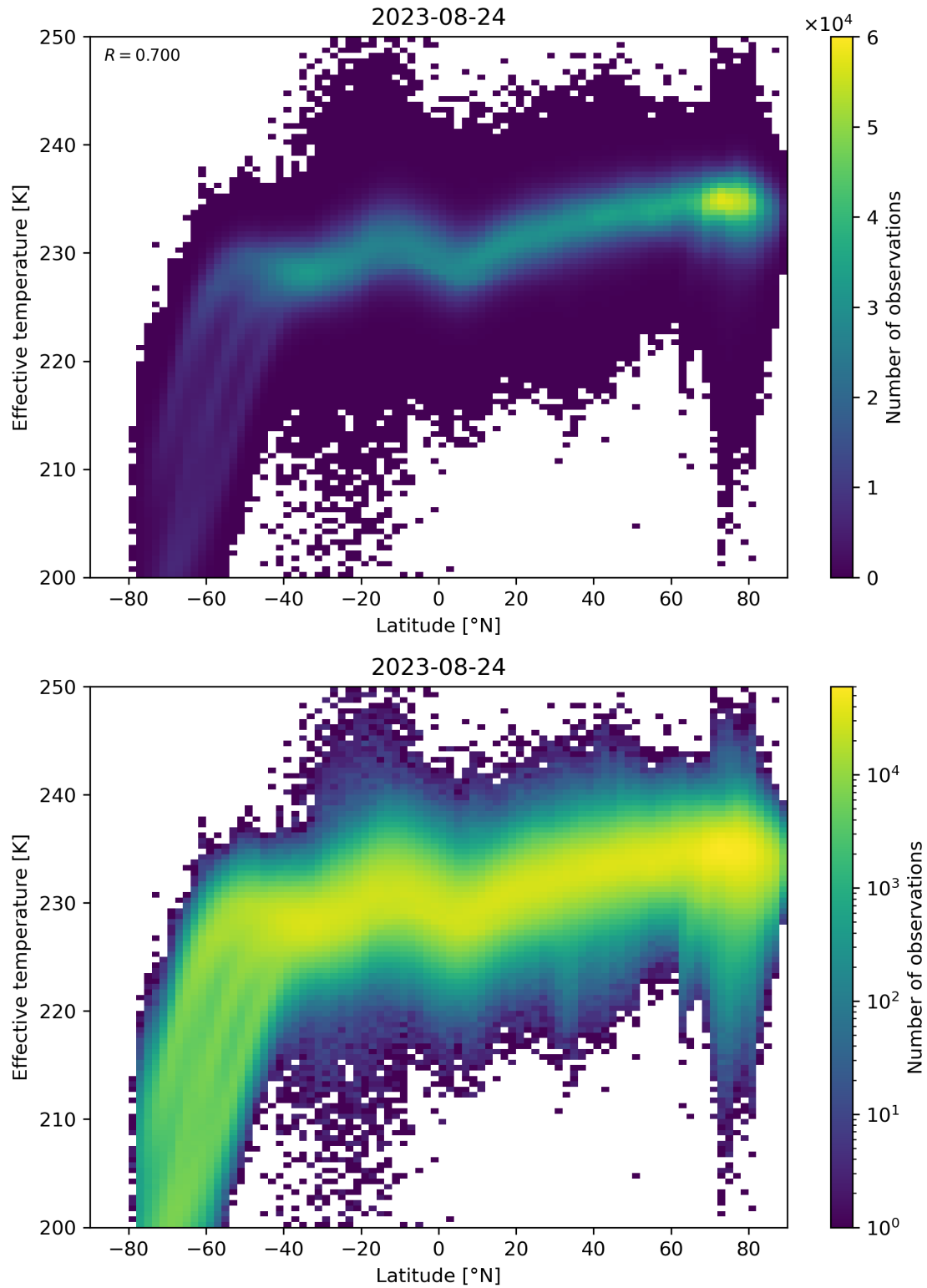
Figure 34: Scatter density plot of “Latitude” against “Effective temperature” for 2023-08-23 to 2023-08-25.
