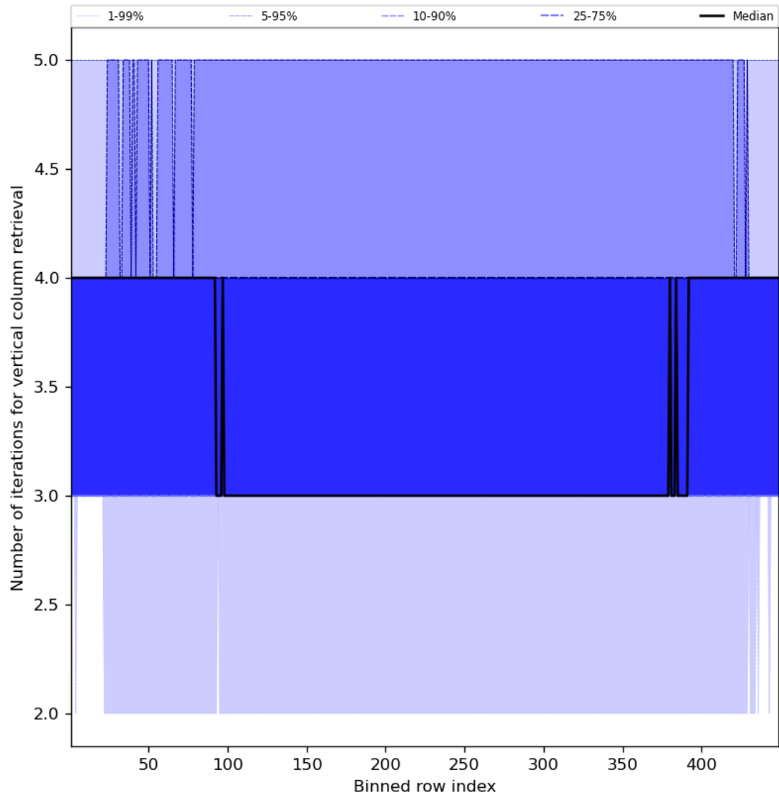
Figure 33: Along track statistics of “Number of iterations for vertical column retrieval” for 2023-08-23 to 2023-08-25
