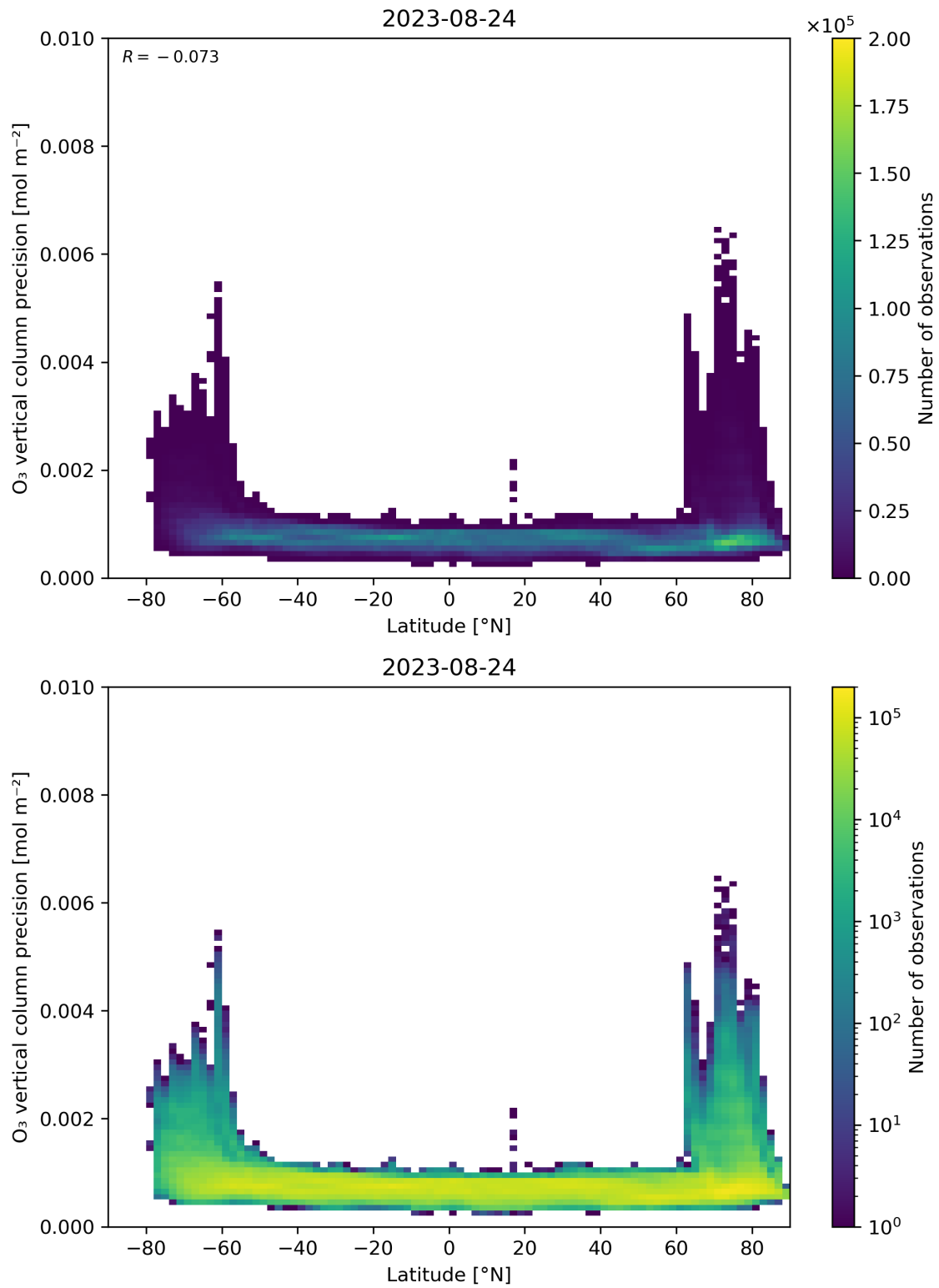
Figure 37: Scatter density plot of “Latitude” against “O 3 vertical column precision” for 2023-08-23 to 2023-08-25.
