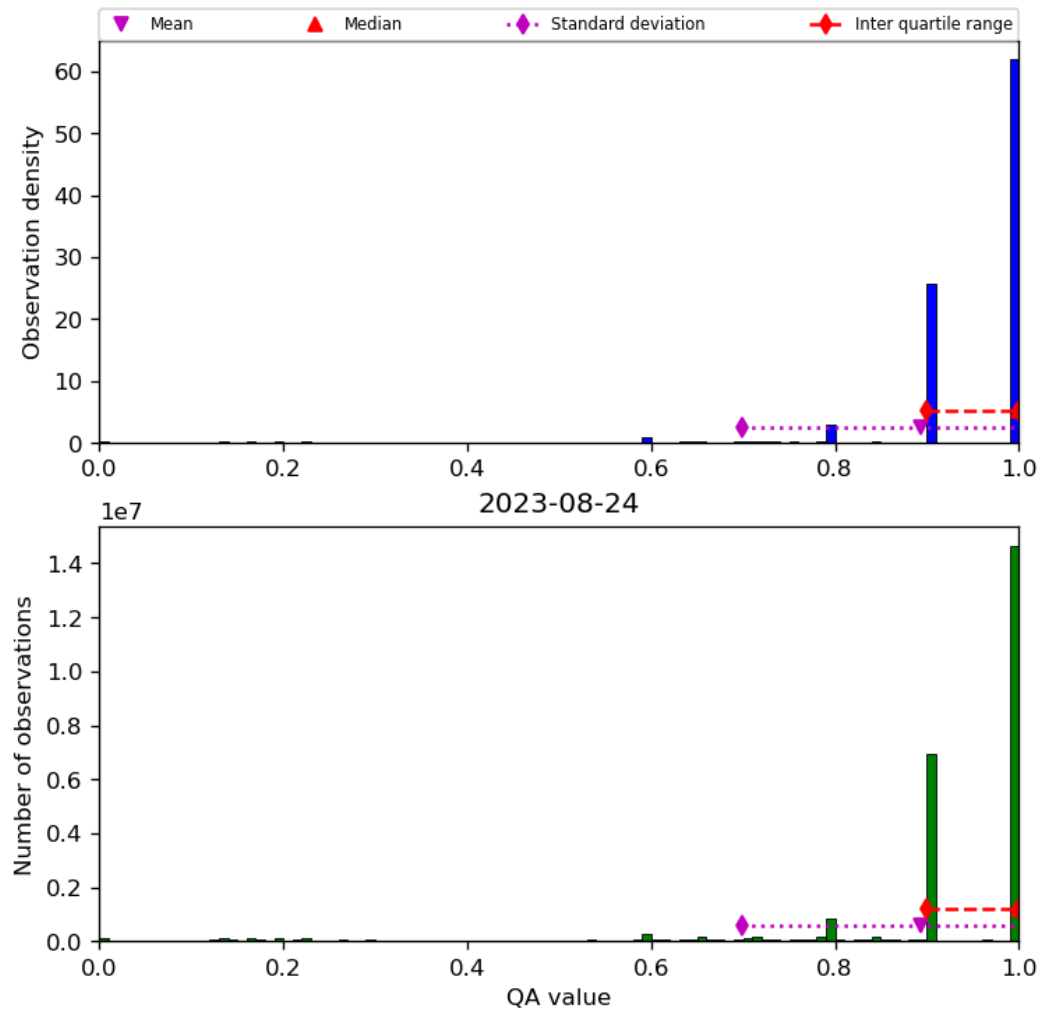
Figure 20: Histogram of “QA value” for 2023-08-23 to 2023-08-25
