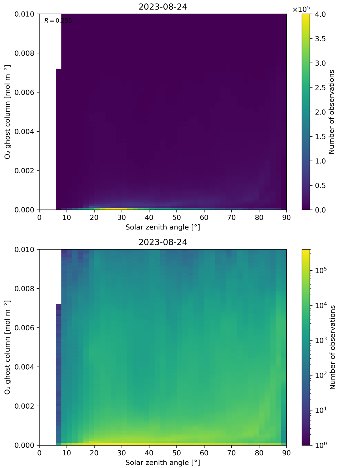
Figure 46: Scatter density plot of “Solar zenith angle” against “O 3 ghost column” for 2023-08-23 to 2023-08-25.
