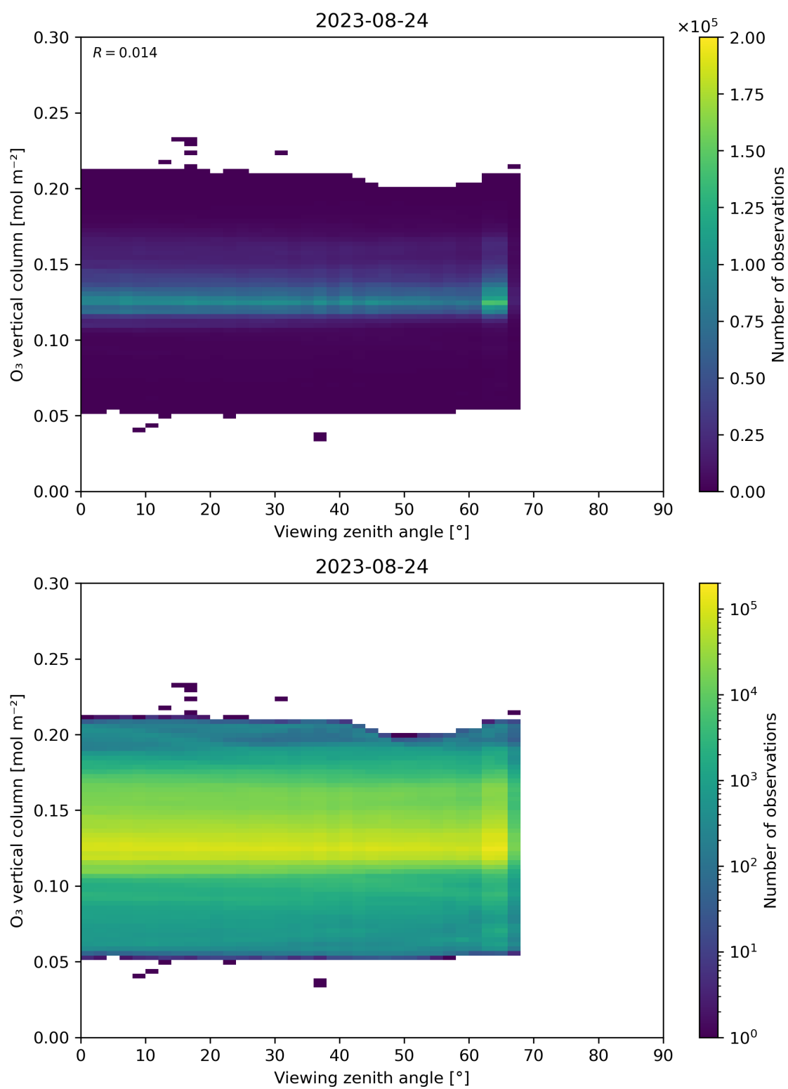
Figure 52: Scatter density plot of “Viewing zenith angle” against “O 3 vertical column” for 2023-08-23 to 2023-08-25.
