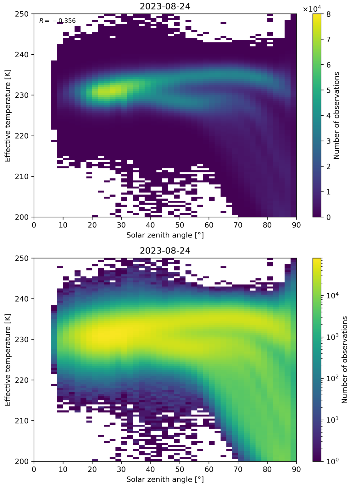
Figure 45: Scatter density plot of “Solar zenith angle” against “Effective temperature” for 2023-08-23 to 2023-08-25.
