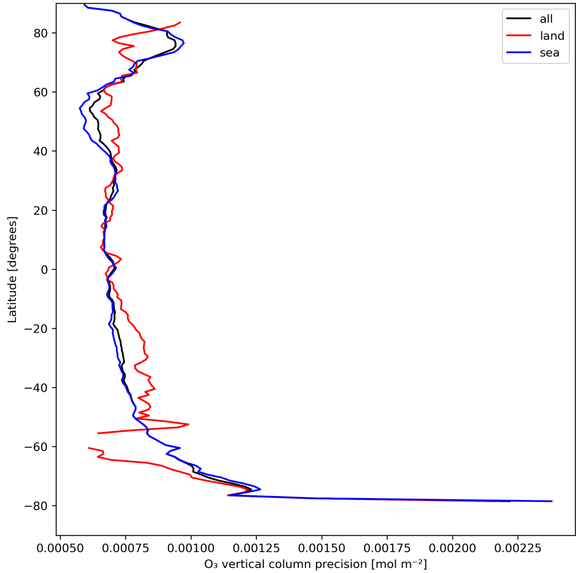
Figure 15: Zonal average of "O 3 vertical column precision" for 2023-08-23 to 2023-08-25.
