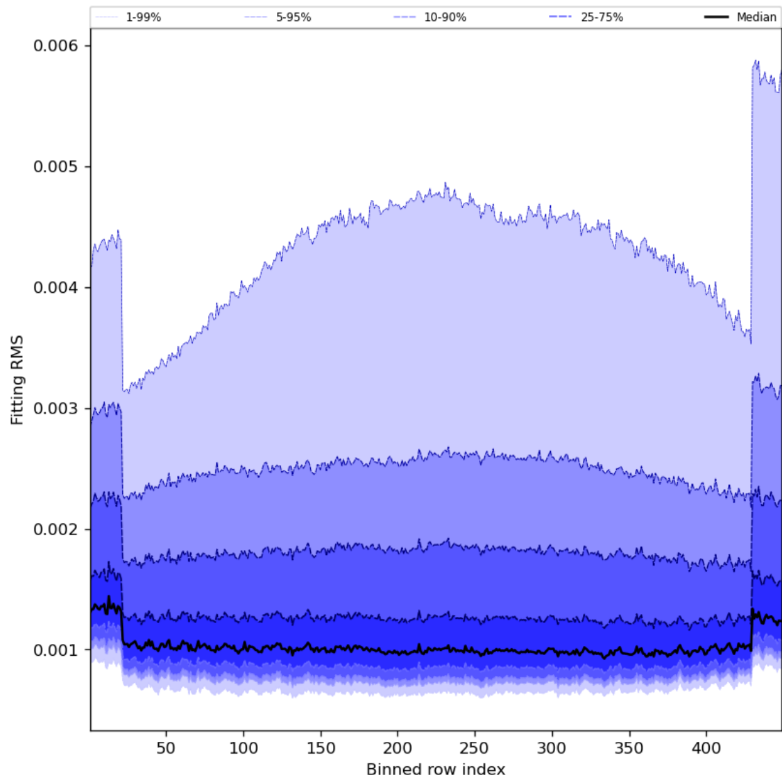
Figure 30: Along track statistics of “Fitting RMS” for 2023-08-23 to 2023-08-25
