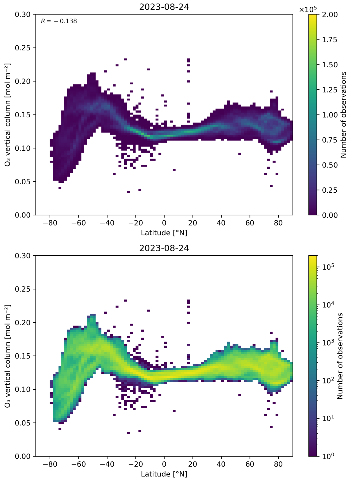
Figure 36: Scatter density plot of “Latitude” against “O 3 vertical column” for 2023-08-23 to 2023-08-25.
