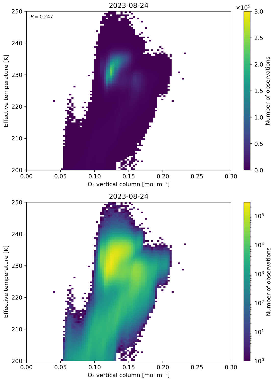
Figure 39: Scatter density plot of “O 3 vertical column” against “Effective temperature” for 2023-08-23 to 2023-08-25.
