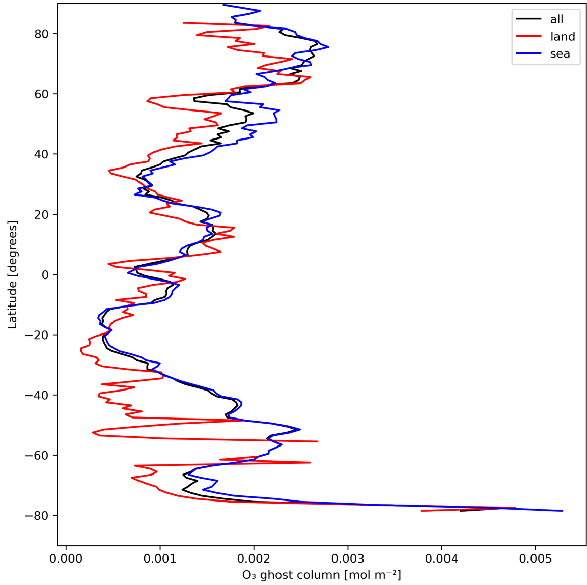
Figure 18: Zonal average of “O 3 ghost column” for 2023-08-23 to 2023-08-25.
