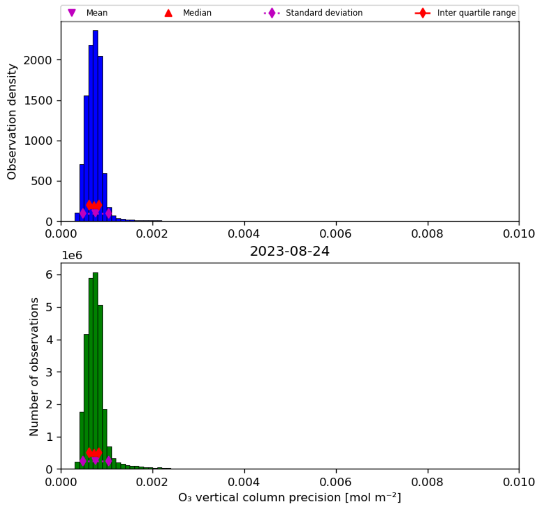
Figure 22: Histogram of “O 3 vertical column precision” for 2023-08-23 to 2023-08-25
