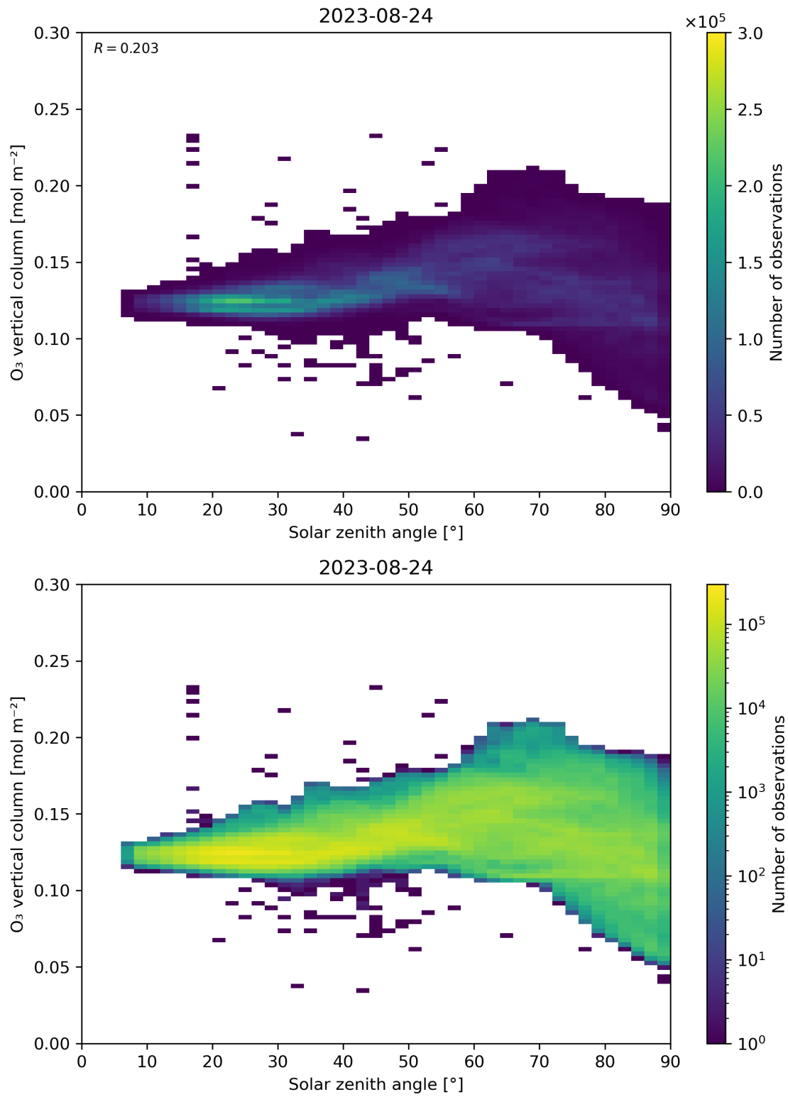
Figure 47: Scatter density plot of “Solar zenith angle” against “O 3 vertical column” for 2023-08-23 to 2023-08-25.
