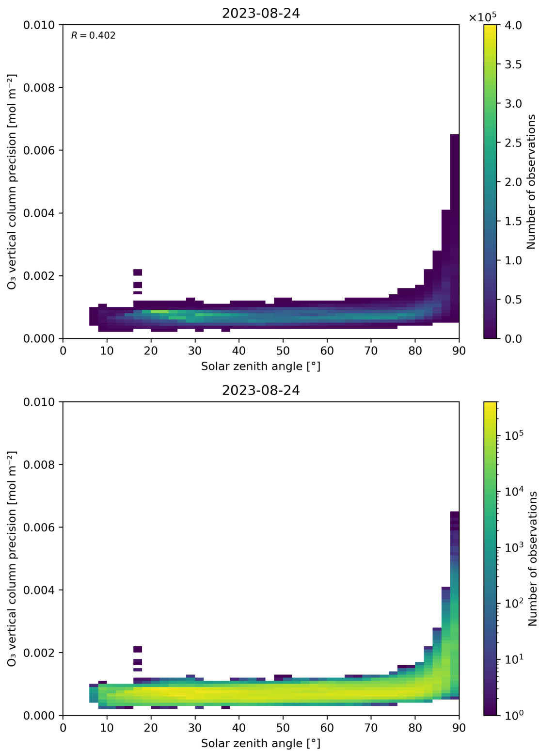
Figure 48: Scatter density plot of “Solar zenith angle” against “O 3 vertical column precision” for 2023-08-23 to 2023-08-25.
