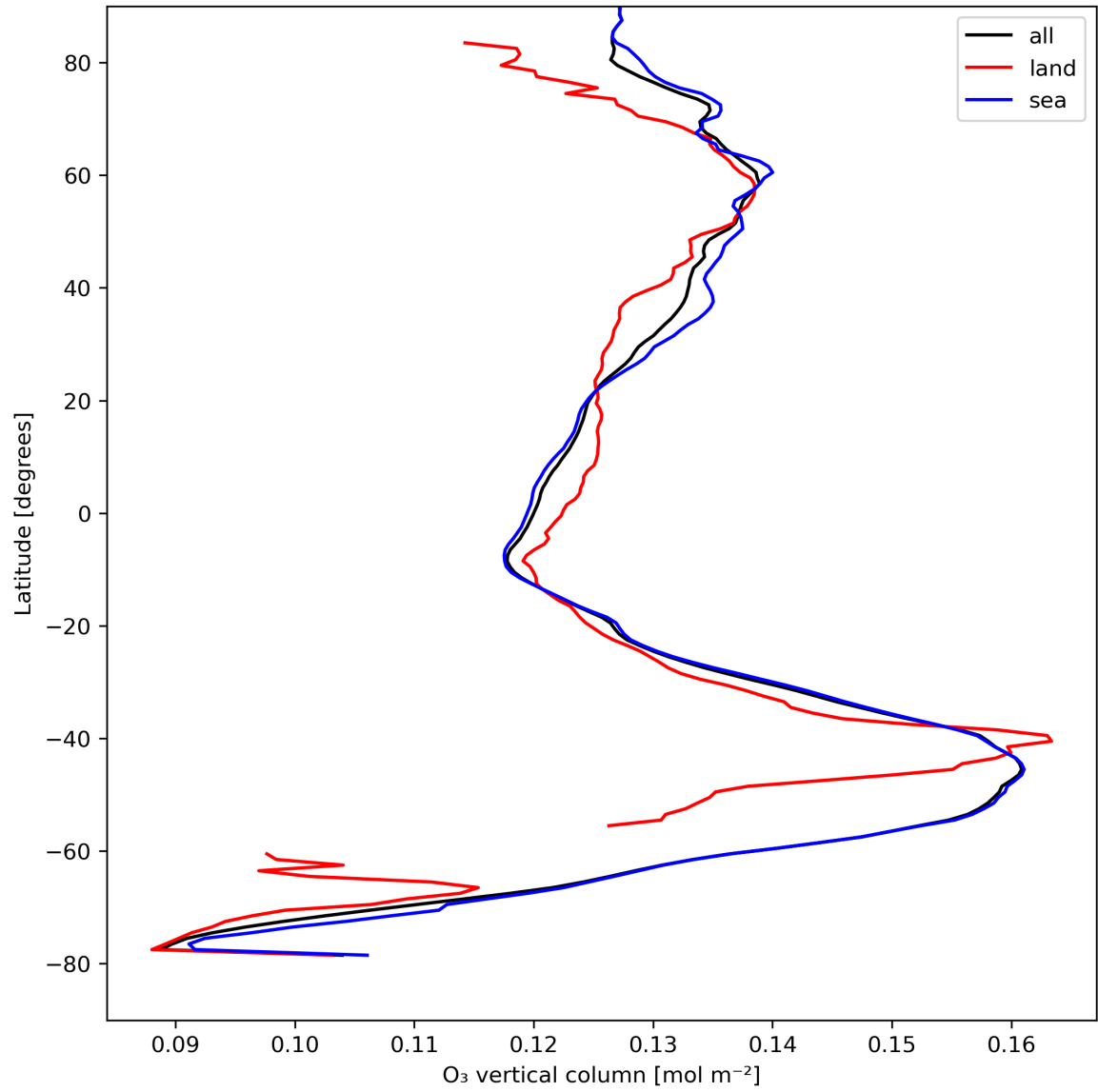
Figure 14: Zonal average of “O 3 vertical column” for 2023-08-23 to 2023-08-25.
