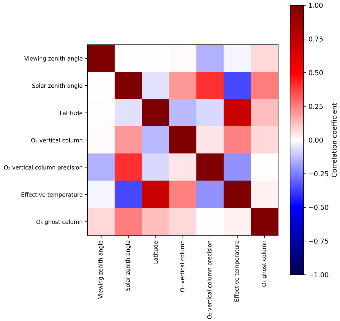
Figure 2: Map of correlation matrix for 2023-08-23 to 2023-08-25.
