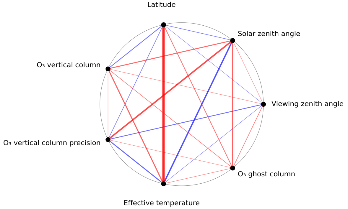
Figure 1: Map of correlation graph for 2023-08-23 to 2023-08-25.
