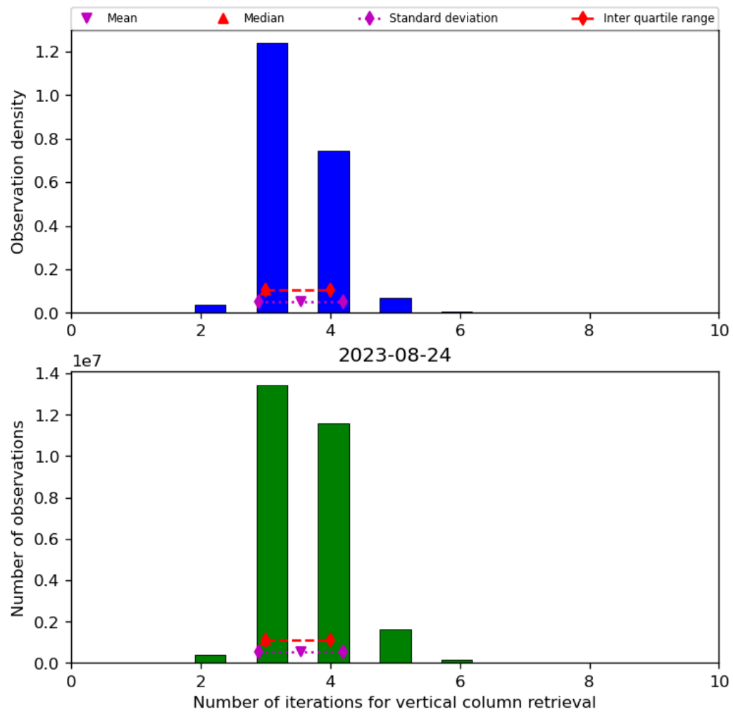
Figure 26: Histogram of “Number of iterations for vertical column retrieval” for 2023-08-23 to 2023-08-25
