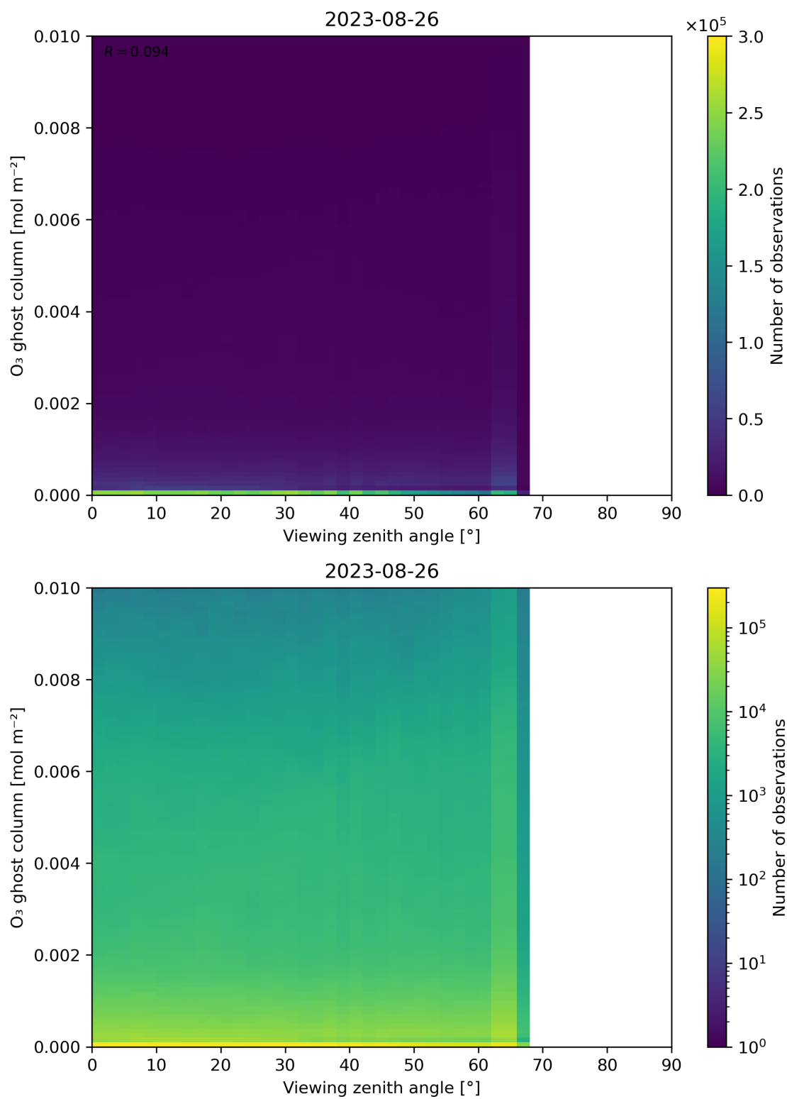
Figure 51: Scatter density plot of “Viewing zenith angle” against “O 3 ghost column” for 2023-08-25 to 2023-08-27.
