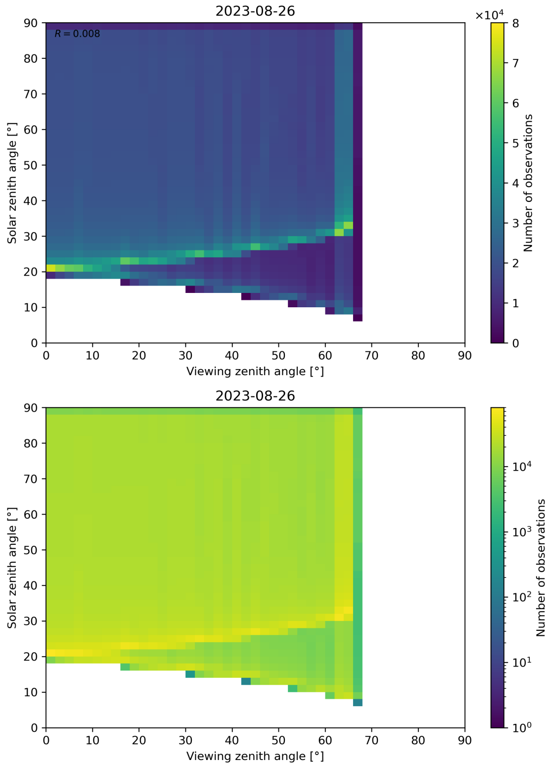
Figure 54: Scatter density plot of “Viewing zenith angle” against “Solar zenith angle” for 2023-08-25 to 2023-08-27.
