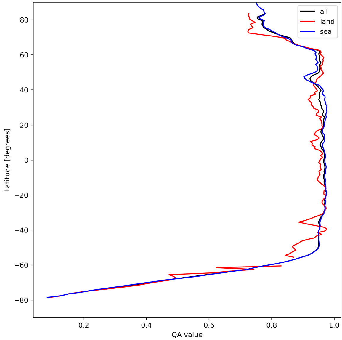
Figure 13: Zonal average of “QA value” for 2023-08-25 to 2023-08-27.
