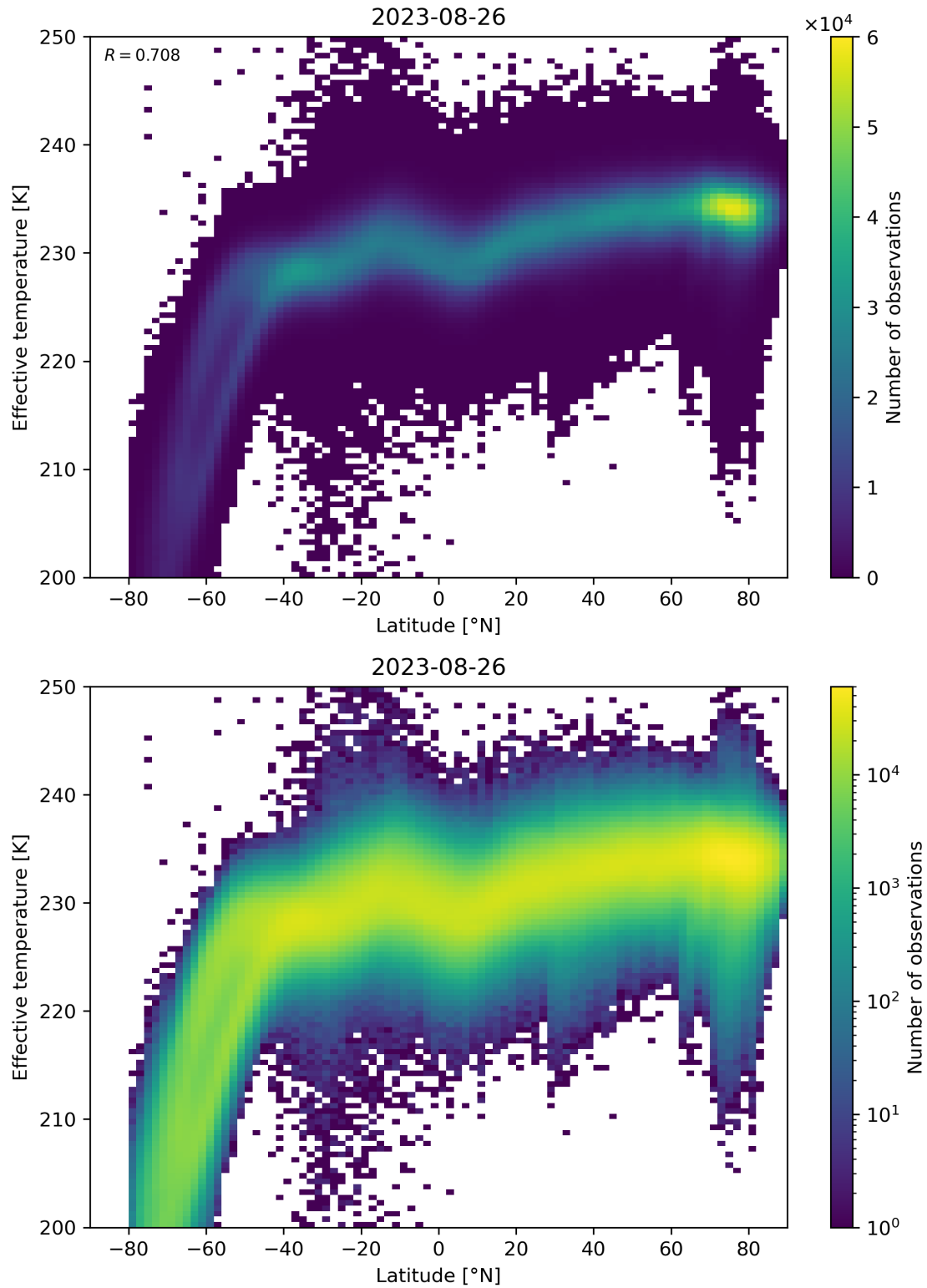
Figure 34: Scatter density plot of “Latitude” against “Effective temperature” for 2023-08-25 to 2023-08-27.
