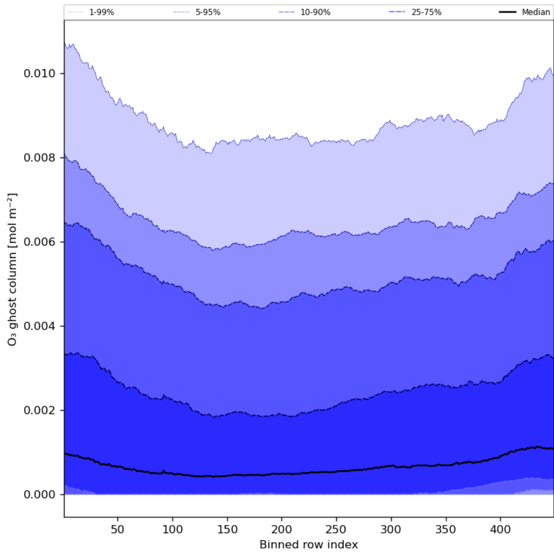
Figure 32: Along track statistics of “O 3 ghost column” for 2023-08-25 to 2023-08-27
