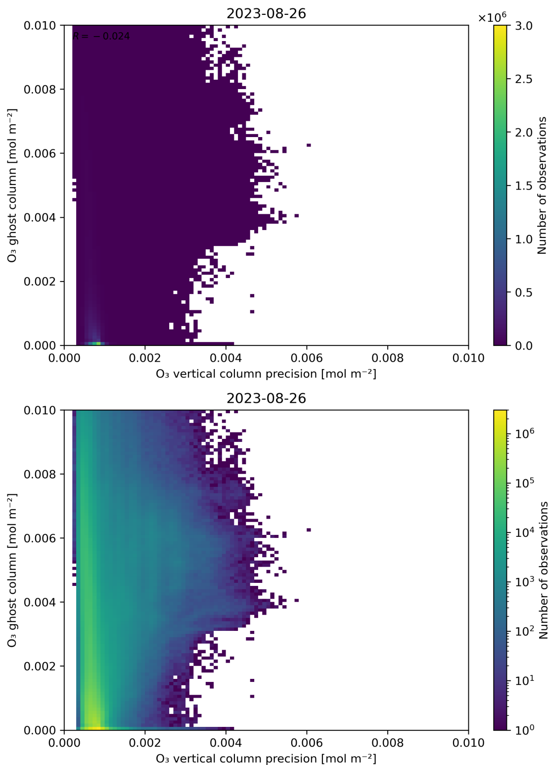
Figure 43: Scatter density plot of “ \text{O}_3 vertical column precision” against “ \text{O}_3 ghost column” for 2023-08-25 to 2023-08-27.
