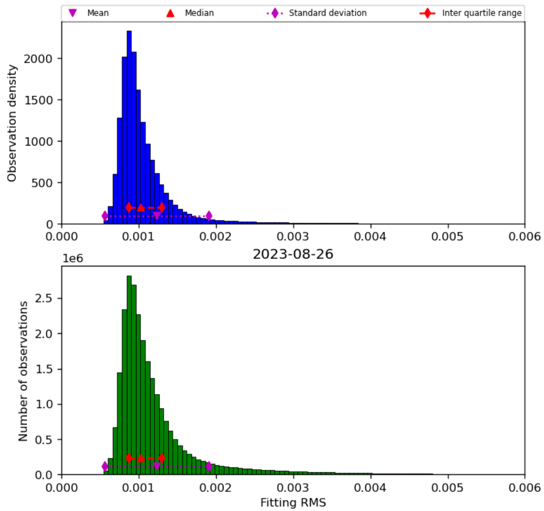
Figure 23: Histogram of “Fitting RMS” for 2023-08-25 to 2023-08-27
