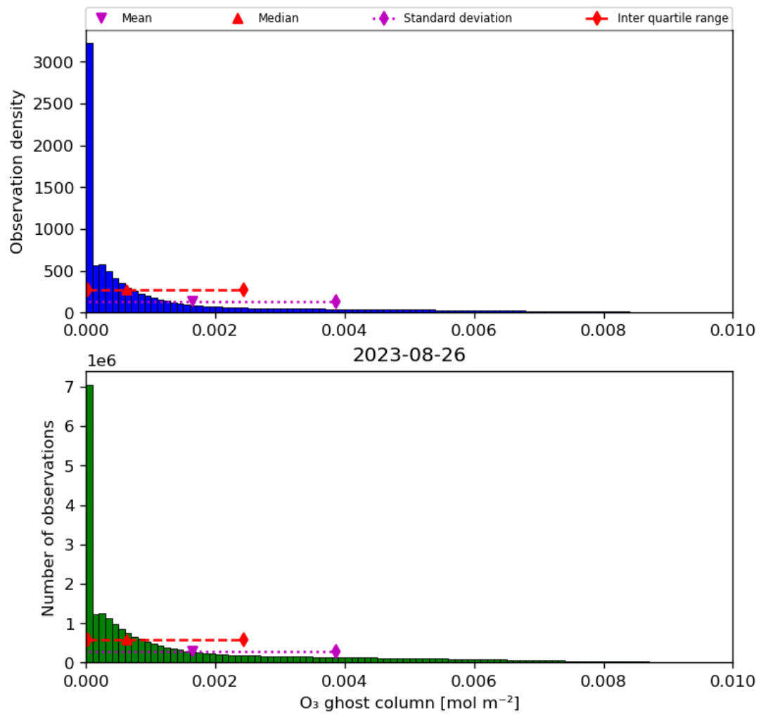
Figure 25: Histogram of “O 3 ghost column” for 2023-08-25 to 2023-08-27
