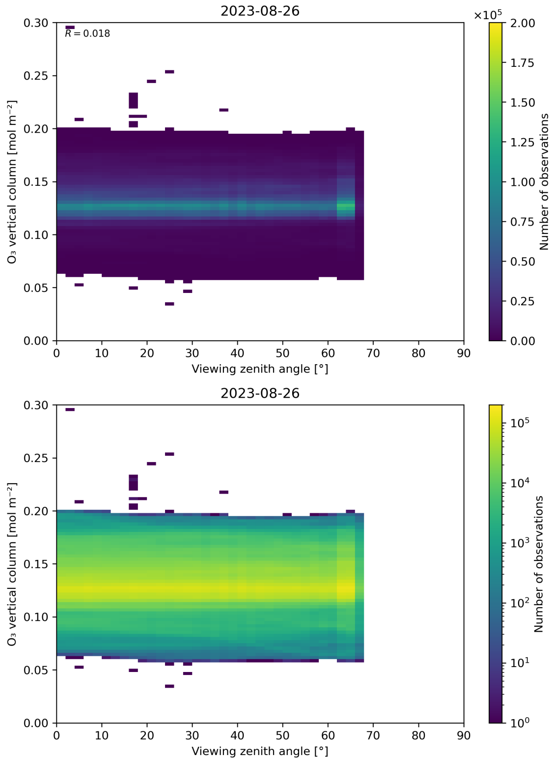
Figure 52: Scatter density plot of “Viewing zenith angle” against “O 3 vertical column” for 2023-08-25 to 2023-08-27.
