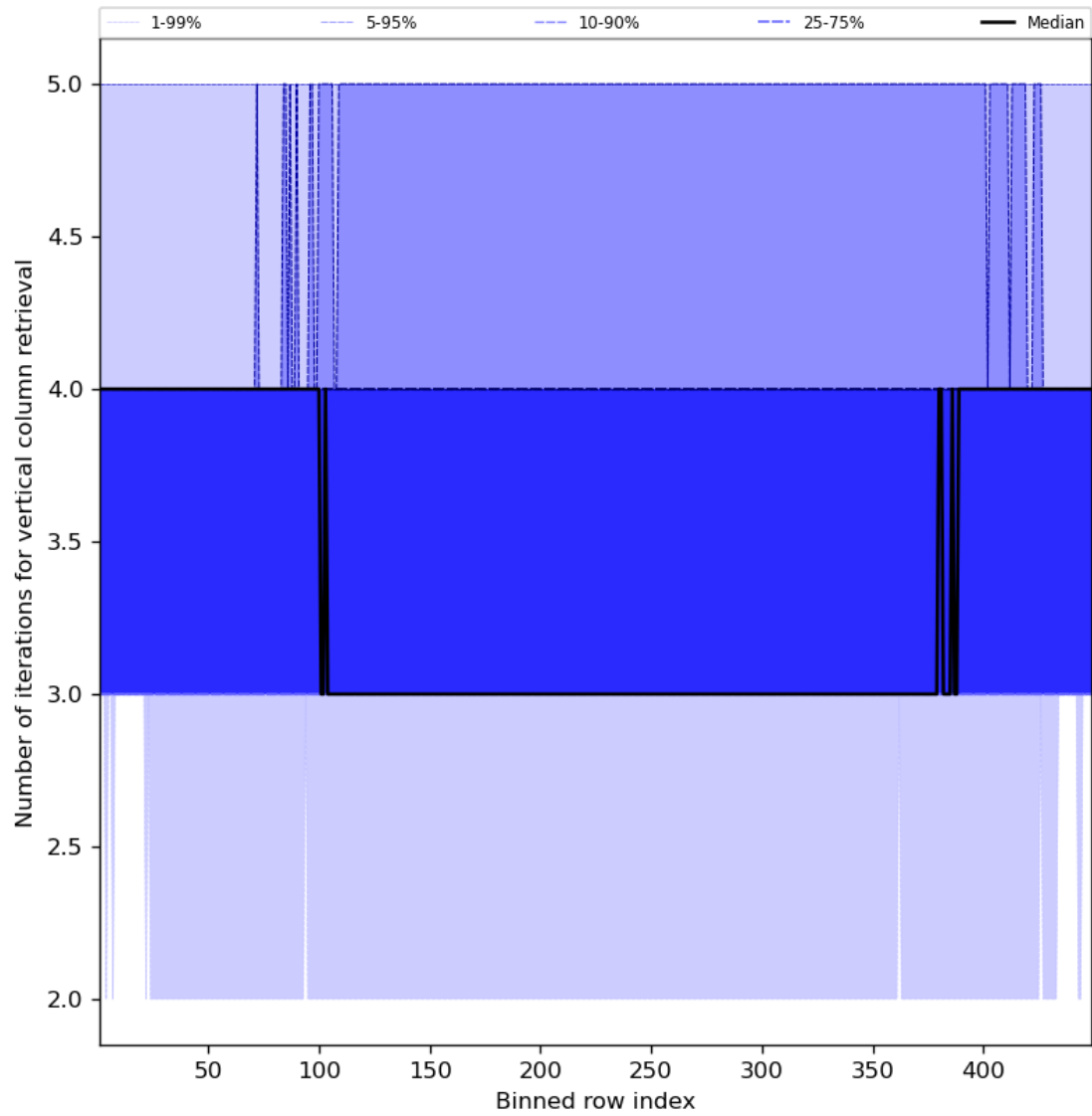
Figure 33: Along track statistics of “Number of iterations for vertical column retrieval” for 2023-08-25 to 2023-08-27
