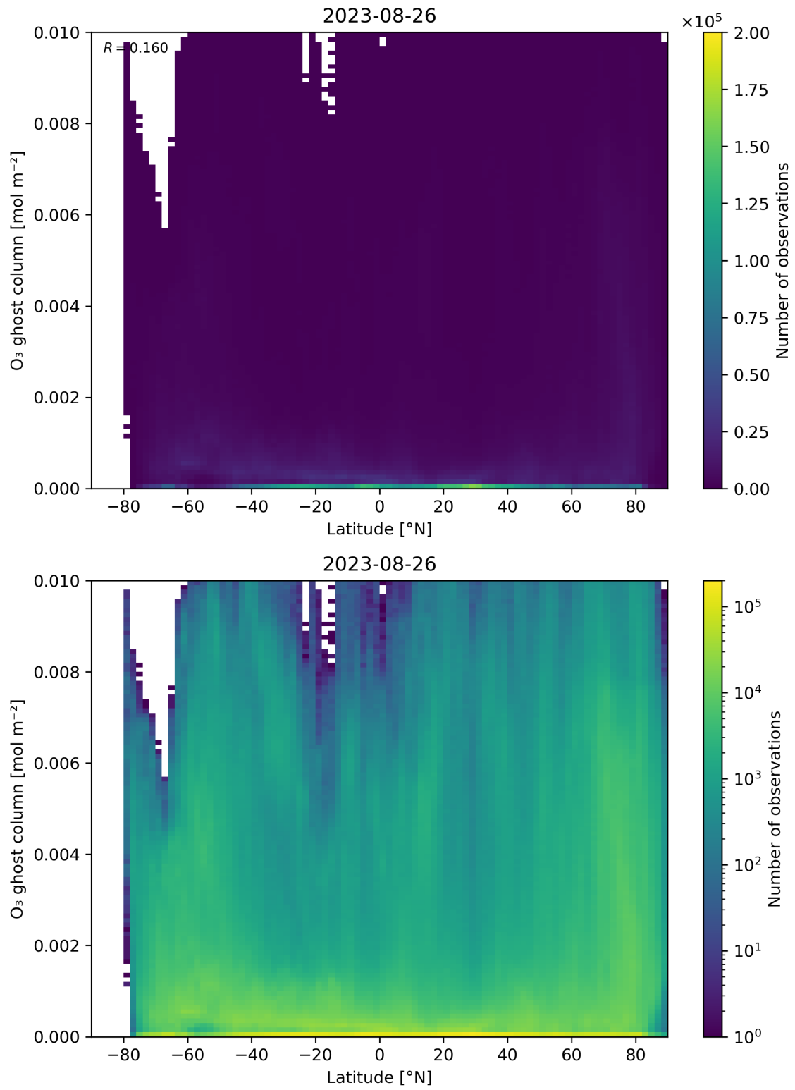
Figure 35: Scatter density plot of “Latitude” against “O 3 ghost column” for 2023-08-25 to 2023-08-27.
