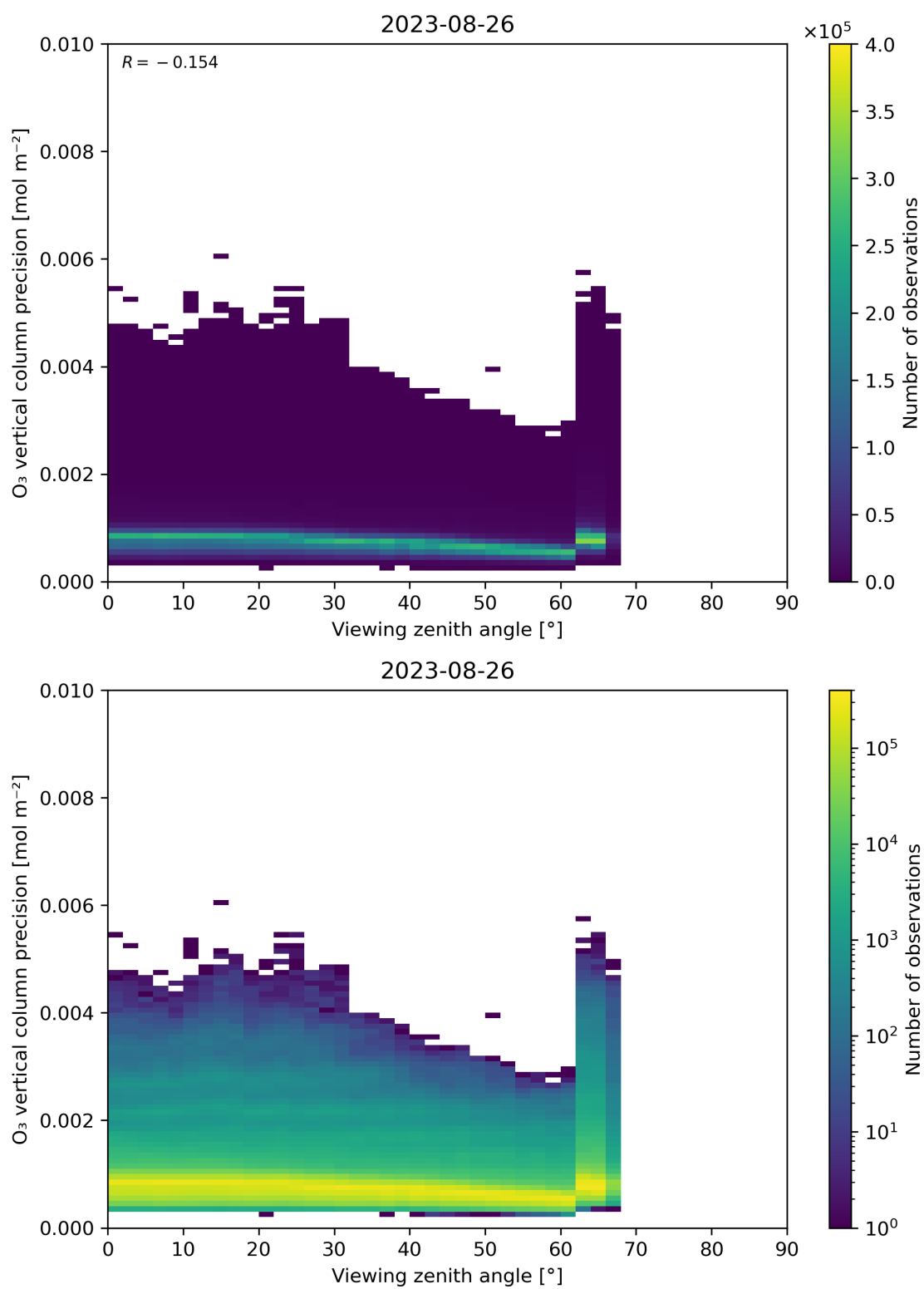
Figure 53: Scatter density plot of “Viewing zenith angle” against “O 3 vertical column precision” for 2023-08-25 to 2023-08-27.
