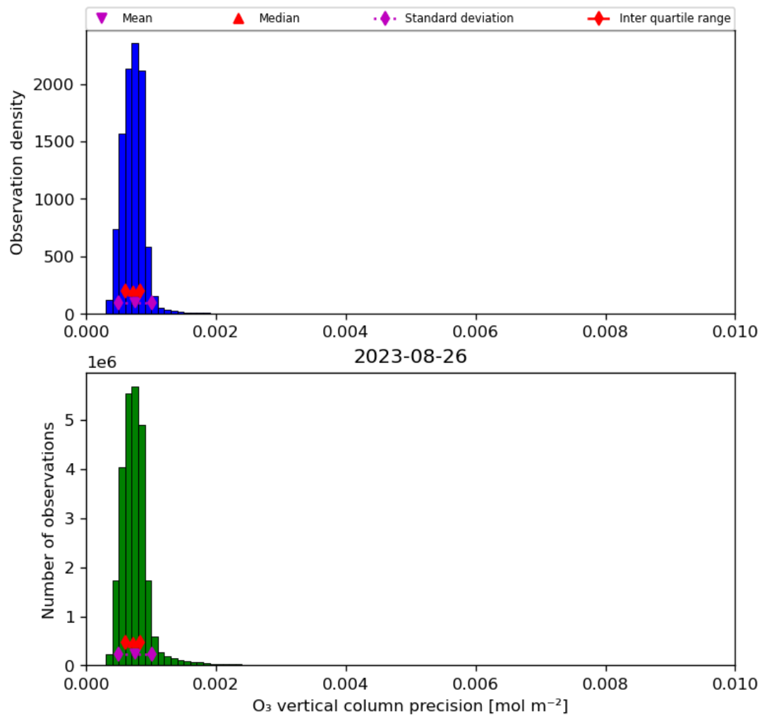
Figure 22: Histogram of “O 3 vertical column precision” for 2023-08-25 to 2023-08-27
