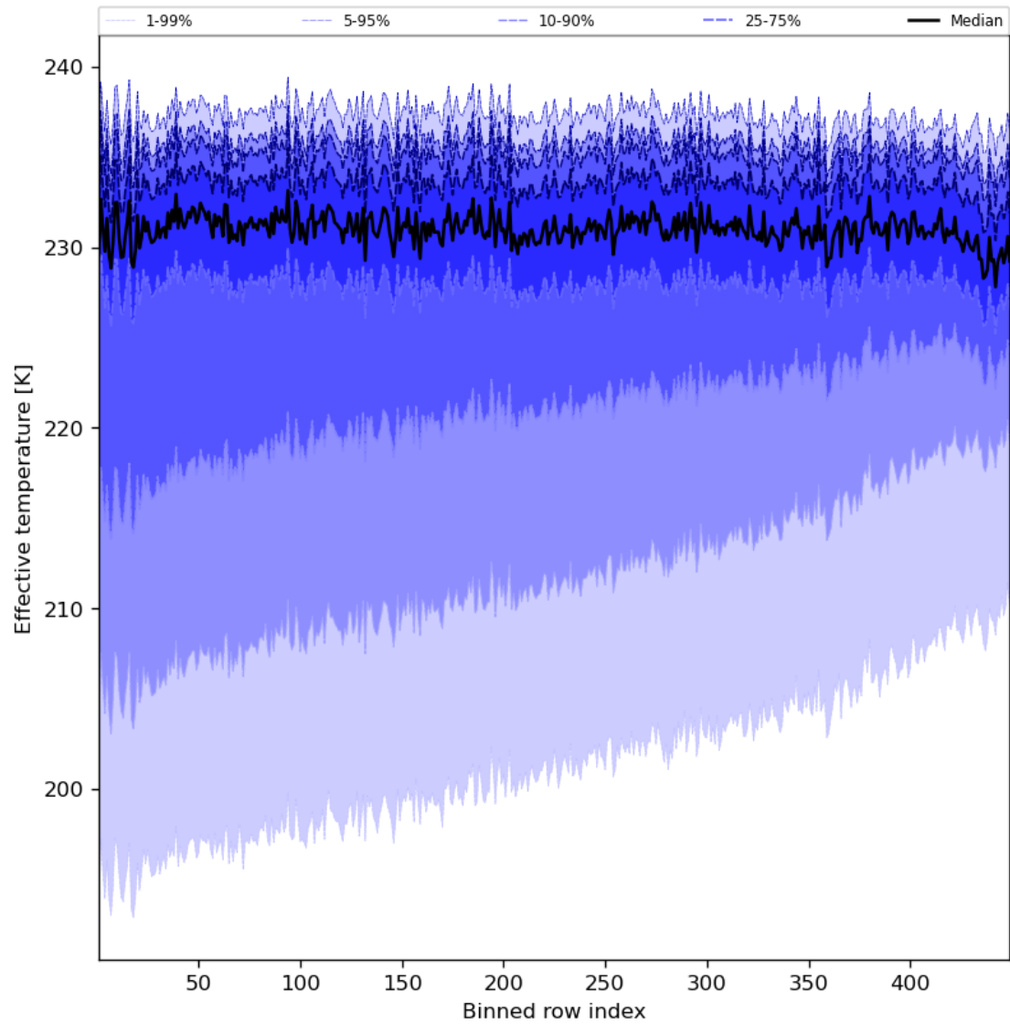
Figure 31: Along track statistics of “Effective temperature” for 2023-08-25 to 2023-08-27
