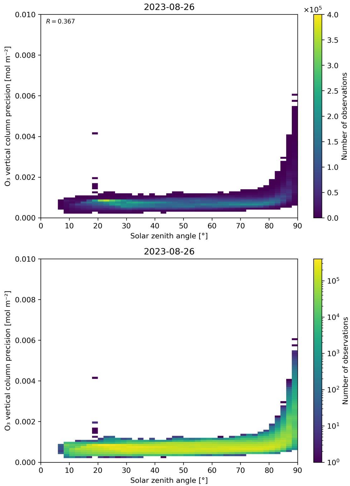
Figure 48: Scatter density plot of “Solar zenith angle” against “O 3 vertical column precision” for 2023-08-25 to 2023-08-27.
