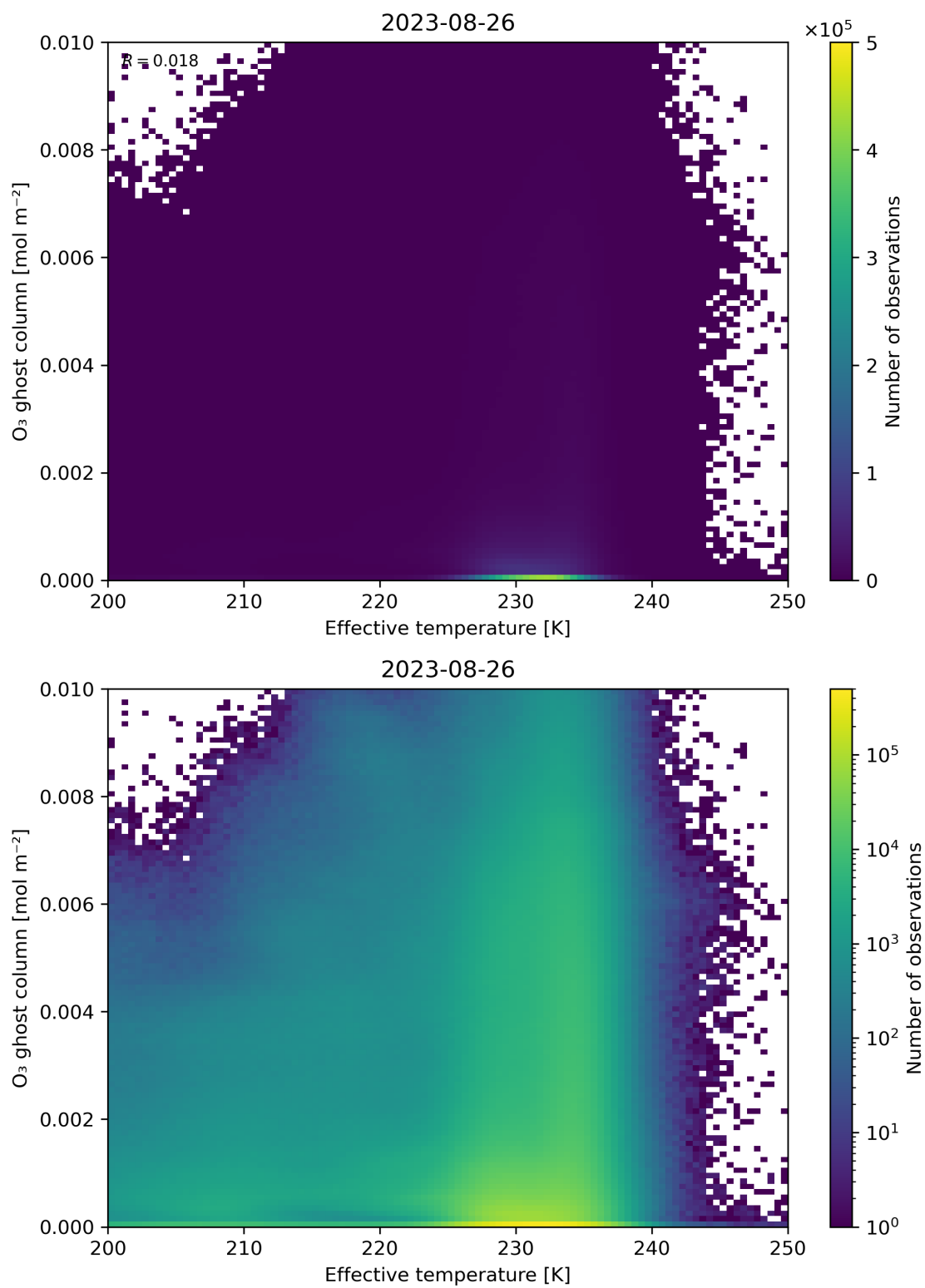
Figure 38: Scatter density plot of “Effective temperature” against “O 3 ghost column” for 2023-08-25 to 2023-08-27.
