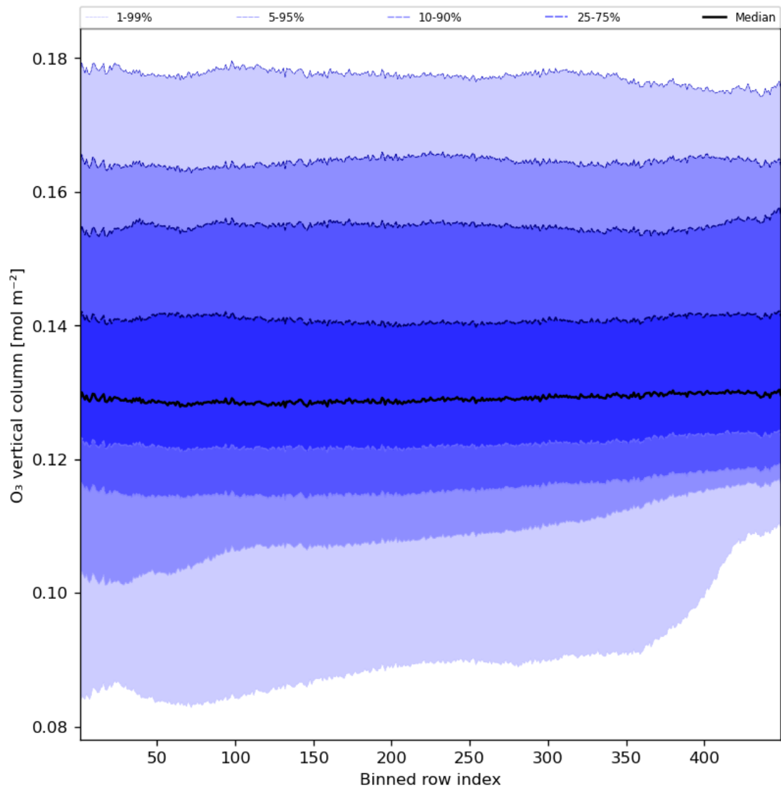
Figure 28: Along track statistics of “O 3 vertical column” for 2023-08-25 to 2023-08-27
