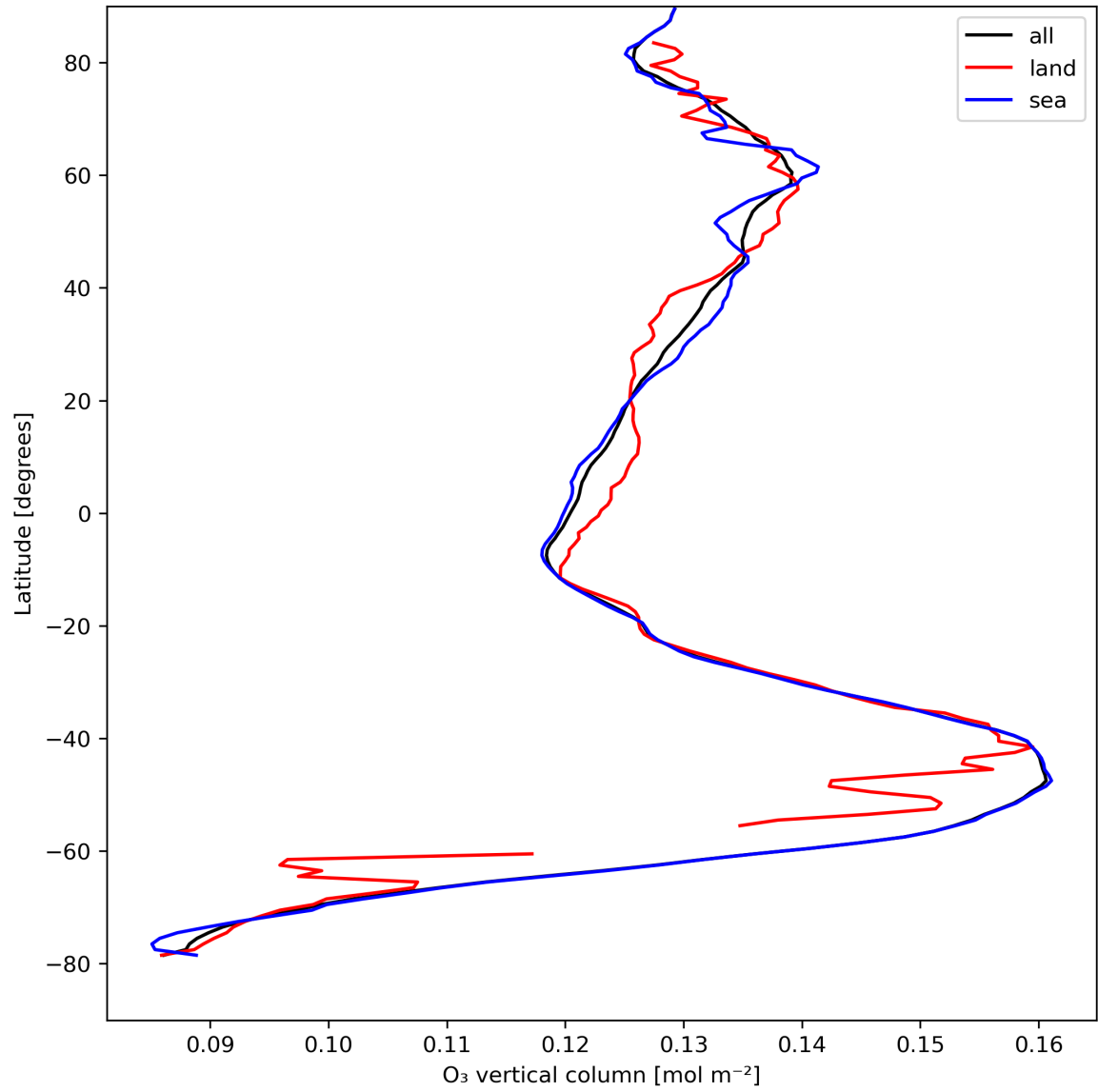
Figure 14: Zonal average of “O 3 vertical column” for 2023-08-25 to 2023-08-27.
