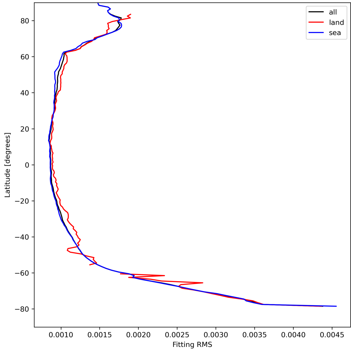
Figure 16: Zonal average of “Fitting RMS” for 2023-08-25 to 2023-08-27.
