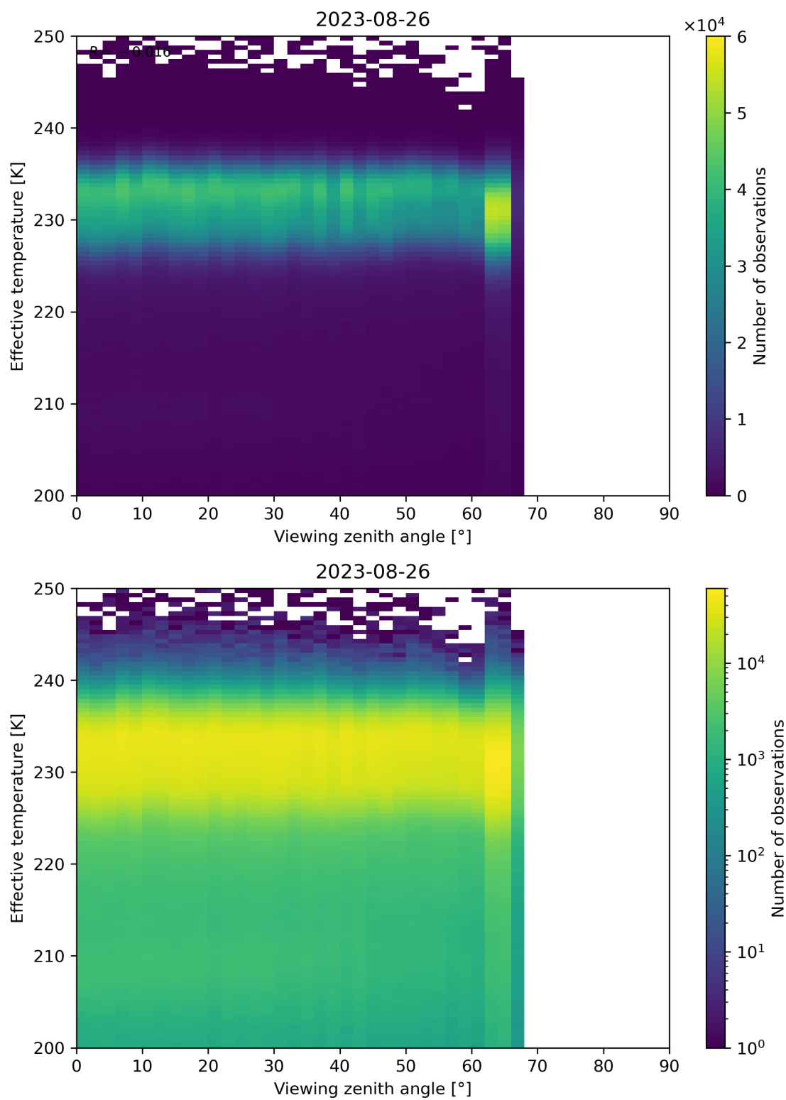
Figure 50: Scatter density plot of “Viewing zenith angle” against “Effective temperature” for 2023-08-25 to 2023-08-27.
