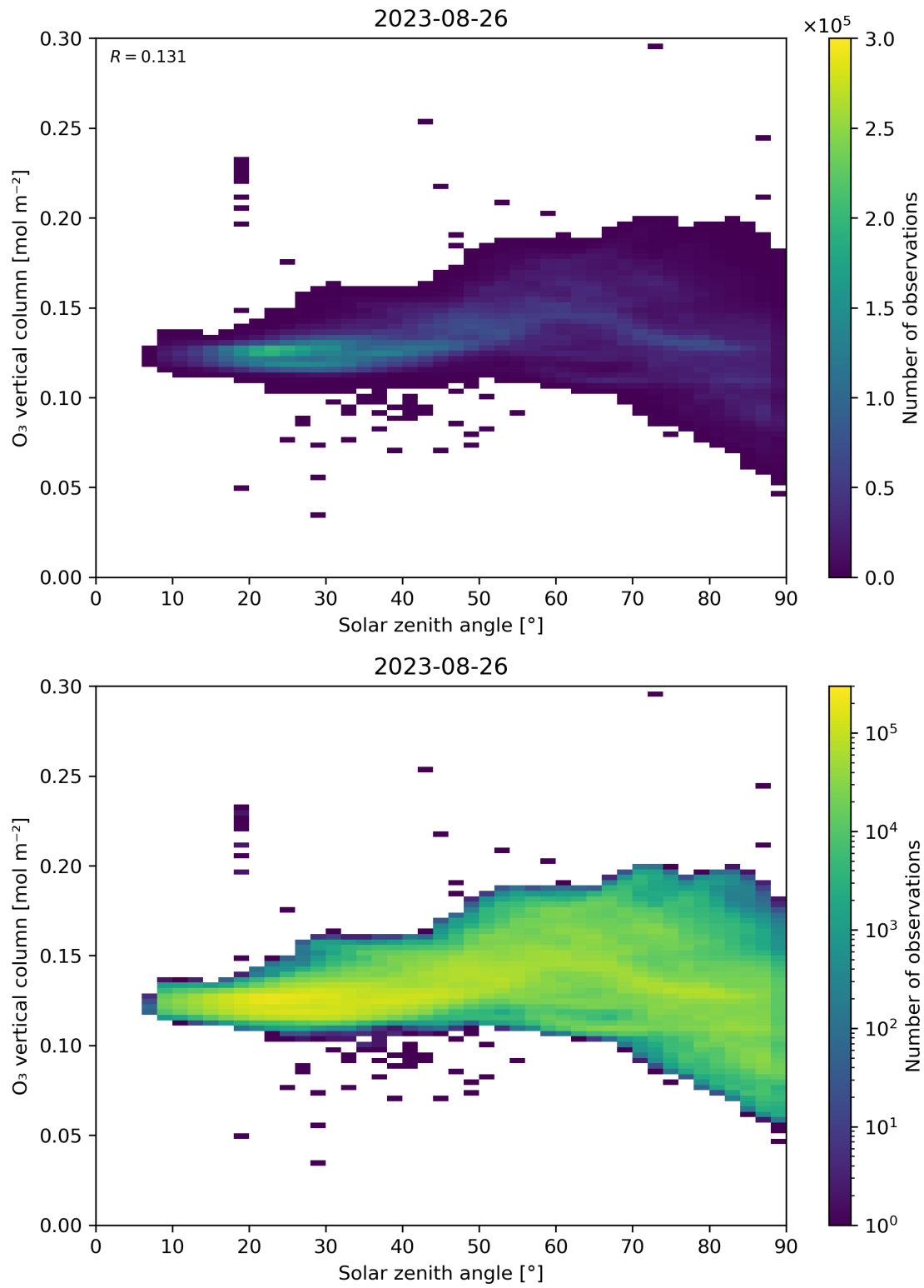
Figure 47: Scatter density plot of “Solar zenith angle” against “O 3 vertical column” for 2023-08-25 to 2023-08-27.
