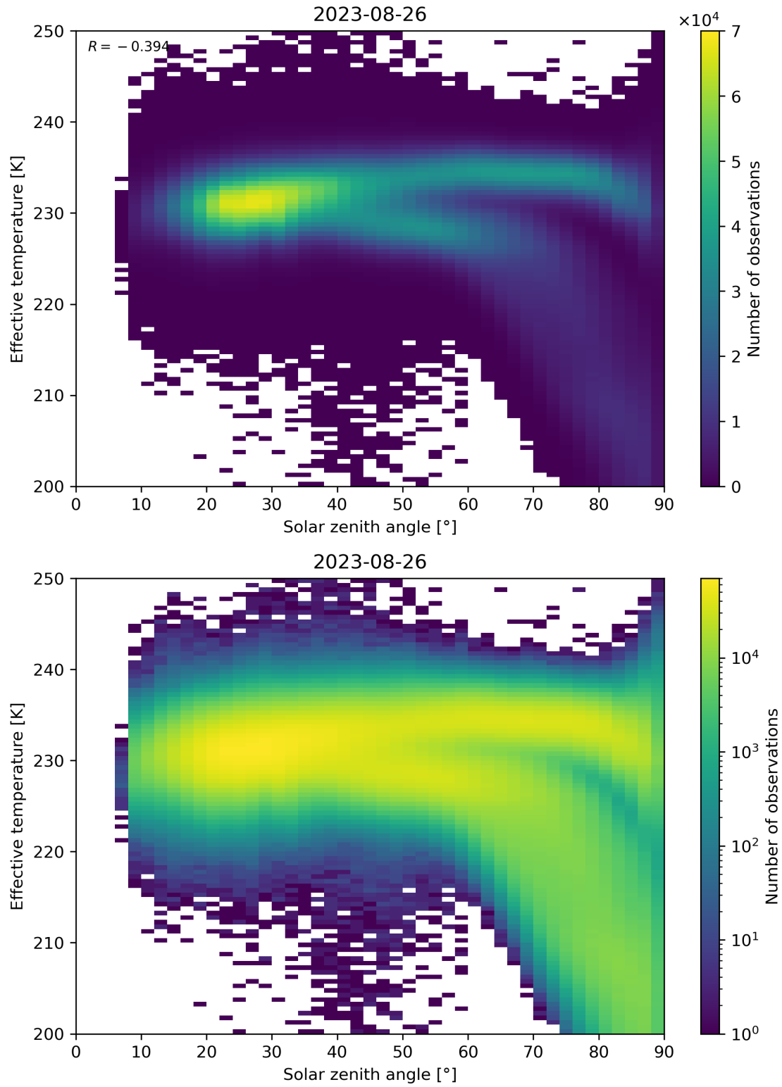
Figure 45: Scatter density plot of “Solar zenith angle” against “Effective temperature” for 2023-08-25 to 2023-08-27.
