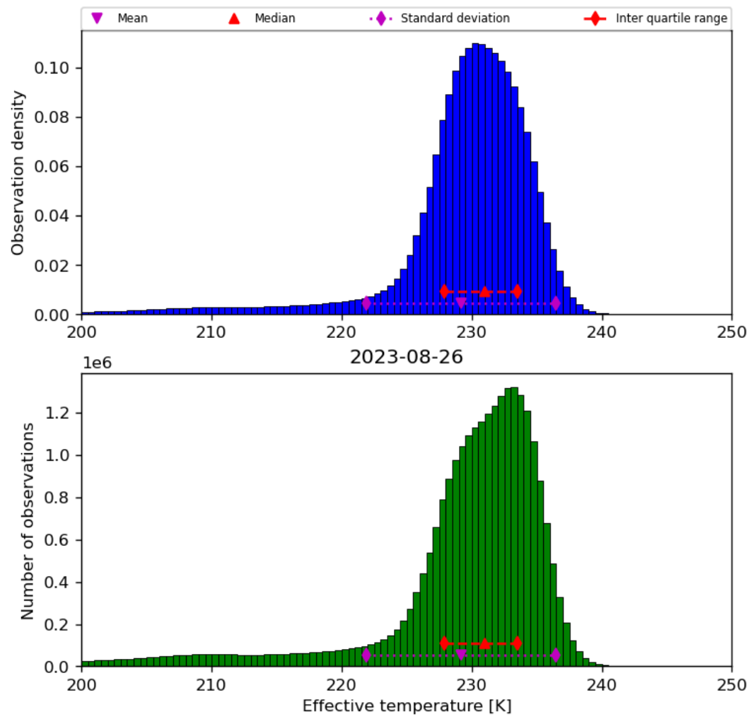
Figure 24: Histogram of “Effective temperature” for 2023-08-25 to 2023-08-27
