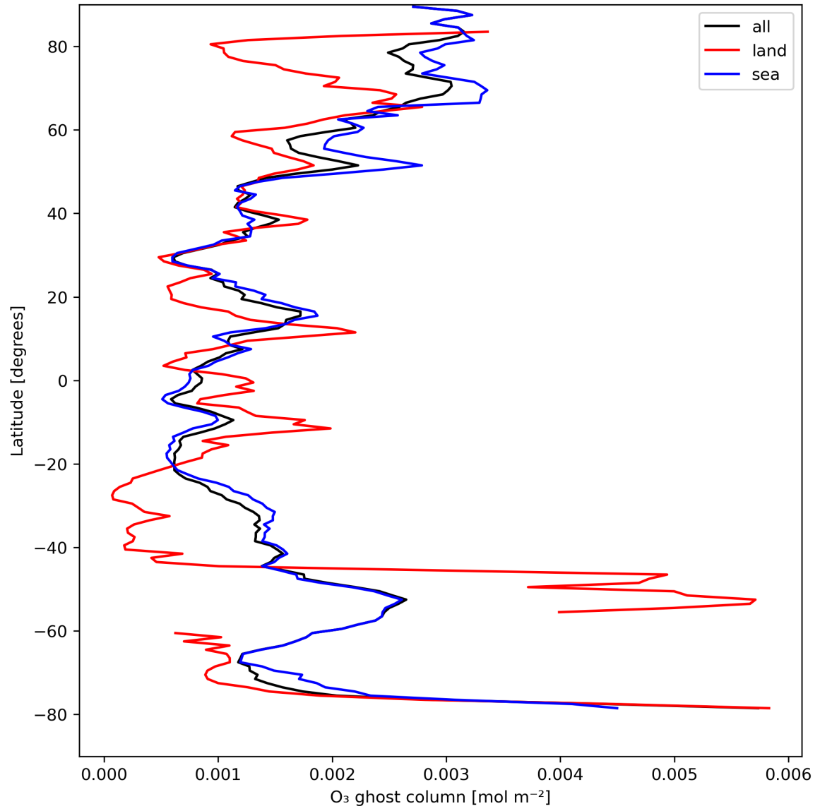
Figure 18: Zonal average of "O 3 ghost column" for 2023-08-25 to 2023-08-27.
