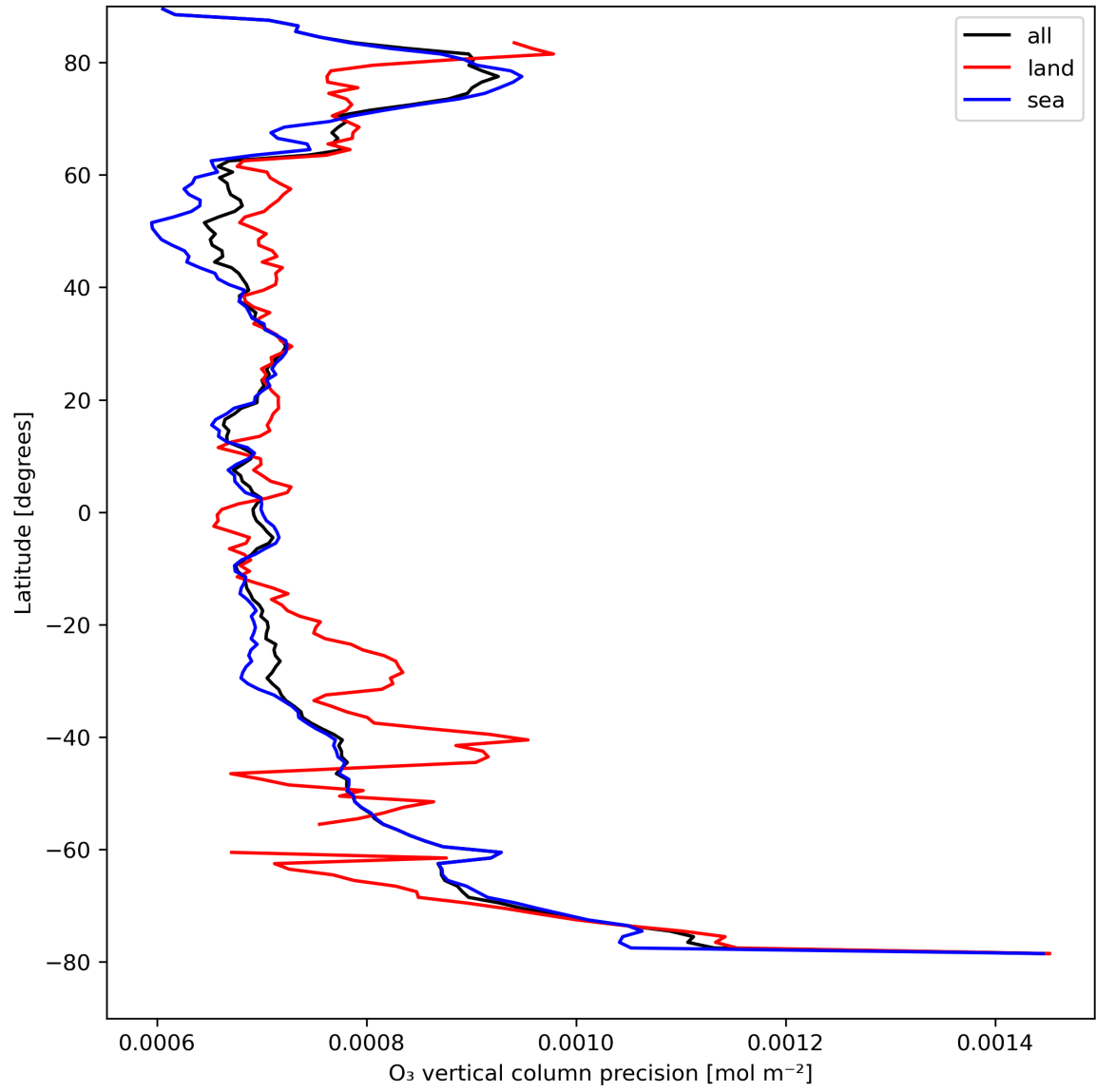
Figure 15: Zonal average of "O 3 vertical column precision" for 2023-08-25 to 2023-08-27.
