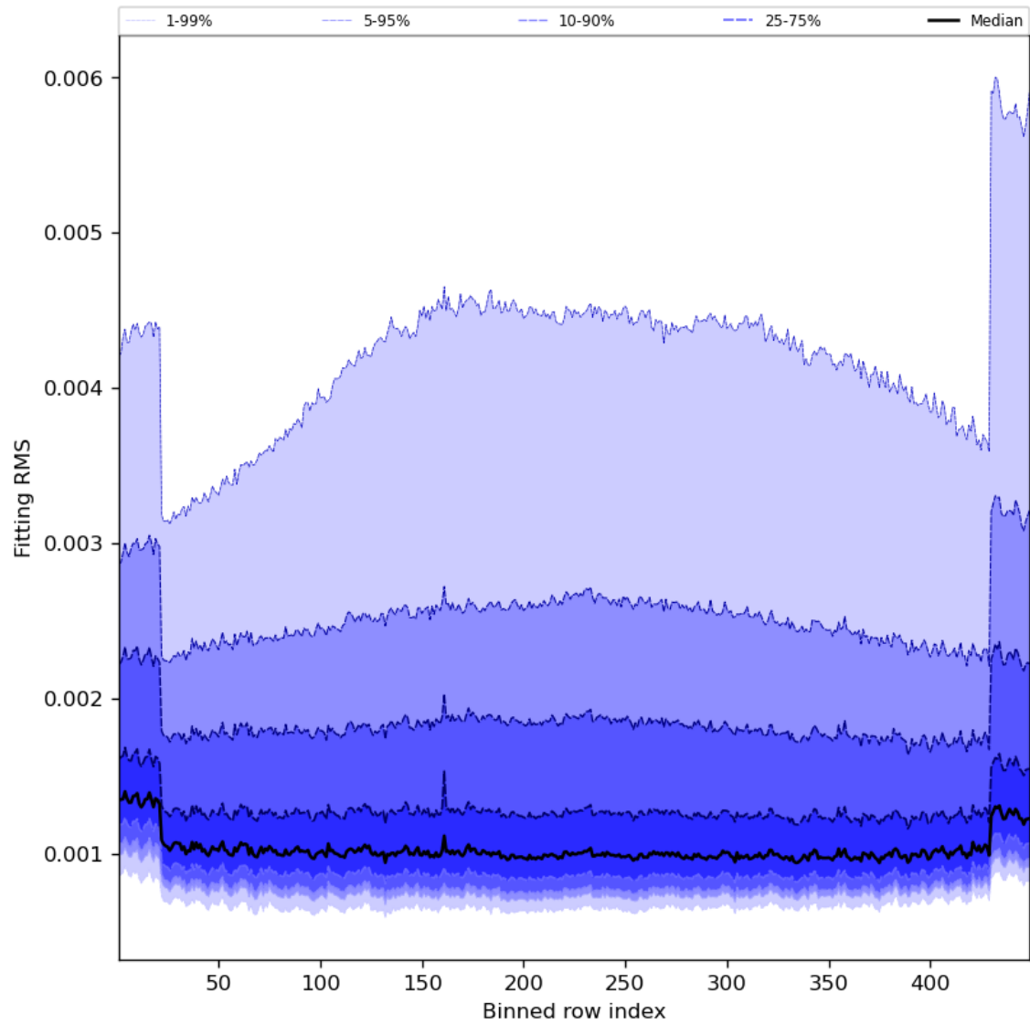
Figure 30: Along track statistics of “Fitting RMS” for 2023-08-25 to 2023-08-27
