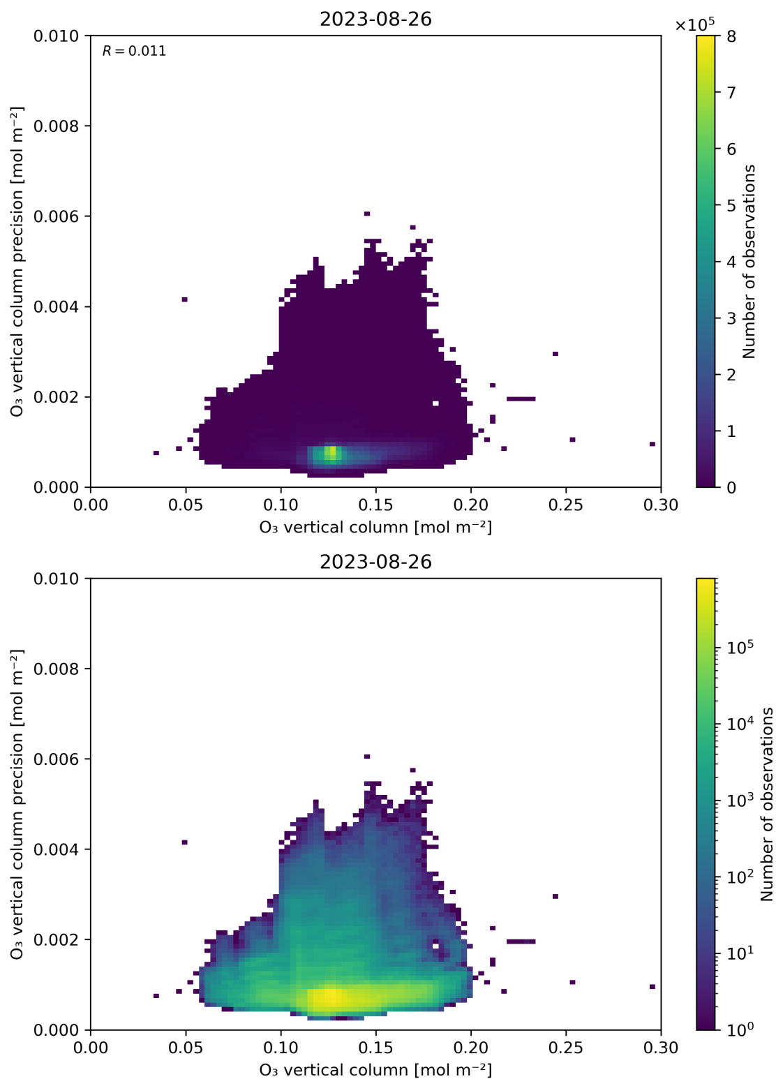
Figure 41: Scatter density plot of “O 3 vertical column” against “O 3 vertical column precision” for 2023-08-25 to 2023-08-27.
