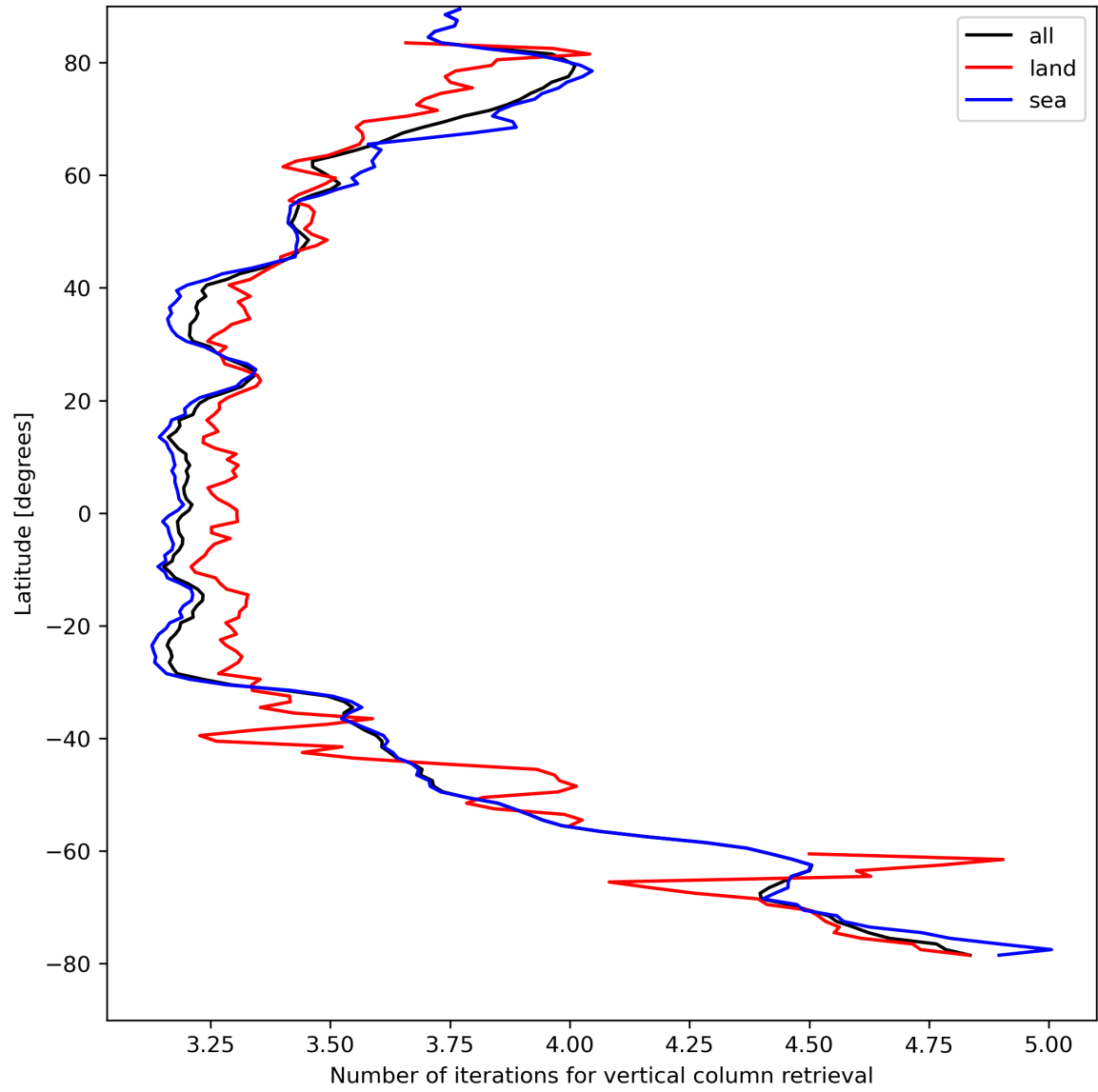
Figure 19: Zonal average of “Number of iterations for vertical column retrieval” for 2023-08-25 to 2023-08-27.
