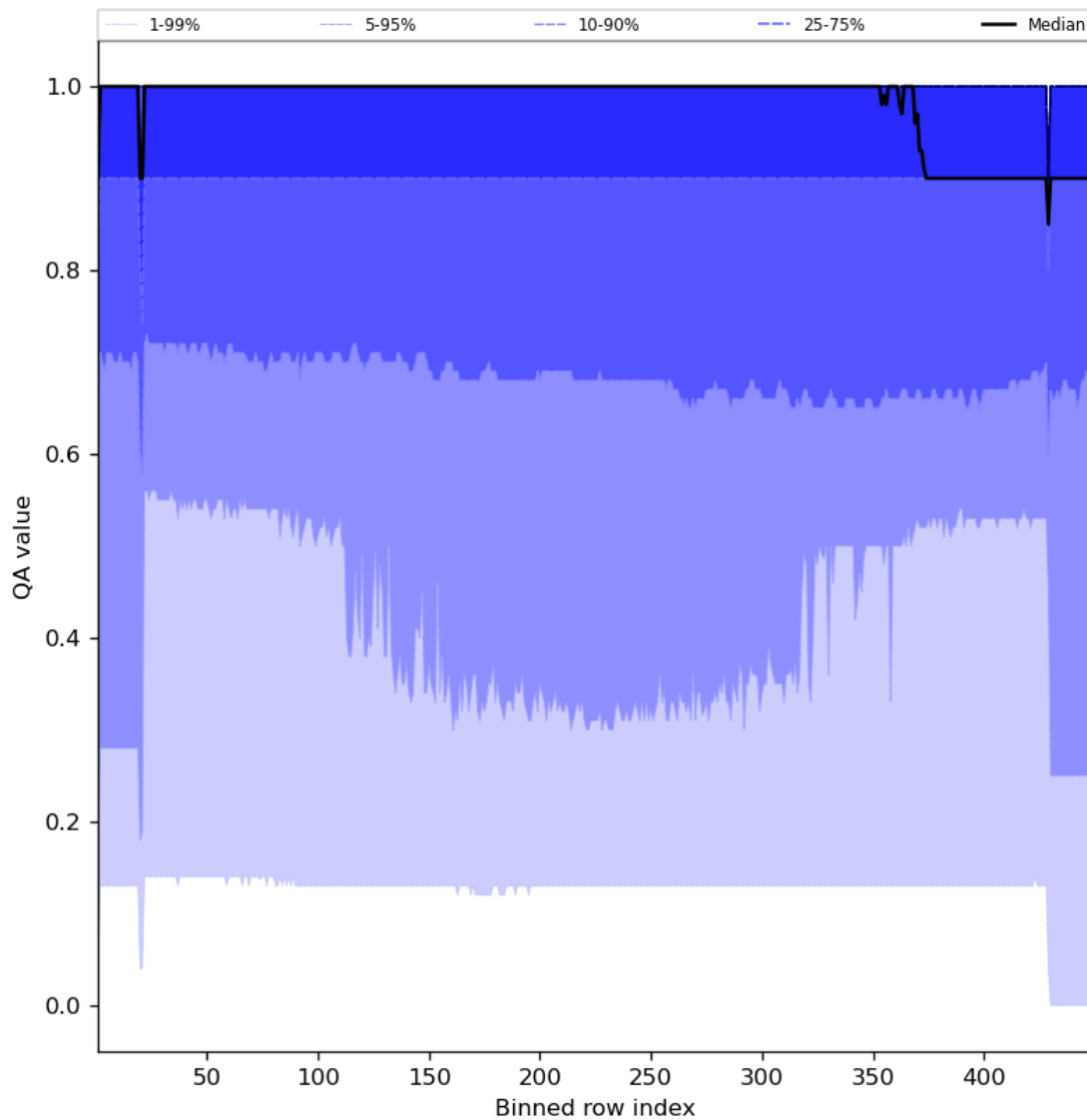
Figure 27: Along track statistics of “QA value” for 2023-08-25 to 2023-08-27
