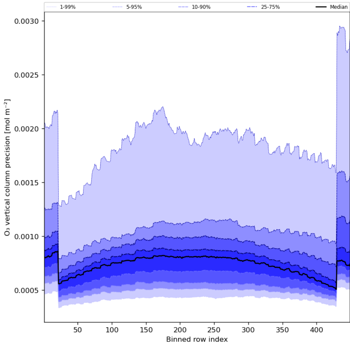
Figure 29: Along track statistics of “O 3 vertical column precision” for 2023-08-25 to 2023-08-27
