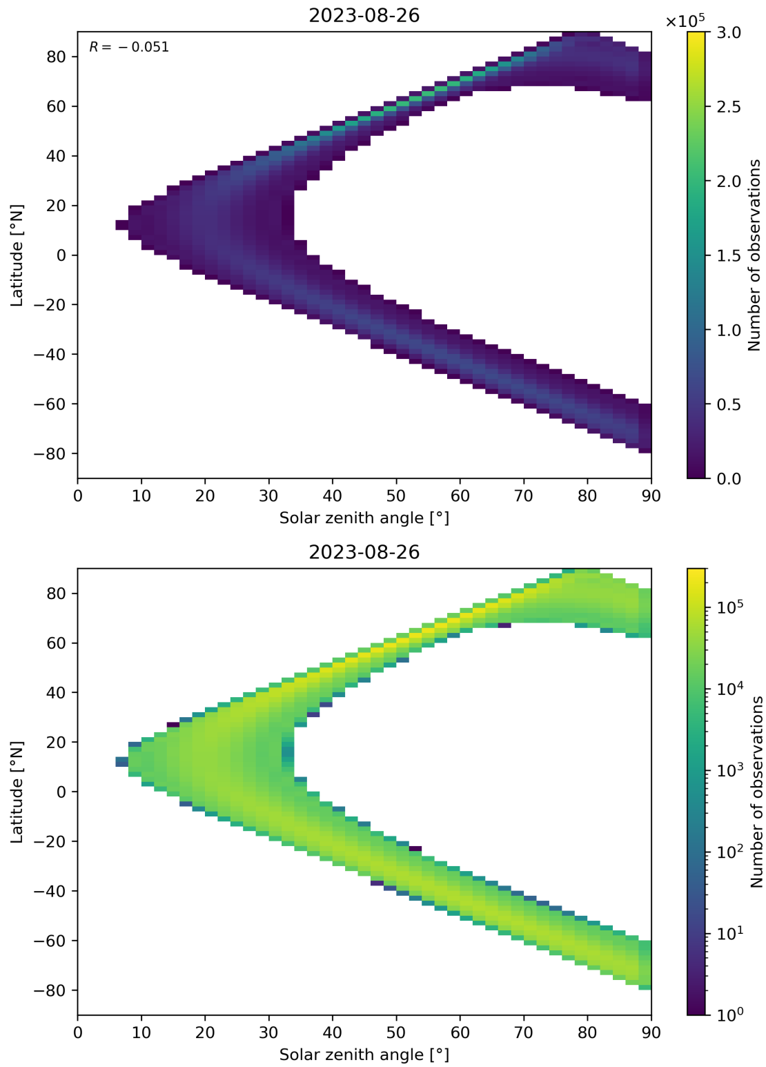
Figure 44: Scatter density plot of “Solar zenith angle” against “Latitude” for 2023-08-25 to 2023-08-27.
