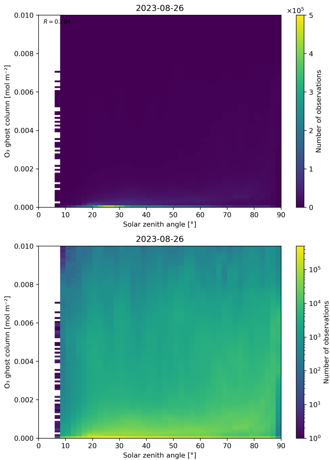
Figure 46: Scatter density plot of “Solar zenith angle” against “O 3 ghost column” for 2023-08-25 to 2023-08-27.
