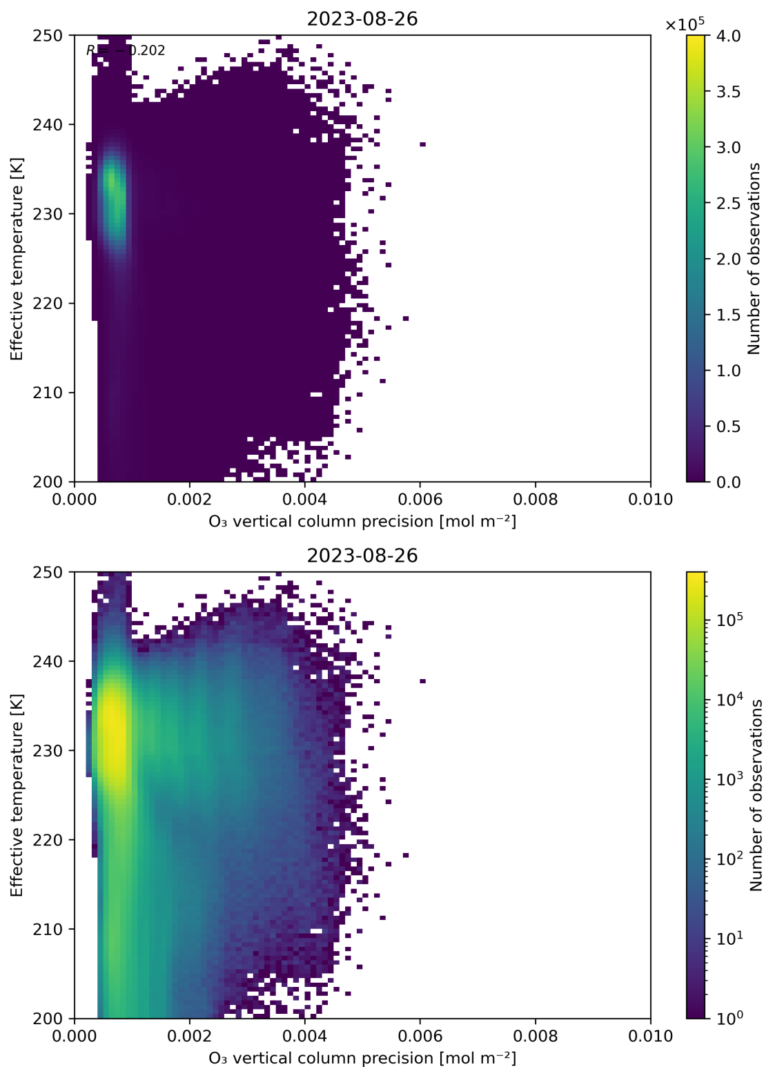
Figure 42: Scatter density plot of “O 3 vertical column precision” against “Effective temperature” for 2023-08-25 to 2023-08-27.
