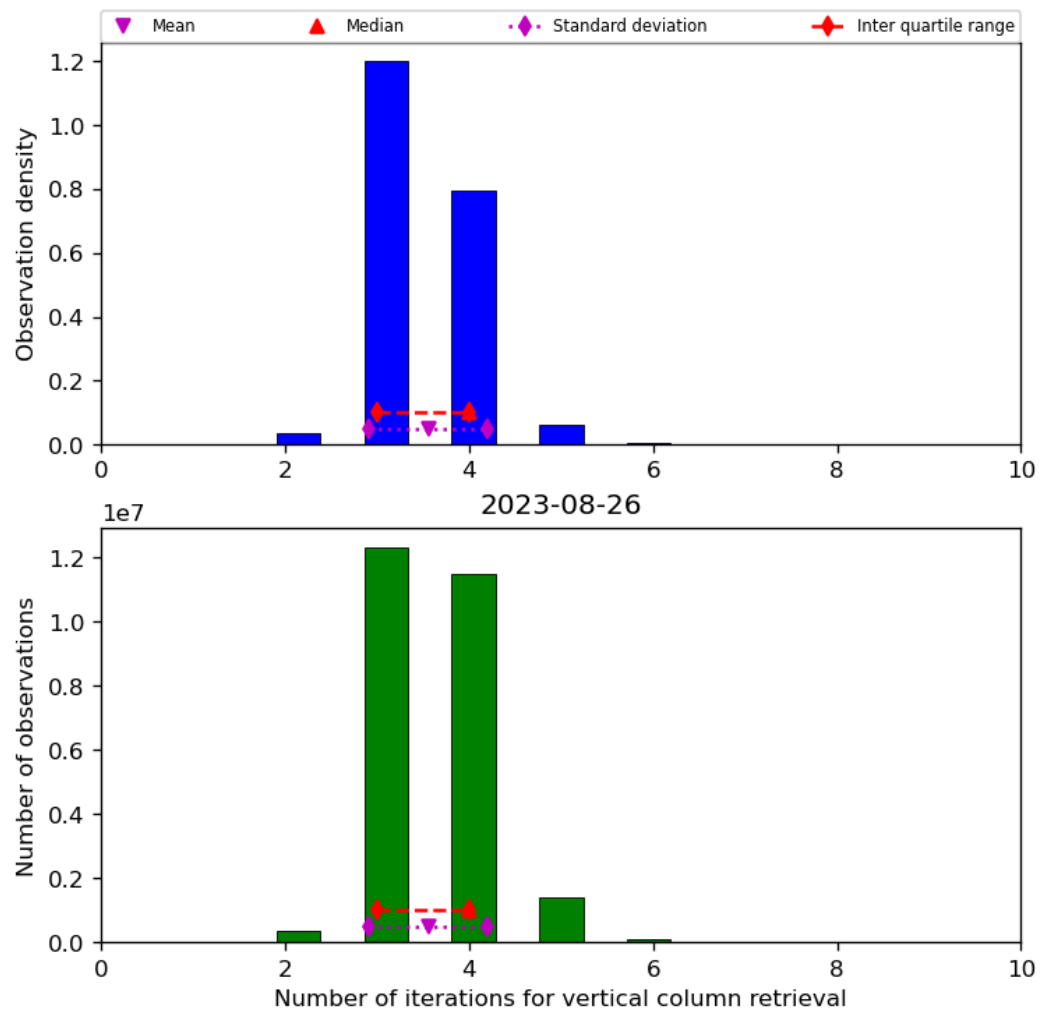
Figure 26: Histogram of “Number of iterations for vertical column retrieval” for 2023-08-25 to 2023-08-27
