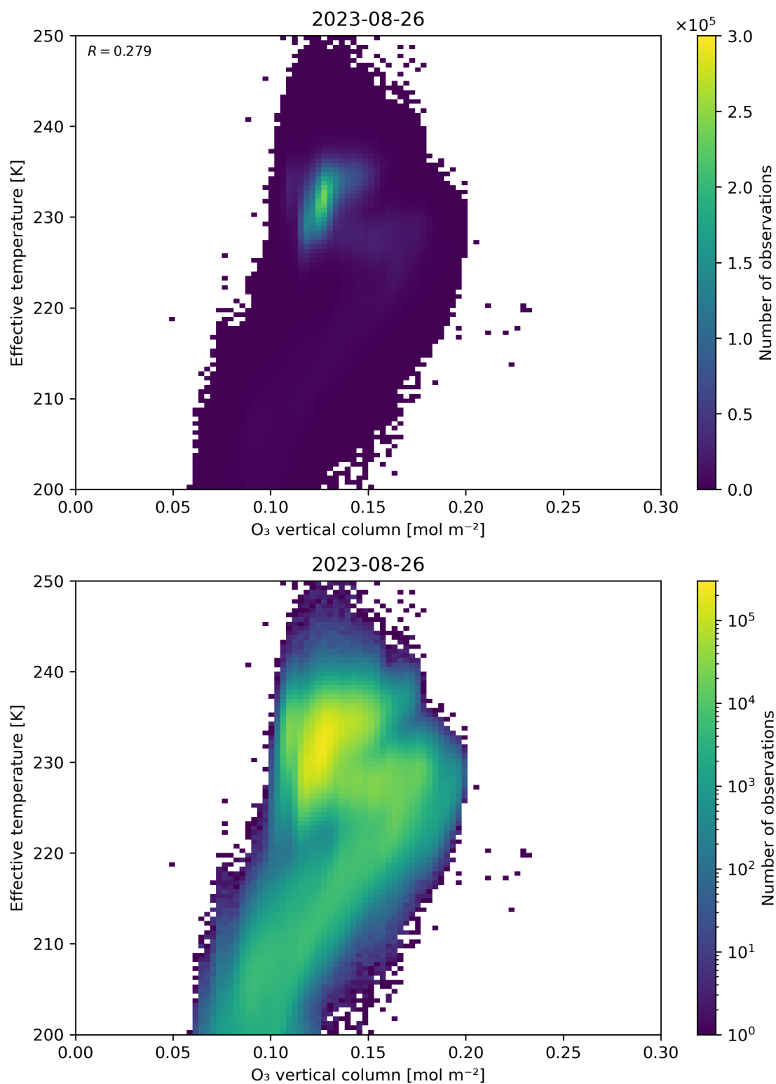
Figure 39: Scatter density plot of “O 3 vertical column” against “Effective temperature” for 2023-08-25 to 2023-08-27.
