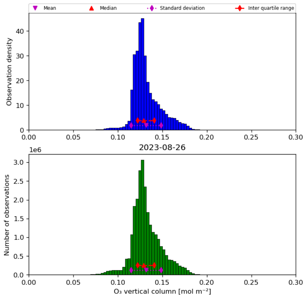
Figure 21: Histogram of “O 3 vertical column” for 2023-08-25 to 2023-08-27
