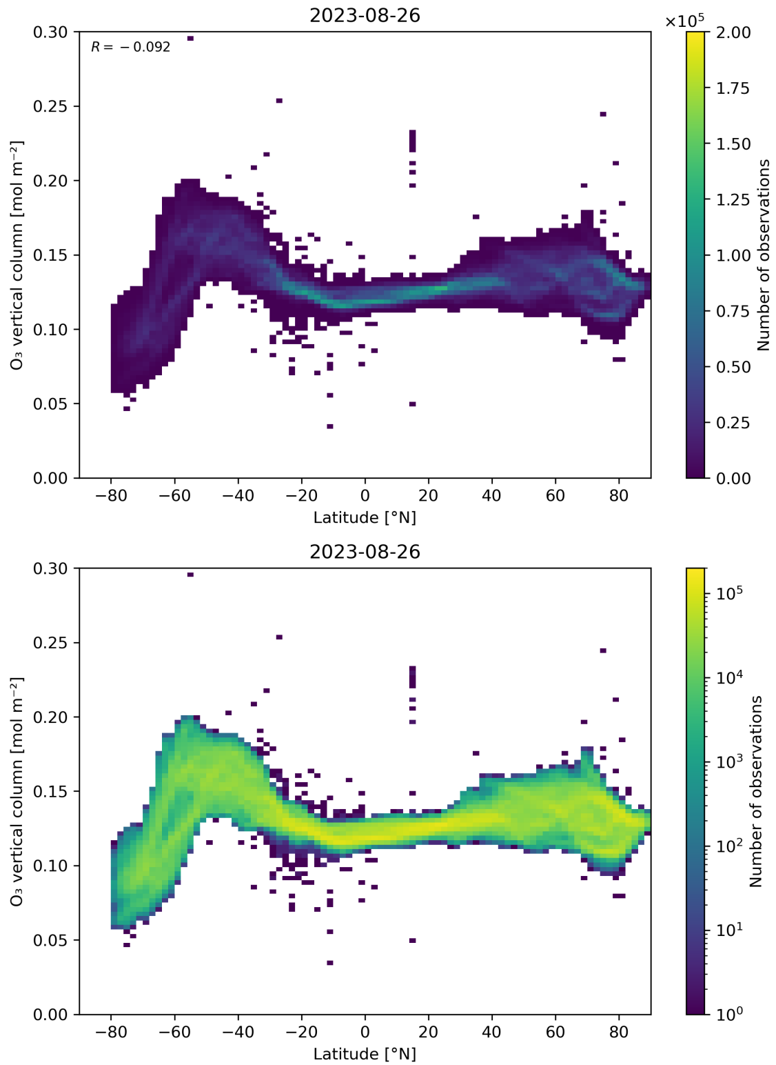
Figure 36: Scatter density plot of “Latitude” against “O 3 vertical column” for 2023-08-25 to 2023-08-27.
