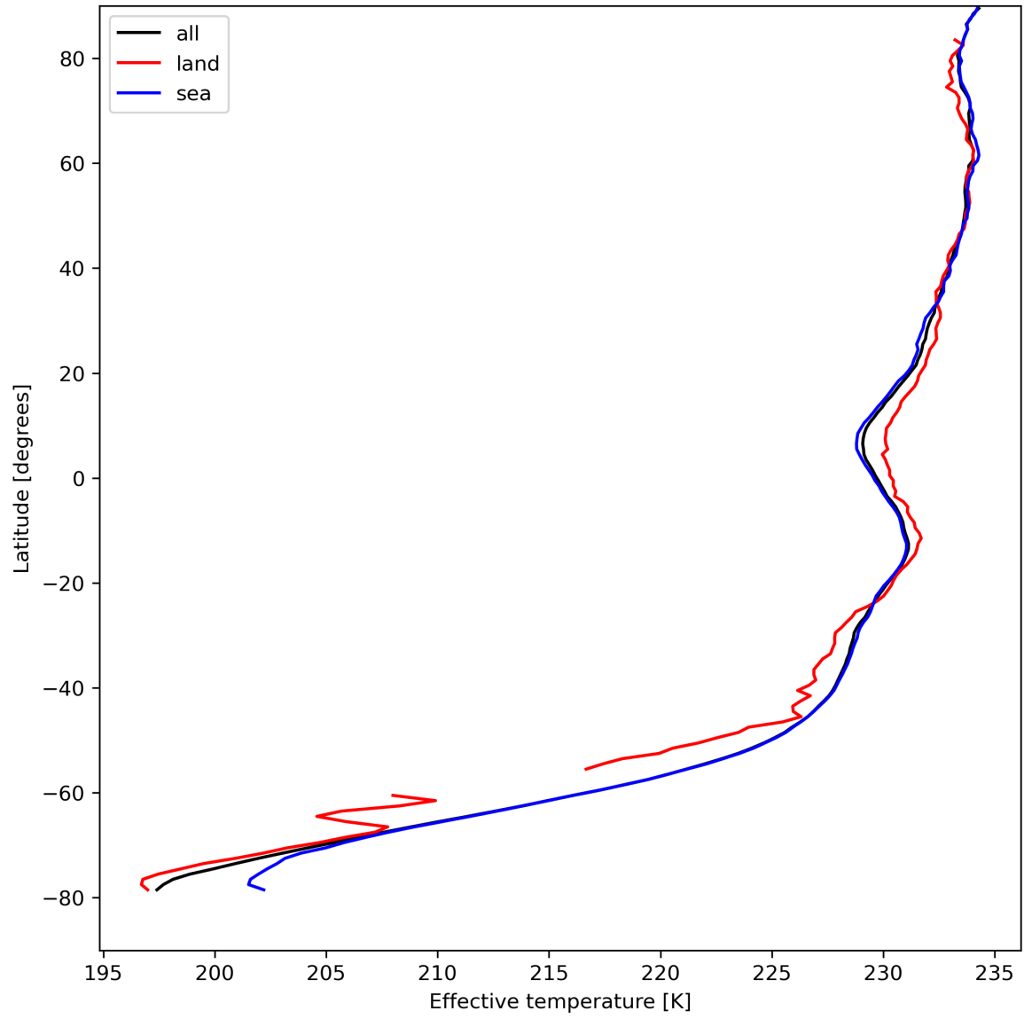
Figure 17: Zonal average of "Effective temperature" for 2023-08-25 to 2023-08-27.
