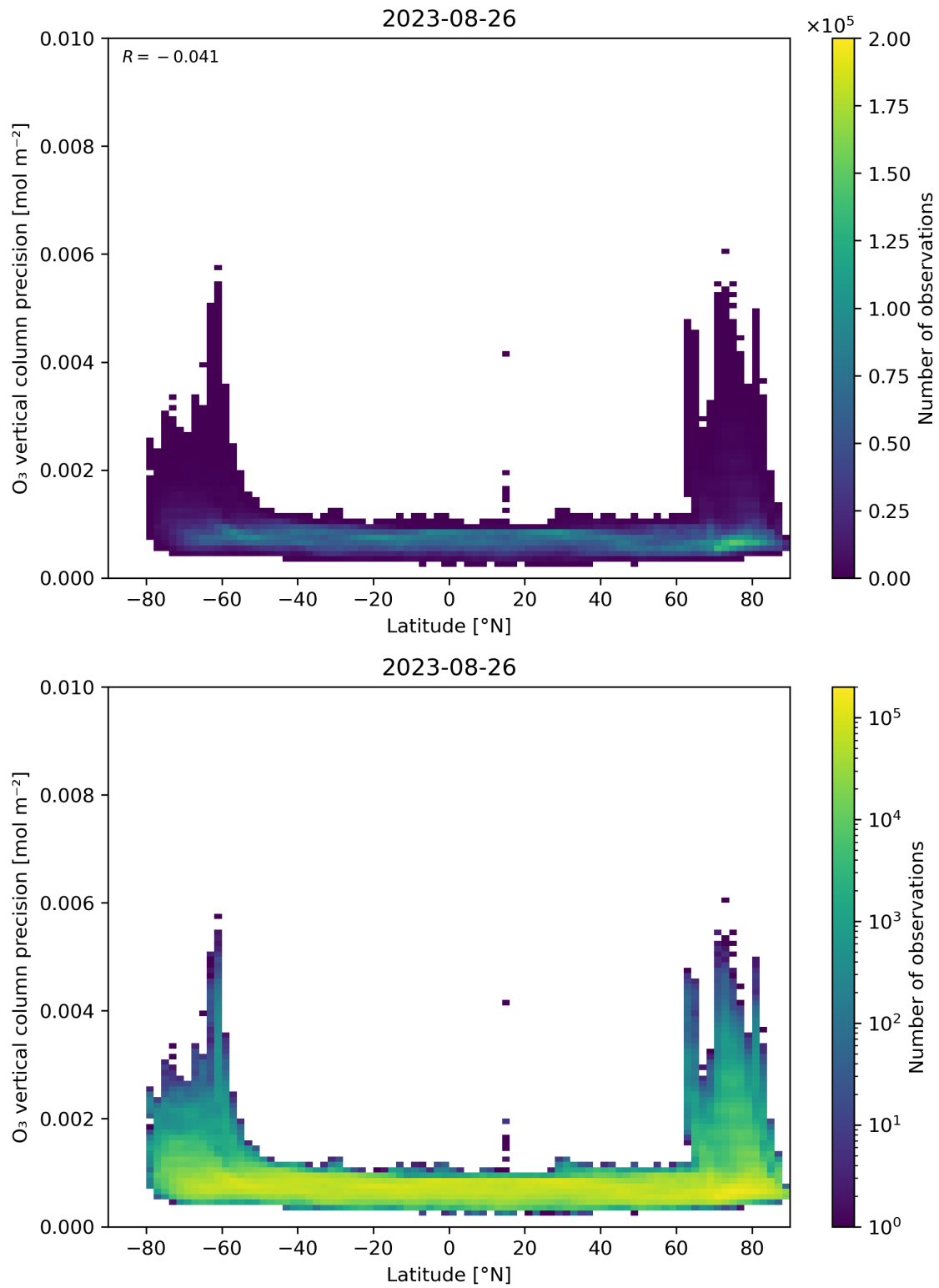
Figure 37: Scatter density plot of “Latitude” against “O 3 vertical column precision” for 2023-08-25 to 2023-08-27.
