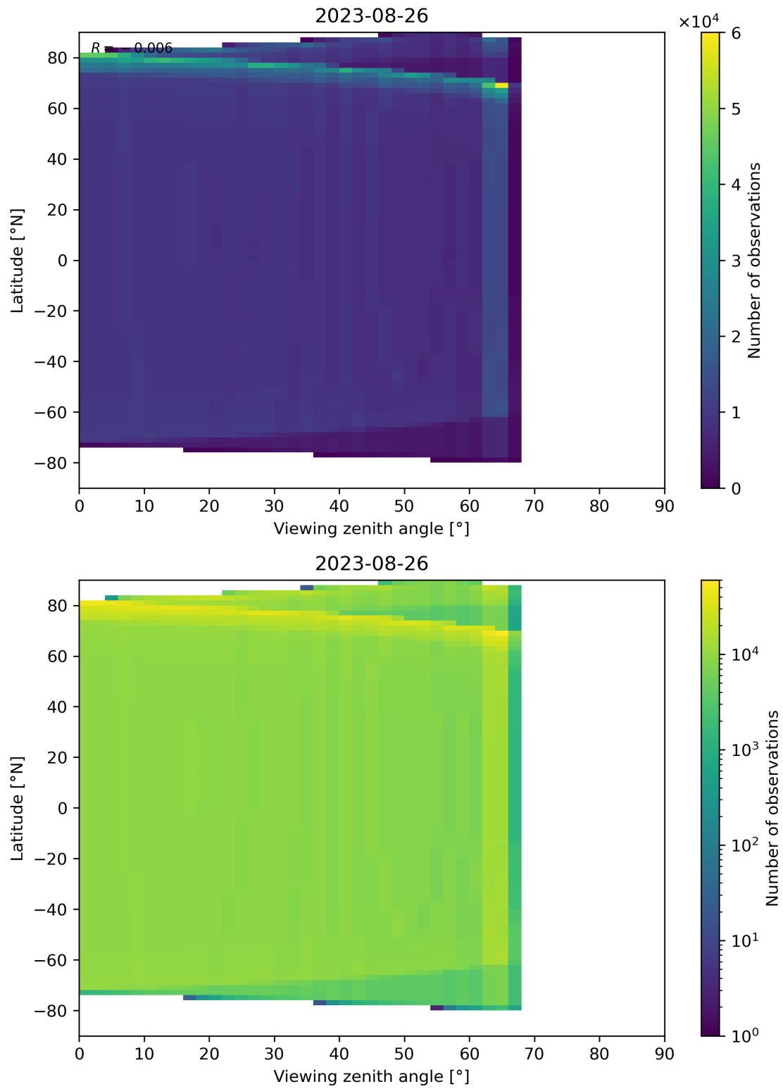
Figure 49: Scatter density plot of “Viewing zenith angle” against “Latitude” for 2023-08-25 to 2023-08-27.
