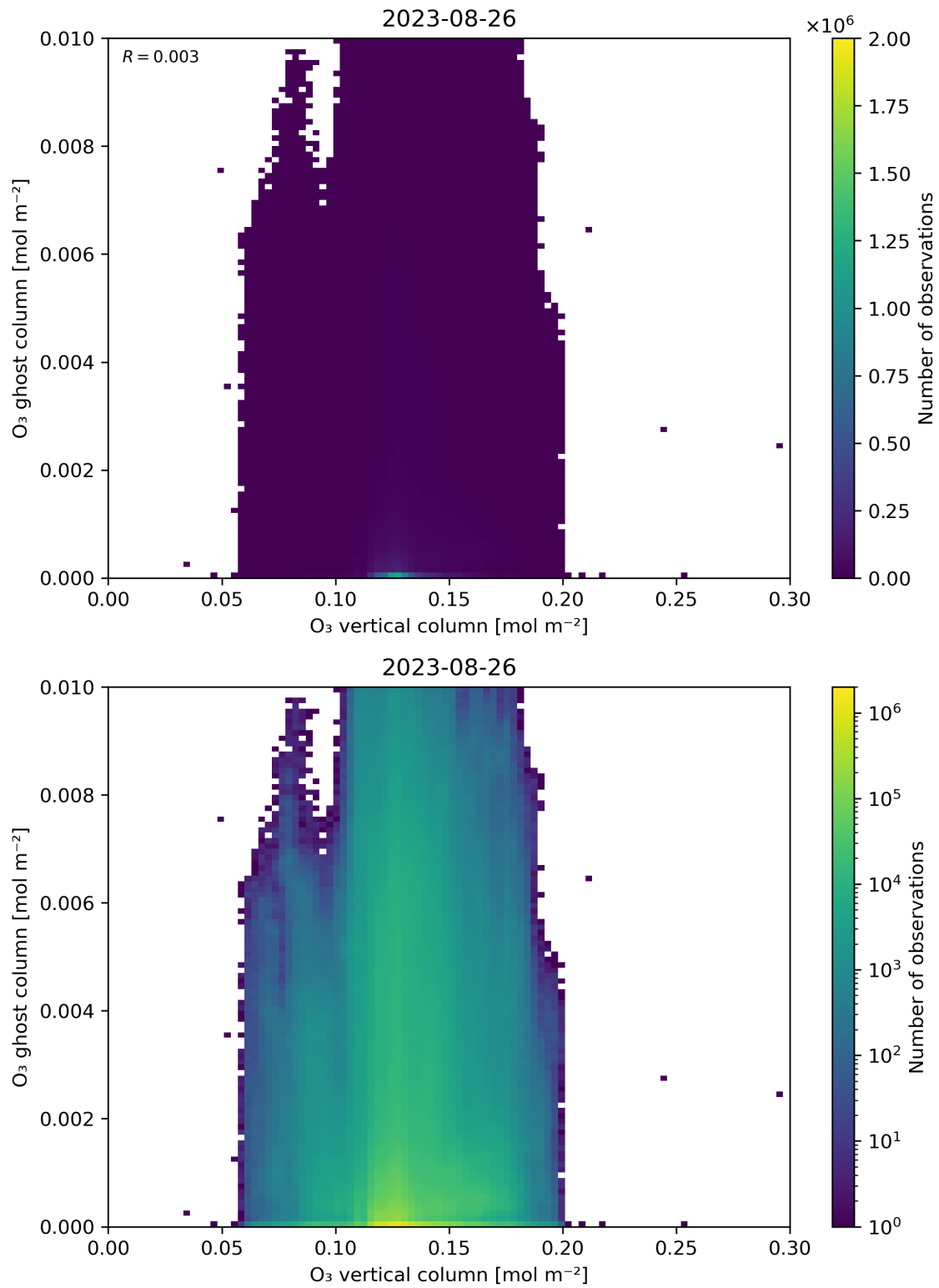
Figure 40: Scatter density plot of “O 3 vertical column” against “O 3 ghost column” for 2023-08-25 to 2023-08-27.
