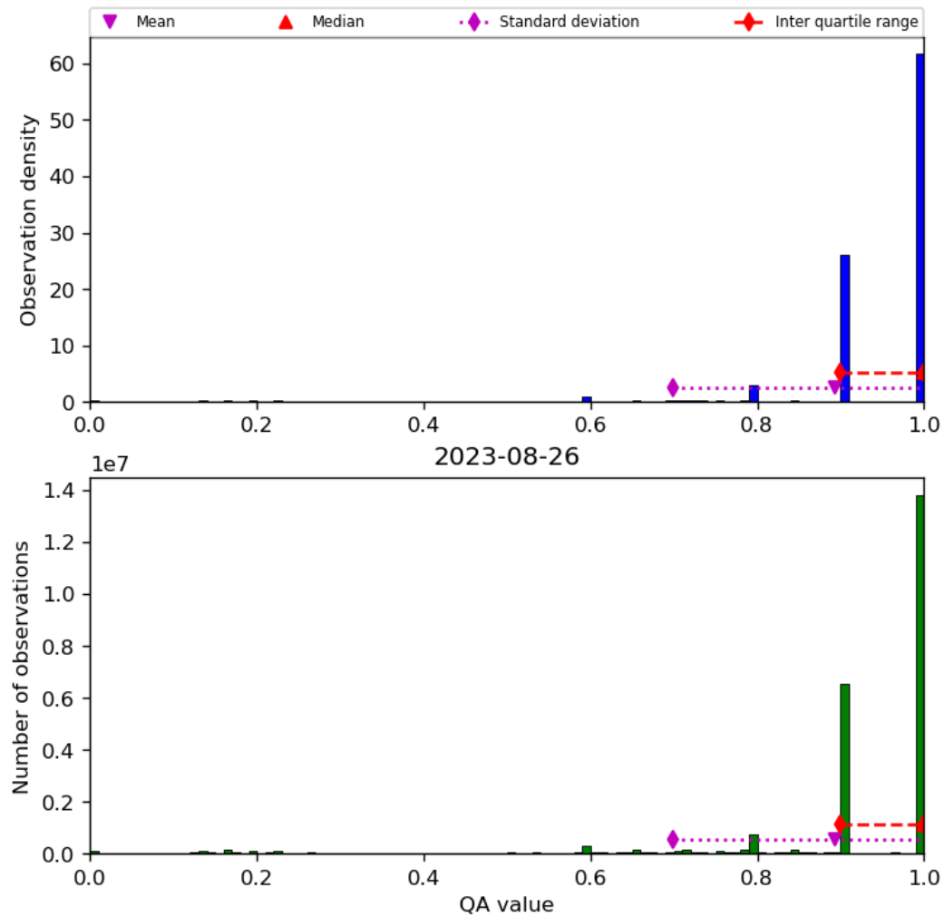
Figure 20: Histogram of “QA value” for 2023-08-25 to 2023-08-27
