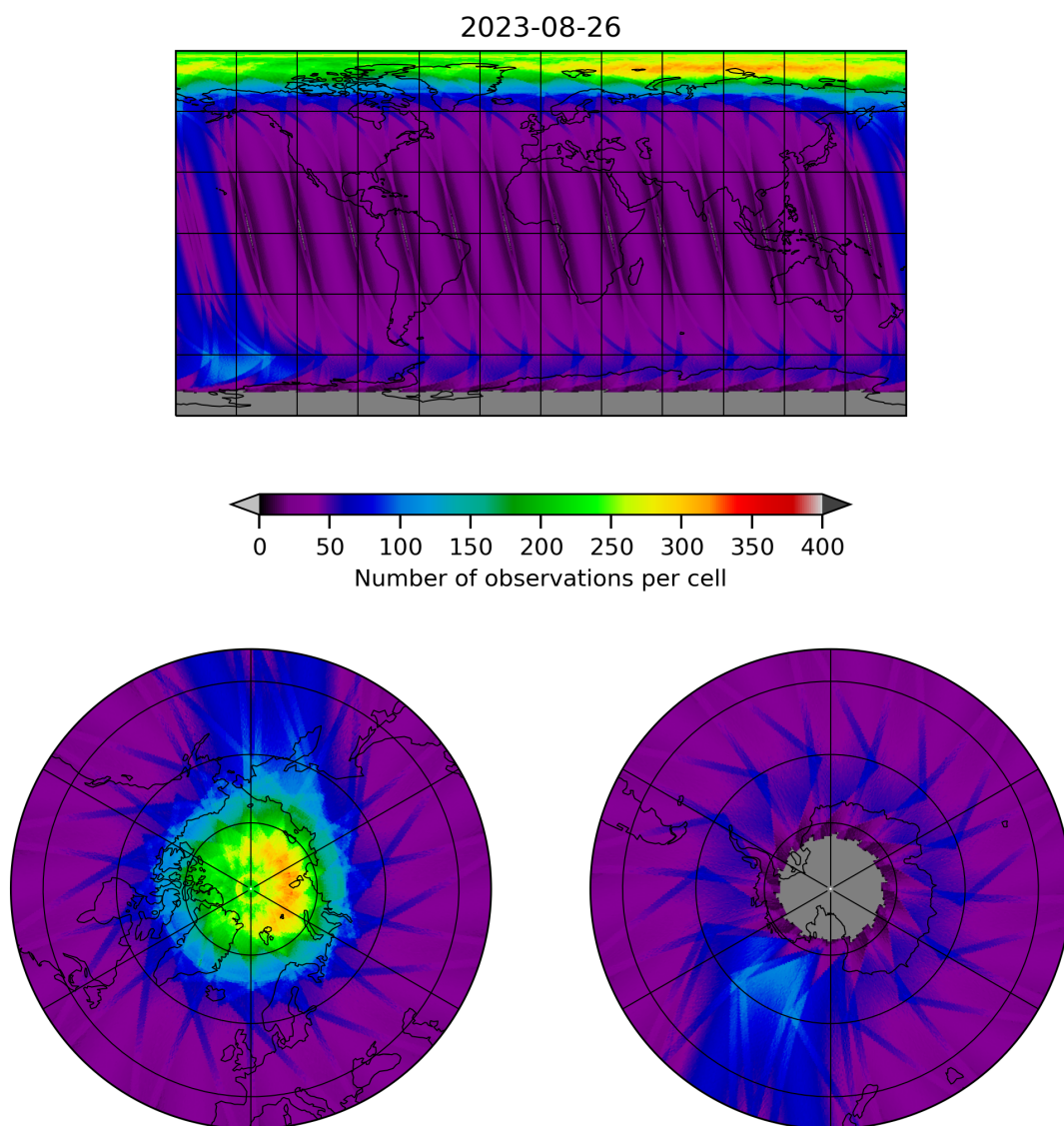
Figure 12: Map of the number of observations for 2023-08-25 to 2023-08-27
