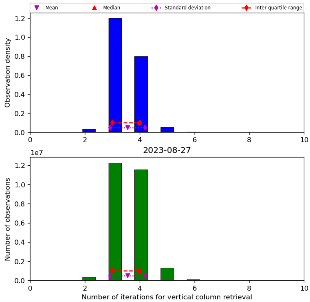
Figure 26: Histogram of “Number of iterations for vertical column retrieval” for 2023-08-26 to 2023-08-28
