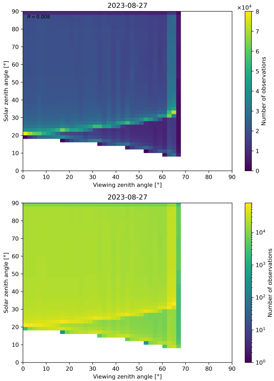
Figure 54: Scatter density plot of “Viewing zenith angle” against “Solar zenith angle” for 2023-08-26 to 2023-08-28.
