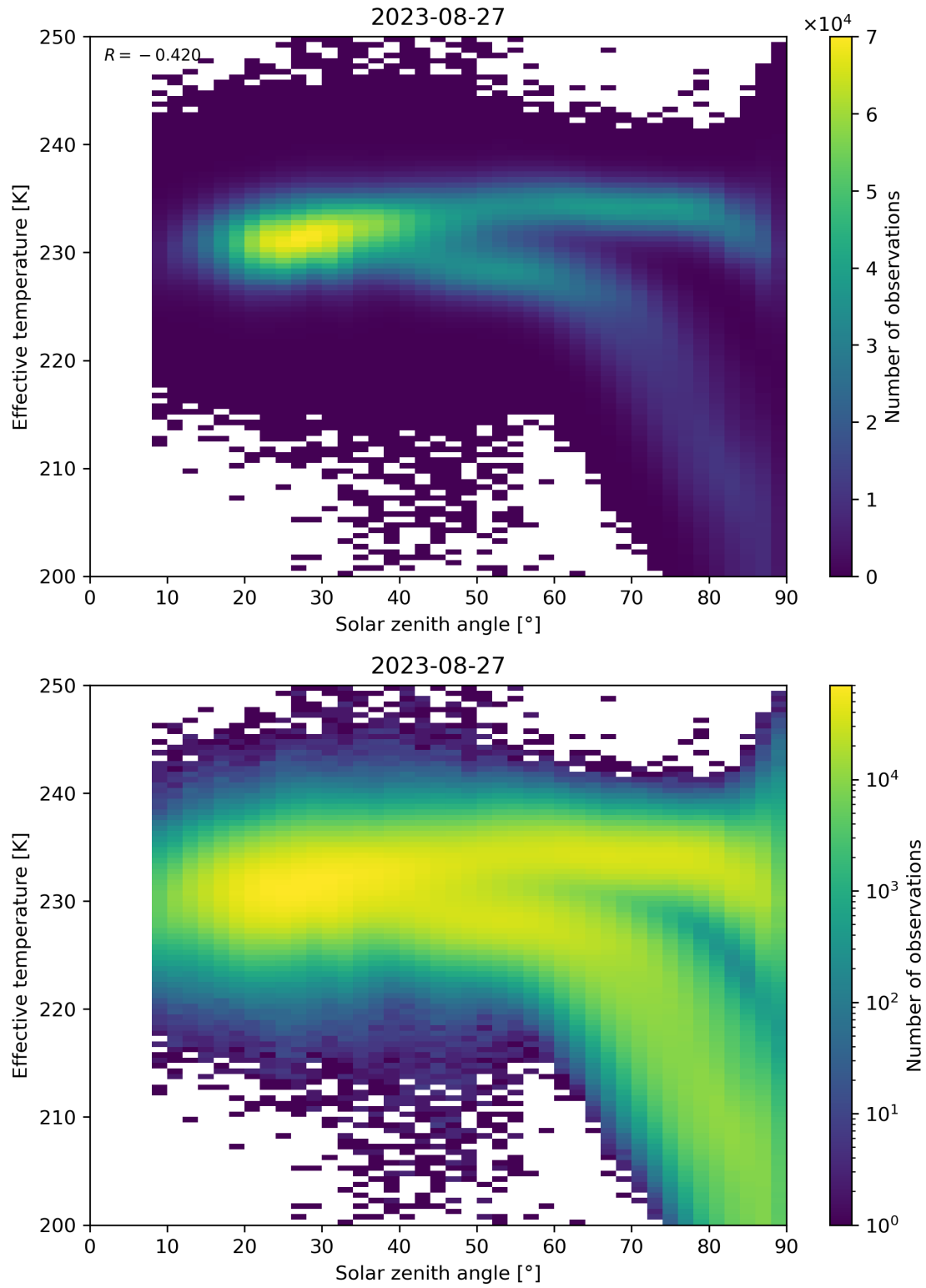
Figure 45: Scatter density plot of “Solar zenith angle” against “Effective temperature” for 2023-08-26 to 2023-08-28.
