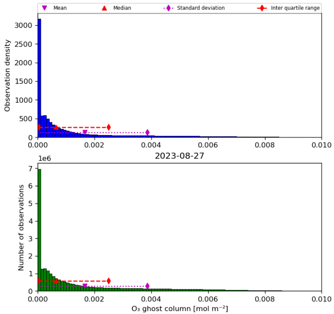
Figure 25: Histogram of “O 3 ghost column” for 2023-08-26 to 2023-08-28
