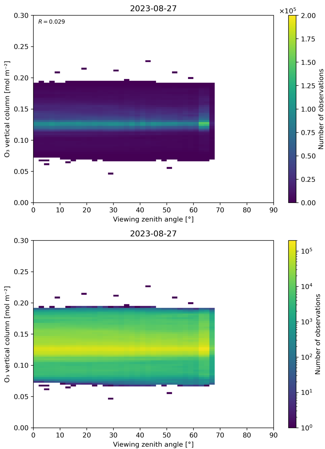
Figure 52: Scatter density plot of “Viewing zenith angle” against “O 3 vertical column” for 2023-08-26 to 2023-08-28.
