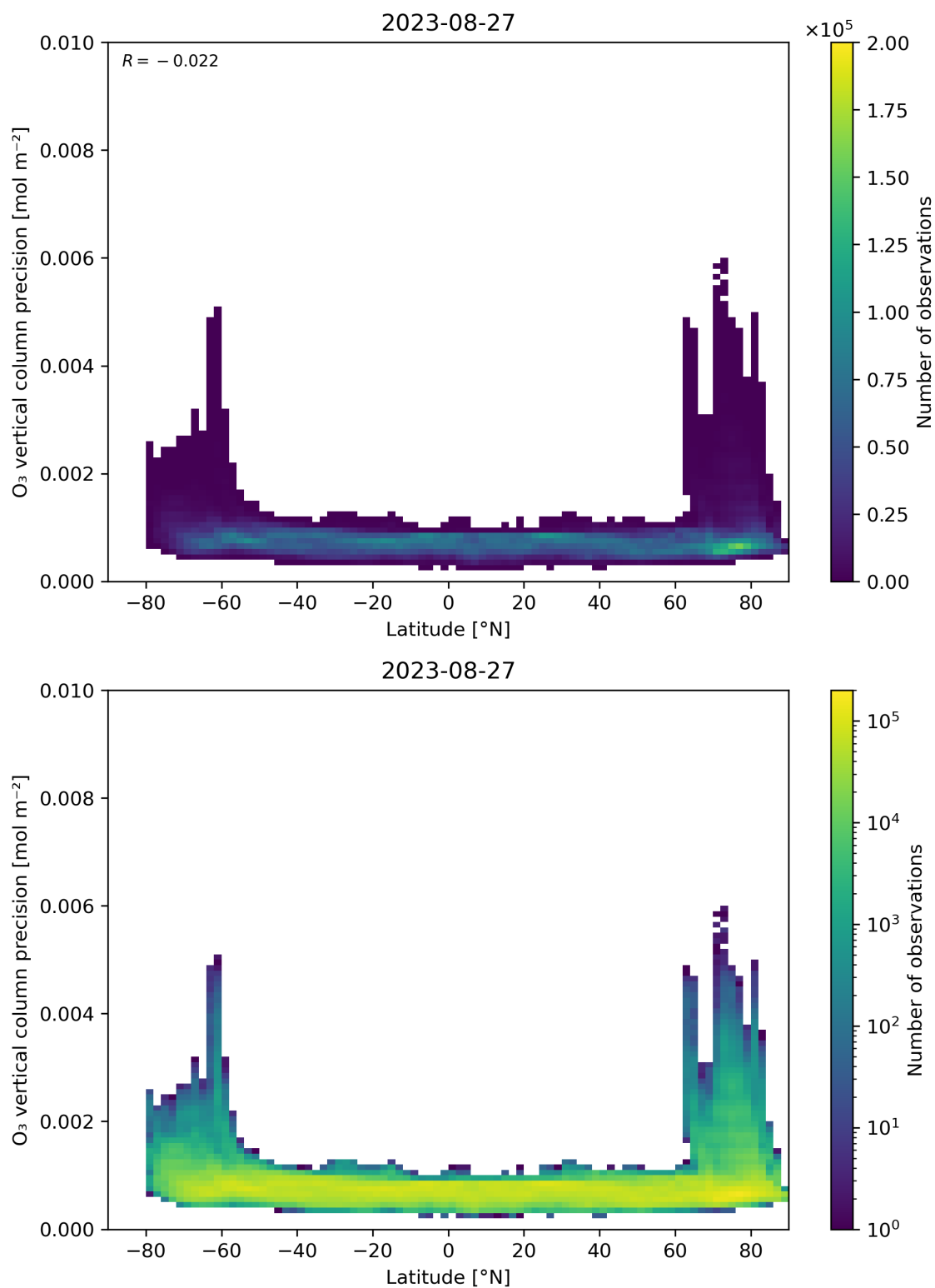
Figure 37: Scatter density plot of “Latitude” against “O 3 vertical column precision” for 2023-08-26 to 2023-08-28.
