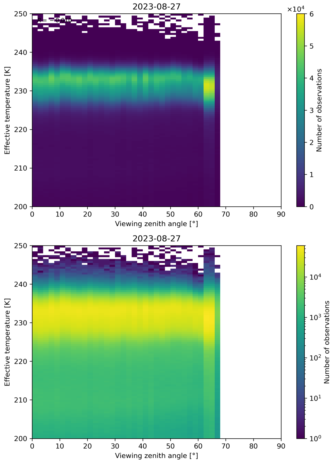
Figure 50: Scatter density plot of “Viewing zenith angle” against “Effective temperature” for 2023-08-26 to 2023-08-28.
