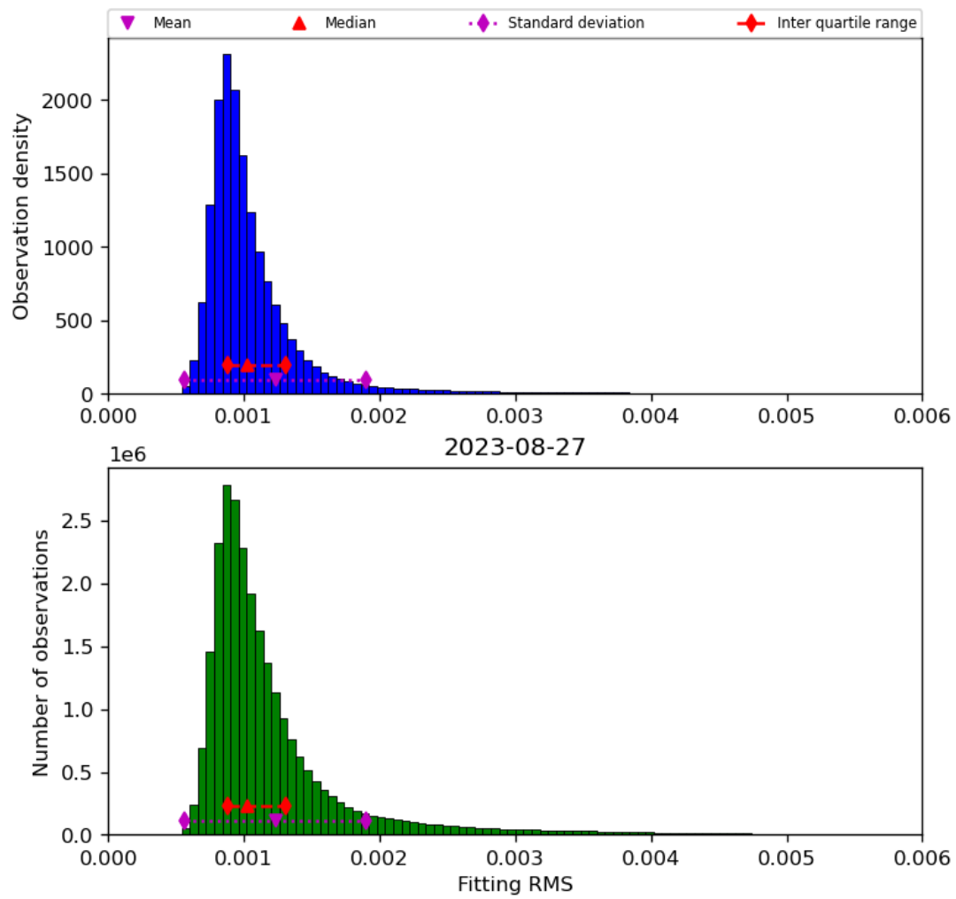
Figure 23: Histogram of “Fitting RMS” for 2023-08-26 to 2023-08-28
