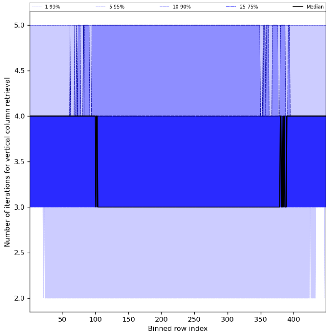
Figure 33: Along track statistics of “Number of iterations for vertical column retrieval” for 2023-08-26 to 2023-08-28
