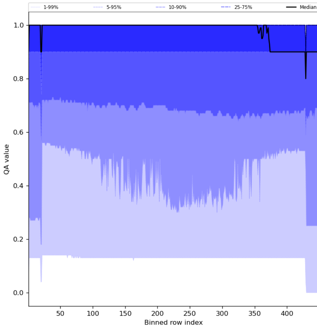
Figure 27: Along track statistics of “QA value” for 2023-08-26 to 2023-08-28
