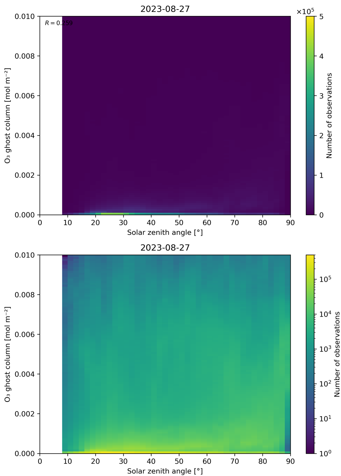
Figure 46: Scatter density plot of “Solar zenith angle” against “O 3 ghost column” for 2023-08-26 to 2023-08-28.
