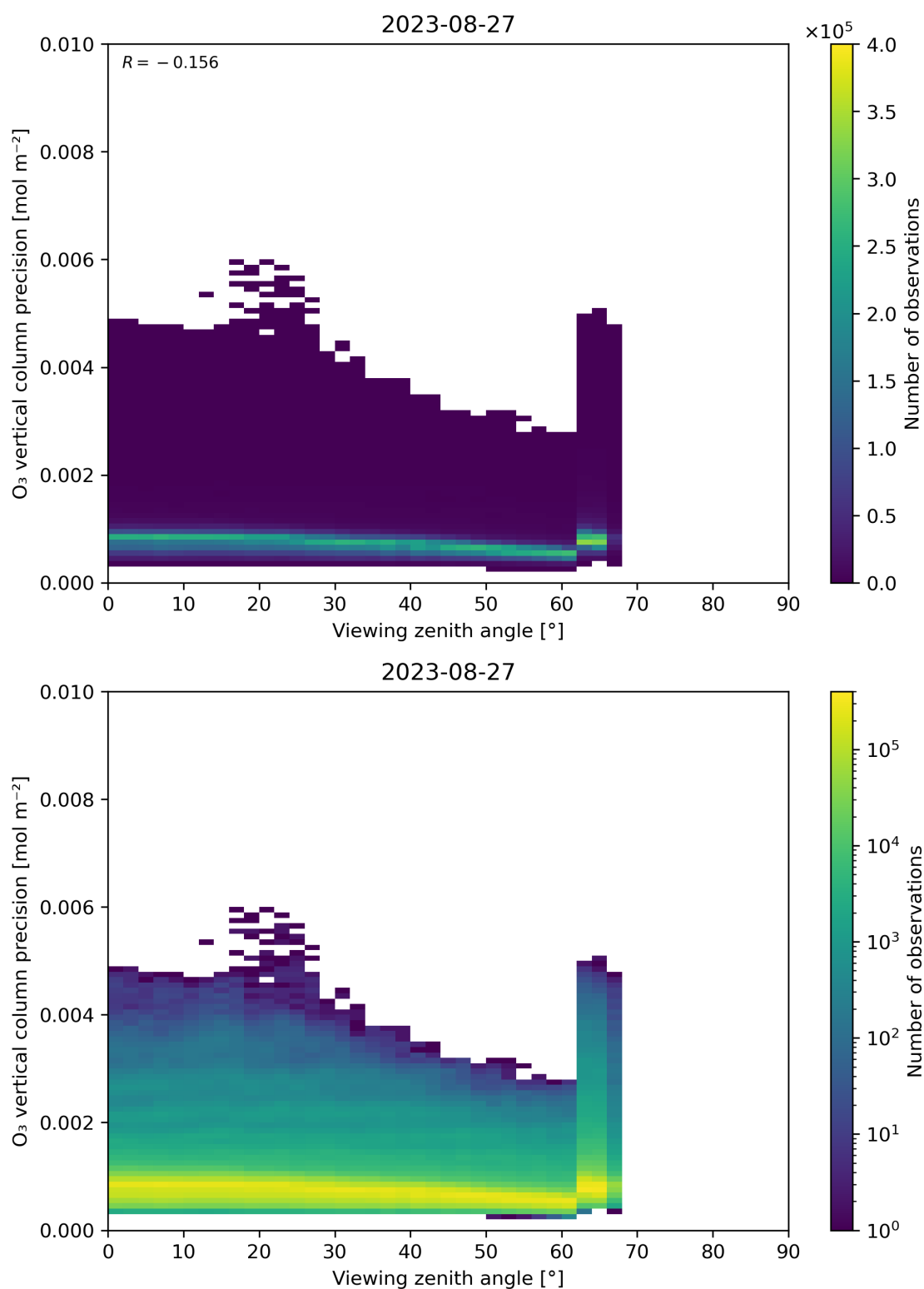
Figure 53: Scatter density plot of “Viewing zenith angle” against “O 3 vertical column precision” for 2023-08-26 to 2023-08-28.
