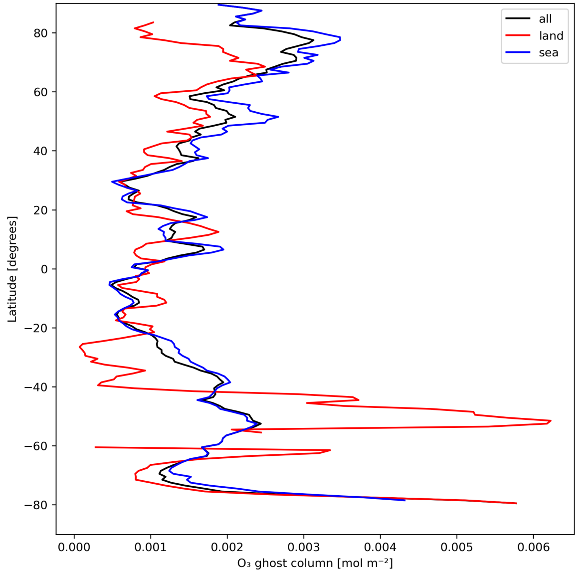
Figure 18: Zonal average of “O 3 ghost column” for 2023-08-26 to 2023-08-28.
