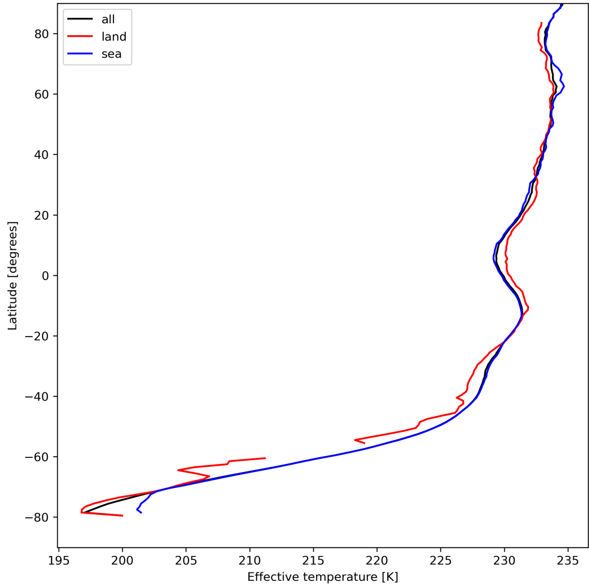
Figure 17: Zonal average of "Effective temperature" for 2023-08-26 to 2023-08-28.
