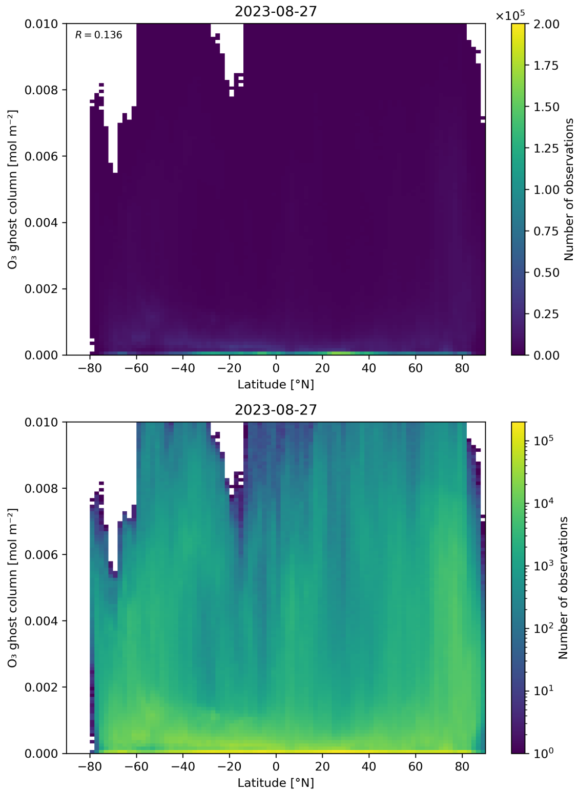
Figure 35: Scatter density plot of “Latitude” against “O 3 ghost column” for 2023-08-26 to 2023-08-28.
