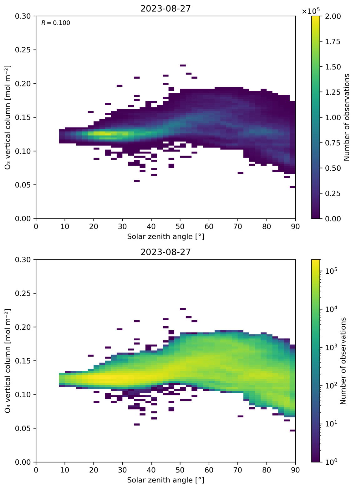
Figure 47: Scatter density plot of “Solar zenith angle” against “O 3 vertical column” for 2023-08-26 to 2023-08-28.
