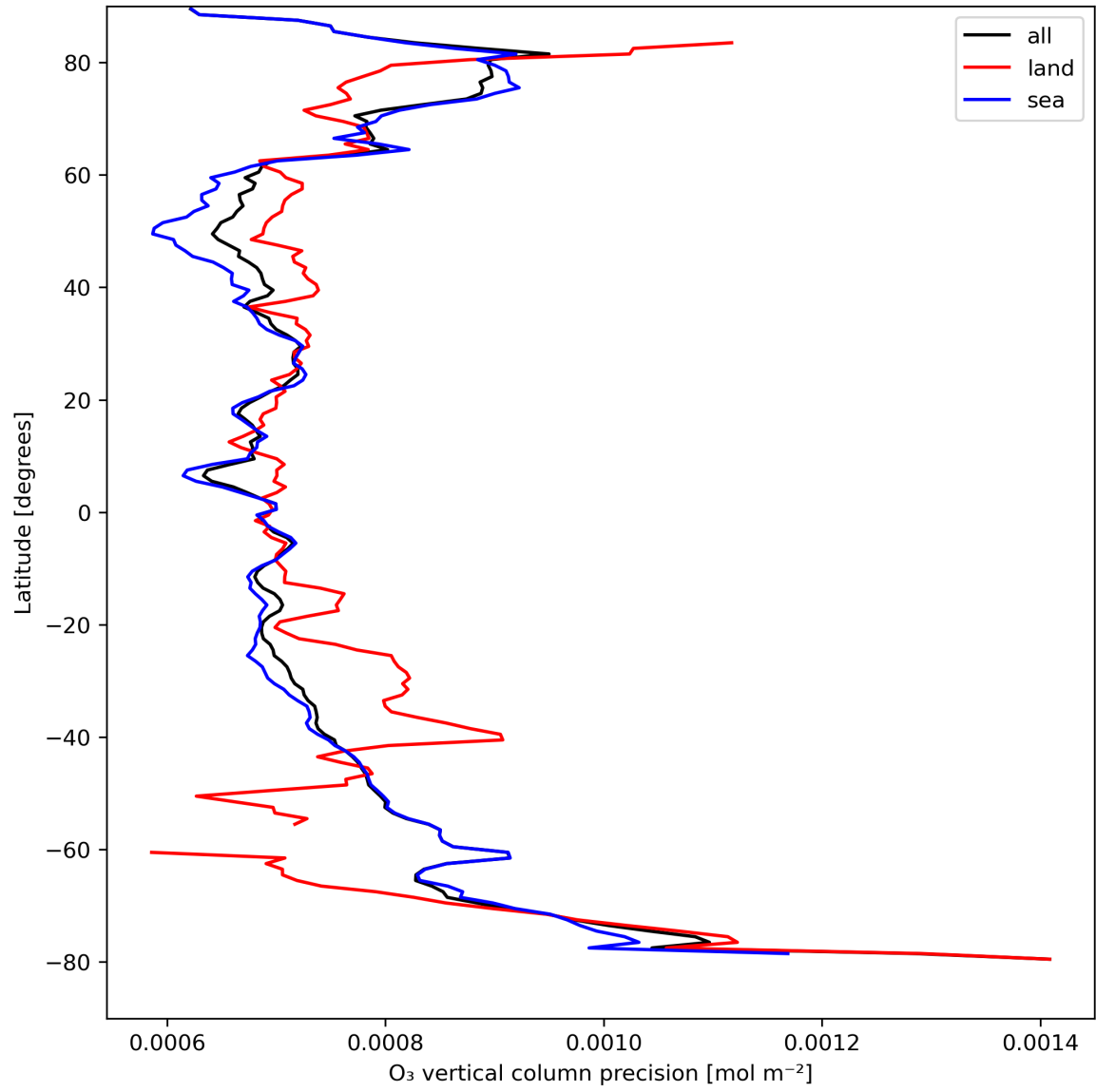
Figure 15: Zonal average of “O 3 vertical column precision” for 2023-08-26 to 2023-08-28.
