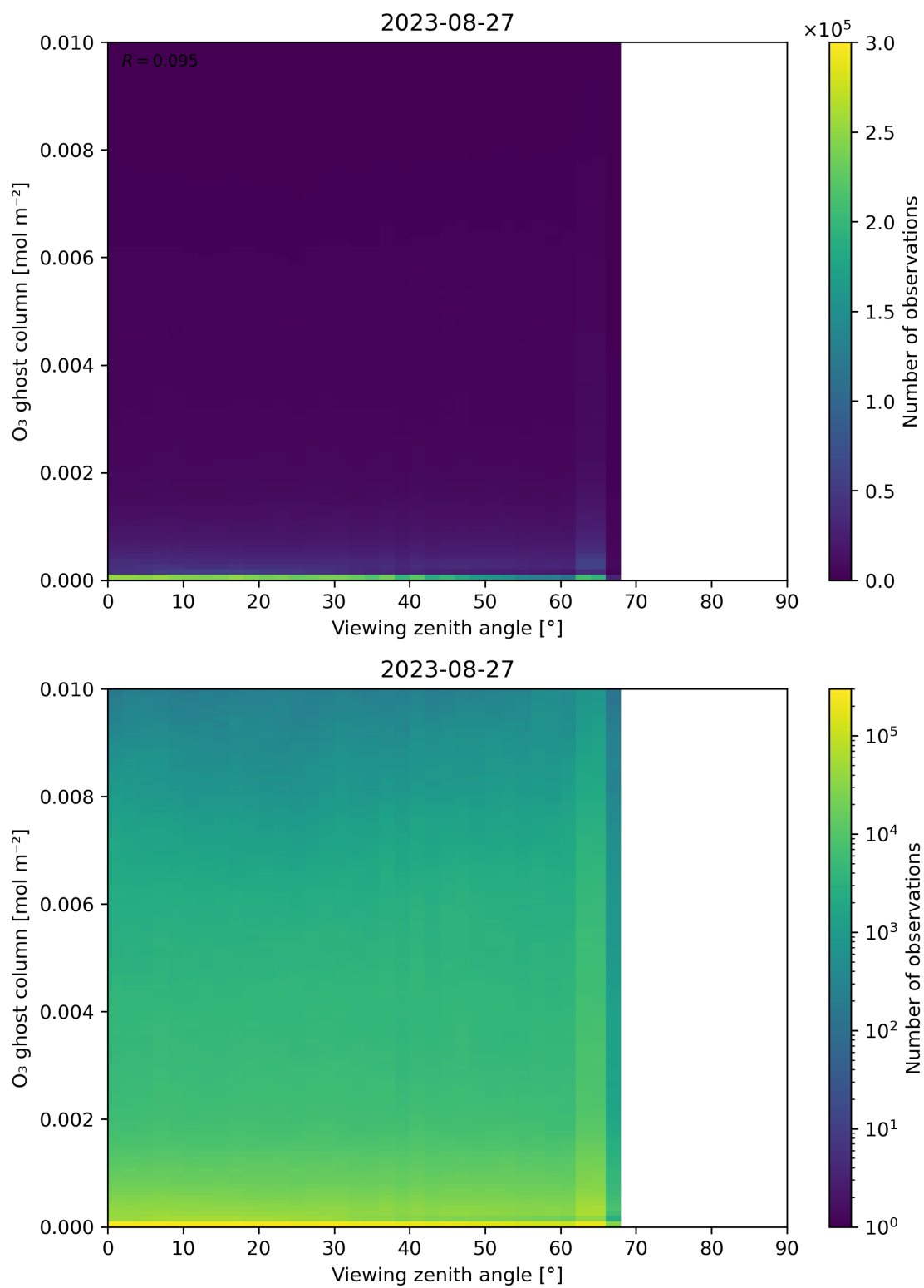
Figure 51: Scatter density plot of “Viewing zenith angle” against “O 3 ghost column” for 2023-08-26 to 2023-08-28.
