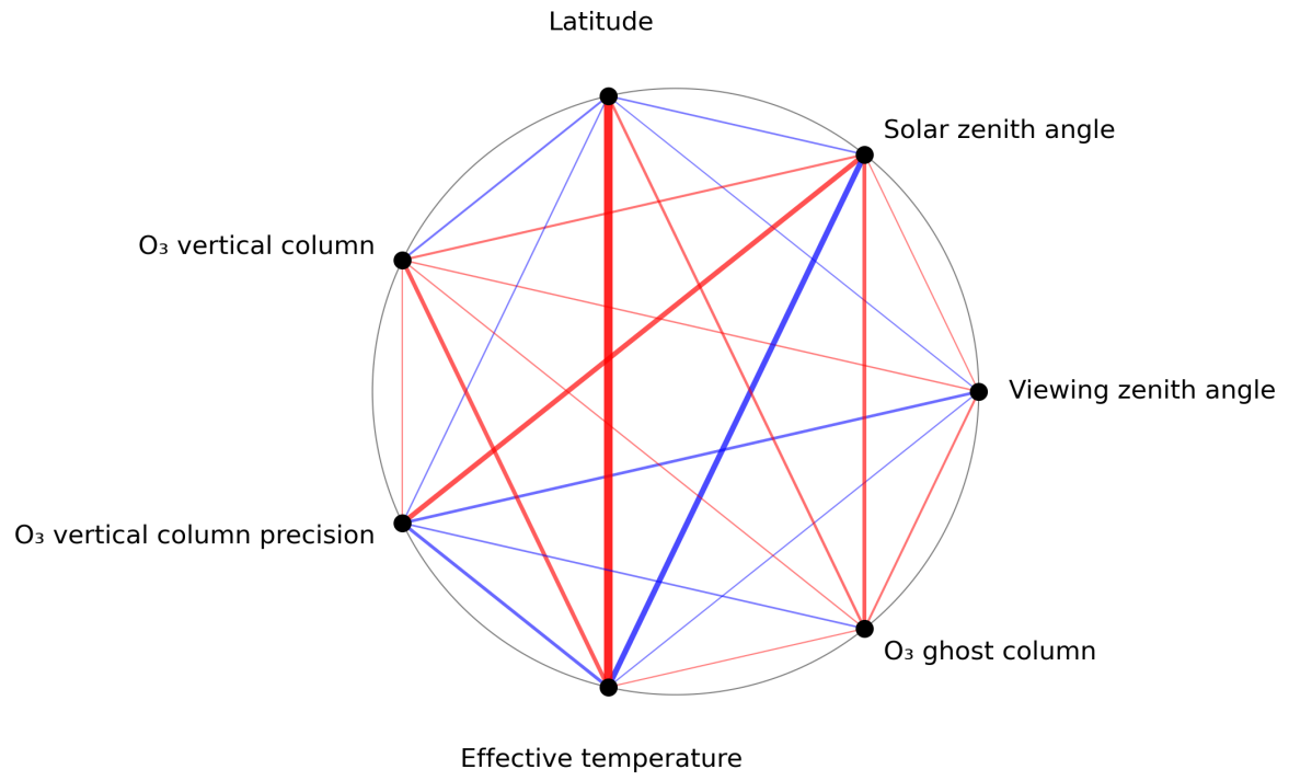
Figure 1: Map of correlation graph for 2023-08-26 to 2023-08-28.
