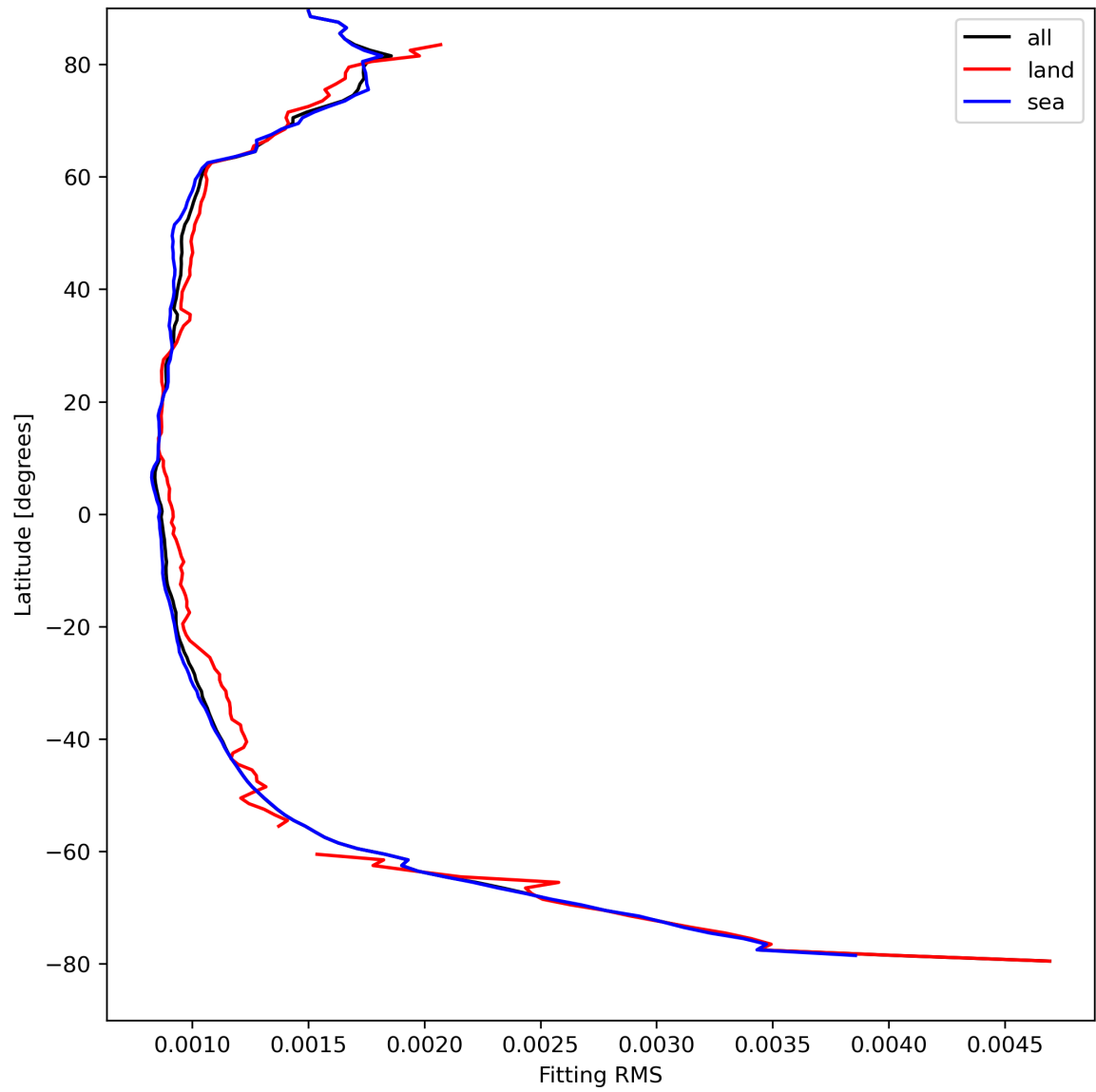
Figure 16: Zonal average of “Fitting RMS” for 2023-08-26 to 2023-08-28.
