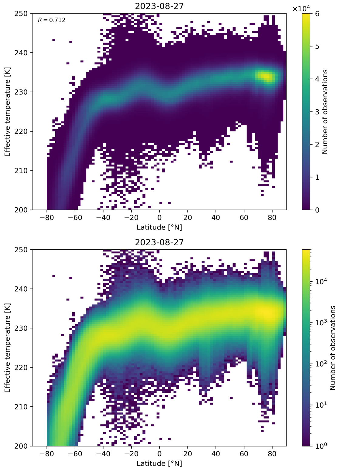
Figure 34: Scatter density plot of “Latitude” against “Effective temperature” for 2023-08-26 to 2023-08-28.
