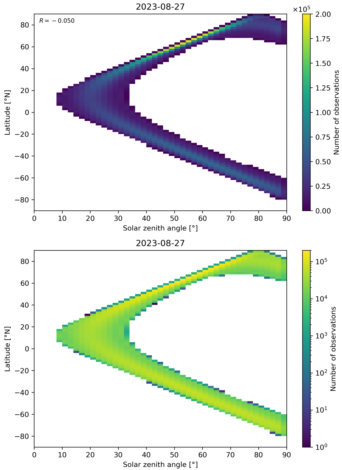
Figure 44: Scatter density plot of “Solar zenith angle” against “Latitude” for 2023-08-26 to 2023-08-28.
