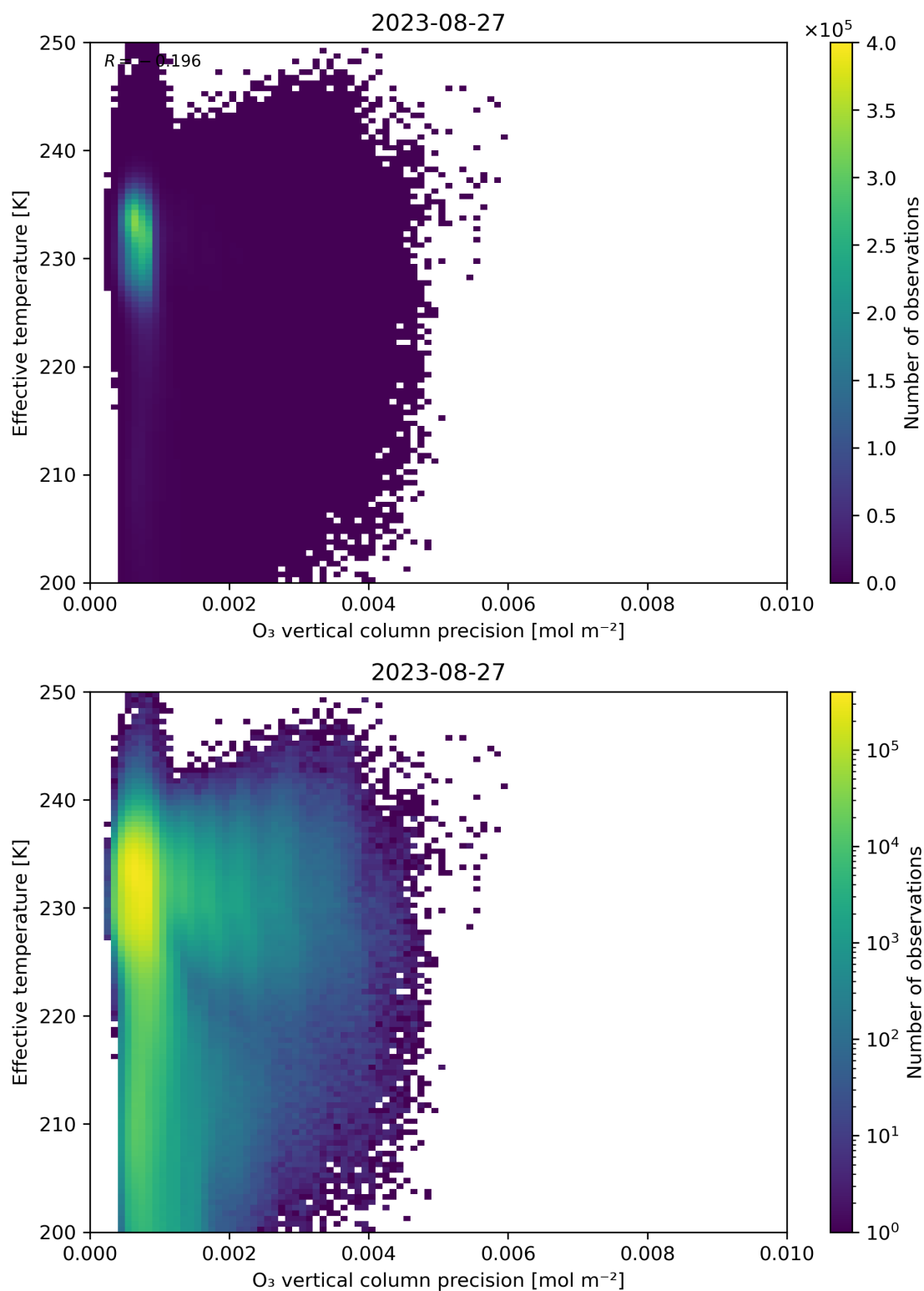
Figure 42: Scatter density plot of “O 3 vertical column precision” against “Effective temperature” for 2023-08-26 to 2023-08-28.
