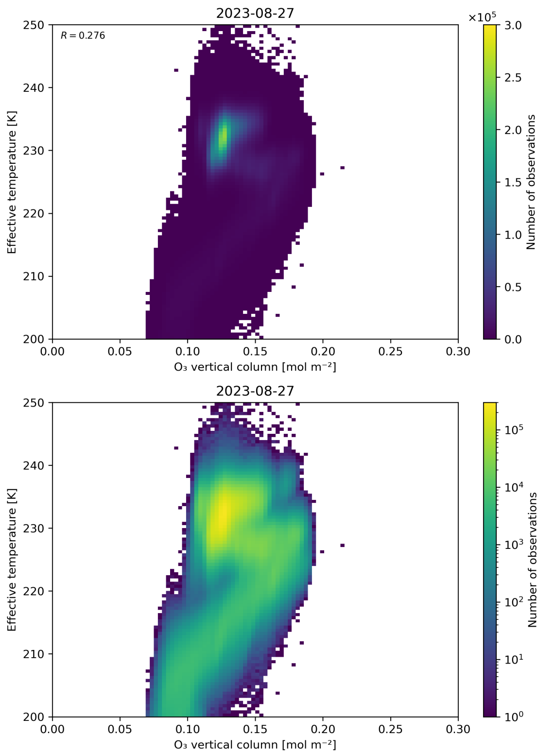
Figure 39: Scatter density plot of “O 3 vertical column” against “Effective temperature” for 2023-08-26 to 2023-08-28.
