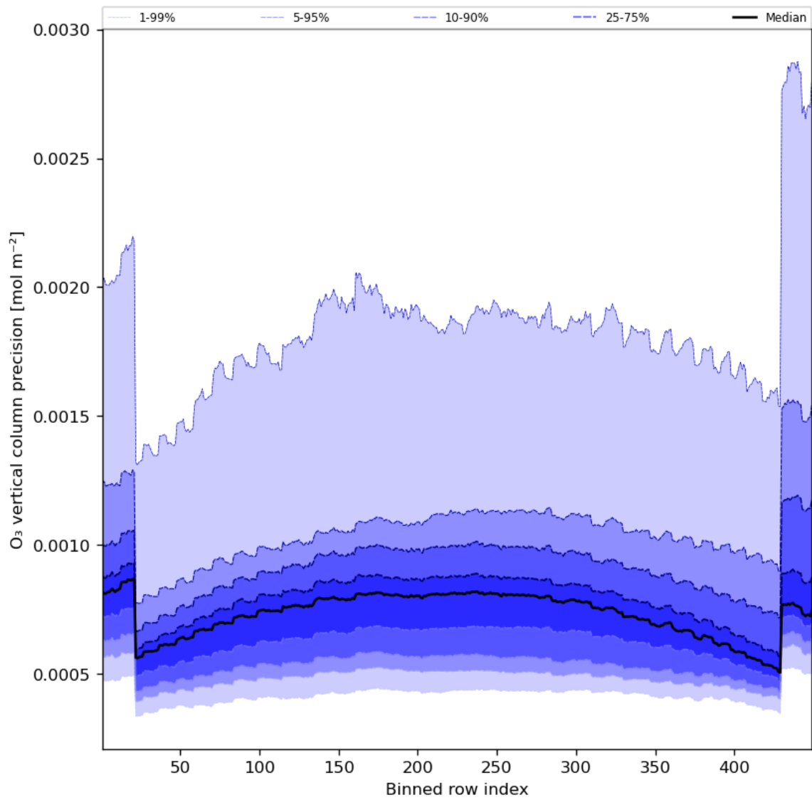
Figure 29: Along track statistics of “O 3 vertical column precision” for 2023-08-26 to 2023-08-28
