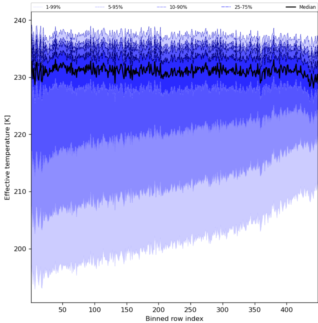
Figure 31: Along track statistics of “Effective temperature” for 2023-08-26 to 2023-08-28
