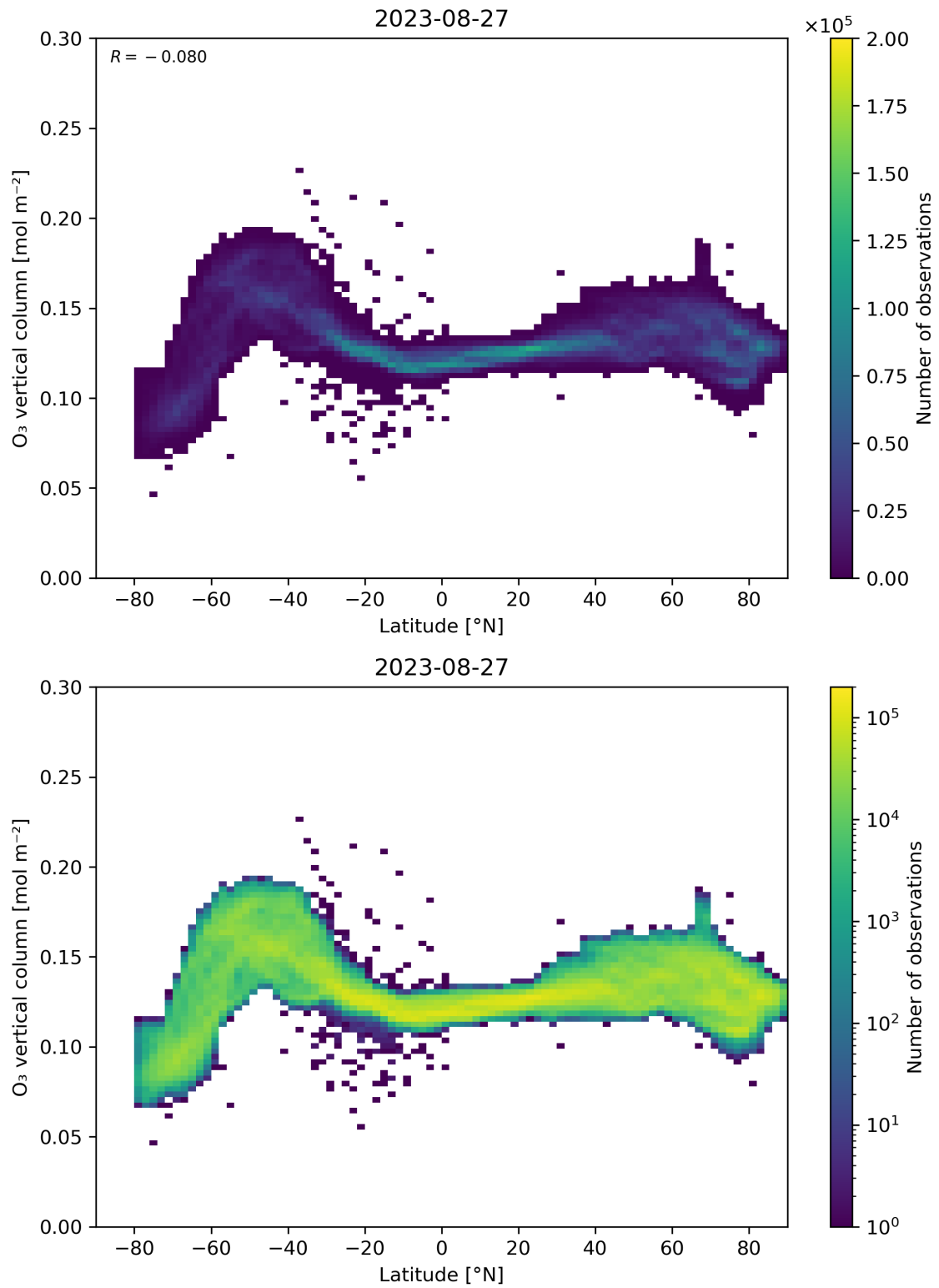
Figure 36: Scatter density plot of “Latitude” against “O 3 vertical column” for 2023-08-26 to 2023-08-28.
