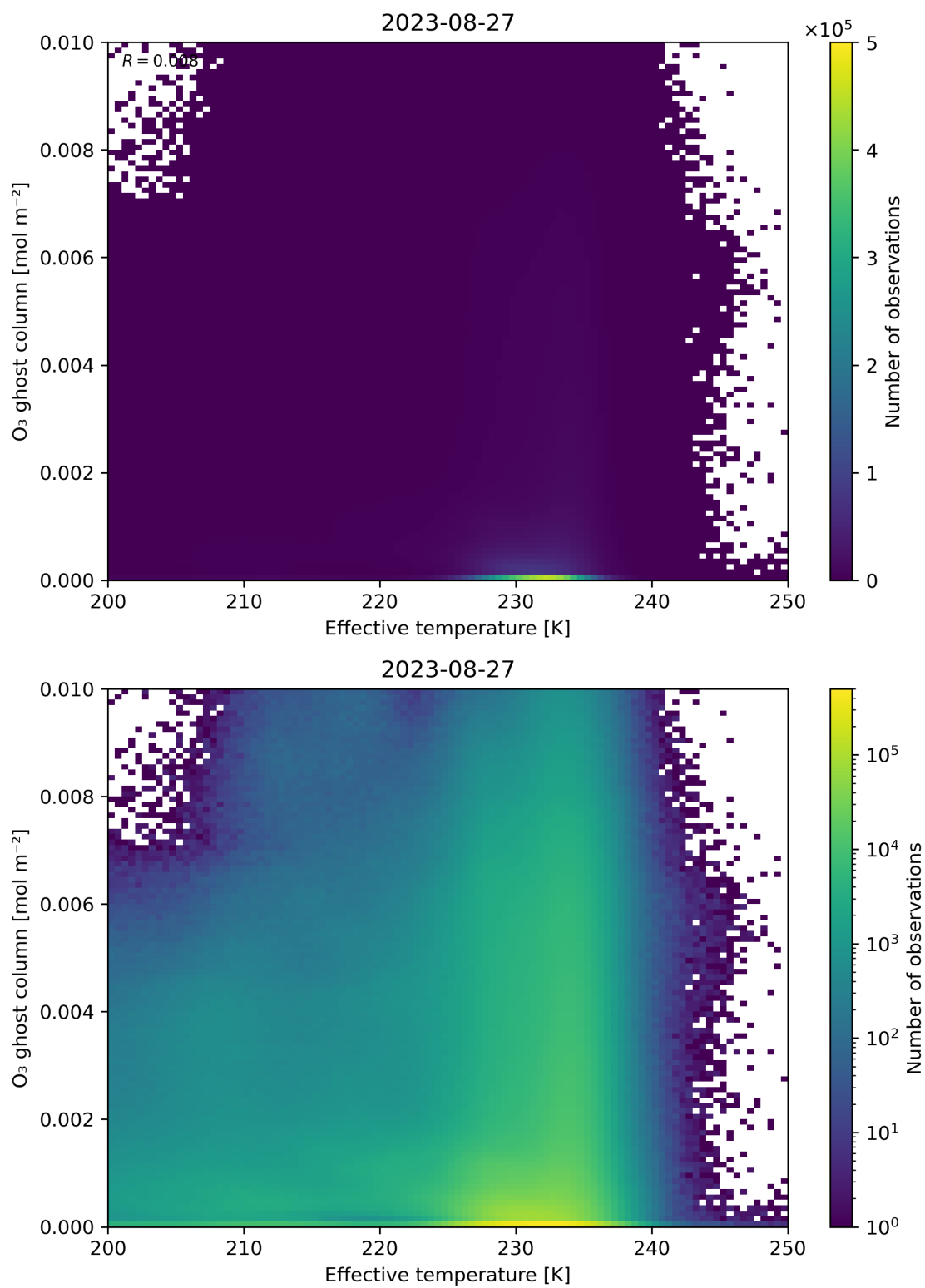
Figure 38: Scatter density plot of “Effective temperature” against “O 3 ghost column” for 2023-08-26 to 2023-08-28.
