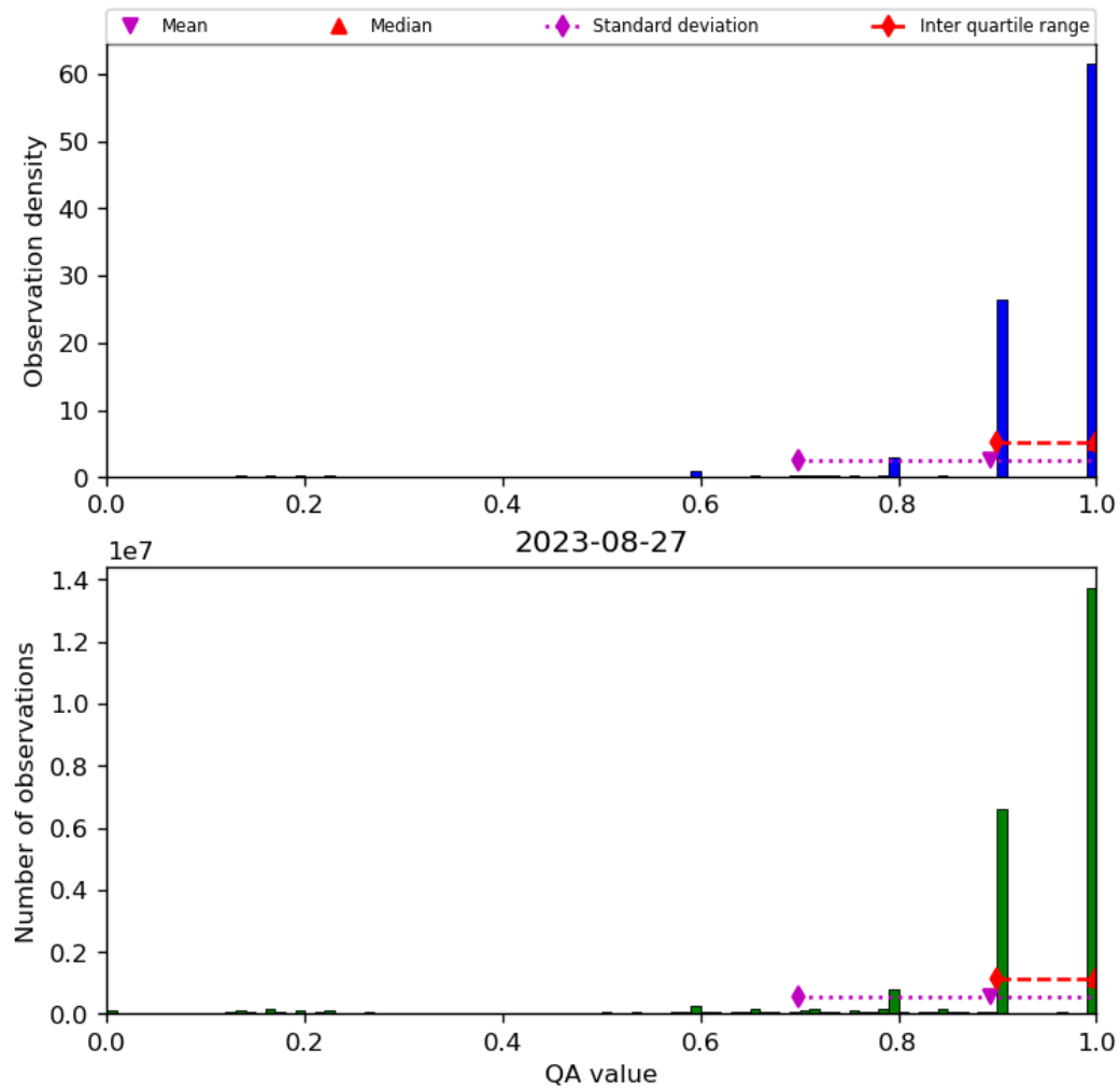
Figure 20: Histogram of “QA value” for 2023-08-26 to 2023-08-28
