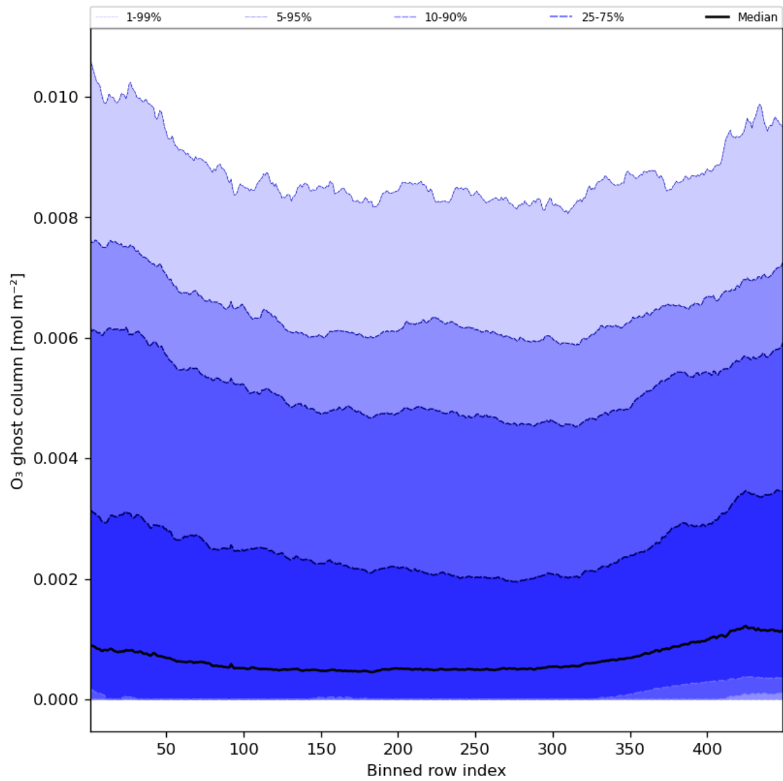
Figure 32: Along track statistics of “O 3 ghost column” for 2023-08-26 to 2023-08-28
