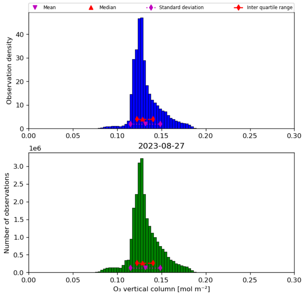
Figure 21: Histogram of “O 3 vertical column” for 2023-08-26 to 2023-08-28
