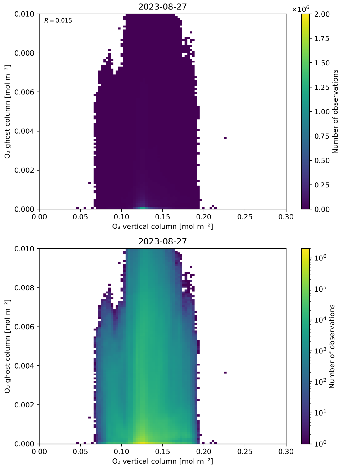
Figure 40: Scatter density plot of “O 3 vertical column” against “O 3 ghost column” for 2023-08-26 to 2023-08-28.
