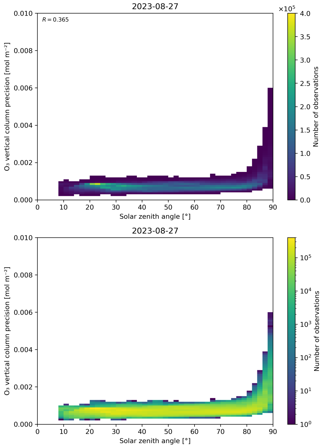
Figure 48: Scatter density plot of “Solar zenith angle” against “O 3 vertical column precision” for 2023-08-26 to 2023-08-28.
