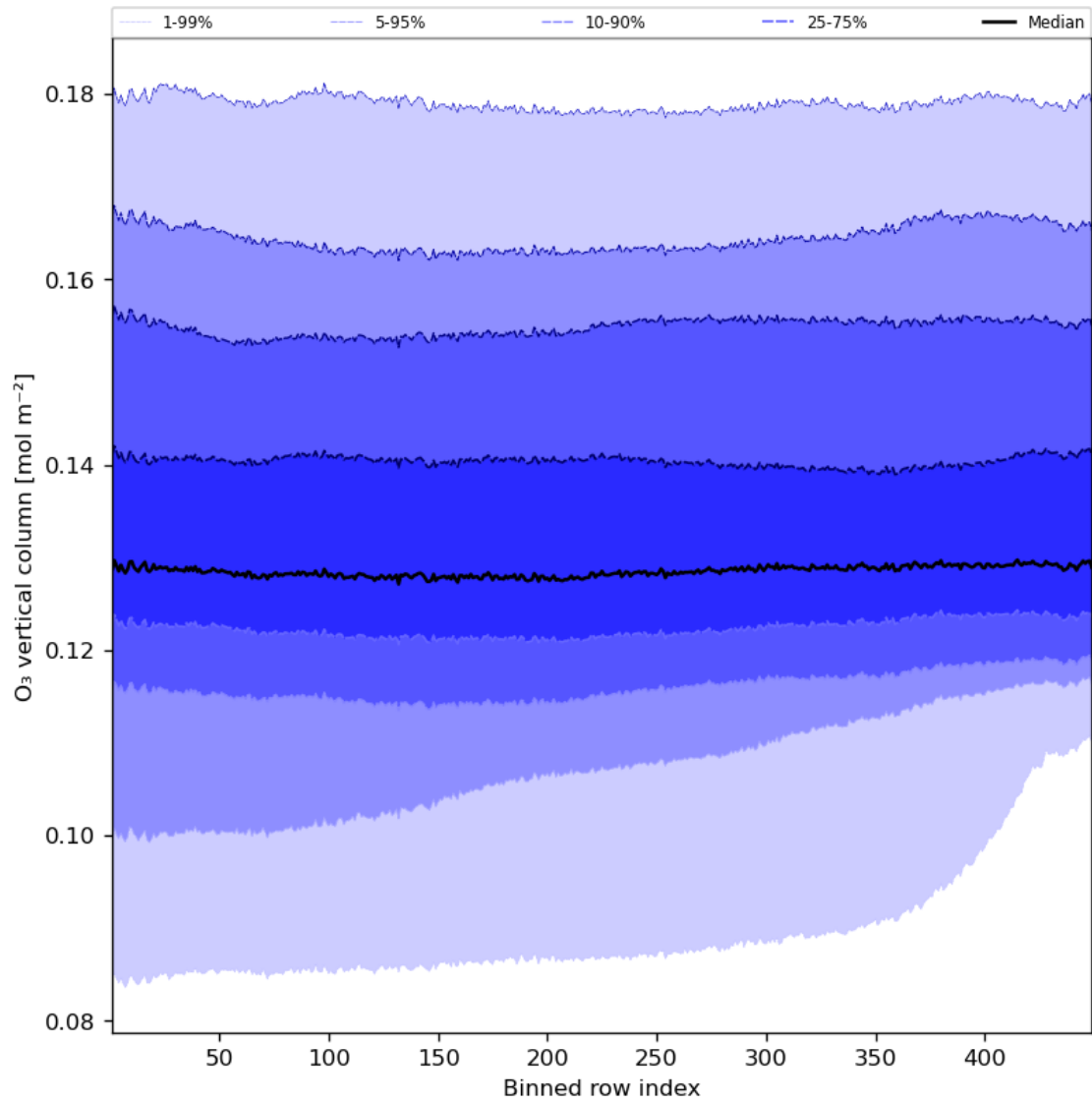
Figure 28: Along track statistics of “O 3 vertical column” for 2023-08-26 to 2023-08-28
