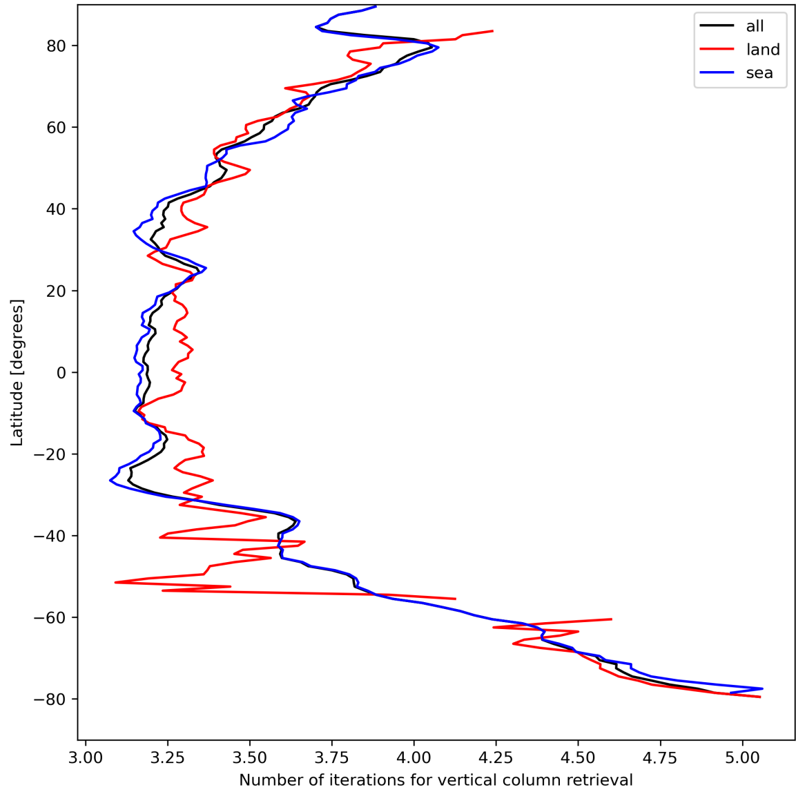
Figure 19: Zonal average of “Number of iterations for vertical column retrieval” for 2023-08-26 to 2023-08-28.
