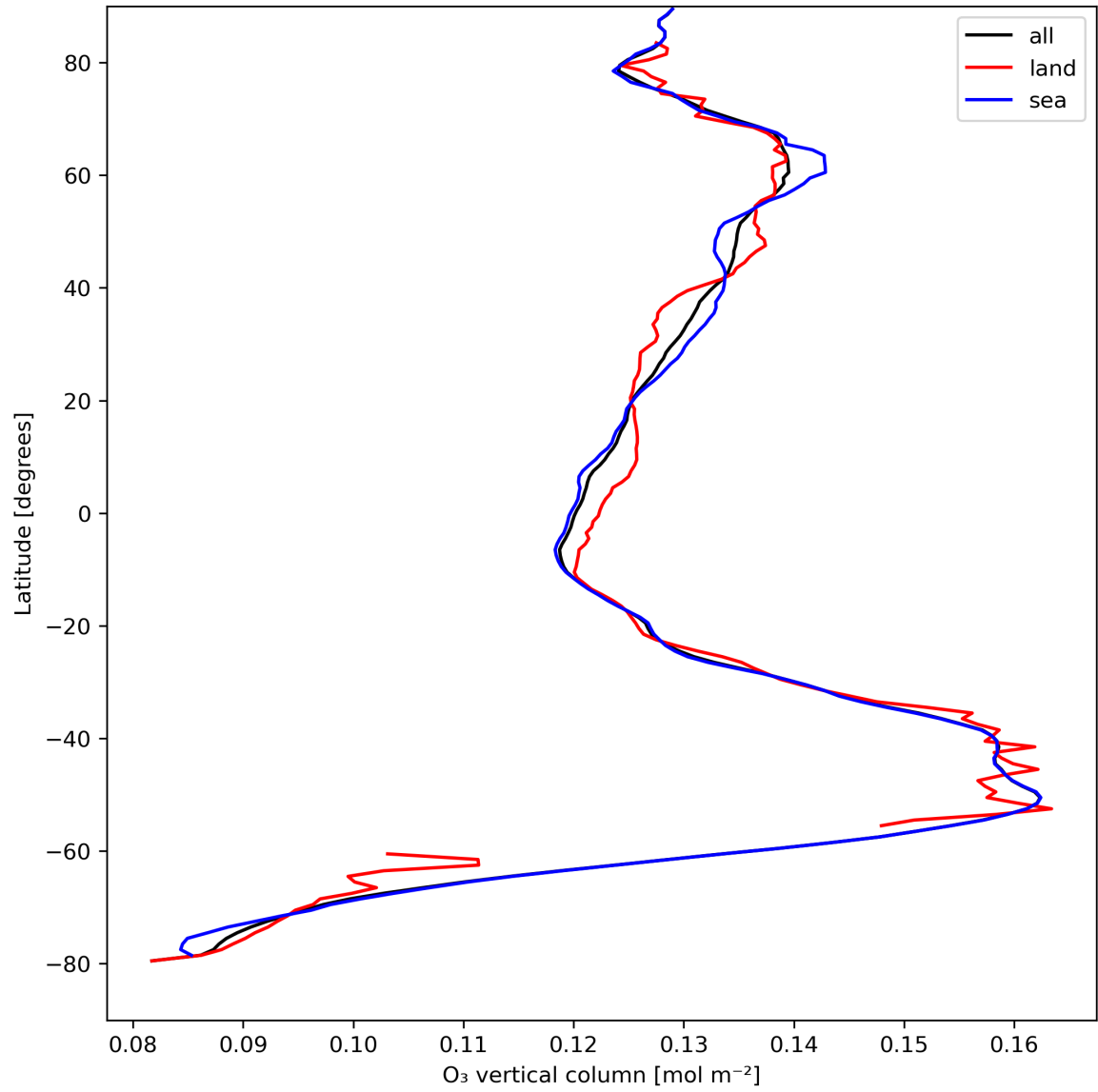
Figure 14: Zonal average of “O 3 vertical column” for 2023-08-26 to 2023-08-28.
