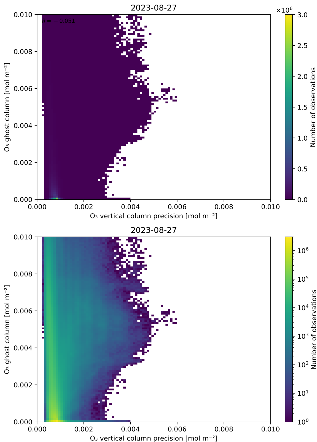
Figure 43: Scatter density plot of “ \text{O}_3 vertical column precision” against “ \text{O}_3 ghost column” for 2023-08-26 to 2023-08-28.
