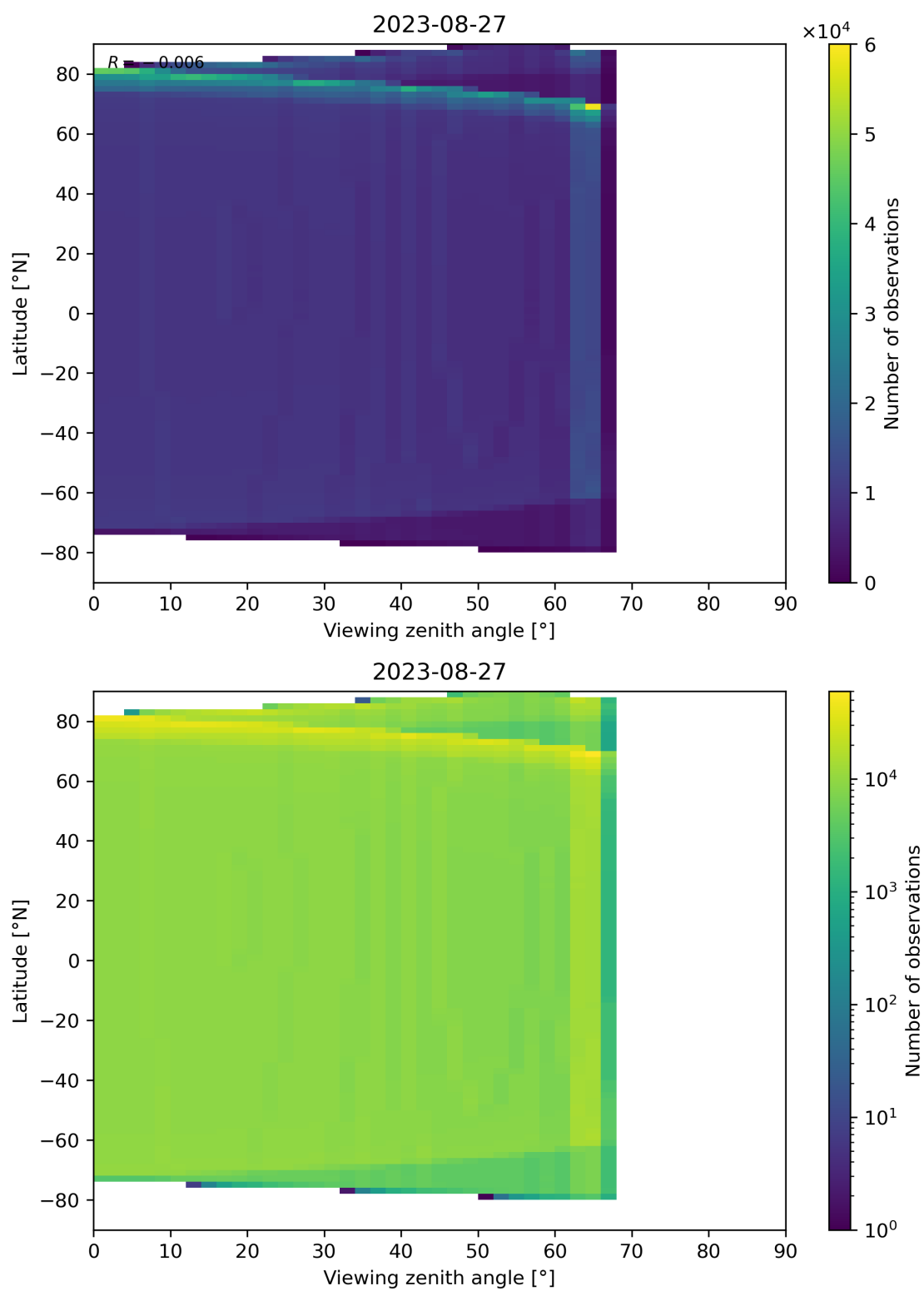
Figure 49: Scatter density plot of “Viewing zenith angle” against “Latitude” for 2023-08-26 to 2023-08-28.
