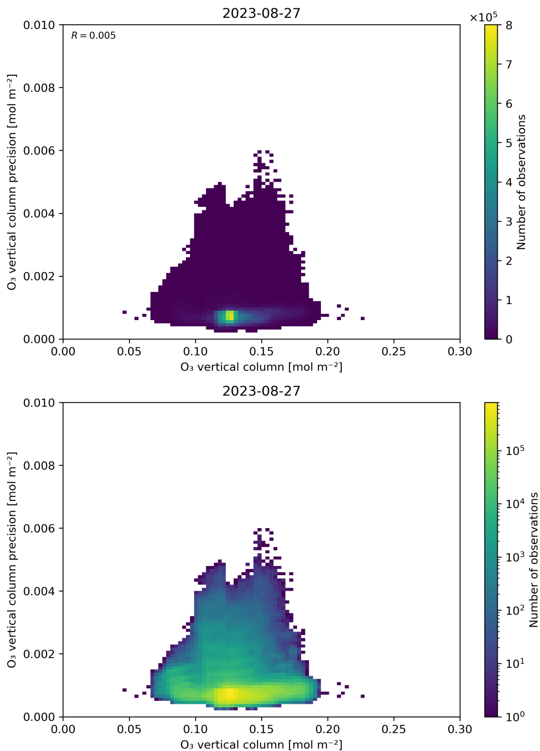
Figure 41: Scatter density plot of “O 3 vertical column” against “O 3 vertical column precision” for 2023-08-26 to 2023-08-28.
