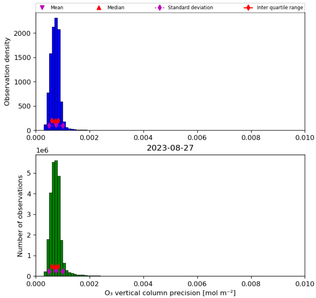
Figure 22: Histogram of “O 3 vertical column precision” for 2023-08-26 to 2023-08-28
