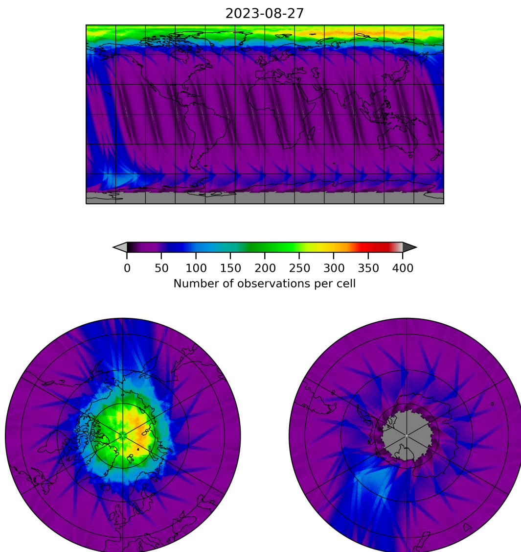
Figure 12: Map of the number of observations for 2023-08-26 to 2023-08-28
