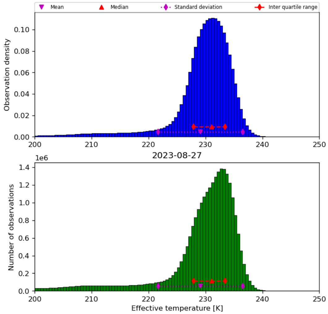
Figure 24: Histogram of “Effective temperature” for 2023-08-26 to 2023-08-28
