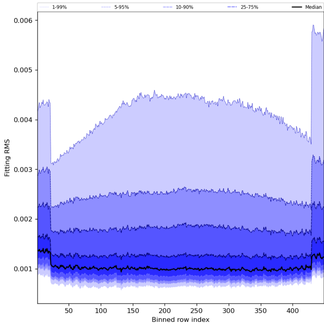
Figure 30: Along track statistics of “Fitting RMS” for 2023-08-26 to 2023-08-28
