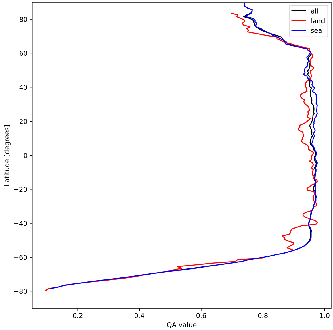
Figure 13: Zonal average of “QA value” for 2023-08-26 to 2023-08-28.
