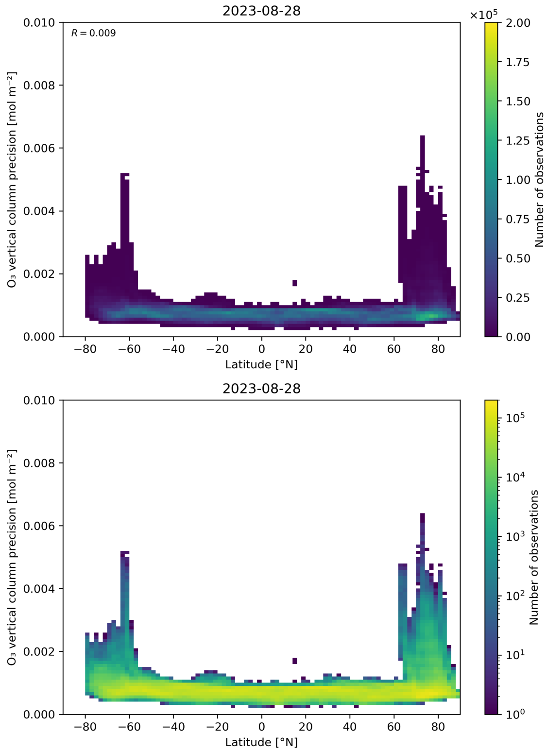
Figure 37: Scatter density plot of “Latitude” against “O 3 vertical column precision” for 2023-08-27 to 2023-08-29.
