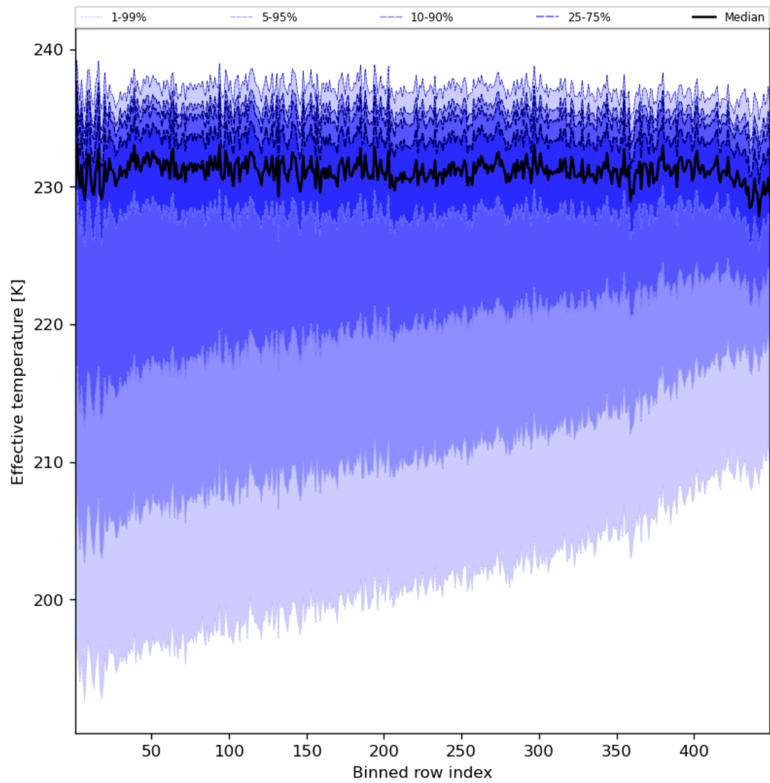
Figure 31: Along track statistics of “Effective temperature” for 2023-08-27 to 2023-08-29
