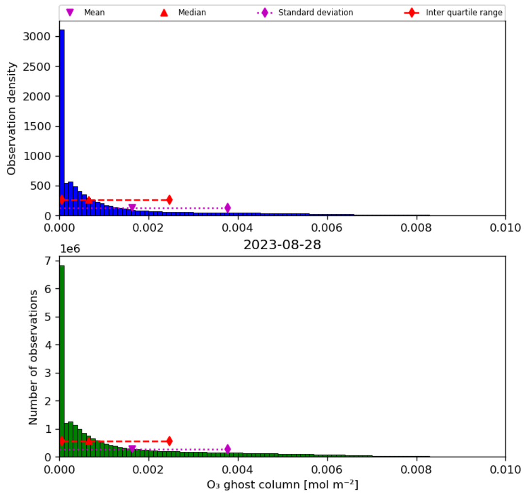
Figure 25: Histogram of “O 3 ghost column” for 2023-08-27 to 2023-08-29
