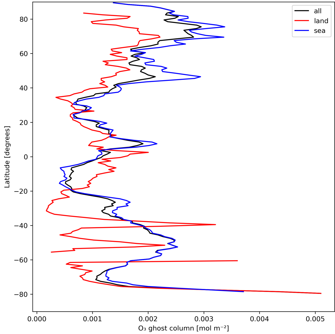
Figure 18: Zonal average of “O 3 ghost column” for 2023-08-27 to 2023-08-29.
