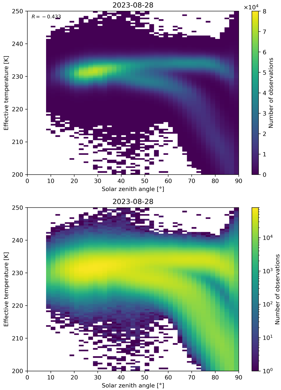
Figure 45: Scatter density plot of “Solar zenith angle” against “Effective temperature” for 2023-08-27 to 2023-08-29.
