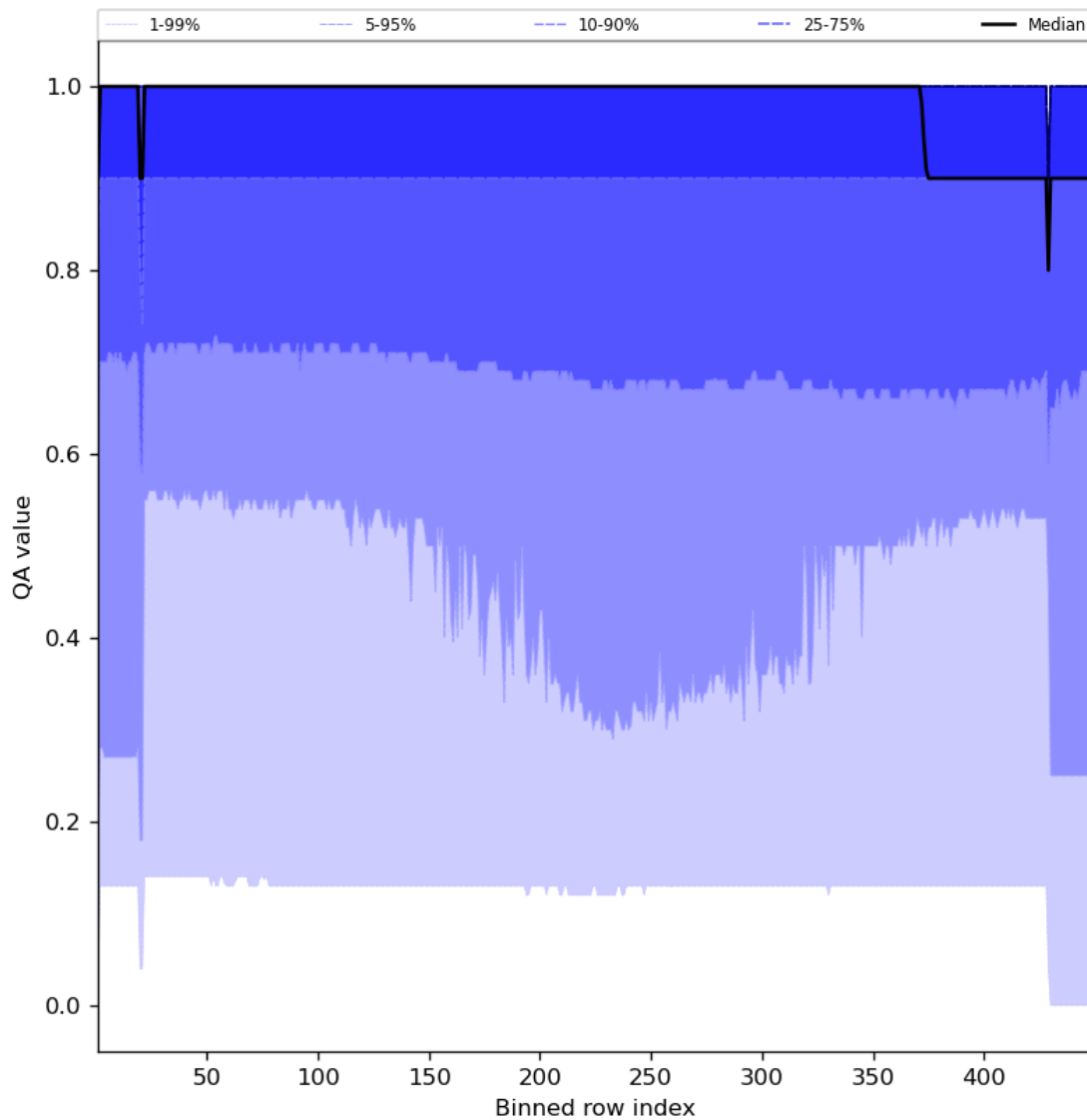
Figure 27: Along track statistics of “QA value” for 2023-08-27 to 2023-08-29
