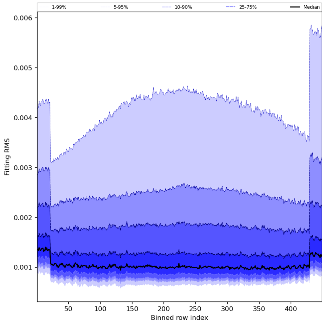
Figure 30: Along track statistics of “Fitting RMS” for 2023-08-27 to 2023-08-29
