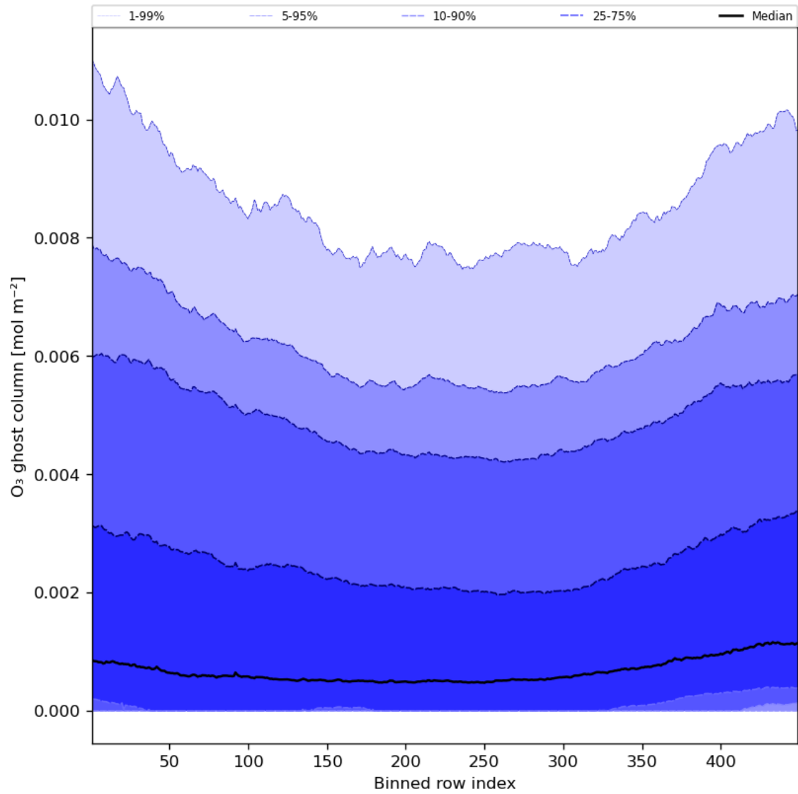
Figure 32: Along track statistics of “O 3 ghost column” for 2023-08-27 to 2023-08-29
