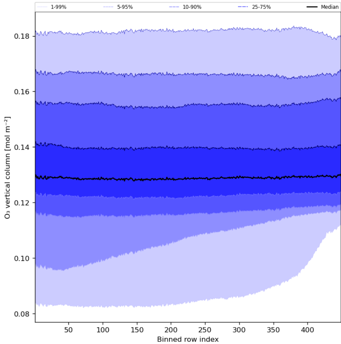
Figure 28: Along track statistics of “O 3 vertical column” for 2023-08-27 to 2023-08-29
