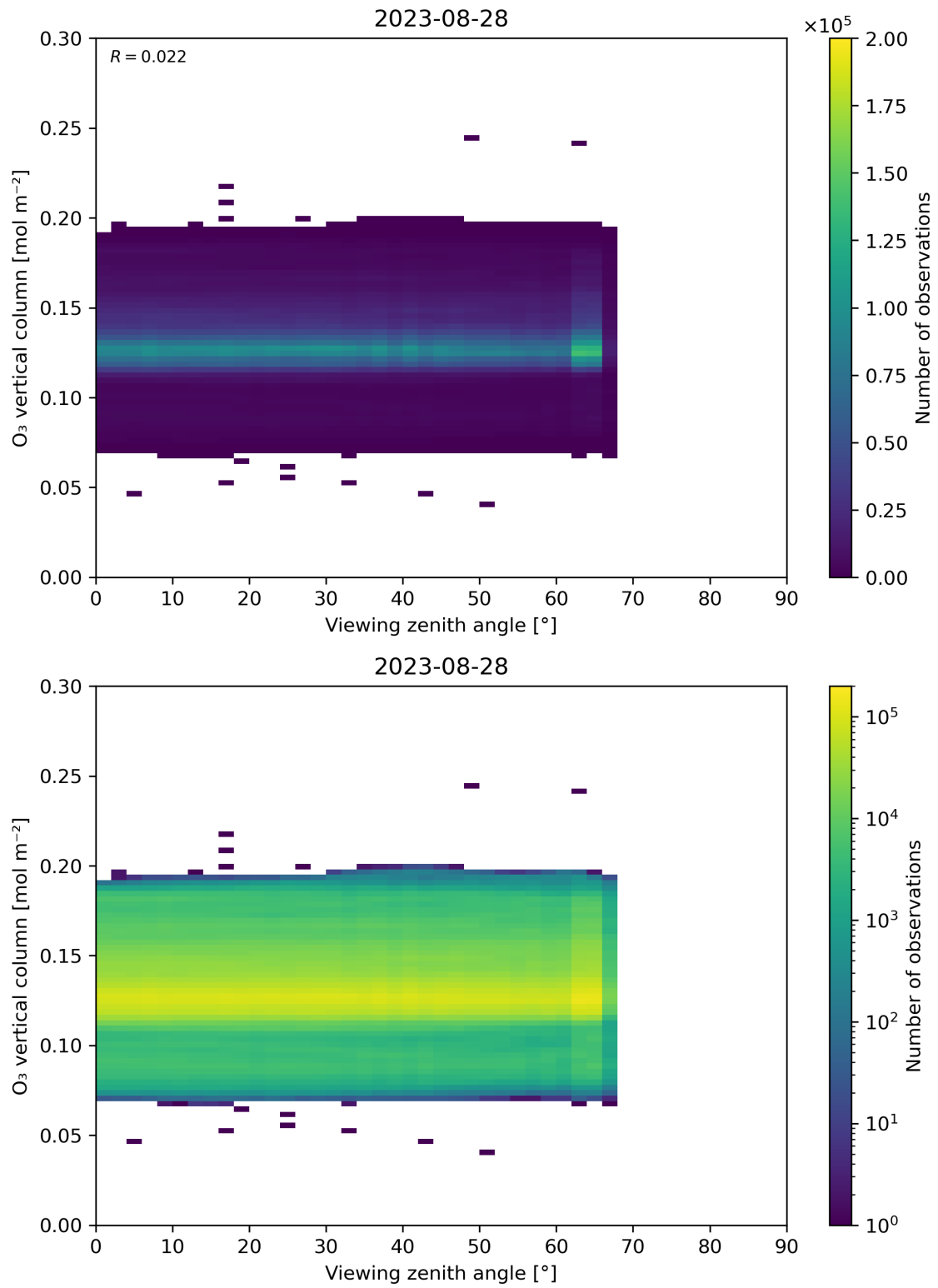
Figure 52: Scatter density plot of “Viewing zenith angle” against “O 3 vertical column” for 2023-08-27 to 2023-08-29.
