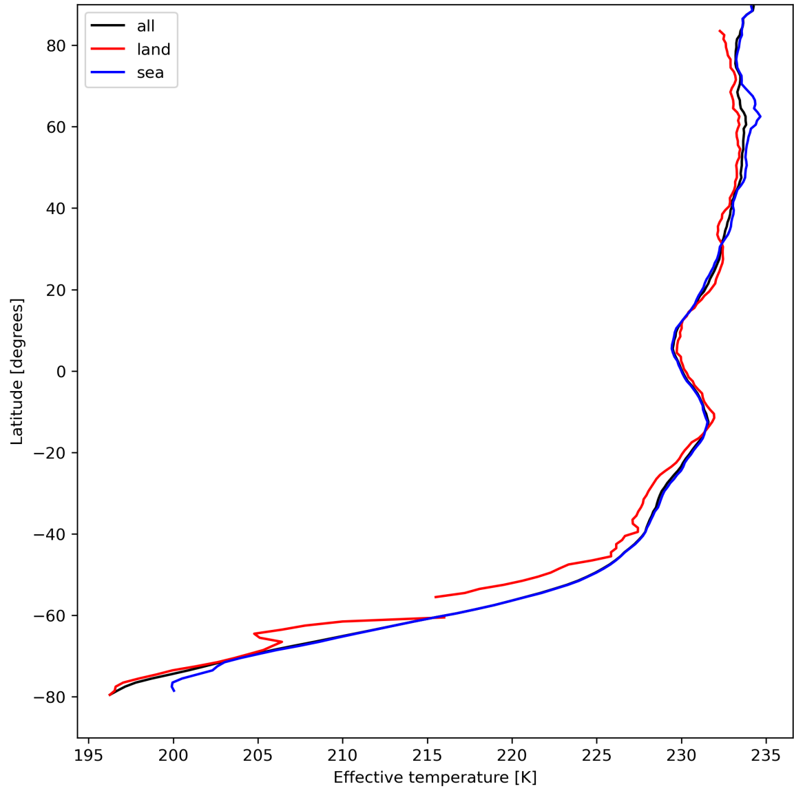
Figure 17: Zonal average of "Effective temperature" for 2023-08-27 to 2023-08-29.
