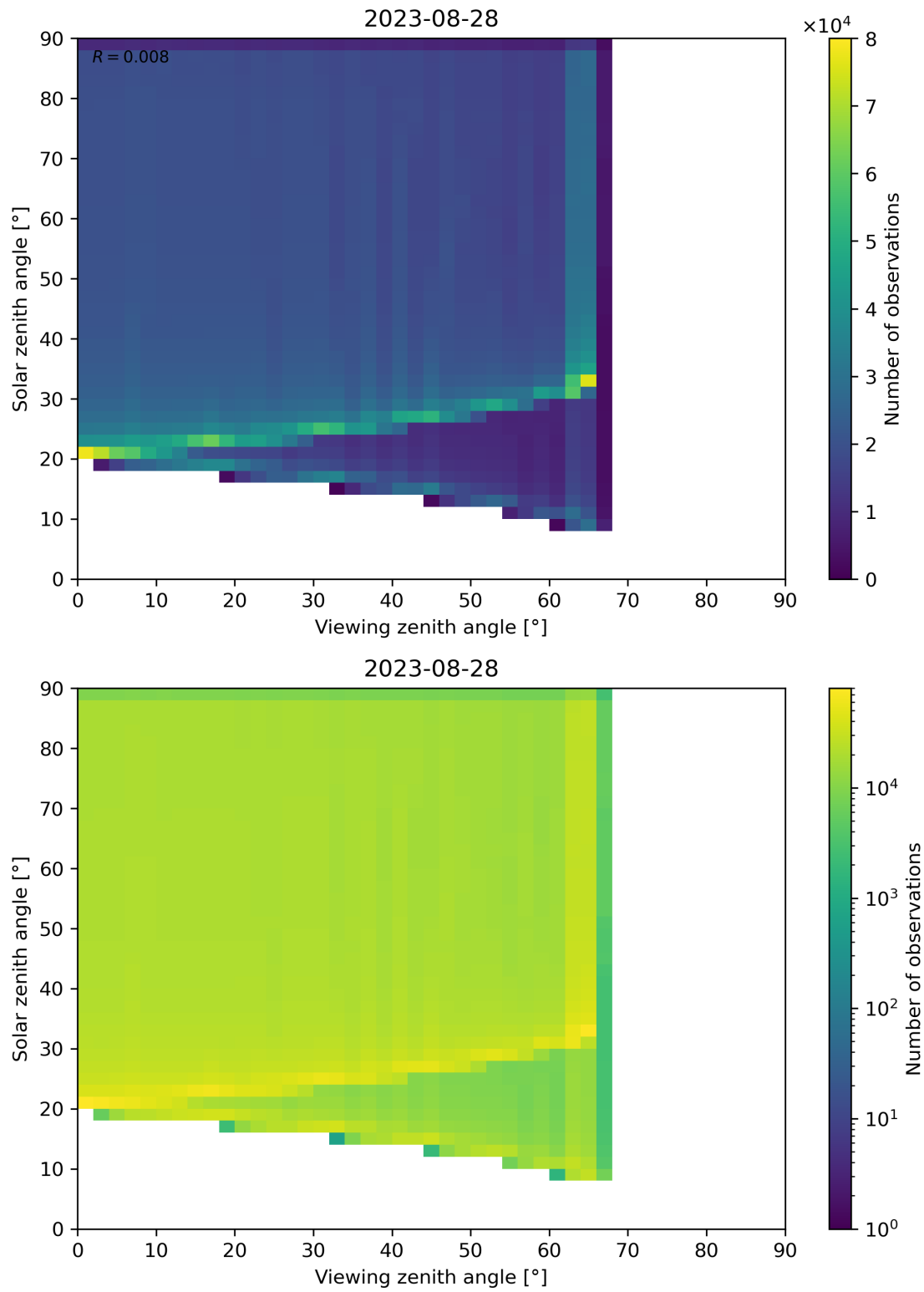
Figure 54: Scatter density plot of “Viewing zenith angle” against “Solar zenith angle” for 2023-08-27 to 2023-08-29.
