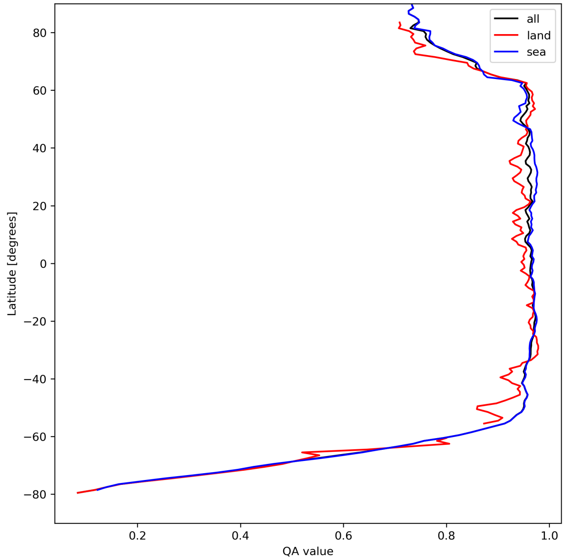
Figure 13: Zonal average of “QA value” for 2023-08-27 to 2023-08-29.
