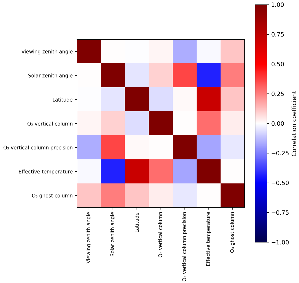
Figure 2: Map of correlation matrix for 2023-08-27 to 2023-08-29.
