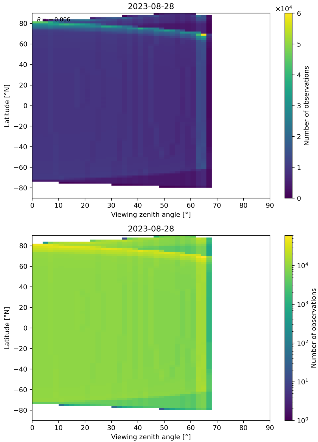
Figure 49: Scatter density plot of “Viewing zenith angle” against “Latitude” for 2023-08-27 to 2023-08-29.
