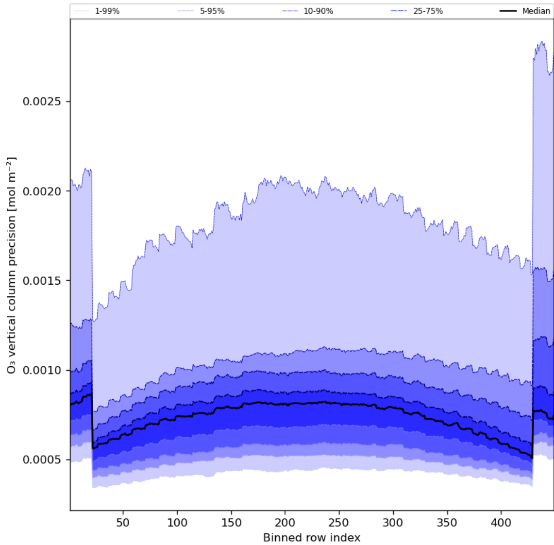
Figure 29: Along track statistics of “O 3 vertical column precision” for 2023-08-27 to 2023-08-29
