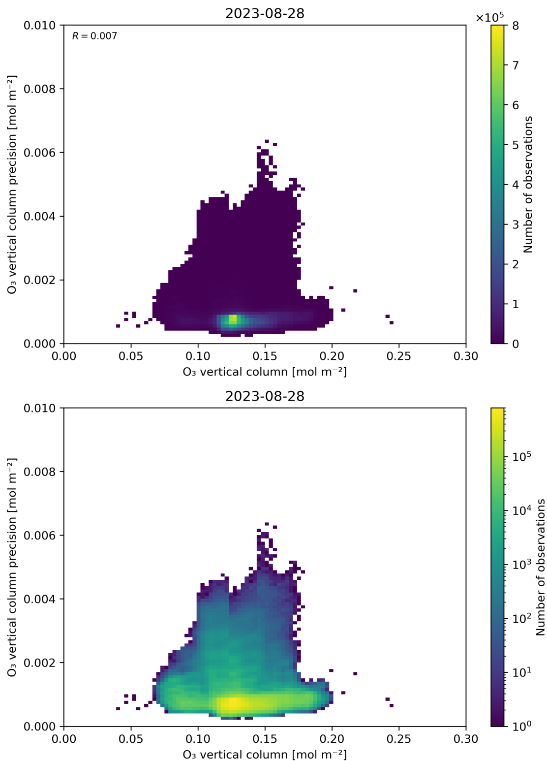
Figure 41: Scatter density plot of “O 3 vertical column” against “O 3 vertical column precision” for 2023-08-27 to 2023-08-29.
