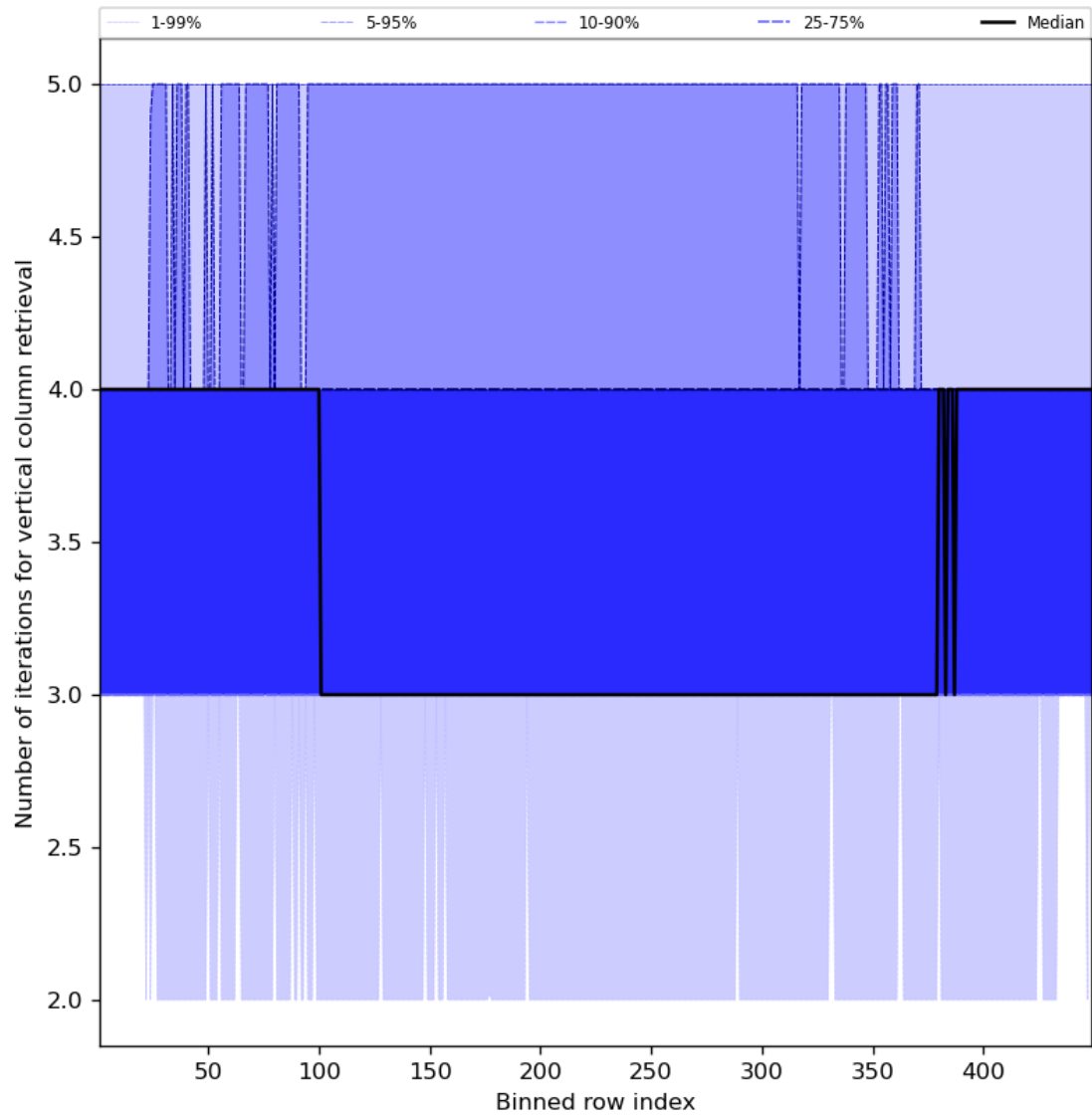
Figure 33: Along track statistics of “Number of iterations for vertical column retrieval” for 2023-08-27 to 2023-08-29
