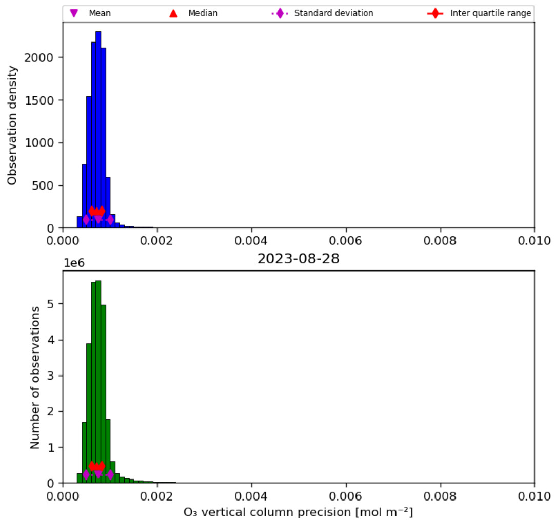
Figure 22: Histogram of “O 3 vertical column precision” for 2023-08-27 to 2023-08-29
