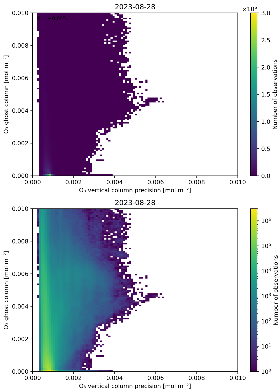
Figure 43: Scatter density plot of “ \text{O}_3 vertical column precision” against “ \text{O}_3 ghost column” for 2023-08-27 to 2023-08-29.
