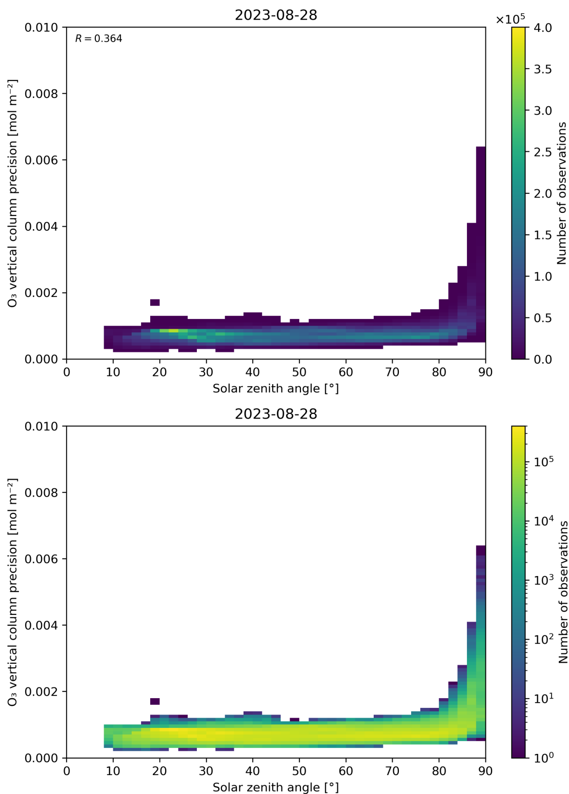
Figure 48: Scatter density plot of “Solar zenith angle” against “O 3 vertical column precision” for 2023-08-27 to 2023-08-29.
