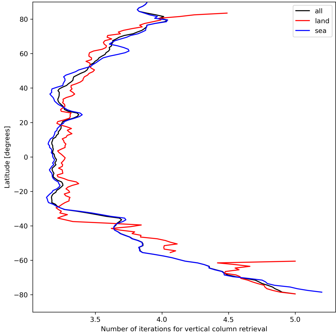
Figure 19: Zonal average of “Number of iterations for vertical column retrieval” for 2023-08-27 to 2023-08-29.
