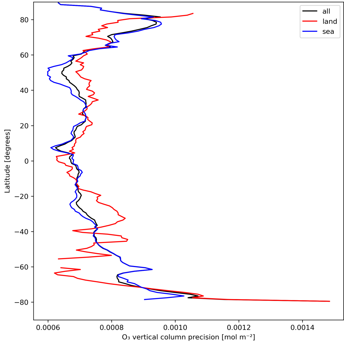
Figure 15: Zonal average of “O 3 vertical column precision” for 2023-08-27 to 2023-08-29.
