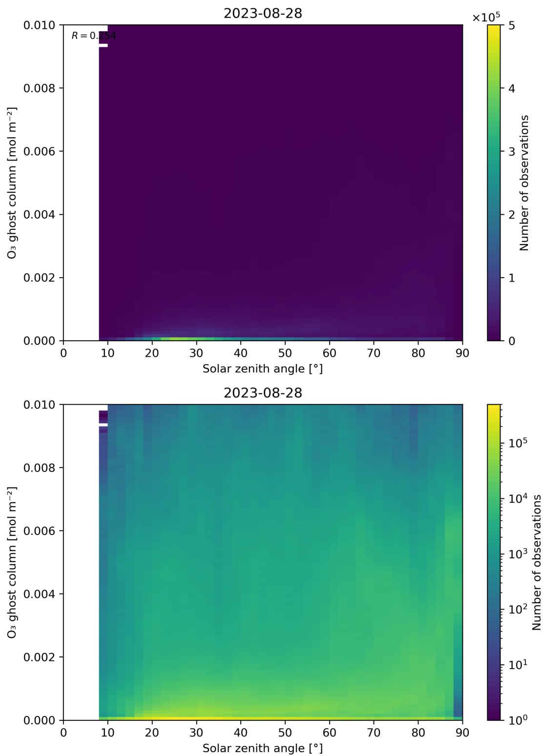
Figure 46: Scatter density plot of “Solar zenith angle” against “O 3 ghost column” for 2023-08-27 to 2023-08-29.
