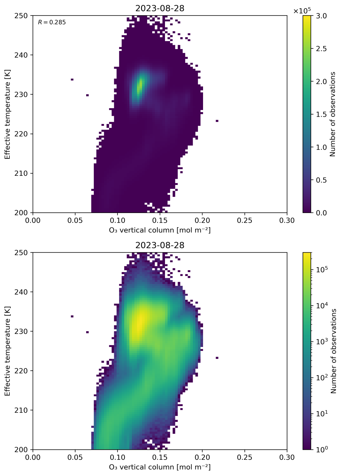
Figure 39: Scatter density plot of “O 3 vertical column” against “Effective temperature” for 2023-08-27 to 2023-08-29.
