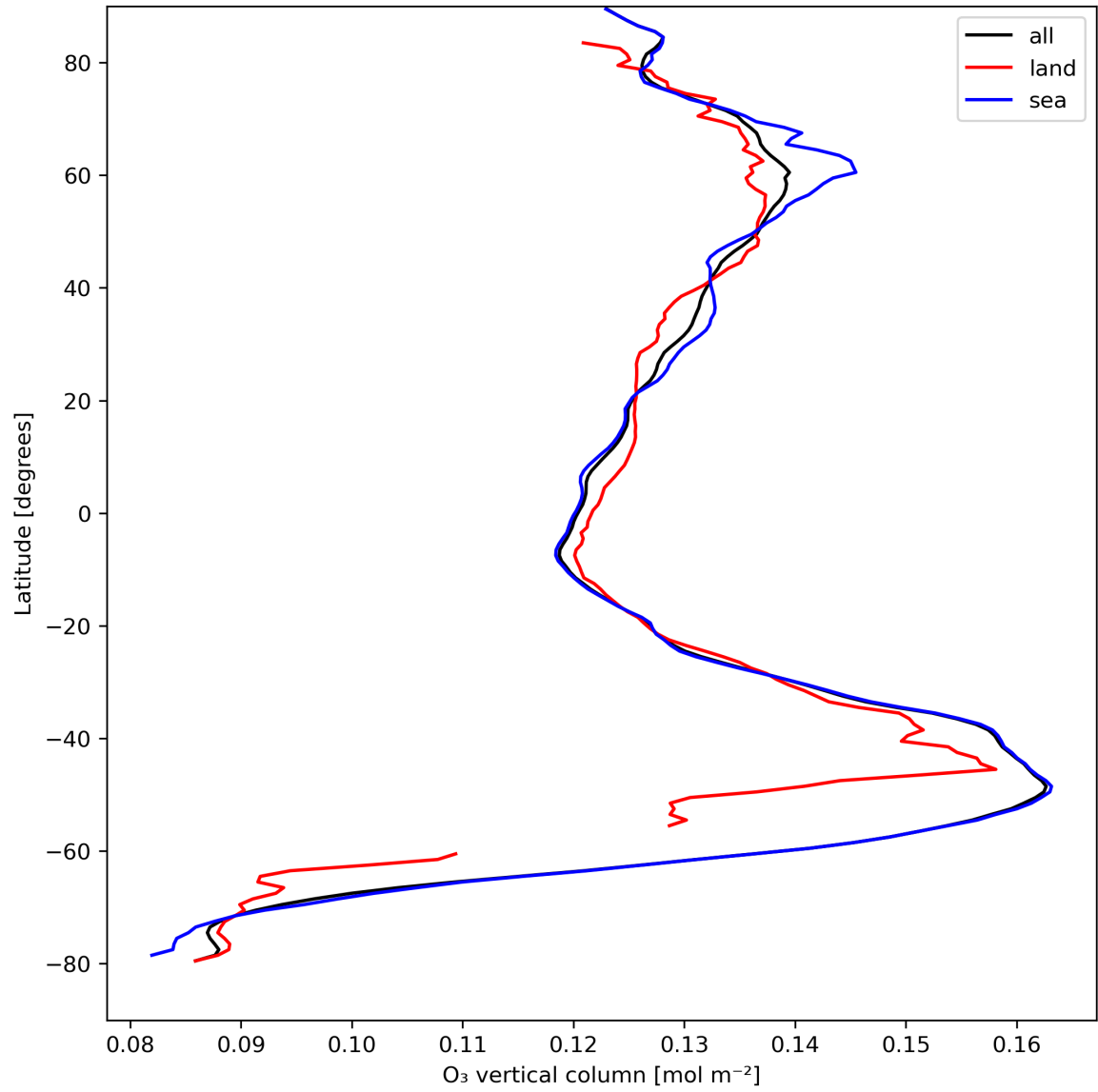
Figure 14: Zonal average of “O 3 vertical column” for 2023-08-27 to 2023-08-29.
