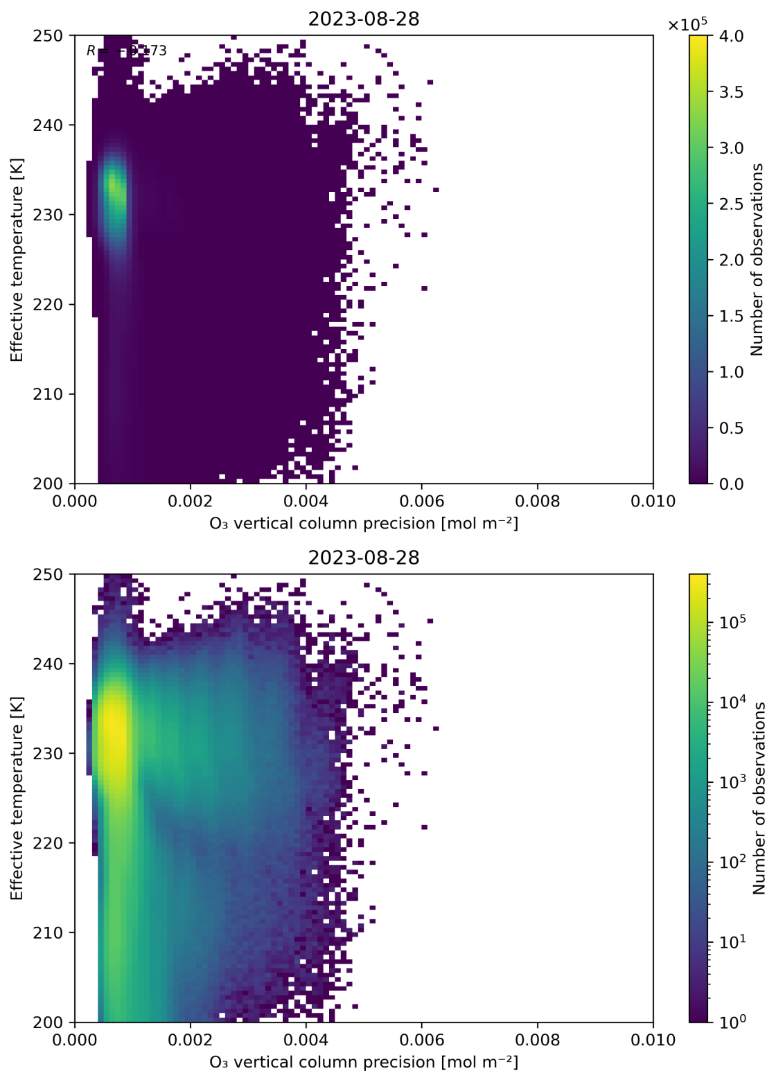
Figure 42: Scatter density plot of “O 3 vertical column precision” against “Effective temperature” for 2023-08-27 to 2023-08-29.
