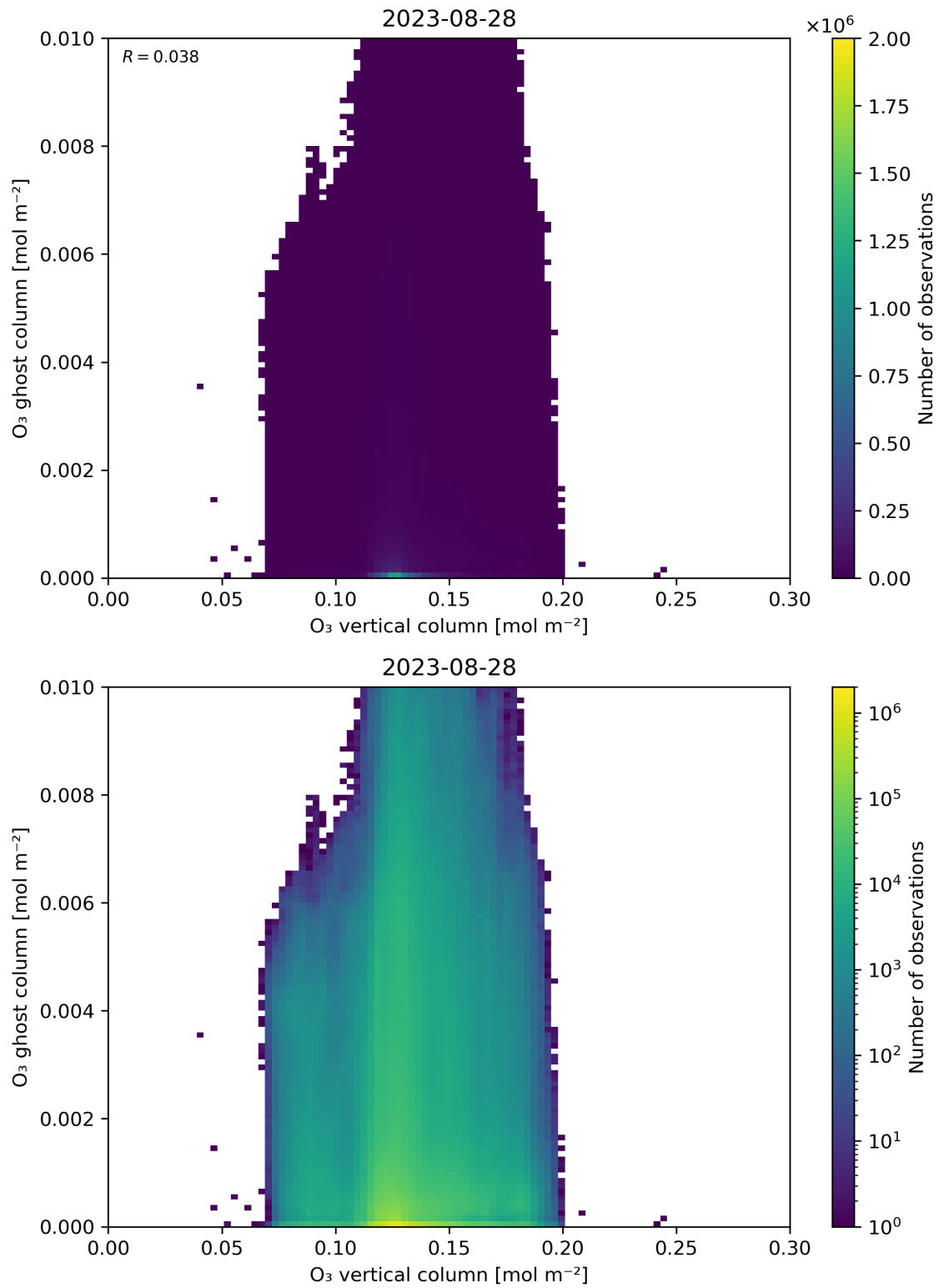
Figure 40: Scatter density plot of “O 3 vertical column” against “O 3 ghost column” for 2023-08-27 to 2023-08-29.
