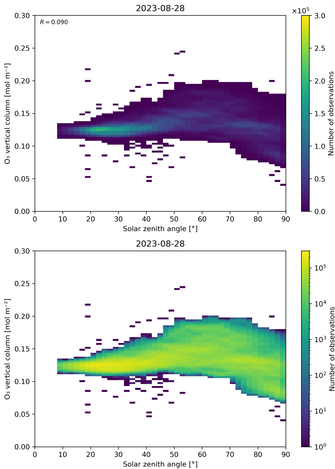
Figure 47: Scatter density plot of “Solar zenith angle” against “O 3 vertical column” for 2023-08-27 to 2023-08-29.
