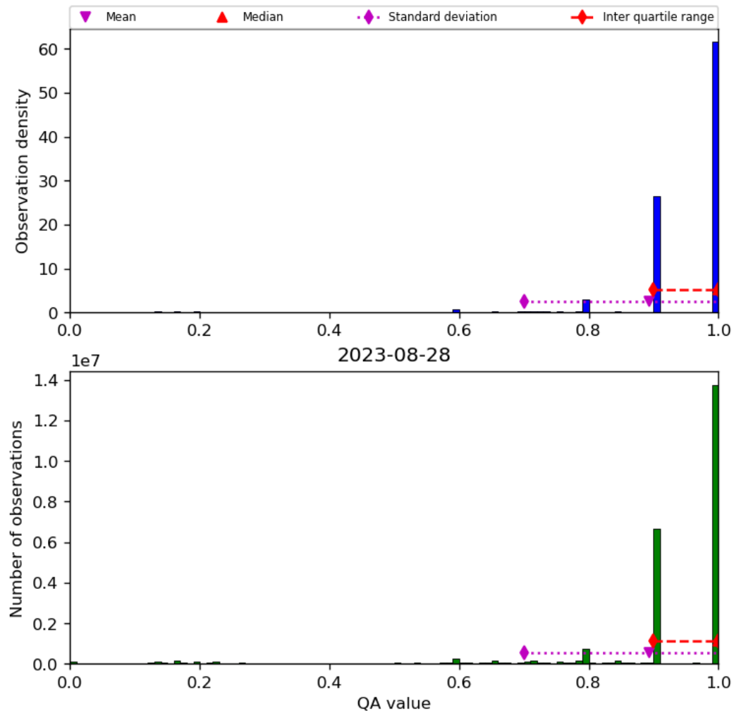
Figure 20: Histogram of “QA value” for 2023-08-27 to 2023-08-29
