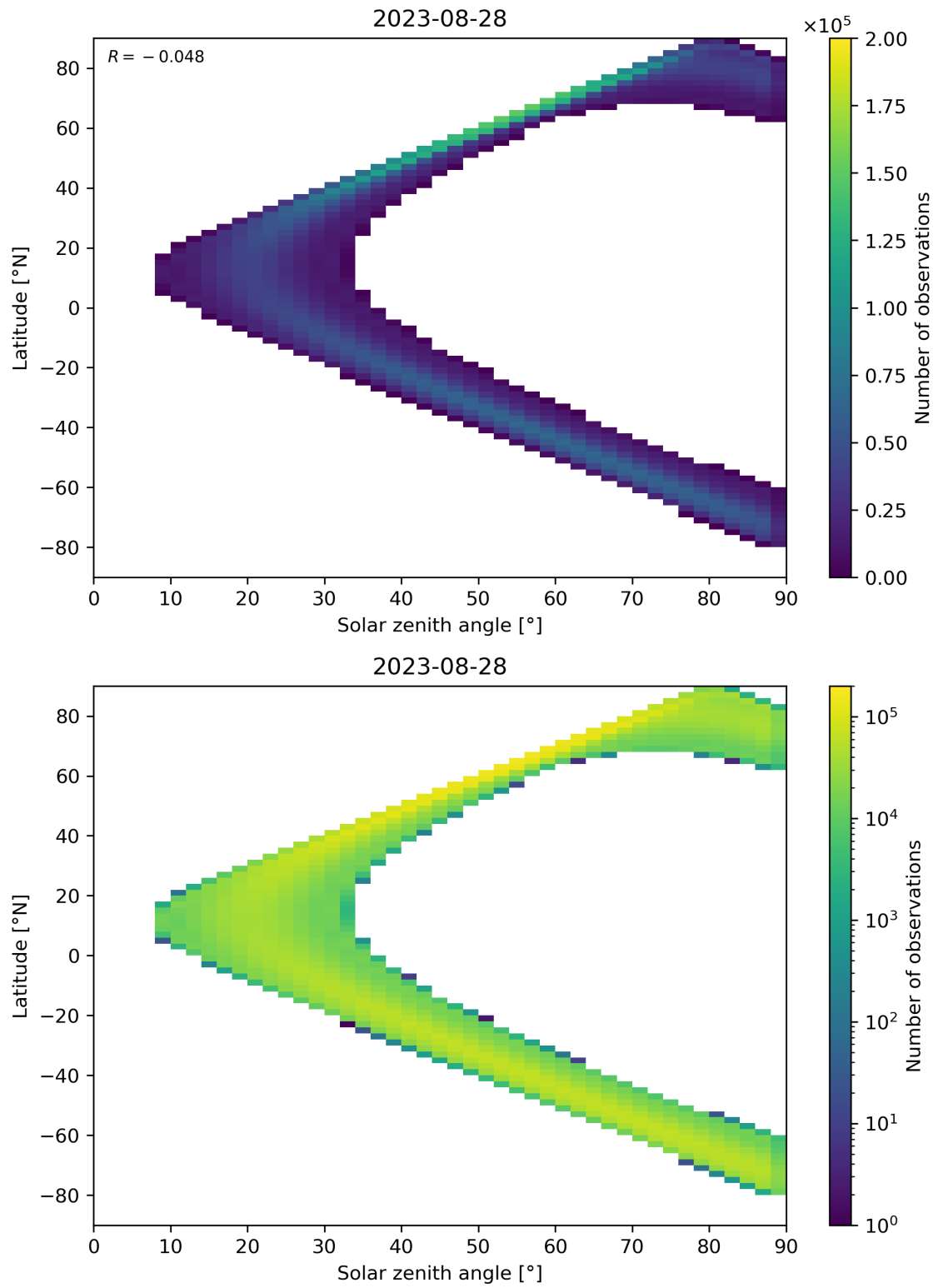
Figure 44: Scatter density plot of “Solar zenith angle” against “Latitude” for 2023-08-27 to 2023-08-29.
