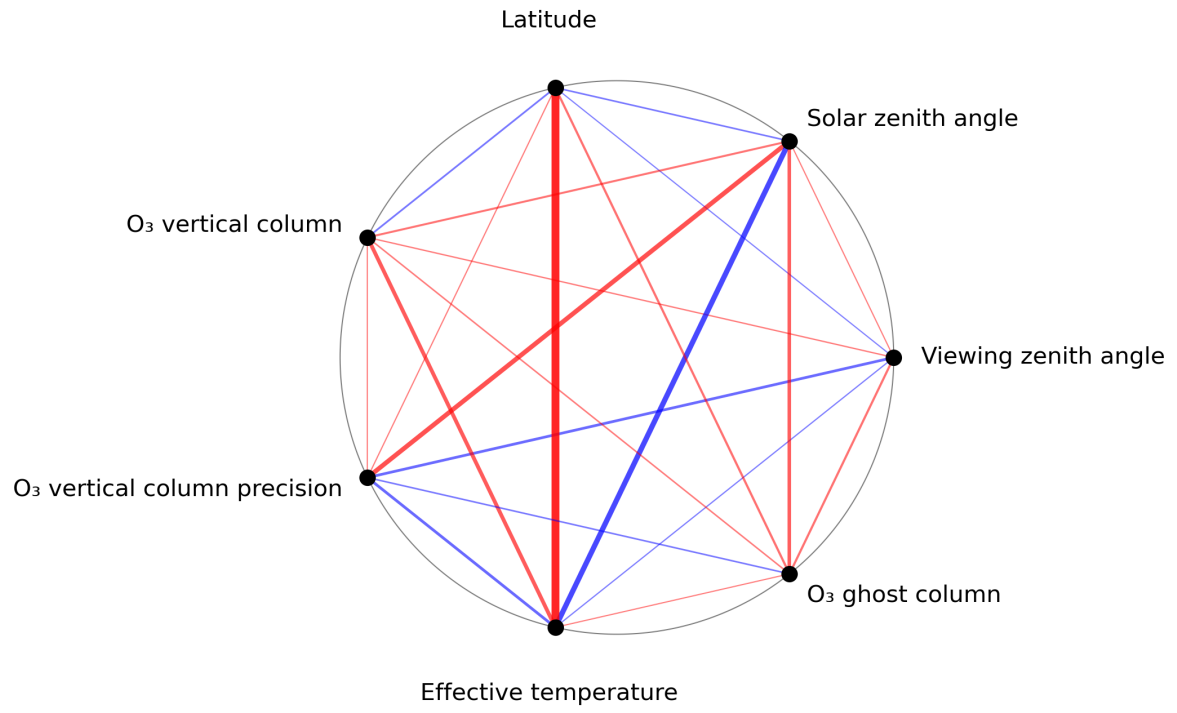
Figure 1: Map of correlation graph for 2023-08-27 to 2023-08-29.
