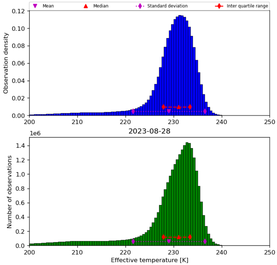
Figure 24: Histogram of “Effective temperature” for 2023-08-27 to 2023-08-29
