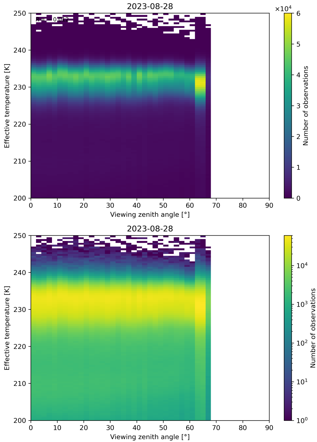
Figure 50: Scatter density plot of “Viewing zenith angle” against “Effective temperature” for 2023-08-27 to 2023-08-29.
