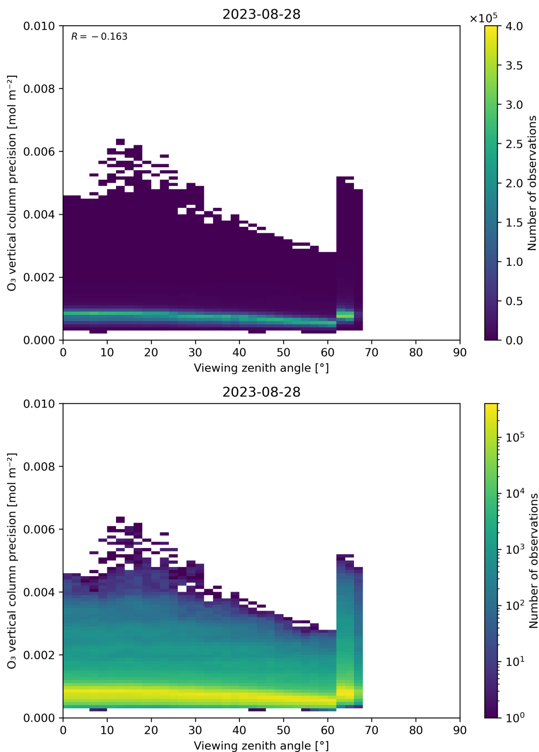
Figure 53: Scatter density plot of “Viewing zenith angle” against “O 3 vertical column precision” for 2023-08-27 to 2023-08-29.
