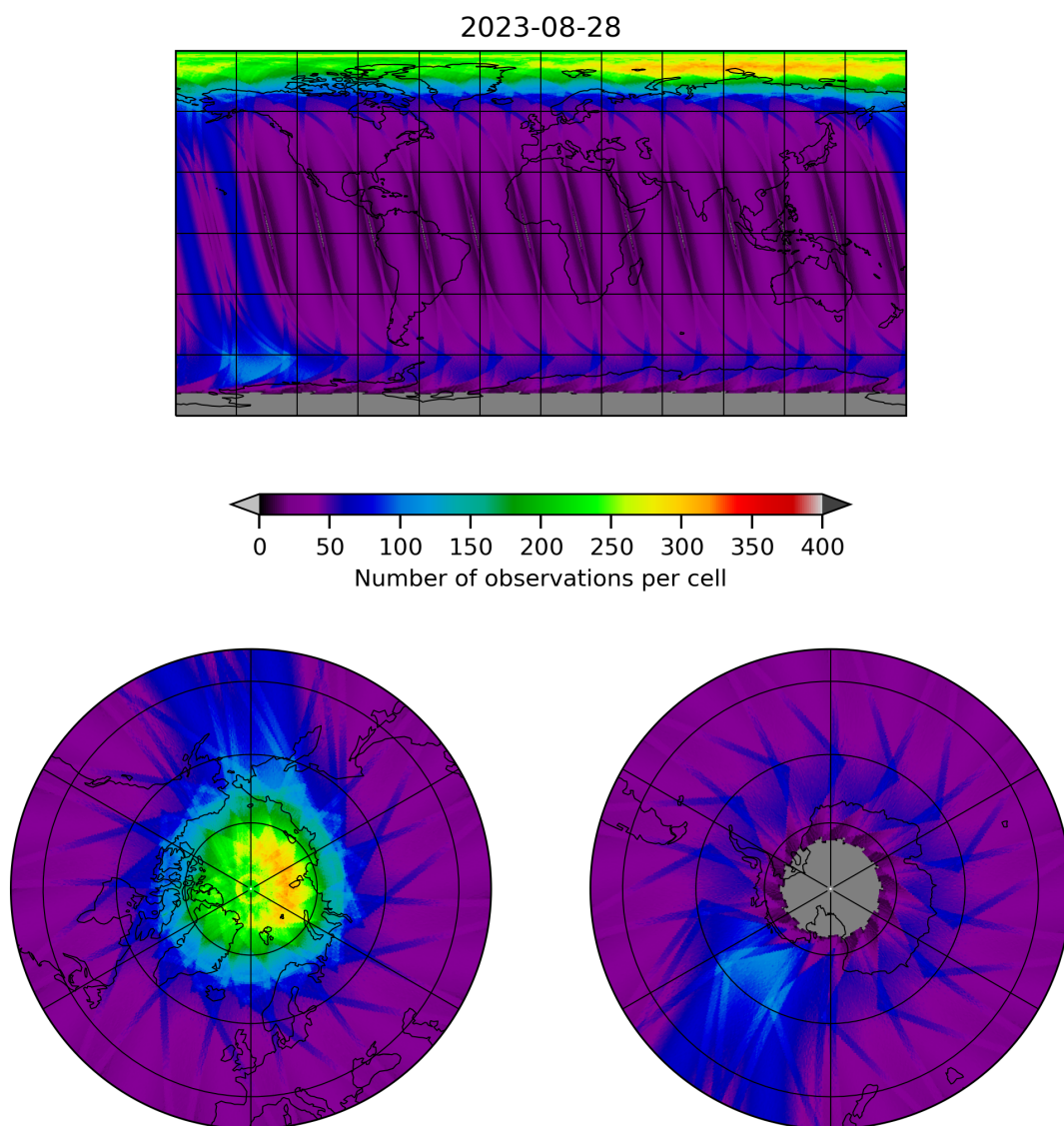
Figure 12: Map of the number of observations for 2023-08-27 to 2023-08-29
