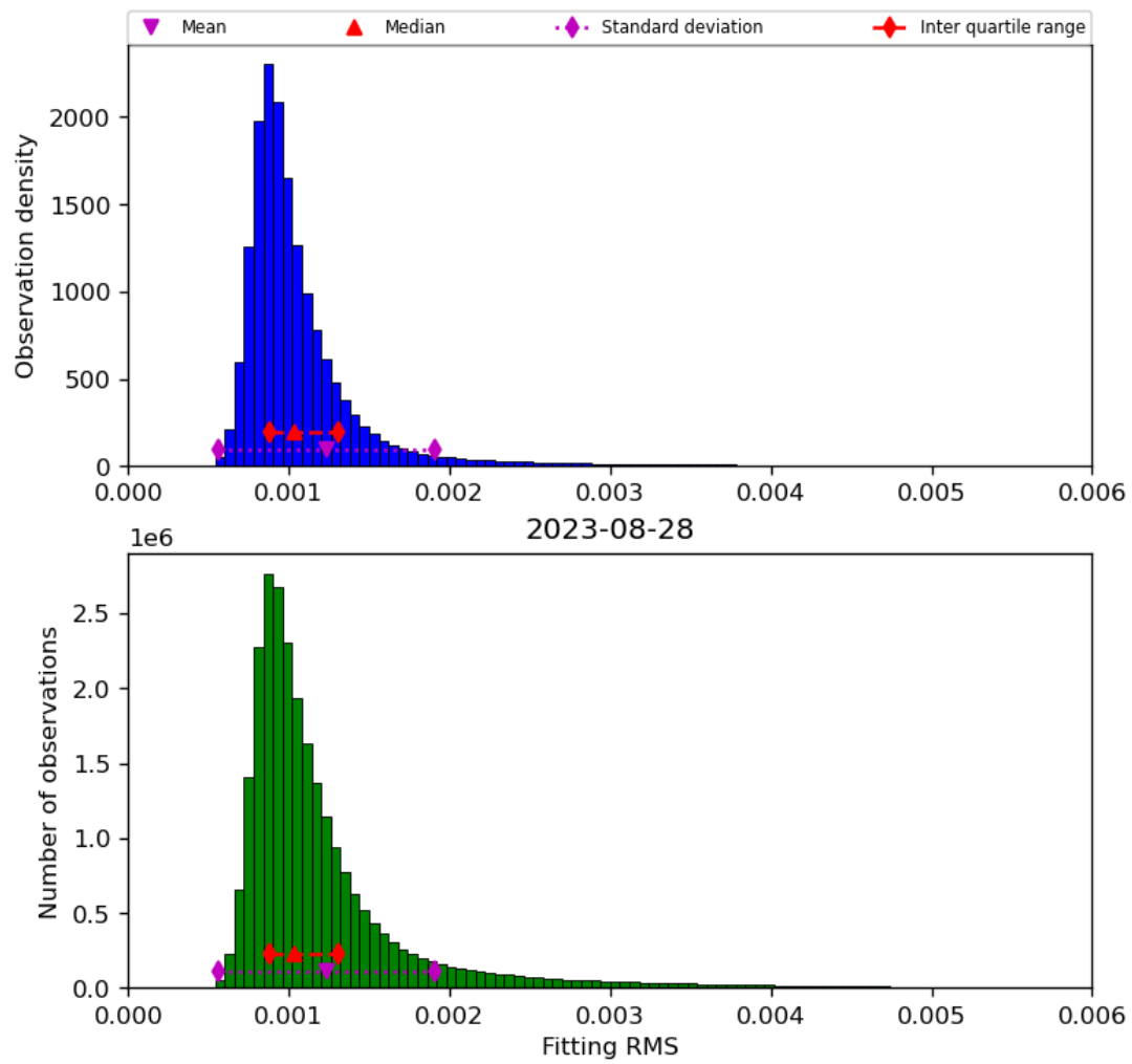
Figure 23: Histogram of “Fitting RMS” for 2023-08-27 to 2023-08-29
