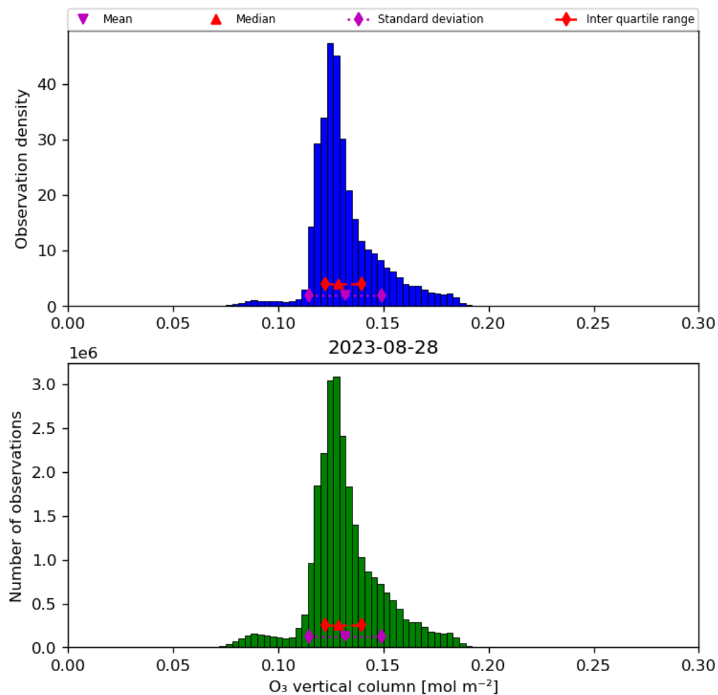
Figure 21: Histogram of “O 3 vertical column” for 2023-08-27 to 2023-08-29
