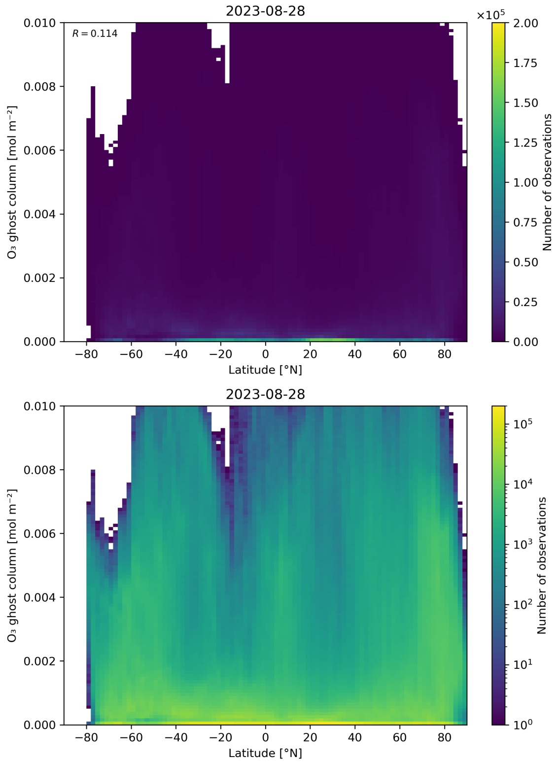
Figure 35: Scatter density plot of “Latitude” against “O 3 ghost column” for 2023-08-27 to 2023-08-29.
