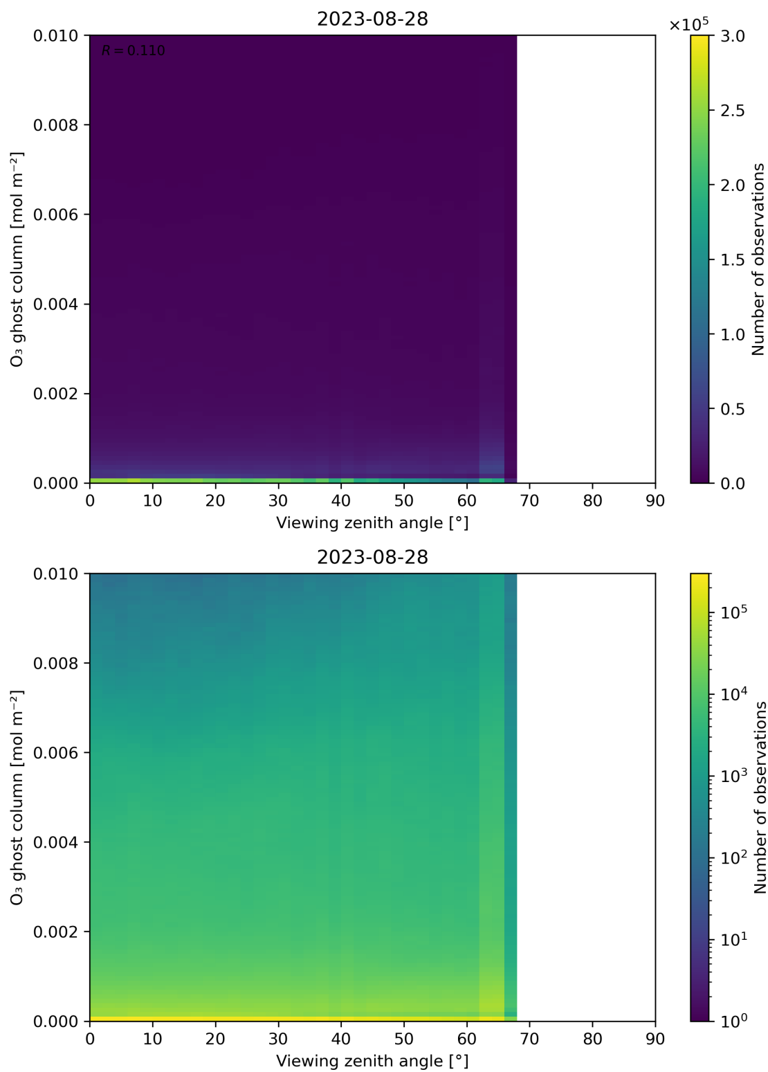
Figure 51: Scatter density plot of “Viewing zenith angle” against “O 3 ghost column” for 2023-08-27 to 2023-08-29.
