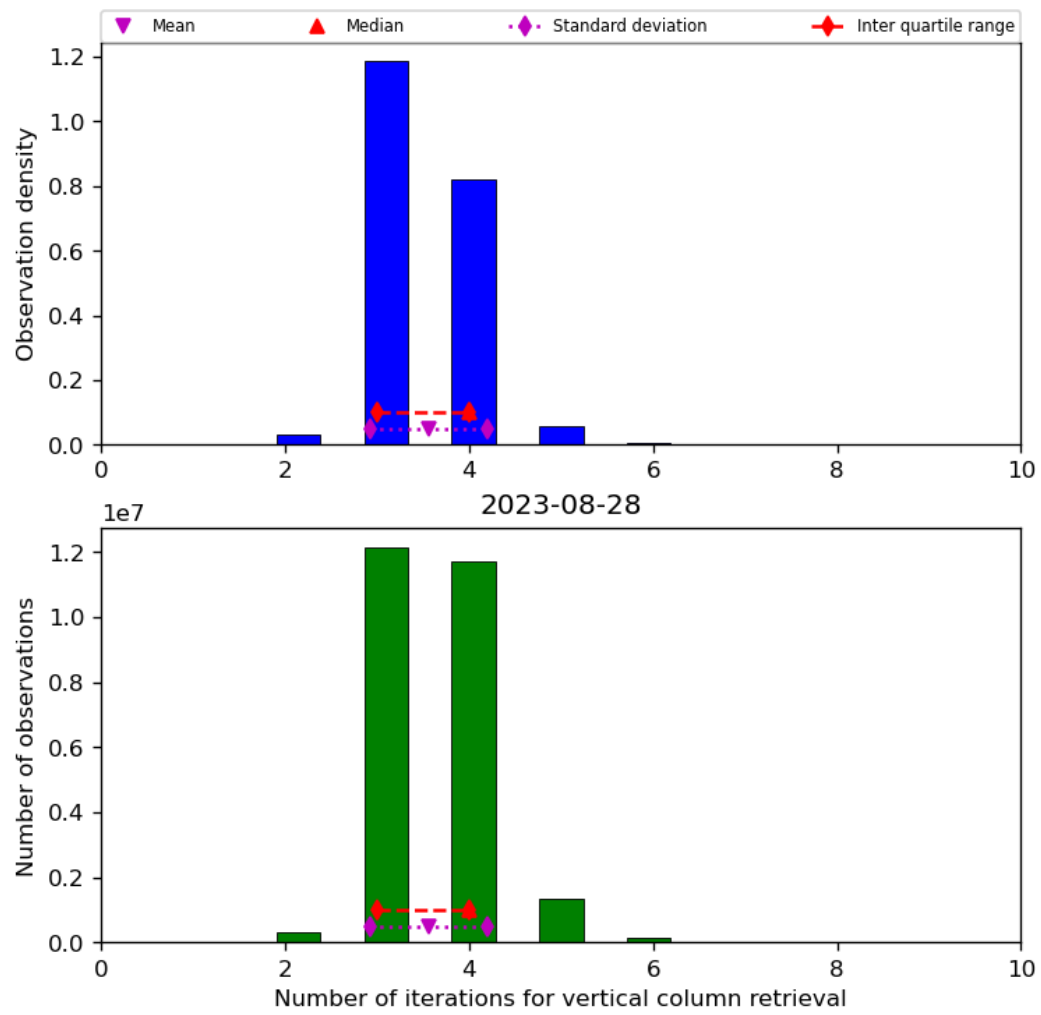
Figure 26: Histogram of “Number of iterations for vertical column retrieval” for 2023-08-27 to 2023-08-29
