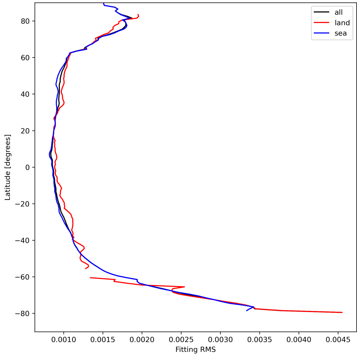
Figure 16: Zonal average of “Fitting RMS” for 2023-08-27 to 2023-08-29.
