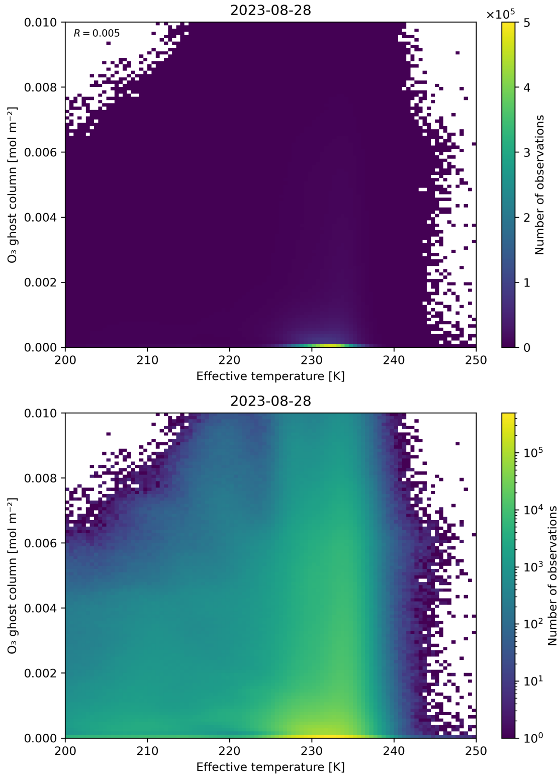
Figure 38: Scatter density plot of “Effective temperature” against “O 3 ghost column” for 2023-08-27 to 2023-08-29.
