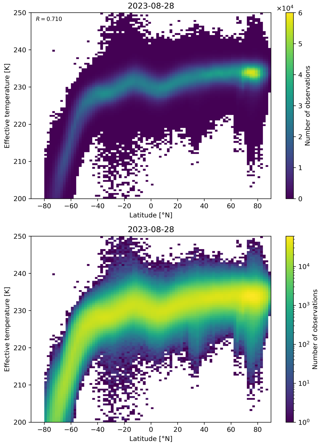
Figure 34: Scatter density plot of “Latitude” against “Effective temperature” for 2023-08-27 to 2023-08-29.
