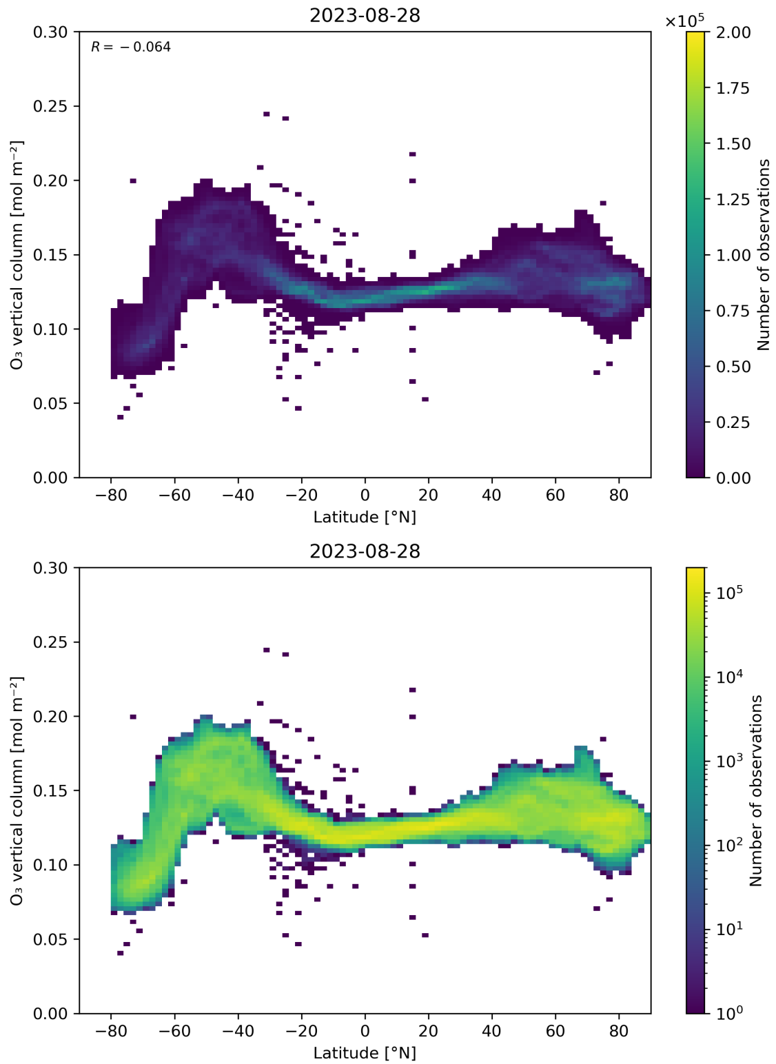
Figure 36: Scatter density plot of “Latitude” against “O 3 vertical column” for 2023-08-27 to 2023-08-29.
