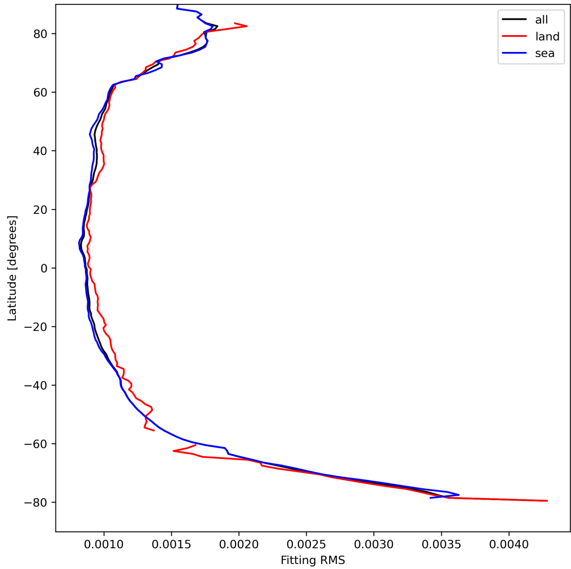
Figure 16: Zonal average of “Fitting RMS” for 2023-08-28 to 2023-08-30.
