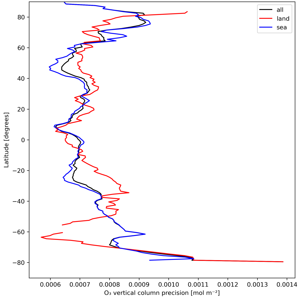
Figure 15: Zonal average of “O 3 vertical column precision” for 2023-08-28 to 2023-08-30.
