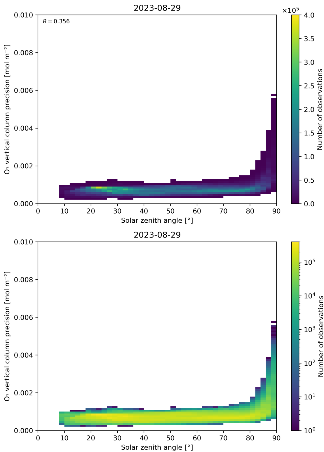
Figure 48: Scatter density plot of “Solar zenith angle” against “O 3 vertical column precision” for 2023-08-28 to 2023-08-30.
