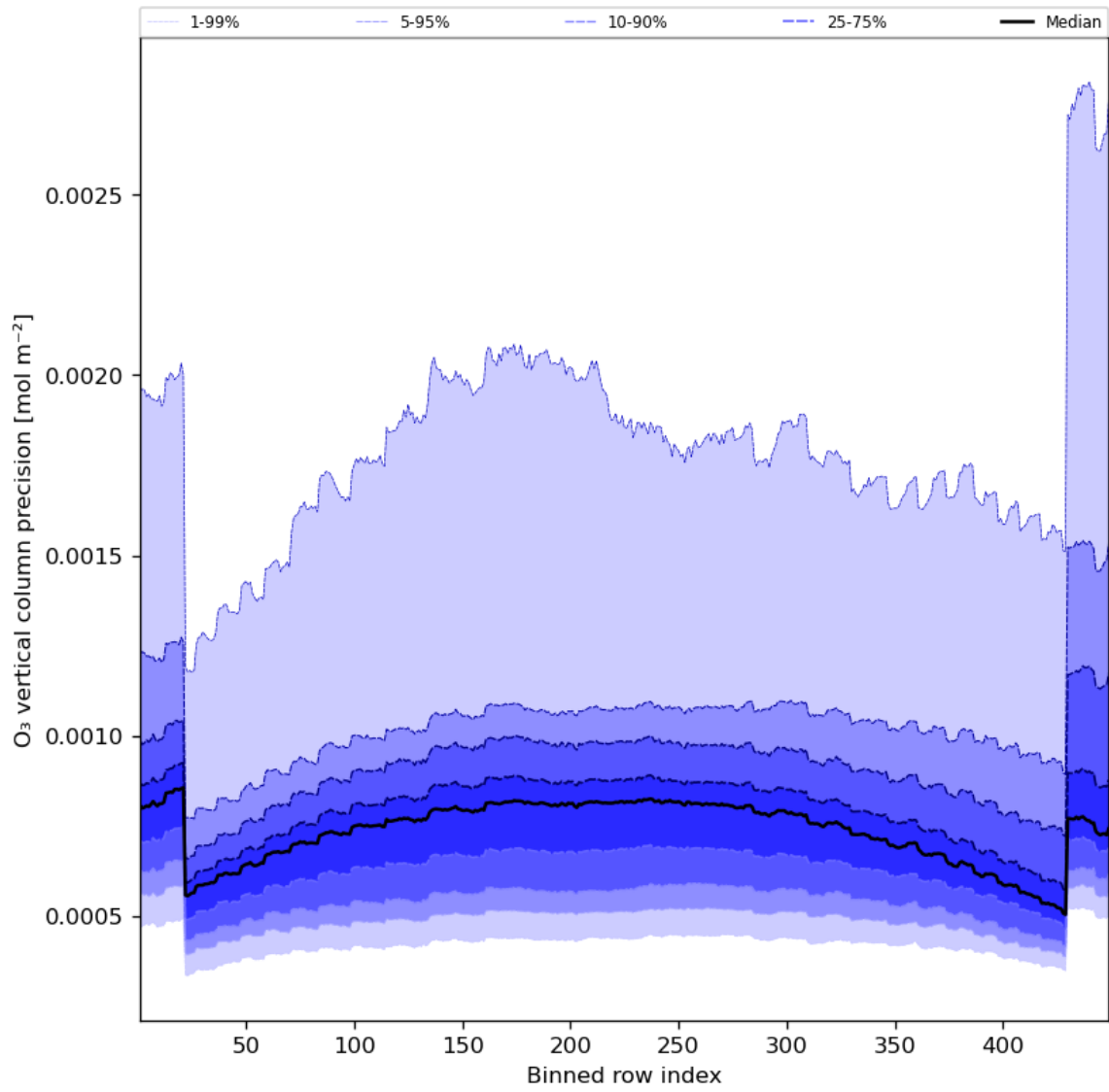
Figure 29: Along track statistics of “O 3 vertical column precision” for 2023-08-28 to 2023-08-30
