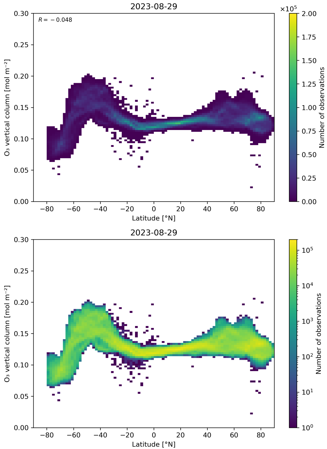
Figure 36: Scatter density plot of “Latitude” against “O 3 vertical column” for 2023-08-28 to 2023-08-30.
