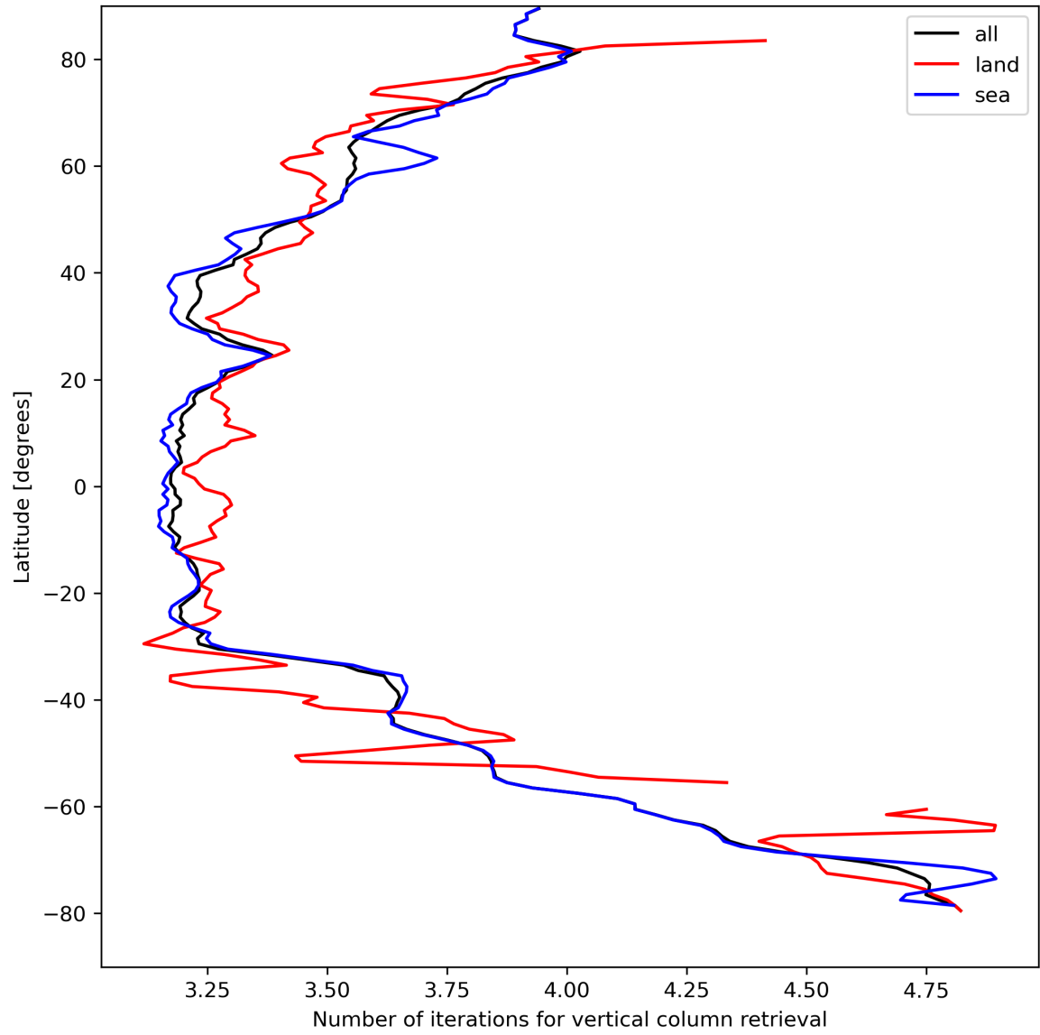
Figure 19: Zonal average of “Number of iterations for vertical column retrieval” for 2023-08-28 to 2023-08-30.
