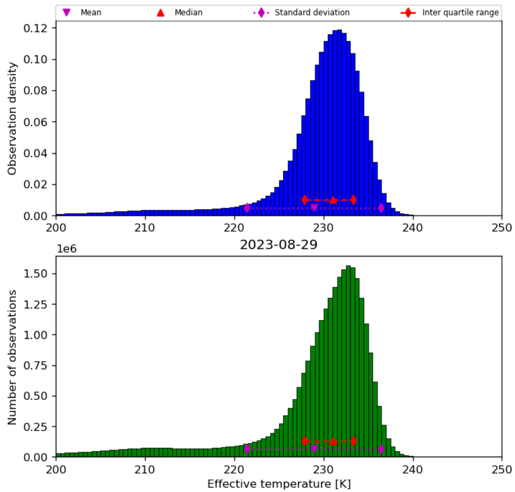
Figure 24: Histogram of “Effective temperature” for 2023-08-28 to 2023-08-30
