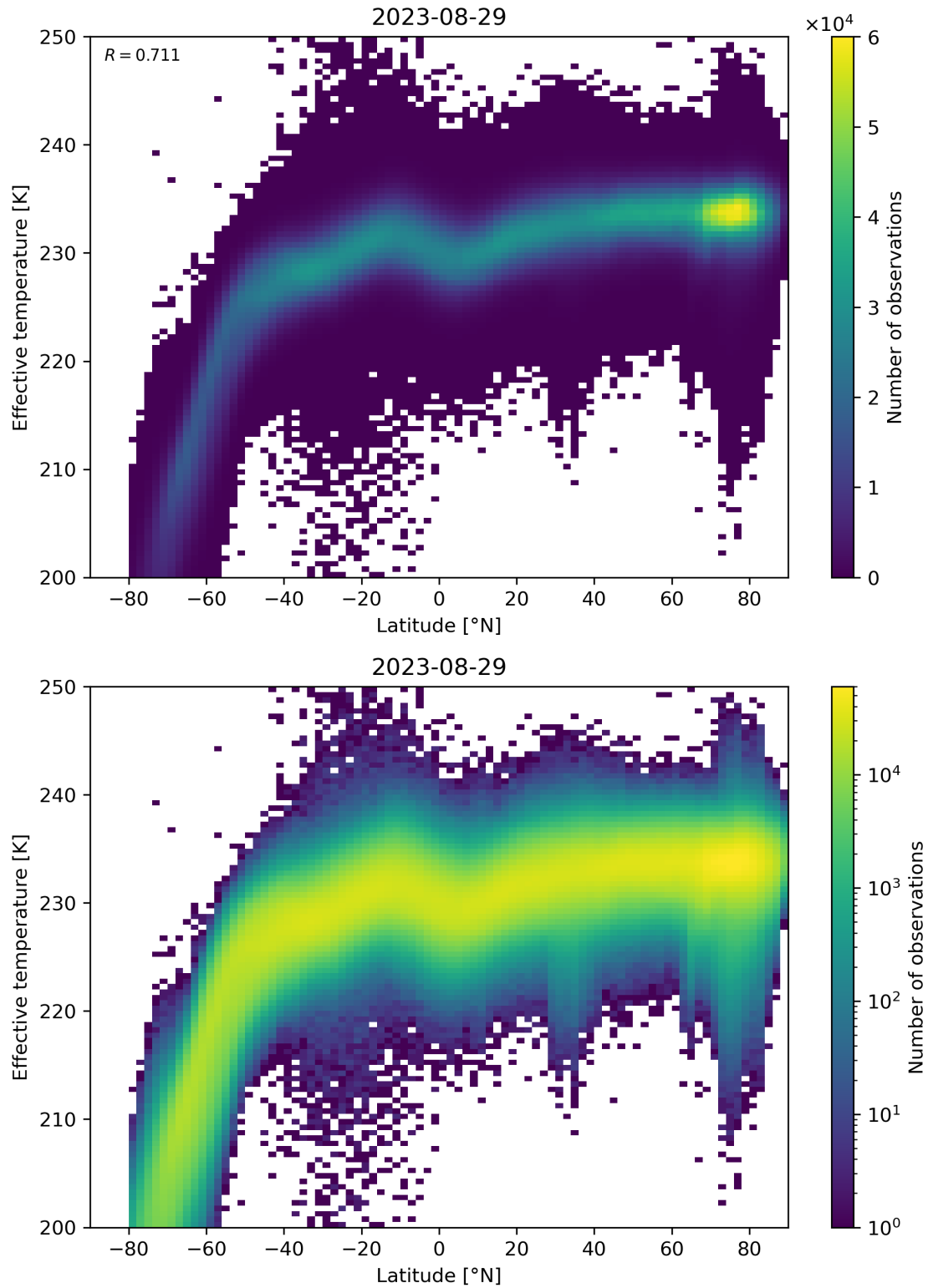
Figure 34: Scatter density plot of “Latitude” against “Effective temperature” for 2023-08-28 to 2023-08-30.
