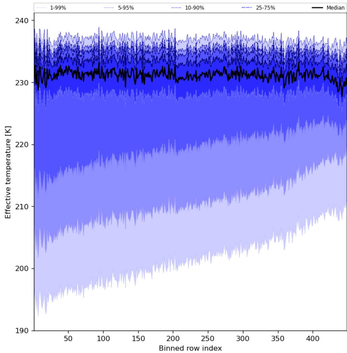
Figure 31: Along track statistics of “Effective temperature” for 2023-08-28 to 2023-08-30
