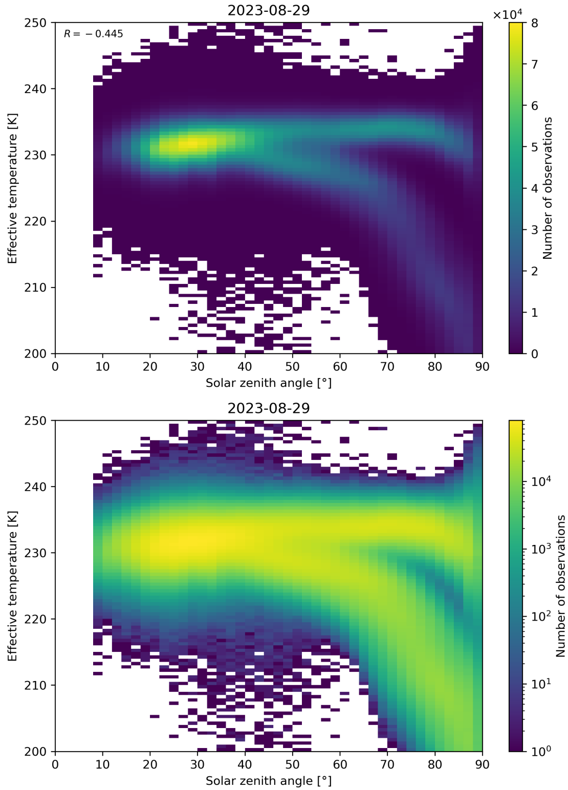
Figure 45: Scatter density plot of “Solar zenith angle” against “Effective temperature” for 2023-08-28 to 2023-08-30.
