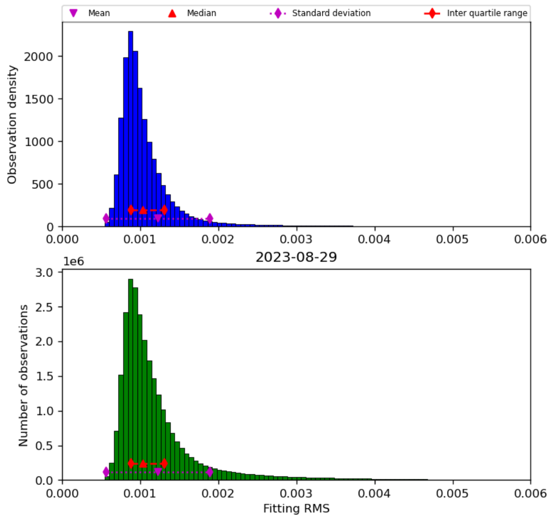
Figure 23: Histogram of “Fitting RMS” for 2023-08-28 to 2023-08-30
