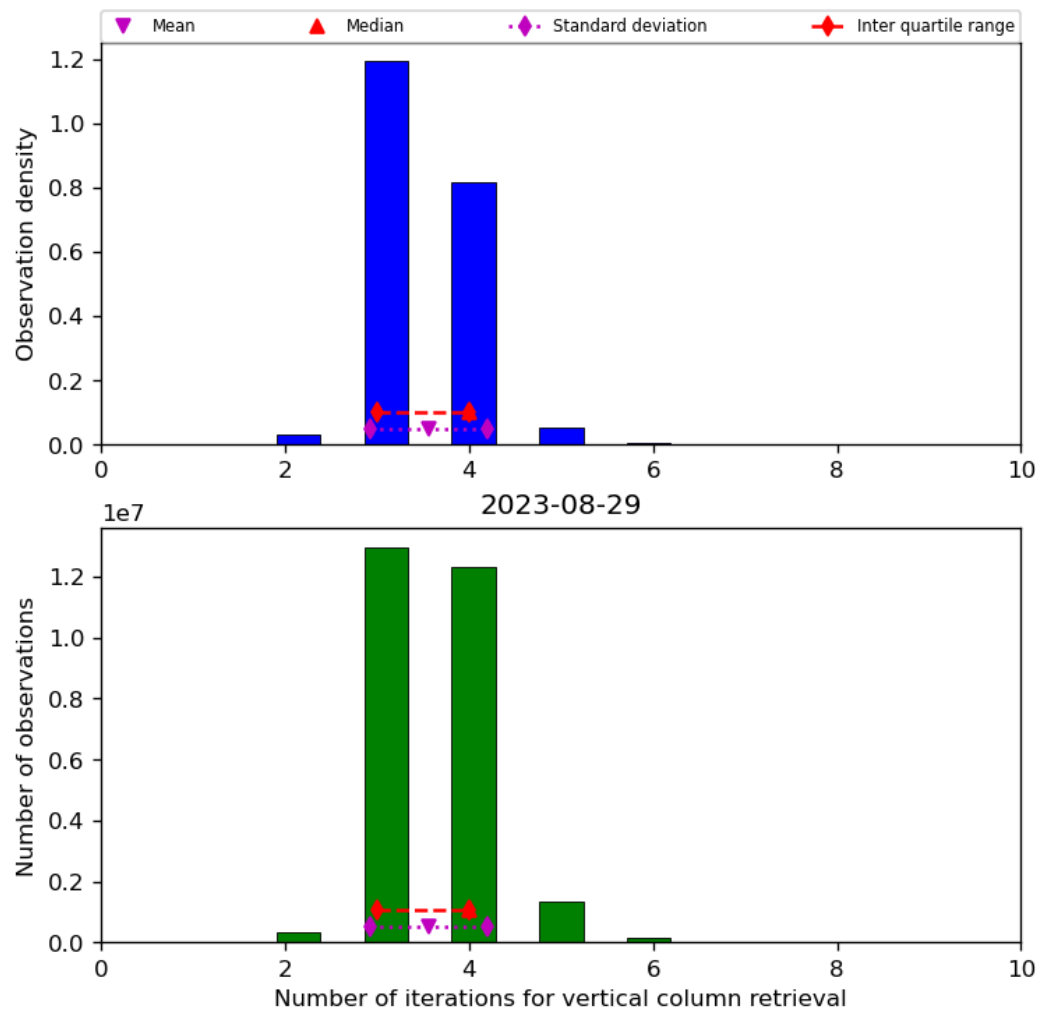
Figure 26: Histogram of “Number of iterations for vertical column retrieval” for 2023-08-28 to 2023-08-30
