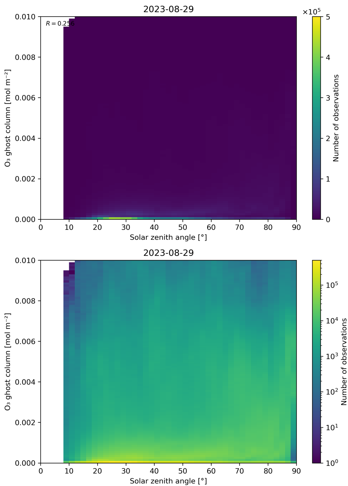
Figure 46: Scatter density plot of “Solar zenith angle” against “O 3 ghost column” for 2023-08-28 to 2023-08-30.
