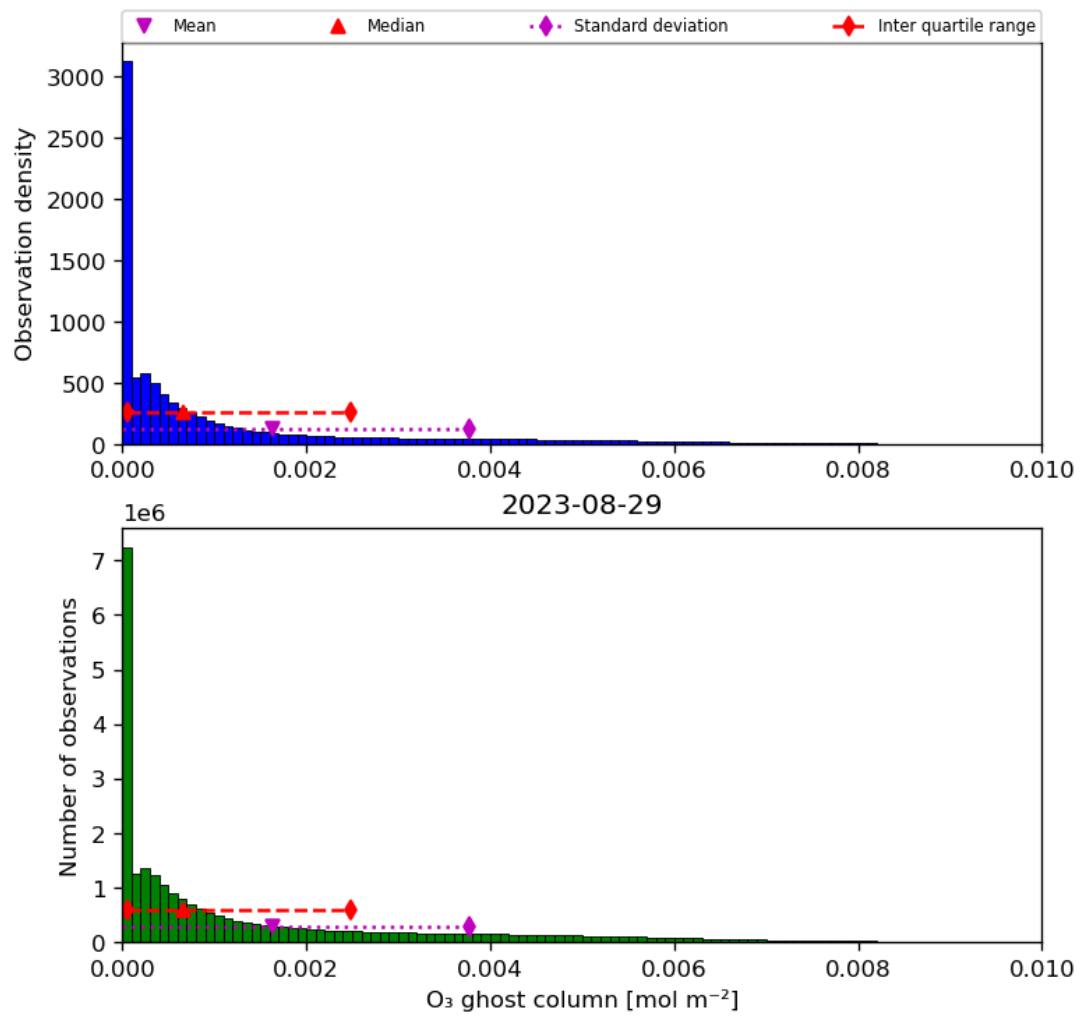
Figure 25: Histogram of “O 3 ghost column” for 2023-08-28 to 2023-08-30
