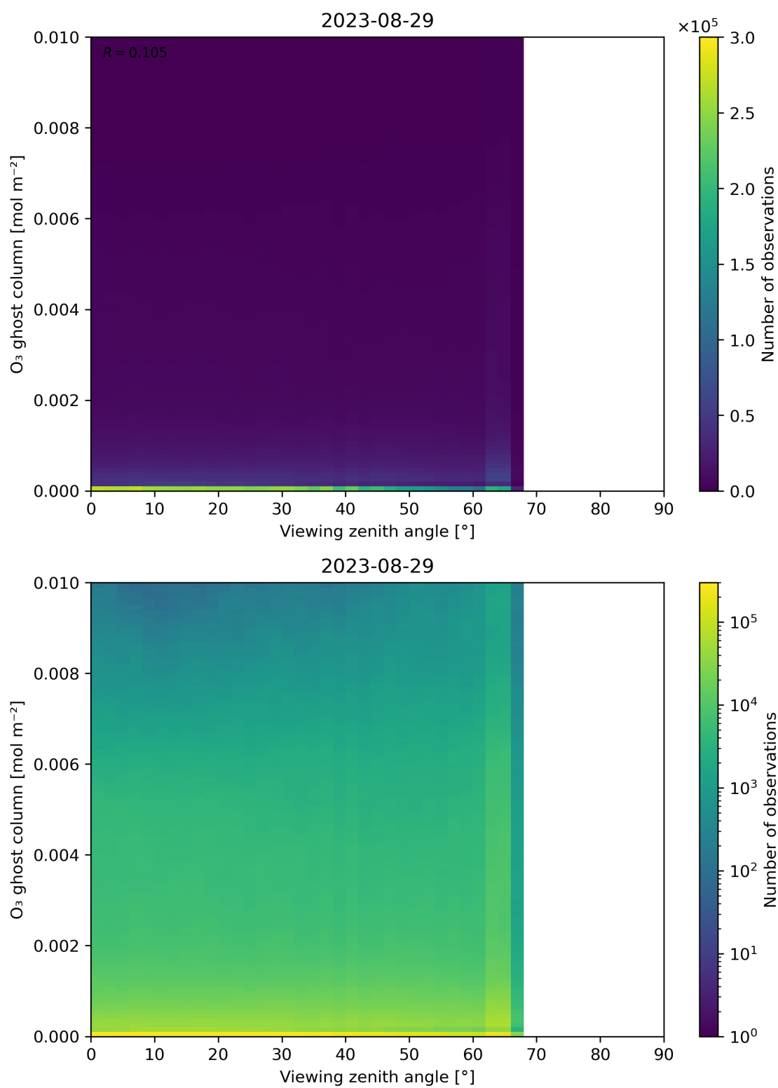
Figure 51: Scatter density plot of “Viewing zenith angle” against “O 3 ghost column” for 2023-08-28 to 2023-08-30.
