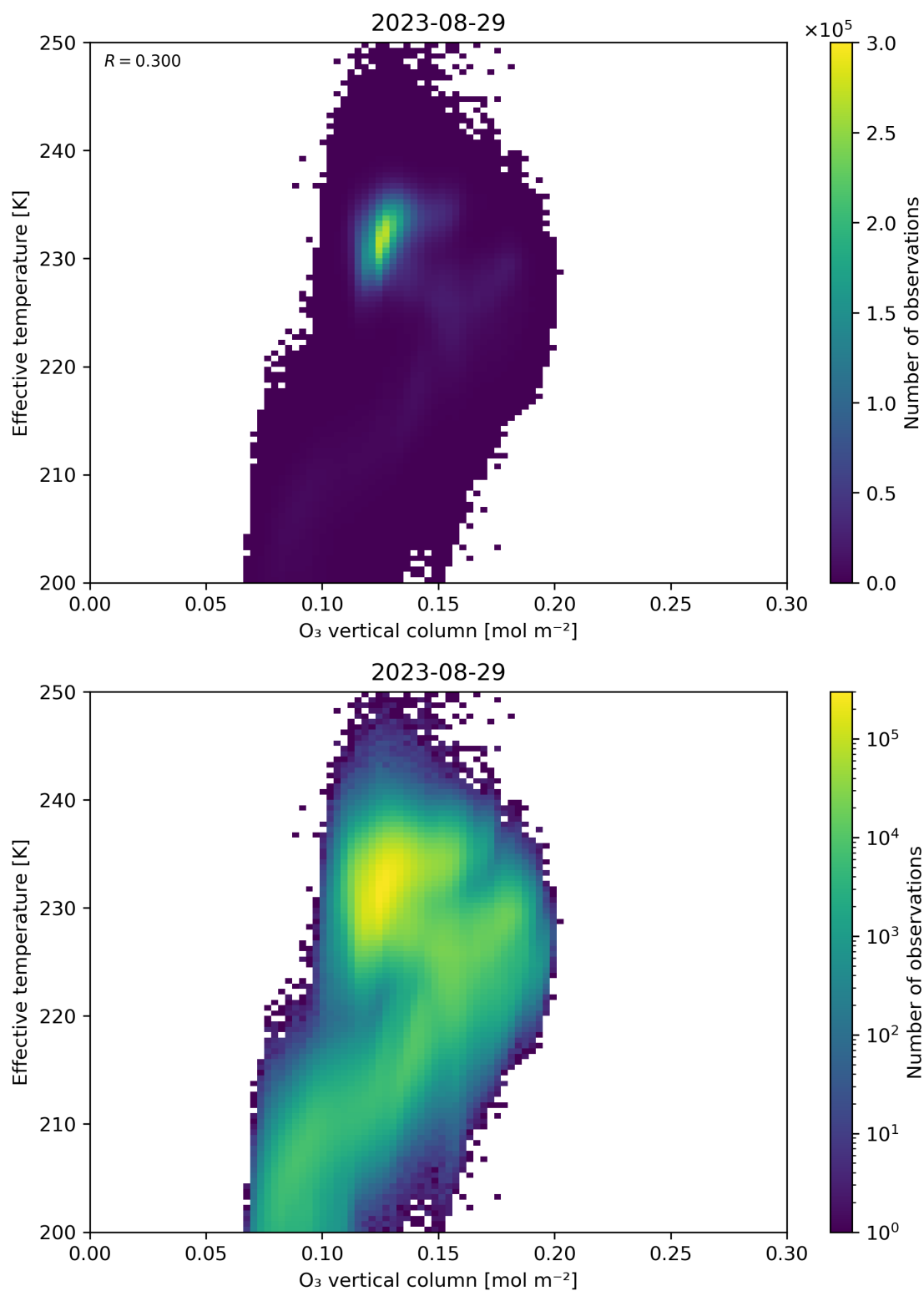
Figure 39: Scatter density plot of “O 3 vertical column” against “Effective temperature” for 2023-08-28 to 2023-08-30.
