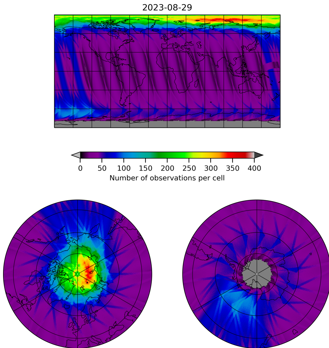
Figure 12: Map of the number of observations for 2023-08-28 to 2023-08-30
