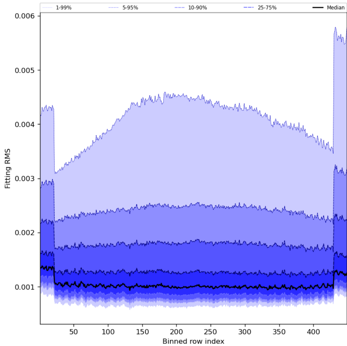
Figure 30: Along track statistics of “Fitting RMS” for 2023-08-28 to 2023-08-30
