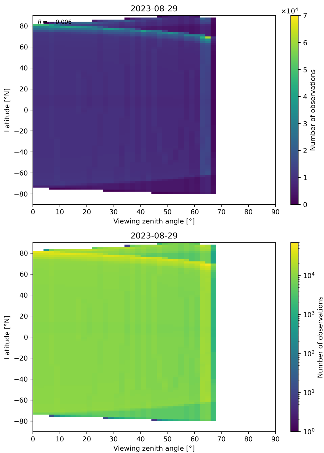
Figure 49: Scatter density plot of “Viewing zenith angle” against “Latitude” for 2023-08-28 to 2023-08-30.
