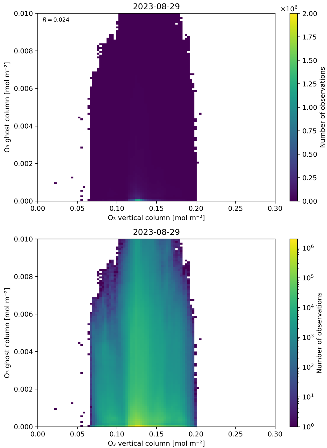
Figure 40: Scatter density plot of “O 3 vertical column” against “O 3 ghost column” for 2023-08-28 to 2023-08-30.
