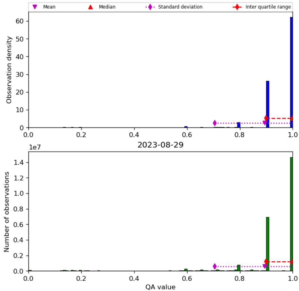
Figure 20: Histogram of “QA value” for 2023-08-28 to 2023-08-30
