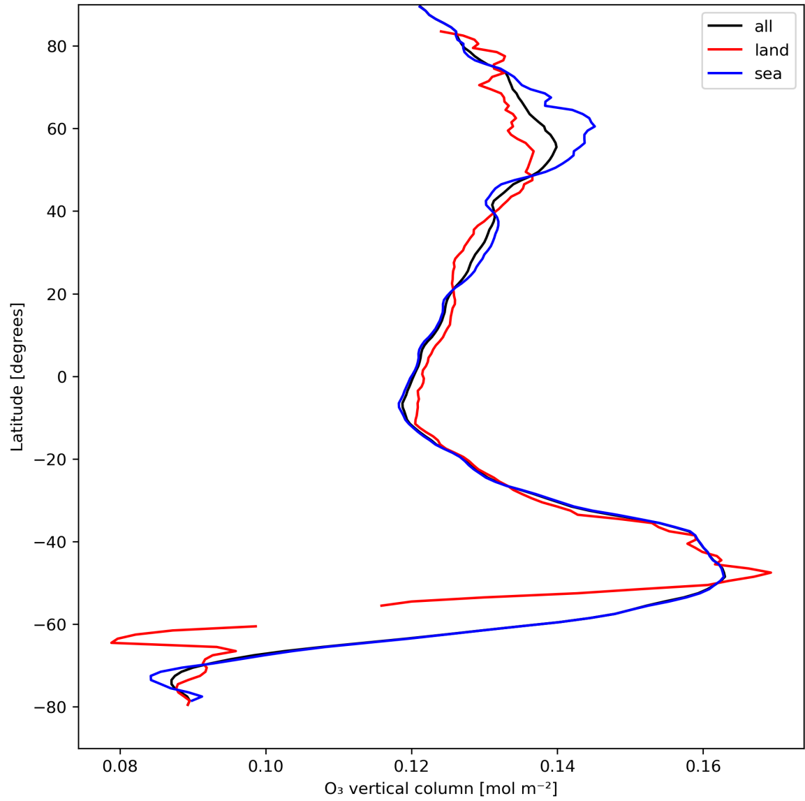
Figure 14: Zonal average of “O 3 vertical column” for 2023-08-28 to 2023-08-30.
