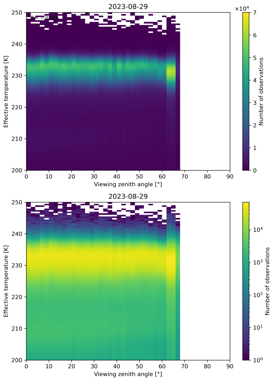
Figure 50: Scatter density plot of “Viewing zenith angle” against “Effective temperature” for 2023-08-28 to 2023-08-30.
