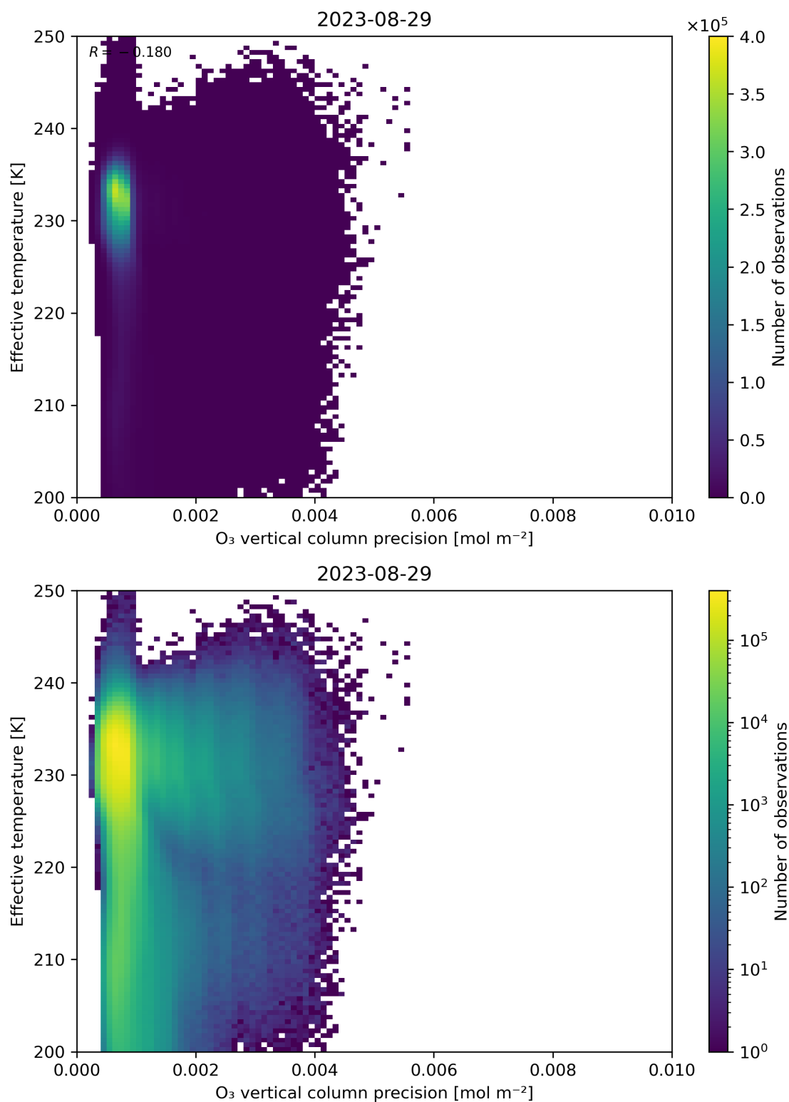
Figure 42: Scatter density plot of “O 3 vertical column precision” against “Effective temperature” for 2023-08-28 to 2023-08-30.
