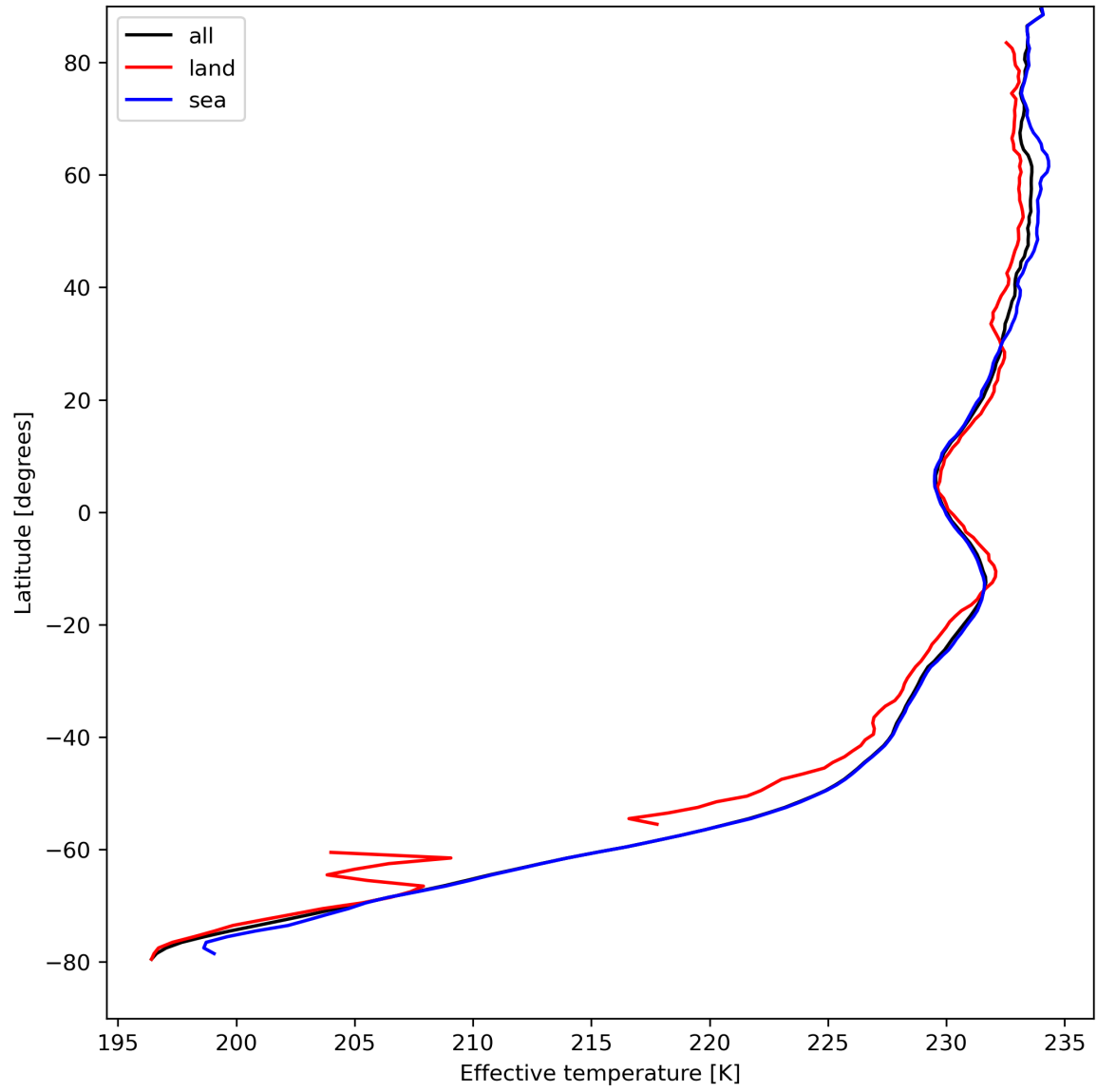
Figure 17: Zonal average of "Effective temperature" for 2023-08-28 to 2023-08-30.
