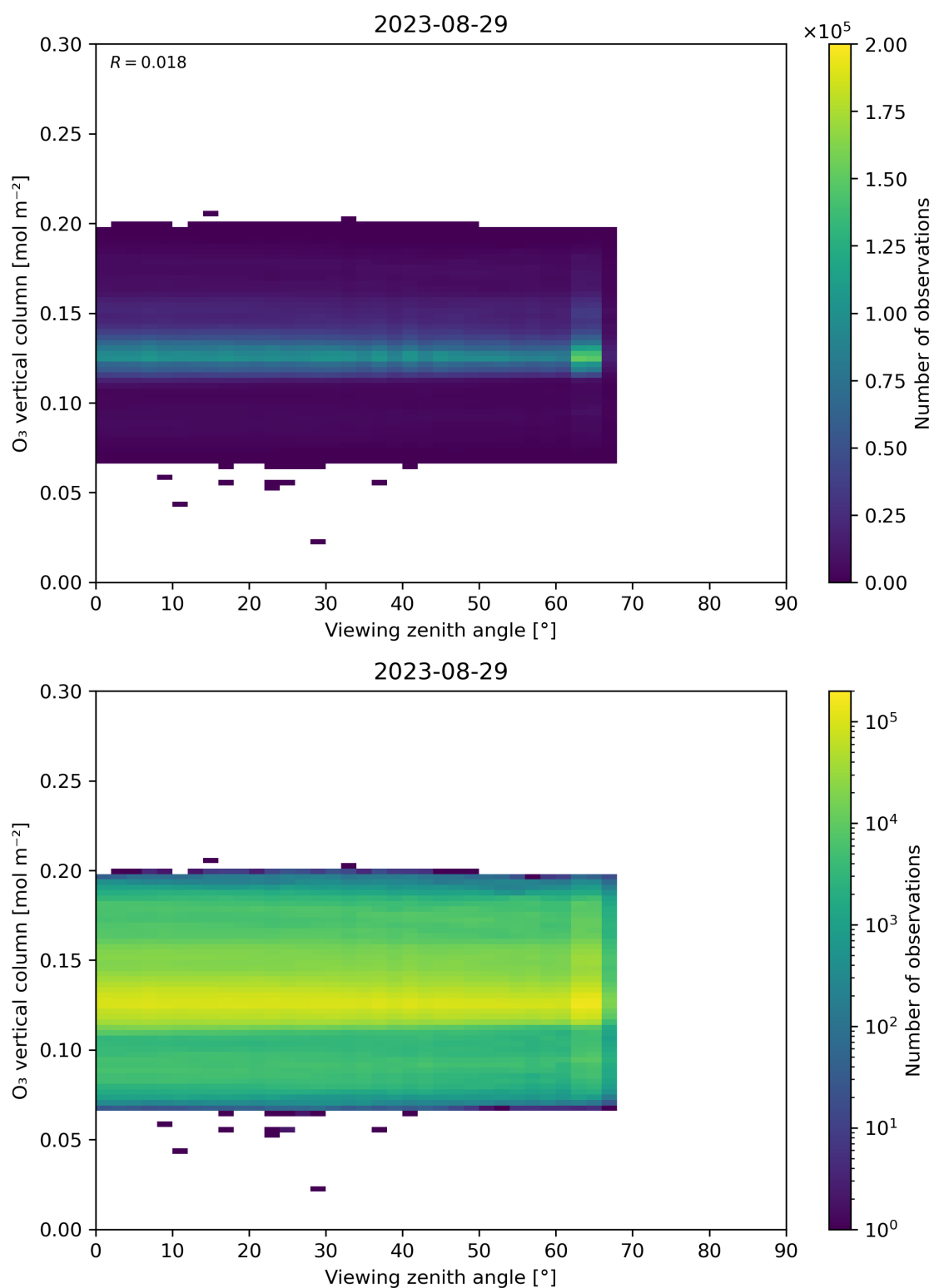
Figure 52: Scatter density plot of “Viewing zenith angle” against “O 3 vertical column” for 2023-08-28 to 2023-08-30.
