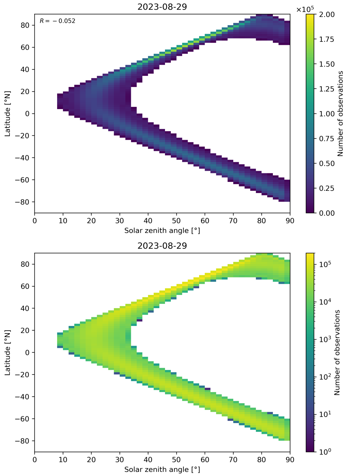
Figure 44: Scatter density plot of “Solar zenith angle” against “Latitude” for 2023-08-28 to 2023-08-30.
