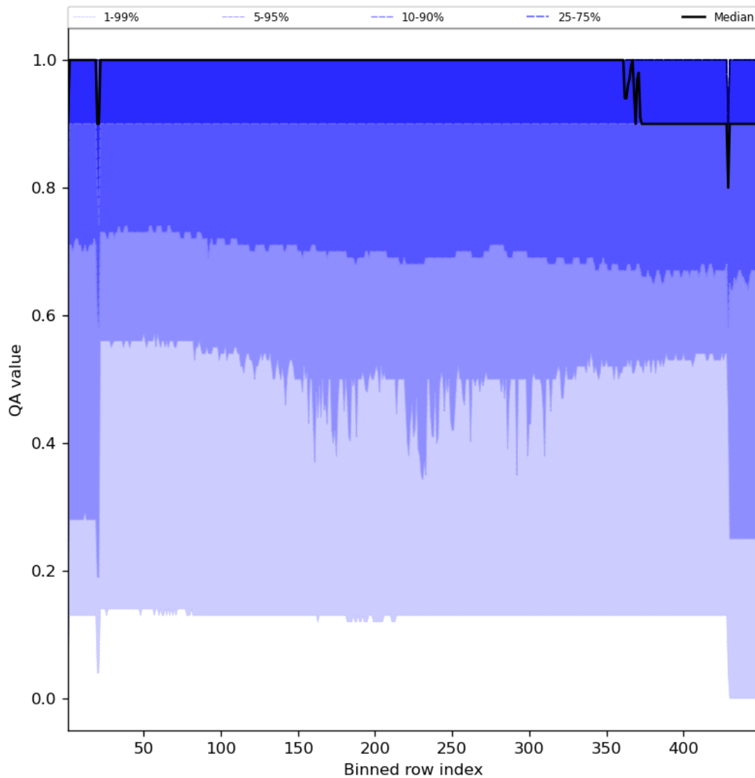
Figure 27: Along track statistics of “QA value” for 2023-08-28 to 2023-08-30
