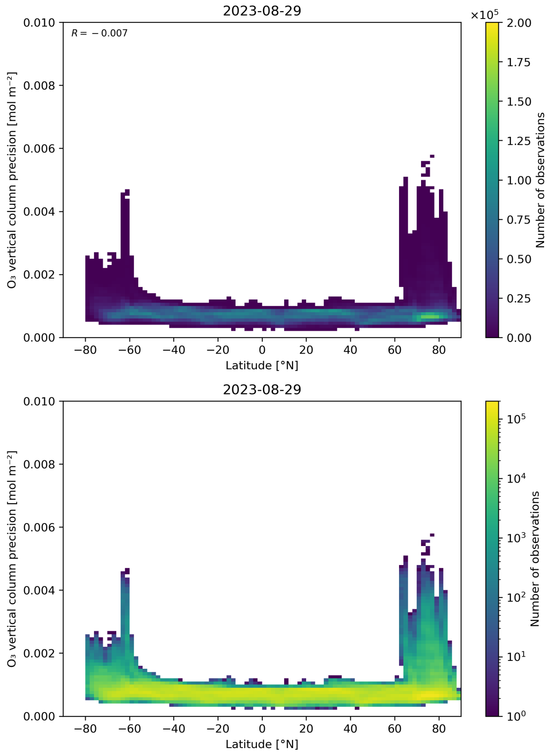
Figure 37: Scatter density plot of “Latitude” against “O 3 vertical column precision” for 2023-08-28 to 2023-08-30.
