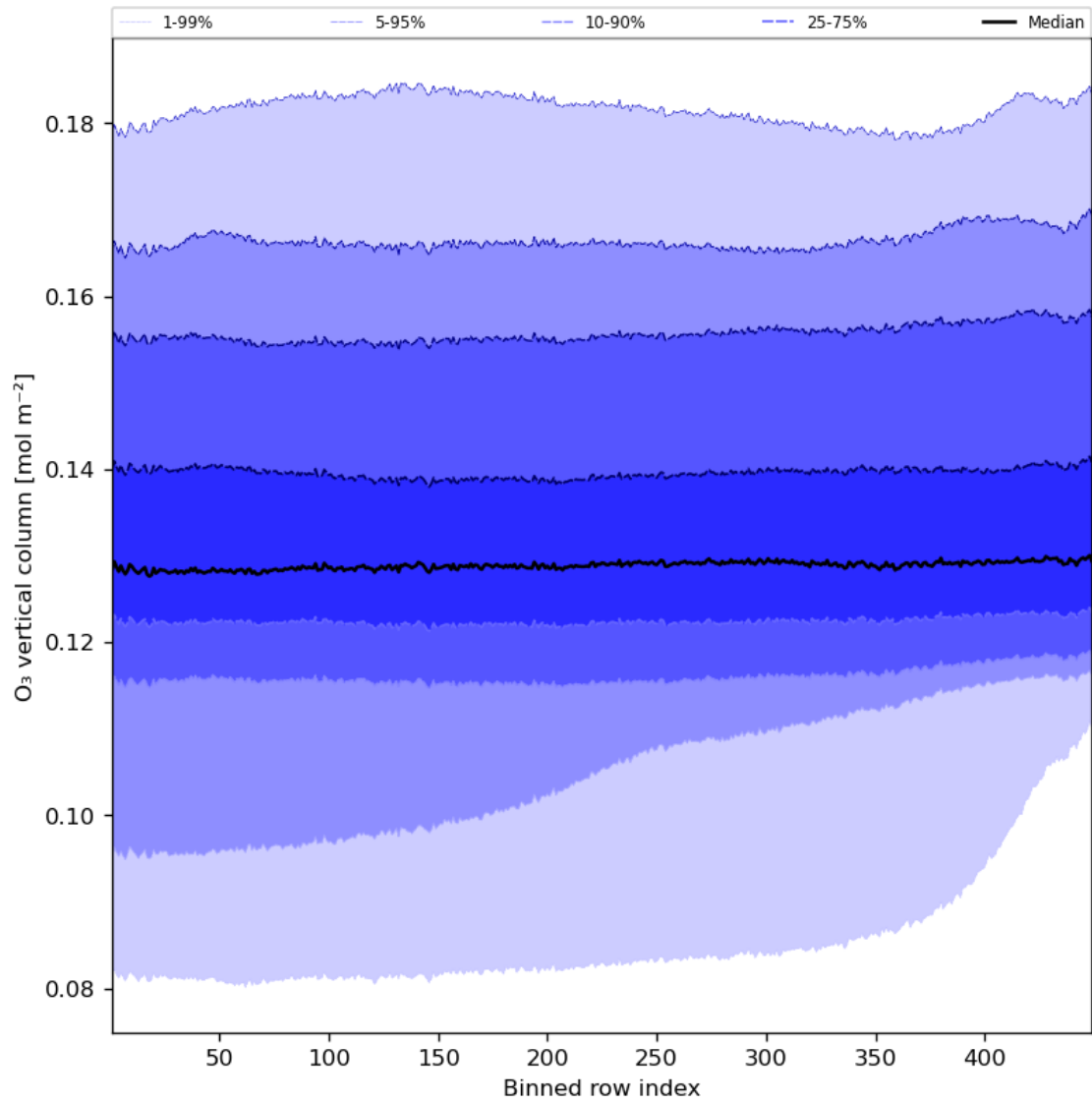
Figure 28: Along track statistics of “O 3 vertical column” for 2023-08-28 to 2023-08-30
