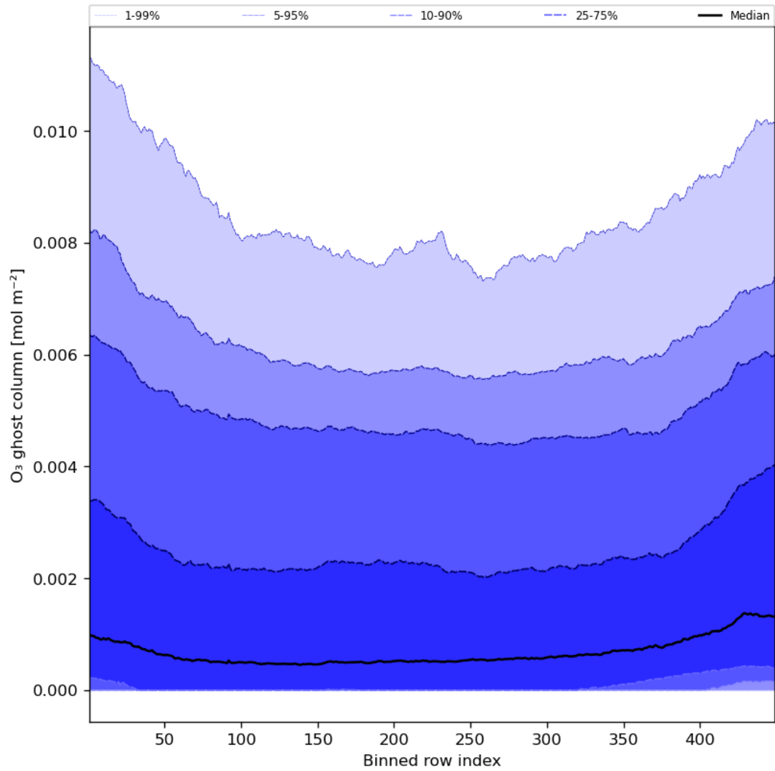
Figure 32: Along track statistics of “O 3 ghost column” for 2023-08-28 to 2023-08-30
