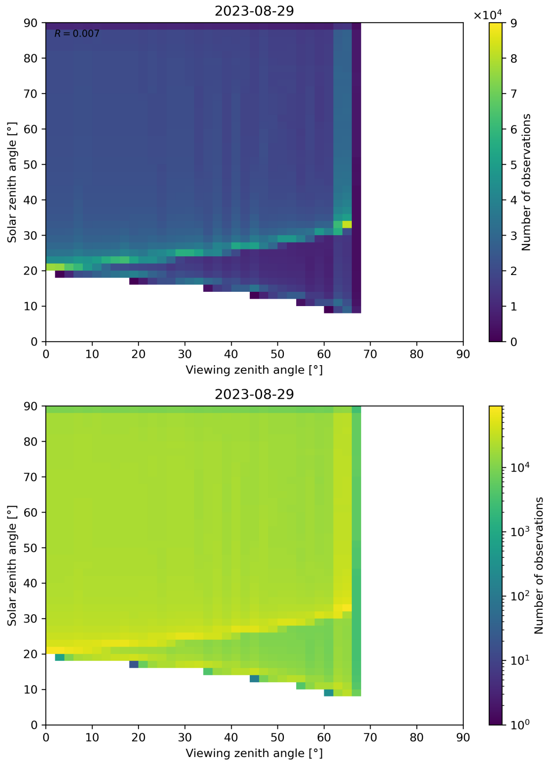
Figure 54: Scatter density plot of “Viewing zenith angle” against “Solar zenith angle” for 2023-08-28 to 2023-08-30.
