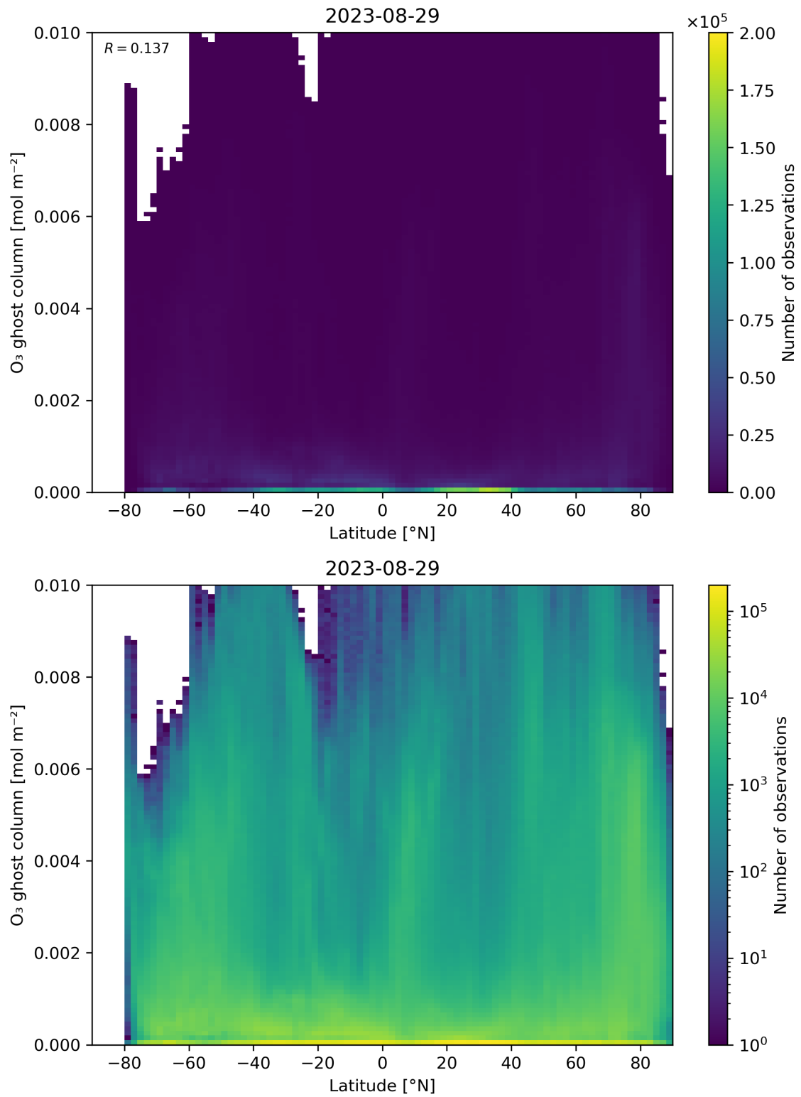
Figure 35: Scatter density plot of “Latitude” against “O 3 ghost column” for 2023-08-28 to 2023-08-30.
