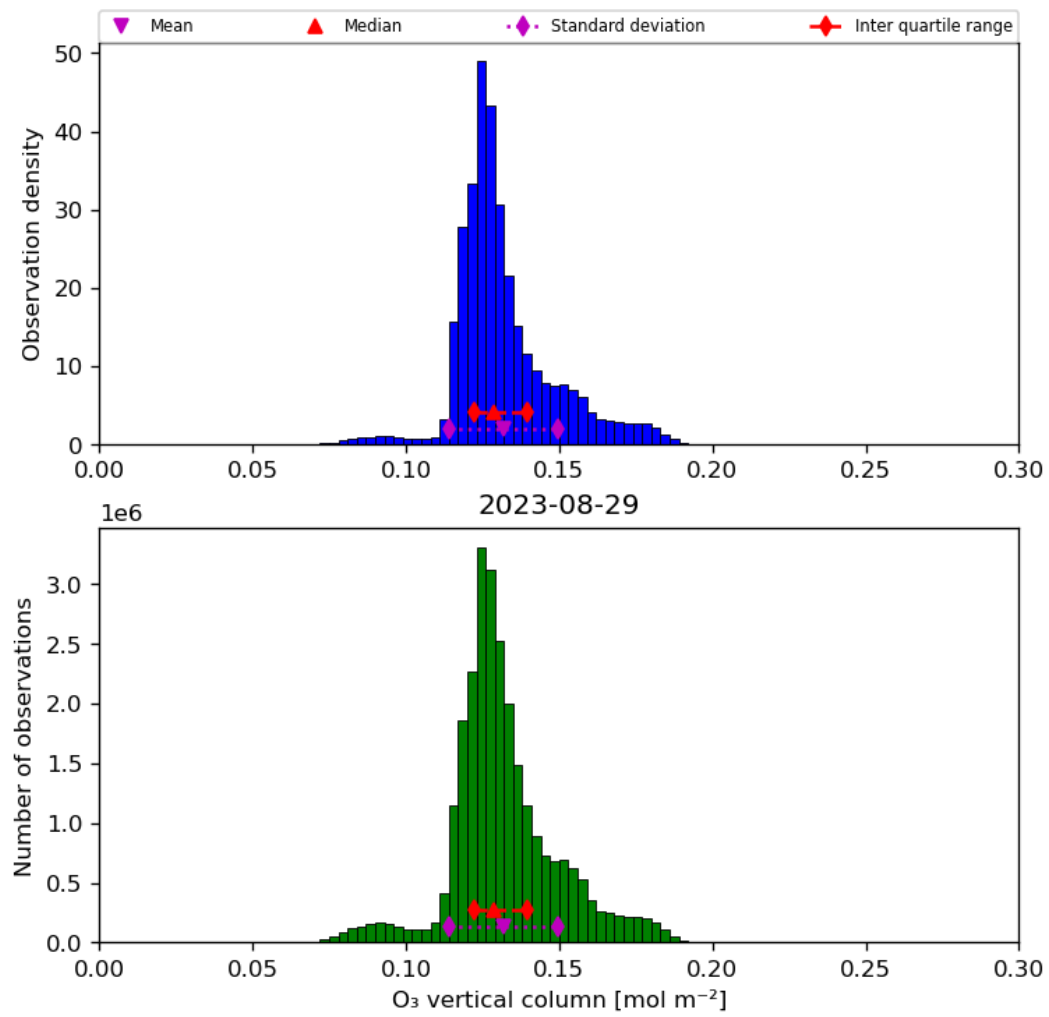
Figure 21: Histogram of “O 3 vertical column” for 2023-08-28 to 2023-08-30
