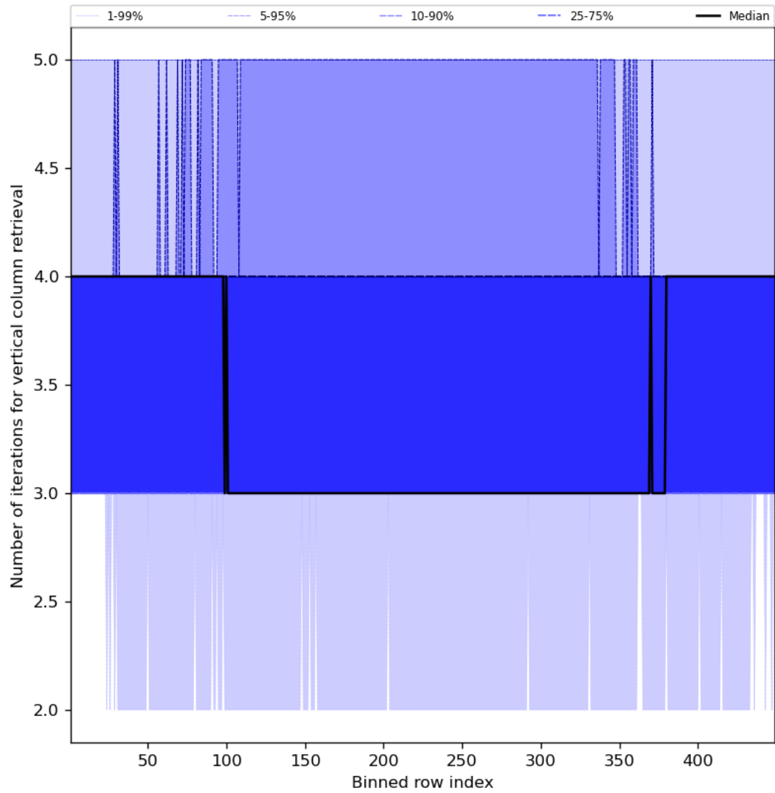
Figure 33: Along track statistics of “Number of iterations for vertical column retrieval” for 2023-08-28 to 2023-08-30
