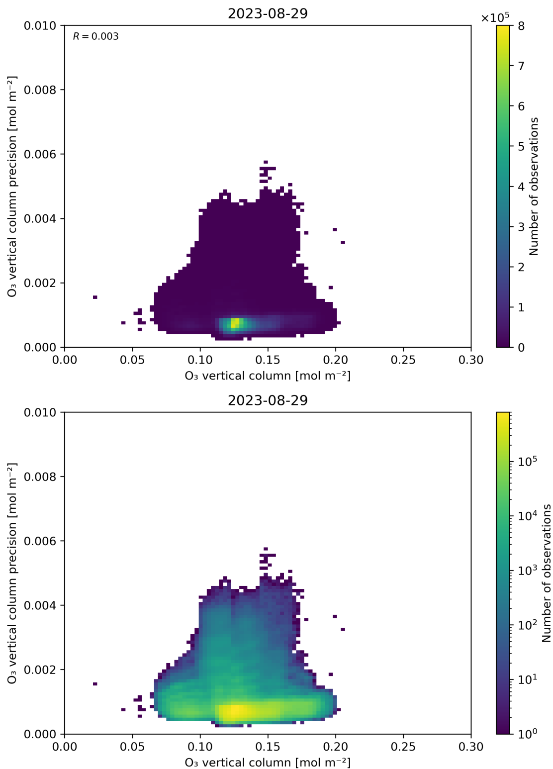
Figure 41: Scatter density plot of “O 3 vertical column” against “O 3 vertical column precision” for 2023-08-28 to 2023-08-30.
