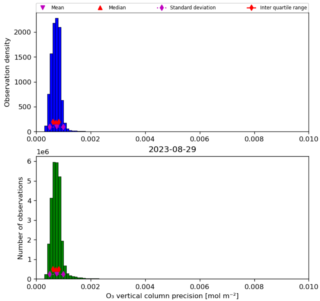
Figure 22: Histogram of “O 3 vertical column precision” for 2023-08-28 to 2023-08-30
