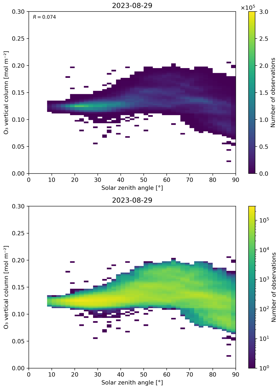
Figure 47: Scatter density plot of “Solar zenith angle” against “O 3 vertical column” for 2023-08-28 to 2023-08-30.
