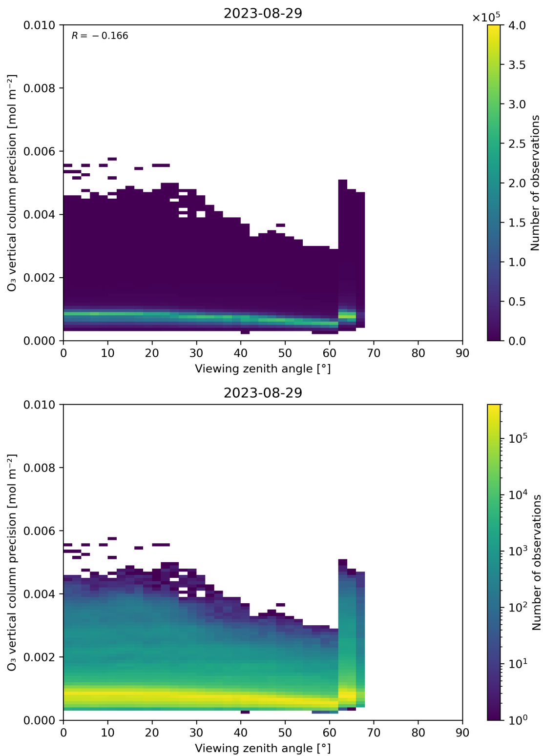
Figure 53: Scatter density plot of “Viewing zenith angle” against “O 3 vertical column precision” for 2023-08-28 to 2023-08-30.
