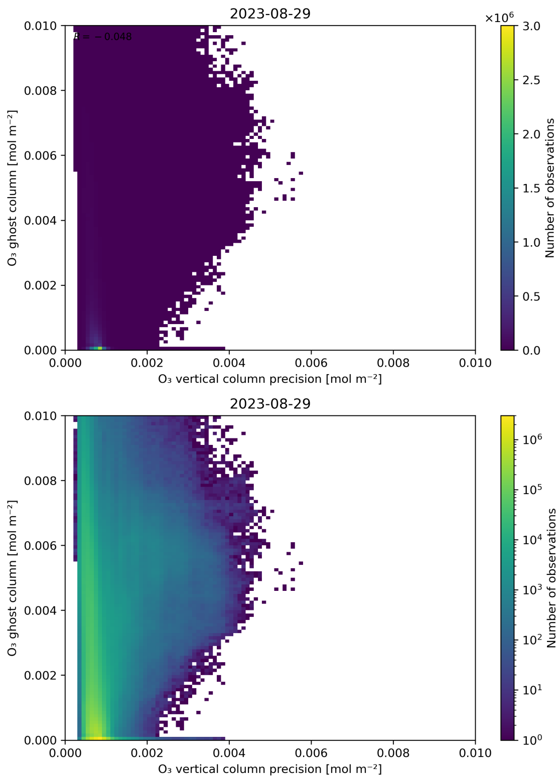
Figure 43: Scatter density plot of “ O_3 vertical column precision” against “ O_3 ghost column” for 2023-08-28 to 2023-08-30.
