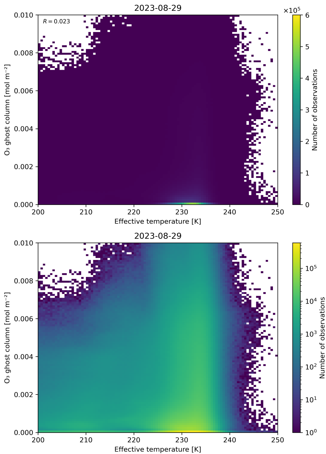
Figure 38: Scatter density plot of “Effective temperature” against “O 3 ghost column” for 2023-08-28 to 2023-08-30.
