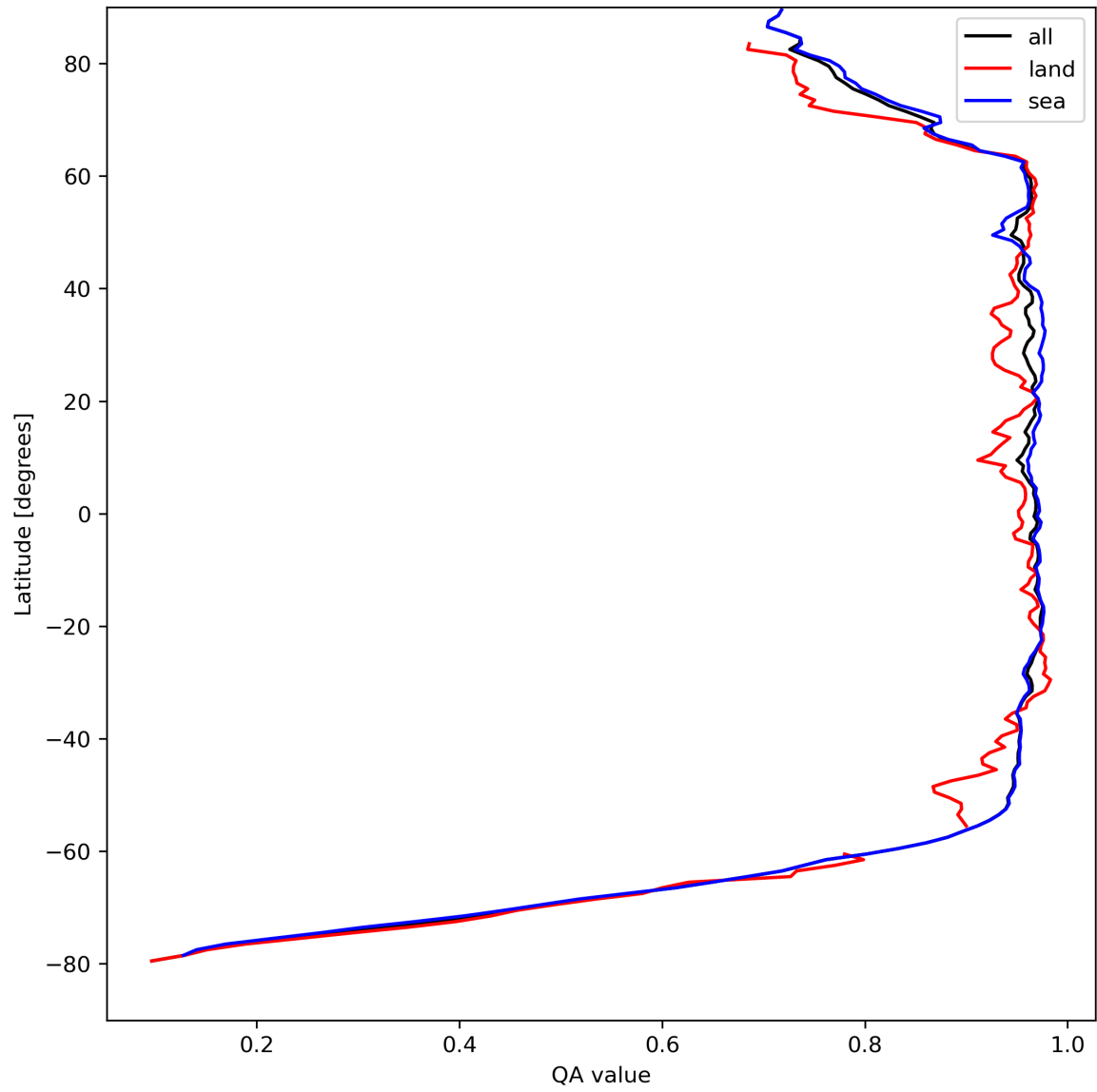
Figure 13: Zonal average of “QA value” for 2023-08-28 to 2023-08-30.
