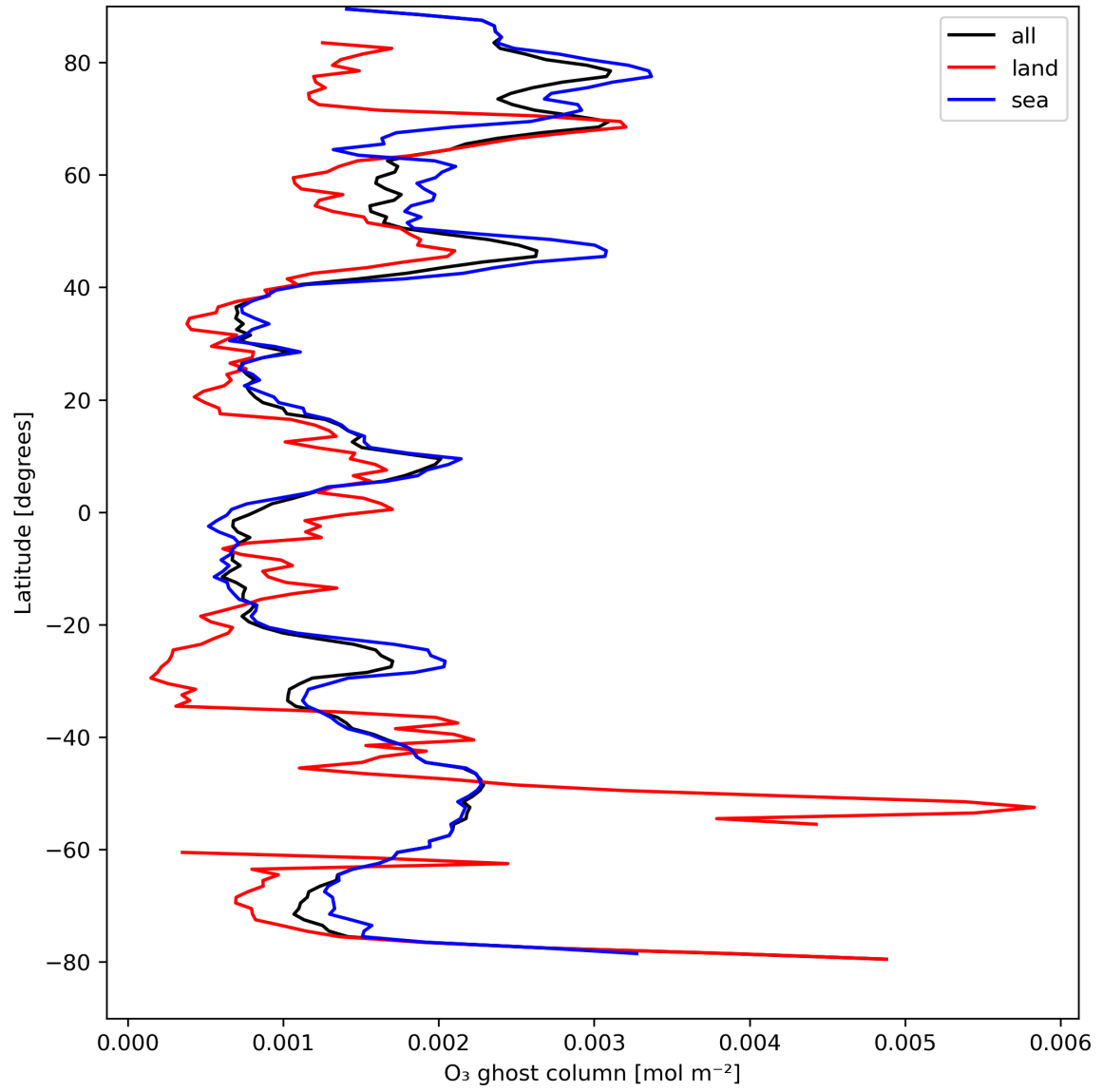
Figure 18: Zonal average of "O 3 ghost column" for 2023-08-28 to 2023-08-30.
