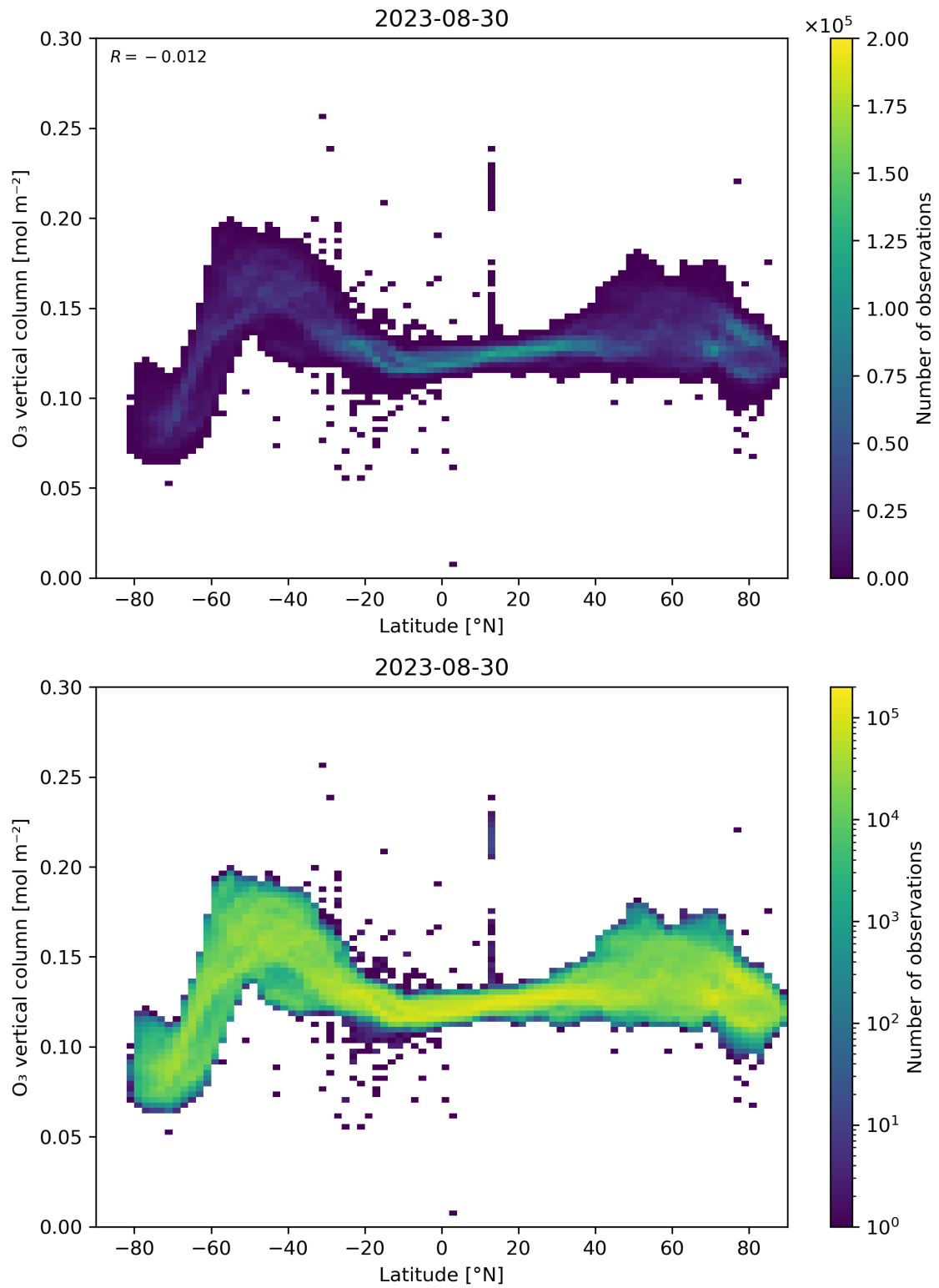
Figure 36: Scatter density plot of “Latitude” against “O 3 vertical column” for 2023-08-30 to 2023-08-31.
