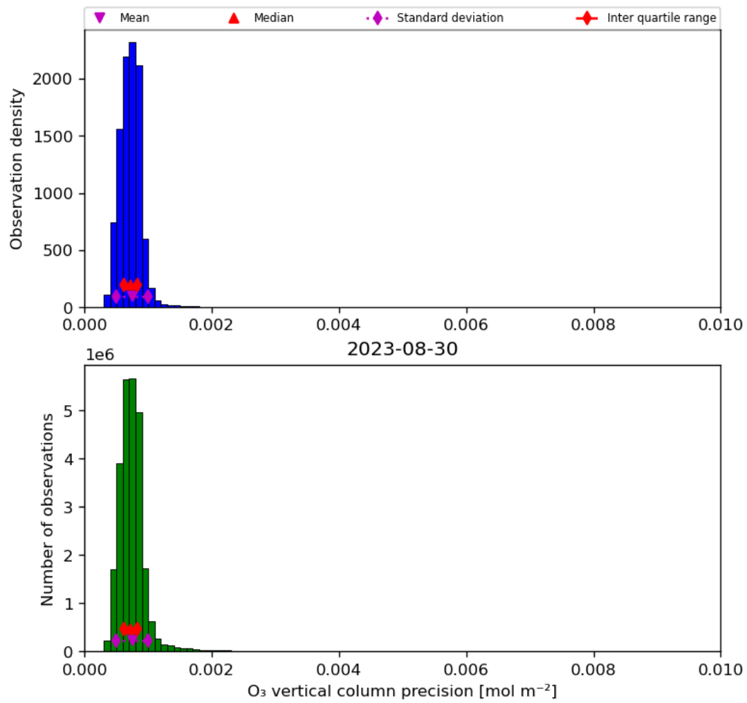
Figure 22: Histogram of “O 3 vertical column precision” for 2023-08-30 to 2023-08-31
