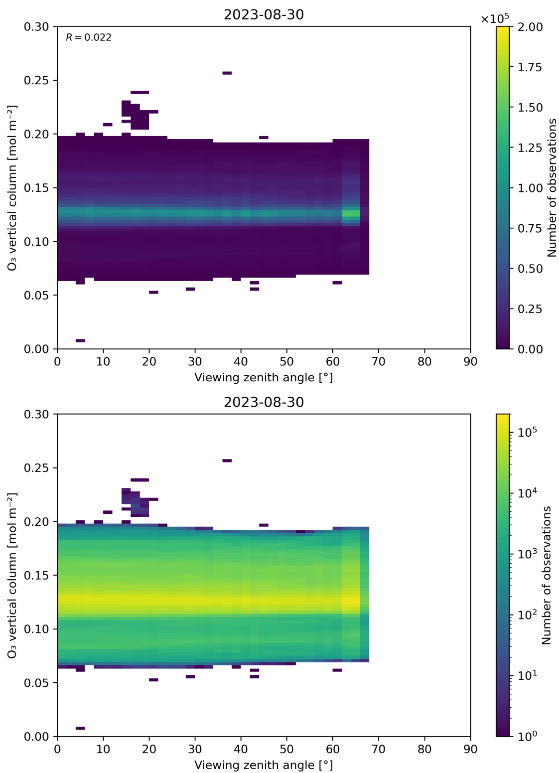
Figure 52: Scatter density plot of “Viewing zenith angle” against “O 3 vertical column” for 2023-08-30 to 2023-08-31.
