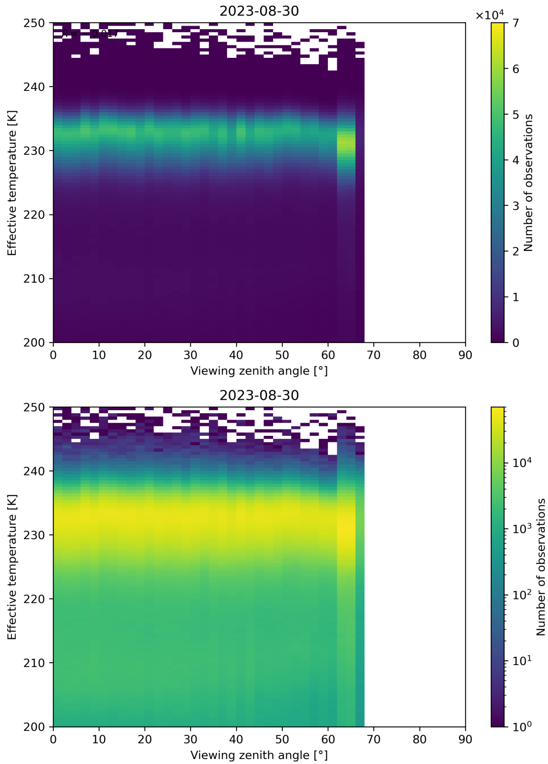
Figure 50: Scatter density plot of “Viewing zenith angle” against “Effective temperature” for 2023-08-30 to 2023-08-31.
