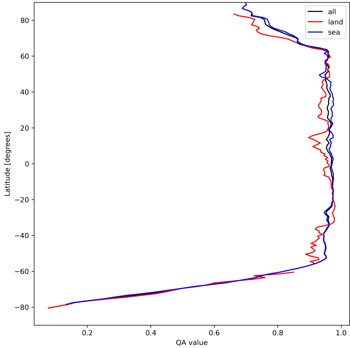
Figure 13: Zonal average of “QA value” for 2023-08-30 to 2023-08-31.
