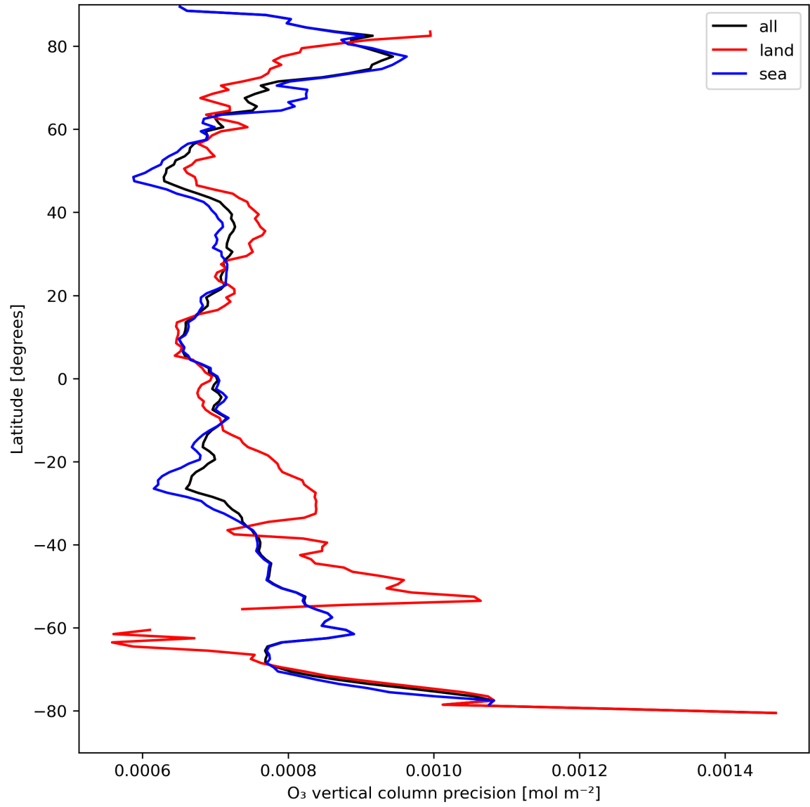
Figure 15: Zonal average of “O 3 vertical column precision” for 2023-08-30 to 2023-08-31.
