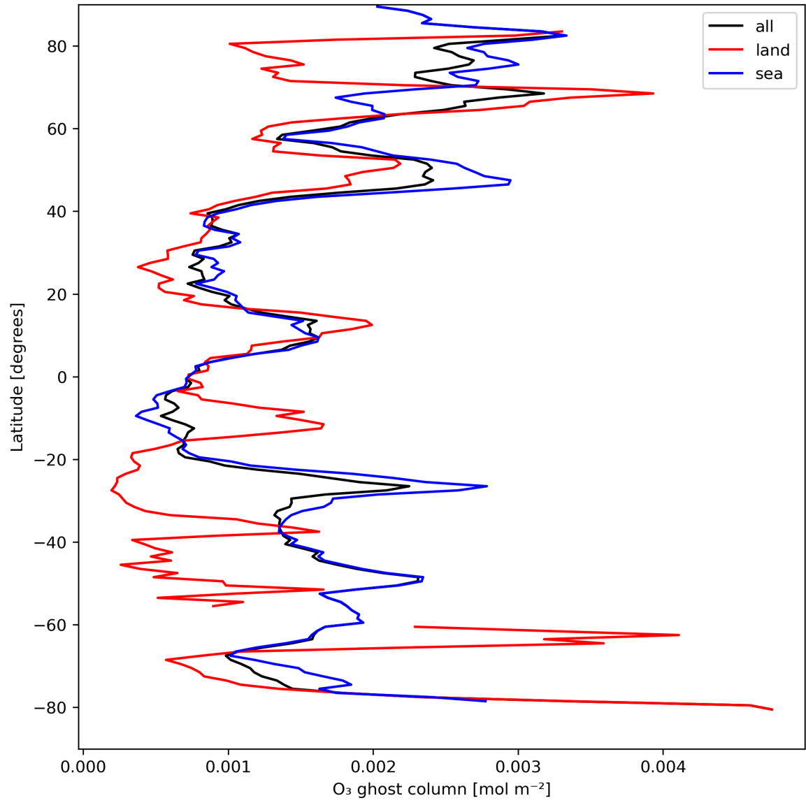
Figure 18: Zonal average of "O 3 ghost column" for 2023-08-30 to 2023-08-31.
