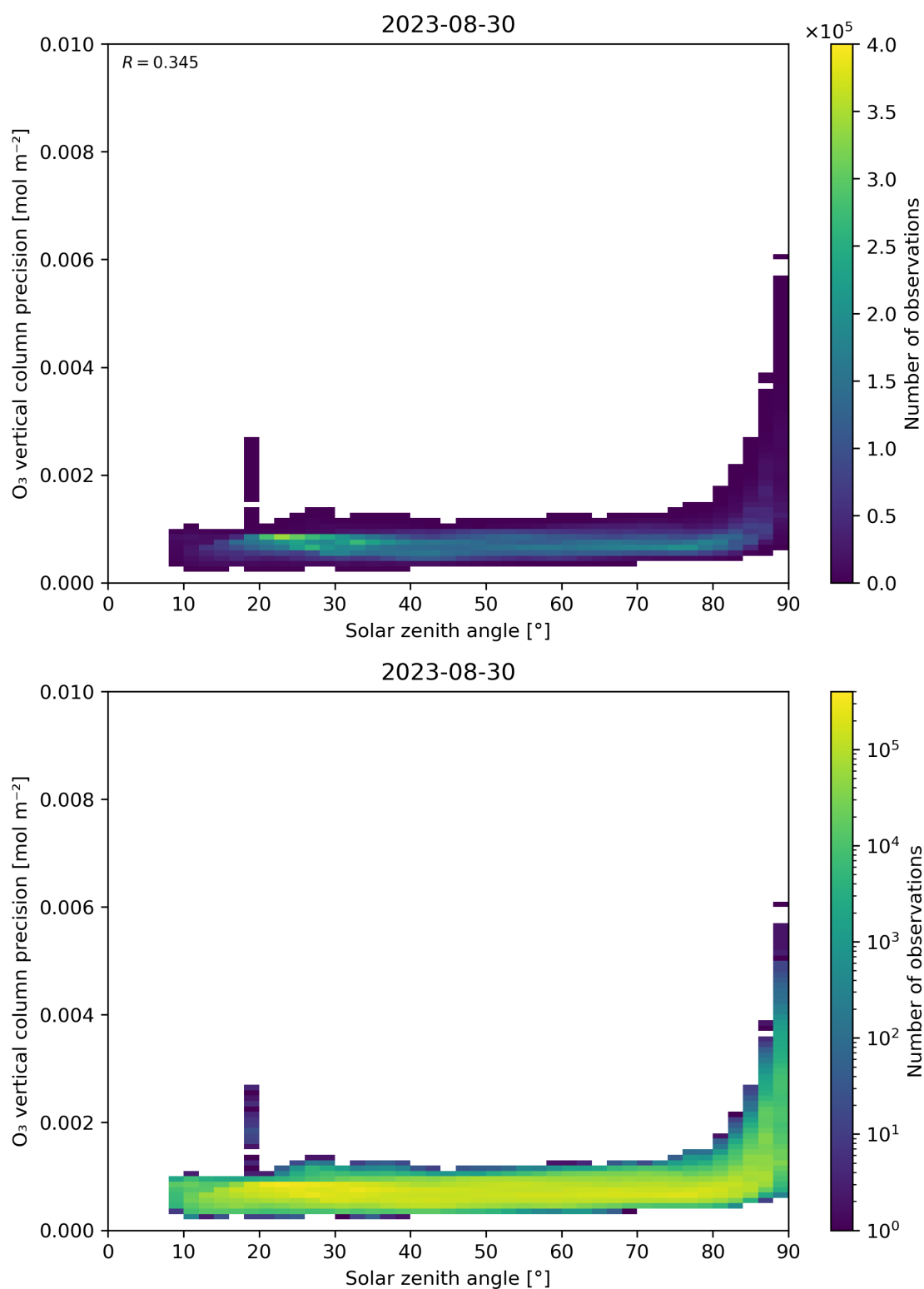
Figure 48: Scatter density plot of “Solar zenith angle” against “O 3 vertical column precision” for 2023-08-30 to 2023-08-31.
