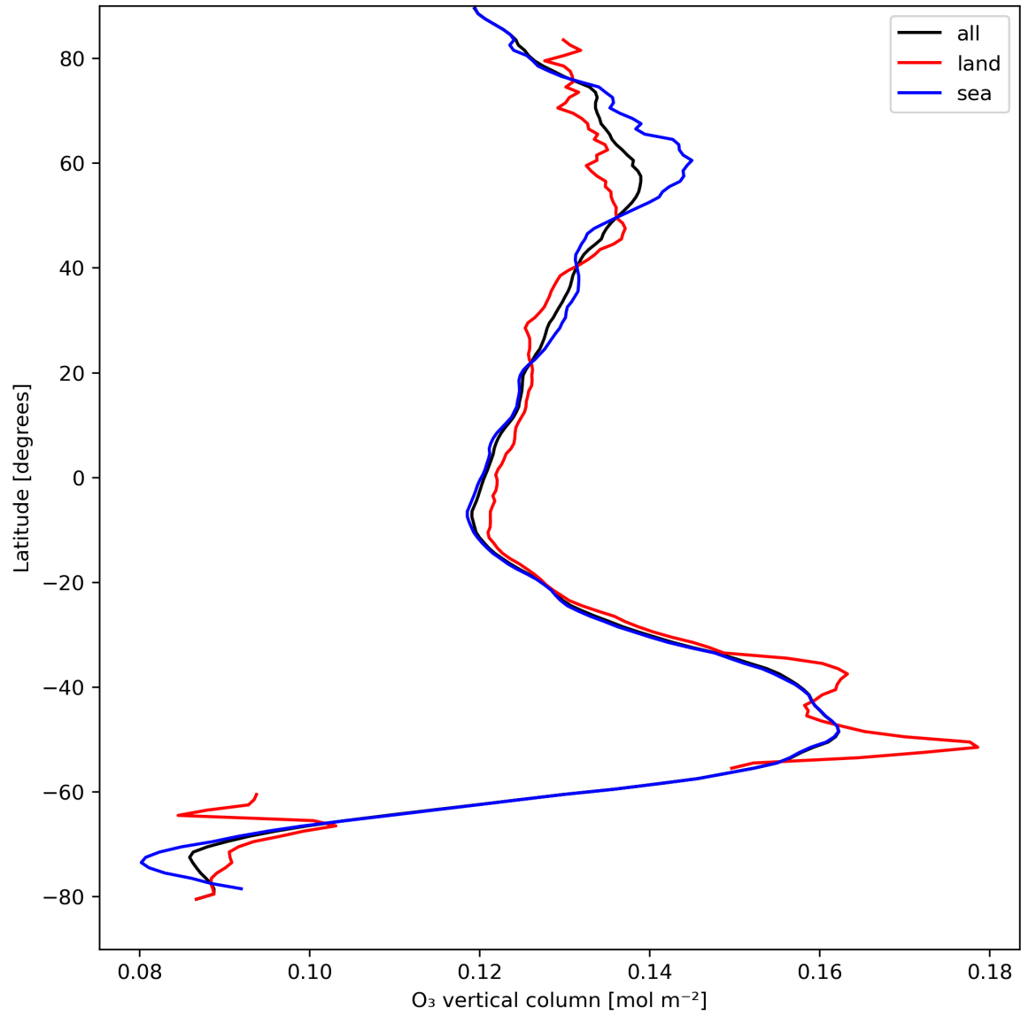
Figure 14: Zonal average of “O 3 vertical column” for 2023-08-30 to 2023-08-31.
