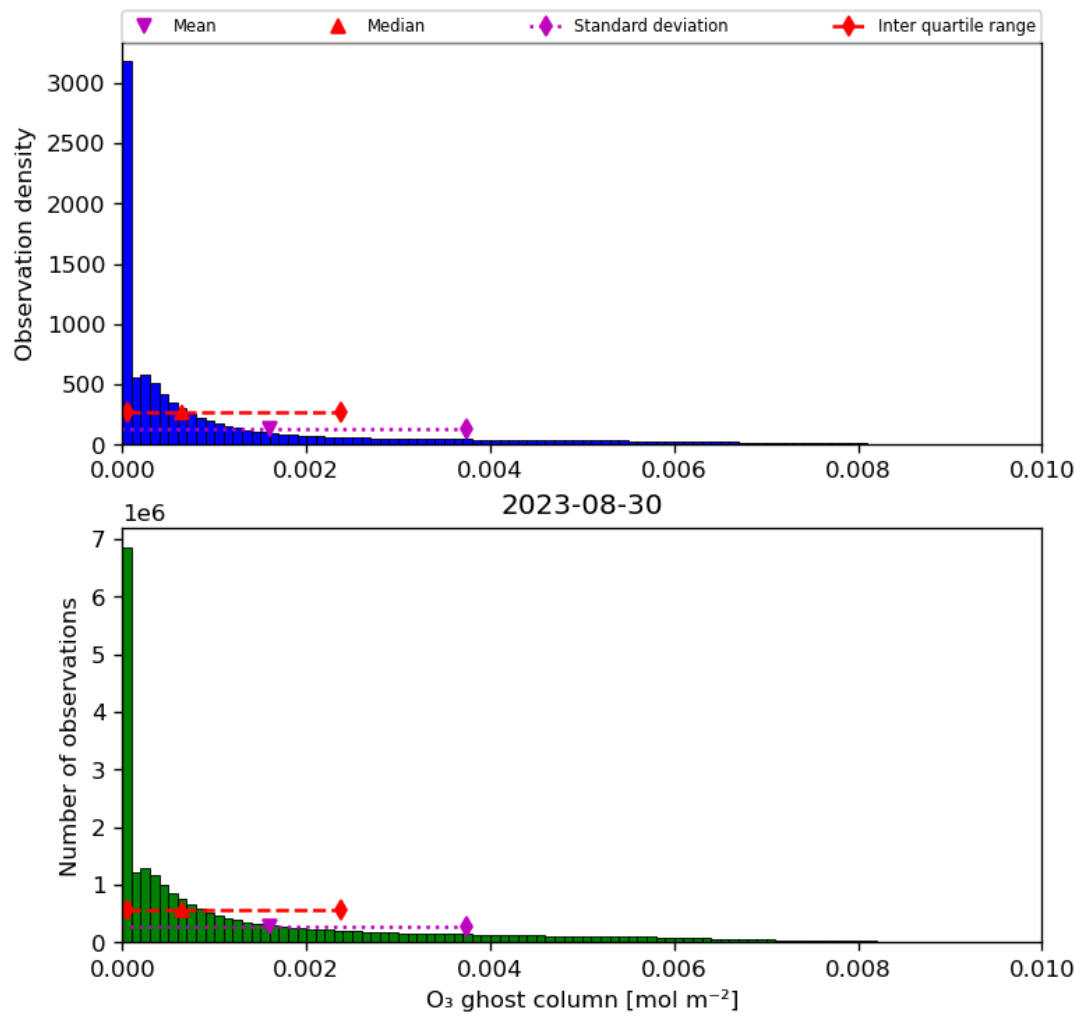
Figure 25: Histogram of “O 3 ghost column” for 2023-08-30 to 2023-08-31
