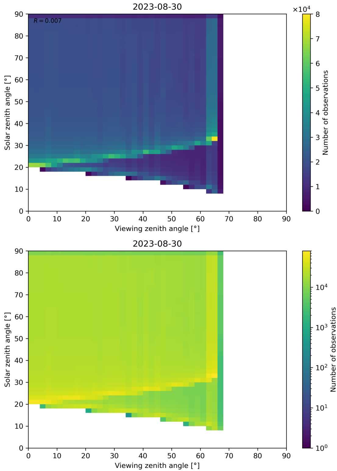
Figure 54: Scatter density plot of “Viewing zenith angle” against “Solar zenith angle” for 2023-08-30 to 2023-08-31.
