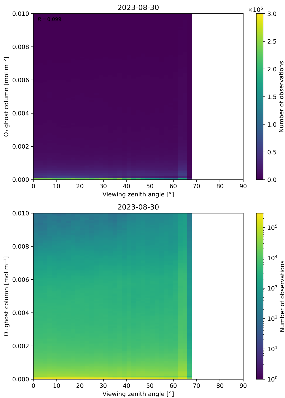
Figure 51: Scatter density plot of “Viewing zenith angle” against “O 3 ghost column” for 2023-08-30 to 2023-08-31.
