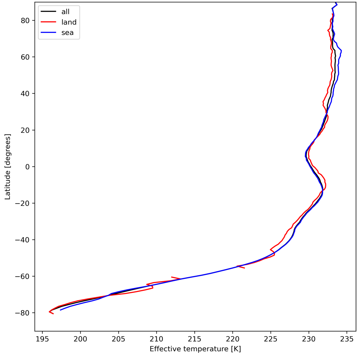
Figure 17: Zonal average of "Effective temperature" for 2023-08-30 to 2023-08-31.
