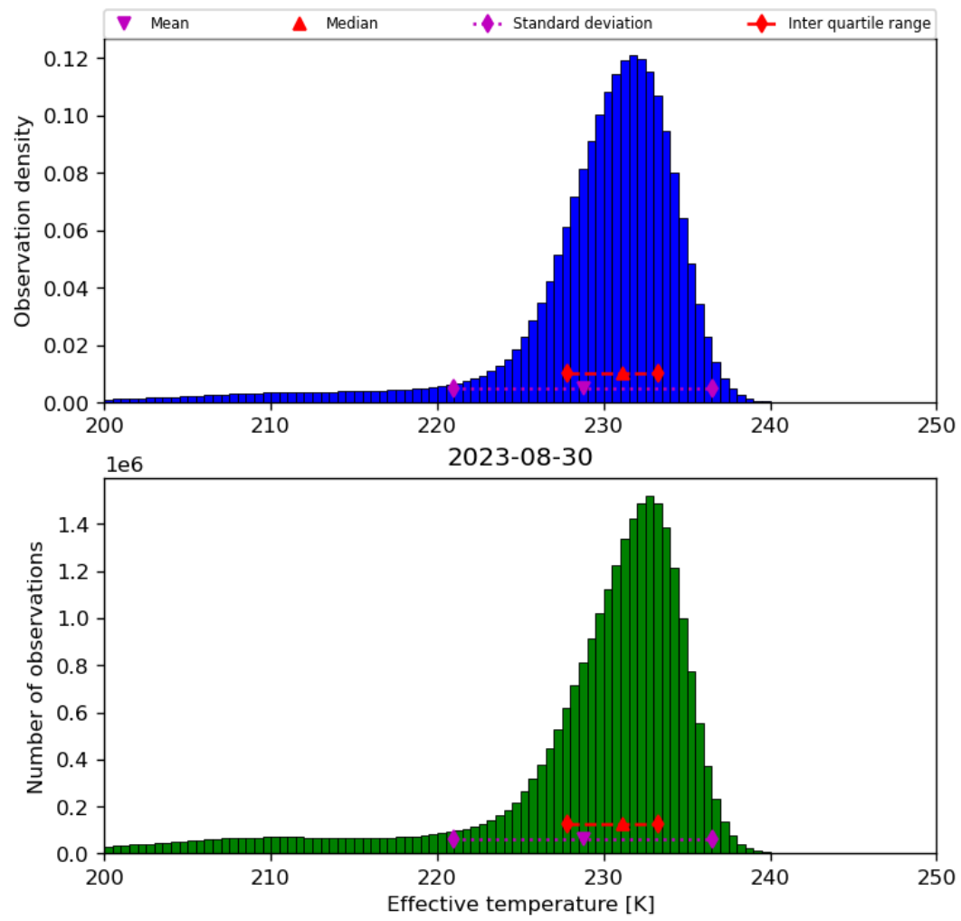
Figure 24: Histogram of “Effective temperature” for 2023-08-30 to 2023-08-31
