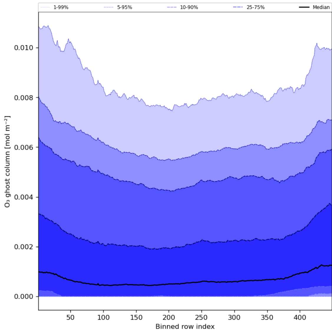
Figure 32: Along track statistics of “O 3 ghost column” for 2023-08-30 to 2023-08-31
