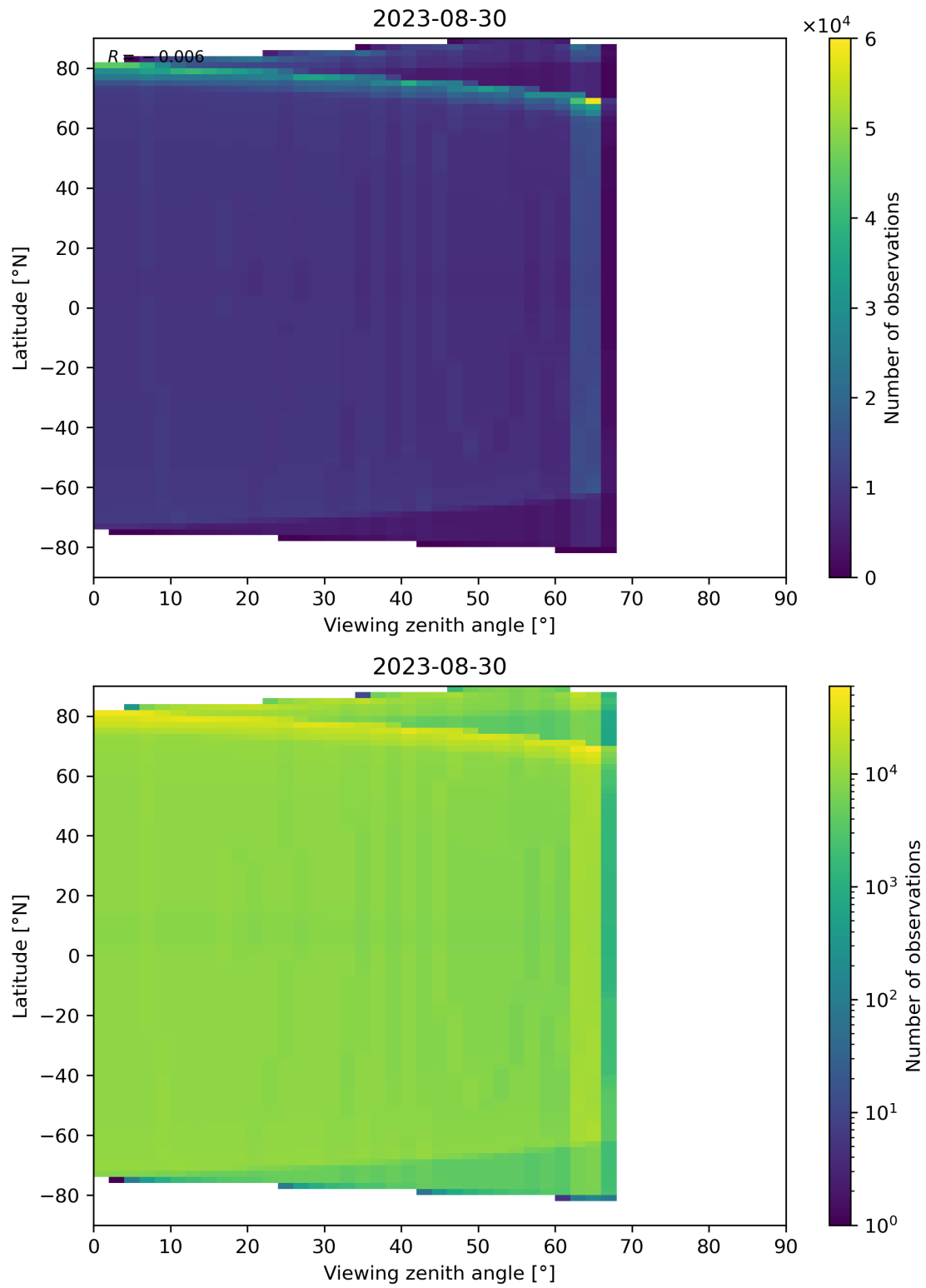
Figure 49: Scatter density plot of “Viewing zenith angle” against “Latitude” for 2023-08-30 to 2023-08-31.
