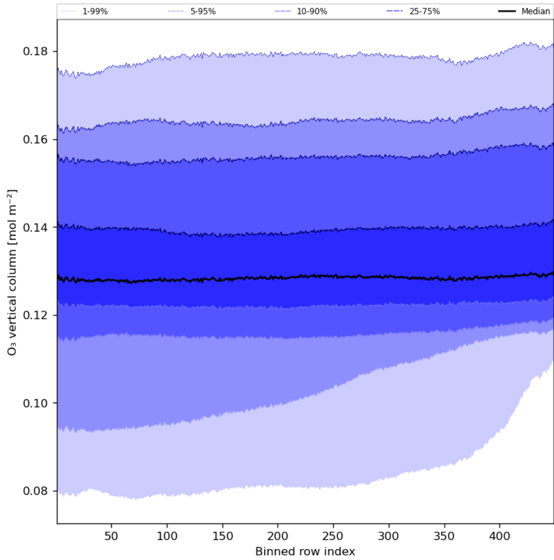
Figure 28: Along track statistics of “O 3 vertical column” for 2023-08-30 to 2023-08-31
