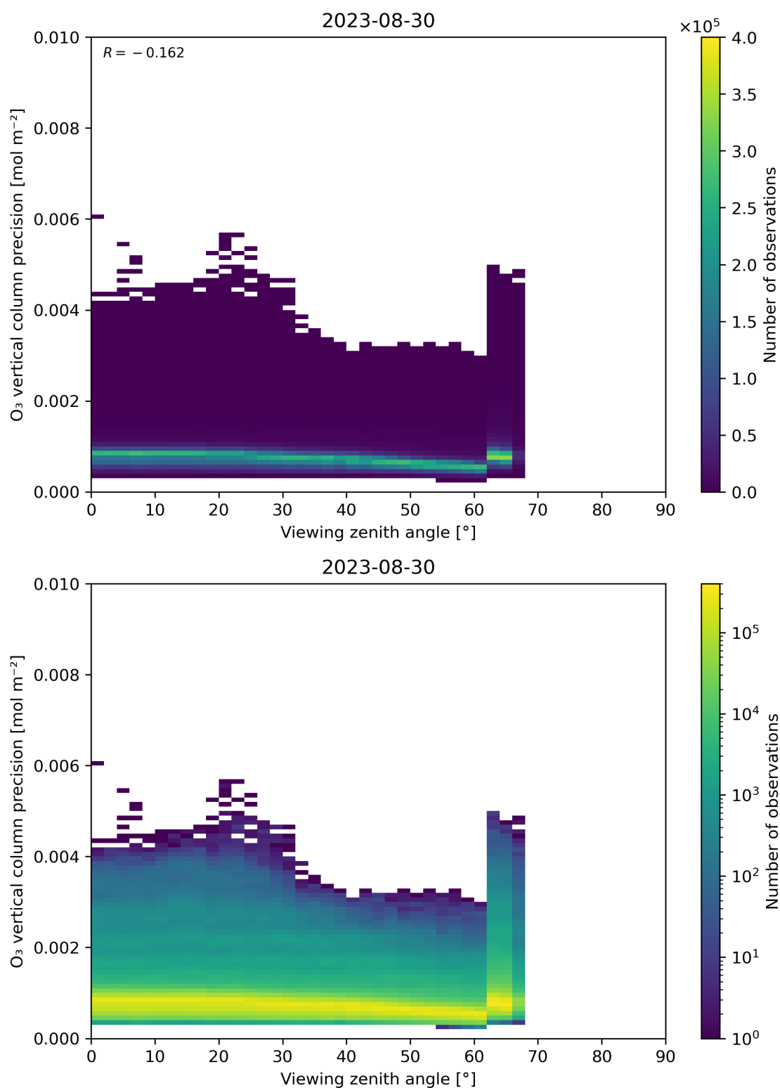
Figure 53: Scatter density plot of “Viewing zenith angle” against “O 3 vertical column precision” for 2023-08-30 to 2023-08-31.
