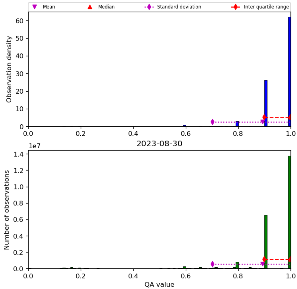
Figure 20: Histogram of “QA value” for 2023-08-30 to 2023-08-31
