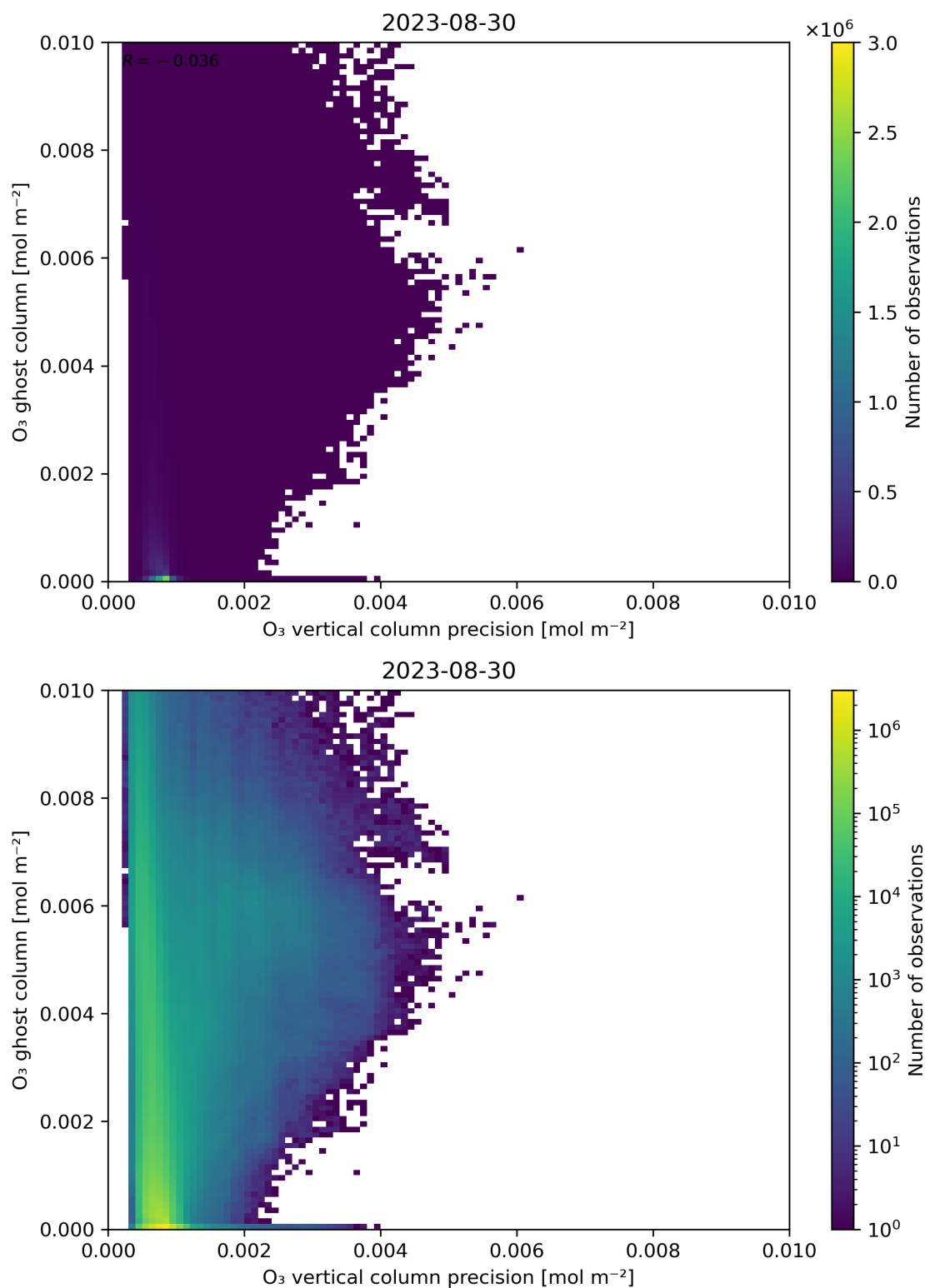
Figure 43: Scatter density plot of “ O_3 vertical column precision” against “ O_3 ghost column” for 2023-08-30 to 2023-08-31.
