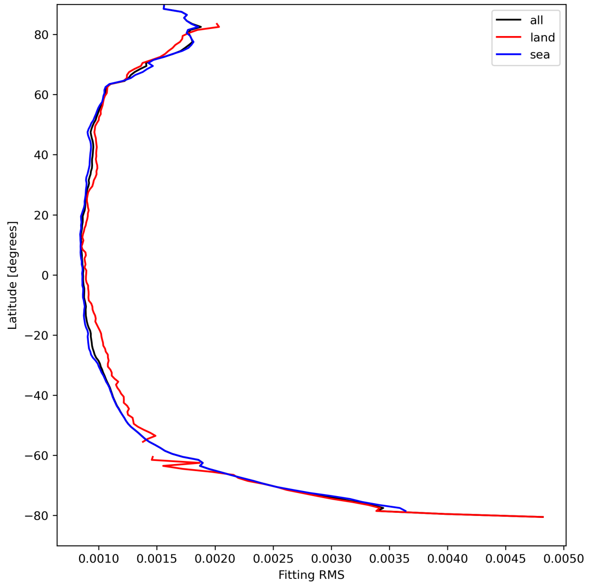
Figure 16: Zonal average of “Fitting RMS” for 2023-08-30 to 2023-08-31.
