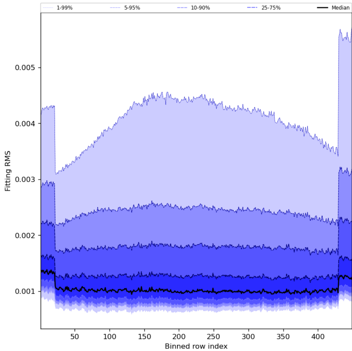
Figure 30: Along track statistics of “Fitting RMS” for 2023-08-30 to 2023-08-31
