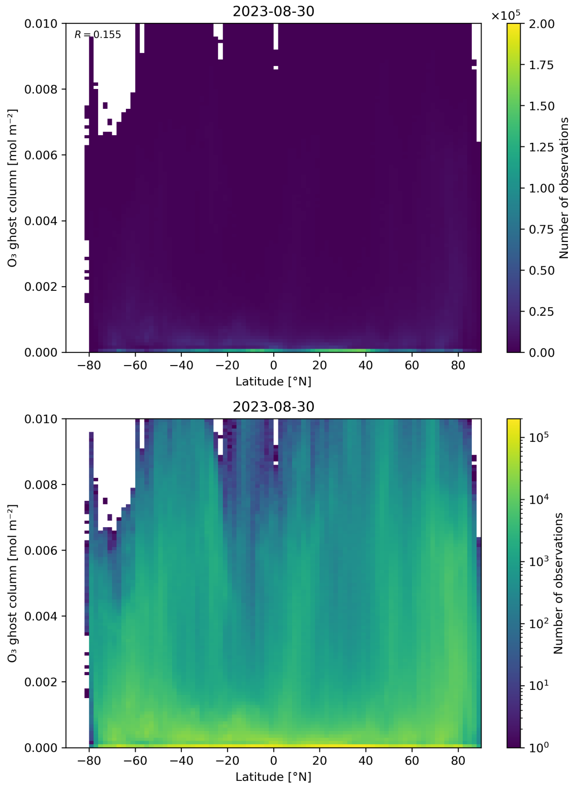
Figure 35: Scatter density plot of “Latitude” against “O 3 ghost column” for 2023-08-30 to 2023-08-31.
