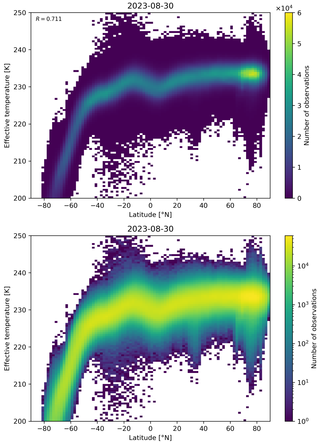
Figure 34: Scatter density plot of “Latitude” against “Effective temperature” for 2023-08-30 to 2023-08-31.
