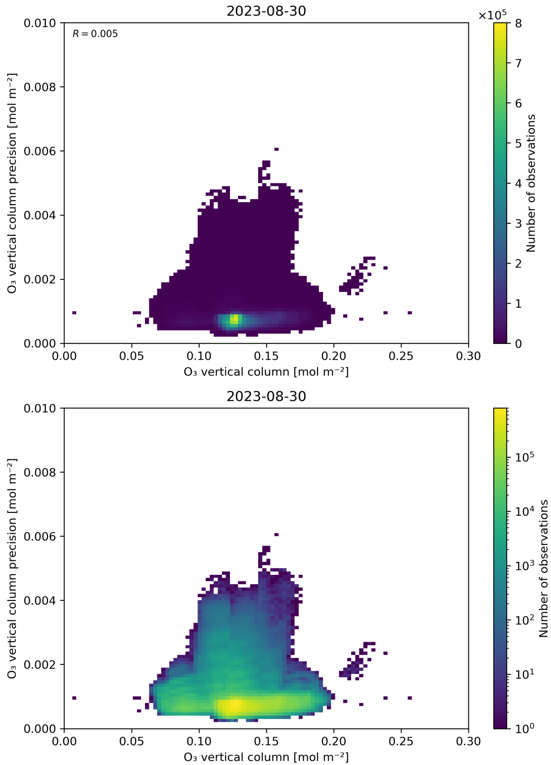
Figure 41: Scatter density plot of “O 3 vertical column” against “O 3 vertical column precision” for 2023-08-30 to 2023-08-31.
