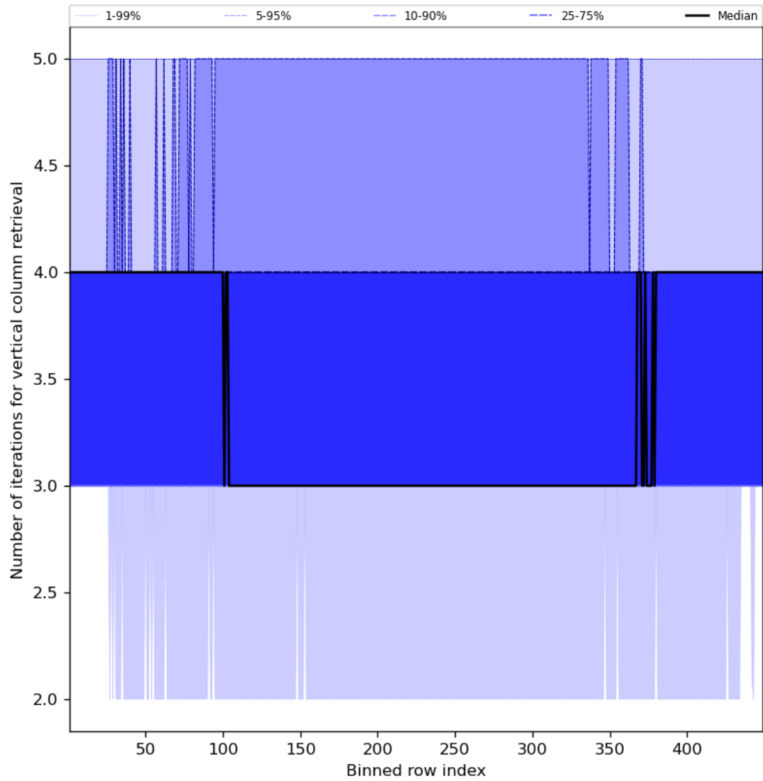
Figure 33: Along track statistics of “Number of iterations for vertical column retrieval” for 2023-08-30 to 2023-08-31
