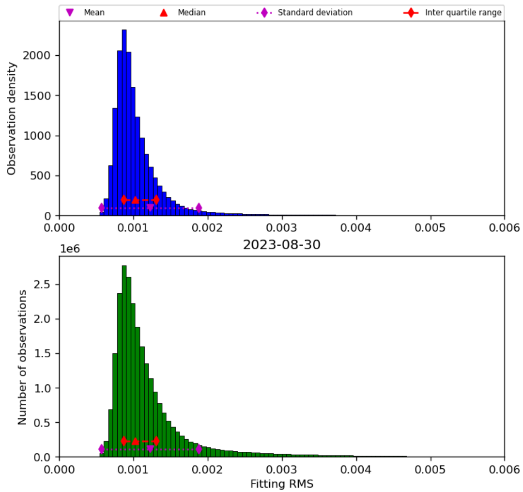
Figure 23: Histogram of “Fitting RMS” for 2023-08-30 to 2023-08-31
