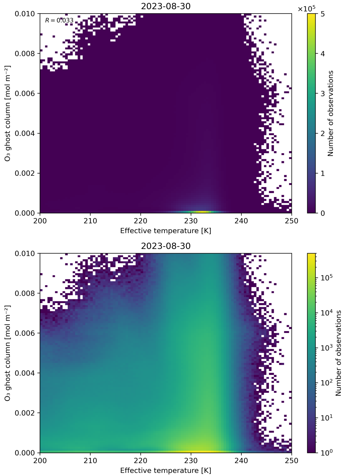
Figure 38: Scatter density plot of “Effective temperature” against “O 3 ghost column” for 2023-08-30 to 2023-08-31.
