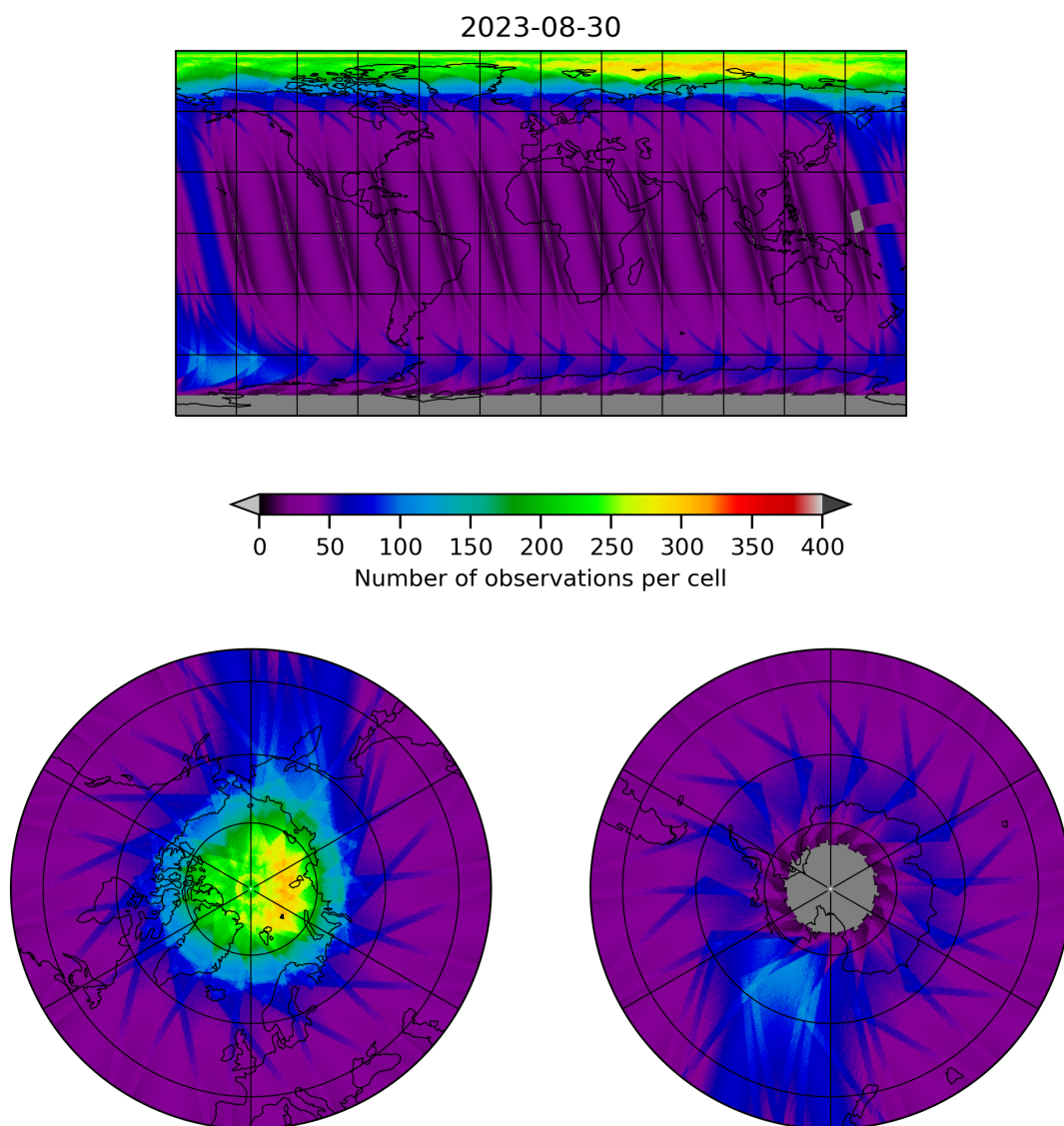
Figure 12: Map of the number of observations for 2023-08-30 to 2023-08-31
