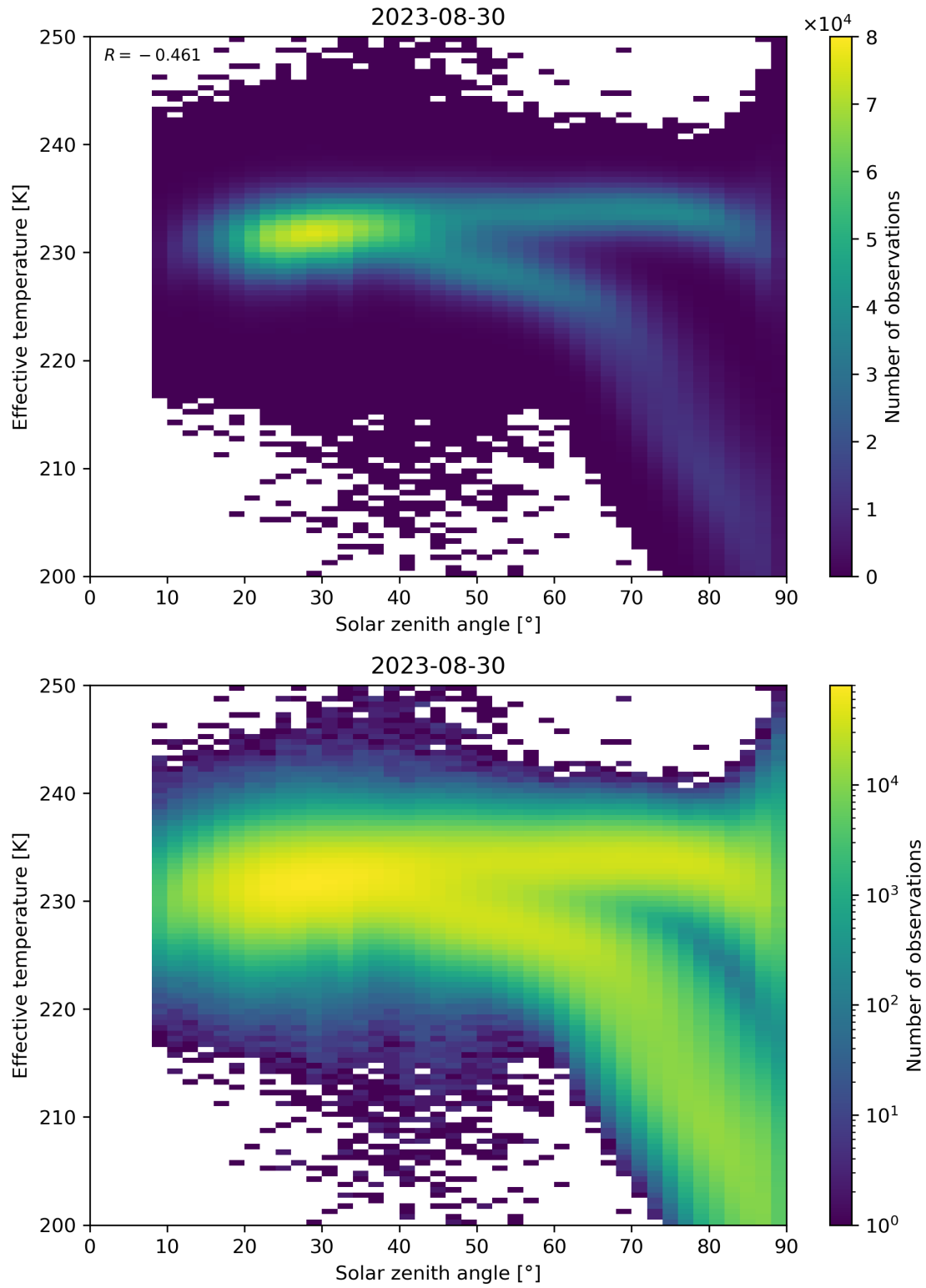
Figure 45: Scatter density plot of “Solar zenith angle” against “Effective temperature” for 2023-08-30 to 2023-08-31.
