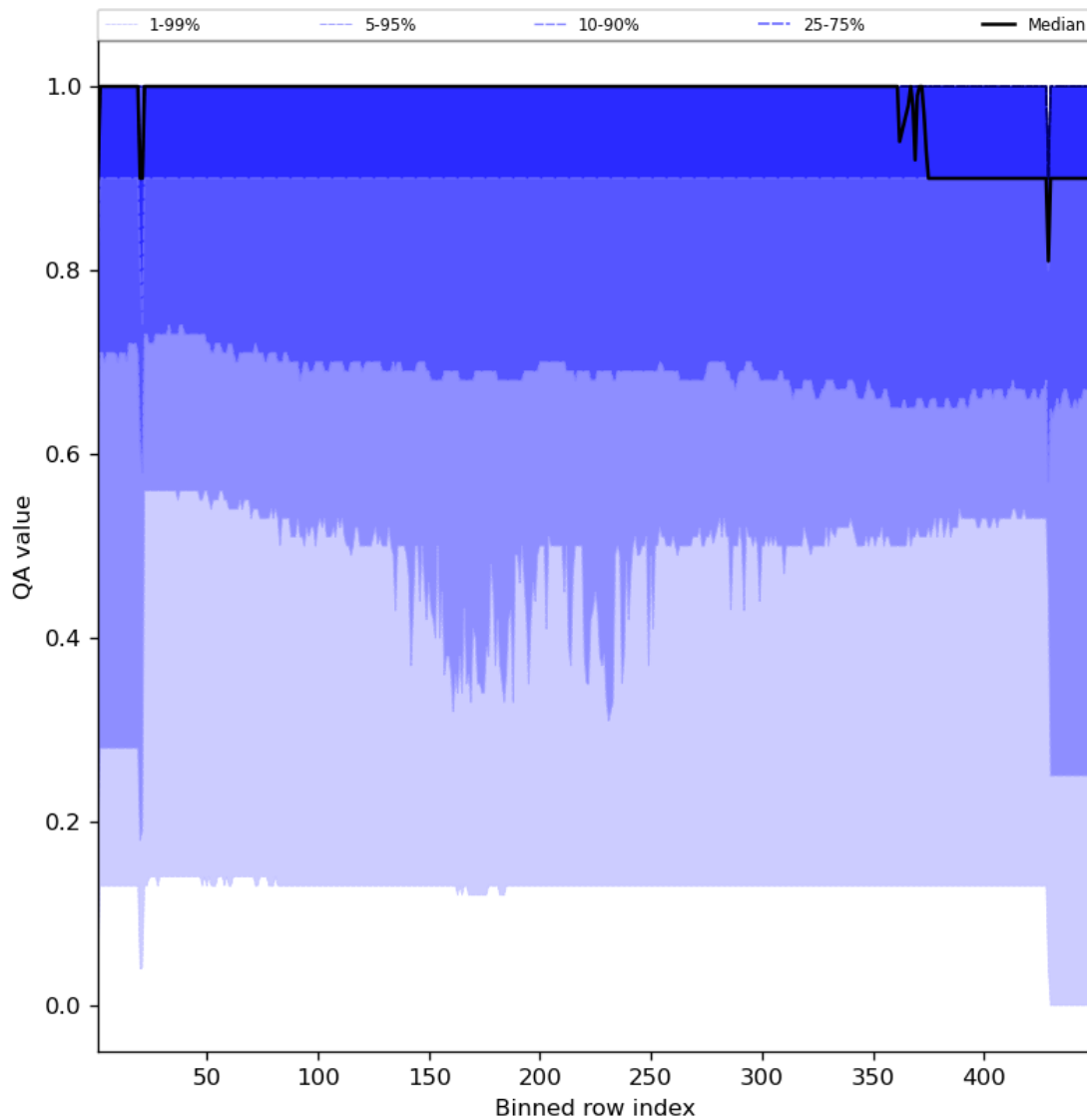
Figure 27: Along track statistics of “QA value” for 2023-08-30 to 2023-08-31
