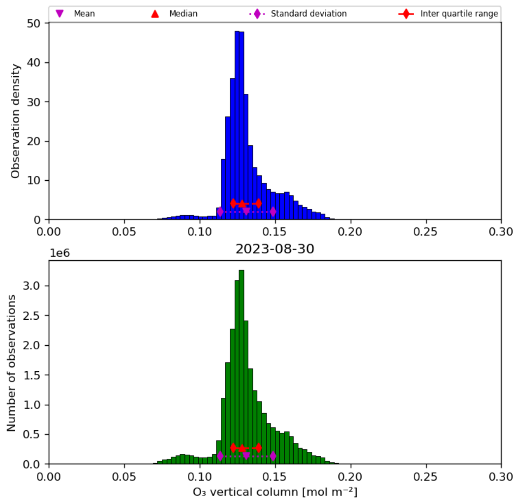
Figure 21: Histogram of “O 3 vertical column” for 2023-08-30 to 2023-08-31
