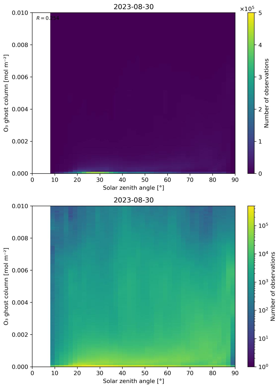
Figure 46: Scatter density plot of “Solar zenith angle” against “O 3 ghost column” for 2023-08-30 to 2023-08-31.
