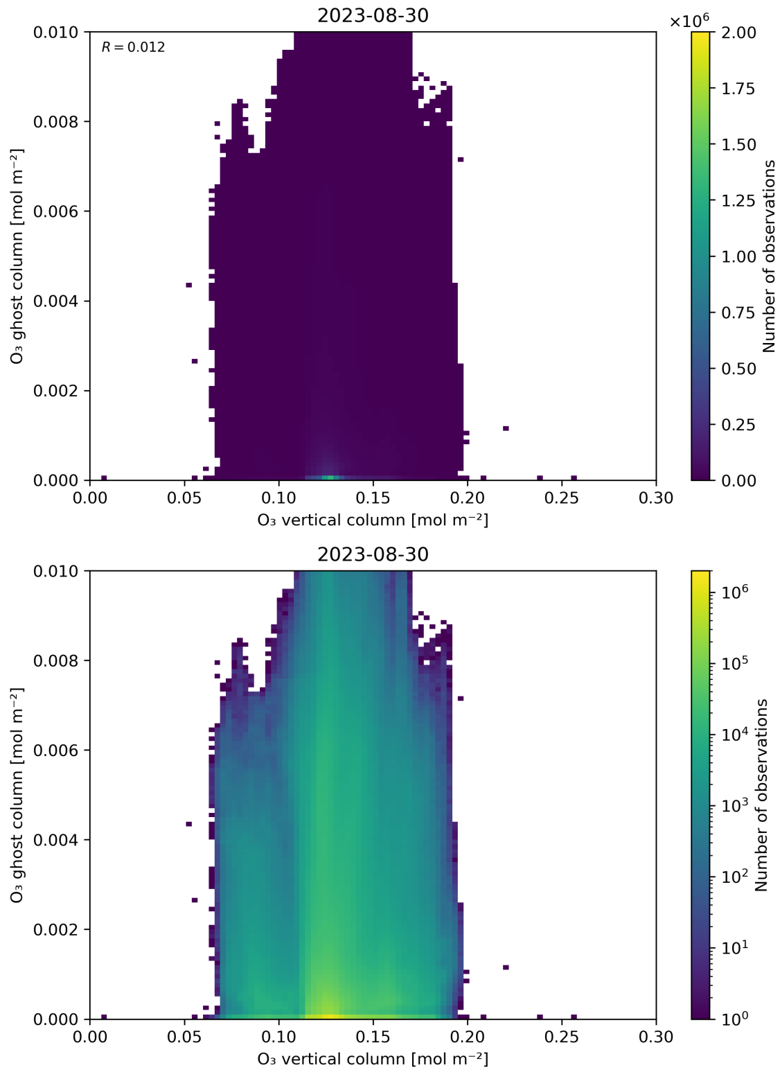
Figure 40: Scatter density plot of “O 3 vertical column” against “O 3 ghost column” for 2023-08-30 to 2023-08-31.
