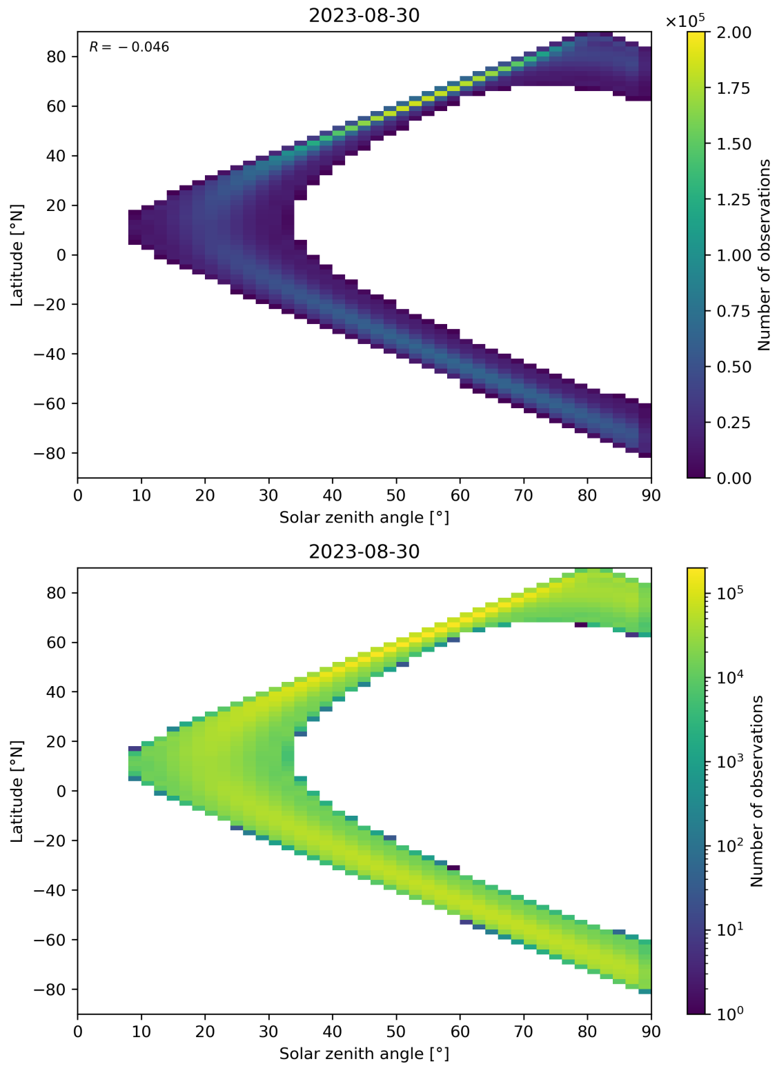
Figure 44: Scatter density plot of “Solar zenith angle” against “Latitude” for 2023-08-30 to 2023-08-31.
