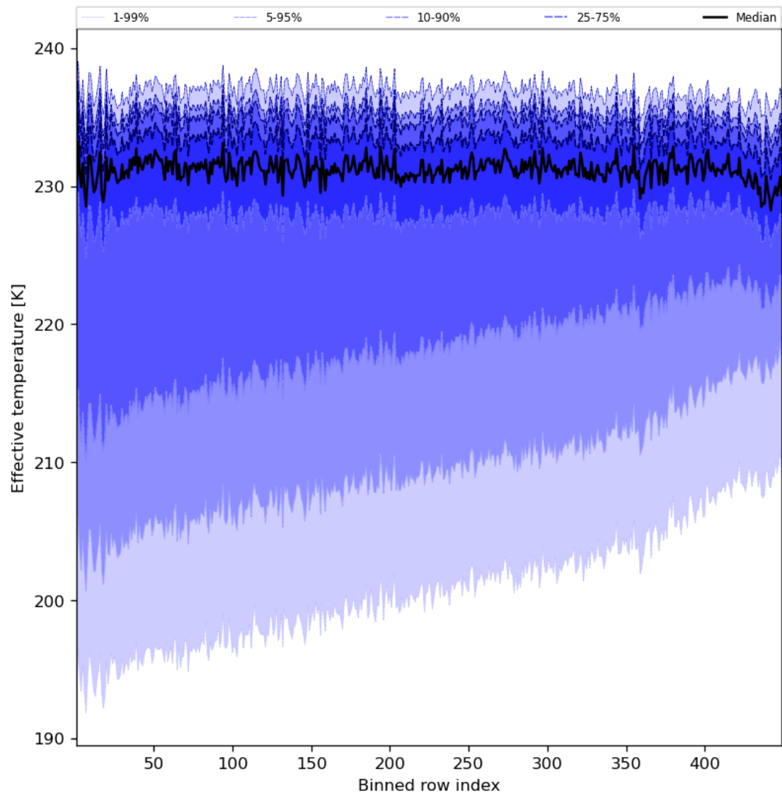
Figure 31: Along track statistics of “Effective temperature” for 2023-08-30 to 2023-08-31
