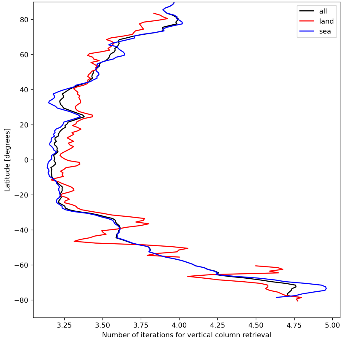
Figure 19: Zonal average of “Number of iterations for vertical column retrieval” for 2023-08-30 to 2023-08-31.
