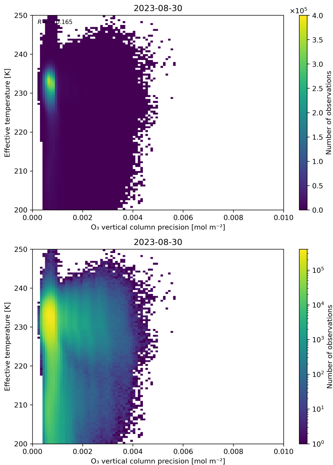
Figure 42: Scatter density plot of “O 3 vertical column precision” against “Effective temperature” for 2023-08-30 to 2023-08-31.
