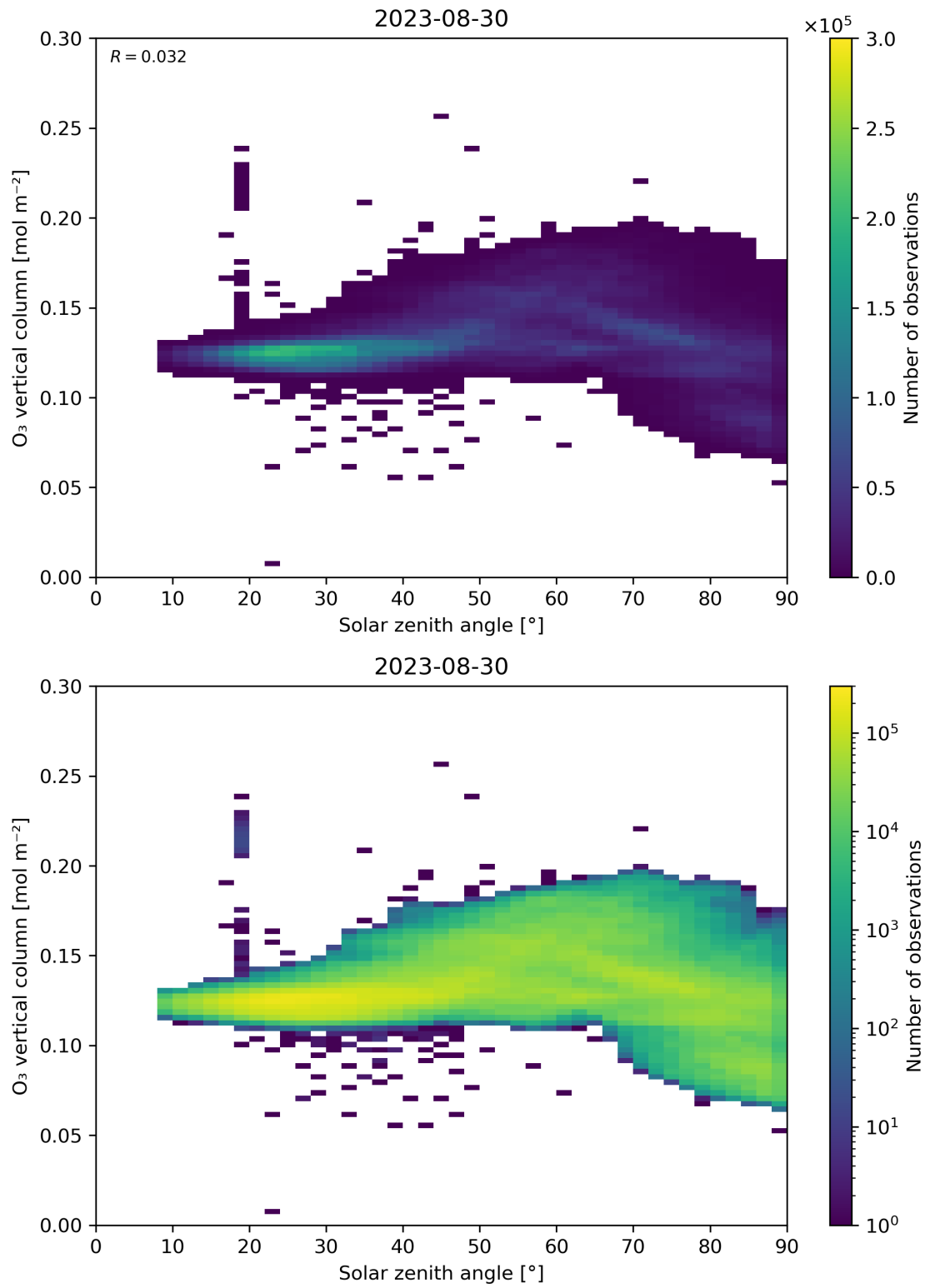
Figure 47: Scatter density plot of “Solar zenith angle” against “O 3 vertical column” for 2023-08-30 to 2023-08-31.
