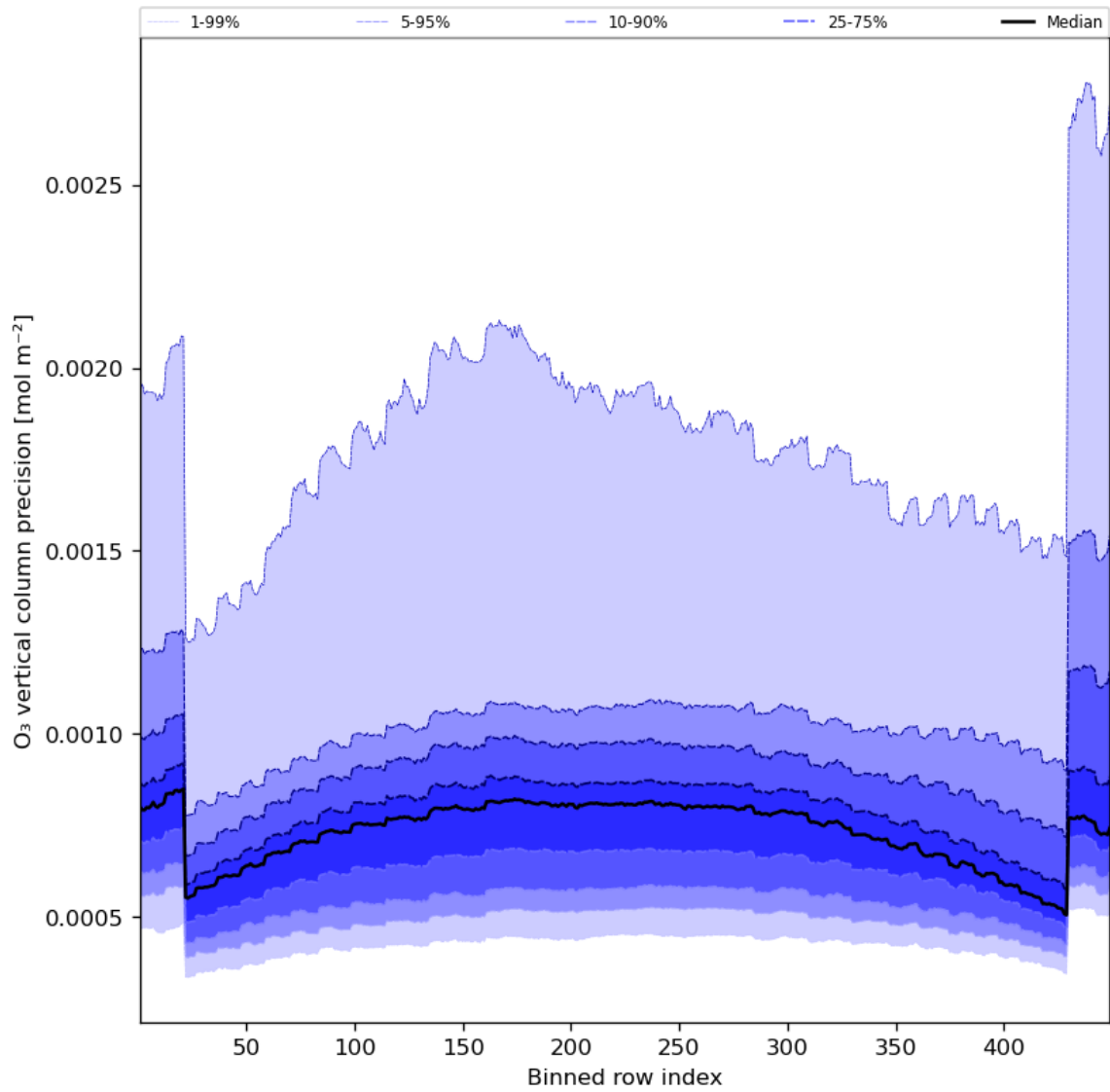
Figure 29: Along track statistics of “O 3 vertical column precision” for 2023-08-30 to 2023-08-31
