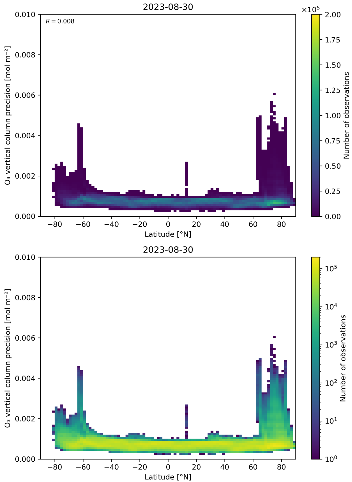
Figure 37: Scatter density plot of “Latitude” against “O 3 vertical column precision” for 2023-08-30 to 2023-08-31.
