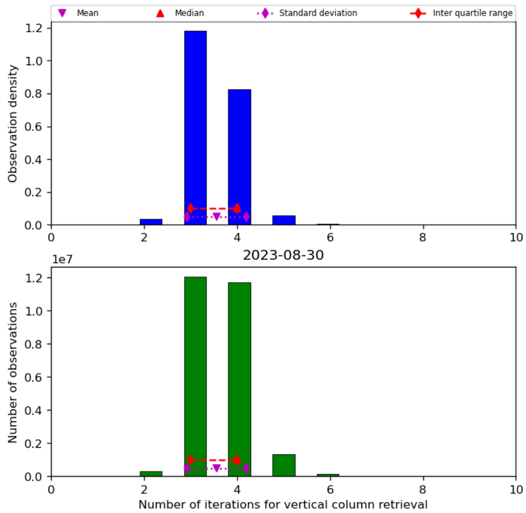
Figure 26: Histogram of “Number of iterations for vertical column retrieval” for 2023-08-30 to 2023-08-31
