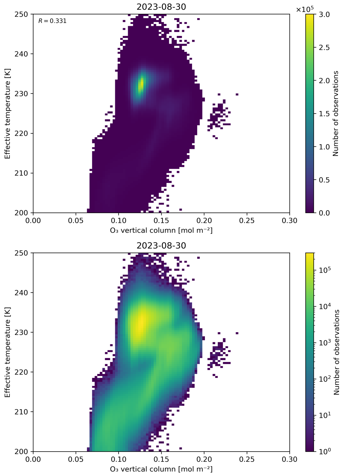
Figure 39: Scatter density plot of “O 3 vertical column” against “Effective temperature” for 2023-08-30 to 2023-08-31.
