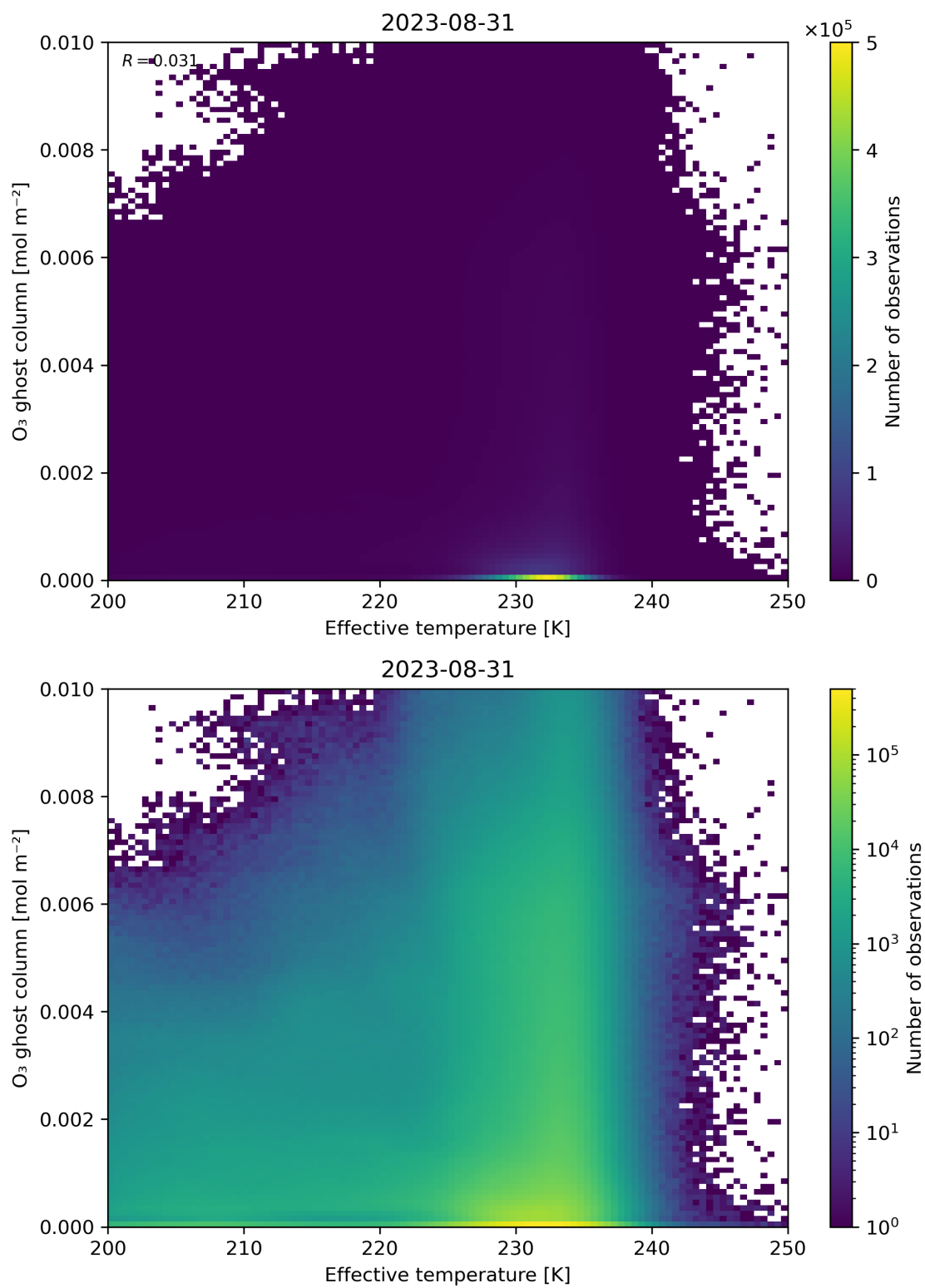
Figure 38: Scatter density plot of “Effective temperature” against “O 3 ghost column” for 2023-08-30 to 2023-09-01.
