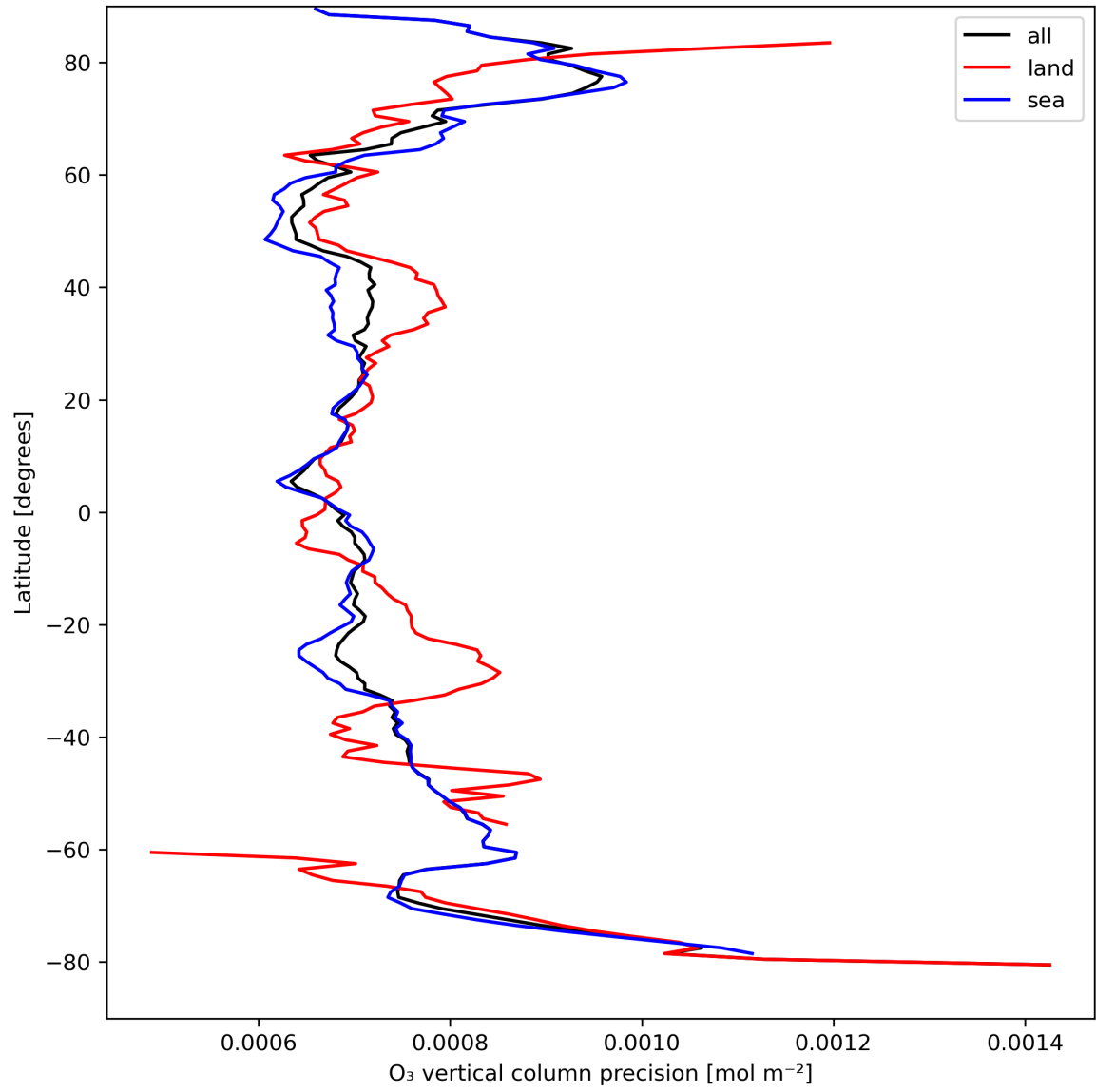
Figure 15: Zonal average of “O 3 vertical column precision” for 2023-08-30 to 2023-09-01.
