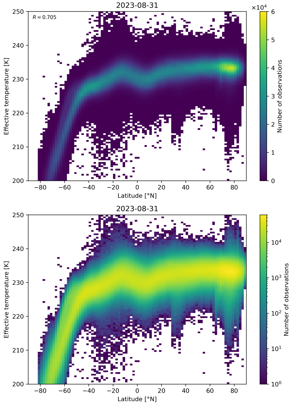
Figure 34: Scatter density plot of “Latitude” against “Effective temperature” for 2023-08-30 to 2023-09-01.
