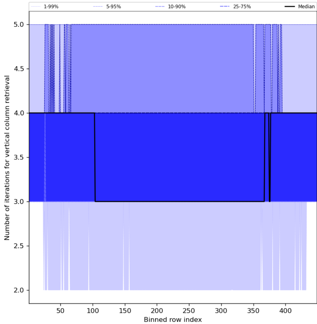
Figure 33: Along track statistics of “Number of iterations for vertical column retrieval” for 2023-08-30 to 2023-09-01
