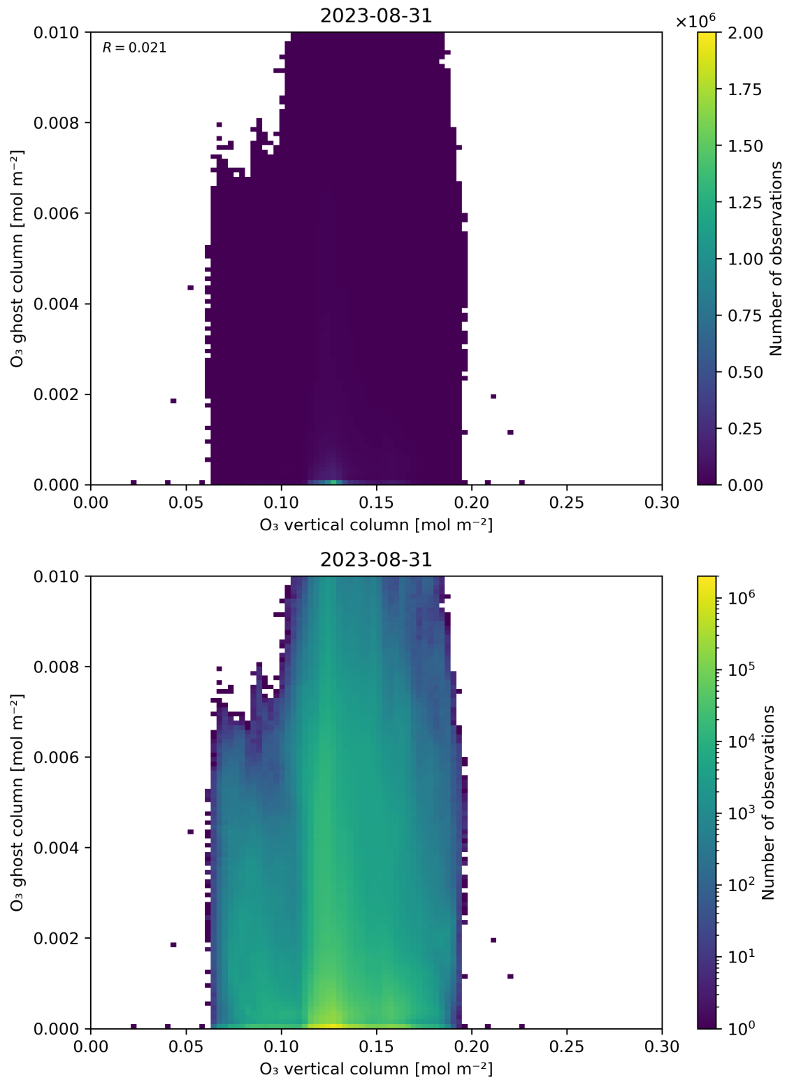
Figure 40: Scatter density plot of “O 3 vertical column” against “O 3 ghost column” for 2023-08-30 to 2023-09-01.
