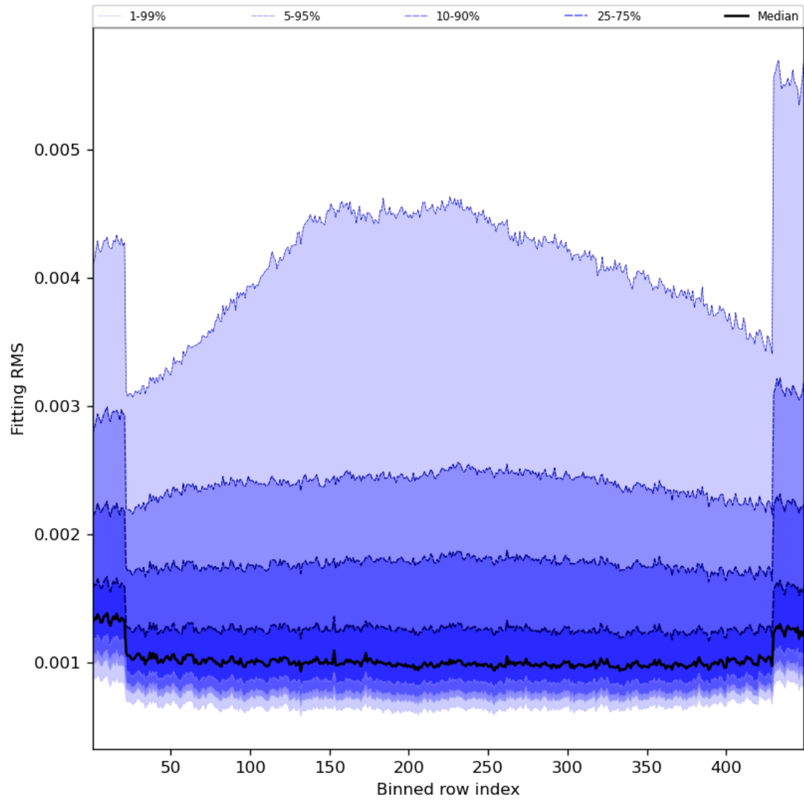
Figure 30: Along track statistics of “Fitting RMS” for 2023-08-30 to 2023-09-01
