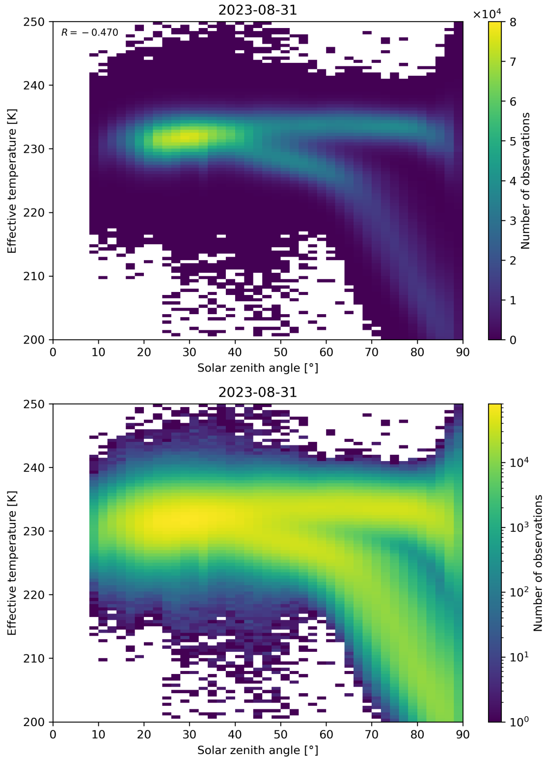
Figure 45: Scatter density plot of “Solar zenith angle” against “Effective temperature” for 2023-08-30 to 2023-09-01.
