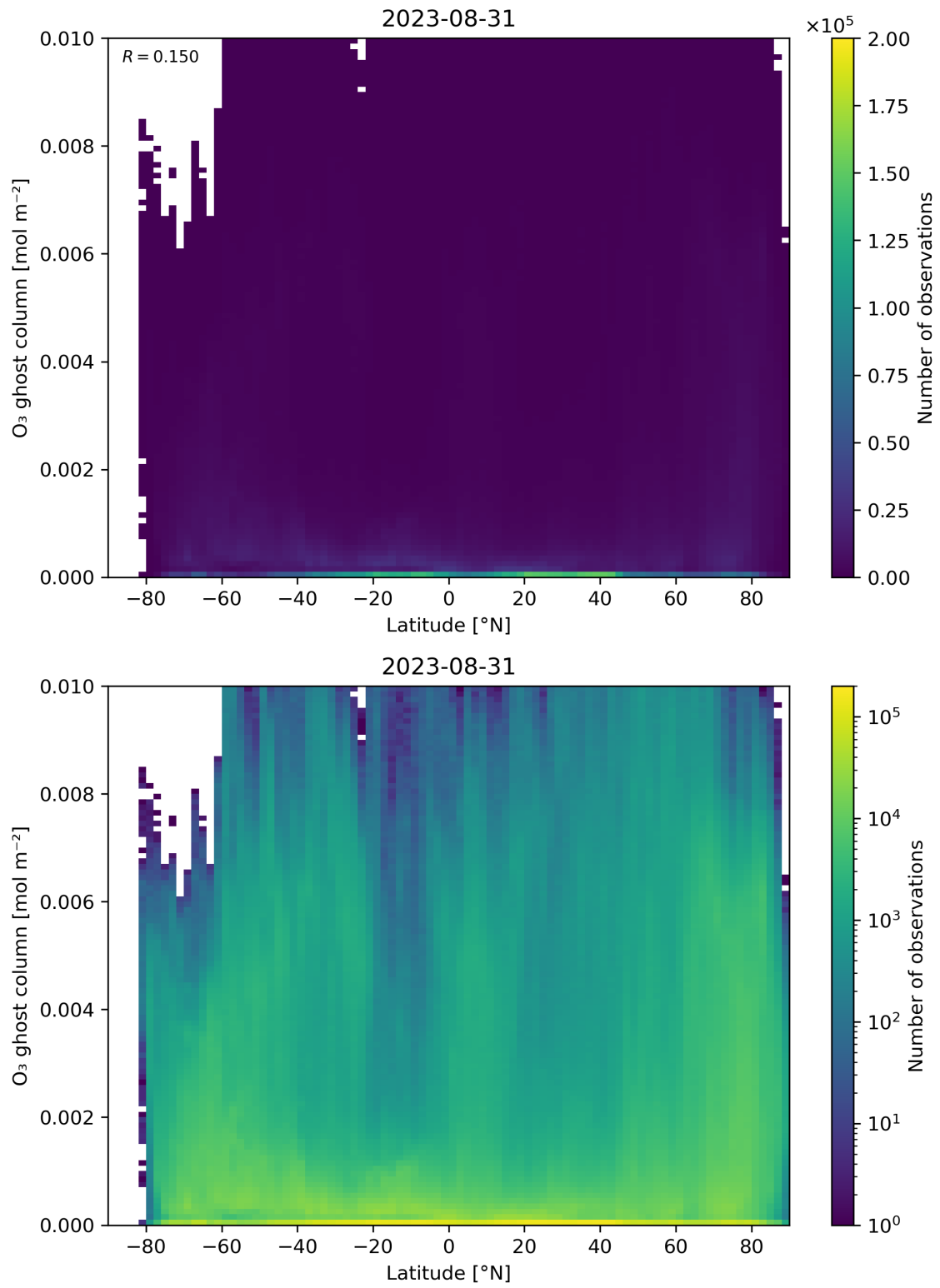
Figure 35: Scatter density plot of “Latitude” against “O 3 ghost column” for 2023-08-30 to 2023-09-01.
