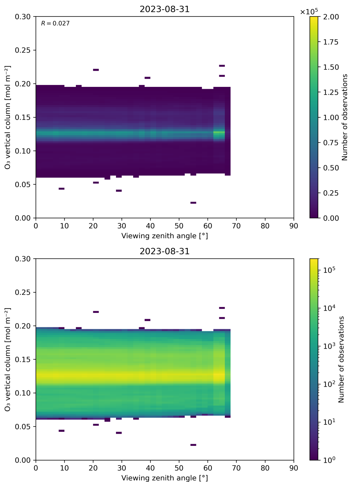
Figure 52: Scatter density plot of “Viewing zenith angle” against “O 3 vertical column” for 2023-08-30 to 2023-09-01.
