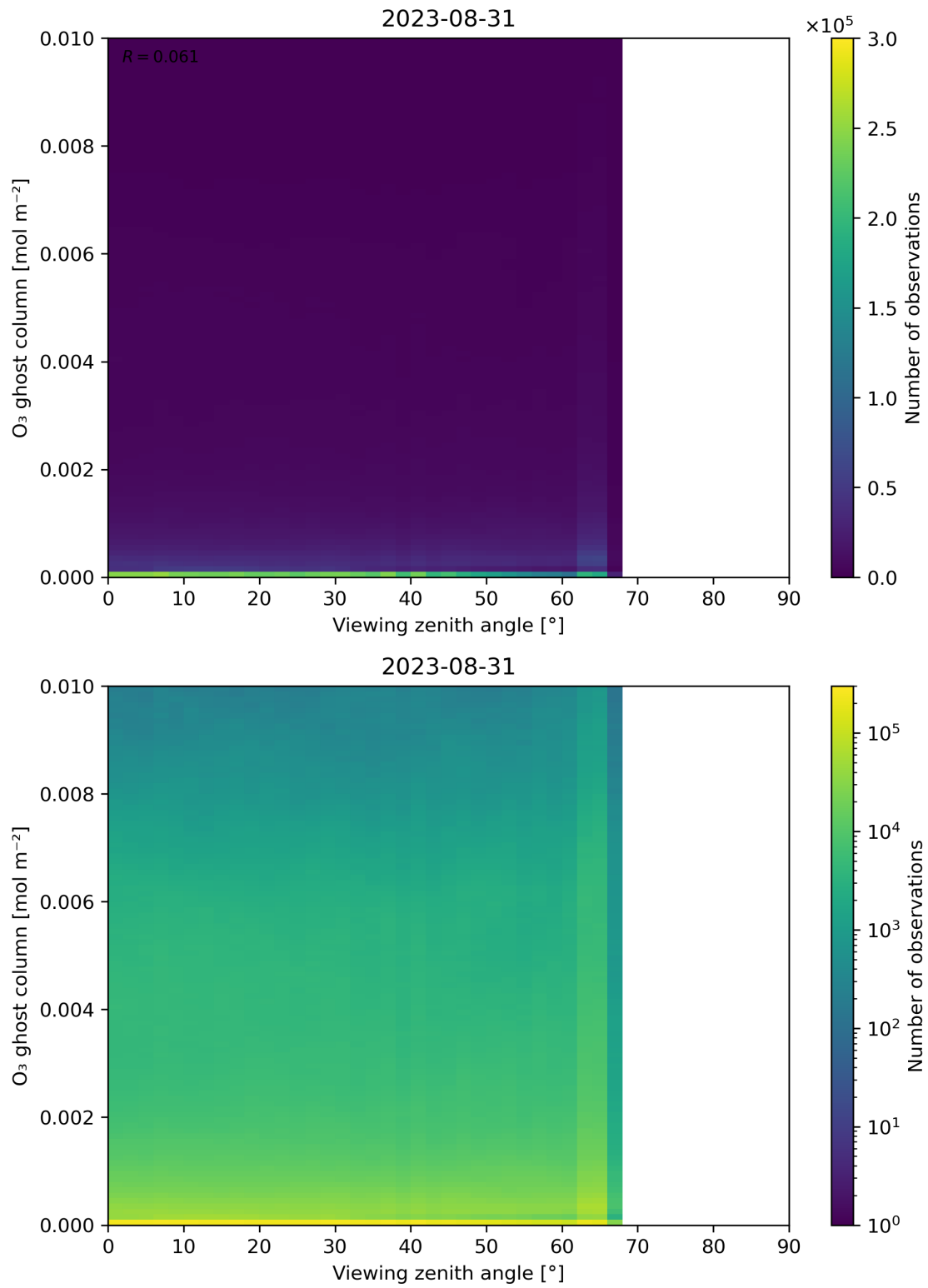
Figure 51: Scatter density plot of “Viewing zenith angle” against “O 3 ghost column” for 2023-08-30 to 2023-09-01.
