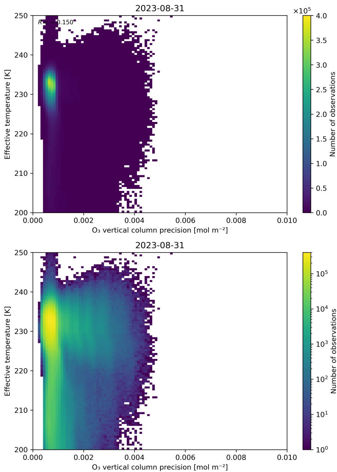
Figure 42: Scatter density plot of “O 3 vertical column precision” against “Effective temperature” for 2023-08-30 to 2023-09-01.
