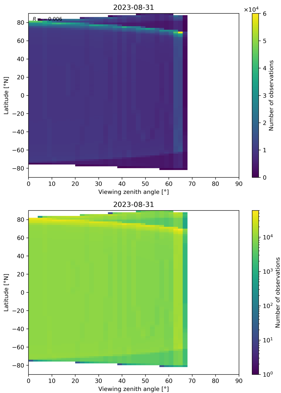
Figure 49: Scatter density plot of “Viewing zenith angle” against “Latitude” for 2023-08-30 to 2023-09-01.
