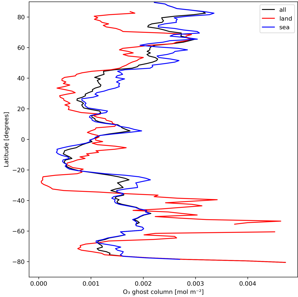
Figure 18: Zonal average of "O 3 ghost column" for 2023-08-30 to 2023-09-01.
