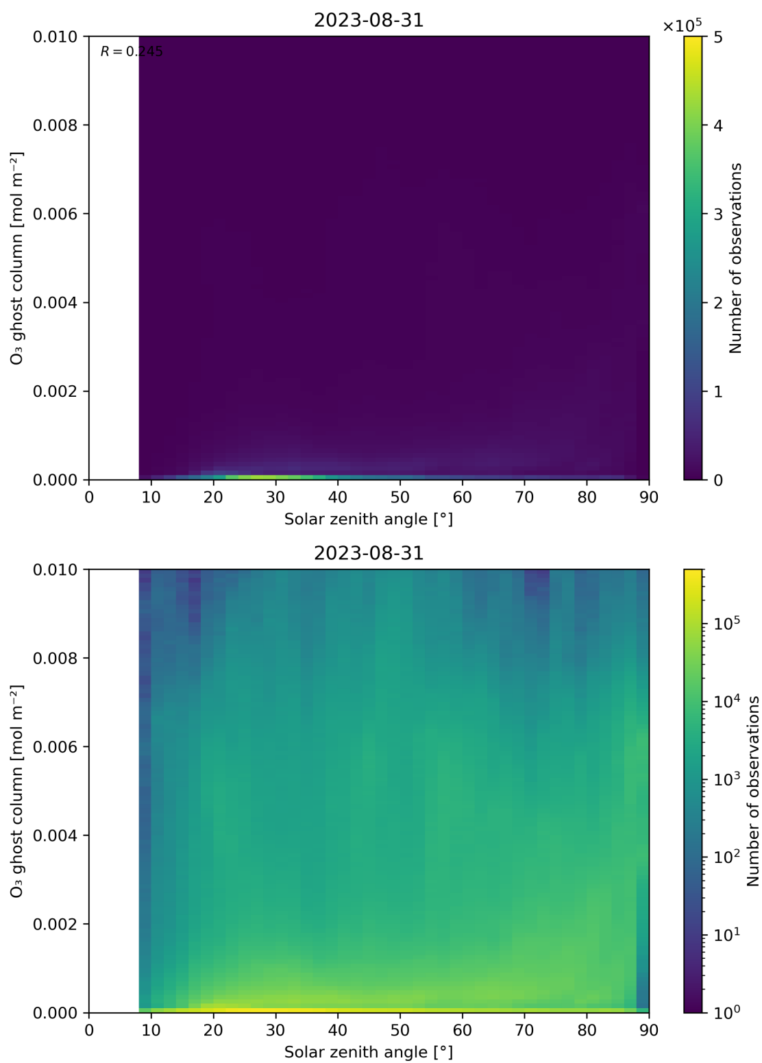
Figure 46: Scatter density plot of “Solar zenith angle” against “O 3 ghost column” for 2023-08-30 to 2023-09-01.
