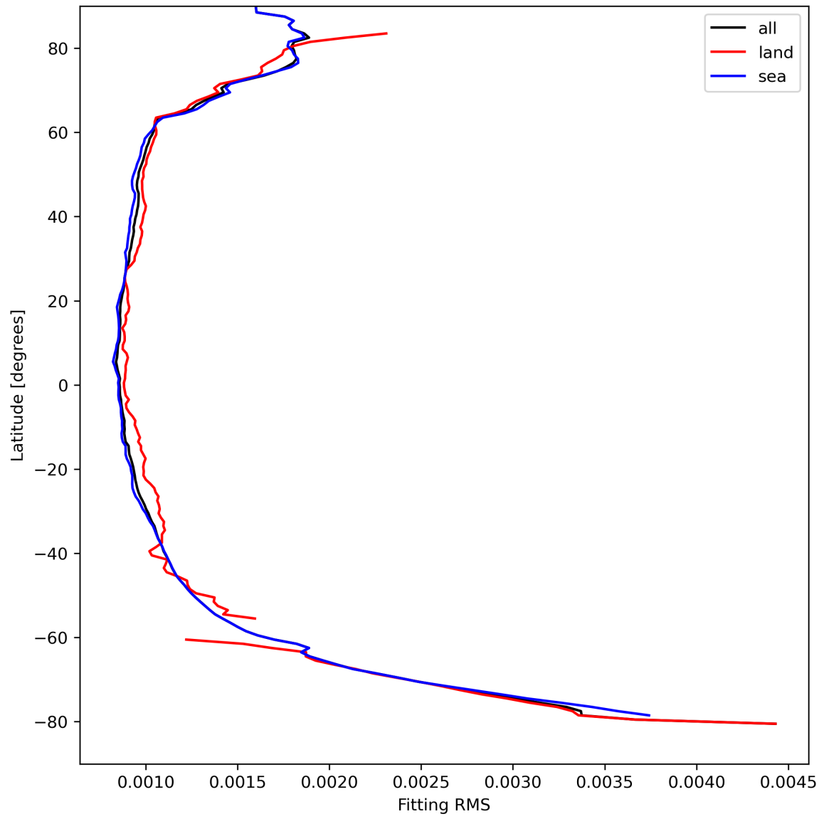
Figure 16: Zonal average of “Fitting RMS” for 2023-08-30 to 2023-09-01.
