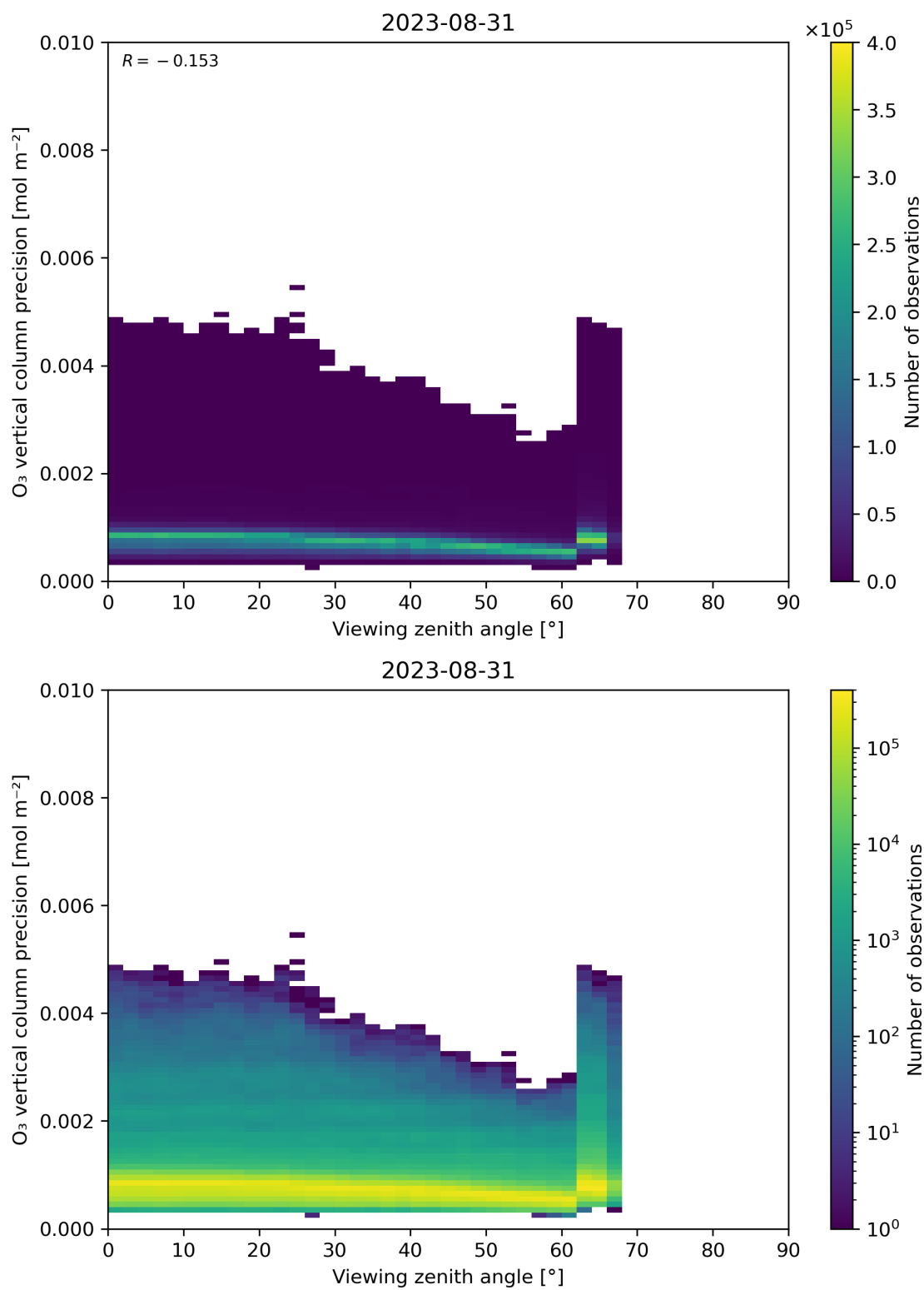
Figure 53: Scatter density plot of “Viewing zenith angle” against “O 3 vertical column precision” for 2023-08-30 to 2023-09-01.
