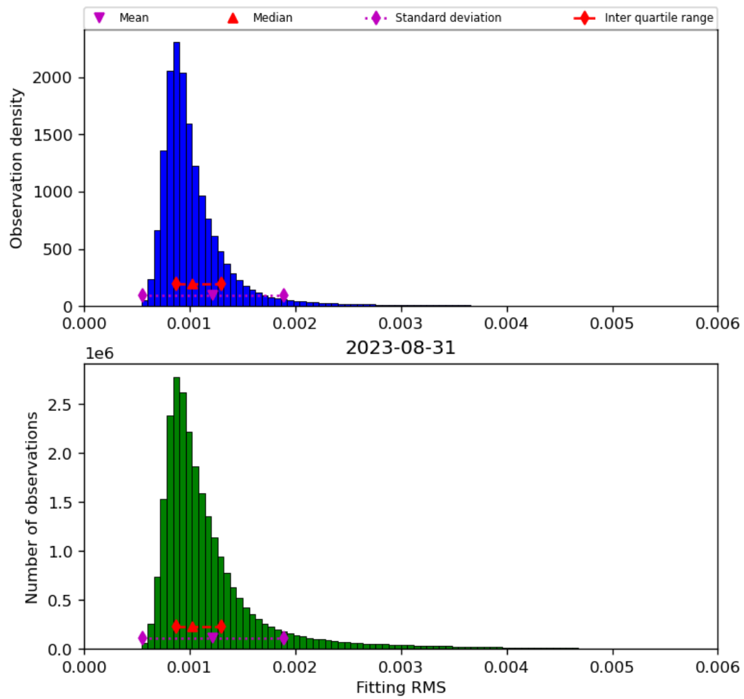
Figure 23: Histogram of “Fitting RMS” for 2023-08-30 to 2023-09-01
