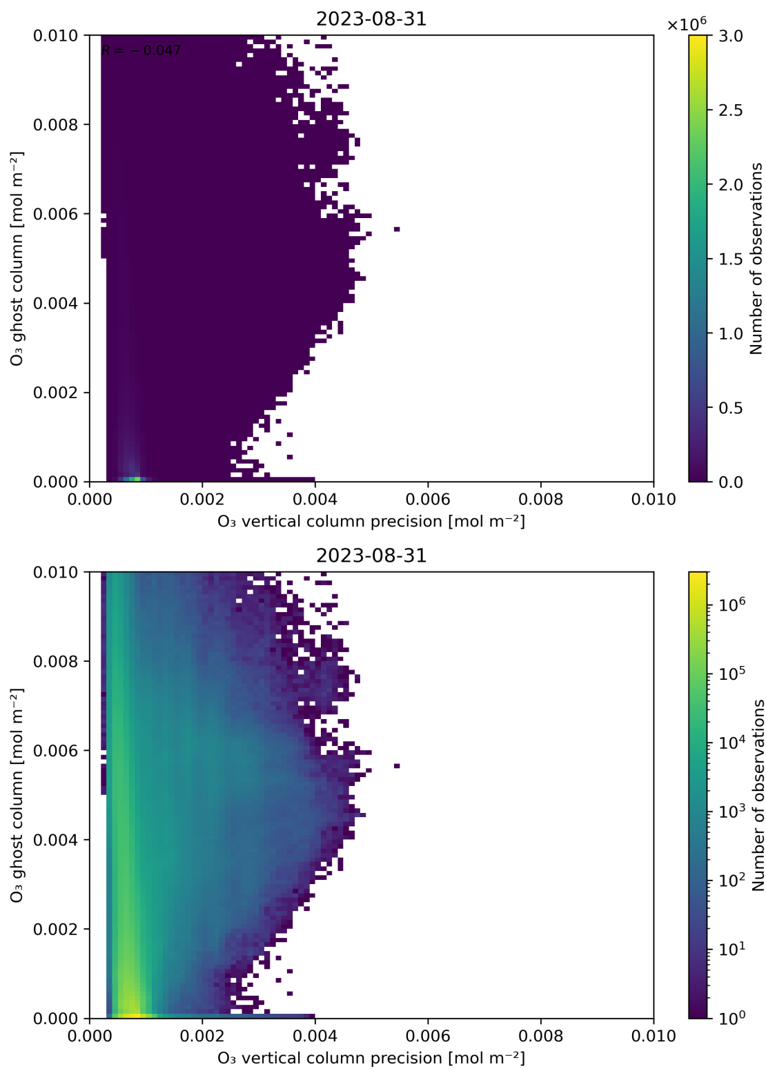
Figure 43: Scatter density plot of “ O_3 vertical column precision” against “ O_3 ghost column” for 2023-08-30 to 2023-09-01.
