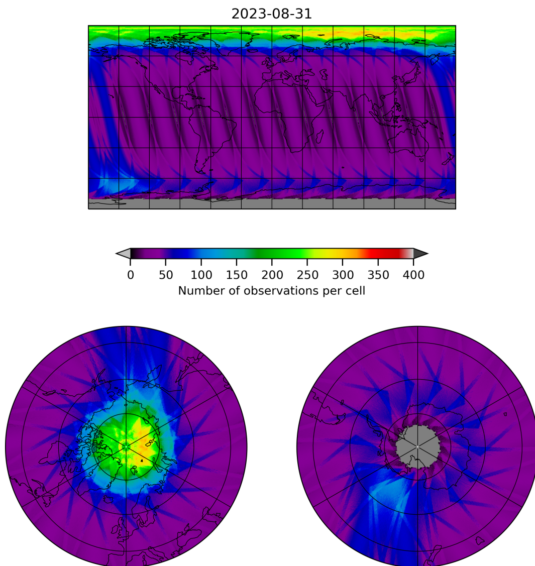
Figure 12: Map of the number of observations for 2023-08-30 to 2023-09-01
