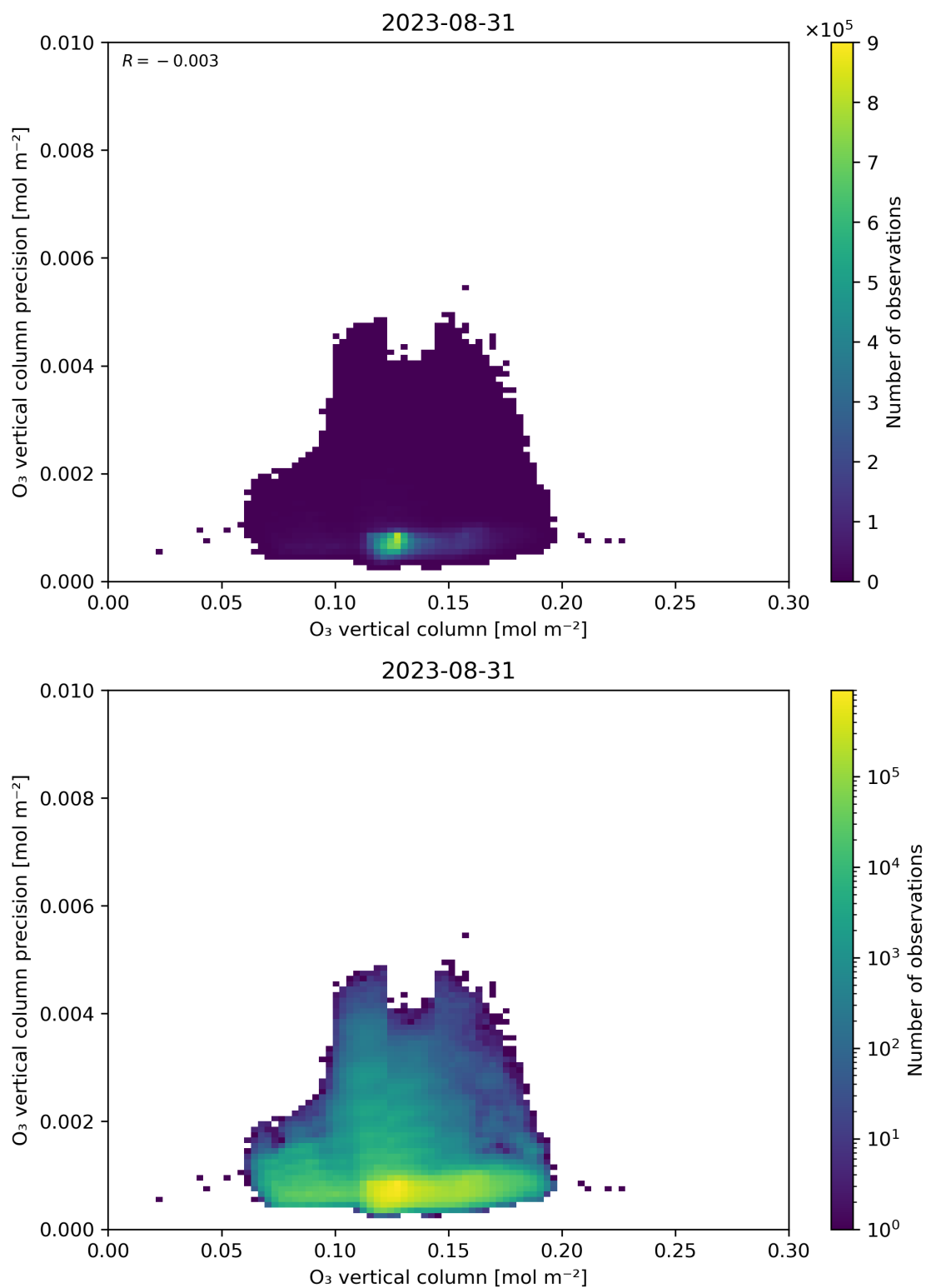
Figure 41: Scatter density plot of “O 3 vertical column” against “O 3 vertical column precision” for 2023-08-30 to 2023-09-01.
