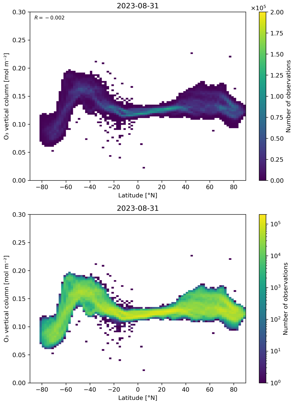
Figure 36: Scatter density plot of “Latitude” against “O 3 vertical column” for 2023-08-30 to 2023-09-01.
