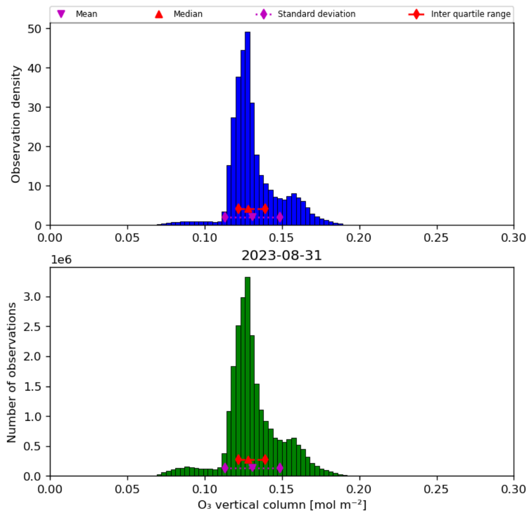
Figure 21: Histogram of “O 3 vertical column” for 2023-08-30 to 2023-09-01
