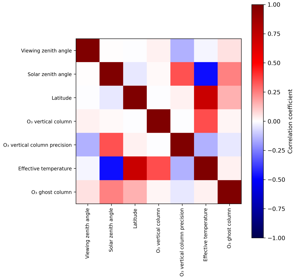
Figure 2: Map of correlation matrix for 2023-08-30 to 2023-09-01.
