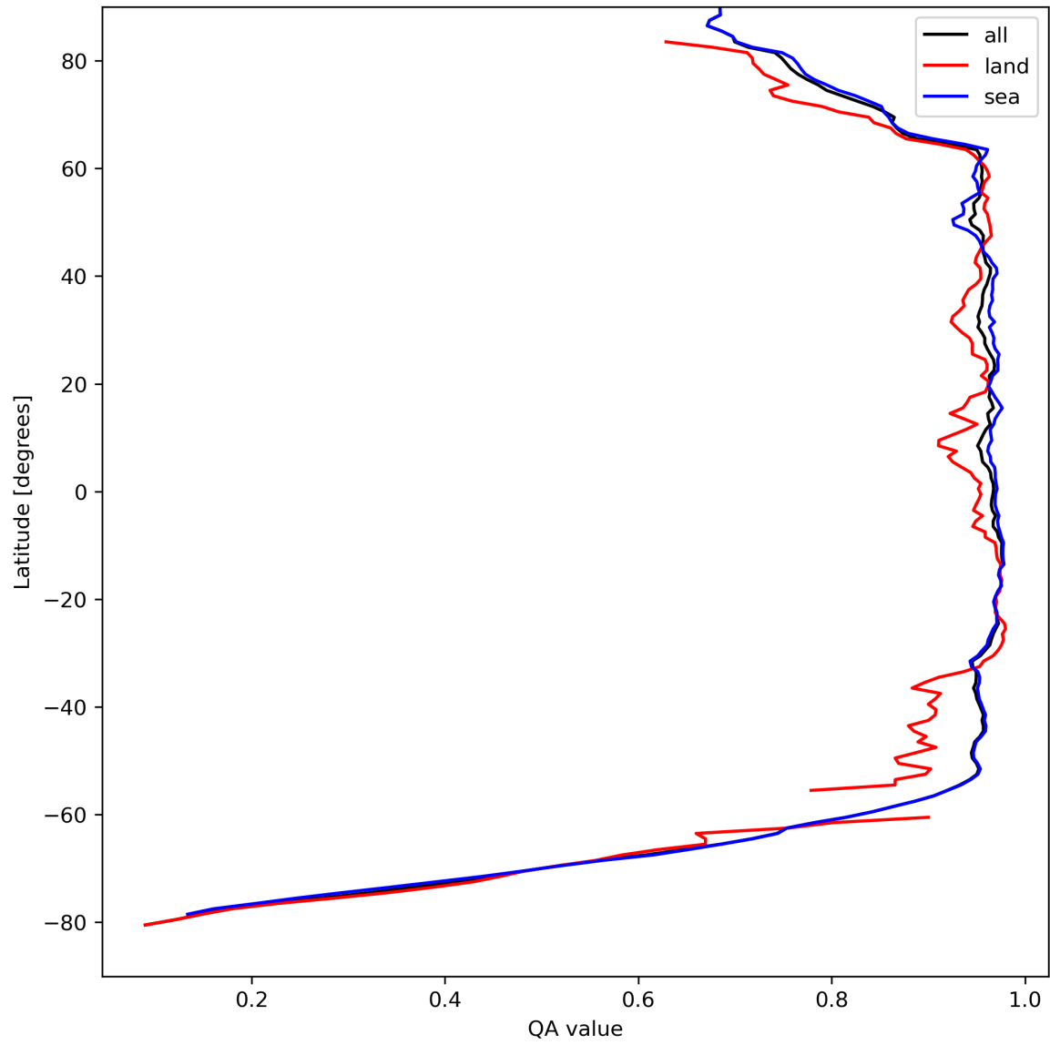
Figure 13: Zonal average of “QA value” for 2023-08-30 to 2023-09-01.
