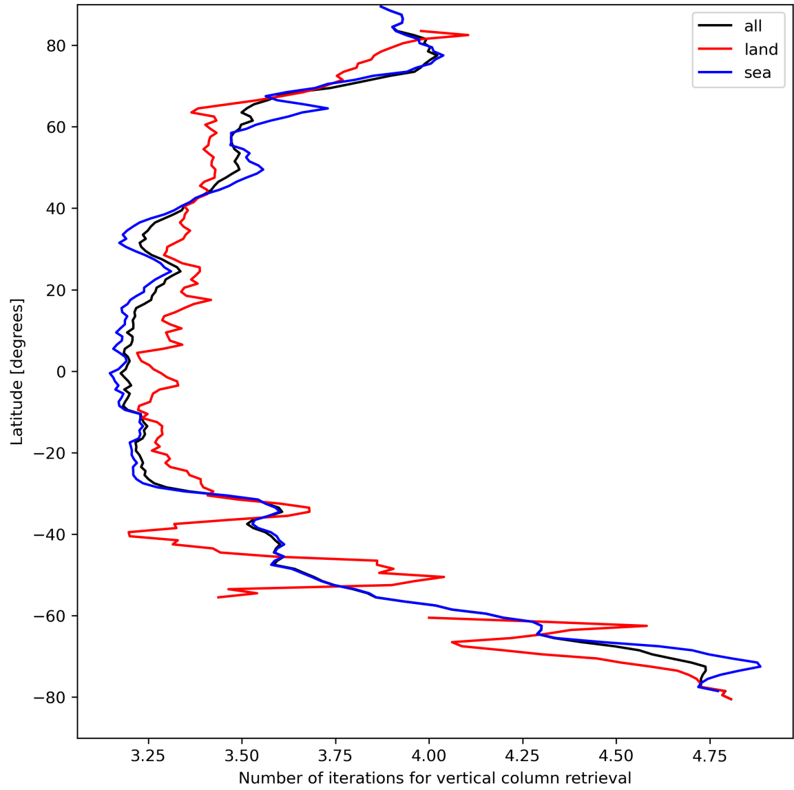
Figure 19: Zonal average of “Number of iterations for vertical column retrieval” for 2023-08-30 to 2023-09-01.
