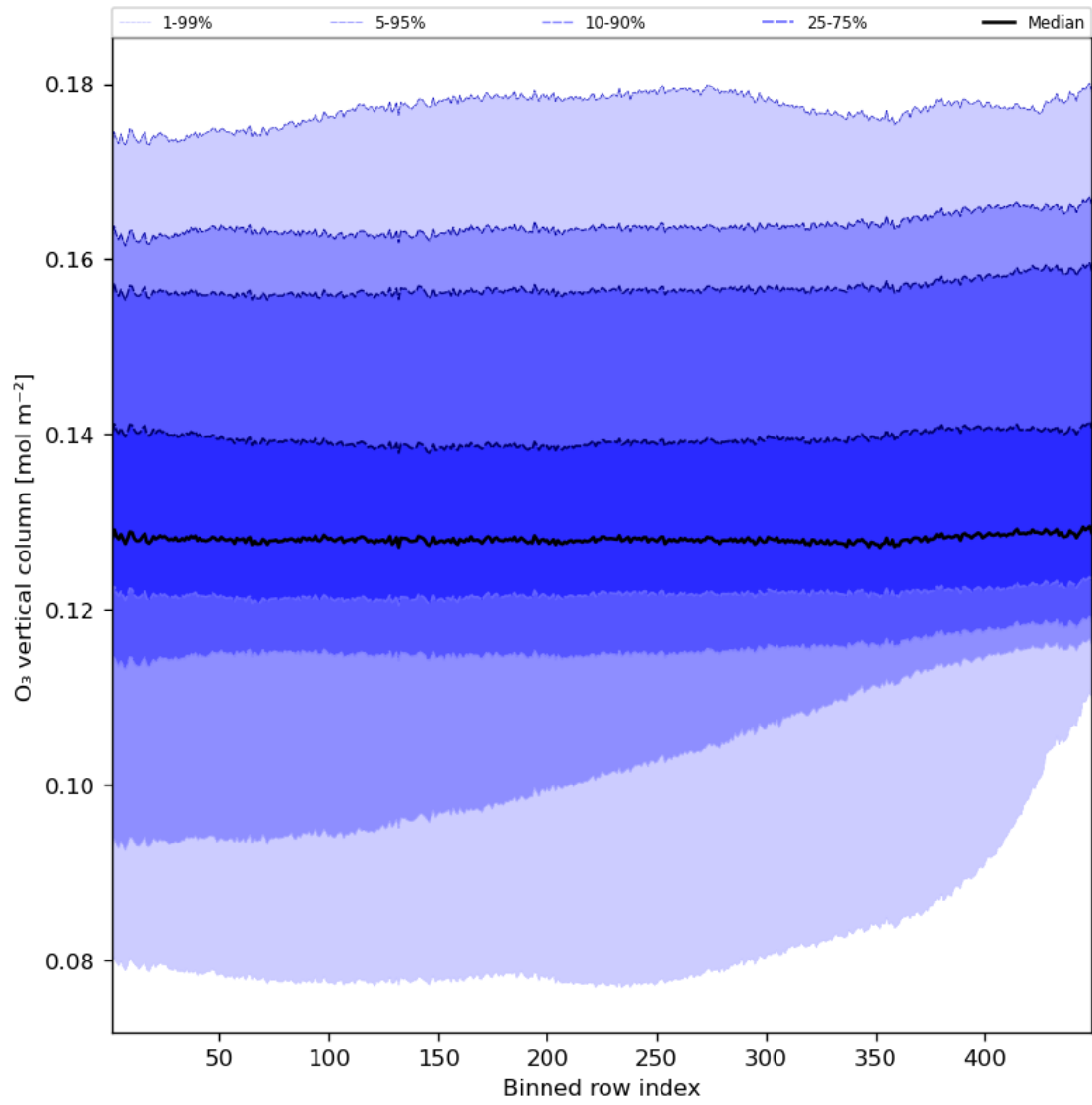
Figure 28: Along track statistics of “O 3 vertical column” for 2023-08-30 to 2023-09-01
