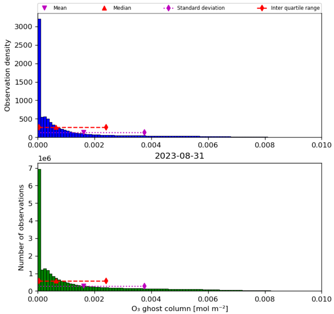
Figure 25: Histogram of “O 3 ghost column” for 2023-08-30 to 2023-09-01
