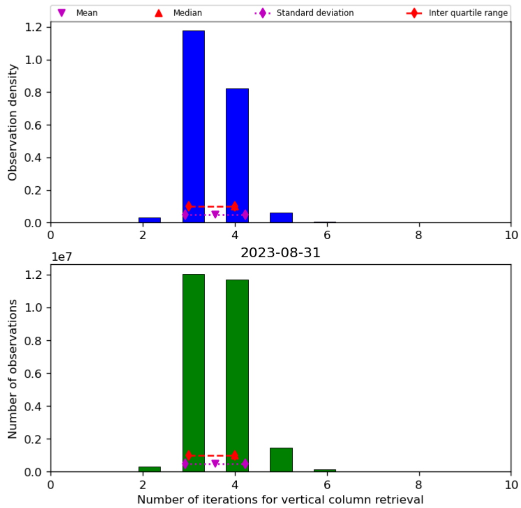
Figure 26: Histogram of “Number of iterations for vertical column retrieval” for 2023-08-30 to 2023-09-01
