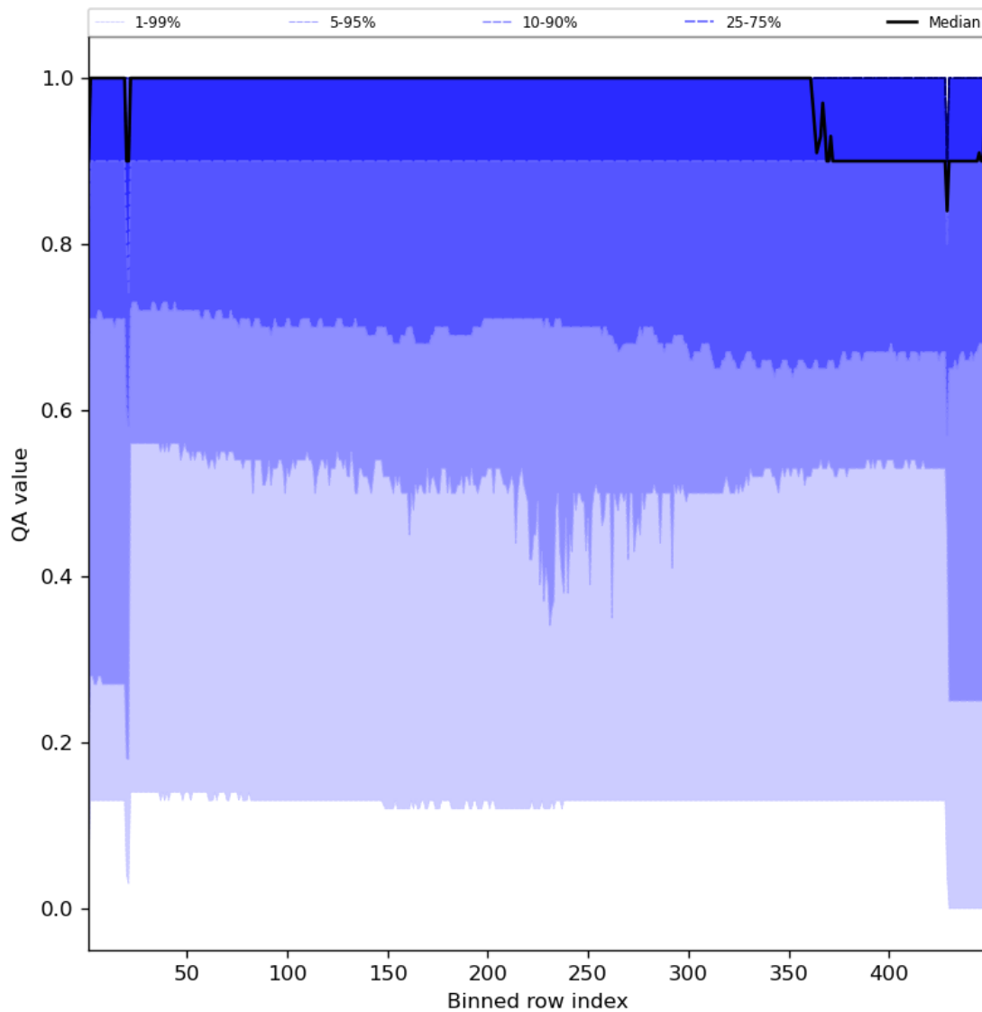
Figure 27: Along track statistics of “QA value” for 2023-08-30 to 2023-09-01
