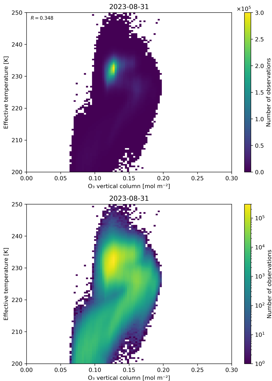
Figure 39: Scatter density plot of “O 3 vertical column” against “Effective temperature” for 2023-08-30 to 2023-09-01.
