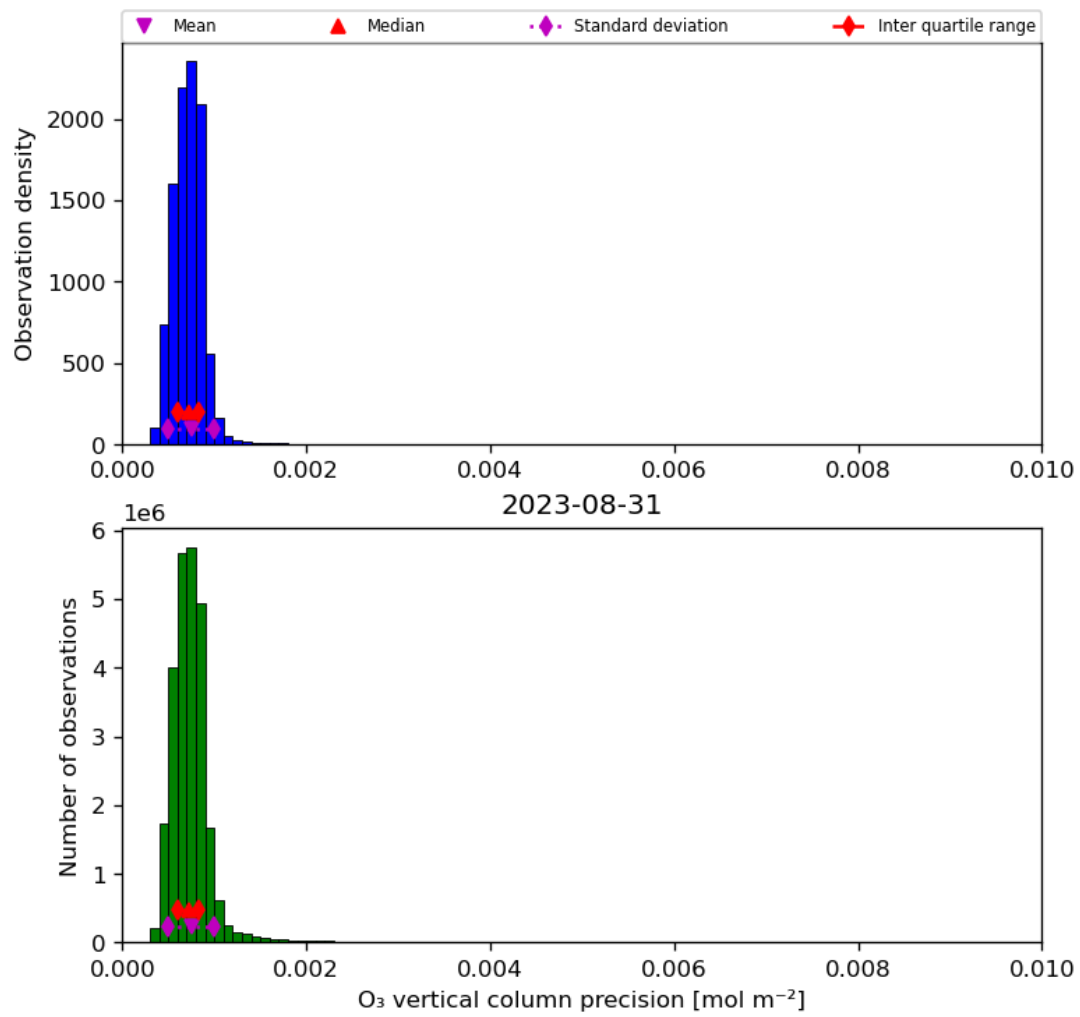
Figure 22: Histogram of “O 3 vertical column precision” for 2023-08-30 to 2023-09-01
