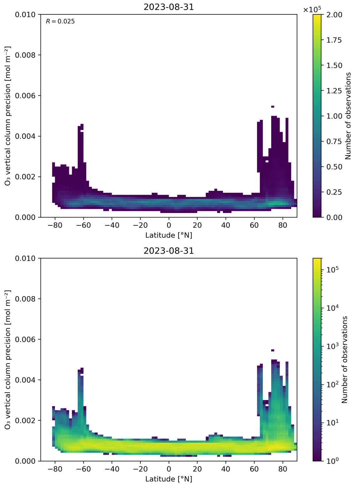
Figure 37: Scatter density plot of “Latitude” against “O 3 vertical column precision” for 2023-08-30 to 2023-09-01.
