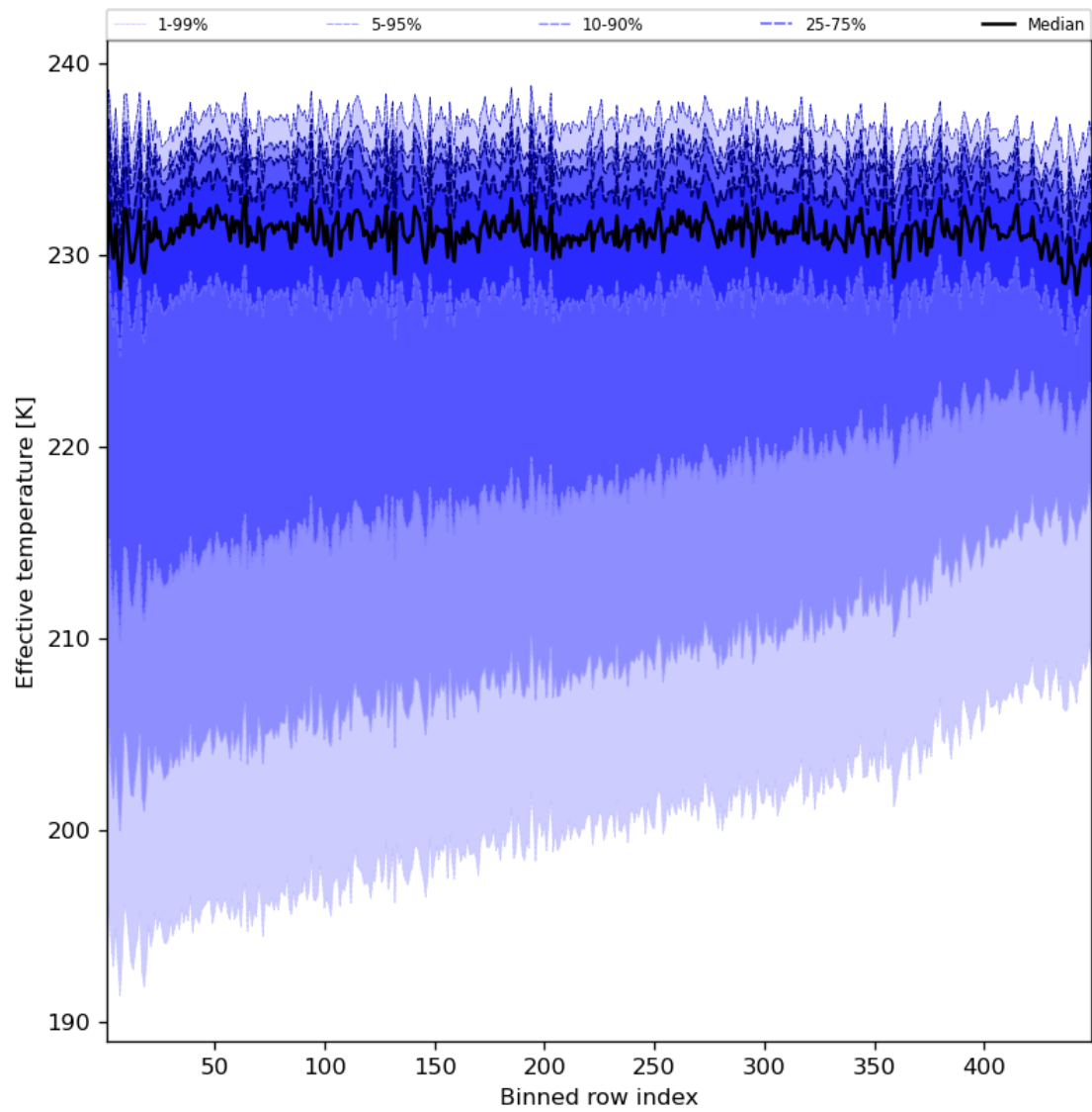
Figure 31: Along track statistics of “Effective temperature” for 2023-08-30 to 2023-09-01
