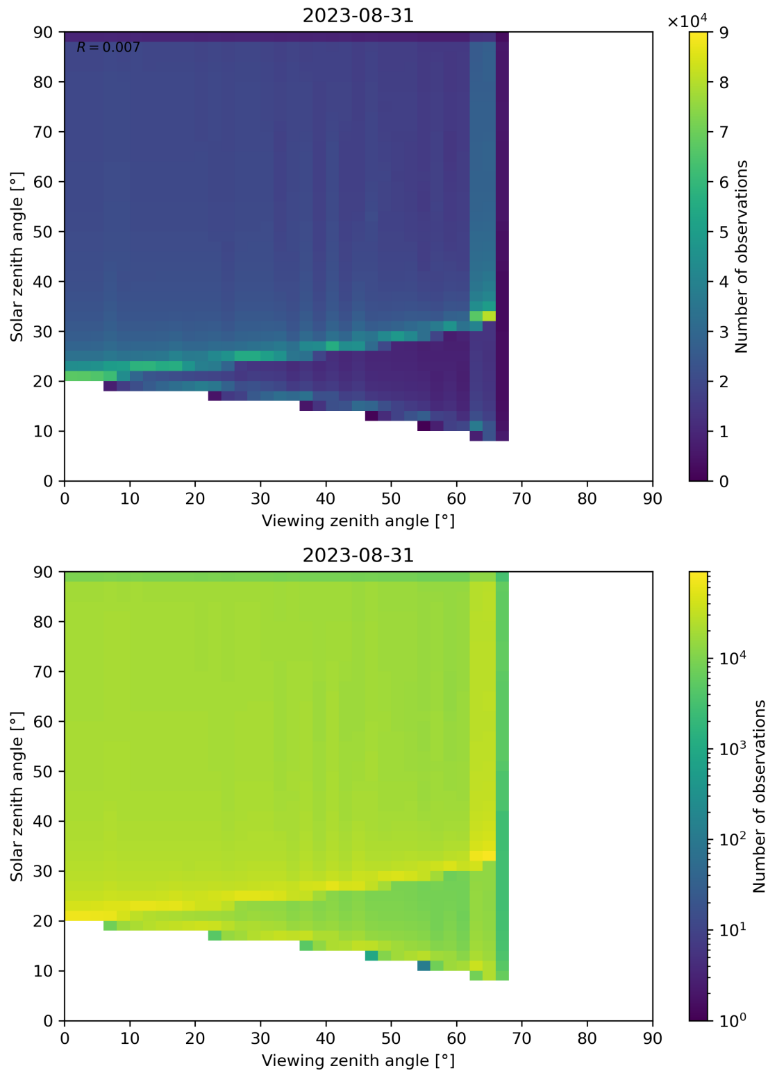
Figure 54: Scatter density plot of “Viewing zenith angle” against “Solar zenith angle” for 2023-08-30 to 2023-09-01.
