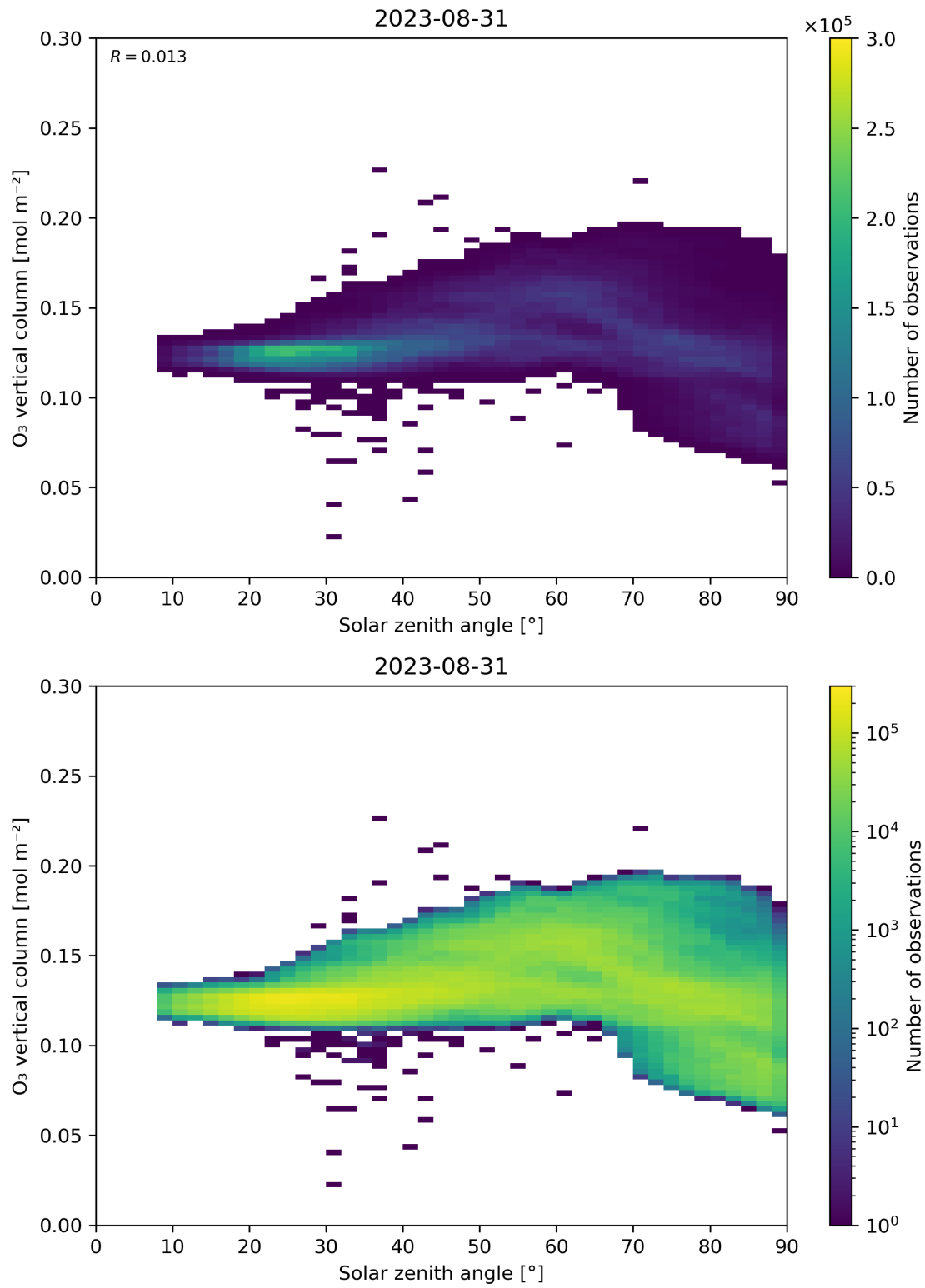
Figure 47: Scatter density plot of “Solar zenith angle” against “O 3 vertical column” for 2023-08-30 to 2023-09-01.
