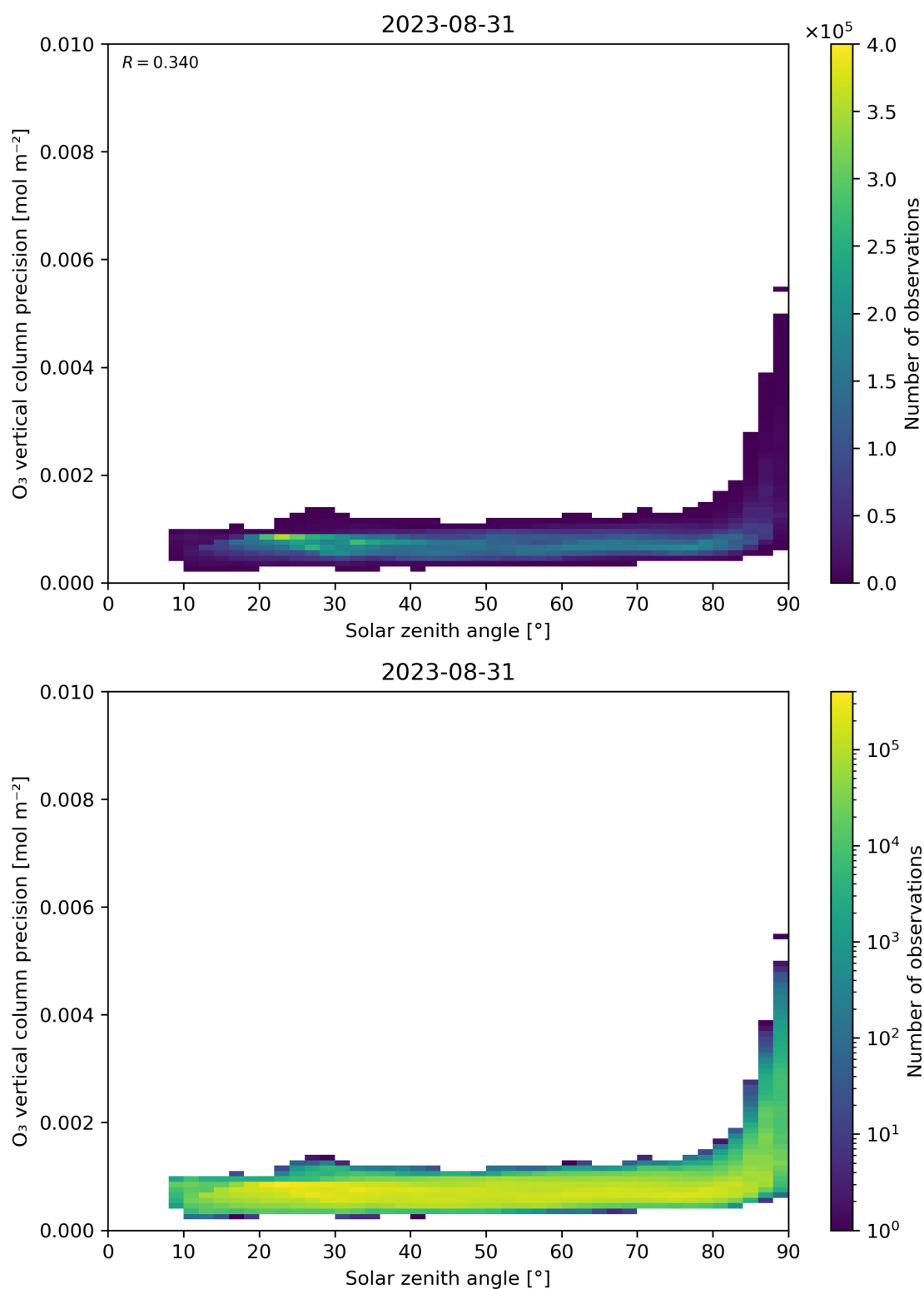
Figure 48: Scatter density plot of “Solar zenith angle” against “O 3 vertical column precision” for 2023-08-30 to 2023-09-01.
