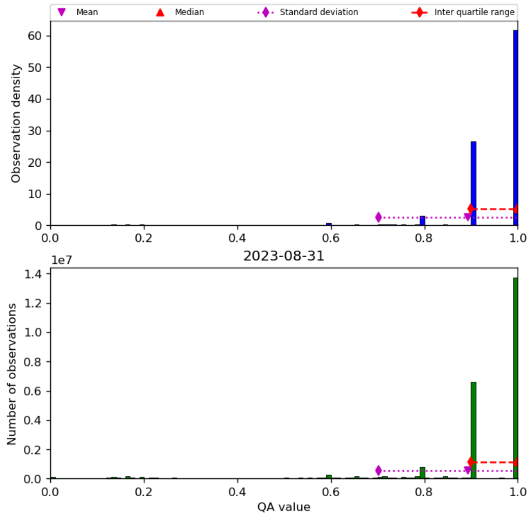
Figure 20: Histogram of “QA value” for 2023-08-30 to 2023-09-01
