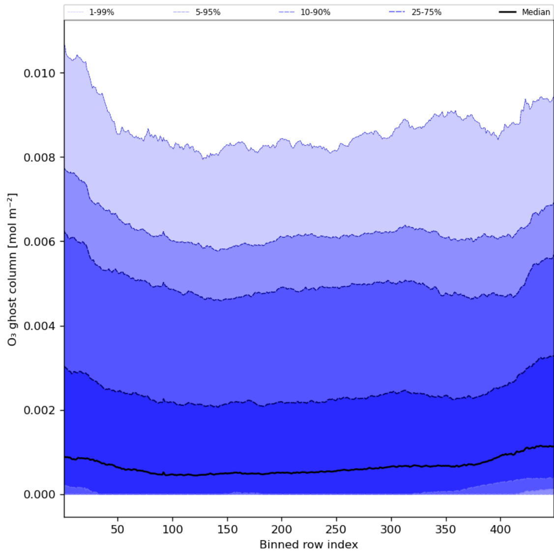
Figure 32: Along track statistics of “O 3 ghost column” for 2023-08-30 to 2023-09-01
