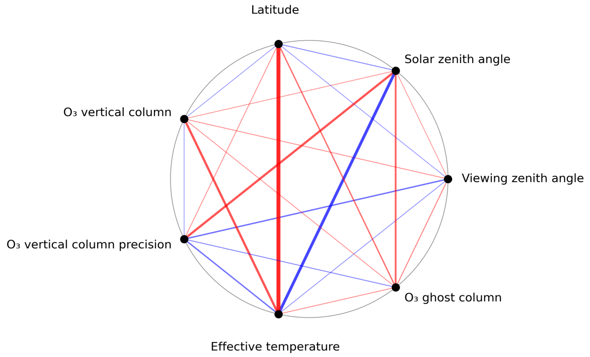
Figure 1: Map of correlation graph for 2023-08-30 to 2023-09-01.
