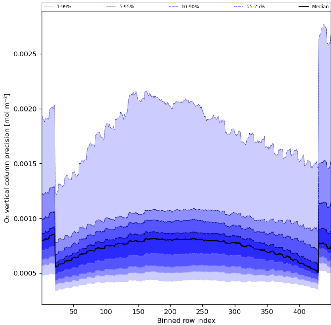
Figure 29: Along track statistics of “O 3 vertical column precision” for 2023-08-30 to 2023-09-01
