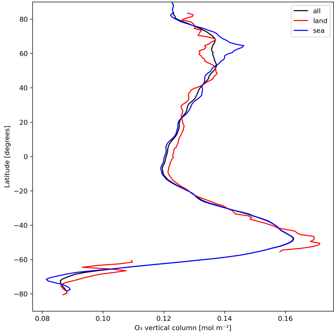
Figure 14: Zonal average of “O 3 vertical column” for 2023-08-30 to 2023-09-01.
