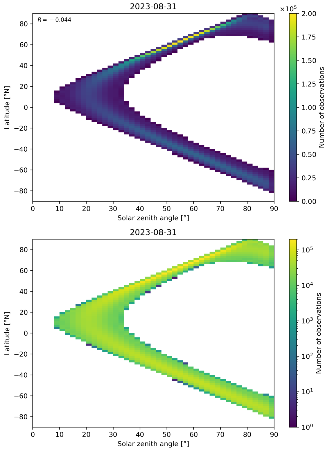
Figure 44: Scatter density plot of “Solar zenith angle” against “Latitude” for 2023-08-30 to 2023-09-01.
