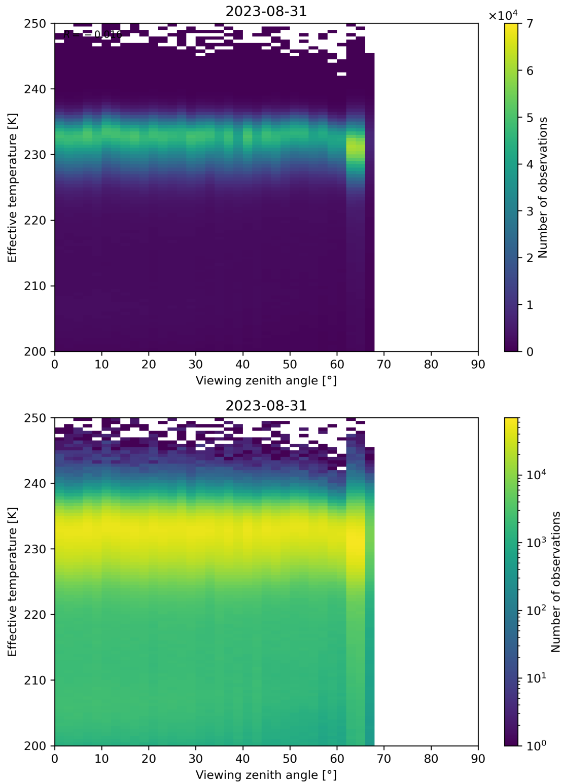
Figure 50: Scatter density plot of “Viewing zenith angle” against “Effective temperature” for 2023-08-30 to 2023-09-01.
