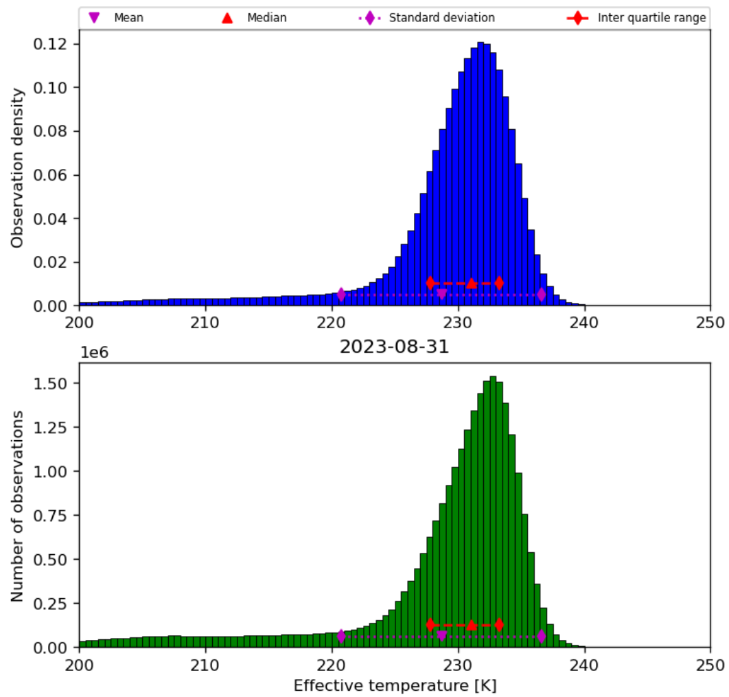
Figure 24: Histogram of “Effective temperature” for 2023-08-30 to 2023-09-01
