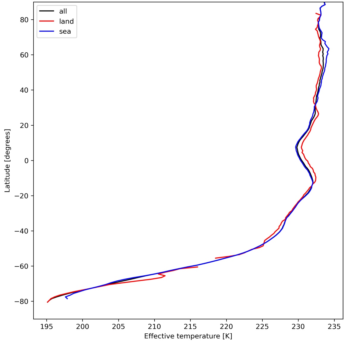
Figure 17: Zonal average of "Effective temperature" for 2023-08-30 to 2023-09-01.
