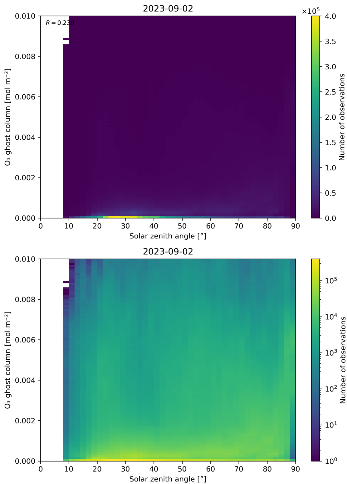
Figure 46: Scatter density plot of “Solar zenith angle” against “O 3 ghost column” for 2023-09-01 to 2023-09-03.
