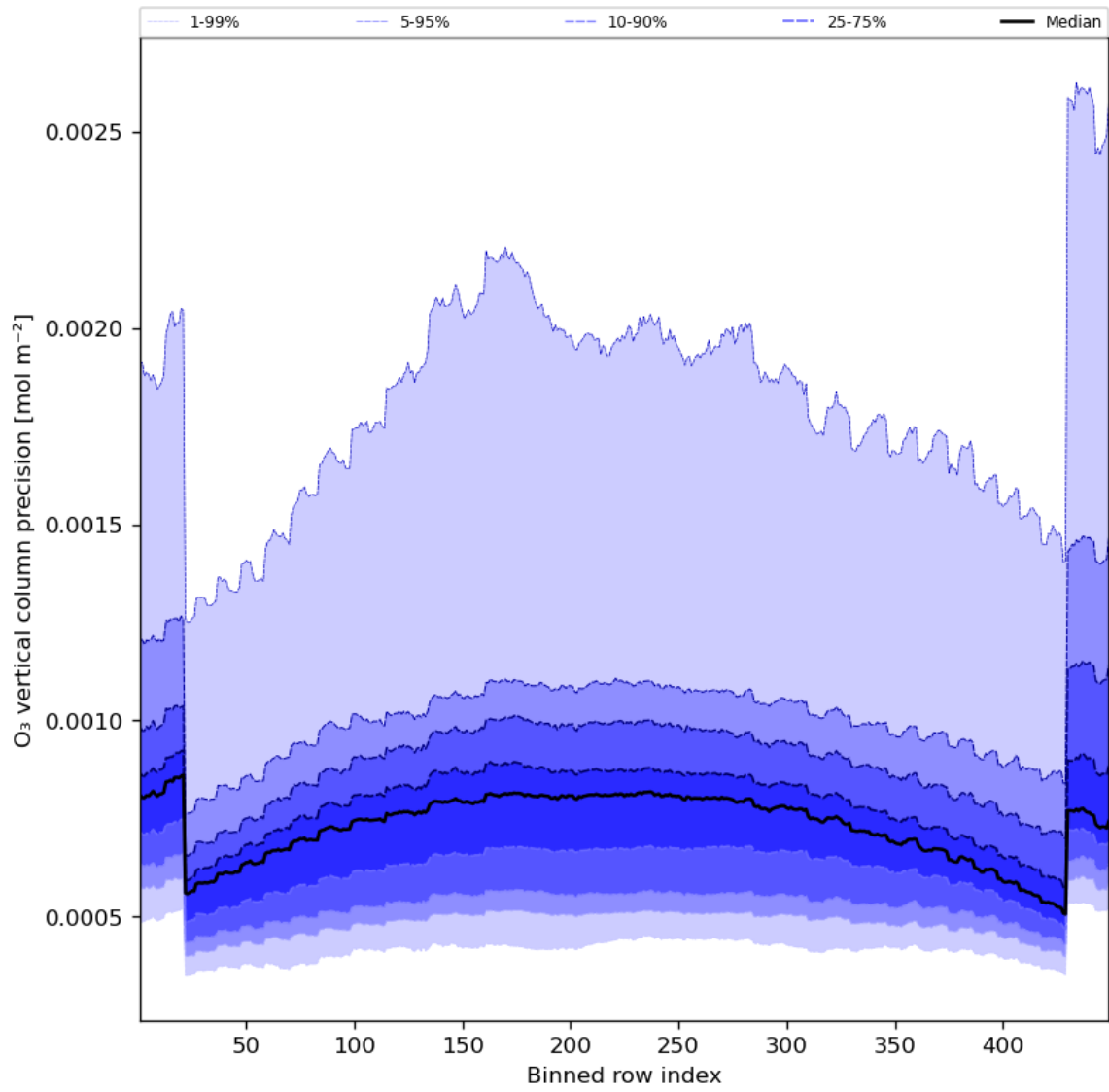
Figure 29: Along track statistics of “O 3 vertical column precision” for 2023-09-01 to 2023-09-03
