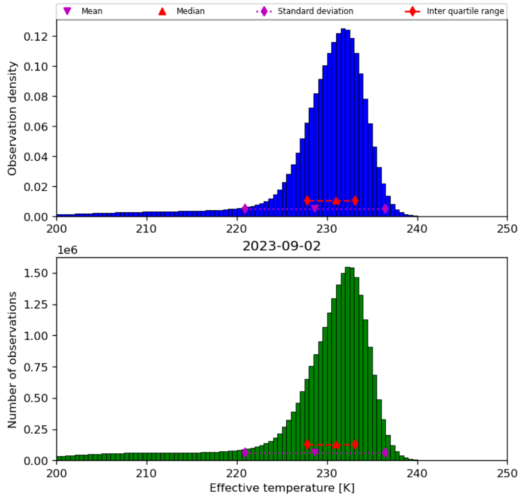
Figure 24: Histogram of “Effective temperature” for 2023-09-01 to 2023-09-03
