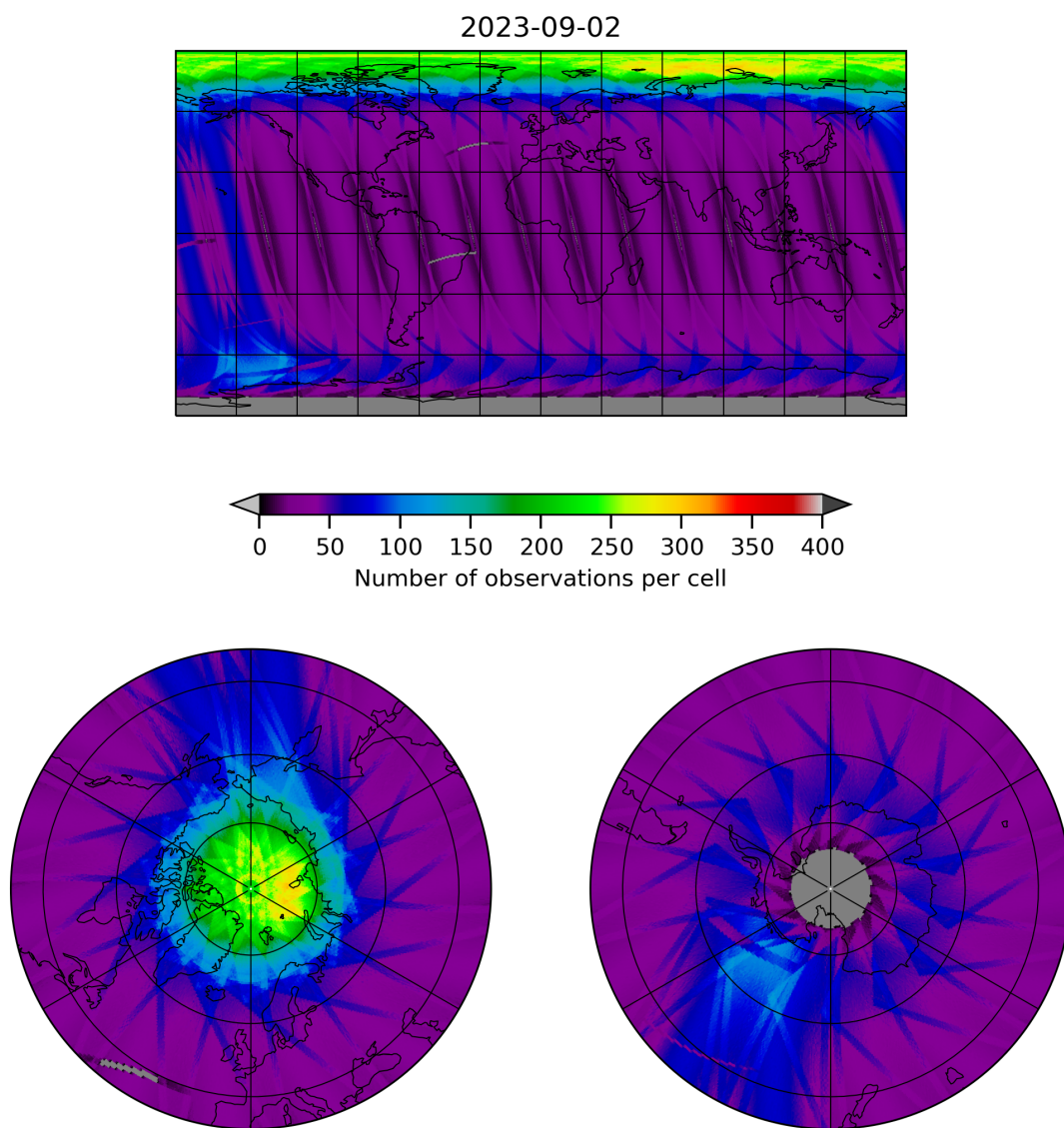
Figure 12: Map of the number of observations for 2023-09-01 to 2023-09-03
