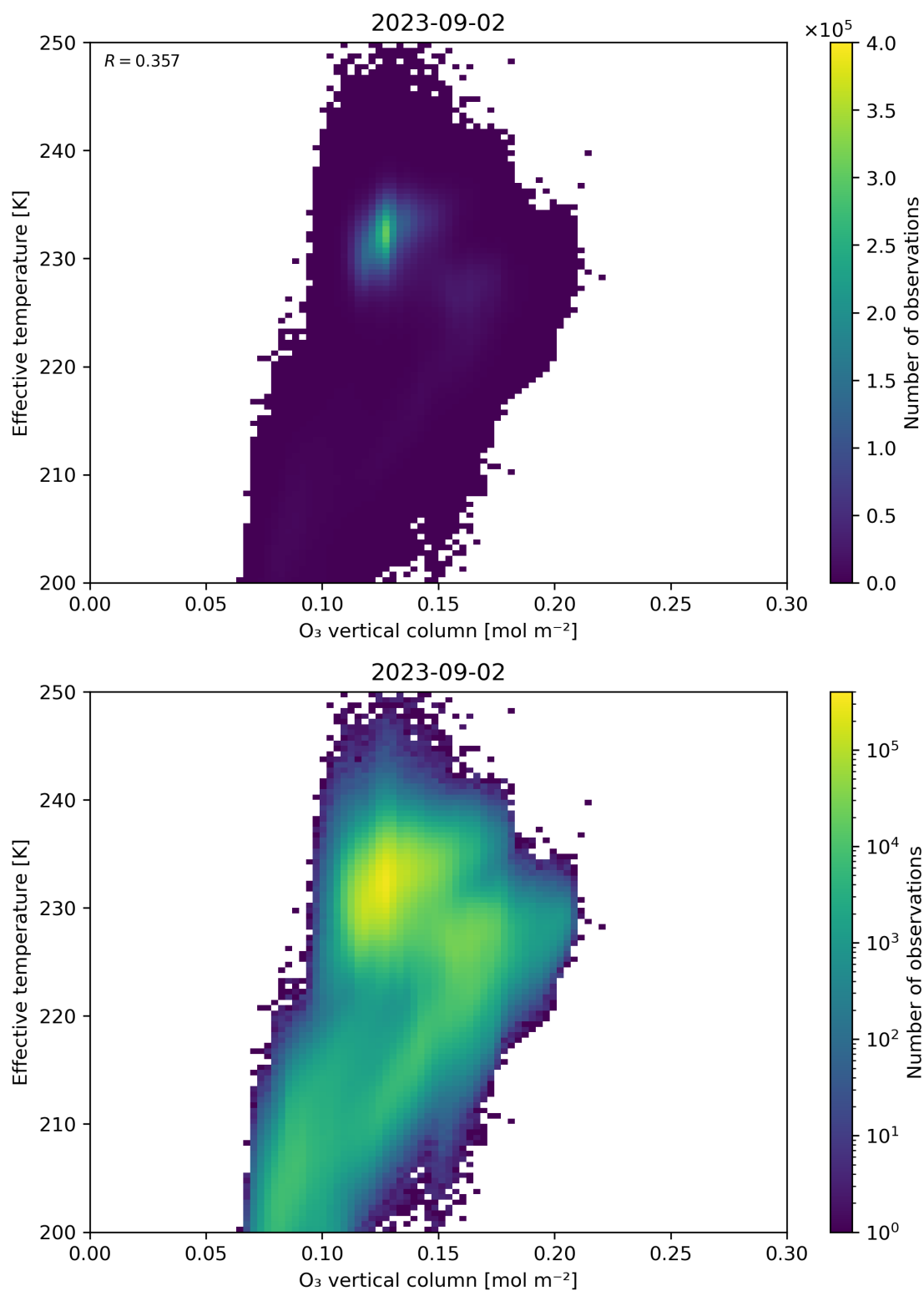
Figure 39: Scatter density plot of “O 3 vertical column” against “Effective temperature” for 2023-09-01 to 2023-09-03.
