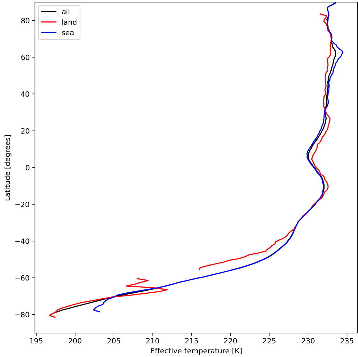
Figure 17: Zonal average of "Effective temperature" for 2023-09-01 to 2023-09-03.
