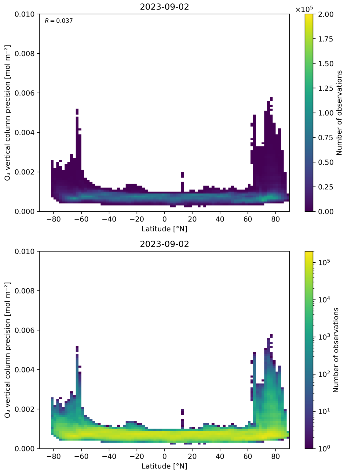
Figure 37: Scatter density plot of “Latitude” against “O 3 vertical column precision” for 2023-09-01 to 2023-09-03.
