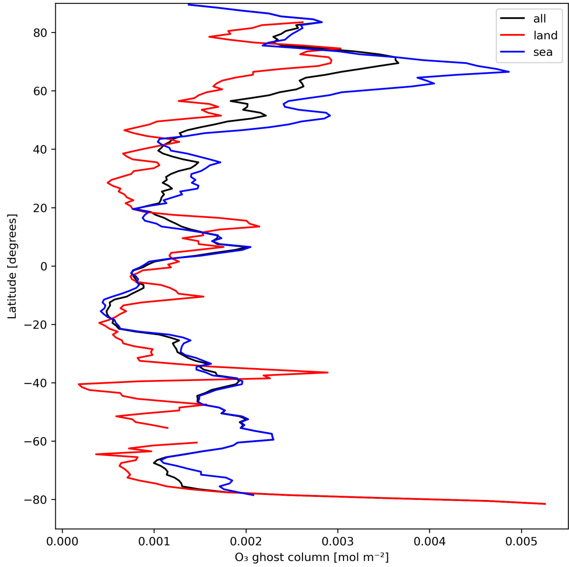
Figure 18: Zonal average of “O 3 ghost column” for 2023-09-01 to 2023-09-03.
