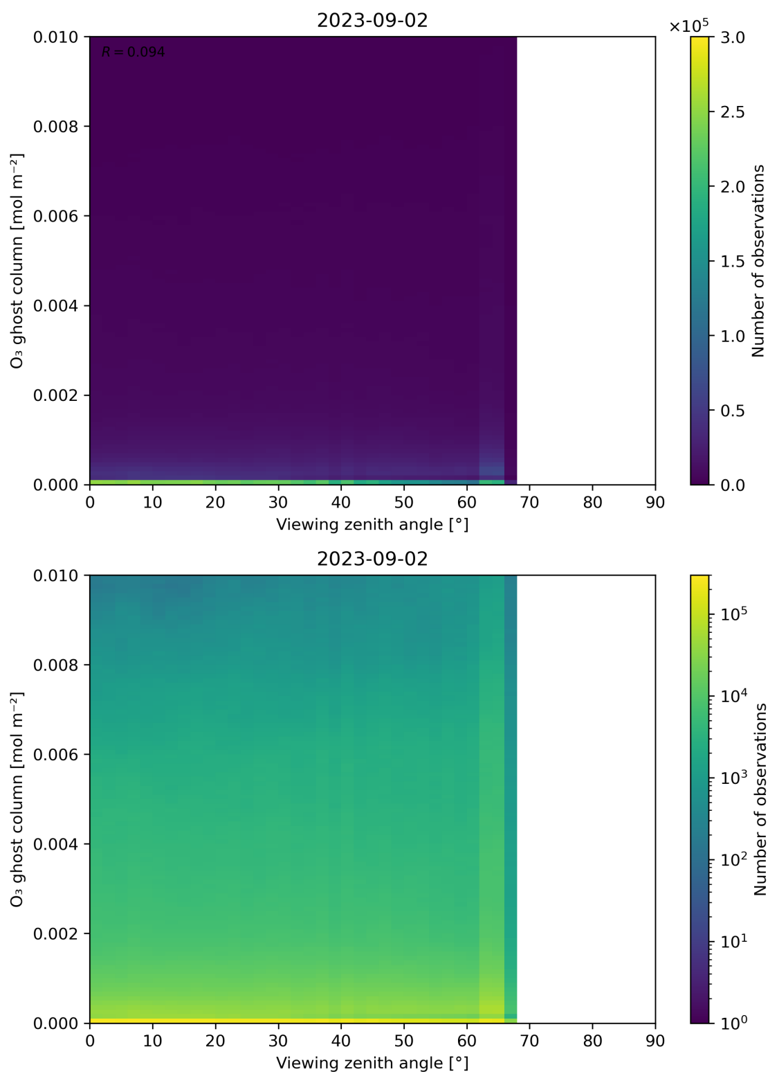
Figure 51: Scatter density plot of “Viewing zenith angle” against “O 3 ghost column” for 2023-09-01 to 2023-09-03.
