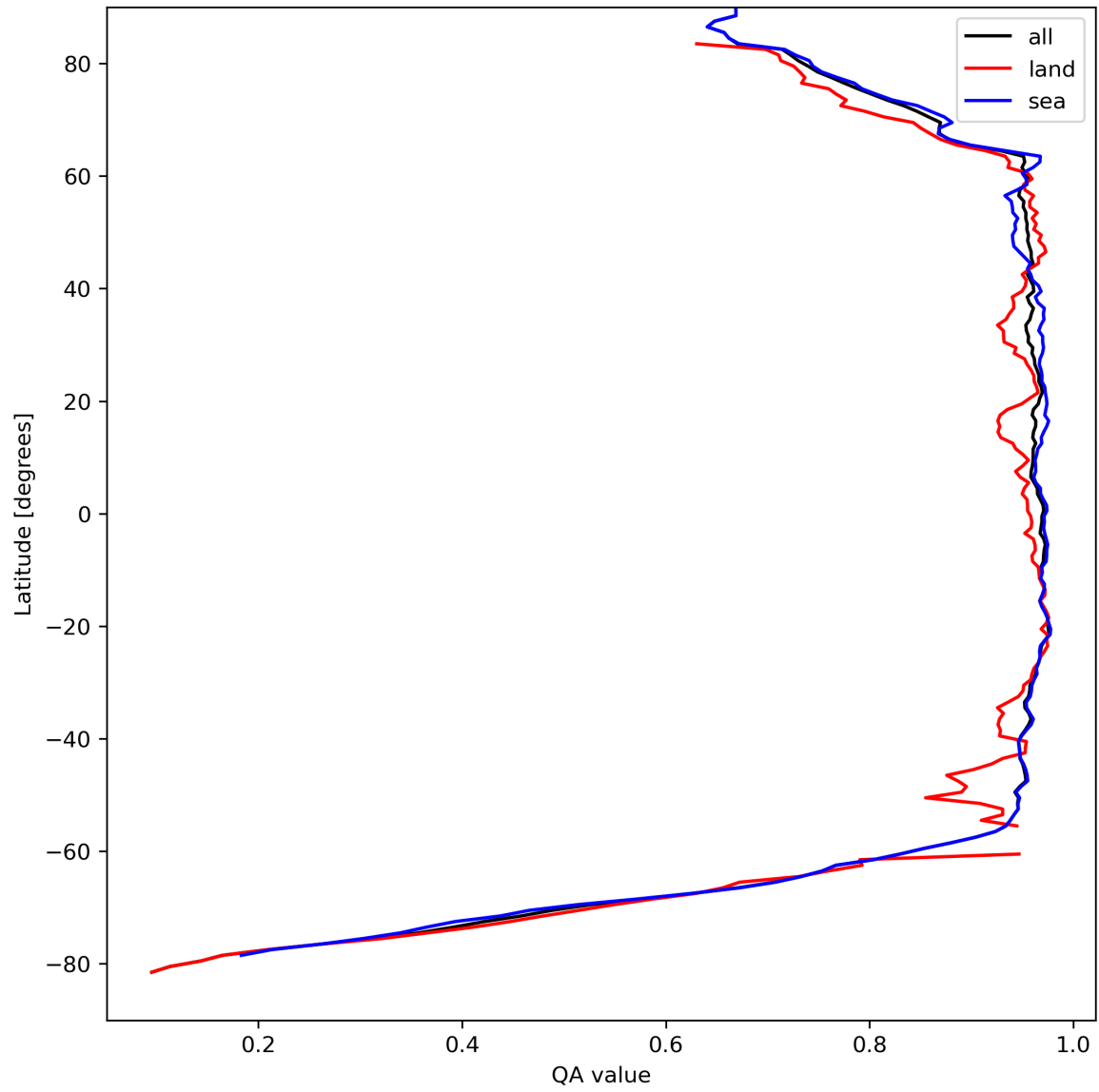
Figure 13: Zonal average of “QA value” for 2023-09-01 to 2023-09-03.
