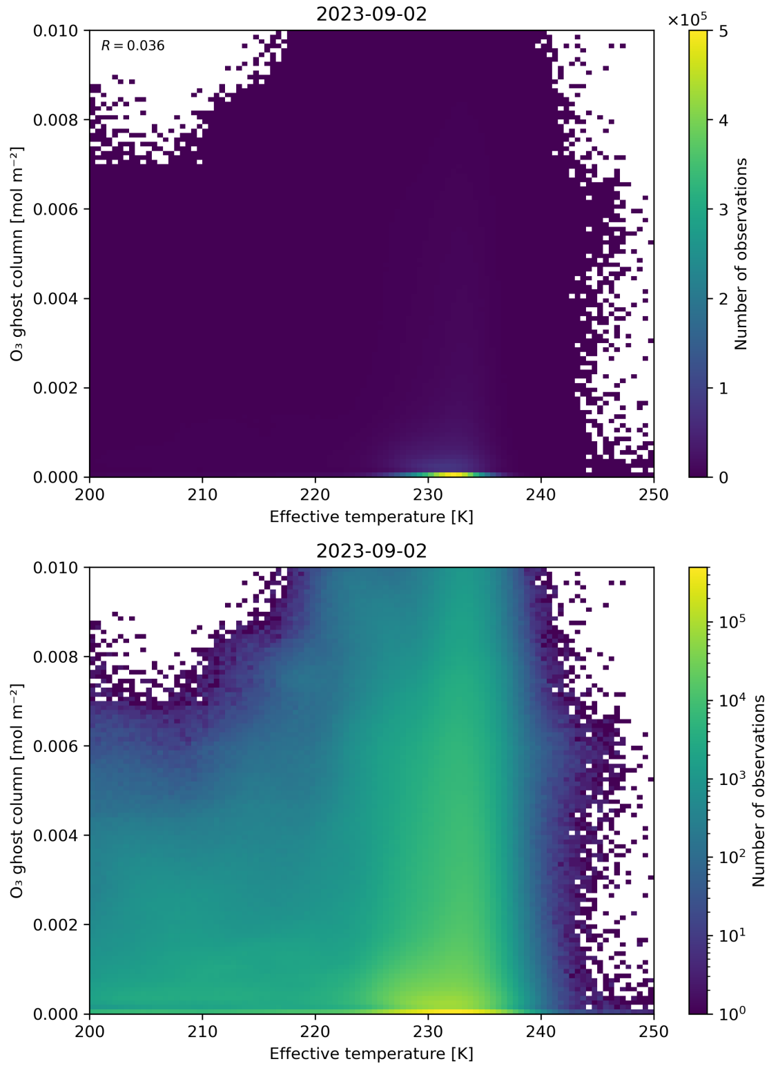
Figure 38: Scatter density plot of “Effective temperature” against “O 3 ghost column” for 2023-09-01 to 2023-09-03.
