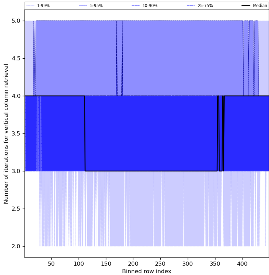
Figure 33: Along track statistics of “Number of iterations for vertical column retrieval” for 2023-09-01 to 2023-09-03
