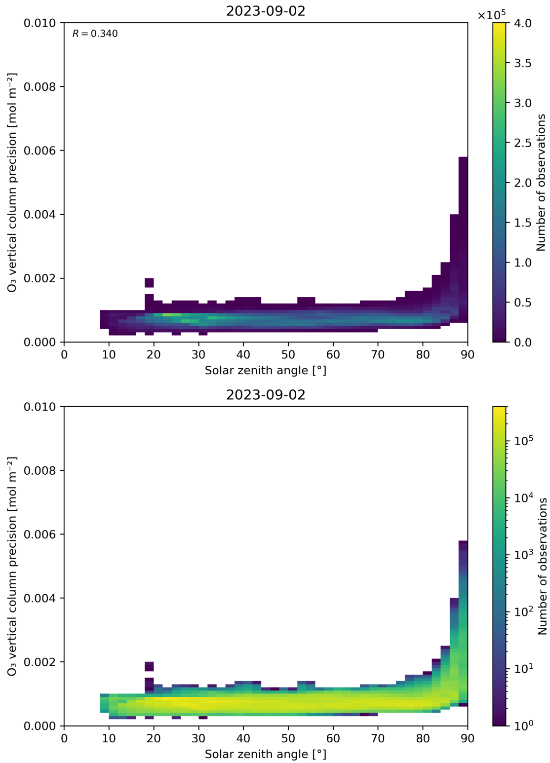
Figure 48: Scatter density plot of “Solar zenith angle” against “O 3 vertical column precision” for 2023-09-01 to 2023-09-03.
