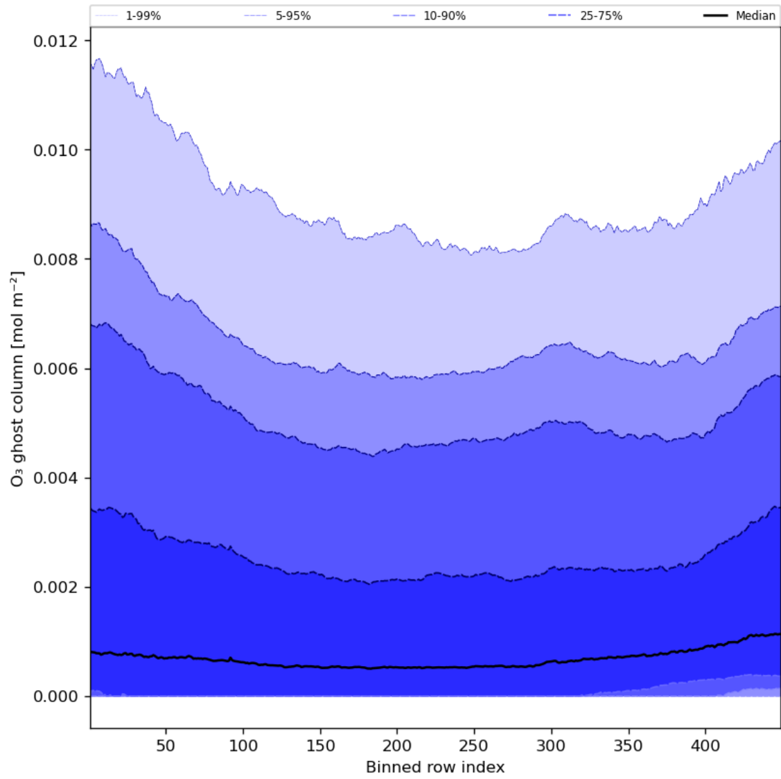
Figure 32: Along track statistics of "O 3 ghost column" for 2023-09-01 to 2023-09-03
