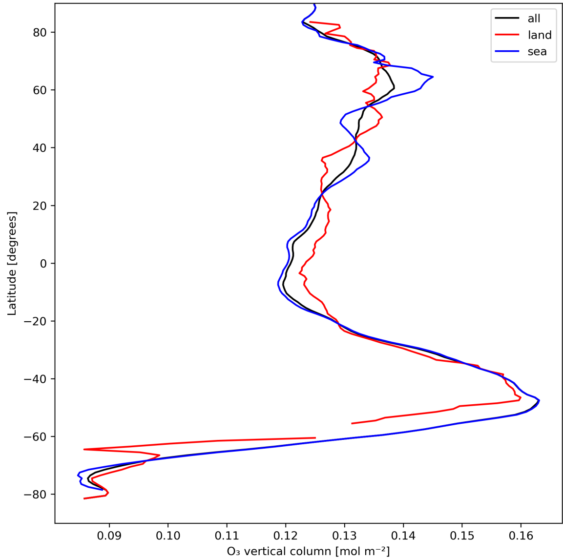
Figure 14: Zonal average of “O 3 vertical column” for 2023-09-01 to 2023-09-03.
