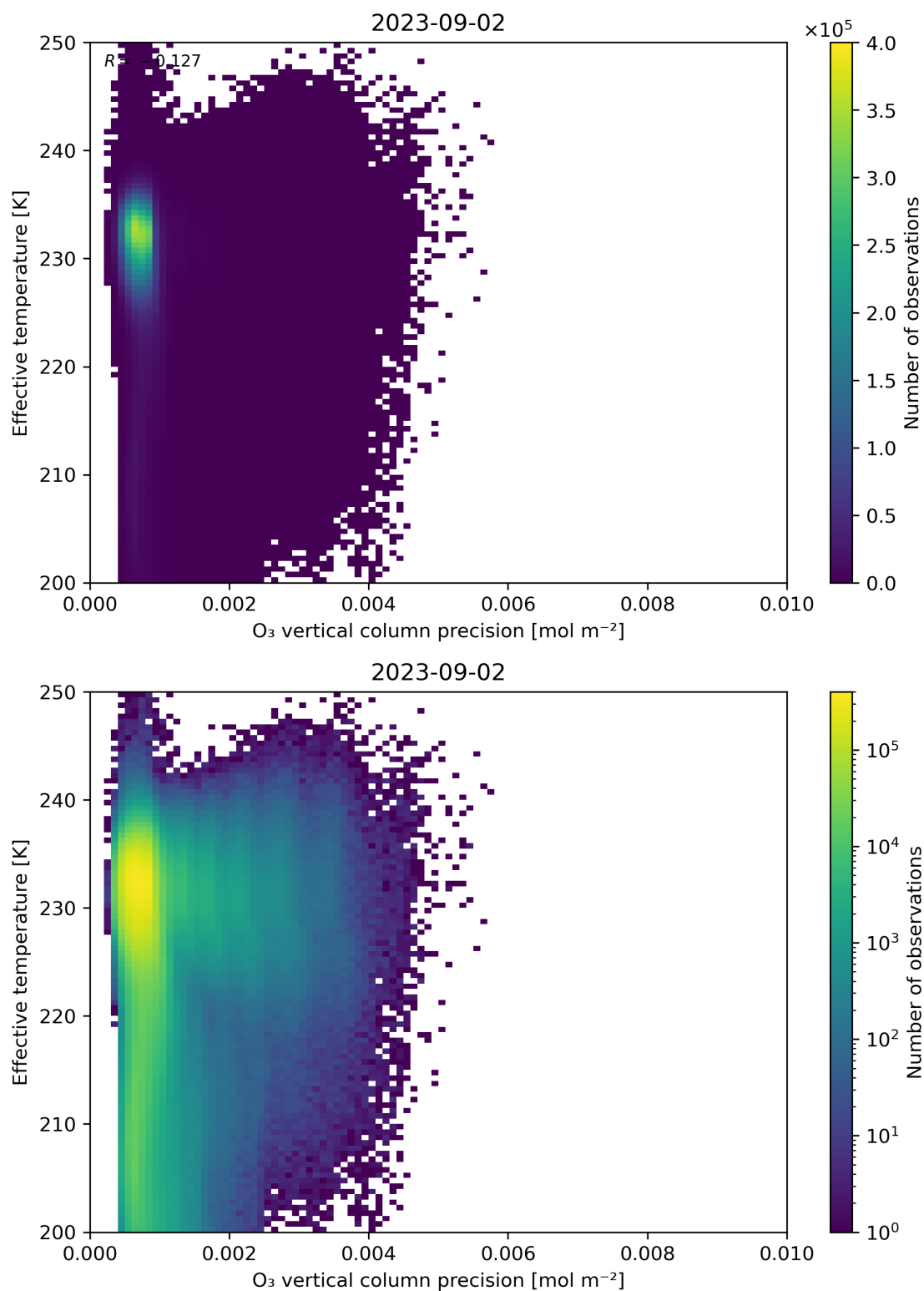
Figure 42: Scatter density plot of “O 3 vertical column precision” against “Effective temperature” for 2023-09-01 to 2023-09-03.
