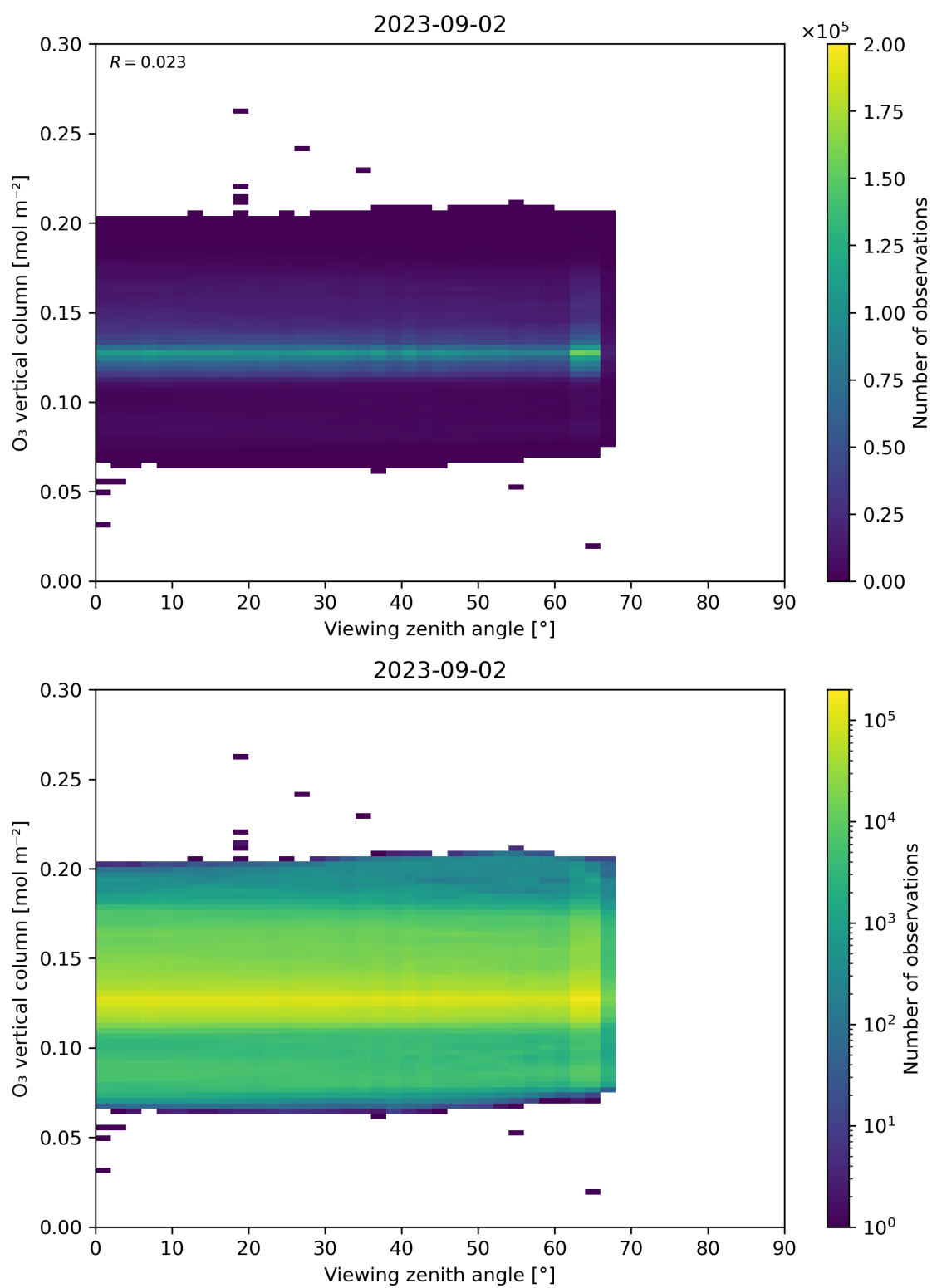
Figure 52: Scatter density plot of “Viewing zenith angle” against “O 3 vertical column” for 2023-09-01 to 2023-09-03.
