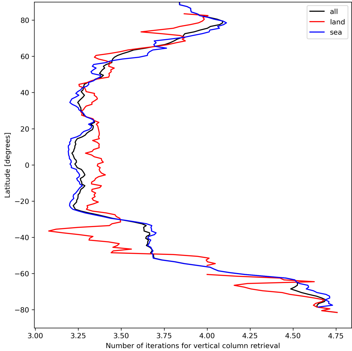
Figure 19: Zonal average of “Number of iterations for vertical column retrieval” for 2023-09-01 to 2023-09-03.
