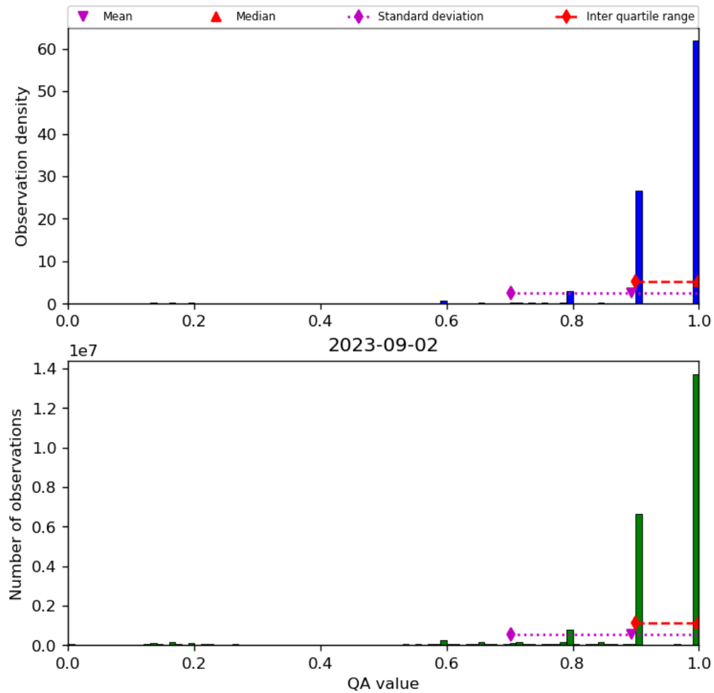
Figure 20: Histogram of “QA value” for 2023-09-01 to 2023-09-03
