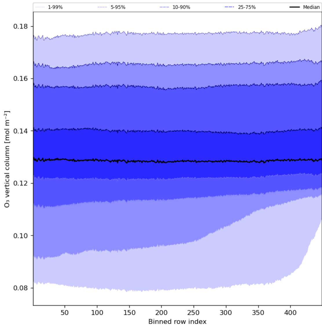
Figure 28: Along track statistics of “O 3 vertical column” for 2023-09-01 to 2023-09-03
