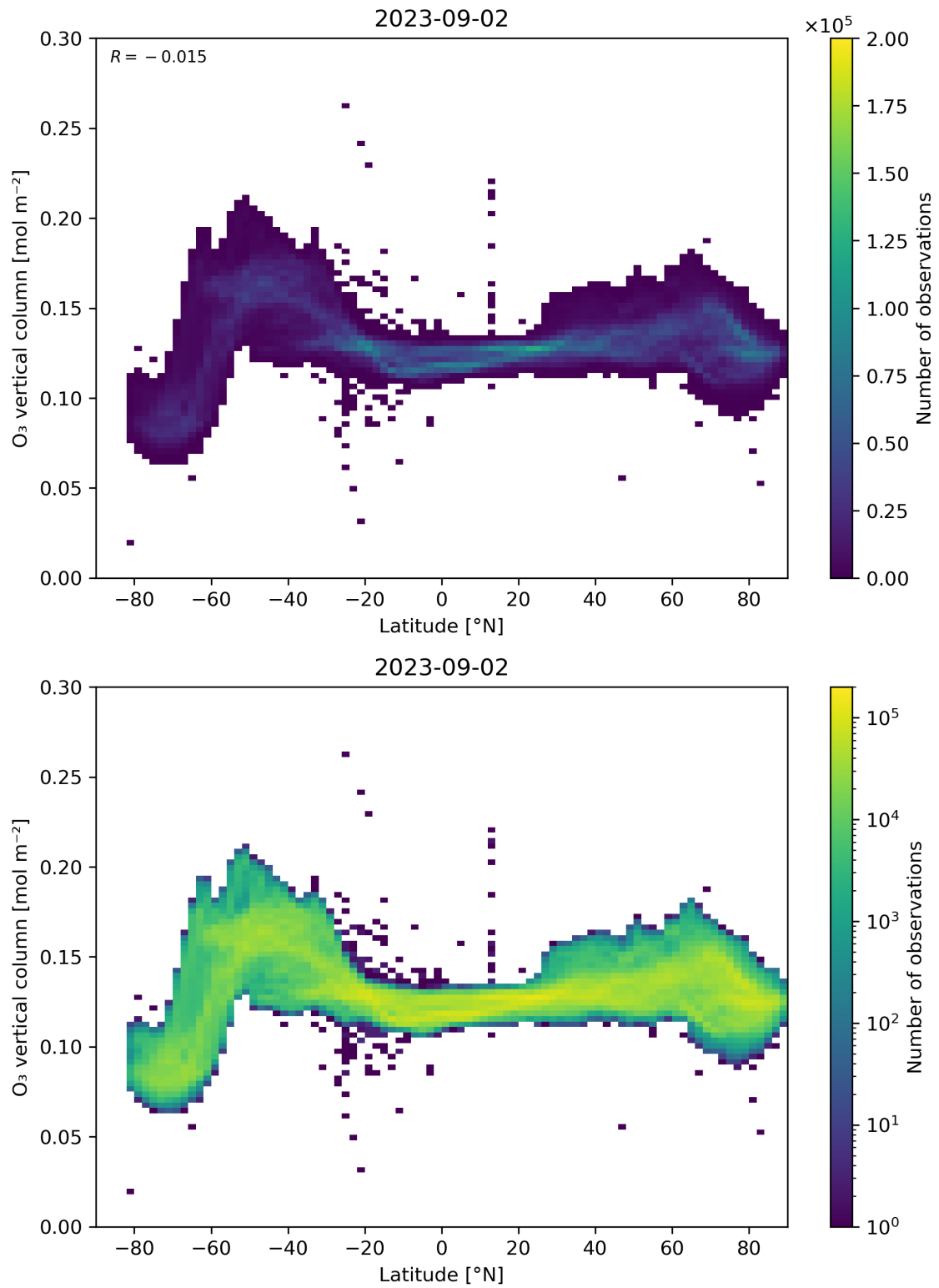
Figure 36: Scatter density plot of “Latitude” against “O 3 vertical column” for 2023-09-01 to 2023-09-03.
