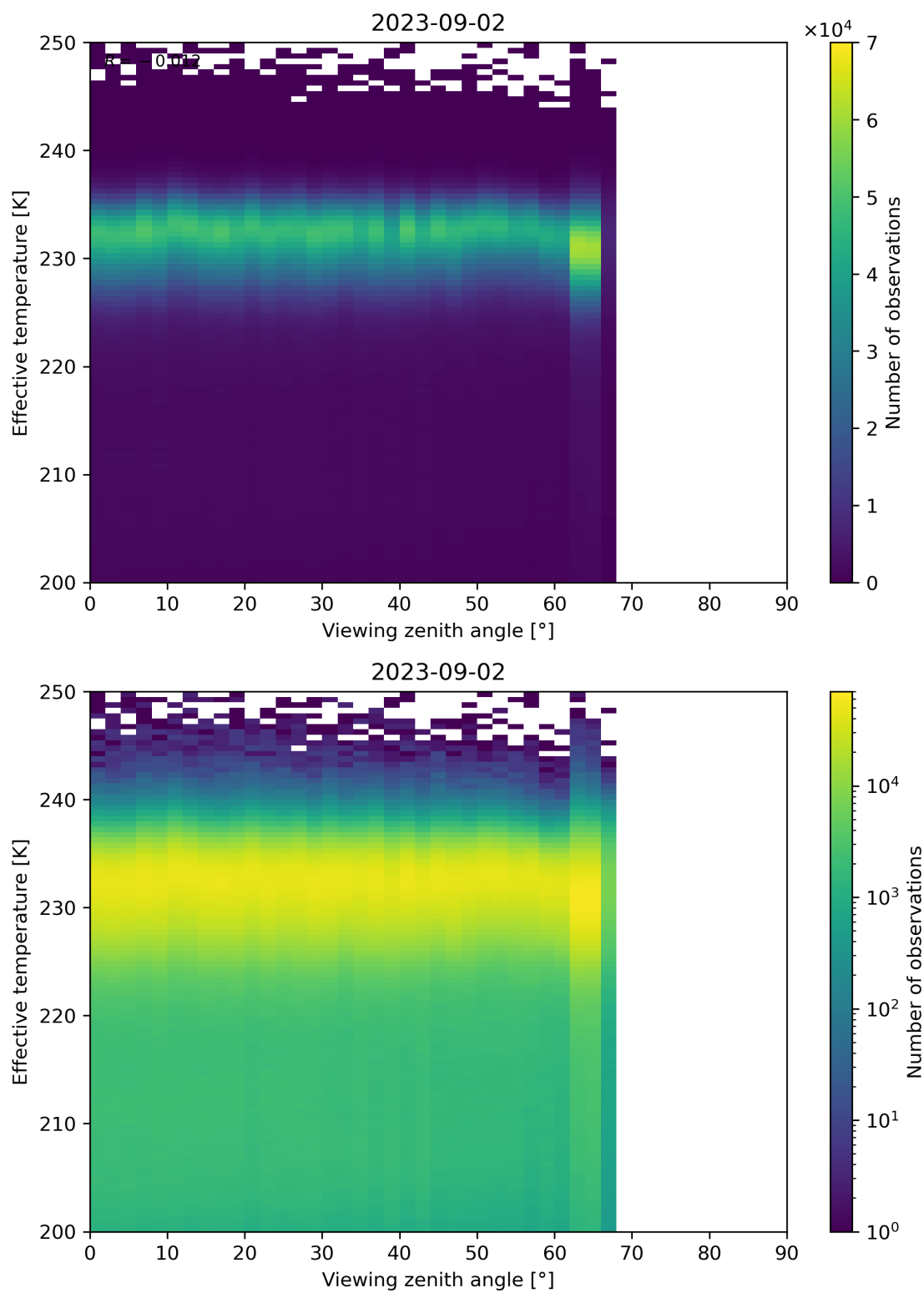
Figure 50: Scatter density plot of “Viewing zenith angle” against “Effective temperature” for 2023-09-01 to 2023-09-03.
