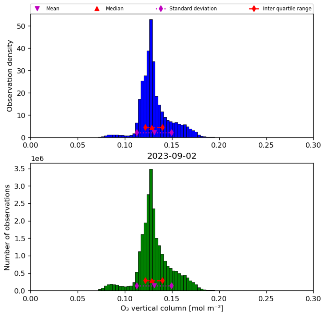
Figure 21: Histogram of “O 3 vertical column” for 2023-09-01 to 2023-09-03
