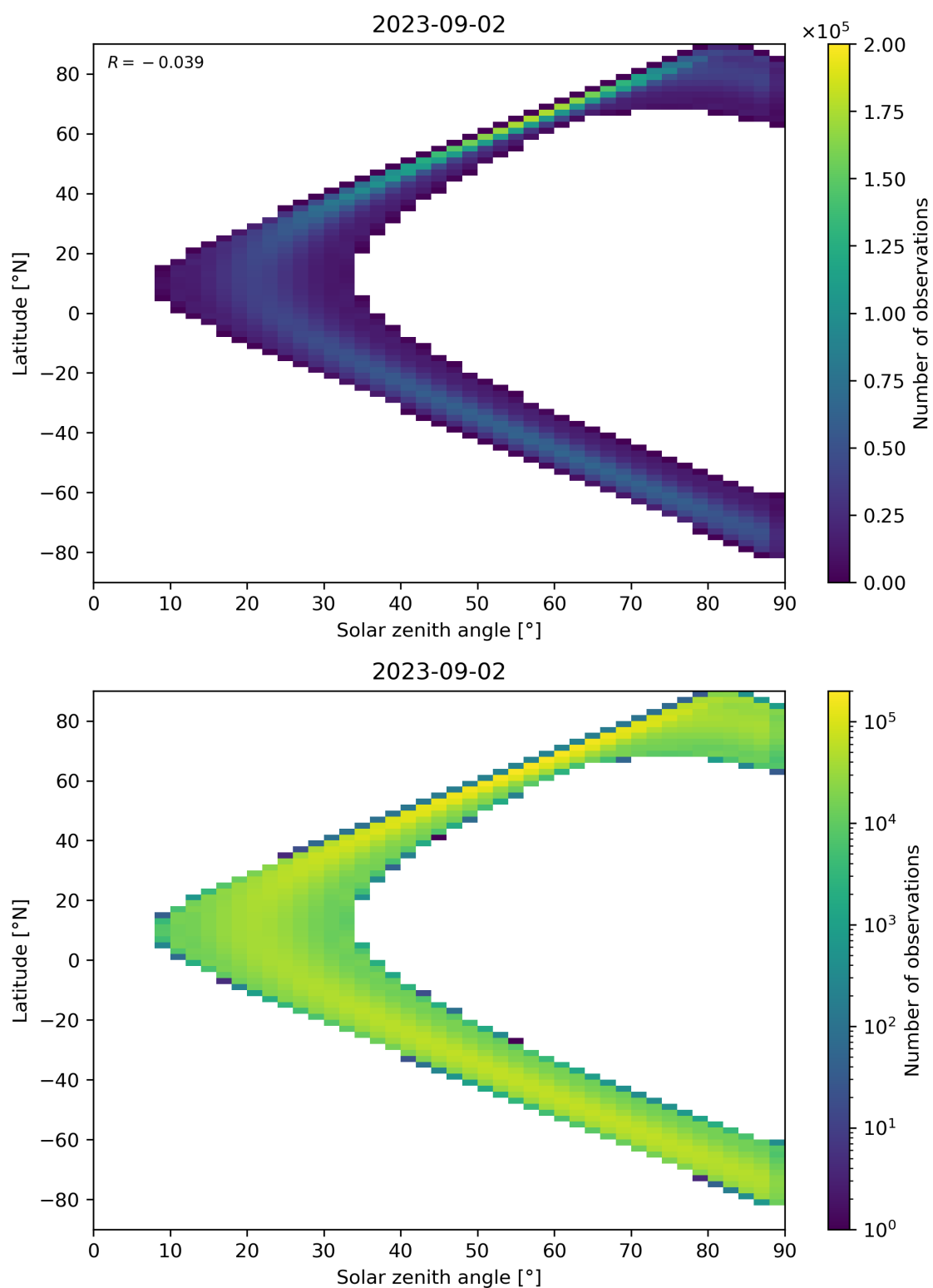
Figure 44: Scatter density plot of “Solar zenith angle” against “Latitude” for 2023-09-01 to 2023-09-03.
