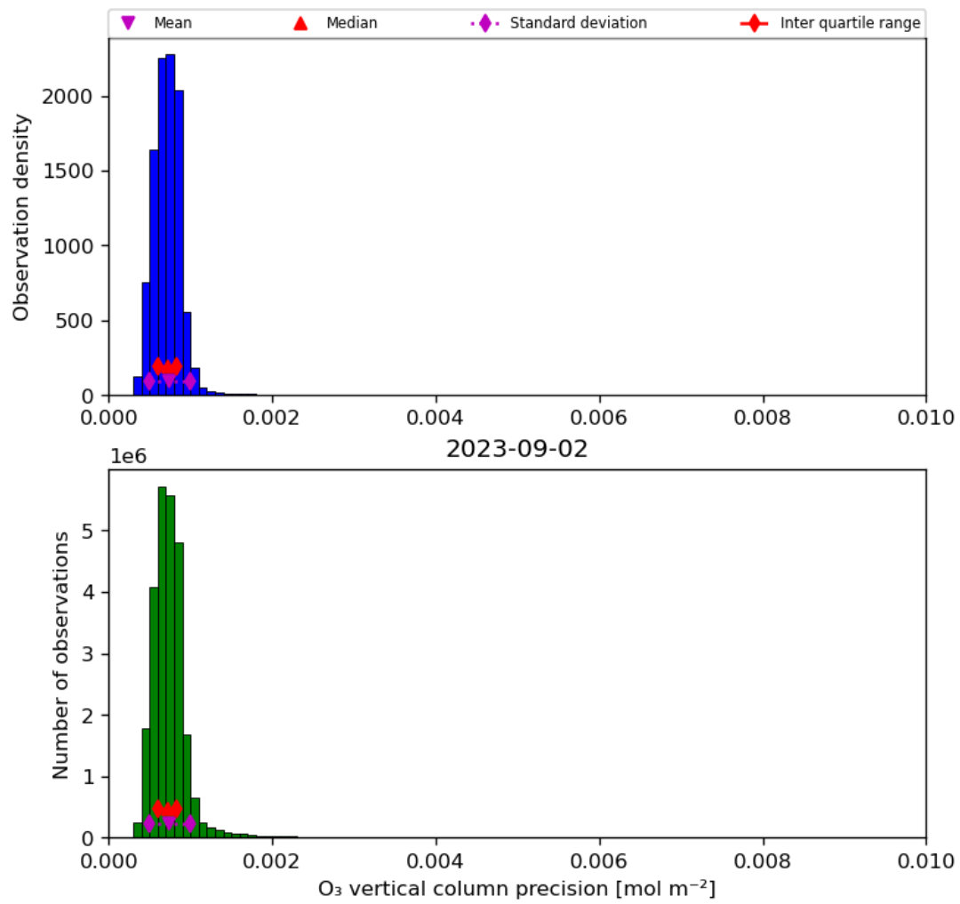
Figure 22: Histogram of “O 3 vertical column precision” for 2023-09-01 to 2023-09-03
