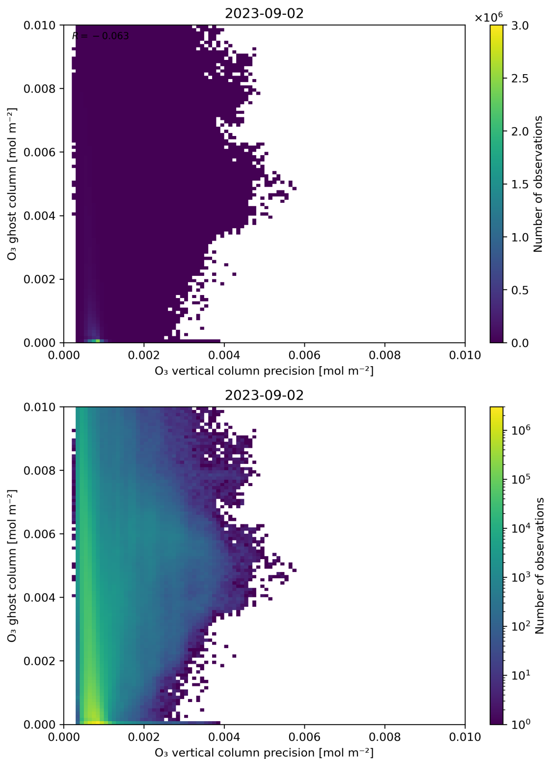
Figure 43: Scatter density plot of “O 3 vertical column precision” against “O 3 ghost column” for 2023-09-01 to 2023-09-03.
