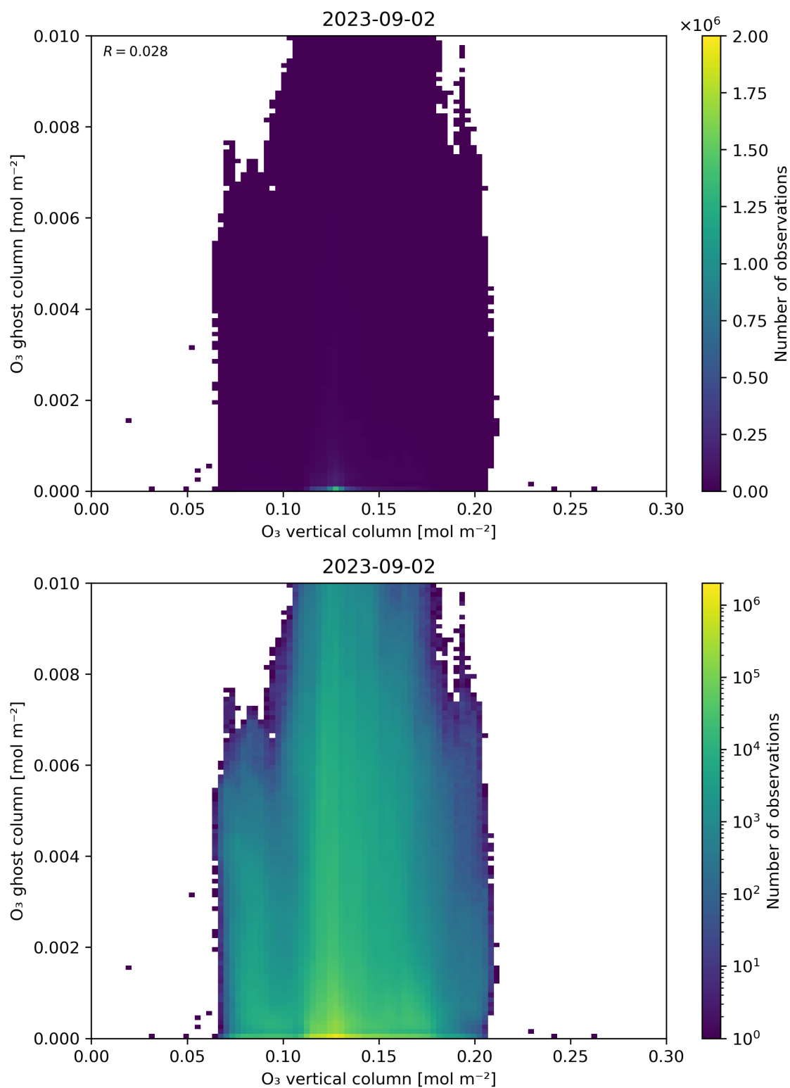
Figure 40: Scatter density plot of “O 3 vertical column” against “O 3 ghost column” for 2023-09-01 to 2023-09-03.
