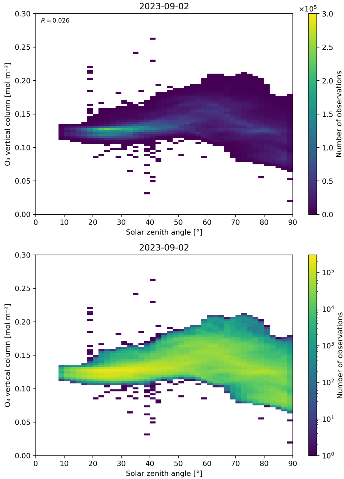
Figure 47: Scatter density plot of “Solar zenith angle” against “O 3 vertical column” for 2023-09-01 to 2023-09-03.
