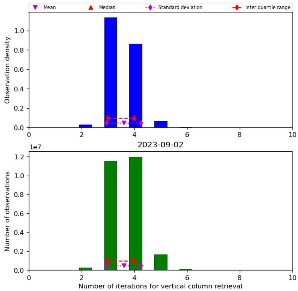
Figure 26: Histogram of “Number of iterations for vertical column retrieval” for 2023-09-01 to 2023-09-03
