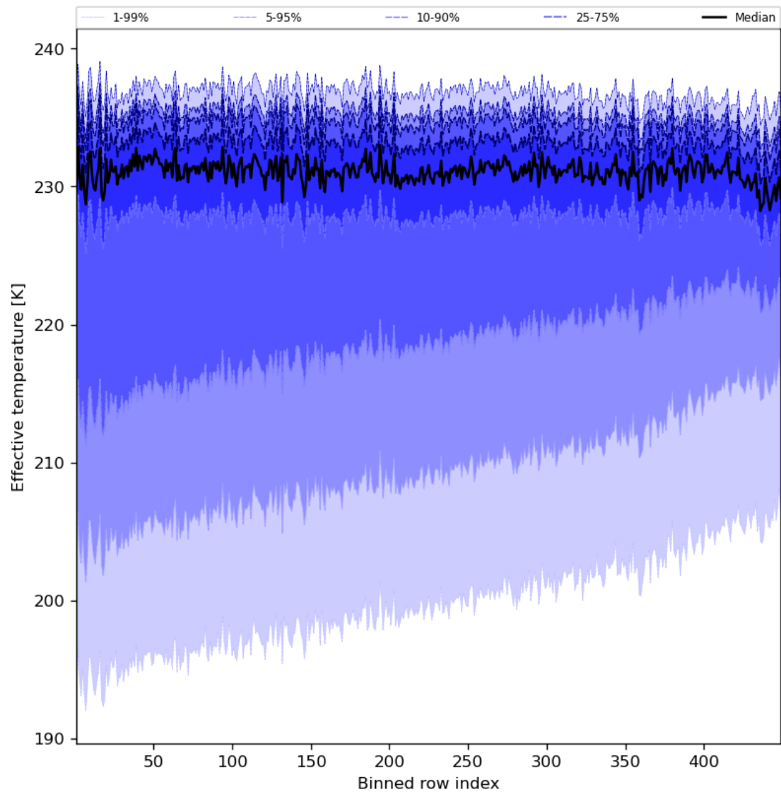
Figure 31: Along track statistics of “Effective temperature” for 2023-09-01 to 2023-09-03
