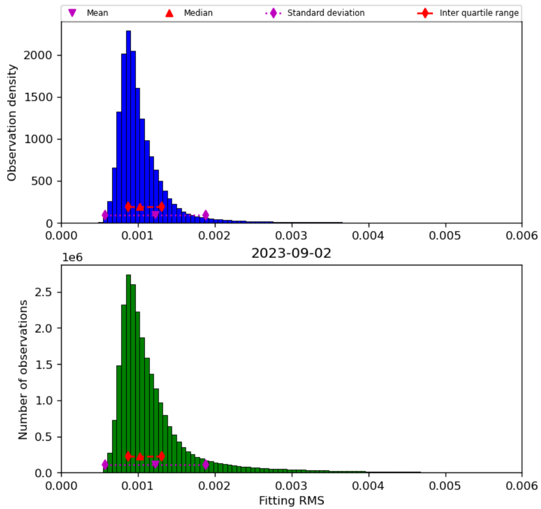
Figure 23: Histogram of “Fitting RMS” for 2023-09-01 to 2023-09-03
