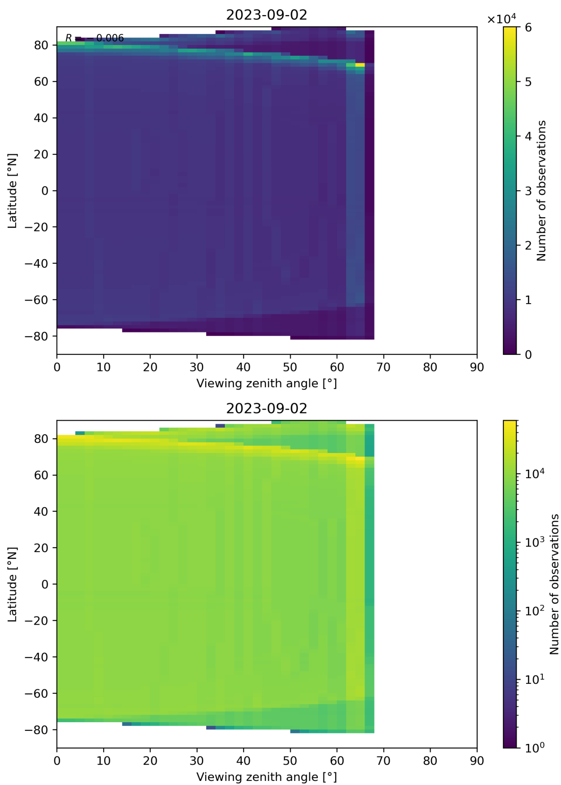
Figure 49: Scatter density plot of “Viewing zenith angle” against “Latitude” for 2023-09-01 to 2023-09-03.
