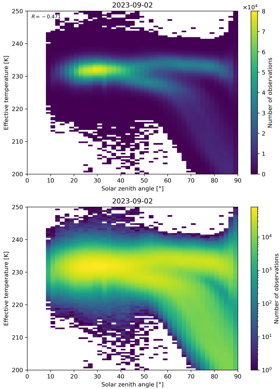
Figure 45: Scatter density plot of “Solar zenith angle” against “Effective temperature” for 2023-09-01 to 2023-09-03.
