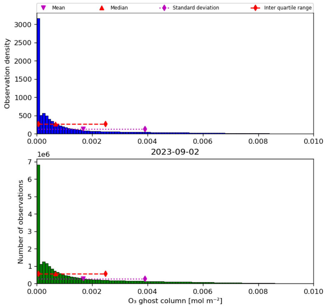
Figure 25: Histogram of “O 3 ghost column” for 2023-09-01 to 2023-09-03
