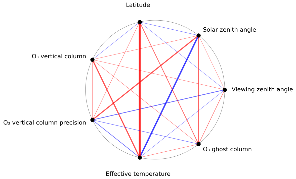
Figure 1: Map of correlation graph for 2023-09-01 to 2023-09-03.
