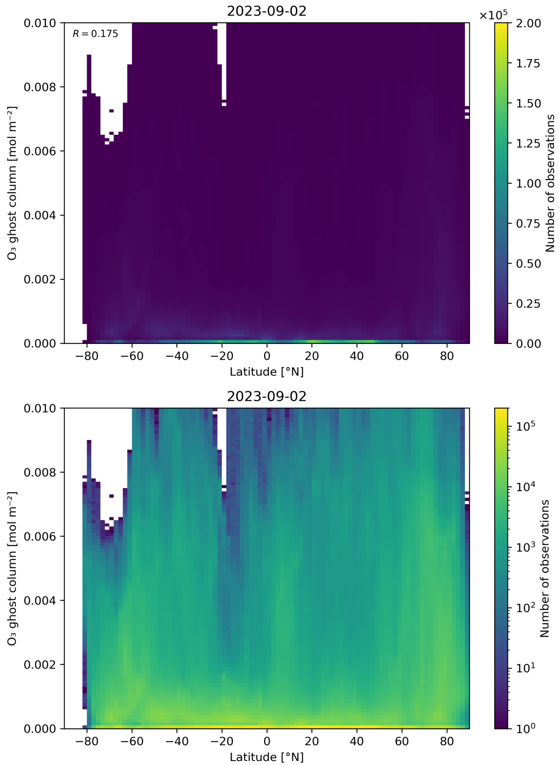
Figure 35: Scatter density plot of “Latitude” against “O 3 ghost column” for 2023-09-01 to 2023-09-03.
