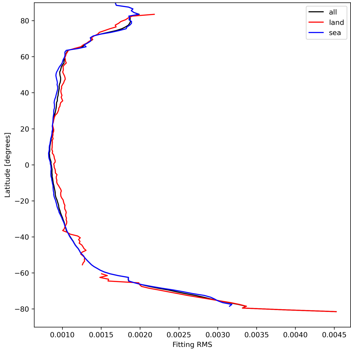
Figure 16: Zonal average of “Fitting RMS” for 2023-09-01 to 2023-09-03.
