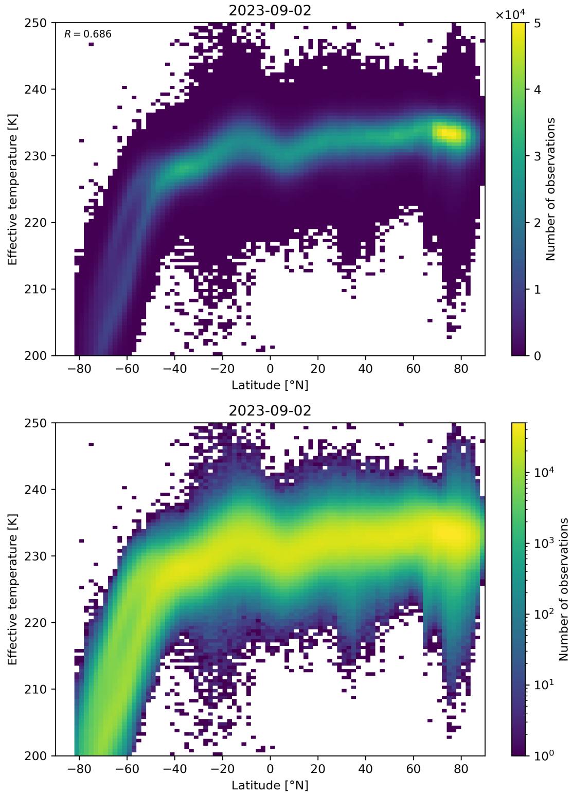
Figure 34: Scatter density plot of “Latitude” against “Effective temperature” for 2023-09-01 to 2023-09-03.
