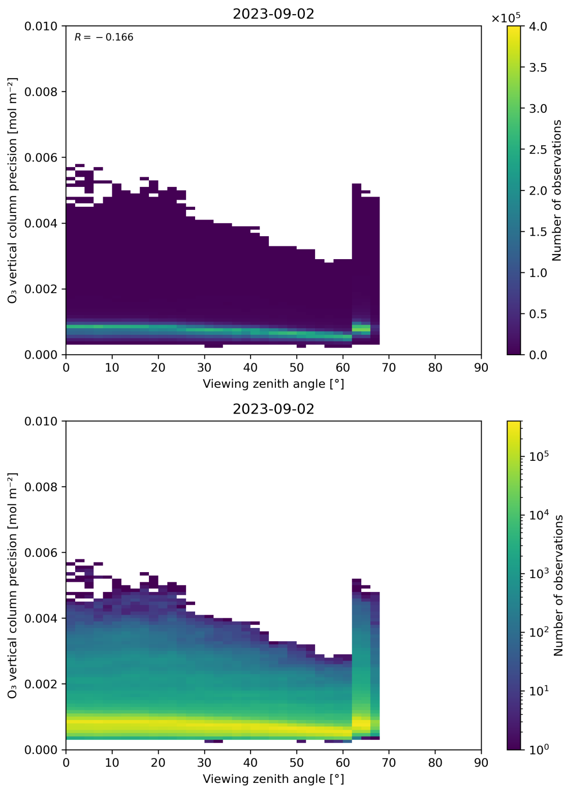
Figure 53: Scatter density plot of “Viewing zenith angle” against “O 3 vertical column precision” for 2023-09-01 to 2023-09-03.
