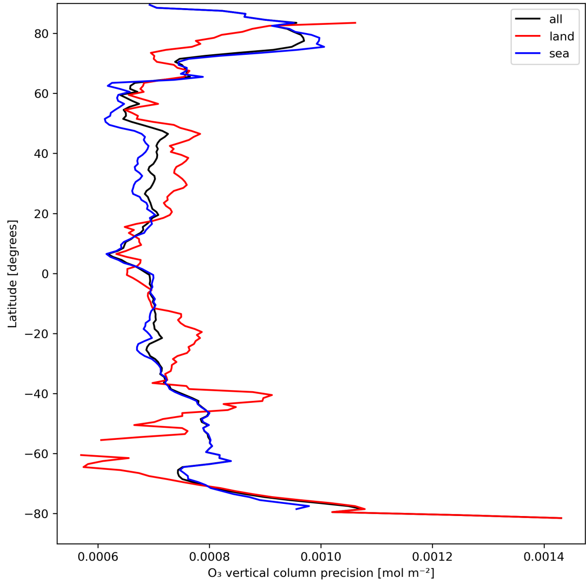
Figure 15: Zonal average of “O 3 vertical column precision” for 2023-09-01 to 2023-09-03.
