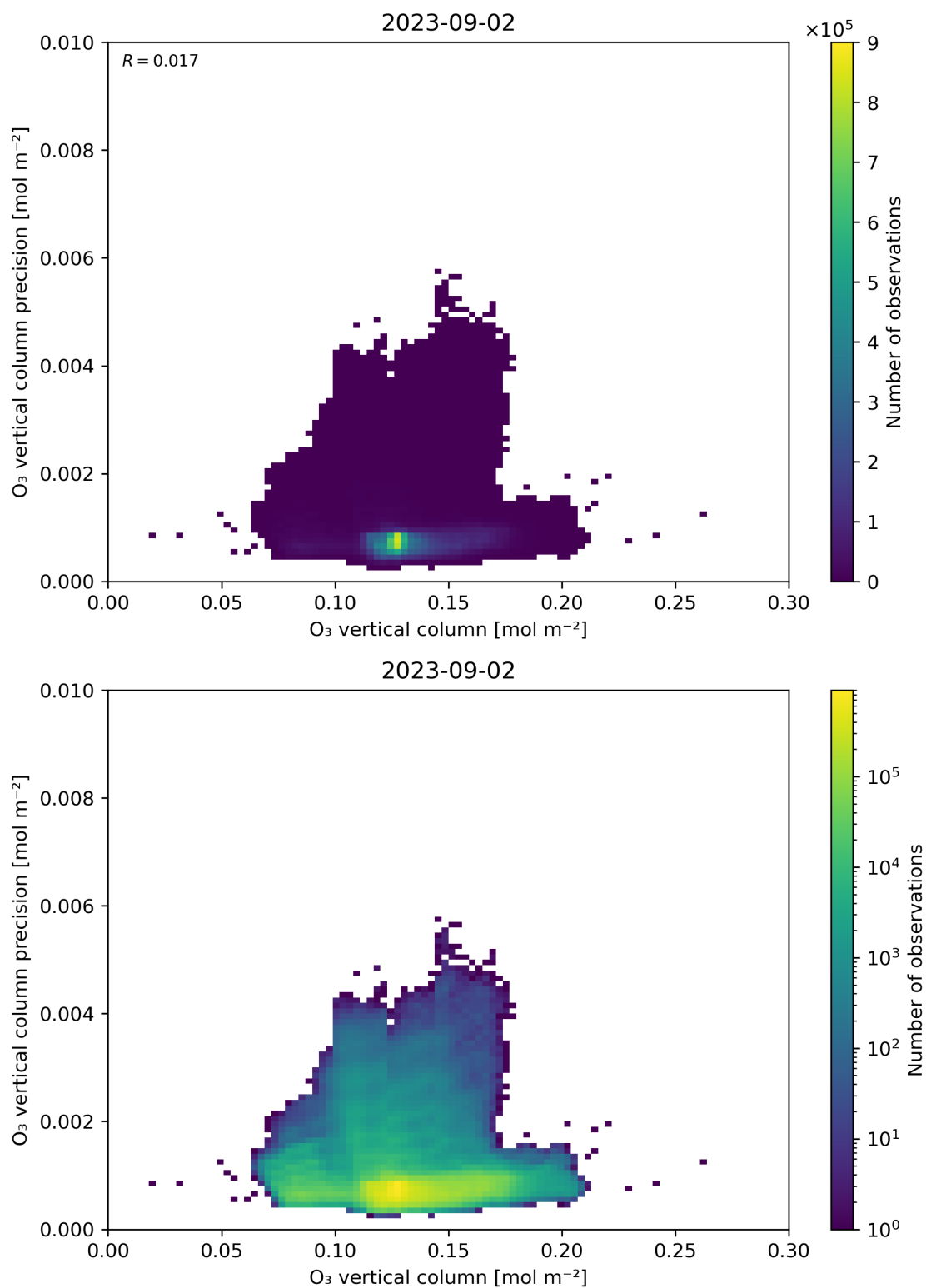
Figure 41: Scatter density plot of “O 3 vertical column” against “O 3 vertical column precision” for 2023-09-01 to 2023-09-03.
