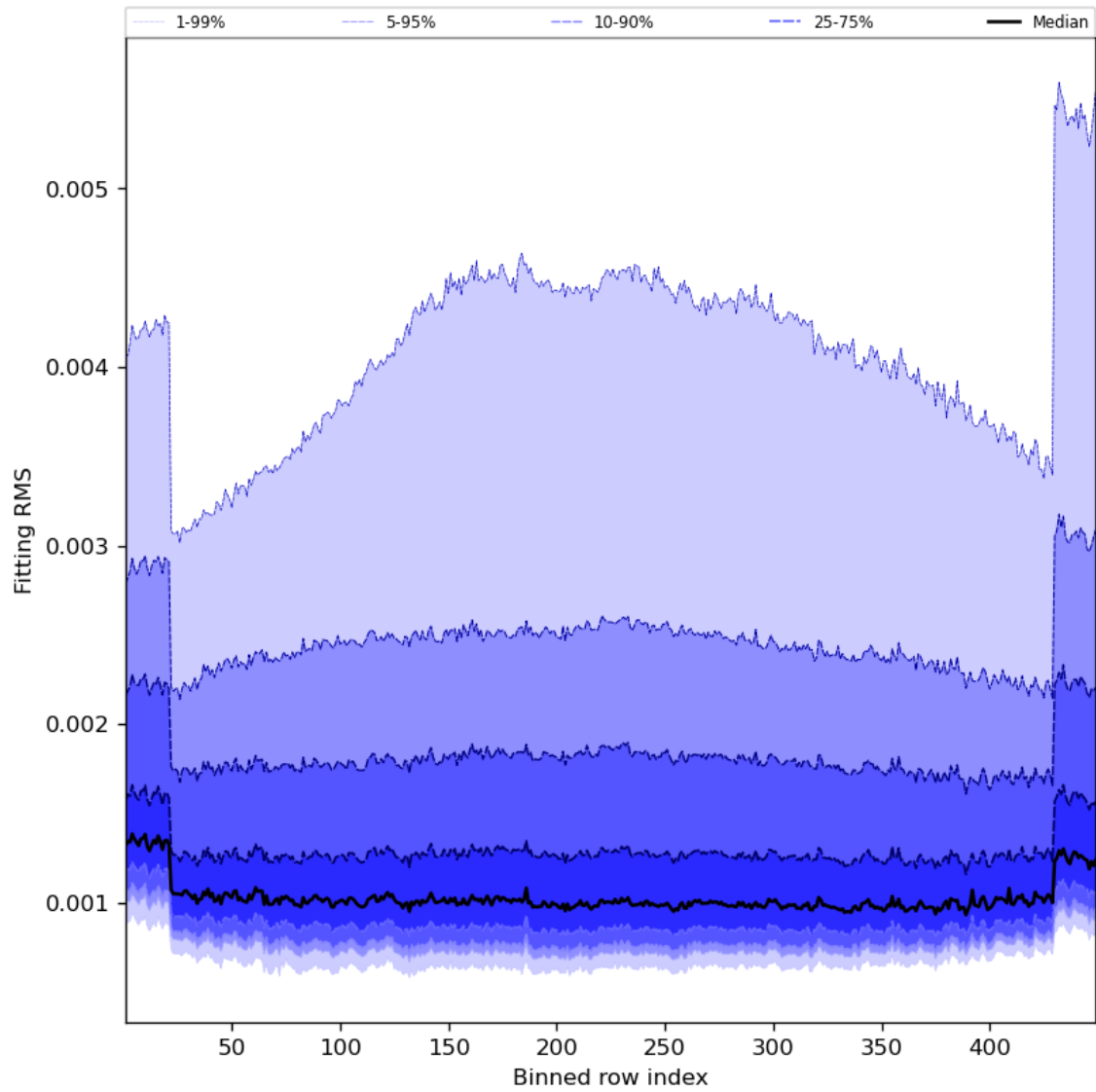
Figure 30: Along track statistics of “Fitting RMS” for 2023-09-01 to 2023-09-03
