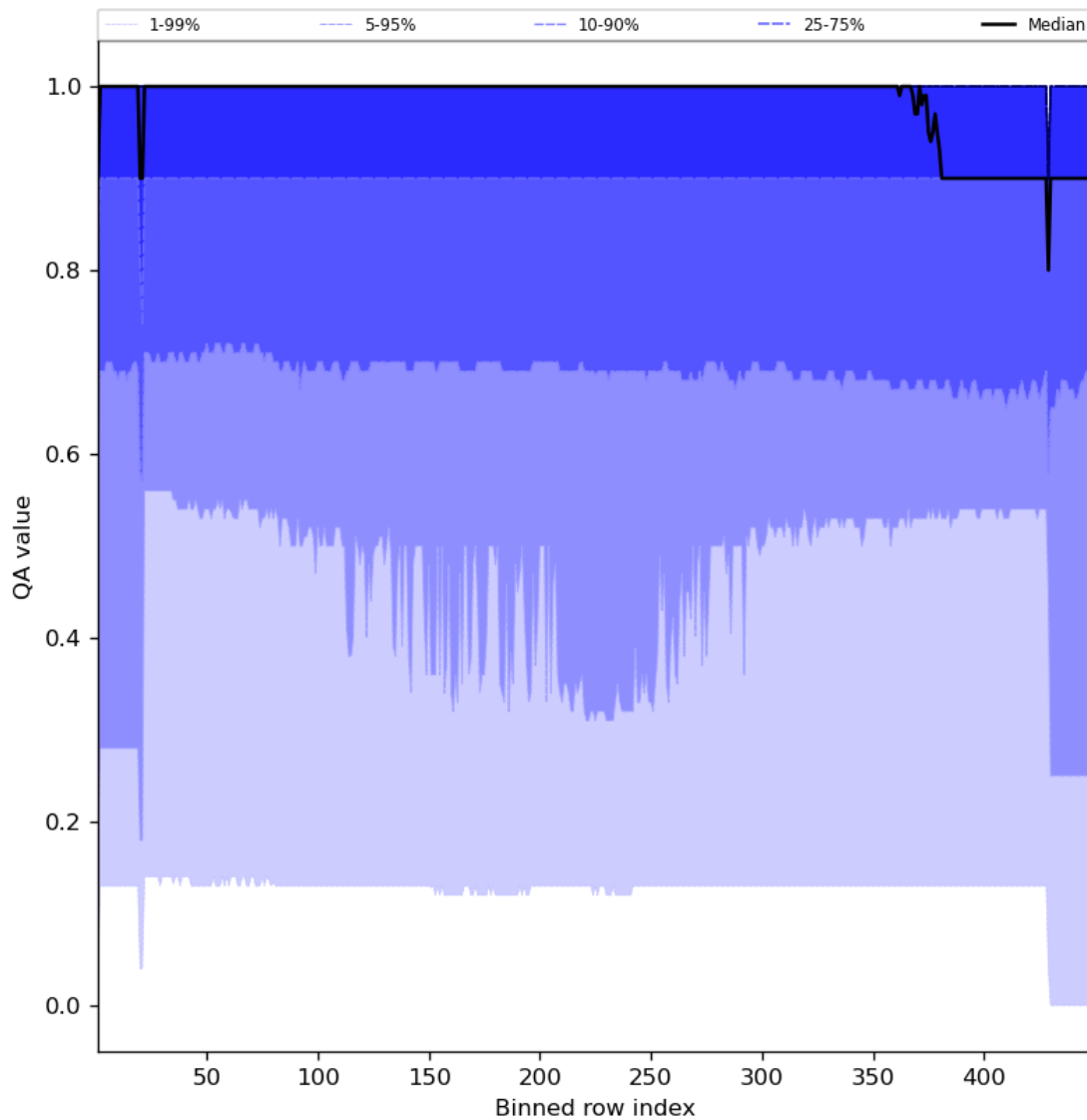
Figure 27: Along track statistics of “QA value” for 2023-09-01 to 2023-09-03
