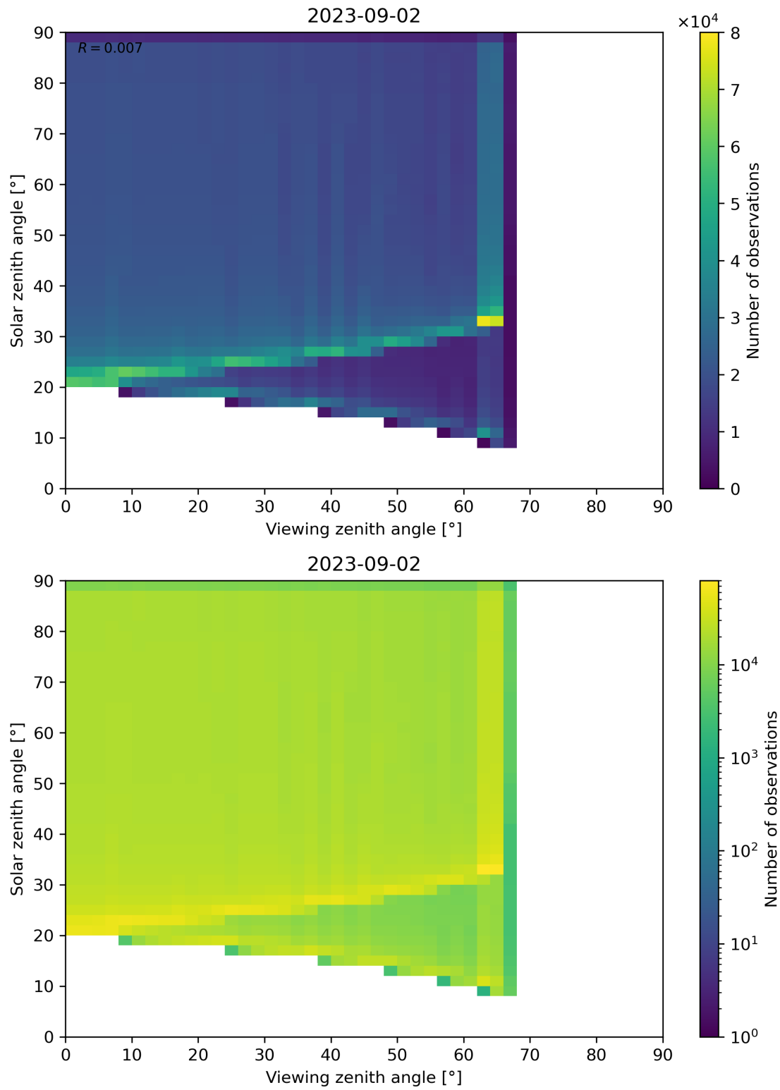
Figure 54: Scatter density plot of “Viewing zenith angle” against “Solar zenith angle” for 2023-09-01 to 2023-09-03.
