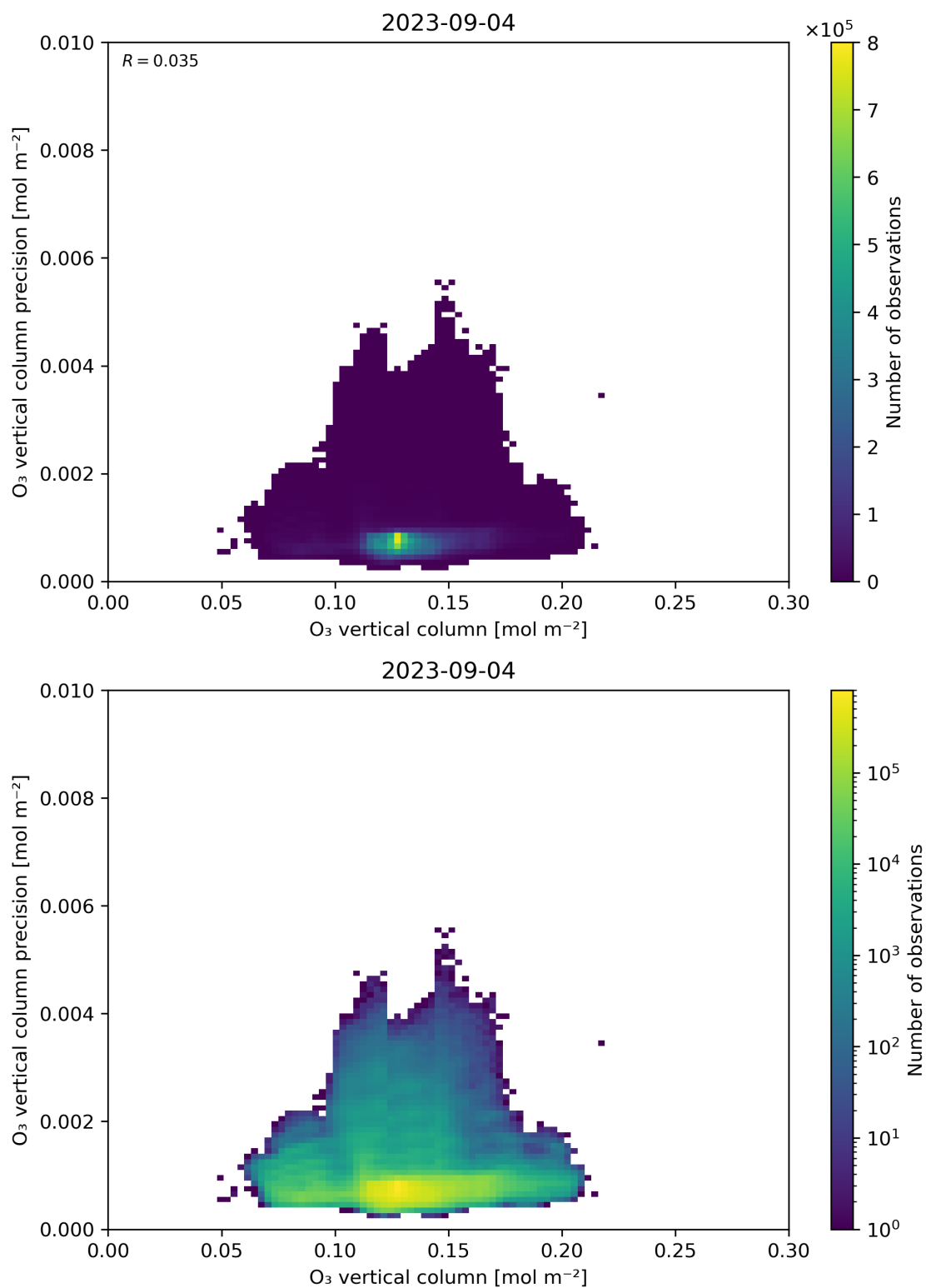
Figure 41: Scatter density plot of “O 3 vertical column” against “O 3 vertical column precision” for 2023-09-04 to 2023-09-05.
