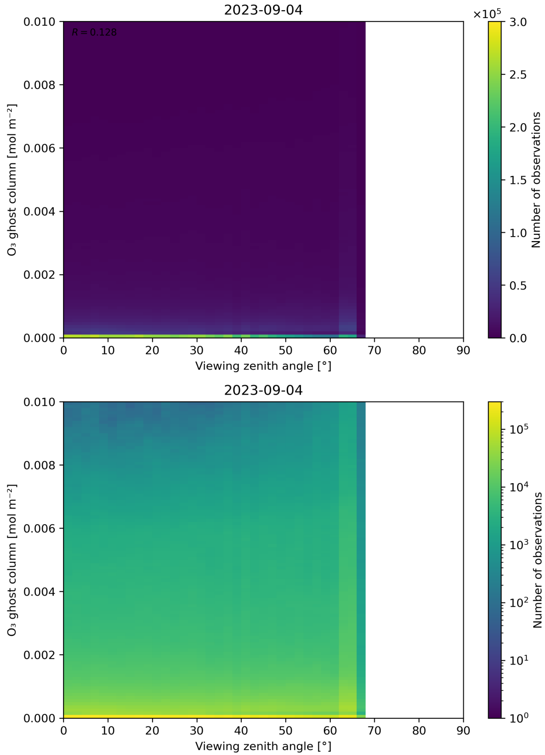
Figure 51: Scatter density plot of “Viewing zenith angle” against “O 3 ghost column” for 2023-09-04 to 2023-09-05.
