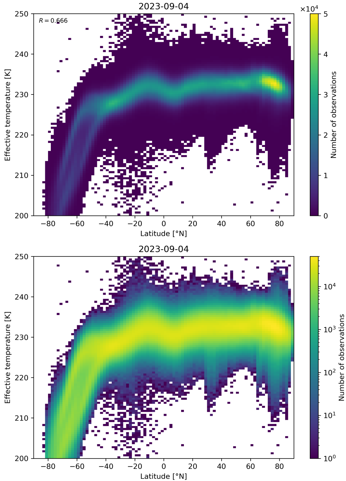
Figure 34: Scatter density plot of “Latitude” against “Effective temperature” for 2023-09-04 to 2023-09-05.
