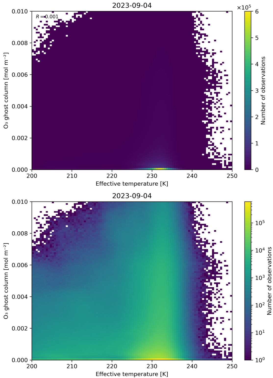
Figure 38: Scatter density plot of “Effective temperature” against “O 3 ghost column” for 2023-09-04 to 2023-09-05.
