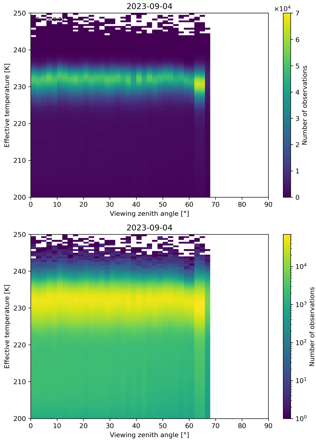
Figure 50: Scatter density plot of “Viewing zenith angle” against “Effective temperature” for 2023-09-04 to 2023-09-05.
