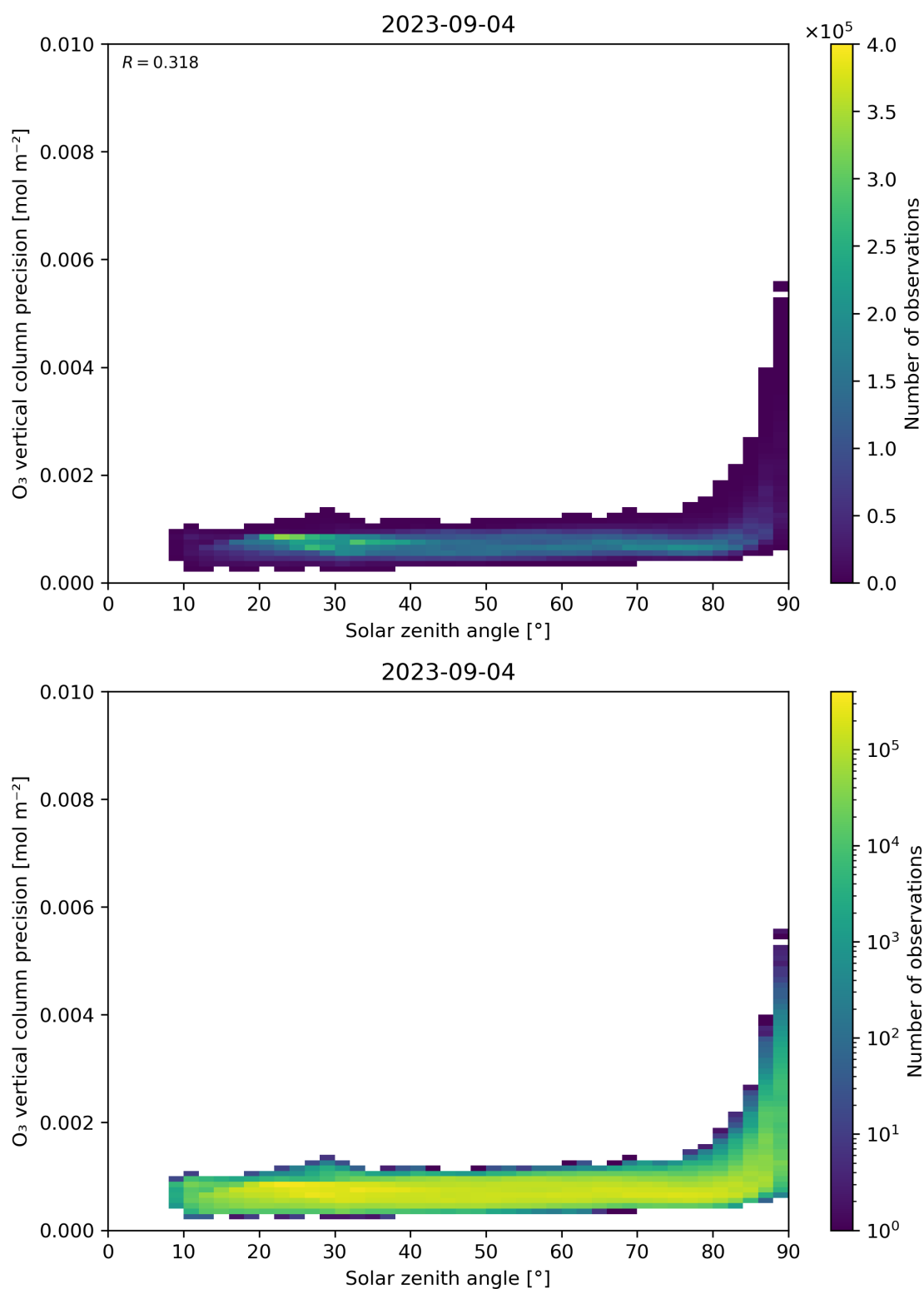
Figure 48: Scatter density plot of “Solar zenith angle” against “O 3 vertical column precision” for 2023-09-04 to 2023-09-05.
