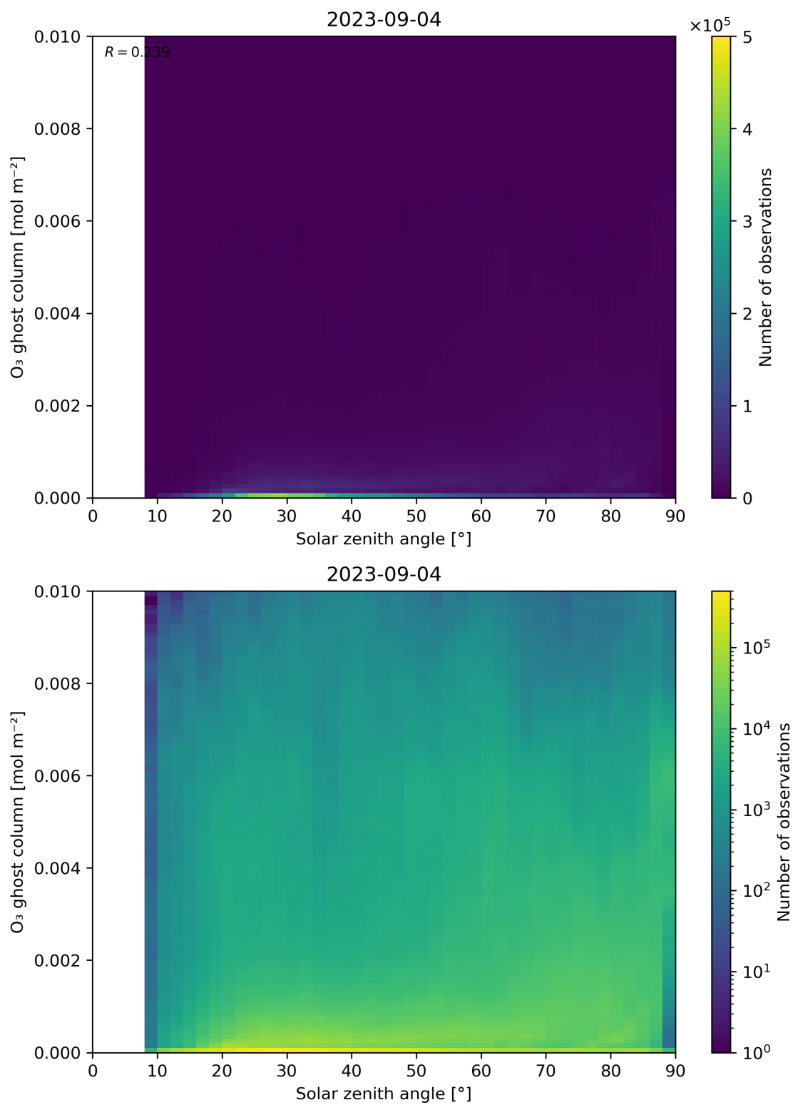
Figure 46: Scatter density plot of “Solar zenith angle” against “O 3 ghost column” for 2023-09-04 to 2023-09-05.
