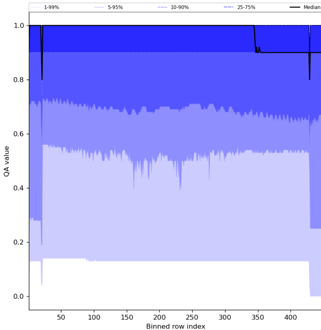
Figure 27: Along track statistics of “QA value” for 2023-09-04 to 2023-09-05
