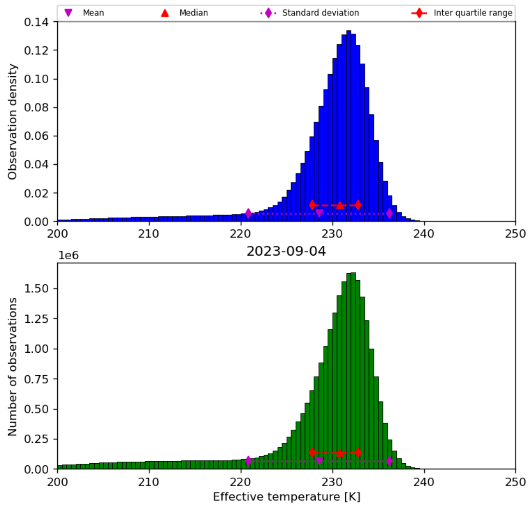
Figure 24: Histogram of “Effective temperature” for 2023-09-04 to 2023-09-05
