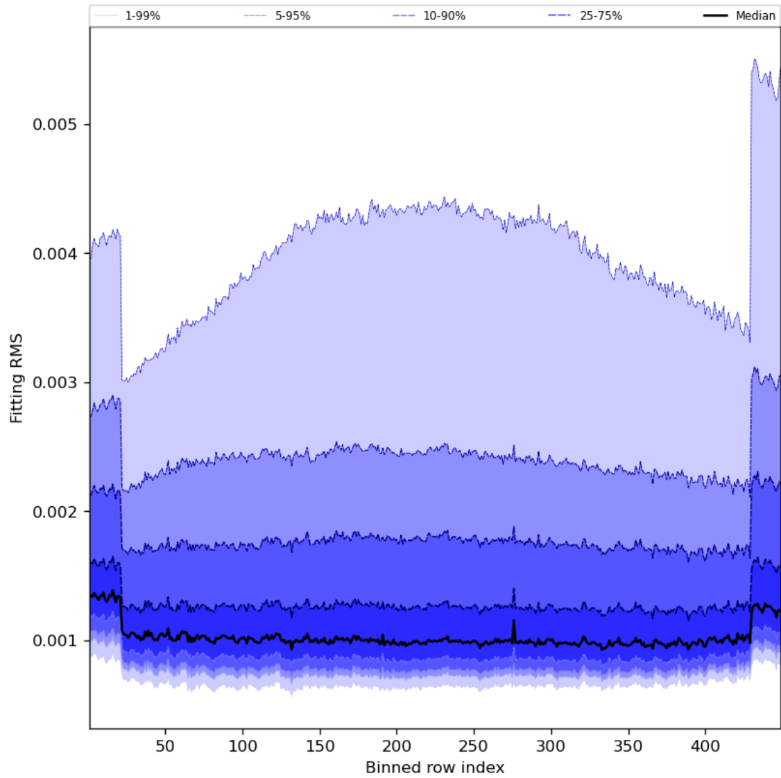
Figure 30: Along track statistics of “Fitting RMS” for 2023-09-04 to 2023-09-05
