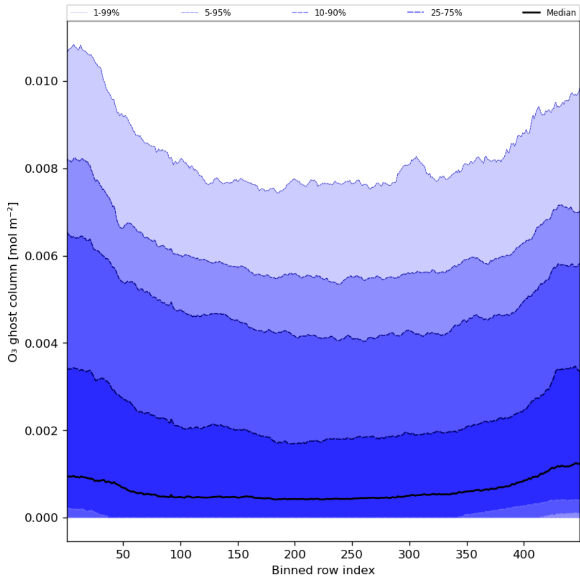
Figure 32: Along track statistics of “O 3 ghost column” for 2023-09-04 to 2023-09-05
