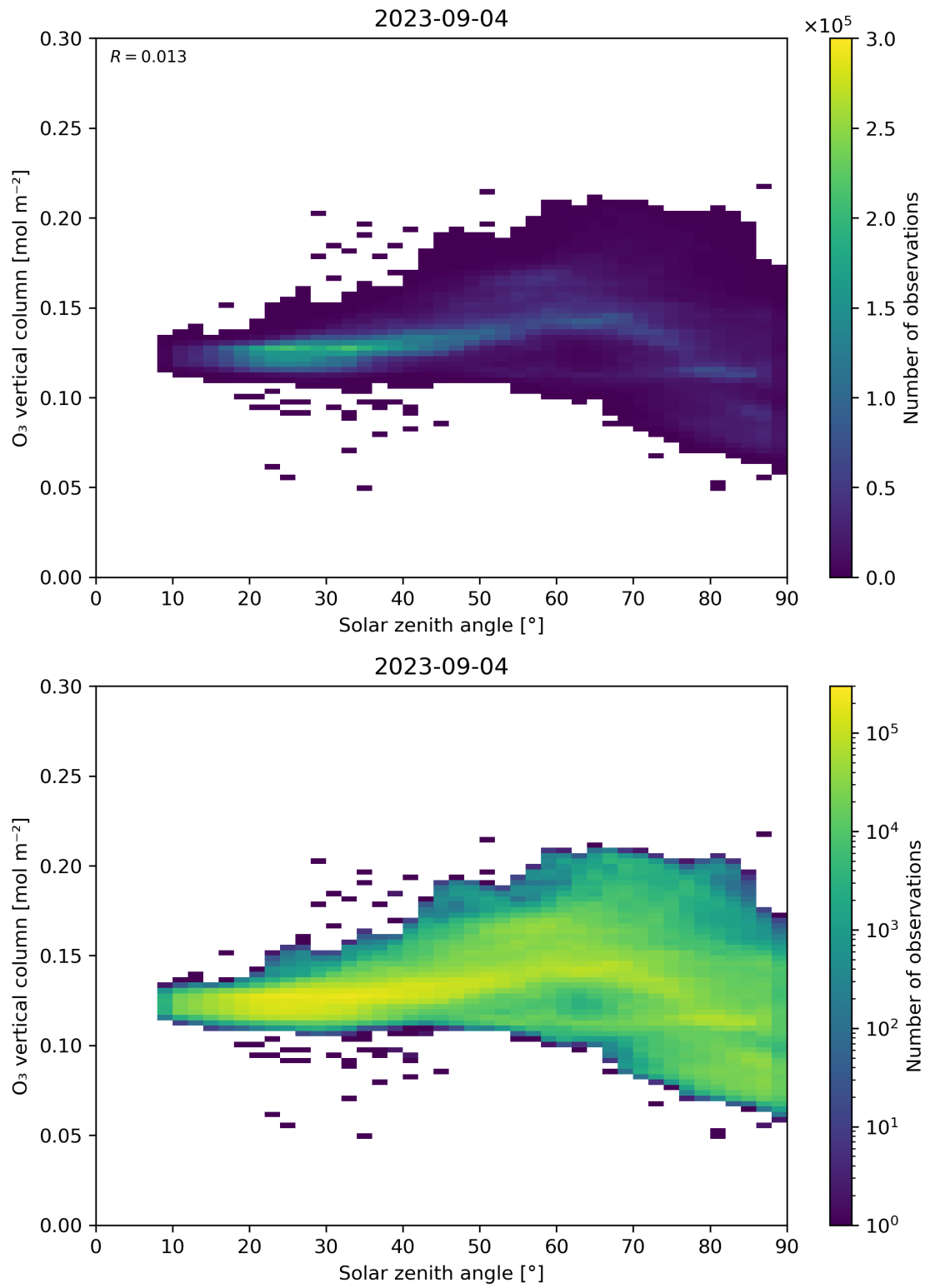
Figure 47: Scatter density plot of “Solar zenith angle” against “O 3 vertical column” for 2023-09-04 to 2023-09-05.
