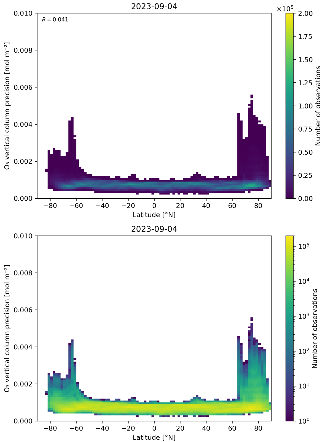
Figure 37: Scatter density plot of “Latitude” against “O 3 vertical column precision” for 2023-09-04 to 2023-09-05.
