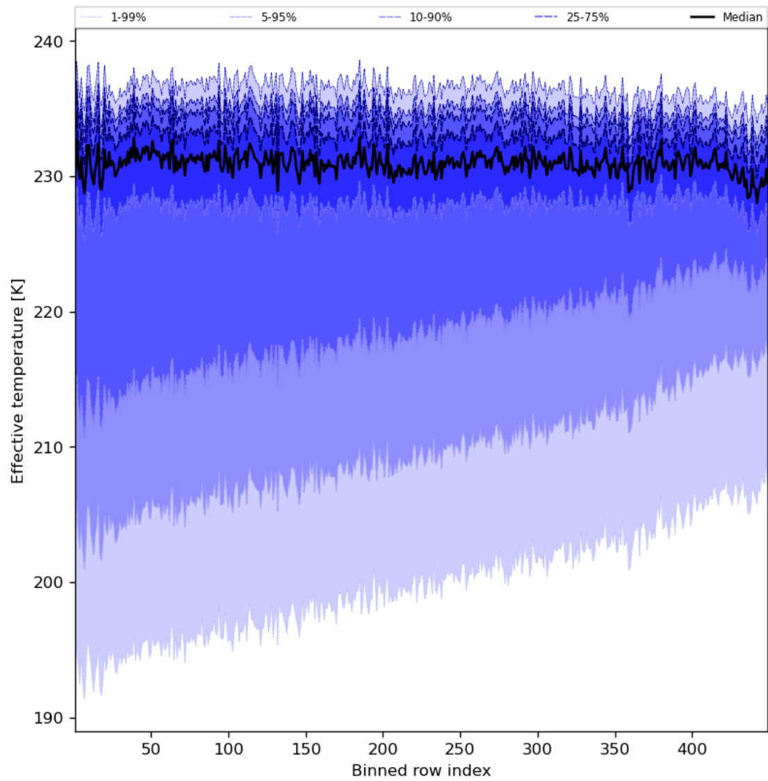
Figure 31: Along track statistics of “Effective temperature” for 2023-09-04 to 2023-09-05
