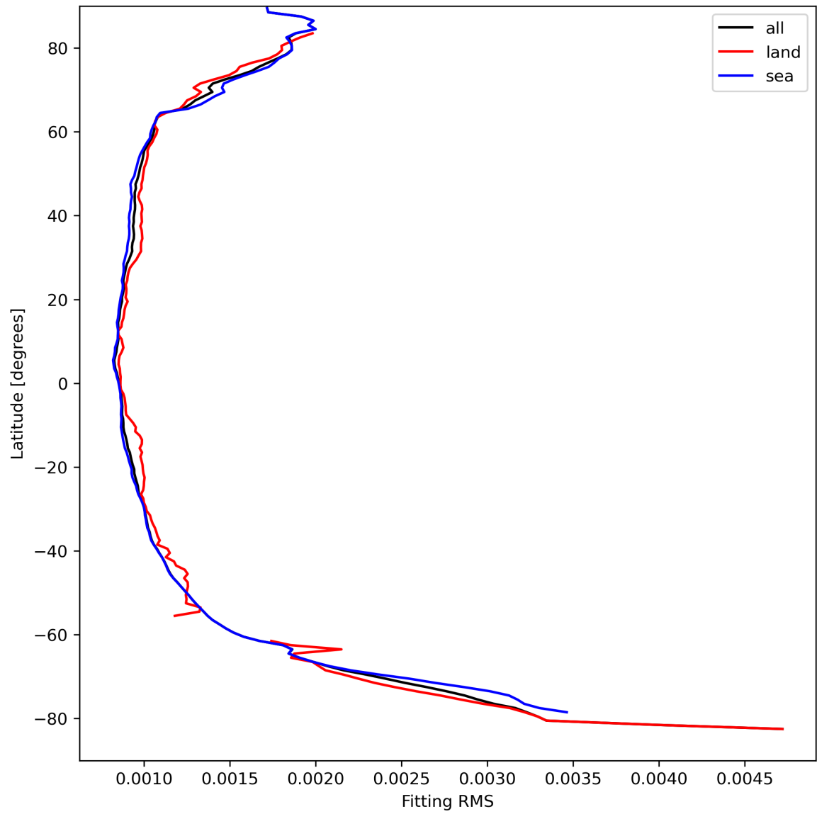
Figure 16: Zonal average of “Fitting RMS” for 2023-09-04 to 2023-09-05.
