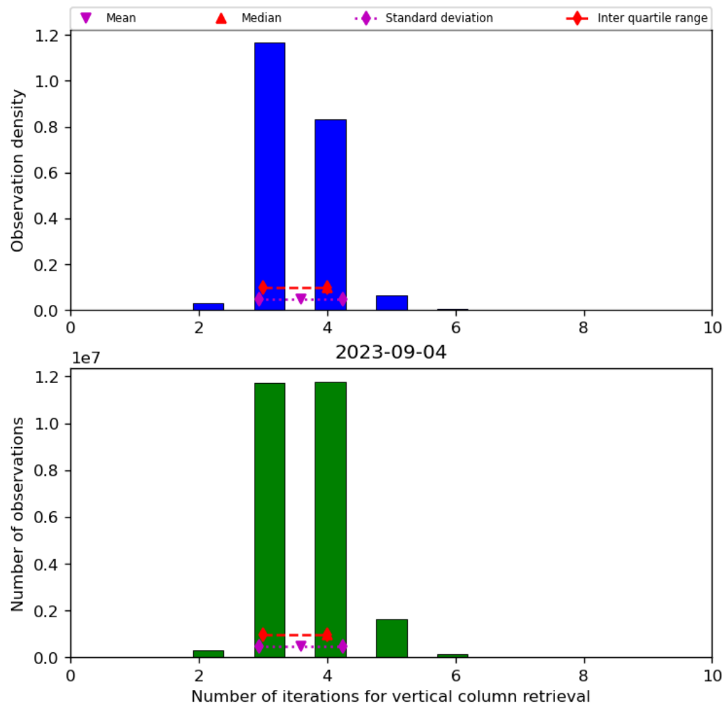
Figure 26: Histogram of “Number of iterations for vertical column retrieval” for 2023-09-04 to 2023-09-05
