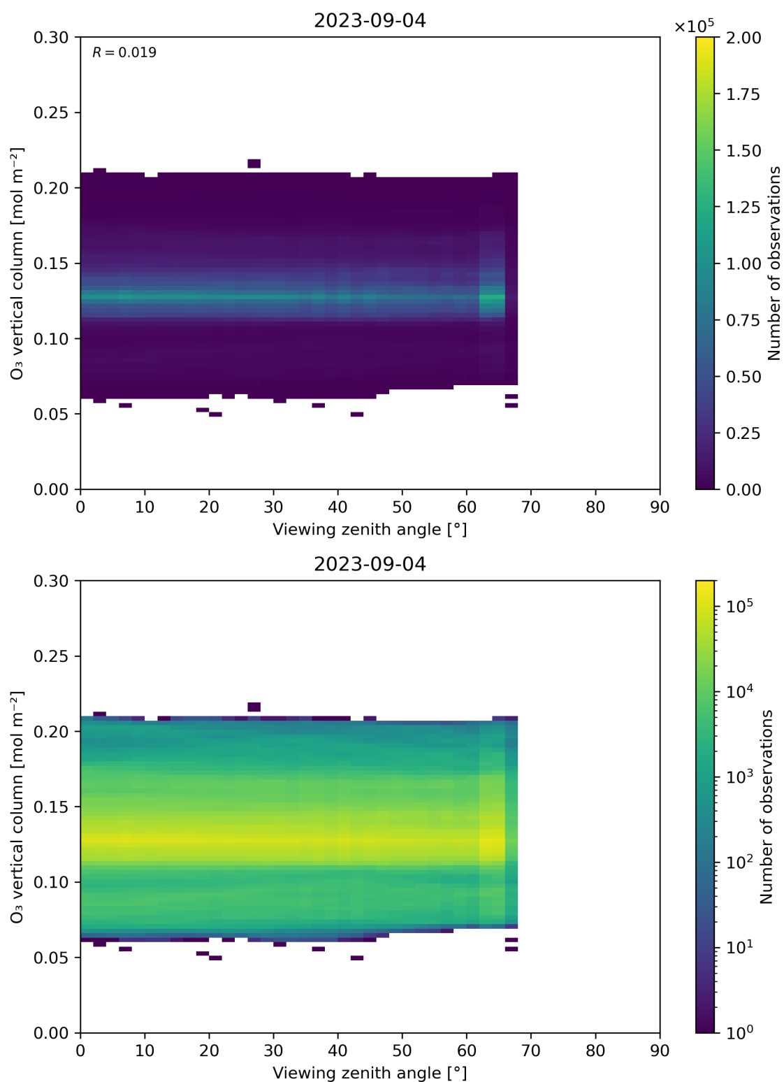
Figure 52: Scatter density plot of “Viewing zenith angle” against “O 3 vertical column” for 2023-09-04 to 2023-09-05.
