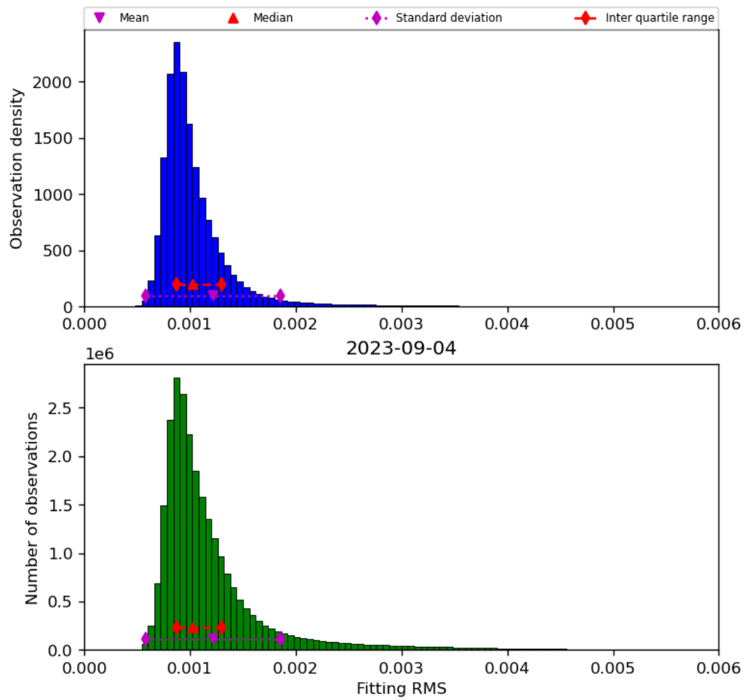
Figure 23: Histogram of “Fitting RMS” for 2023-09-04 to 2023-09-05
