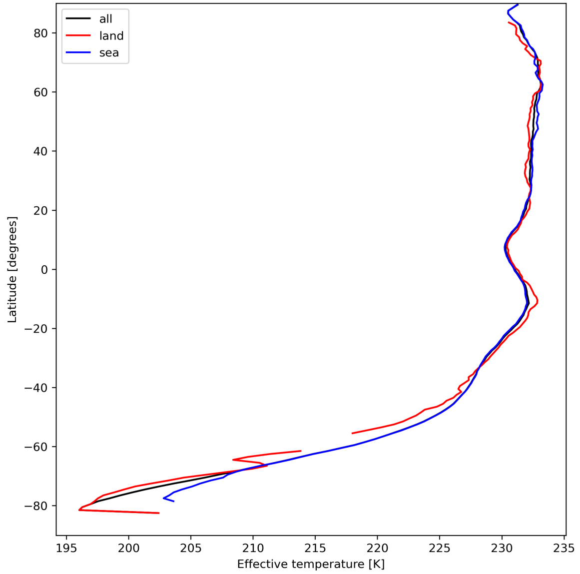
Figure 17: Zonal average of "Effective temperature" for 2023-09-04 to 2023-09-05.
