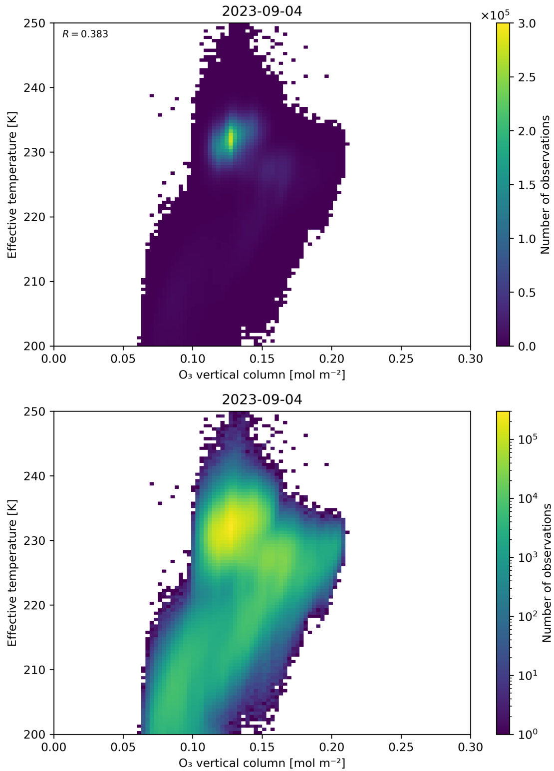
Figure 39: Scatter density plot of “O 3 vertical column” against “Effective temperature” for 2023-09-04 to 2023-09-05.
