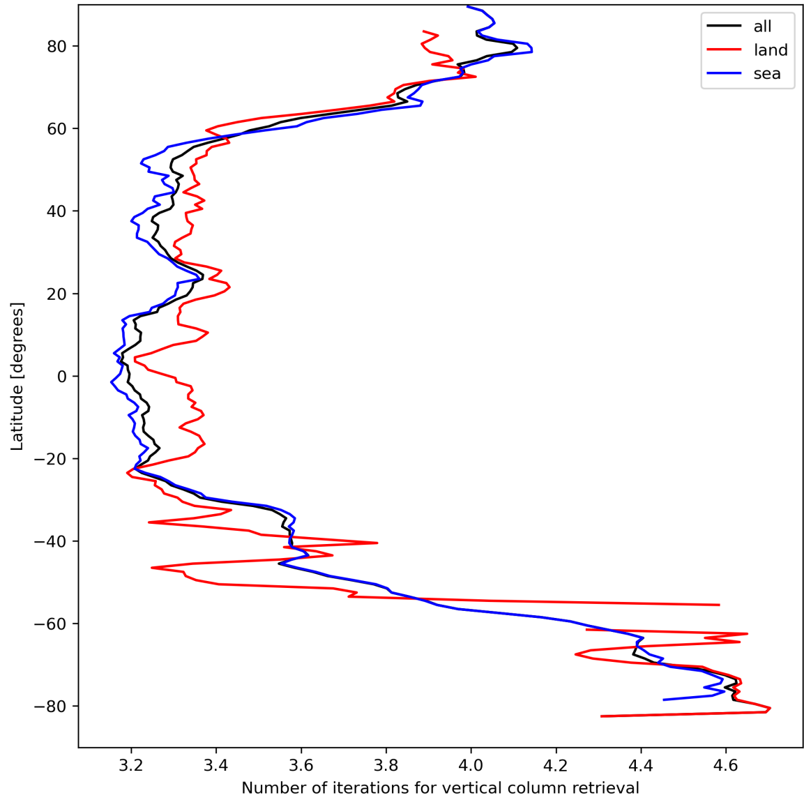
Figure 19: Zonal average of “Number of iterations for vertical column retrieval” for 2023-09-04 to 2023-09-05.
