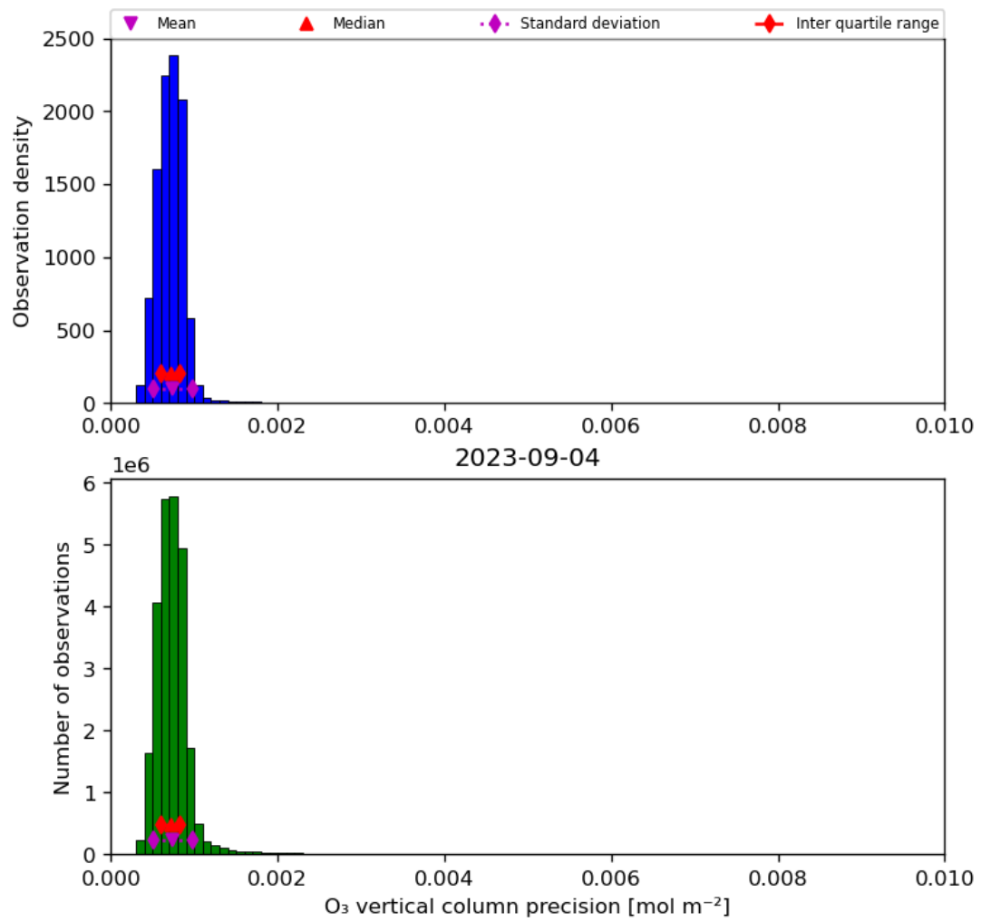
Figure 22: Histogram of “O 3 vertical column precision” for 2023-09-04 to 2023-09-05
