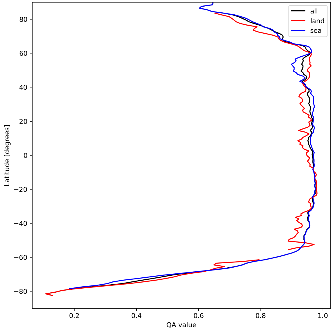
Figure 13: Zonal average of “QA value” for 2023-09-04 to 2023-09-05.
