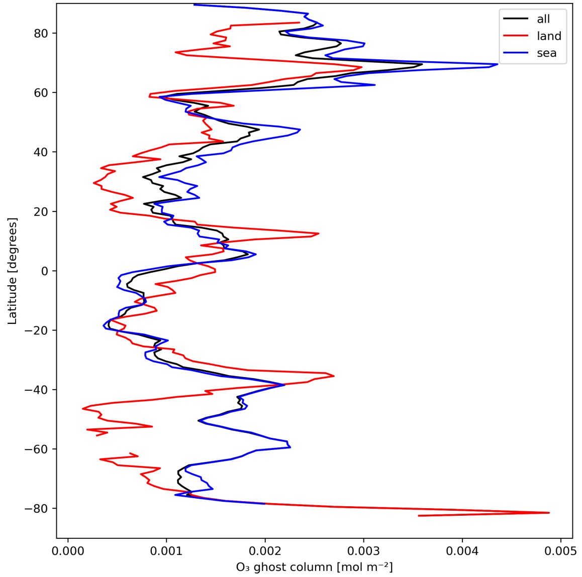
Figure 18: Zonal average of "O 3 ghost column" for 2023-09-04 to 2023-09-05.
