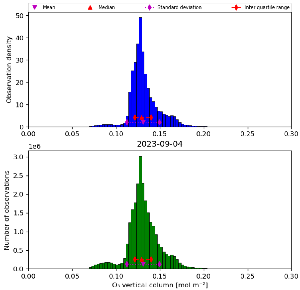
Figure 21: Histogram of “O 3 vertical column” for 2023-09-04 to 2023-09-05
