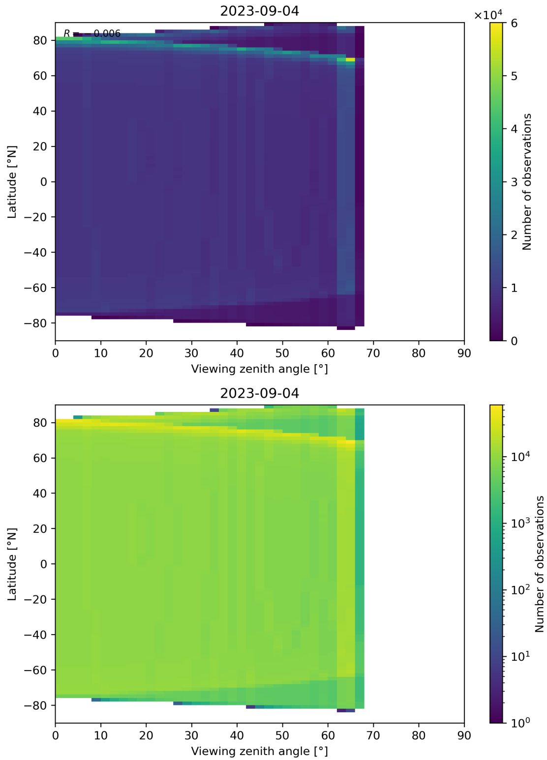
Figure 49: Scatter density plot of “Viewing zenith angle” against “Latitude” for 2023-09-04 to 2023-09-05.
