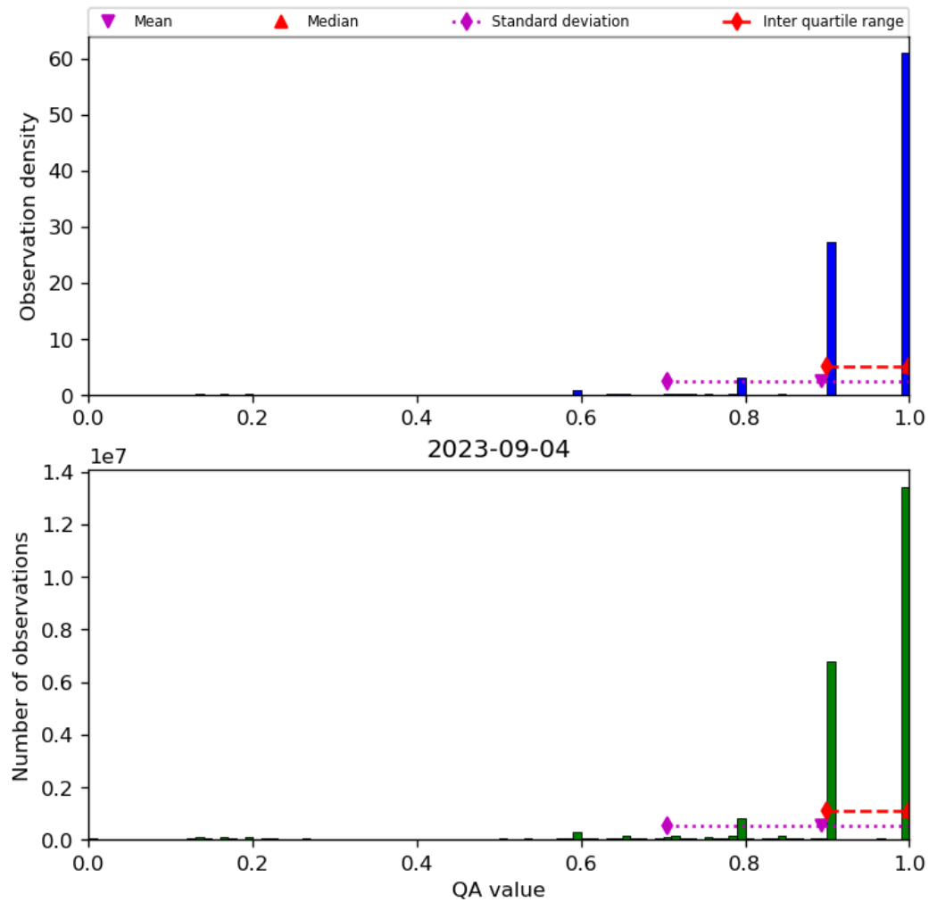
Figure 20: Histogram of “QA value” for 2023-09-04 to 2023-09-05
