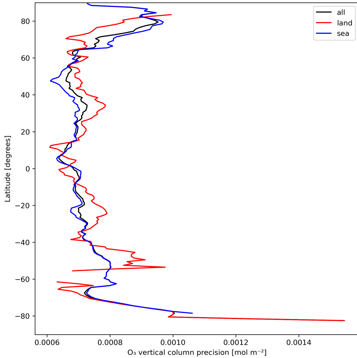
Figure 15: Zonal average of “O 3 vertical column precision” for 2023-09-04 to 2023-09-05.
