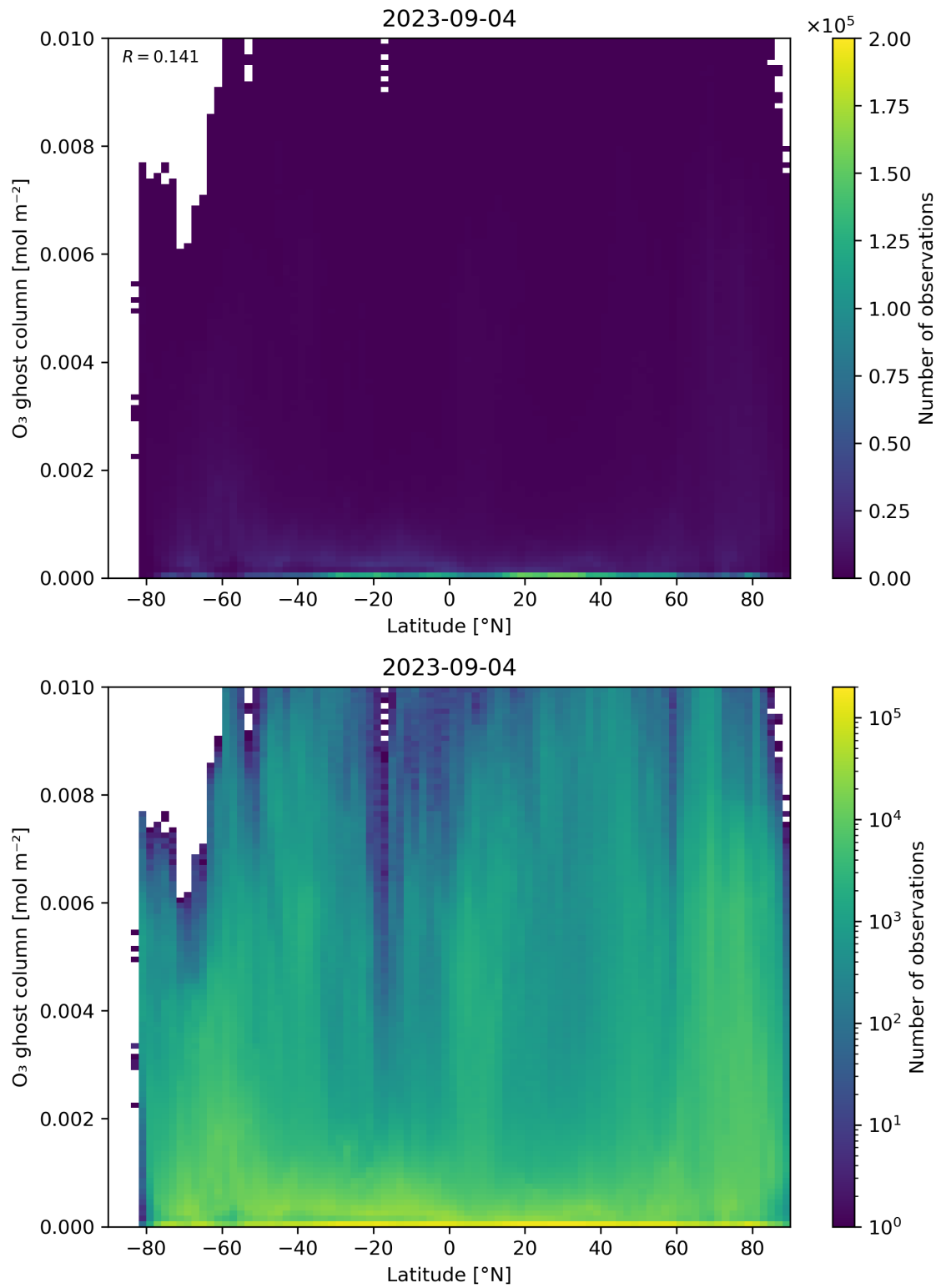
Figure 35: Scatter density plot of “Latitude” against “O 3 ghost column” for 2023-09-04 to 2023-09-05.
