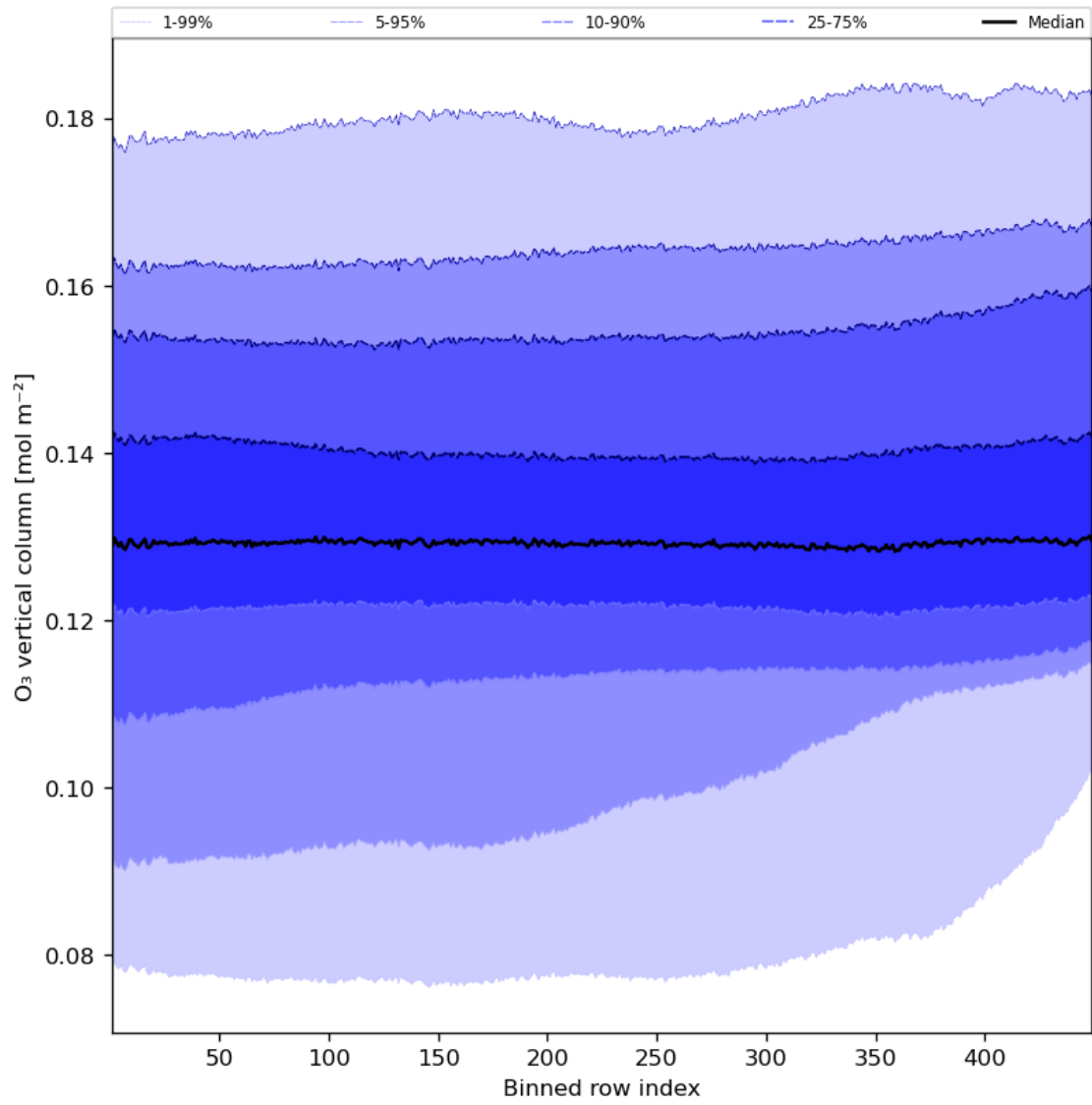
Figure 28: Along track statistics of “O 3 vertical column” for 2023-09-04 to 2023-09-05
