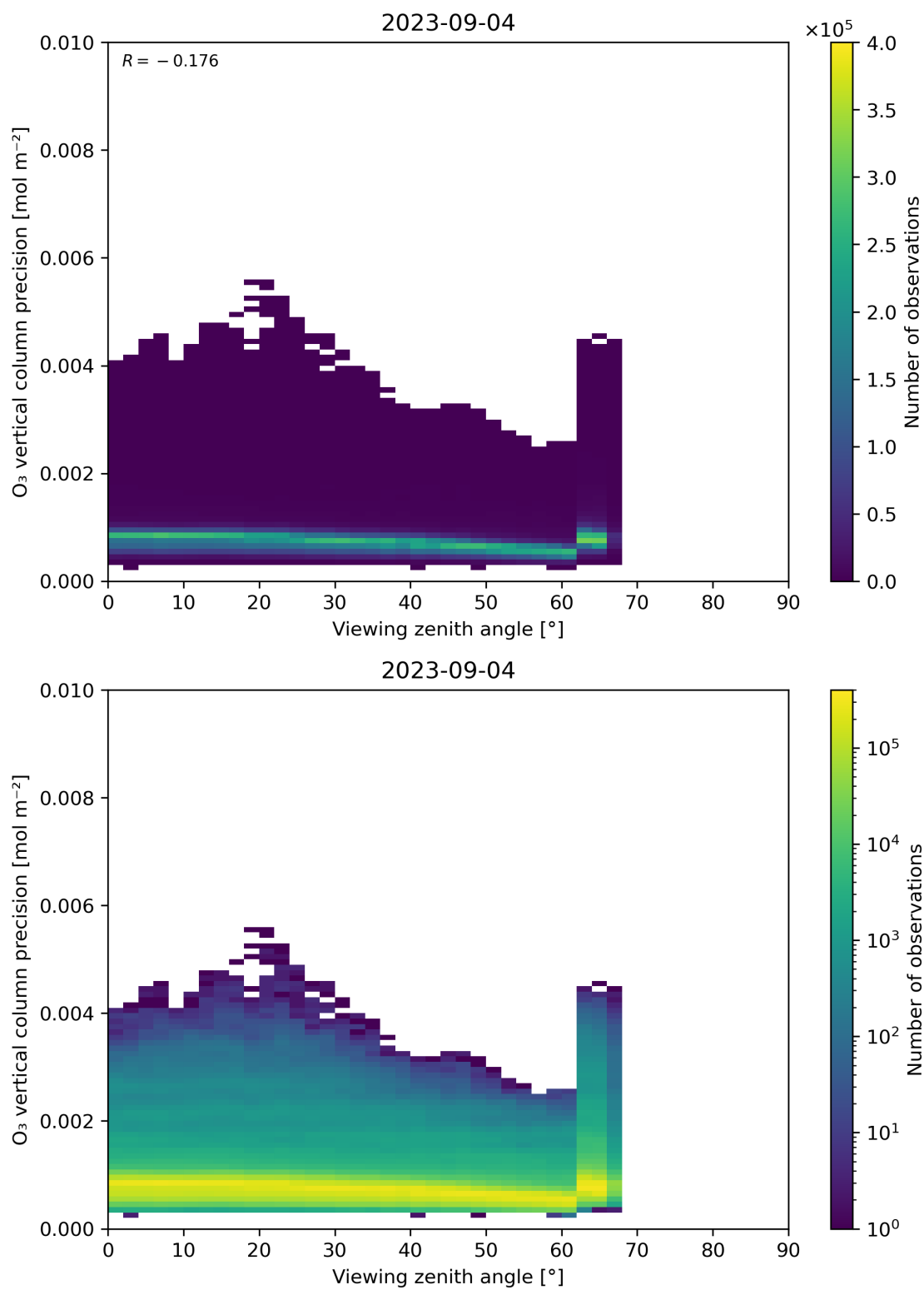
Figure 53: Scatter density plot of “Viewing zenith angle” against “O 3 vertical column precision” for 2023-09-04 to 2023-09-05.
