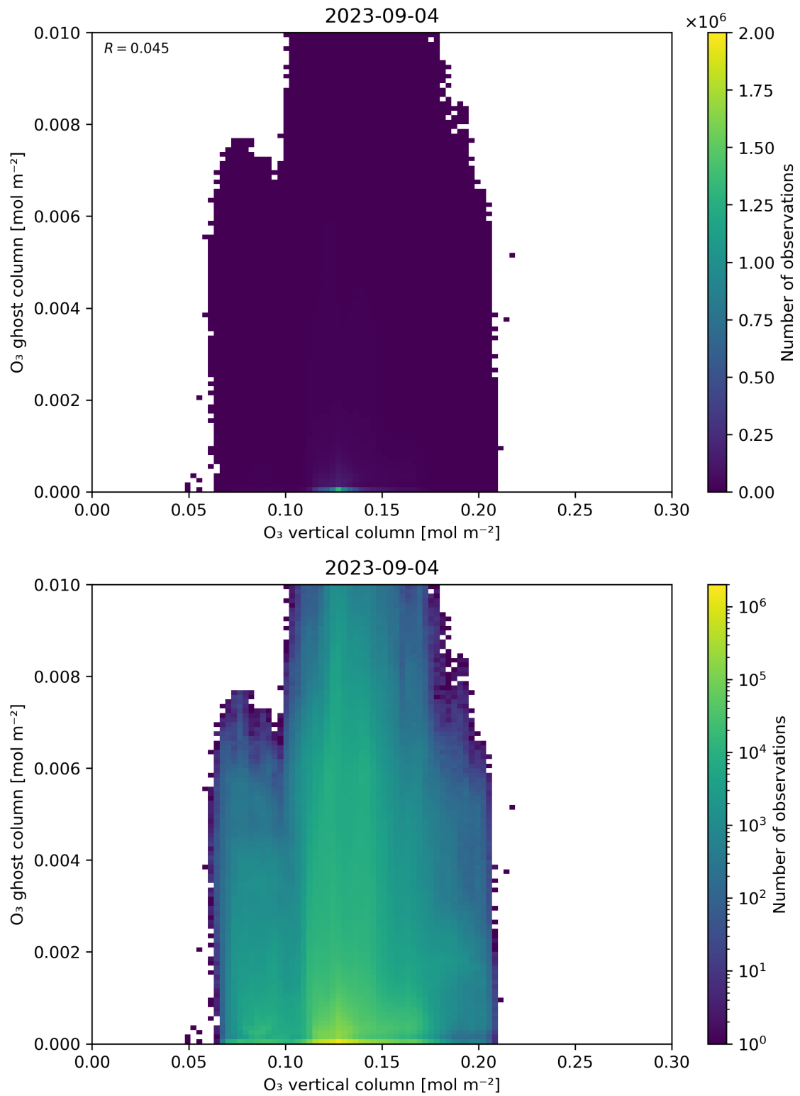
Figure 40: Scatter density plot of “O 3 vertical column” against “O 3 ghost column” for 2023-09-04 to 2023-09-05.
