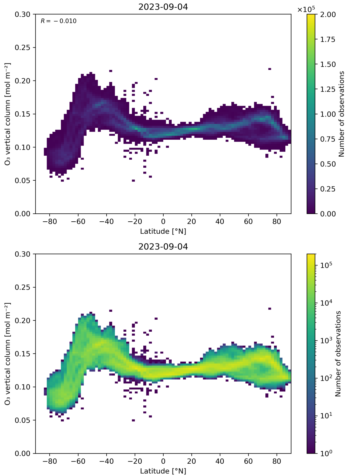
Figure 36: Scatter density plot of “Latitude” against “O 3 vertical column” for 2023-09-04 to 2023-09-05.
