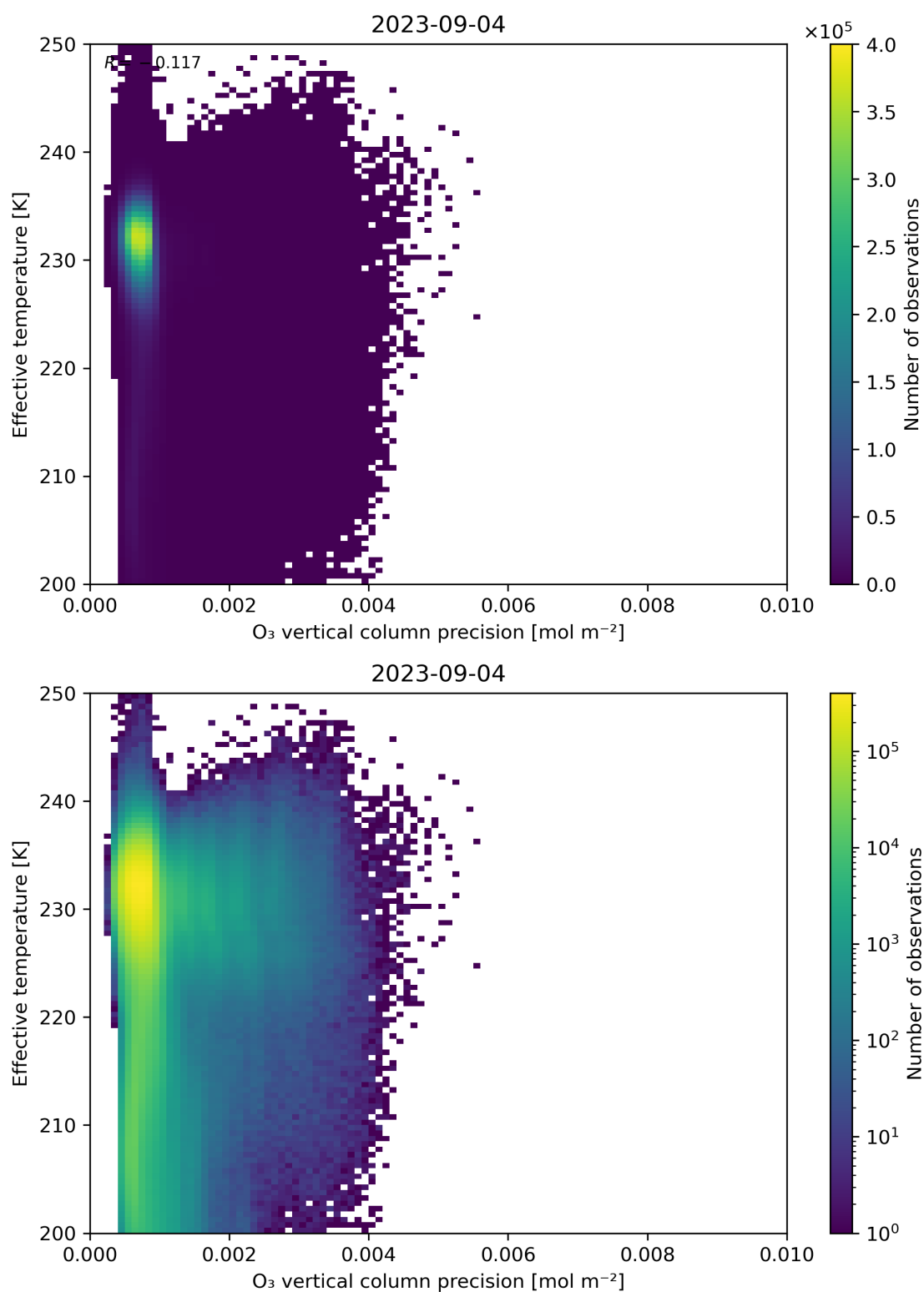
Figure 42: Scatter density plot of “O 3 vertical column precision” against “Effective temperature” for 2023-09-04 to 2023-09-05.
