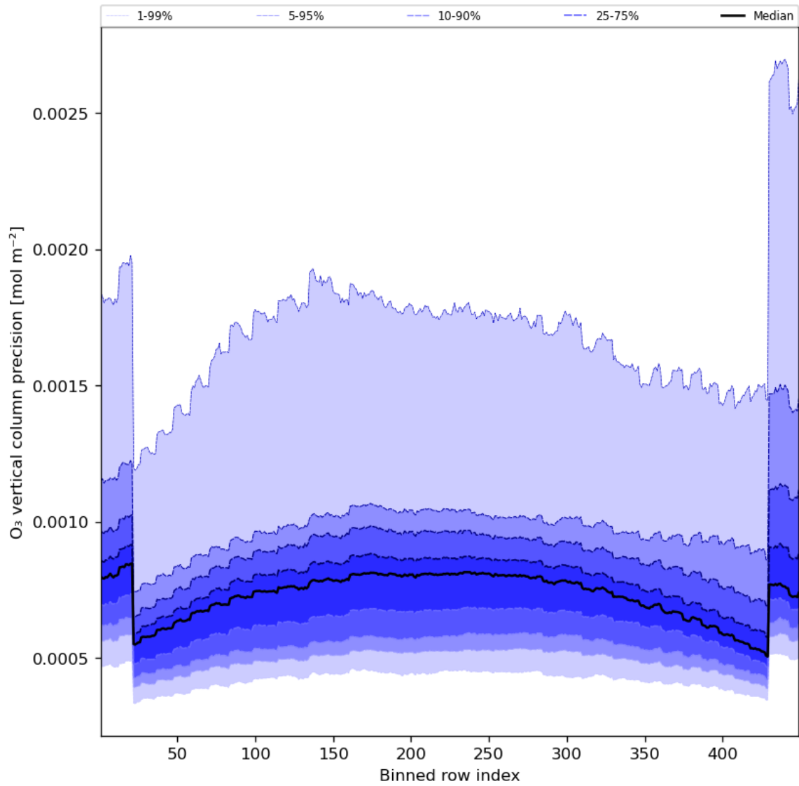
Figure 29: Along track statistics of “O 3 vertical column precision” for 2023-09-04 to 2023-09-05
