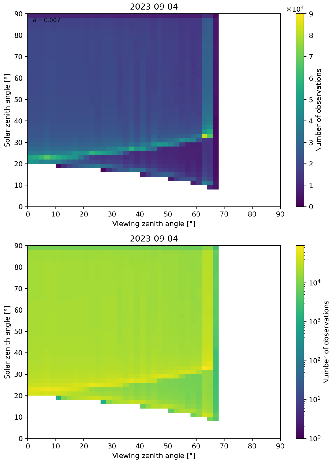
Figure 54: Scatter density plot of “Viewing zenith angle” against “Solar zenith angle” for 2023-09-04 to 2023-09-05.
