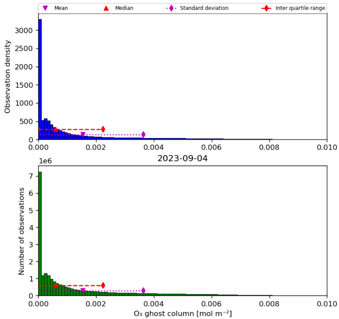
Figure 25: Histogram of “O 3 ghost column” for 2023-09-04 to 2023-09-05
