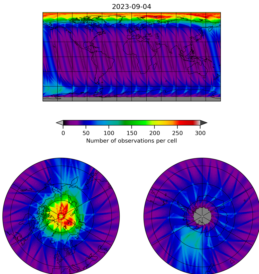
Figure 12: Map of the number of observations for 2023-09-04 to 2023-09-05
