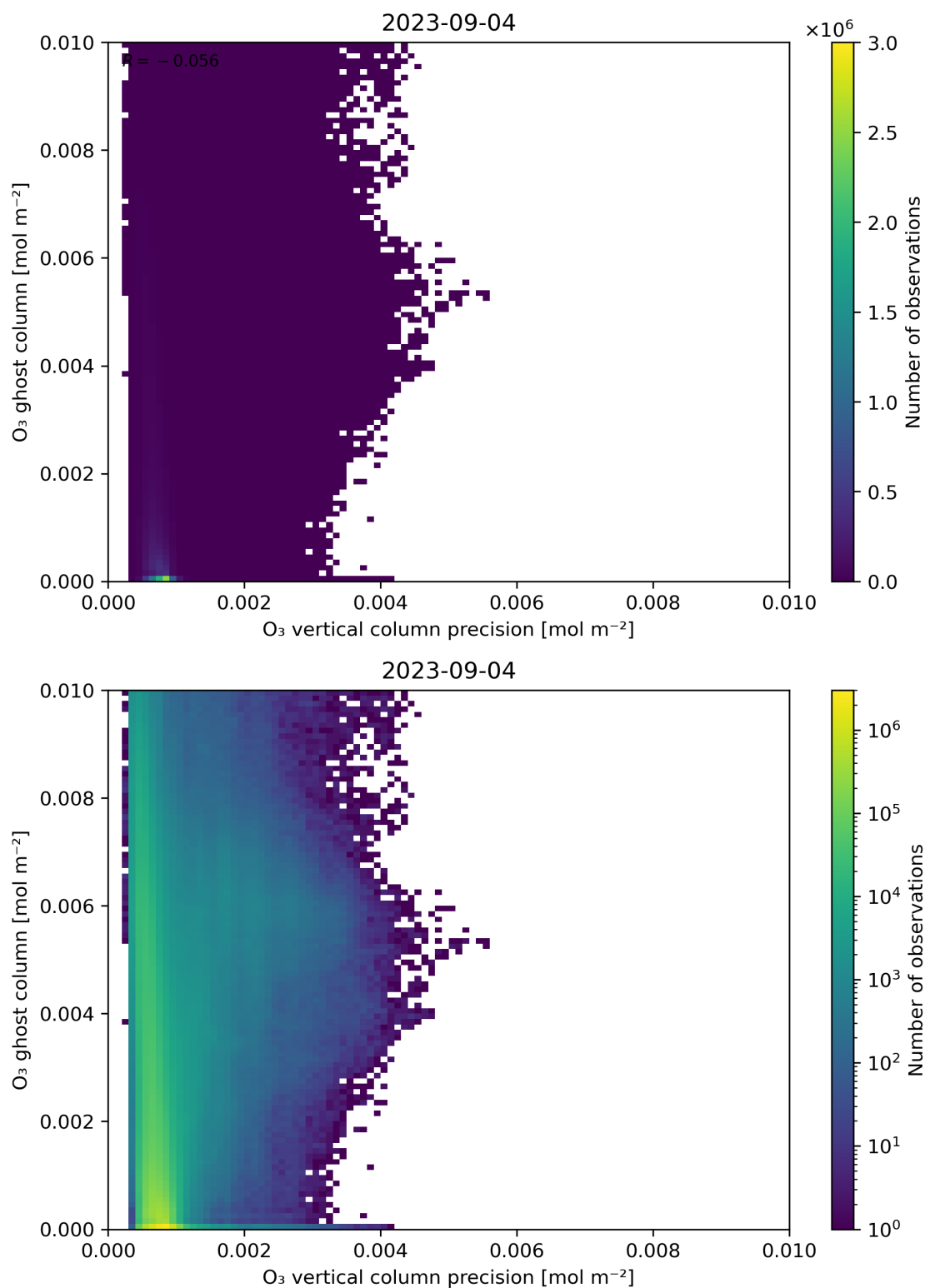
Figure 43: Scatter density plot of “ O_3 vertical column precision” against “ O_3 ghost column” for 2023-09-04 to 2023-09-05.
