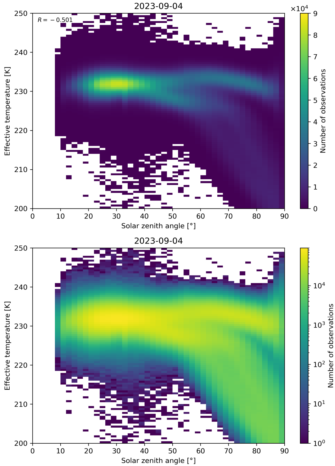
Figure 45: Scatter density plot of “Solar zenith angle” against “Effective temperature” for 2023-09-04 to 2023-09-05.
