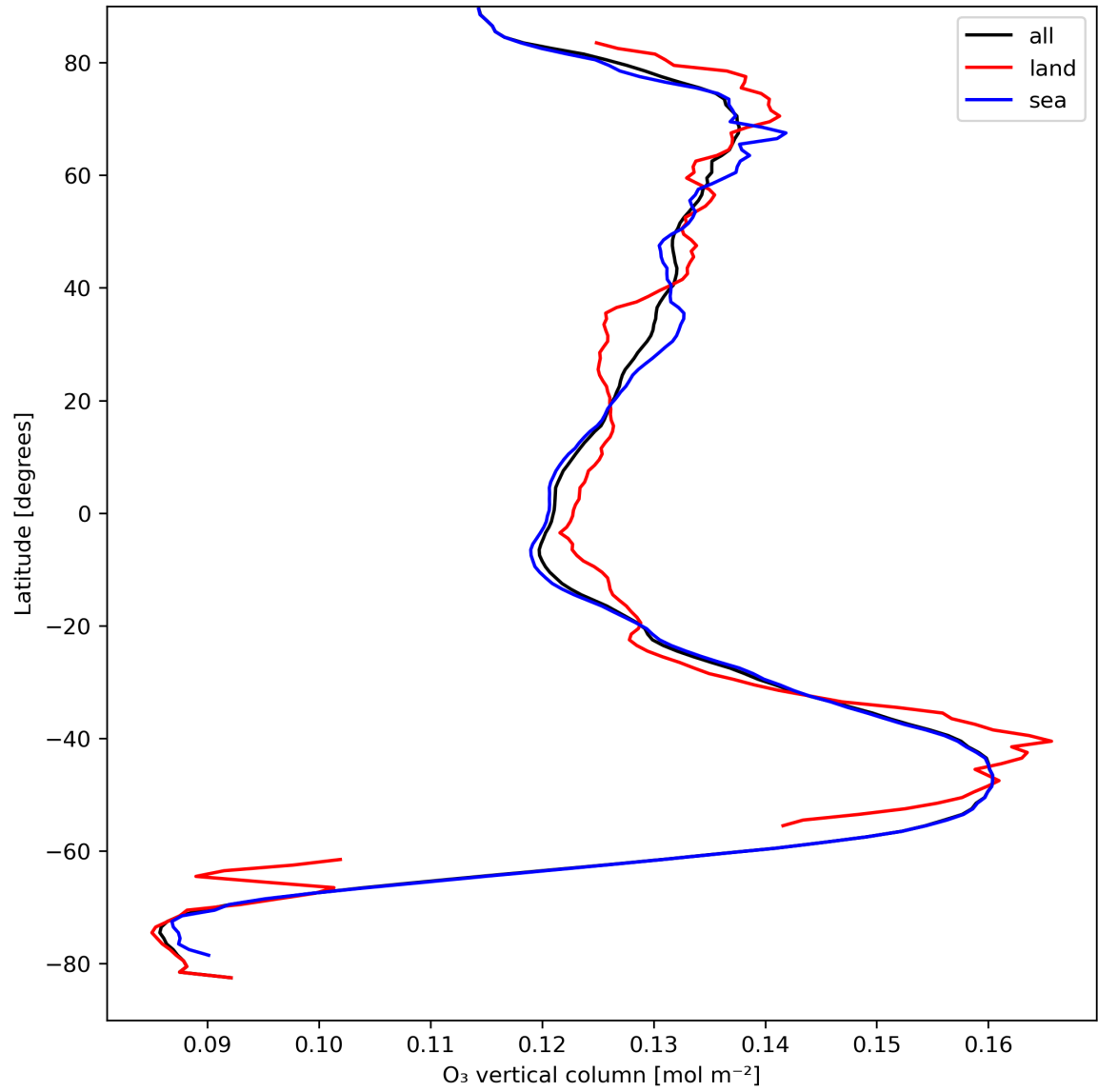
Figure 14: Zonal average of “O 3 vertical column” for 2023-09-04 to 2023-09-05.
