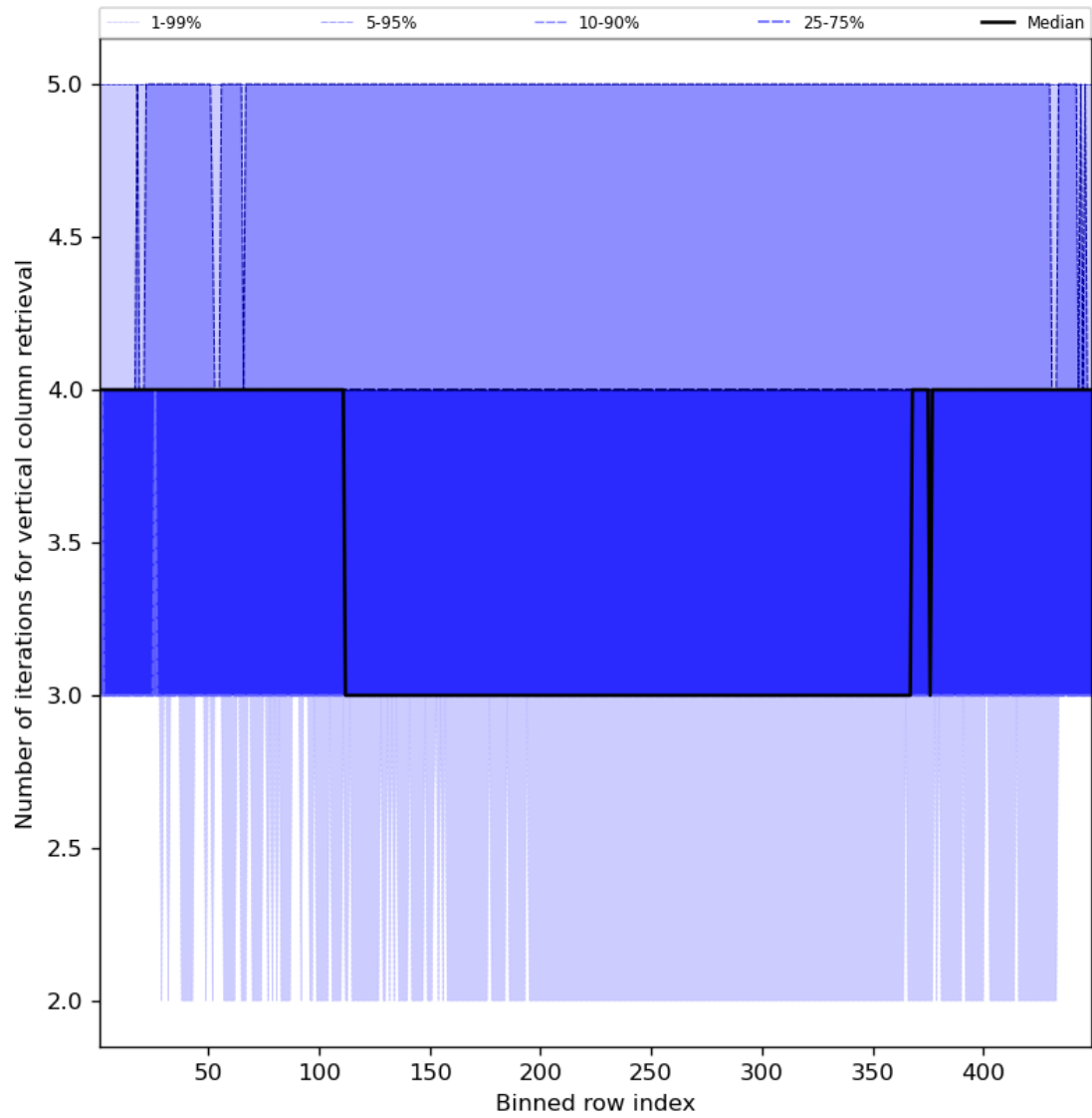
Figure 33: Along track statistics of “Number of iterations for vertical column retrieval” for 2023-09-04 to 2023-09-05
