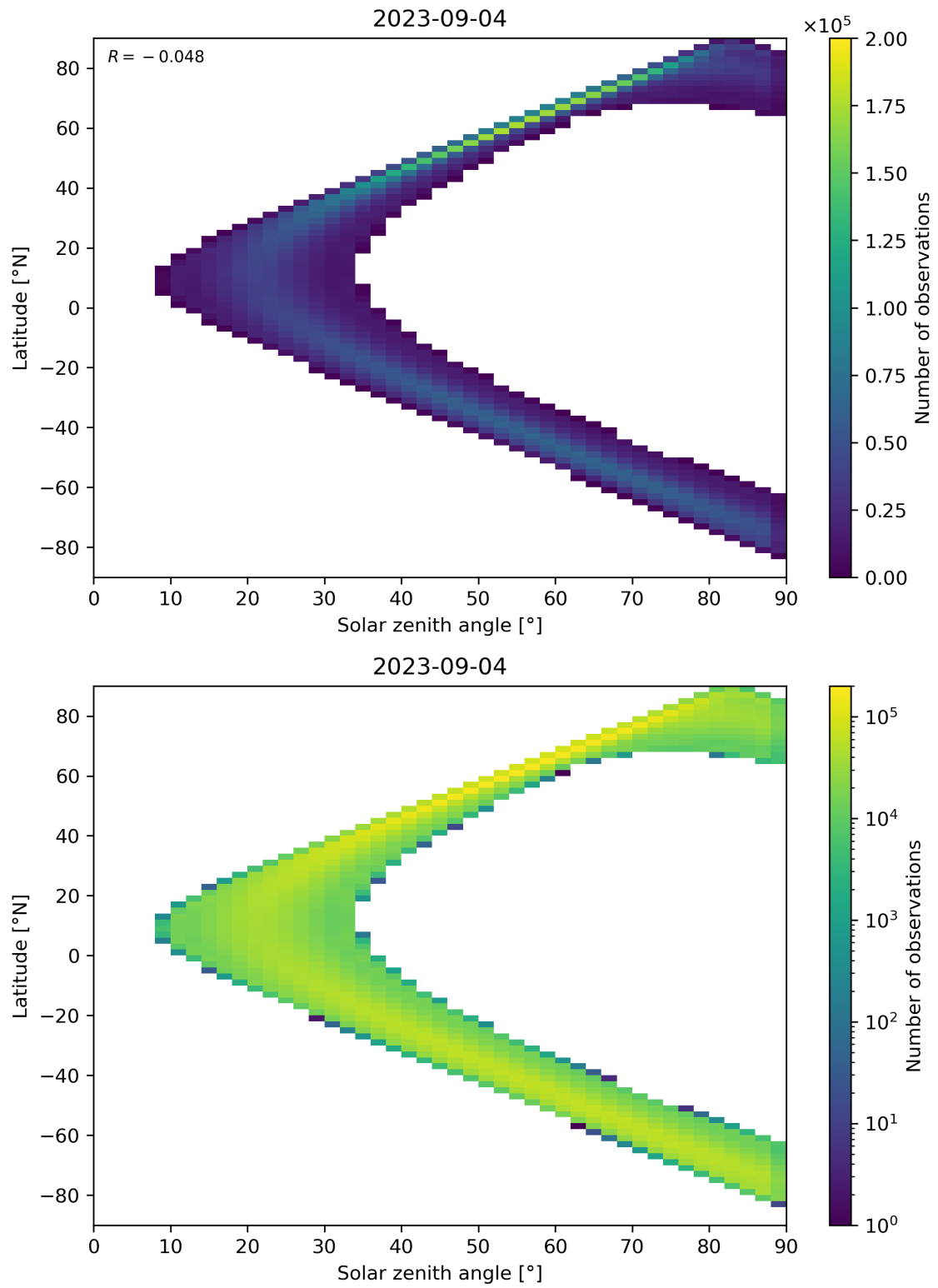
Figure 44: Scatter density plot of “Solar zenith angle” against “Latitude” for 2023-09-04 to 2023-09-05.
