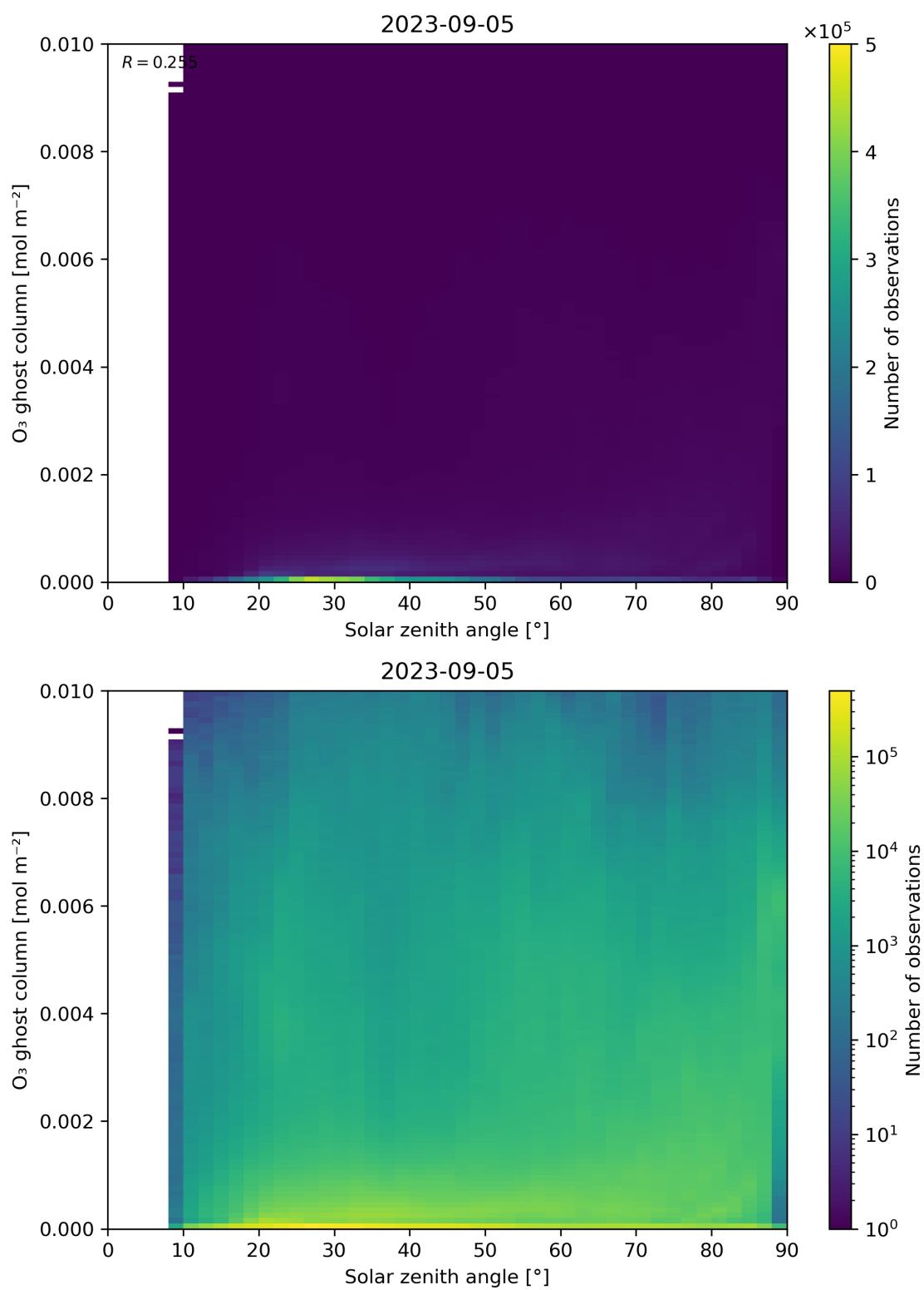
Figure 46: Scatter density plot of “Solar zenith angle” against “O 3 ghost column” for 2023-09-05 to 2023-09-06.
