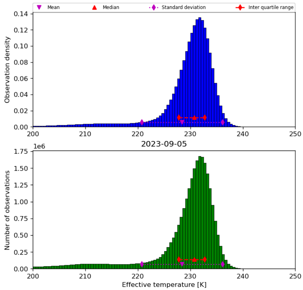
Figure 24: Histogram of “Effective temperature” for 2023-09-05 to 2023-09-06
