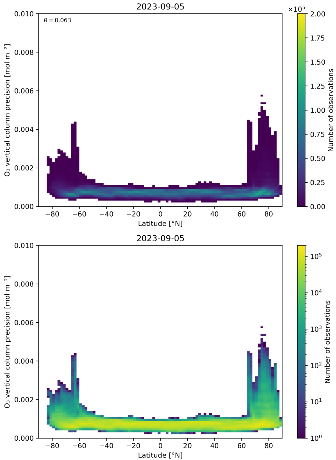
Figure 37: Scatter density plot of “Latitude” against “O 3 vertical column precision” for 2023-09-05 to 2023-09-06.
