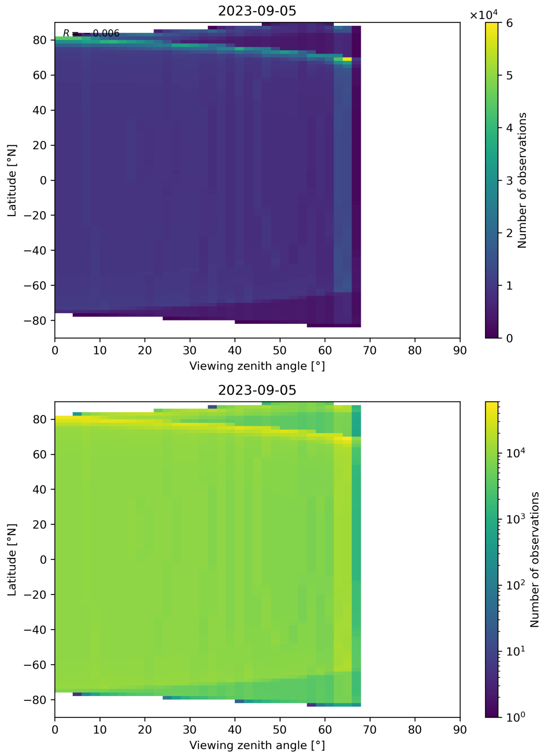
Figure 49: Scatter density plot of “Viewing zenith angle” against “Latitude” for 2023-09-05 to 2023-09-06.
