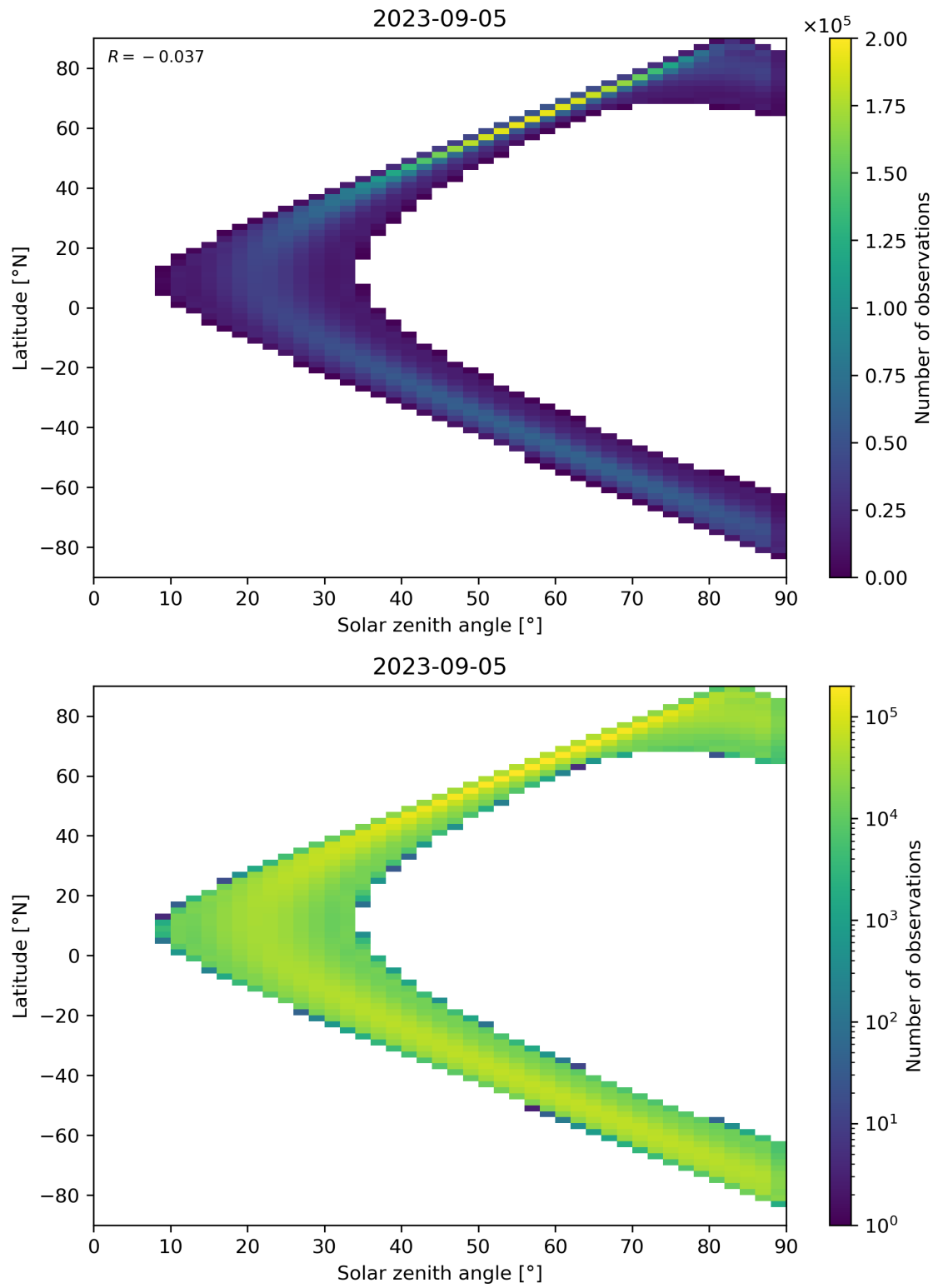
Figure 44: Scatter density plot of “Solar zenith angle” against “Latitude” for 2023-09-05 to 2023-09-06.
