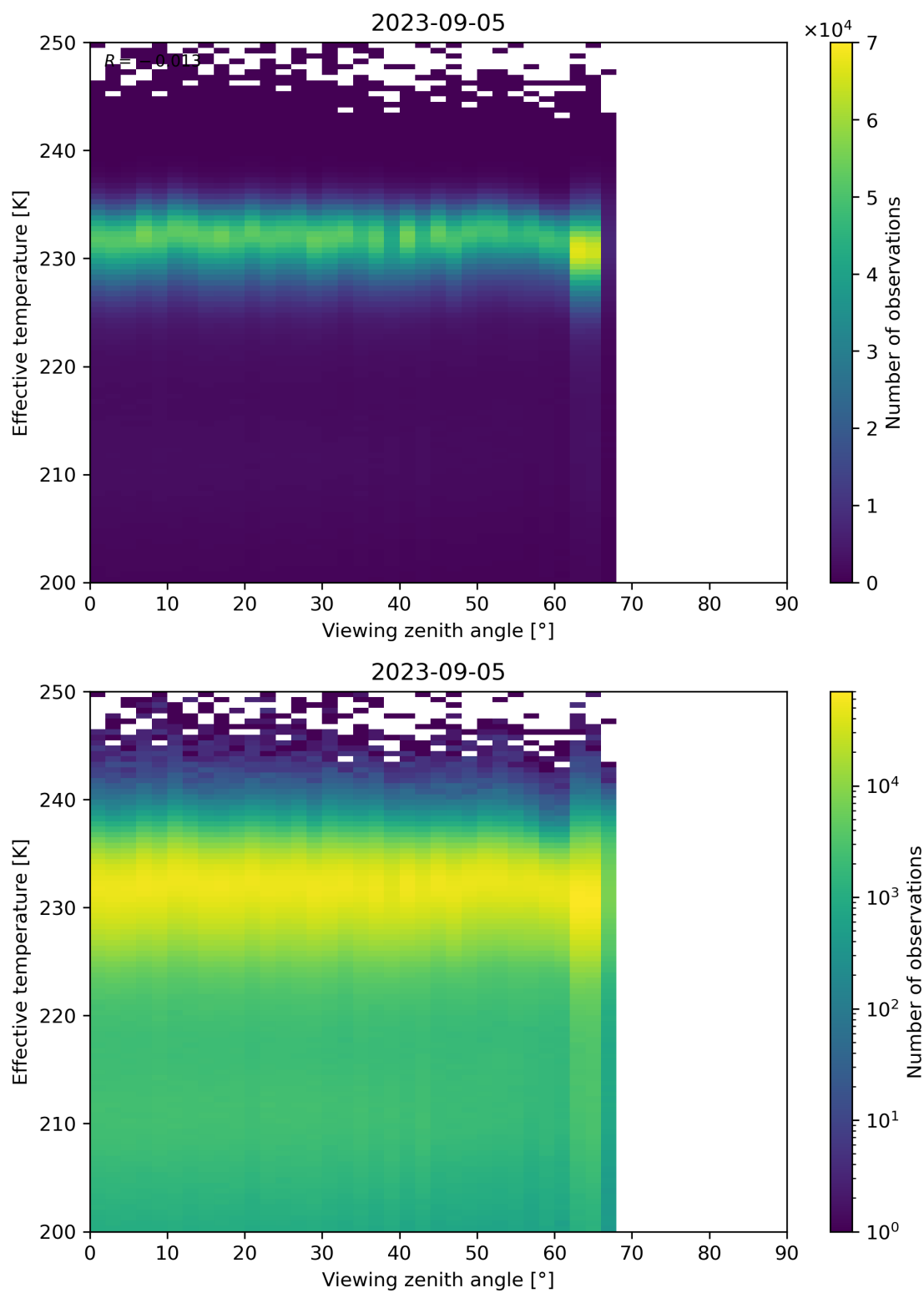
Figure 50: Scatter density plot of “Viewing zenith angle” against “Effective temperature” for 2023-09-05 to 2023-09-06.
