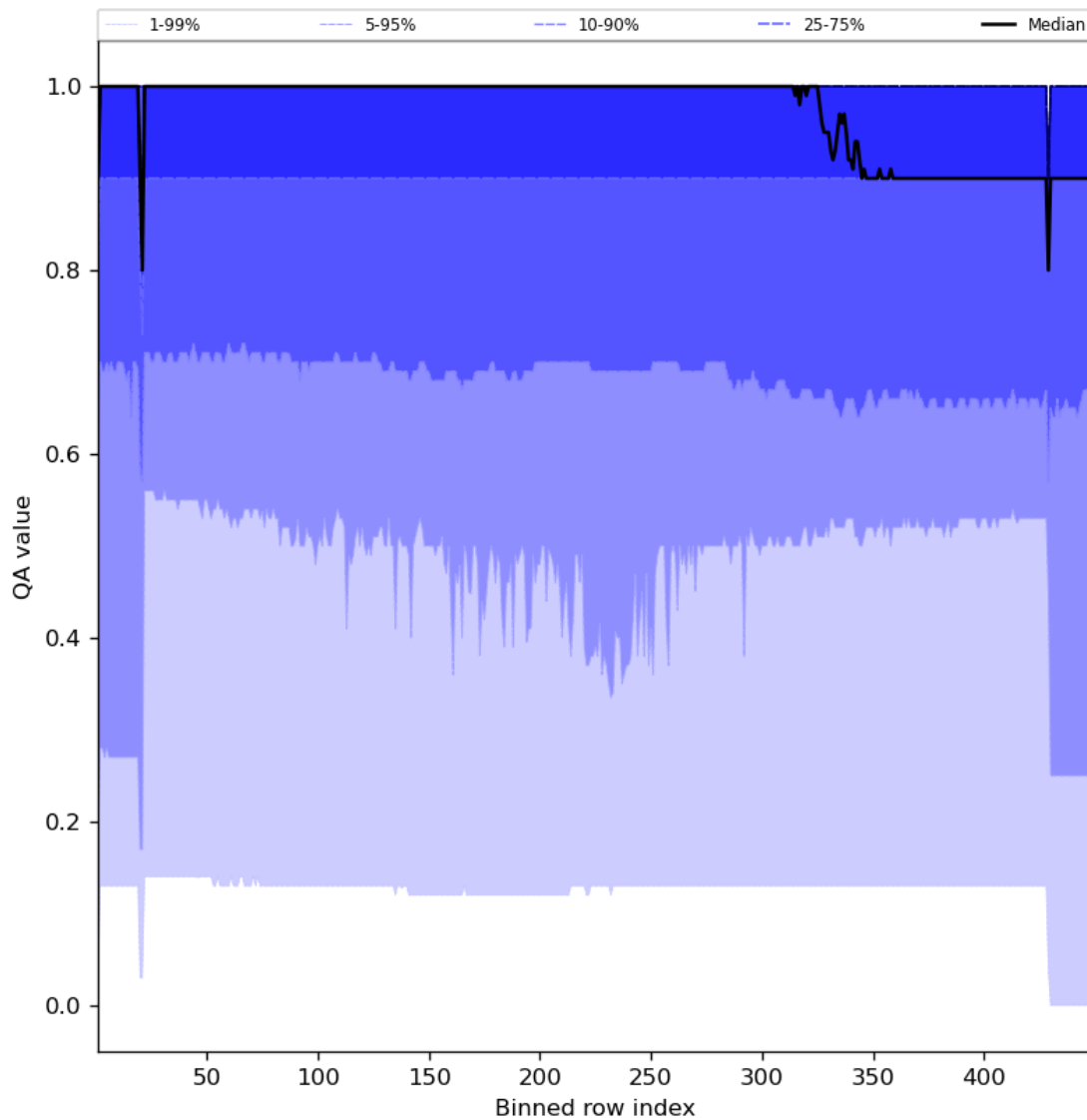
Figure 27: Along track statistics of “QA value” for 2023-09-05 to 2023-09-06
