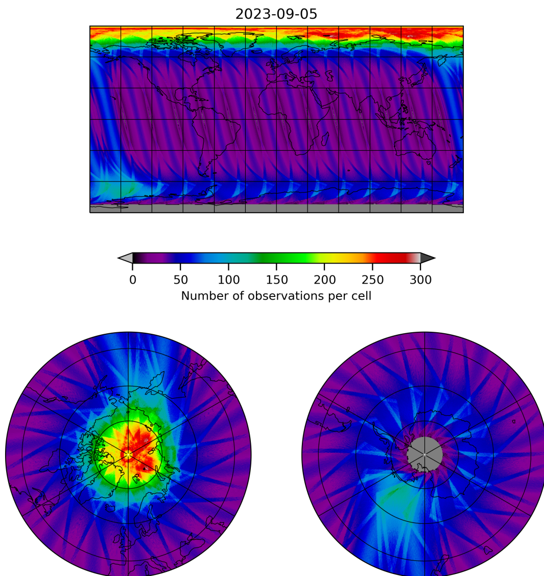
Figure 12: Map of the number of observations for 2023-09-05 to 2023-09-06
