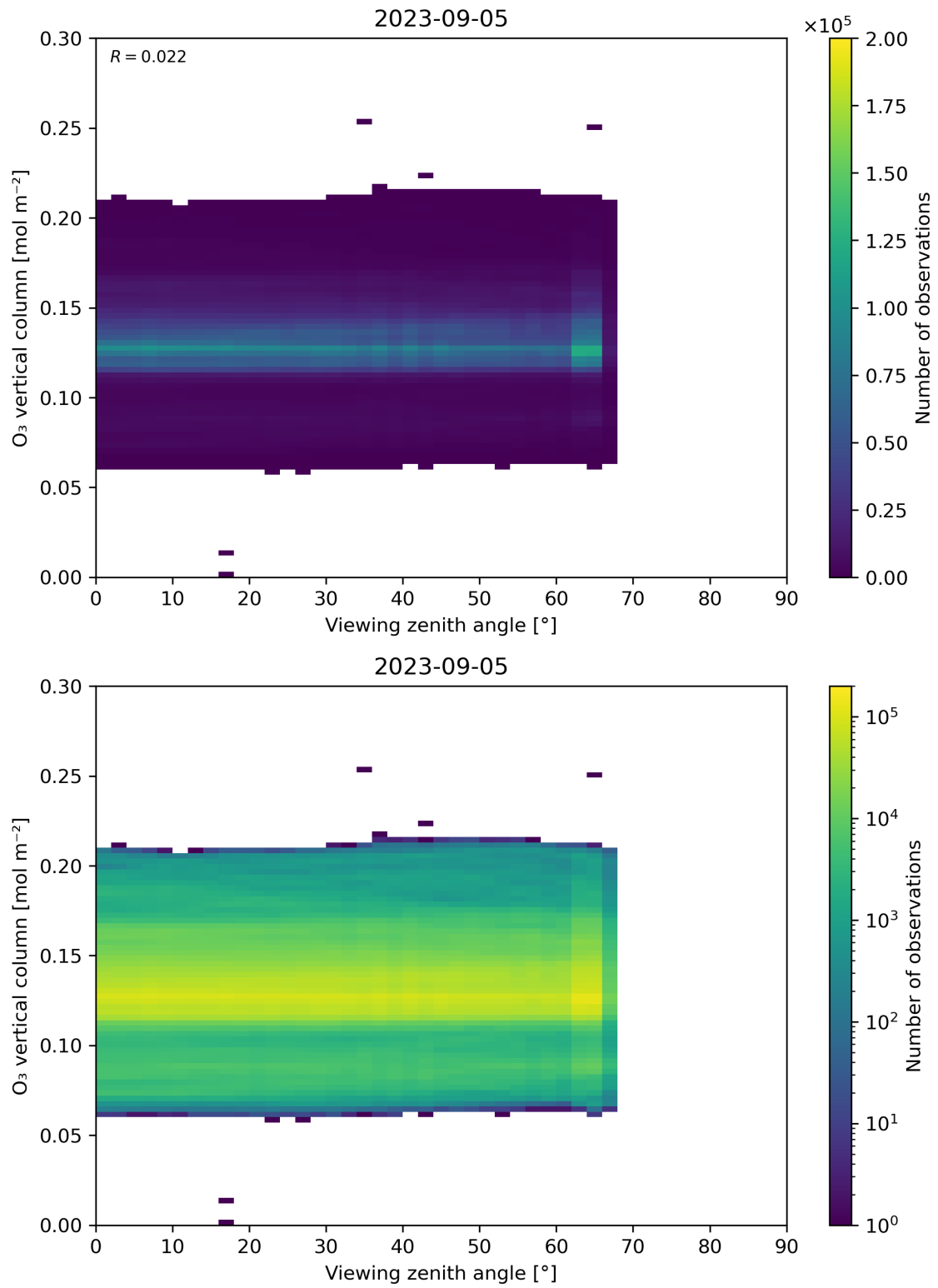
Figure 52: Scatter density plot of “Viewing zenith angle” against “O 3 vertical column” for 2023-09-05 to 2023-09-06.
