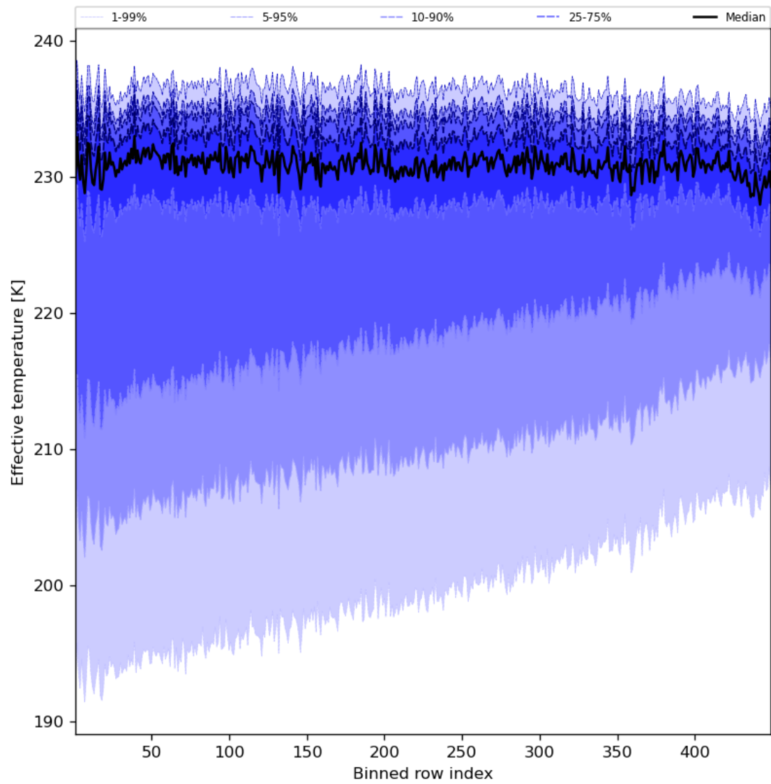
Figure 31: Along track statistics of “Effective temperature” for 2023-09-05 to 2023-09-06
