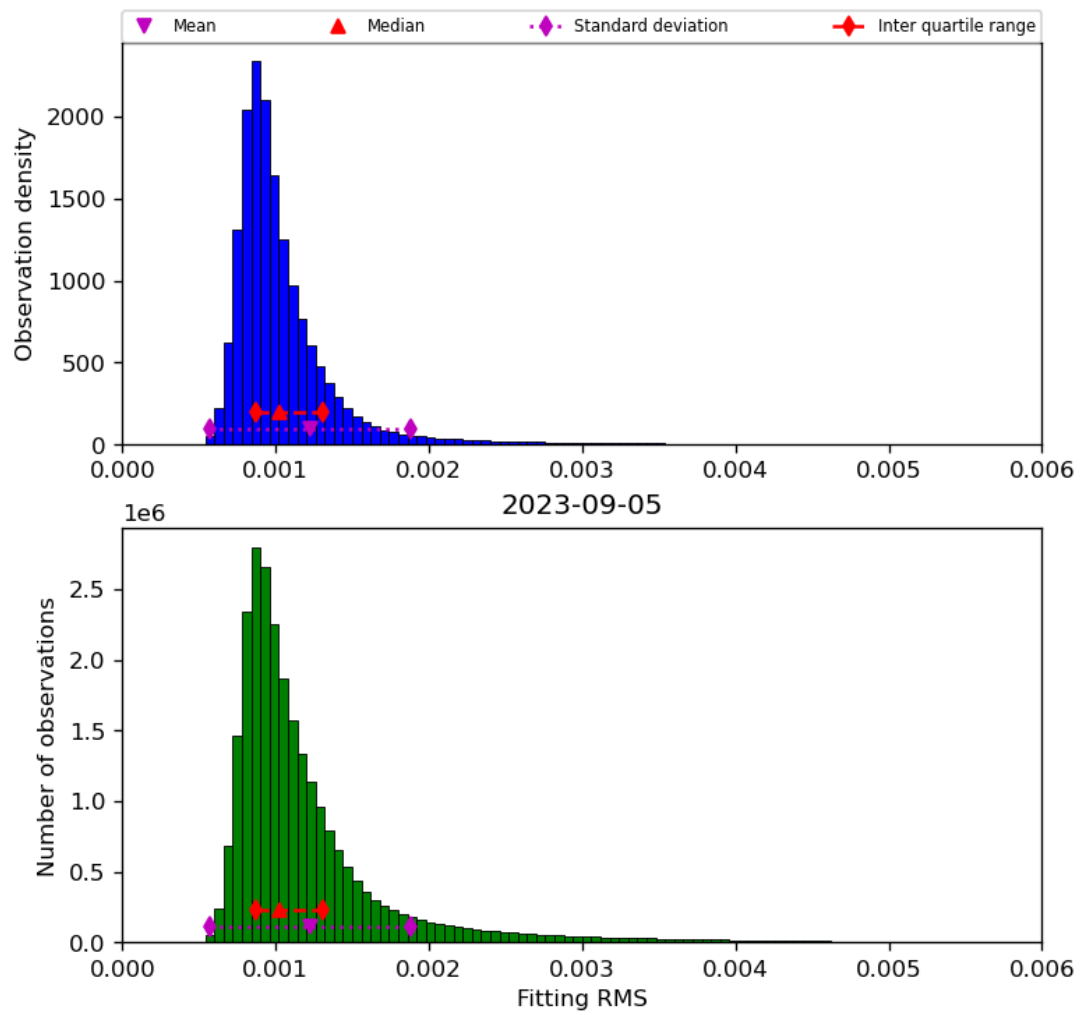
Figure 23: Histogram of “Fitting RMS” for 2023-09-05 to 2023-09-06
