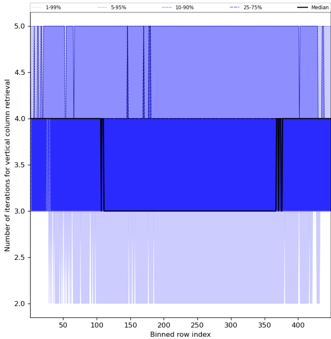
Figure 33: Along track statistics of “Number of iterations for vertical column retrieval” for 2023-09-05 to 2023-09-06
