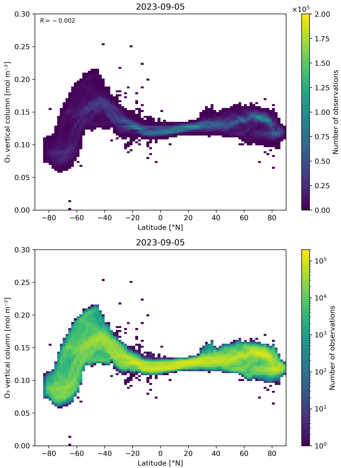
Figure 36: Scatter density plot of “Latitude” against “O 3 vertical column” for 2023-09-05 to 2023-09-06.
