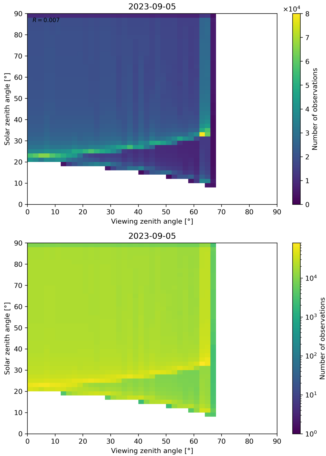
Figure 54: Scatter density plot of “Viewing zenith angle” against “Solar zenith angle” for 2023-09-05 to 2023-09-06.
