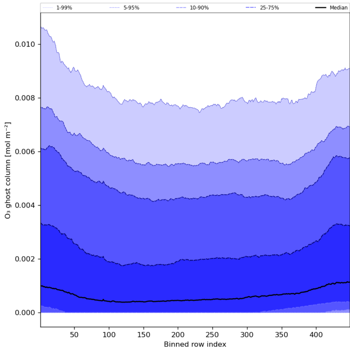
Figure 32: Along track statistics of “O 3 ghost column” for 2023-09-05 to 2023-09-06
