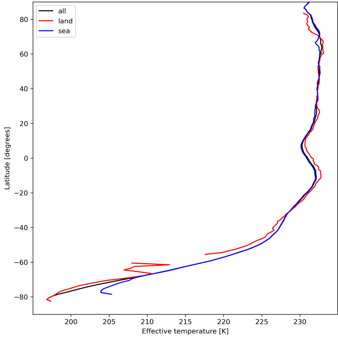
Figure 17: Zonal average of "Effective temperature" for 2023-09-05 to 2023-09-06.
