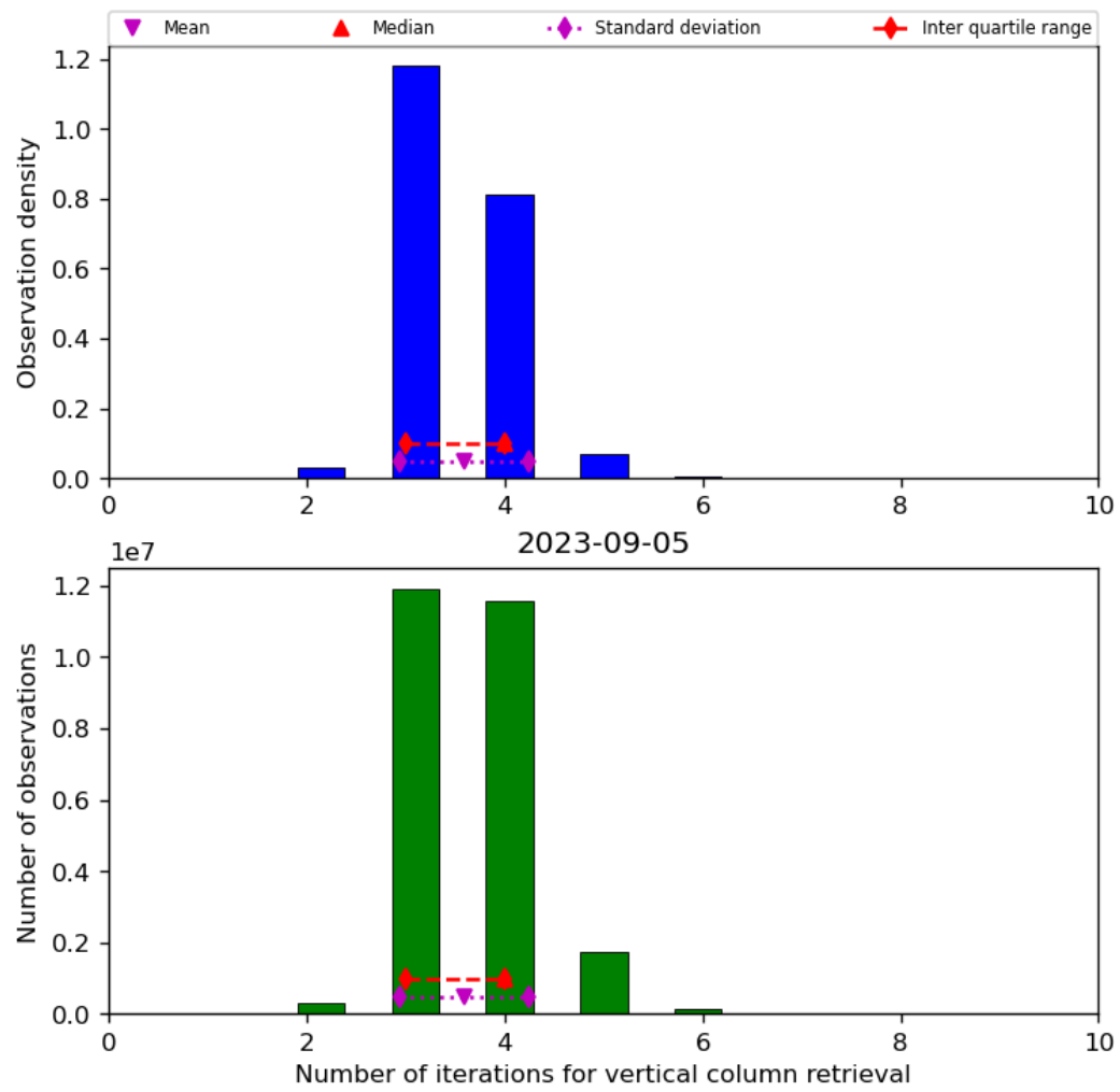
Figure 26: Histogram of “Number of iterations for vertical column retrieval” for 2023-09-05 to 2023-09-06
