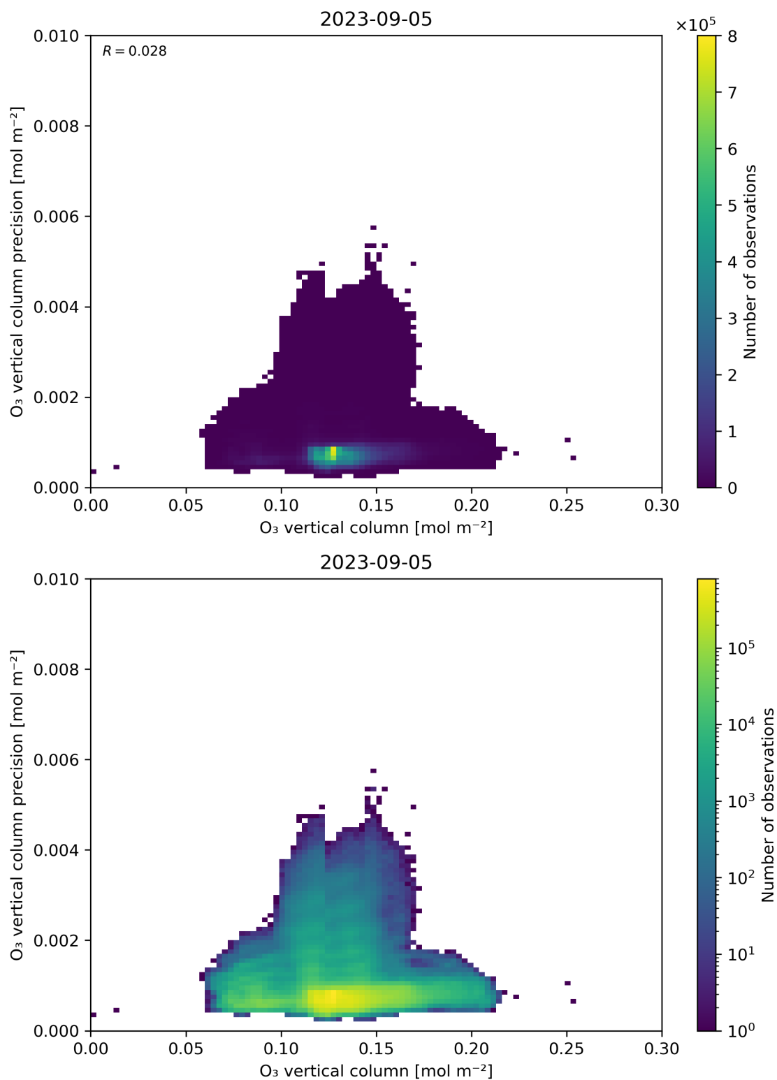
Figure 41: Scatter density plot of “O 3 vertical column” against “O 3 vertical column precision” for 2023-09-05 to 2023-09-06.
