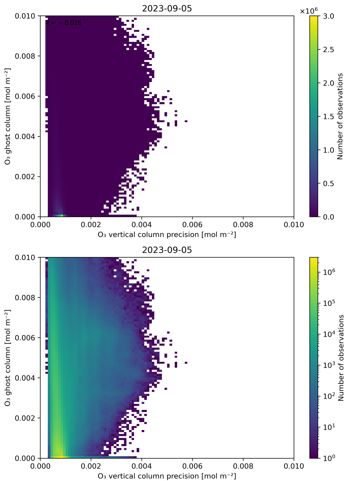
Figure 43: Scatter density plot of “O 3 vertical column precision” against “O 3 ghost column” for 2023-09-05 to 2023-09-06.
