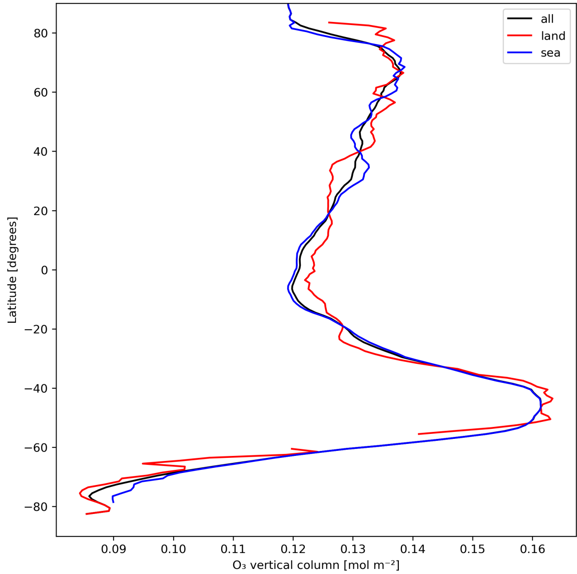
Figure 14: Zonal average of “O 3 vertical column” for 2023-09-05 to 2023-09-06.
