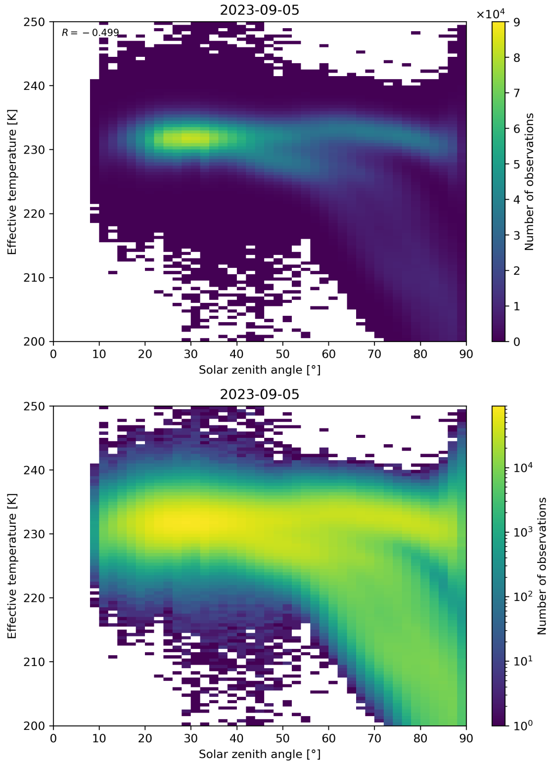
Figure 45: Scatter density plot of “Solar zenith angle” against “Effective temperature” for 2023-09-05 to 2023-09-06.
