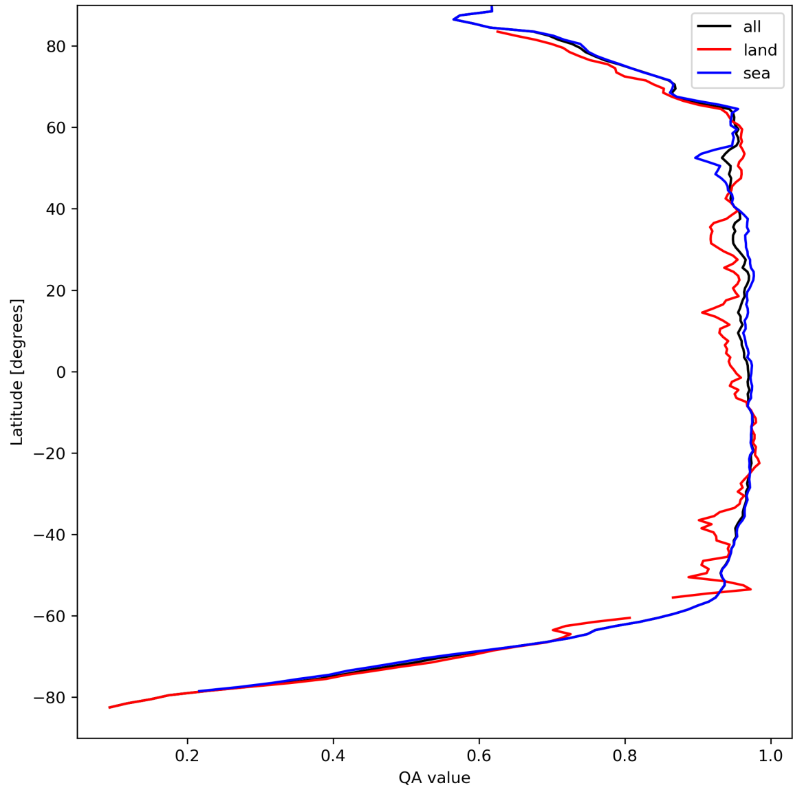
Figure 13: Zonal average of “QA value” for 2023-09-05 to 2023-09-06.
