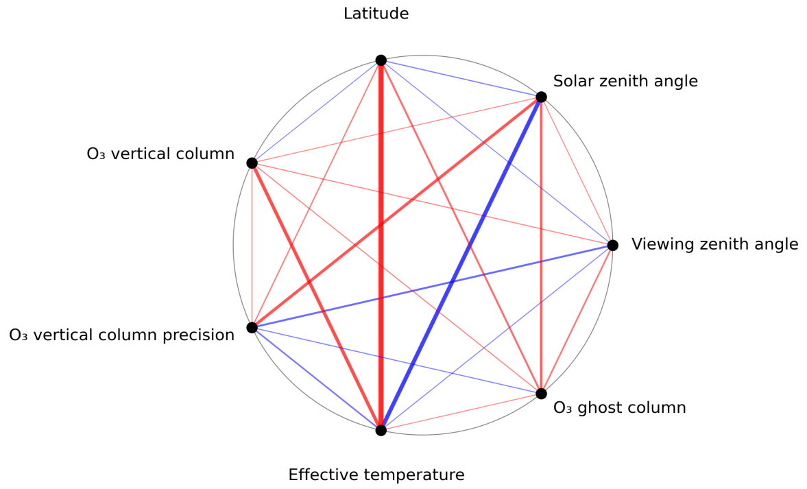
Figure 1: Map of correlation graph for 2023-09-05 to 2023-09-06.
