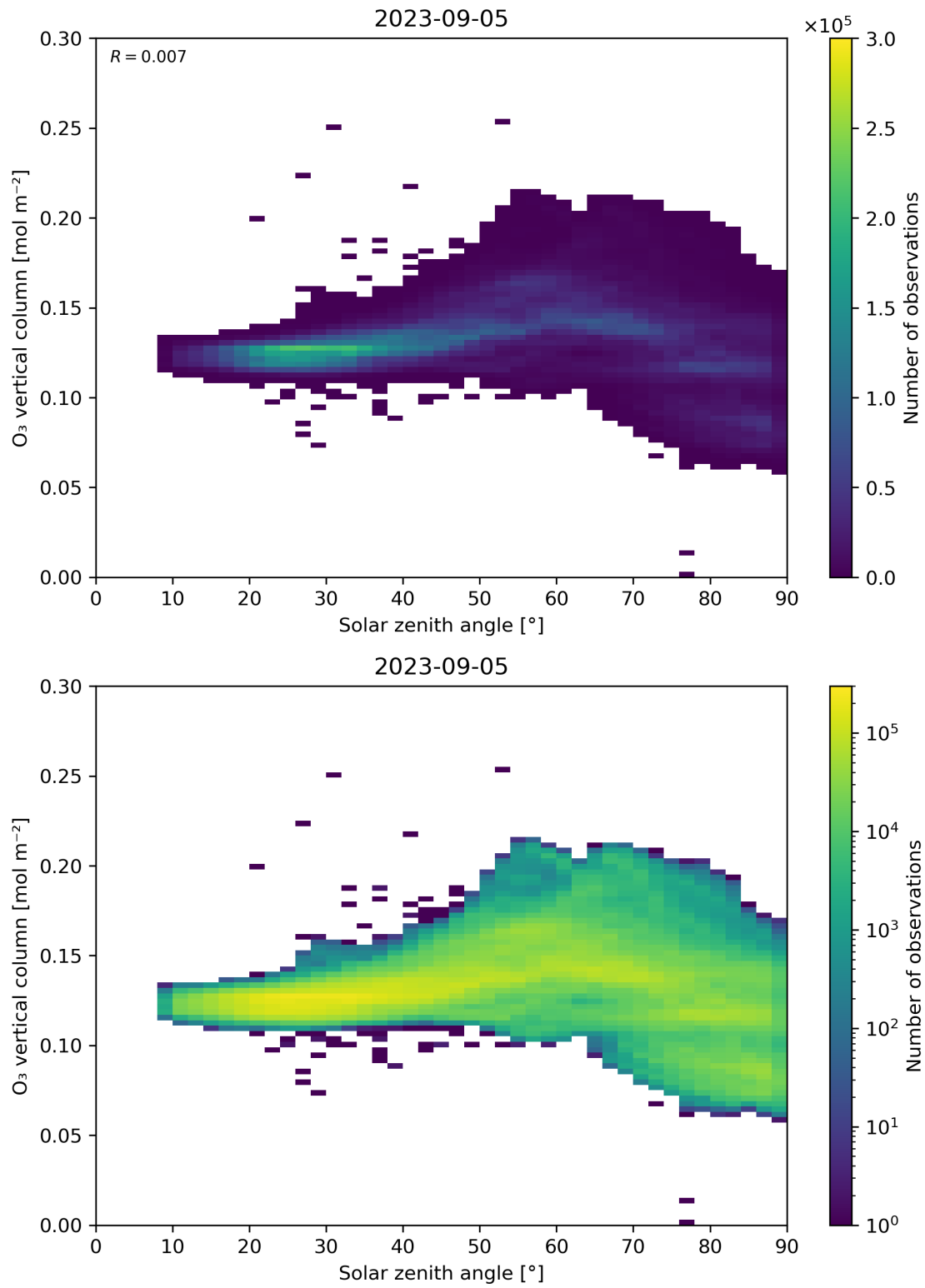
Figure 47: Scatter density plot of “Solar zenith angle” against “O 3 vertical column” for 2023-09-05 to 2023-09-06.
