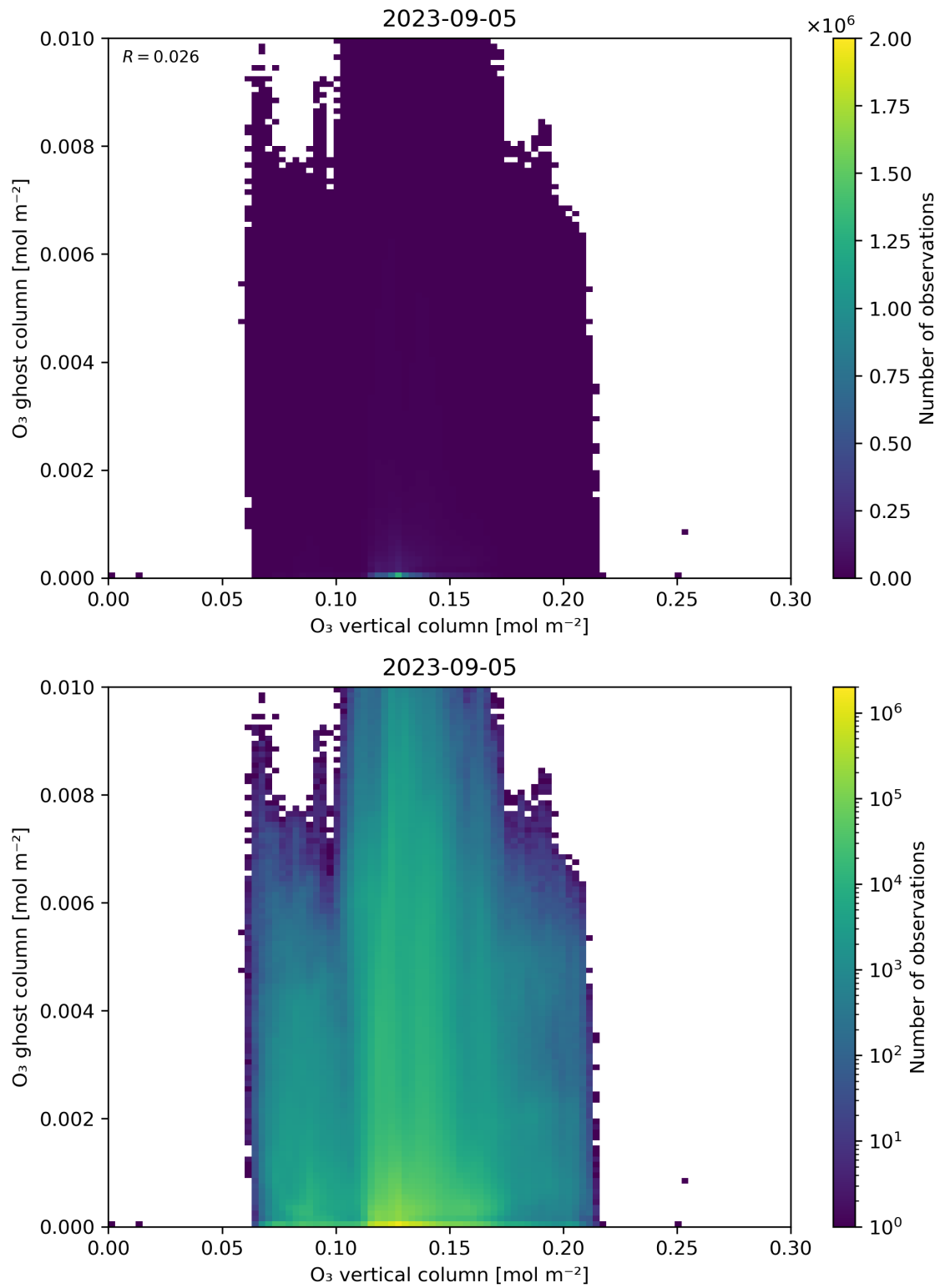
Figure 40: Scatter density plot of “O 3 vertical column” against “O 3 ghost column” for 2023-09-05 to 2023-09-06.
