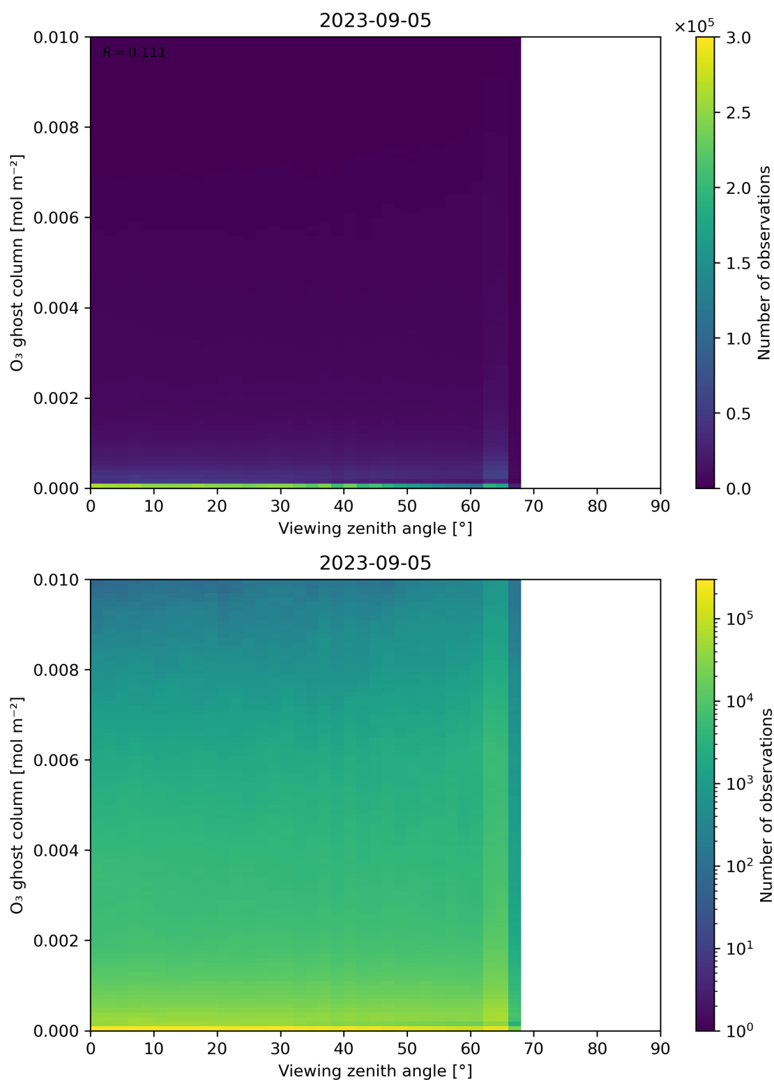
Figure 51: Scatter density plot of “Viewing zenith angle” against “O 3 ghost column” for 2023-09-05 to 2023-09-06.
