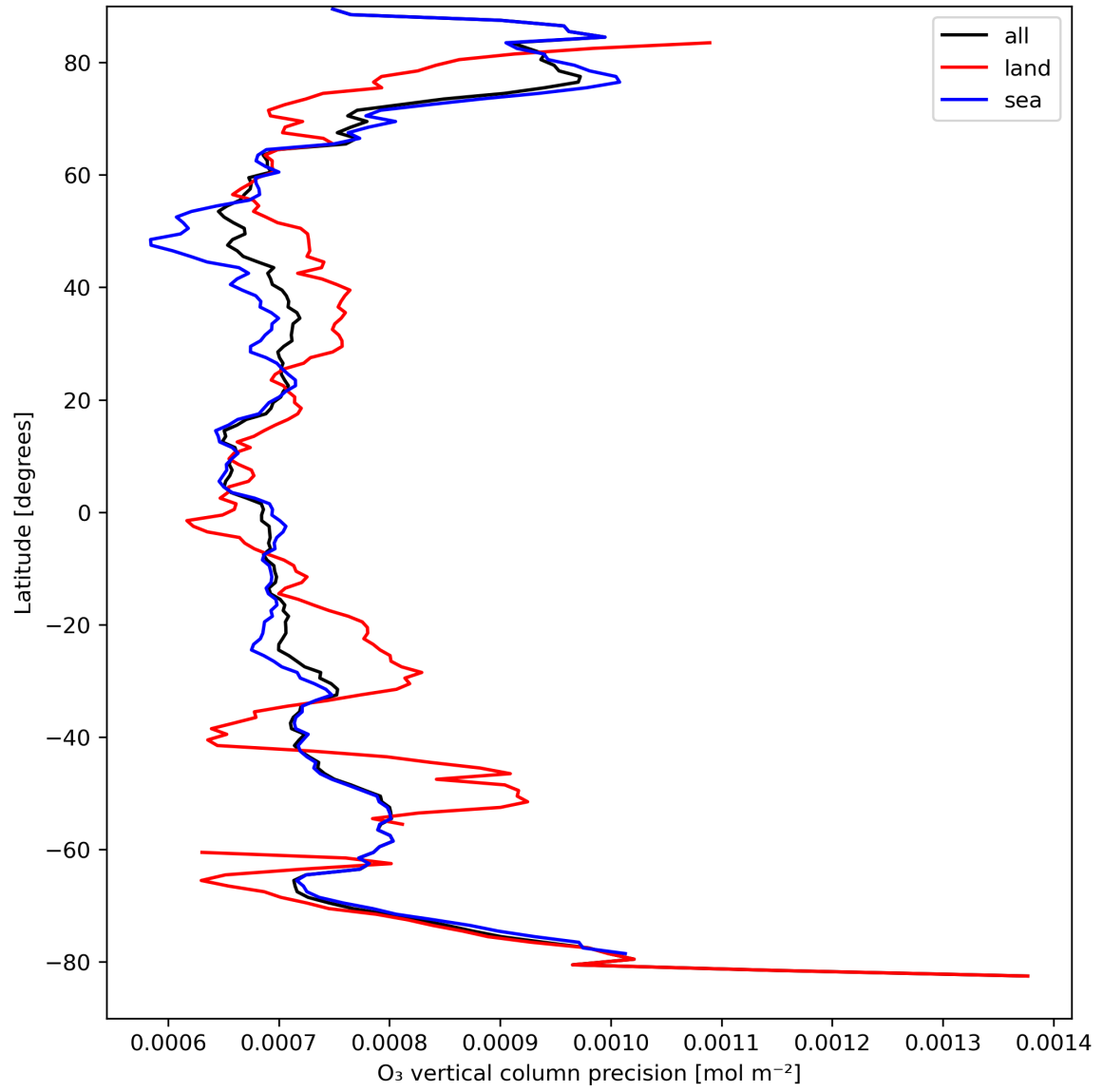
Figure 15: Zonal average of “O 3 vertical column precision” for 2023-09-05 to 2023-09-06.
