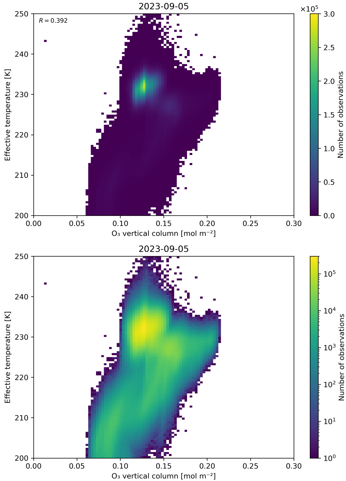
Figure 39: Scatter density plot of “O 3 vertical column” against “Effective temperature” for 2023-09-05 to 2023-09-06.
