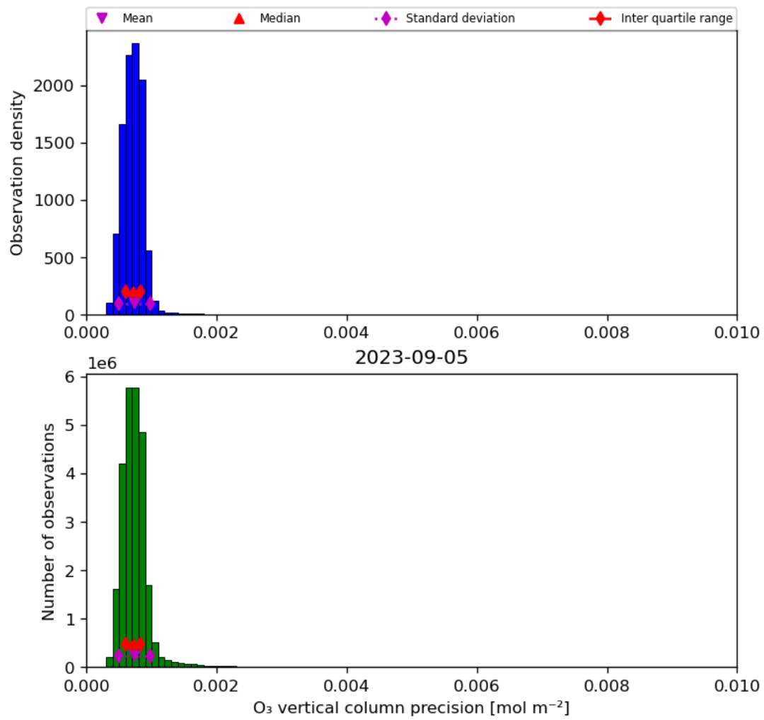
Figure 22: Histogram of “O 3 vertical column precision” for 2023-09-05 to 2023-09-06
