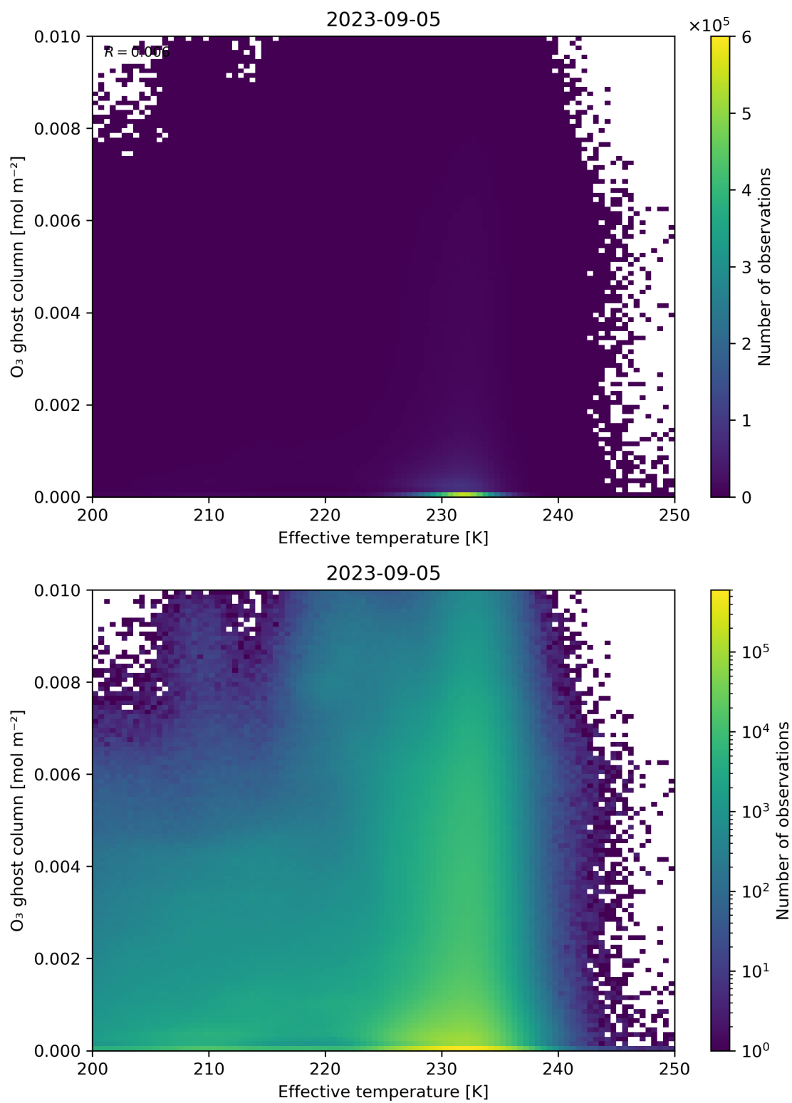
Figure 38: Scatter density plot of “Effective temperature” against “O 3 ghost column” for 2023-09-05 to 2023-09-06.
