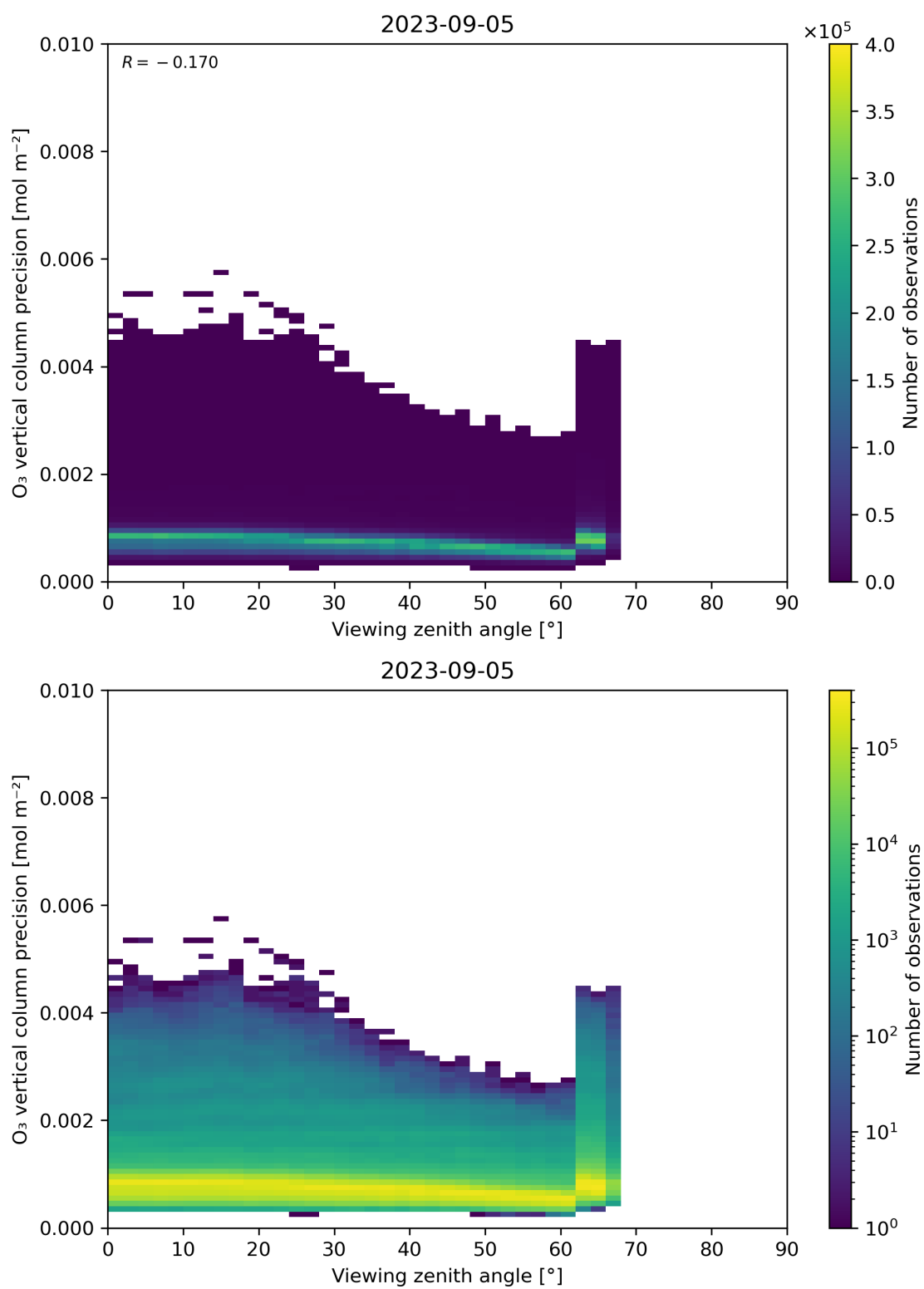
Figure 53: Scatter density plot of “Viewing zenith angle” against “O 3 vertical column precision” for 2023-09-05 to 2023-09-06.
