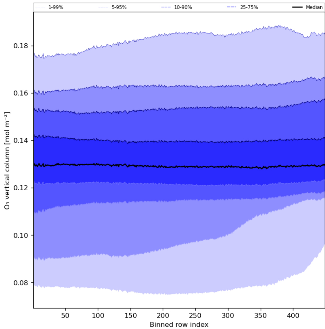
Figure 28: Along track statistics of “O 3 vertical column” for 2023-09-05 to 2023-09-06
