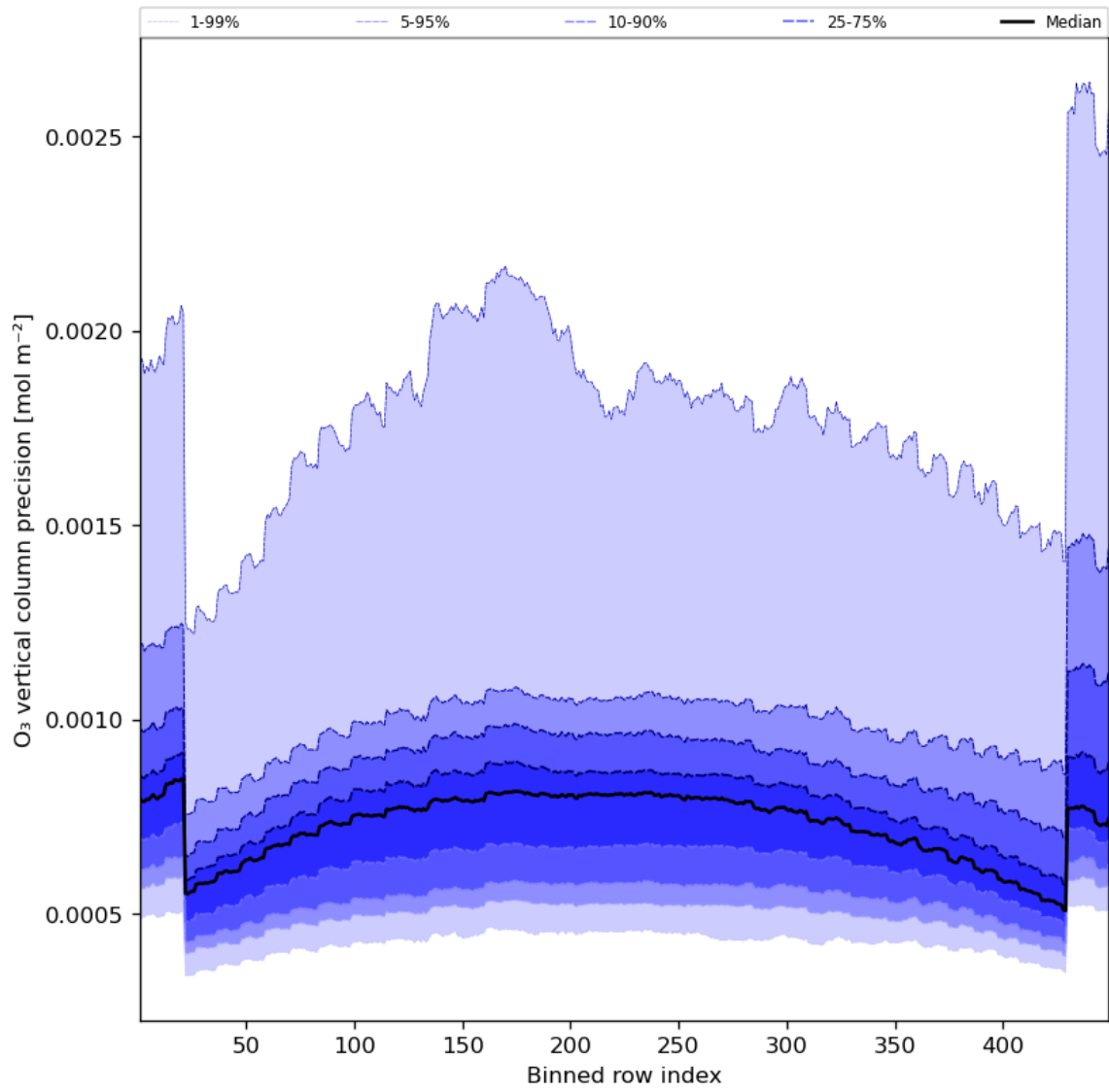
Figure 29: Along track statistics of “O 3 vertical column precision” for 2023-09-05 to 2023-09-06
