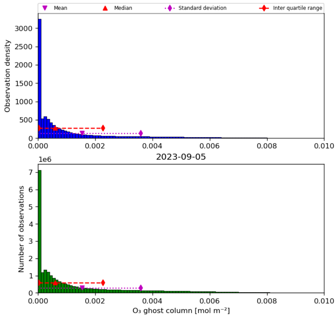
Figure 25: Histogram of “O 3 ghost column” for 2023-09-05 to 2023-09-06
