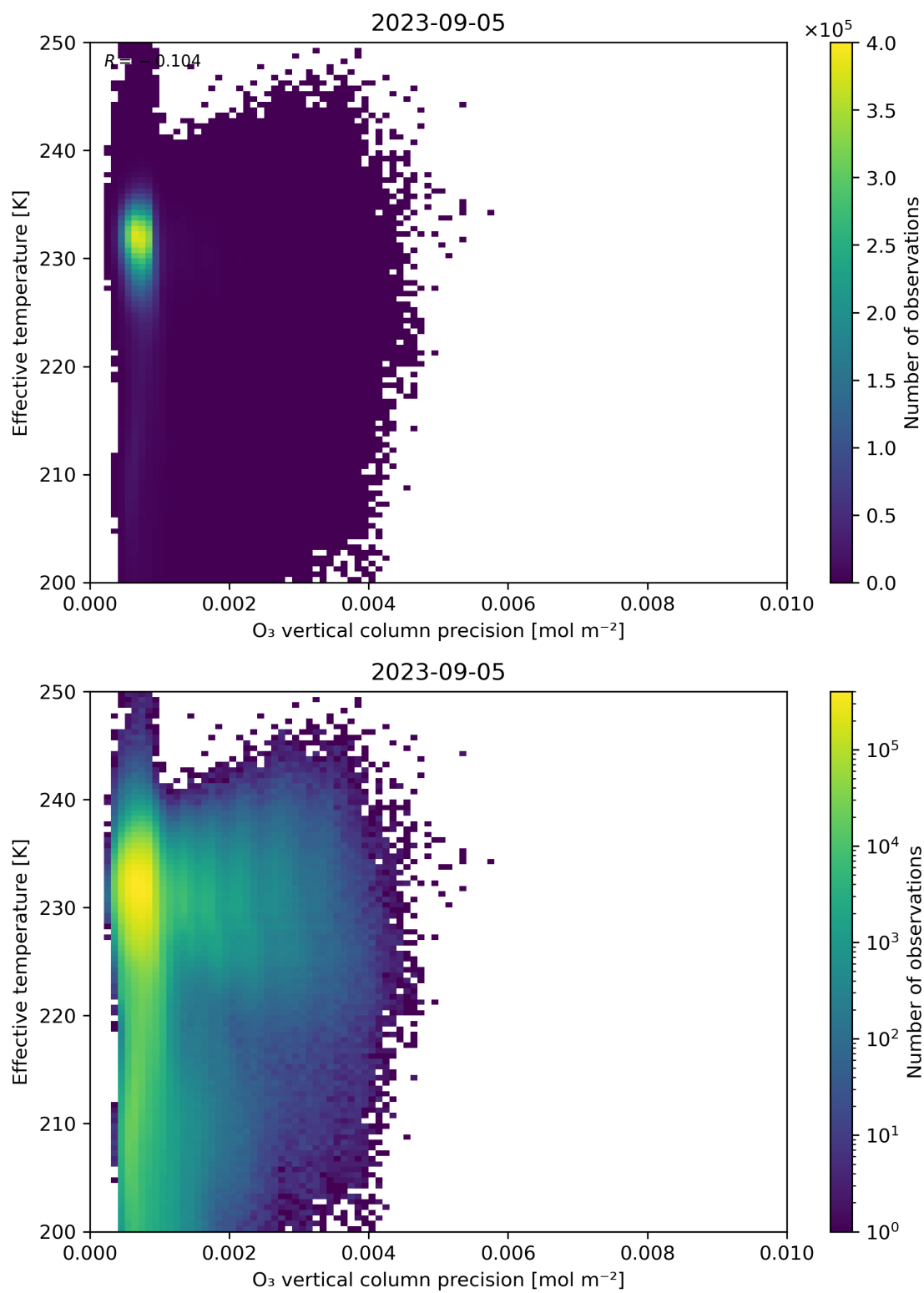
Figure 42: Scatter density plot of “O 3 vertical column precision” against “Effective temperature” for 2023-09-05 to 2023-09-06.
