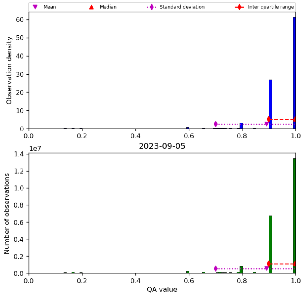
Figure 20: Histogram of “QA value” for 2023-09-05 to 2023-09-06
