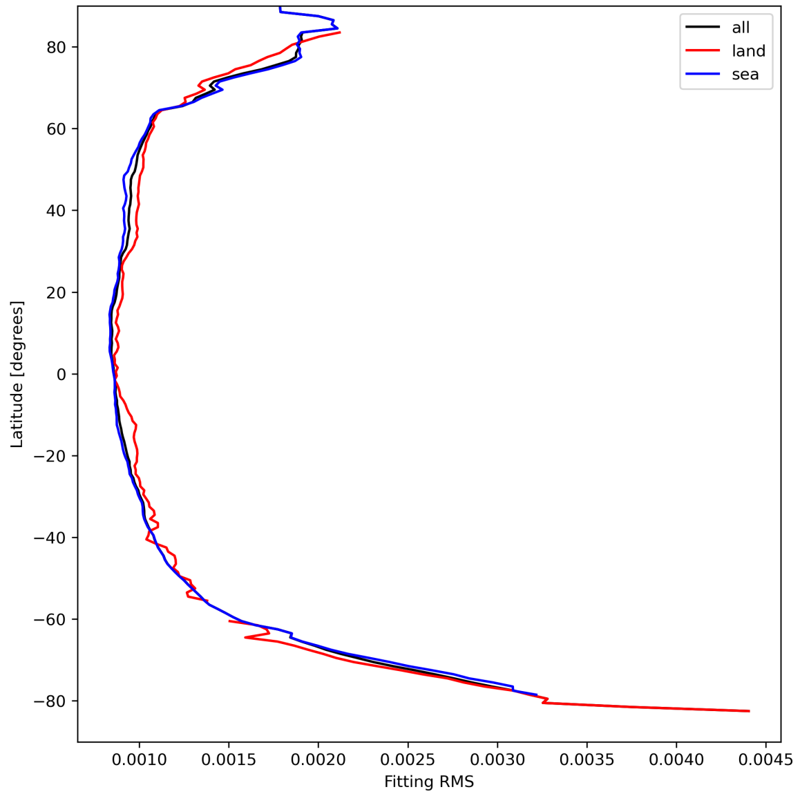
Figure 16: Zonal average of “Fitting RMS” for 2023-09-05 to 2023-09-06.
