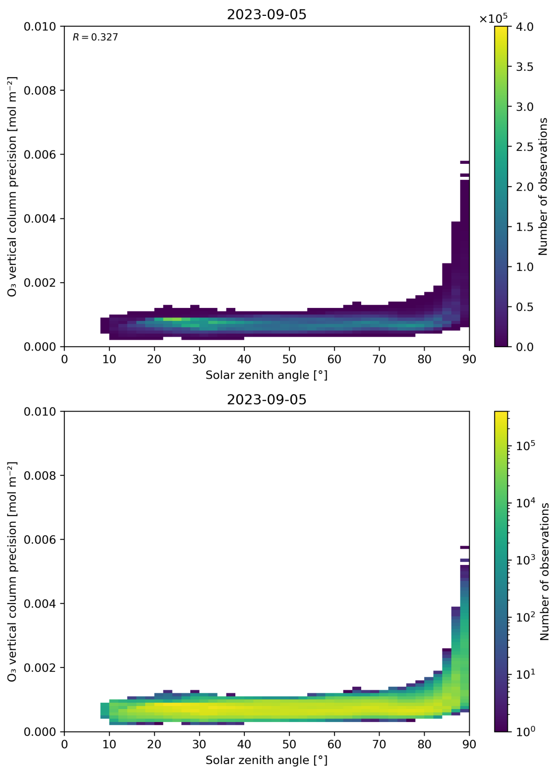
Figure 48: Scatter density plot of “Solar zenith angle” against “O 3 vertical column precision” for 2023-09-05 to 2023-09-06.
