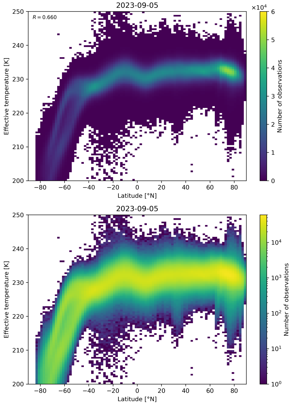
Figure 34: Scatter density plot of “Latitude” against “Effective temperature” for 2023-09-05 to 2023-09-06.
