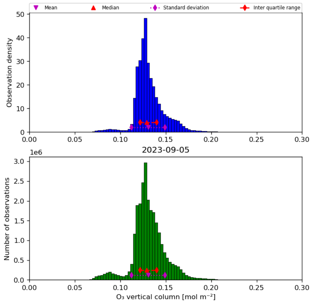
Figure 21: Histogram of “O 3 vertical column” for 2023-09-05 to 2023-09-06
