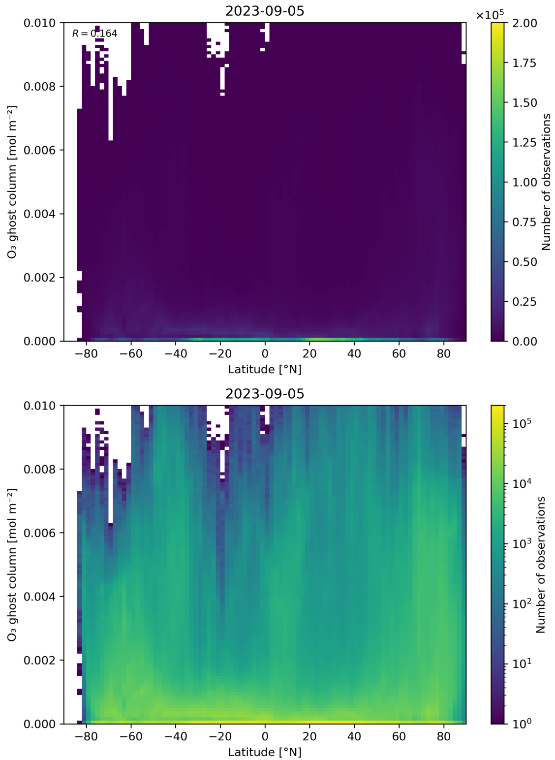
Figure 35: Scatter density plot of “Latitude” against “O 3 ghost column” for 2023-09-05 to 2023-09-06.
