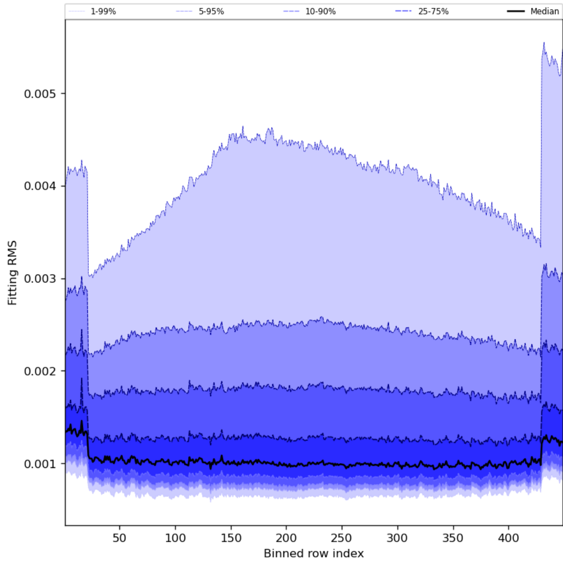
Figure 30: Along track statistics of “Fitting RMS” for 2023-09-05 to 2023-09-06
