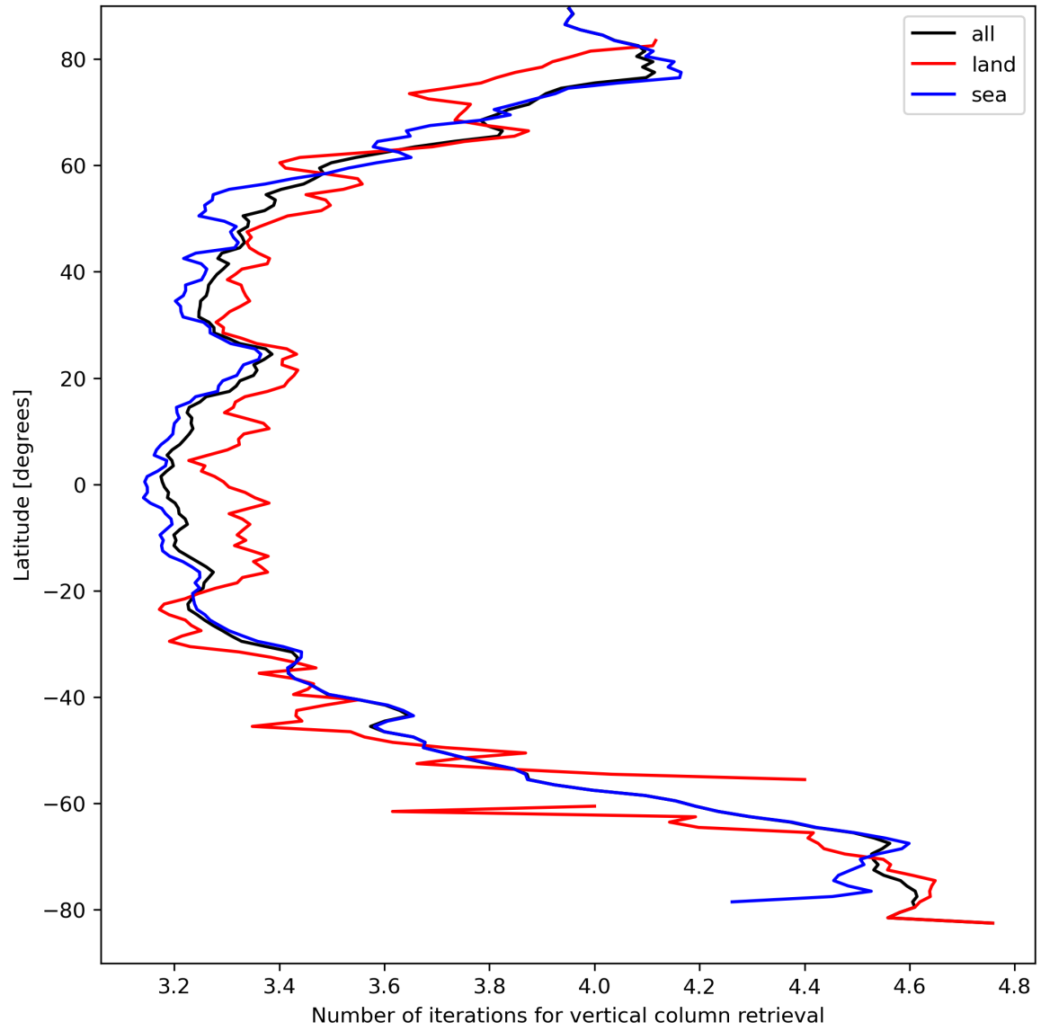
Figure 19: Zonal average of “Number of iterations for vertical column retrieval” for 2023-09-05 to 2023-09-06.
