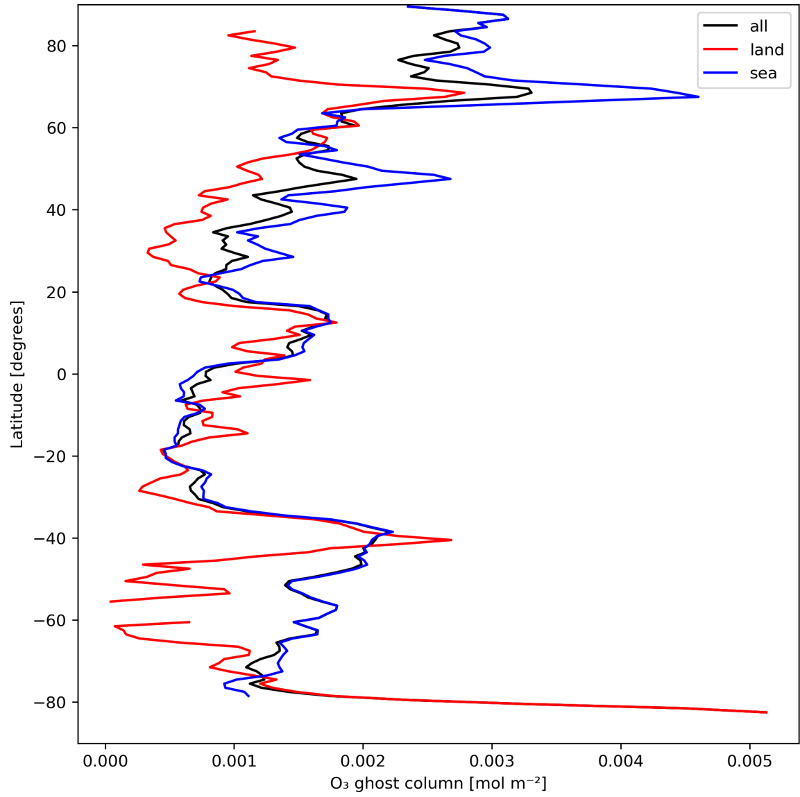
Figure 18: Zonal average of “O 3 ghost column” for 2023-09-05 to 2023-09-06.
