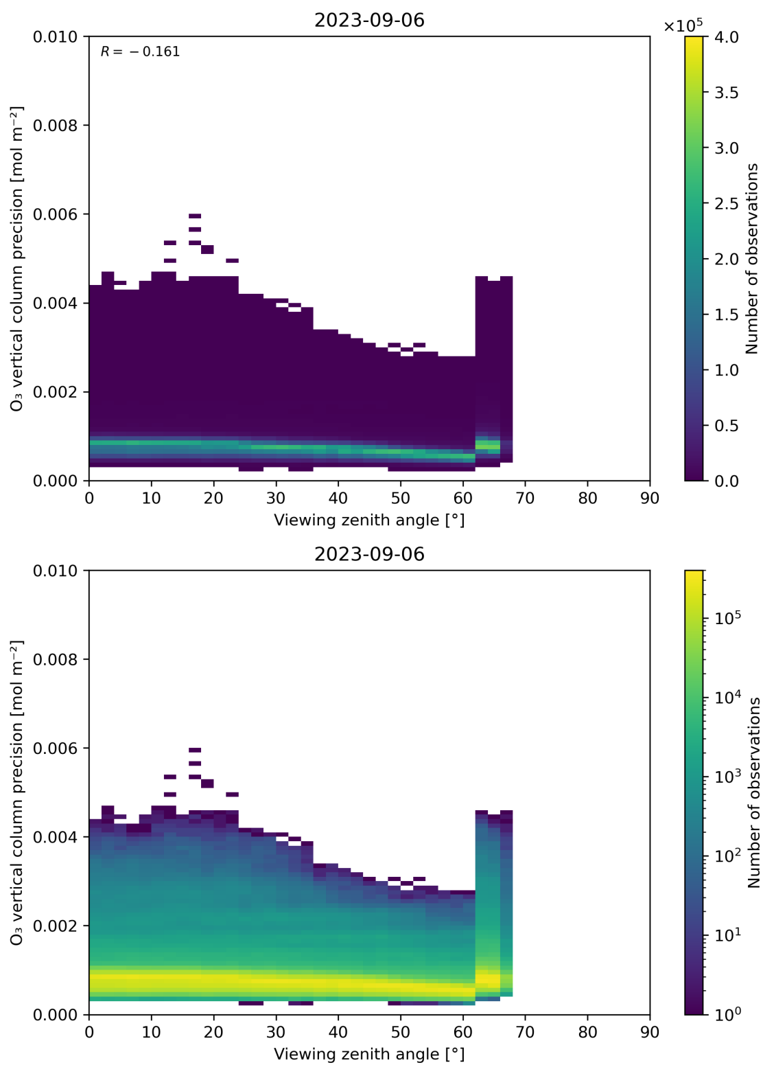
Figure 53: Scatter density plot of “Viewing zenith angle” against “O 3 vertical column precision” for 2023-09-05 to 2023-09-07.
