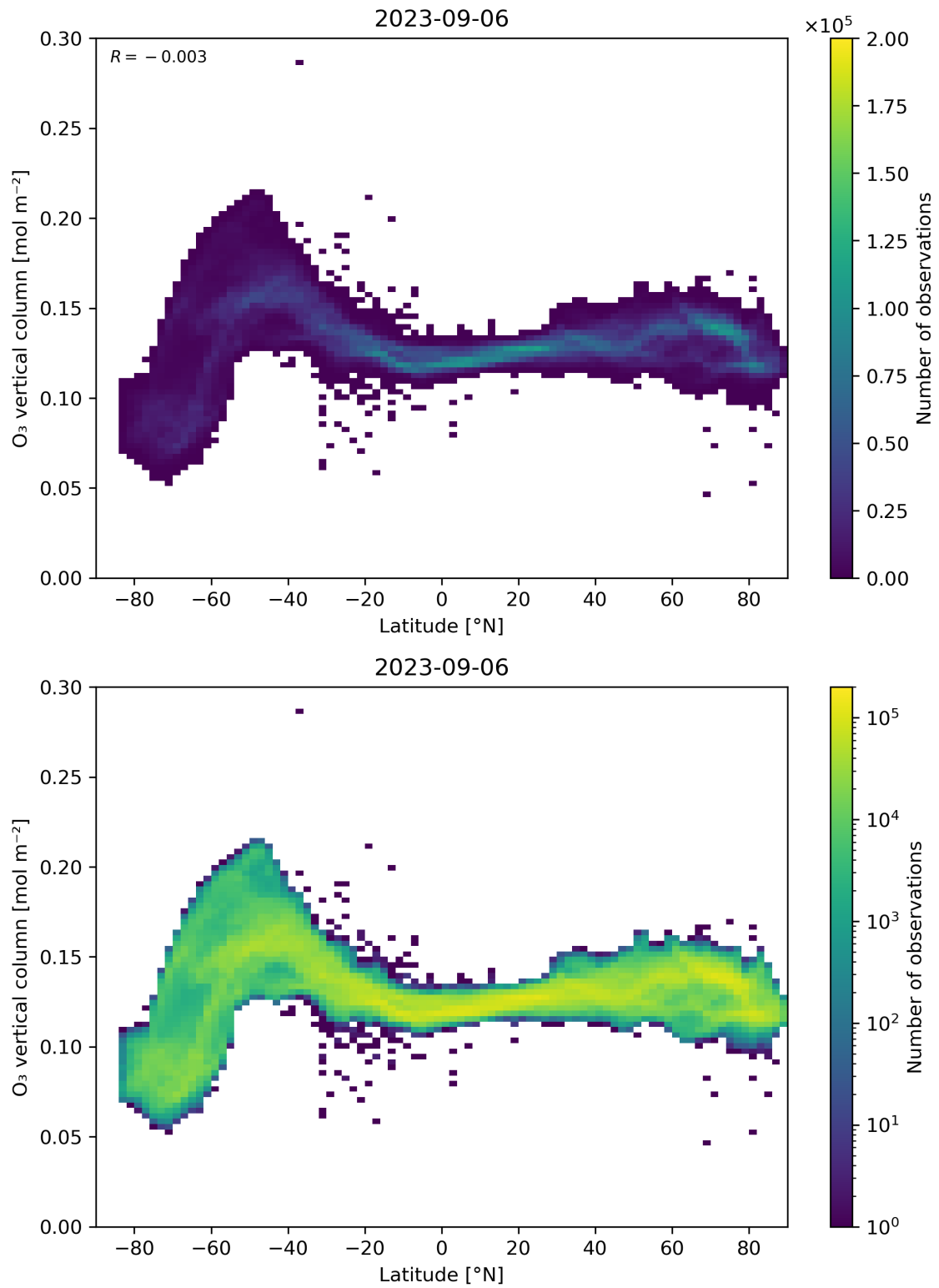
Figure 36: Scatter density plot of “Latitude” against “O 3 vertical column” for 2023-09-05 to 2023-09-07.
