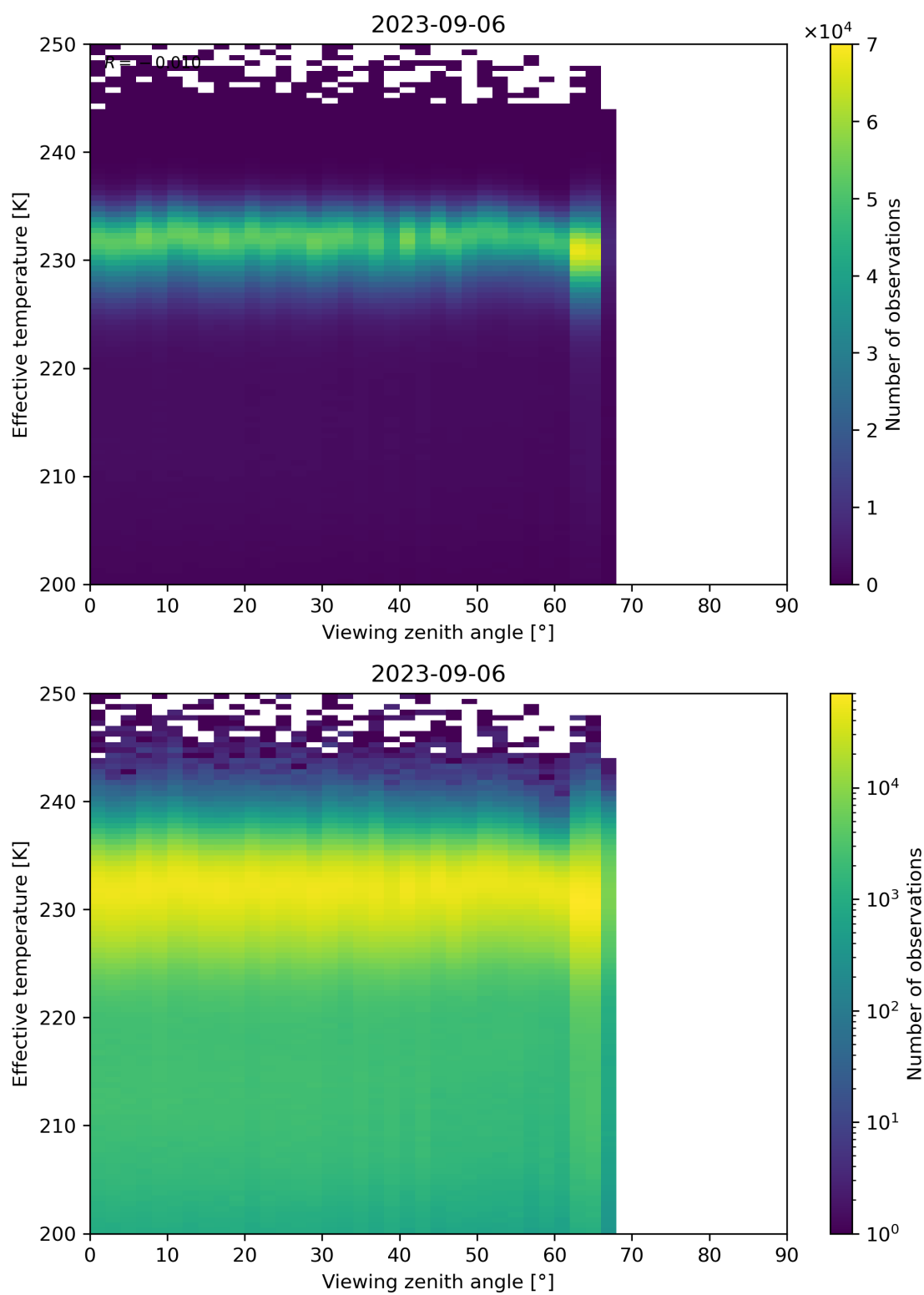
Figure 50: Scatter density plot of “Viewing zenith angle” against “Effective temperature” for 2023-09-05 to 2023-09-07.
