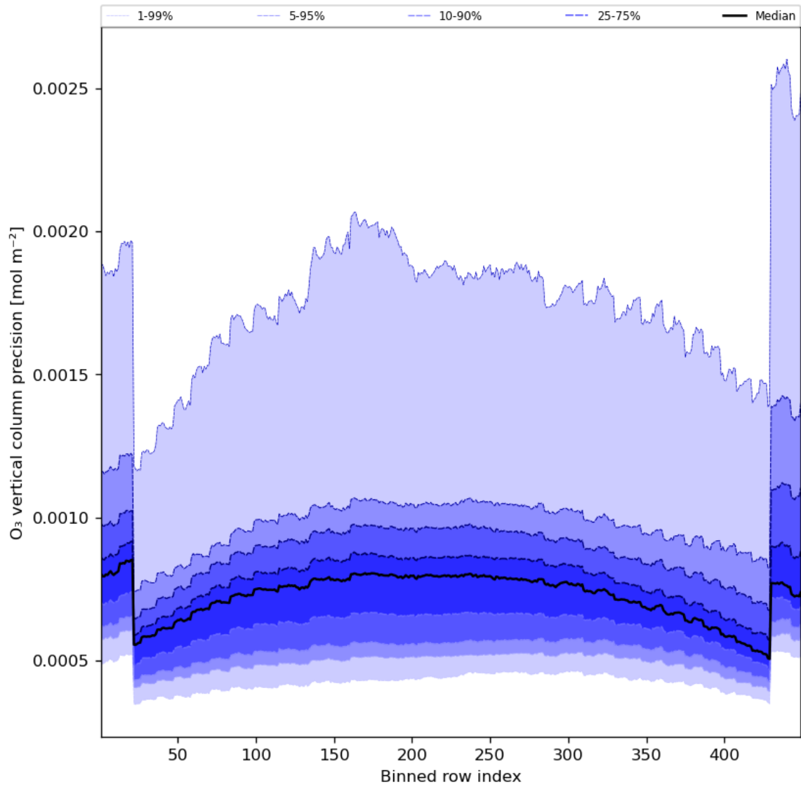
Figure 29: Along track statistics of “O 3 vertical column precision” for 2023-09-05 to 2023-09-07
