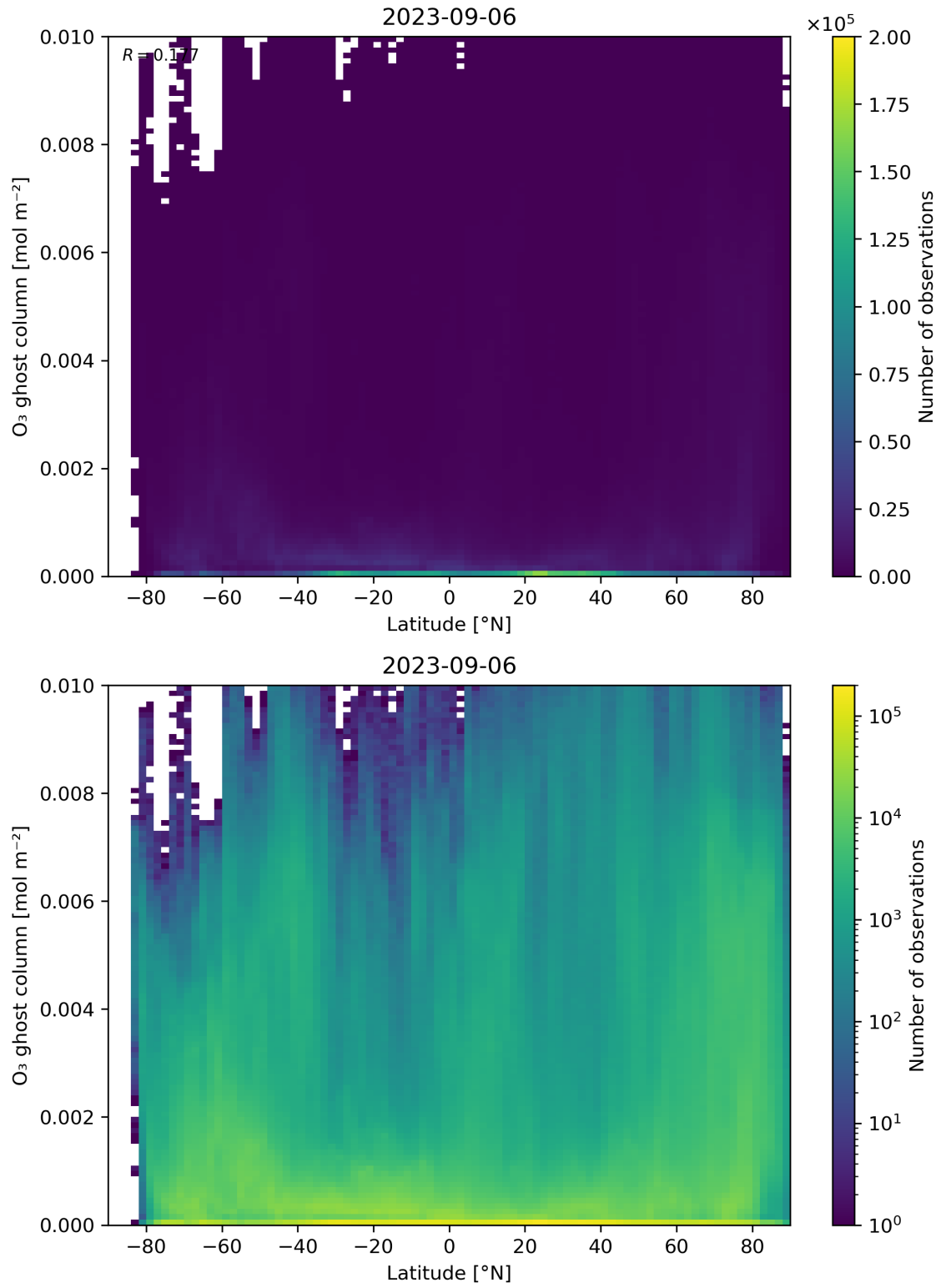
Figure 35: Scatter density plot of “Latitude” against “O 3 ghost column” for 2023-09-05 to 2023-09-07.
