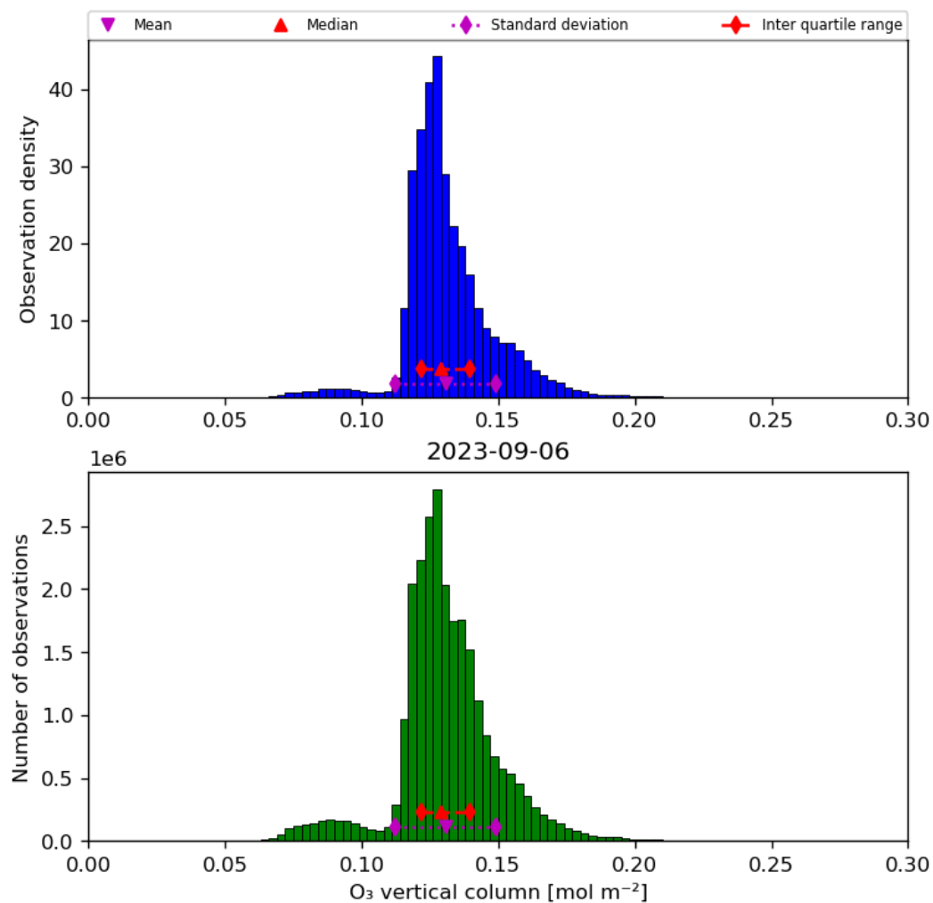
Figure 21: Histogram of “O 3 vertical column” for 2023-09-05 to 2023-09-07
