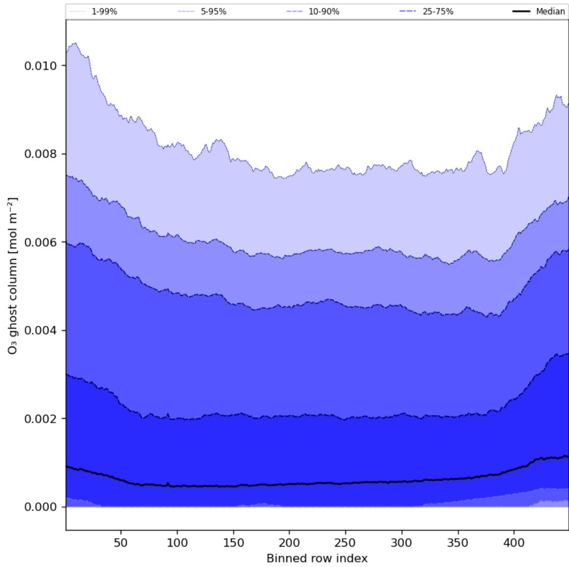
Figure 32: Along track statistics of “O 3 ghost column” for 2023-09-05 to 2023-09-07
