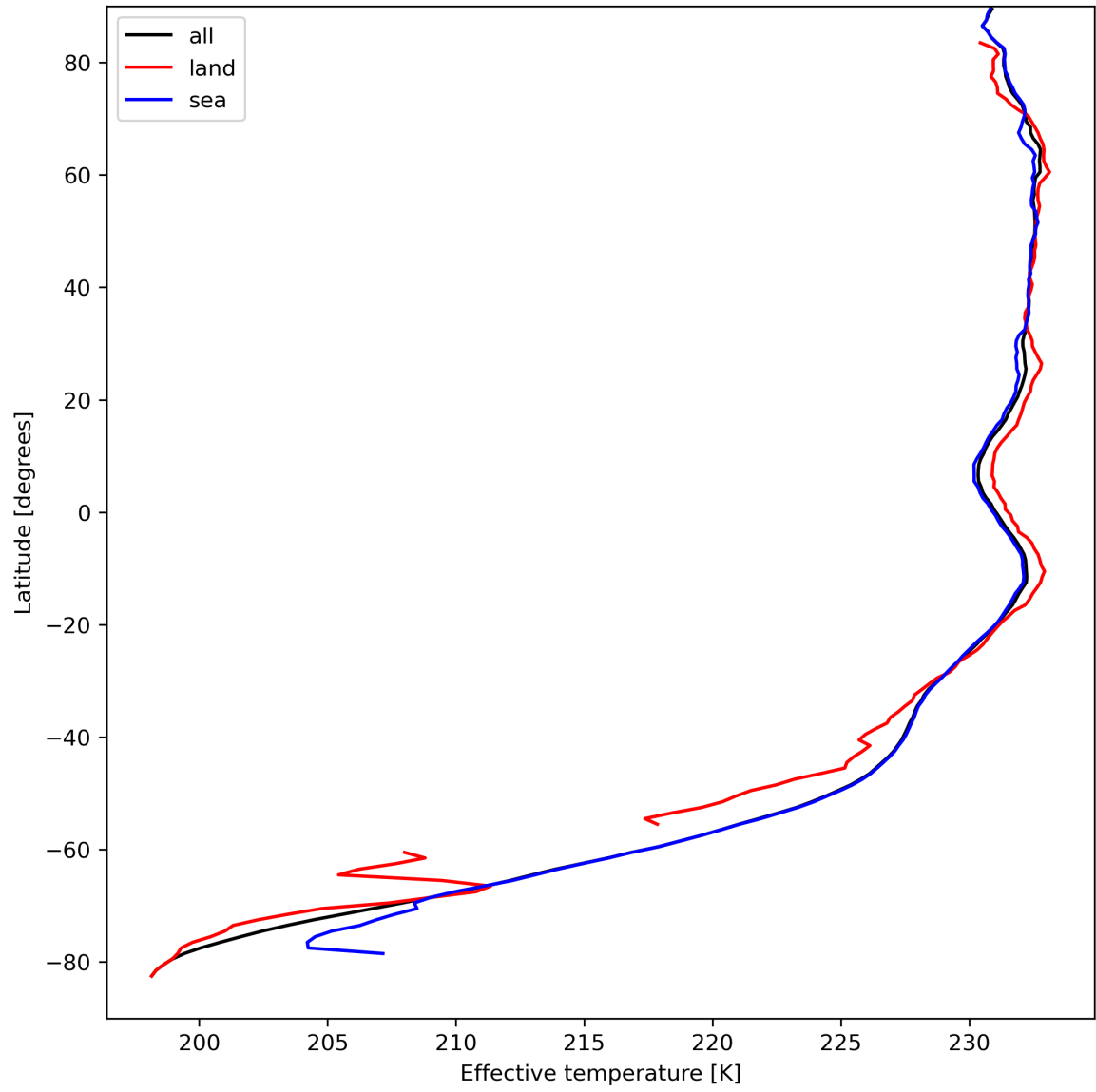
Figure 17: Zonal average of "Effective temperature" for 2023-09-05 to 2023-09-07.
