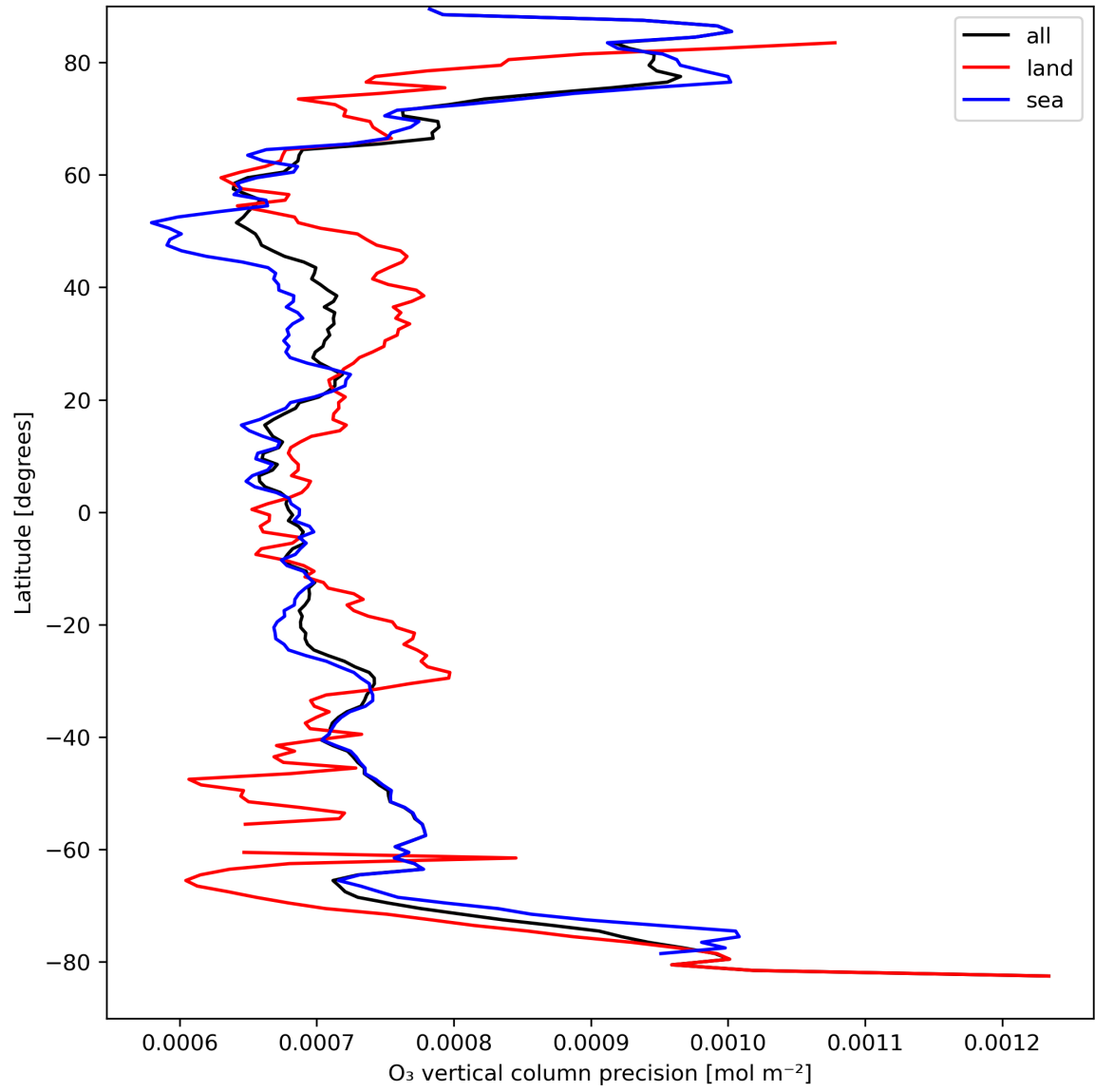
Figure 15: Zonal average of “O 3 vertical column precision” for 2023-09-05 to 2023-09-07.
