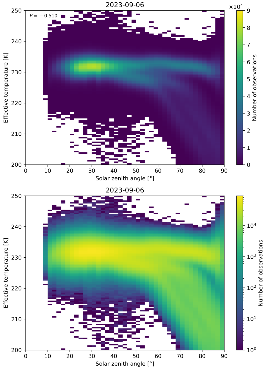
Figure 45: Scatter density plot of “Solar zenith angle” against “Effective temperature” for 2023-09-05 to 2023-09-07.
