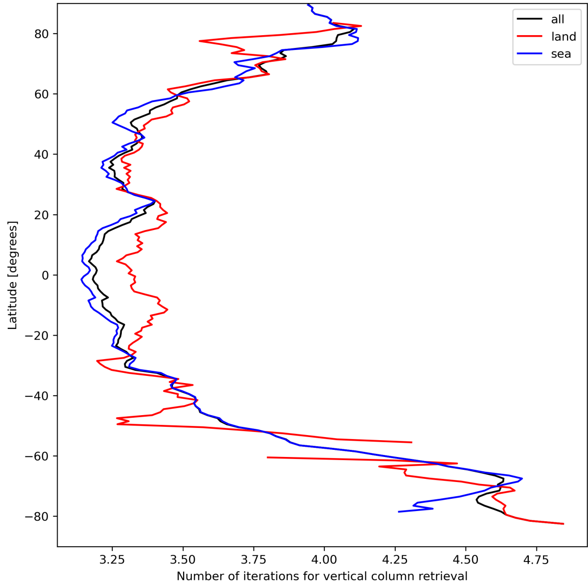
Figure 19: Zonal average of “Number of iterations for vertical column retrieval” for 2023-09-05 to 2023-09-07.
