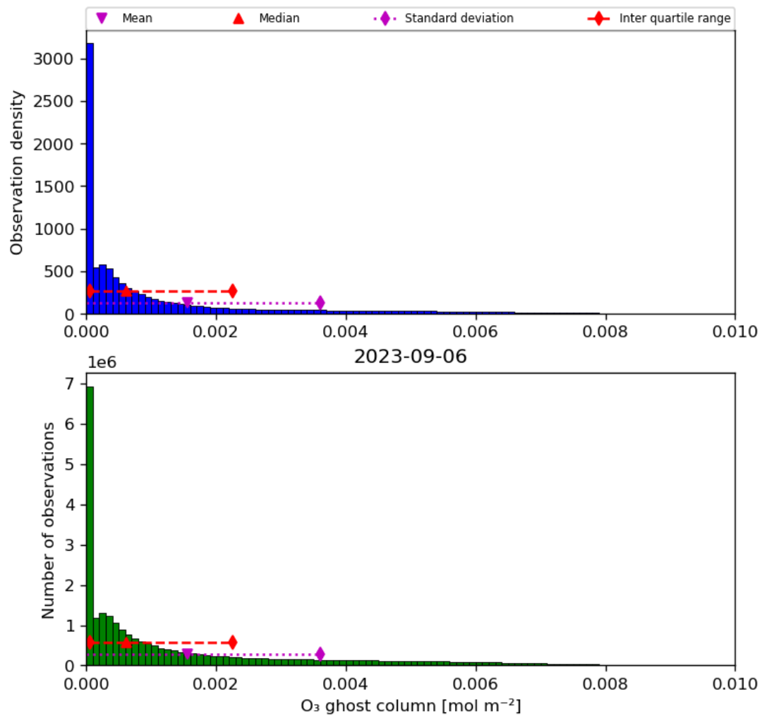
Figure 25: Histogram of “O 3 ghost column” for 2023-09-05 to 2023-09-07
