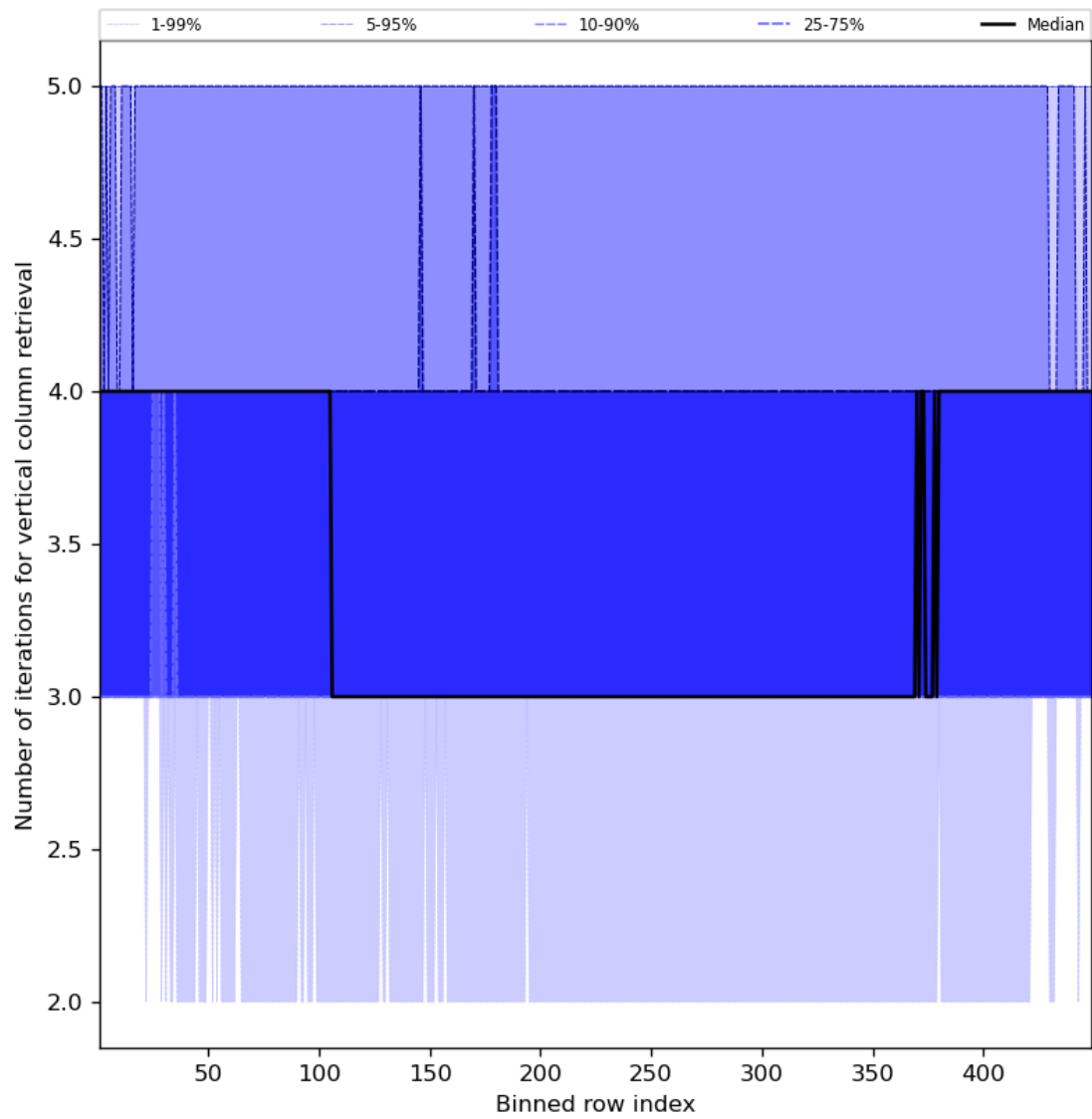
Figure 33: Along track statistics of “Number of iterations for vertical column retrieval” for 2023-09-05 to 2023-09-07
