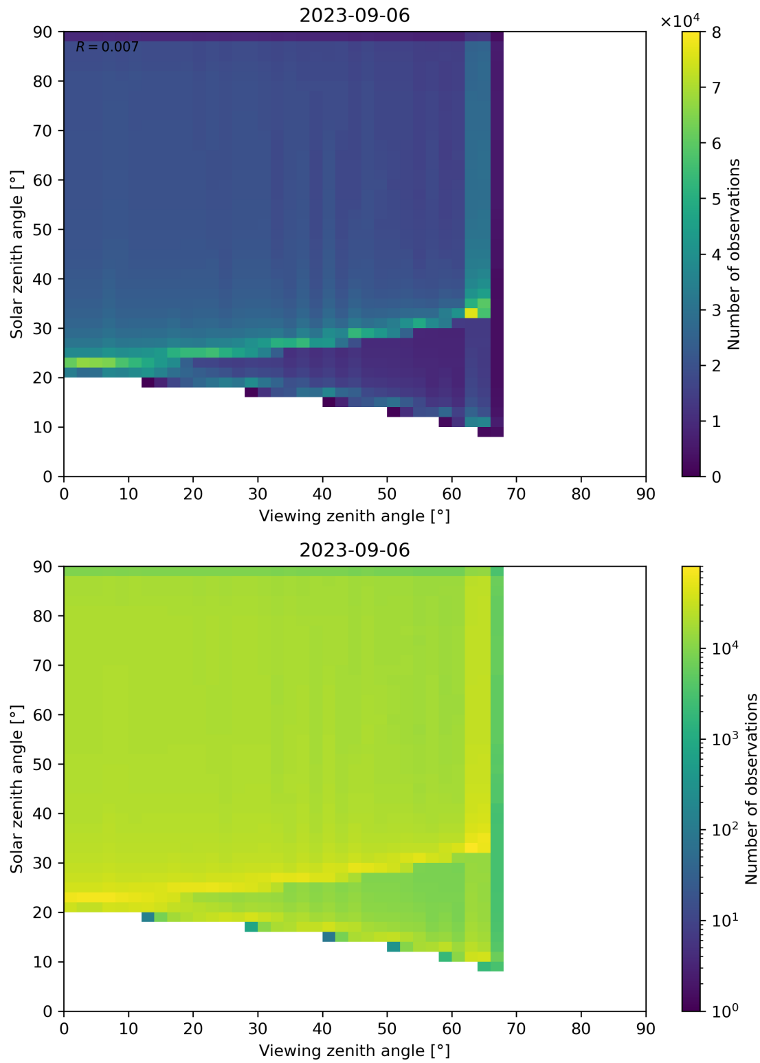
Figure 54: Scatter density plot of “Viewing zenith angle” against “Solar zenith angle” for 2023-09-05 to 2023-09-07.
