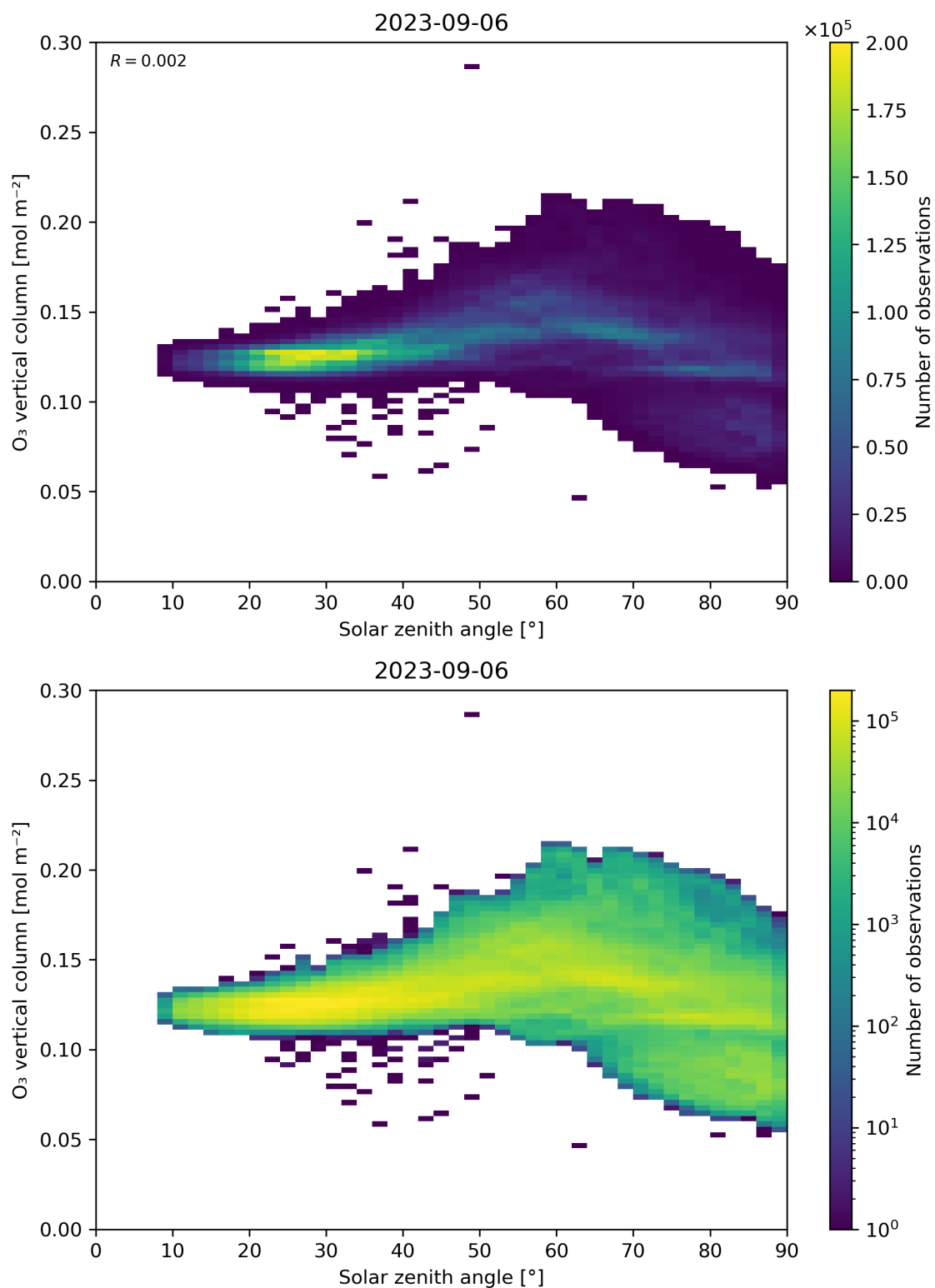
Figure 47: Scatter density plot of “Solar zenith angle” against “O 3 vertical column” for 2023-09-05 to 2023-09-07.
