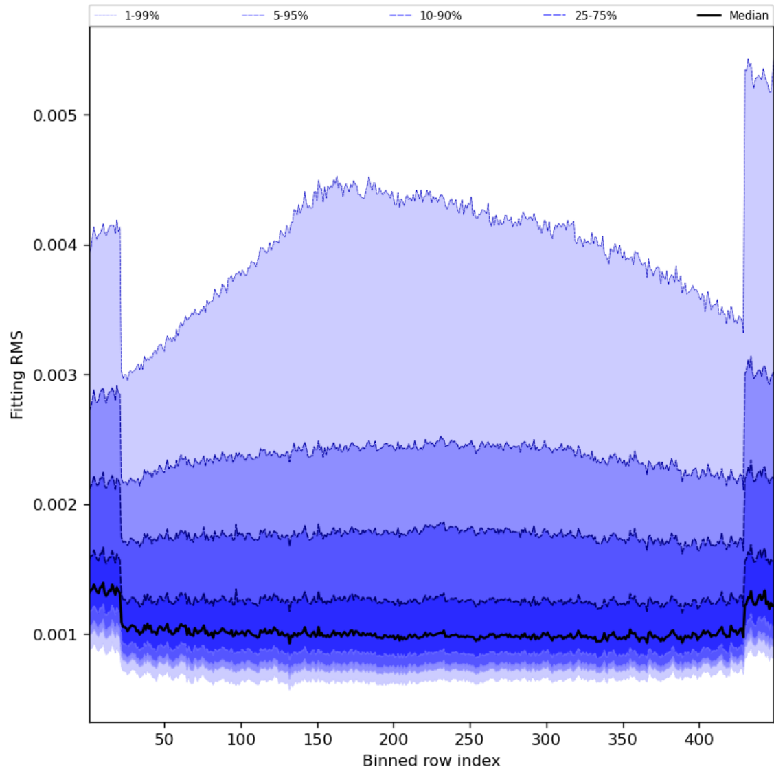
Figure 30: Along track statistics of “Fitting RMS” for 2023-09-05 to 2023-09-07
