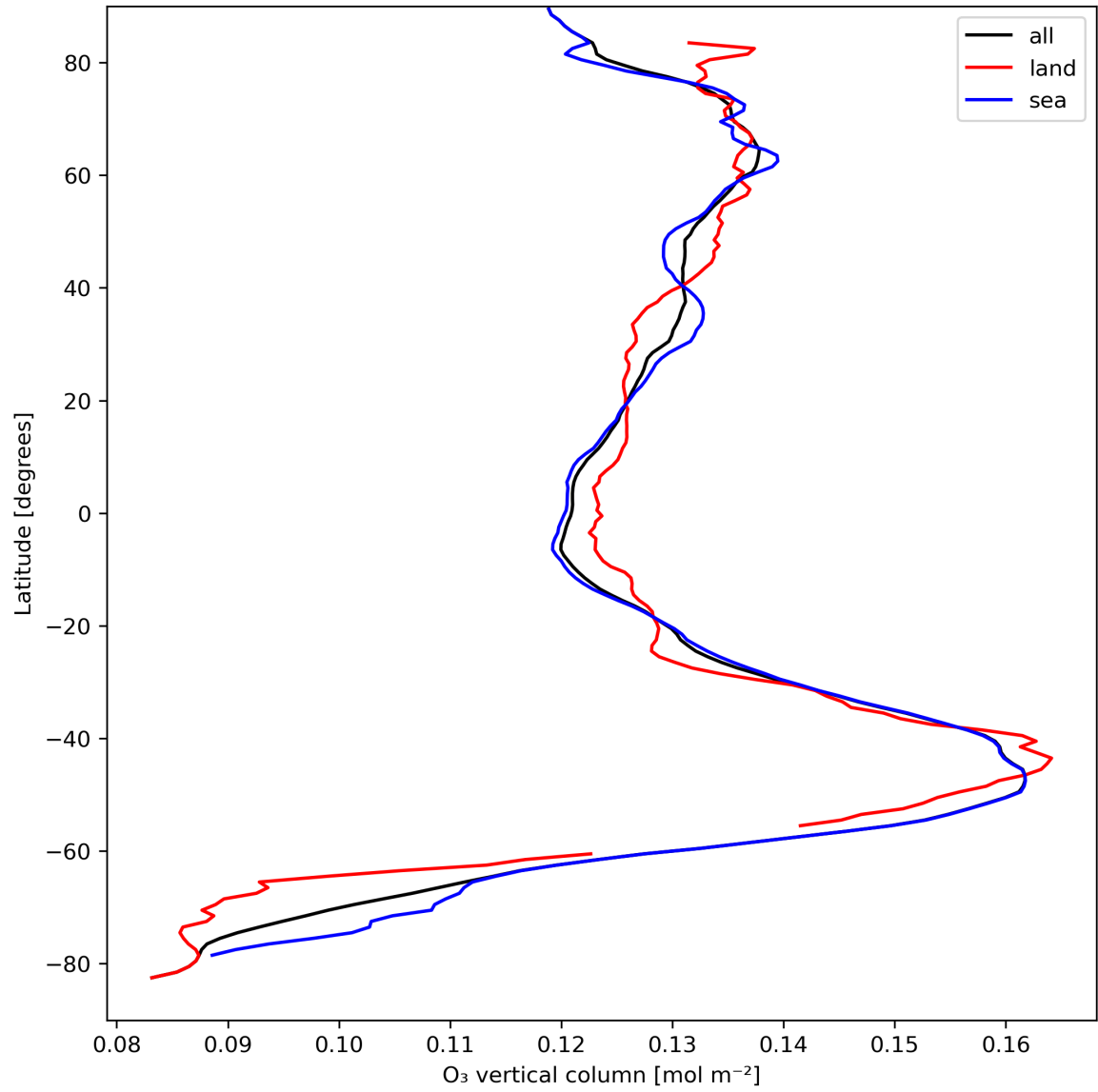
Figure 14: Zonal average of “O 3 vertical column” for 2023-09-05 to 2023-09-07.
