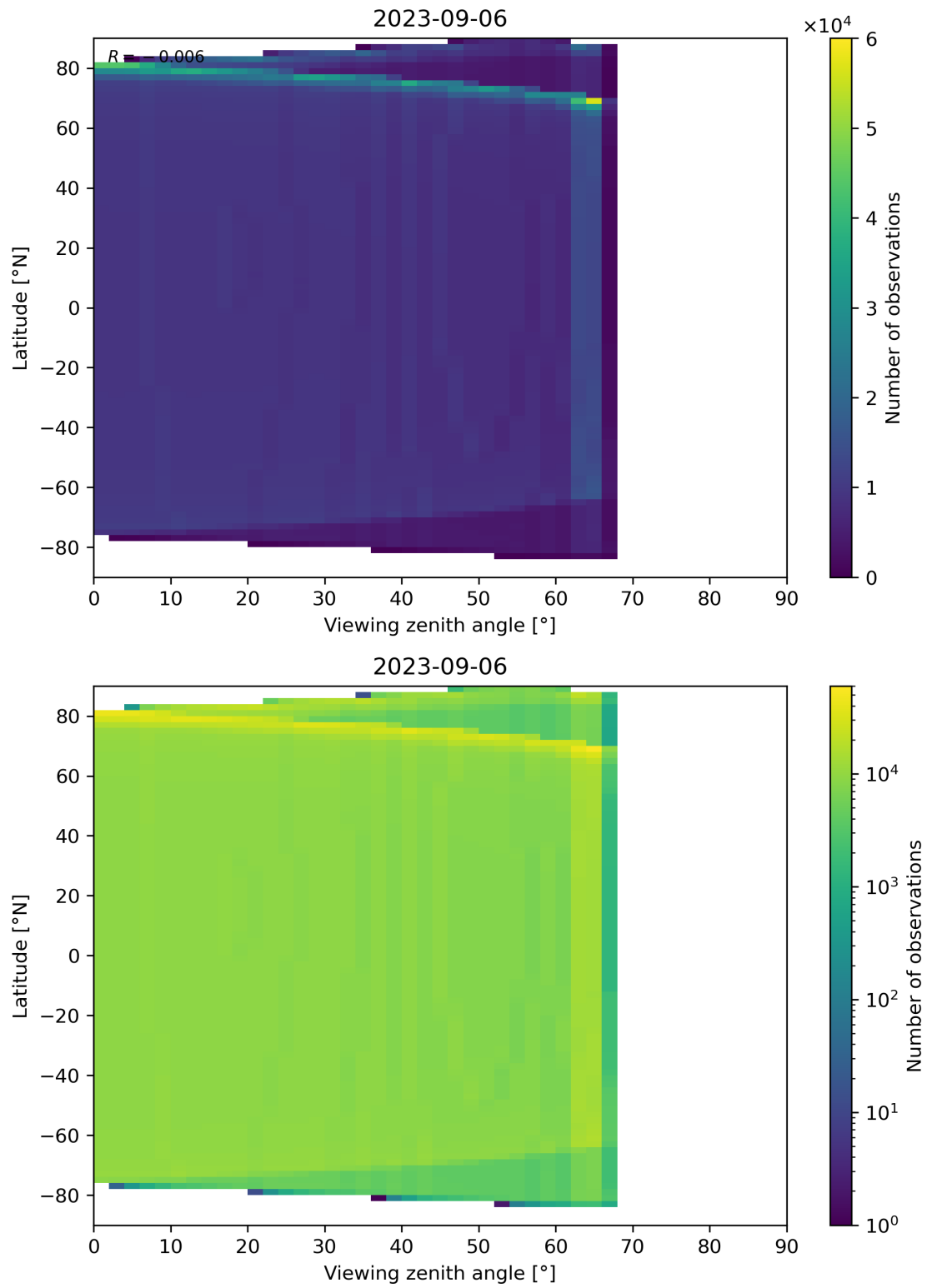
Figure 49: Scatter density plot of “Viewing zenith angle” against “Latitude” for 2023-09-05 to 2023-09-07.
