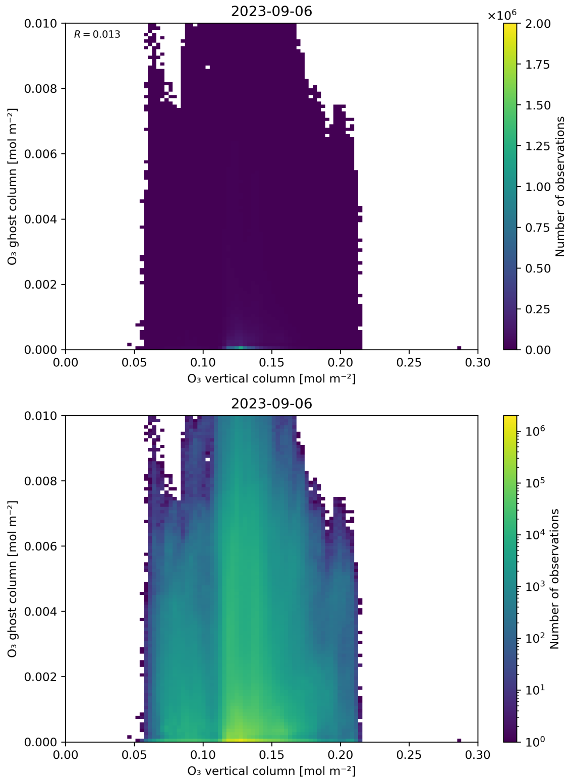
Figure 40: Scatter density plot of “O 3 vertical column” against “O 3 ghost column” for 2023-09-05 to 2023-09-07.
