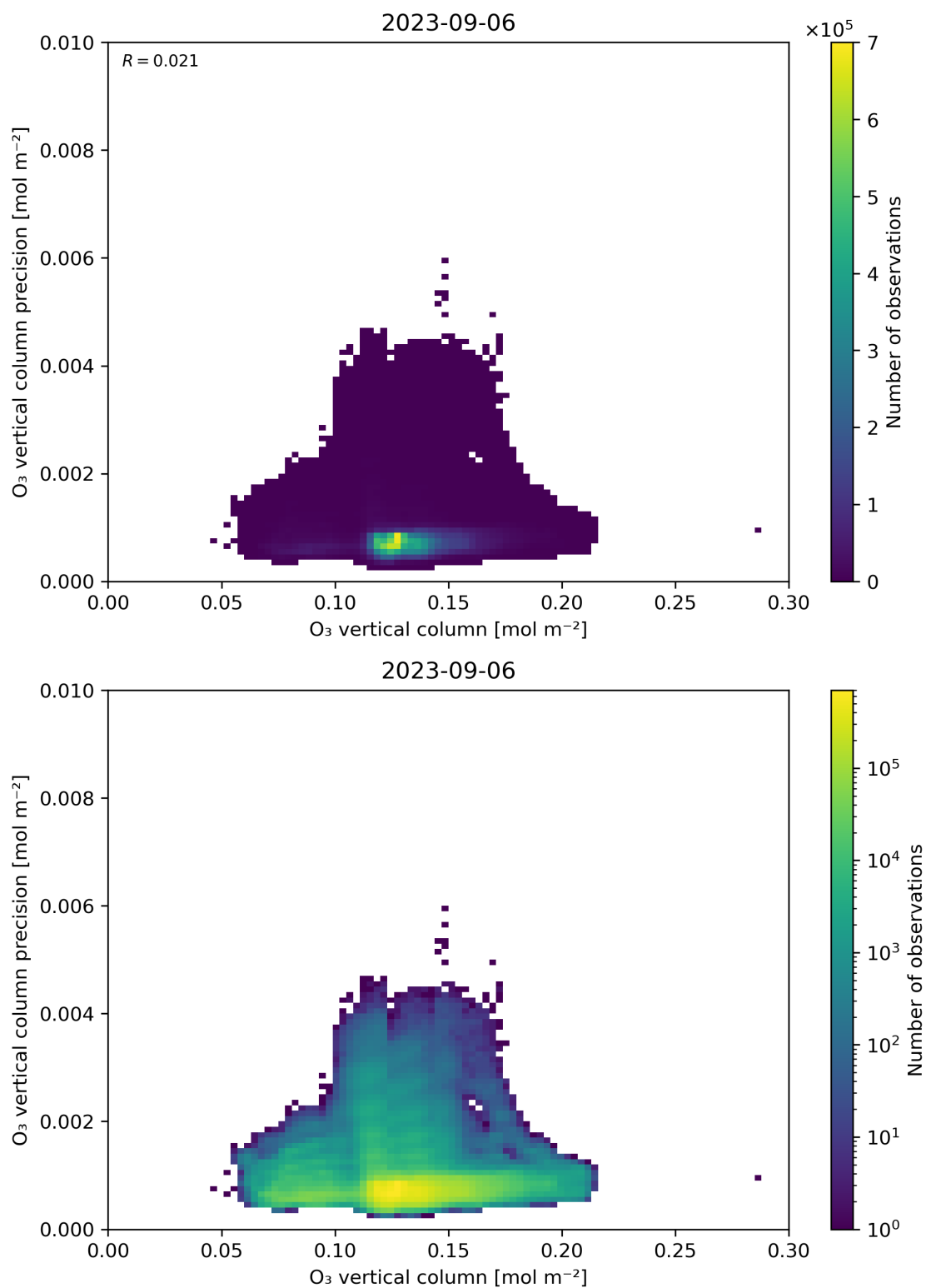
Figure 41: Scatter density plot of “O 3 vertical column” against “O 3 vertical column precision” for 2023-09-05 to 2023-09-07.
