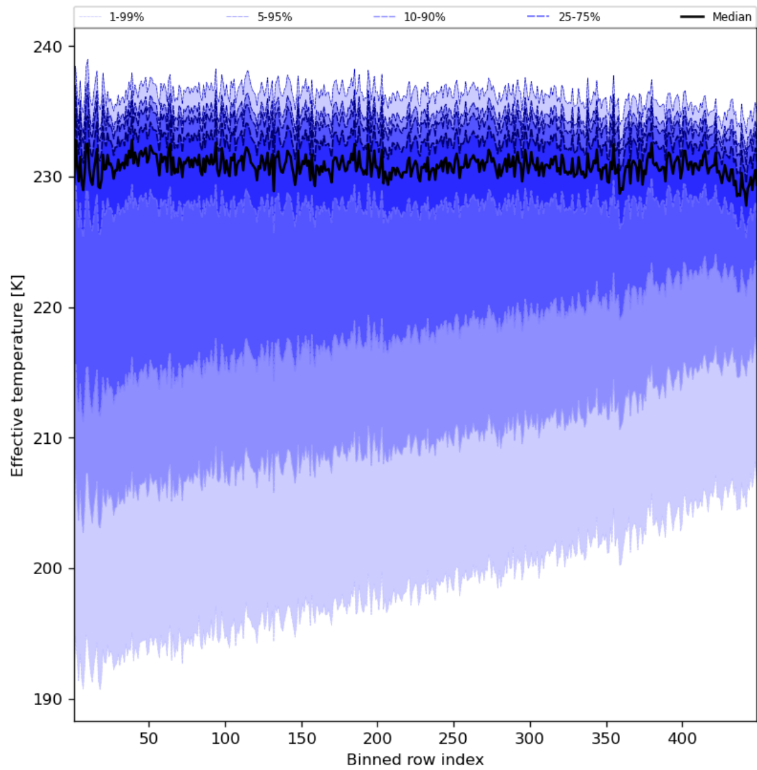
Figure 31: Along track statistics of “Effective temperature” for 2023-09-05 to 2023-09-07
