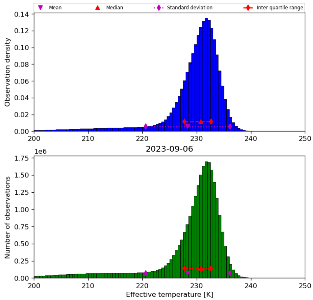
Figure 24: Histogram of “Effective temperature” for 2023-09-05 to 2023-09-07
