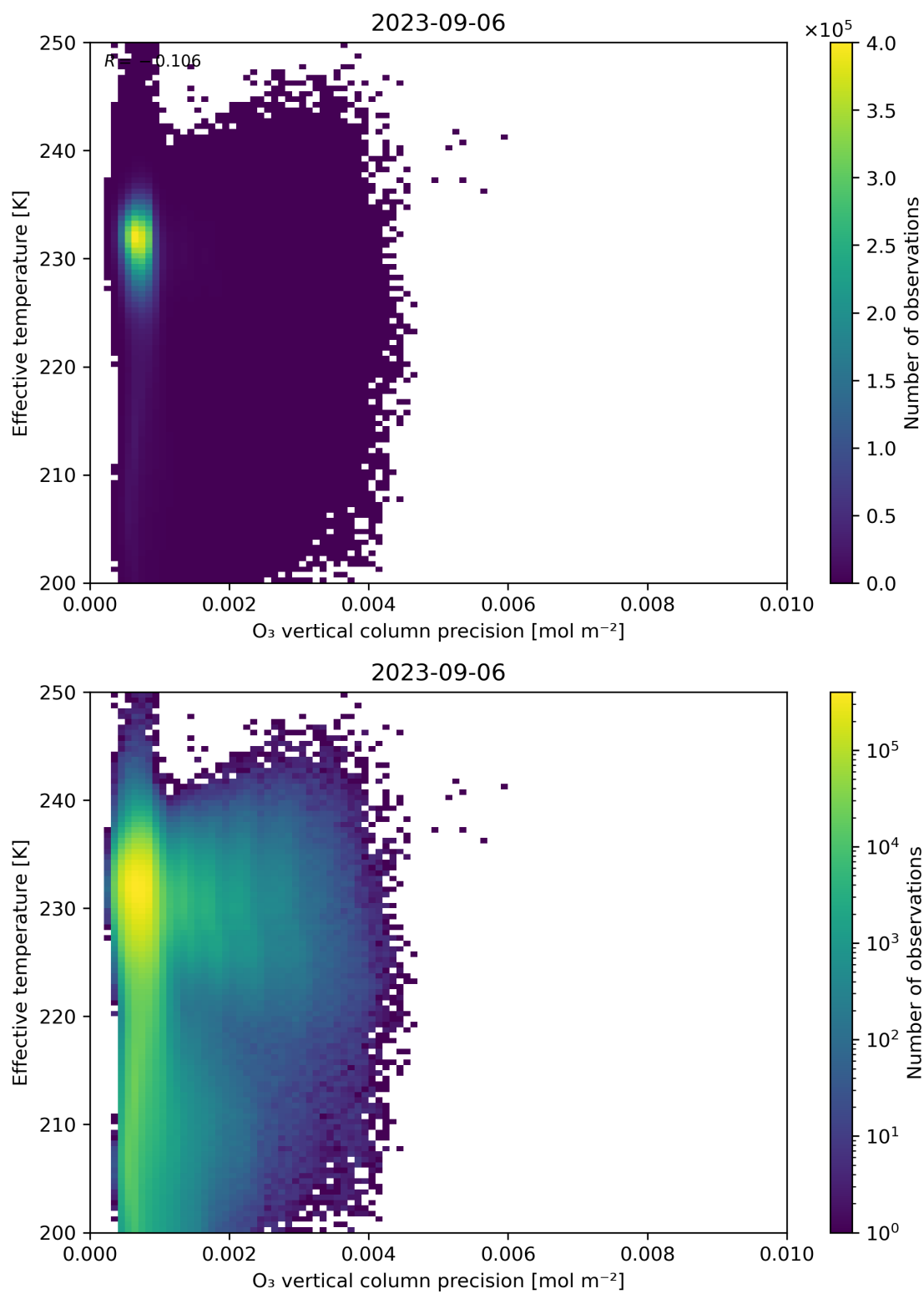
Figure 42: Scatter density plot of “O 3 vertical column precision” against “Effective temperature” for 2023-09-05 to 2023-09-07.
