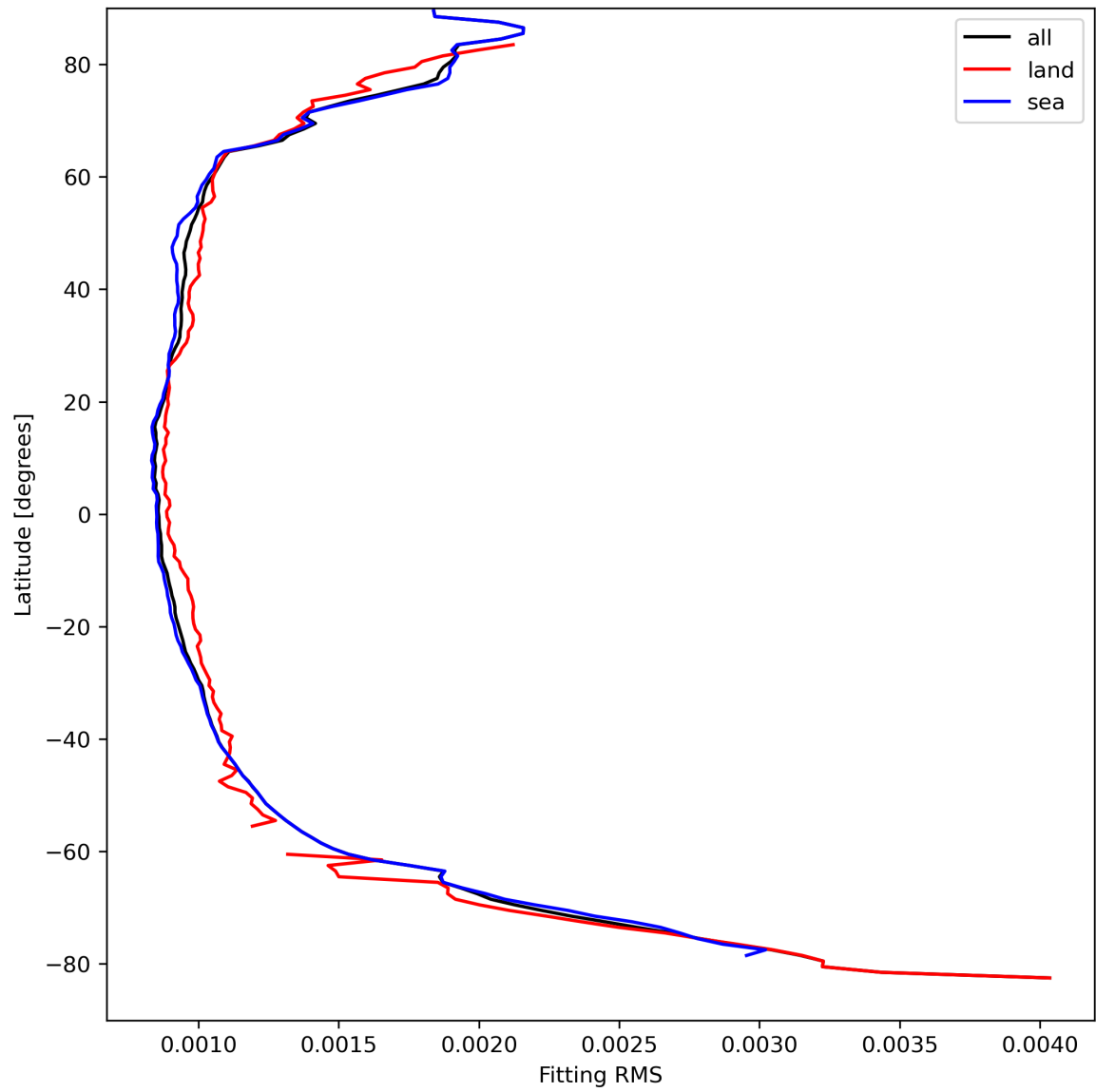
Figure 16: Zonal average of “Fitting RMS” for 2023-09-05 to 2023-09-07.
