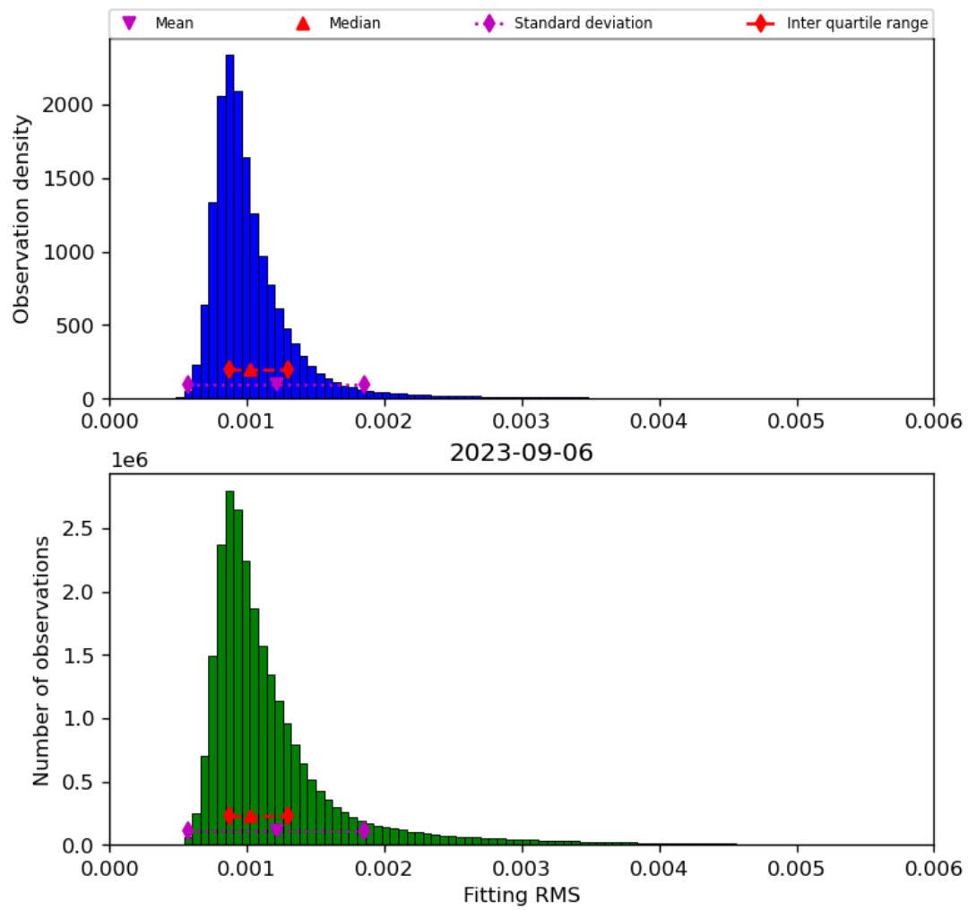
Figure 23: Histogram of “Fitting RMS” for 2023-09-05 to 2023-09-07
