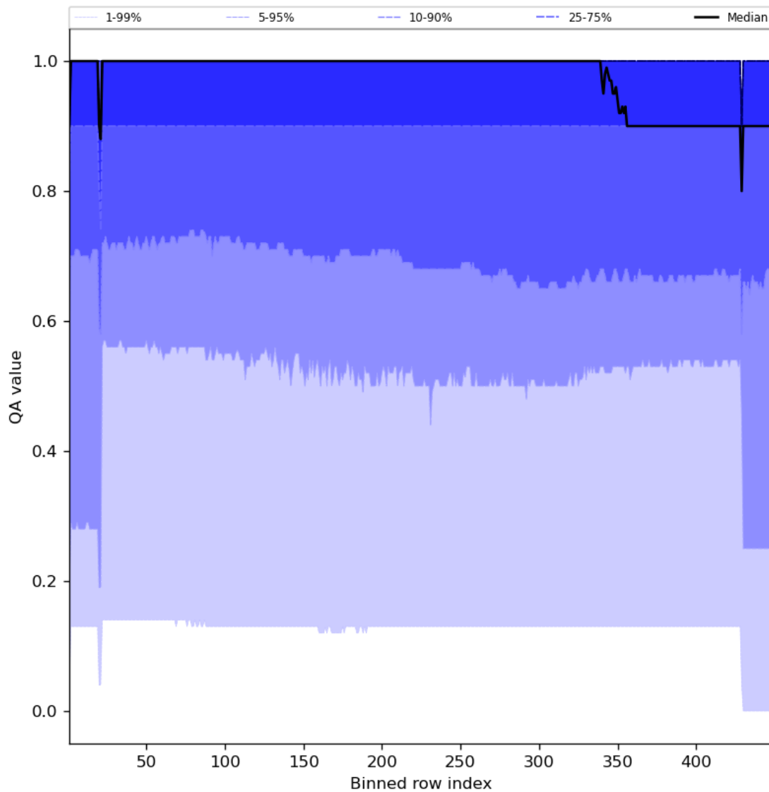
Figure 27: Along track statistics of “QA value” for 2023-09-05 to 2023-09-07
