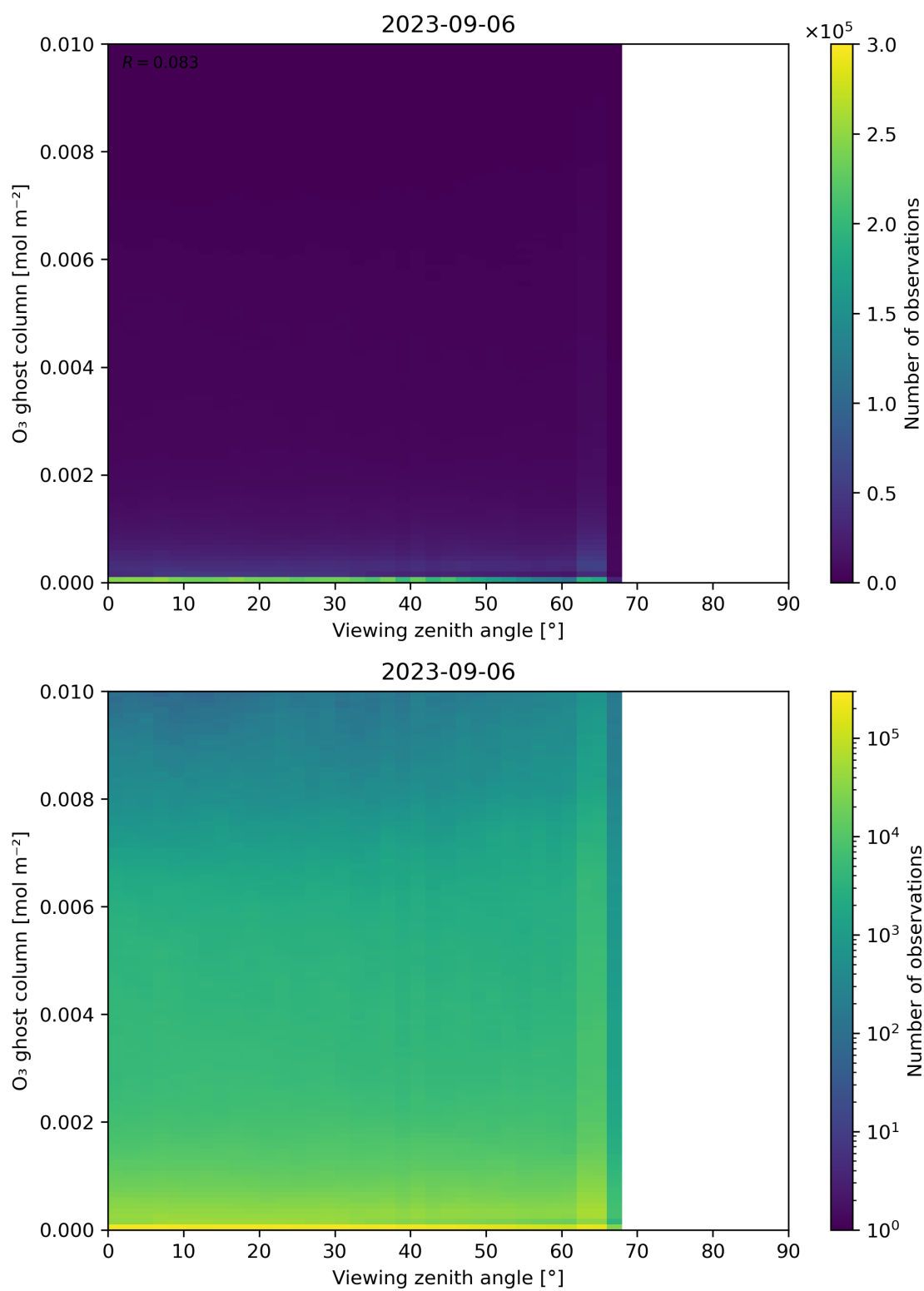
Figure 51: Scatter density plot of “Viewing zenith angle” against “O 3 ghost column” for 2023-09-05 to 2023-09-07.
