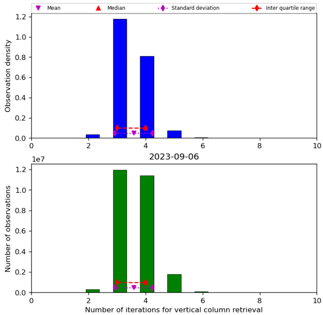
Figure 26: Histogram of “Number of iterations for vertical column retrieval” for 2023-09-05 to 2023-09-07
