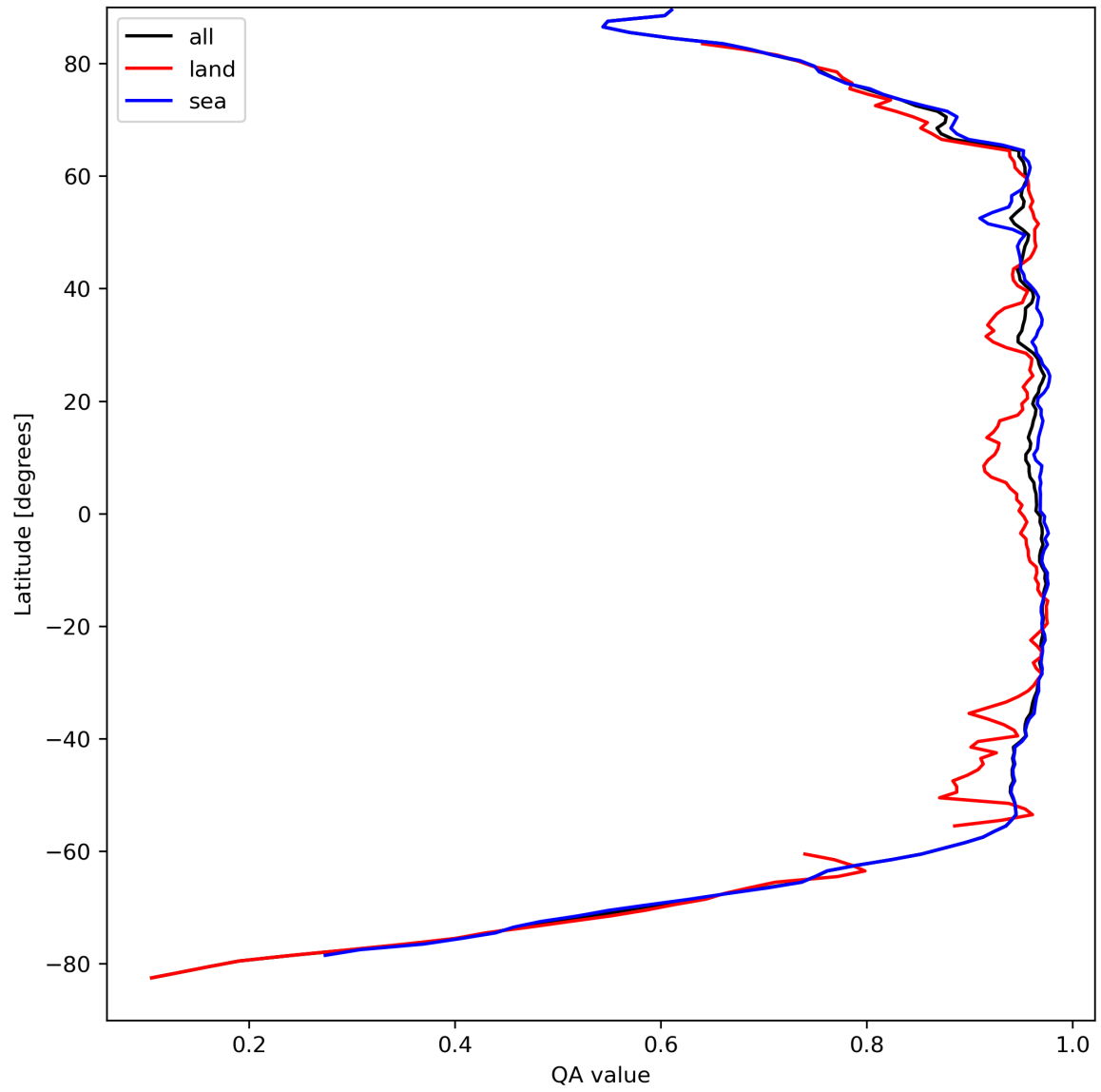
Figure 13: Zonal average of “QA value” for 2023-09-05 to 2023-09-07.
