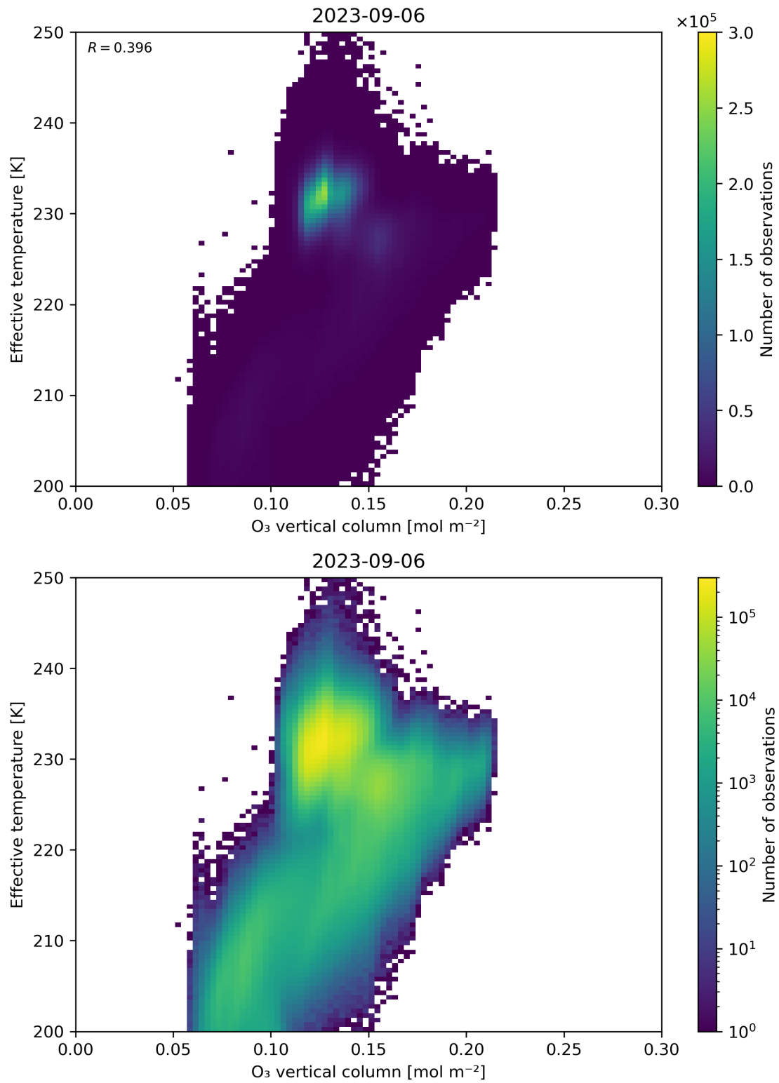
Figure 39: Scatter density plot of “O 3 vertical column” against “Effective temperature” for 2023-09-05 to 2023-09-07.
