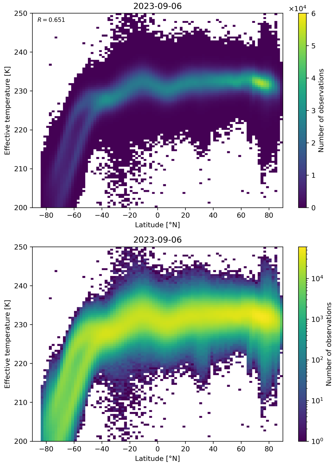
Figure 34: Scatter density plot of “Latitude” against “Effective temperature” for 2023-09-05 to 2023-09-07.
