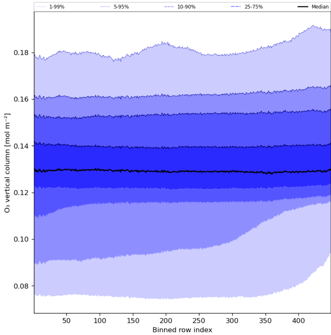
Figure 28: Along track statistics of “O 3 vertical column” for 2023-09-05 to 2023-09-07
