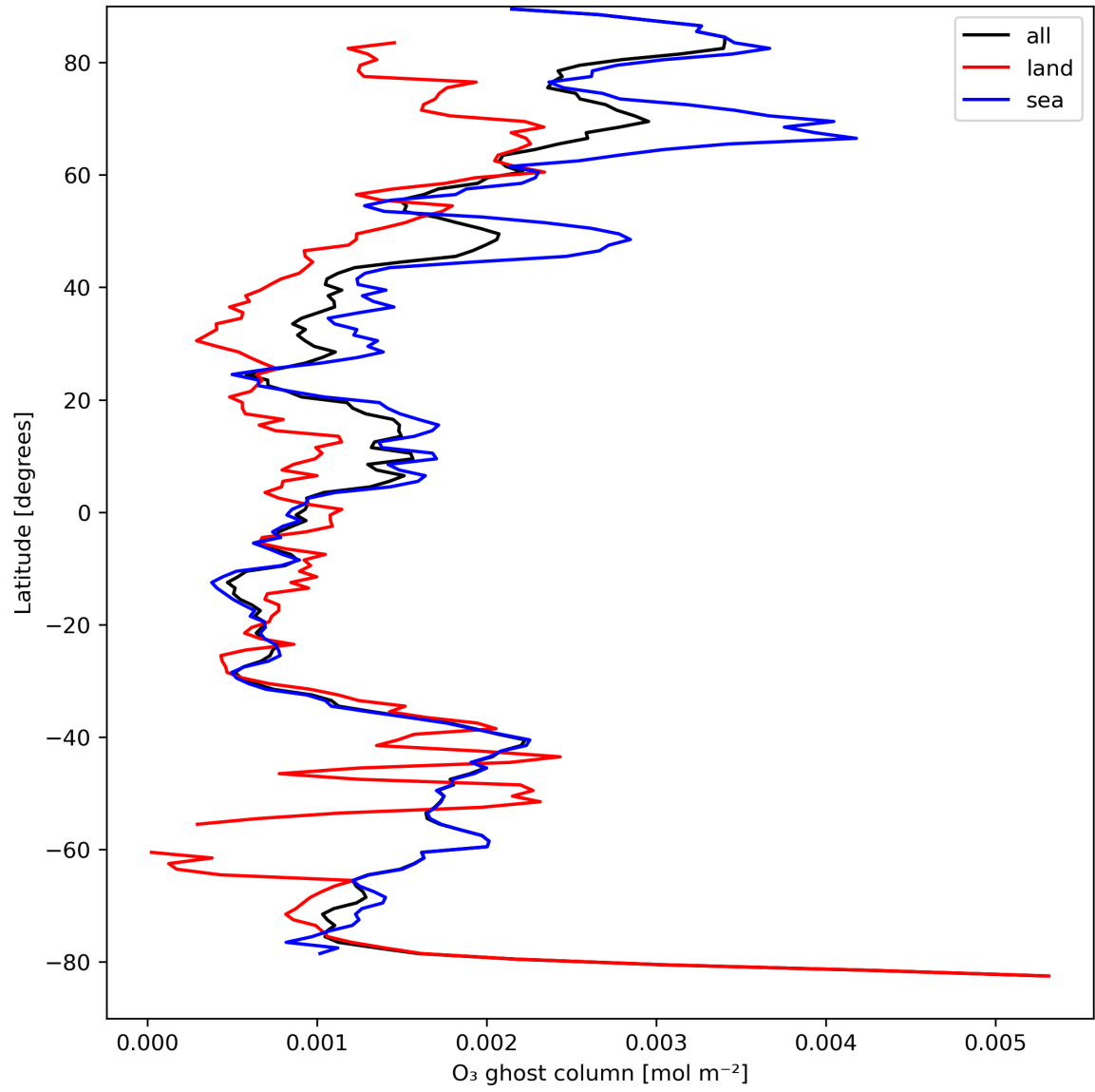
Figure 18: Zonal average of “O 3 ghost column” for 2023-09-05 to 2023-09-07.
