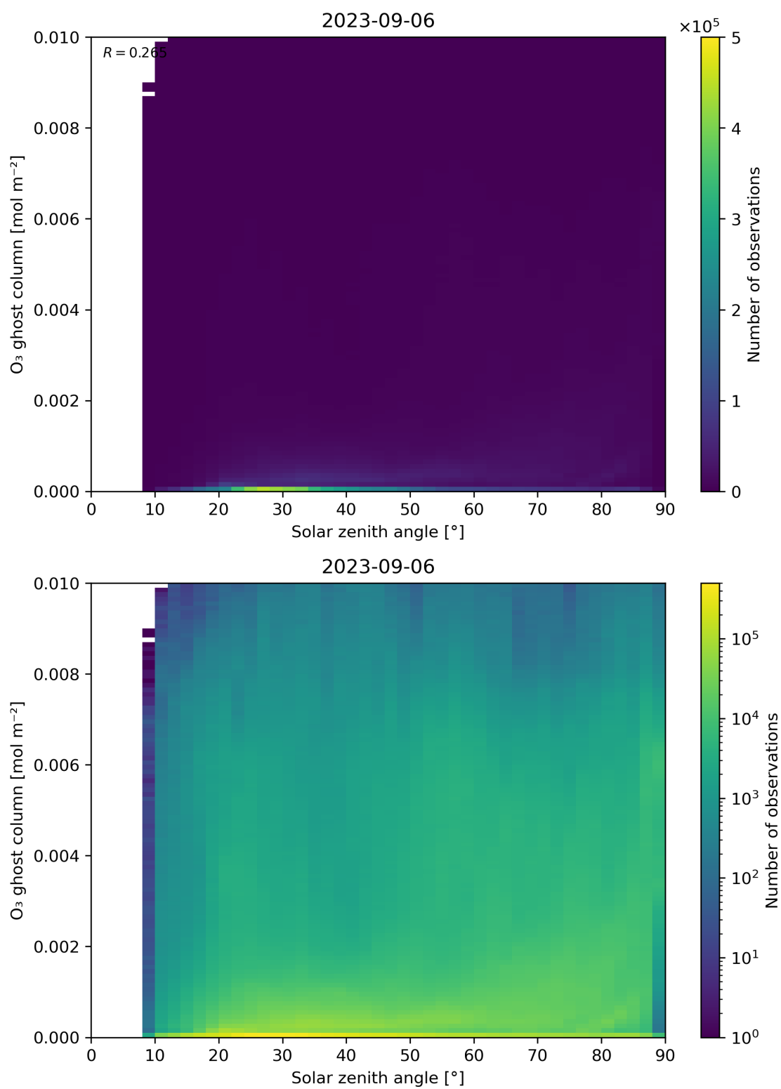
Figure 46: Scatter density plot of “Solar zenith angle” against “O 3 ghost column” for 2023-09-05 to 2023-09-07.
