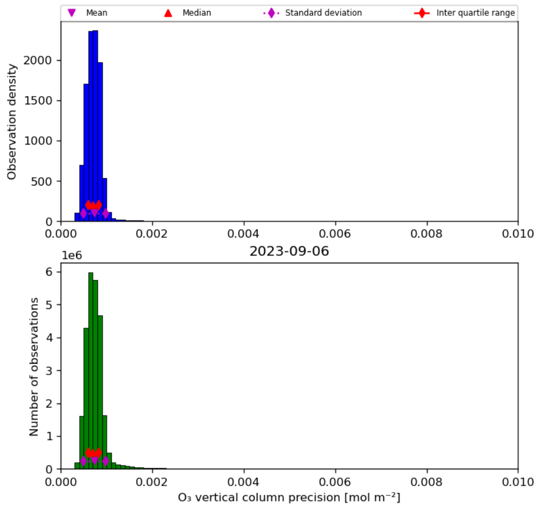
Figure 22: Histogram of “O 3 vertical column precision” for 2023-09-05 to 2023-09-07
