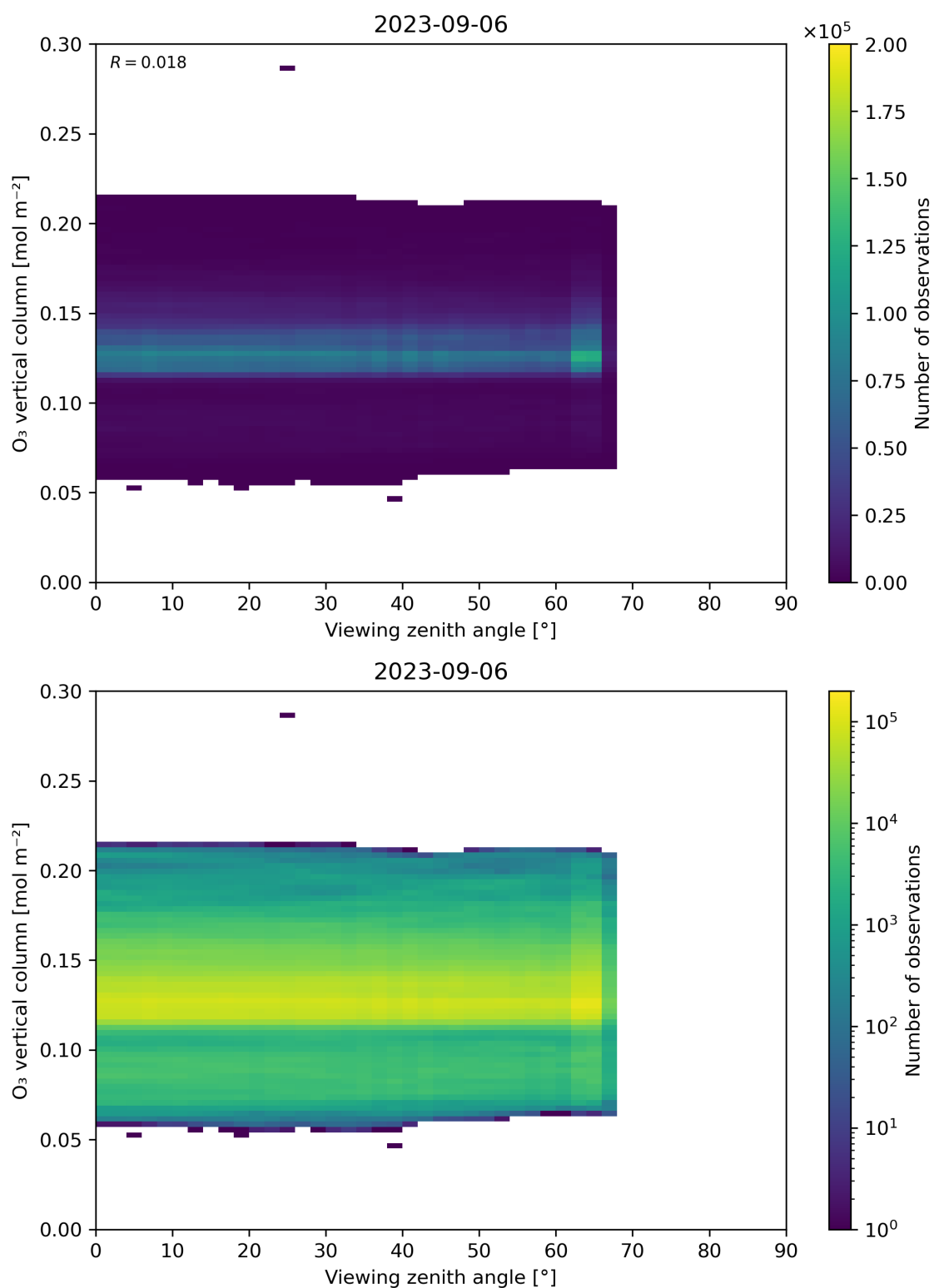
Figure 52: Scatter density plot of “Viewing zenith angle” against “O 3 vertical column” for 2023-09-05 to 2023-09-07.
