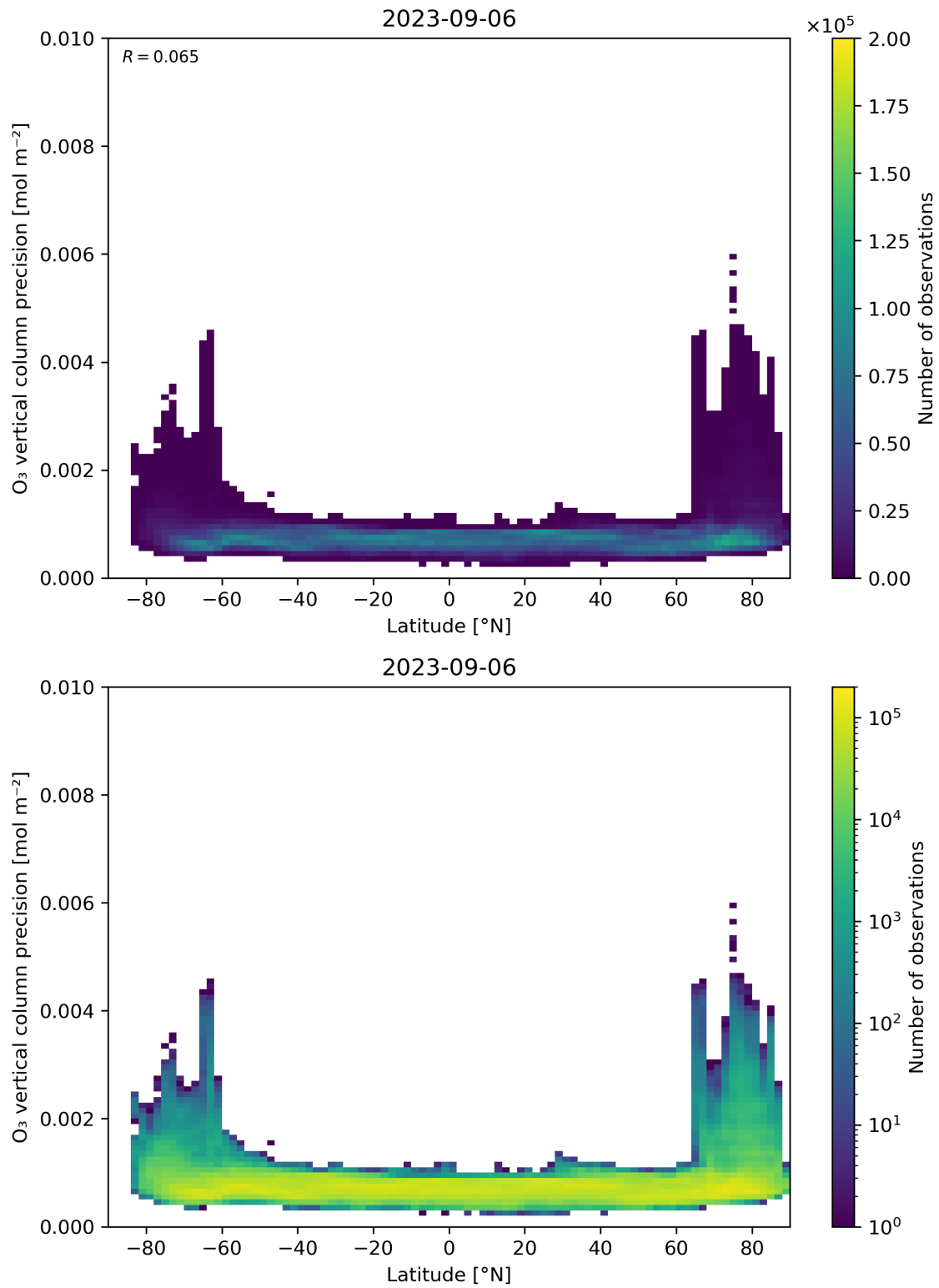
Figure 37: Scatter density plot of “Latitude” against “O 3 vertical column precision” for 2023-09-05 to 2023-09-07.
