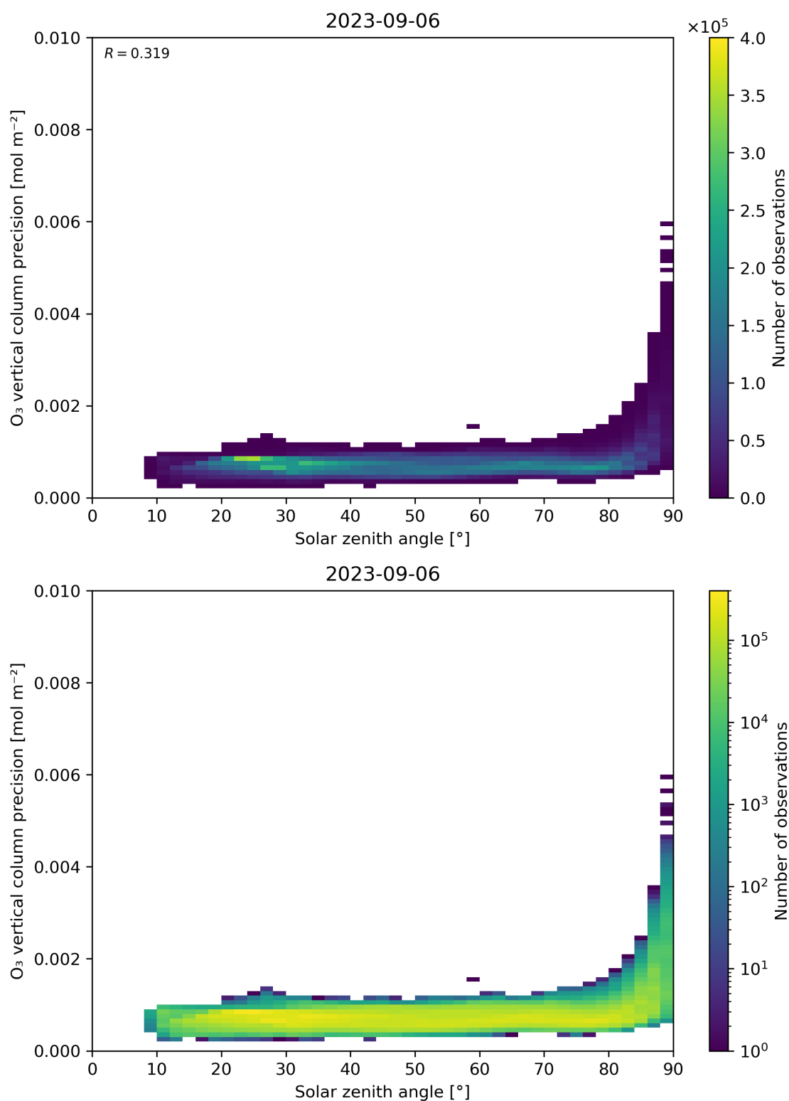
Figure 48: Scatter density plot of “Solar zenith angle” against “O 3 vertical column precision” for 2023-09-05 to 2023-09-07.
