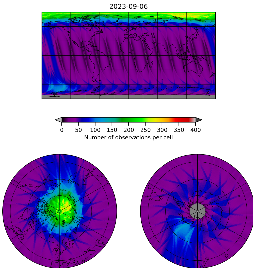
Figure 12: Map of the number of observations for 2023-09-05 to 2023-09-07
