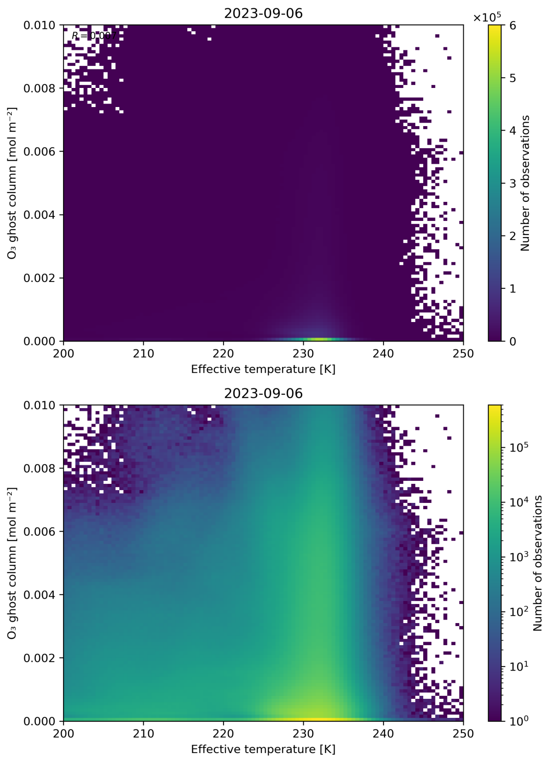
Figure 38: Scatter density plot of “Effective temperature” against “O 3 ghost column” for 2023-09-05 to 2023-09-07.
