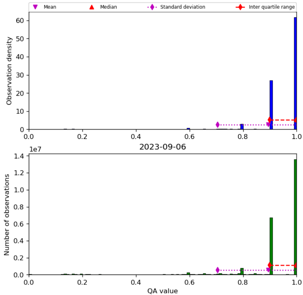
Figure 20: Histogram of “QA value” for 2023-09-05 to 2023-09-07
