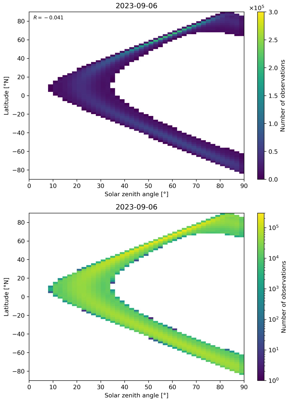
Figure 44: Scatter density plot of “Solar zenith angle” against “Latitude” for 2023-09-05 to 2023-09-07.
