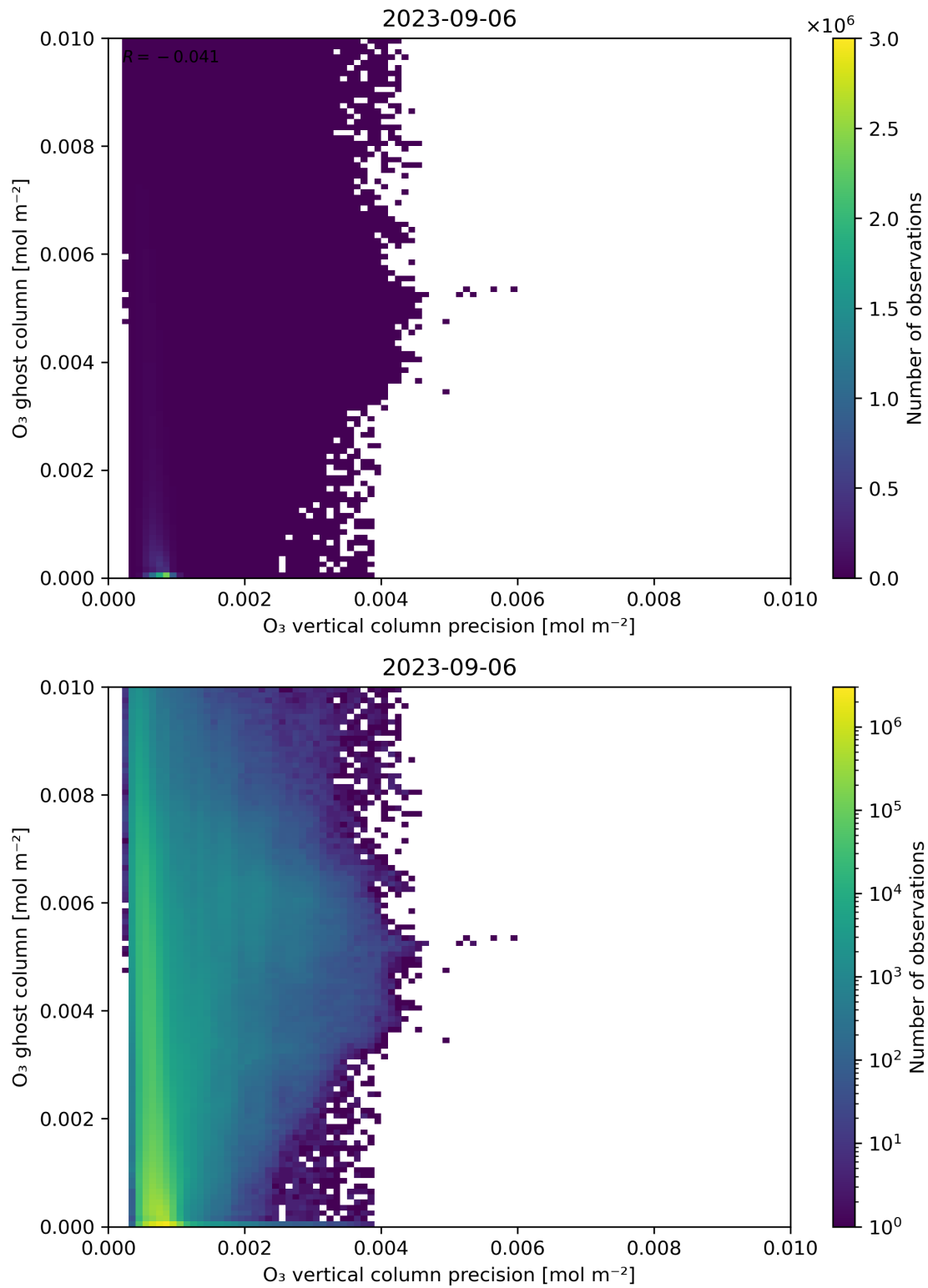
Figure 43: Scatter density plot of “O 3 vertical column precision” against “O 3 ghost column” for 2023-09-05 to 2023-09-07.
