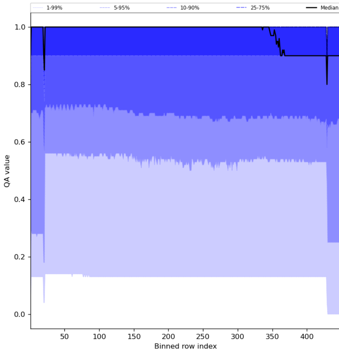
Figure 27: Along track statistics of “QA value” for 2023-09-06 to 2023-09-08
