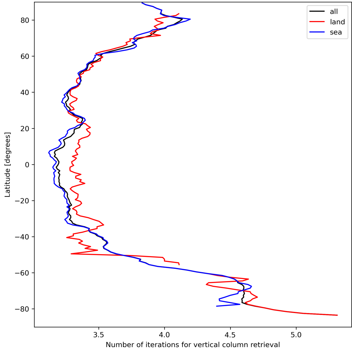
Figure 19: Zonal average of “Number of iterations for vertical column retrieval” for 2023-09-06 to 2023-09-08.
