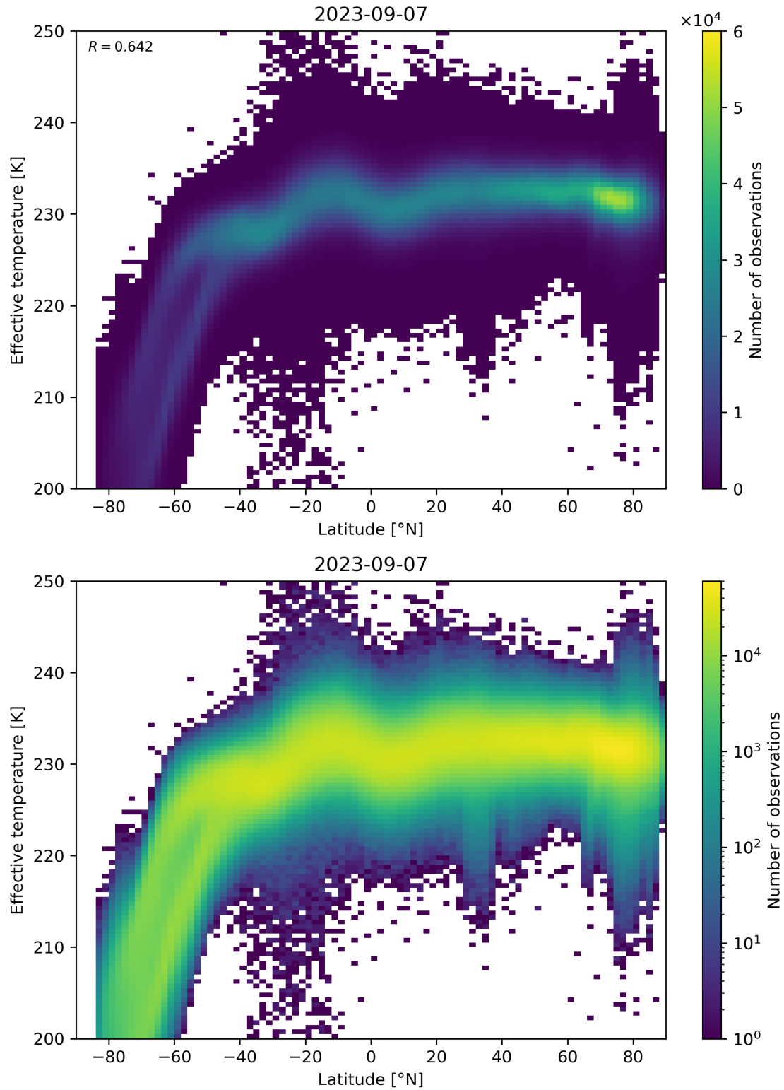
Figure 34: Scatter density plot of “Latitude” against “Effective temperature” for 2023-09-06 to 2023-09-08.
