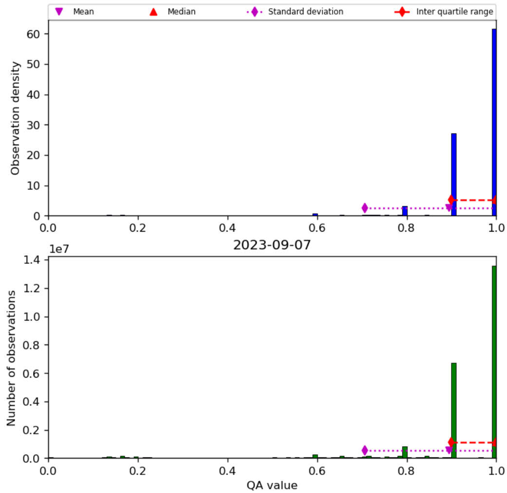
Figure 20: Histogram of “QA value” for 2023-09-06 to 2023-09-08
