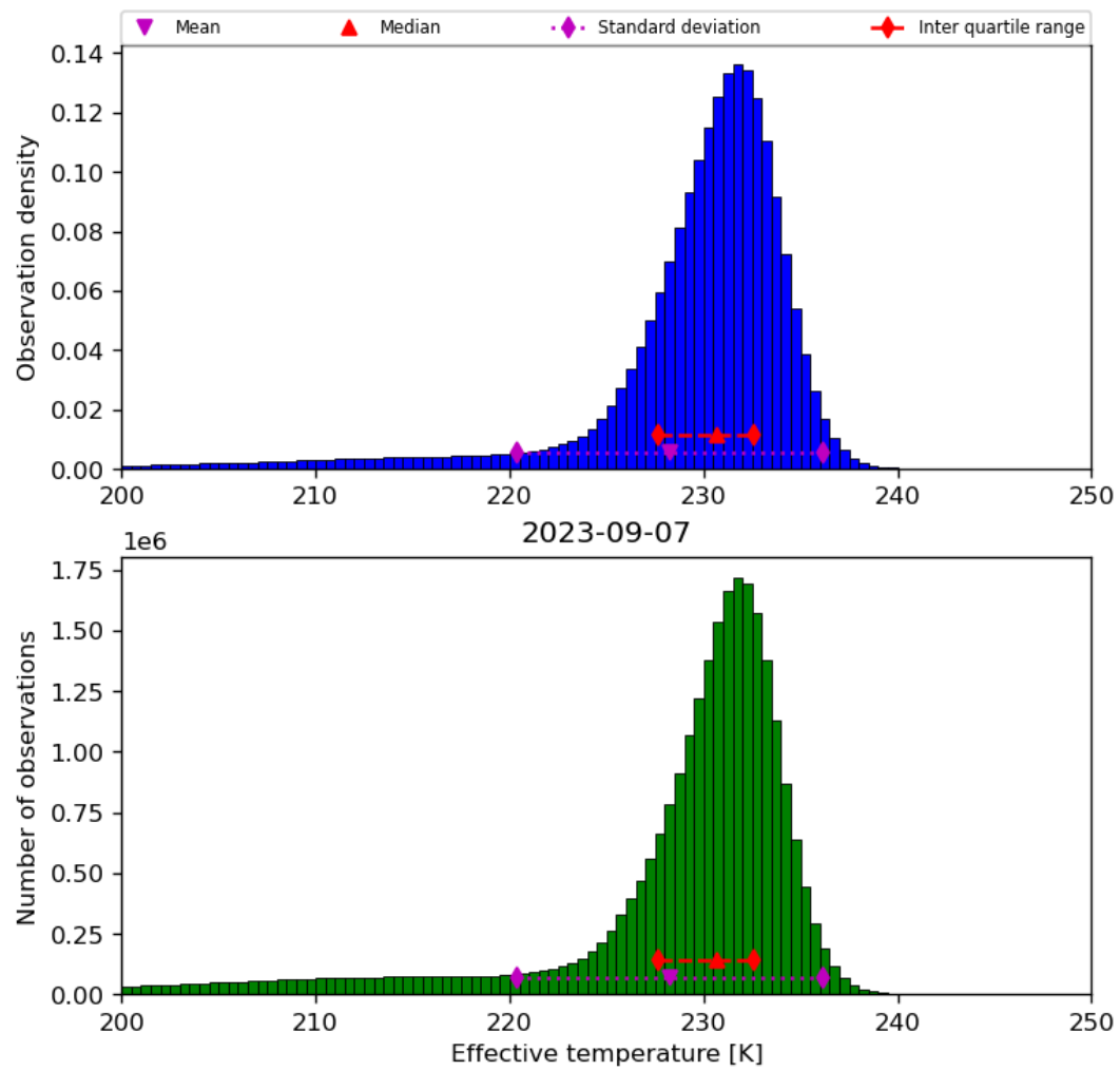
Figure 24: Histogram of “Effective temperature” for 2023-09-06 to 2023-09-08
