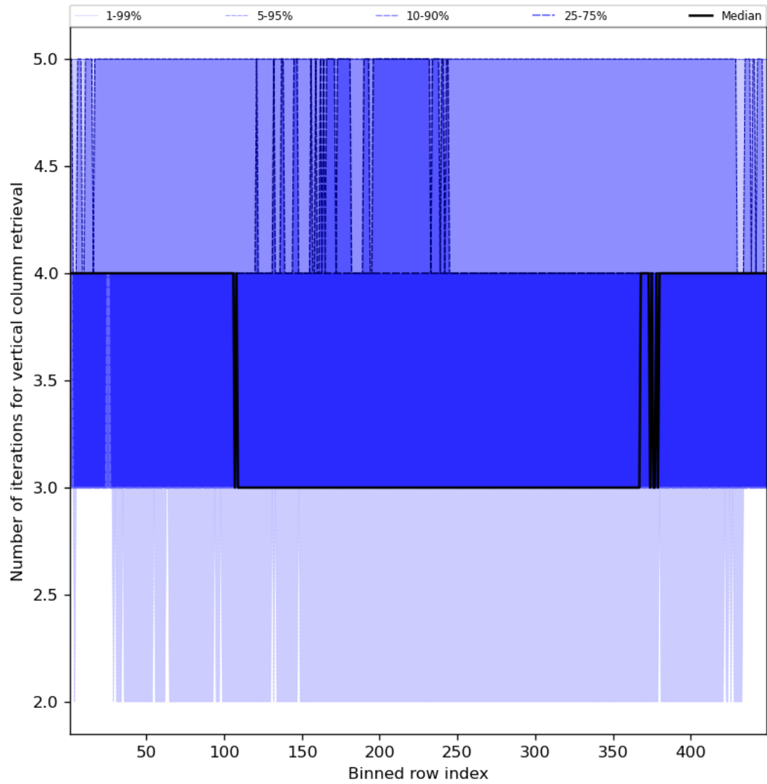
Figure 33: Along track statistics of “Number of iterations for vertical column retrieval” for 2023-09-06 to 2023-09-08
