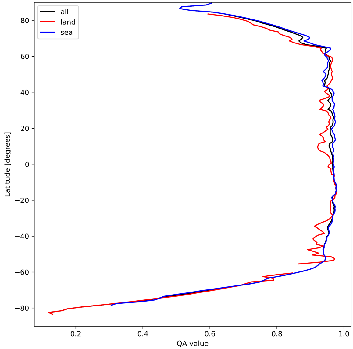
Figure 13: Zonal average of “QA value” for 2023-09-06 to 2023-09-08.
