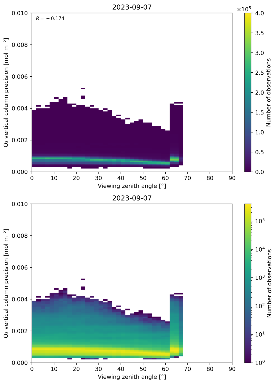
Figure 53: Scatter density plot of “Viewing zenith angle” against “O 3 vertical column precision” for 2023-09-06 to 2023-09-08.
