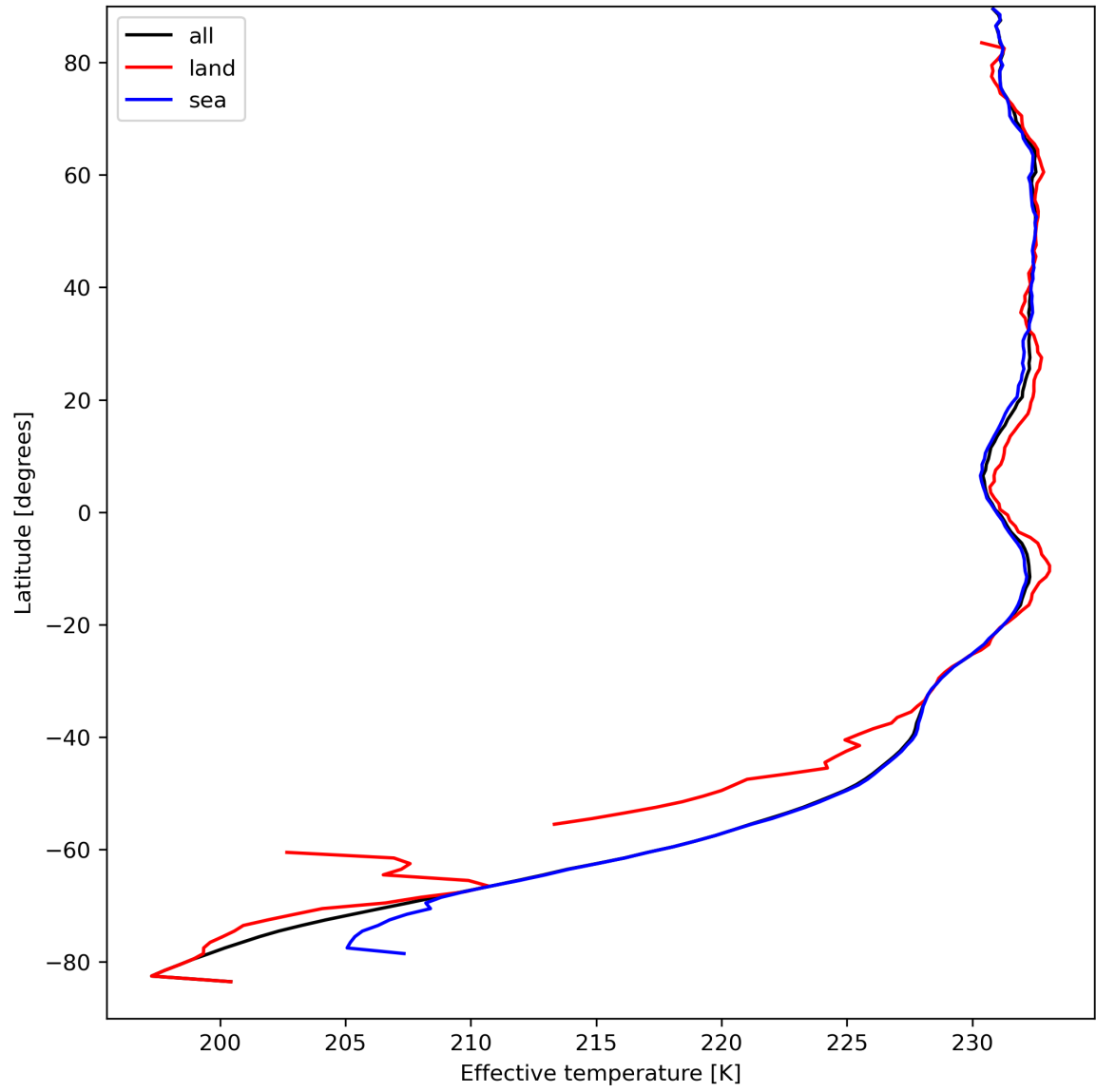
Figure 17: Zonal average of "Effective temperature" for 2023-09-06 to 2023-09-08.
