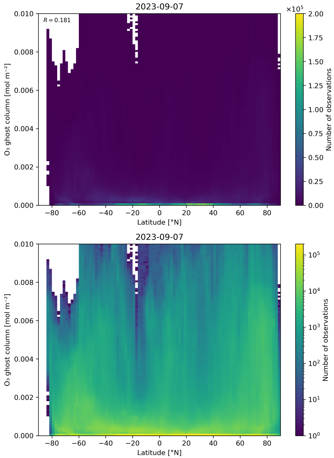
Figure 35: Scatter density plot of “Latitude” against “O 3 ghost column” for 2023-09-06 to 2023-09-08.
