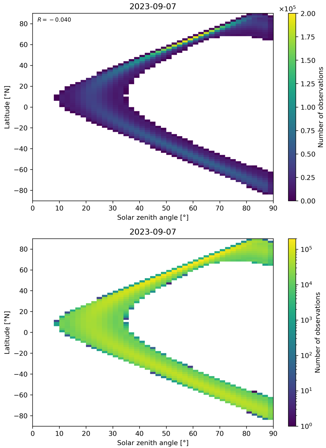
Figure 44: Scatter density plot of “Solar zenith angle” against “Latitude” for 2023-09-06 to 2023-09-08.
