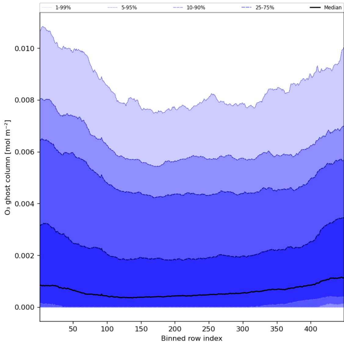
Figure 32: Along track statistics of "O 3 ghost column" for 2023-09-06 to 2023-09-08
