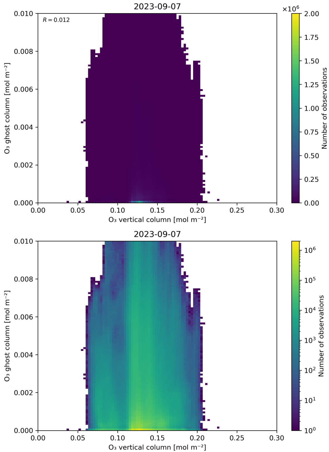
Figure 40: Scatter density plot of “O 3 vertical column” against “O 3 ghost column” for 2023-09-06 to 2023-09-08.
