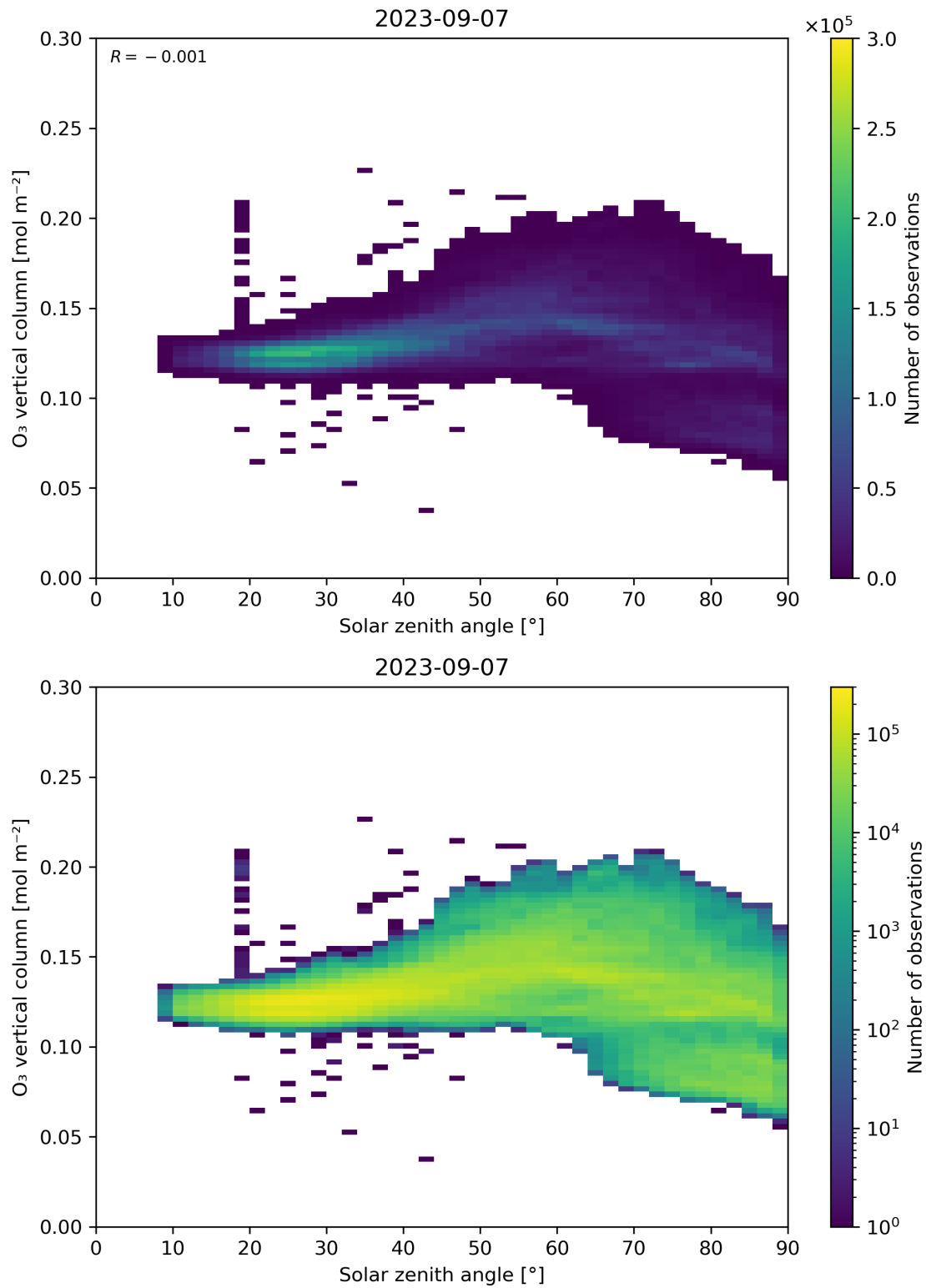
Figure 47: Scatter density plot of “Solar zenith angle” against “O 3 vertical column” for 2023-09-06 to 2023-09-08.
