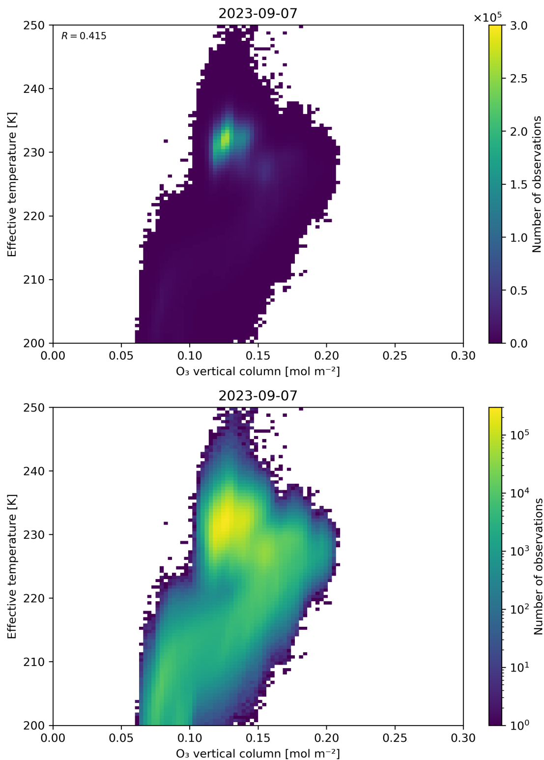
Figure 39: Scatter density plot of “O 3 vertical column” against “Effective temperature” for 2023-09-06 to 2023-09-08.
