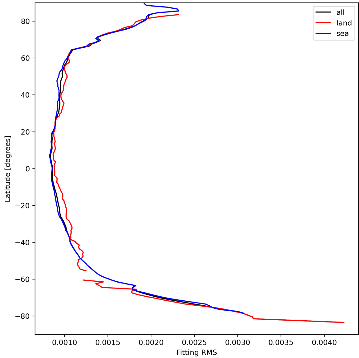
Figure 16: Zonal average of “Fitting RMS” for 2023-09-06 to 2023-09-08.
