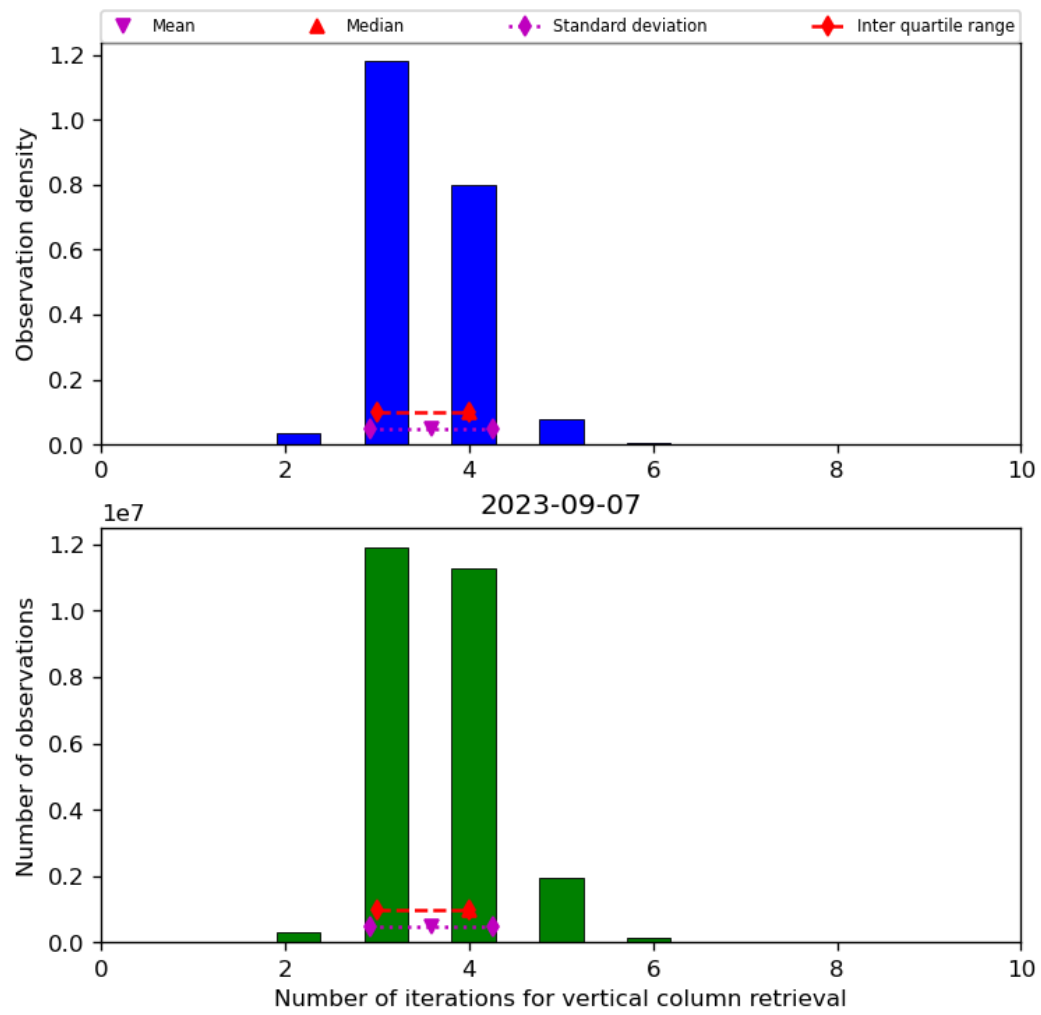
Figure 26: Histogram of “Number of iterations for vertical column retrieval” for 2023-09-06 to 2023-09-08
