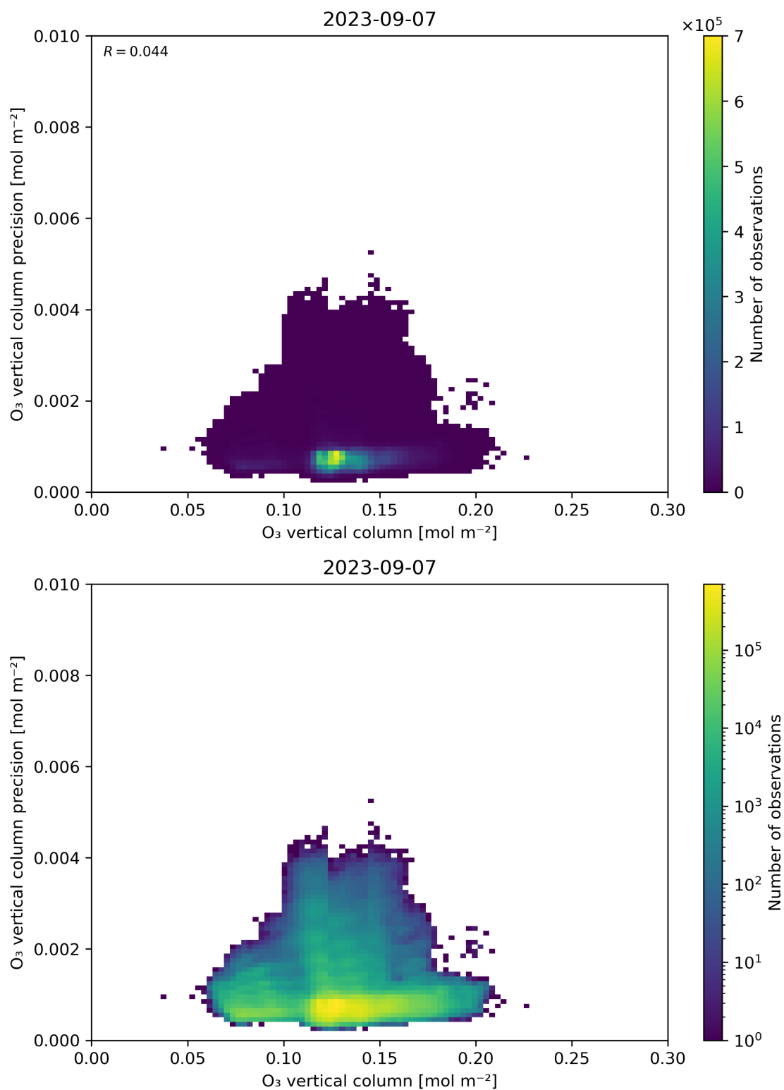
Figure 41: Scatter density plot of “O 3 vertical column” against “O 3 vertical column precision” for 2023-09-06 to 2023-09-08.
