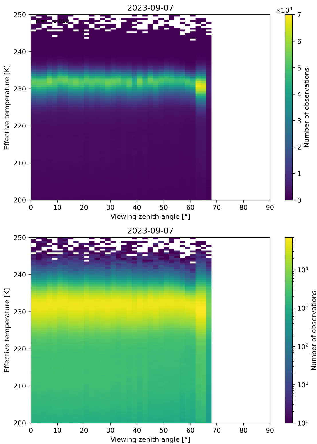
Figure 50: Scatter density plot of “Viewing zenith angle” against “Effective temperature” for 2023-09-06 to 2023-09-08.
