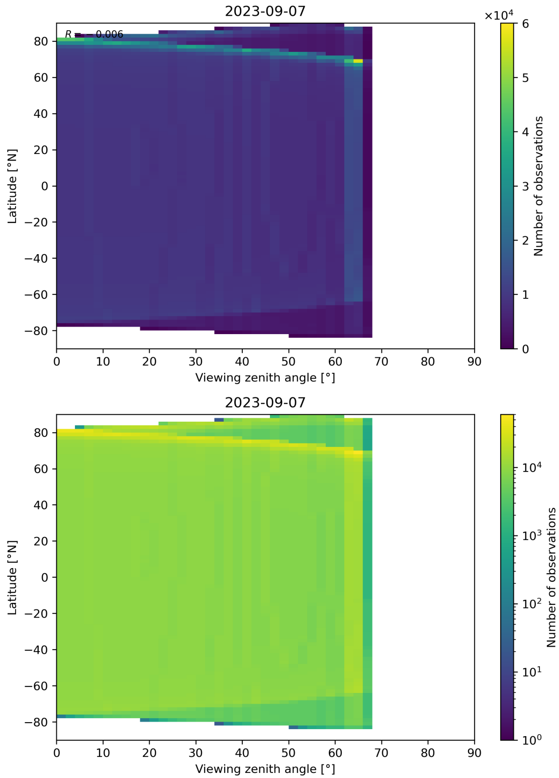
Figure 49: Scatter density plot of “Viewing zenith angle” against “Latitude” for 2023-09-06 to 2023-09-08.
