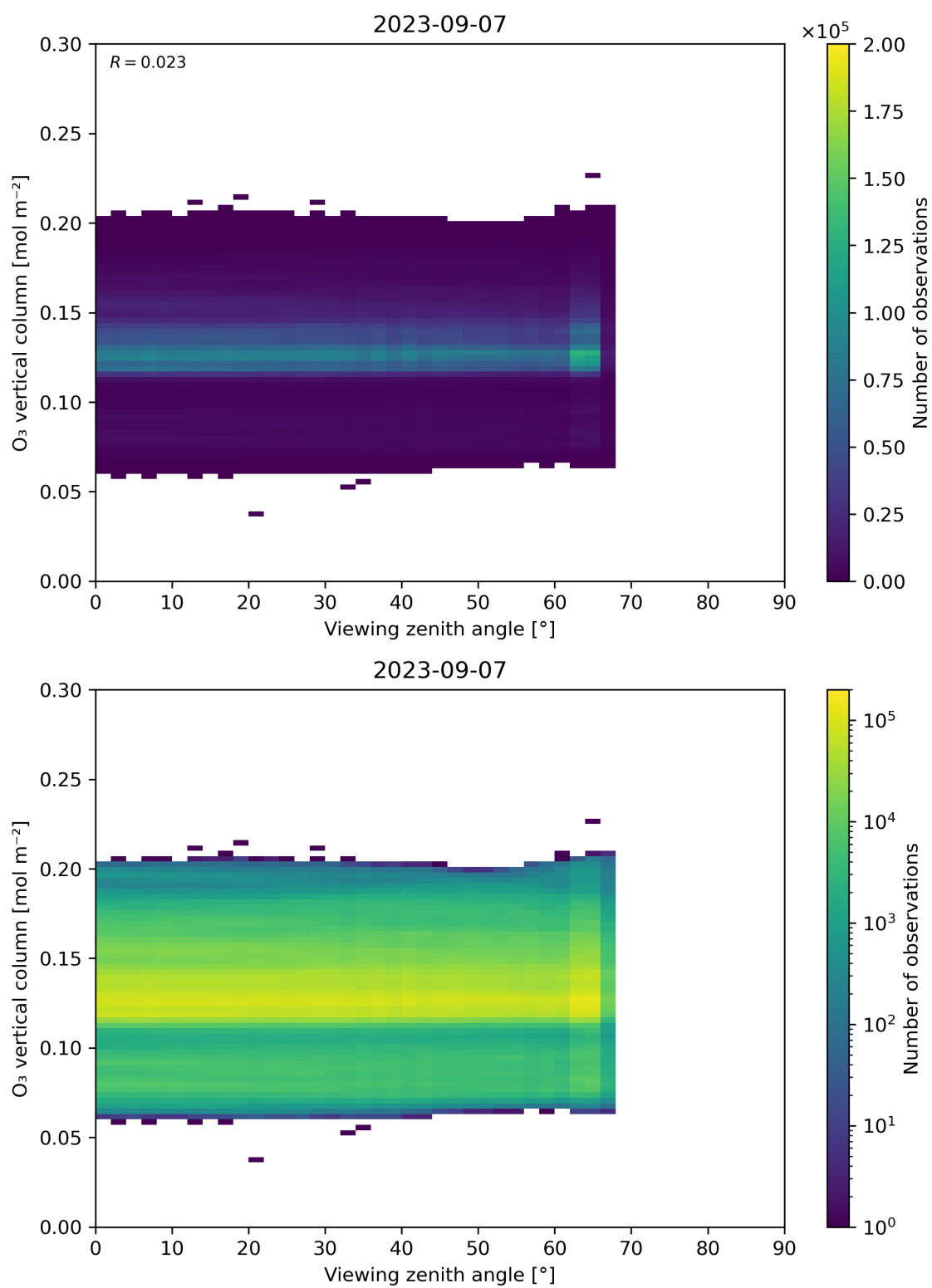
Figure 52: Scatter density plot of “Viewing zenith angle” against “O 3 vertical column” for 2023-09-06 to 2023-09-08.
