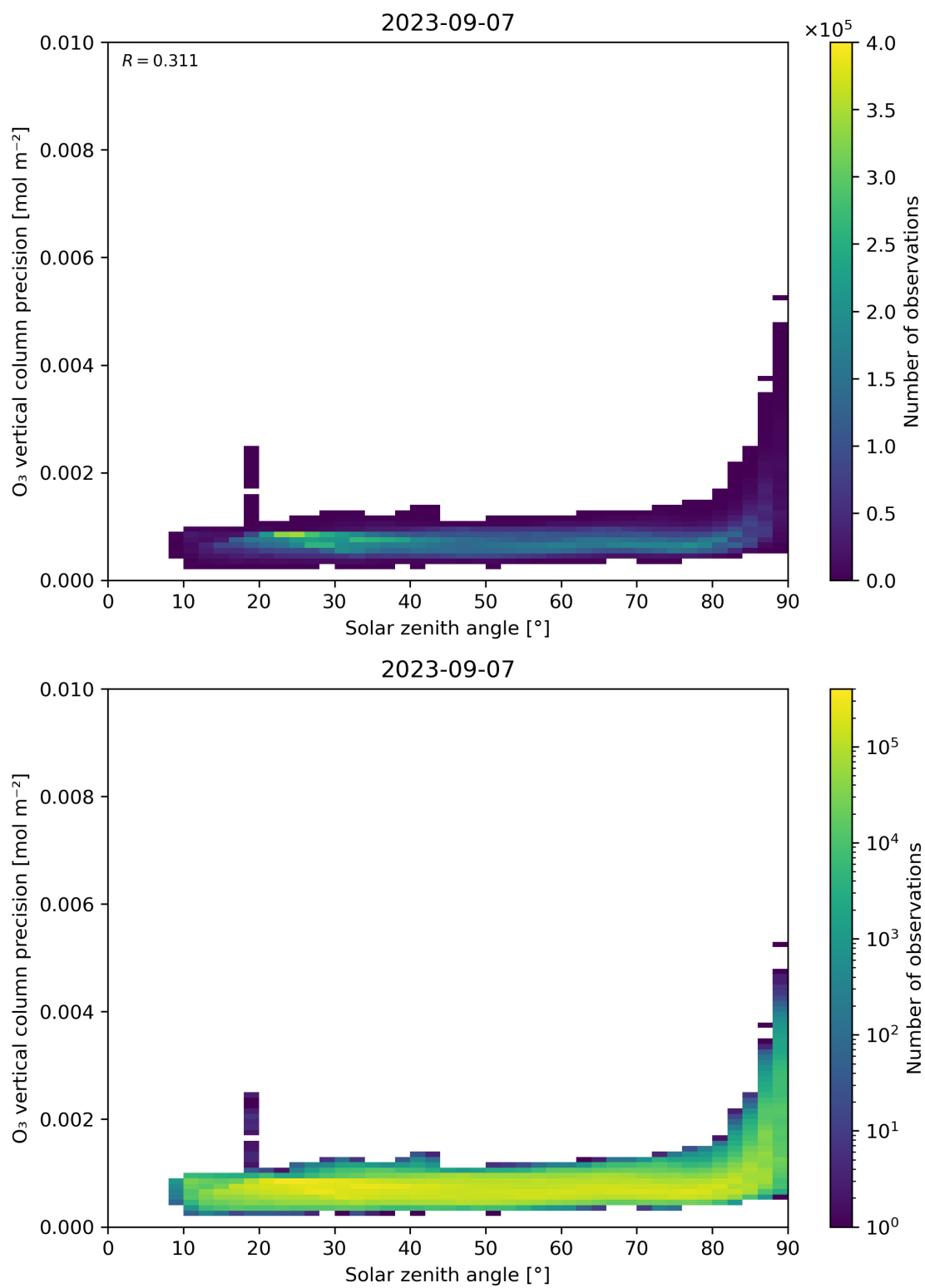
Figure 48: Scatter density plot of “Solar zenith angle” against “O 3 vertical column precision” for 2023-09-06 to 2023-09-08.
