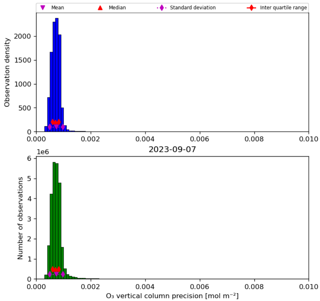
Figure 22: Histogram of “O 3 vertical column precision” for 2023-09-06 to 2023-09-08
