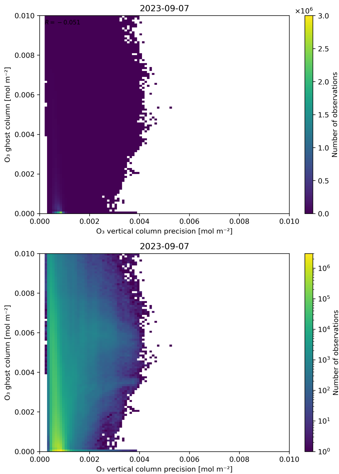
Figure 43: Scatter density plot of “ \text{O}_3 vertical column precision” against “ \text{O}_3 ghost column” for 2023-09-06 to 2023-09-08.
