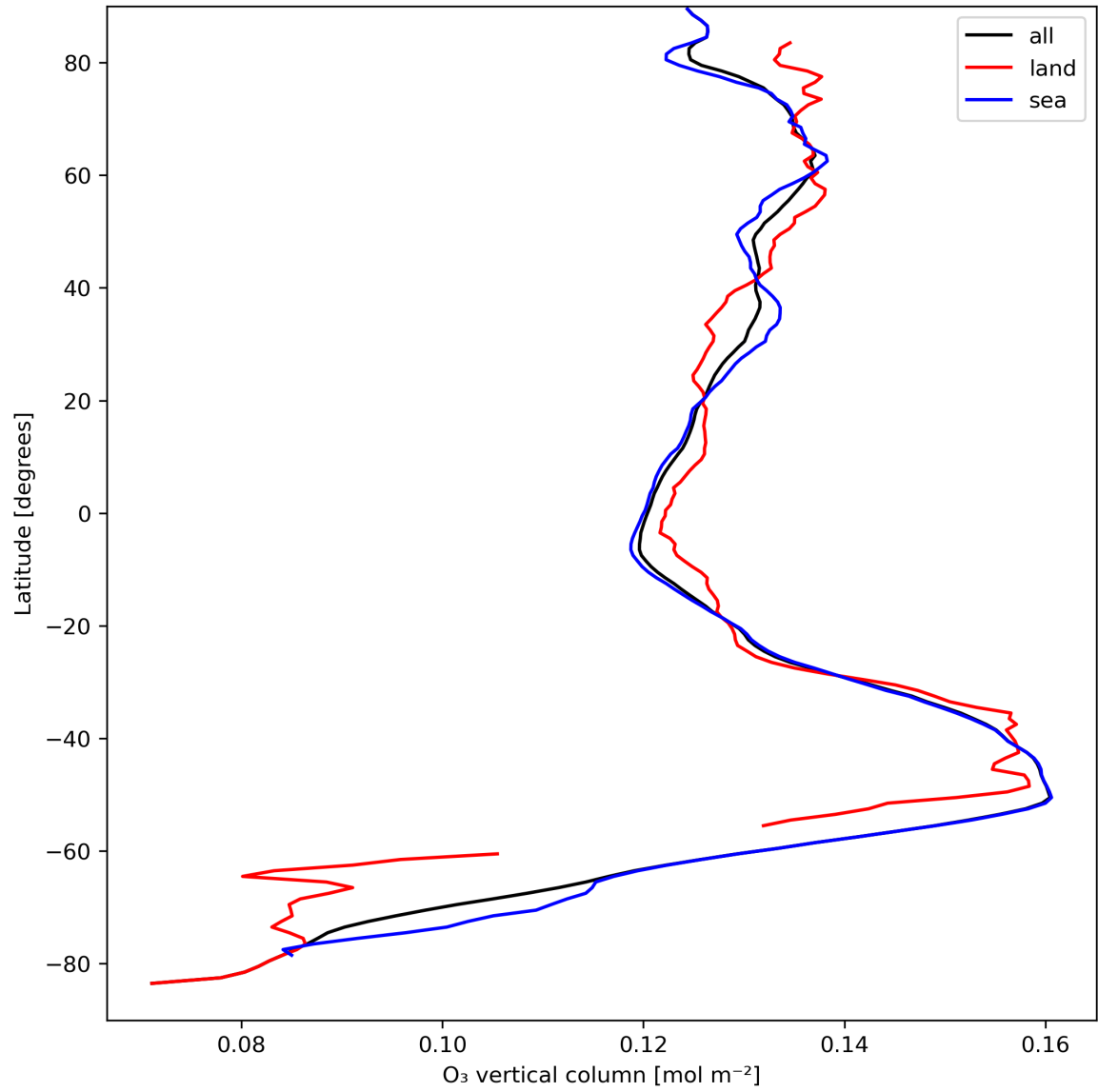
Figure 14: Zonal average of “O 3 vertical column” for 2023-09-06 to 2023-09-08.
