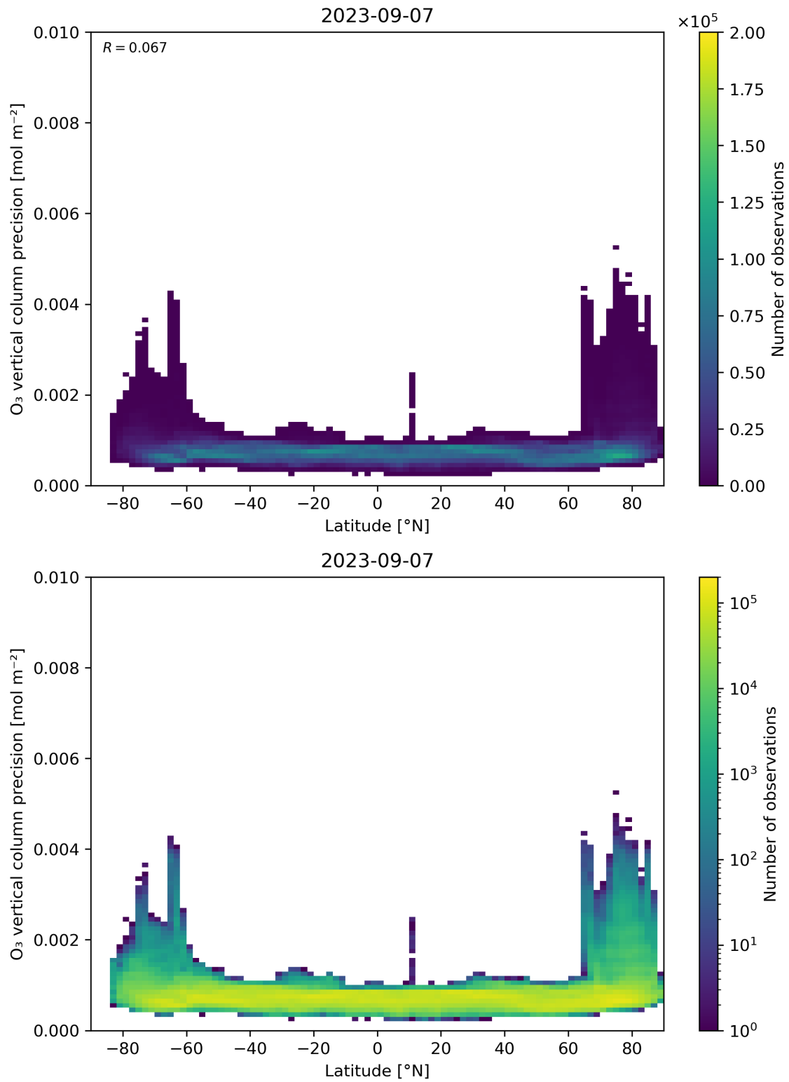
Figure 37: Scatter density plot of “Latitude” against “O 3 vertical column precision” for 2023-09-06 to 2023-09-08.
