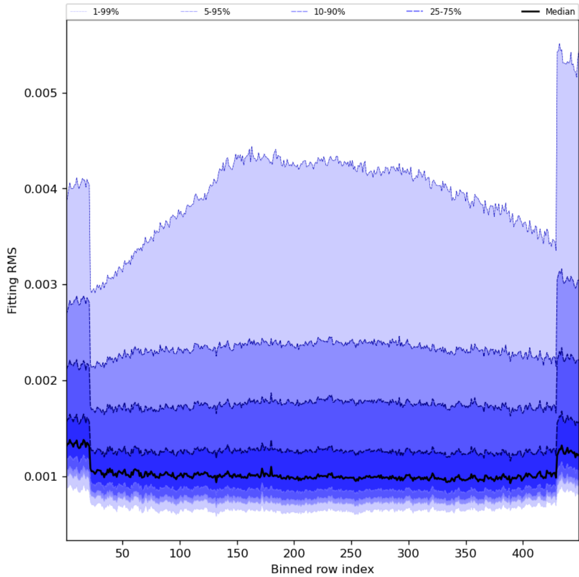
Figure 30: Along track statistics of “Fitting RMS” for 2023-09-06 to 2023-09-08
