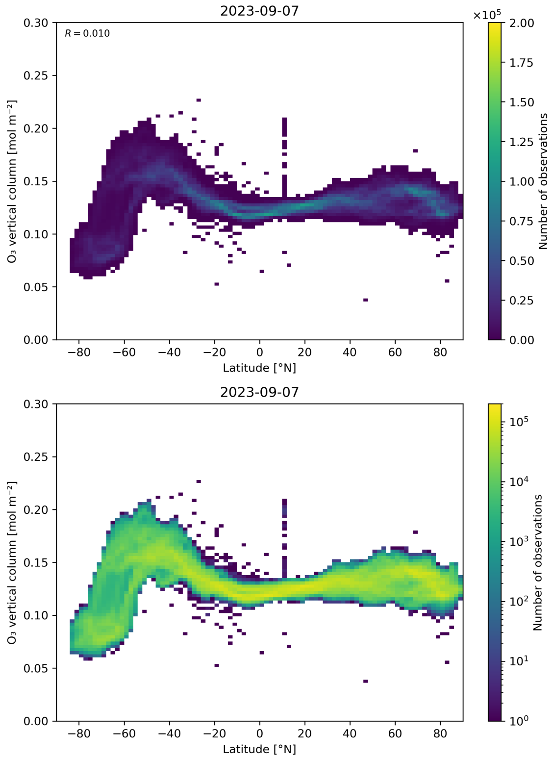
Figure 36: Scatter density plot of “Latitude” against “O 3 vertical column” for 2023-09-06 to 2023-09-08.
