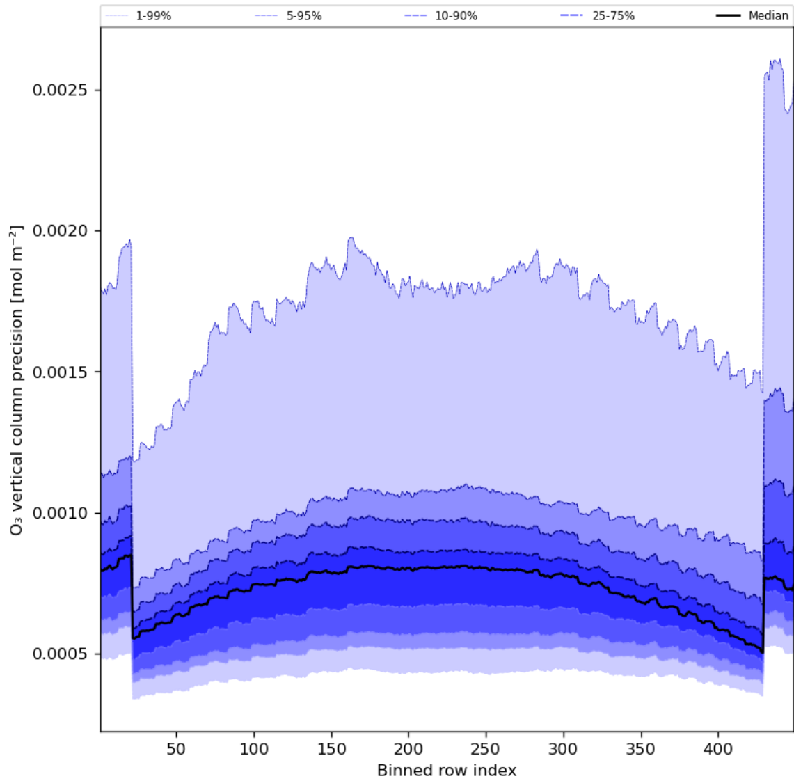
Figure 29: Along track statistics of “O 3 vertical column precision” for 2023-09-06 to 2023-09-08
