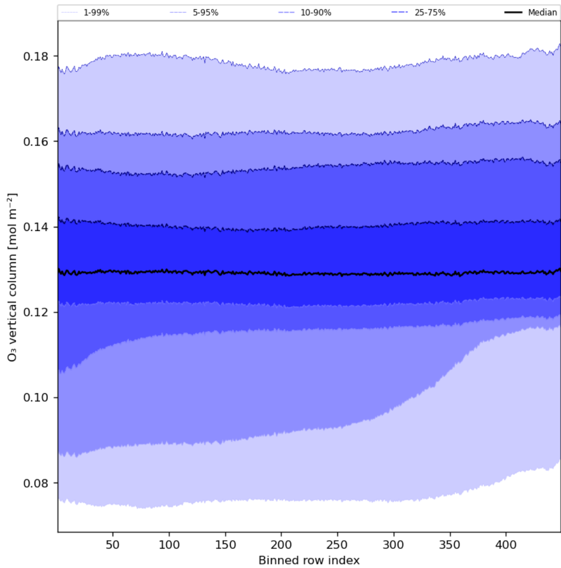
Figure 28: Along track statistics of “O 3 vertical column” for 2023-09-06 to 2023-09-08
