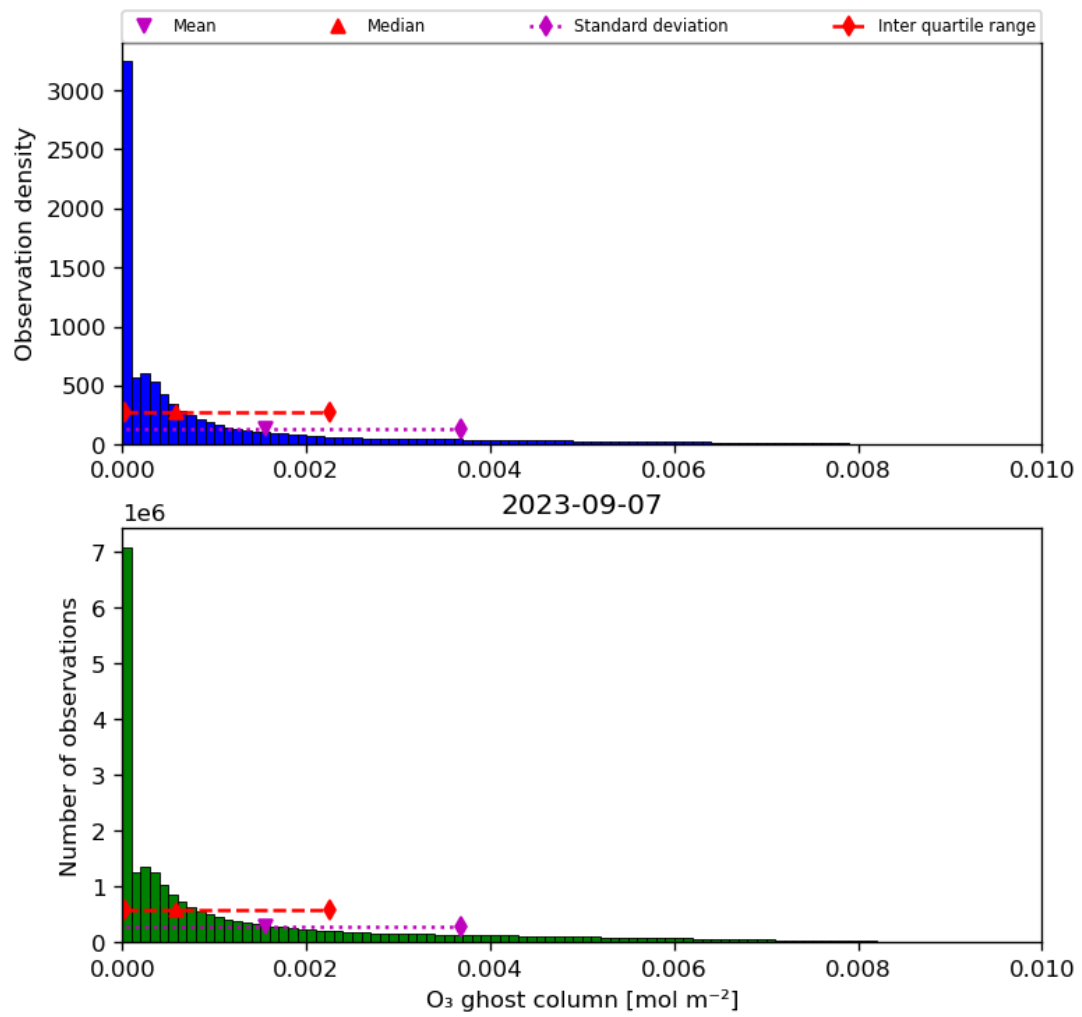
Figure 25: Histogram of “O 3 ghost column” for 2023-09-06 to 2023-09-08
