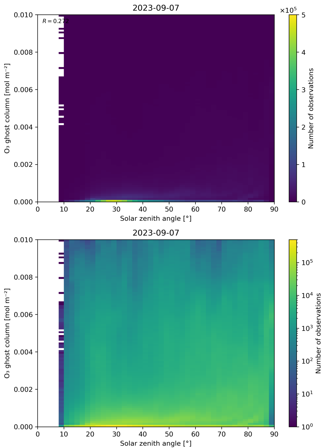
Figure 46: Scatter density plot of “Solar zenith angle” against “O 3 ghost column” for 2023-09-06 to 2023-09-08.
