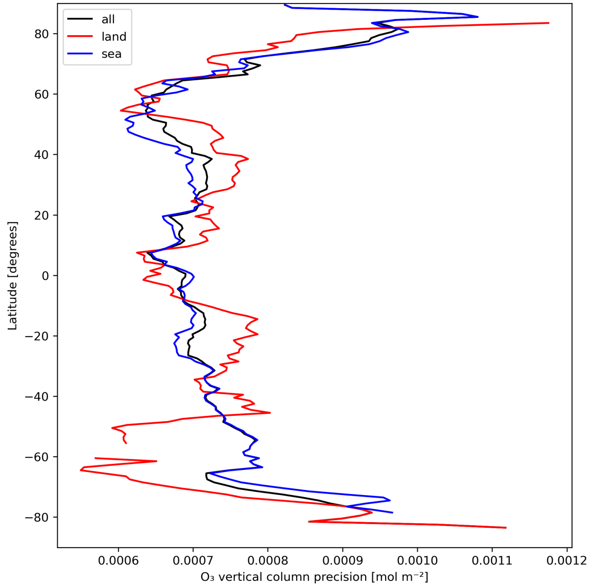
Figure 15: Zonal average of “O 3 vertical column precision” for 2023-09-06 to 2023-09-08.
