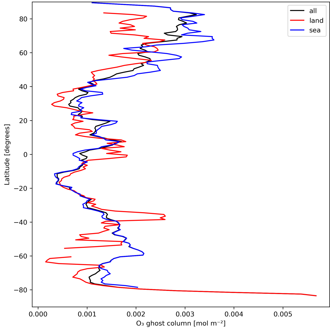
Figure 18: Zonal average of "O 3 ghost column" for 2023-09-06 to 2023-09-08.
