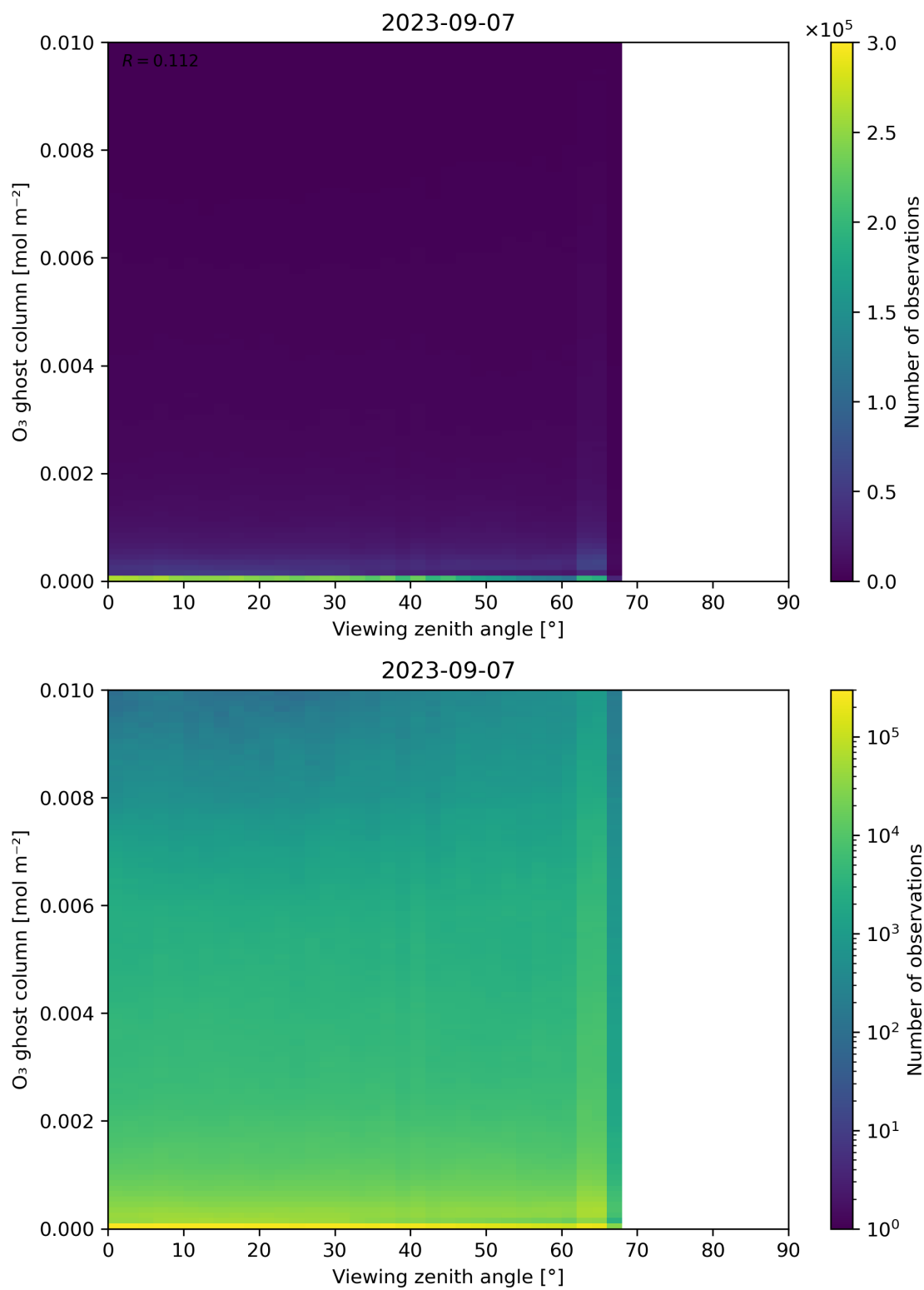
Figure 51: Scatter density plot of “Viewing zenith angle” against “O 3 ghost column” for 2023-09-06 to 2023-09-08.
