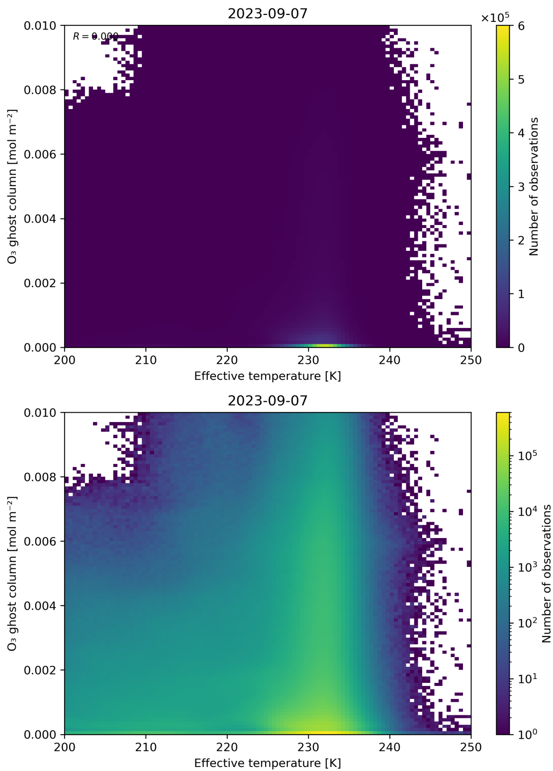
Figure 38: Scatter density plot of “Effective temperature” against “O 3 ghost column” for 2023-09-06 to 2023-09-08.
