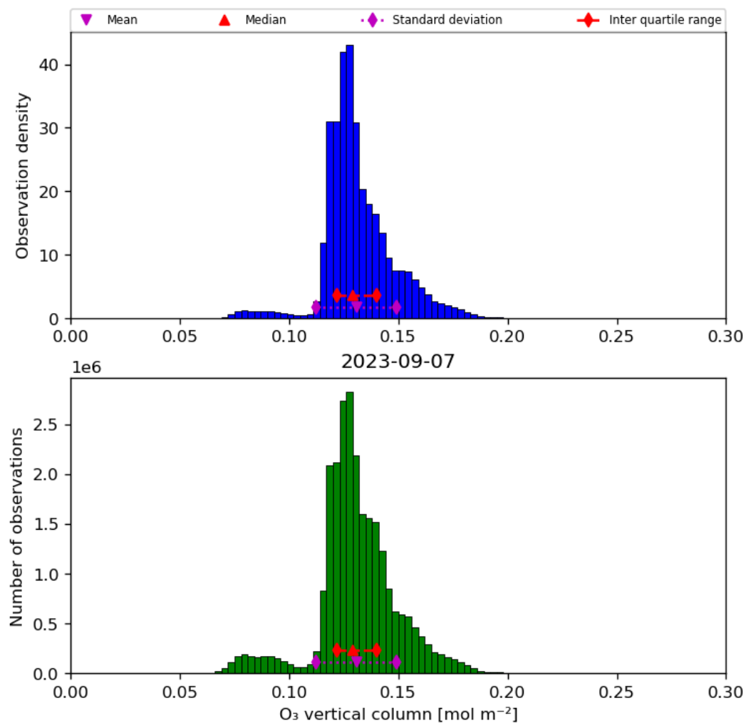
Figure 21: Histogram of “O 3 vertical column” for 2023-09-06 to 2023-09-08
