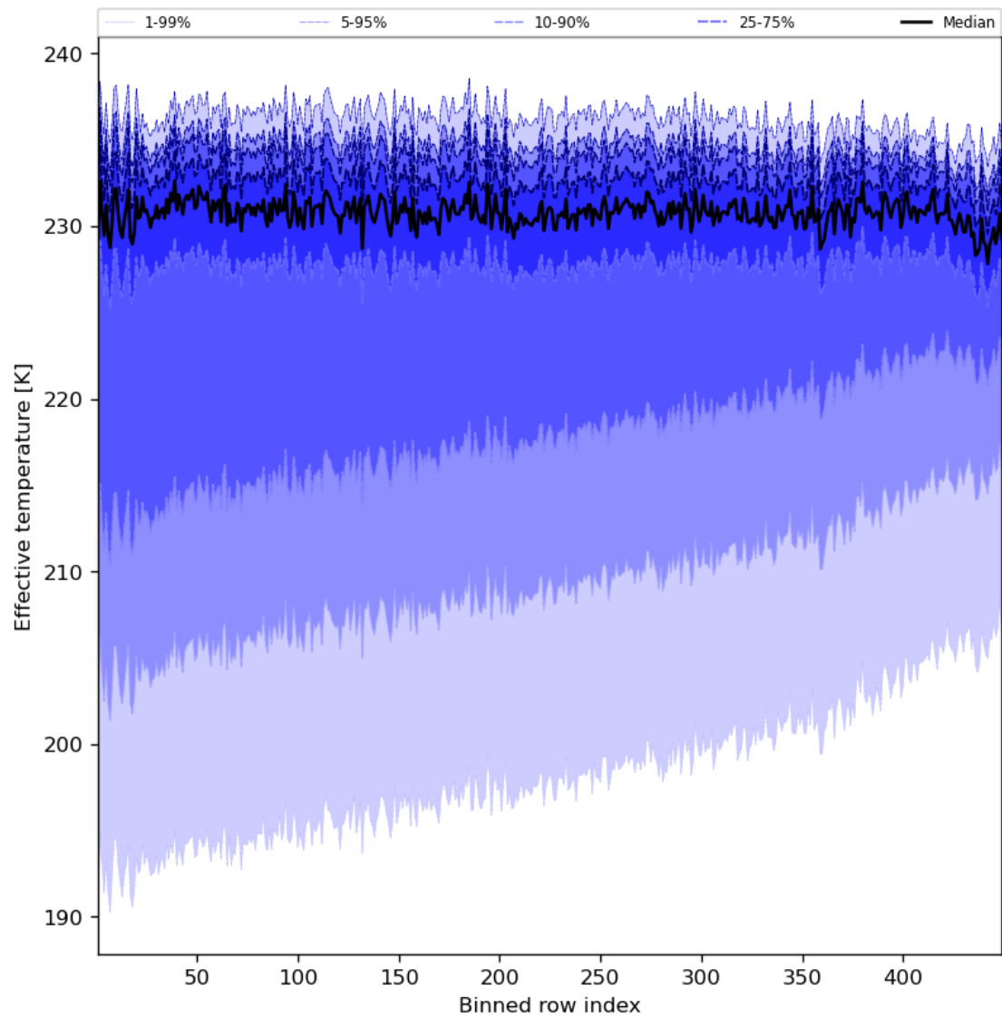
Figure 31: Along track statistics of “Effective temperature” for 2023-09-06 to 2023-09-08
