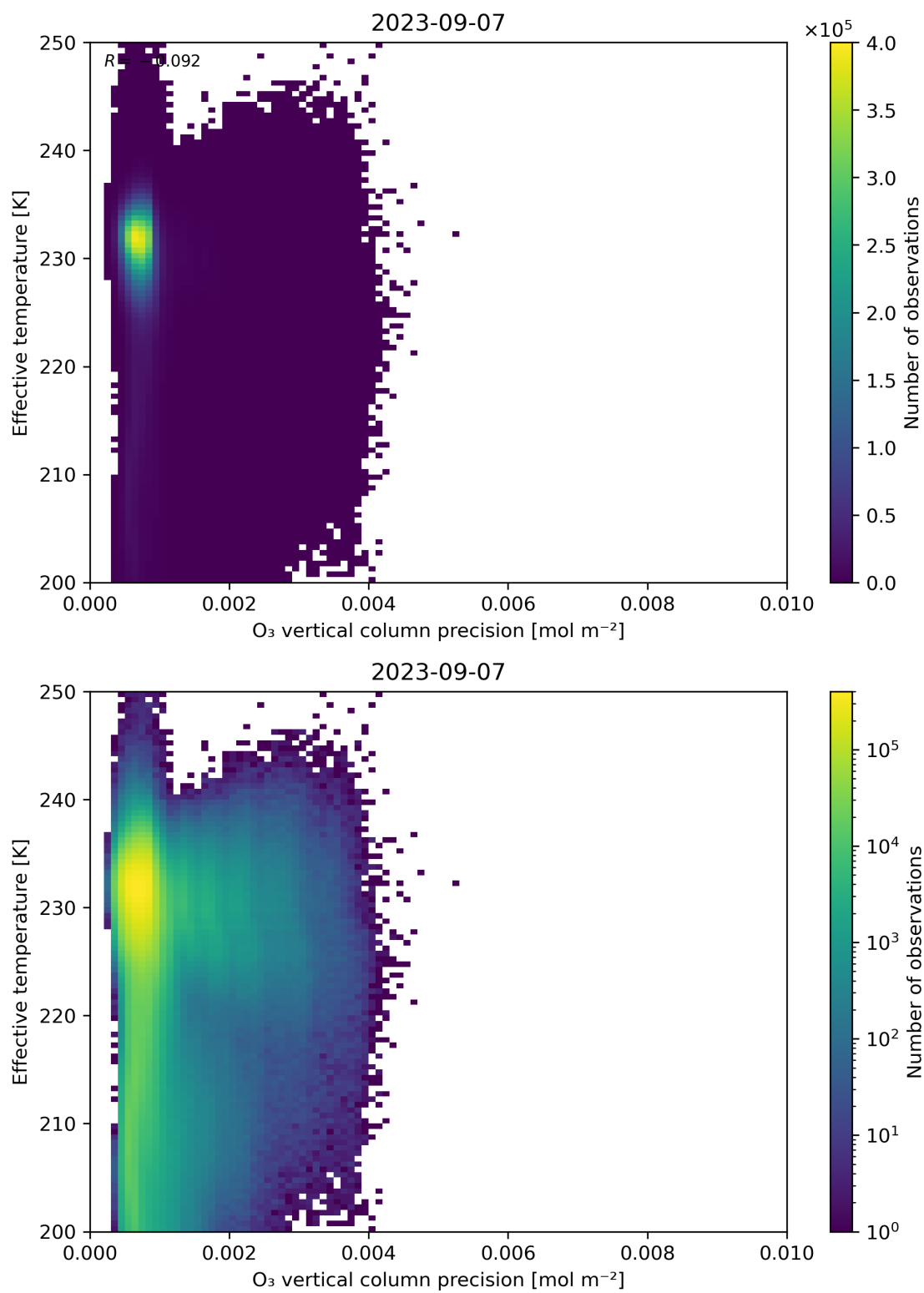
Figure 42: Scatter density plot of “O 3 vertical column precision” against “Effective temperature” for 2023-09-06 to 2023-09-08.
