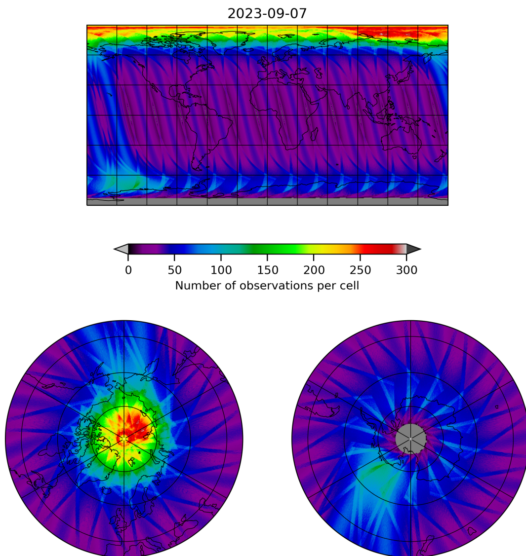
Figure 12: Map of the number of observations for 2023-09-06 to 2023-09-08
