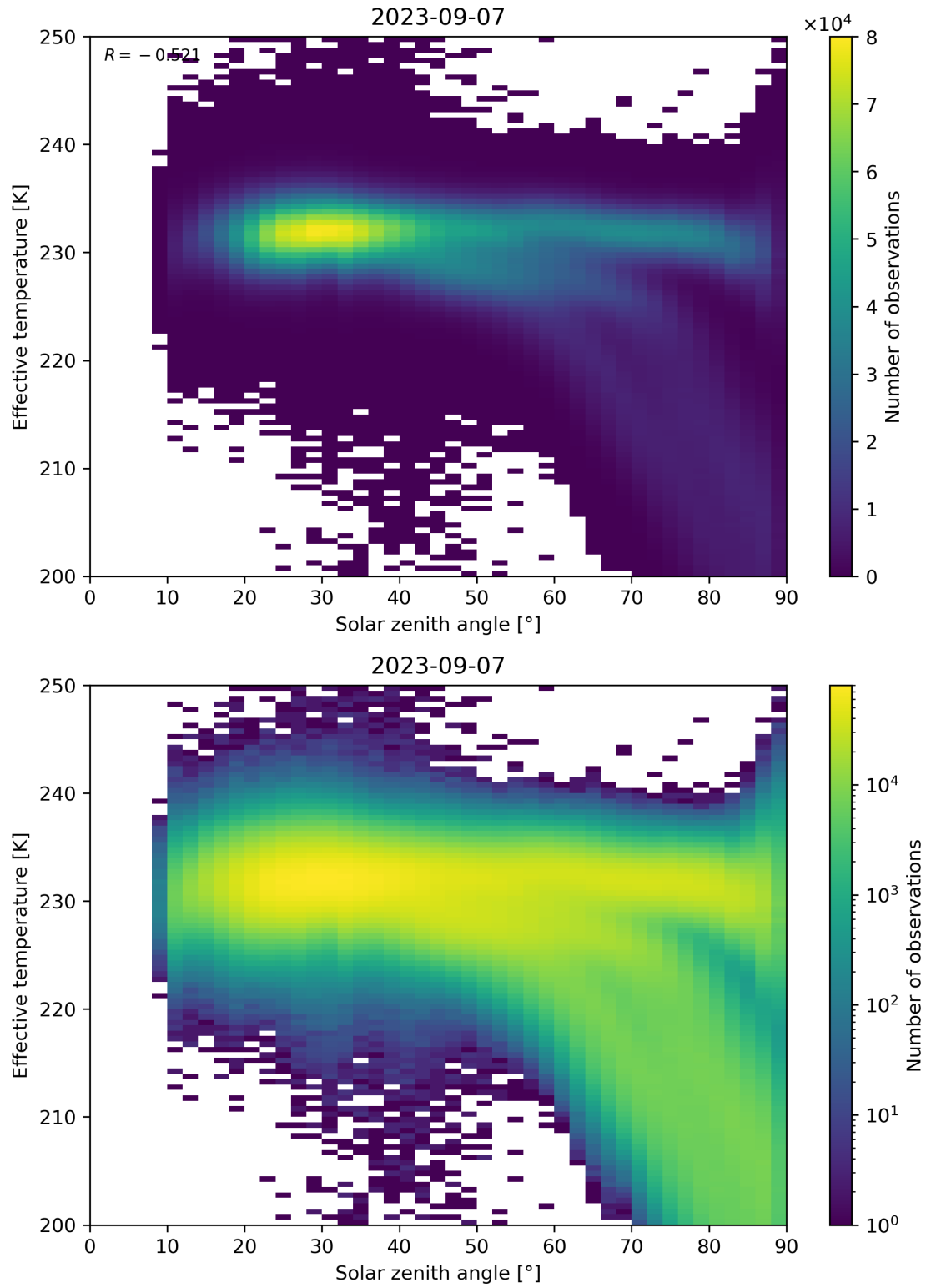
Figure 45: Scatter density plot of “Solar zenith angle” against “Effective temperature” for 2023-09-06 to 2023-09-08.
