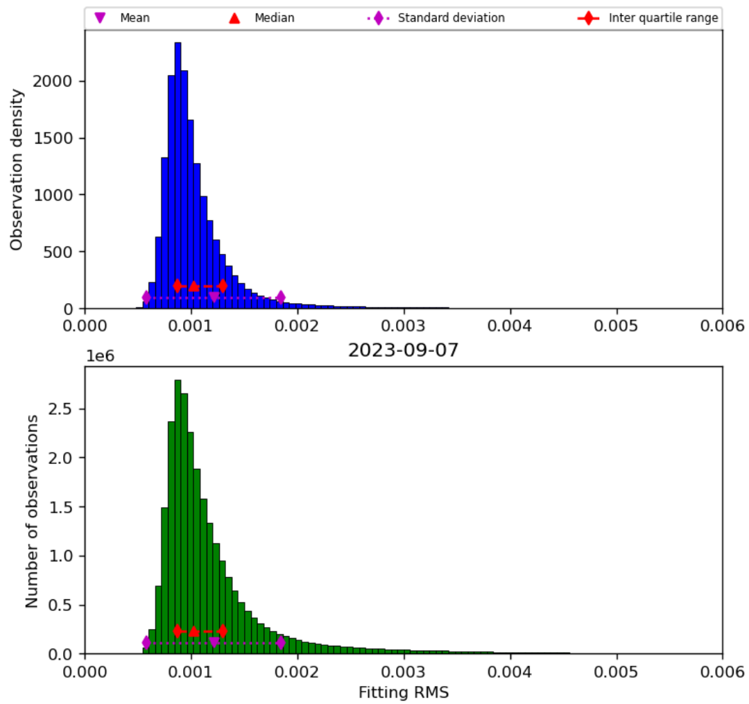
Figure 23: Histogram of “Fitting RMS” for 2023-09-06 to 2023-09-08
