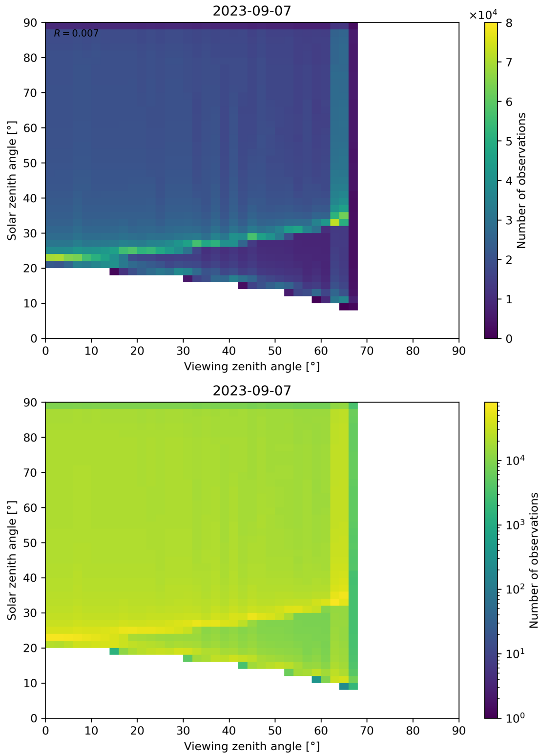
Figure 54: Scatter density plot of “Viewing zenith angle” against “Solar zenith angle” for 2023-09-06 to 2023-09-08.
