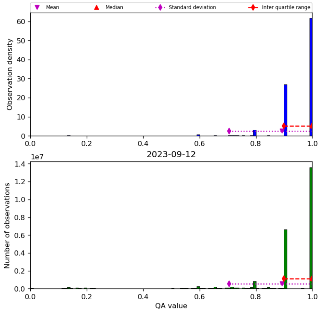
Figure 20: Histogram of “QA value” for 2023-09-11 to 2023-09-13
