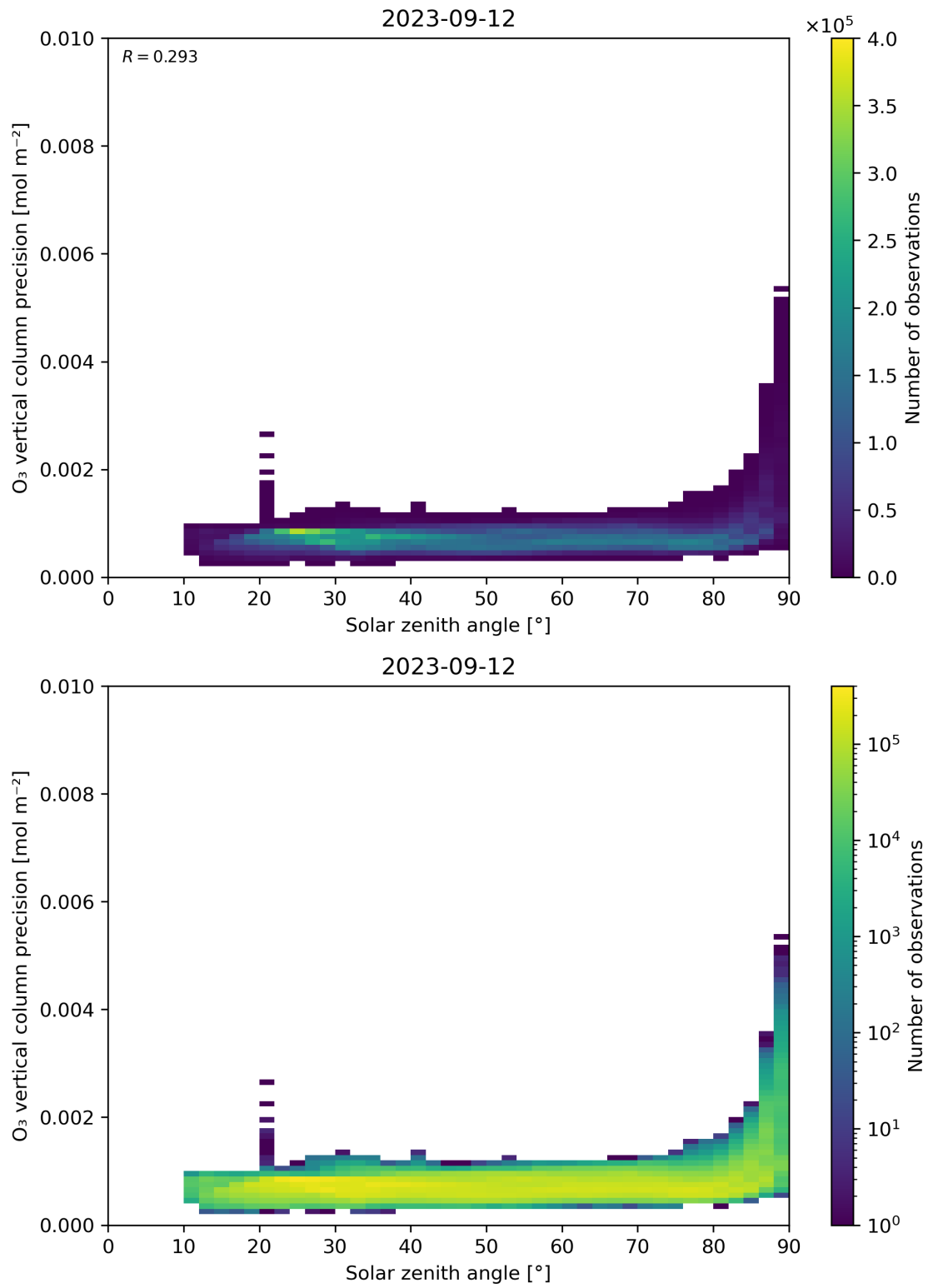
Figure 48: Scatter density plot of “Solar zenith angle” against “O 3 vertical column precision” for 2023-09-11 to 2023-09-13.
