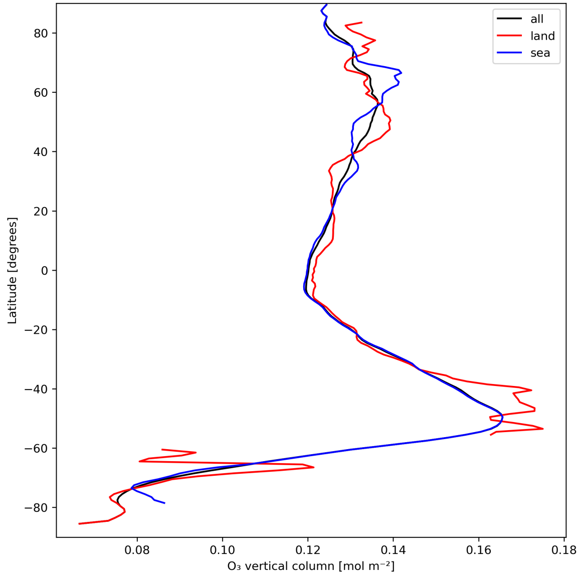
Figure 14: Zonal average of “O 3 vertical column” for 2023-09-11 to 2023-09-13.
