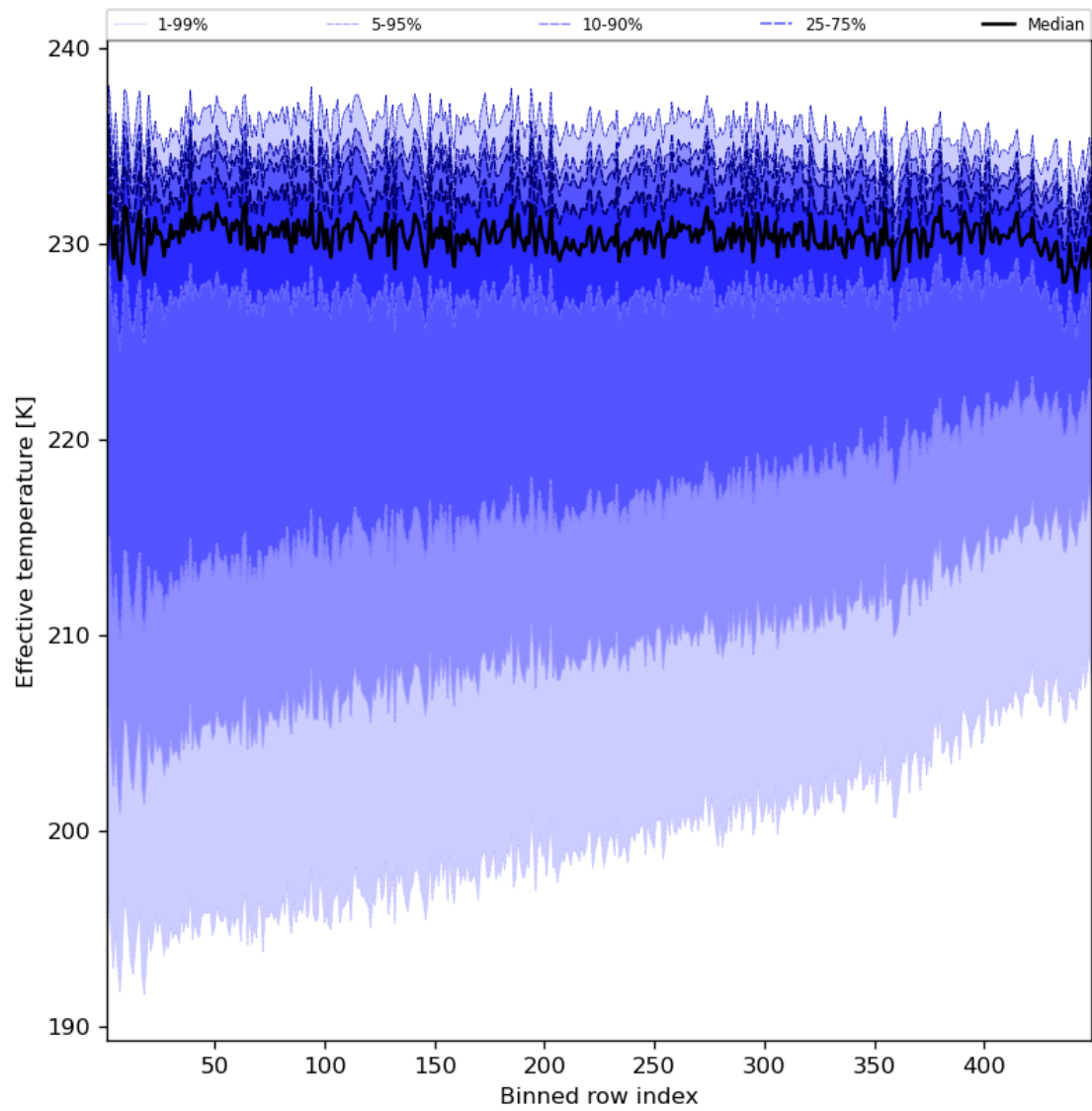
Figure 31: Along track statistics of “Effective temperature” for 2023-09-11 to 2023-09-13
