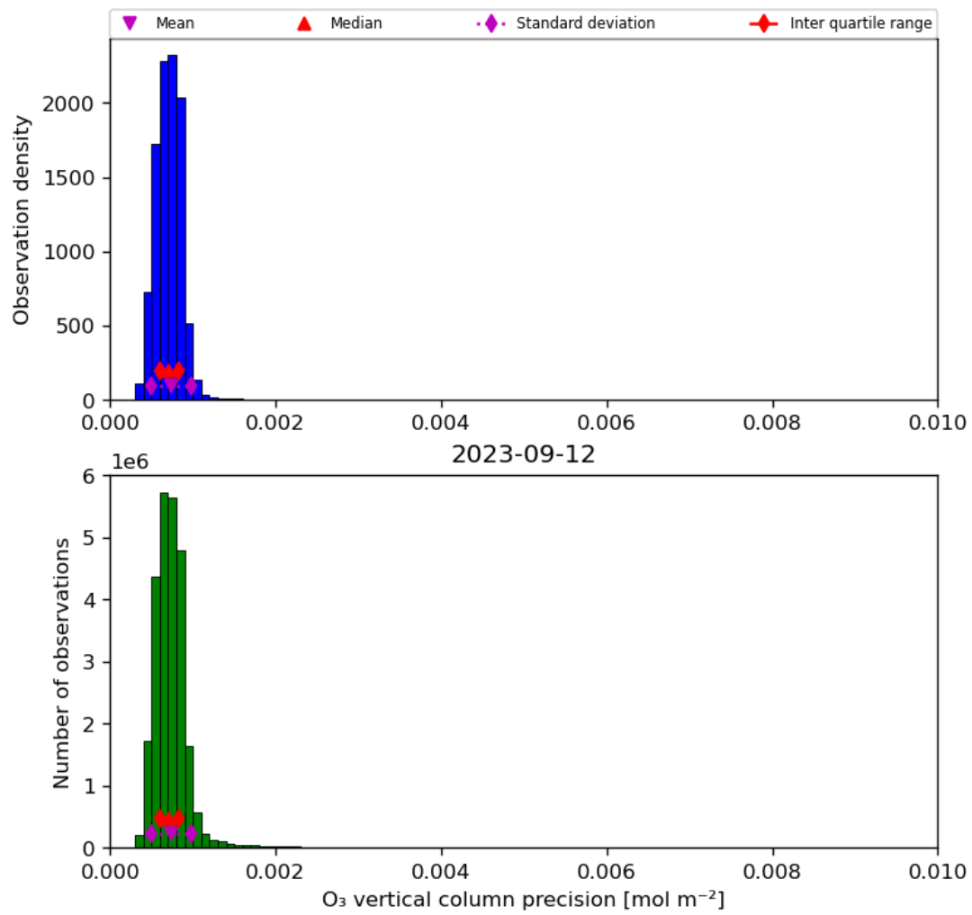
Figure 22: Histogram of “O 3 vertical column precision” for 2023-09-11 to 2023-09-13
