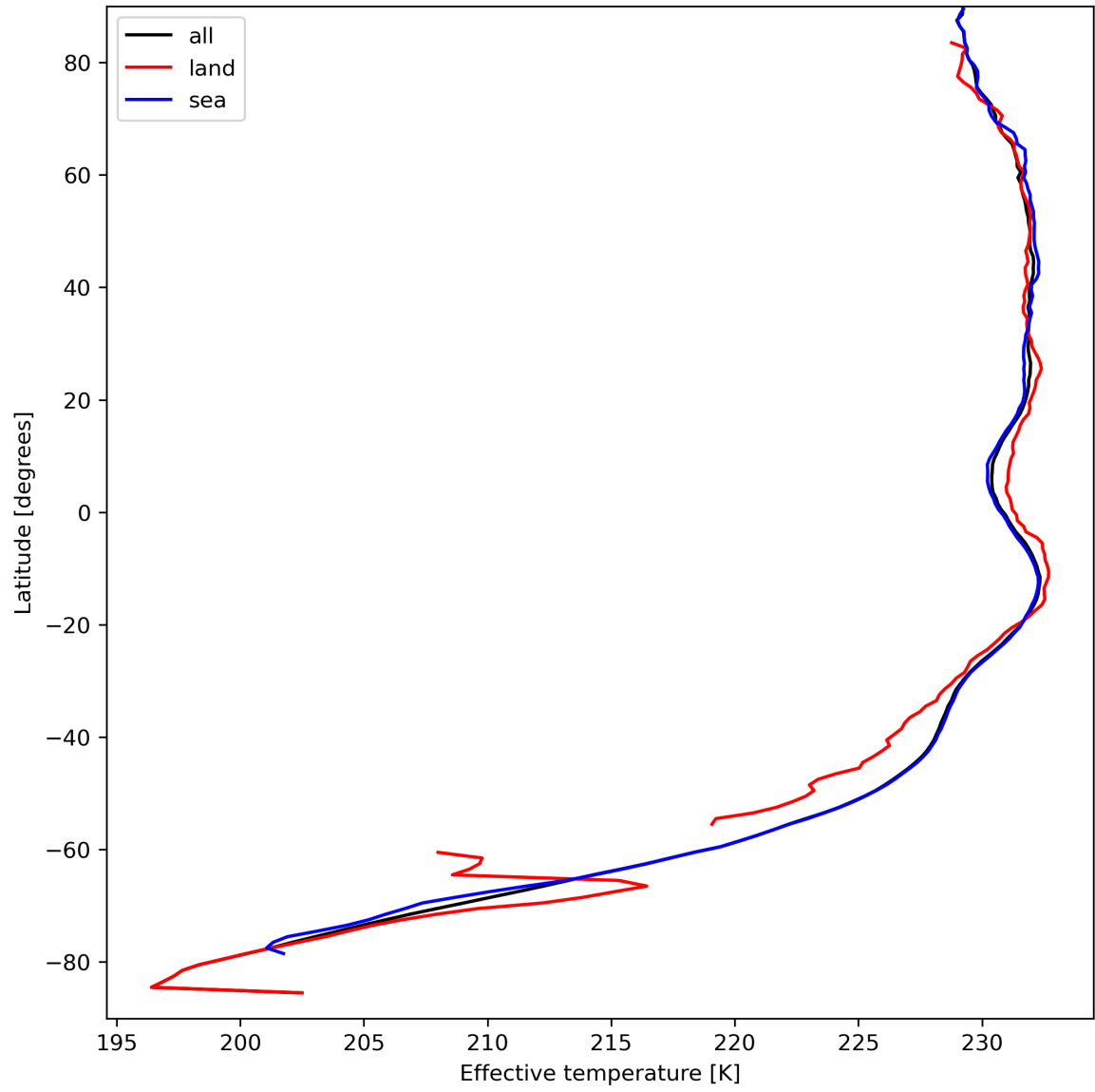
Figure 17: Zonal average of "Effective temperature" for 2023-09-11 to 2023-09-13.
