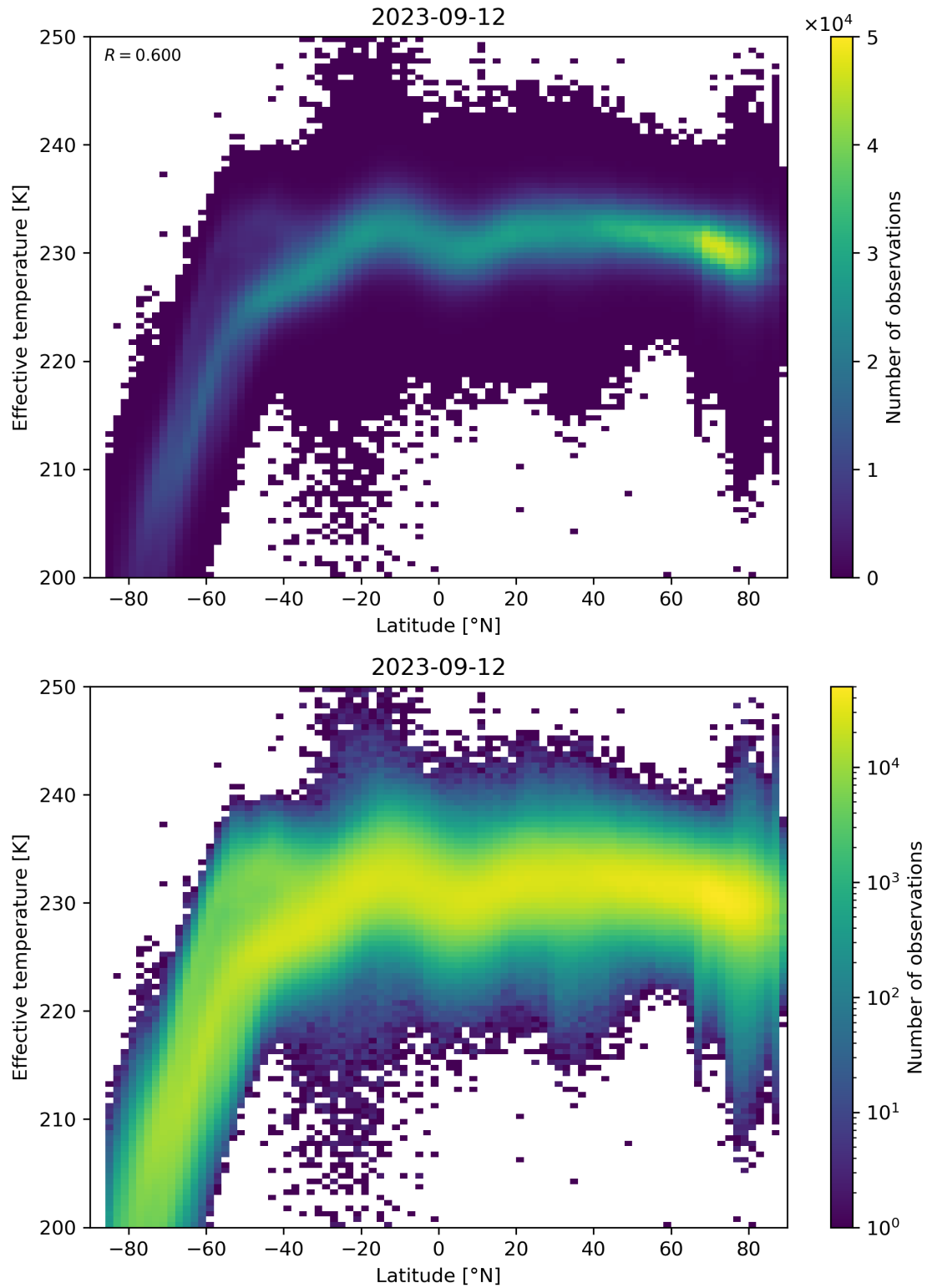
Figure 34: Scatter density plot of “Latitude” against “Effective temperature” for 2023-09-11 to 2023-09-13.
