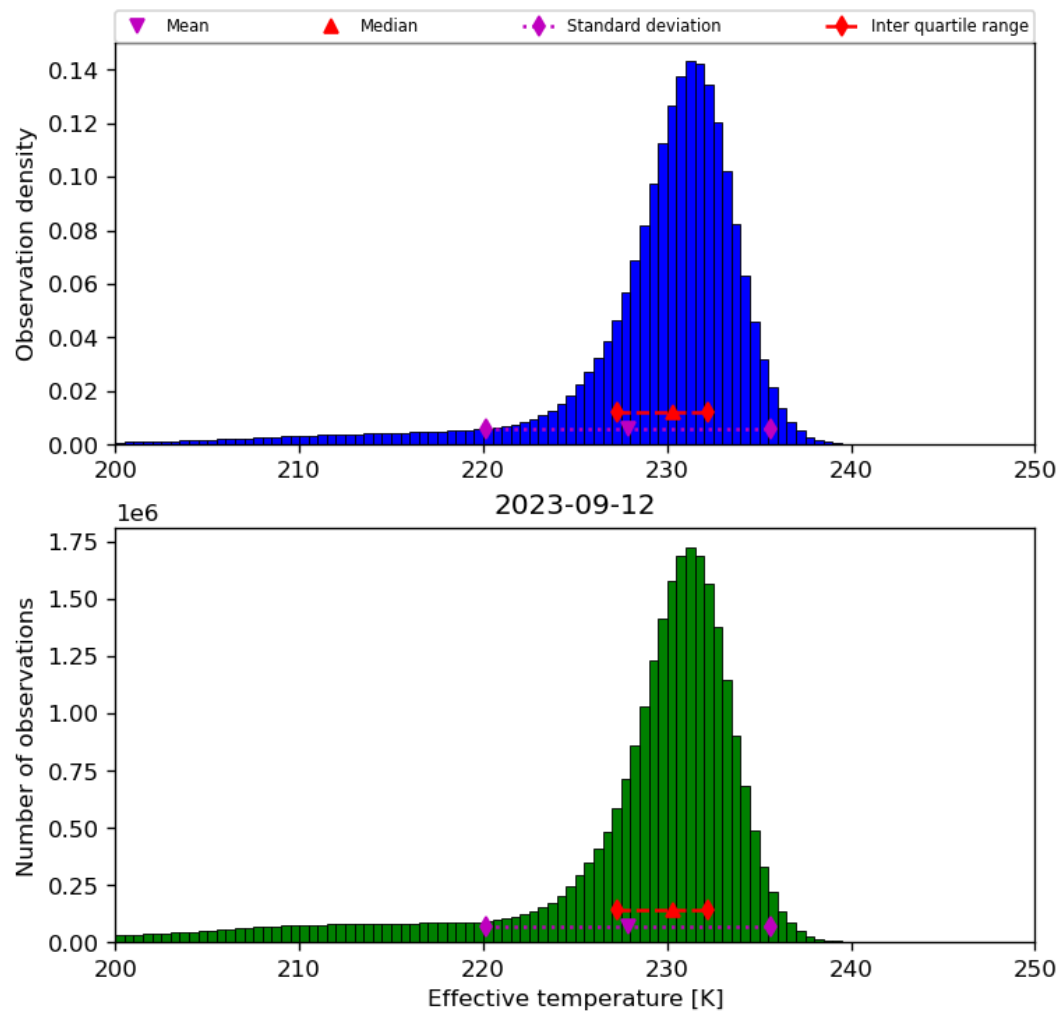
Figure 24: Histogram of “Effective temperature” for 2023-09-11 to 2023-09-13
