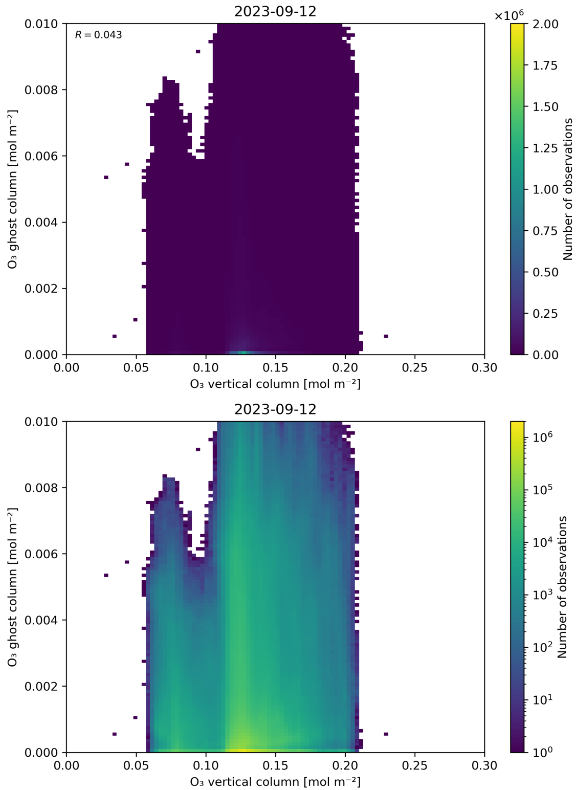
Figure 40: Scatter density plot of “O 3 vertical column” against “O 3 ghost column” for 2023-09-11 to 2023-09-13.
