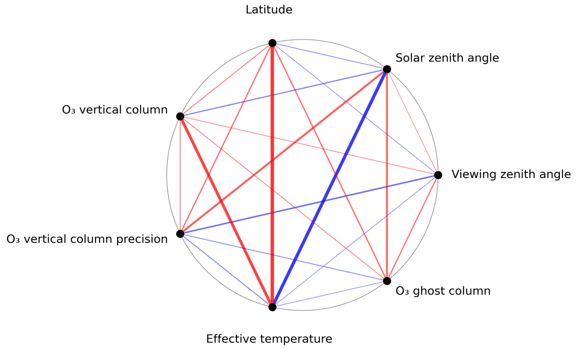
Figure 1: Map of correlation graph for 2023-09-11 to 2023-09-13.
