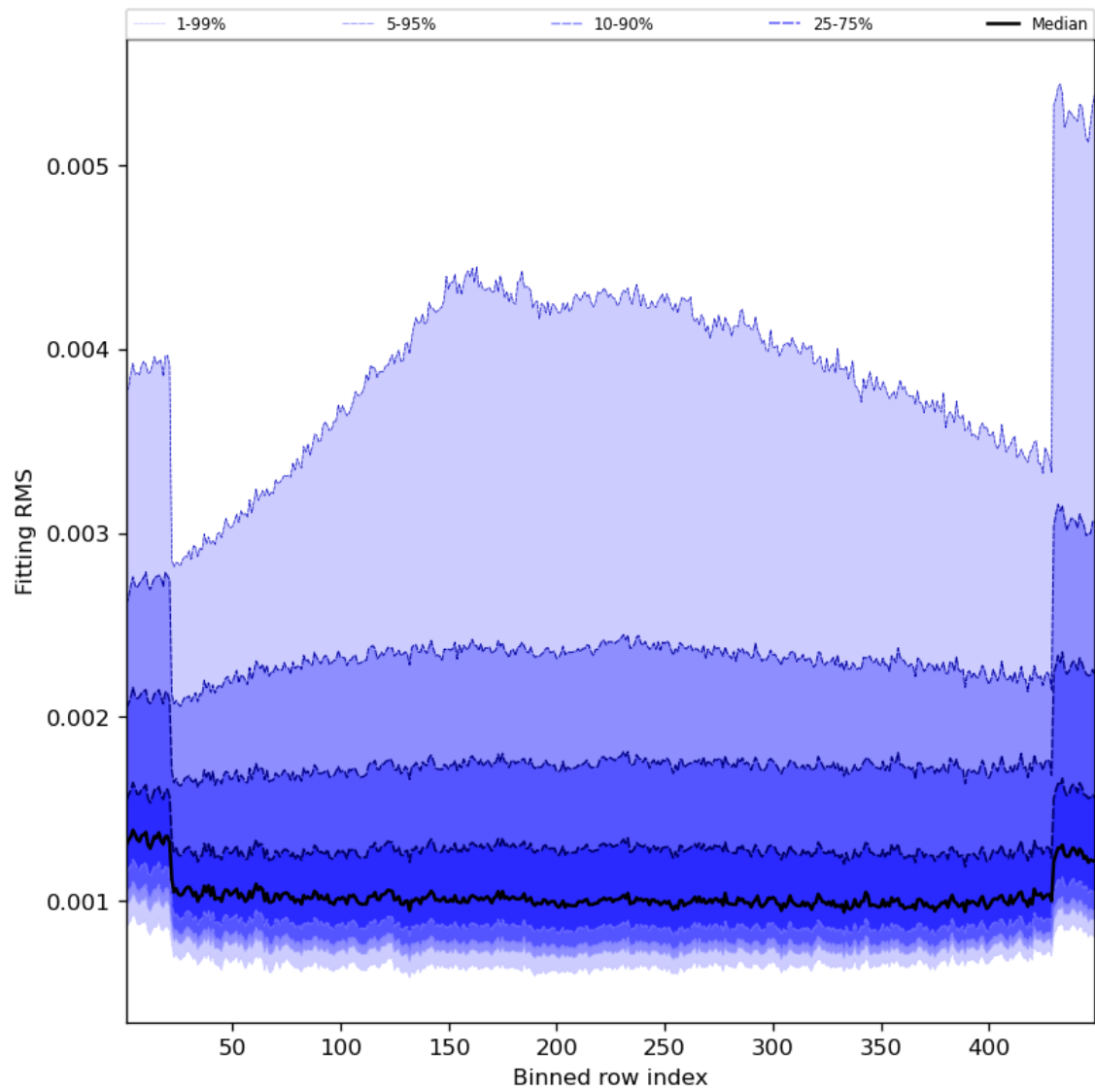
Figure 30: Along track statistics of “Fitting RMS” for 2023-09-11 to 2023-09-13
