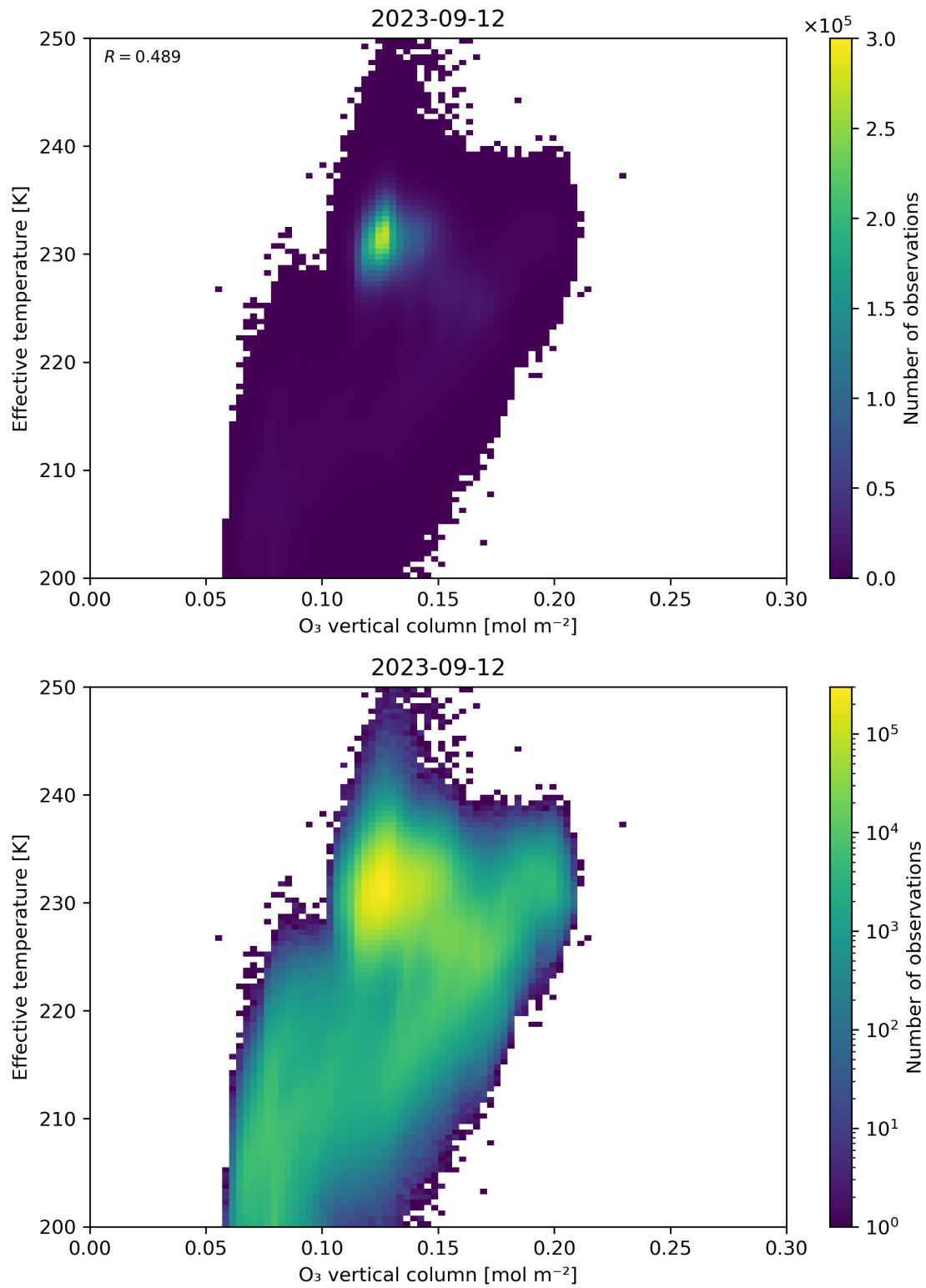
Figure 39: Scatter density plot of “O 3 vertical column” against “Effective temperature” for 2023-09-11 to 2023-09-13.
