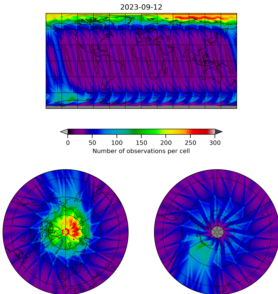
Figure 12: Map of the number of observations for 2023-09-11 to 2023-09-13
