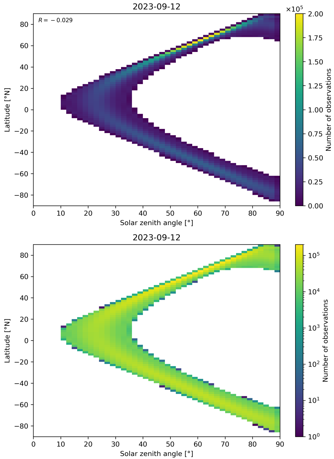
Figure 44: Scatter density plot of “Solar zenith angle” against “Latitude” for 2023-09-11 to 2023-09-13.
