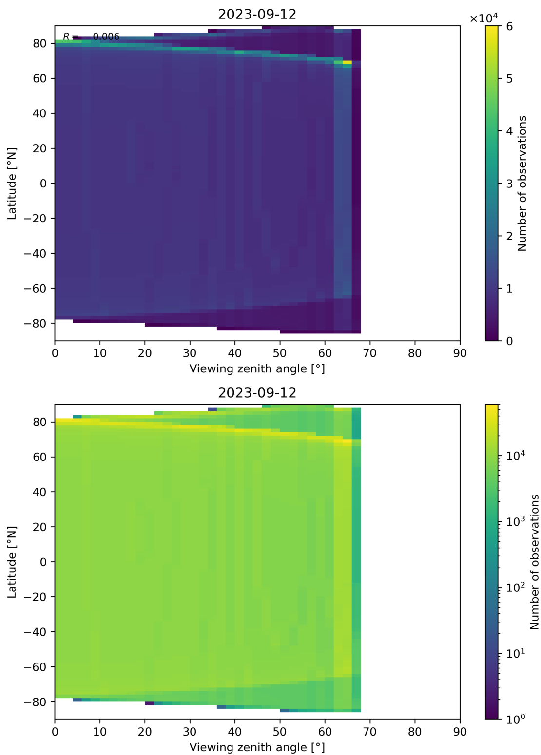
Figure 49: Scatter density plot of “Viewing zenith angle” against “Latitude” for 2023-09-11 to 2023-09-13.
