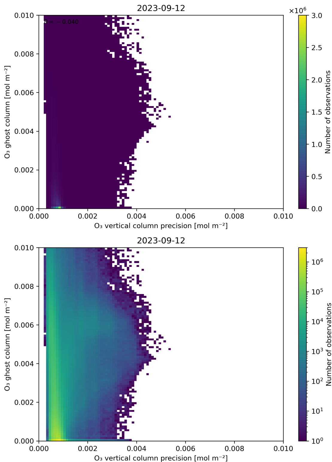
Figure 43: Scatter density plot of “O 3 vertical column precision” against “O 3 ghost column” for 2023-09-11 to 2023-09-13.
