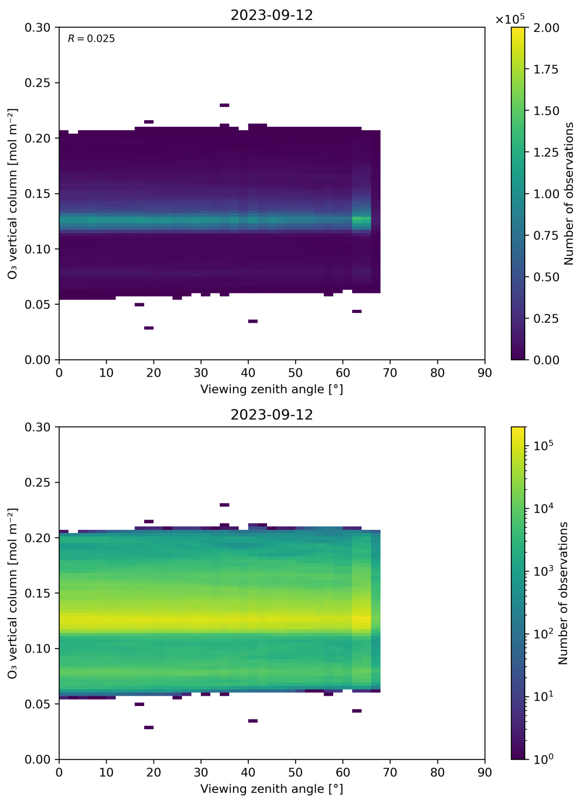
Figure 52: Scatter density plot of “Viewing zenith angle” against “O 3 vertical column” for 2023-09-11 to 2023-09-13.
