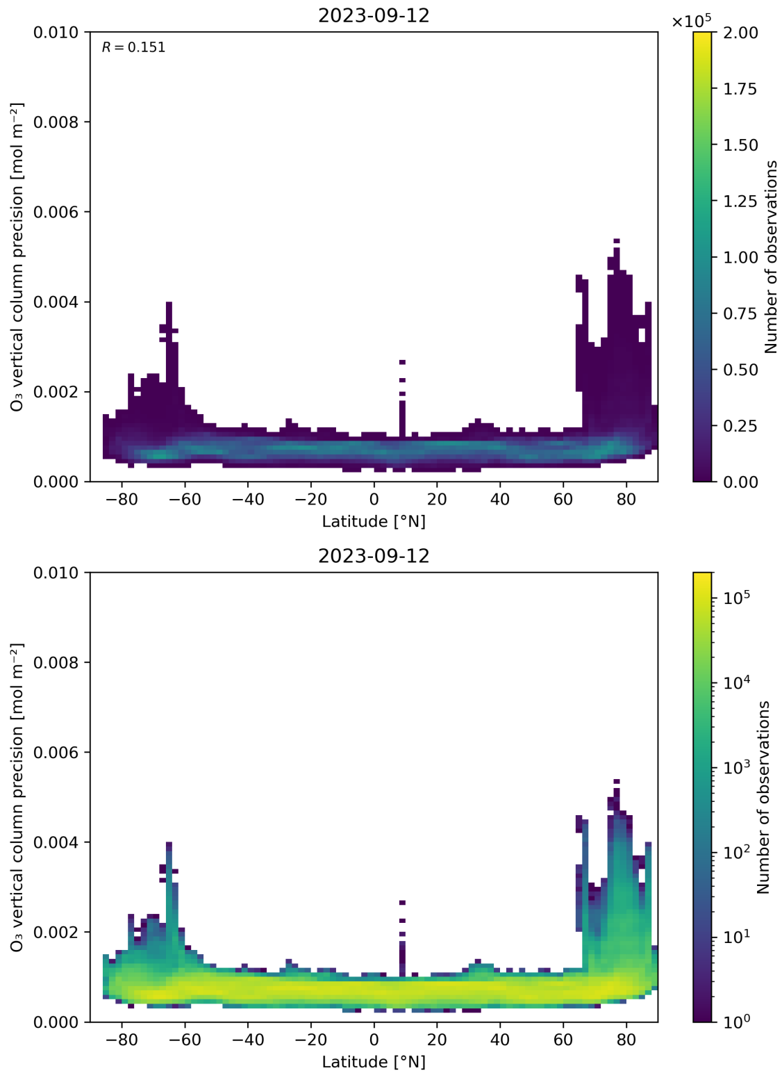
Figure 37: Scatter density plot of “Latitude” against “O 3 vertical column precision” for 2023-09-11 to 2023-09-13.
