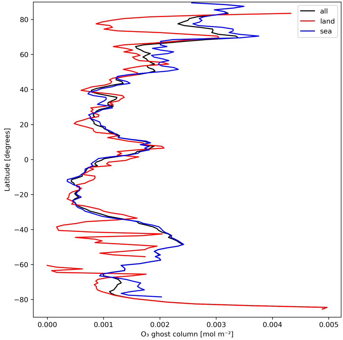
Figure 18: Zonal average of “O 3 ghost column” for 2023-09-11 to 2023-09-13.
