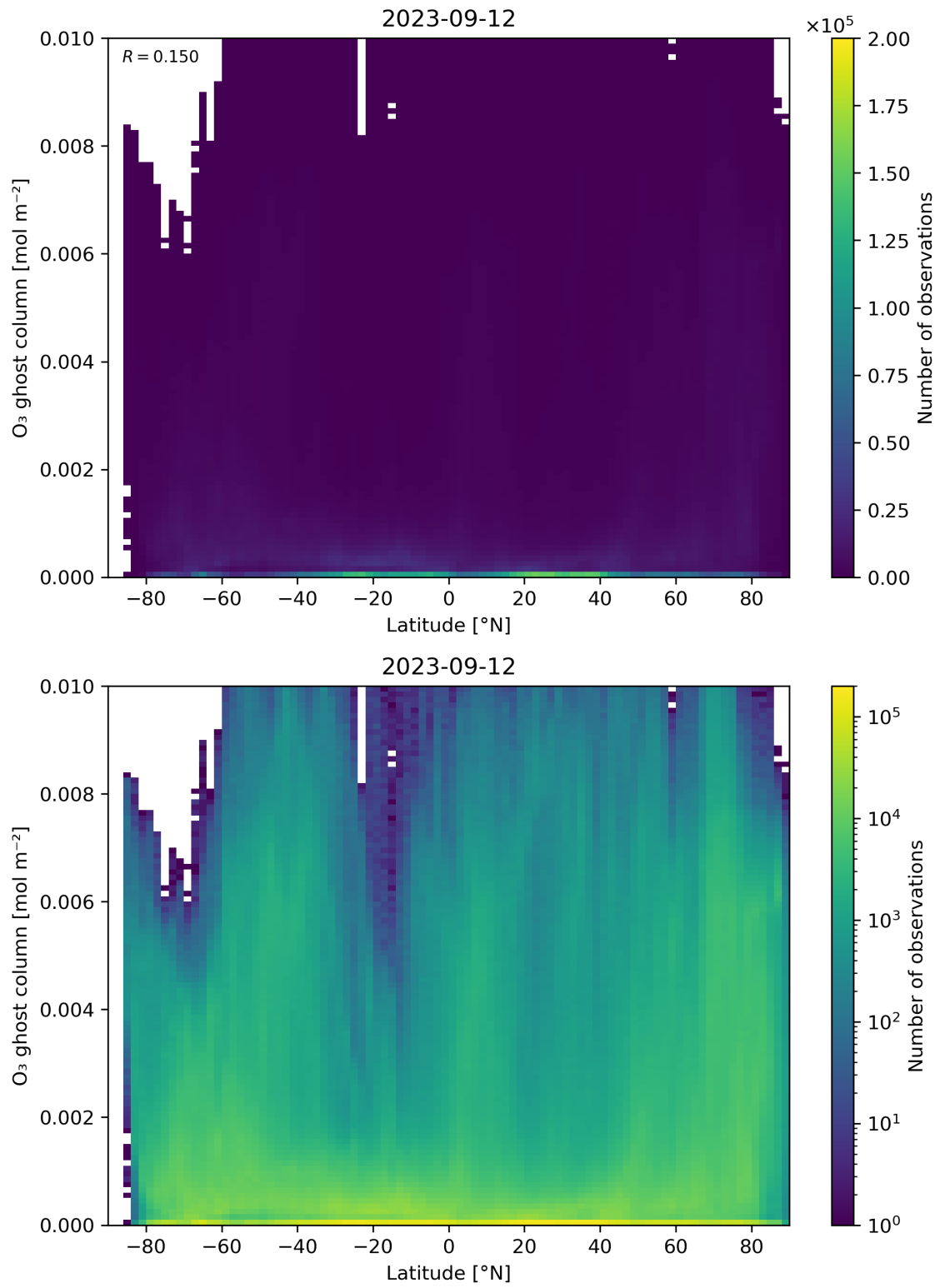
Figure 35: Scatter density plot of “Latitude” against “O 3 ghost column” for 2023-09-11 to 2023-09-13.
