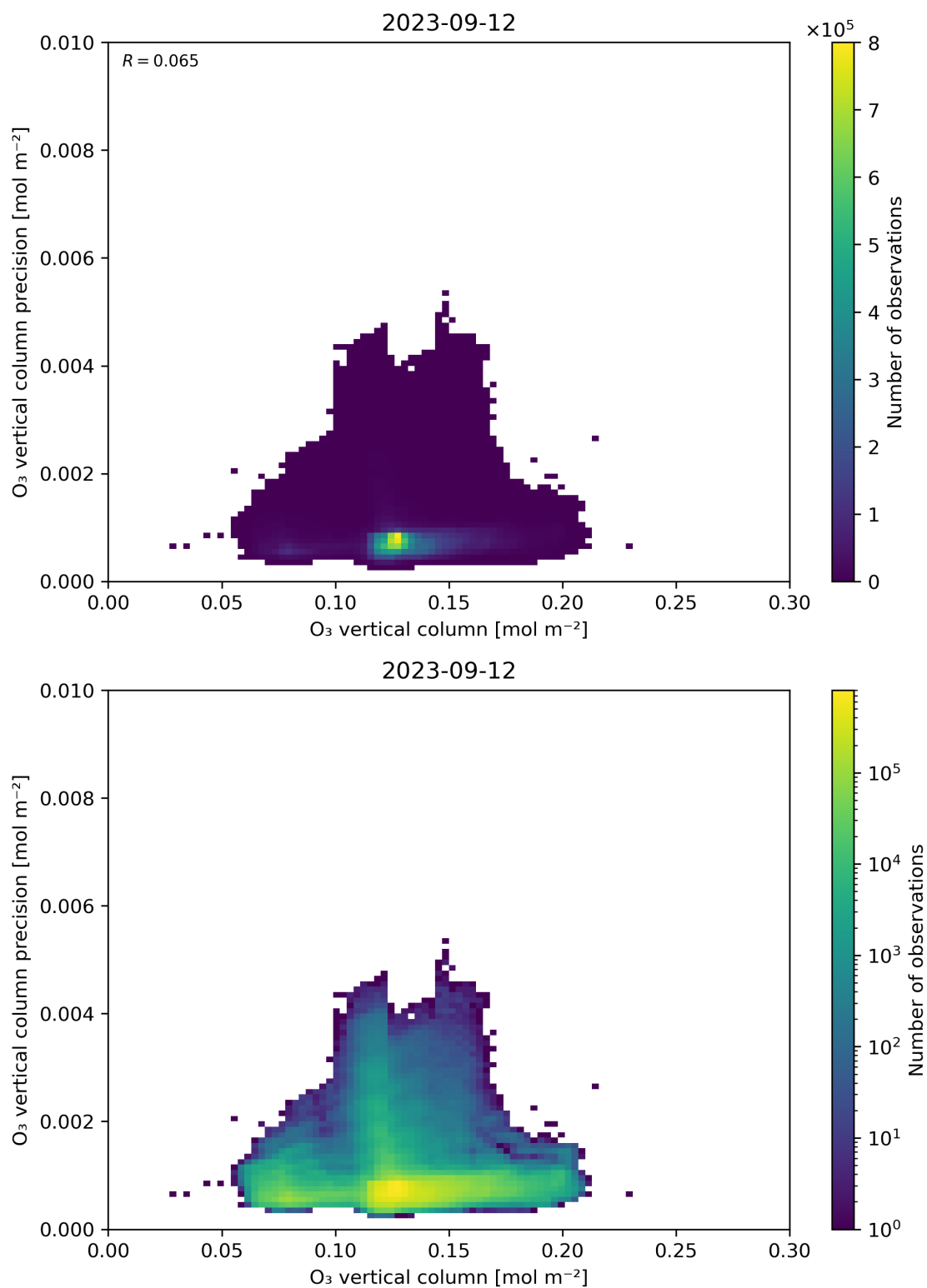
Figure 41: Scatter density plot of “O 3 vertical column” against “O 3 vertical column precision” for 2023-09-11 to 2023-09-13.
