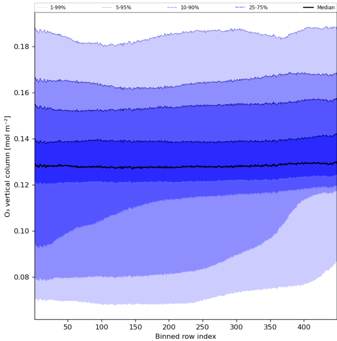
Figure 28: Along track statistics of “O 3 vertical column” for 2023-09-11 to 2023-09-13
