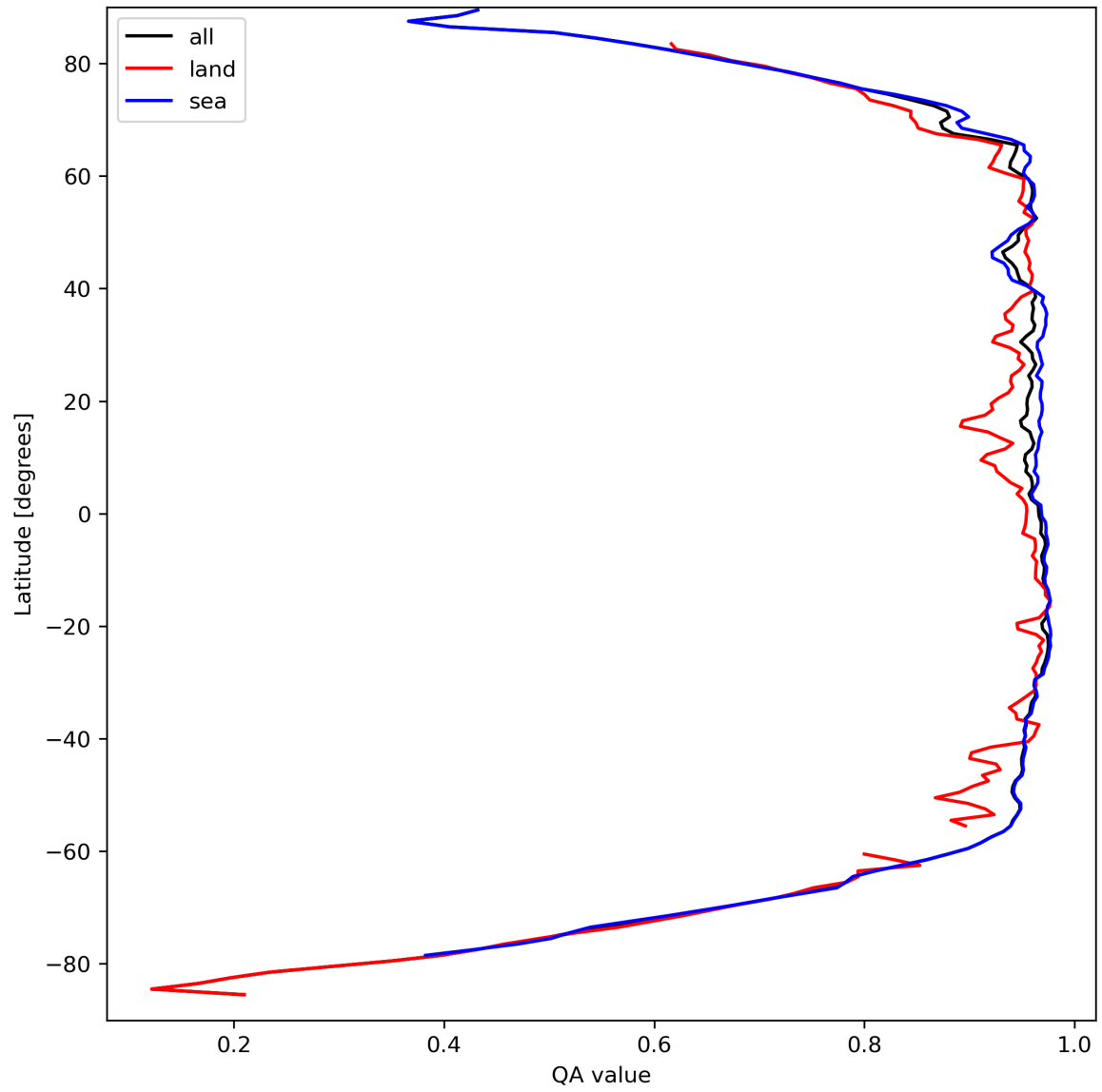
Figure 13: Zonal average of “QA value” for 2023-09-11 to 2023-09-13.
