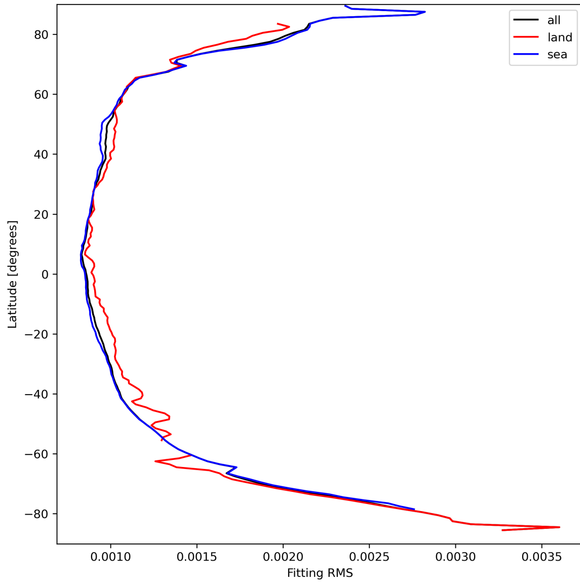
Figure 16: Zonal average of “Fitting RMS” for 2023-09-11 to 2023-09-13.
