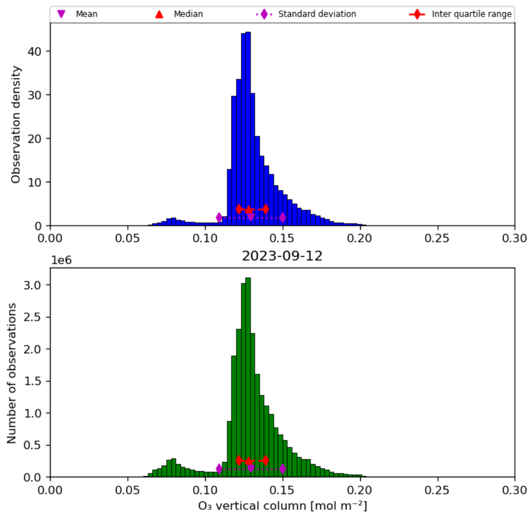
Figure 21: Histogram of “O 3 vertical column” for 2023-09-11 to 2023-09-13
