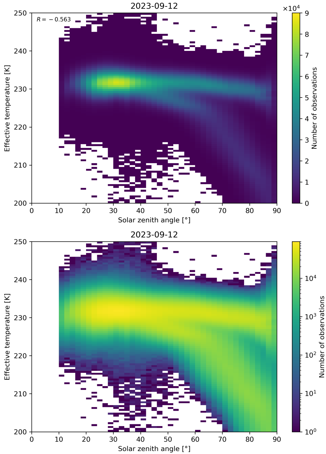
Figure 45: Scatter density plot of “Solar zenith angle” against “Effective temperature” for 2023-09-11 to 2023-09-13.
