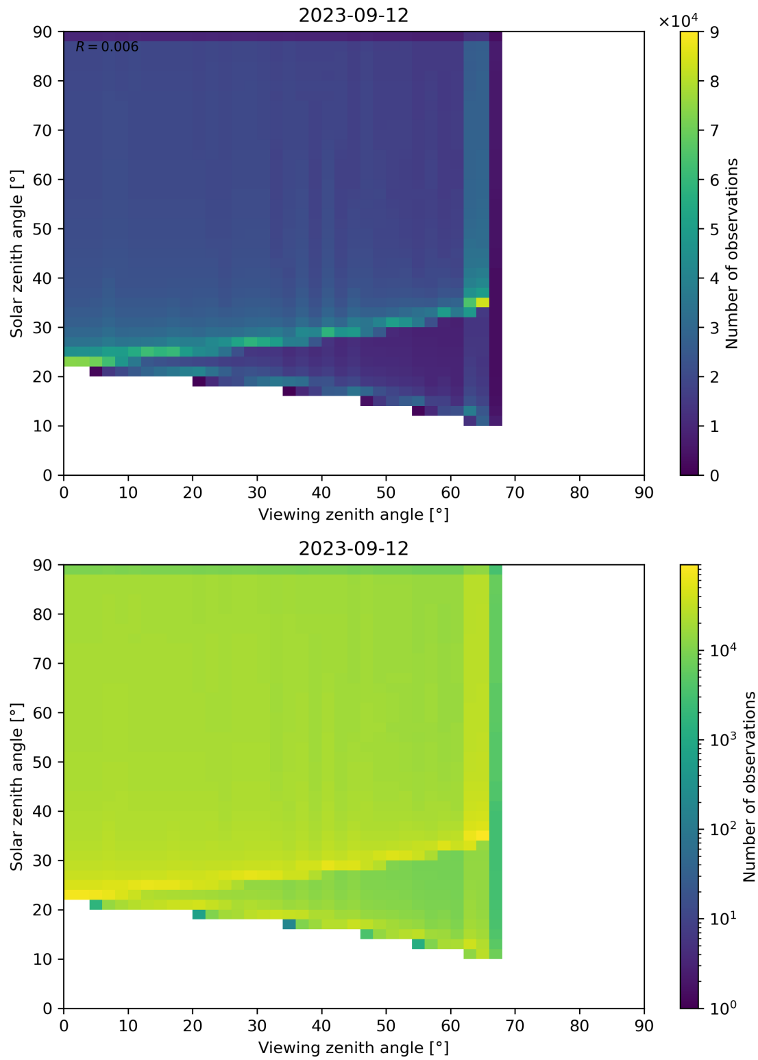
Figure 54: Scatter density plot of “Viewing zenith angle” against “Solar zenith angle” for 2023-09-11 to 2023-09-13.
