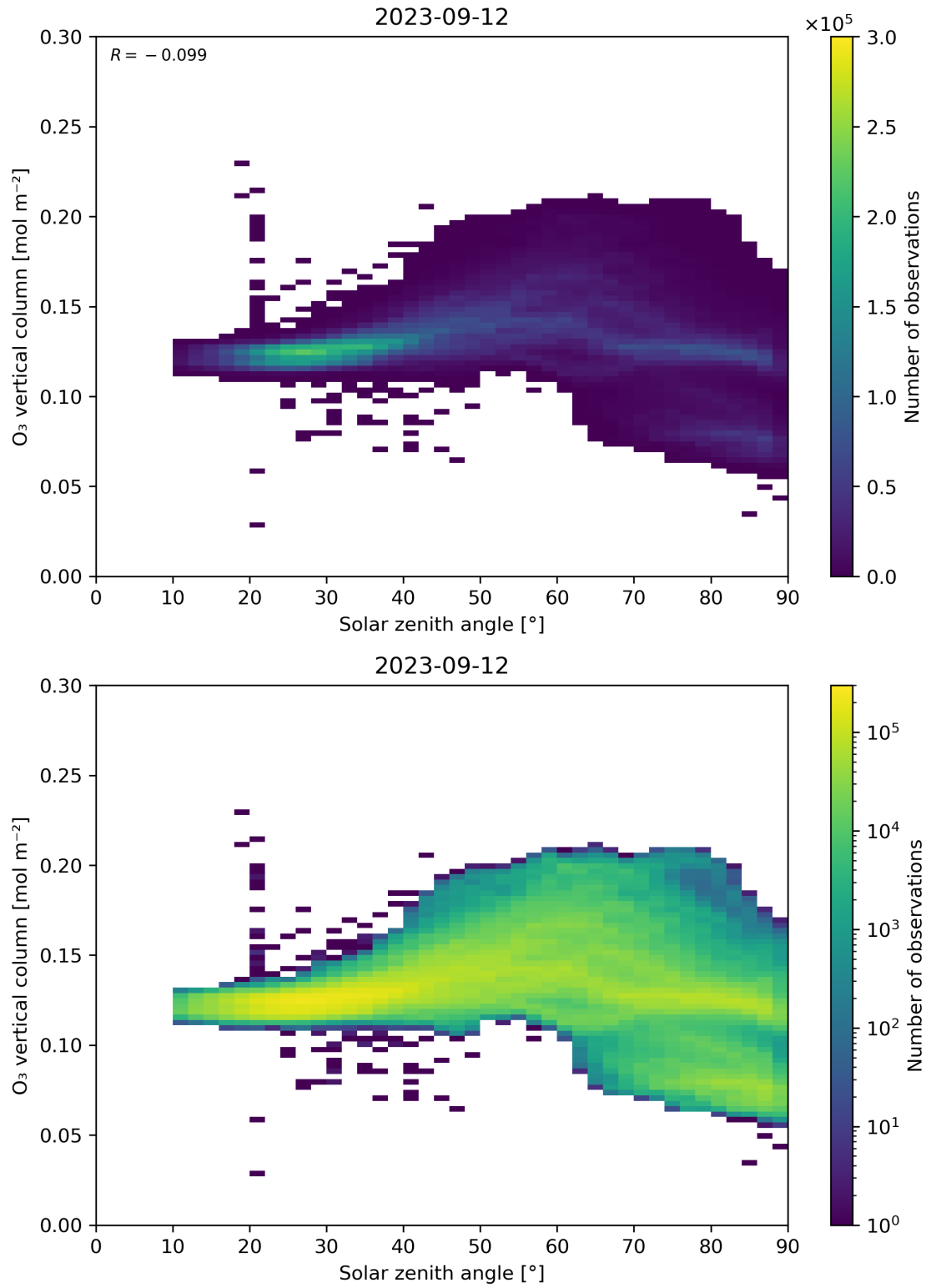
Figure 47: Scatter density plot of “Solar zenith angle” against “O 3 vertical column” for 2023-09-11 to 2023-09-13.
