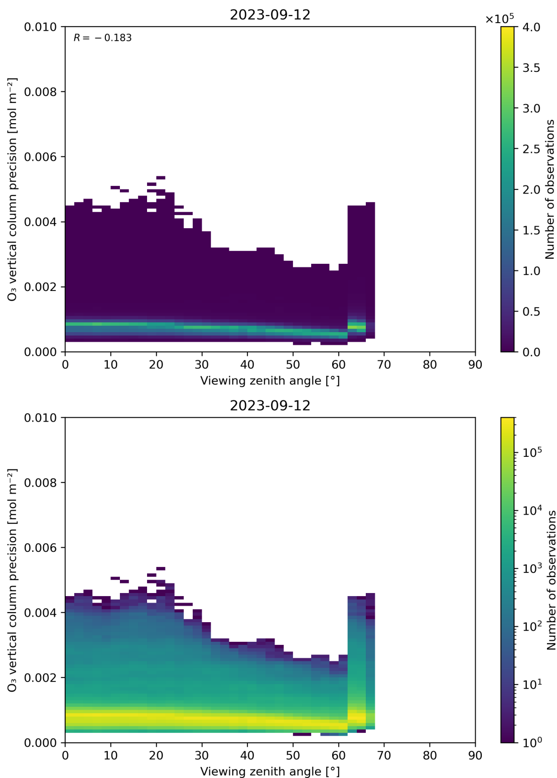
Figure 53: Scatter density plot of “Viewing zenith angle” against “O 3 vertical column precision” for 2023-09-11 to 2023-09-13.
