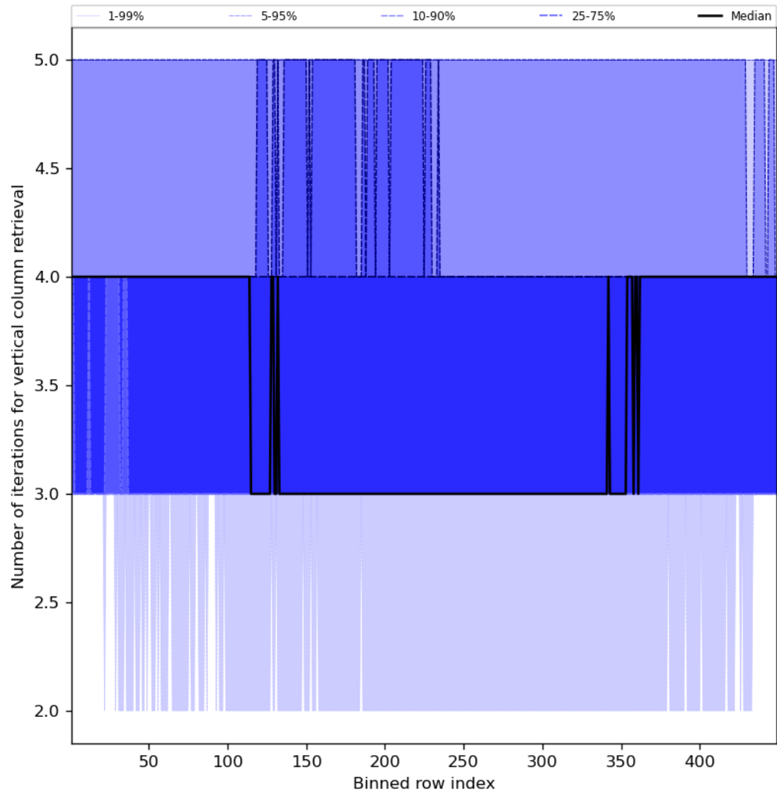
Figure 33: Along track statistics of “Number of iterations for vertical column retrieval” for 2023-09-11 to 2023-09-13
