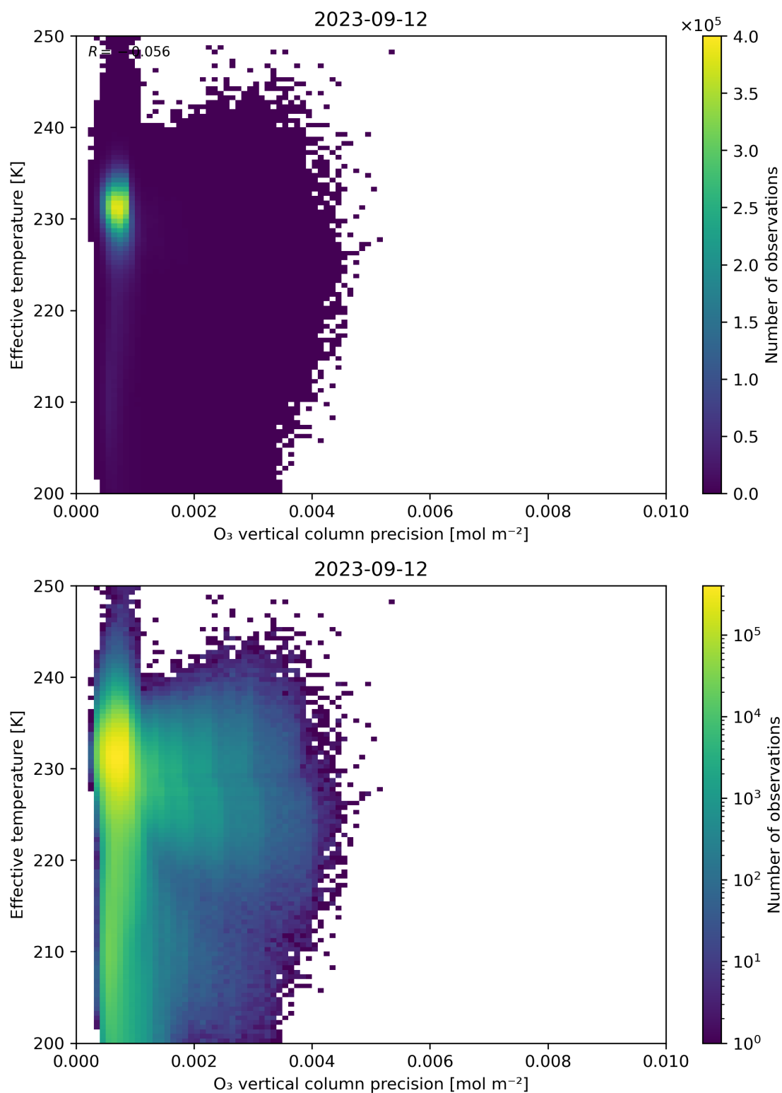
Figure 42: Scatter density plot of “O 3 vertical column precision” against “Effective temperature” for 2023-09-11 to 2023-09-13.
