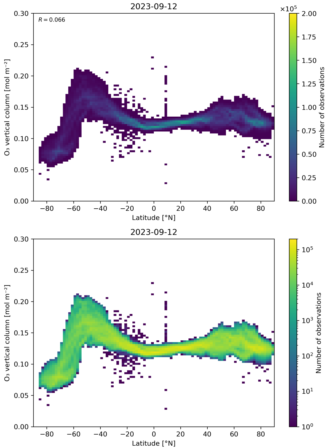
Figure 36: Scatter density plot of “Latitude” against “O 3 vertical column” for 2023-09-11 to 2023-09-13.
