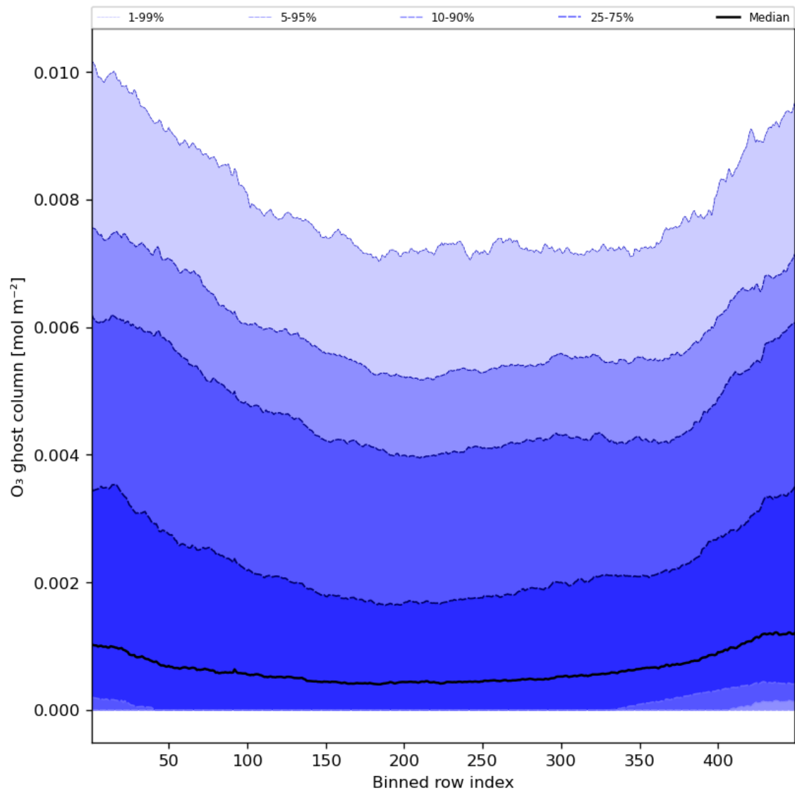
Figure 32: Along track statistics of “O 3 ghost column” for 2023-09-11 to 2023-09-13
