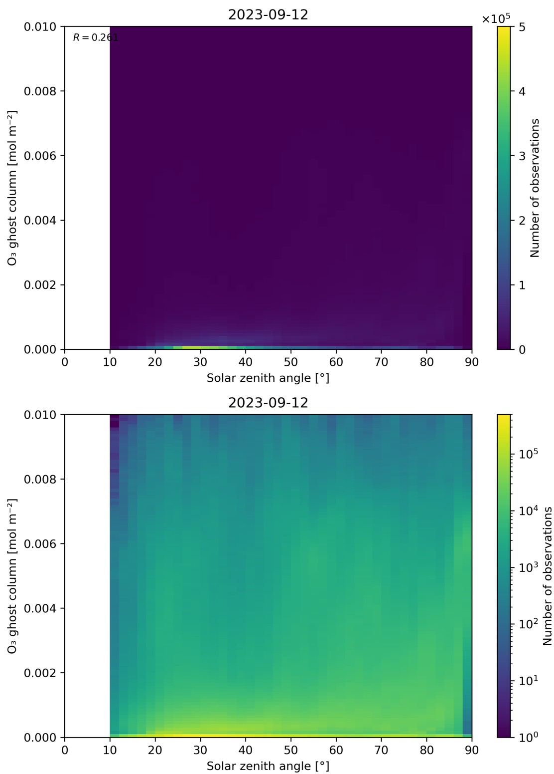
Figure 46: Scatter density plot of “Solar zenith angle” against “O 3 ghost column” for 2023-09-11 to 2023-09-13.
