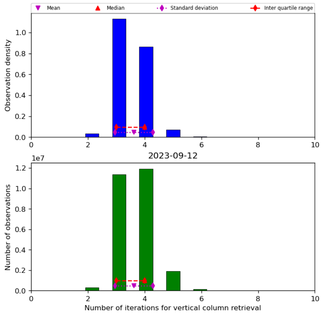
Figure 26: Histogram of “Number of iterations for vertical column retrieval” for 2023-09-11 to 2023-09-13
