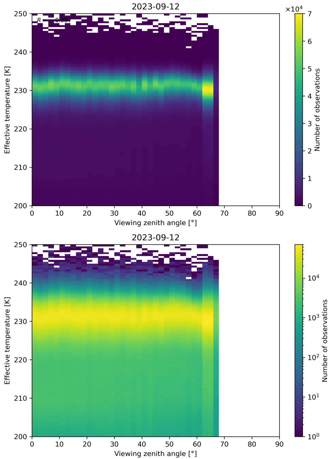
Figure 50: Scatter density plot of “Viewing zenith angle” against “Effective temperature” for 2023-09-11 to 2023-09-13.
