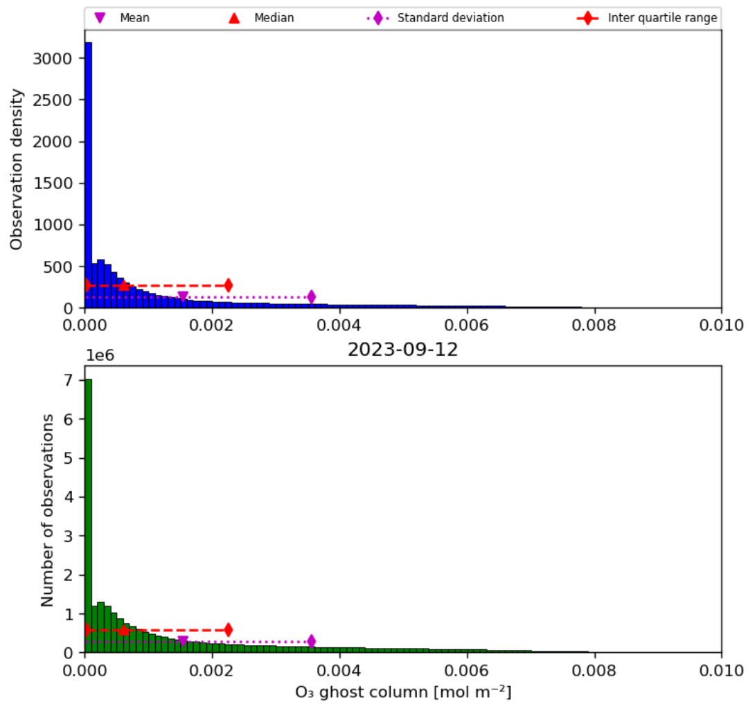
Figure 25: Histogram of "O 3 ghost column" for 2023-09-11 to 2023-09-13
