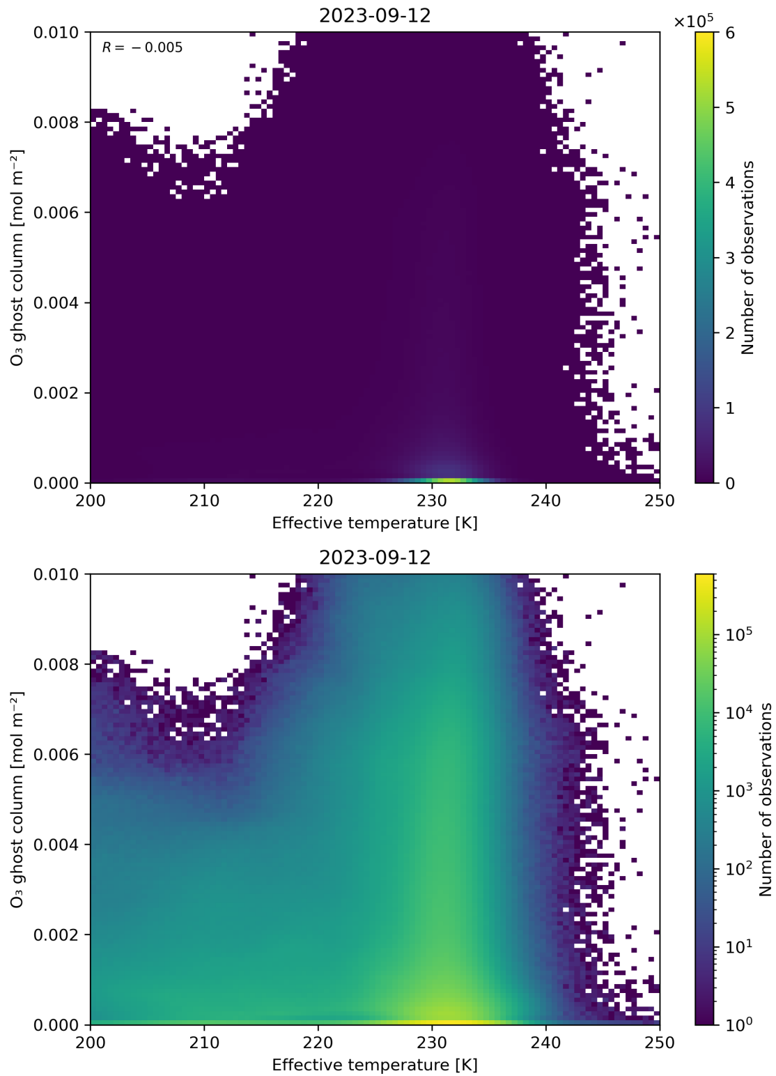
Figure 38: Scatter density plot of “Effective temperature” against “O 3 ghost column” for 2023-09-11 to 2023-09-13.
