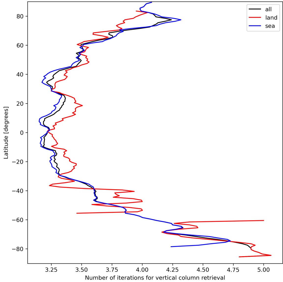
Figure 19: Zonal average of “Number of iterations for vertical column retrieval” for 2023-09-11 to 2023-09-13.
