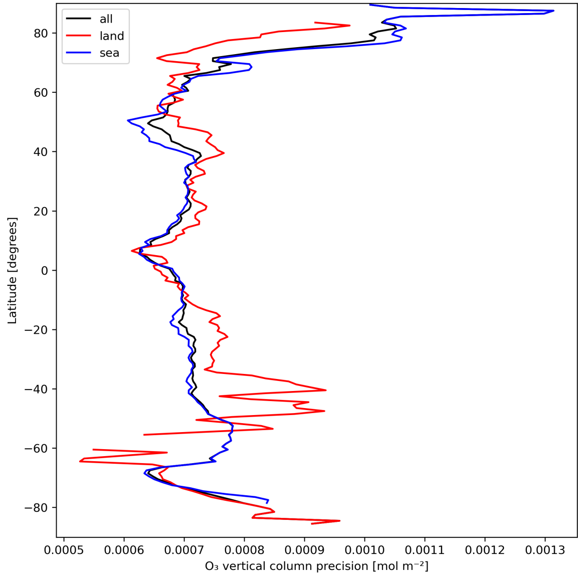
Figure 15: Zonal average of “O 3 vertical column precision” for 2023-09-11 to 2023-09-13.
