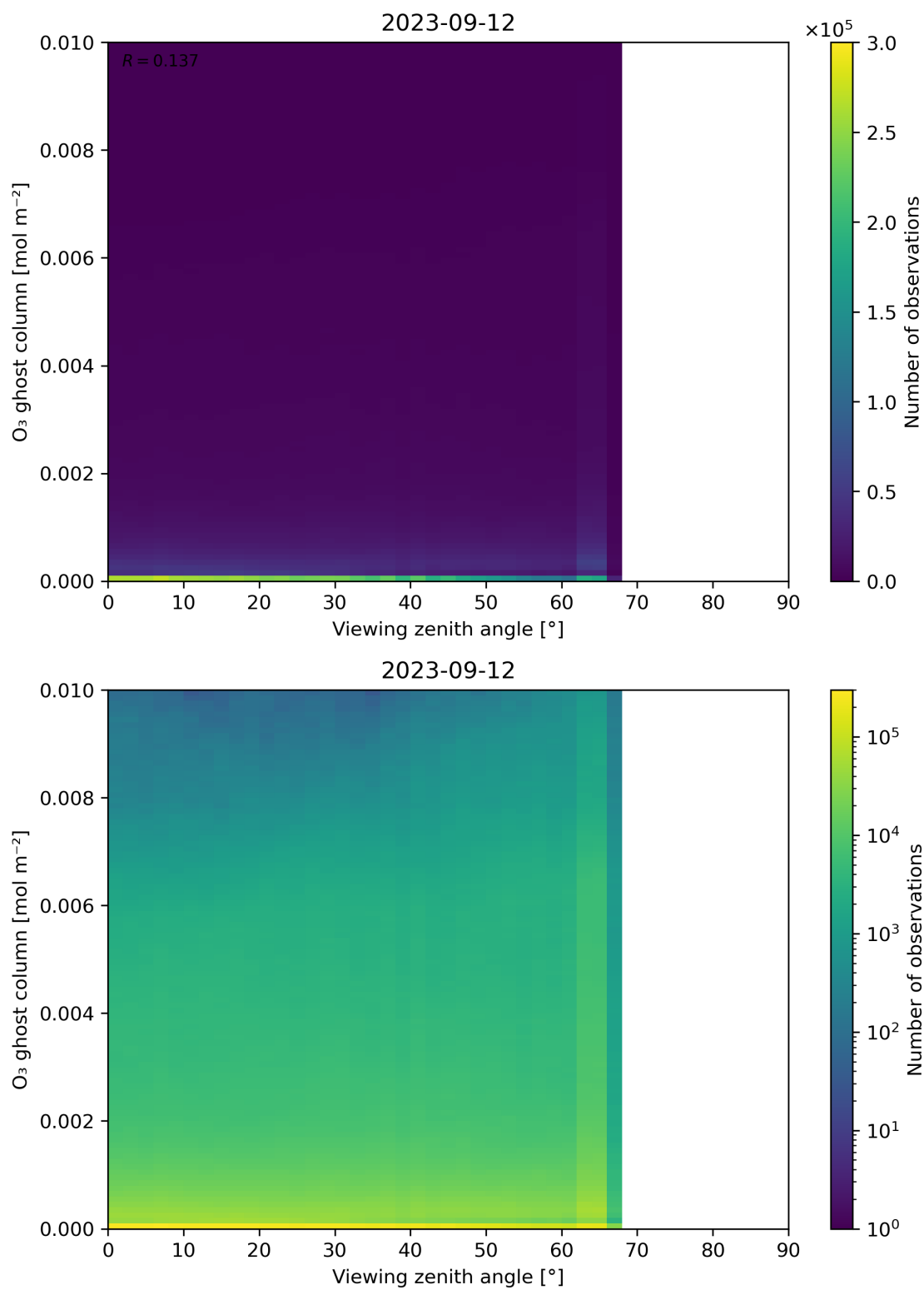
Figure 51: Scatter density plot of “Viewing zenith angle” against “O 3 ghost column” for 2023-09-11 to 2023-09-13.
