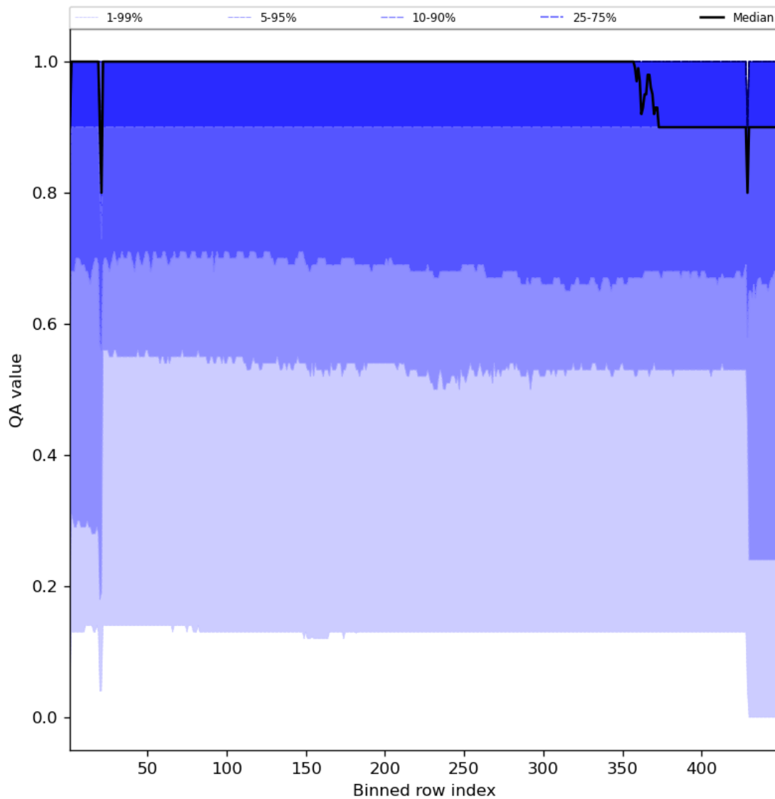
Figure 27: Along track statistics of “QA value” for 2023-09-11 to 2023-09-13
