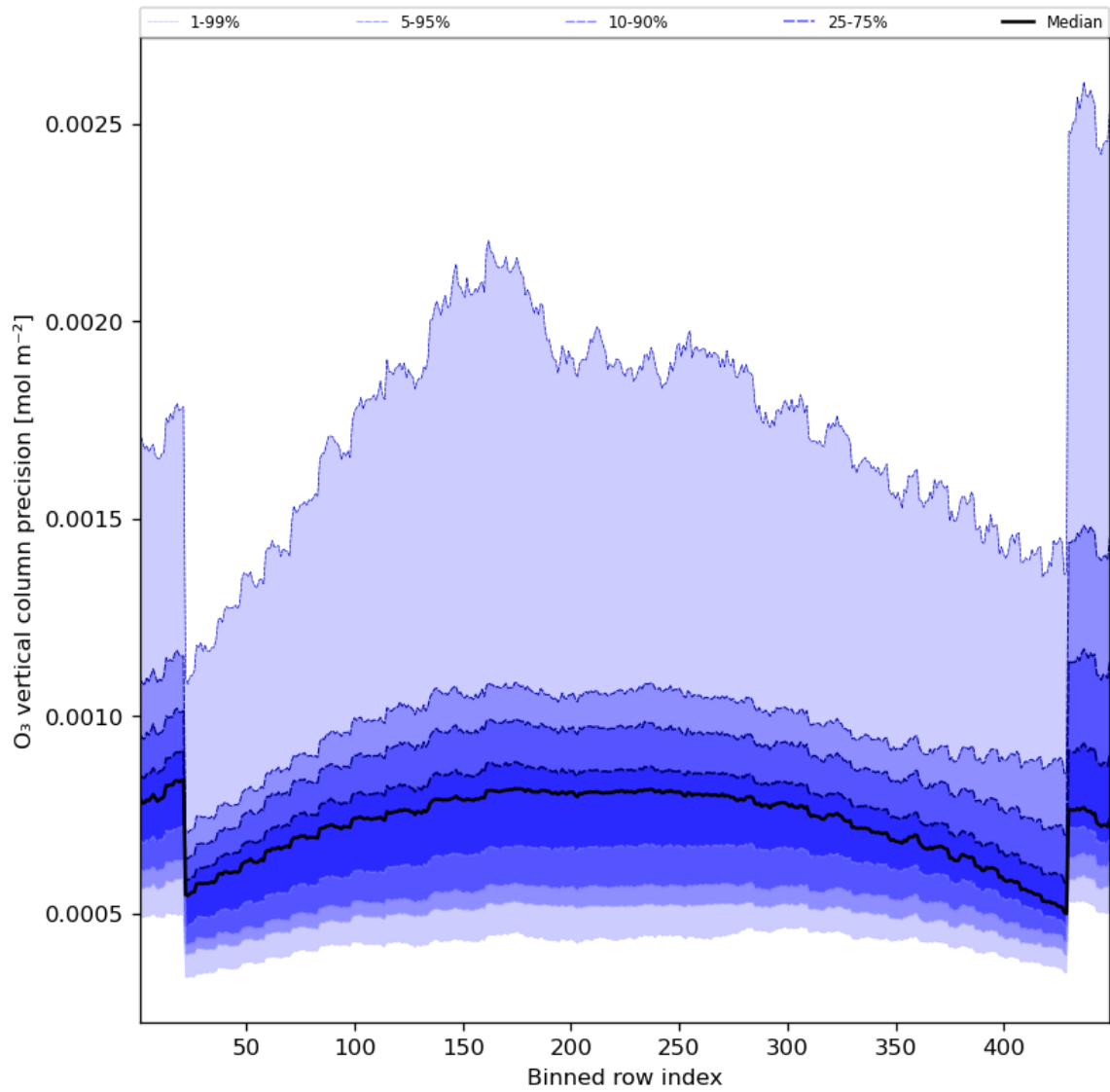
Figure 29: Along track statistics of “O 3 vertical column precision” for 2023-09-11 to 2023-09-13
