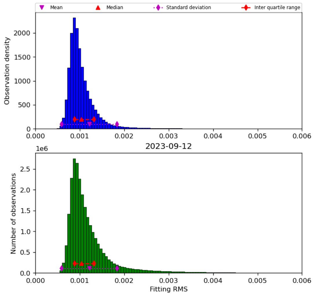
Figure 23: Histogram of “Fitting RMS” for 2023-09-11 to 2023-09-13
