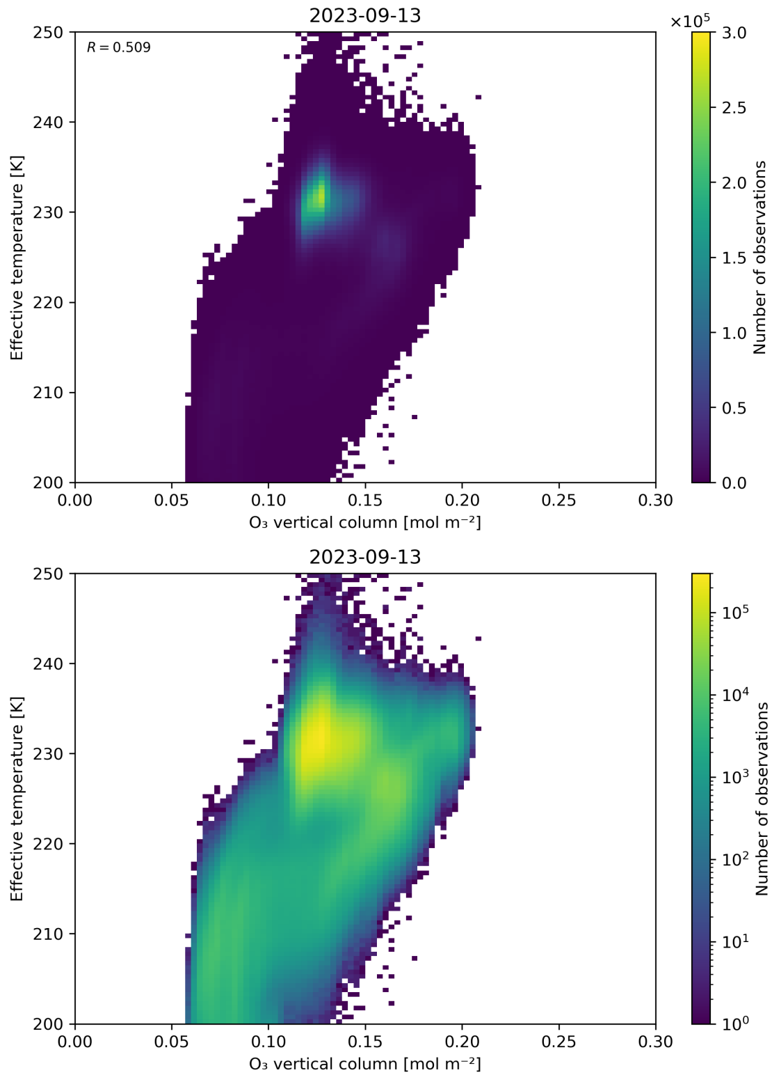
Figure 39: Scatter density plot of “O 3 vertical column” against “Effective temperature” for 2023-09-12 to 2023-09-14.
