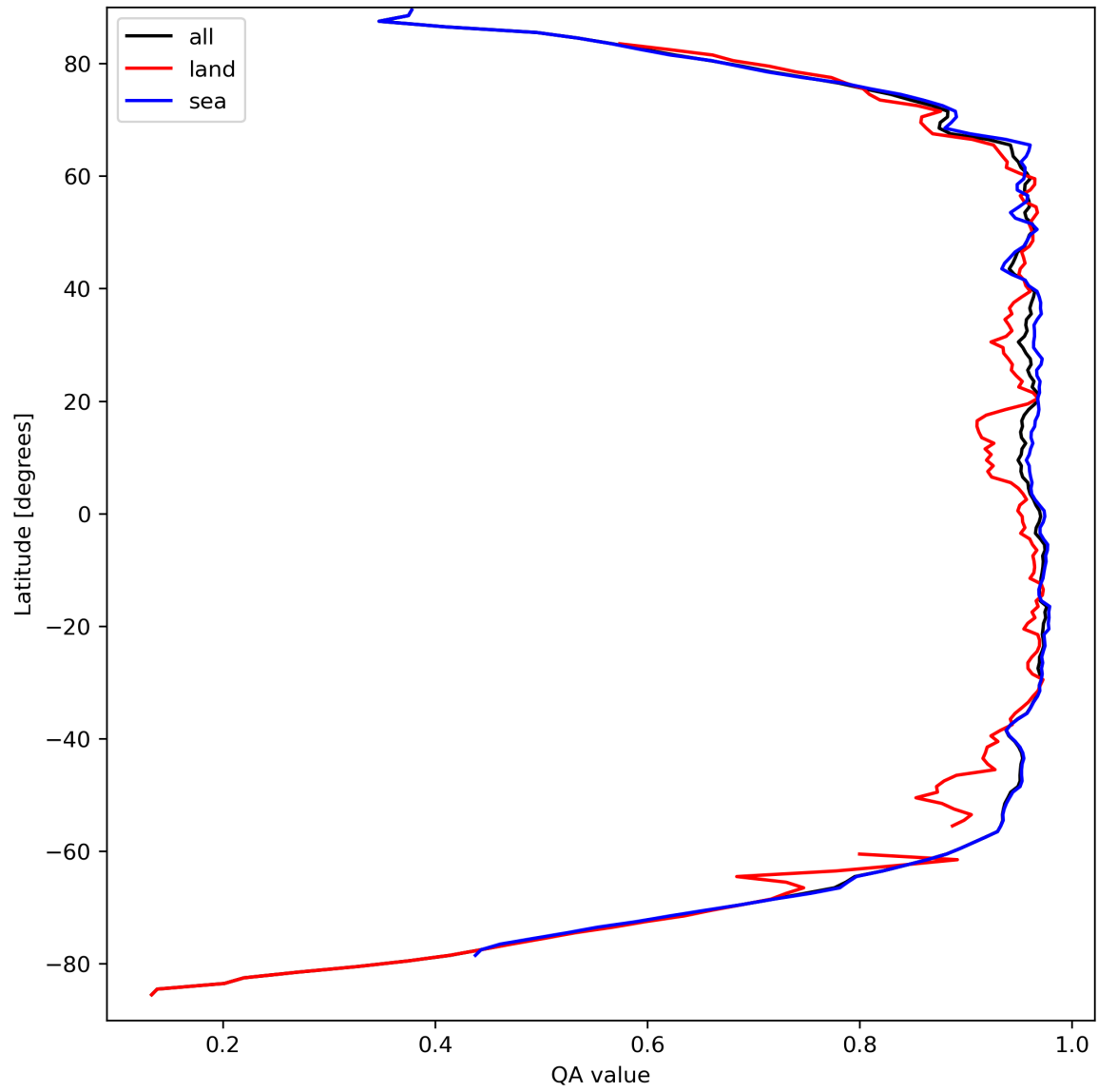
Figure 13: Zonal average of “QA value” for 2023-09-12 to 2023-09-14.
