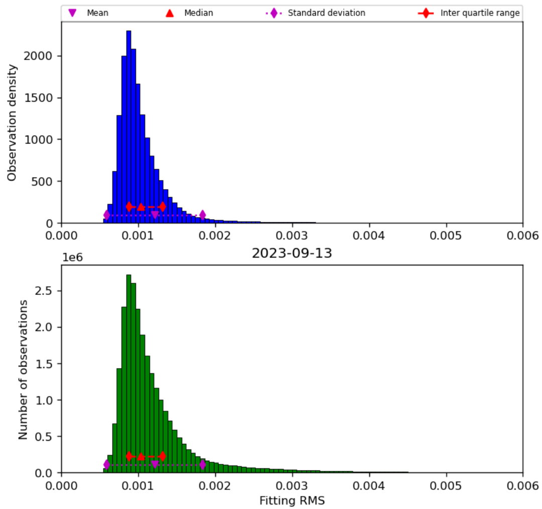
Figure 23: Histogram of “Fitting RMS” for 2023-09-12 to 2023-09-14
