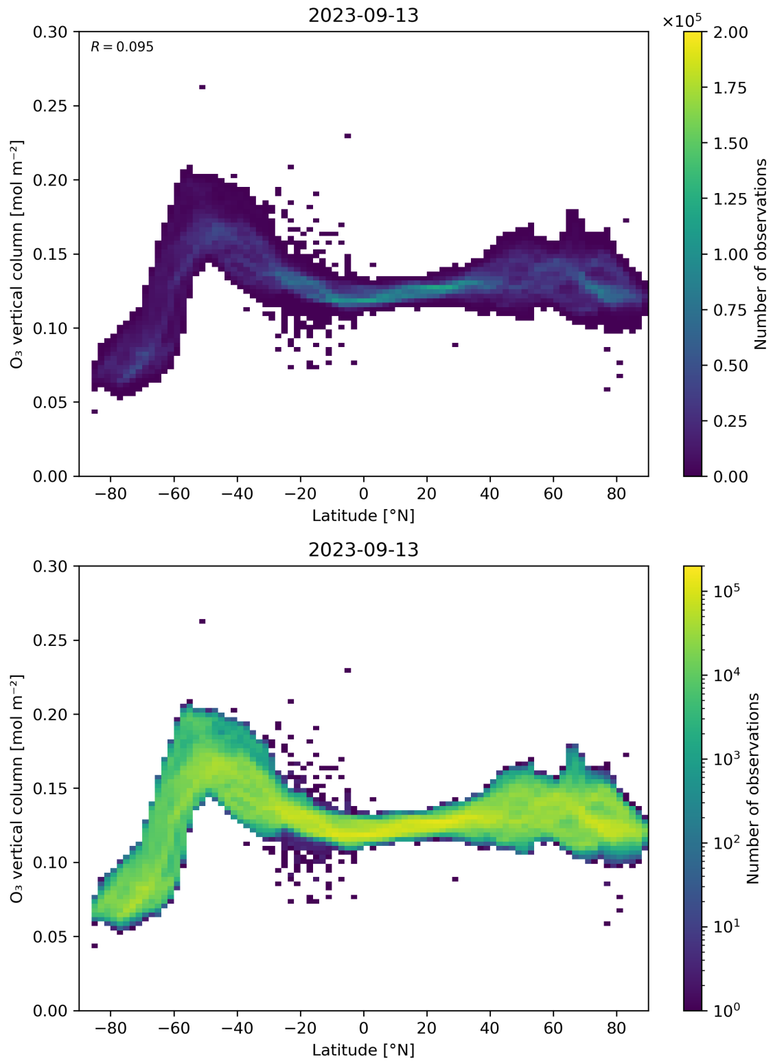
Figure 36: Scatter density plot of “Latitude” against “O 3 vertical column” for 2023-09-12 to 2023-09-14.
