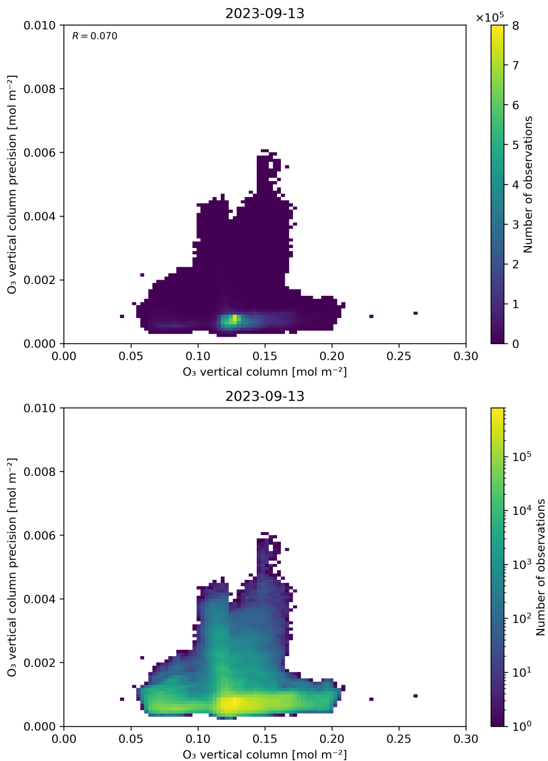
Figure 41: Scatter density plot of “O 3 vertical column” against “O 3 vertical column precision” for 2023-09-12 to 2023-09-14.
