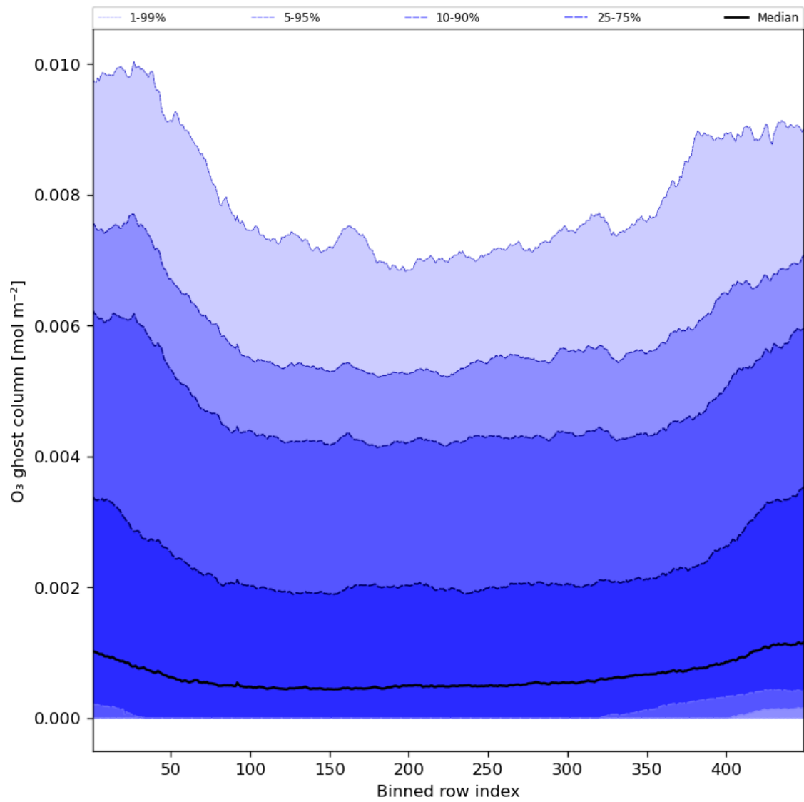
Figure 32: Along track statistics of “O 3 ghost column” for 2023-09-12 to 2023-09-14
