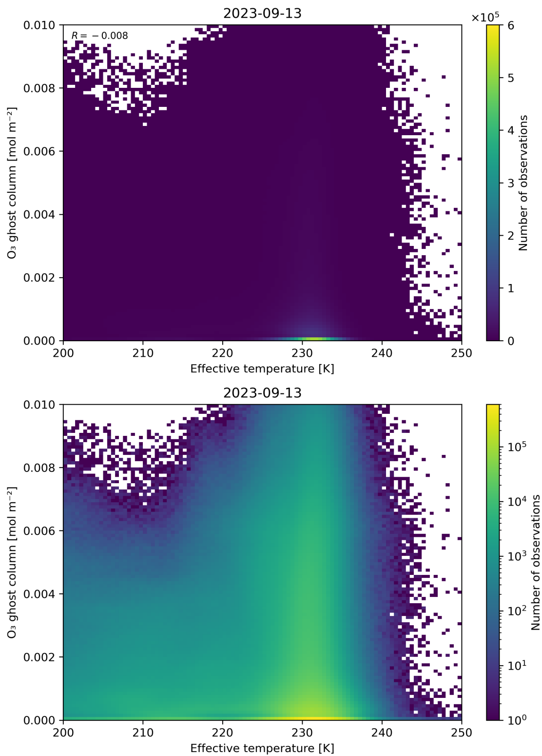
Figure 38: Scatter density plot of “Effective temperature” against “O 3 ghost column” for 2023-09-12 to 2023-09-14.
