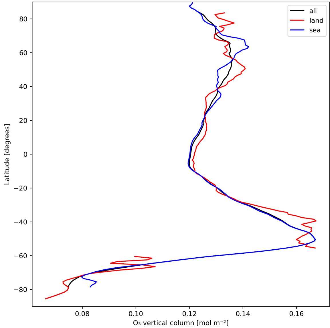
Figure 14: Zonal average of “O 3 vertical column” for 2023-09-12 to 2023-09-14.
