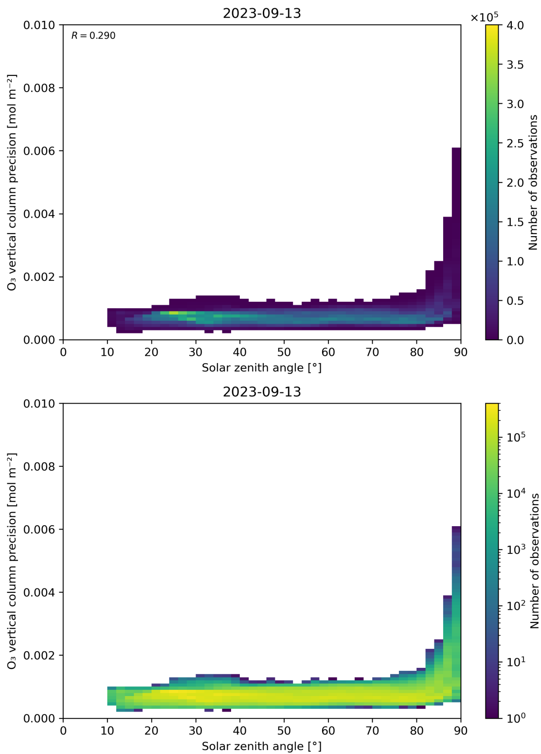
Figure 48: Scatter density plot of “Solar zenith angle” against “O 3 vertical column precision” for 2023-09-12 to 2023-09-14.
