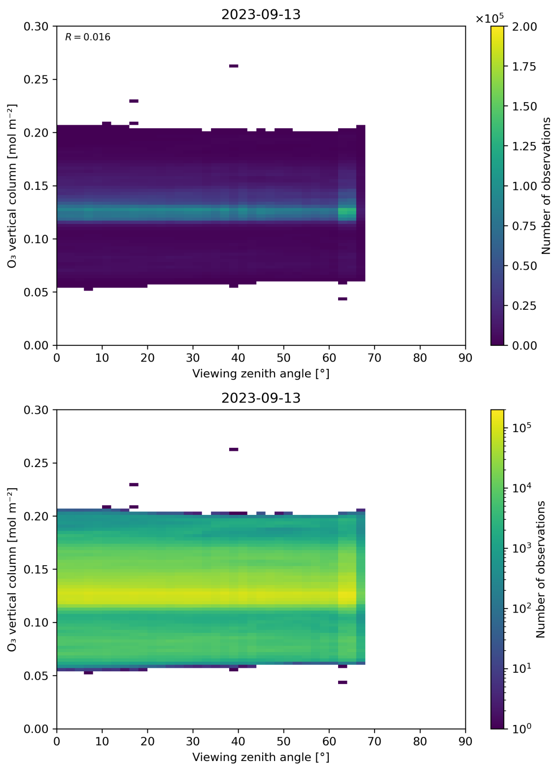
Figure 52: Scatter density plot of “Viewing zenith angle” against “O 3 vertical column” for 2023-09-12 to 2023-09-14.
