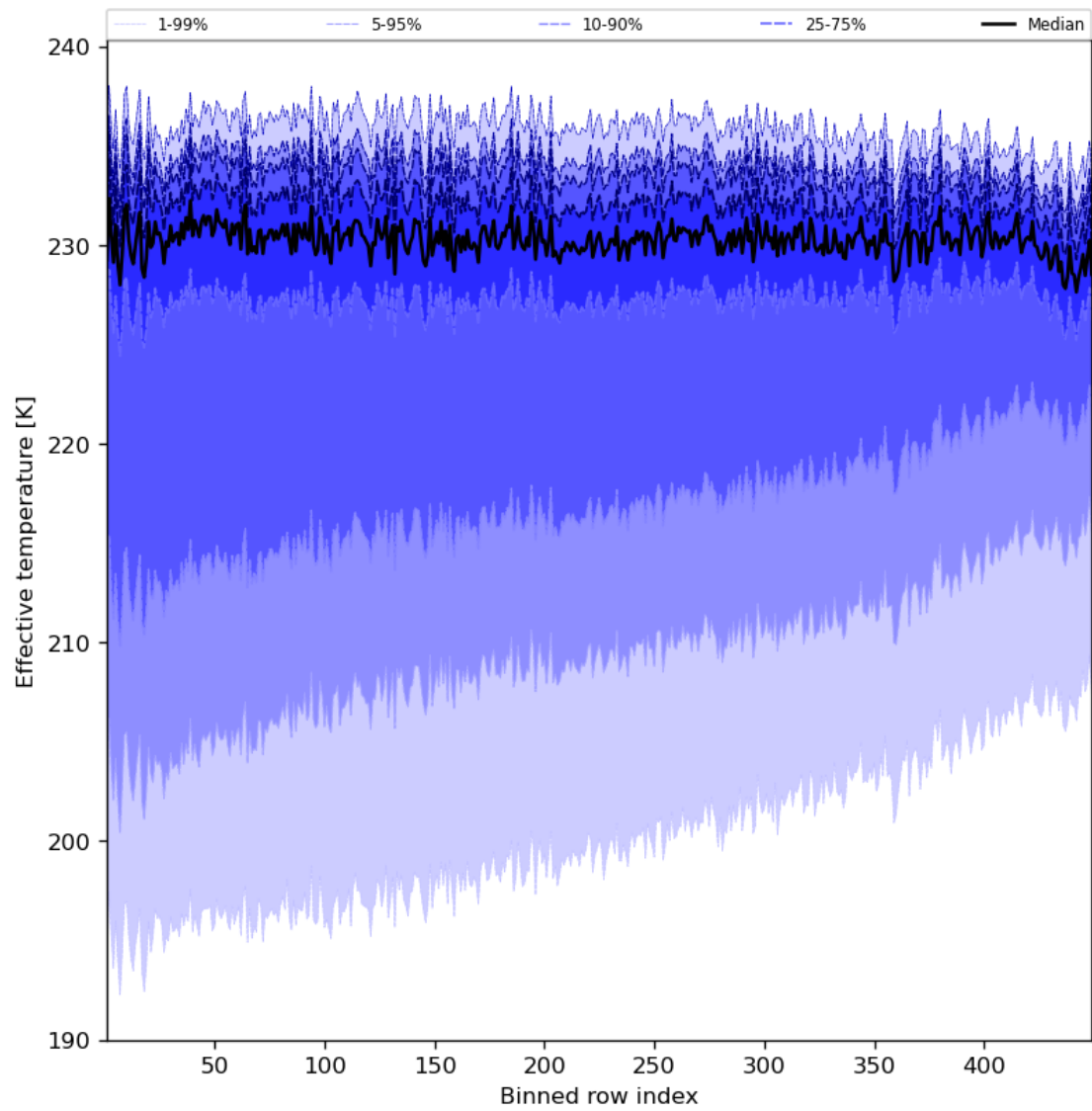
Figure 31: Along track statistics of “Effective temperature” for 2023-09-12 to 2023-09-14
