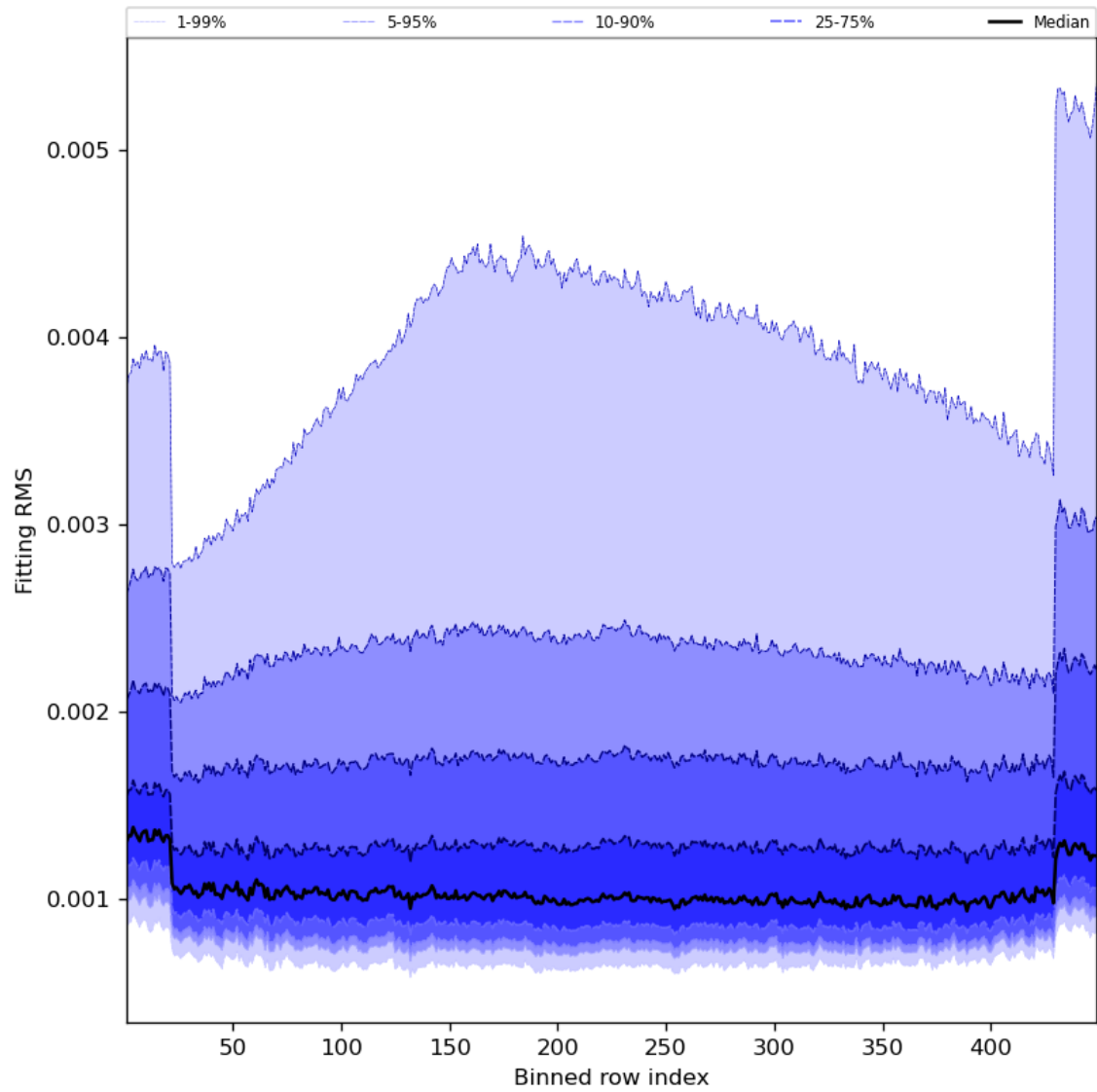
Figure 30: Along track statistics of “Fitting RMS” for 2023-09-12 to 2023-09-14
