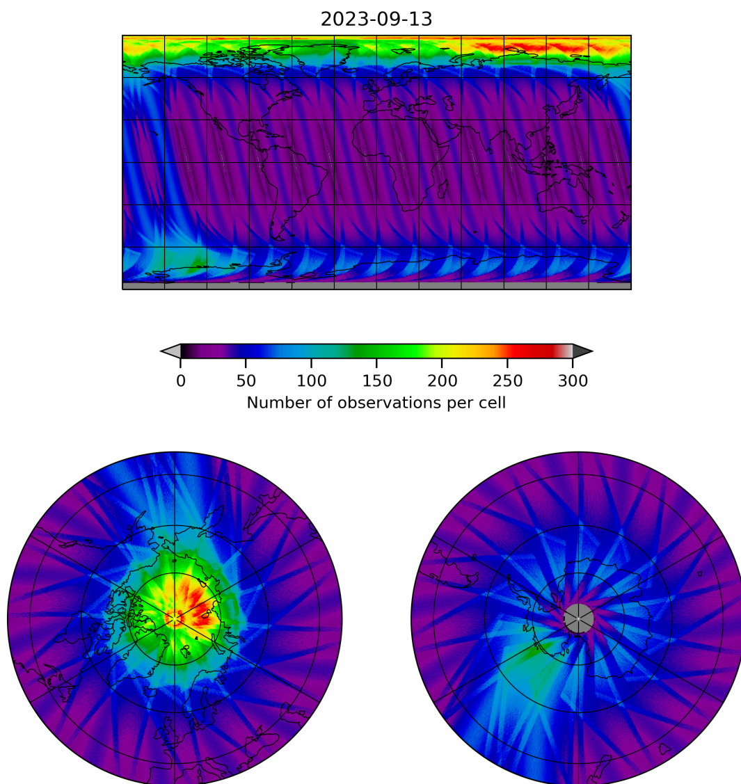
Figure 12: Map of the number of observations for 2023-09-12 to 2023-09-14
