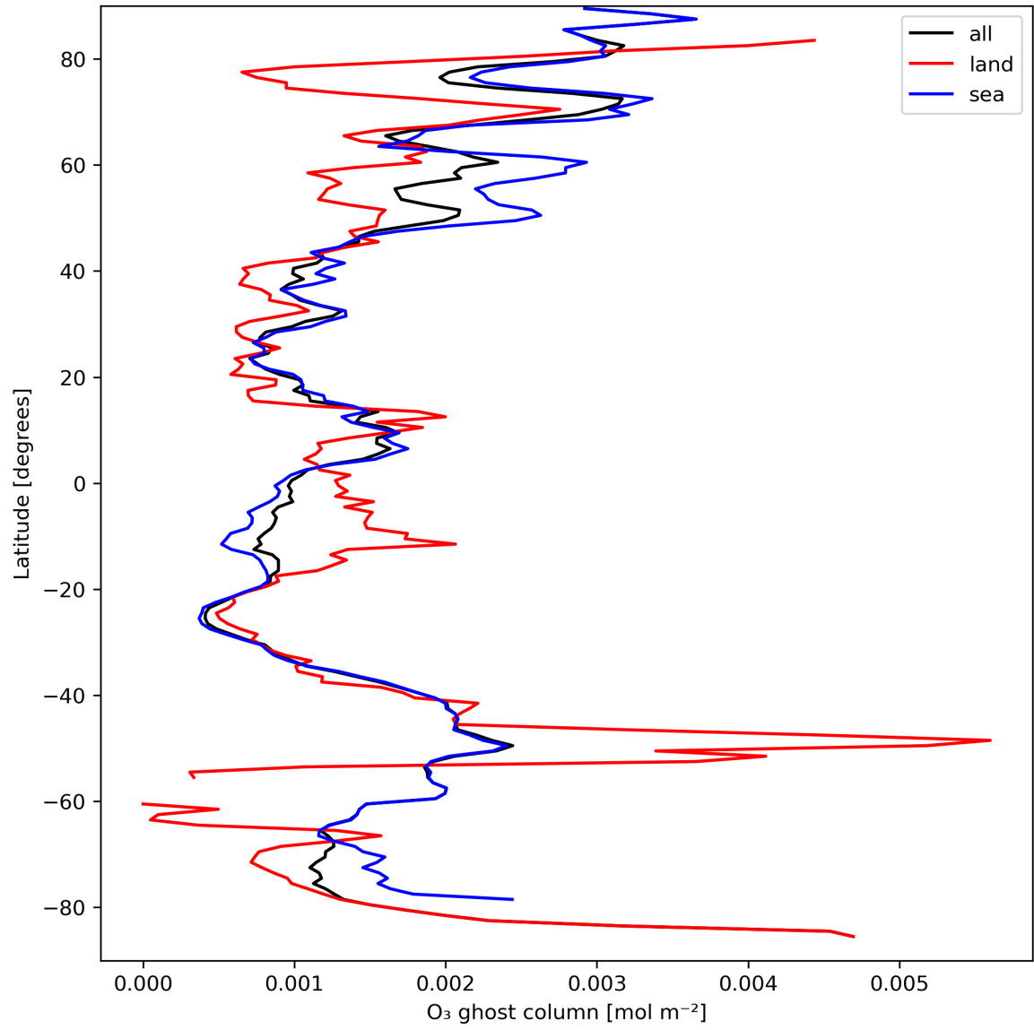
Figure 18: Zonal average of “O 3 ghost column” for 2023-09-12 to 2023-09-14.
