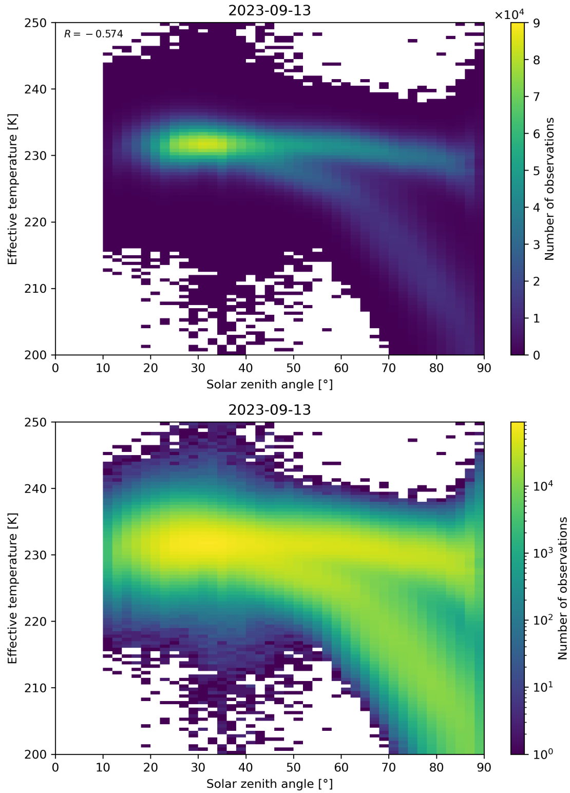
Figure 45: Scatter density plot of “Solar zenith angle” against “Effective temperature” for 2023-09-12 to 2023-09-14.
