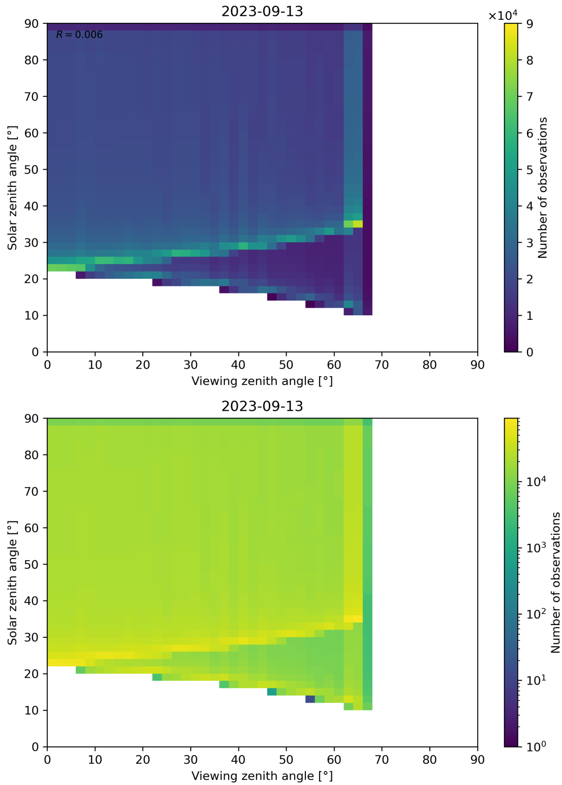
Figure 54: Scatter density plot of “Viewing zenith angle” against “Solar zenith angle” for 2023-09-12 to 2023-09-14.
