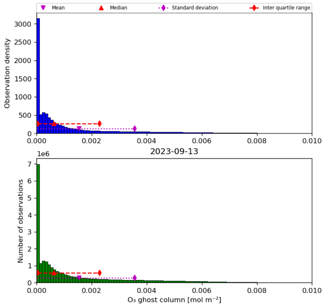
Figure 25: Histogram of “O 3 ghost column” for 2023-09-12 to 2023-09-14
