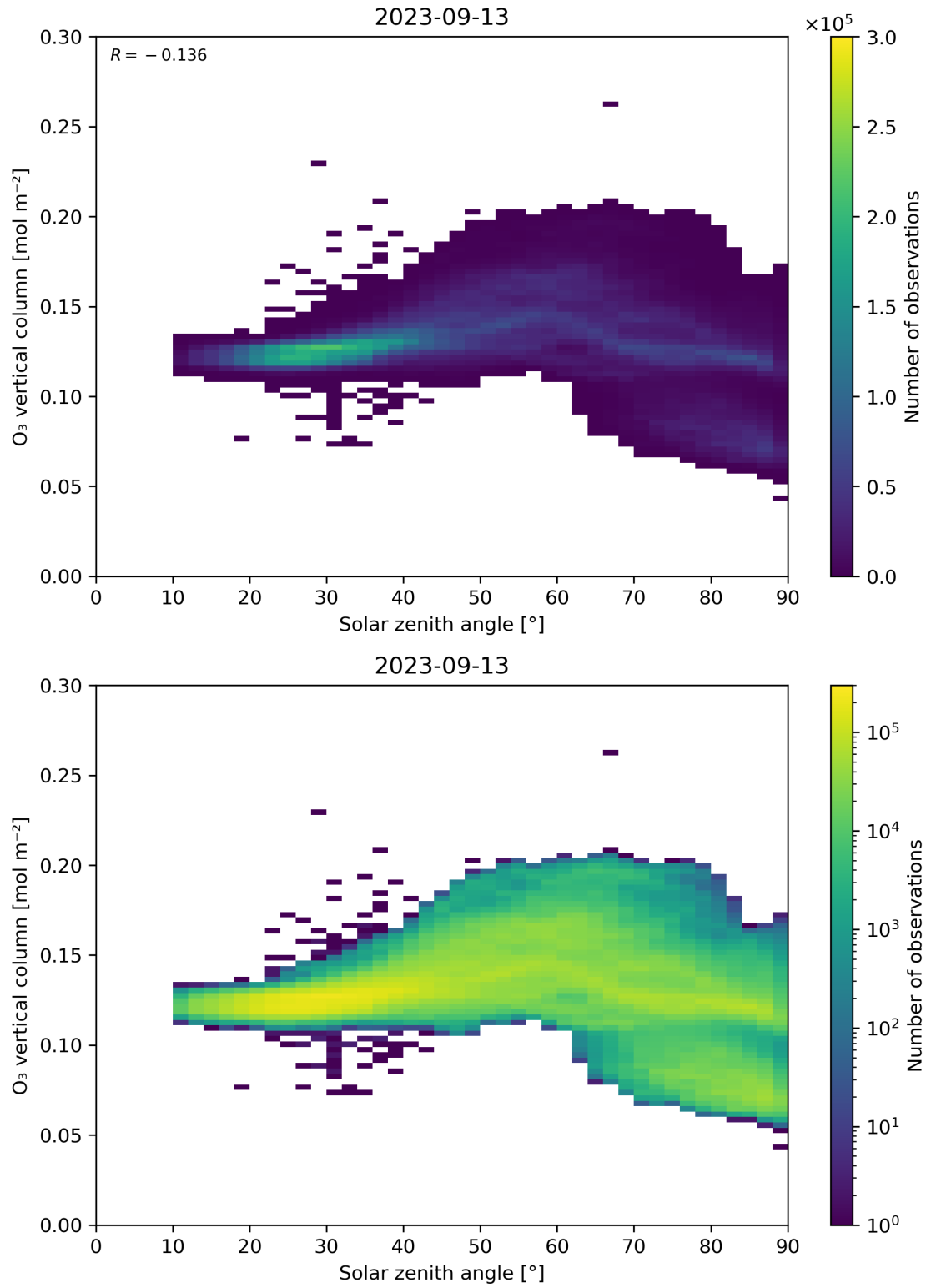
Figure 47: Scatter density plot of “Solar zenith angle” against “O 3 vertical column” for 2023-09-12 to 2023-09-14.
