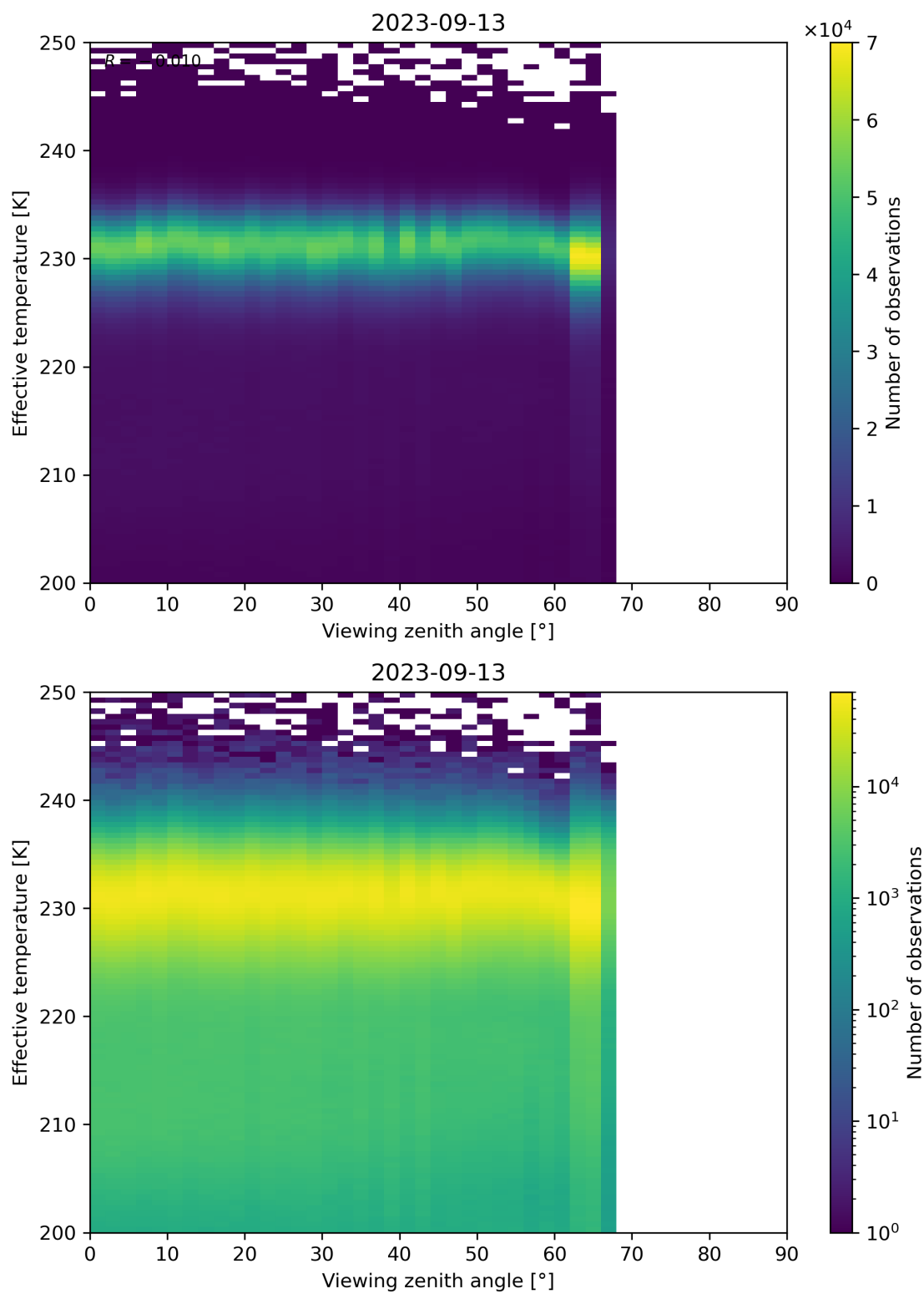
Figure 50: Scatter density plot of “Viewing zenith angle” against “Effective temperature” for 2023-09-12 to 2023-09-14.
