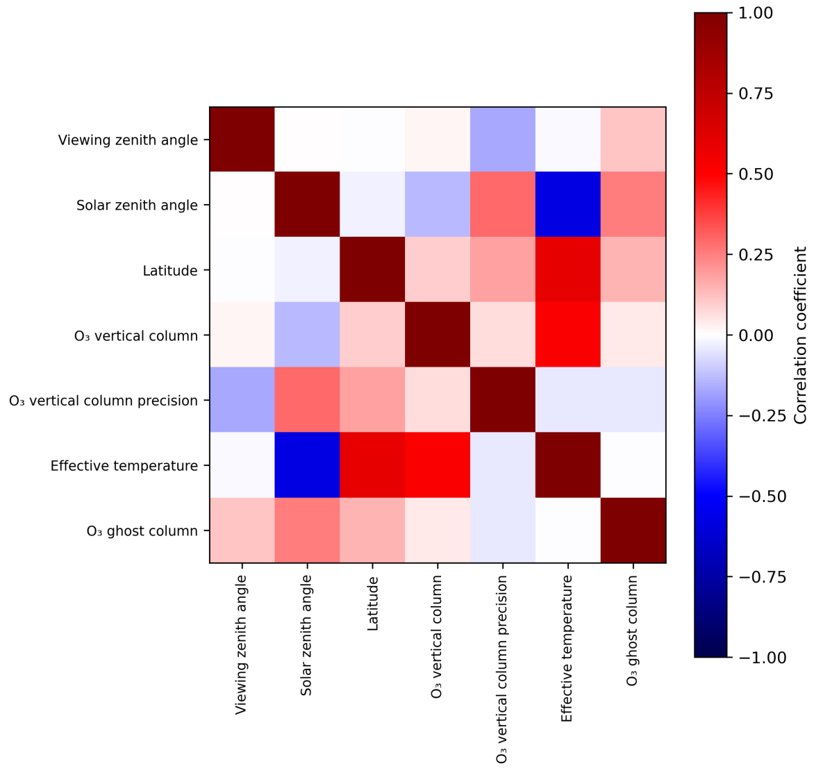
Figure 2: Map of correlation matrix for 2023-09-12 to 2023-09-14.
