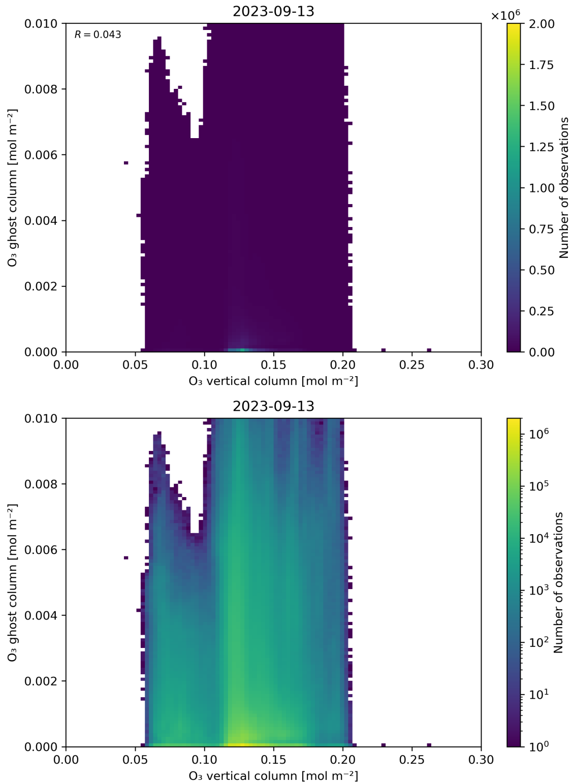
Figure 40: Scatter density plot of “O 3 vertical column” against “O 3 ghost column” for 2023-09-12 to 2023-09-14.
