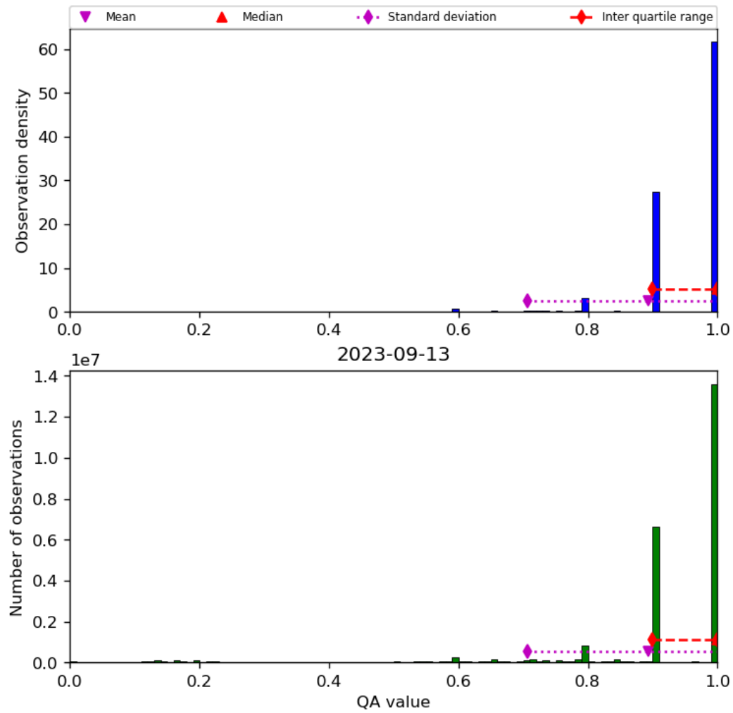
Figure 20: Histogram of “QA value” for 2023-09-12 to 2023-09-14
