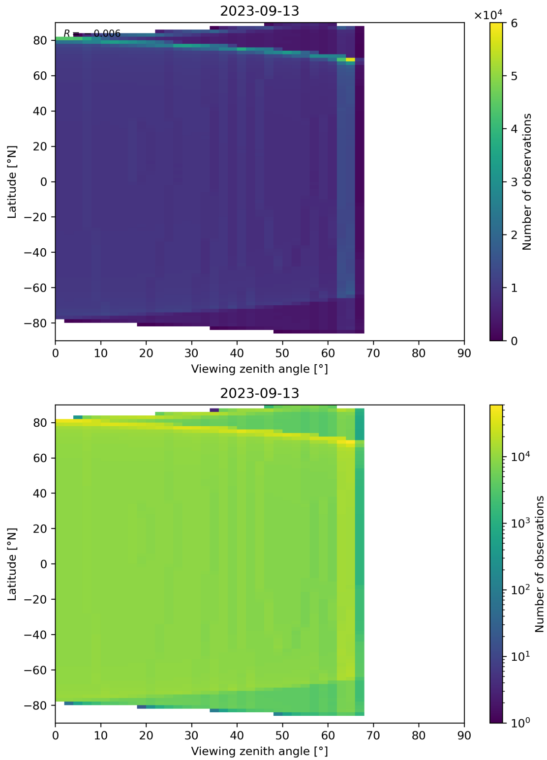
Figure 49: Scatter density plot of “Viewing zenith angle” against “Latitude” for 2023-09-12 to 2023-09-14.
