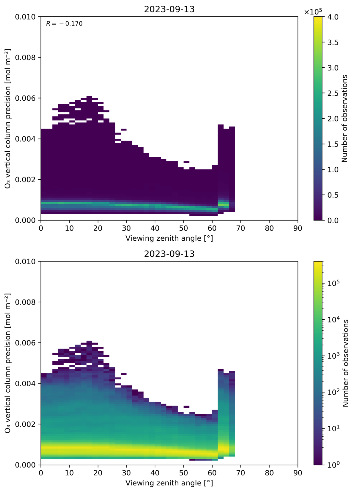
Figure 53: Scatter density plot of “Viewing zenith angle” against “O 3 vertical column precision” for 2023-09-12 to 2023-09-14.
