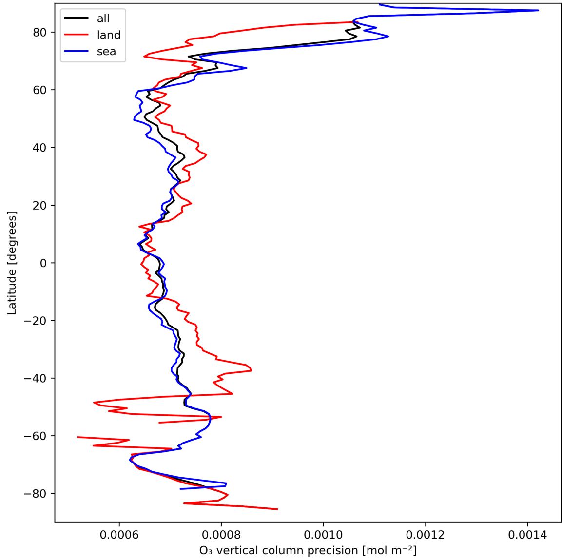
Figure 15: Zonal average of “O 3 vertical column precision” for 2023-09-12 to 2023-09-14.
