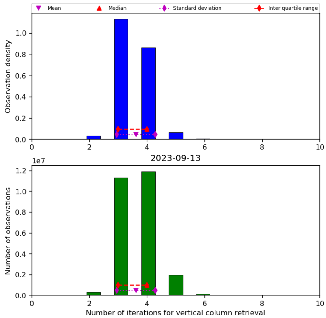
Figure 26: Histogram of “Number of iterations for vertical column retrieval” for 2023-09-12 to 2023-09-14
