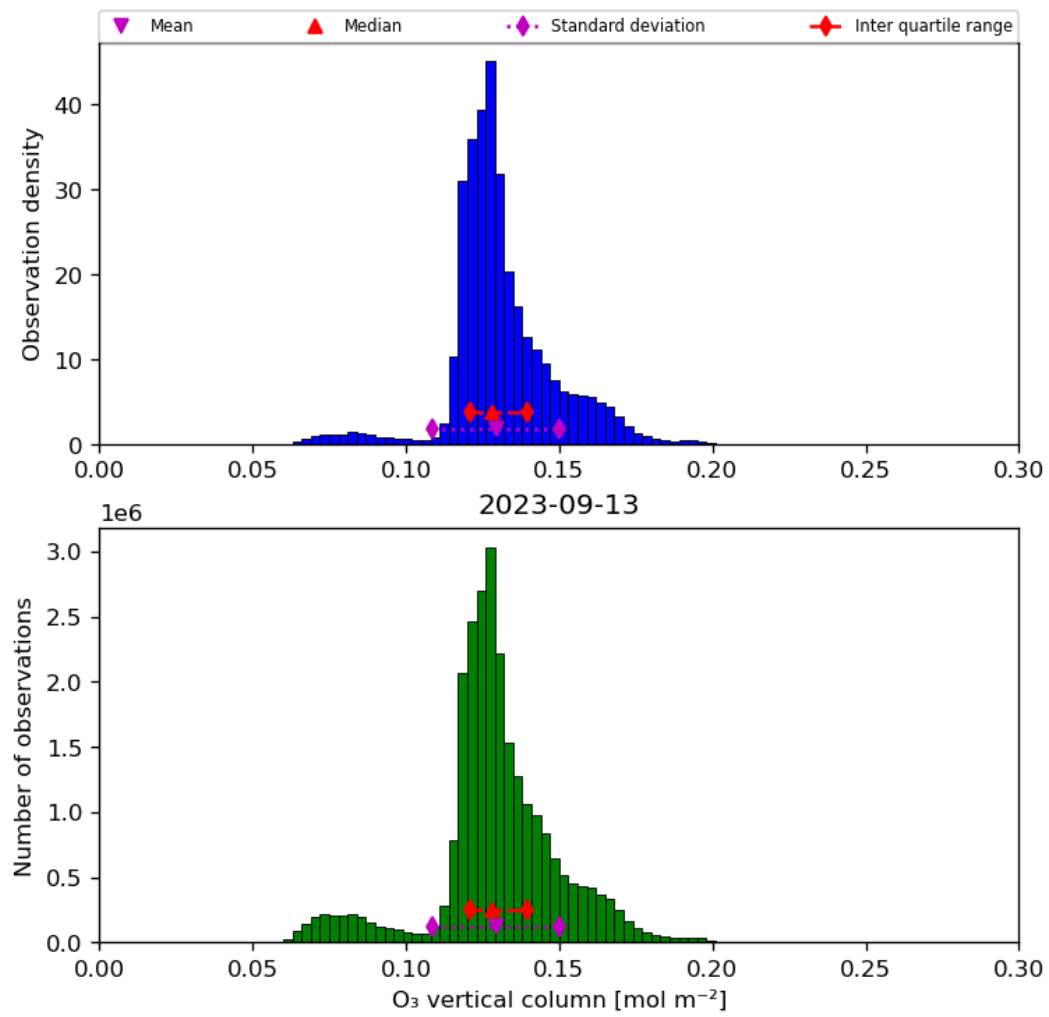
Figure 21: Histogram of “O 3 vertical column” for 2023-09-12 to 2023-09-14
