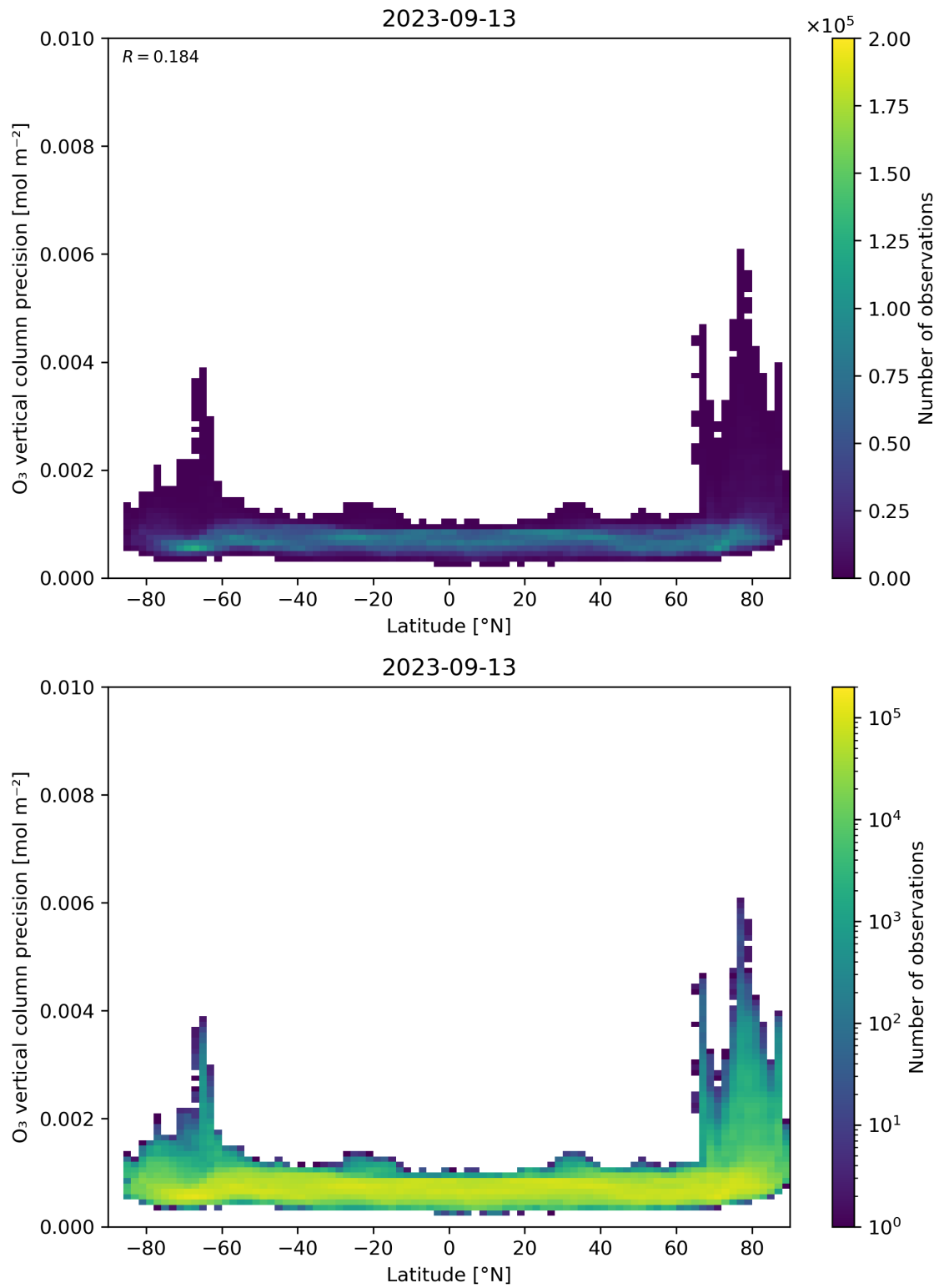
Figure 37: Scatter density plot of “Latitude” against “O 3 vertical column precision” for 2023-09-12 to 2023-09-14.
