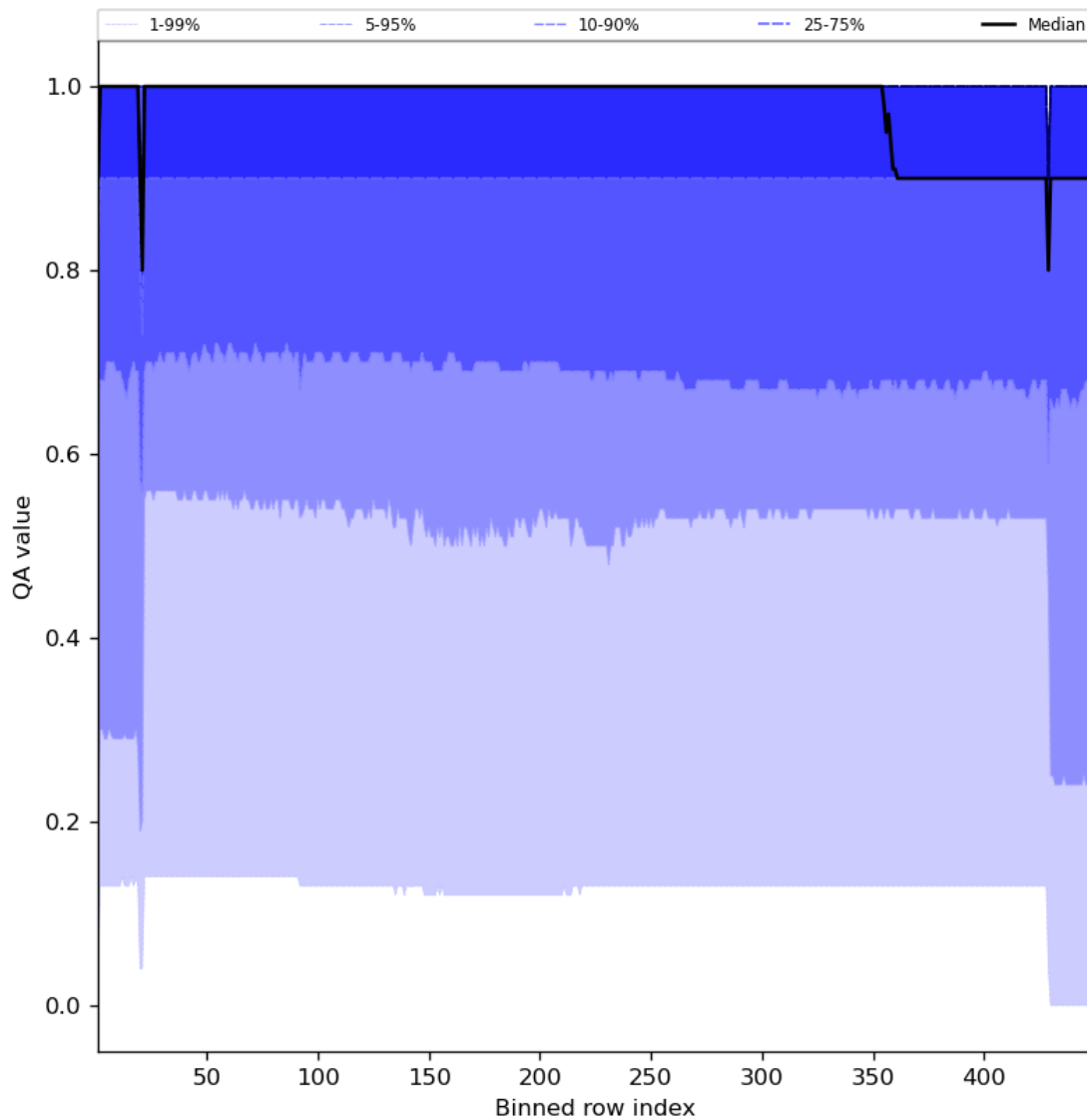
Figure 27: Along track statistics of “QA value” for 2023-09-12 to 2023-09-14
