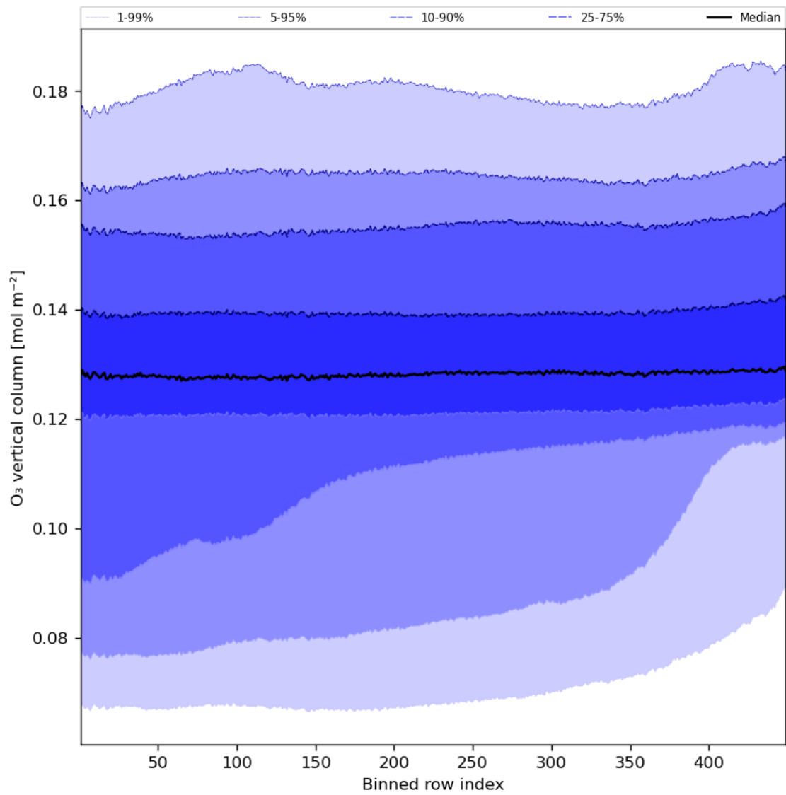
Figure 28: Along track statistics of “O 3 vertical column” for 2023-09-12 to 2023-09-14
