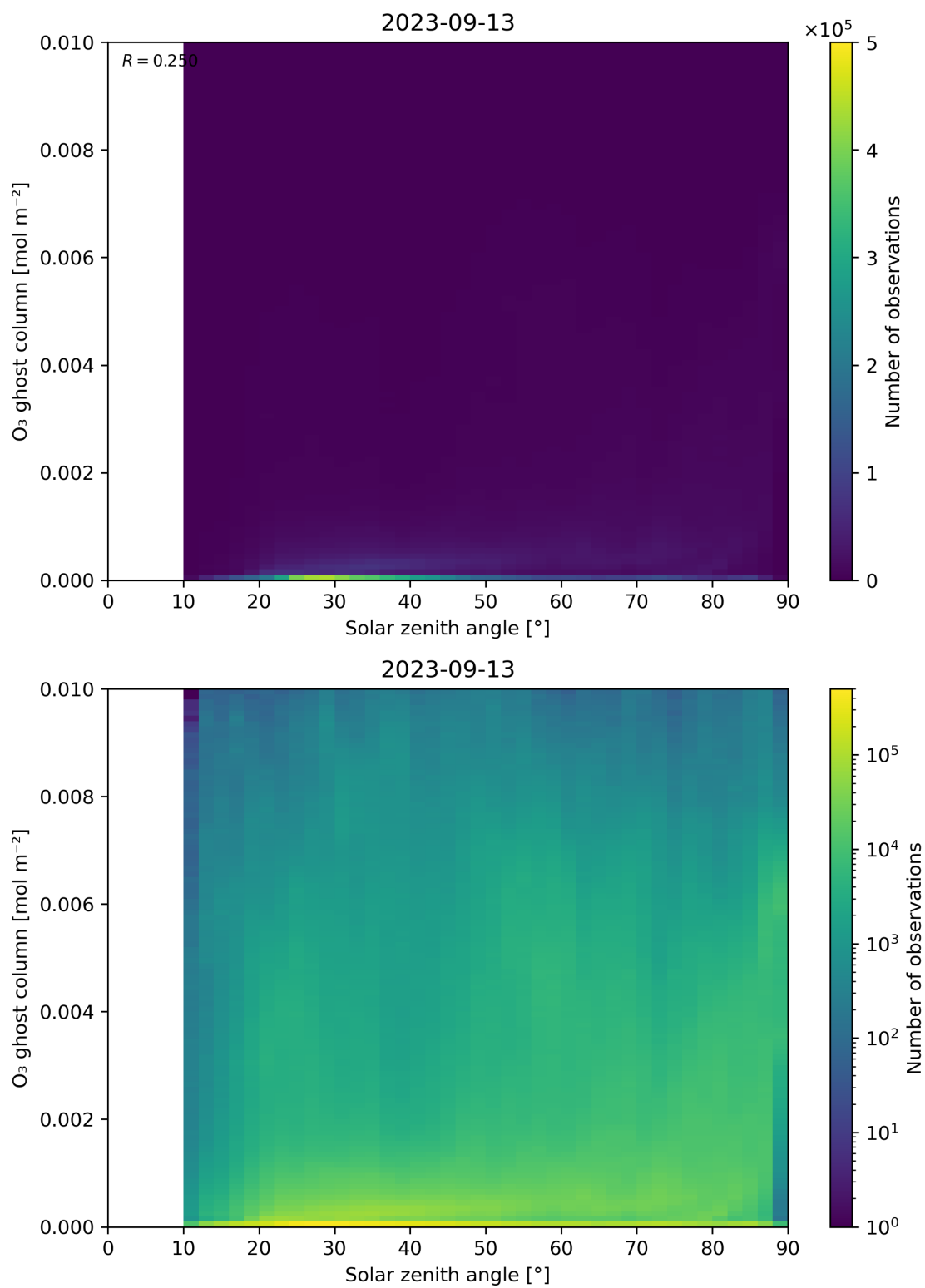
Figure 46: Scatter density plot of “Solar zenith angle” against “O 3 ghost column” for 2023-09-12 to 2023-09-14.
