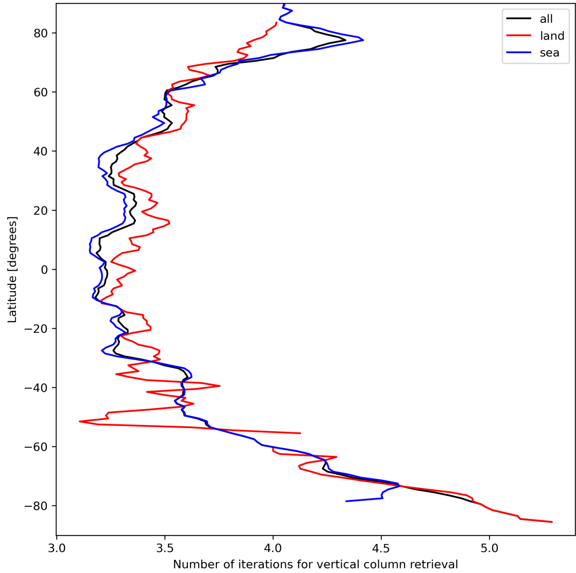
Figure 19: Zonal average of “Number of iterations for vertical column retrieval” for 2023-09-12 to 2023-09-14.
