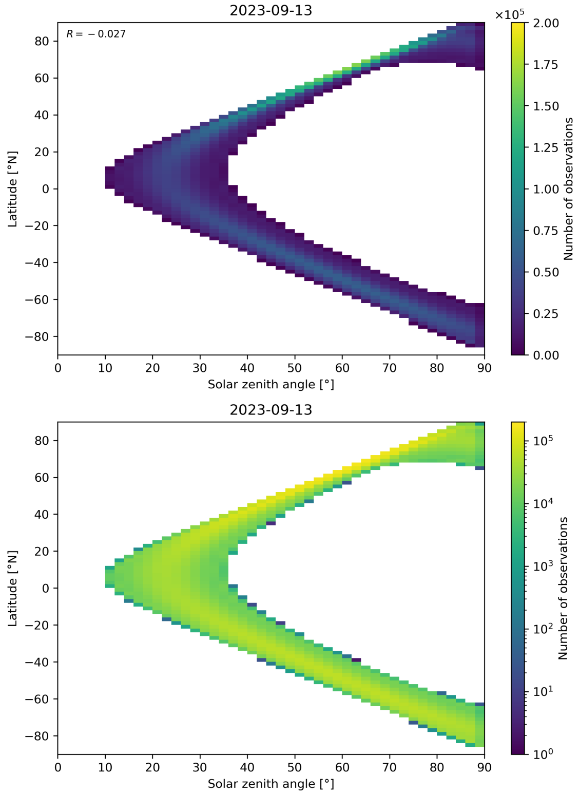
Figure 44: Scatter density plot of “Solar zenith angle” against “Latitude” for 2023-09-12 to 2023-09-14.
