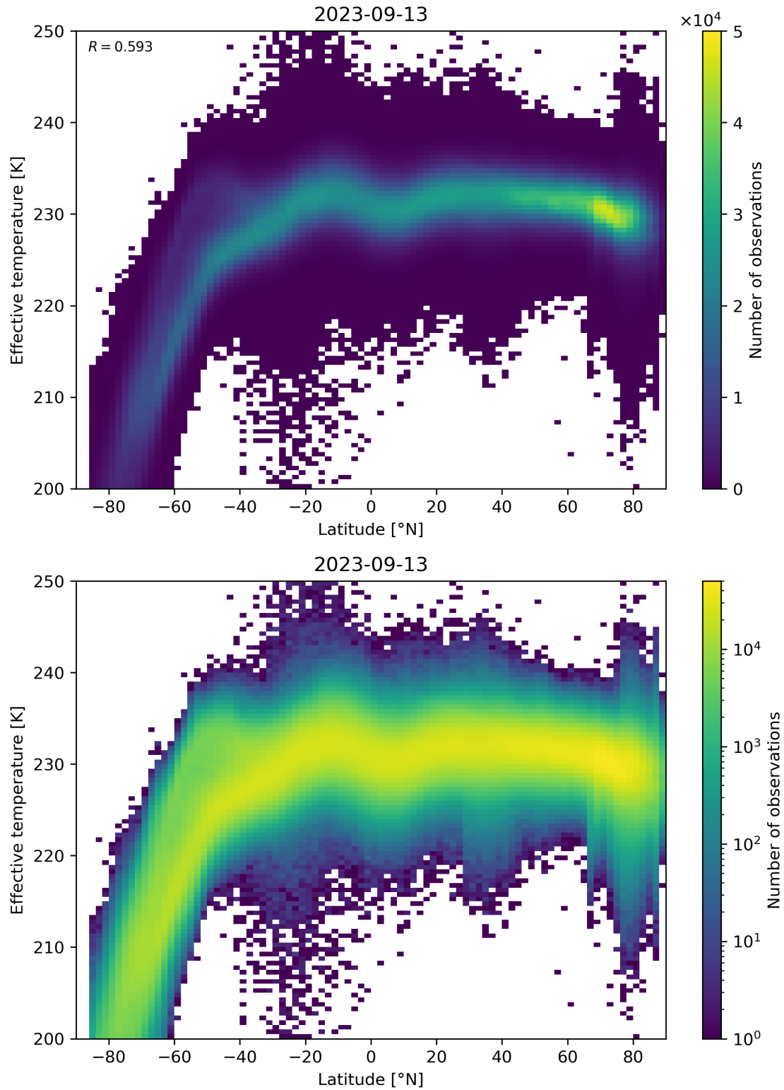
Figure 34: Scatter density plot of “Latitude” against “Effective temperature” for 2023-09-12 to 2023-09-14.
