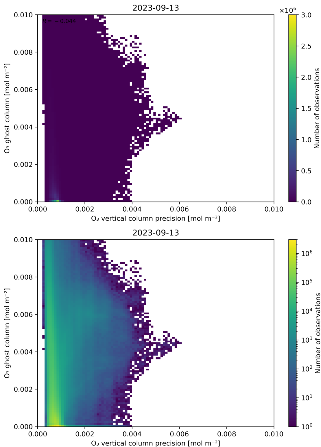
Figure 43: Scatter density plot of “ \text{O}_3 vertical column precision” against “ \text{O}_3 ghost column” for 2023-09-12 to 2023-09-14.
