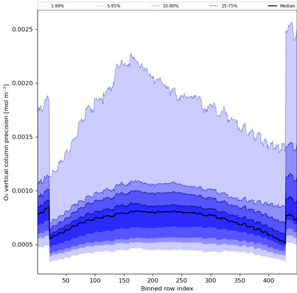
Figure 29: Along track statistics of “O 3 vertical column precision” for 2023-09-12 to 2023-09-14
