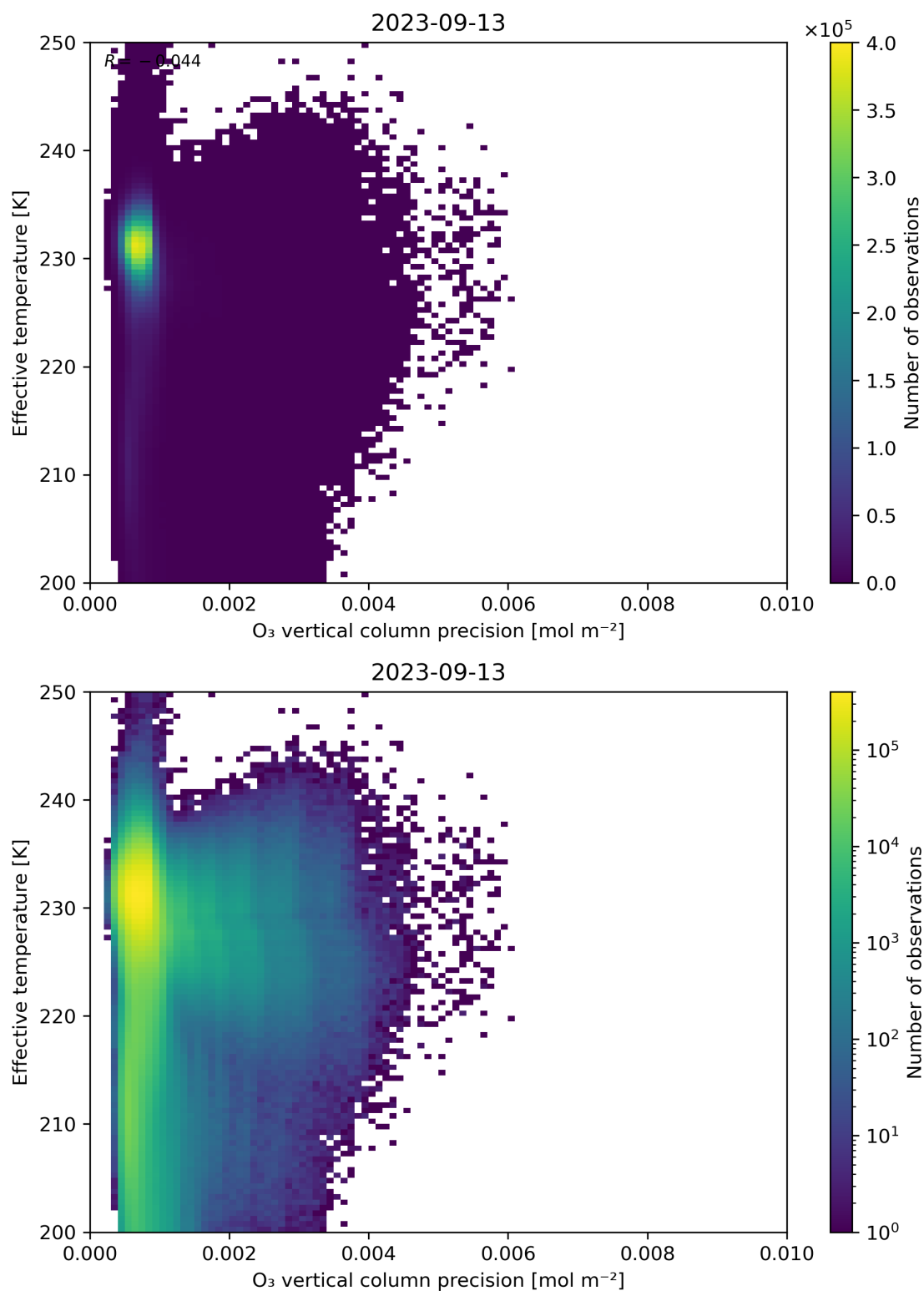
Figure 42: Scatter density plot of “O 3 vertical column precision” against “Effective temperature” for 2023-09-12 to 2023-09-14.
