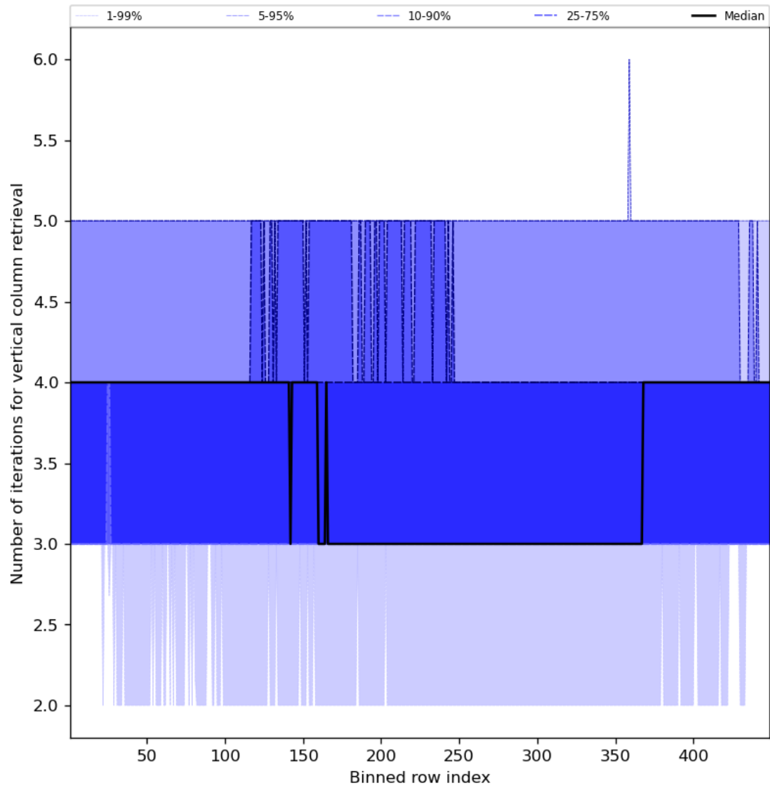
Figure 33: Along track statistics of “Number of iterations for vertical column retrieval” for 2023-09-12 to 2023-09-14
