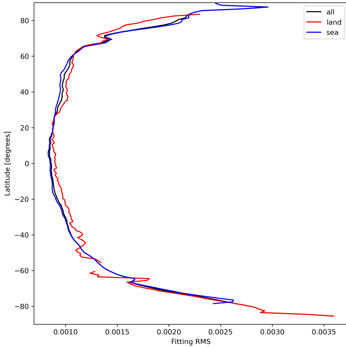
Figure 16: Zonal average of “Fitting RMS” for 2023-09-12 to 2023-09-14.
