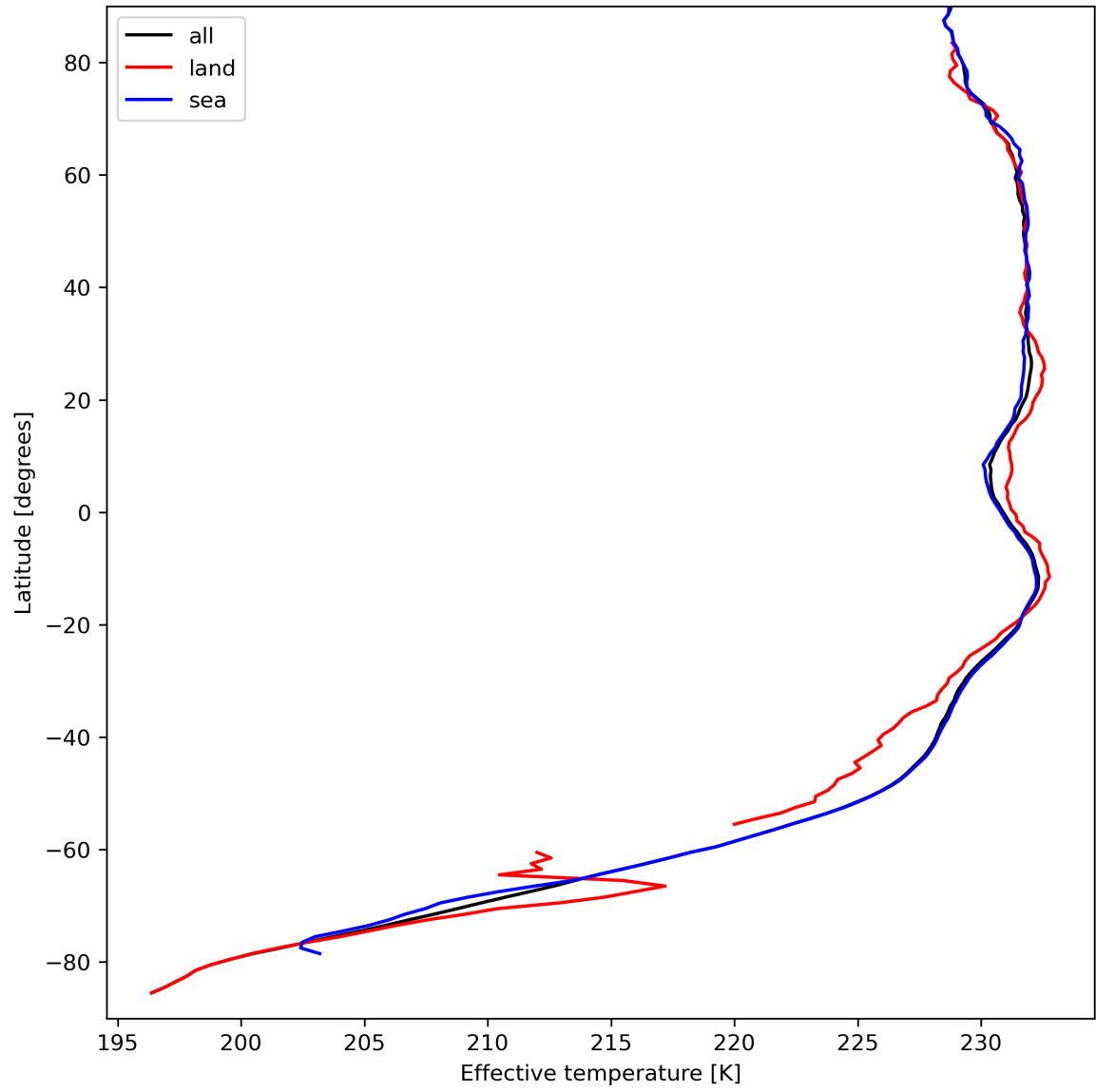
Figure 17: Zonal average of "Effective temperature" for 2023-09-12 to 2023-09-14.
