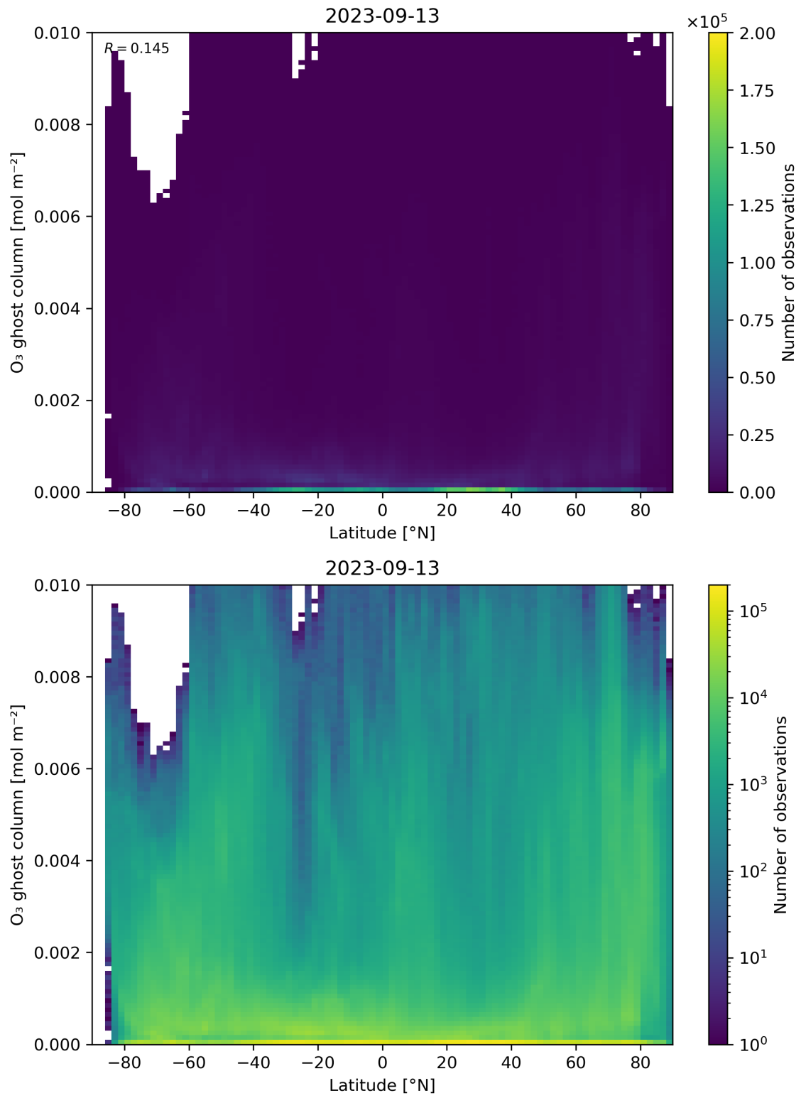
Figure 35: Scatter density plot of “Latitude” against “O 3 ghost column” for 2023-09-12 to 2023-09-14.
