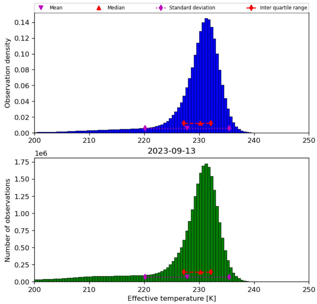
Figure 24: Histogram of “Effective temperature” for 2023-09-12 to 2023-09-14
