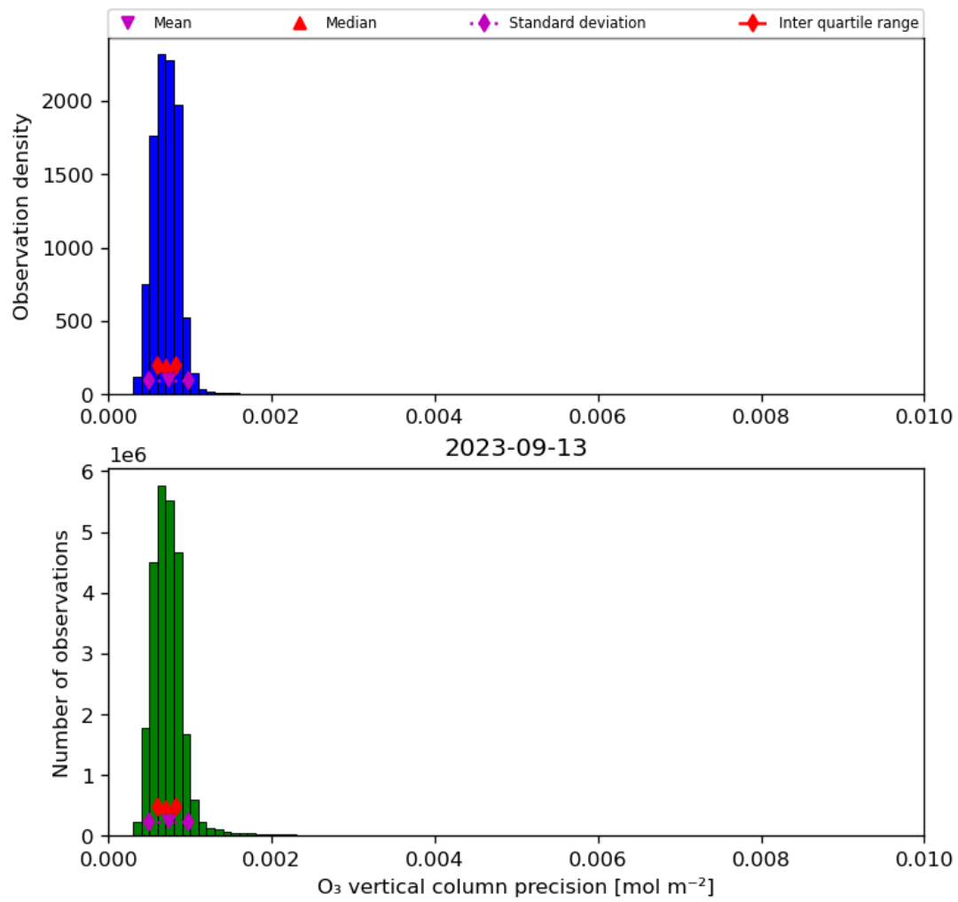
Figure 22: Histogram of “O 3 vertical column precision” for 2023-09-12 to 2023-09-14
