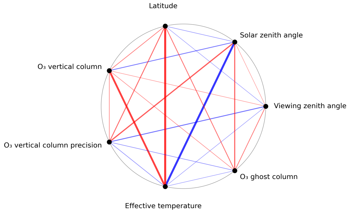
Figure 1: Map of correlation graph for 2023-09-12 to 2023-09-14.
