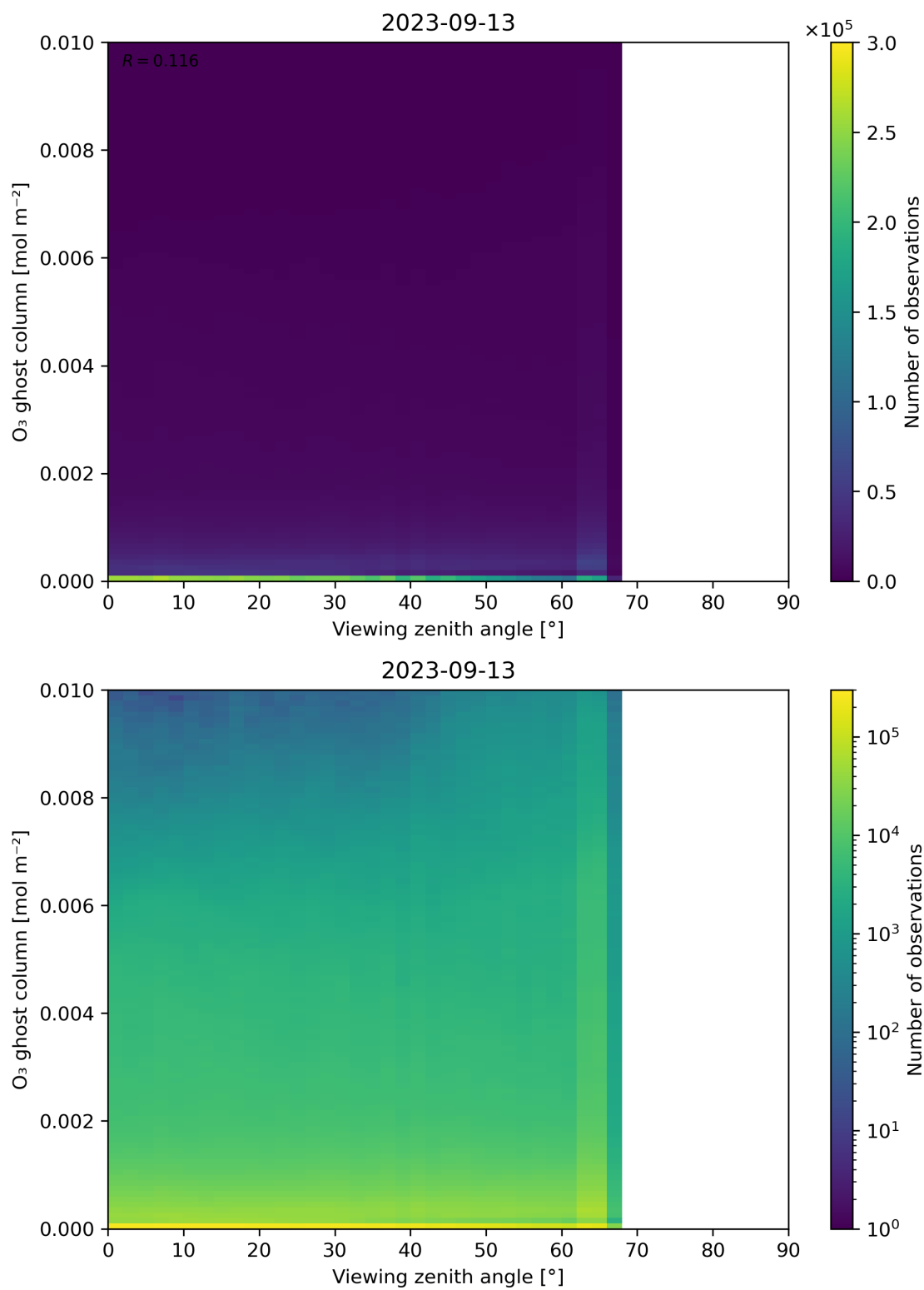
Figure 51: Scatter density plot of “Viewing zenith angle” against “O 3 ghost column” for 2023-09-12 to 2023-09-14.
