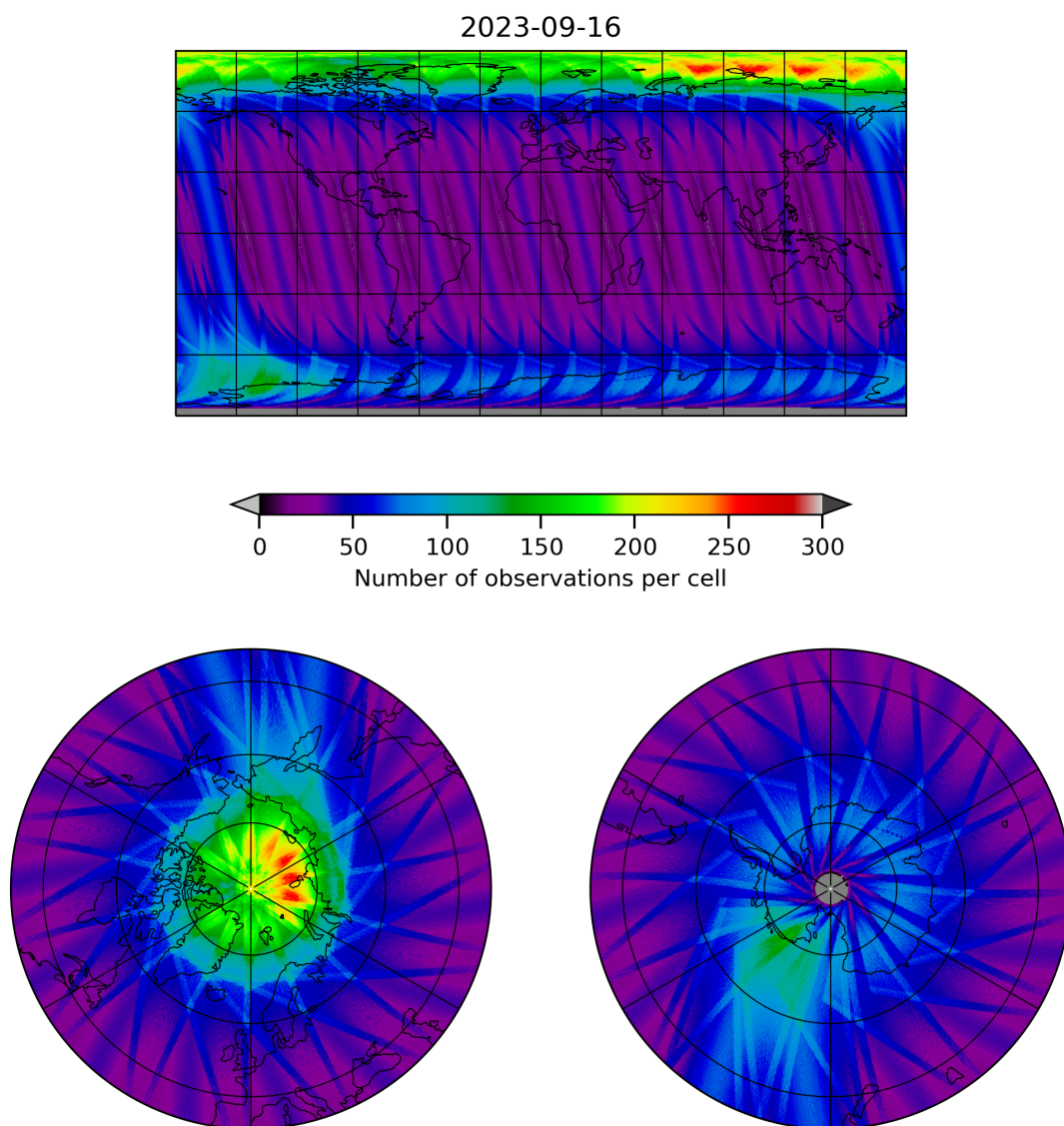
Figure 12: Map of the number of observations for 2023-09-15 to 2023-09-17
