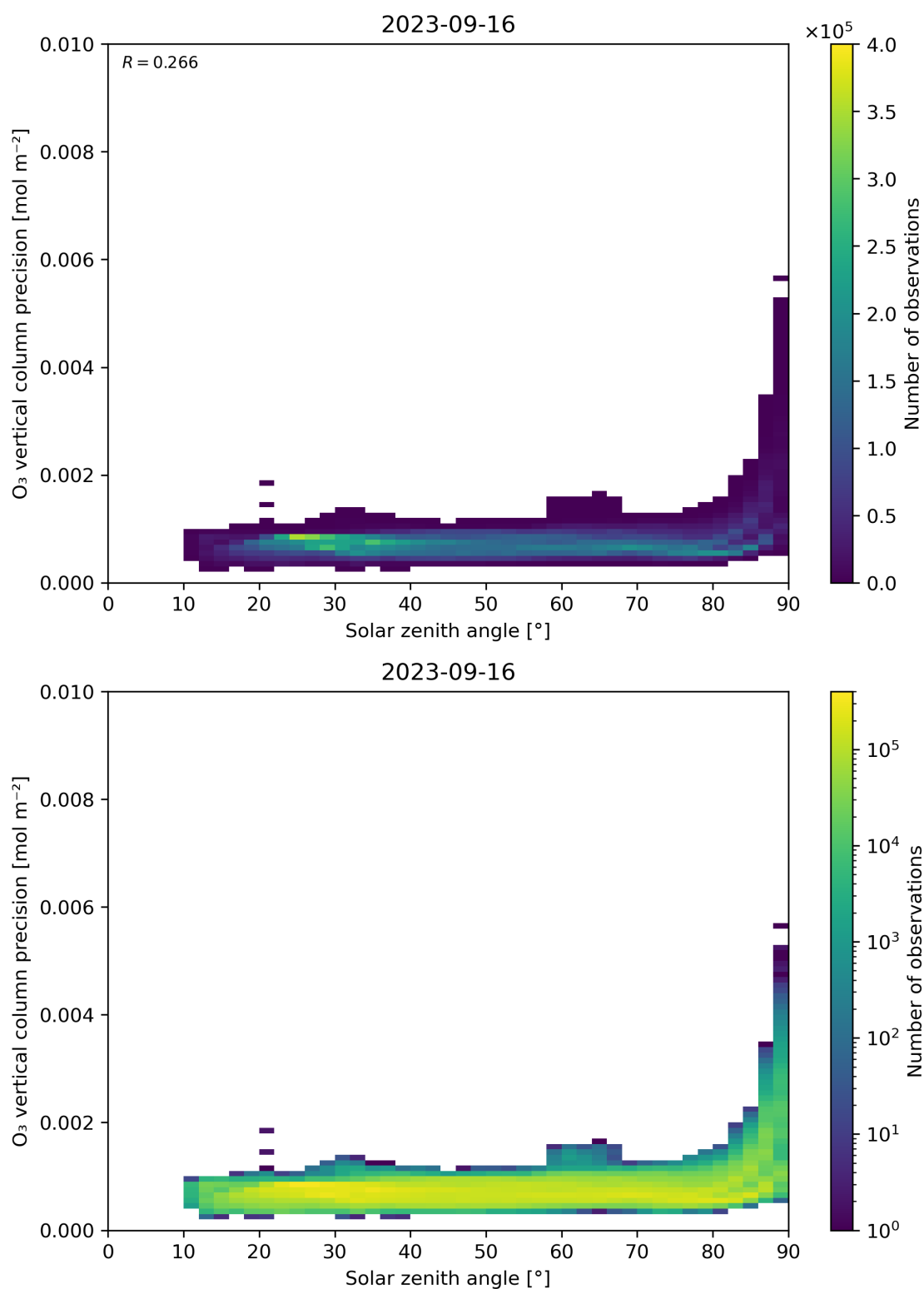
Figure 48: Scatter density plot of “Solar zenith angle” against “O 3 vertical column precision” for 2023-09-15 to 2023-09-17.
