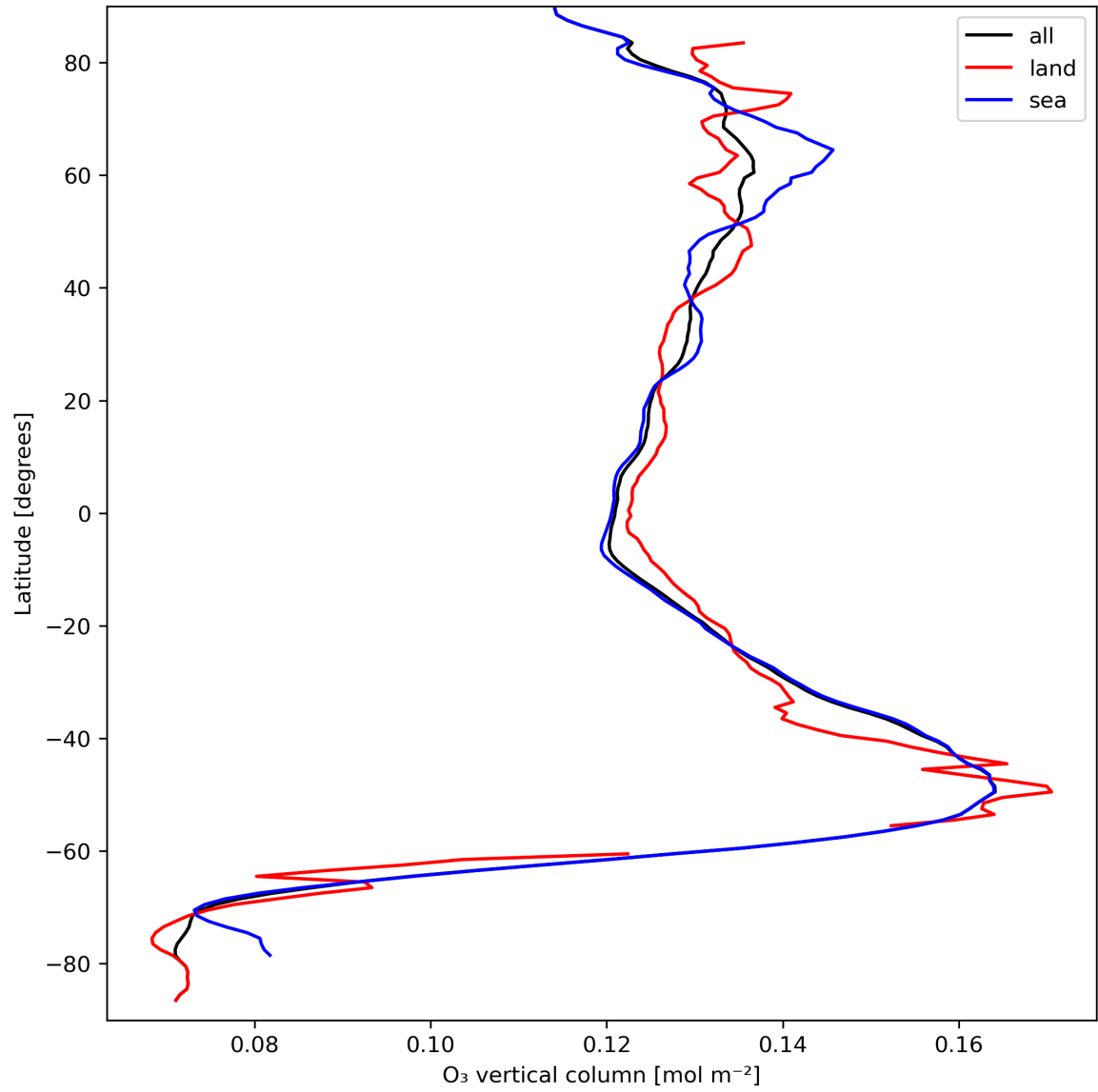
Figure 14: Zonal average of “O 3 vertical column” for 2023-09-15 to 2023-09-17.
