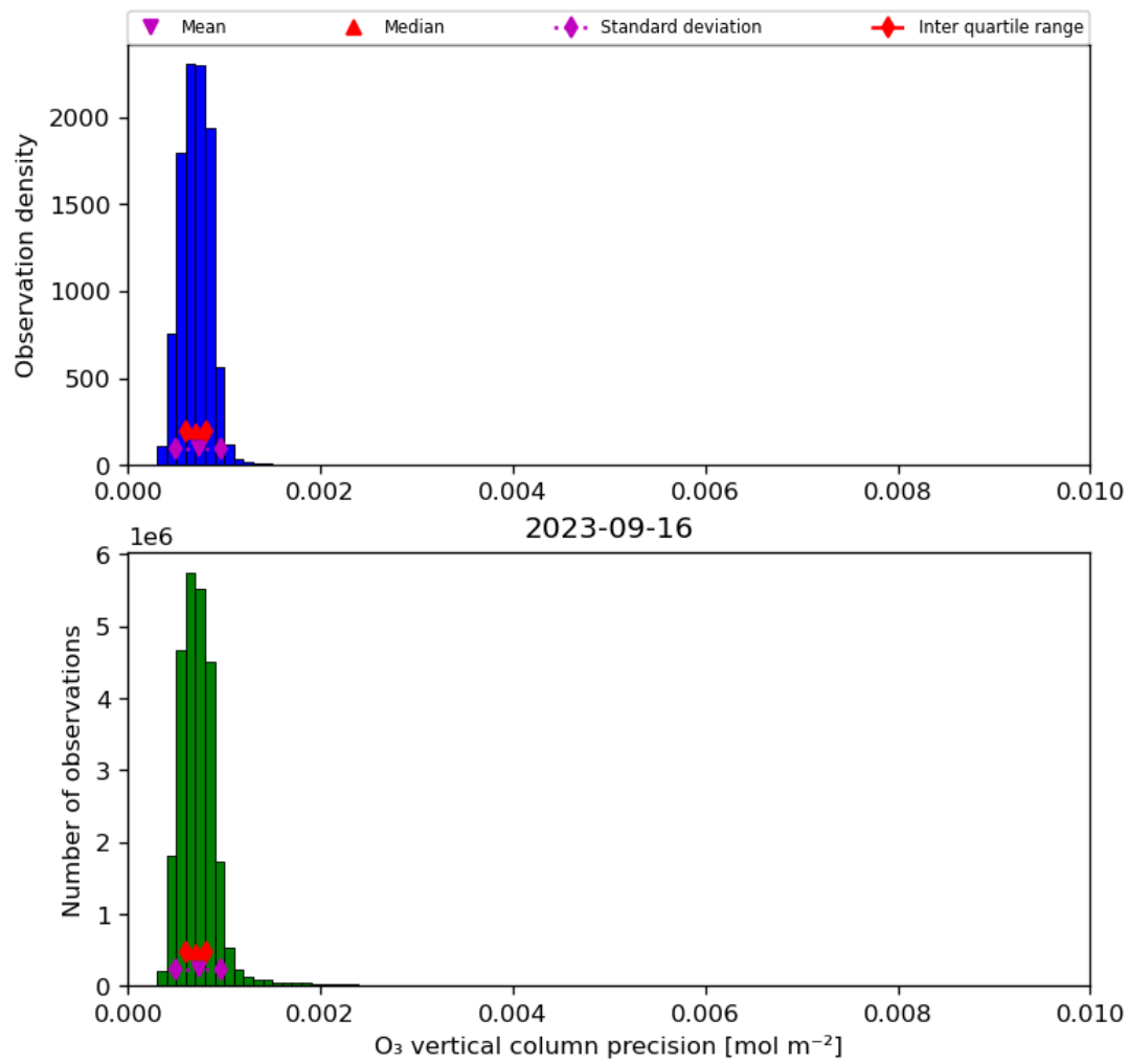
Figure 22: Histogram of “O 3 vertical column precision” for 2023-09-15 to 2023-09-17
