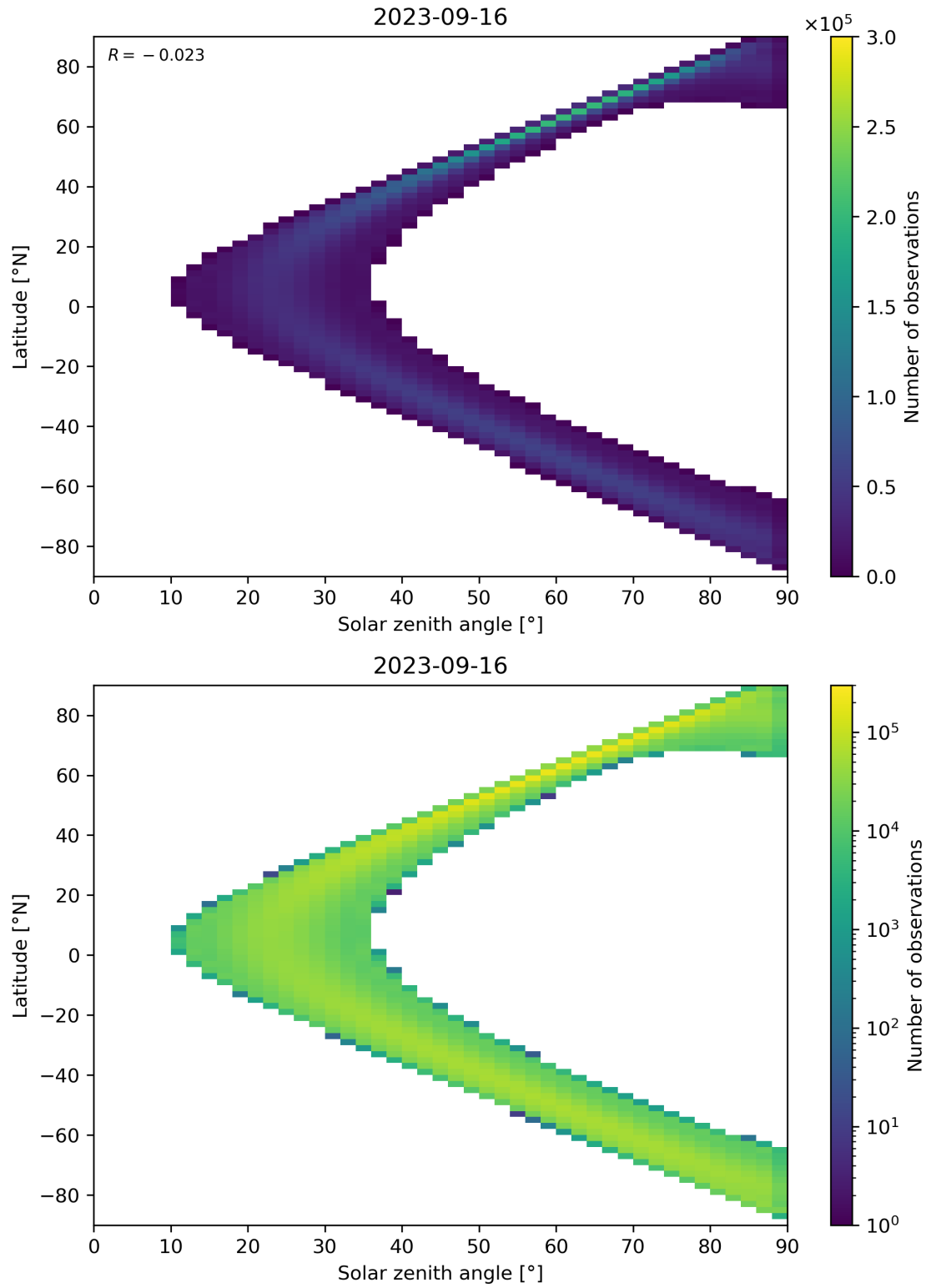
Figure 44: Scatter density plot of “Solar zenith angle” against “Latitude” for 2023-09-15 to 2023-09-17.
