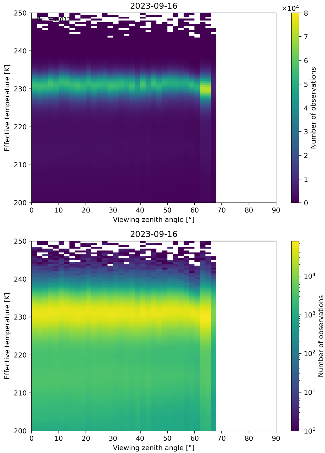
Figure 50: Scatter density plot of “Viewing zenith angle” against “Effective temperature” for 2023-09-15 to 2023-09-17.
