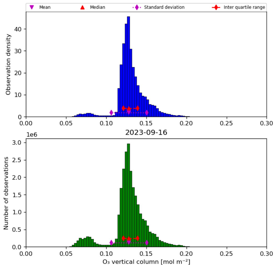
Figure 21: Histogram of “O 3 vertical column” for 2023-09-15 to 2023-09-17
