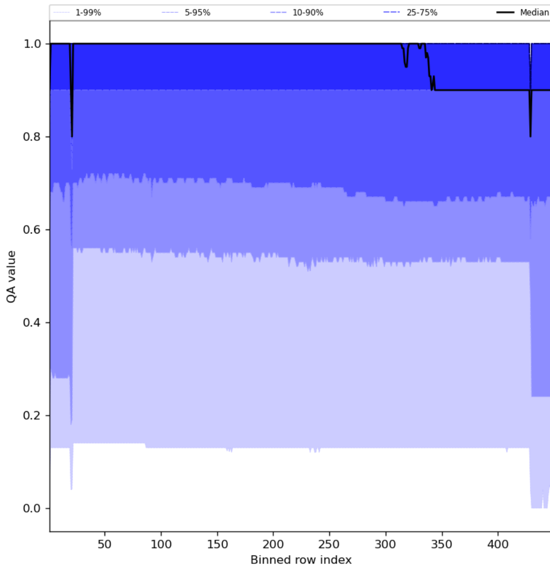
Figure 27: Along track statistics of “QA value” for 2023-09-15 to 2023-09-17
