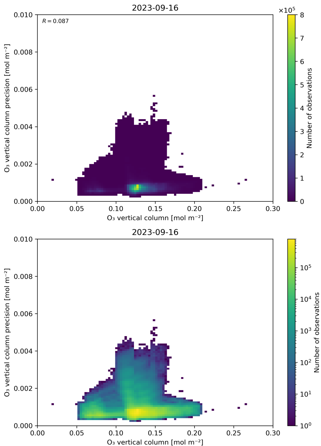
Figure 41: Scatter density plot of “O 3 vertical column” against “O 3 vertical column precision” for 2023-09-15 to 2023-09-17.
