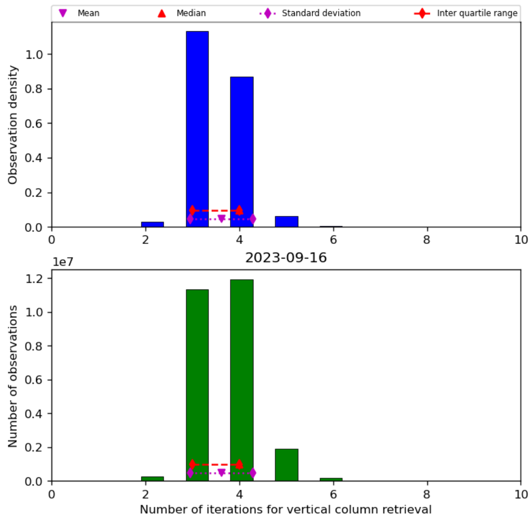
Figure 26: Histogram of “Number of iterations for vertical column retrieval” for 2023-09-15 to 2023-09-17
