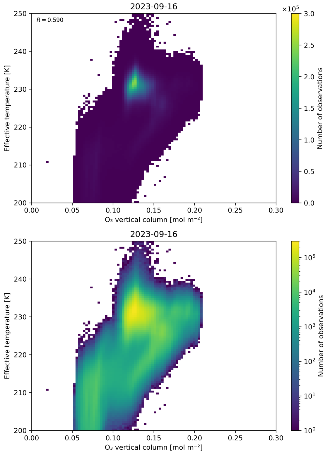
Figure 39: Scatter density plot of “O 3 vertical column” against “Effective temperature” for 2023-09-15 to 2023-09-17.
