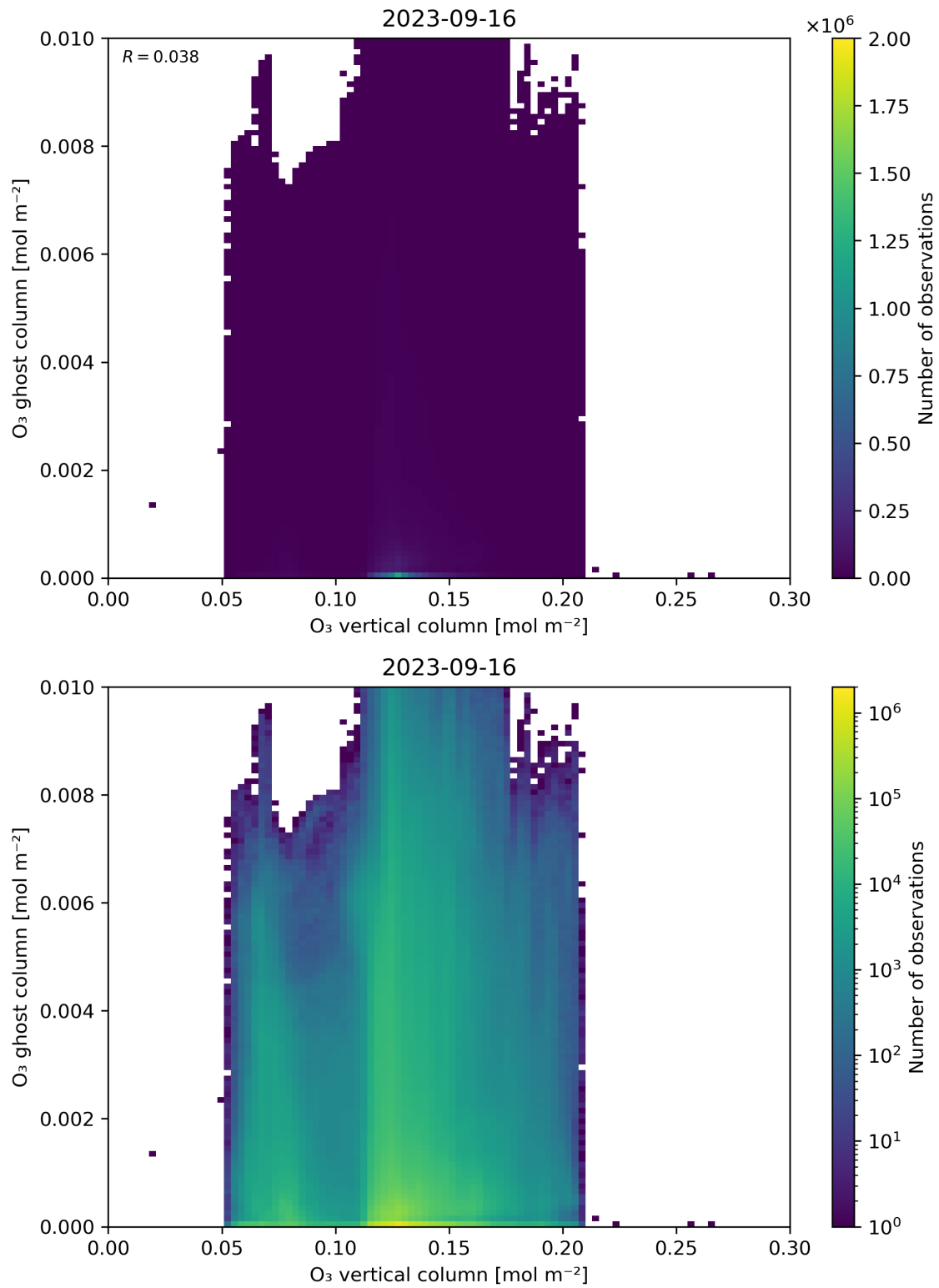
Figure 40: Scatter density plot of “O 3 vertical column” against “O 3 ghost column” for 2023-09-15 to 2023-09-17.
