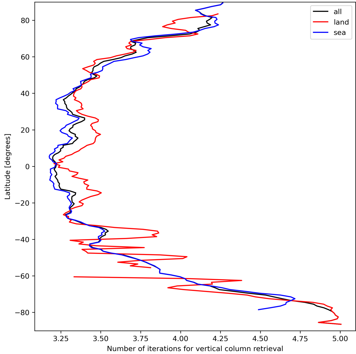
Figure 19: Zonal average of “Number of iterations for vertical column retrieval” for 2023-09-15 to 2023-09-17.
