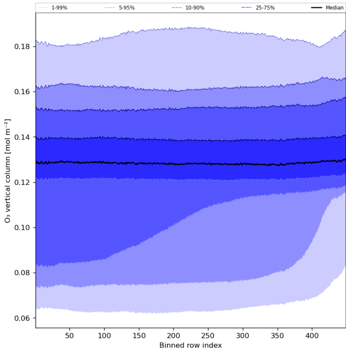
Figure 28: Along track statistics of “O 3 vertical column” for 2023-09-15 to 2023-09-17
