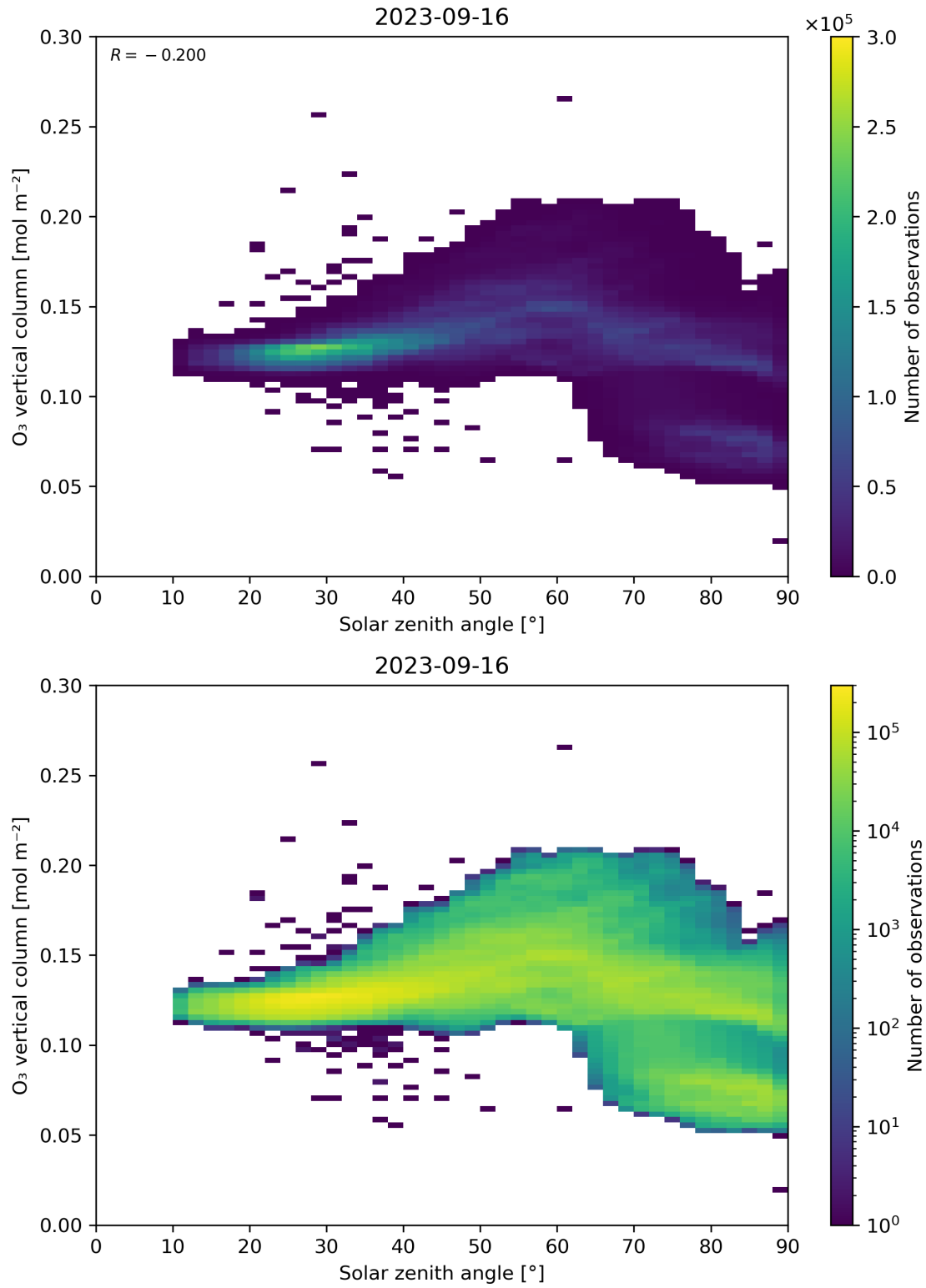
Figure 47: Scatter density plot of “Solar zenith angle” against “O 3 vertical column” for 2023-09-15 to 2023-09-17.
