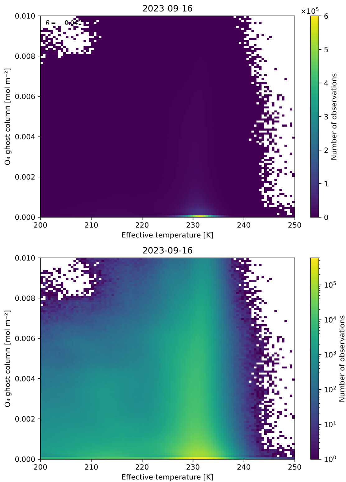
Figure 38: Scatter density plot of “Effective temperature” against “O 3 ghost column” for 2023-09-15 to 2023-09-17.
