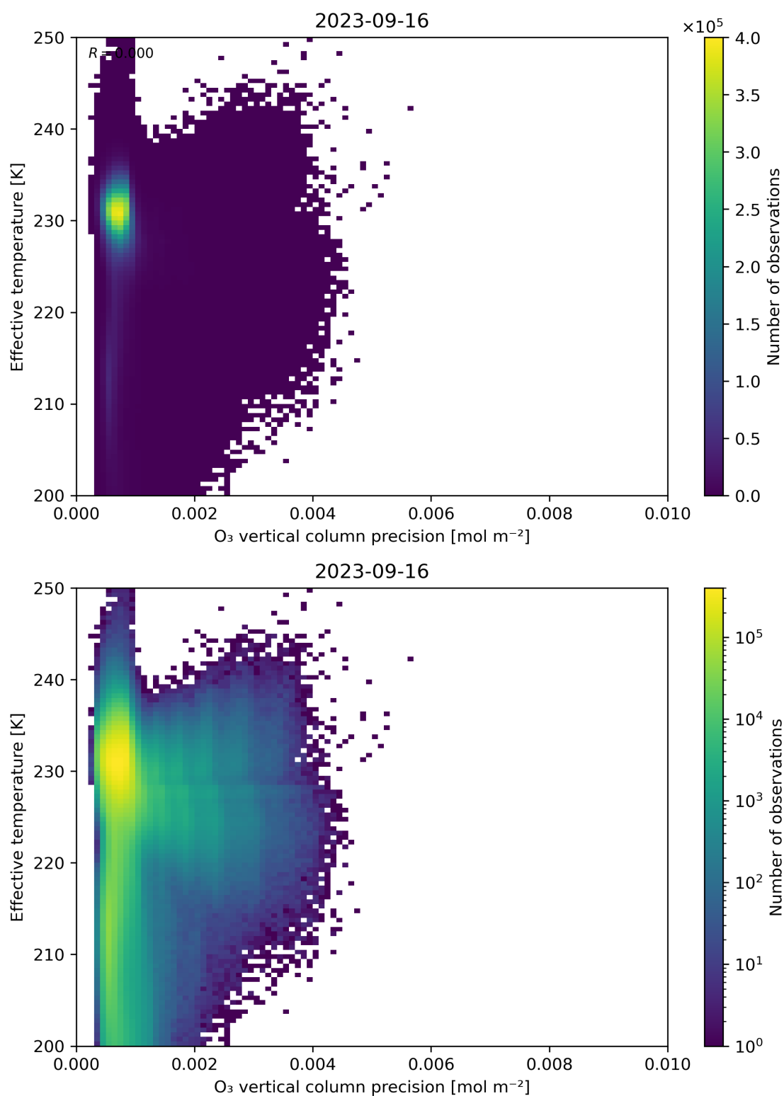
Figure 42: Scatter density plot of “O 3 vertical column precision” against “Effective temperature” for 2023-09-15 to 2023-09-17.
