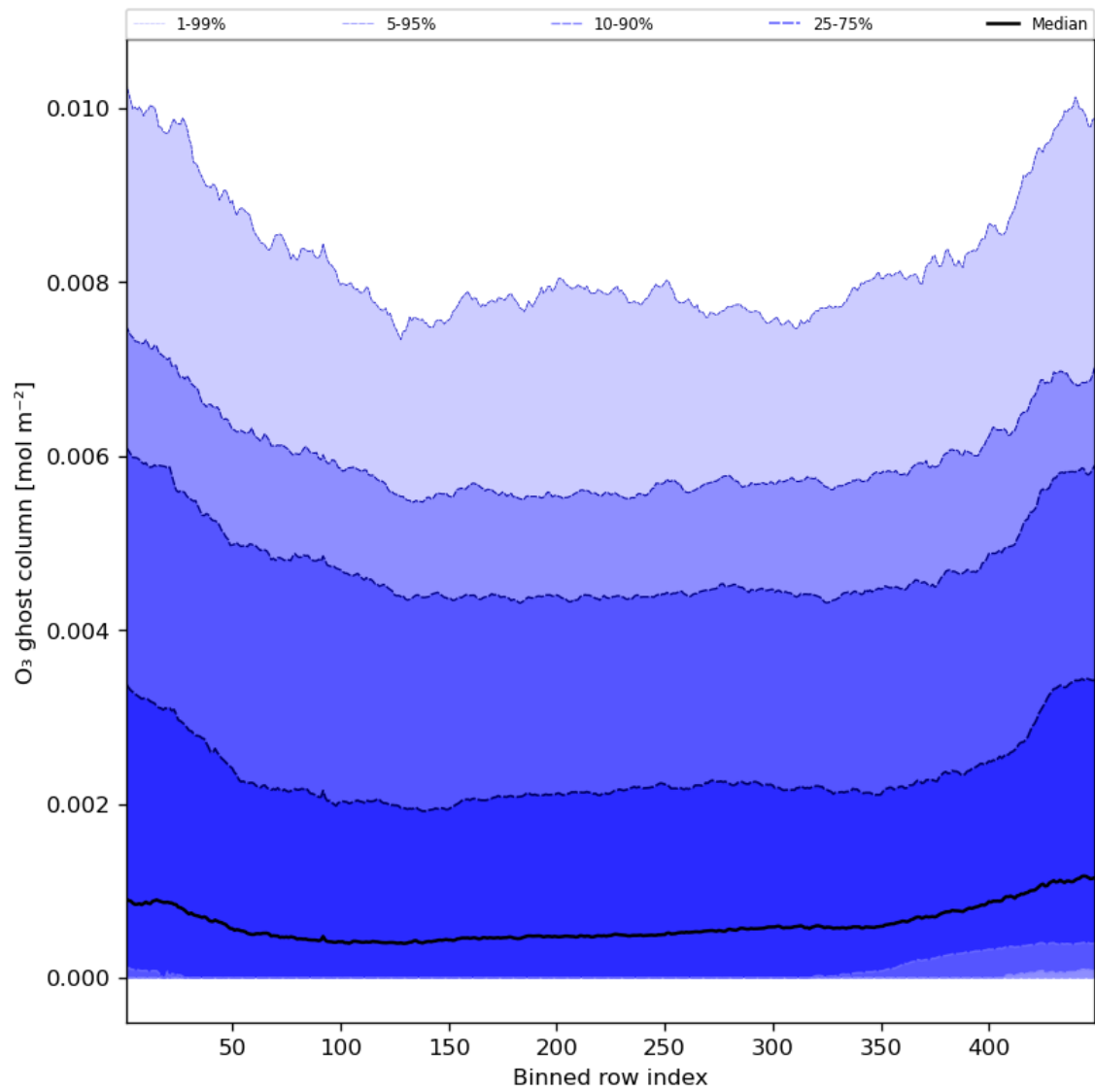
Figure 32: Along track statistics of “O 3 ghost column” for 2023-09-15 to 2023-09-17
