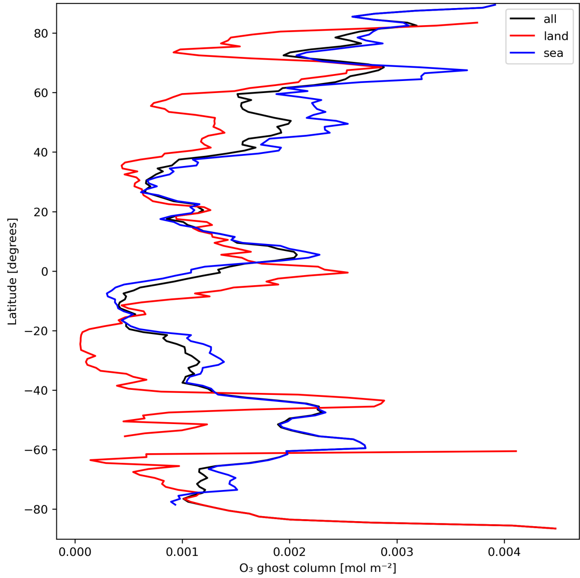
Figure 18: Zonal average of "O 3 ghost column" for 2023-09-15 to 2023-09-17.
