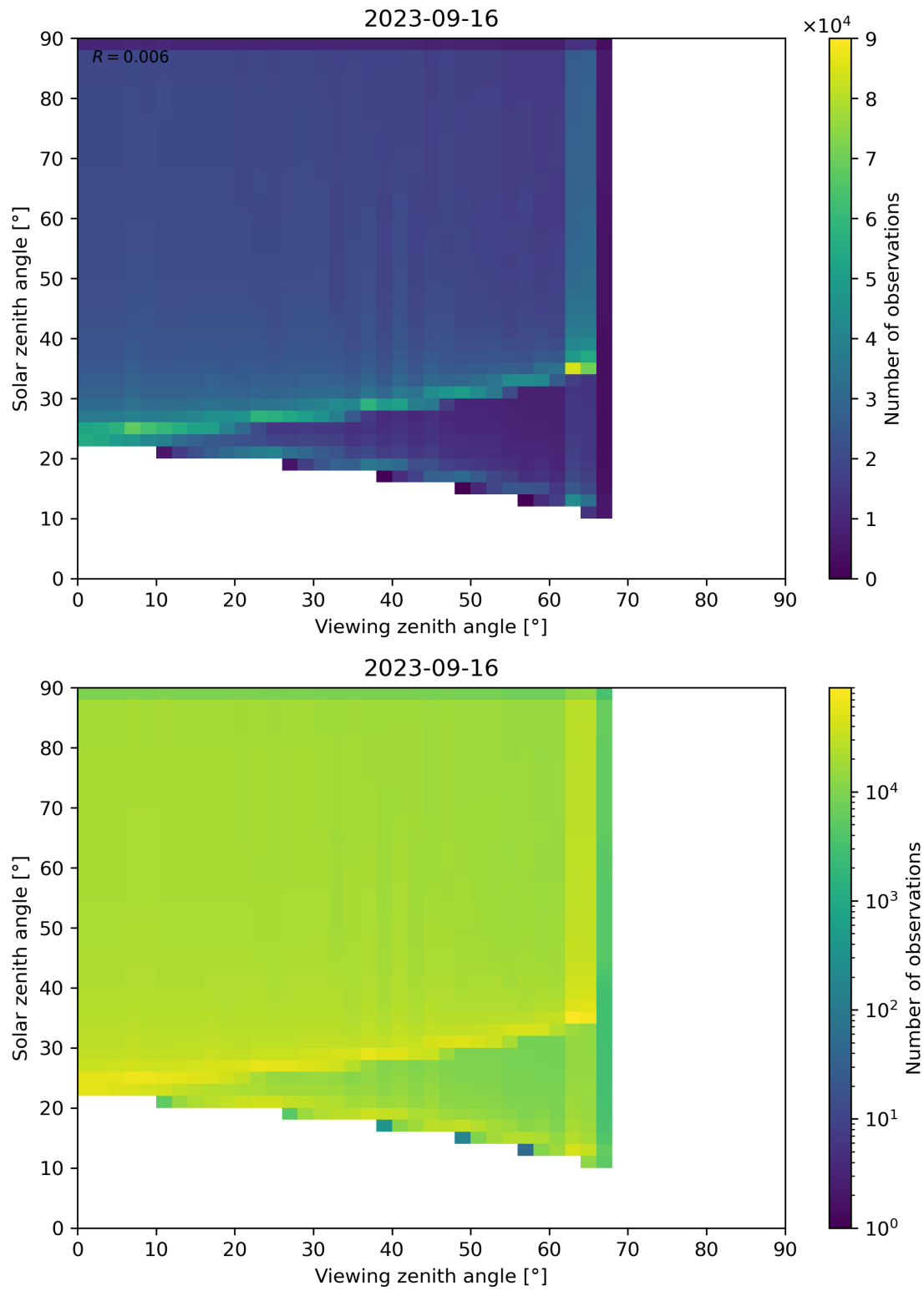
Figure 54: Scatter density plot of “Viewing zenith angle” against “Solar zenith angle” for 2023-09-15 to 2023-09-17.
