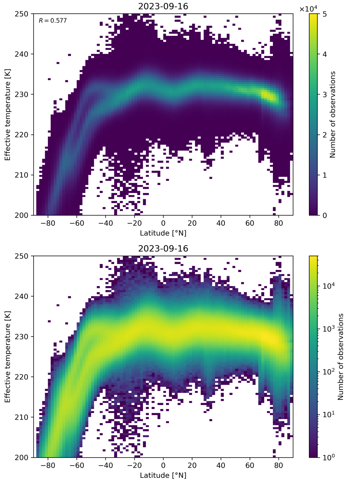
Figure 34: Scatter density plot of “Latitude” against “Effective temperature” for 2023-09-15 to 2023-09-17.
