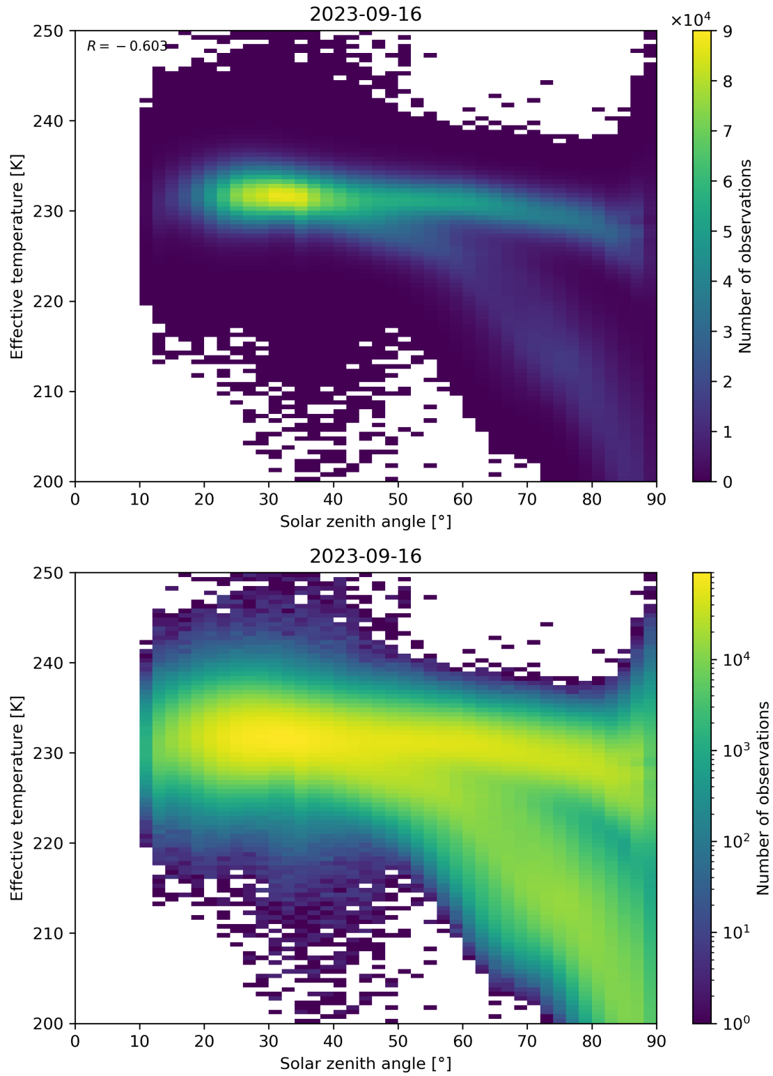
Figure 45: Scatter density plot of “Solar zenith angle” against “Effective temperature” for 2023-09-15 to 2023-09-17.
