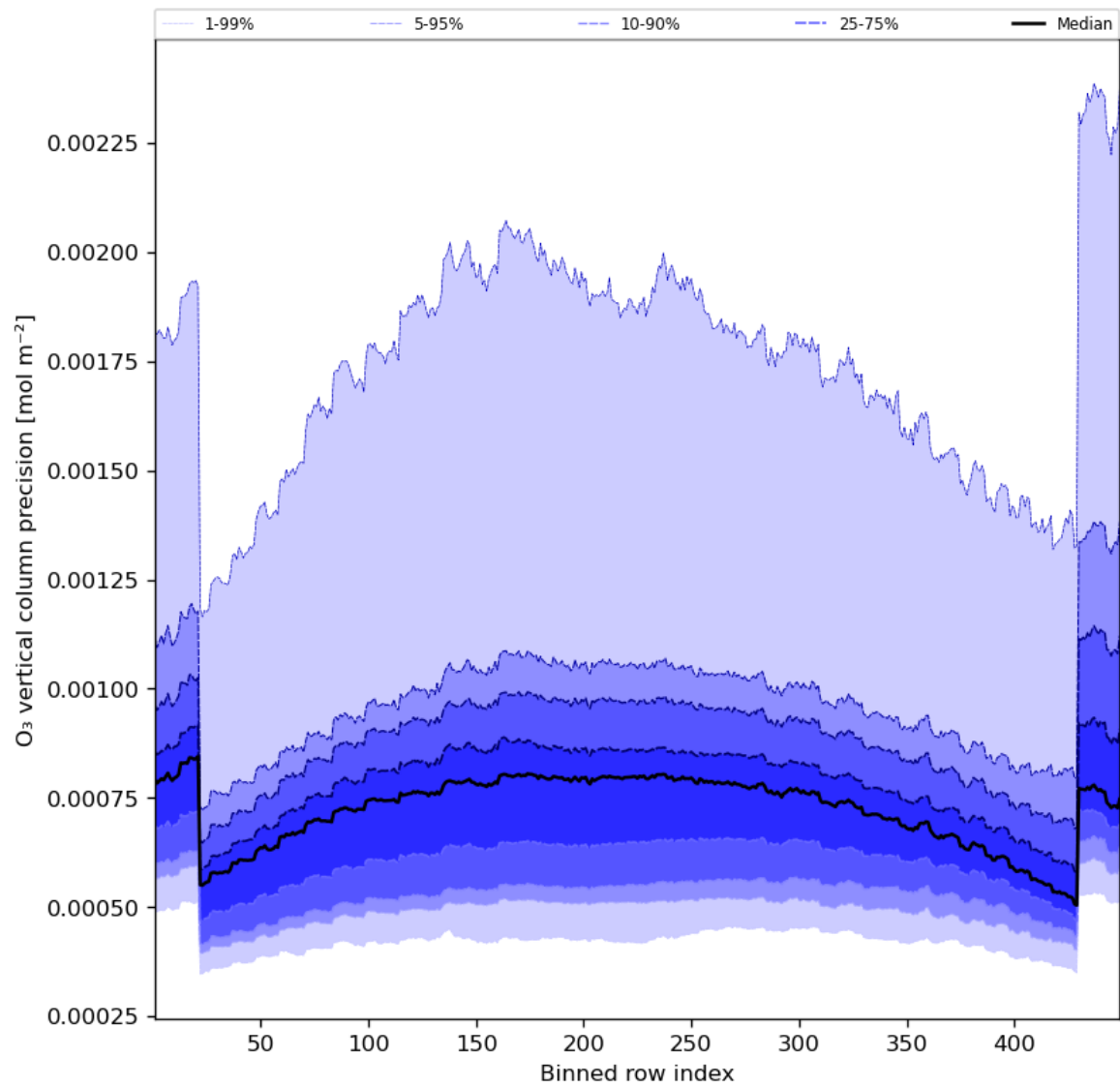
Figure 29: Along track statistics of “O 3 vertical column precision” for 2023-09-15 to 2023-09-17
