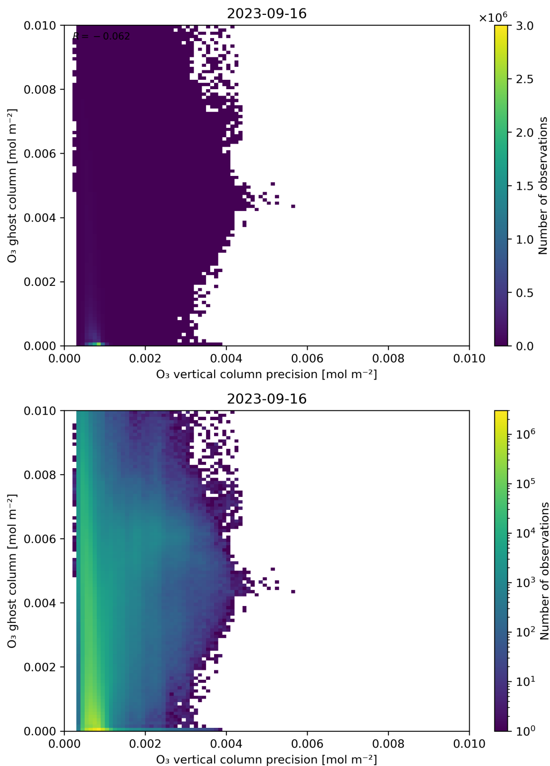
Figure 43: Scatter density plot of “ O_3 vertical column precision” against “ O_3 ghost column” for 2023-09-15 to 2023-09-17.
