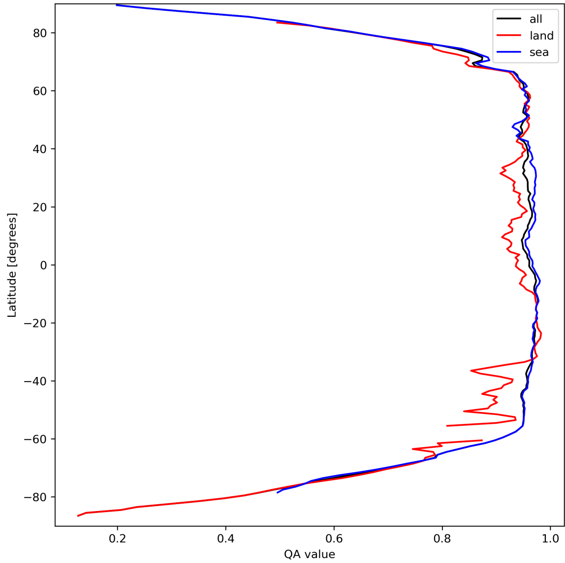
Figure 13: Zonal average of “QA value” for 2023-09-15 to 2023-09-17.
