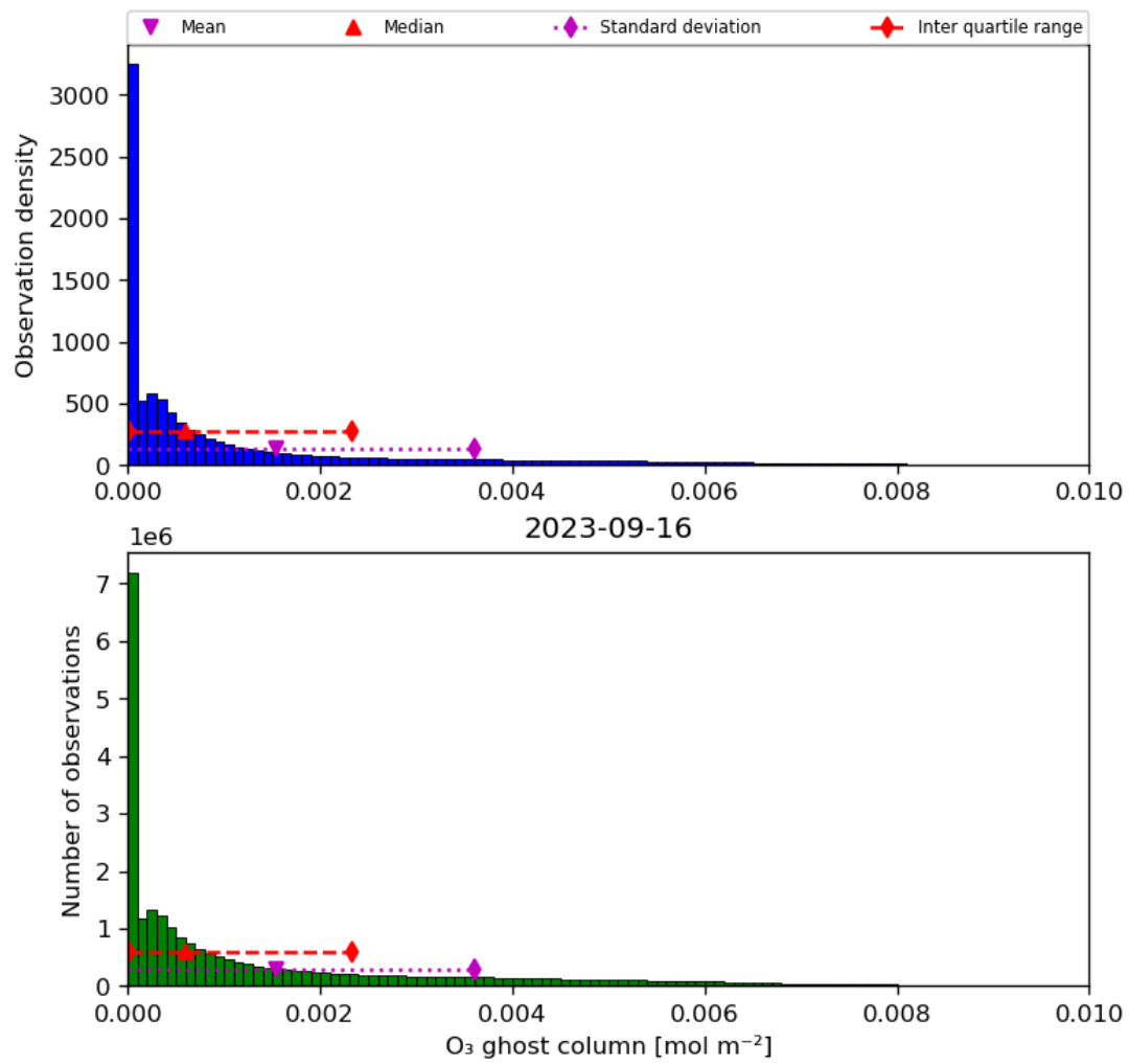
Figure 25: Histogram of “O 3 ghost column” for 2023-09-15 to 2023-09-17
