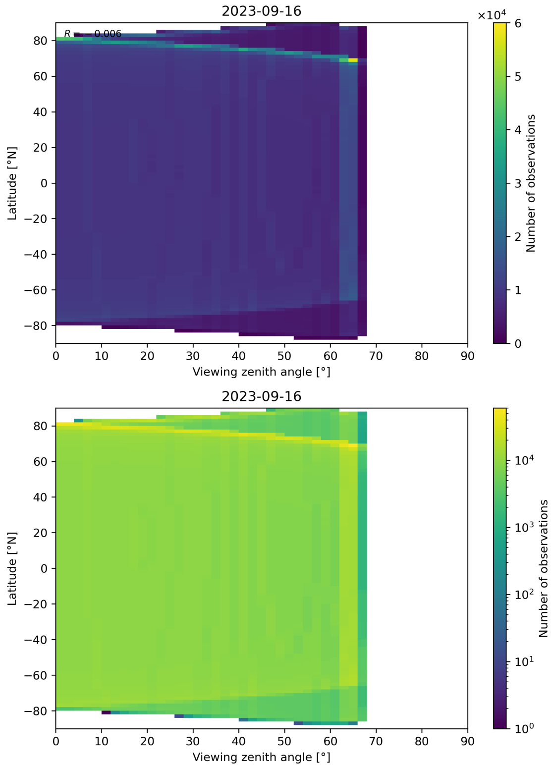
Figure 49: Scatter density plot of “Viewing zenith angle” against “Latitude” for 2023-09-15 to 2023-09-17.
