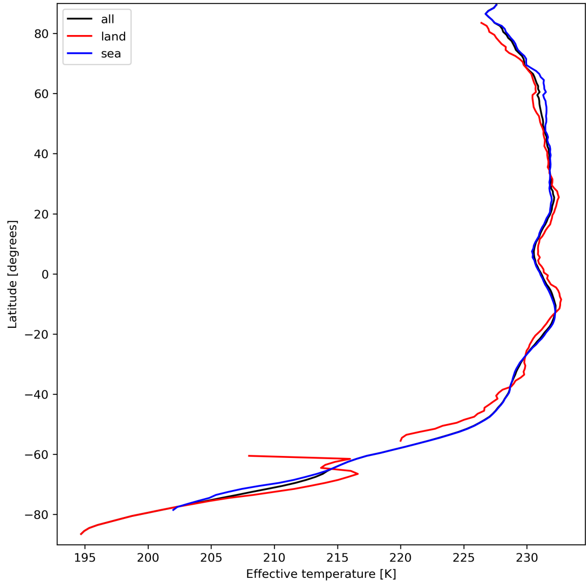
Figure 17: Zonal average of "Effective temperature" for 2023-09-15 to 2023-09-17.
