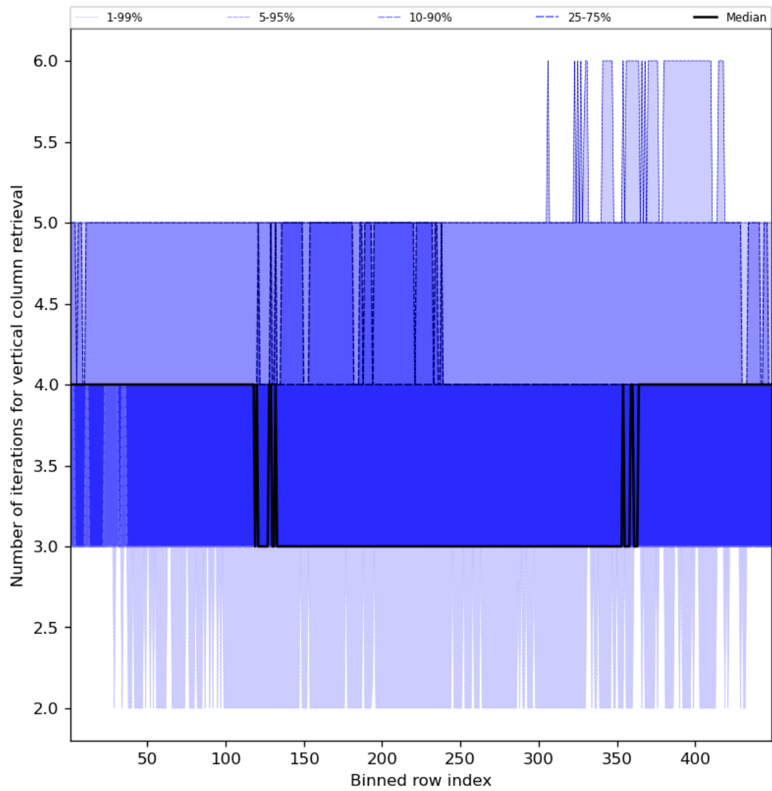
Figure 33: Along track statistics of “Number of iterations for vertical column retrieval” for 2023-09-15 to 2023-09-17
