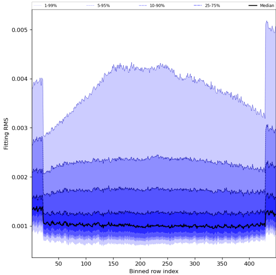
Figure 30: Along track statistics of “Fitting RMS” for 2023-09-15 to 2023-09-17
