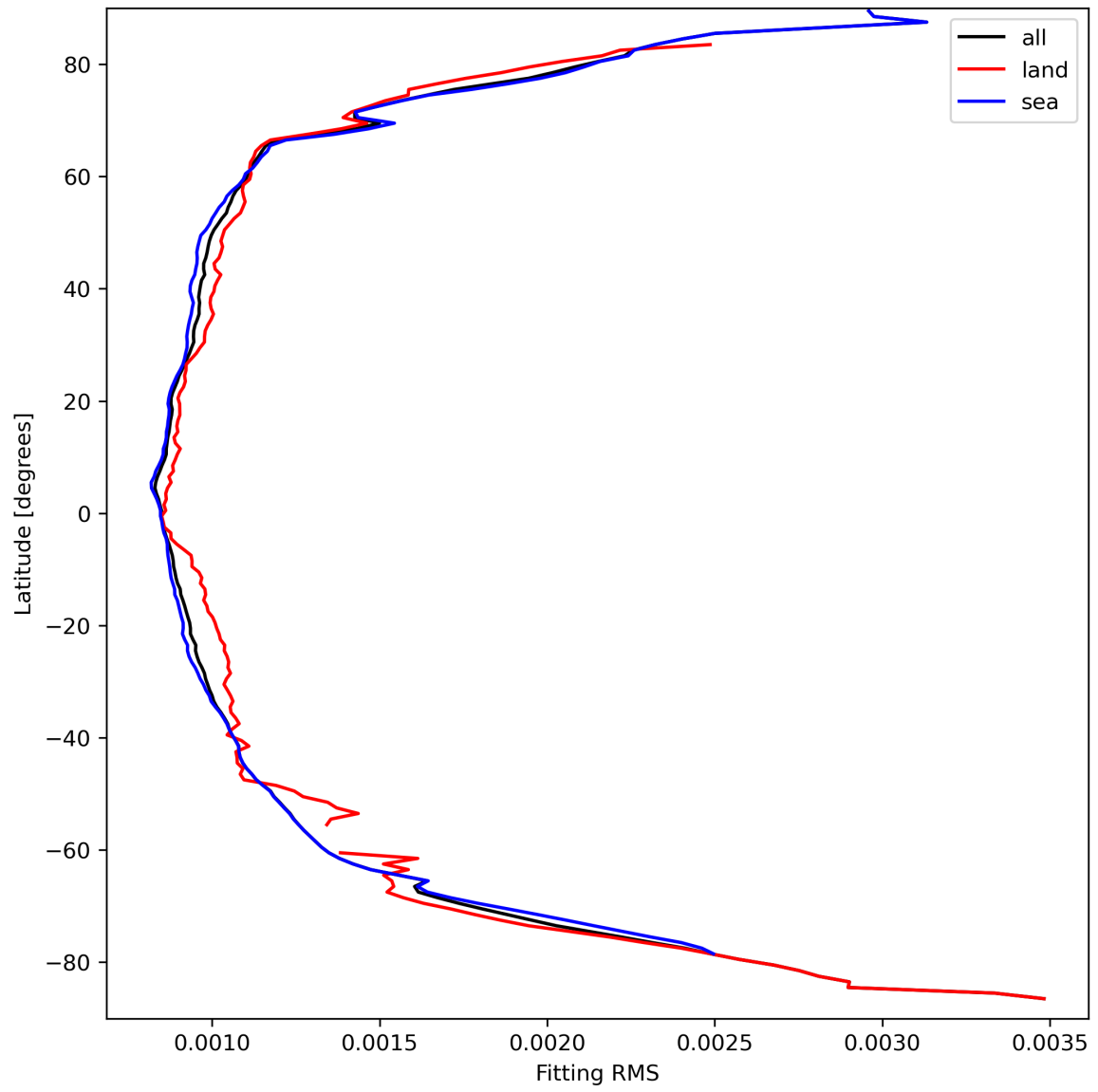
Figure 16: Zonal average of “Fitting RMS” for 2023-09-15 to 2023-09-17.
