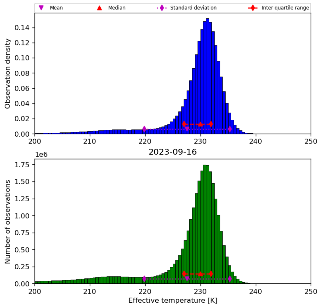
Figure 24: Histogram of “Effective temperature” for 2023-09-15 to 2023-09-17
