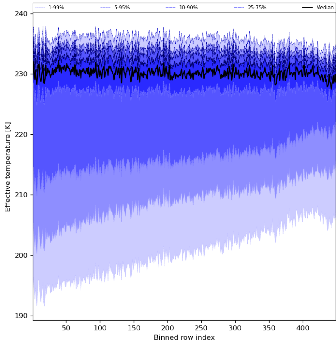
Figure 31: Along track statistics of “Effective temperature” for 2023-09-15 to 2023-09-17
