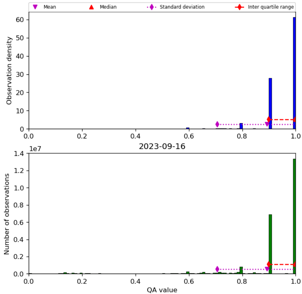
Figure 20: Histogram of “QA value” for 2023-09-15 to 2023-09-17
