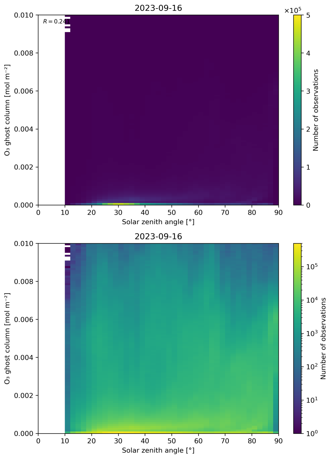
Figure 46: Scatter density plot of “Solar zenith angle” against “O 3 ghost column” for 2023-09-15 to 2023-09-17.
