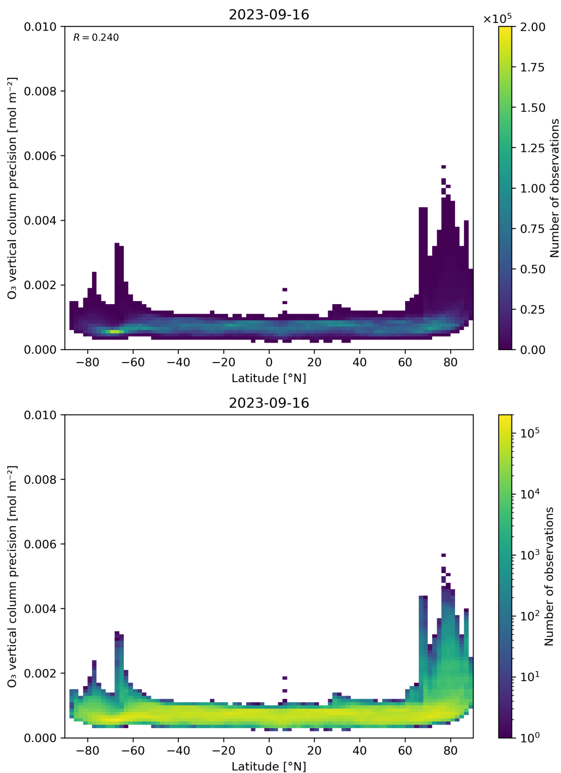
Figure 37: Scatter density plot of “Latitude” against “O 3 vertical column precision” for 2023-09-15 to 2023-09-17.
