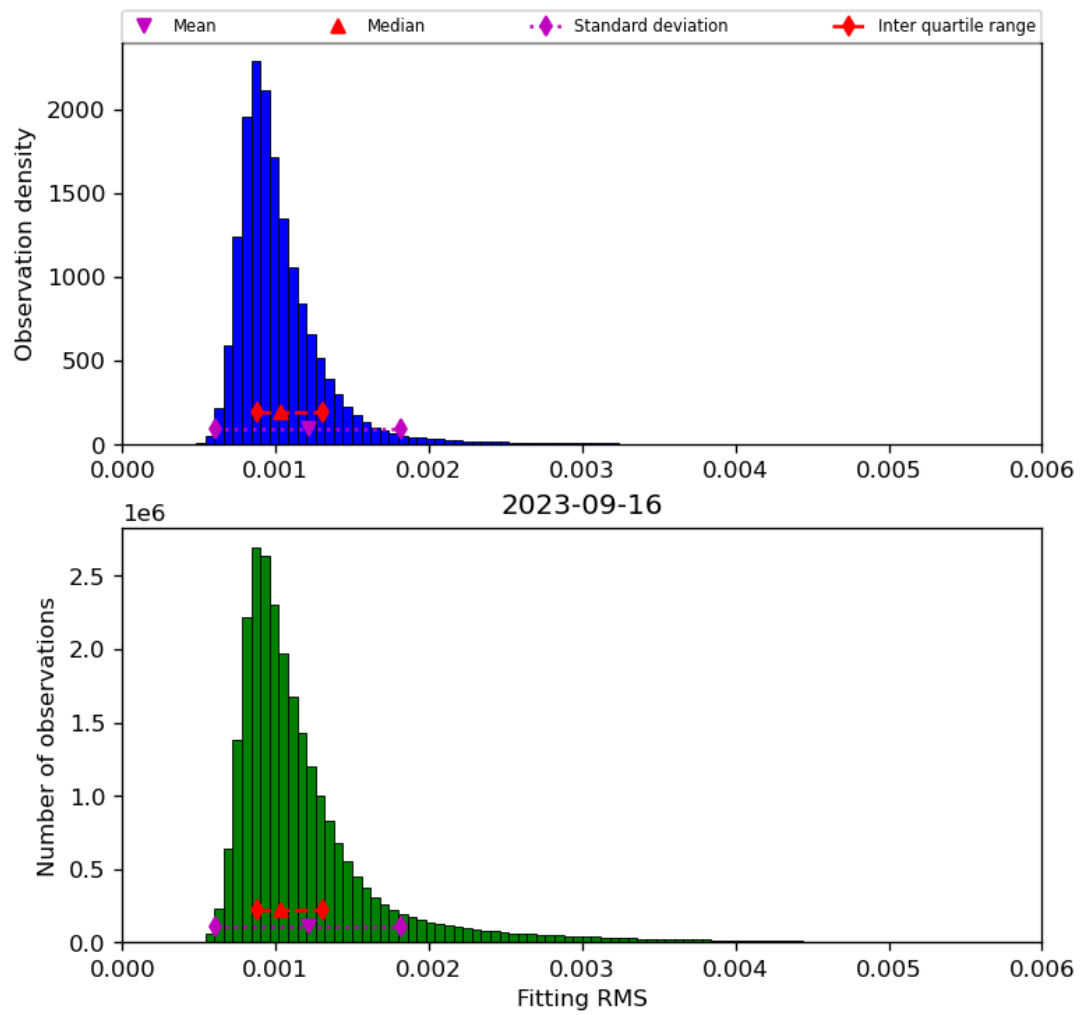
Figure 23: Histogram of “Fitting RMS” for 2023-09-15 to 2023-09-17
