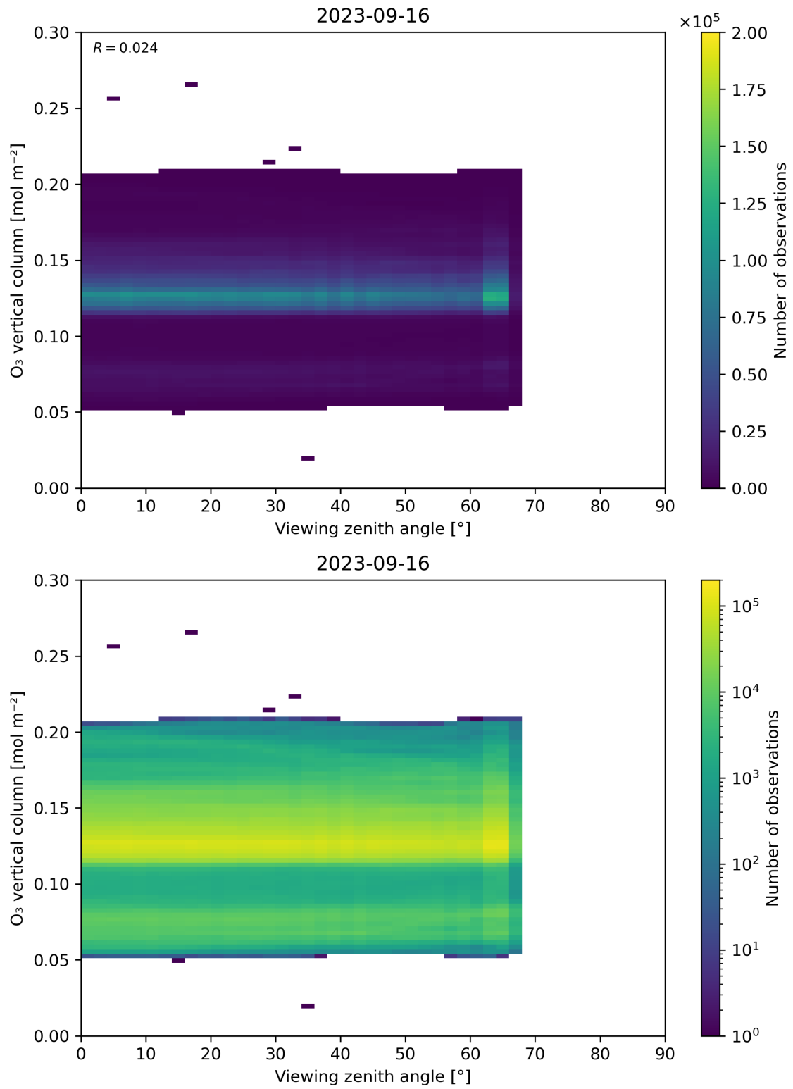
Figure 52: Scatter density plot of “Viewing zenith angle” against “O 3 vertical column” for 2023-09-15 to 2023-09-17.
