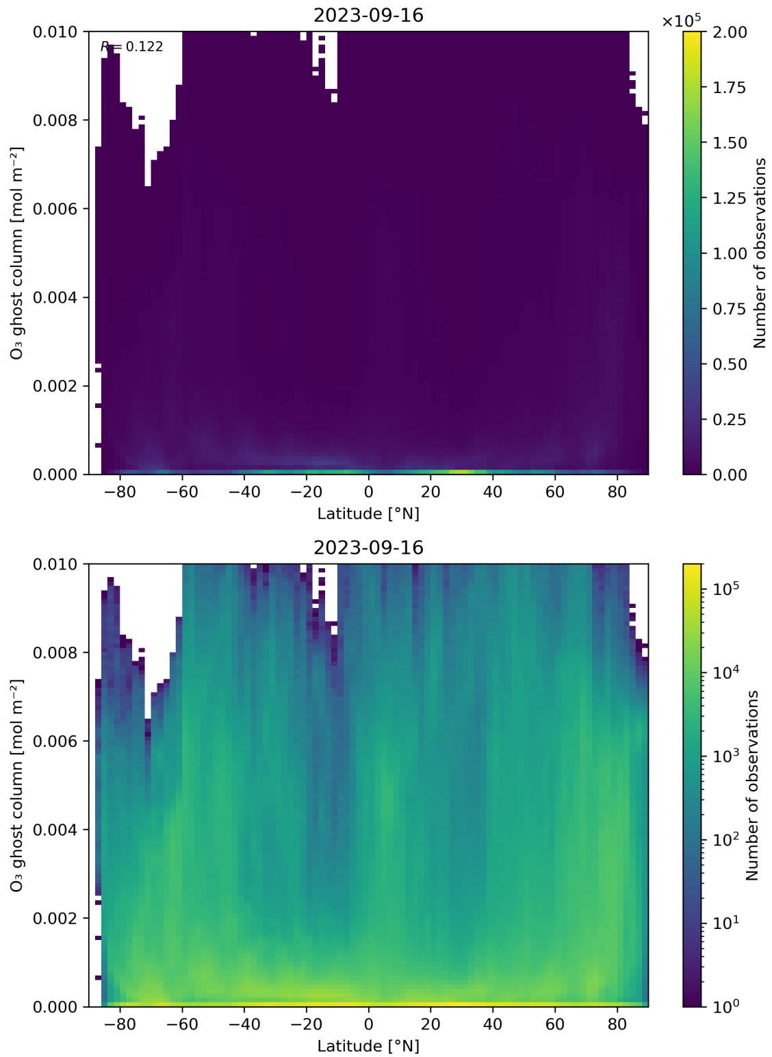
Figure 35: Scatter density plot of “Latitude” against “O 3 ghost column” for 2023-09-15 to 2023-09-17.
