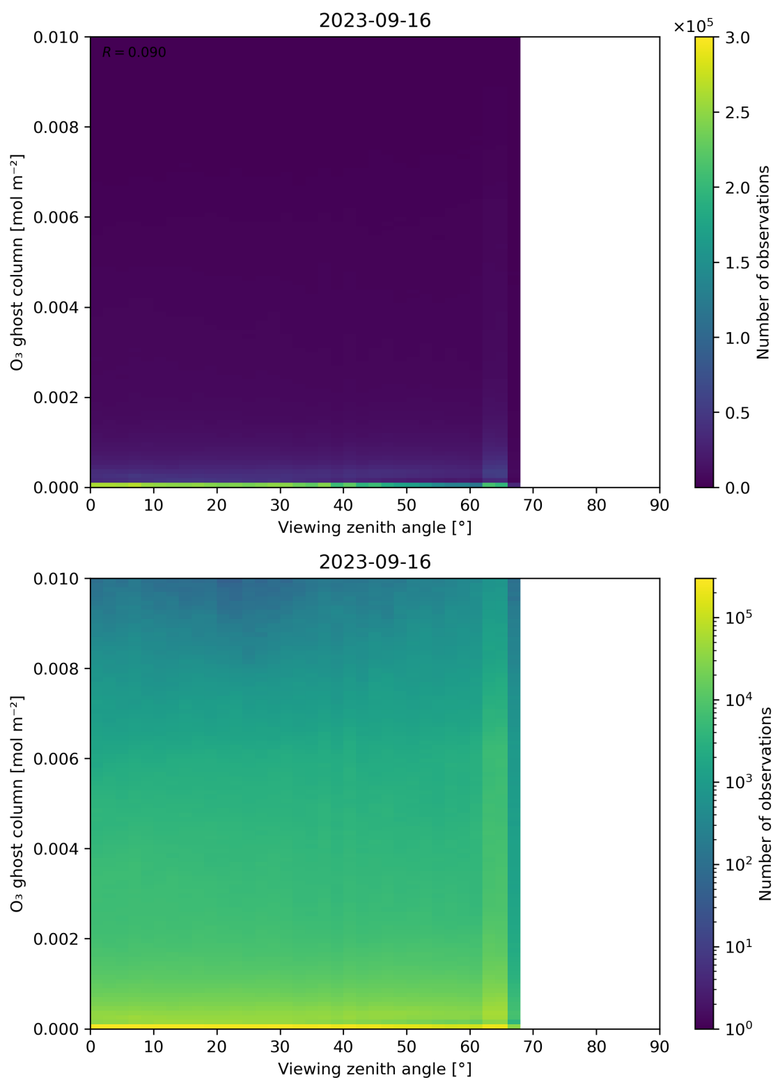
Figure 51: Scatter density plot of “Viewing zenith angle” against “O 3 ghost column” for 2023-09-15 to 2023-09-17.
