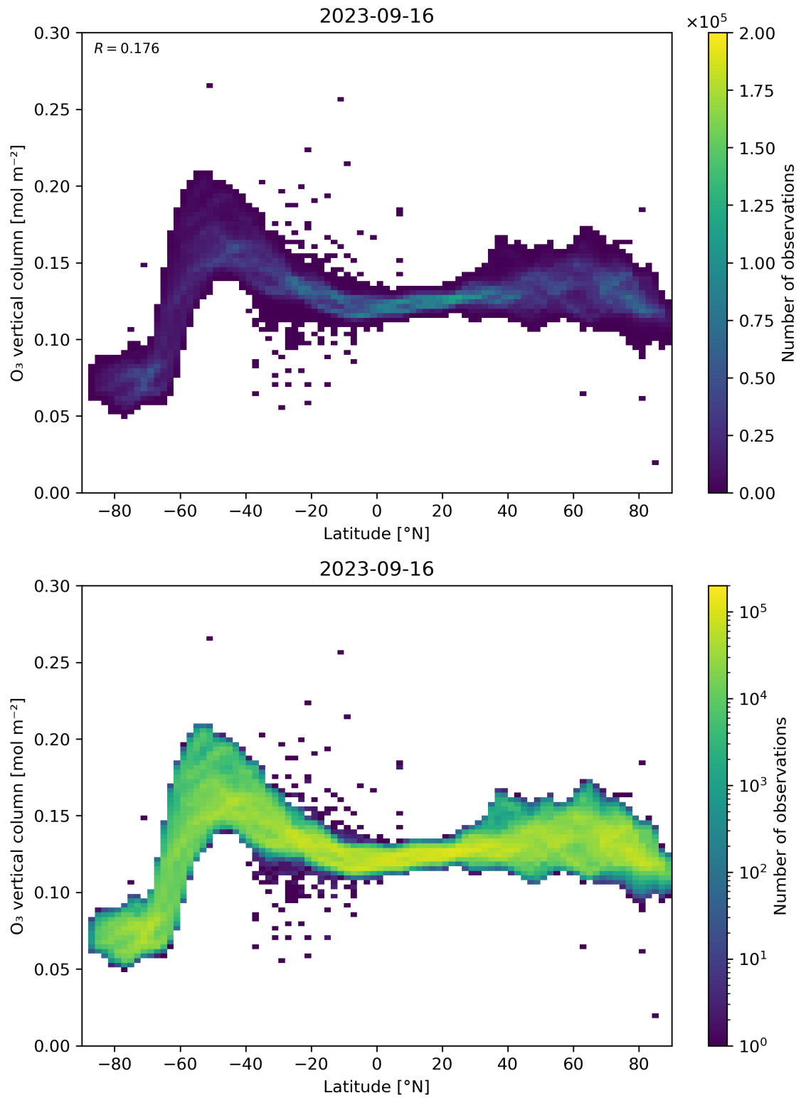
Figure 36: Scatter density plot of “Latitude” against “O 3 vertical column” for 2023-09-15 to 2023-09-17.
