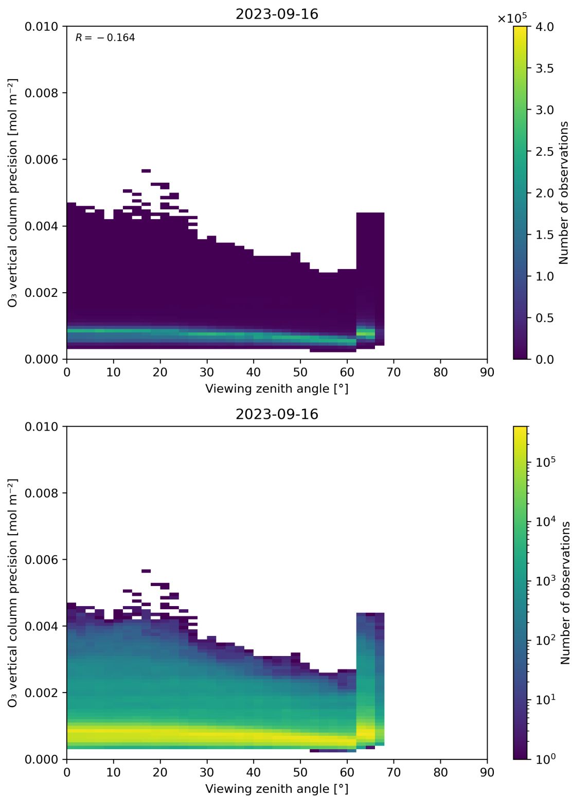
Figure 53: Scatter density plot of “Viewing zenith angle” against “O 3 vertical column precision” for 2023-09-15 to 2023-09-17.
