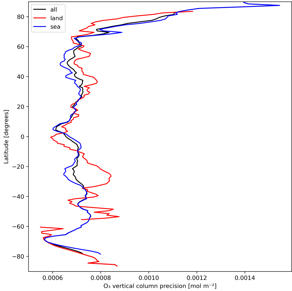
Figure 15: Zonal average of "O 3 vertical column precision" for 2023-09-15 to 2023-09-17.
