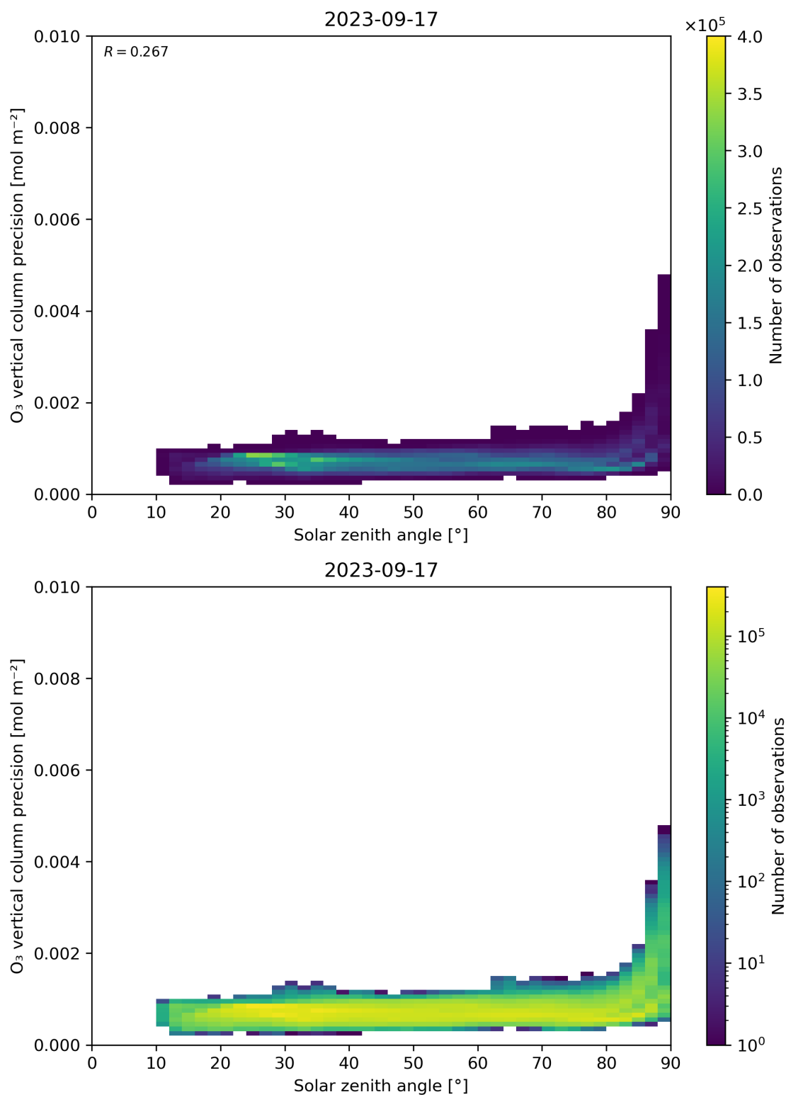
Figure 48: Scatter density plot of “Solar zenith angle” against “O 3 vertical column precision” for 2023-09-16 to 2023-09-18.
