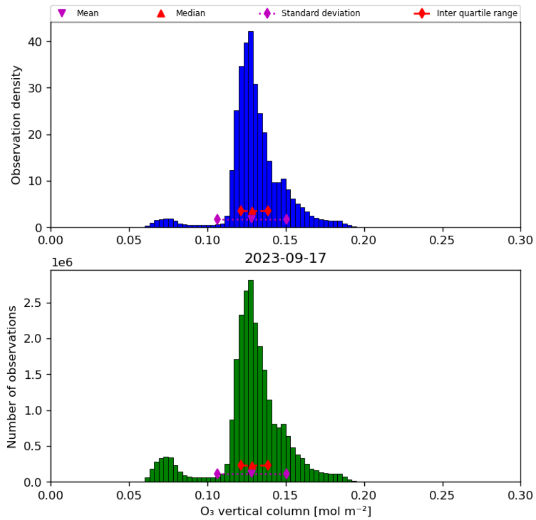
Figure 21: Histogram of “O 3 vertical column” for 2023-09-16 to 2023-09-18
