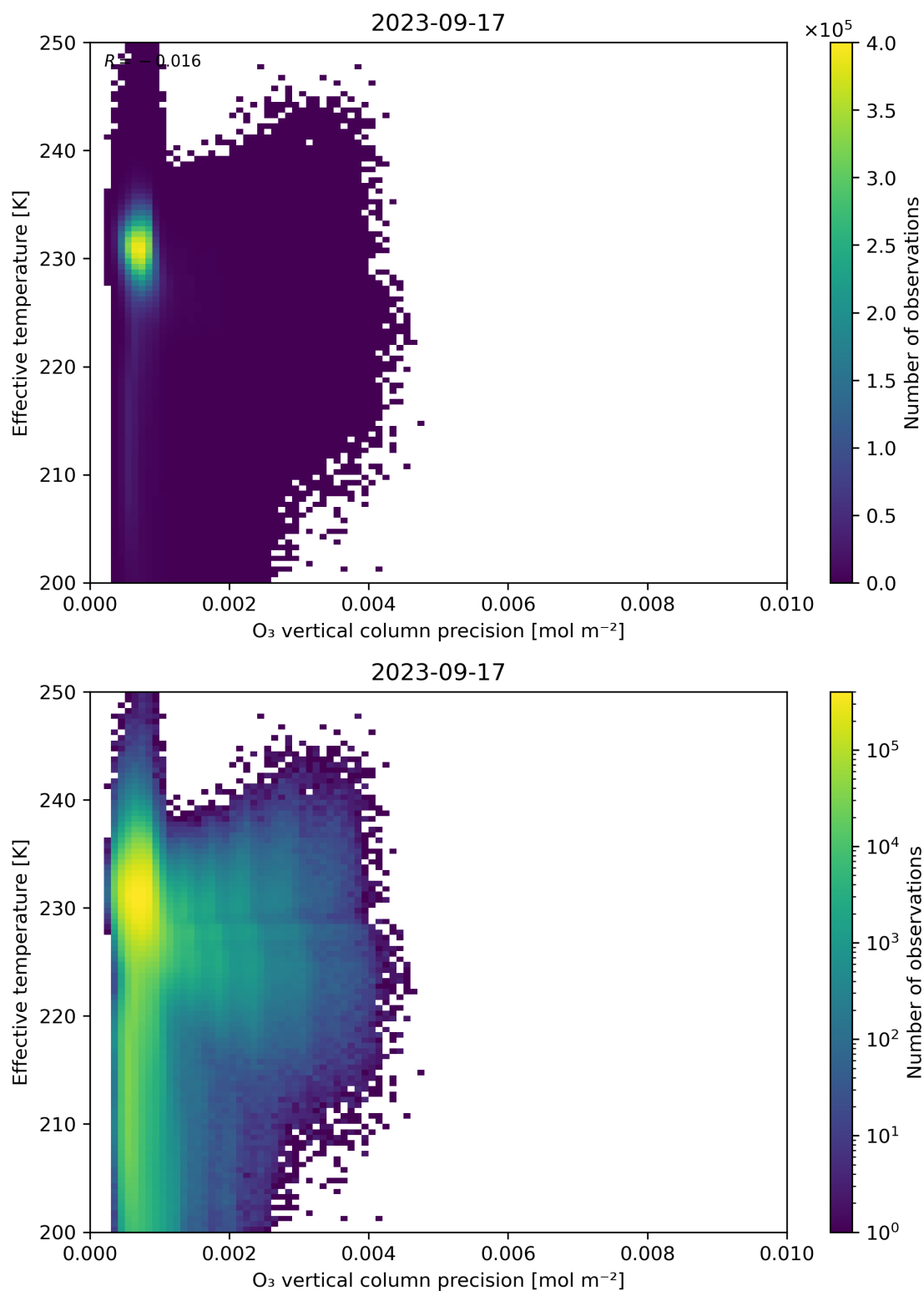
Figure 42: Scatter density plot of “O 3 vertical column precision” against “Effective temperature” for 2023-09-16 to 2023-09-18.
