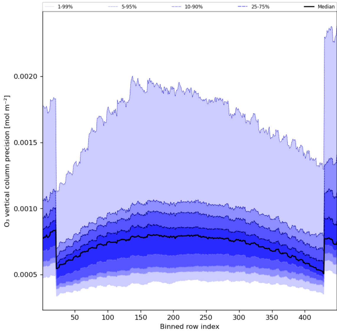
Figure 29: Along track statistics of “O 3 vertical column precision” for 2023-09-16 to 2023-09-18
