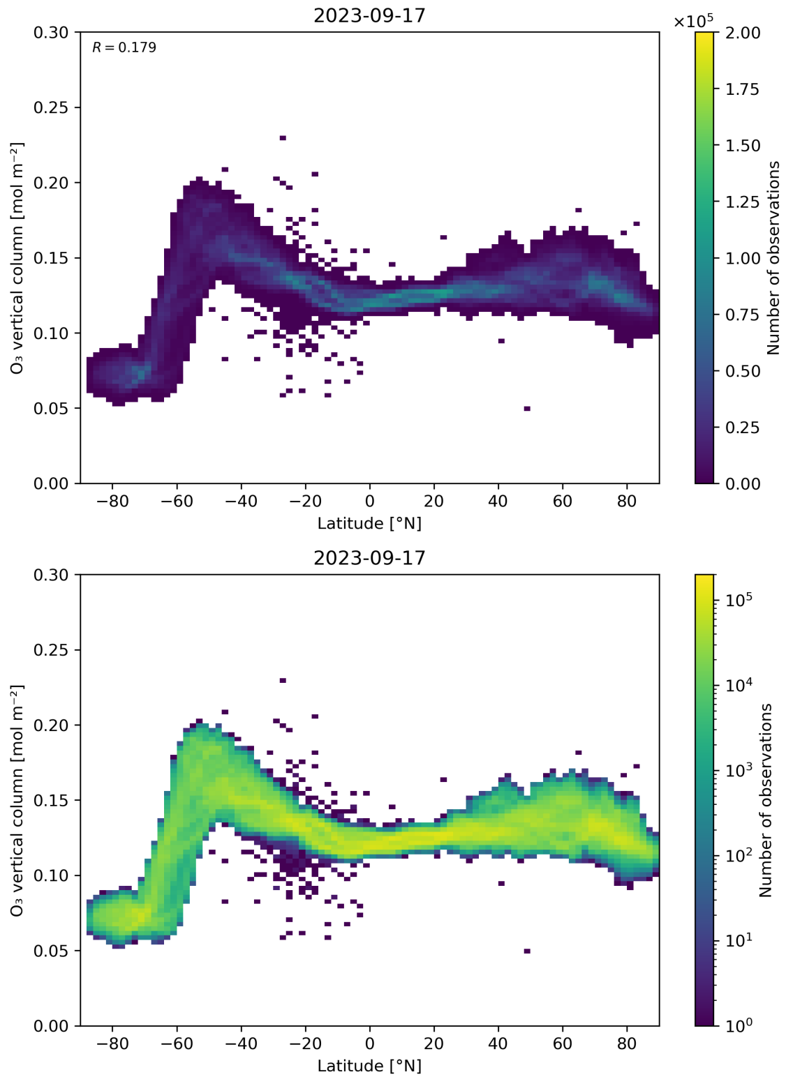
Figure 36: Scatter density plot of “Latitude” against “O 3 vertical column” for 2023-09-16 to 2023-09-18.
