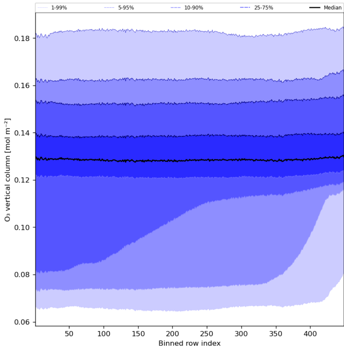
Figure 28: Along track statistics of “O 3 vertical column” for 2023-09-16 to 2023-09-18
