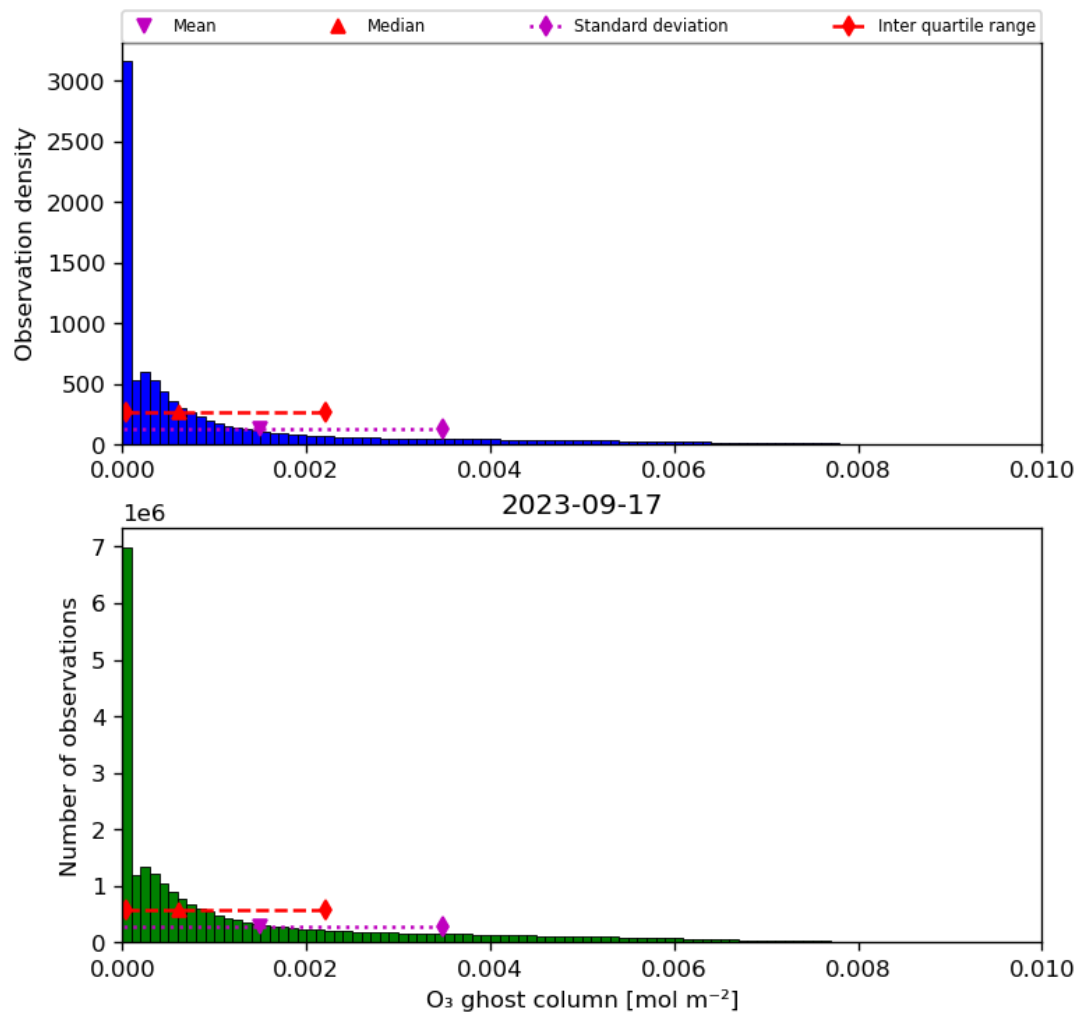
Figure 25: Histogram of “O 3 ghost column” for 2023-09-16 to 2023-09-18
