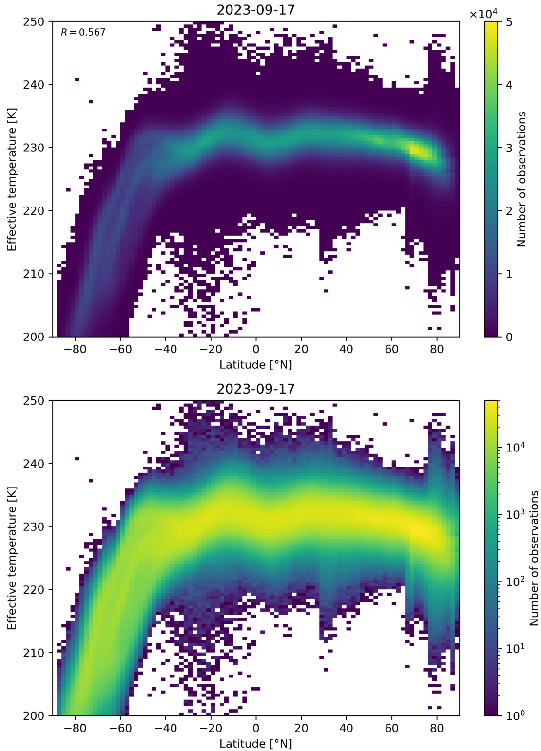
Figure 34: Scatter density plot of “Latitude” against “Effective temperature” for 2023-09-16 to 2023-09-18.
