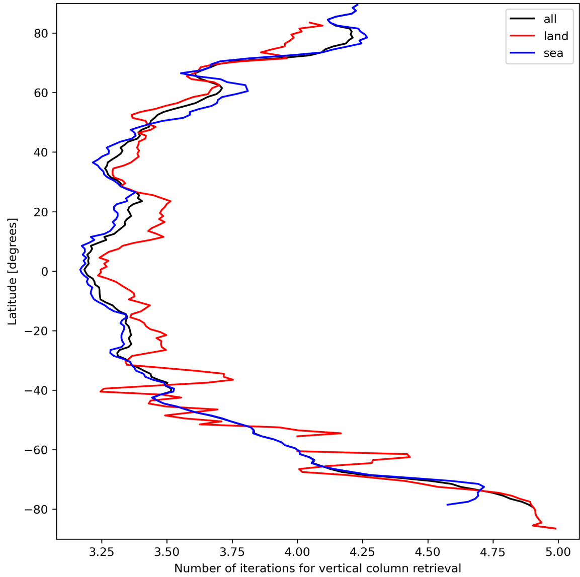
Figure 19: Zonal average of “Number of iterations for vertical column retrieval” for 2023-09-16 to 2023-09-18.
