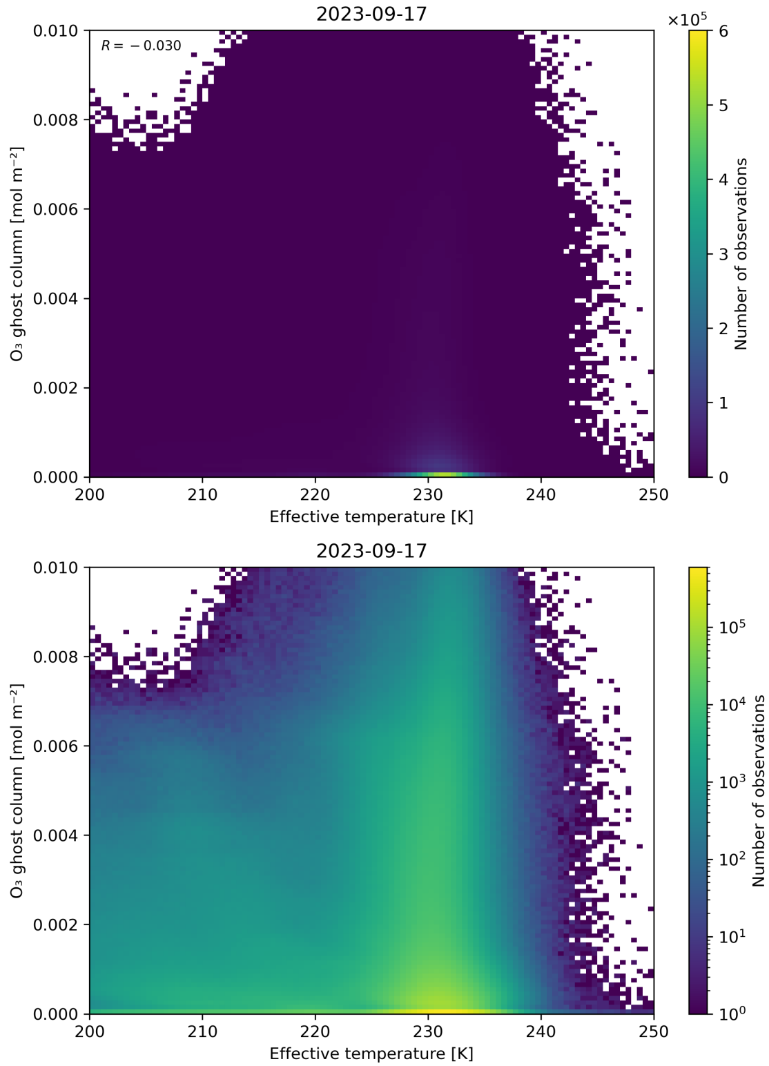
Figure 38: Scatter density plot of “Effective temperature” against “O 3 ghost column” for 2023-09-16 to 2023-09-18.
