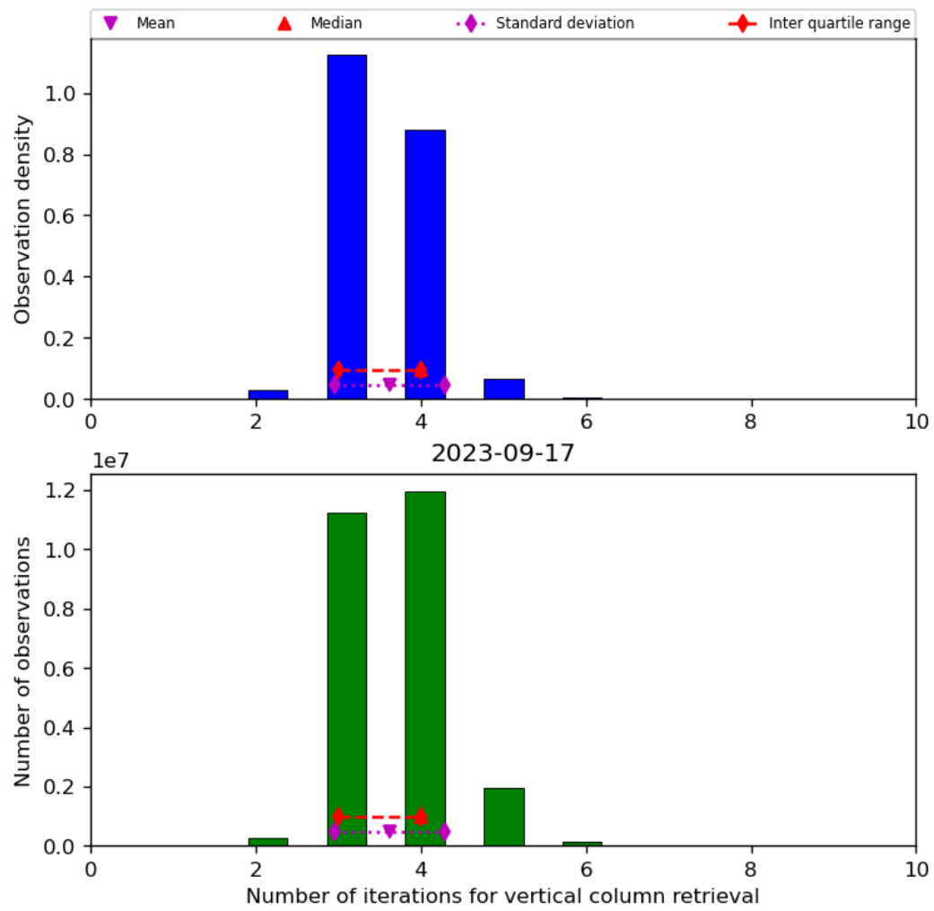
Figure 26: Histogram of “Number of iterations for vertical column retrieval” for 2023-09-16 to 2023-09-18
