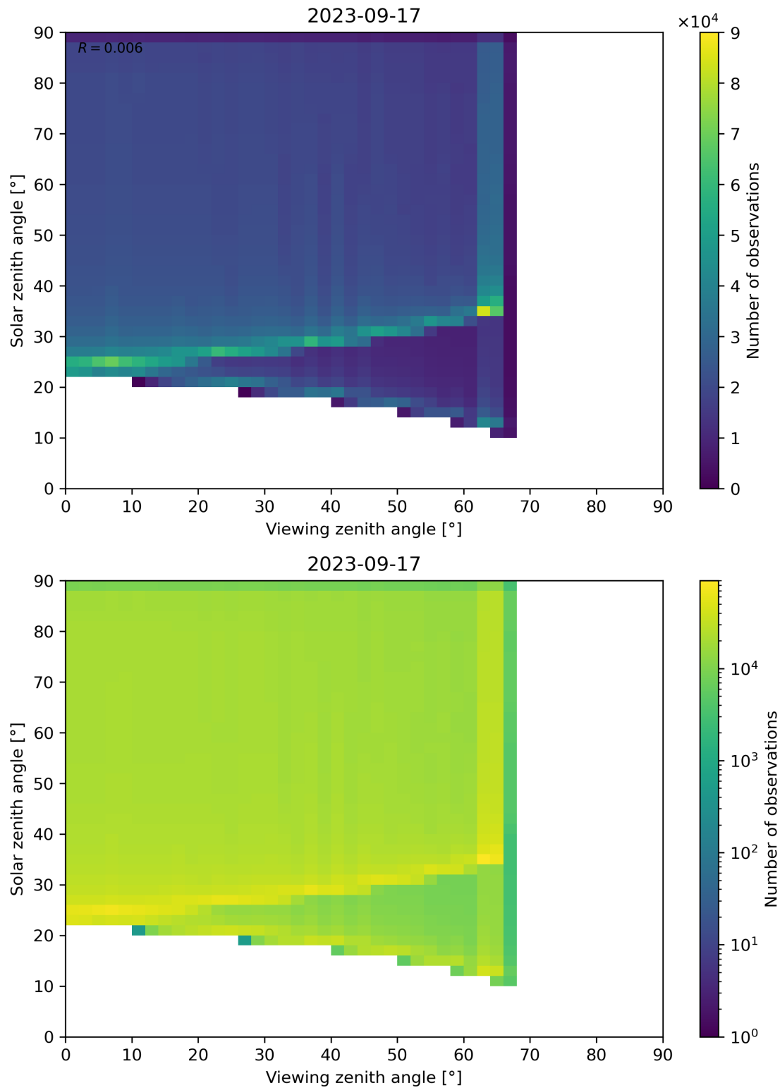
Figure 54: Scatter density plot of “Viewing zenith angle” against “Solar zenith angle” for 2023-09-16 to 2023-09-18.
