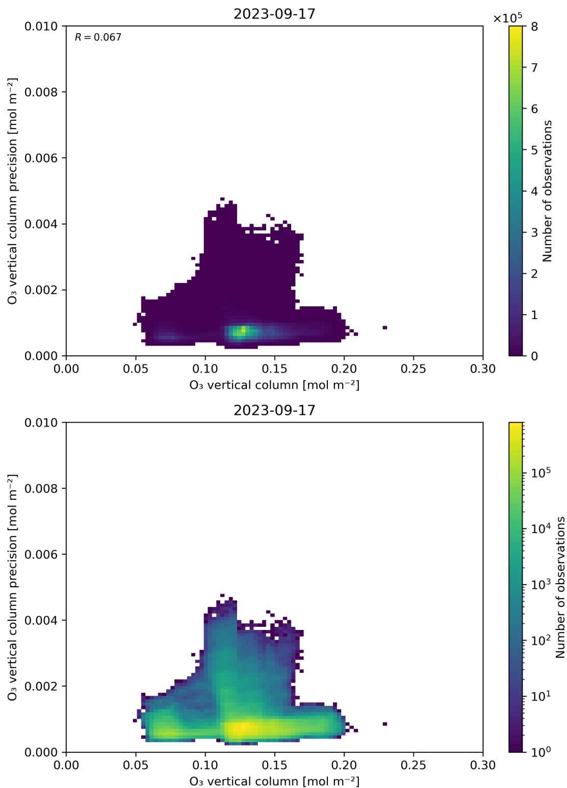
Figure 41: Scatter density plot of “O 3 vertical column” against “O 3 vertical column precision” for 2023-09-16 to 2023-09-18.
