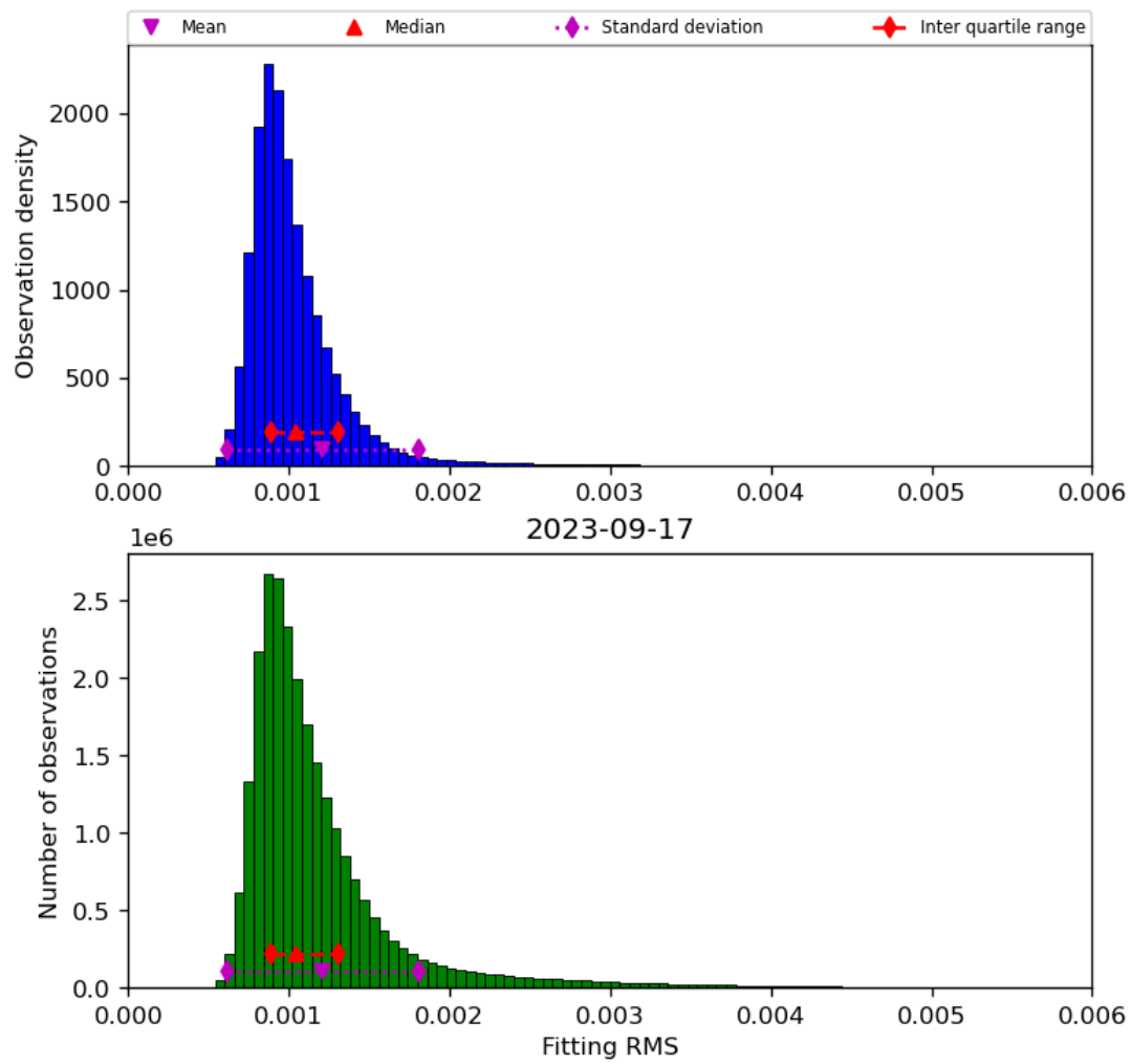
Figure 23: Histogram of “Fitting RMS” for 2023-09-16 to 2023-09-18
