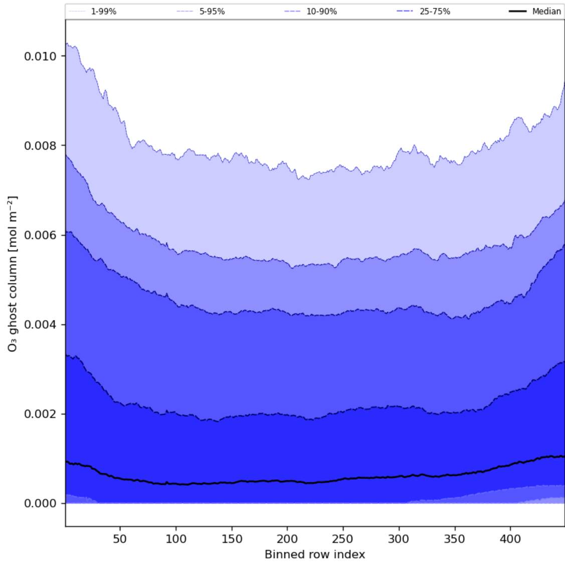
Figure 32: Along track statistics of "O 3 ghost column" for 2023-09-16 to 2023-09-18
