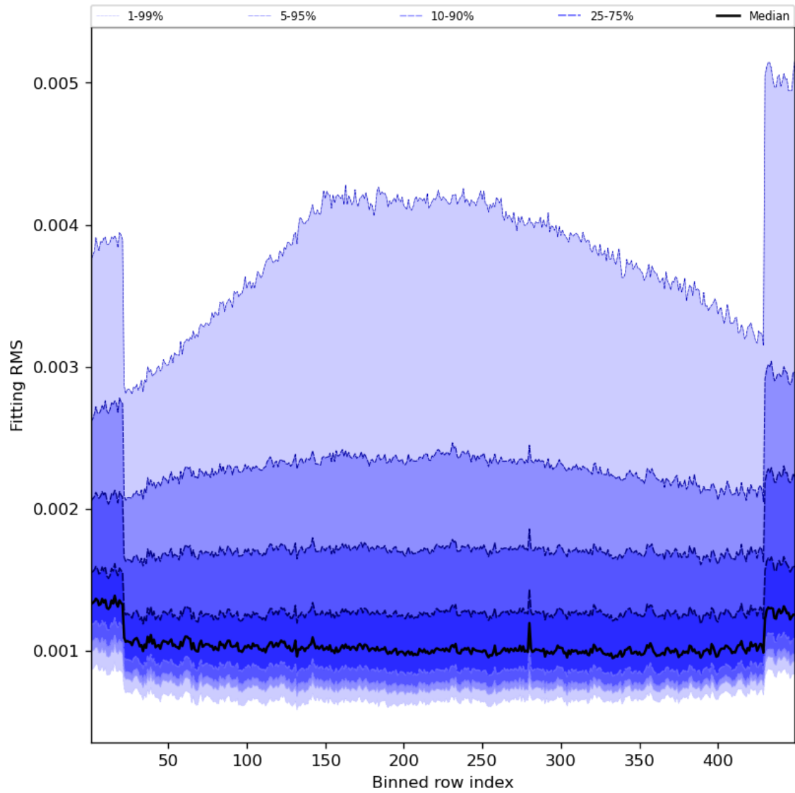
Figure 30: Along track statistics of “Fitting RMS” for 2023-09-16 to 2023-09-18
