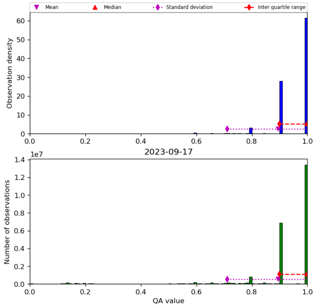
Figure 20: Histogram of “QA value” for 2023-09-16 to 2023-09-18
