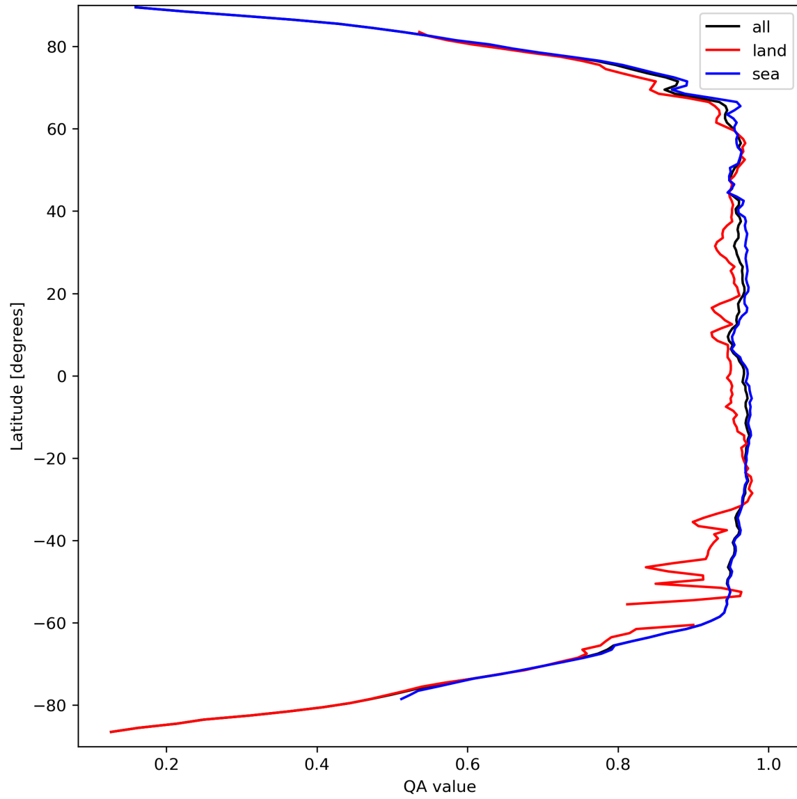
Figure 13: Zonal average of “QA value” for 2023-09-16 to 2023-09-18.
