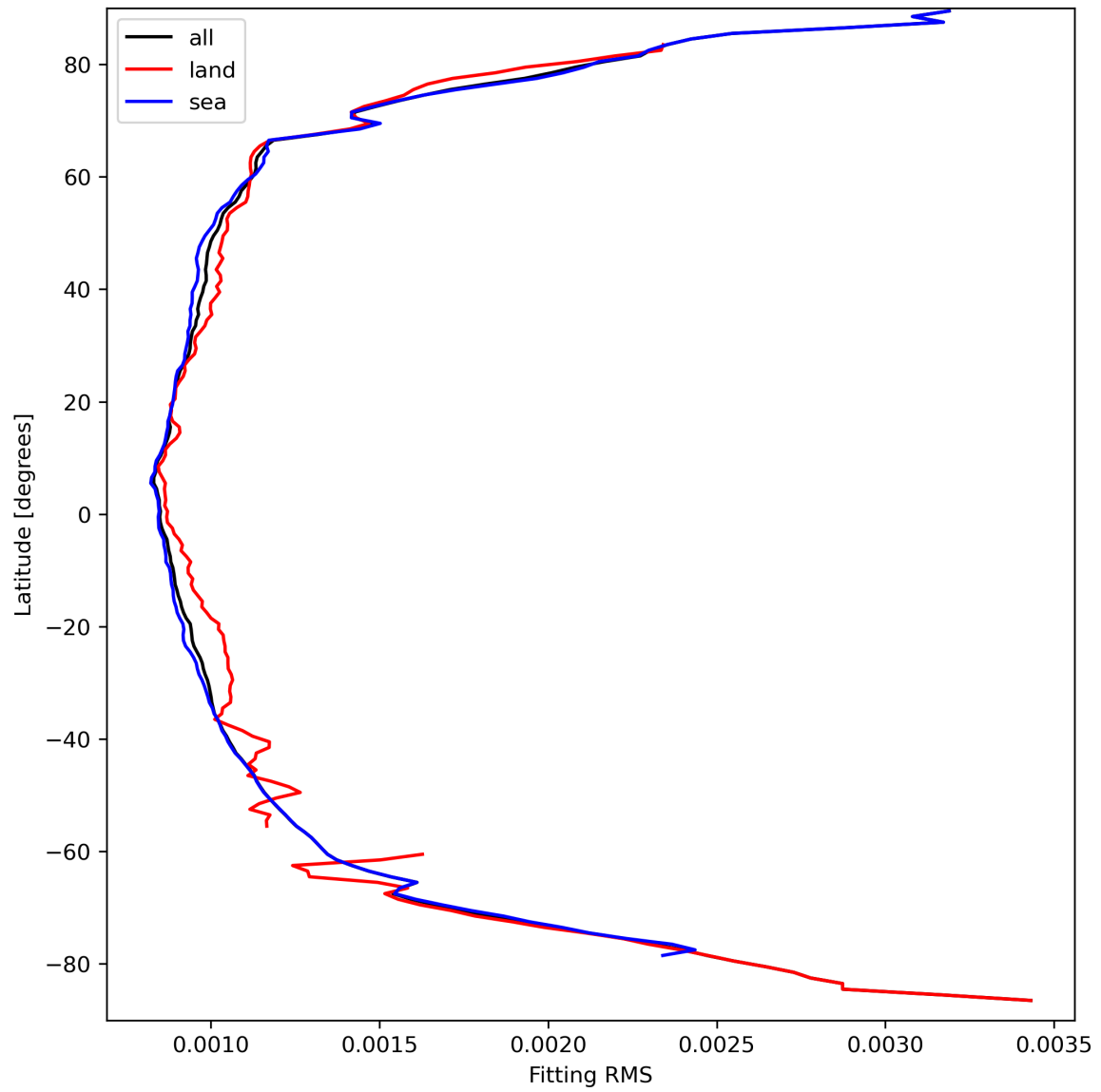
Figure 16: Zonal average of “Fitting RMS” for 2023-09-16 to 2023-09-18.
