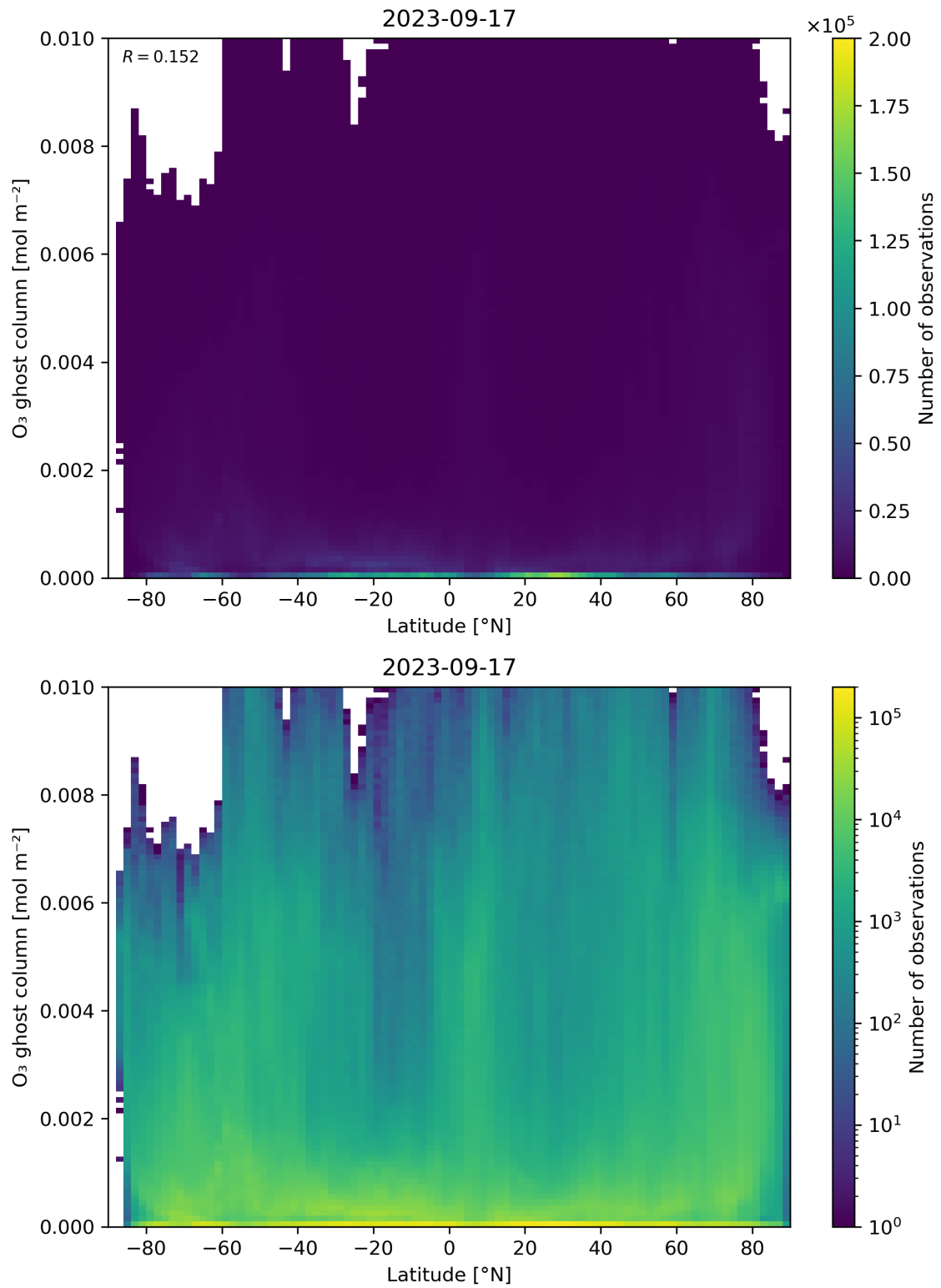
Figure 35: Scatter density plot of “Latitude” against “O 3 ghost column” for 2023-09-16 to 2023-09-18.
