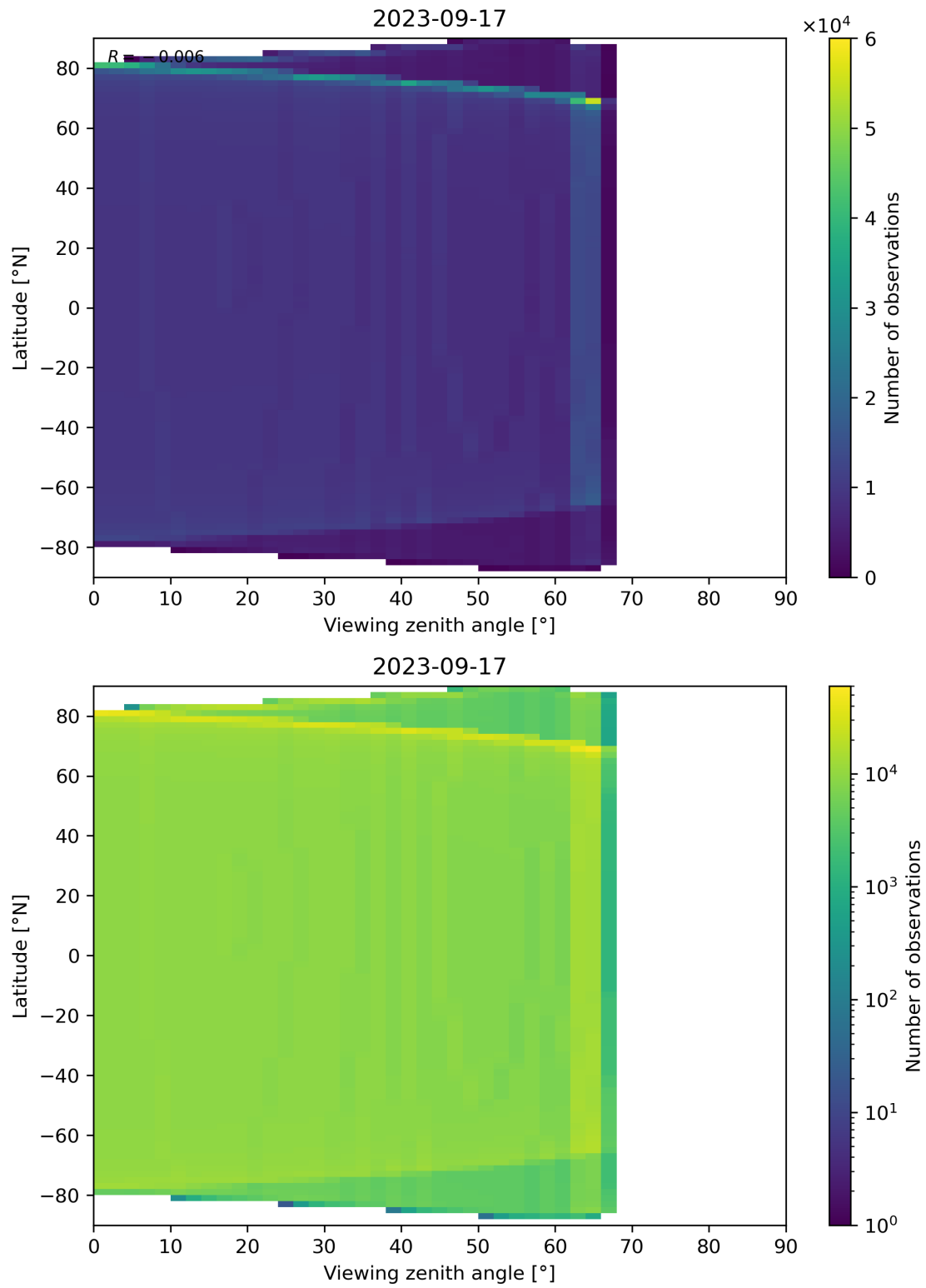
Figure 49: Scatter density plot of “Viewing zenith angle” against “Latitude” for 2023-09-16 to 2023-09-18.
