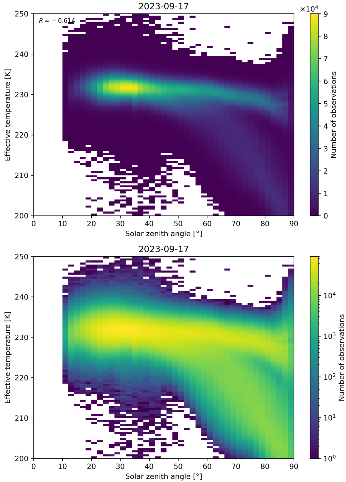
Figure 45: Scatter density plot of “Solar zenith angle” against “Effective temperature” for 2023-09-16 to 2023-09-18.
