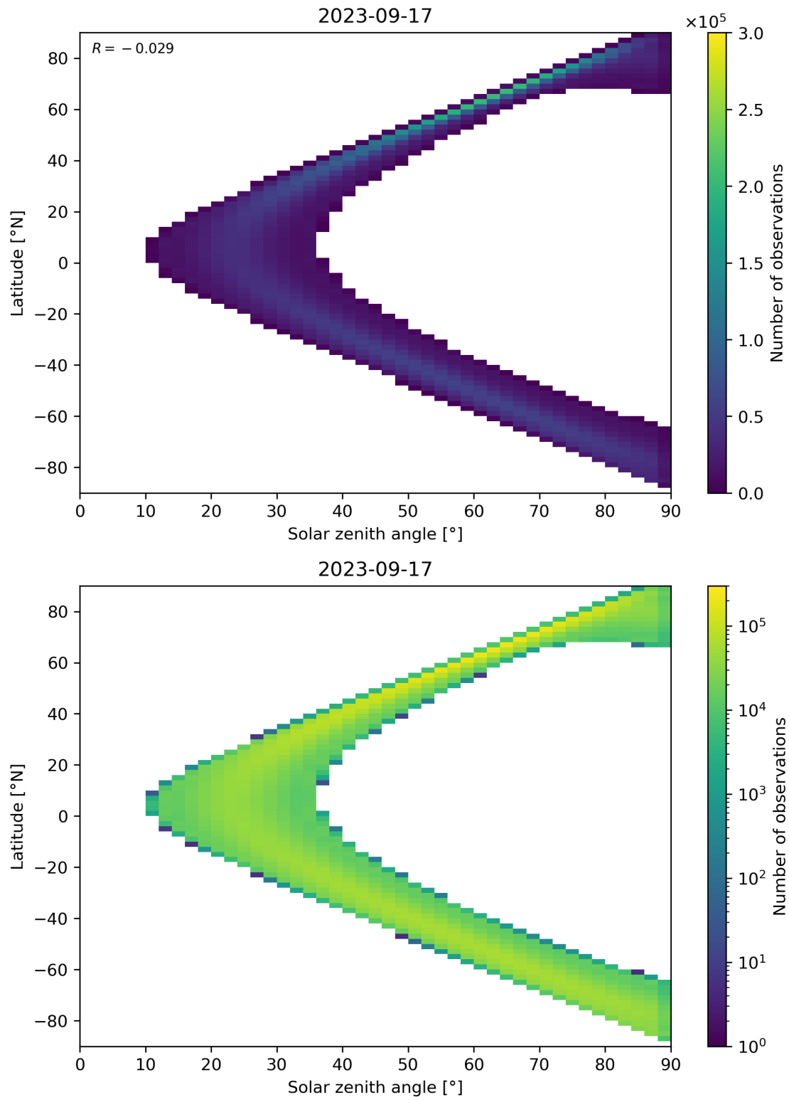
Figure 44: Scatter density plot of “Solar zenith angle” against “Latitude” for 2023-09-16 to 2023-09-18.
