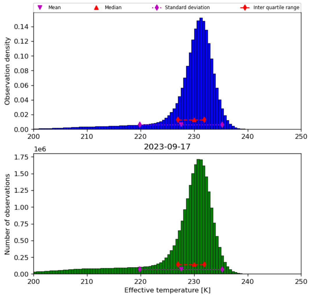
Figure 24: Histogram of “Effective temperature” for 2023-09-16 to 2023-09-18
