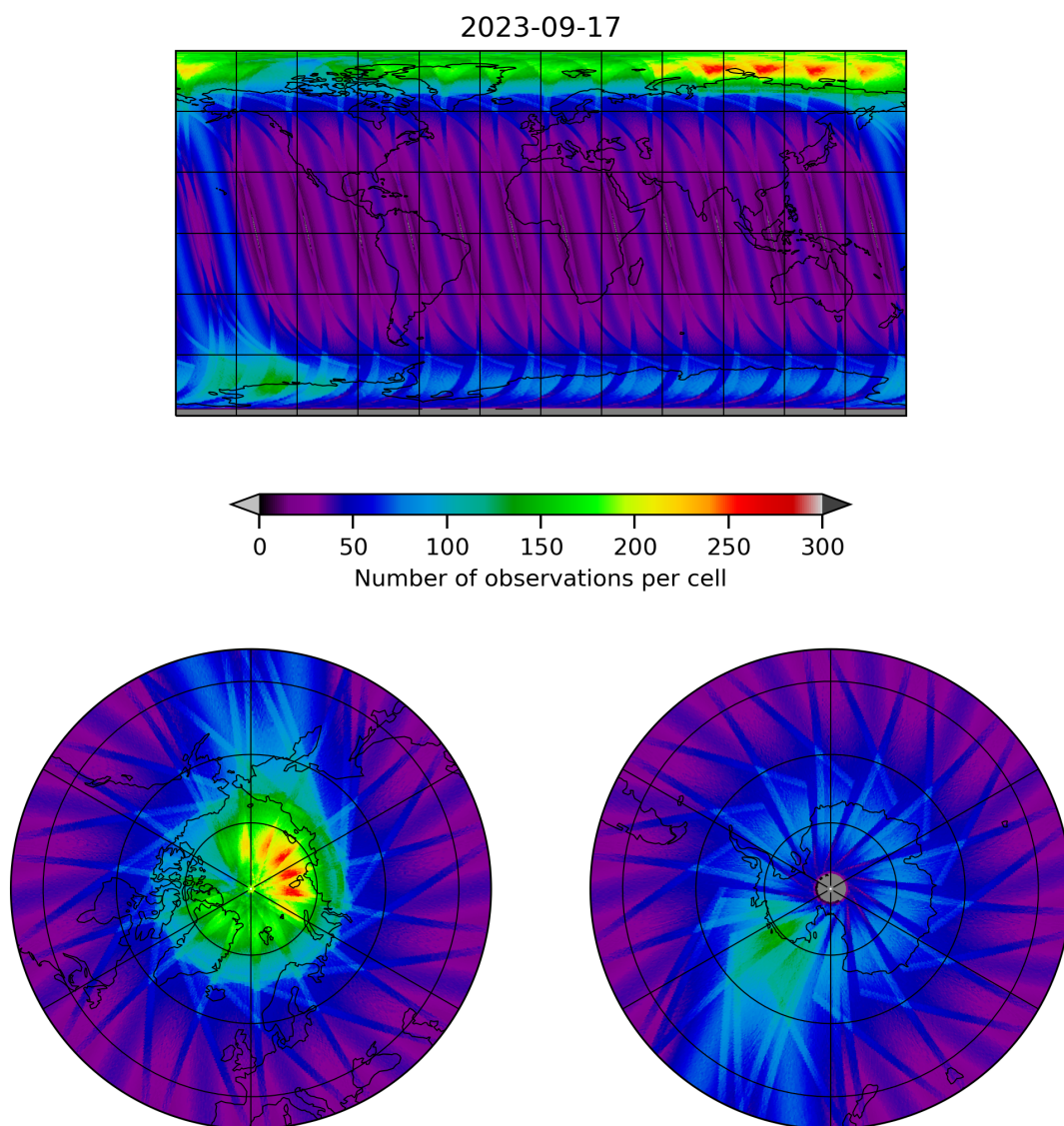
Figure 12: Map of the number of observations for 2023-09-16 to 2023-09-18
