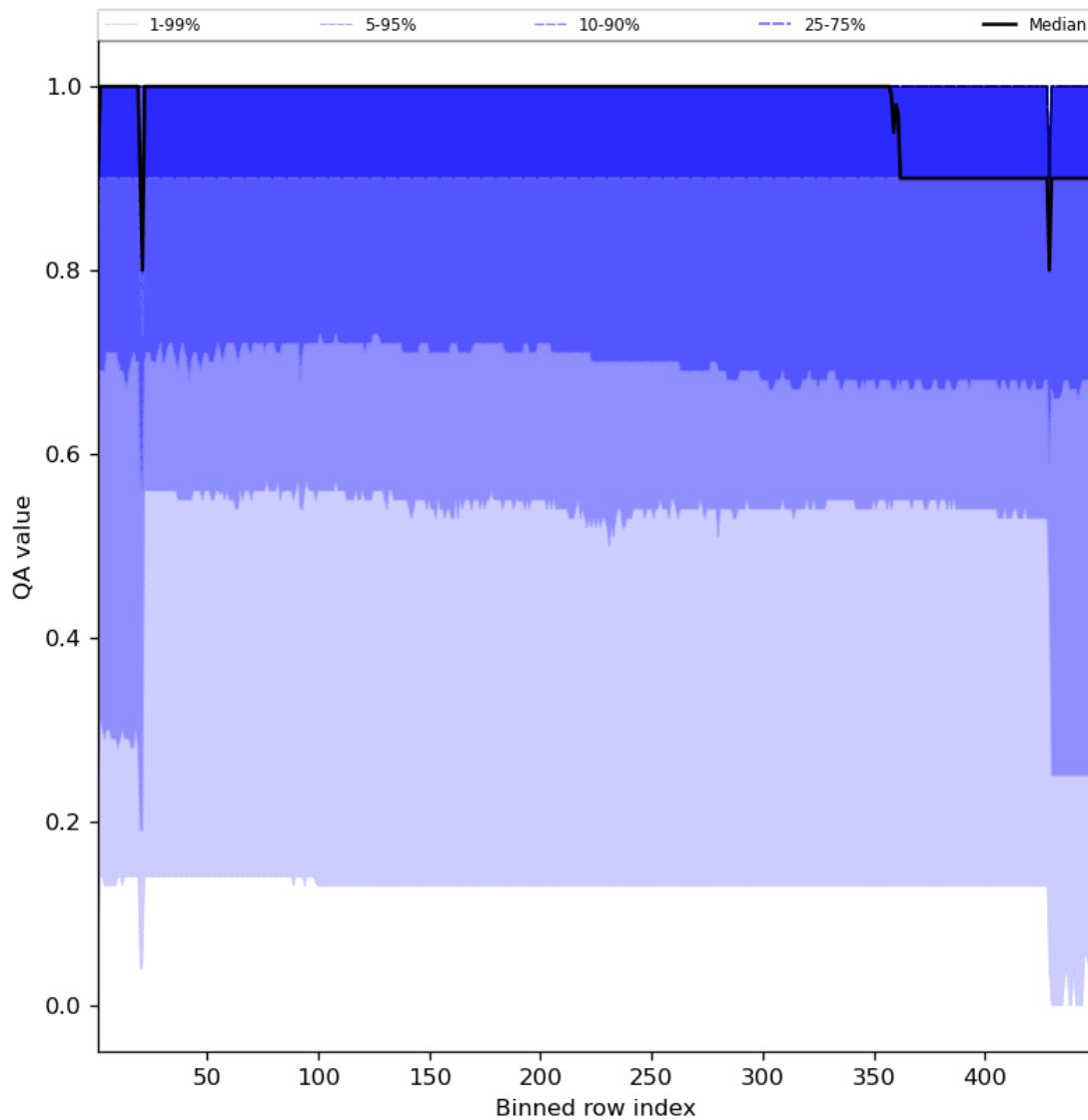
Figure 27: Along track statistics of “QA value” for 2023-09-16 to 2023-09-18
