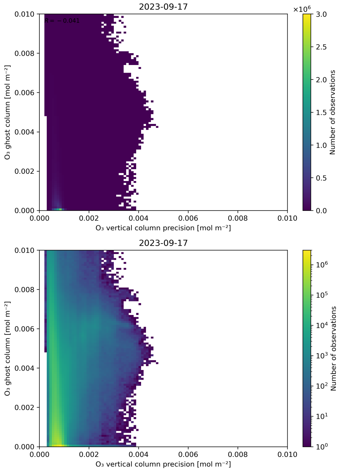
Figure 43: Scatter density plot of “ \text{O}_3 vertical column precision” against “ \text{O}_3 ghost column” for 2023-09-16 to 2023-09-18.
