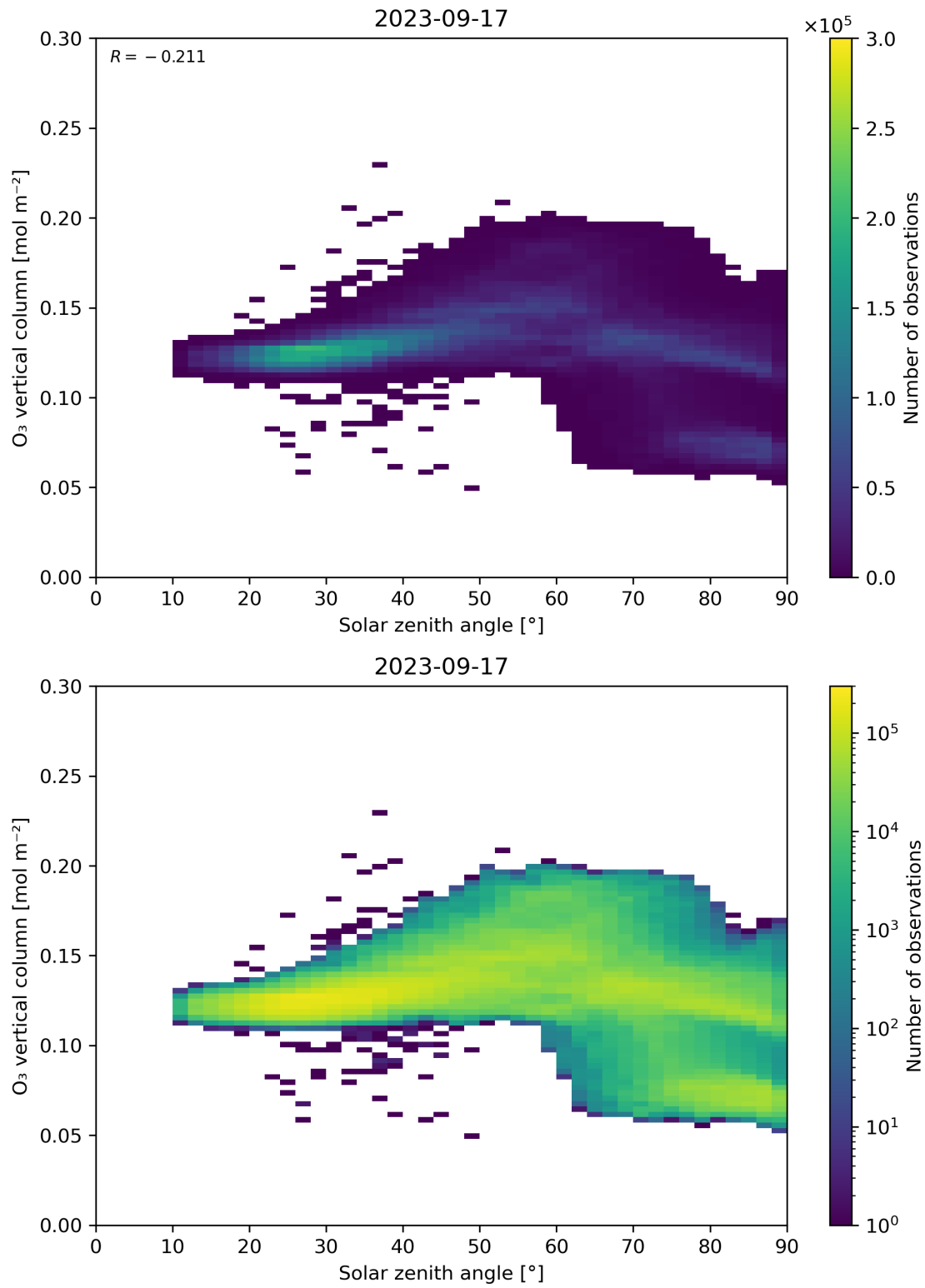
Figure 47: Scatter density plot of “Solar zenith angle” against “O 3 vertical column” for 2023-09-16 to 2023-09-18.
