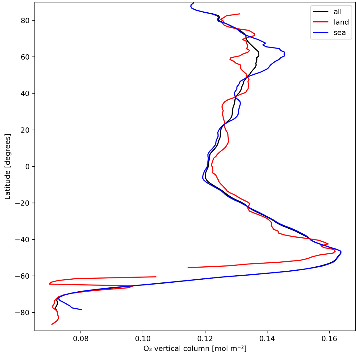
Figure 14: Zonal average of “O 3 vertical column” for 2023-09-16 to 2023-09-18.
