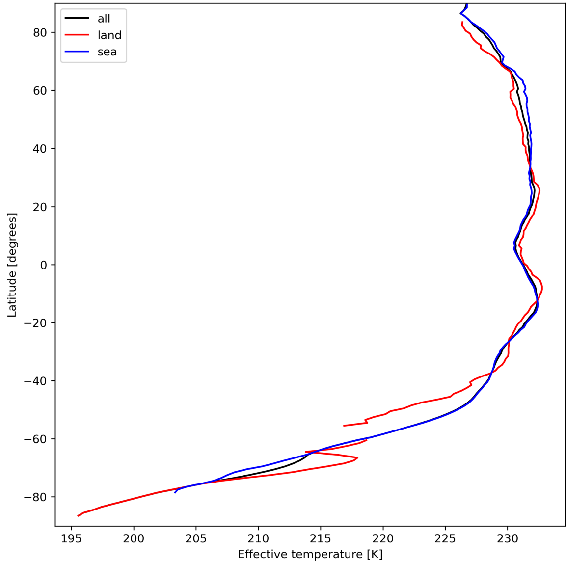
Figure 17: Zonal average of “Effective temperature” for 2023-09-16 to 2023-09-18.
