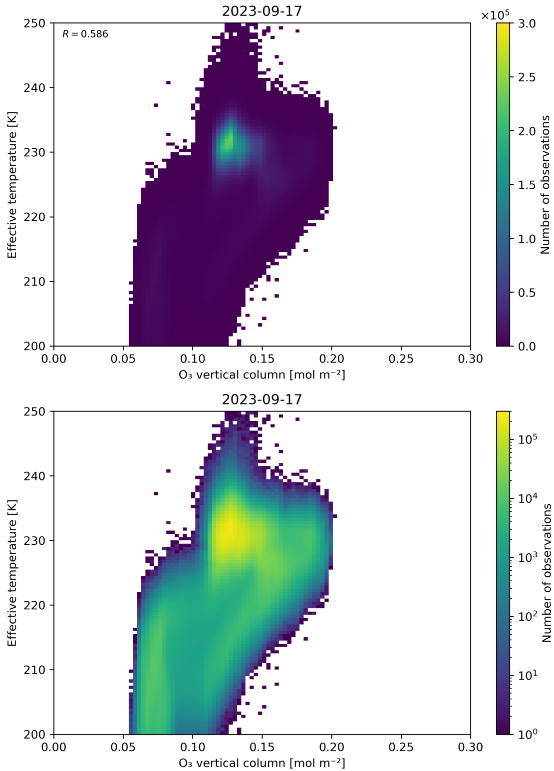
Figure 39: Scatter density plot of “O 3 vertical column” against “Effective temperature” for 2023-09-16 to 2023-09-18.
