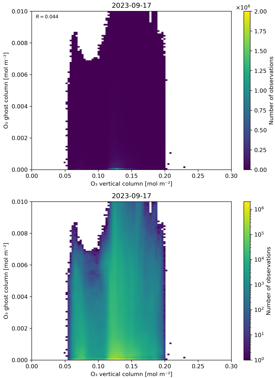
Figure 40: Scatter density plot of “O 3 vertical column” against “O 3 ghost column” for 2023-09-16 to 2023-09-18.
