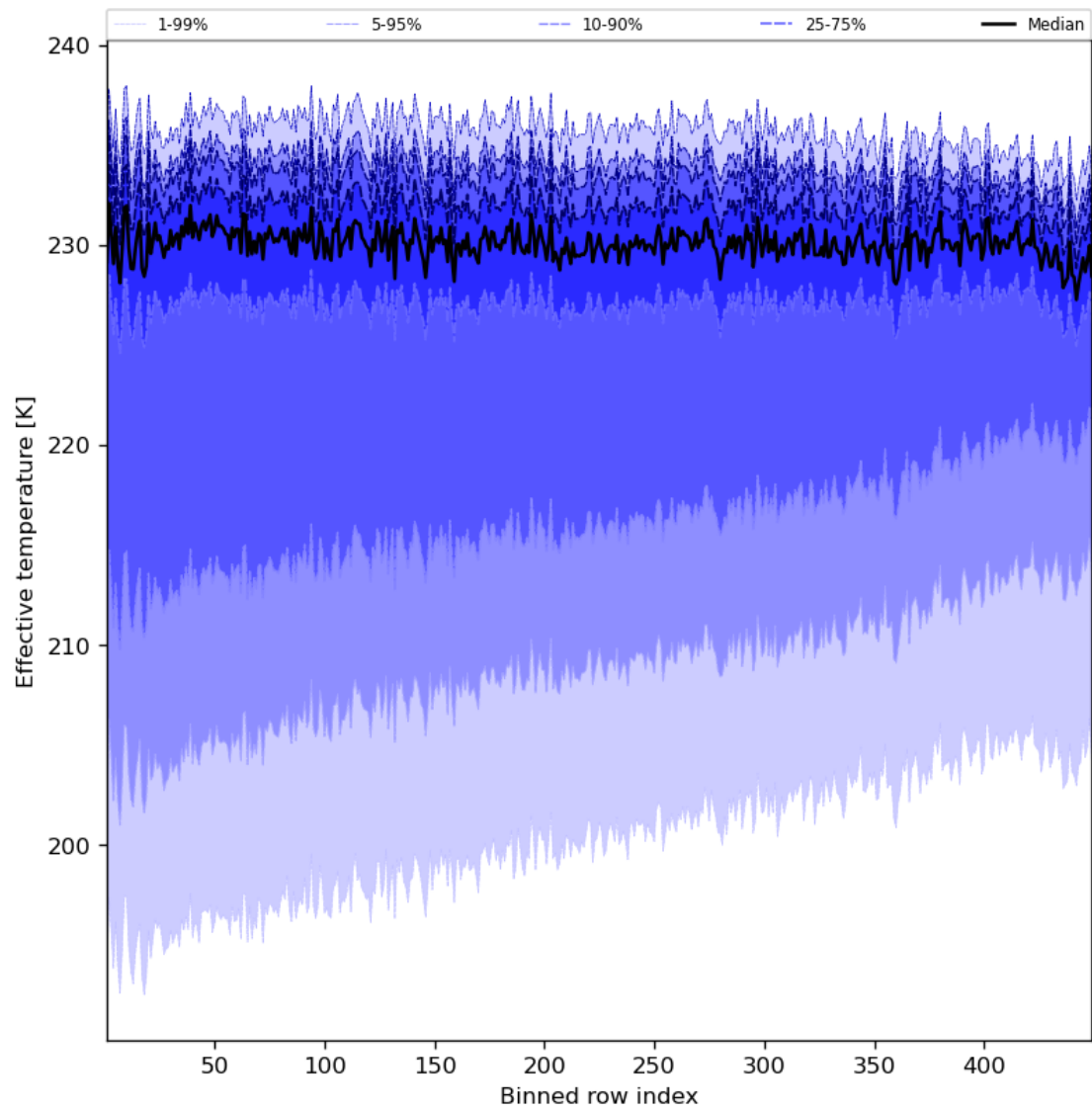
Figure 31: Along track statistics of “Effective temperature” for 2023-09-16 to 2023-09-18
