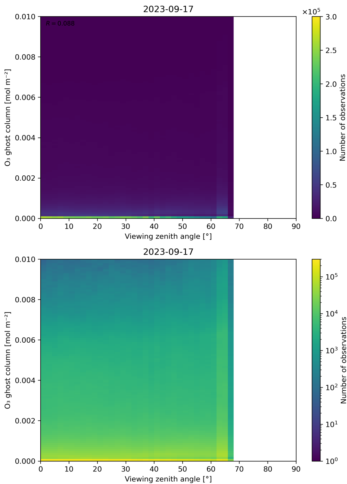
Figure 51: Scatter density plot of “Viewing zenith angle” against “O 3 ghost column” for 2023-09-16 to 2023-09-18.
