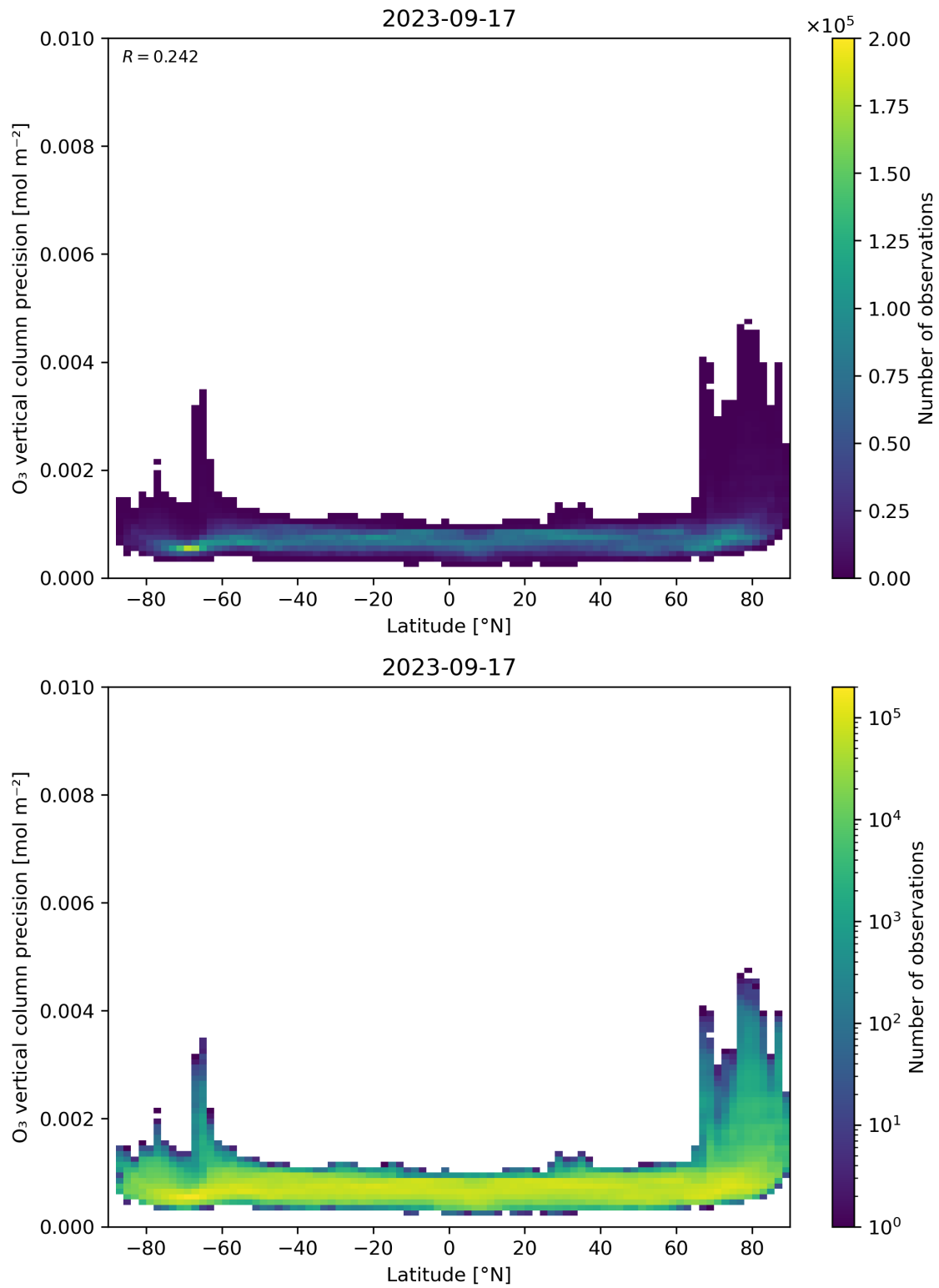
Figure 37: Scatter density plot of “Latitude” against “O 3 vertical column precision” for 2023-09-16 to 2023-09-18.
