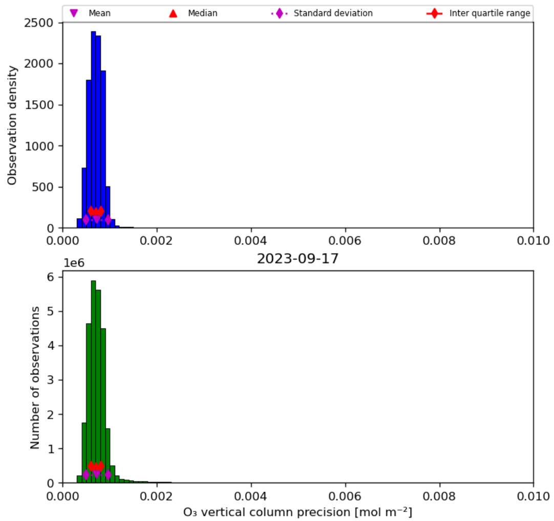
Figure 22: Histogram of “O 3 vertical column precision” for 2023-09-16 to 2023-09-18
