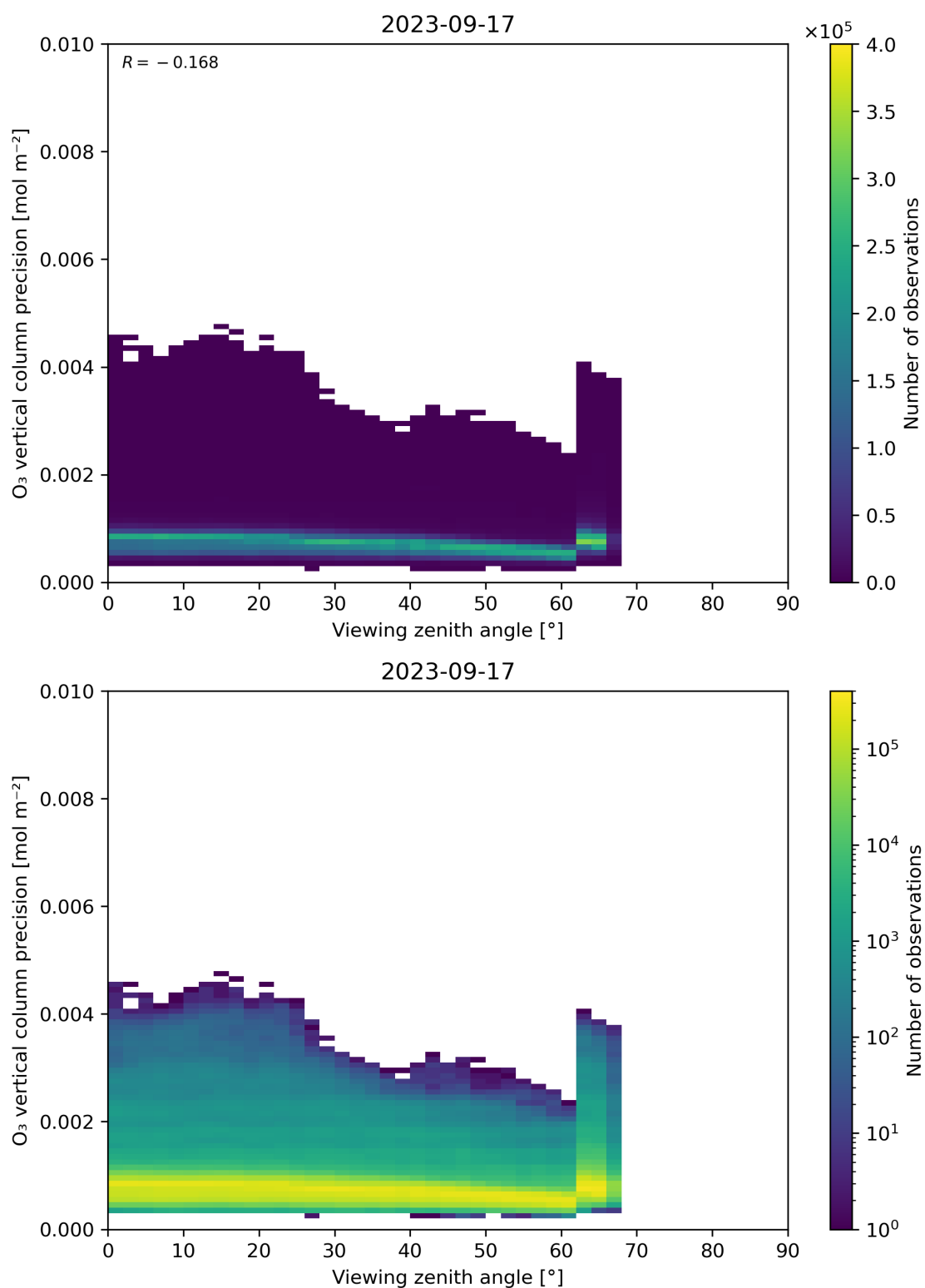
Figure 53: Scatter density plot of “Viewing zenith angle” against “O 3 vertical column precision” for 2023-09-16 to 2023-09-18.
