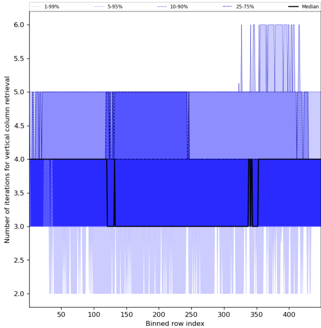
Figure 33: Along track statistics of “Number of iterations for vertical column retrieval” for 2023-09-16 to 2023-09-18
