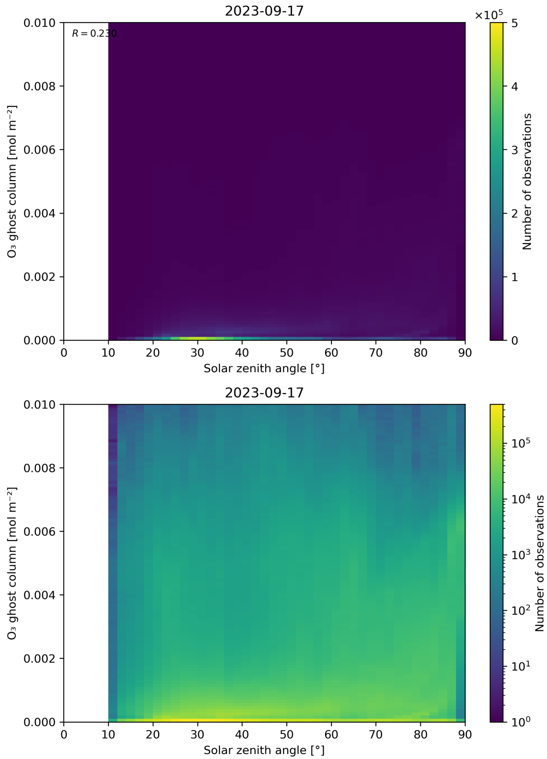
Figure 46: Scatter density plot of “Solar zenith angle” against “O 3 ghost column” for 2023-09-16 to 2023-09-18.
