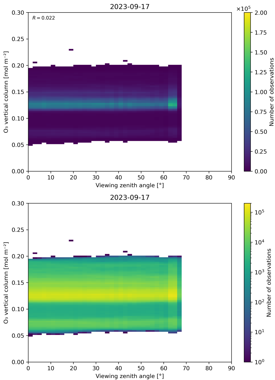
Figure 52: Scatter density plot of “Viewing zenith angle” against “O 3 vertical column” for 2023-09-16 to 2023-09-18.
