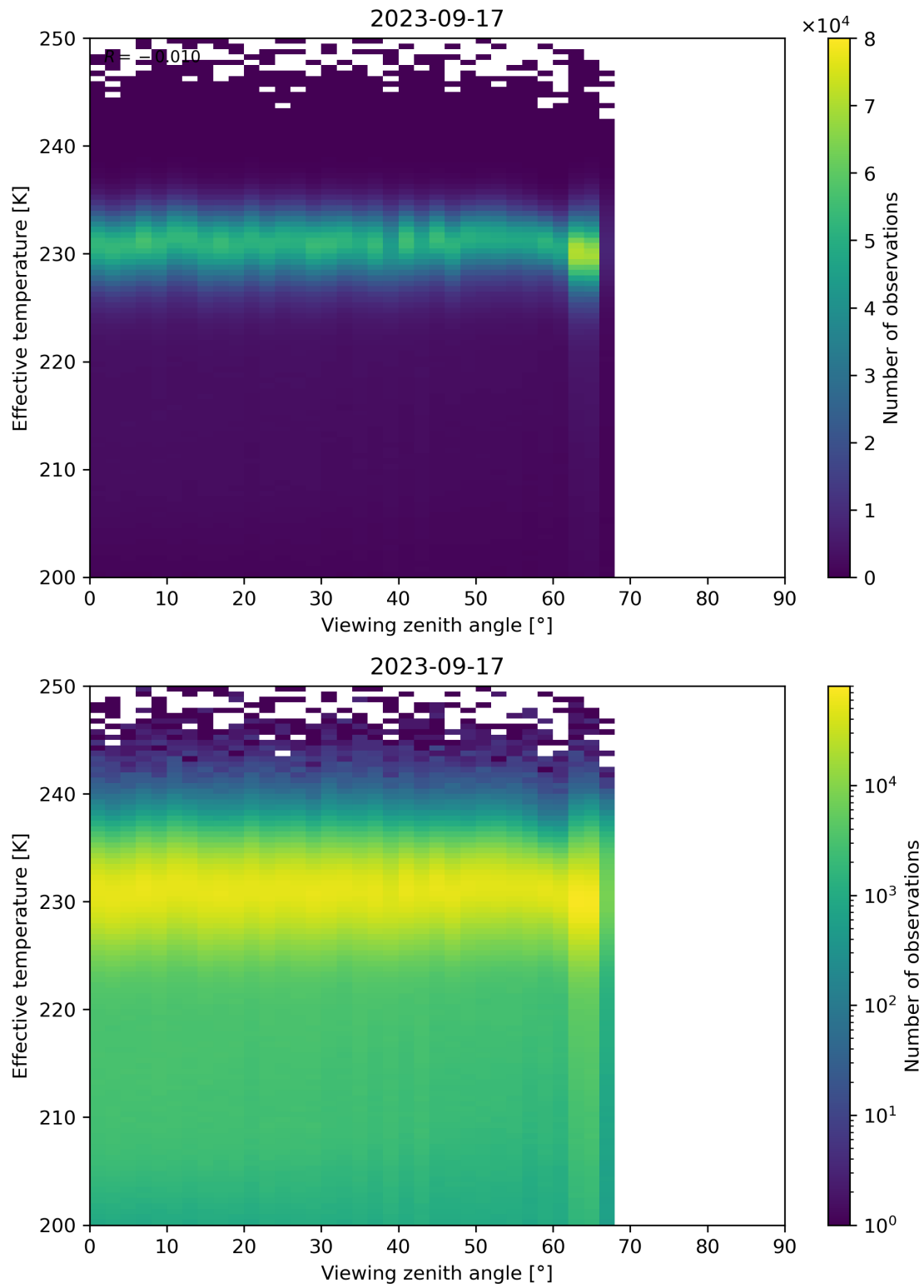
Figure 50: Scatter density plot of “Viewing zenith angle” against “Effective temperature” for 2023-09-16 to 2023-09-18.
