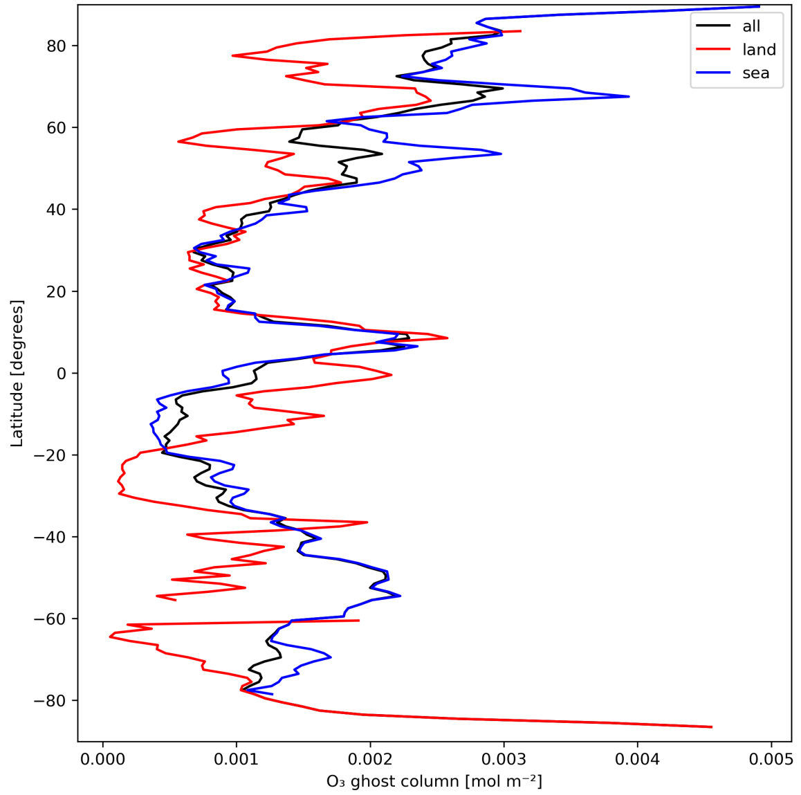
Figure 18: Zonal average of “O 3 ghost column” for 2023-09-16 to 2023-09-18.
