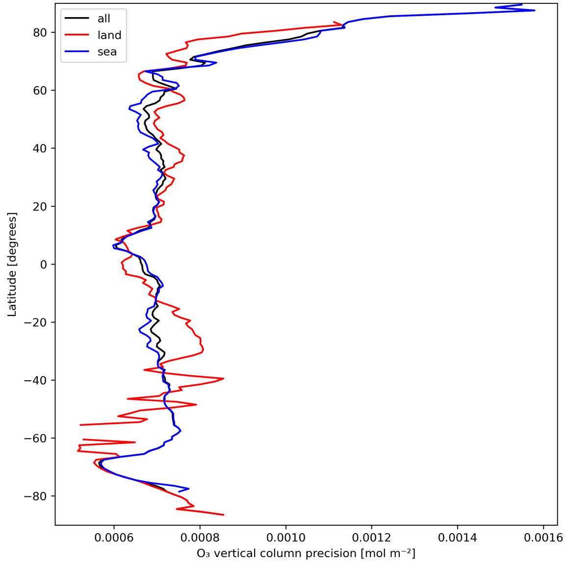
Figure 15: Zonal average of “O 3 vertical column precision” for 2023-09-16 to 2023-09-18.
