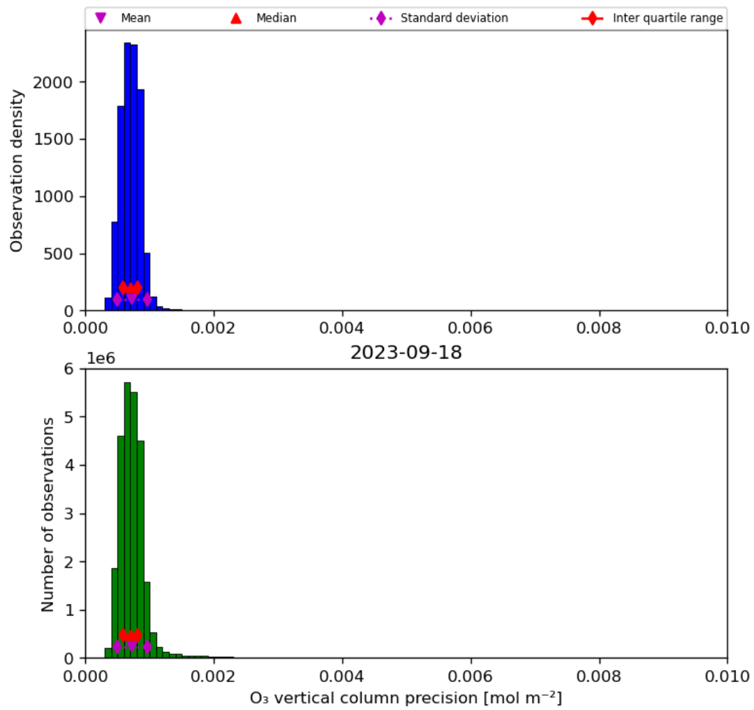
Figure 22: Histogram of “O 3 vertical column precision” for 2023-09-17 to 2023-09-19
