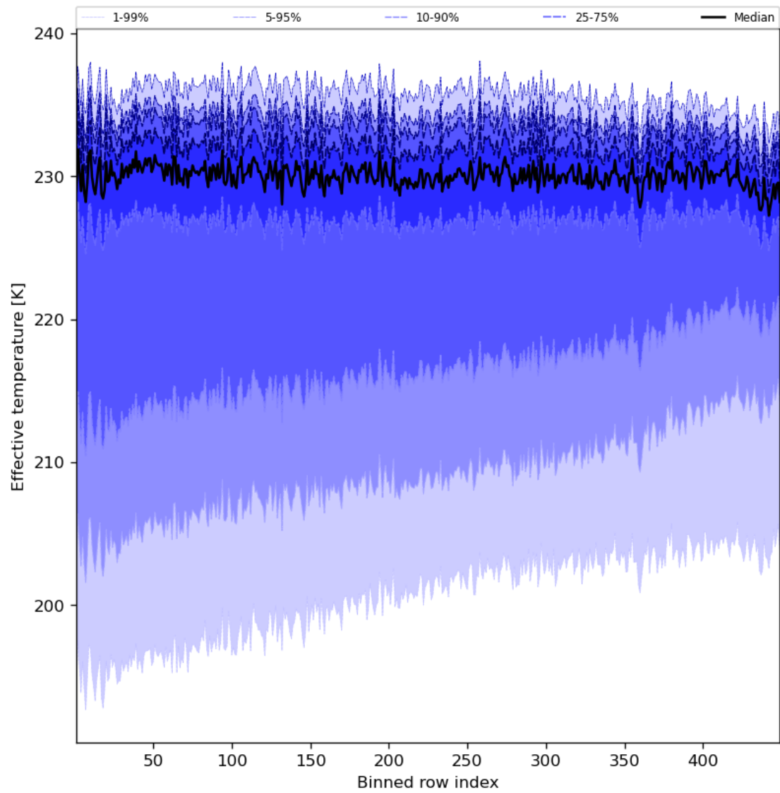
Figure 31: Along track statistics of “Effective temperature” for 2023-09-17 to 2023-09-19
