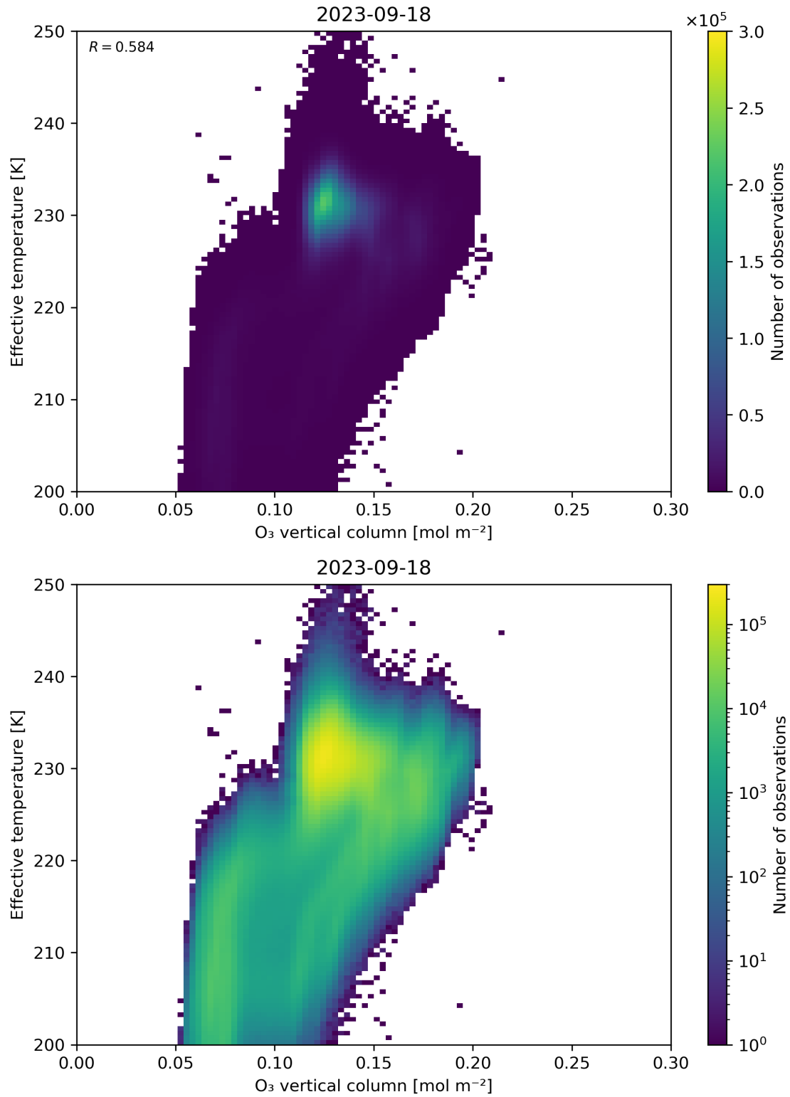
Figure 39: Scatter density plot of “O 3 vertical column” against “Effective temperature” for 2023-09-17 to 2023-09-19.
