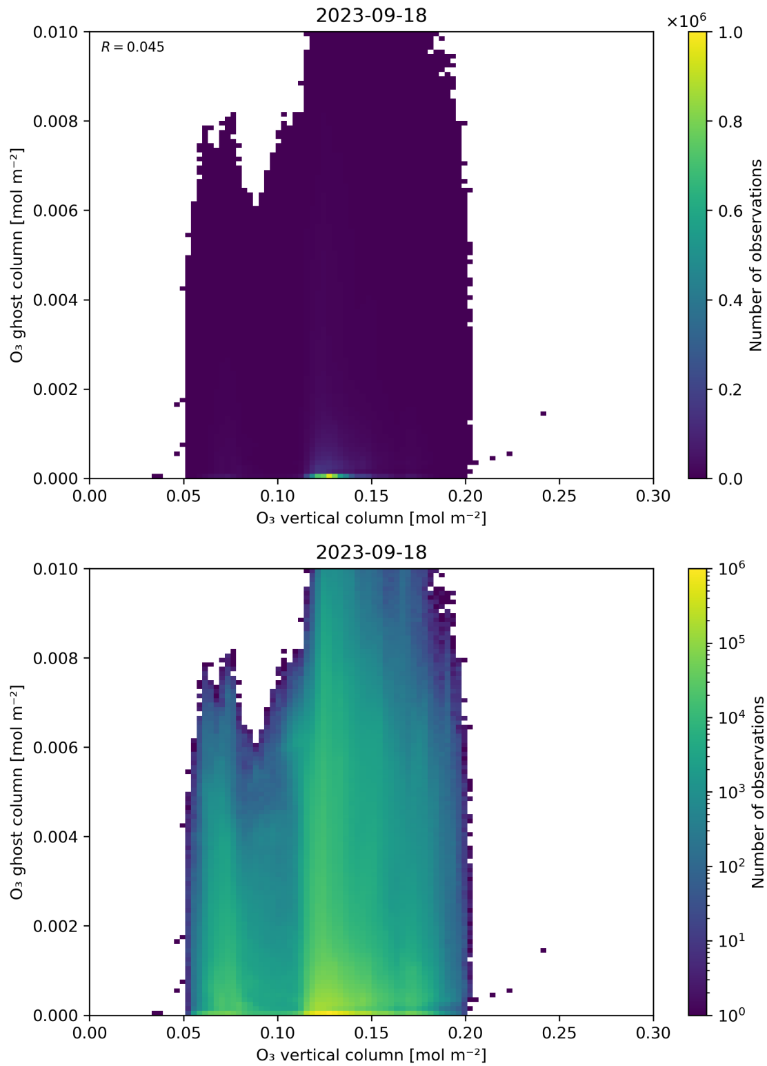
Figure 40: Scatter density plot of “O 3 vertical column” against “O 3 ghost column” for 2023-09-17 to 2023-09-19.
