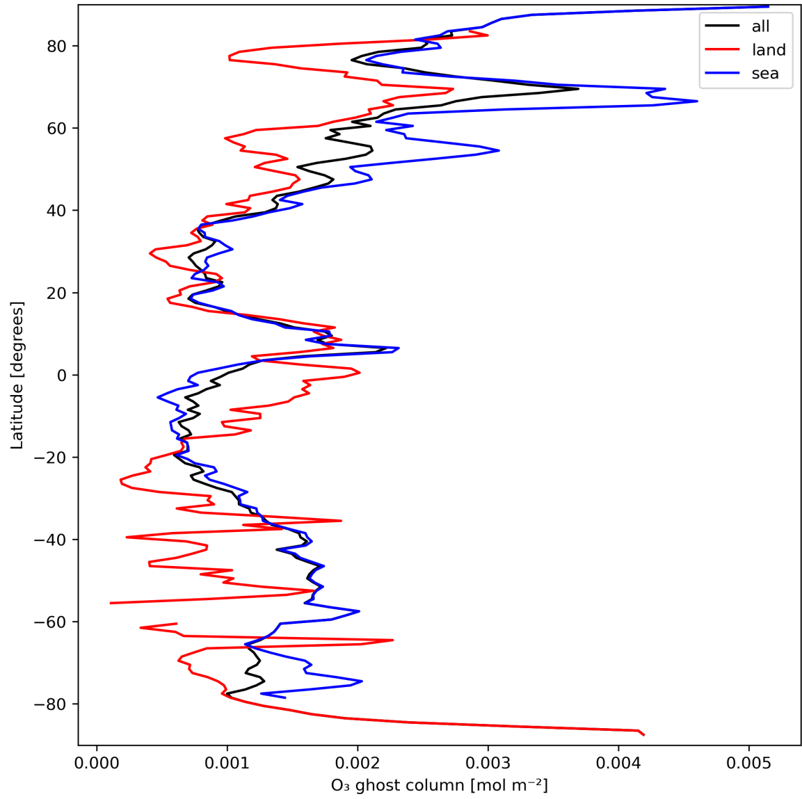
Figure 18: Zonal average of “O 3 ghost column” for 2023-09-17 to 2023-09-19.
