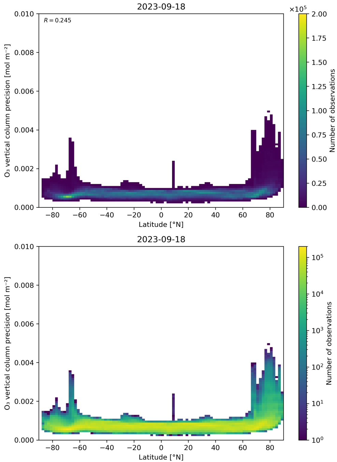
Figure 37: Scatter density plot of “Latitude” against “O 3 vertical column precision” for 2023-09-17 to 2023-09-19.
