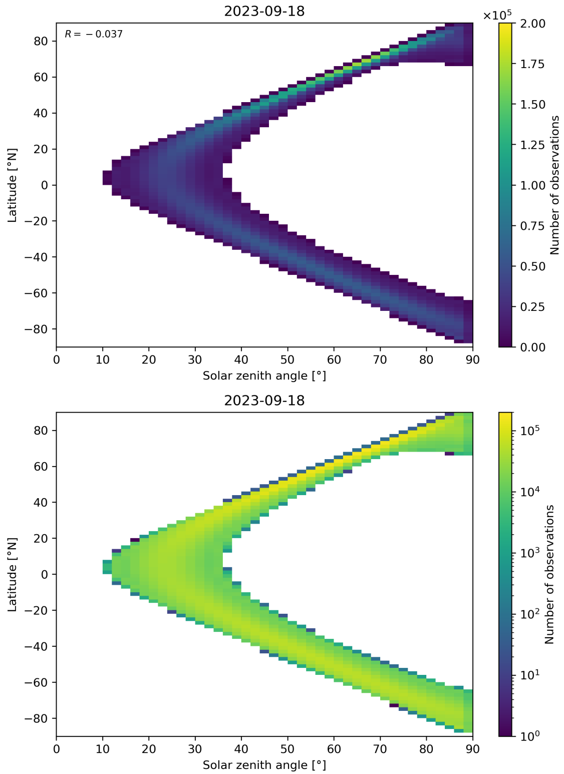
Figure 44: Scatter density plot of “Solar zenith angle” against “Latitude” for 2023-09-17 to 2023-09-19.
