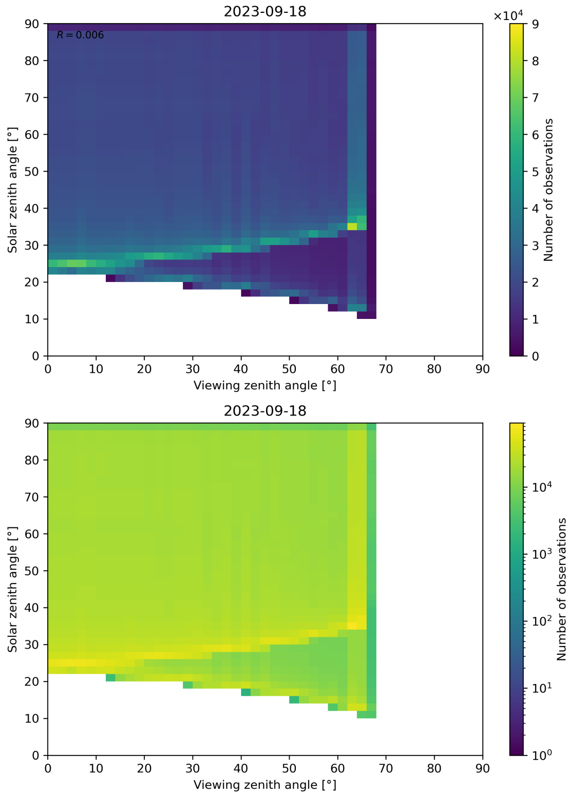
Figure 54: Scatter density plot of “Viewing zenith angle” against “Solar zenith angle” for 2023-09-17 to 2023-09-19.
