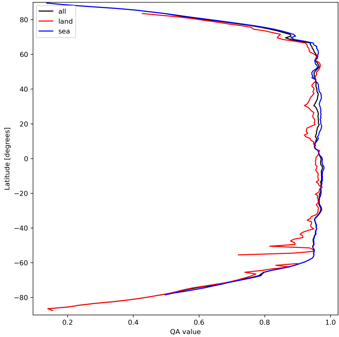
Figure 13: Zonal average of “QA value” for 2023-09-17 to 2023-09-19.
