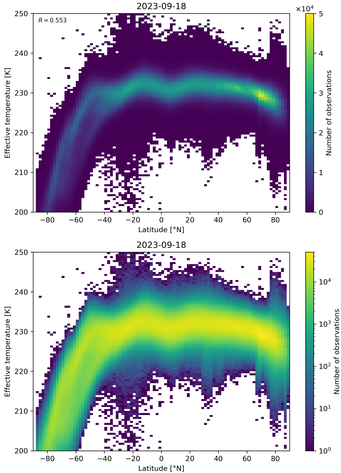
Figure 34: Scatter density plot of “Latitude” against “Effective temperature” for 2023-09-17 to 2023-09-19.
