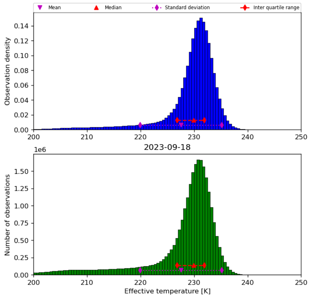
Figure 24: Histogram of “Effective temperature” for 2023-09-17 to 2023-09-19
