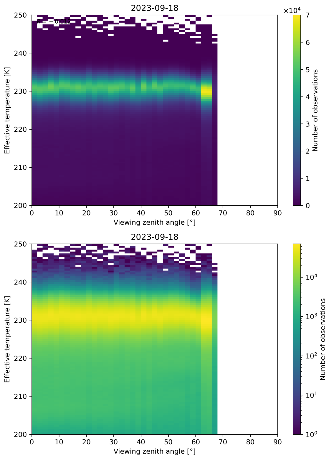
Figure 50: Scatter density plot of “Viewing zenith angle” against “Effective temperature” for 2023-09-17 to 2023-09-19.
