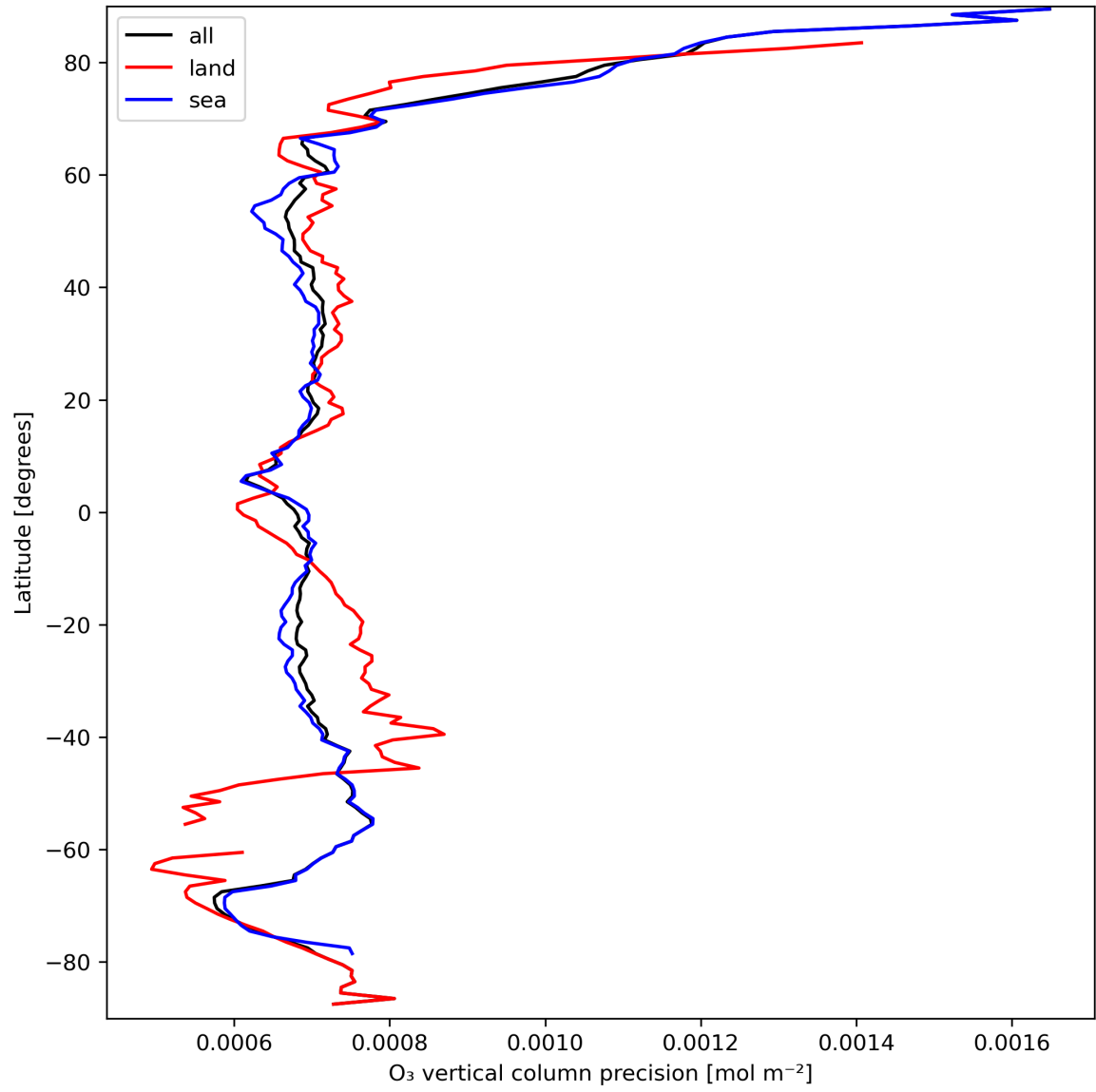
Figure 15: Zonal average of “O 3 vertical column precision” for 2023-09-17 to 2023-09-19.
