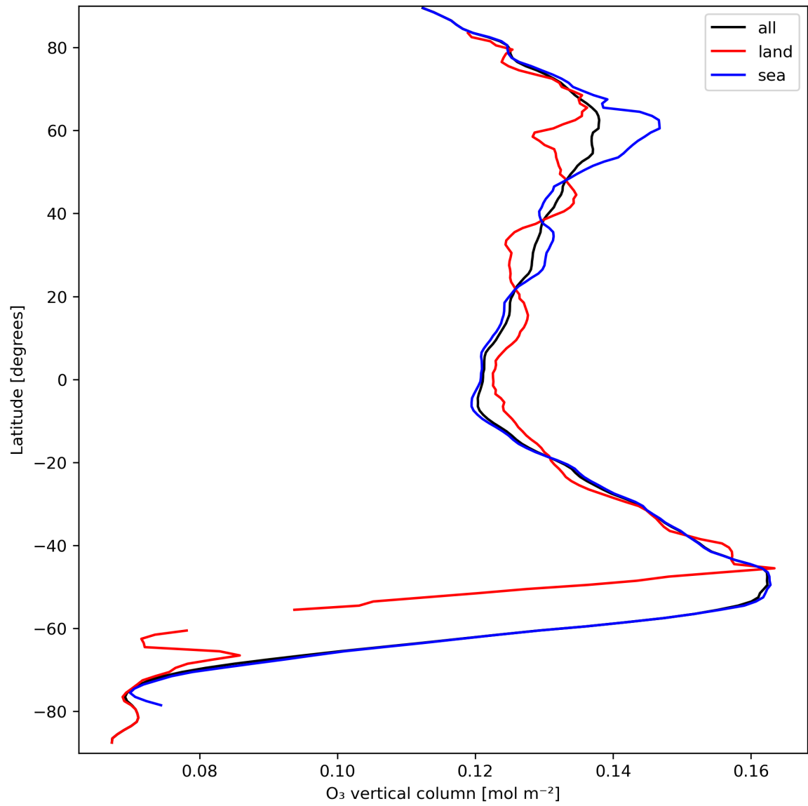
Figure 14: Zonal average of “O 3 vertical column” for 2023-09-17 to 2023-09-19.
