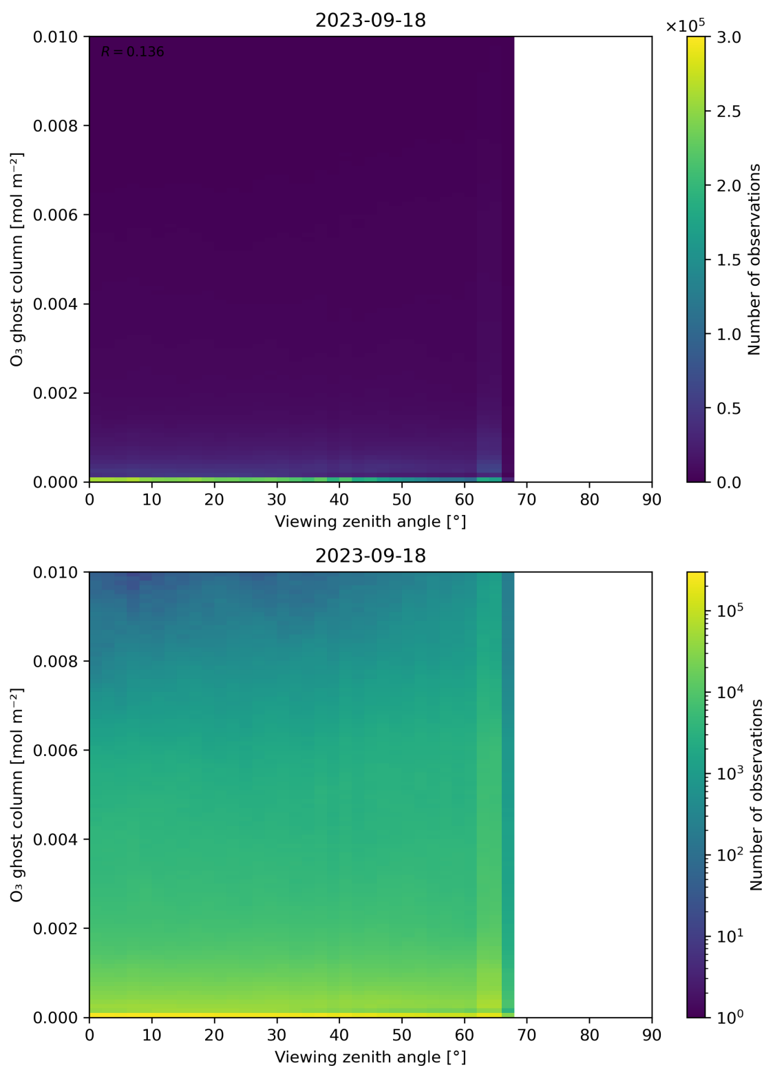
Figure 51: Scatter density plot of “Viewing zenith angle” against “O 3 ghost column” for 2023-09-17 to 2023-09-19.
