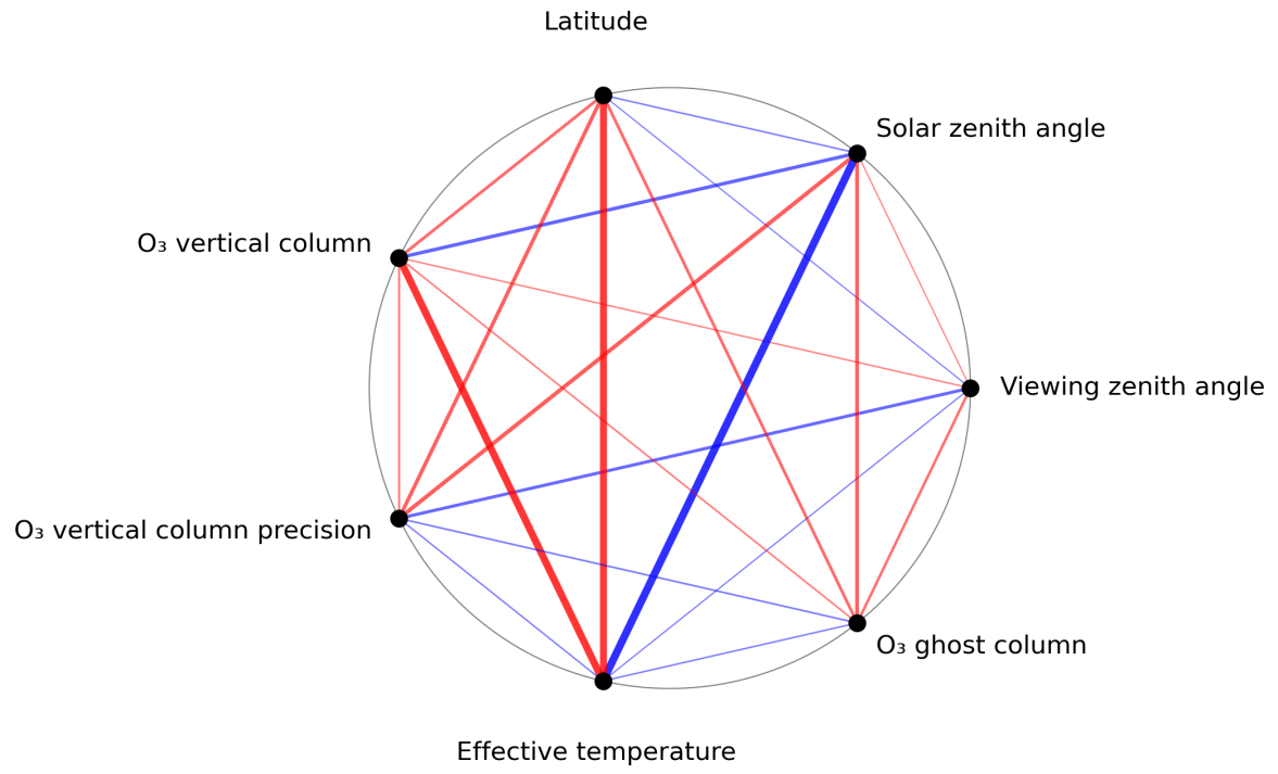
Figure 1: Map of correlation graph for 2023-09-17 to 2023-09-19.
