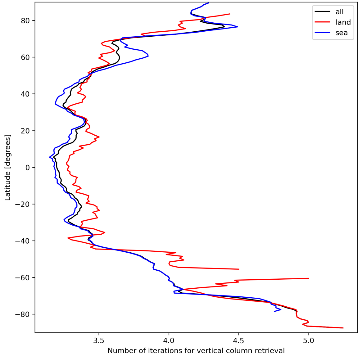
Figure 19: Zonal average of “Number of iterations for vertical column retrieval” for 2023-09-17 to 2023-09-19.
