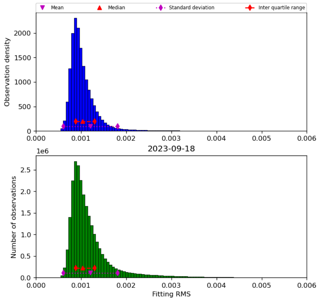
Figure 23: Histogram of “Fitting RMS” for 2023-09-17 to 2023-09-19
