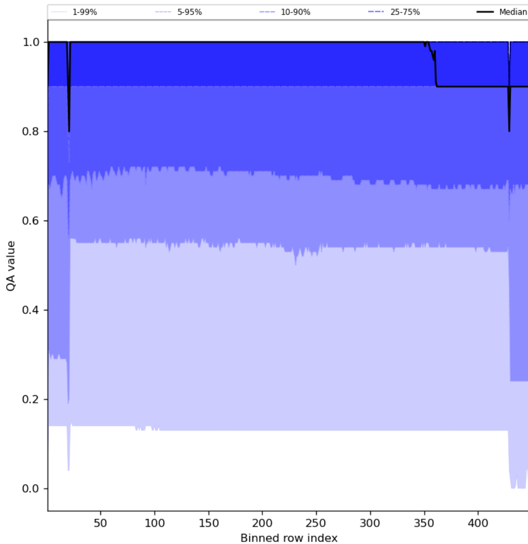
Figure 27: Along track statistics of “QA value” for 2023-09-17 to 2023-09-19
