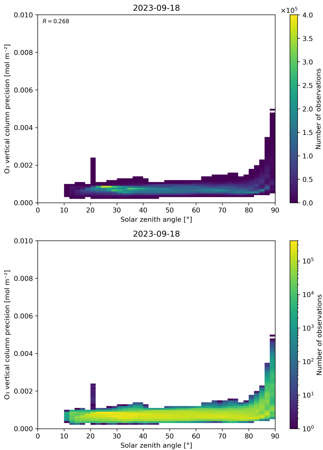
Figure 48: Scatter density plot of “Solar zenith angle” against “O 3 vertical column precision” for 2023-09-17 to 2023-09-19.
