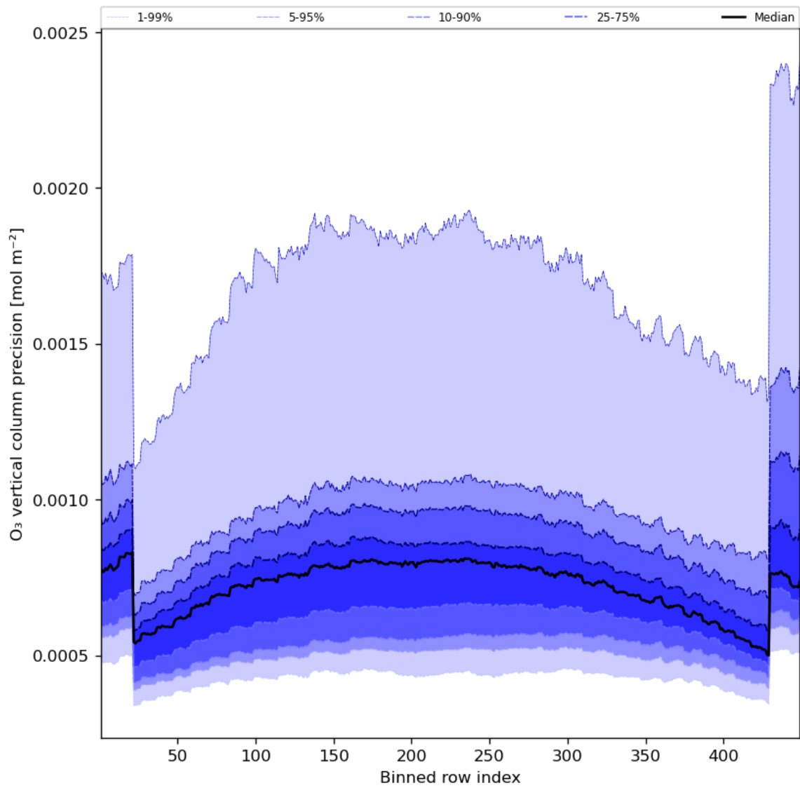
Figure 29: Along track statistics of “O 3 vertical column precision” for 2023-09-17 to 2023-09-19
