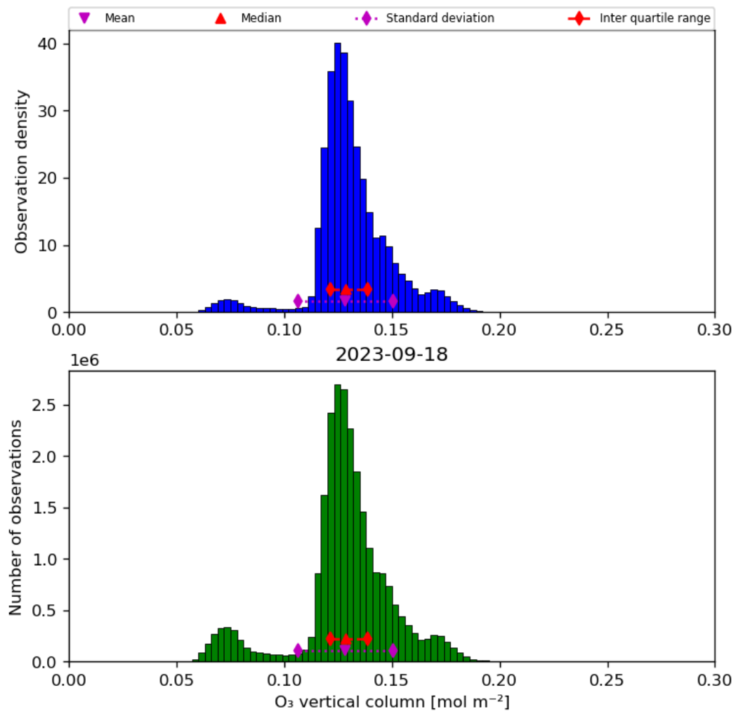
Figure 21: Histogram of “O 3 vertical column” for 2023-09-17 to 2023-09-19
