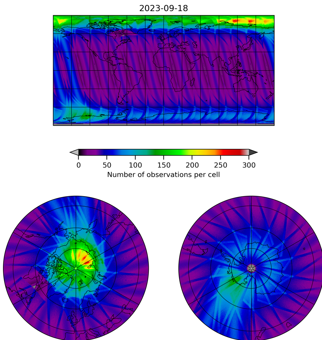
Figure 12: Map of the number of observations for 2023-09-17 to 2023-09-19
