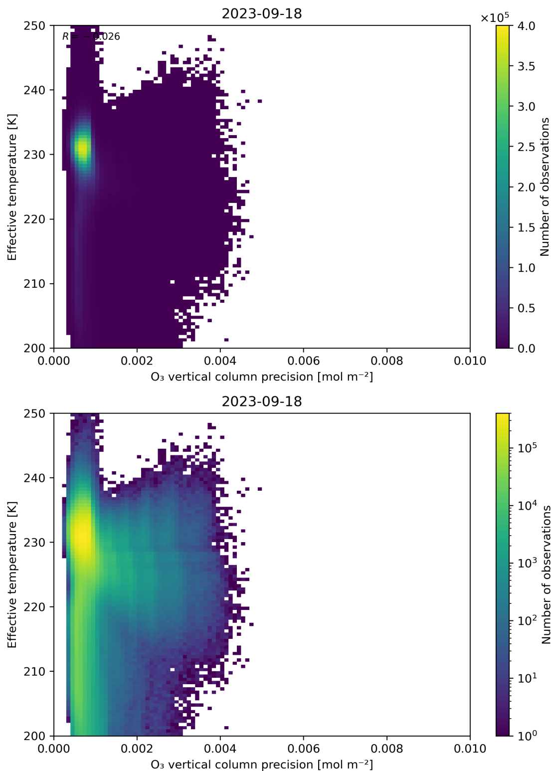
Figure 42: Scatter density plot of “O 3 vertical column precision” against “Effective temperature” for 2023-09-17 to 2023-09-19.
