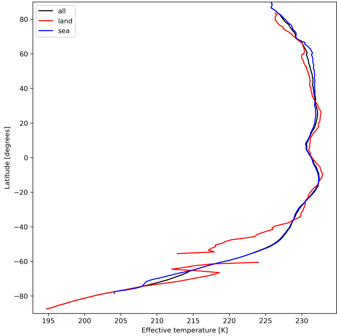
Figure 17: Zonal average of "Effective temperature" for 2023-09-17 to 2023-09-19.
