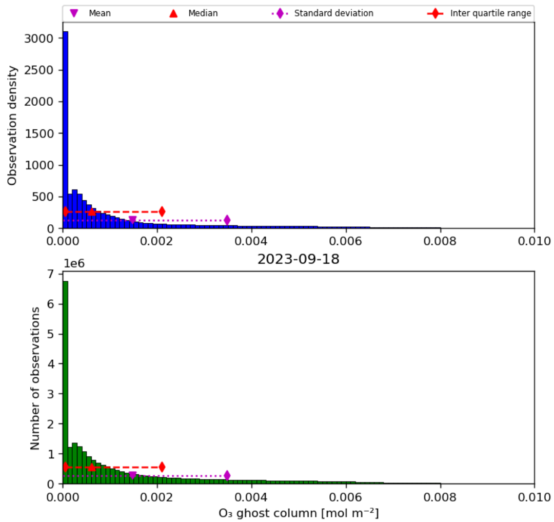
Figure 25: Histogram of “O 3 ghost column” for 2023-09-17 to 2023-09-19
