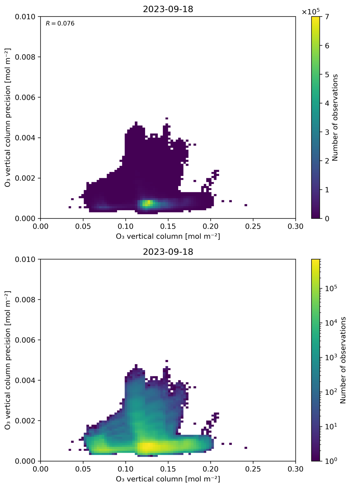
Figure 41: Scatter density plot of “O 3 vertical column” against “O 3 vertical column precision” for 2023-09-17 to 2023-09-19.
