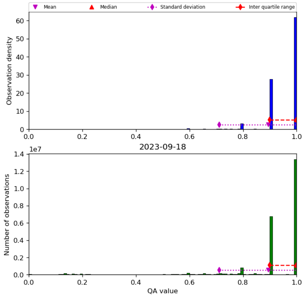
Figure 20: Histogram of “QA value” for 2023-09-17 to 2023-09-19
