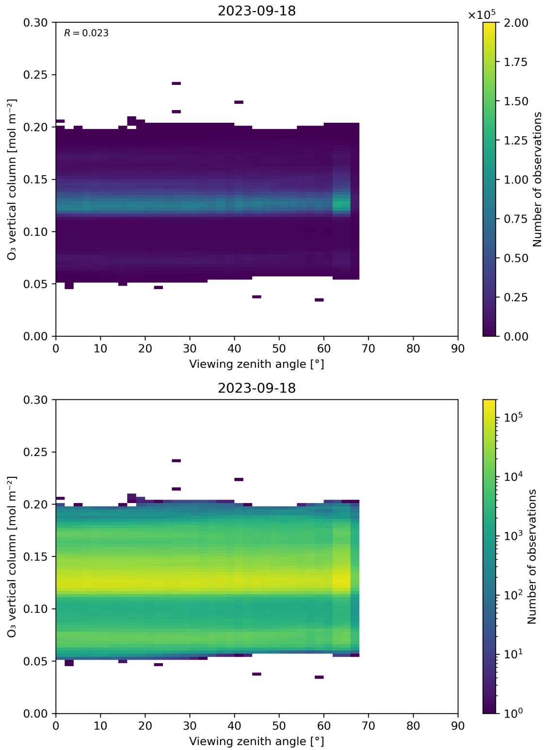
Figure 52: Scatter density plot of “Viewing zenith angle” against “O 3 vertical column” for 2023-09-17 to 2023-09-19.
