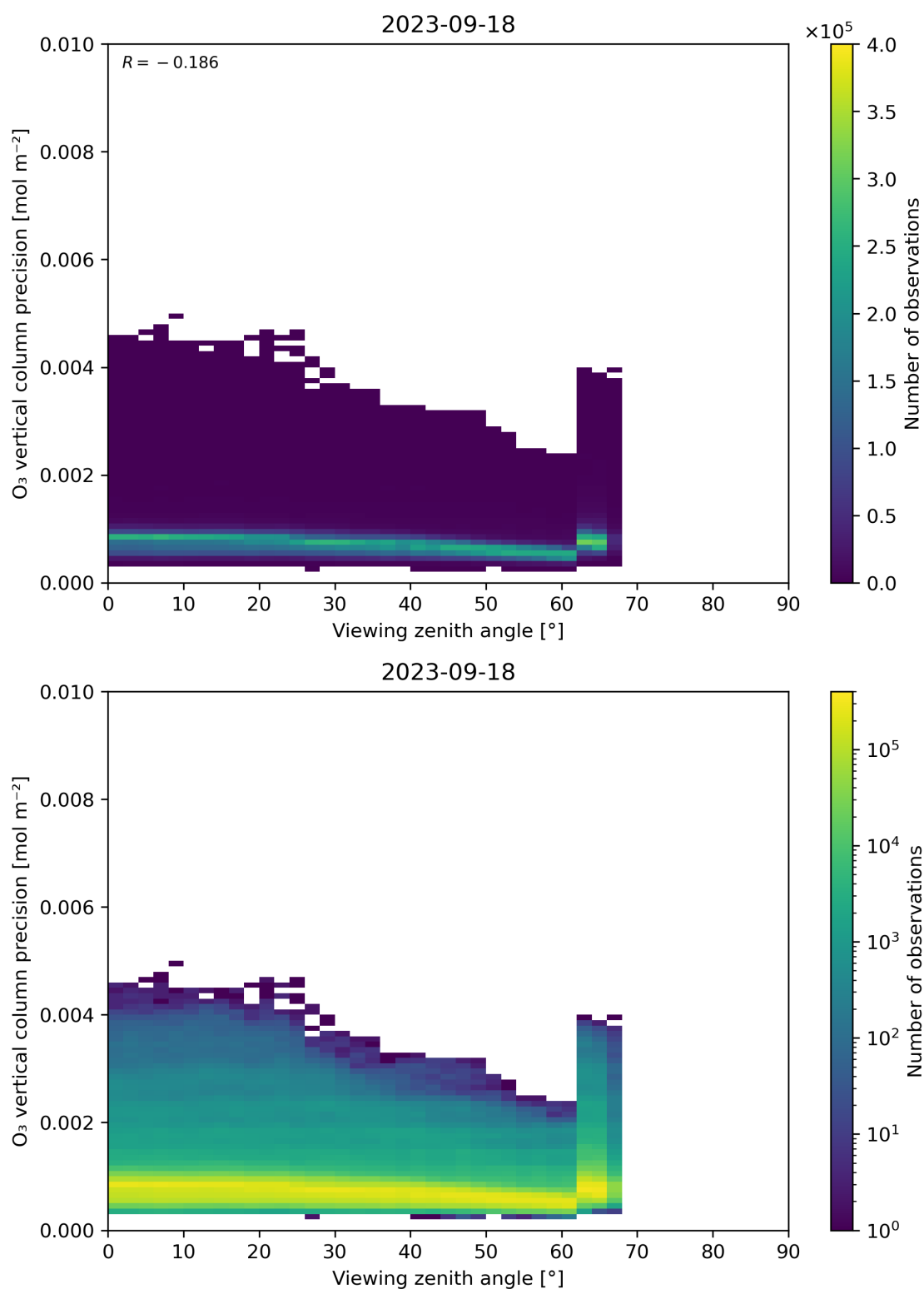
Figure 53: Scatter density plot of “Viewing zenith angle” against “O 3 vertical column precision” for 2023-09-17 to 2023-09-19.
