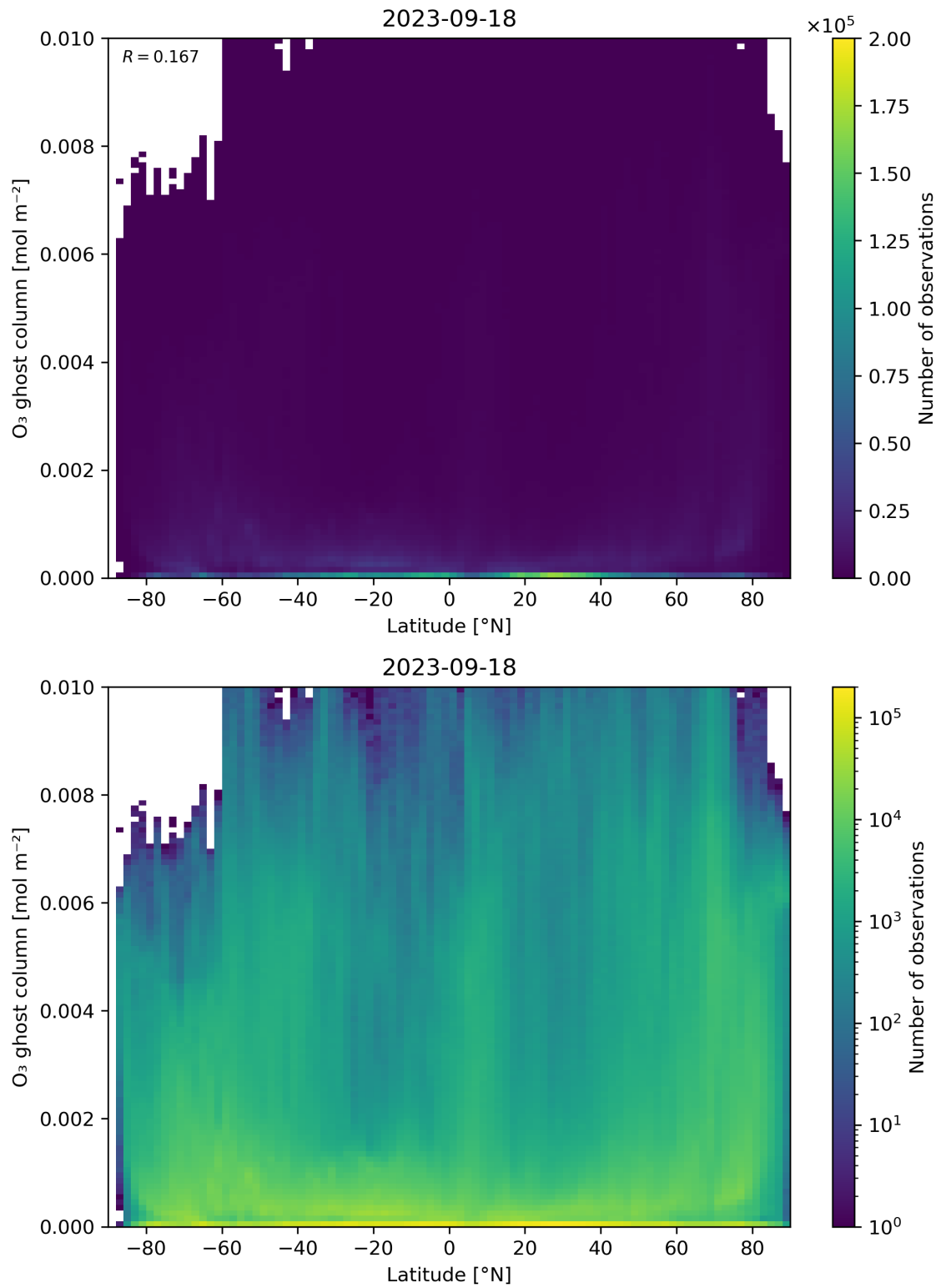
Figure 35: Scatter density plot of “Latitude” against “O 3 ghost column” for 2023-09-17 to 2023-09-19.
