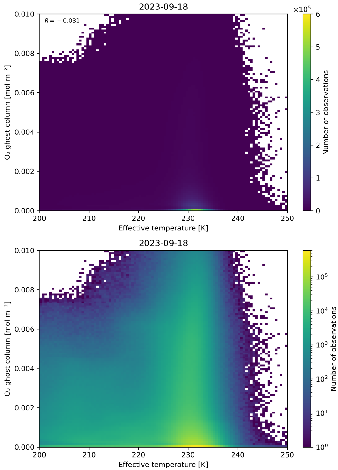
Figure 38: Scatter density plot of “Effective temperature” against “O 3 ghost column” for 2023-09-17 to 2023-09-19.
