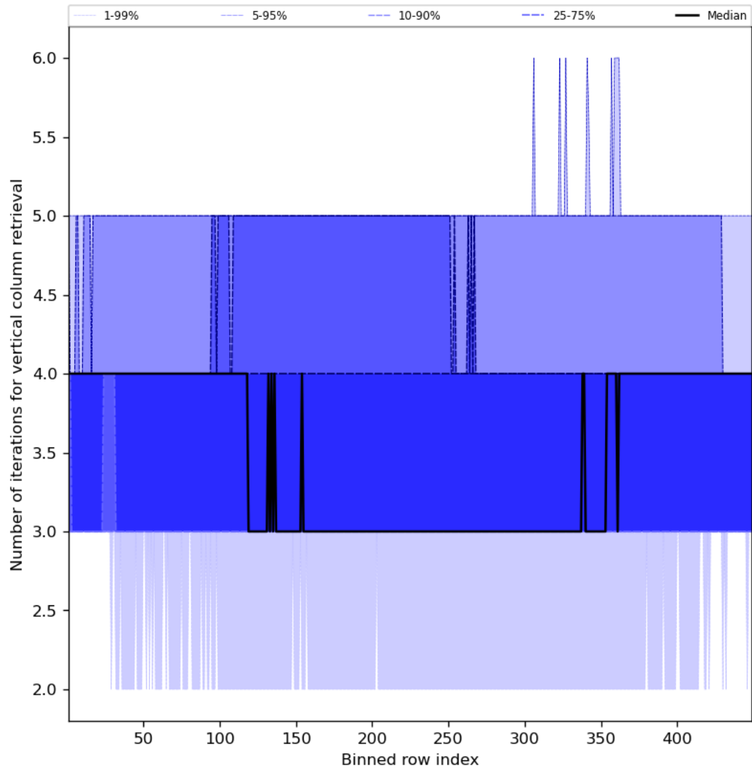
Figure 33: Along track statistics of “Number of iterations for vertical column retrieval” for 2023-09-17 to 2023-09-19
