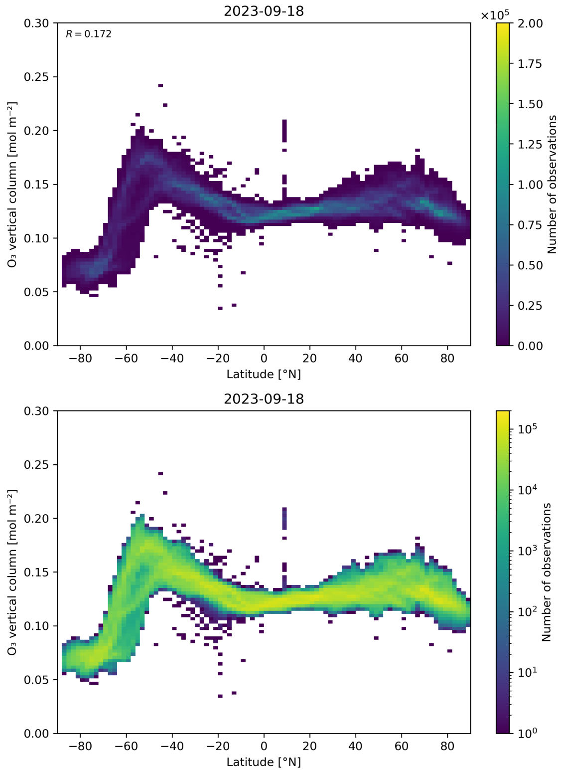
Figure 36: Scatter density plot of “Latitude” against “O 3 vertical column” for 2023-09-17 to 2023-09-19.
