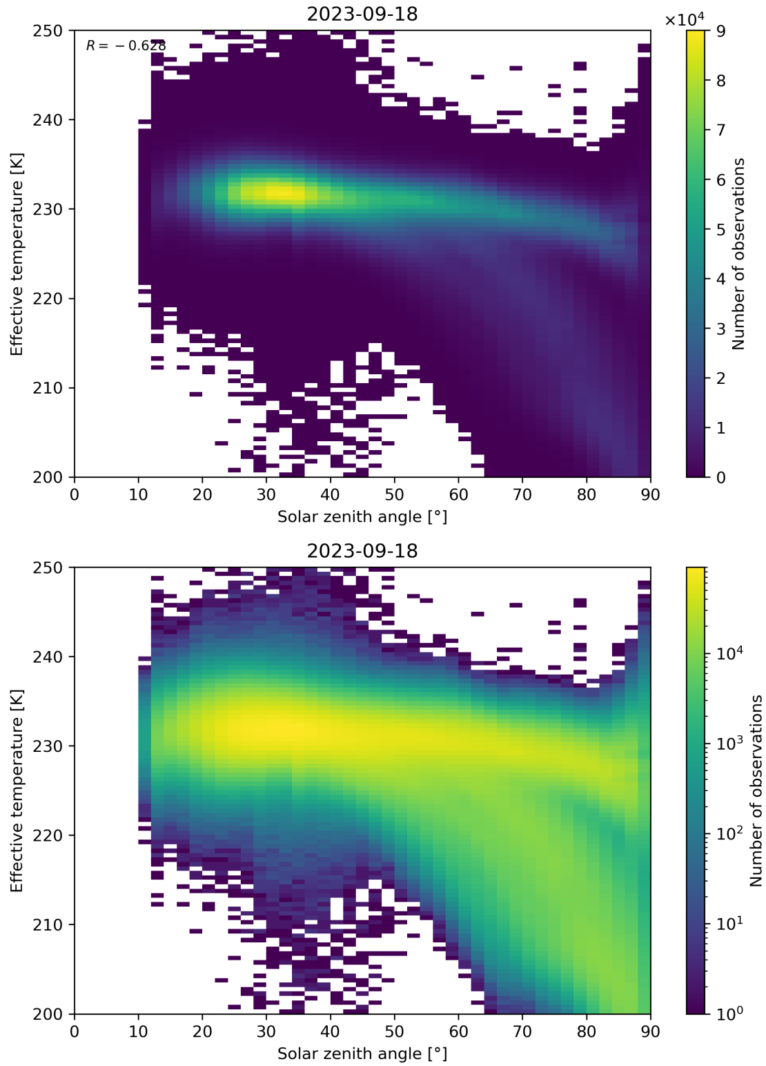
Figure 45: Scatter density plot of “Solar zenith angle” against “Effective temperature” for 2023-09-17 to 2023-09-19.
