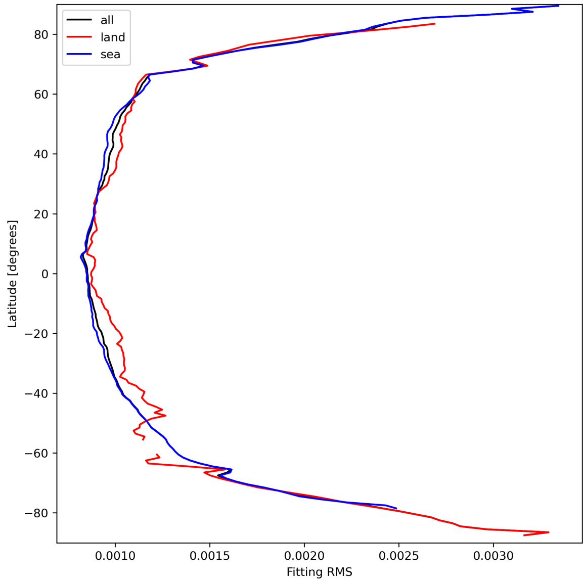
Figure 16: Zonal average of “Fitting RMS” for 2023-09-17 to 2023-09-19.
