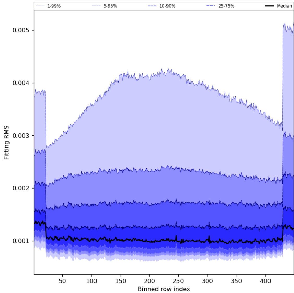
Figure 30: Along track statistics of “Fitting RMS” for 2023-09-17 to 2023-09-19
