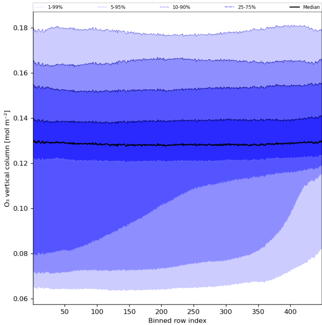
Figure 28: Along track statistics of “O 3 vertical column” for 2023-09-17 to 2023-09-19
