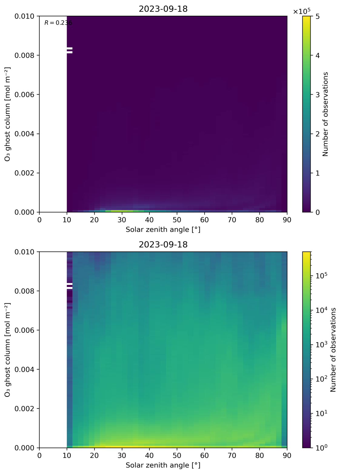
Figure 46: Scatter density plot of “Solar zenith angle” against “O 3 ghost column” for 2023-09-17 to 2023-09-19.
