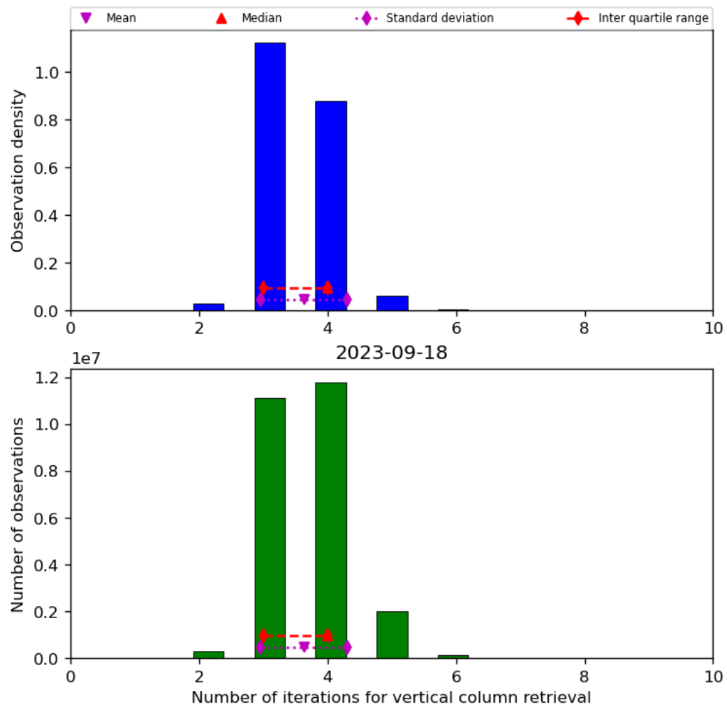
Figure 26: Histogram of “Number of iterations for vertical column retrieval” for 2023-09-17 to 2023-09-19
