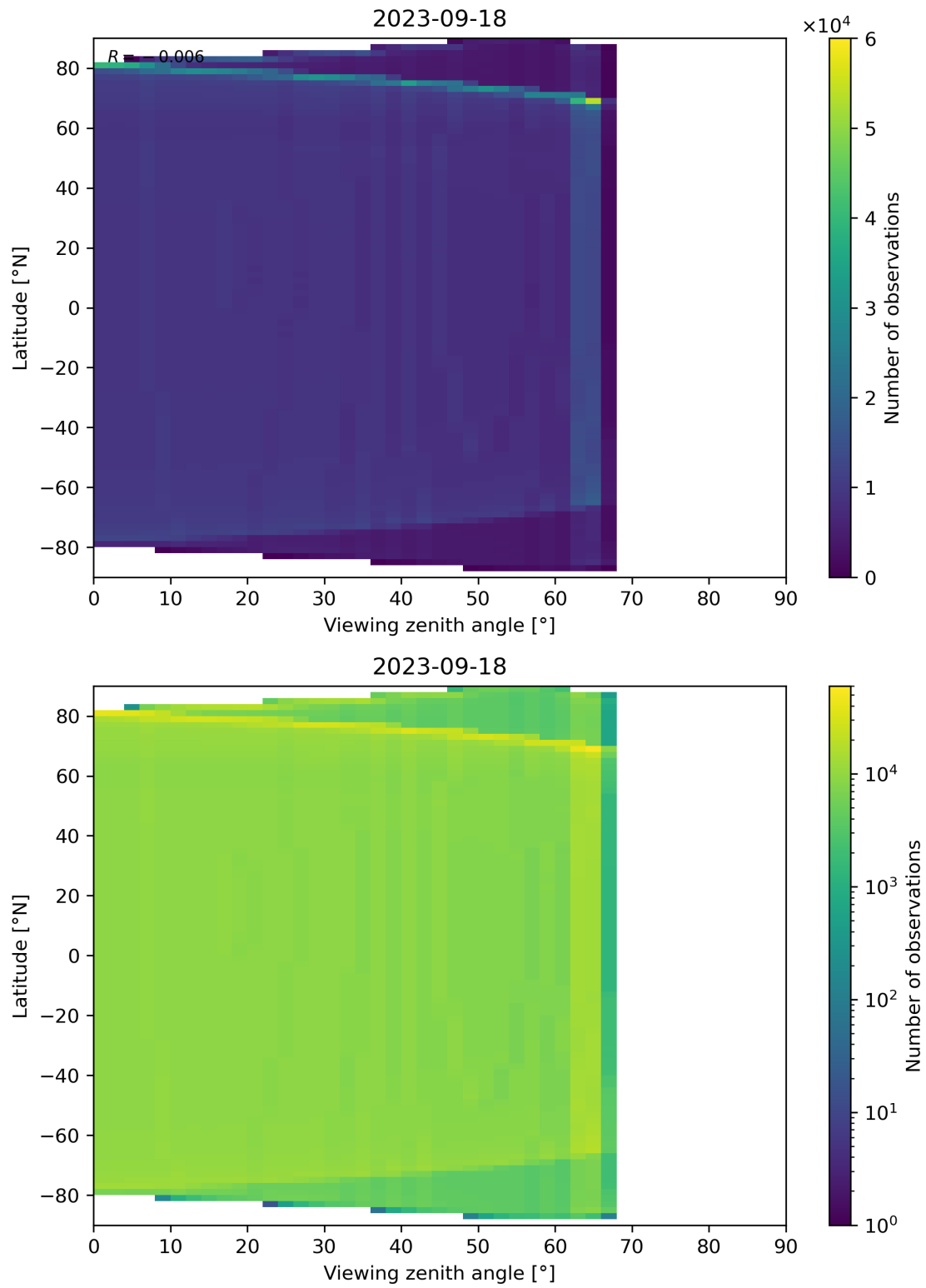
Figure 49: Scatter density plot of “Viewing zenith angle” against “Latitude” for 2023-09-17 to 2023-09-19.
