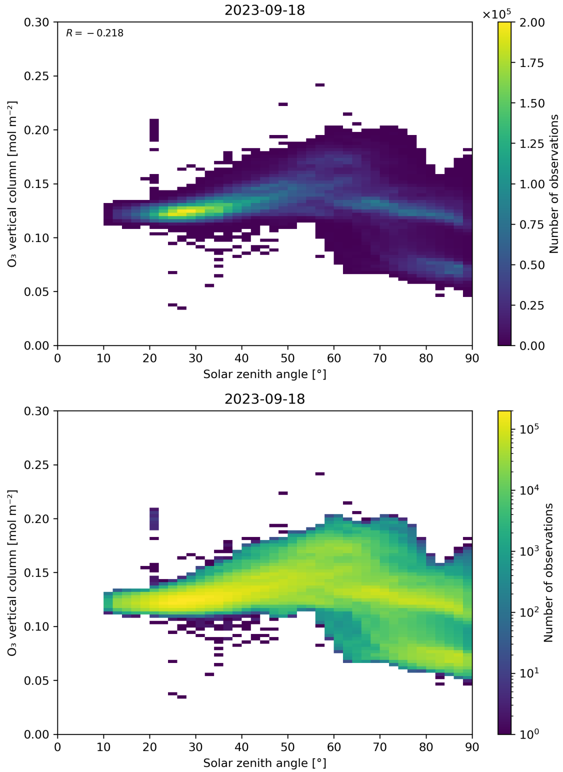
Figure 47: Scatter density plot of “Solar zenith angle” against “O 3 vertical column” for 2023-09-17 to 2023-09-19.
