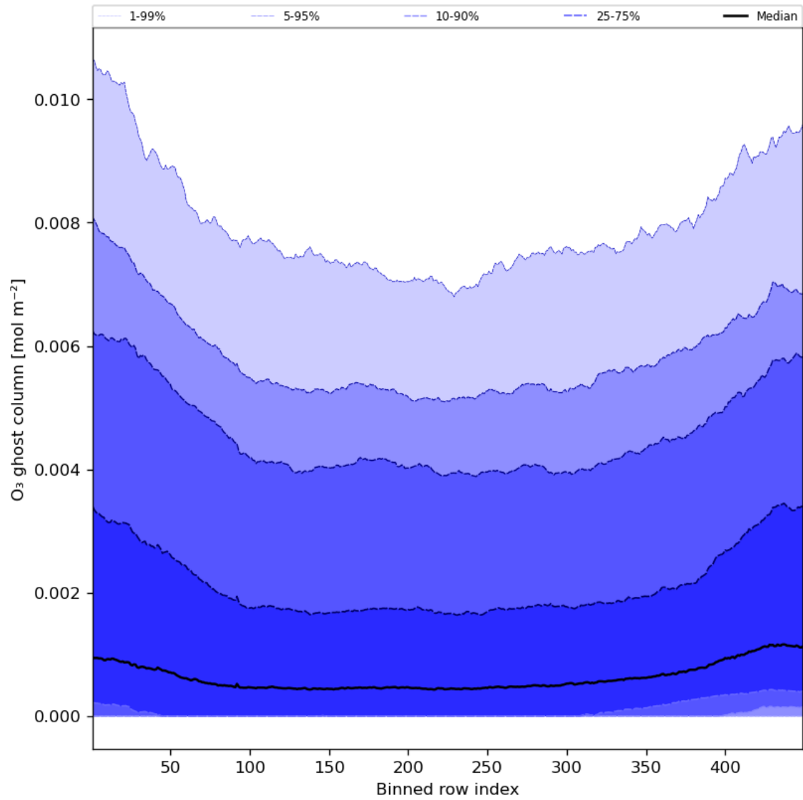
Figure 32: Along track statistics of “O 3 ghost column” for 2023-09-17 to 2023-09-19
