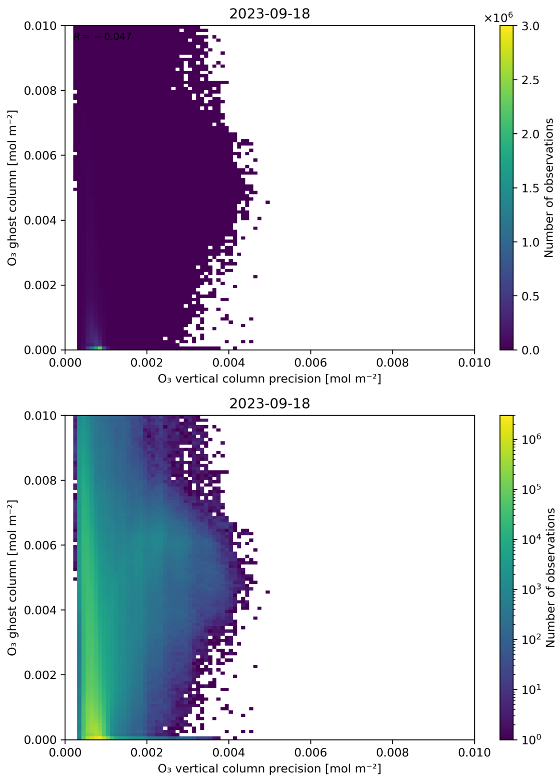
Figure 43: Scatter density plot of “ \text{O}_3 vertical column precision” against “ \text{O}_3 ghost column” for 2023-09-17 to 2023-09-19.
