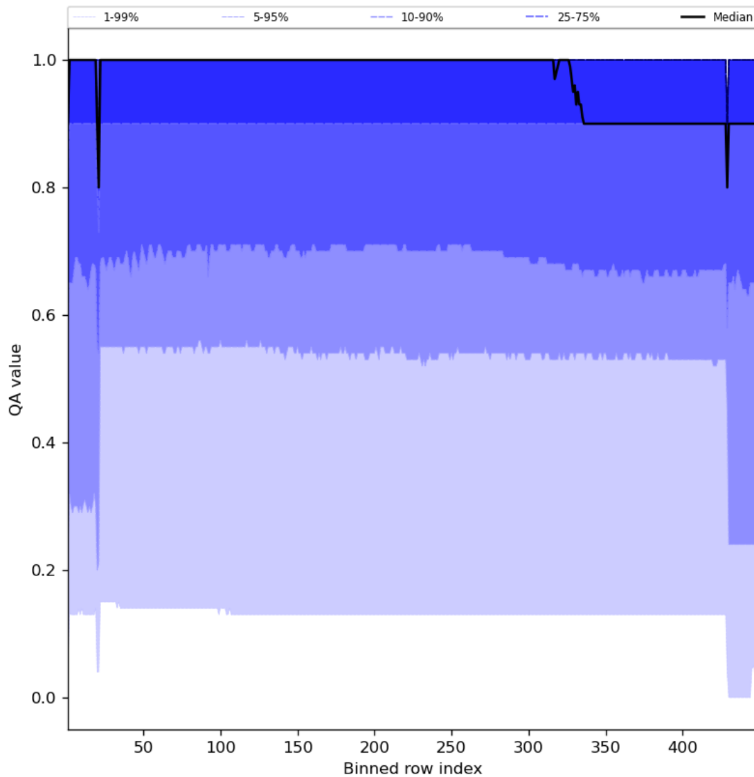
Figure 27: Along track statistics of “QA value” for 2023-09-20 to 2023-09-22
