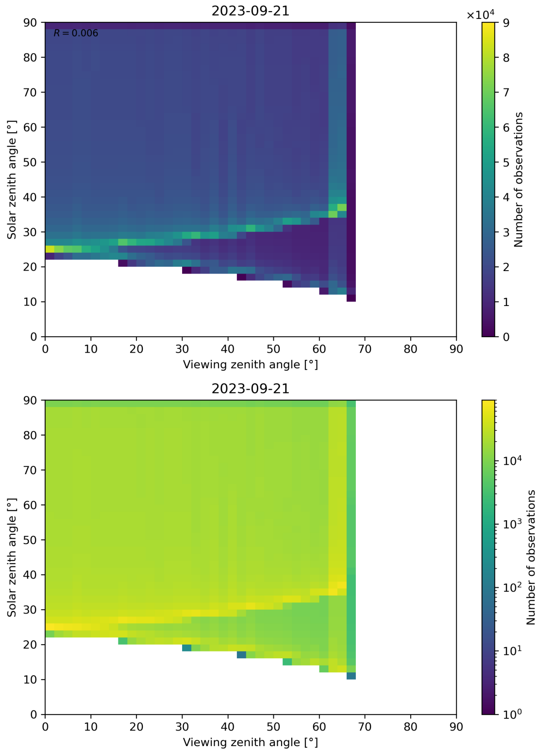
Figure 54: Scatter density plot of “Viewing zenith angle” against “Solar zenith angle” for 2023-09-20 to 2023-09-22.
