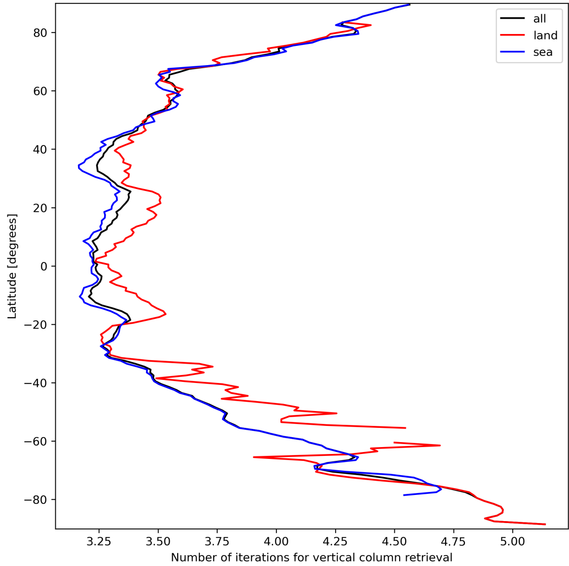
Figure 19: Zonal average of “Number of iterations for vertical column retrieval” for 2023-09-20 to 2023-09-22.
