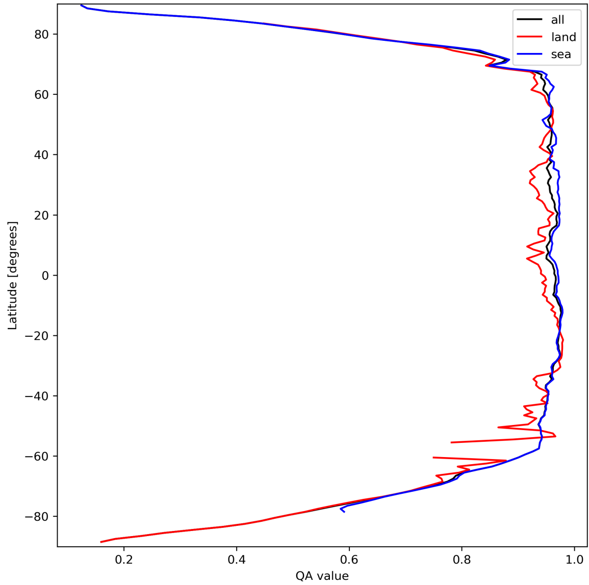
Figure 13: Zonal average of “QA value” for 2023-09-20 to 2023-09-22.
