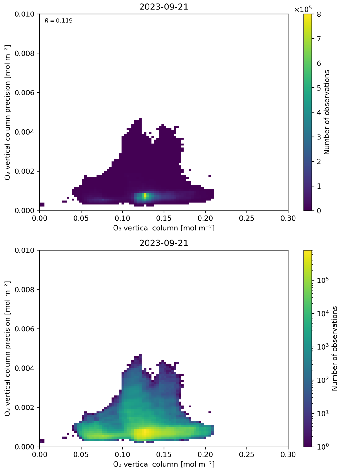
Figure 41: Scatter density plot of “O 3 vertical column” against “O 3 vertical column precision” for 2023-09-20 to 2023-09-22.
