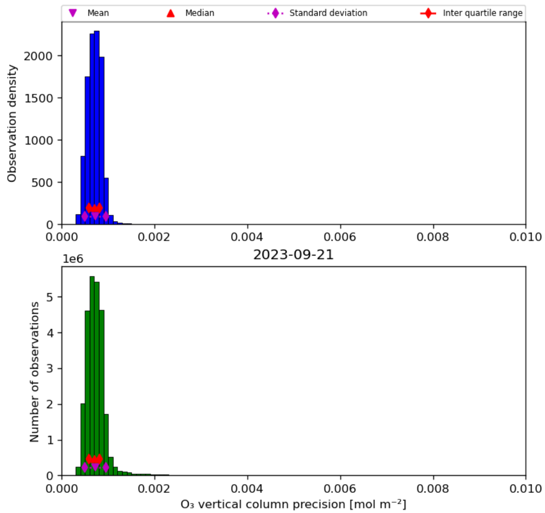
Figure 22: Histogram of “O 3 vertical column precision” for 2023-09-20 to 2023-09-22
