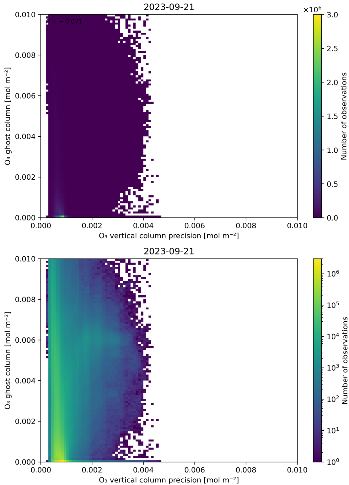
Figure 43: Scatter density plot of “O 3 vertical column precision” against “O 3 ghost column” for 2023-09-20 to 2023-09-22.
