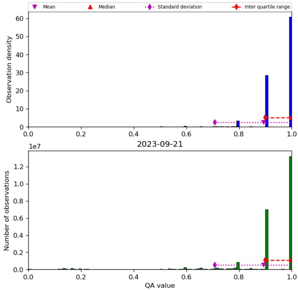
Figure 20: Histogram of “QA value” for 2023-09-20 to 2023-09-22
