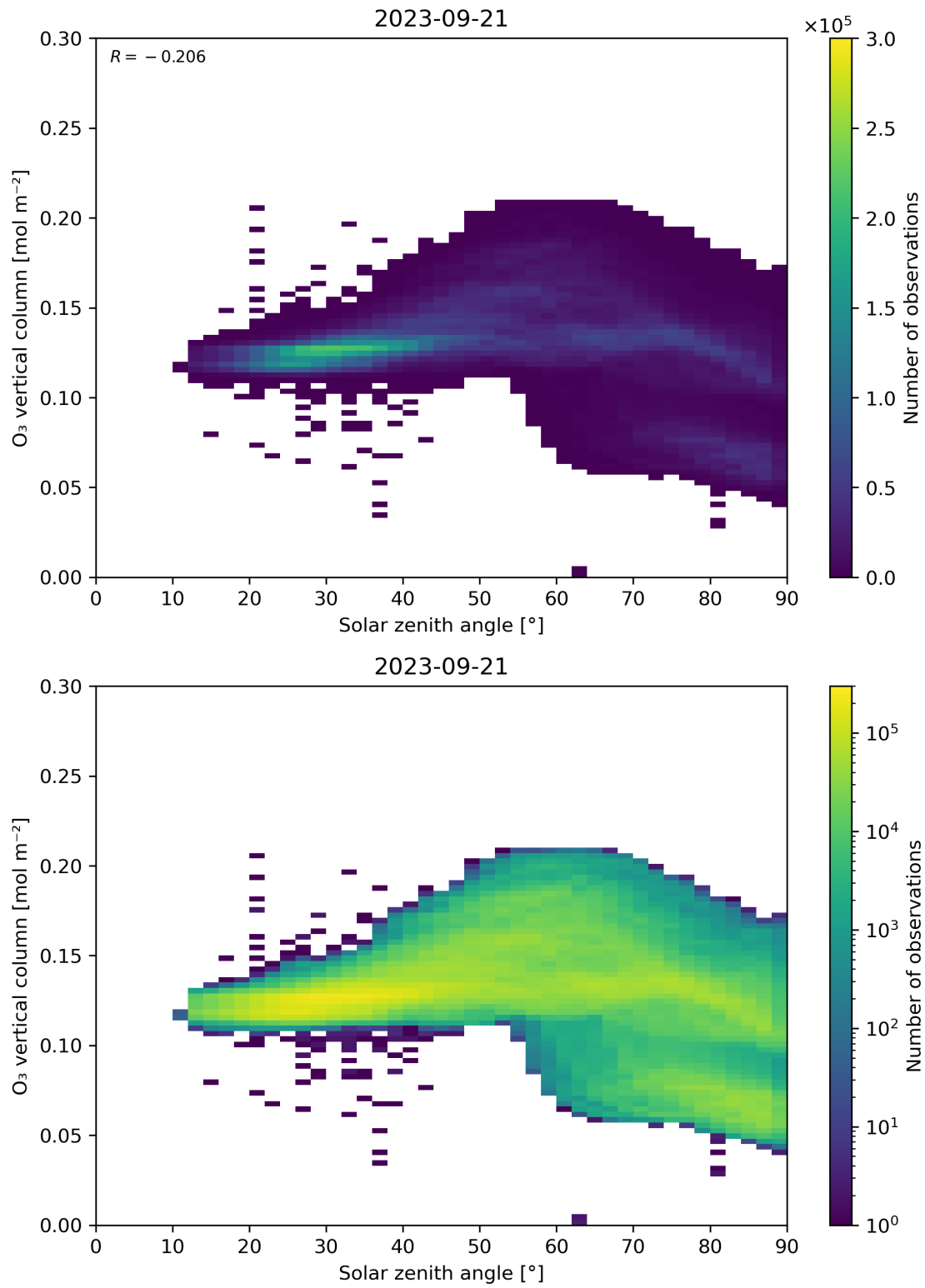
Figure 47: Scatter density plot of “Solar zenith angle” against “O 3 vertical column” for 2023-09-20 to 2023-09-22.
