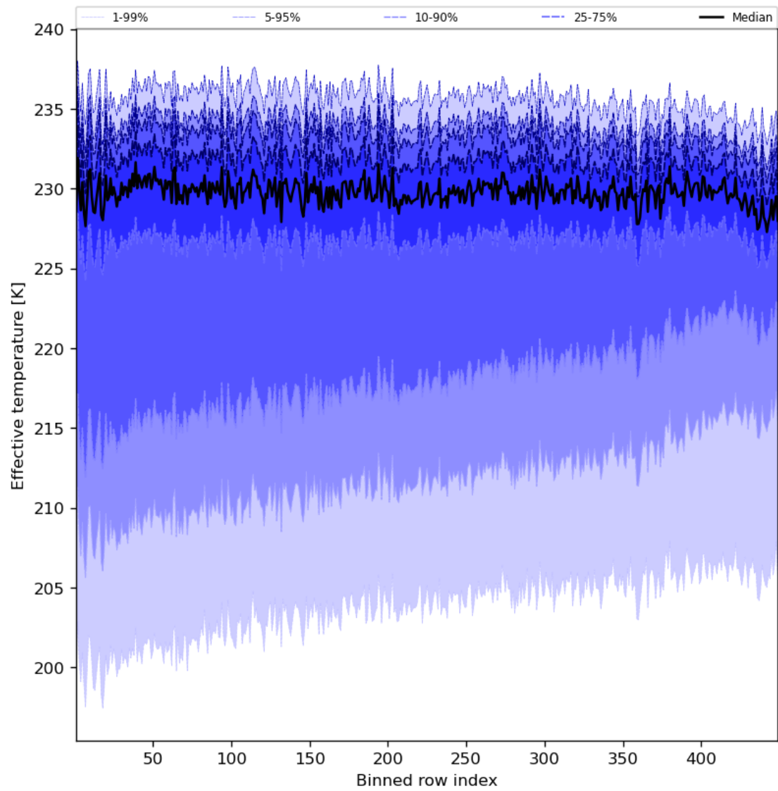
Figure 31: Along track statistics of “Effective temperature” for 2023-09-20 to 2023-09-22
