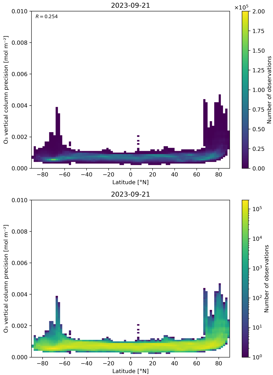
Figure 37: Scatter density plot of “Latitude” against “O 3 vertical column precision” for 2023-09-20 to 2023-09-22.
