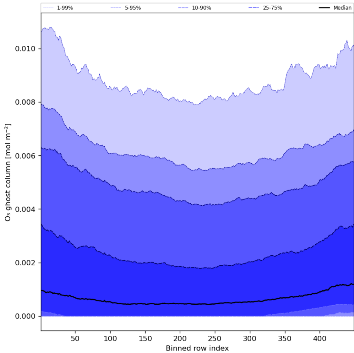
Figure 32: Along track statistics of “O 3 ghost column” for 2023-09-20 to 2023-09-22
