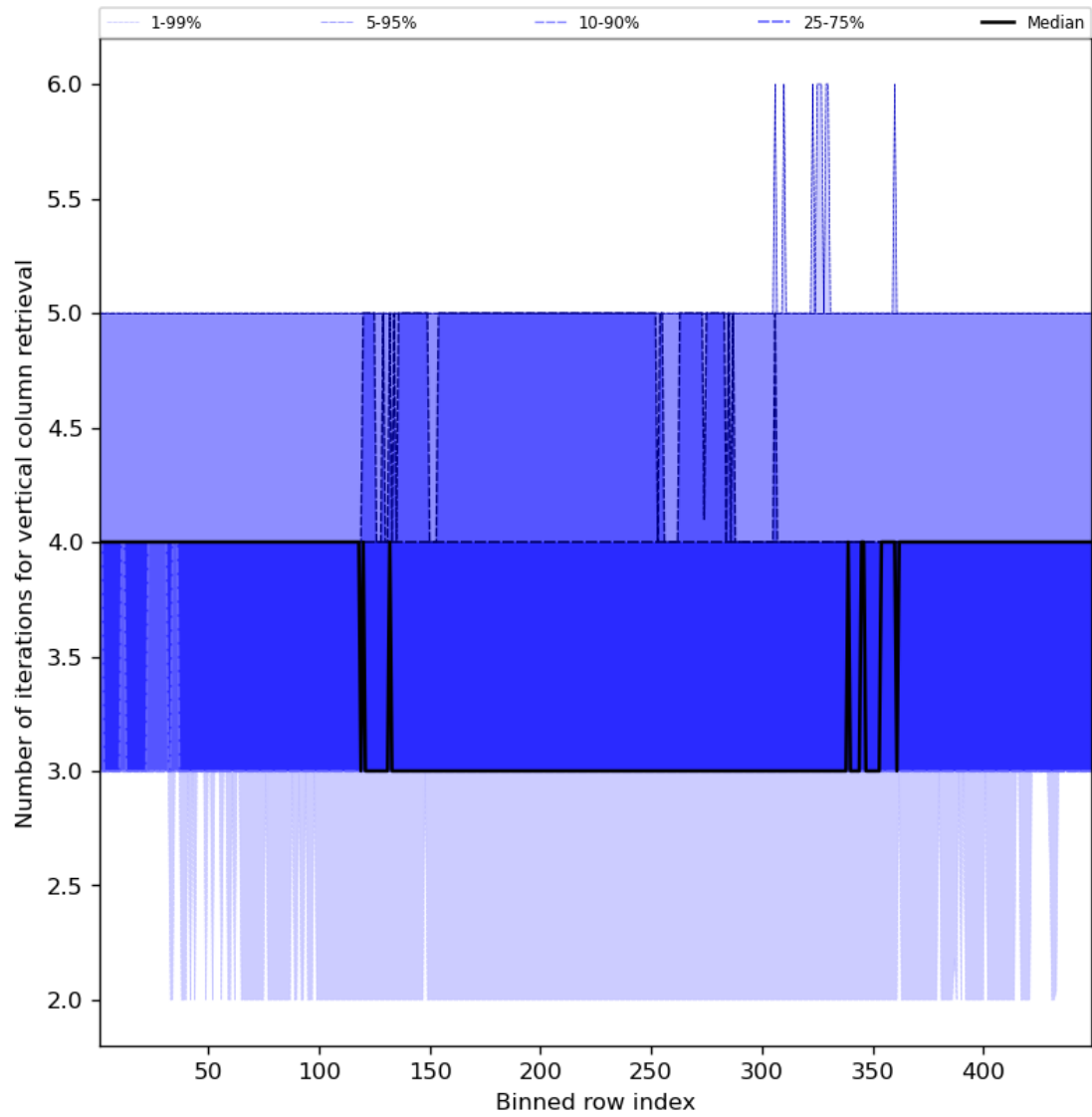
Figure 33: Along track statistics of “Number of iterations for vertical column retrieval” for 2023-09-20 to 2023-09-22
