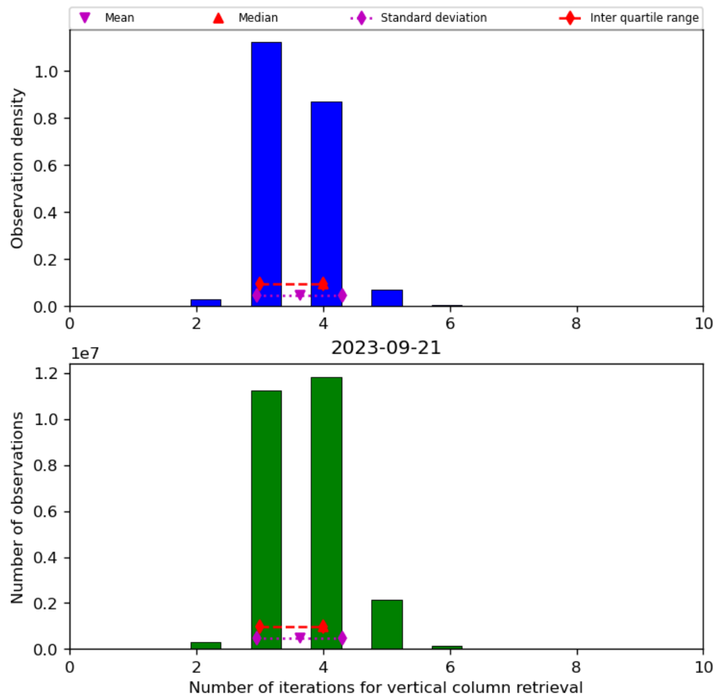
Figure 26: Histogram of “Number of iterations for vertical column retrieval” for 2023-09-20 to 2023-09-22
