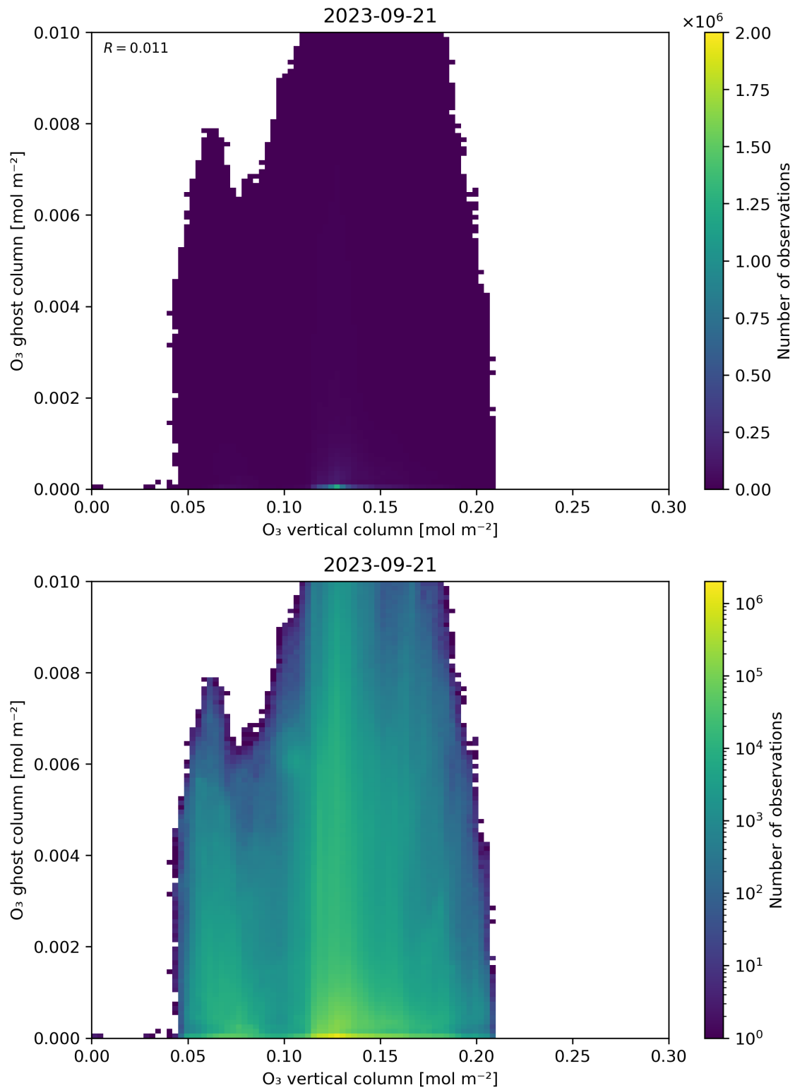
Figure 40: Scatter density plot of “O 3 vertical column” against “O 3 ghost column” for 2023-09-20 to 2023-09-22.
