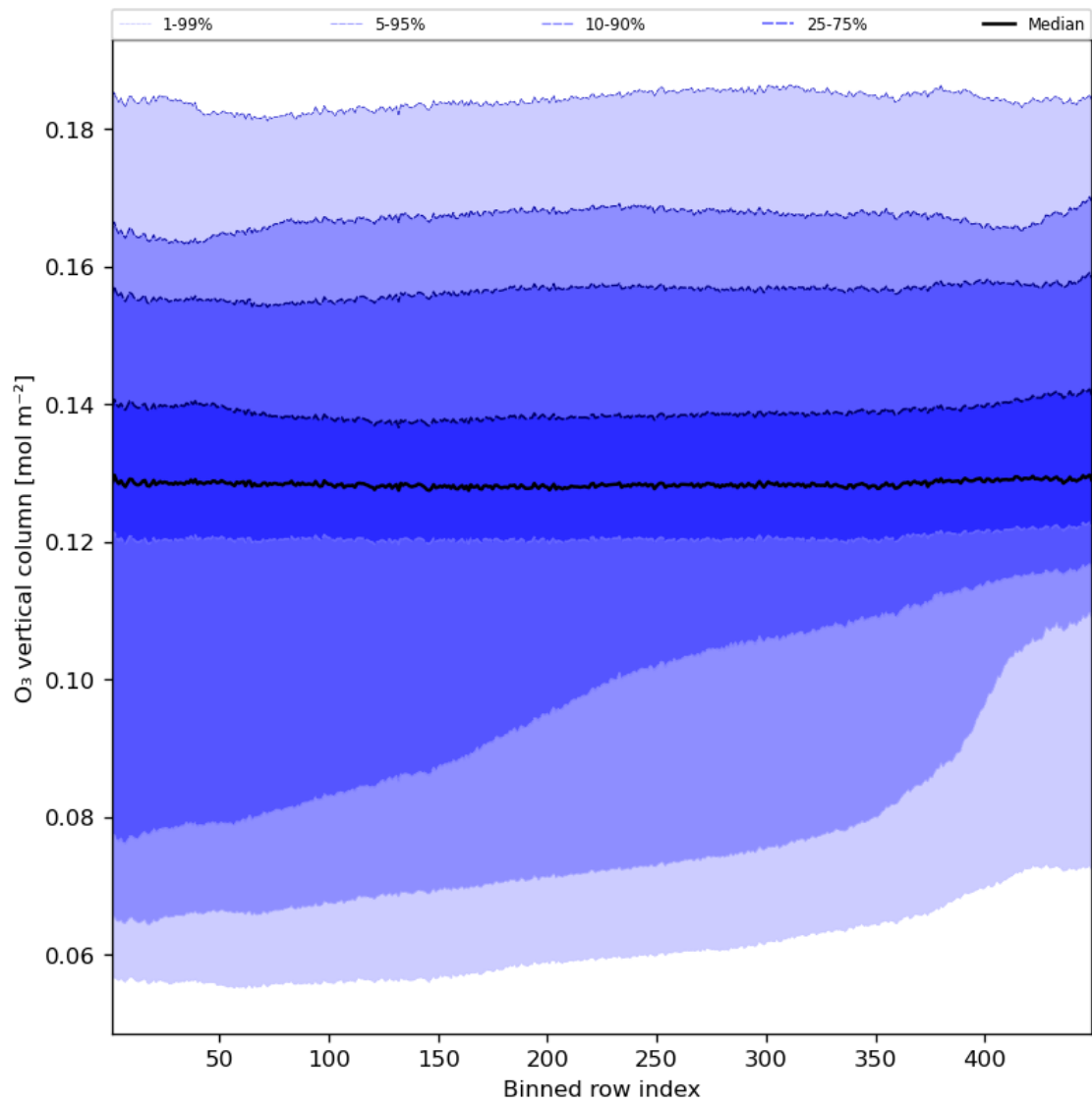
Figure 28: Along track statistics of “O 3 vertical column” for 2023-09-20 to 2023-09-22
