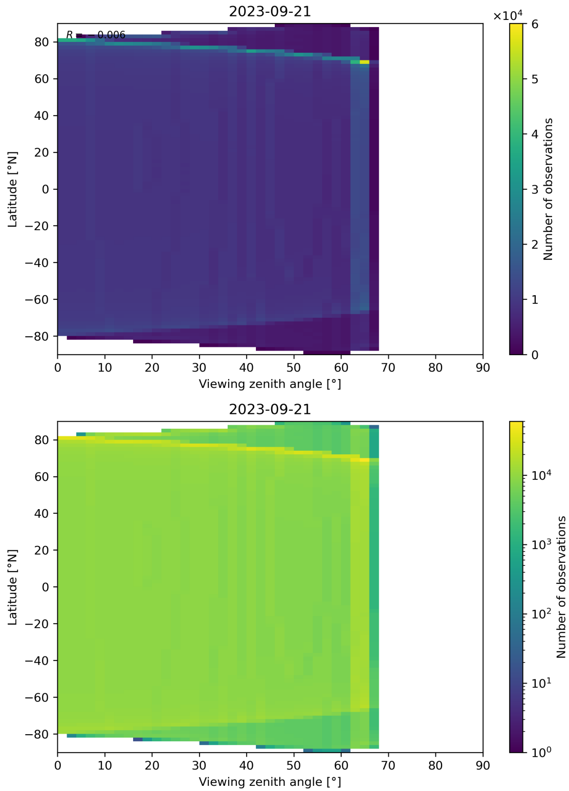
Figure 49: Scatter density plot of “Viewing zenith angle” against “Latitude” for 2023-09-20 to 2023-09-22.
