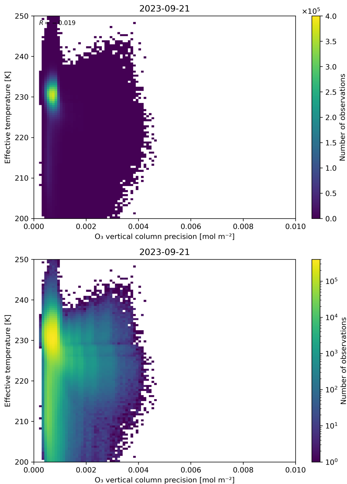
Figure 42: Scatter density plot of “O 3 vertical column precision” against “Effective temperature” for 2023-09-20 to 2023-09-22.
