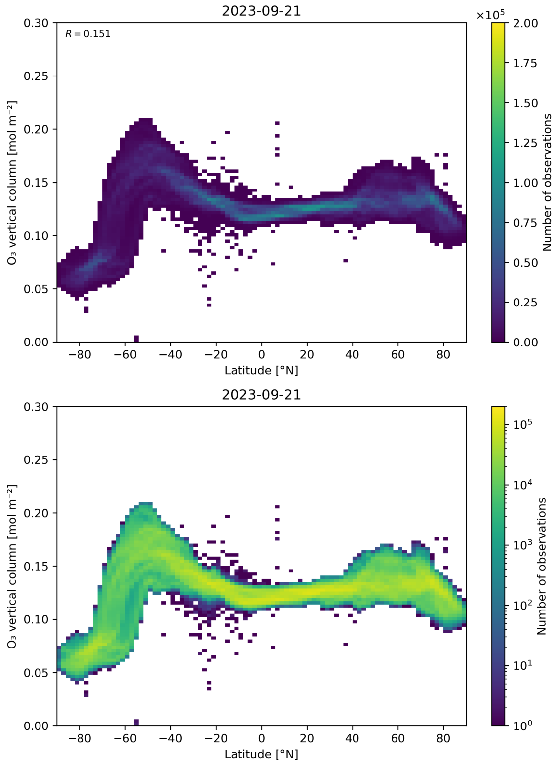
Figure 36: Scatter density plot of “Latitude” against “O 3 vertical column” for 2023-09-20 to 2023-09-22.
