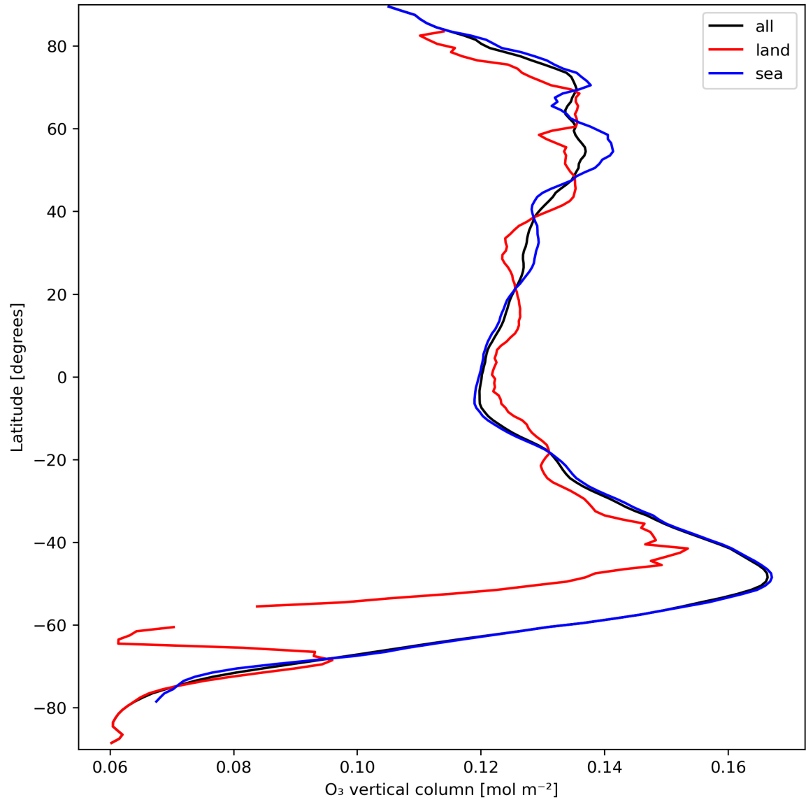
Figure 14: Zonal average of “O 3 vertical column” for 2023-09-20 to 2023-09-22.
