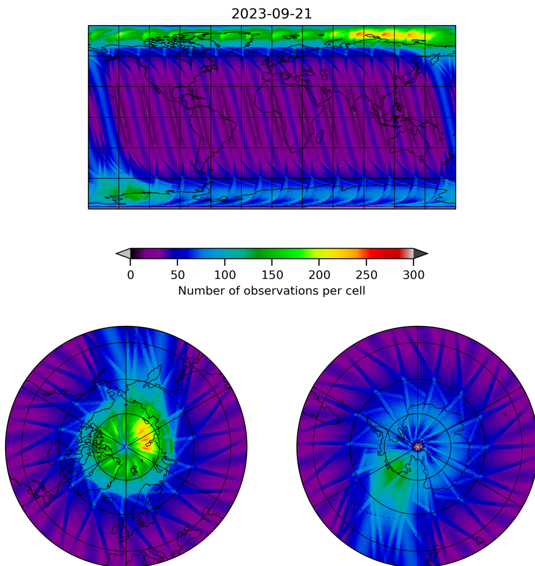
Figure 12: Map of the number of observations for 2023-09-20 to 2023-09-22
