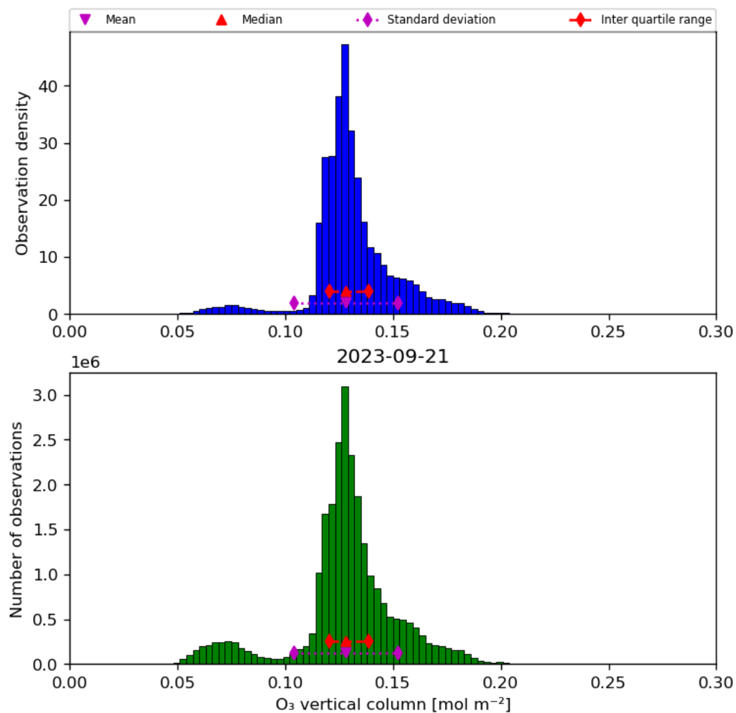
Figure 21: Histogram of “O 3 vertical column” for 2023-09-20 to 2023-09-22
