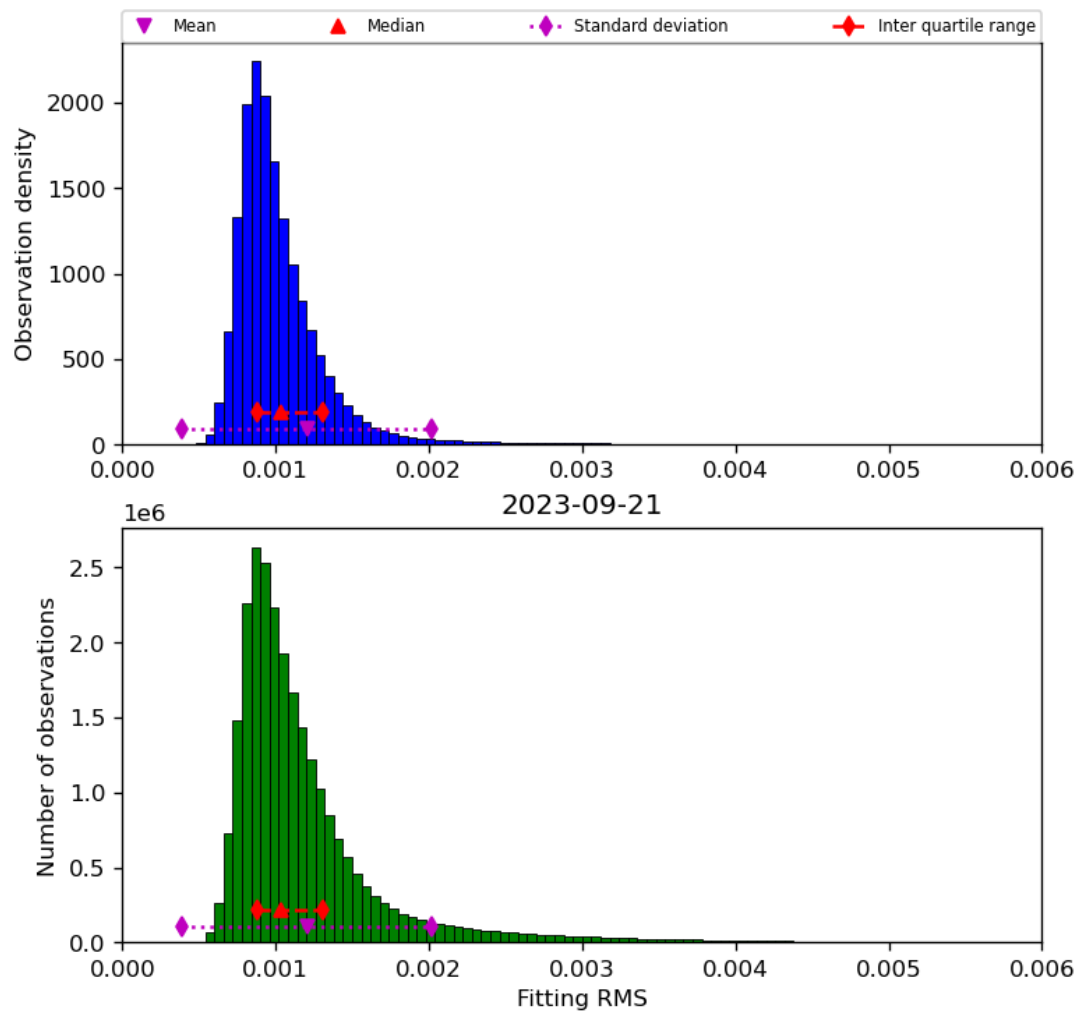
Figure 23: Histogram of “Fitting RMS” for 2023-09-20 to 2023-09-22
