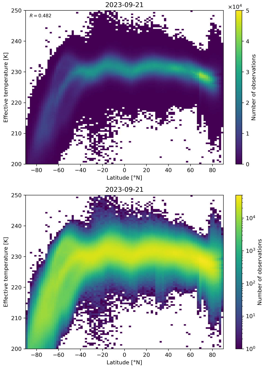
Figure 34: Scatter density plot of “Latitude” against “Effective temperature” for 2023-09-20 to 2023-09-22.
