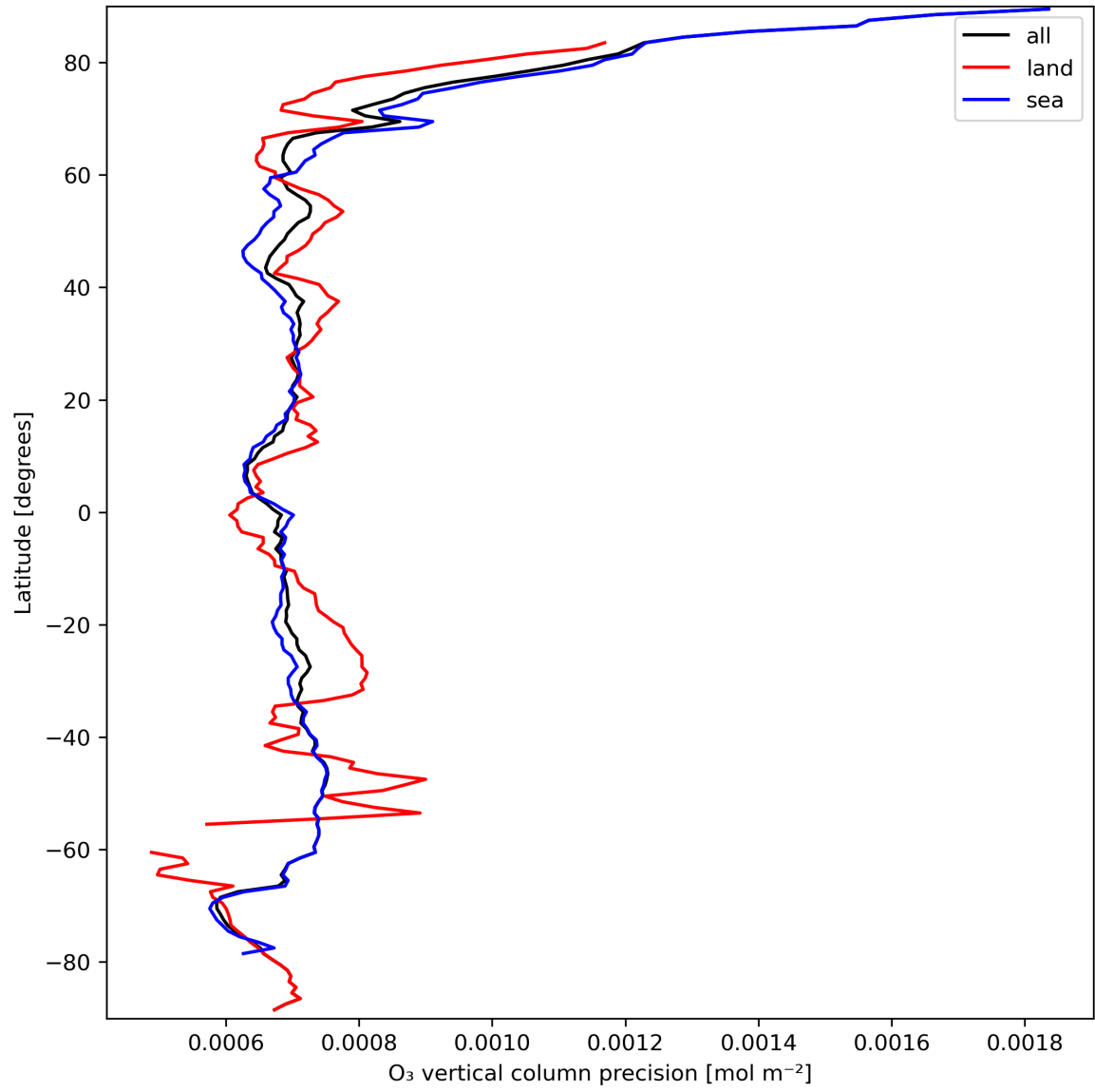
Figure 15: Zonal average of “O 3 vertical column precision” for 2023-09-20 to 2023-09-22.
