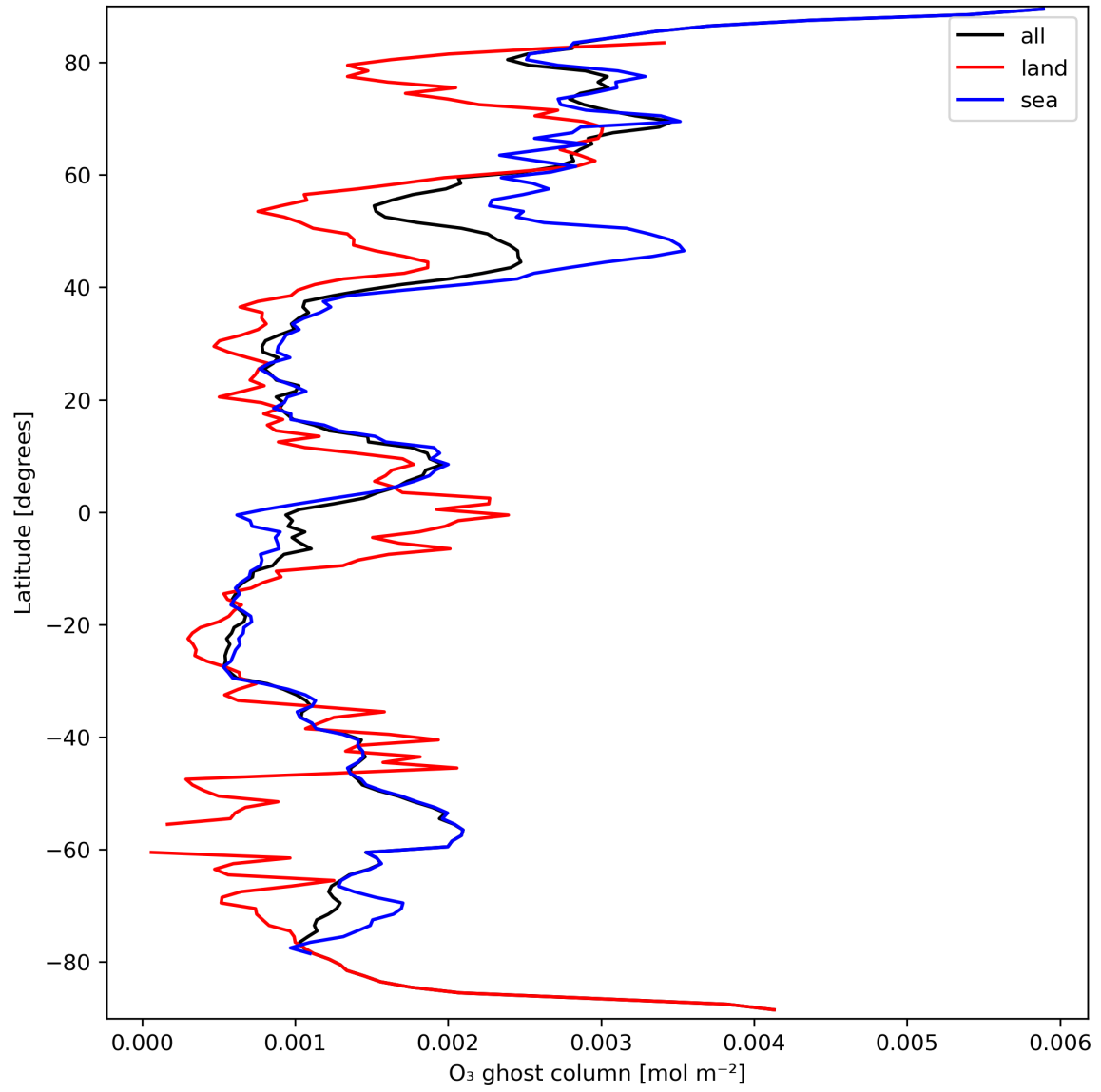
Figure 18: Zonal average of "O 3 ghost column" for 2023-09-20 to 2023-09-22.
