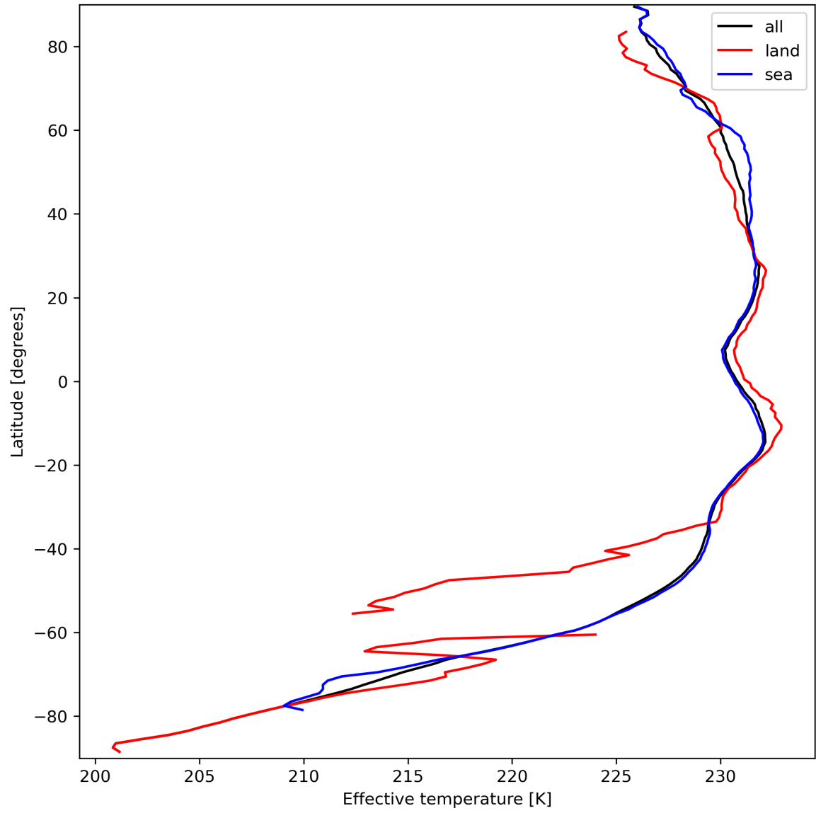
Figure 17: Zonal average of “Effective temperature” for 2023-09-20 to 2023-09-22.
