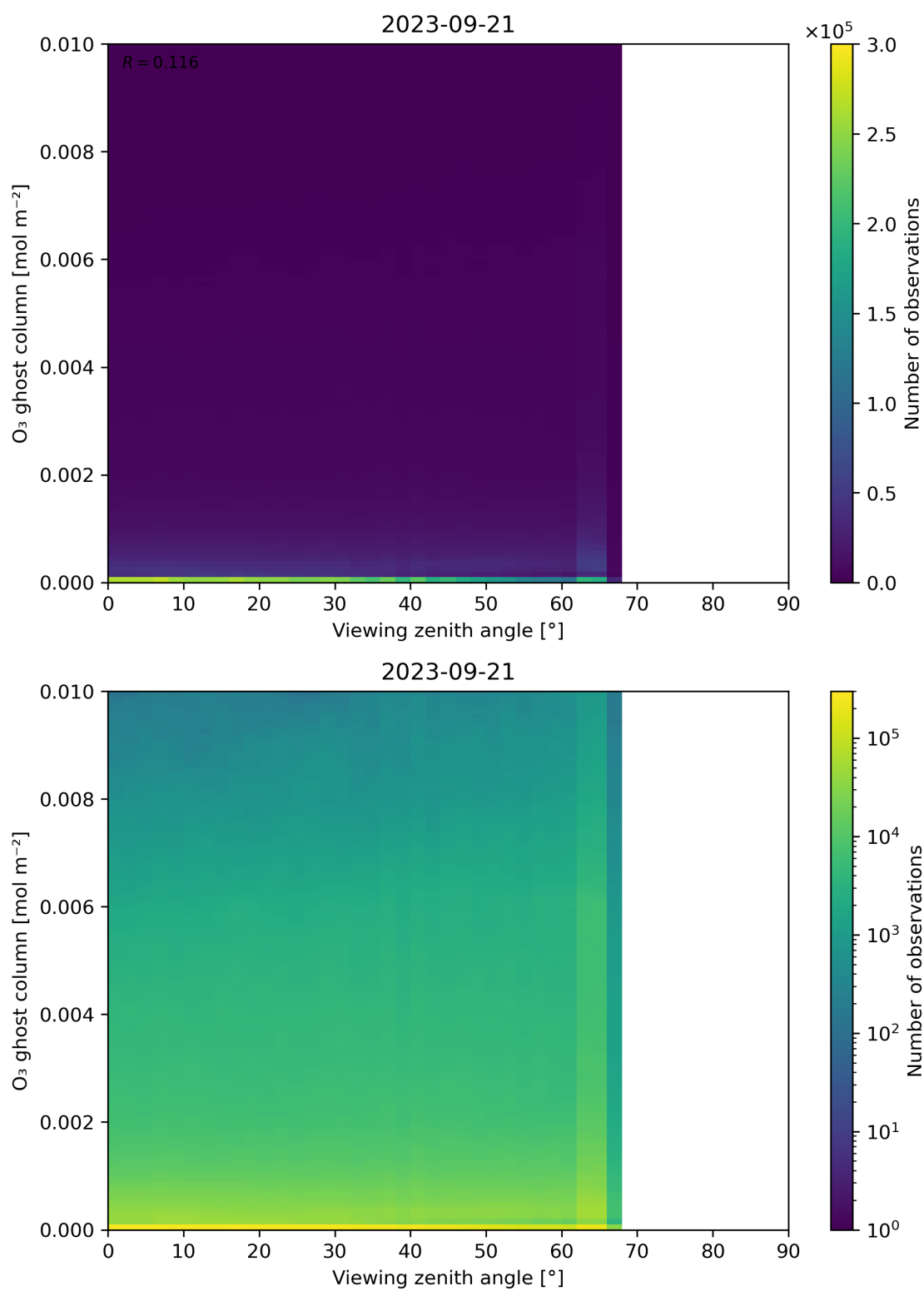
Figure 51: Scatter density plot of “Viewing zenith angle” against “O 3 ghost column” for 2023-09-20 to 2023-09-22.
