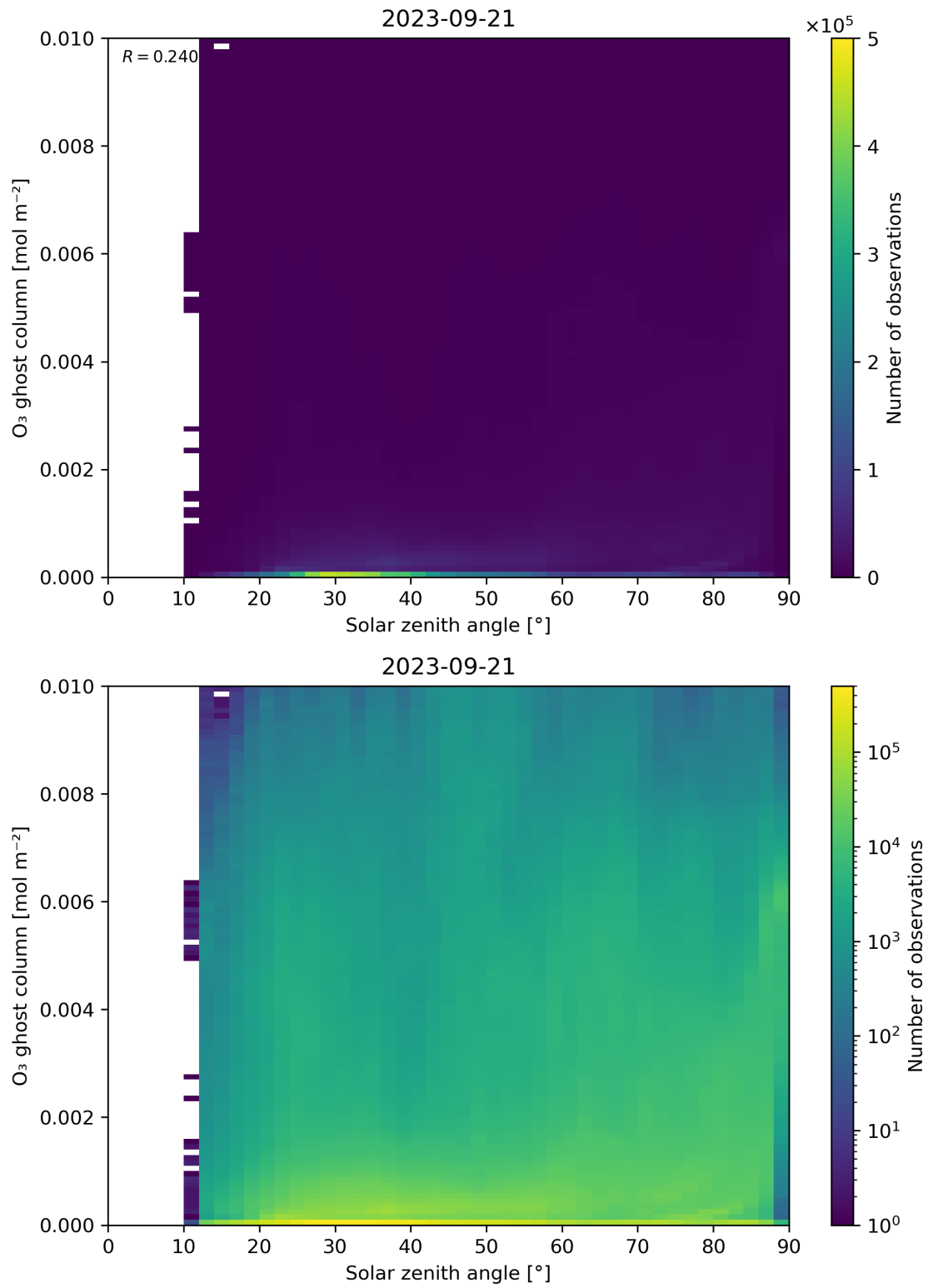
Figure 46: Scatter density plot of “Solar zenith angle” against “O 3 ghost column” for 2023-09-20 to 2023-09-22.
