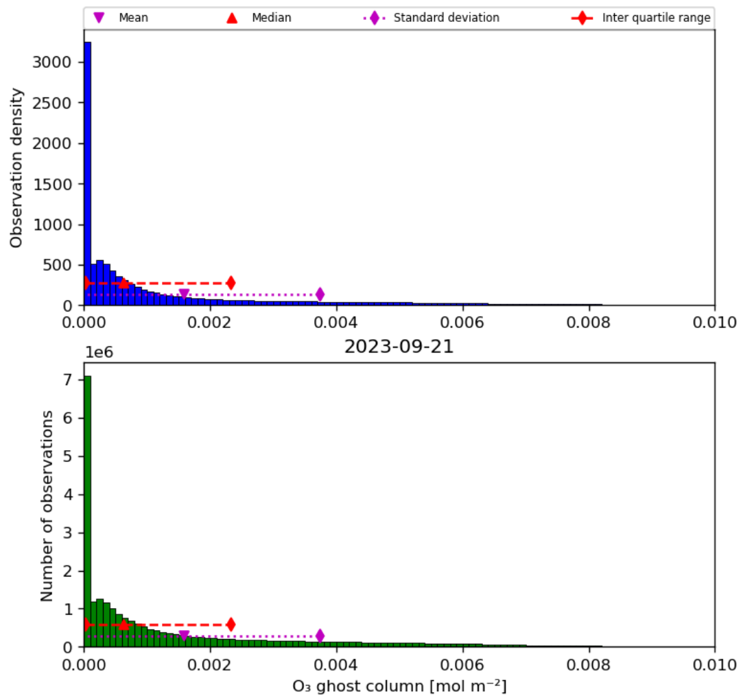
Figure 25: Histogram of “O 3 ghost column” for 2023-09-20 to 2023-09-22
