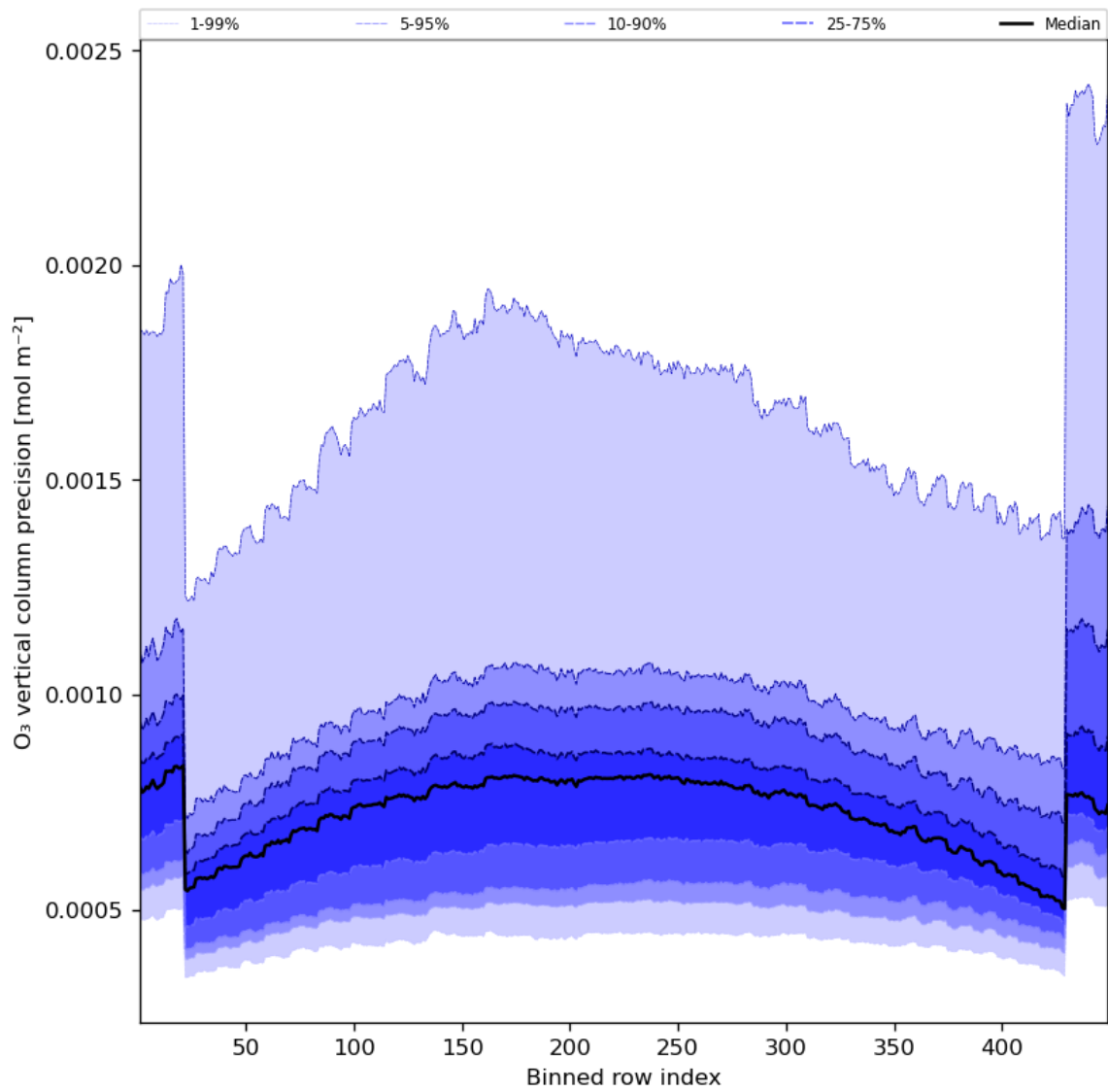
Figure 29: Along track statistics of “O 3 vertical column precision” for 2023-09-20 to 2023-09-22
