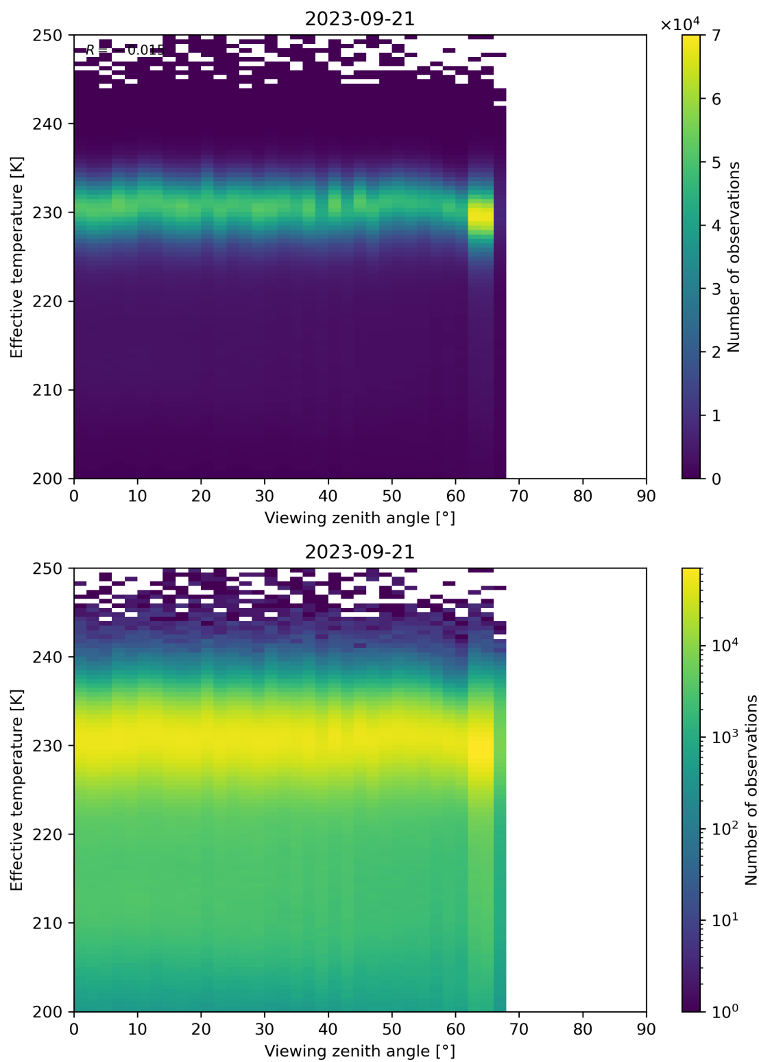
Figure 50: Scatter density plot of “Viewing zenith angle” against “Effective temperature” for 2023-09-20 to 2023-09-22.
