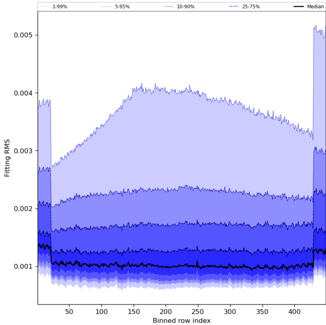
Figure 30: Along track statistics of “Fitting RMS” for 2023-09-20 to 2023-09-22
