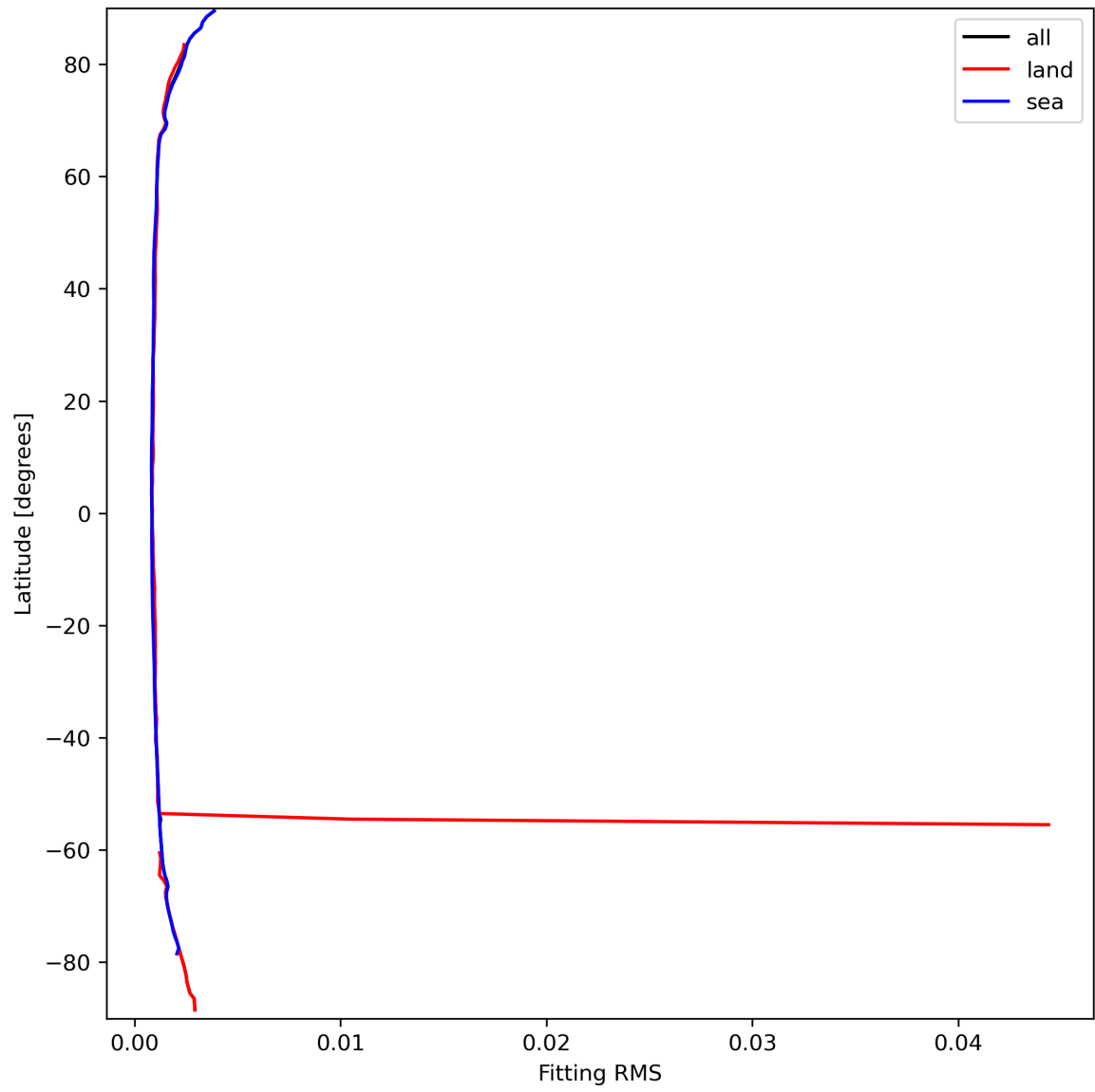
Figure 16: Zonal average of “Fitting RMS” for 2023-09-20 to 2023-09-22.
