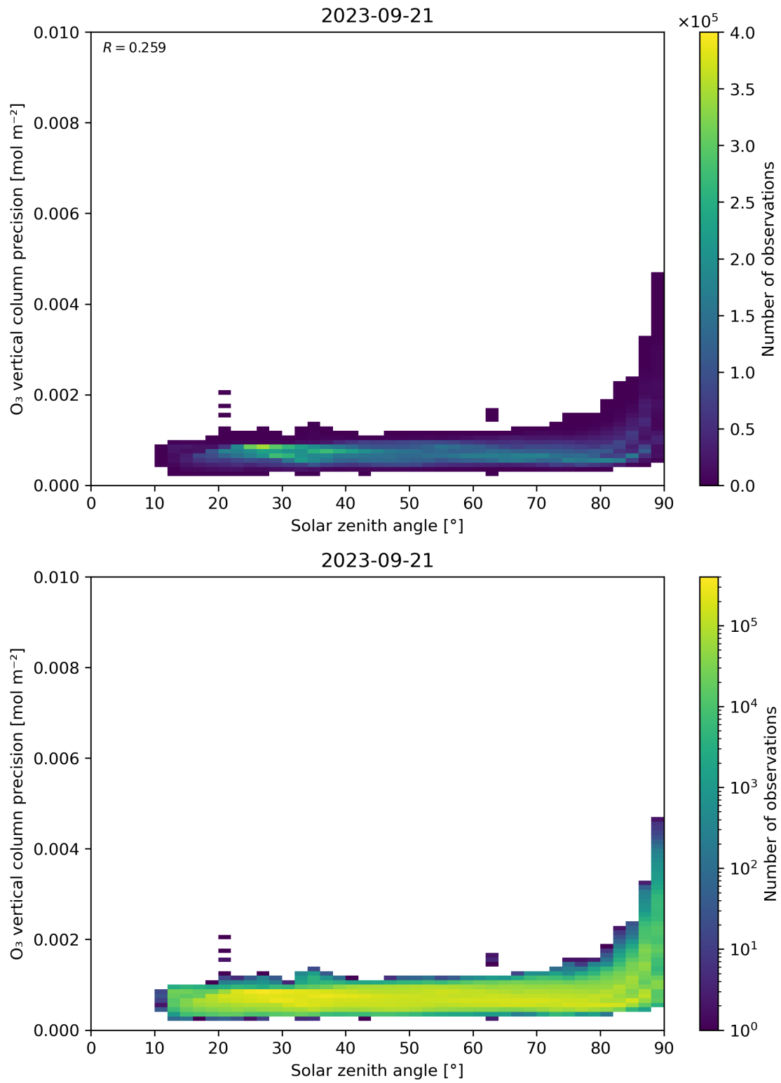
Figure 48: Scatter density plot of “Solar zenith angle” against “O 3 vertical column precision” for 2023-09-20 to 2023-09-22.
