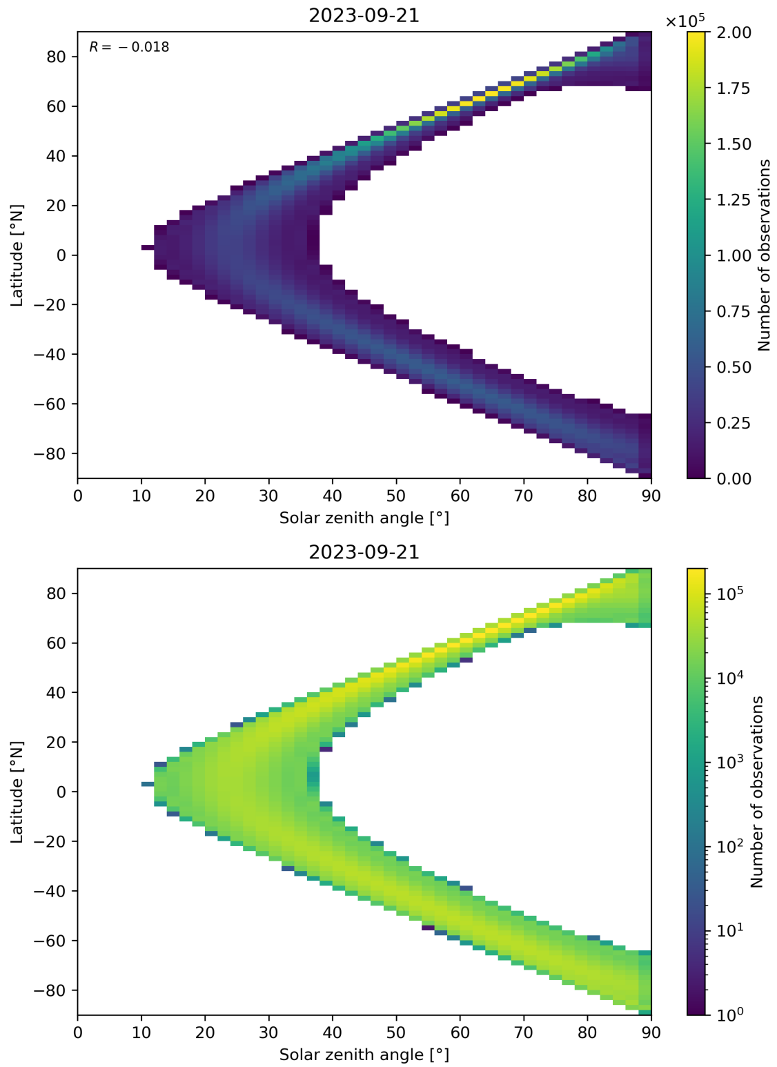
Figure 44: Scatter density plot of “Solar zenith angle” against “Latitude” for 2023-09-20 to 2023-09-22.
