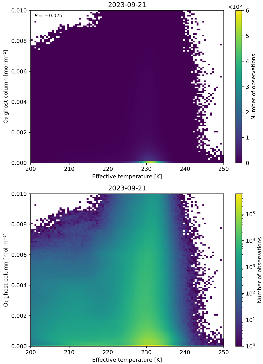
Figure 38: Scatter density plot of “Effective temperature” against “O 3 ghost column” for 2023-09-20 to 2023-09-22.
