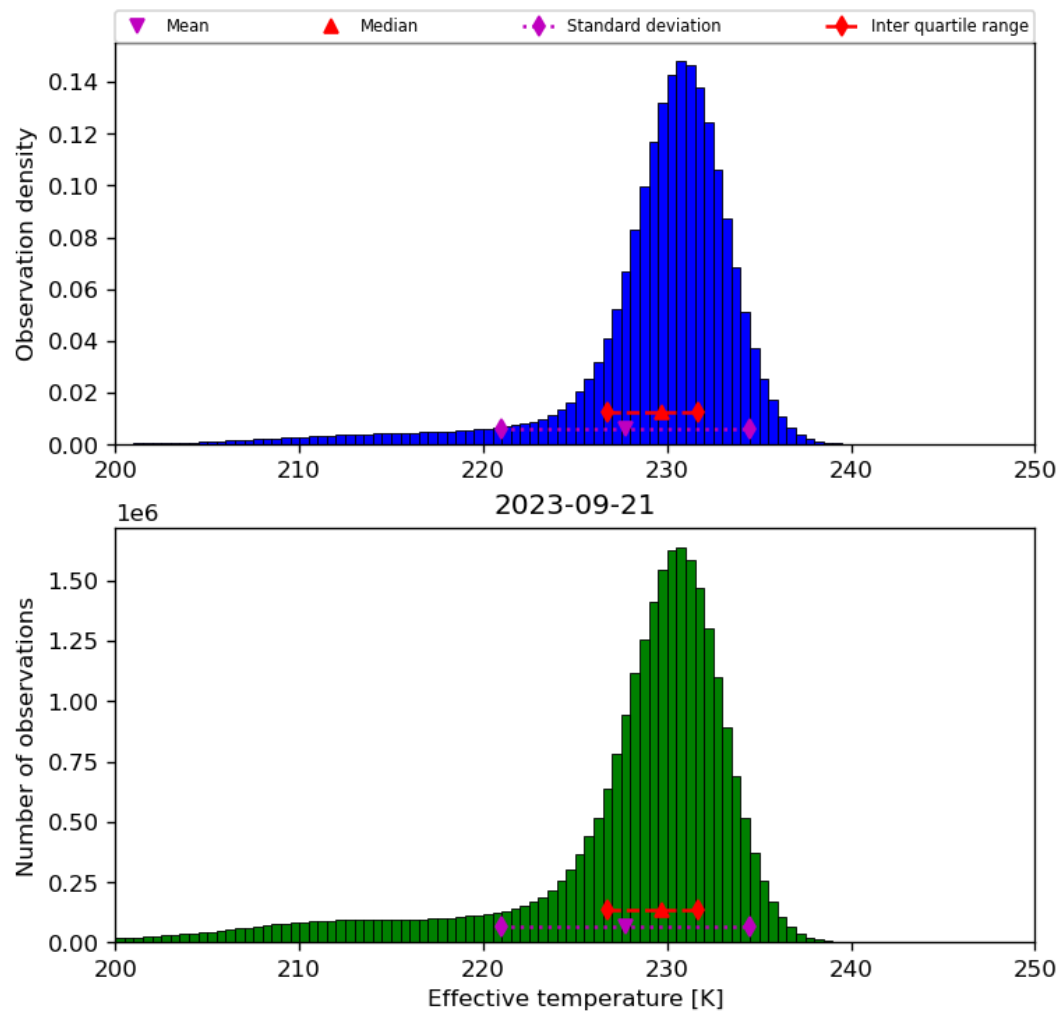
Figure 24: Histogram of “Effective temperature” for 2023-09-20 to 2023-09-22
