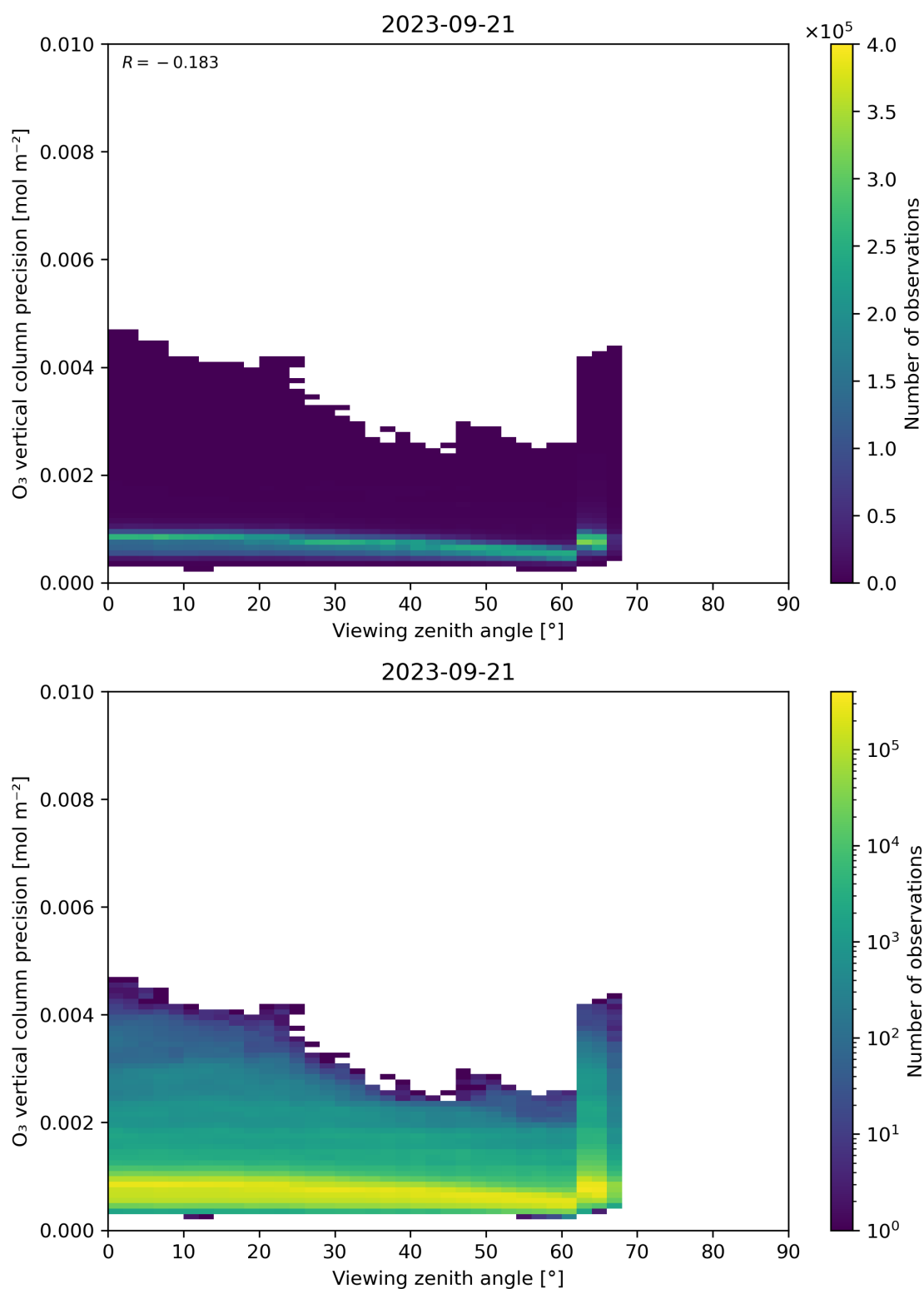
Figure 53: Scatter density plot of “Viewing zenith angle” against “O 3 vertical column precision” for 2023-09-20 to 2023-09-22.
