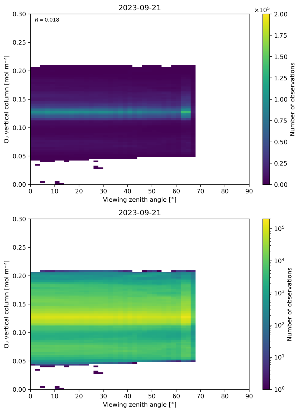
Figure 52: Scatter density plot of “Viewing zenith angle” against “O 3 vertical column” for 2023-09-20 to 2023-09-22.
