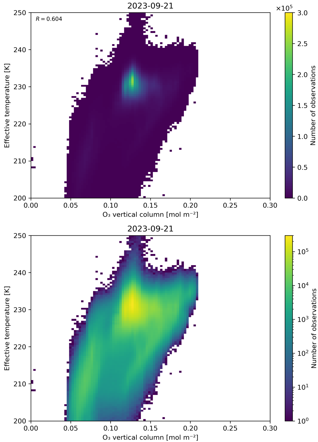
Figure 39: Scatter density plot of “O 3 vertical column” against “Effective temperature” for 2023-09-20 to 2023-09-22.
