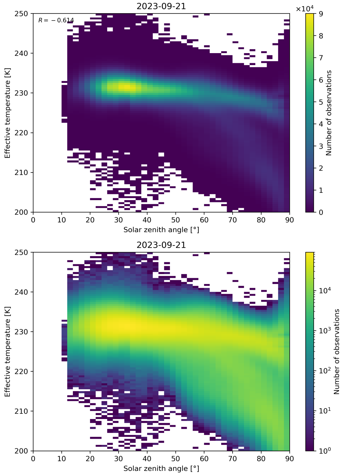
Figure 45: Scatter density plot of “Solar zenith angle” against “Effective temperature” for 2023-09-20 to 2023-09-22.
