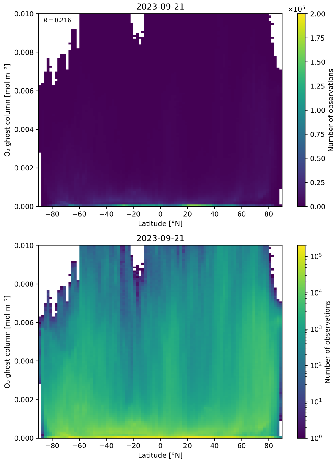
Figure 35: Scatter density plot of “Latitude” against “O 3 ghost column” for 2023-09-20 to 2023-09-22.
