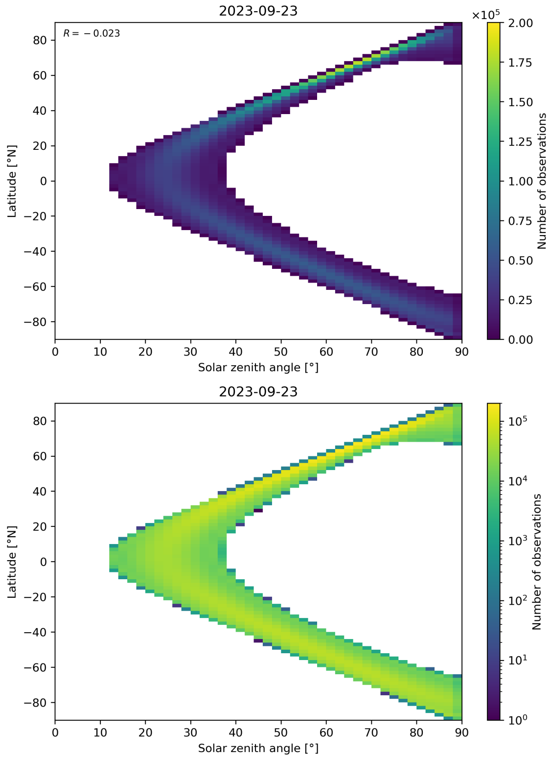
Figure 44: Scatter density plot of “Solar zenith angle” against “Latitude” for 2023-09-22 to 2023-09-24.
