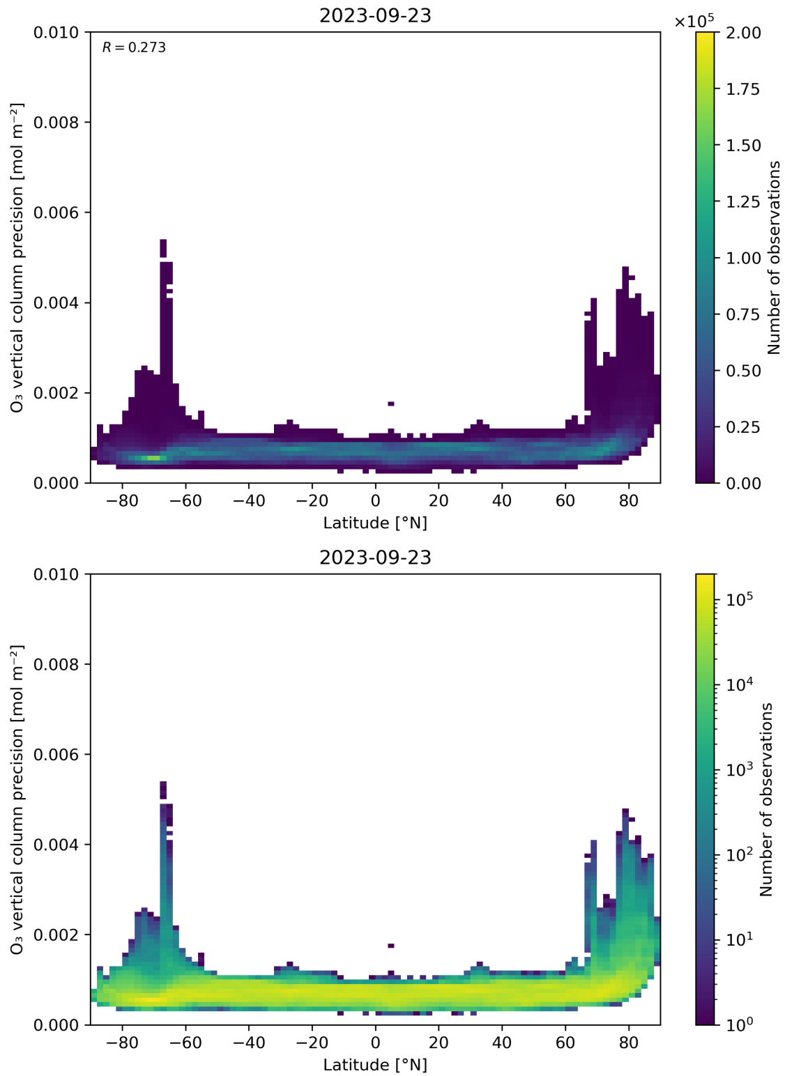
Figure 37: Scatter density plot of “Latitude” against “O 3 vertical column precision” for 2023-09-22 to 2023-09-24.
