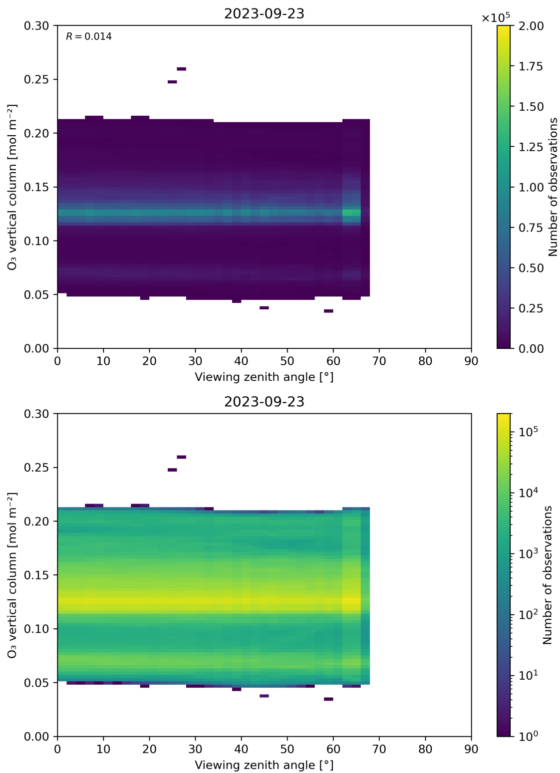
Figure 52: Scatter density plot of “Viewing zenith angle” against “O 3 vertical column” for 2023-09-22 to 2023-09-24.
