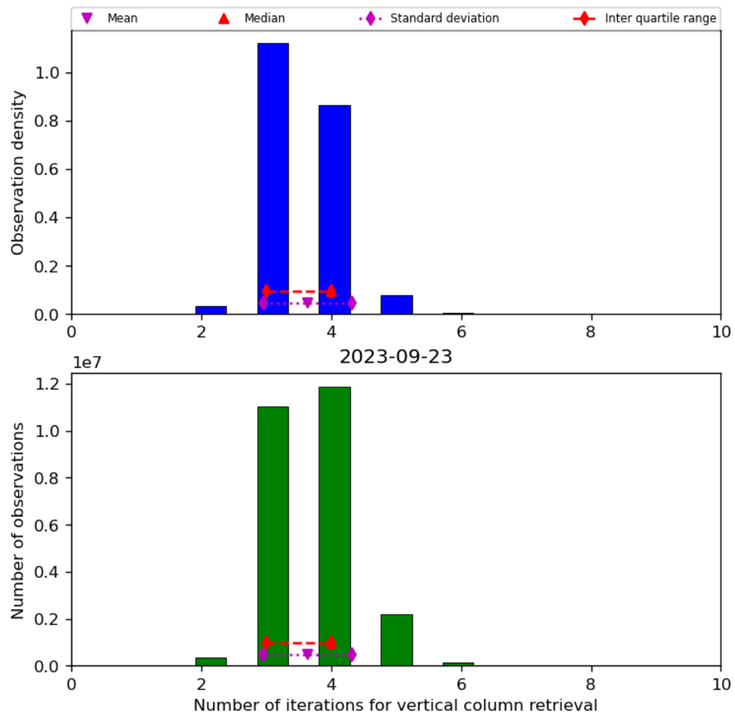
Figure 26: Histogram of “Number of iterations for vertical column retrieval” for 2023-09-22 to 2023-09-24
