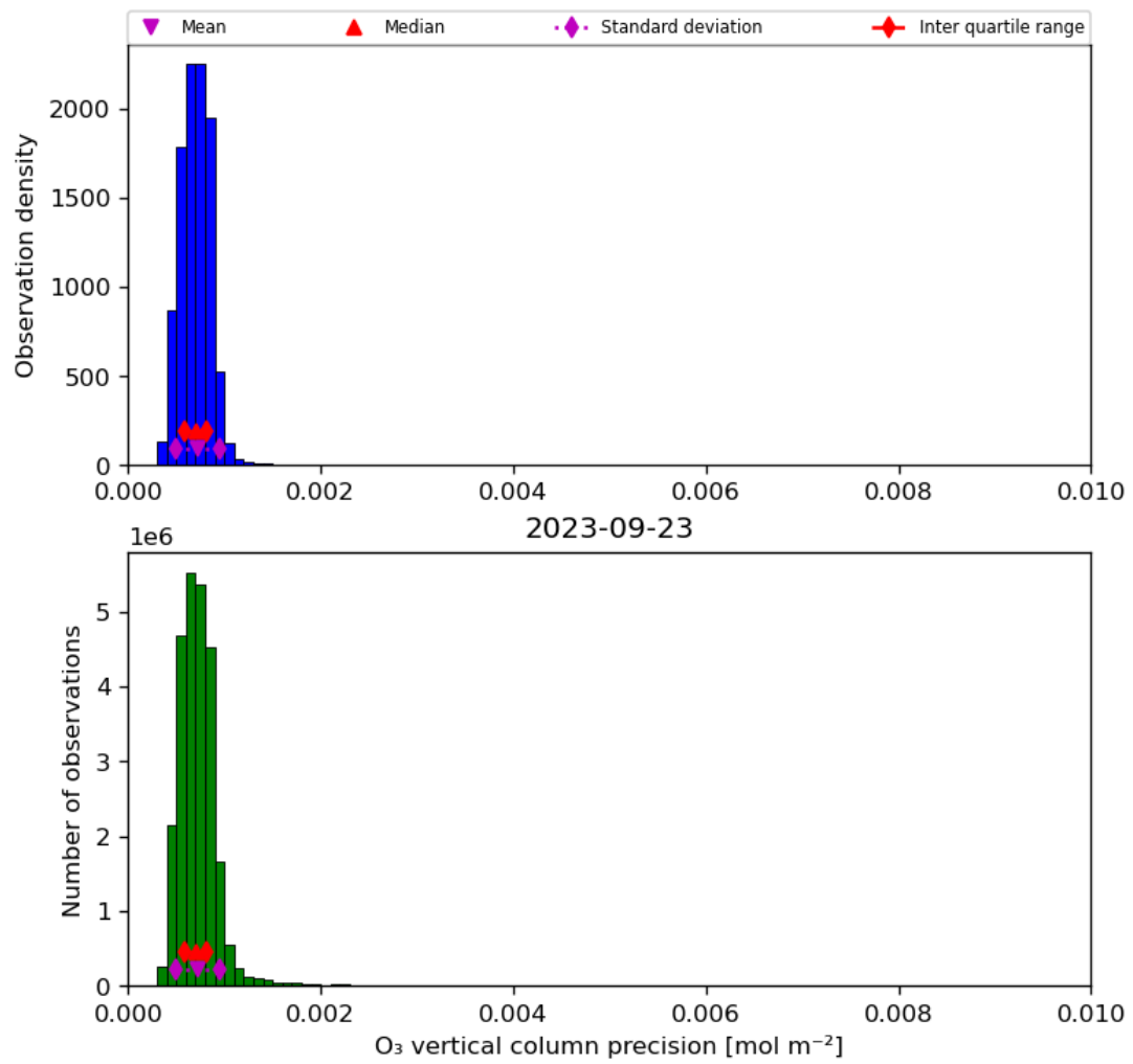
Figure 22: Histogram of “O 3 vertical column precision” for 2023-09-22 to 2023-09-24
