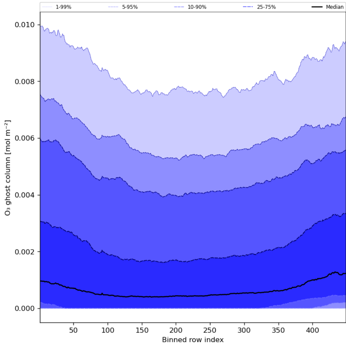
Figure 32: Along track statistics of “O 3 ghost column” for 2023-09-22 to 2023-09-24
