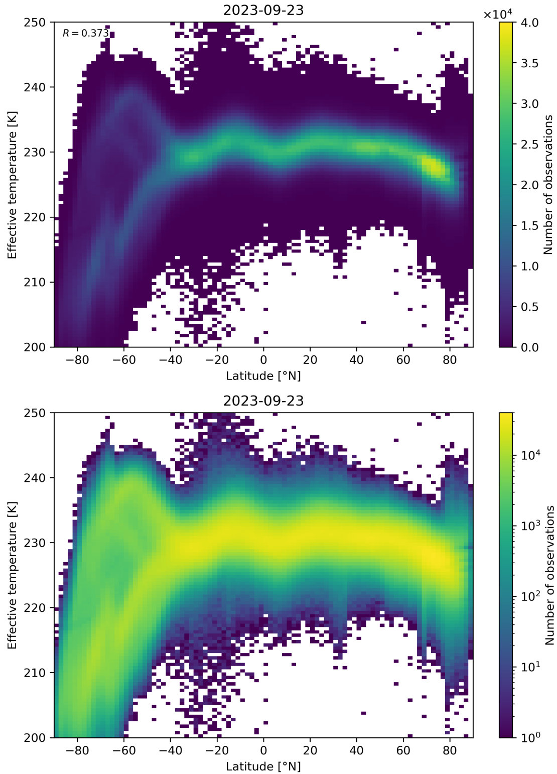
Figure 34: Scatter density plot of “Latitude” against “Effective temperature” for 2023-09-22 to 2023-09-24.
