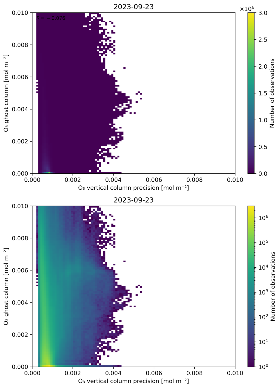
Figure 43: Scatter density plot of “ \text{O}_3 vertical column precision” against “ \text{O}_3 ghost column” for 2023-09-22 to 2023-09-24.
