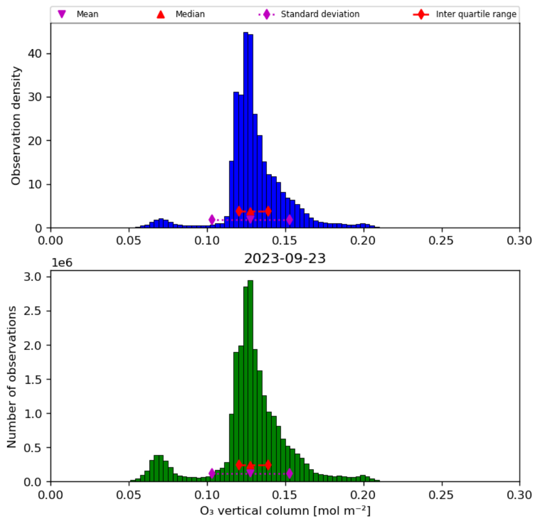
Figure 21: Histogram of “O 3 vertical column” for 2023-09-22 to 2023-09-24
