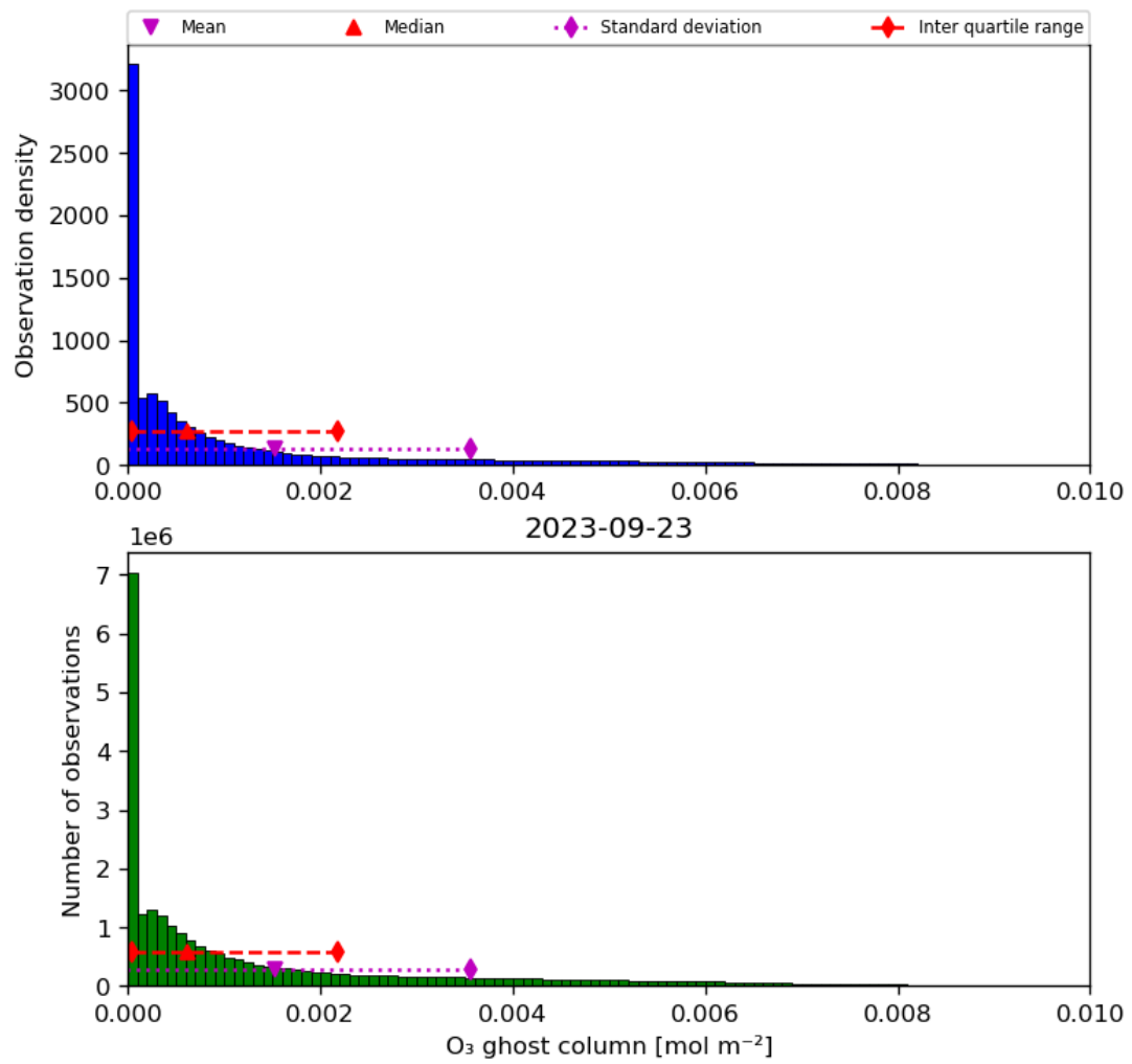
Figure 25: Histogram of “O 3 ghost column” for 2023-09-22 to 2023-09-24
