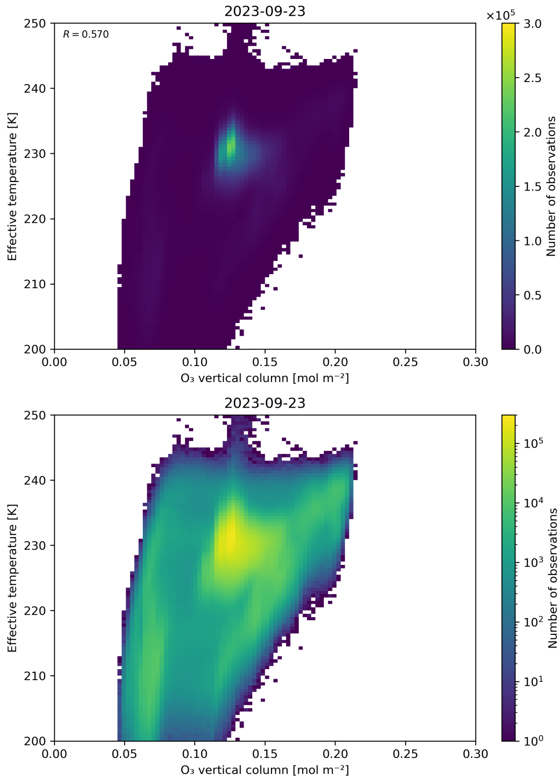
Figure 39: Scatter density plot of “O 3 vertical column” against “Effective temperature” for 2023-09-22 to 2023-09-24.
