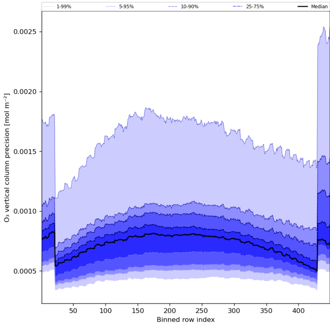
Figure 29: Along track statistics of “O 3 vertical column precision” for 2023-09-22 to 2023-09-24
