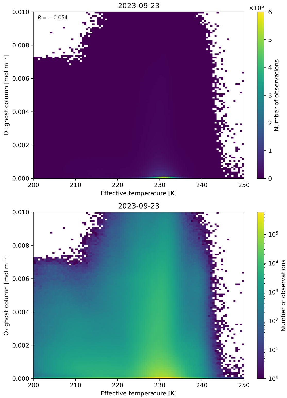
Figure 38: Scatter density plot of “Effective temperature” against “O 3 ghost column” for 2023-09-22 to 2023-09-24.
