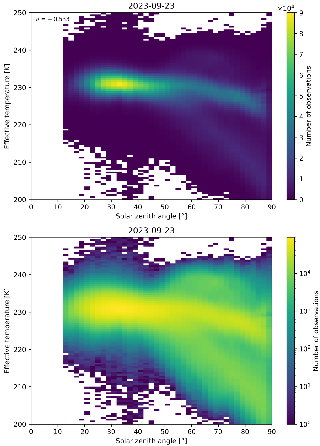
Figure 45: Scatter density plot of “Solar zenith angle” against “Effective temperature” for 2023-09-22 to 2023-09-24.
