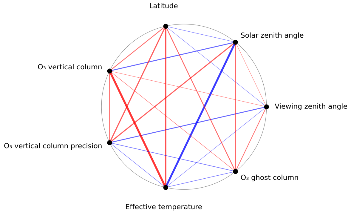
Figure 1: Map of correlation graph for 2023-09-22 to 2023-09-24.
