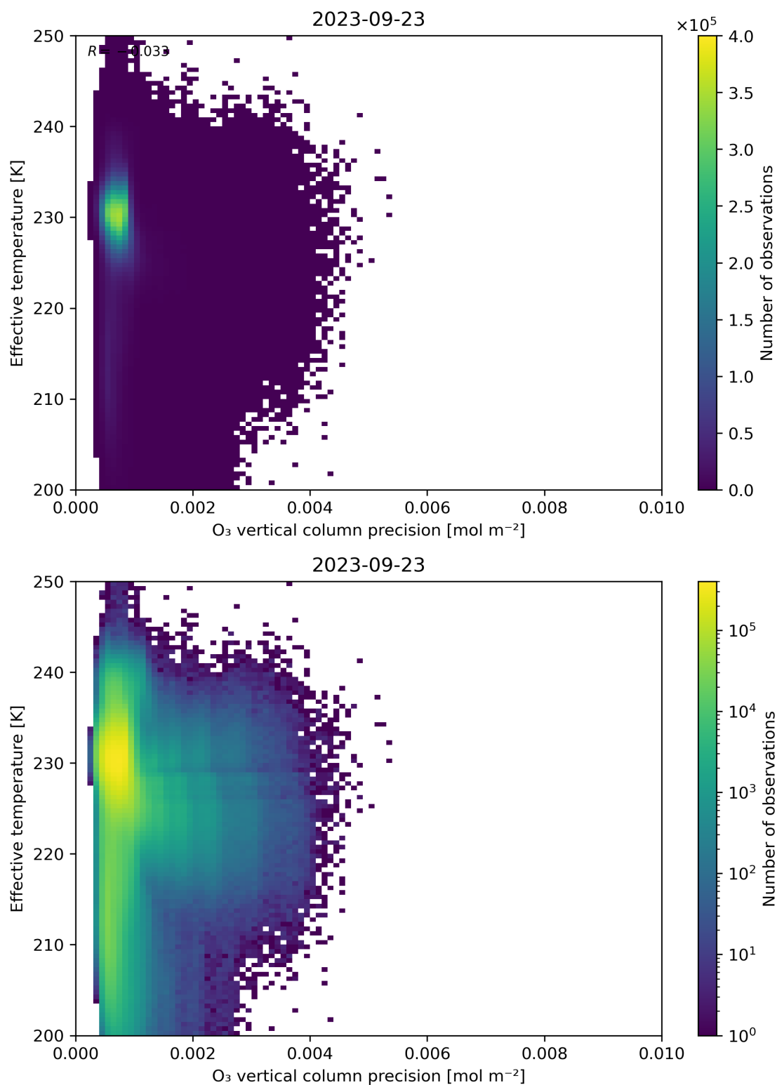
Figure 42: Scatter density plot of “O 3 vertical column precision” against “Effective temperature” for 2023-09-22 to 2023-09-24.
