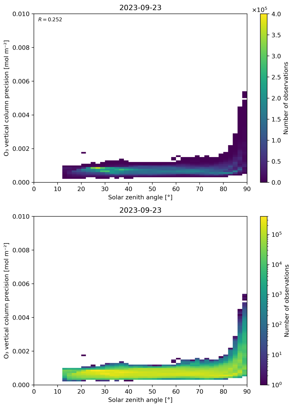
Figure 48: Scatter density plot of “Solar zenith angle” against “O 3 vertical column precision” for 2023-09-22 to 2023-09-24.
