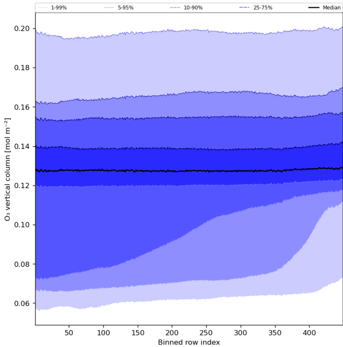
Figure 28: Along track statistics of “O 3 vertical column” for 2023-09-22 to 2023-09-24
