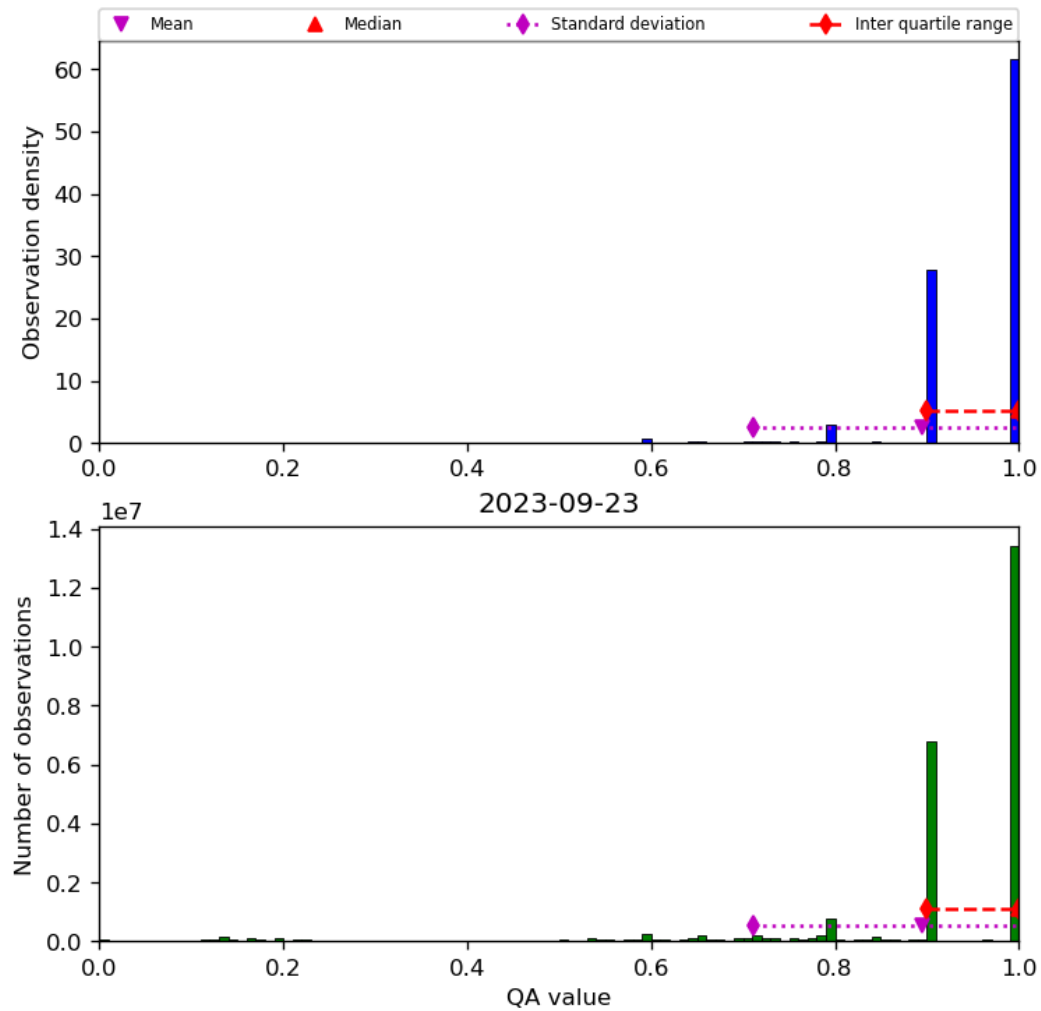
Figure 20: Histogram of “QA value” for 2023-09-22 to 2023-09-24
