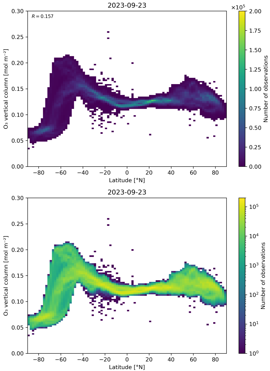
Figure 36: Scatter density plot of “Latitude” against “O 3 vertical column” for 2023-09-22 to 2023-09-24.
