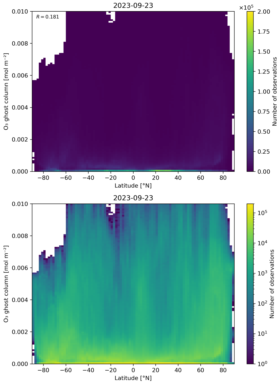
Figure 35: Scatter density plot of “Latitude” against “O 3 ghost column” for 2023-09-22 to 2023-09-24.
