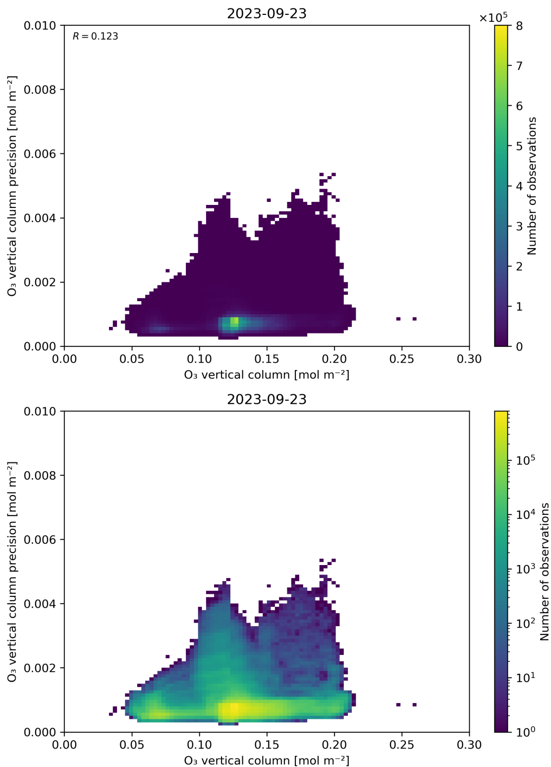
Figure 41: Scatter density plot of “O 3 vertical column” against “O 3 vertical column precision” for 2023-09-22 to 2023-09-24.
