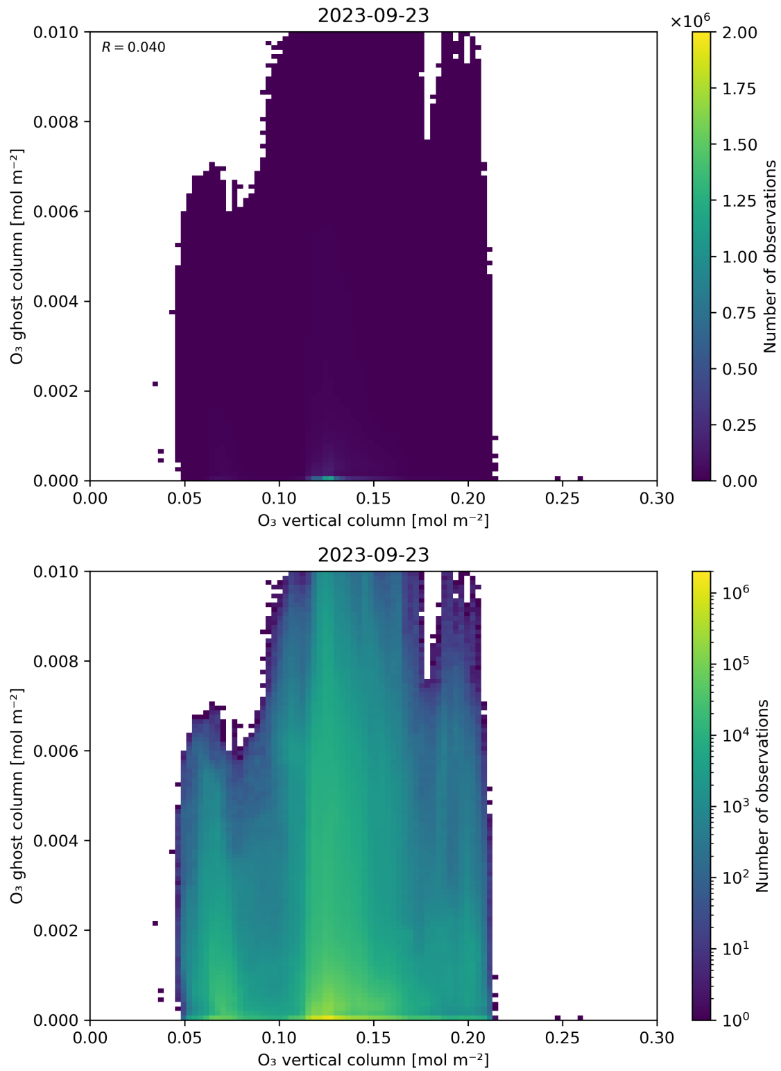
Figure 40: Scatter density plot of “O 3 vertical column” against “O 3 ghost column” for 2023-09-22 to 2023-09-24.
