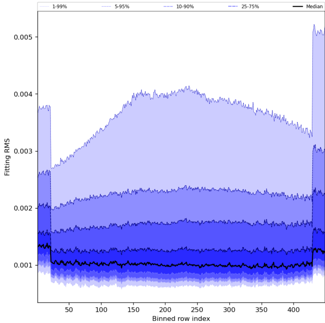
Figure 30: Along track statistics of “Fitting RMS” for 2023-09-22 to 2023-09-24
