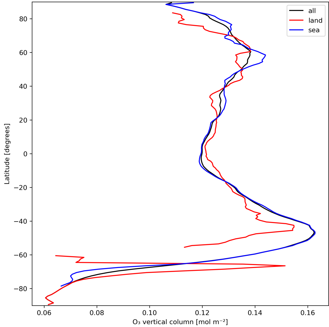
Figure 14: Zonal average of “O 3 vertical column” for 2023-09-22 to 2023-09-24.
