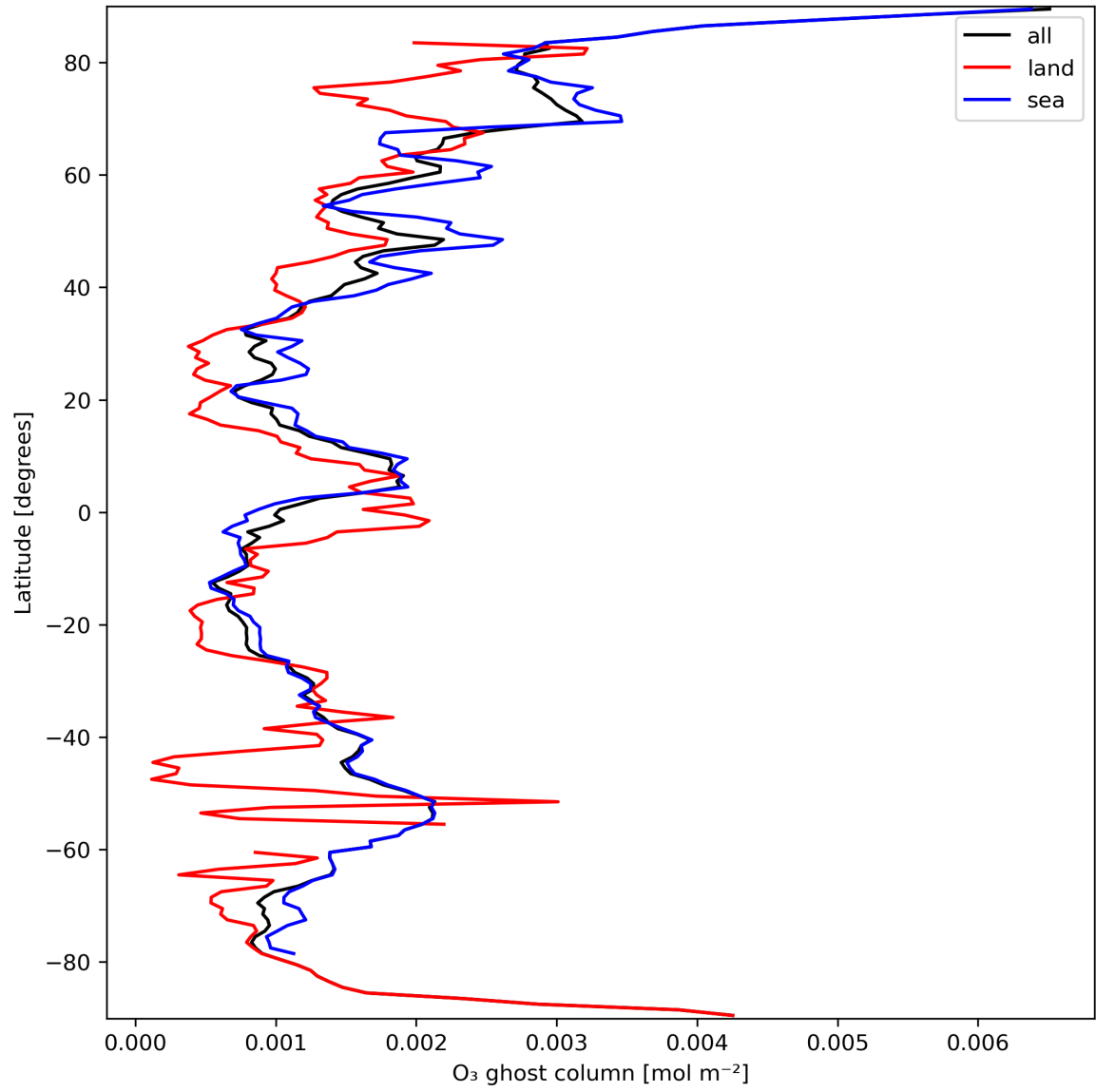
Figure 18: Zonal average of “O 3 ghost column” for 2023-09-22 to 2023-09-24.
