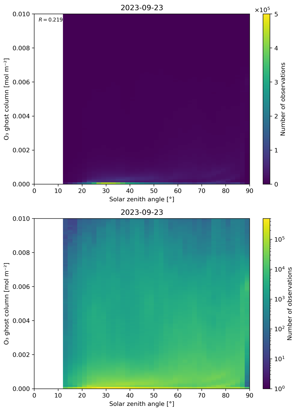
Figure 46: Scatter density plot of “Solar zenith angle” against “O 3 ghost column” for 2023-09-22 to 2023-09-24.
