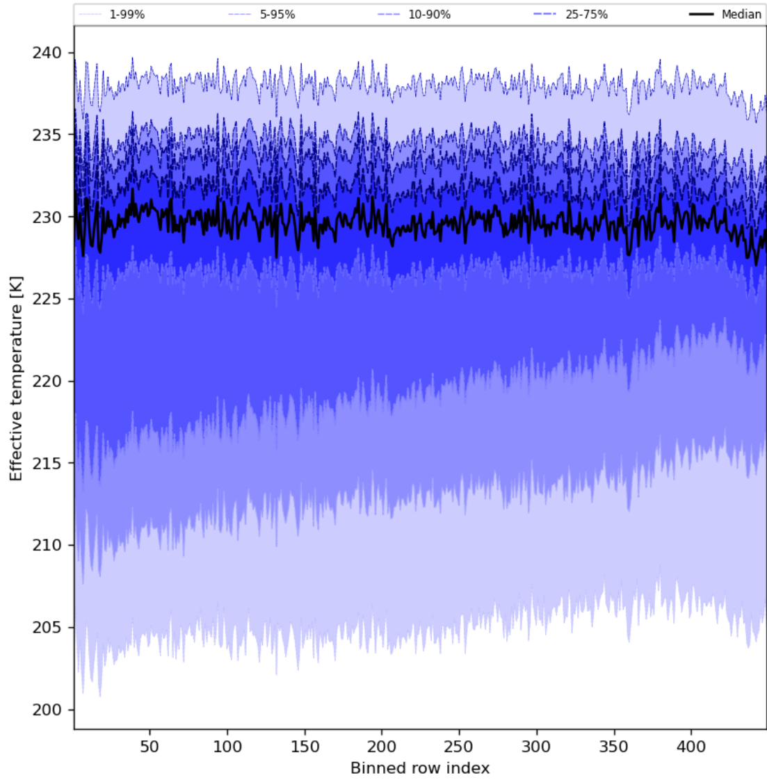
Figure 31: Along track statistics of “Effective temperature” for 2023-09-22 to 2023-09-24
