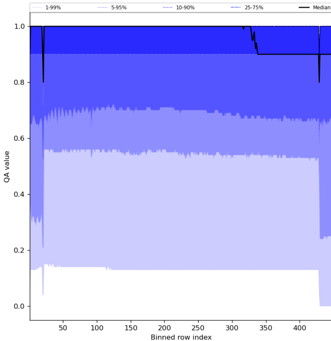
Figure 27: Along track statistics of “QA value” for 2023-09-22 to 2023-09-24
