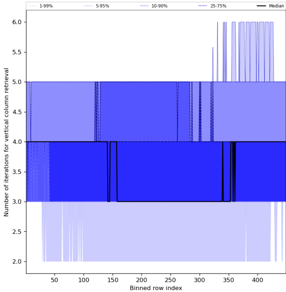
Figure 33: Along track statistics of “Number of iterations for vertical column retrieval” for 2023-09-22 to 2023-09-24
