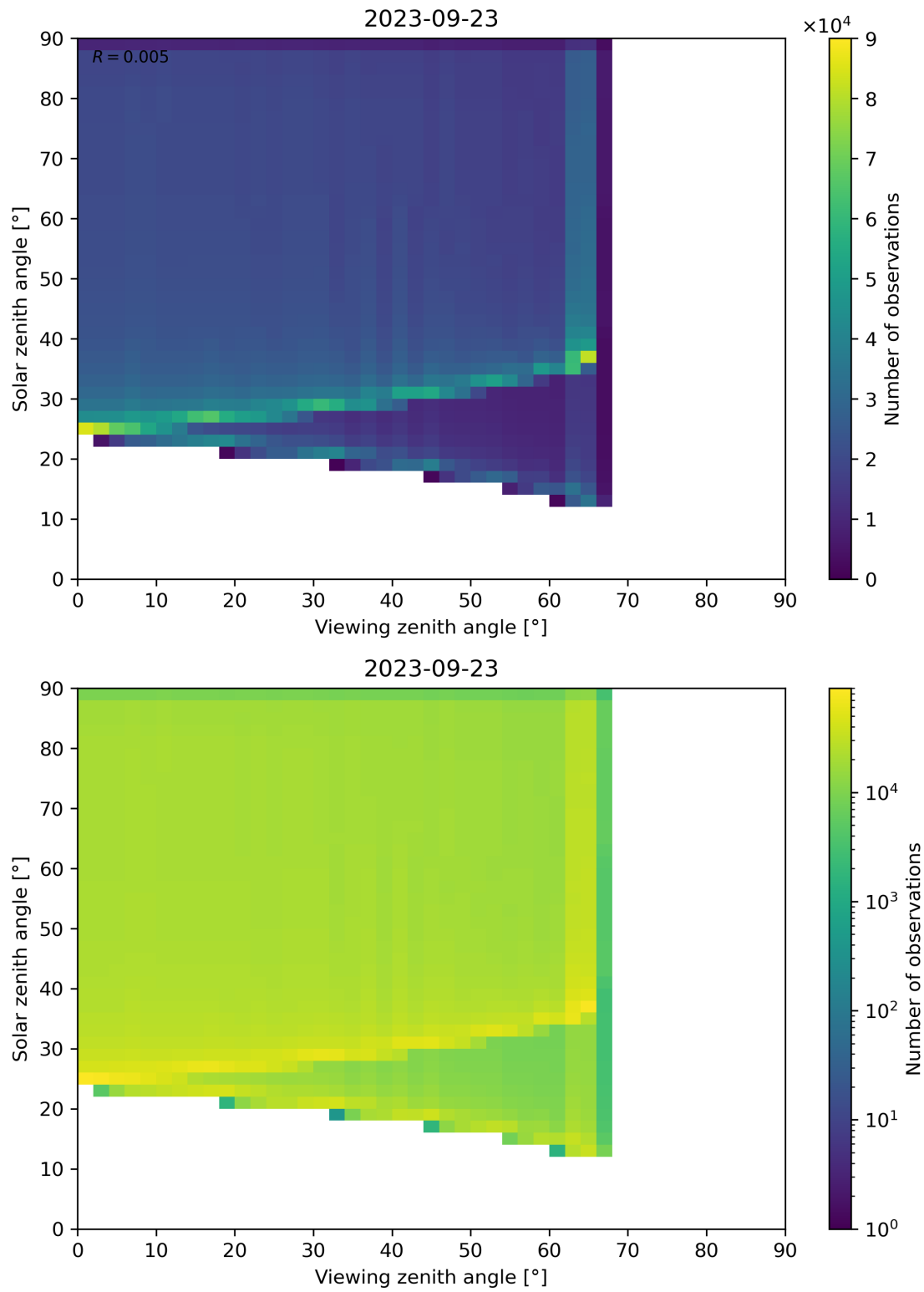
Figure 54: Scatter density plot of “Viewing zenith angle” against “Solar zenith angle” for 2023-09-22 to 2023-09-24.
