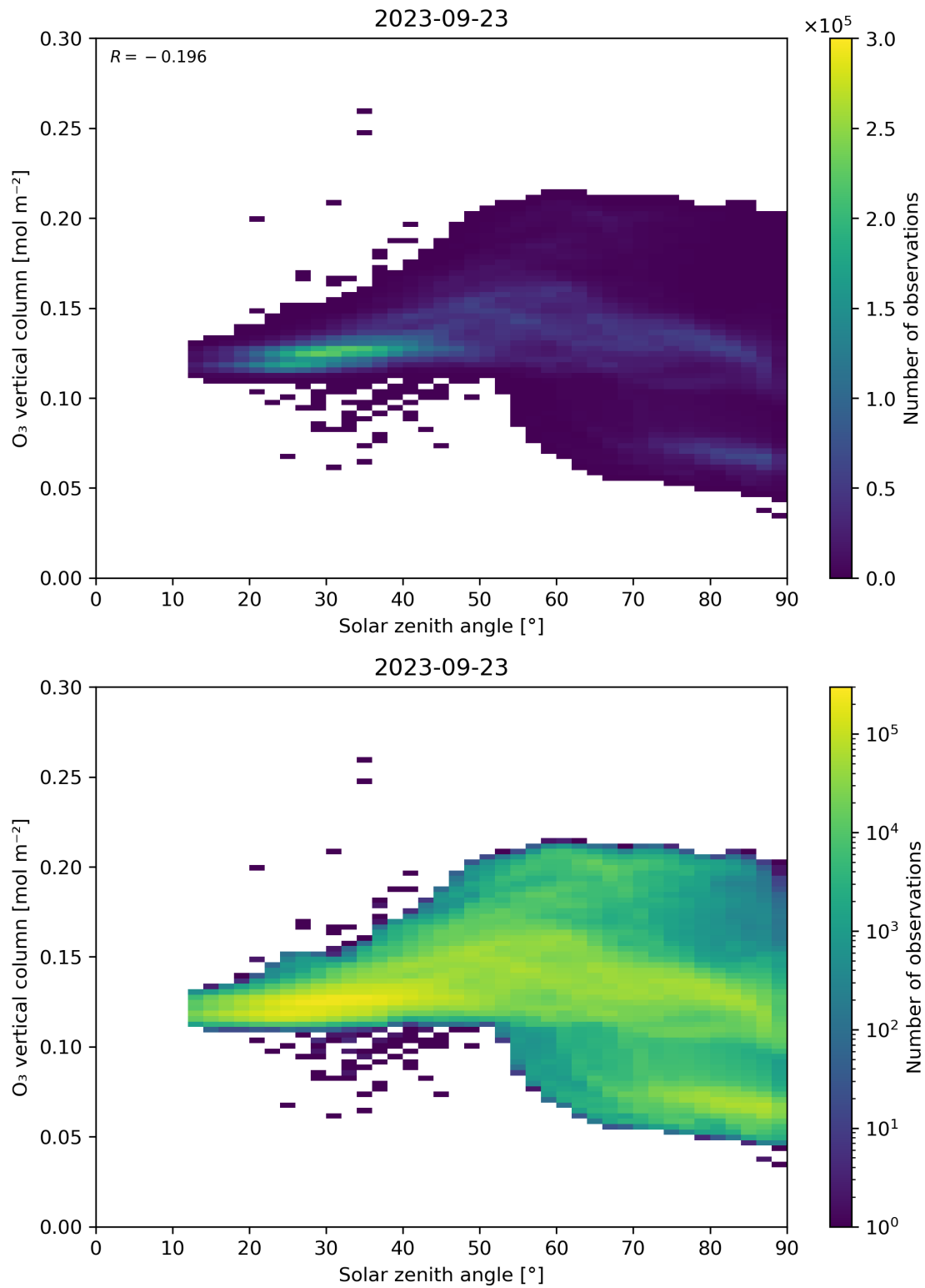
Figure 47: Scatter density plot of “Solar zenith angle” against “O 3 vertical column” for 2023-09-22 to 2023-09-24.
