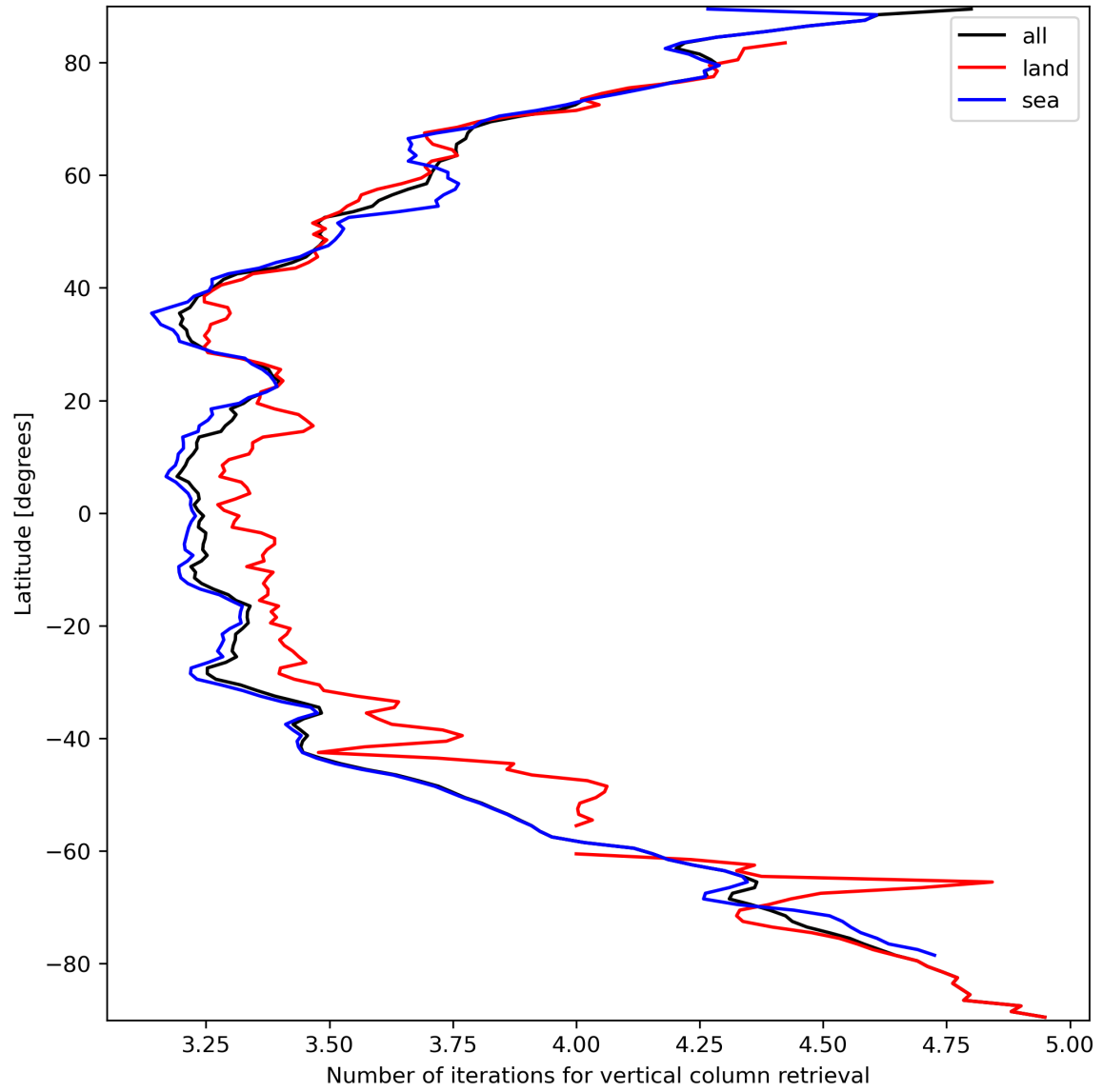
Figure 19: Zonal average of “Number of iterations for vertical column retrieval” for 2023-09-22 to 2023-09-24.
