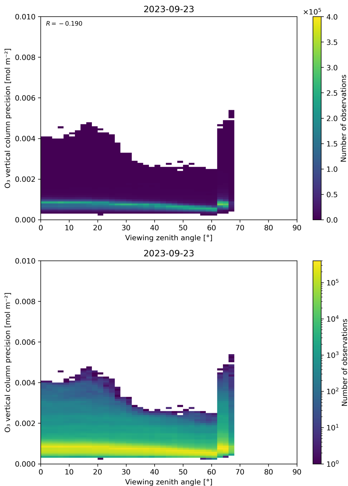
Figure 53: Scatter density plot of “Viewing zenith angle” against “O 3 vertical column precision” for 2023-09-22 to 2023-09-24.
