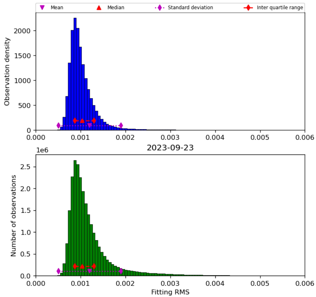
Figure 23: Histogram of “Fitting RMS” for 2023-09-22 to 2023-09-24
