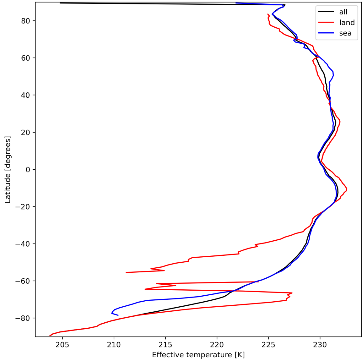
Figure 17: Zonal average of “Effective temperature” for 2023-09-22 to 2023-09-24.
