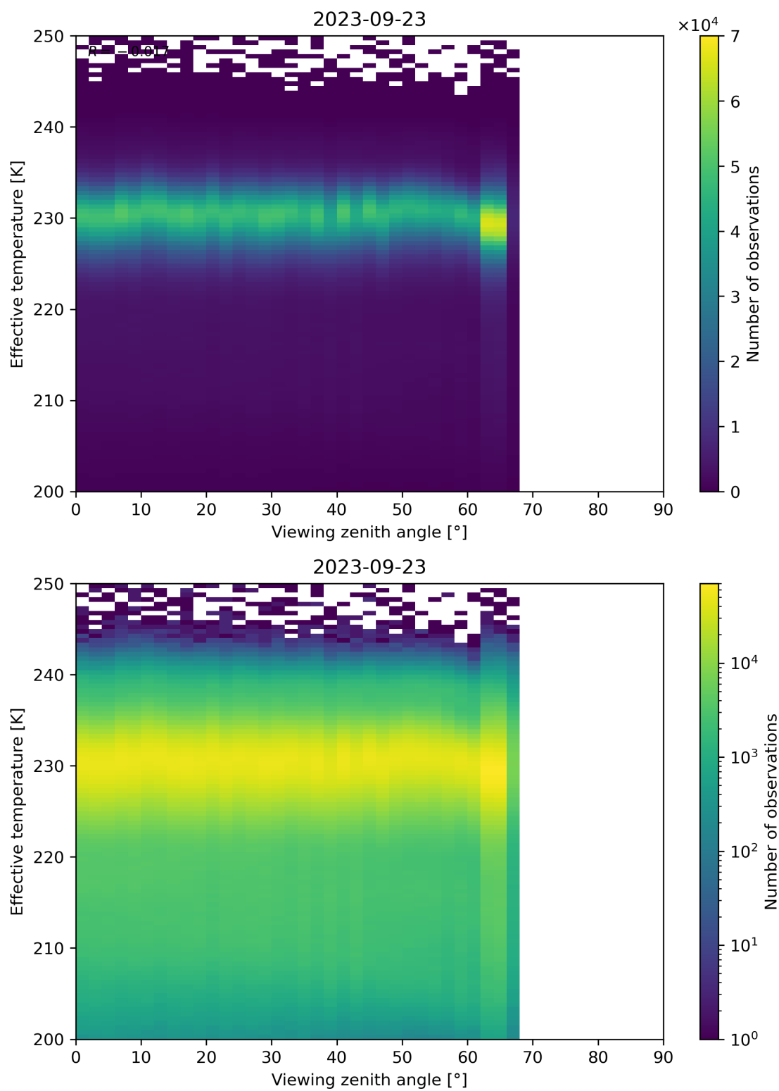
Figure 50: Scatter density plot of “Viewing zenith angle” against “Effective temperature” for 2023-09-22 to 2023-09-24.
