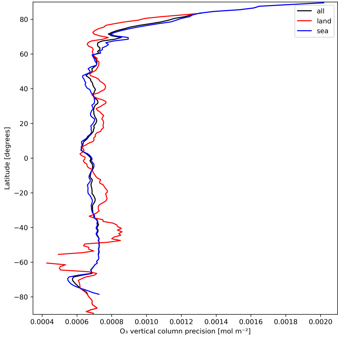
Figure 15: Zonal average of “O 3 vertical column precision” for 2023-09-22 to 2023-09-24.
