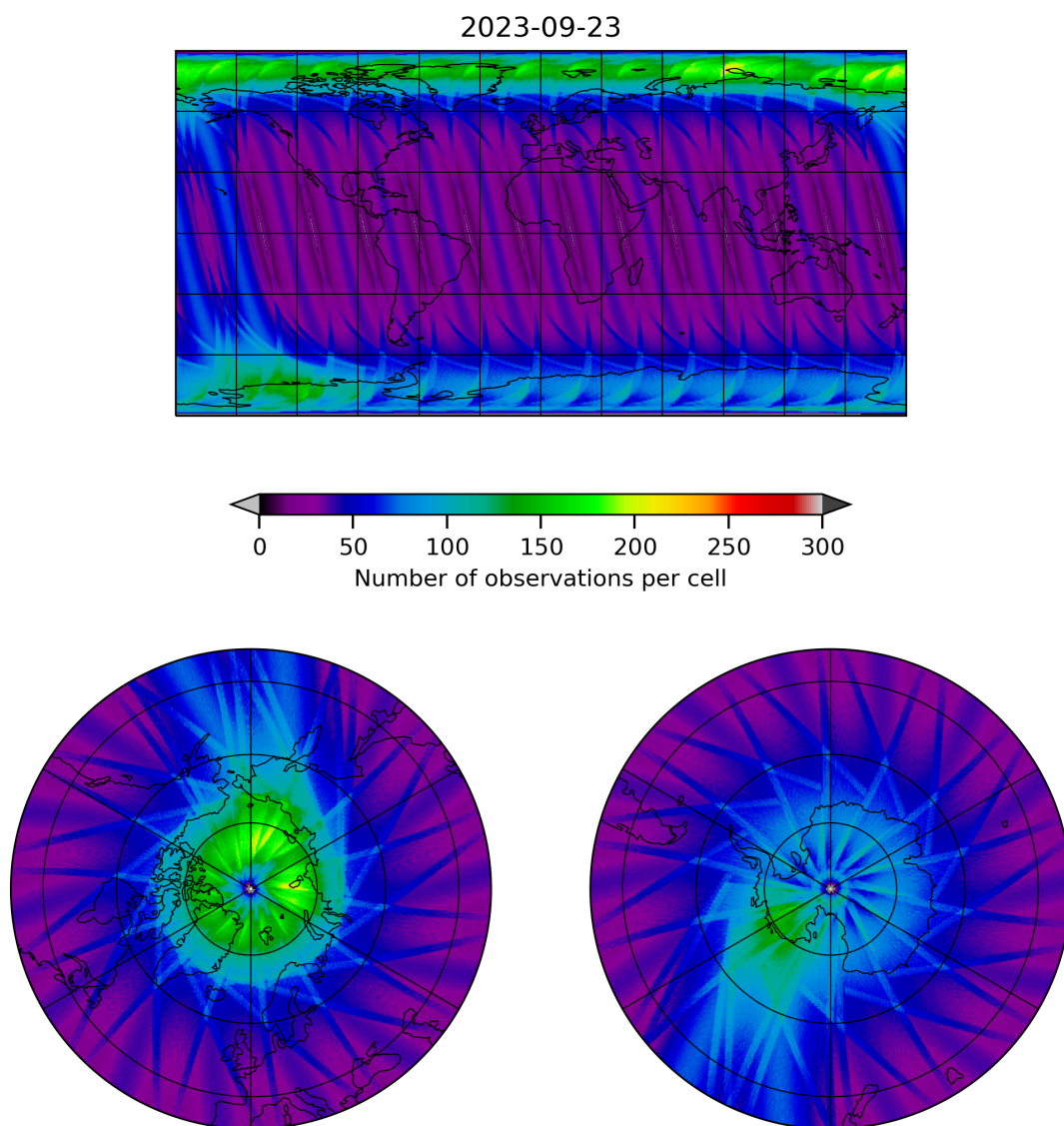
Figure 12: Map of the number of observations for 2023-09-22 to 2023-09-24
