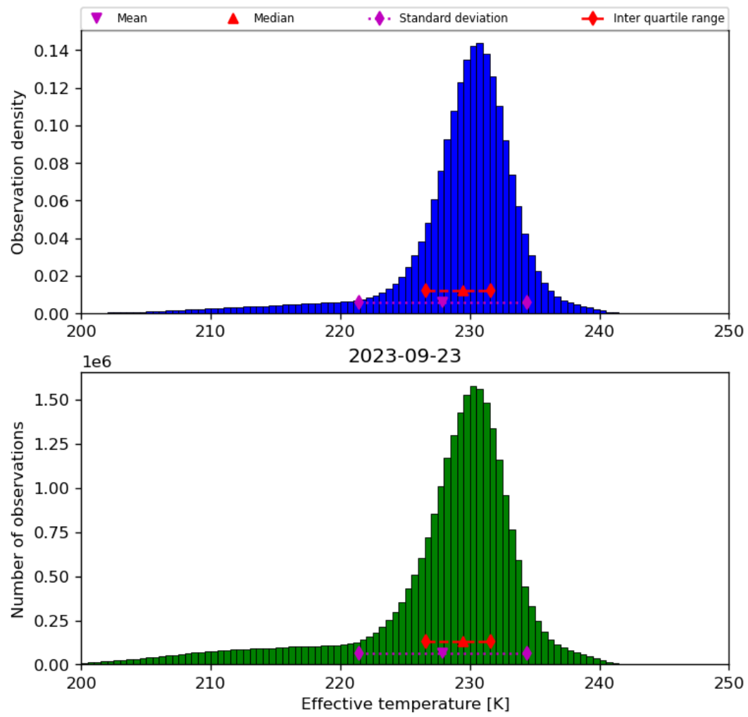
Figure 24: Histogram of “Effective temperature” for 2023-09-22 to 2023-09-24
