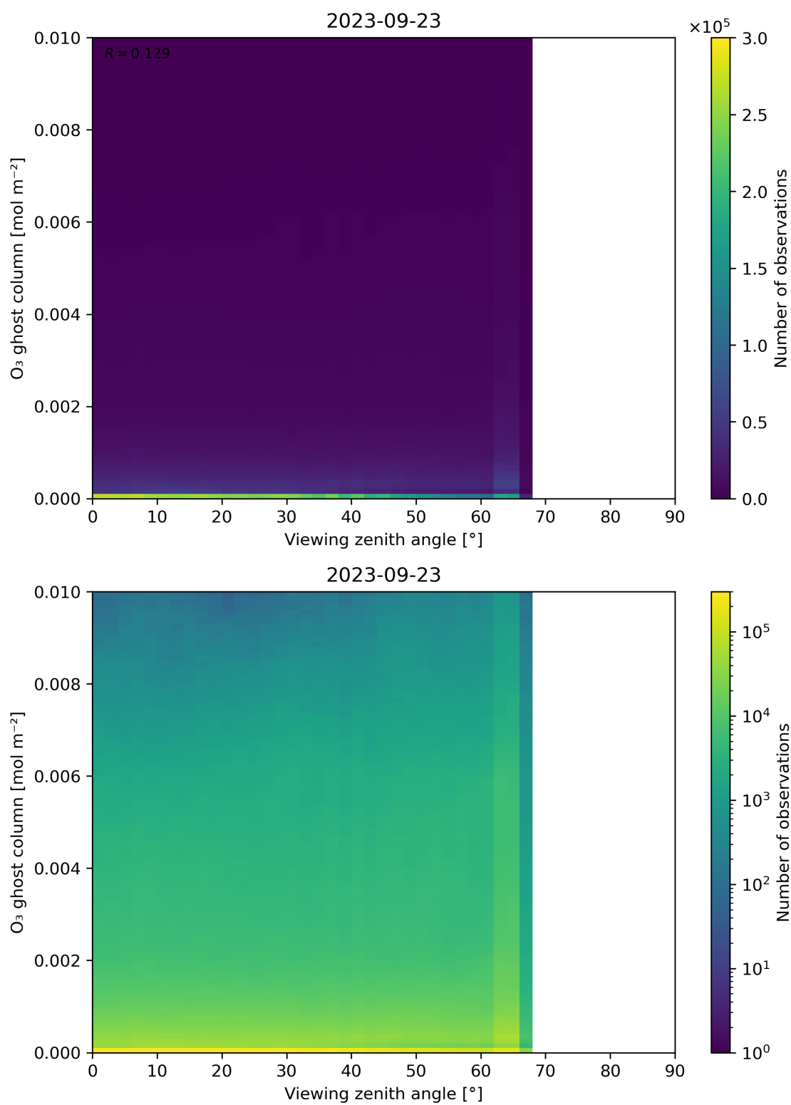
Figure 51: Scatter density plot of “Viewing zenith angle” against “O 3 ghost column” for 2023-09-22 to 2023-09-24.
