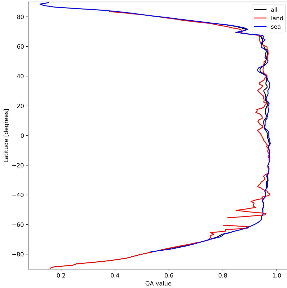
Figure 13: Zonal average of “QA value” for 2023-09-22 to 2023-09-24.
