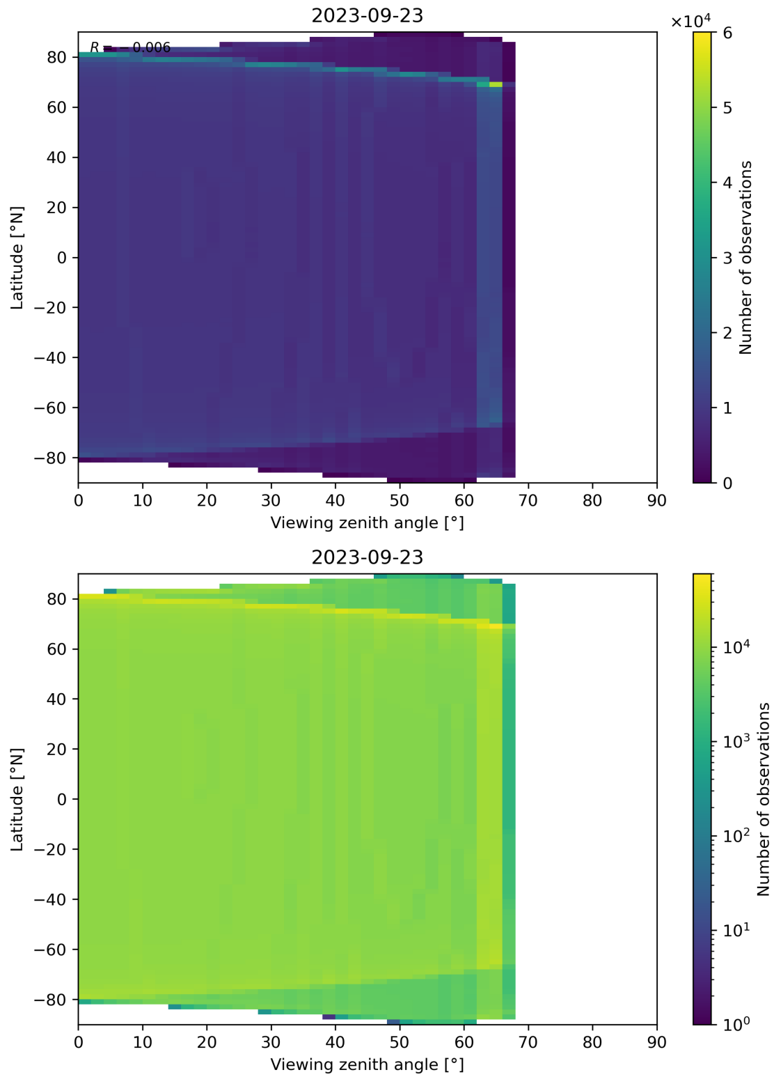
Figure 49: Scatter density plot of “Viewing zenith angle” against “Latitude” for 2023-09-22 to 2023-09-24.
