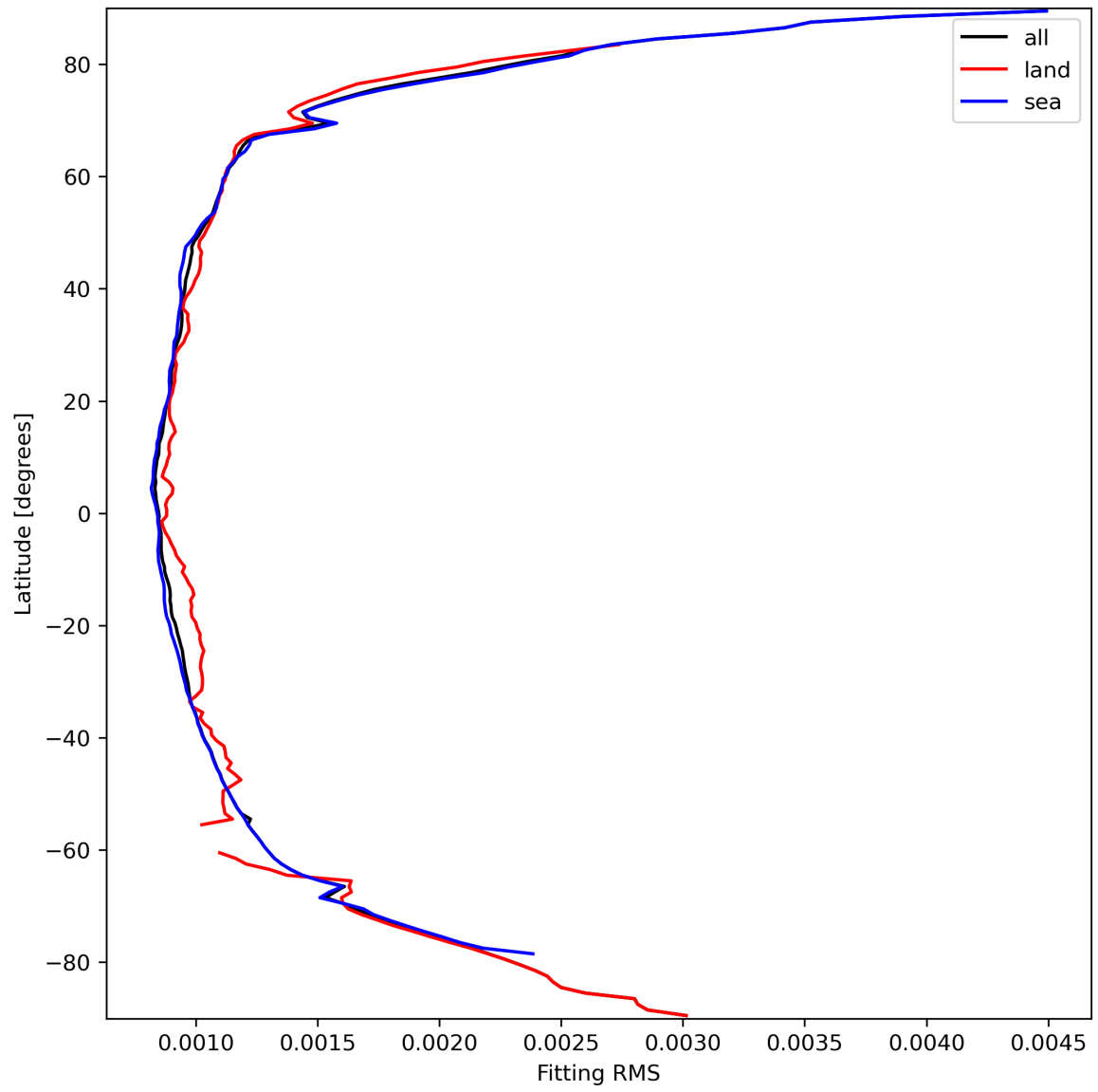
Figure 16: Zonal average of “Fitting RMS” for 2023-09-22 to 2023-09-24.
