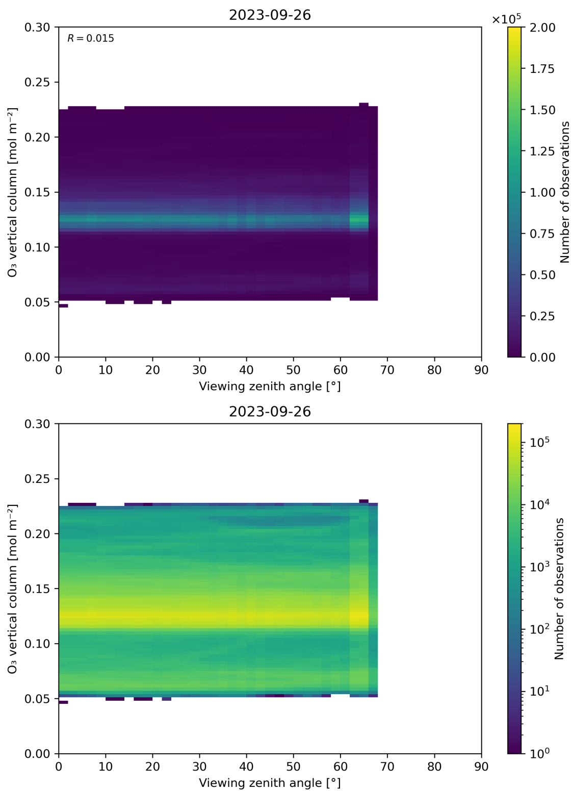
Figure 52: Scatter density plot of “Viewing zenith angle” against “O 3 vertical column” for 2023-09-26 to 2023-09-27.
