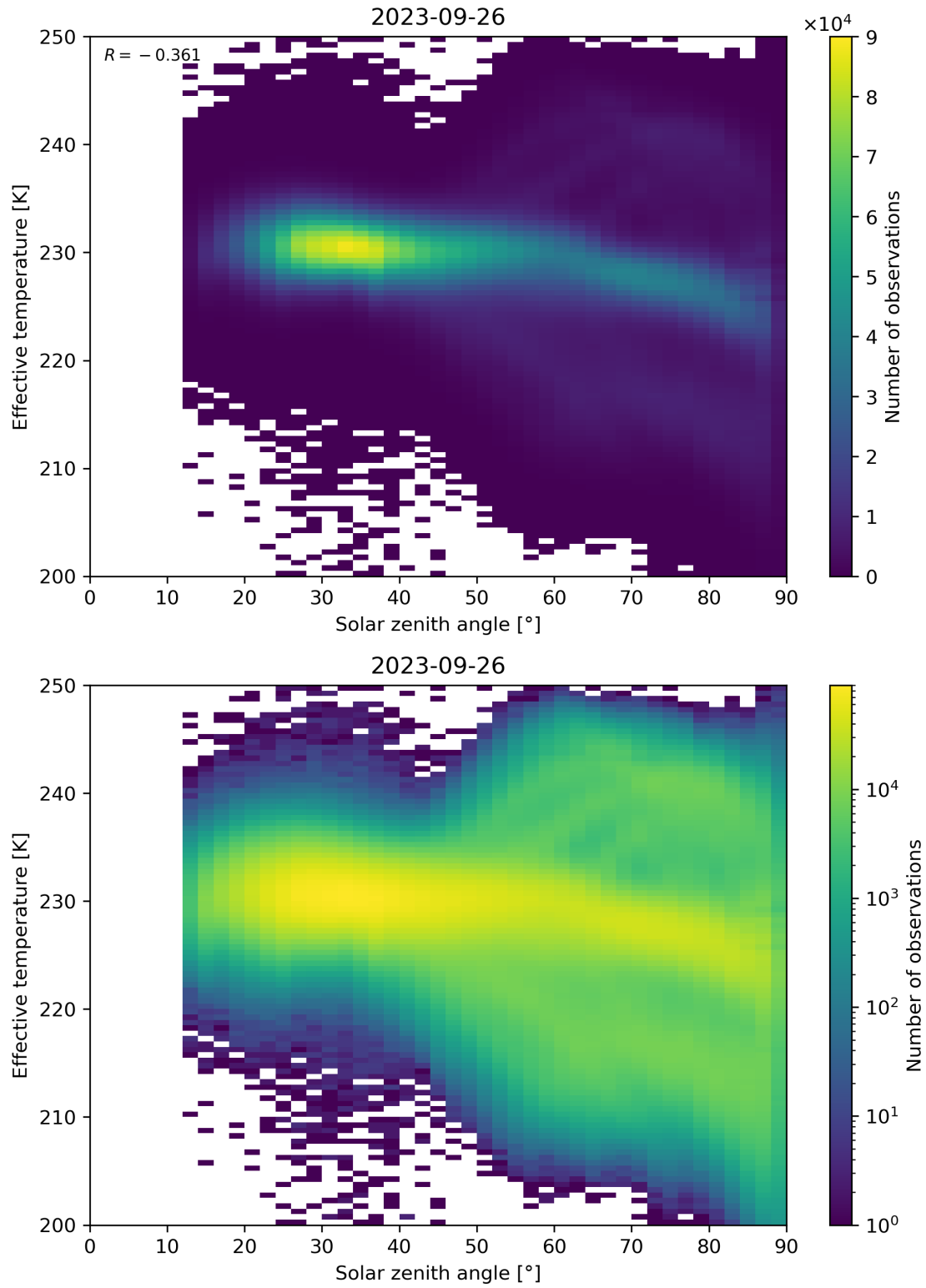
Figure 45: Scatter density plot of “Solar zenith angle” against “Effective temperature” for 2023-09-26 to 2023-09-27.
