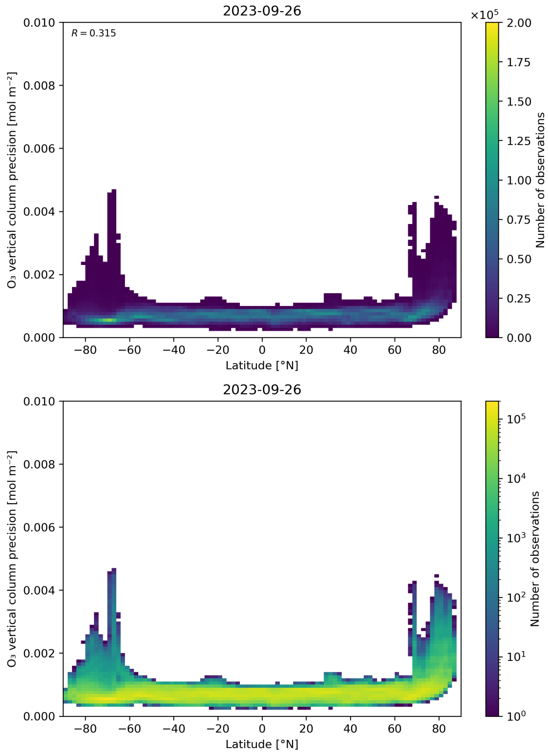
Figure 37: Scatter density plot of “Latitude” against “O 3 vertical column precision” for 2023-09-26 to 2023-09-27.
