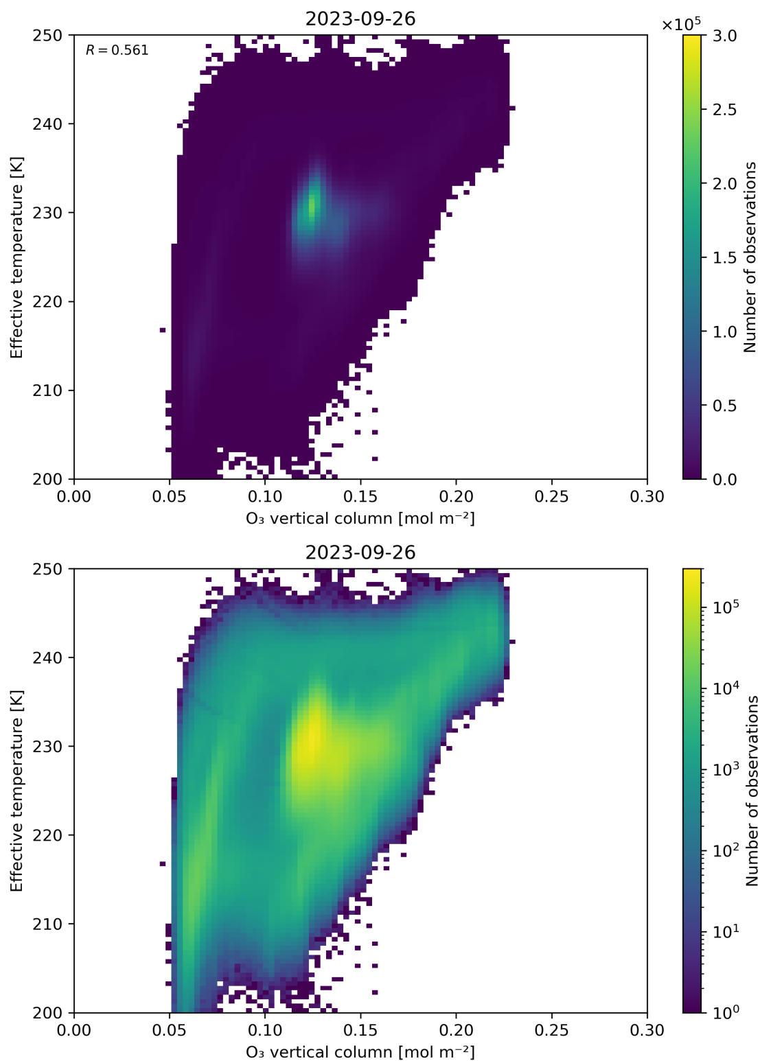
Figure 39: Scatter density plot of “O 3 vertical column” against “Effective temperature” for 2023-09-26 to 2023-09-27.
