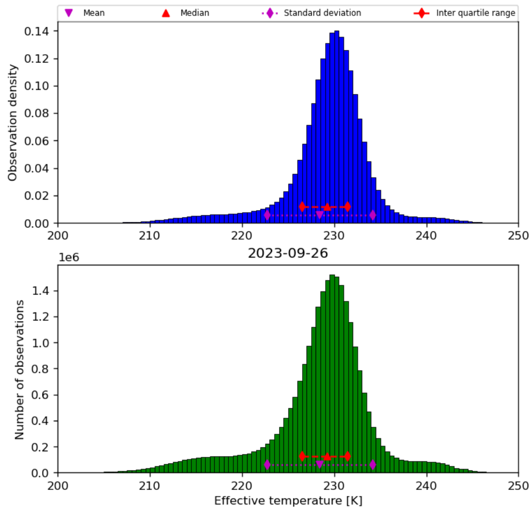
Figure 24: Histogram of “Effective temperature” for 2023-09-26 to 2023-09-27
