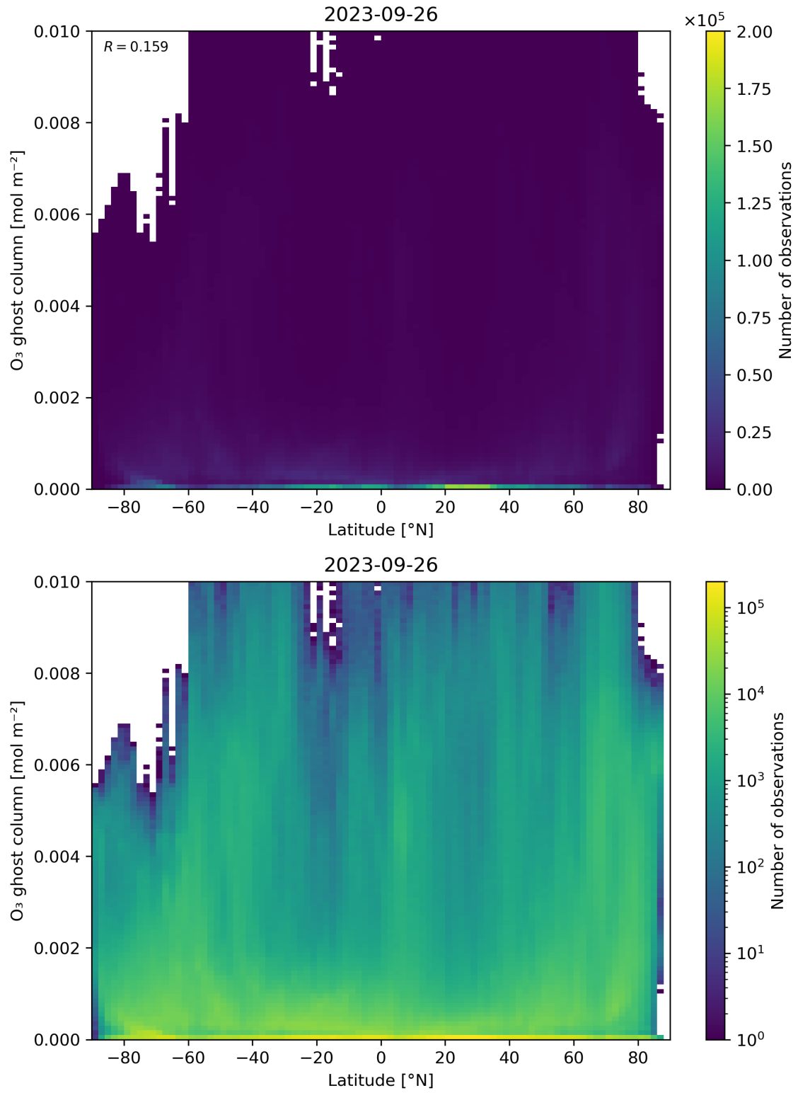
Figure 35: Scatter density plot of “Latitude” against “O 3 ghost column” for 2023-09-26 to 2023-09-27.
