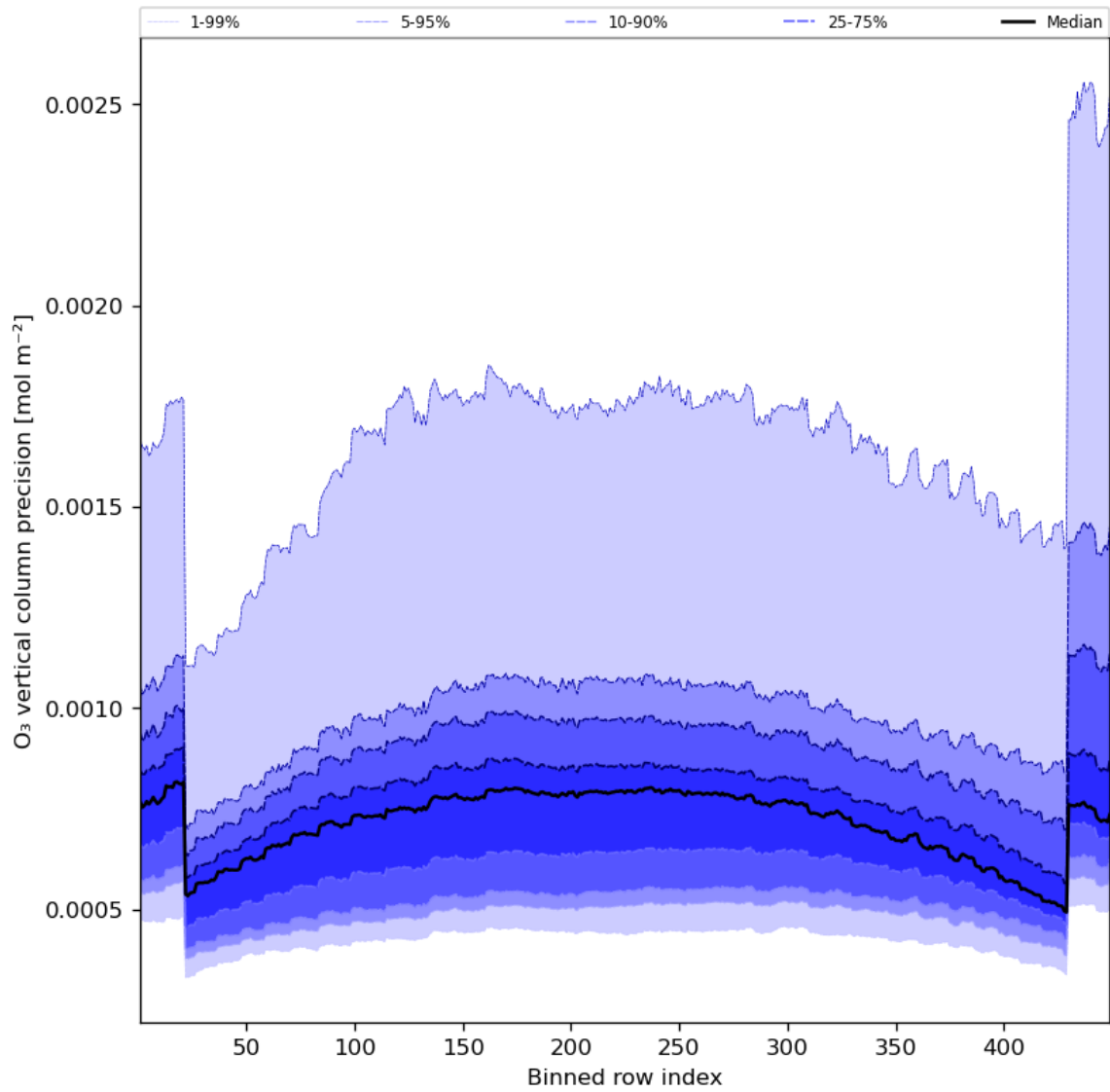
Figure 29: Along track statistics of “O 3 vertical column precision” for 2023-09-26 to 2023-09-27
