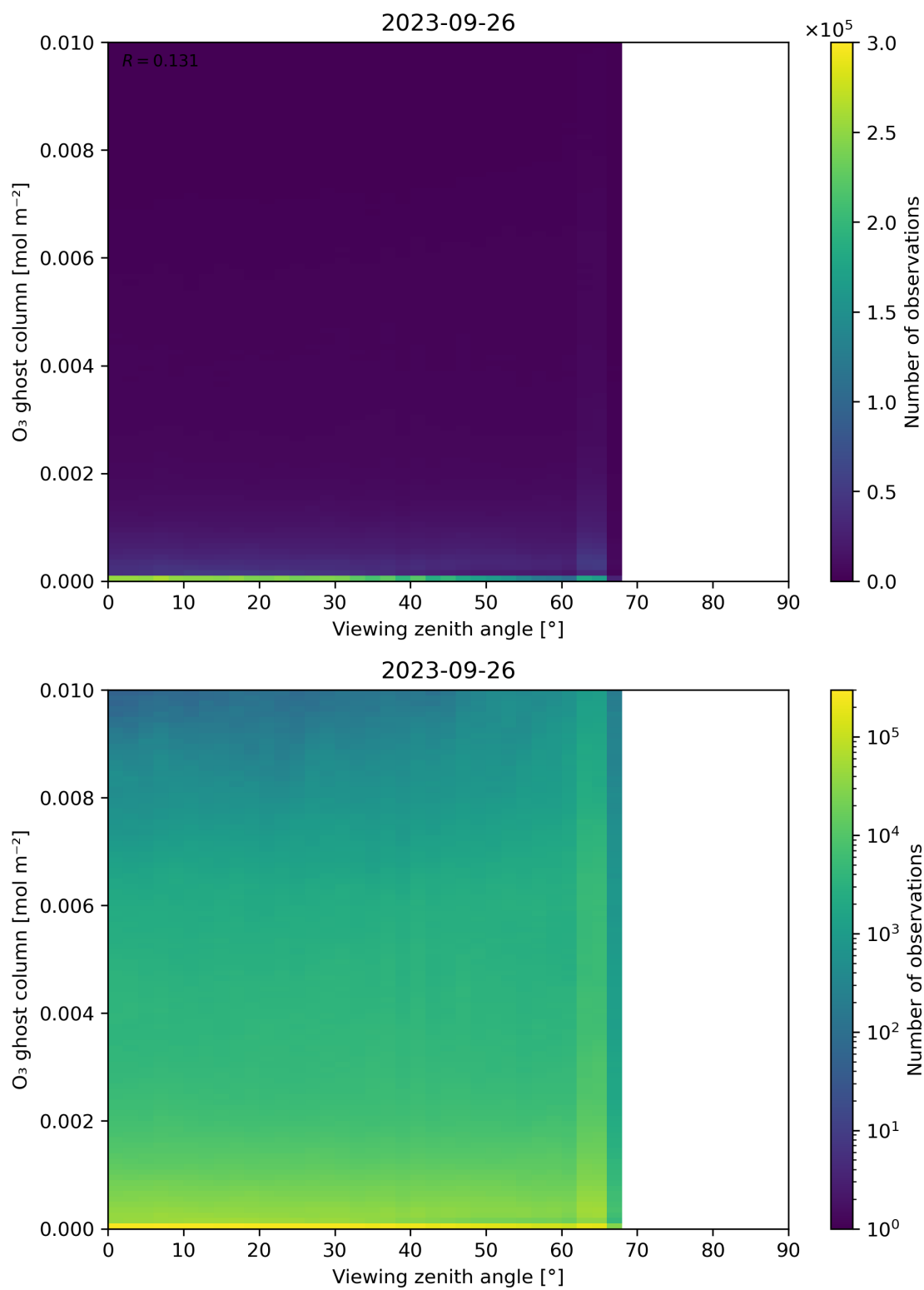
Figure 51: Scatter density plot of “Viewing zenith angle” against “O 3 ghost column” for 2023-09-26 to 2023-09-27.
