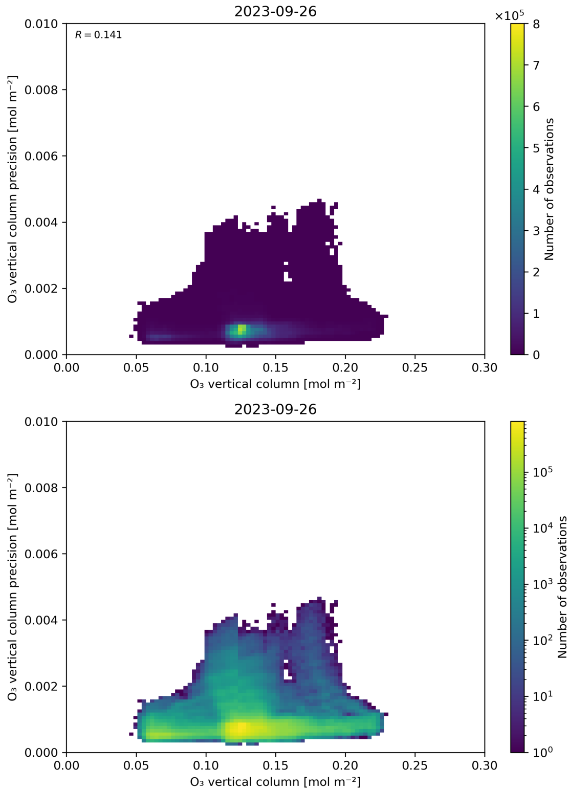
Figure 41: Scatter density plot of “O 3 vertical column” against “O 3 vertical column precision” for 2023-09-26 to 2023-09-27.
