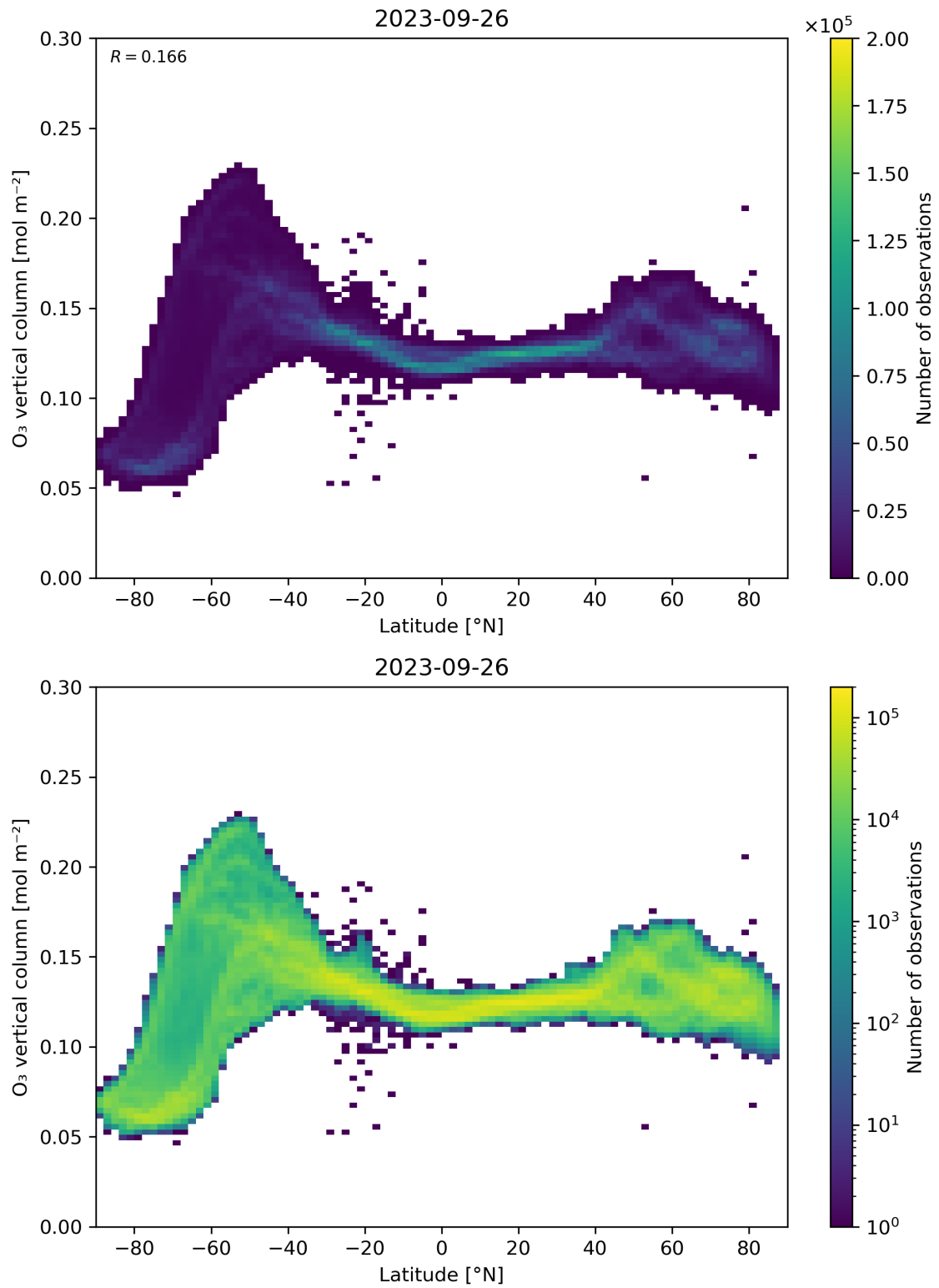
Figure 36: Scatter density plot of “Latitude” against “O 3 vertical column” for 2023-09-26 to 2023-09-27.
