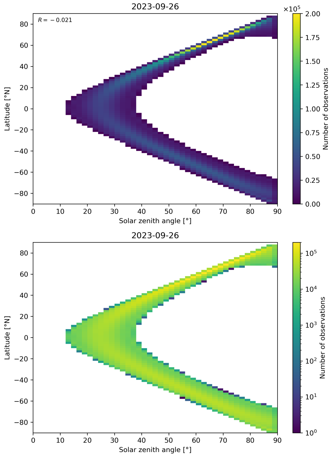
Figure 44: Scatter density plot of “Solar zenith angle” against “Latitude” for 2023-09-26 to 2023-09-27.
