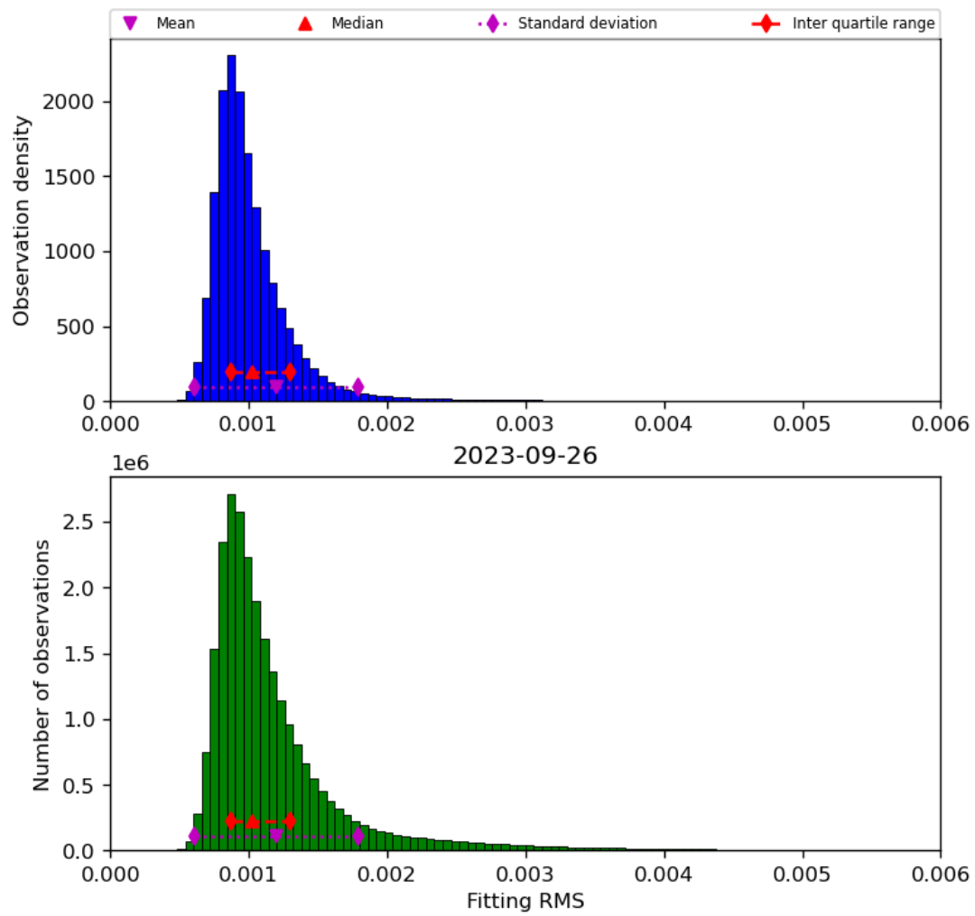
Figure 23: Histogram of “Fitting RMS” for 2023-09-26 to 2023-09-27
