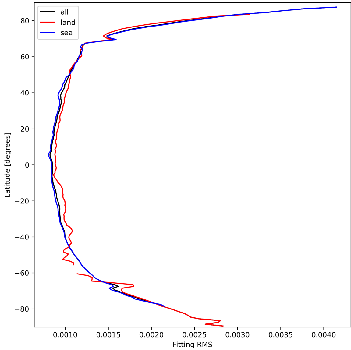
Figure 16: Zonal average of “Fitting RMS” for 2023-09-26 to 2023-09-27.
