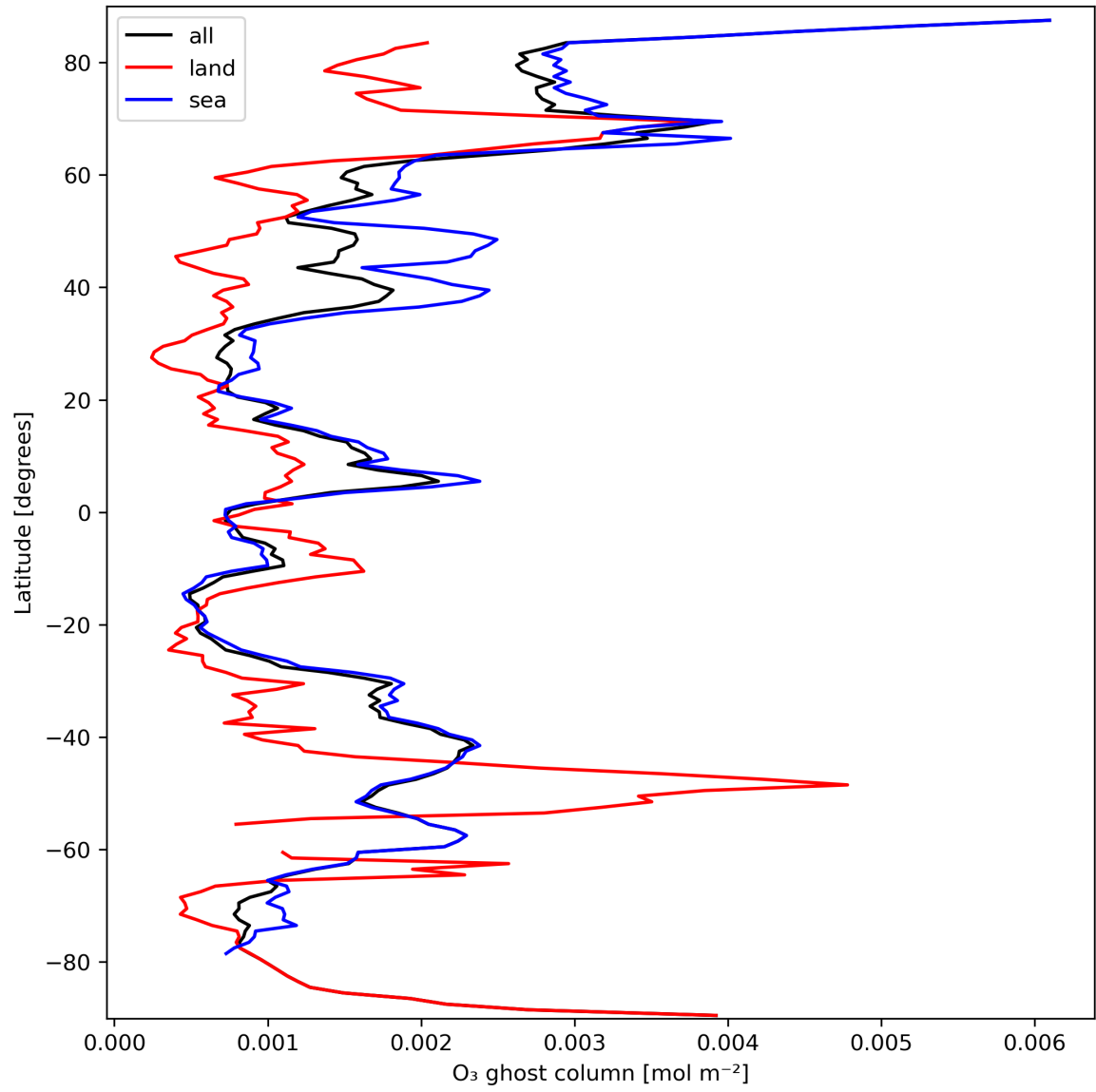
Figure 18: Zonal average of “O 3 ghost column” for 2023-09-26 to 2023-09-27.
