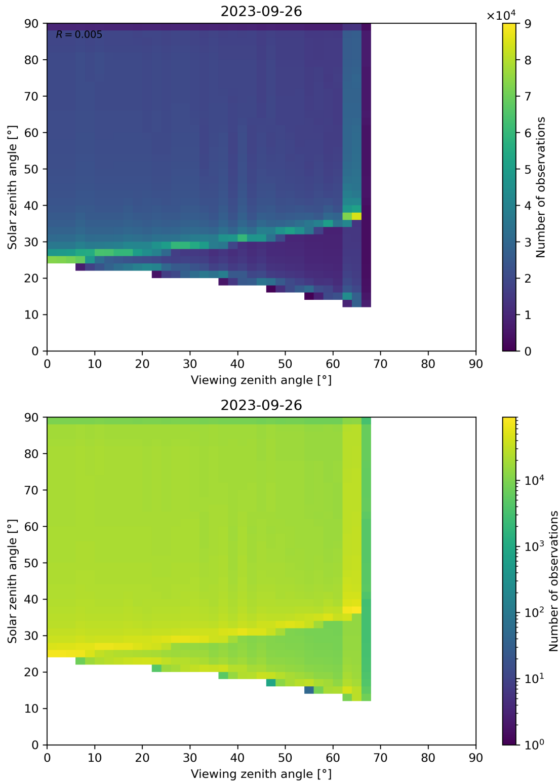
Figure 54: Scatter density plot of “Viewing zenith angle” against “Solar zenith angle” for 2023-09-26 to 2023-09-27.
