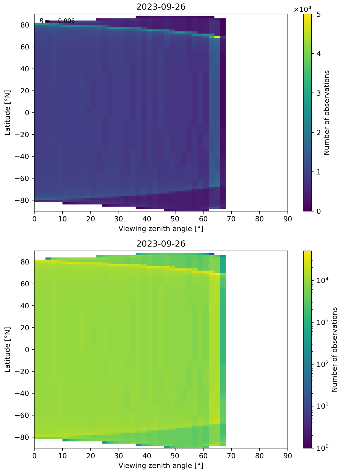
Figure 49: Scatter density plot of “Viewing zenith angle” against “Latitude” for 2023-09-26 to 2023-09-27.
