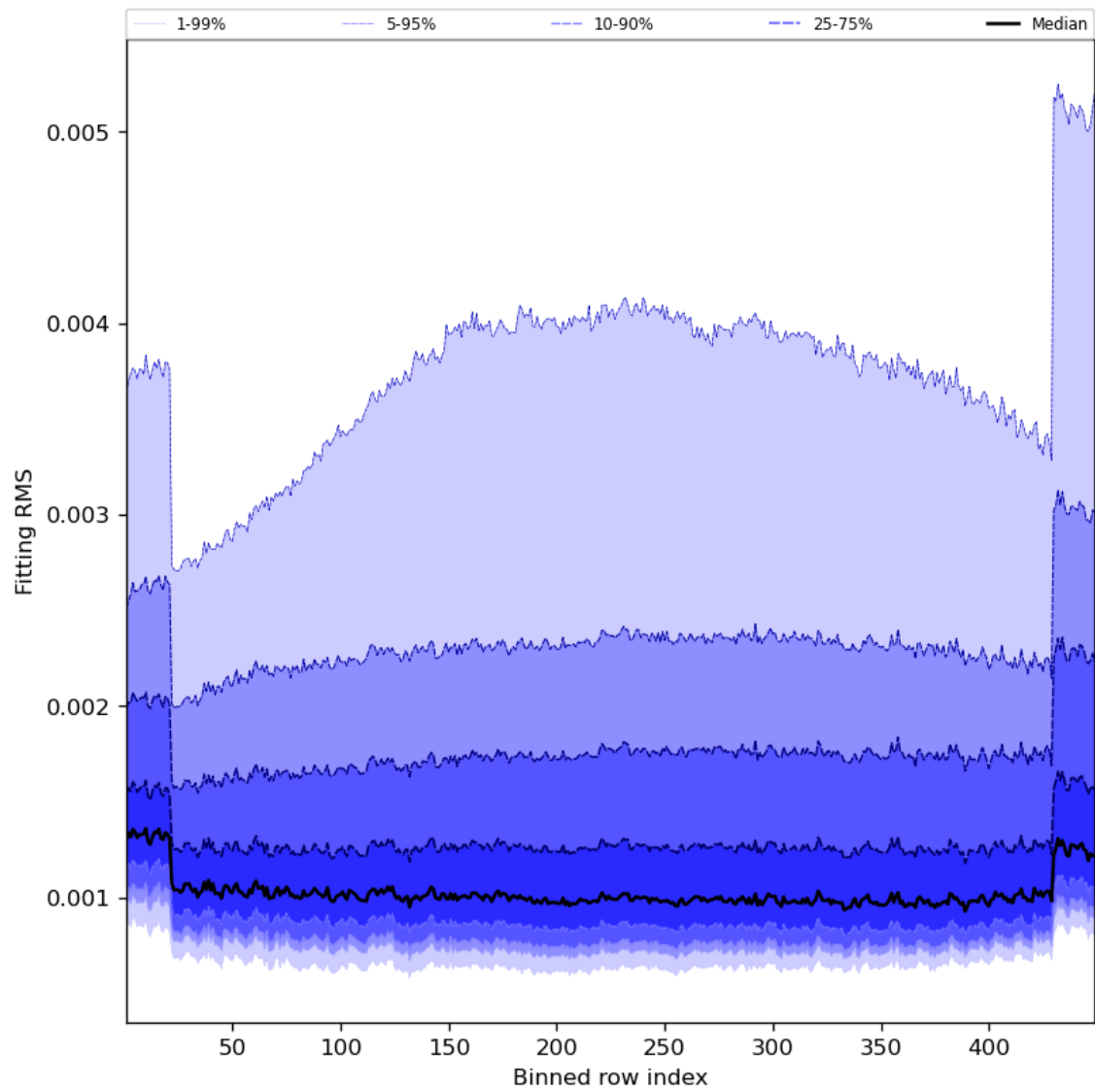
Figure 30: Along track statistics of “Fitting RMS” for 2023-09-26 to 2023-09-27
