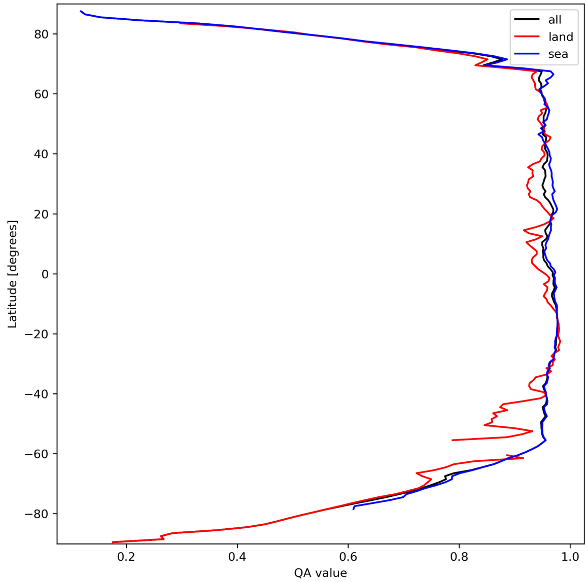
Figure 13: Zonal average of “QA value” for 2023-09-26 to 2023-09-27.
