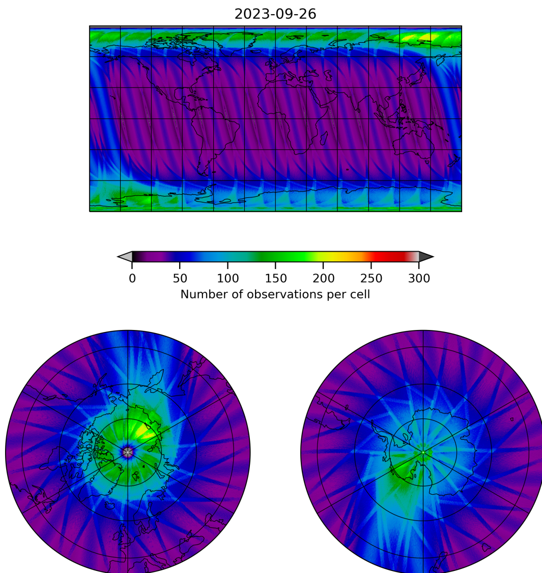
Figure 12: Map of the number of observations for 2023-09-26 to 2023-09-27
