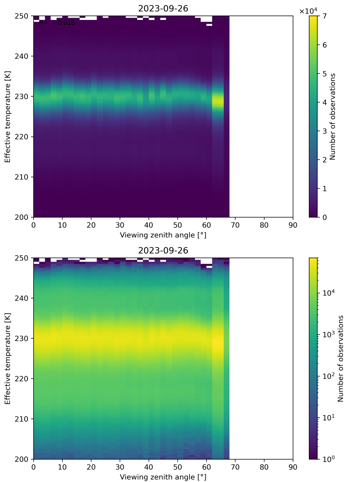
Figure 50: Scatter density plot of “Viewing zenith angle” against “Effective temperature” for 2023-09-26 to 2023-09-27.
