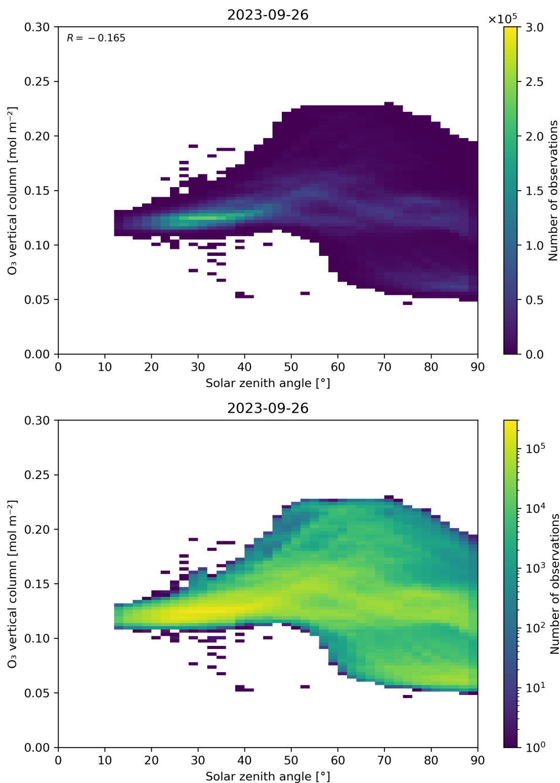
Figure 47: Scatter density plot of “Solar zenith angle” against “O 3 vertical column” for 2023-09-26 to 2023-09-27.
