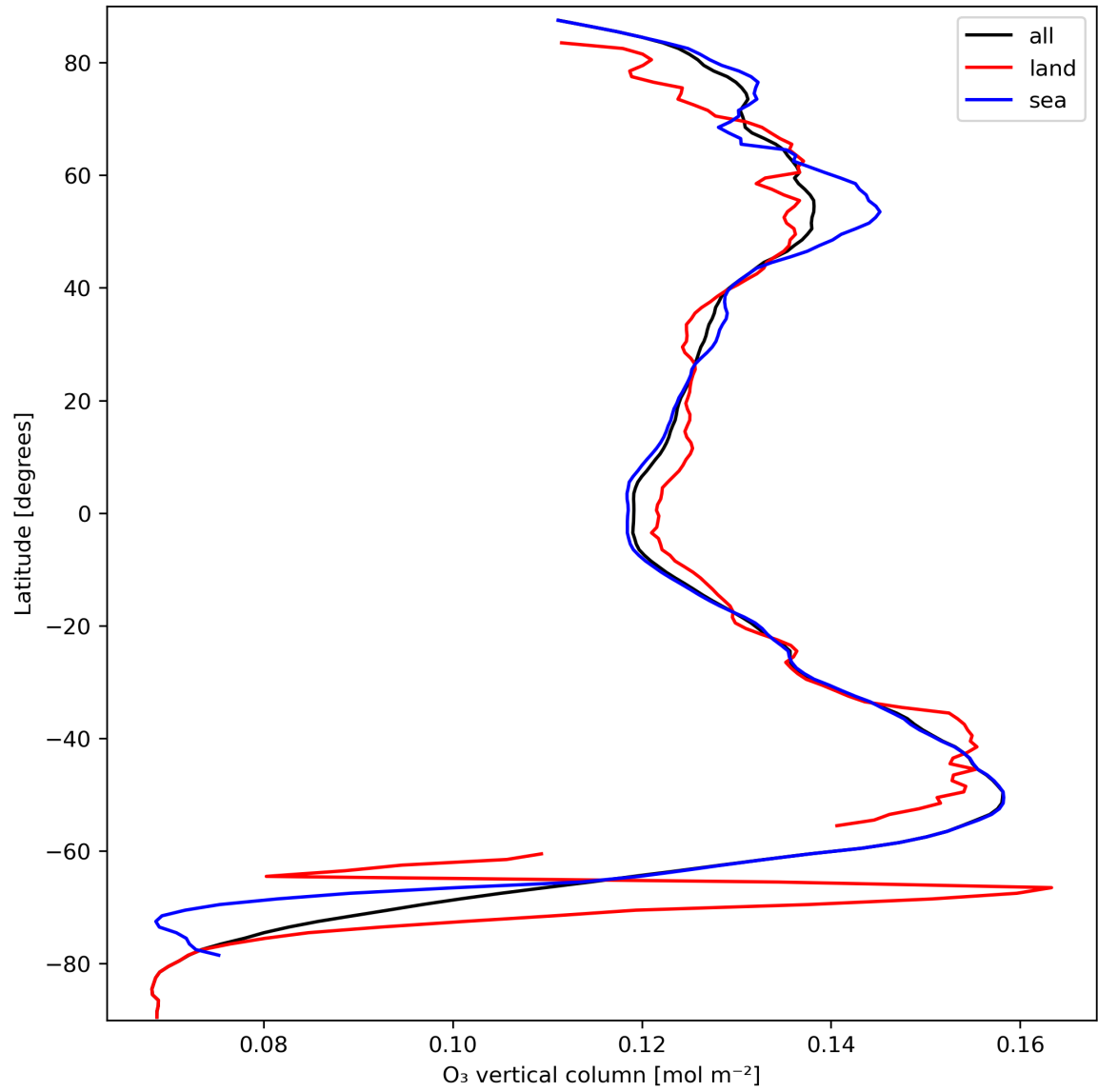
Figure 14: Zonal average of “O 3 vertical column” for 2023-09-26 to 2023-09-27.
