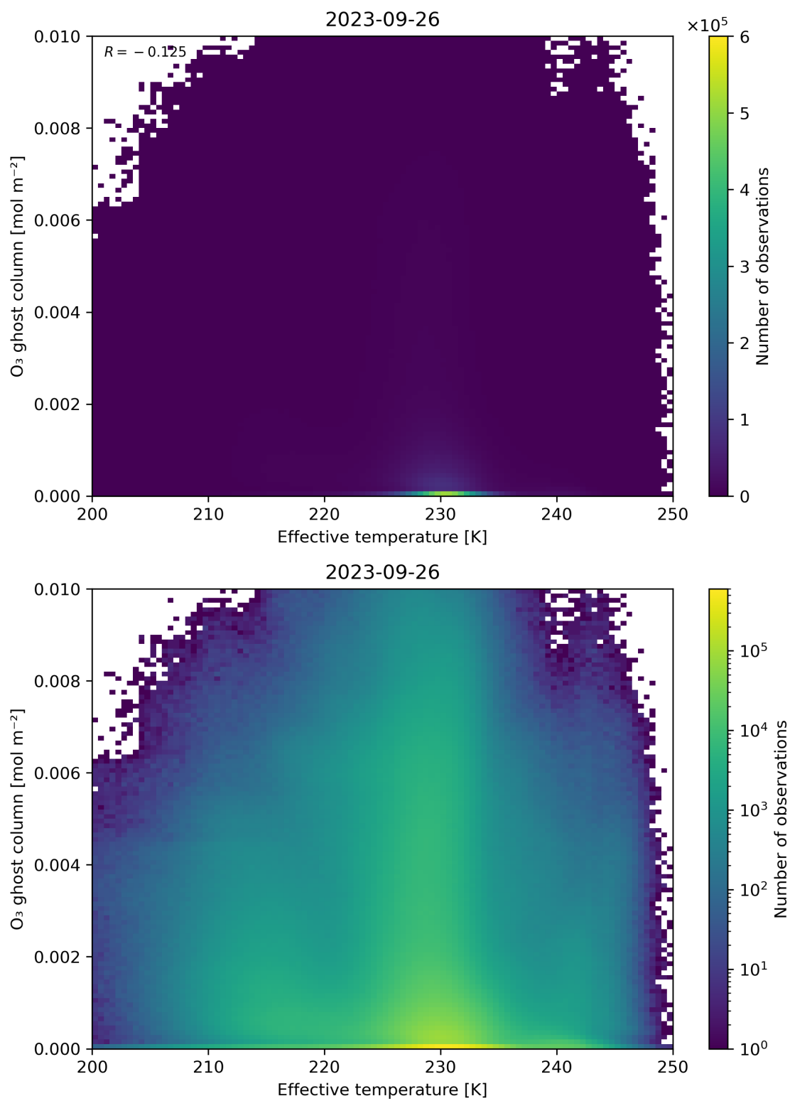
Figure 38: Scatter density plot of “Effective temperature” against “O 3 ghost column” for 2023-09-26 to 2023-09-27.
