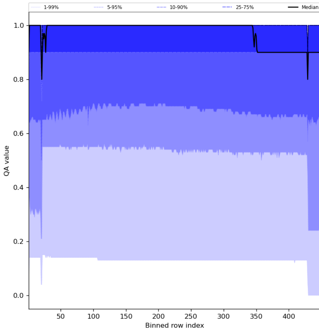
Figure 27: Along track statistics of “QA value” for 2023-09-26 to 2023-09-27
