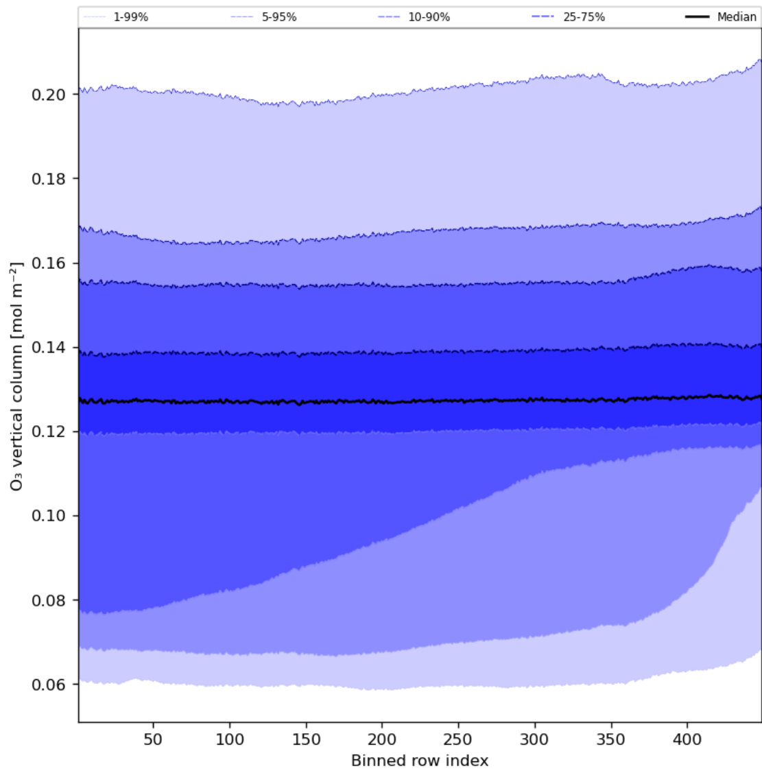
Figure 28: Along track statistics of “O 3 vertical column” for 2023-09-26 to 2023-09-27
