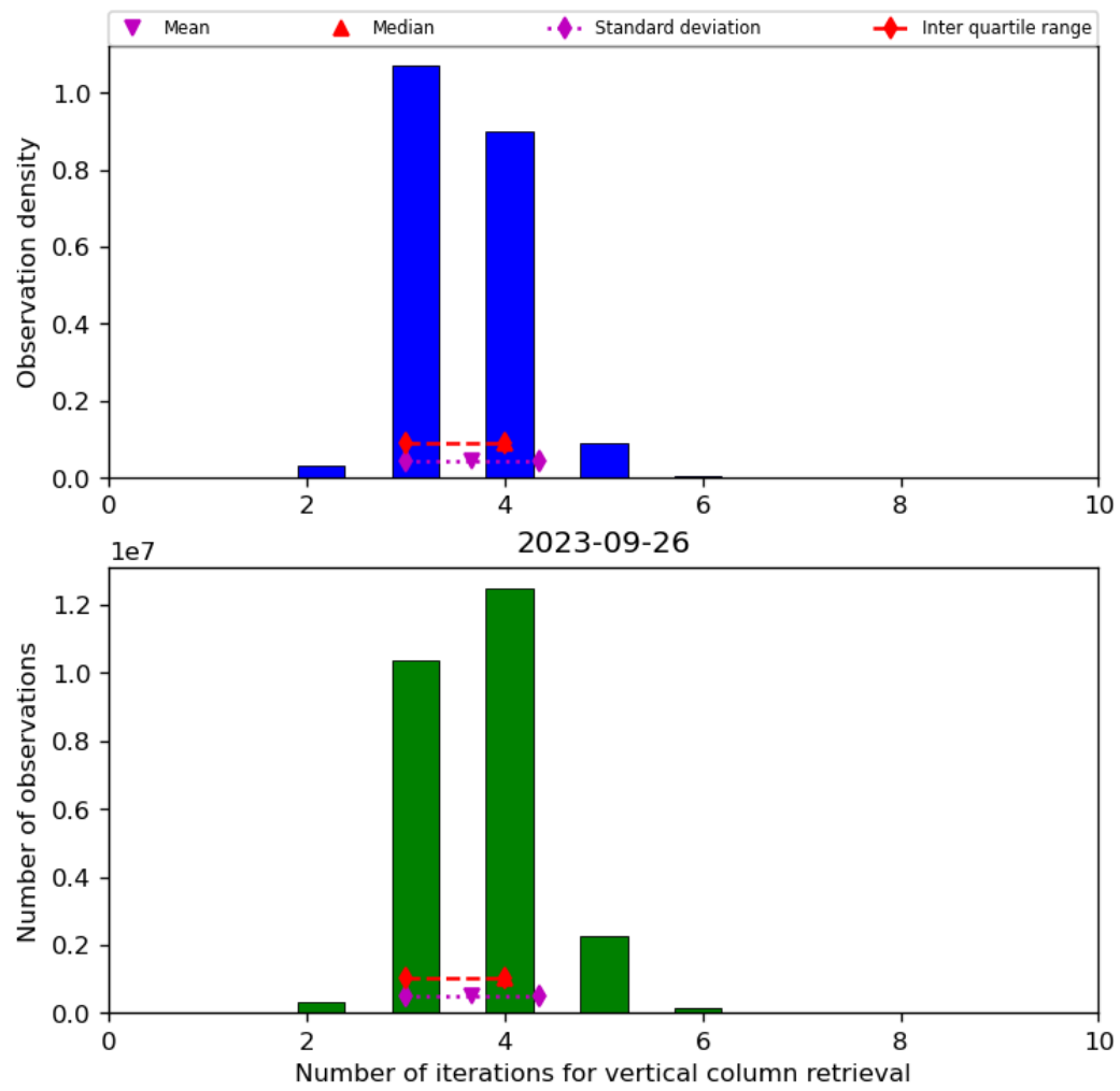
Figure 26: Histogram of “Number of iterations for vertical column retrieval” for 2023-09-26 to 2023-09-27
