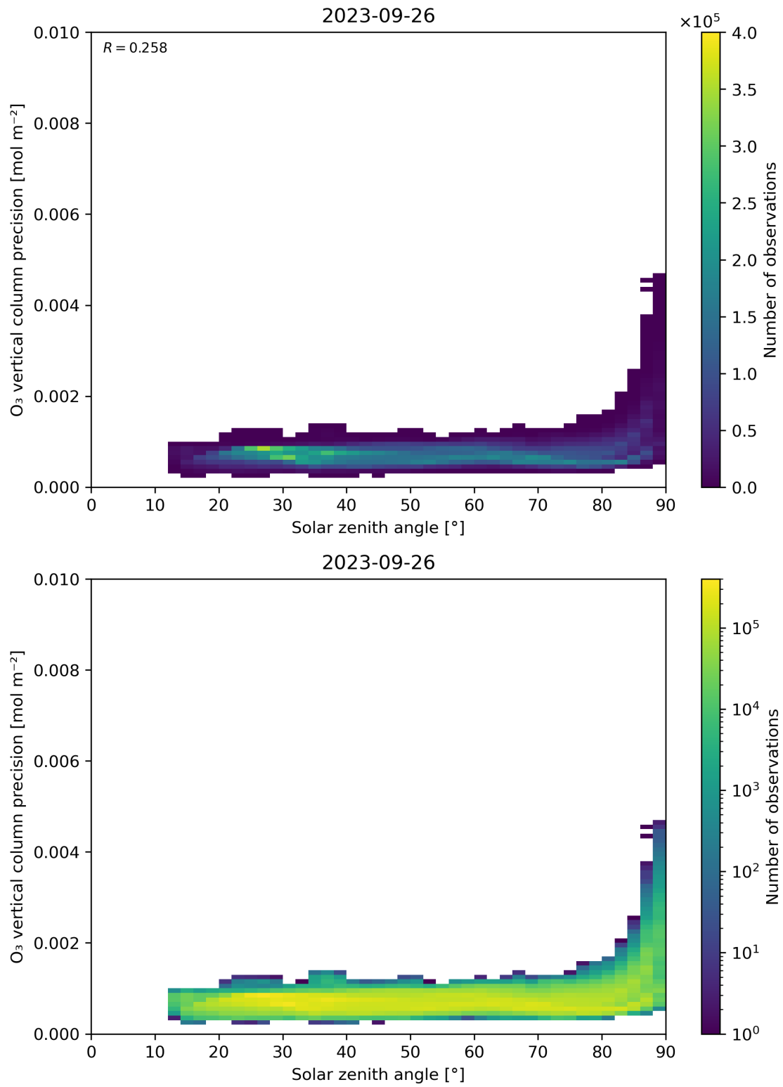
Figure 48: Scatter density plot of “Solar zenith angle” against “O 3 vertical column precision” for 2023-09-26 to 2023-09-27.
