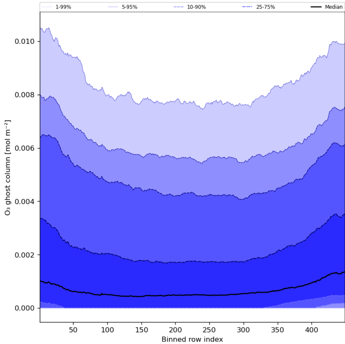
Figure 32: Along track statistics of “O 3 ghost column” for 2023-09-26 to 2023-09-27
