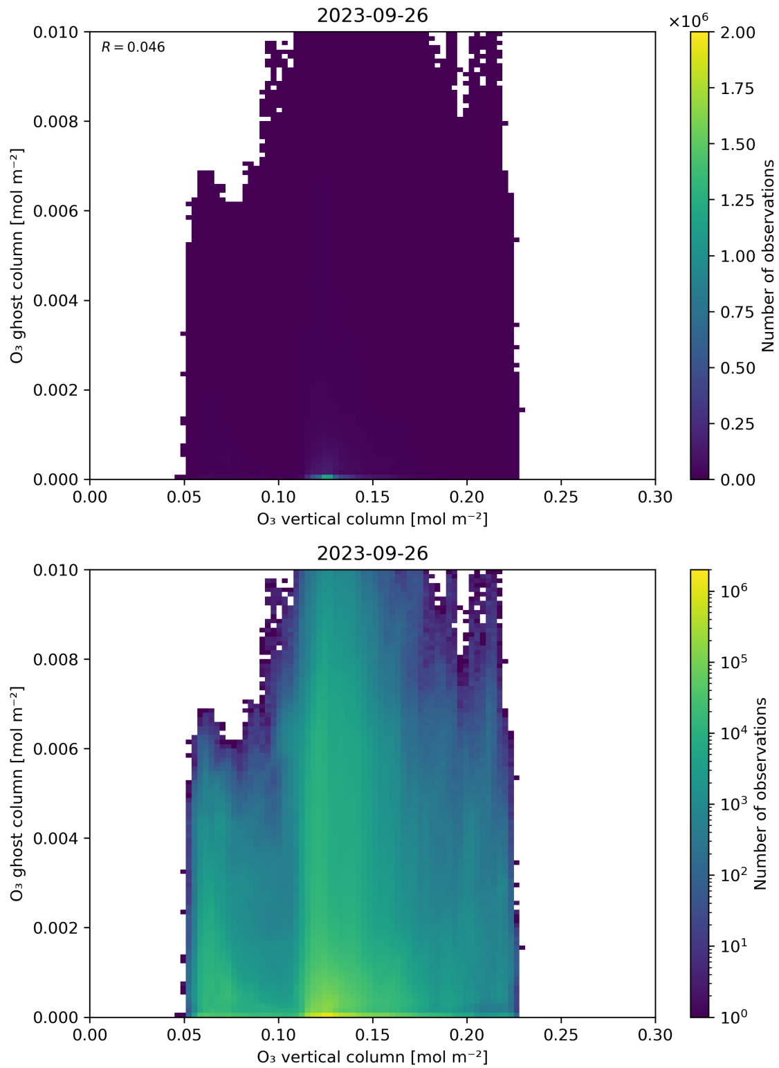
Figure 40: Scatter density plot of “O 3 vertical column” against “O 3 ghost column” for 2023-09-26 to 2023-09-27.
