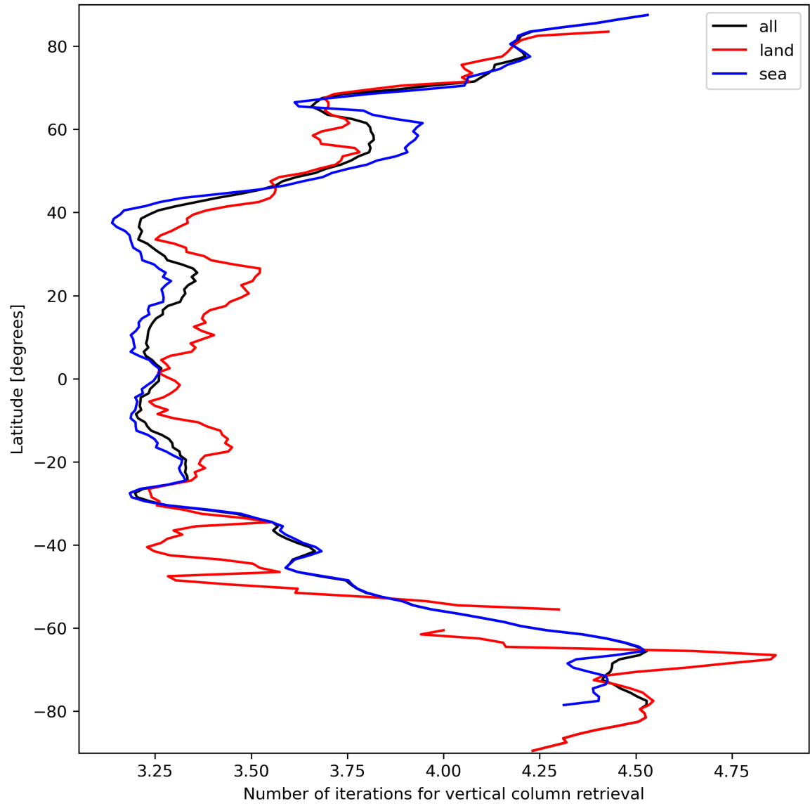
Figure 19: Zonal average of “Number of iterations for vertical column retrieval” for 2023-09-26 to 2023-09-27.
