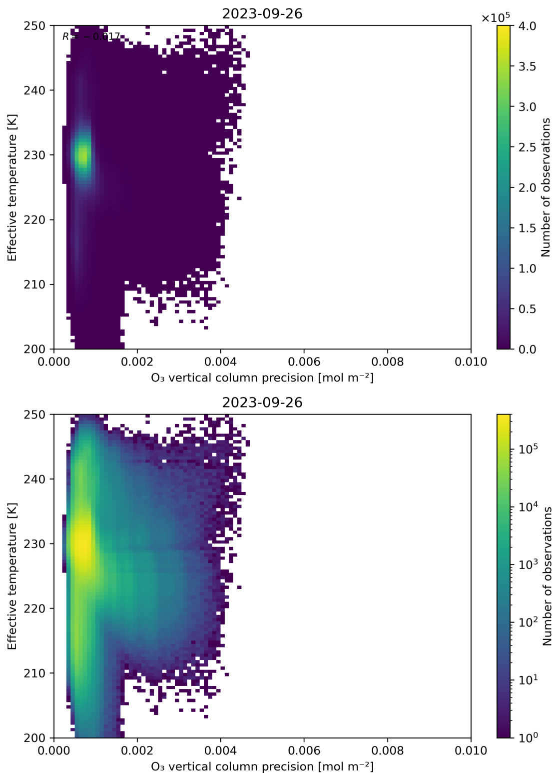
Figure 42: Scatter density plot of “O 3 vertical column precision” against “Effective temperature” for 2023-09-26 to 2023-09-27.
