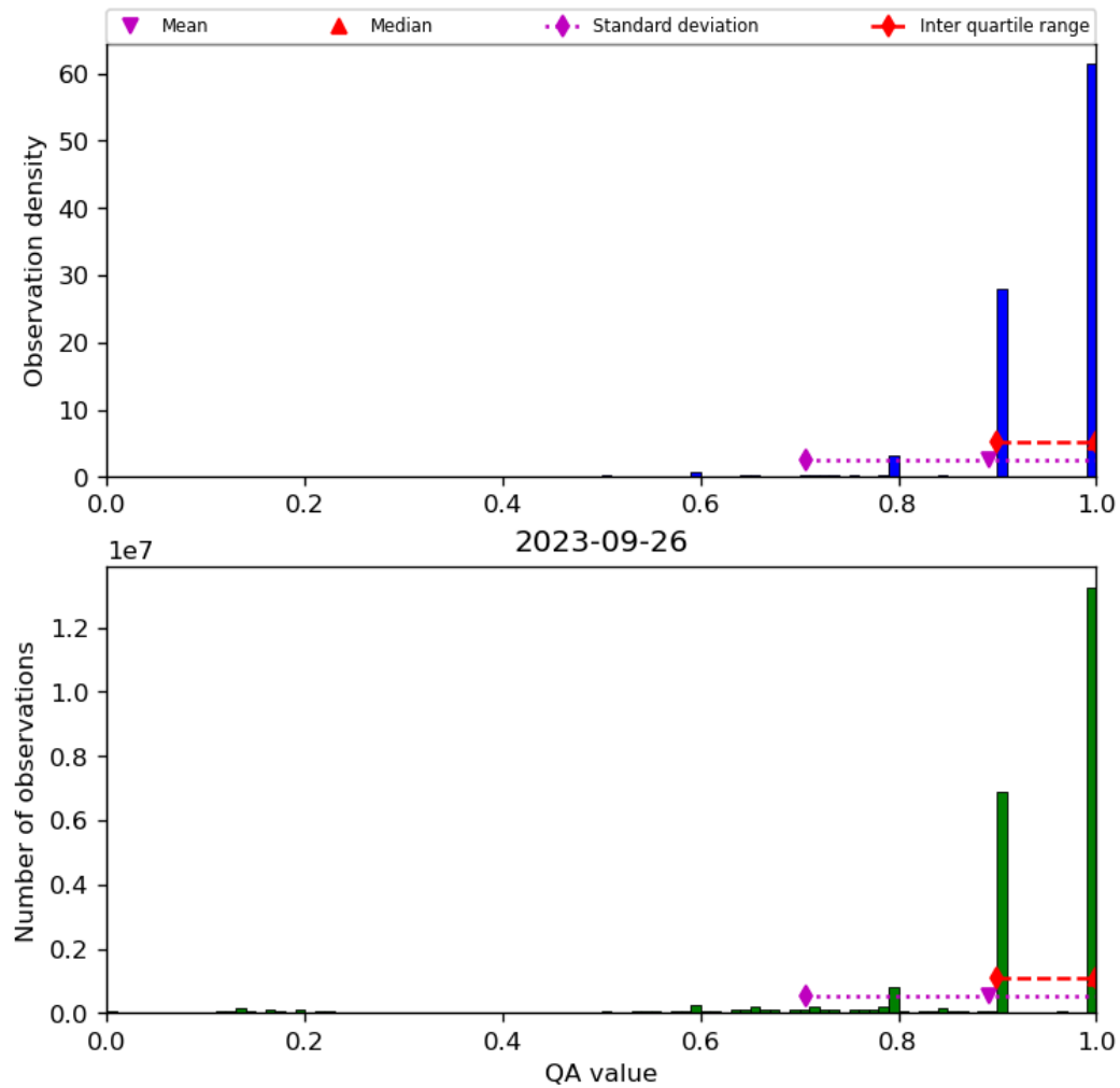
Figure 20: Histogram of “QA value” for 2023-09-26 to 2023-09-27
