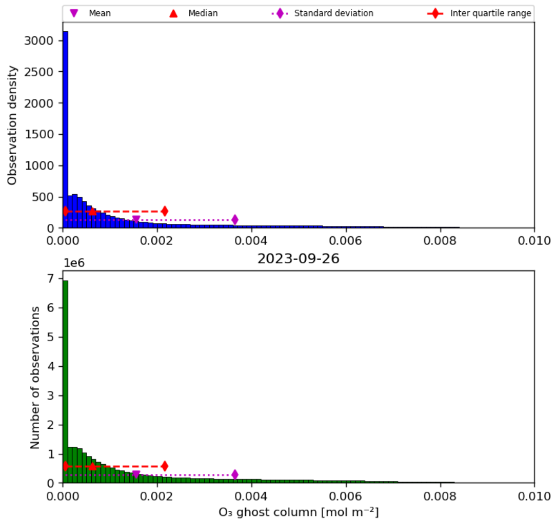
Figure 25: Histogram of “O 3 ghost column” for 2023-09-26 to 2023-09-27
