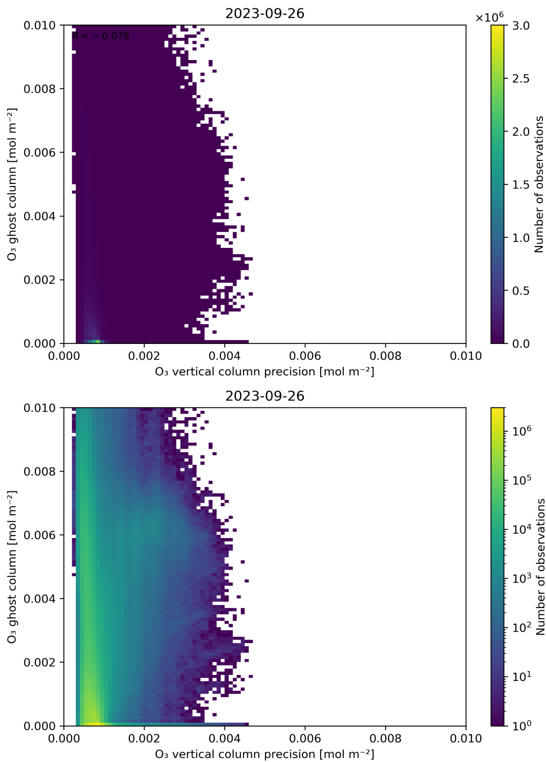
Figure 43: Scatter density plot of “ \text{O}_3 vertical column precision” against “ \text{O}_3 ghost column” for 2023-09-26 to 2023-09-27.
