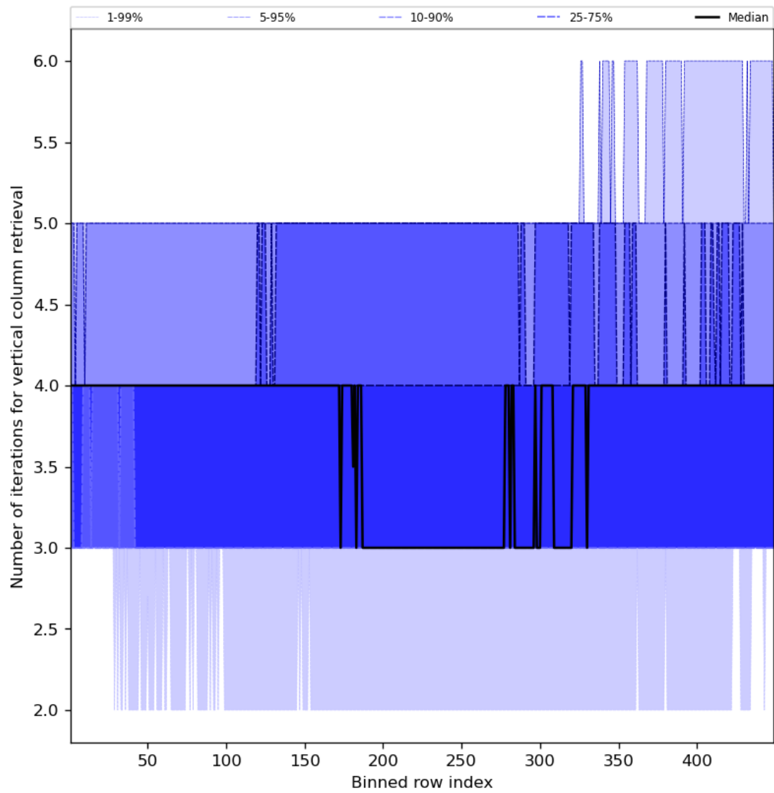
Figure 33: Along track statistics of “Number of iterations for vertical column retrieval” for 2023-09-26 to 2023-09-27
