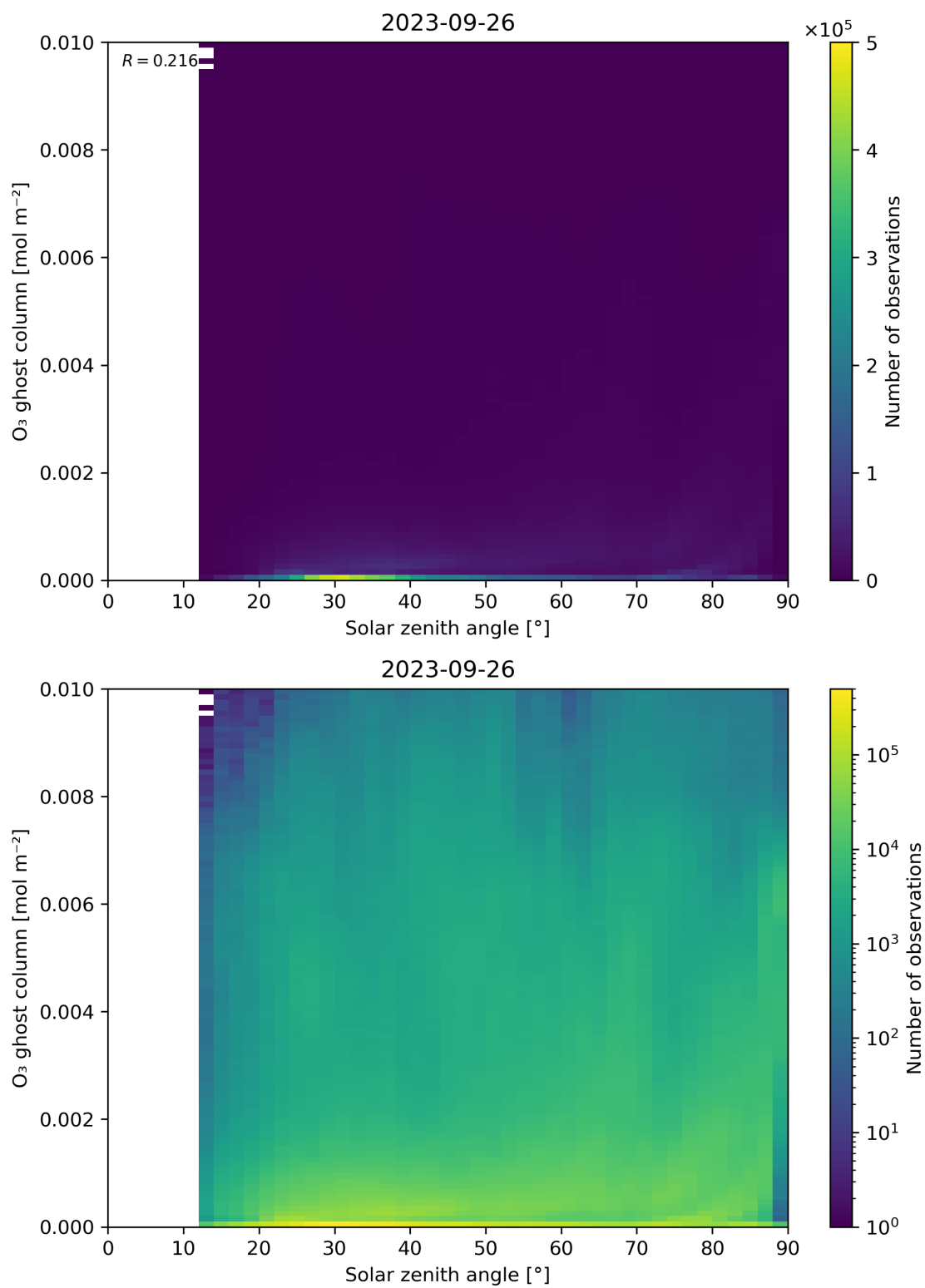
Figure 46: Scatter density plot of “Solar zenith angle” against “O 3 ghost column” for 2023-09-26 to 2023-09-27.
