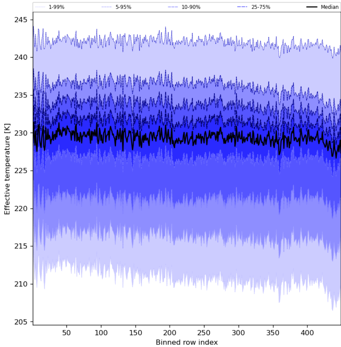
Figure 31: Along track statistics of “Effective temperature” for 2023-09-26 to 2023-09-27
