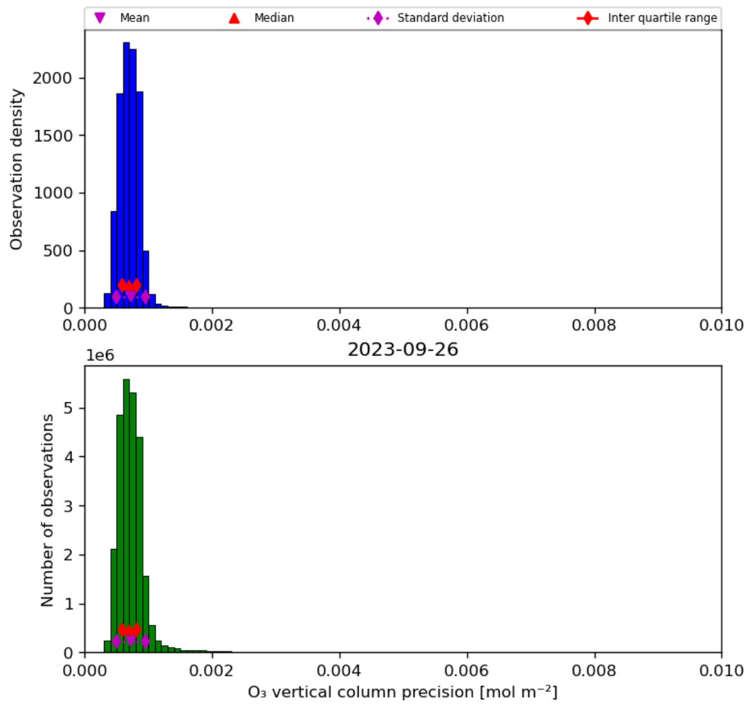
Figure 22: Histogram of “O 3 vertical column precision” for 2023-09-26 to 2023-09-27
