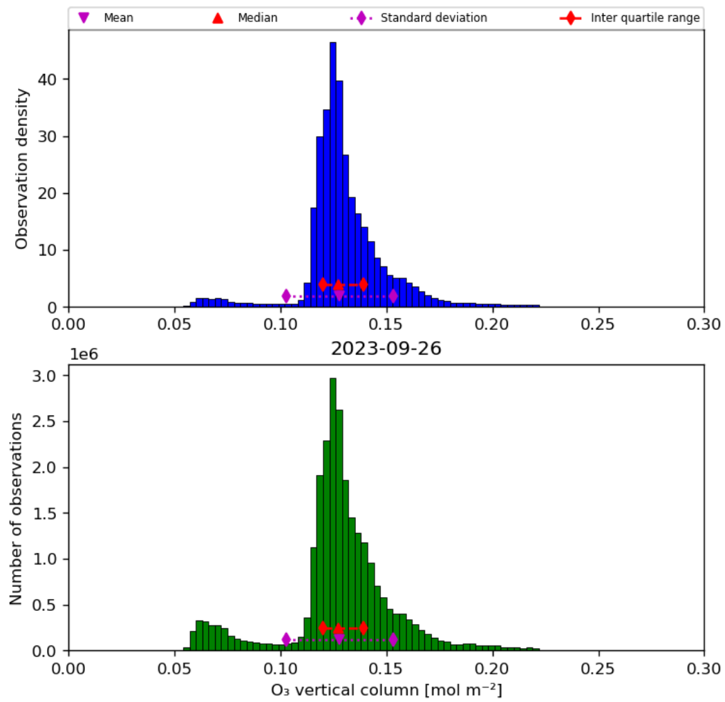
Figure 21: Histogram of “O 3 vertical column” for 2023-09-26 to 2023-09-27
