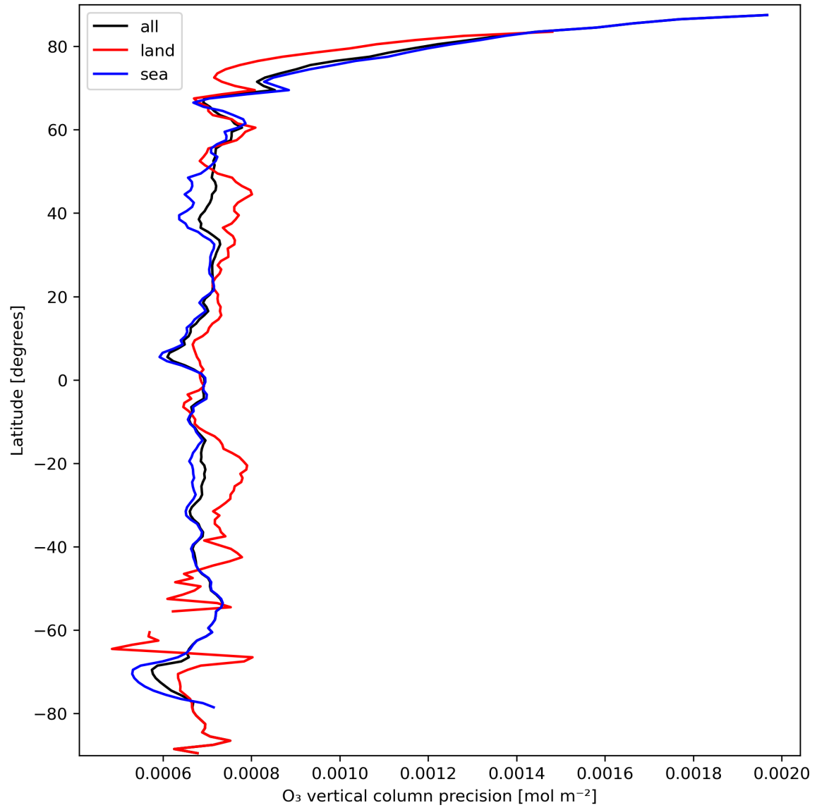
Figure 15: Zonal average of “O 3 vertical column precision” for 2023-09-26 to 2023-09-27.
