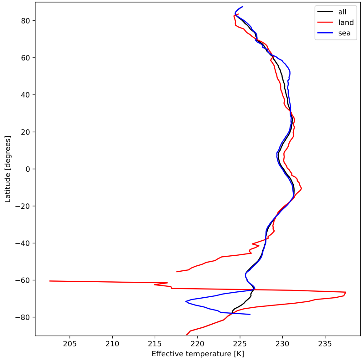
Figure 17: Zonal average of “Effective temperature” for 2023-09-26 to 2023-09-27.
