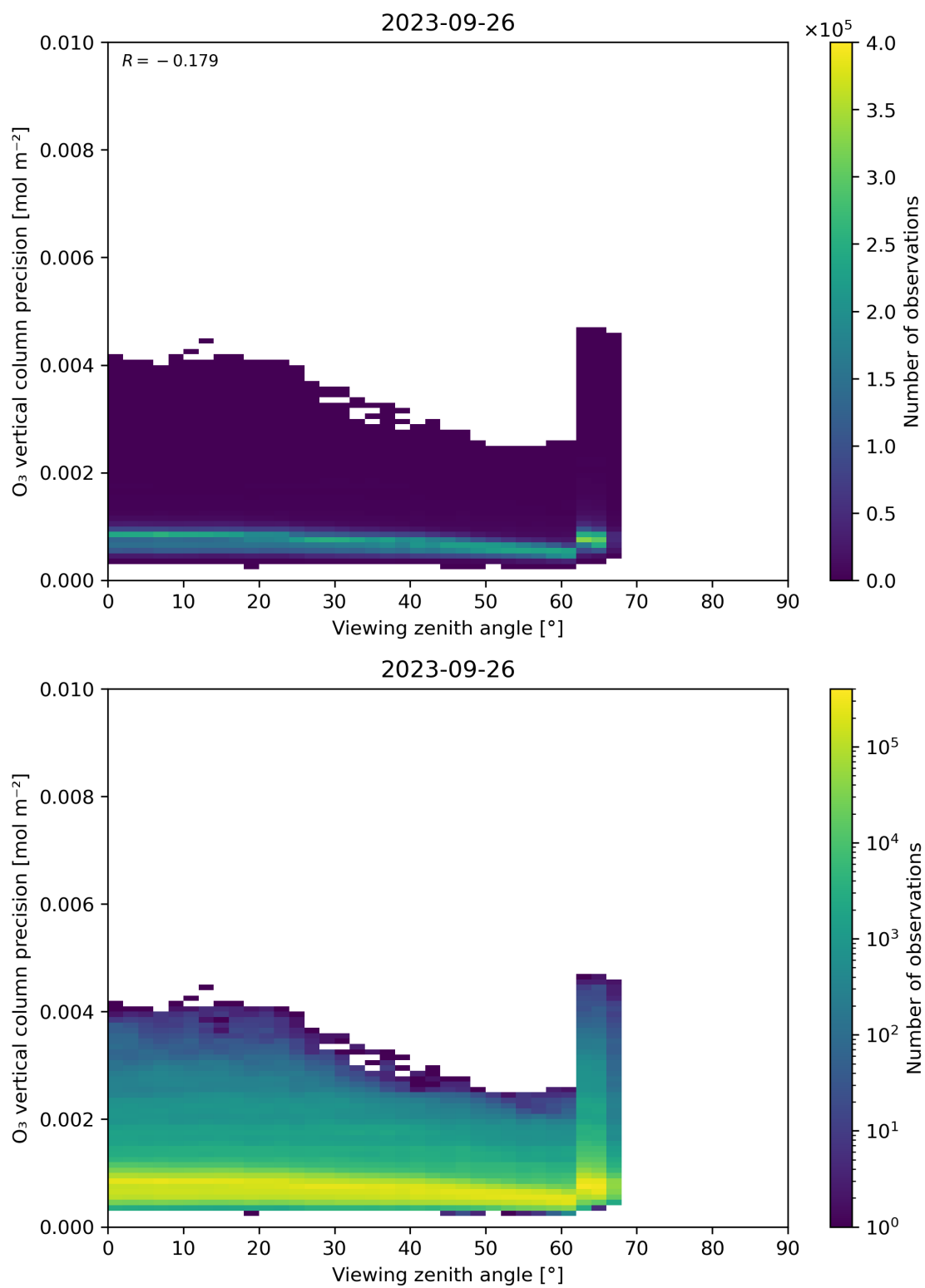
Figure 53: Scatter density plot of “Viewing zenith angle” against “O 3 vertical column precision” for 2023-09-26 to 2023-09-27.
