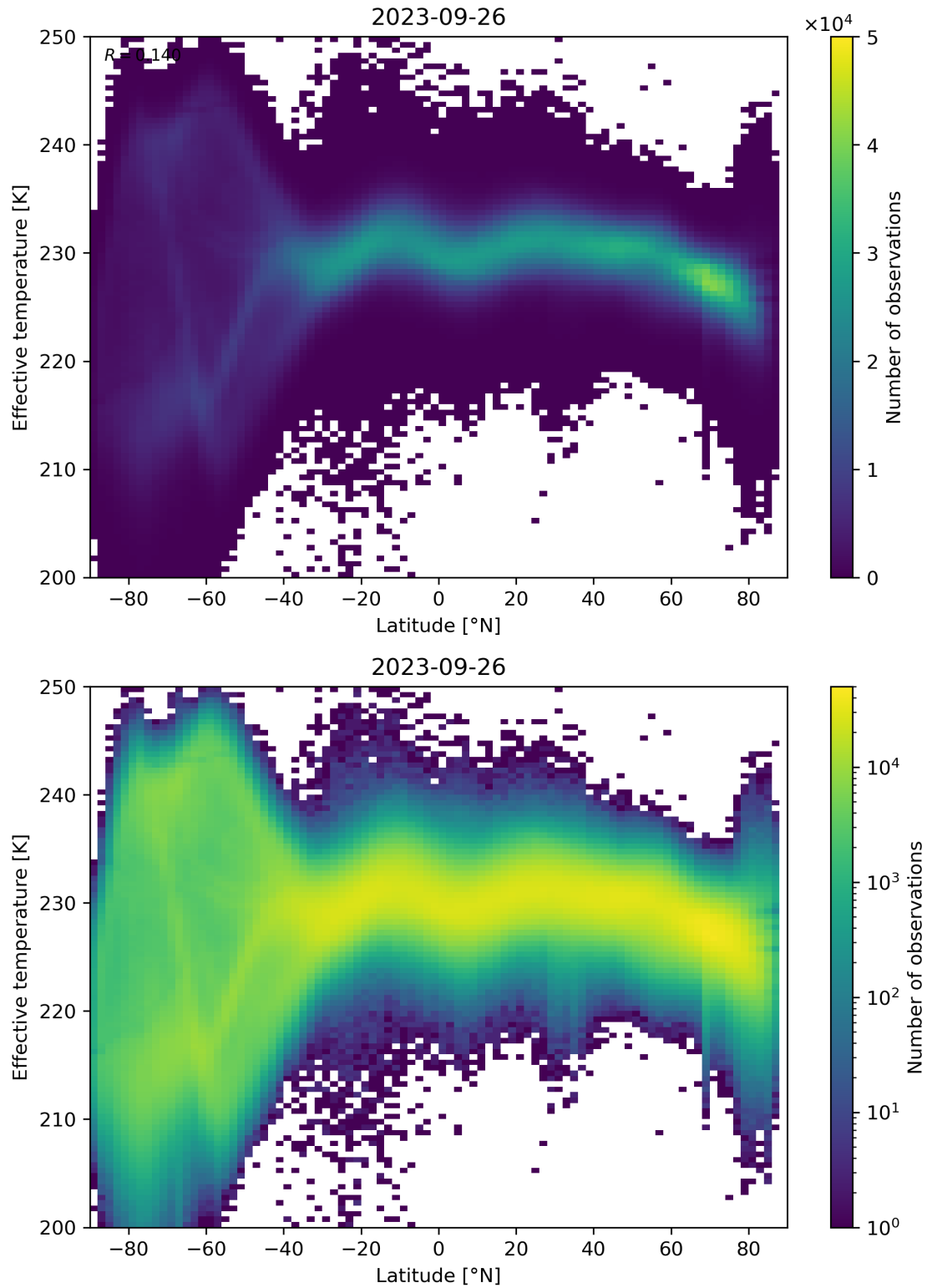
Figure 34: Scatter density plot of “Latitude” against “Effective temperature” for 2023-09-26 to 2023-09-27.
