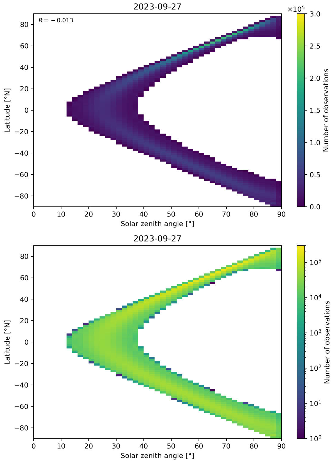
Figure 44: Scatter density plot of “Solar zenith angle” against “Latitude” for 2023-09-26 to 2023-09-28.
