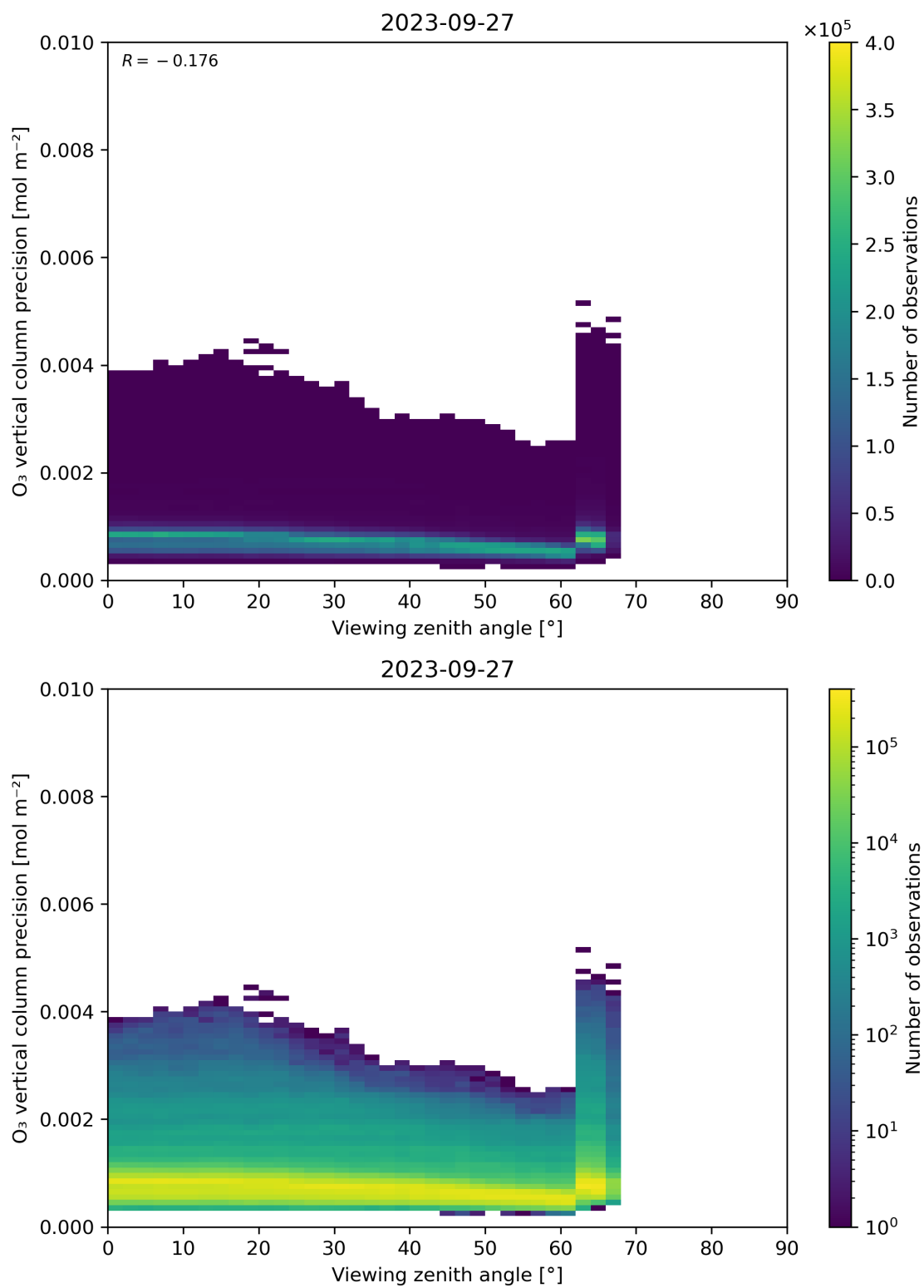
Figure 53: Scatter density plot of “Viewing zenith angle” against “O 3 vertical column precision” for 2023-09-26 to 2023-09-28.
