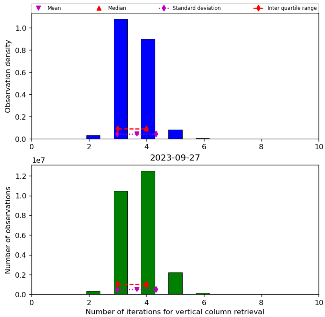
Figure 26: Histogram of “Number of iterations for vertical column retrieval” for 2023-09-26 to 2023-09-28
