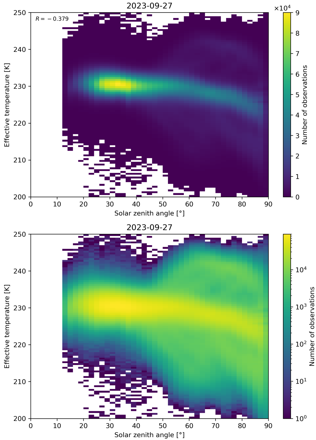
Figure 45: Scatter density plot of “Solar zenith angle” against “Effective temperature” for 2023-09-26 to 2023-09-28.
