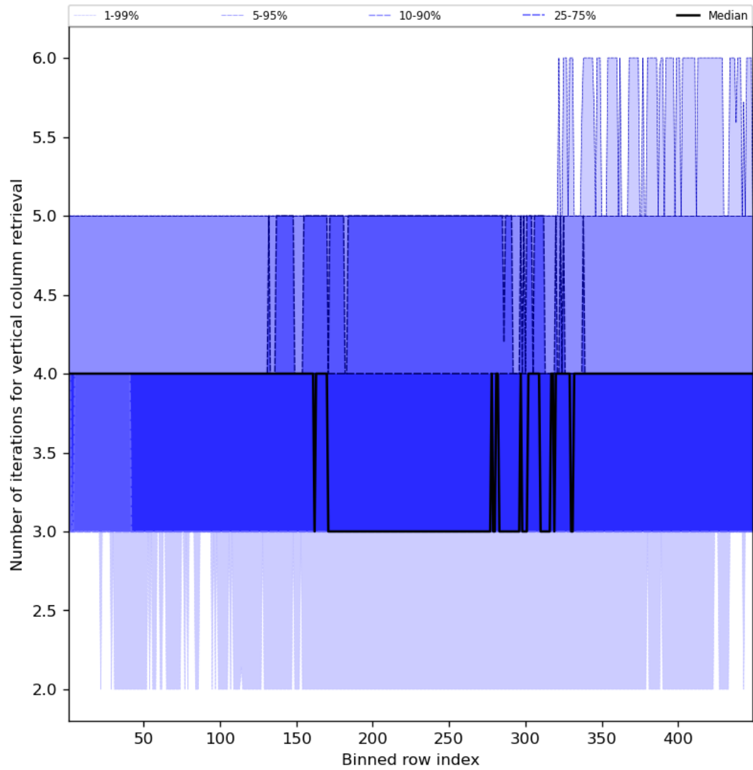
Figure 33: Along track statistics of “Number of iterations for vertical column retrieval” for 2023-09-26 to 2023-09-28
