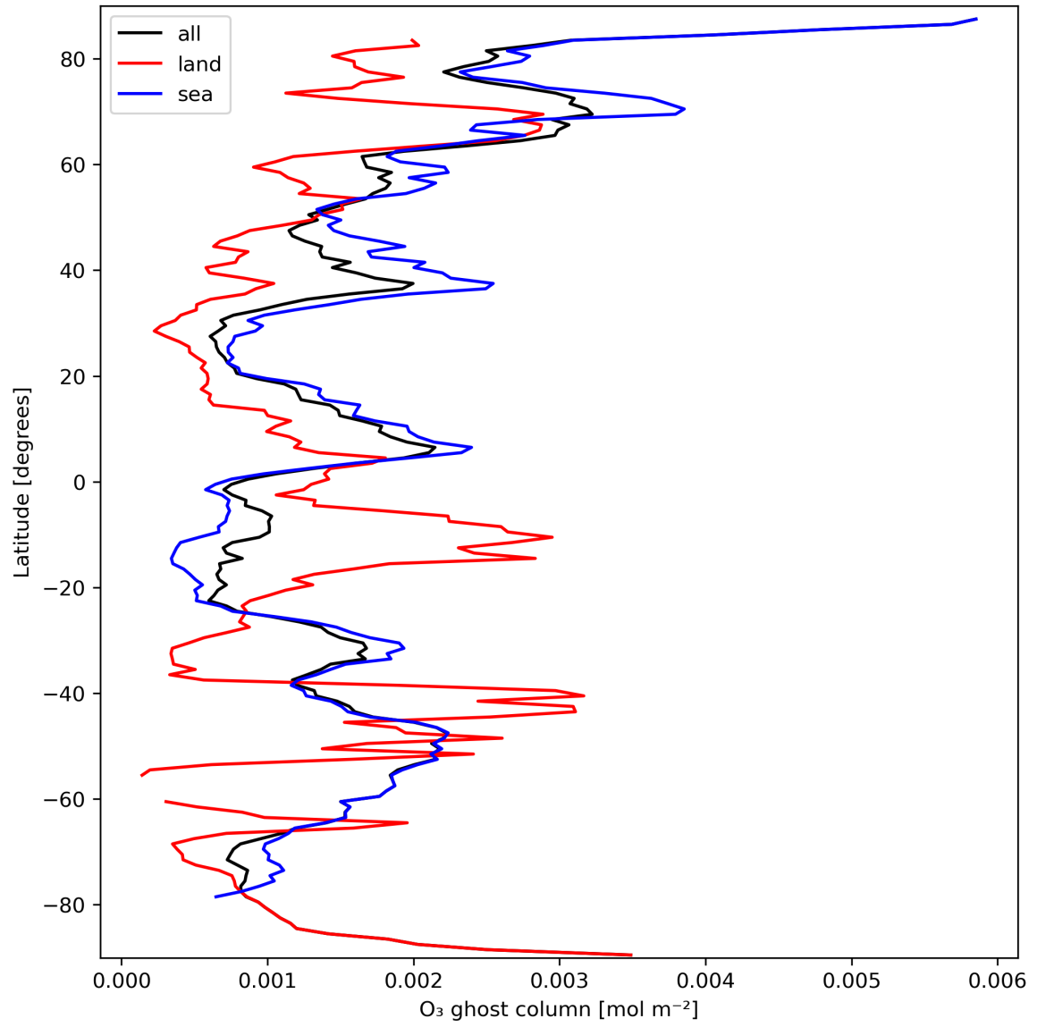
Figure 18: Zonal average of "O 3 ghost column" for 2023-09-26 to 2023-09-28.
