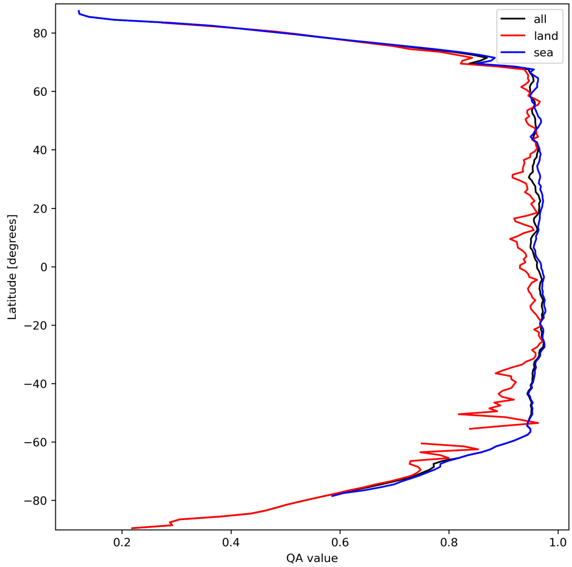
Figure 13: Zonal average of “QA value” for 2023-09-26 to 2023-09-28.
