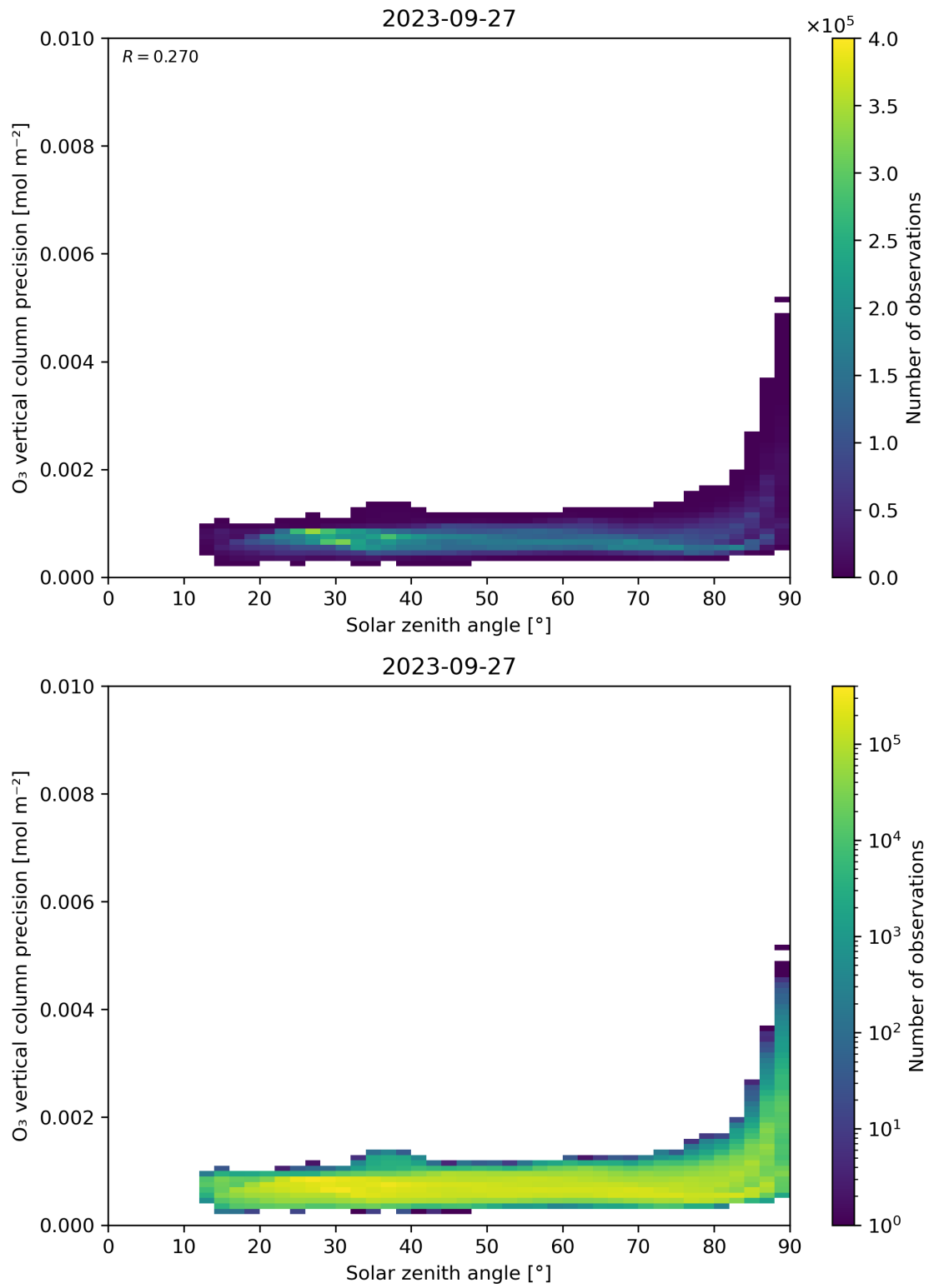
Figure 48: Scatter density plot of “Solar zenith angle” against “O 3 vertical column precision” for 2023-09-26 to 2023-09-28.
