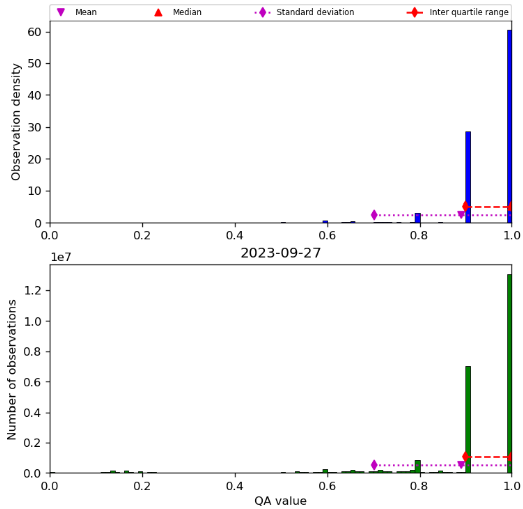
Figure 20: Histogram of “QA value” for 2023-09-26 to 2023-09-28
