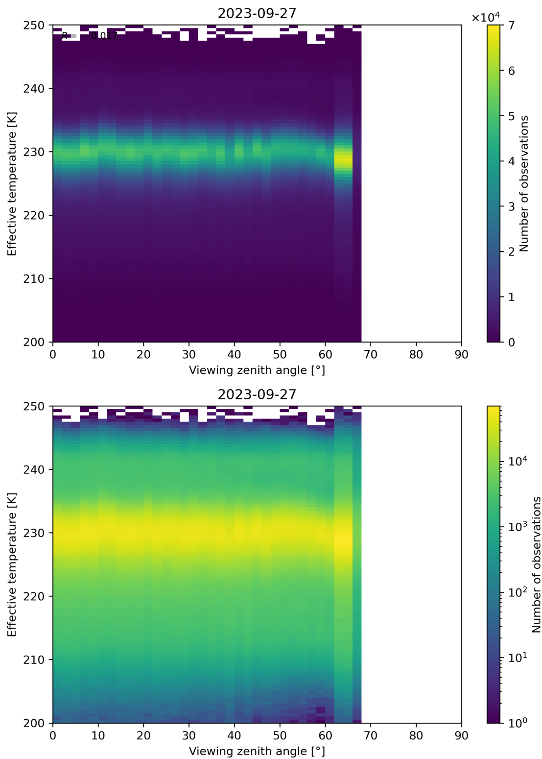
Figure 50: Scatter density plot of “Viewing zenith angle” against “Effective temperature” for 2023-09-26 to 2023-09-28.
