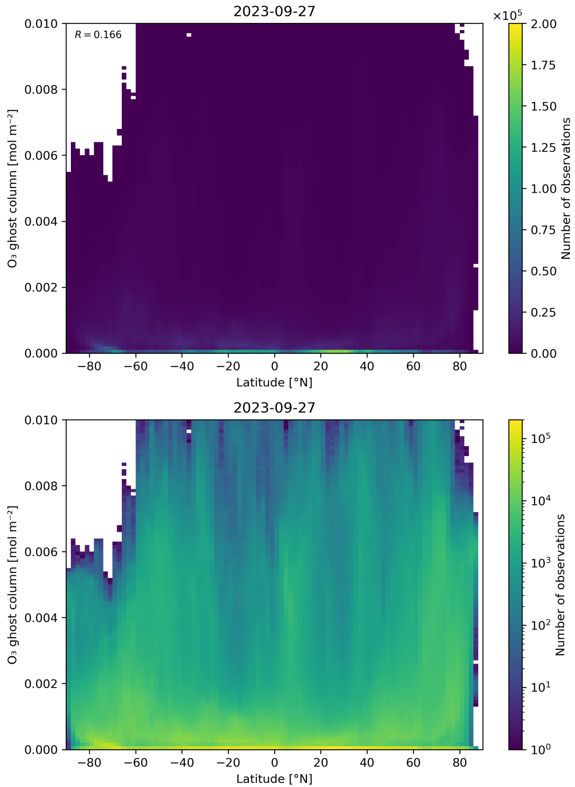
Figure 35: Scatter density plot of “Latitude” against “O 3 ghost column” for 2023-09-26 to 2023-09-28.
