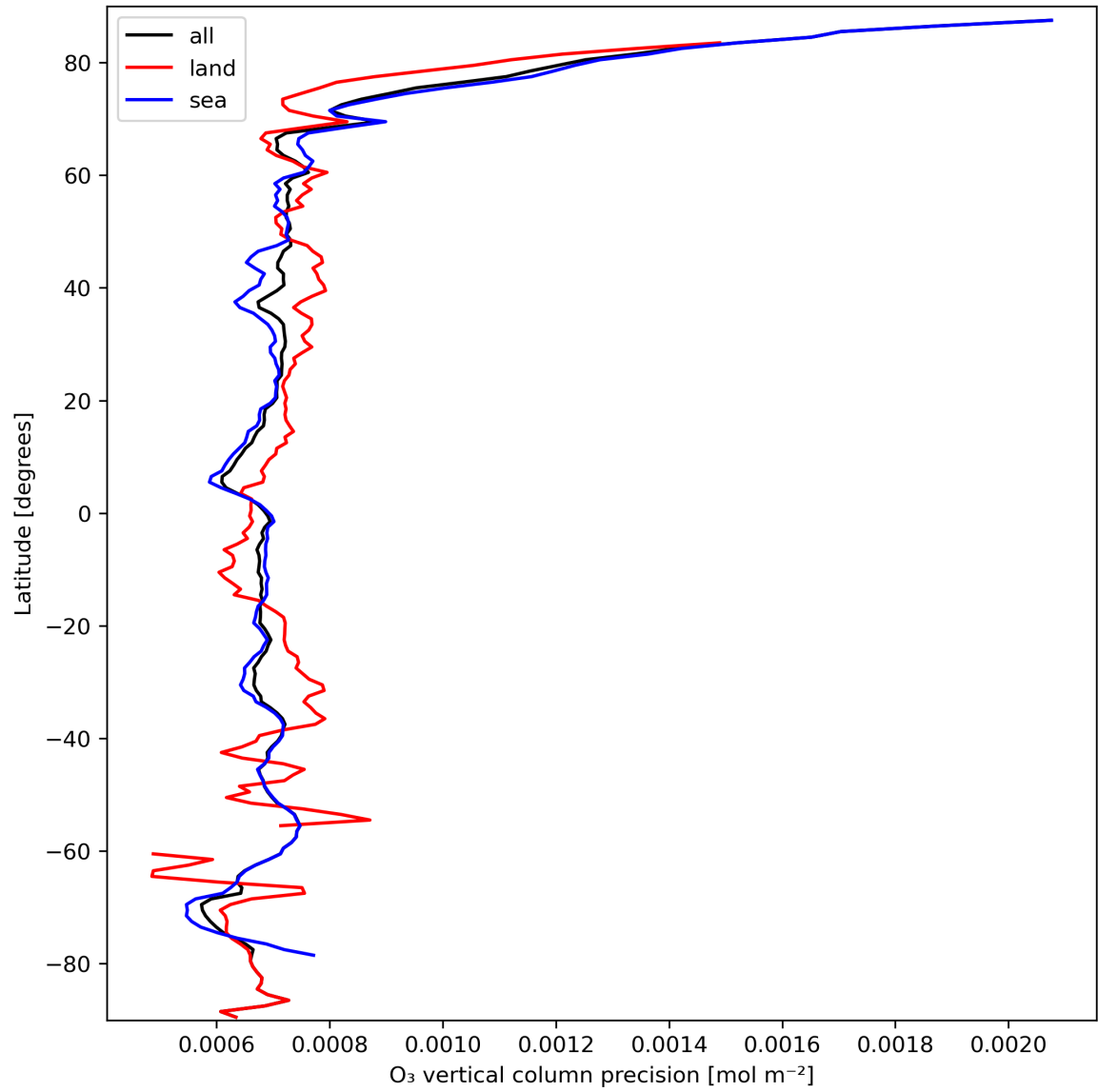
Figure 15: Zonal average of “O 3 vertical column precision” for 2023-09-26 to 2023-09-28.
