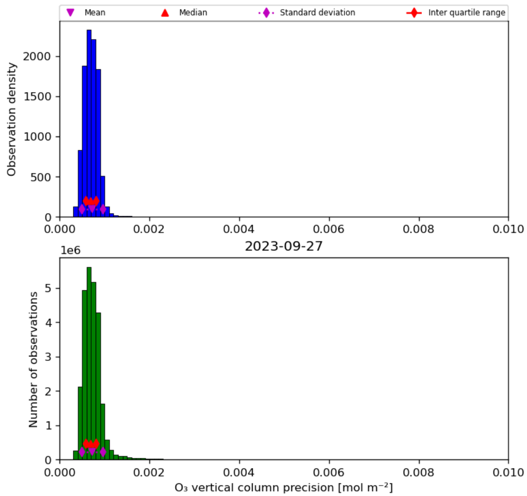
Figure 22: Histogram of “O 3 vertical column precision” for 2023-09-26 to 2023-09-28
