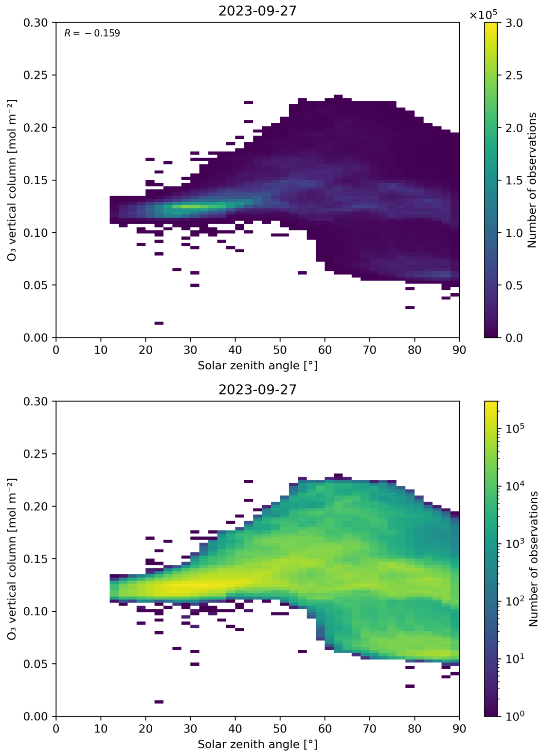
Figure 47: Scatter density plot of “Solar zenith angle” against “O 3 vertical column” for 2023-09-26 to 2023-09-28.
