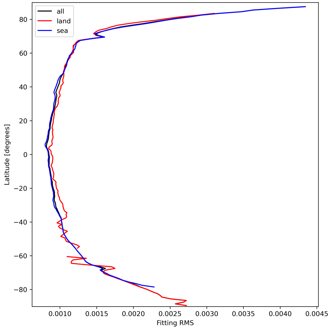
Figure 16: Zonal average of “Fitting RMS” for 2023-09-26 to 2023-09-28.
