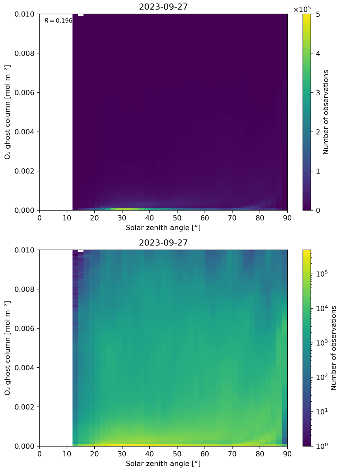
Figure 46: Scatter density plot of “Solar zenith angle” against “O 3 ghost column” for 2023-09-26 to 2023-09-28.
