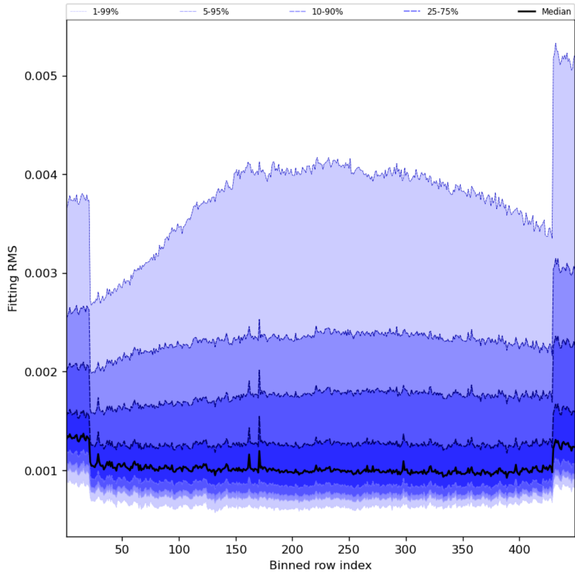
Figure 30: Along track statistics of “Fitting RMS” for 2023-09-26 to 2023-09-28
