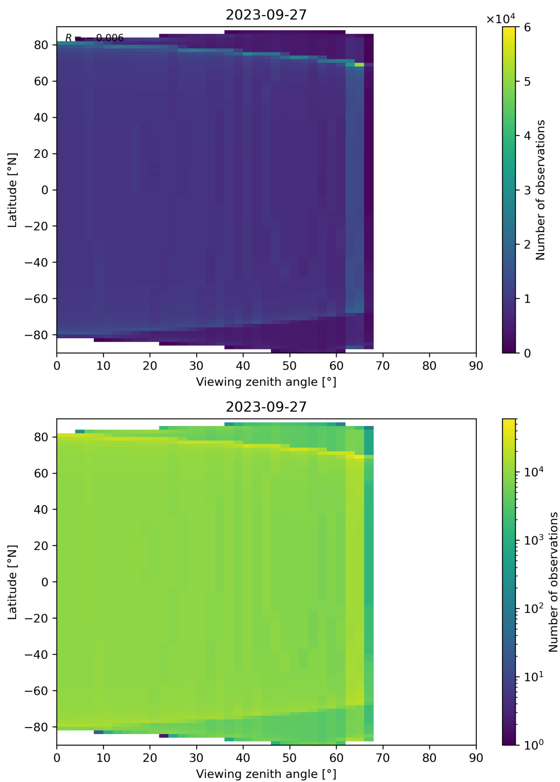
Figure 49: Scatter density plot of “Viewing zenith angle” against “Latitude” for 2023-09-26 to 2023-09-28.
