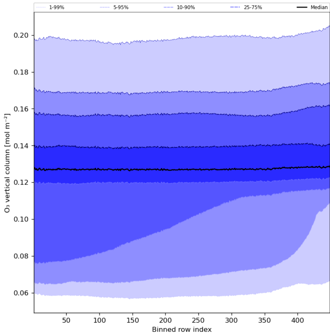
Figure 28: Along track statistics of “O 3 vertical column” for 2023-09-26 to 2023-09-28
