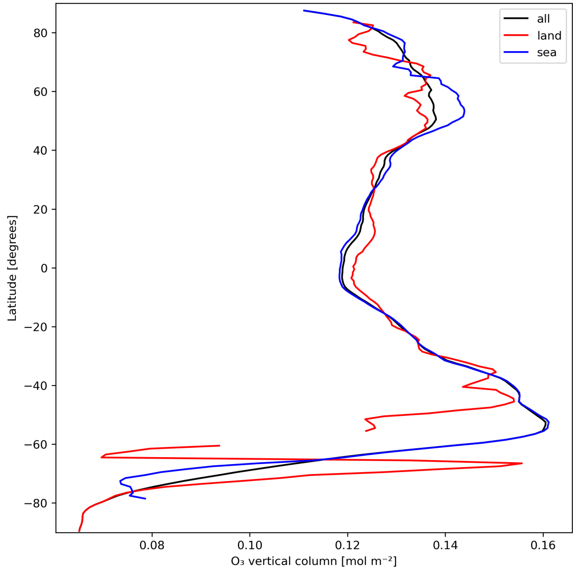
Figure 14: Zonal average of “O 3 vertical column” for 2023-09-26 to 2023-09-28.
