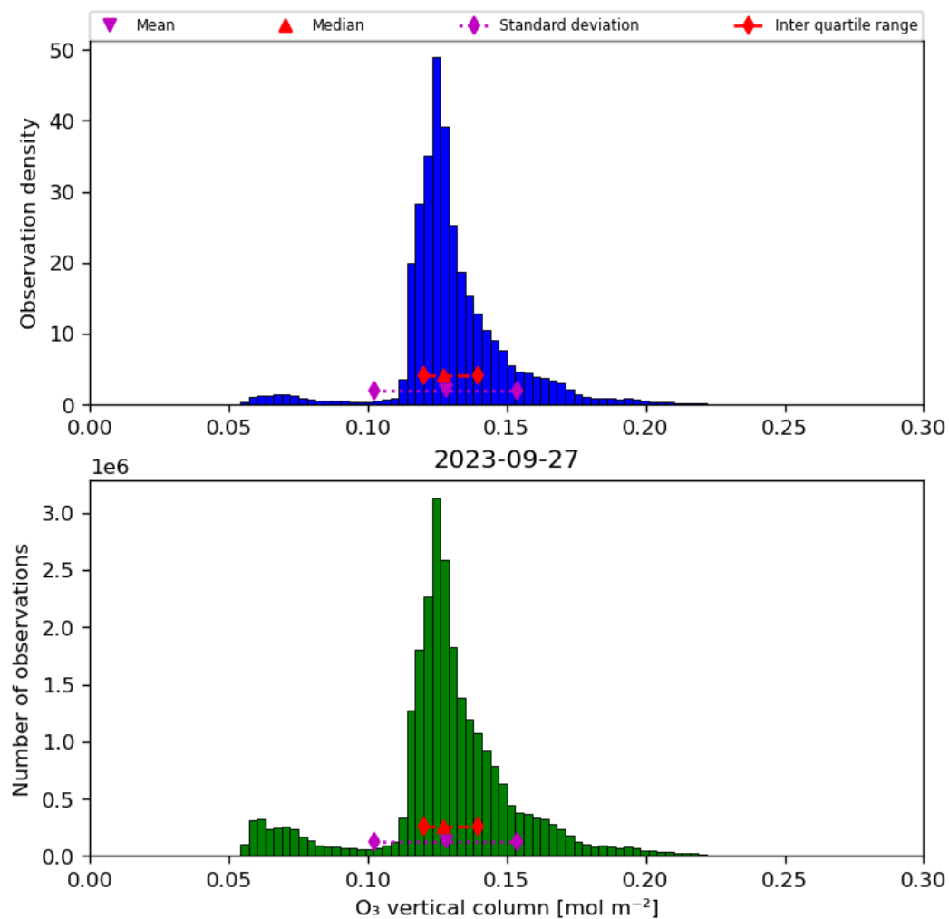
Figure 21: Histogram of “O 3 vertical column” for 2023-09-26 to 2023-09-28
