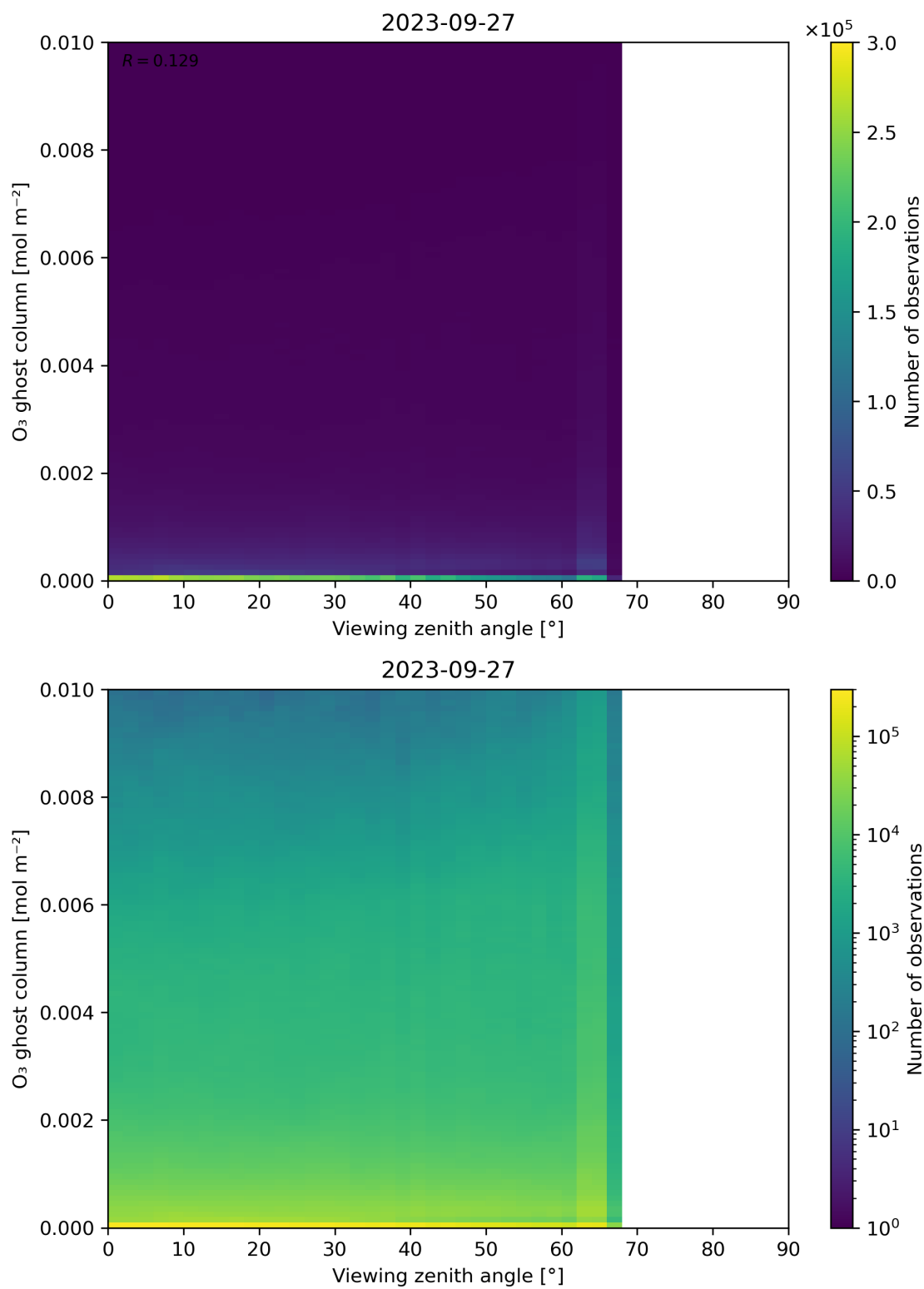
Figure 51: Scatter density plot of “Viewing zenith angle” against “O 3 ghost column” for 2023-09-26 to 2023-09-28.
