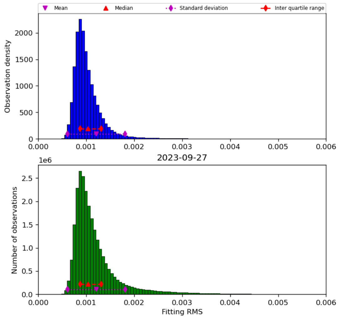
Figure 23: Histogram of “Fitting RMS” for 2023-09-26 to 2023-09-28
