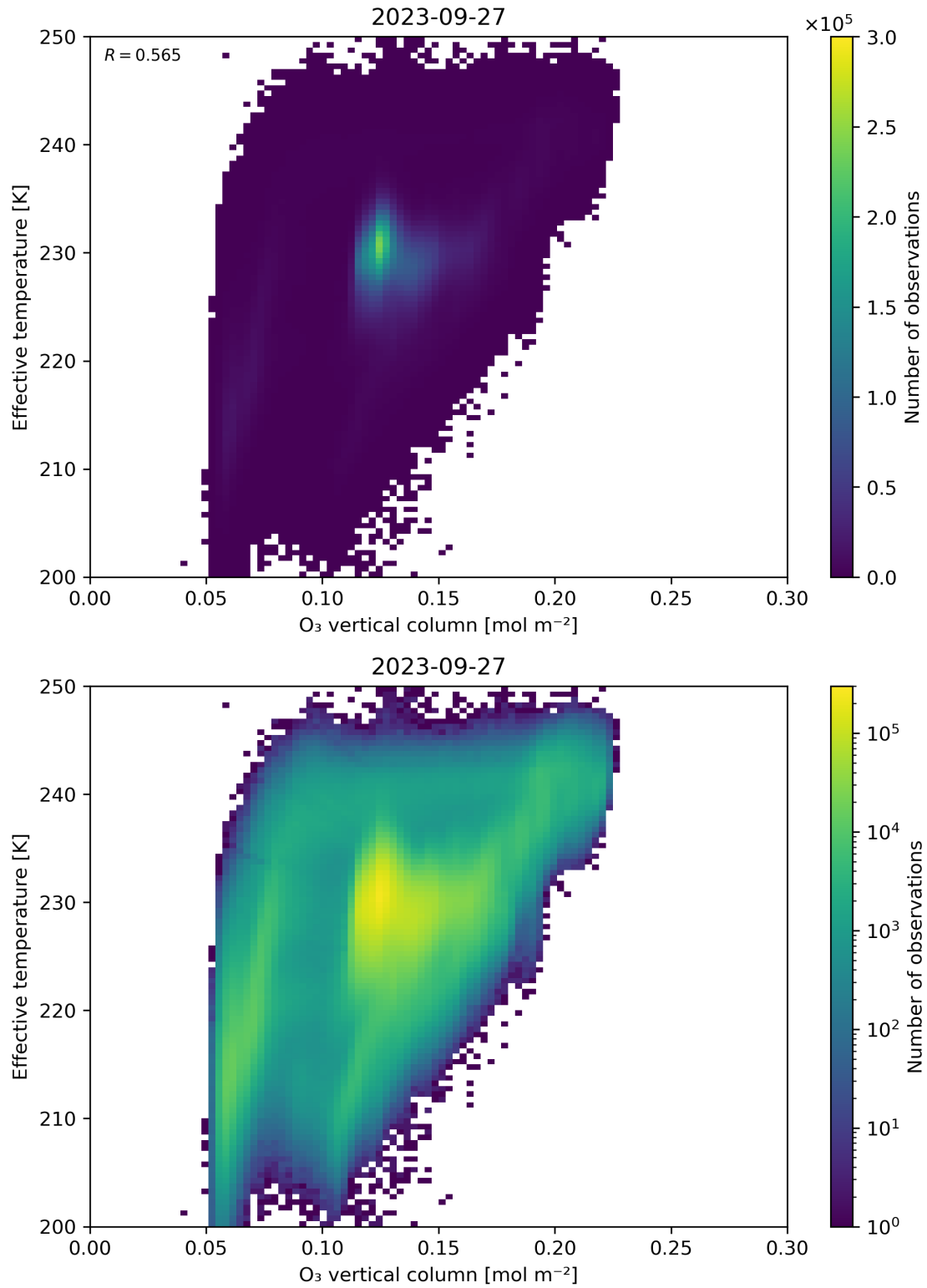
Figure 39: Scatter density plot of “O 3 vertical column” against “Effective temperature” for 2023-09-26 to 2023-09-28.
