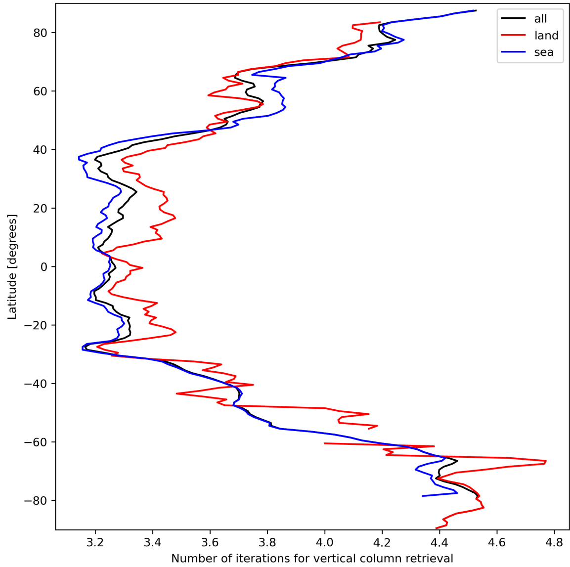
Figure 19: Zonal average of “Number of iterations for vertical column retrieval” for 2023-09-26 to 2023-09-28.
