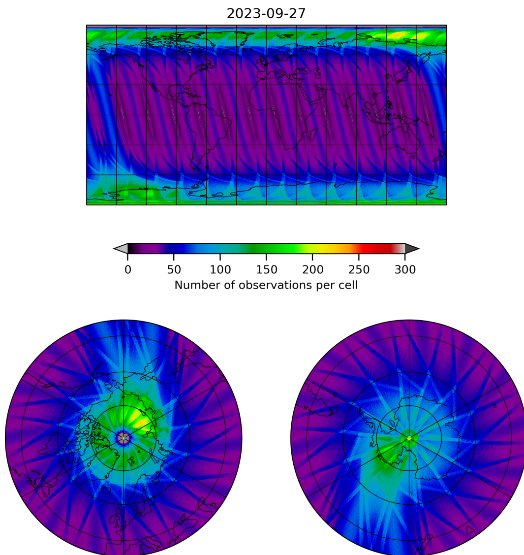
Figure 12: Map of the number of observations for 2023-09-26 to 2023-09-28
