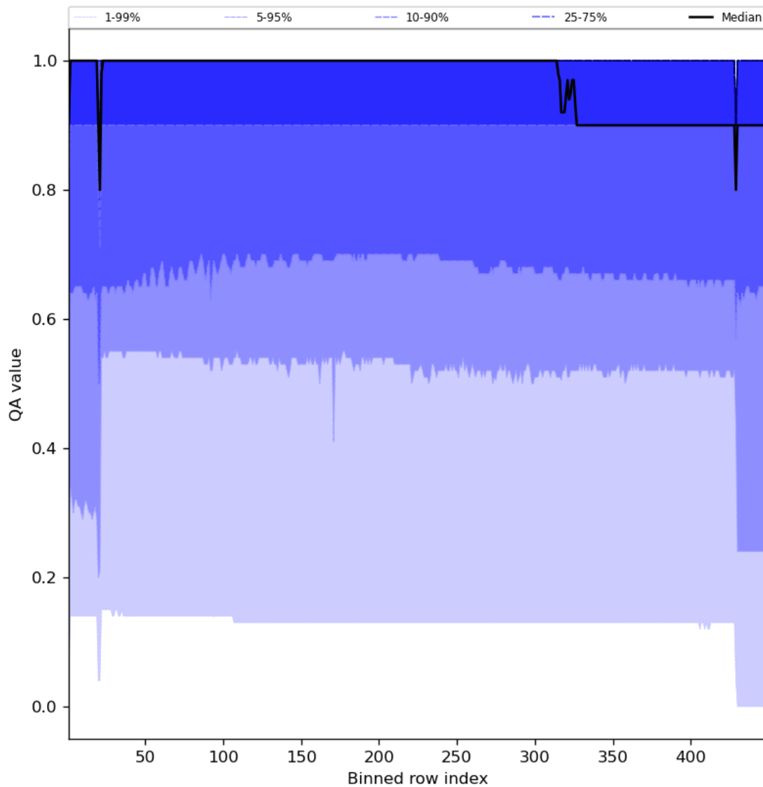
Figure 27: Along track statistics of “QA value” for 2023-09-26 to 2023-09-28
