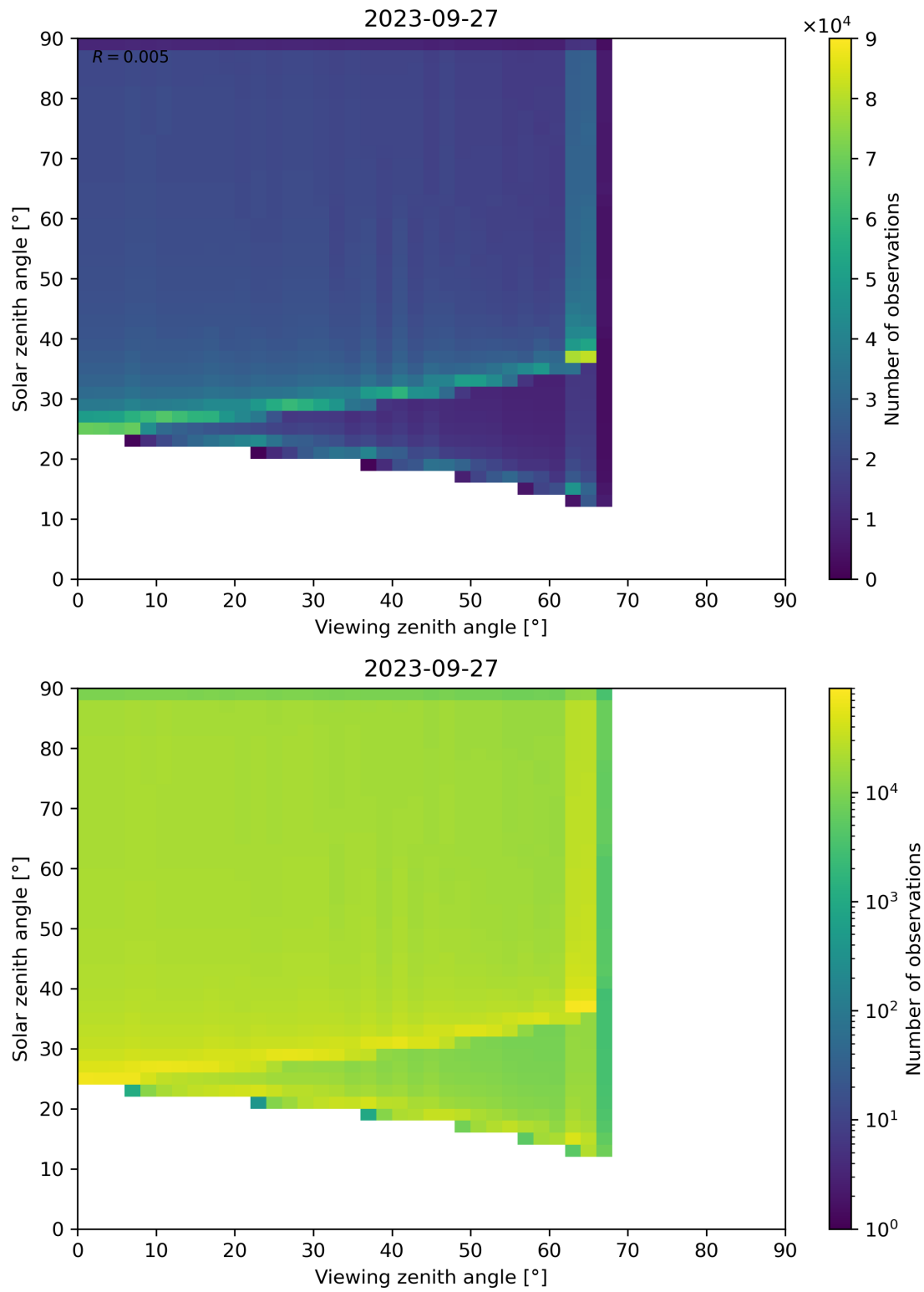
Figure 54: Scatter density plot of “Viewing zenith angle” against “Solar zenith angle” for 2023-09-26 to 2023-09-28.
