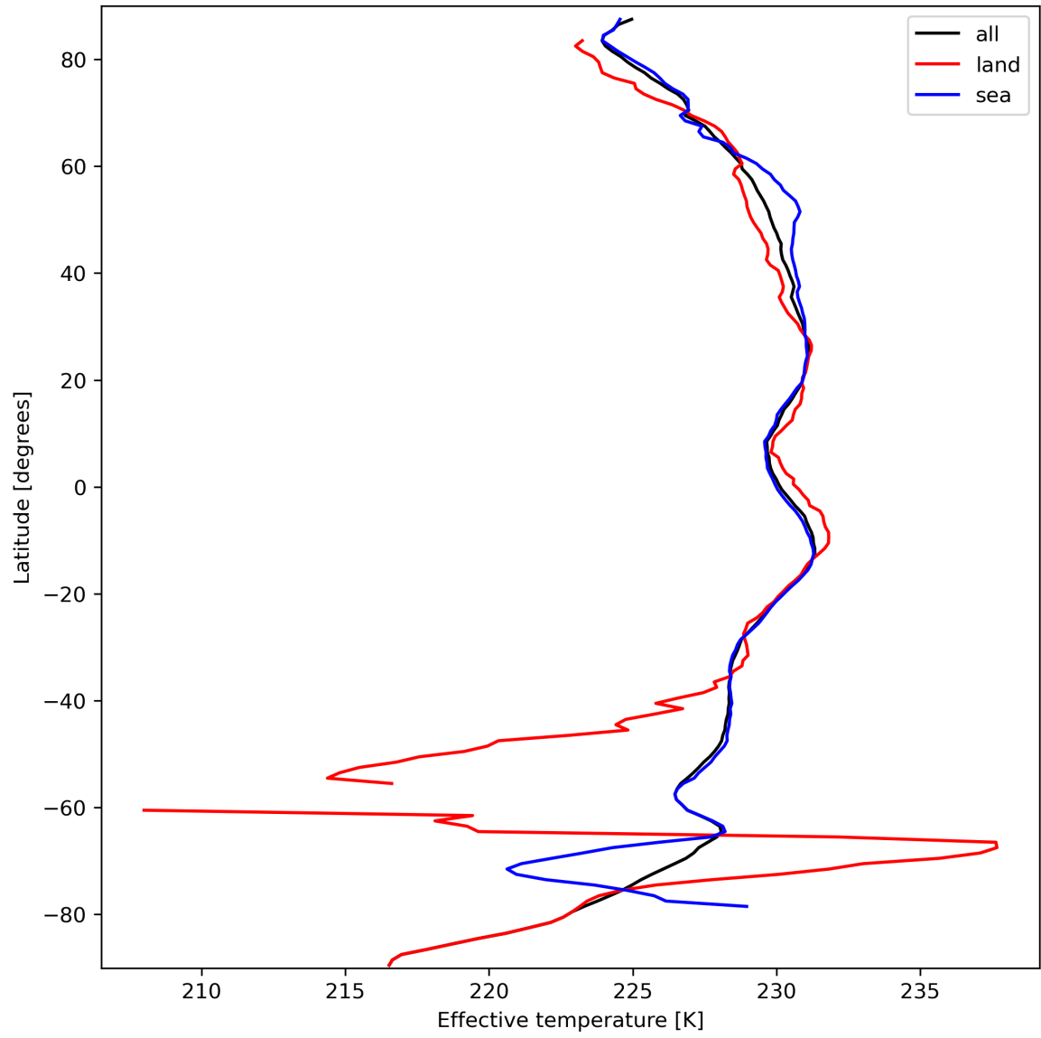
Figure 17: Zonal average of "Effective temperature" for 2023-09-26 to 2023-09-28.
