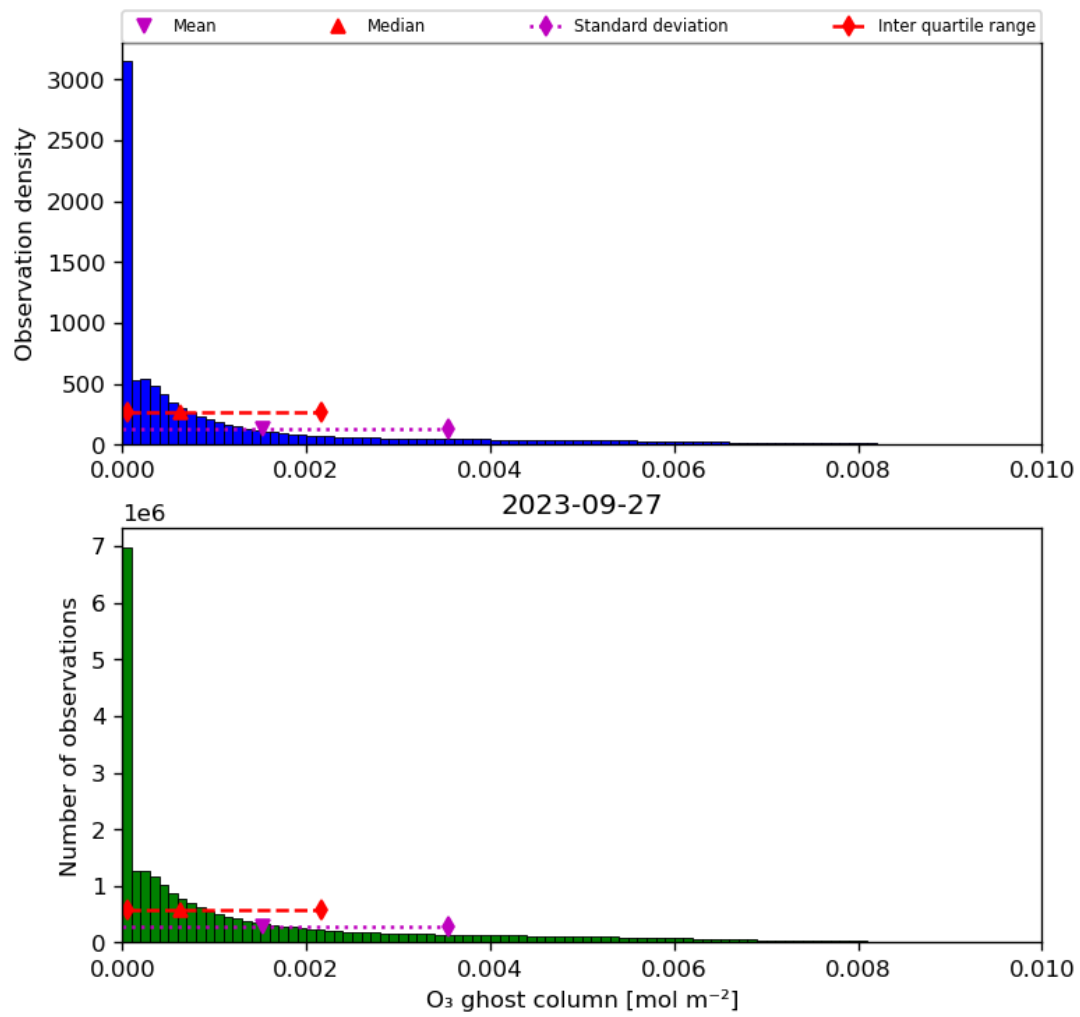
Figure 25: Histogram of “O 3 ghost column” for 2023-09-26 to 2023-09-28
