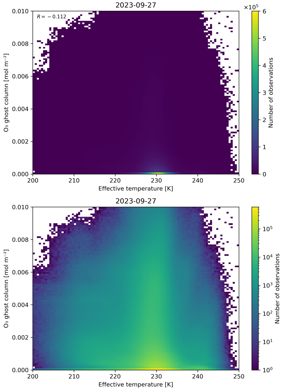
Figure 38: Scatter density plot of “Effective temperature” against “O 3 ghost column” for 2023-09-26 to 2023-09-28.
