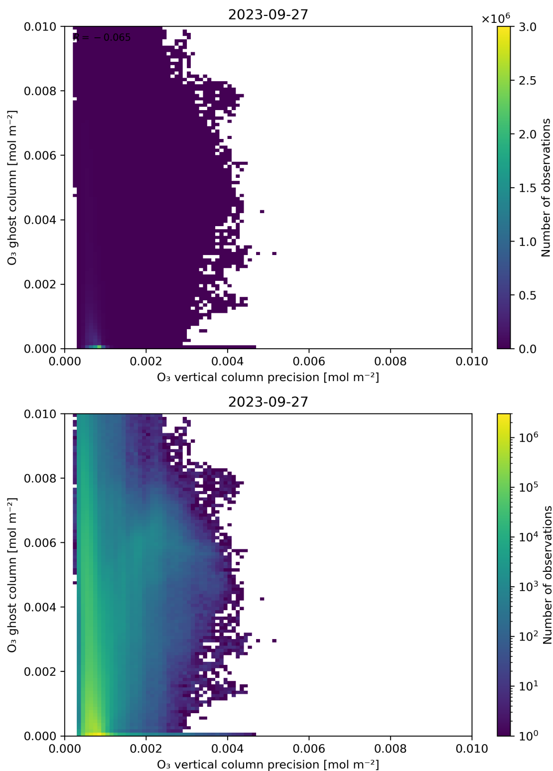
Figure 43: Scatter density plot of “ \text{O}_3 vertical column precision” against “ \text{O}_3 ghost column” for 2023-09-26 to 2023-09-28.
