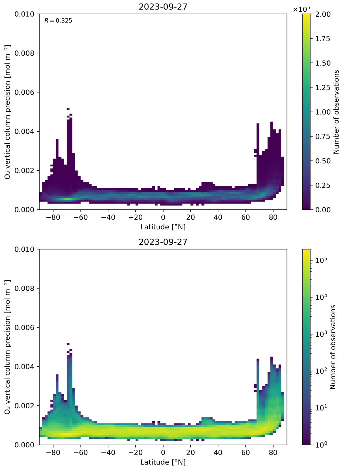
Figure 37: Scatter density plot of “Latitude” against “O 3 vertical column precision” for 2023-09-26 to 2023-09-28.
