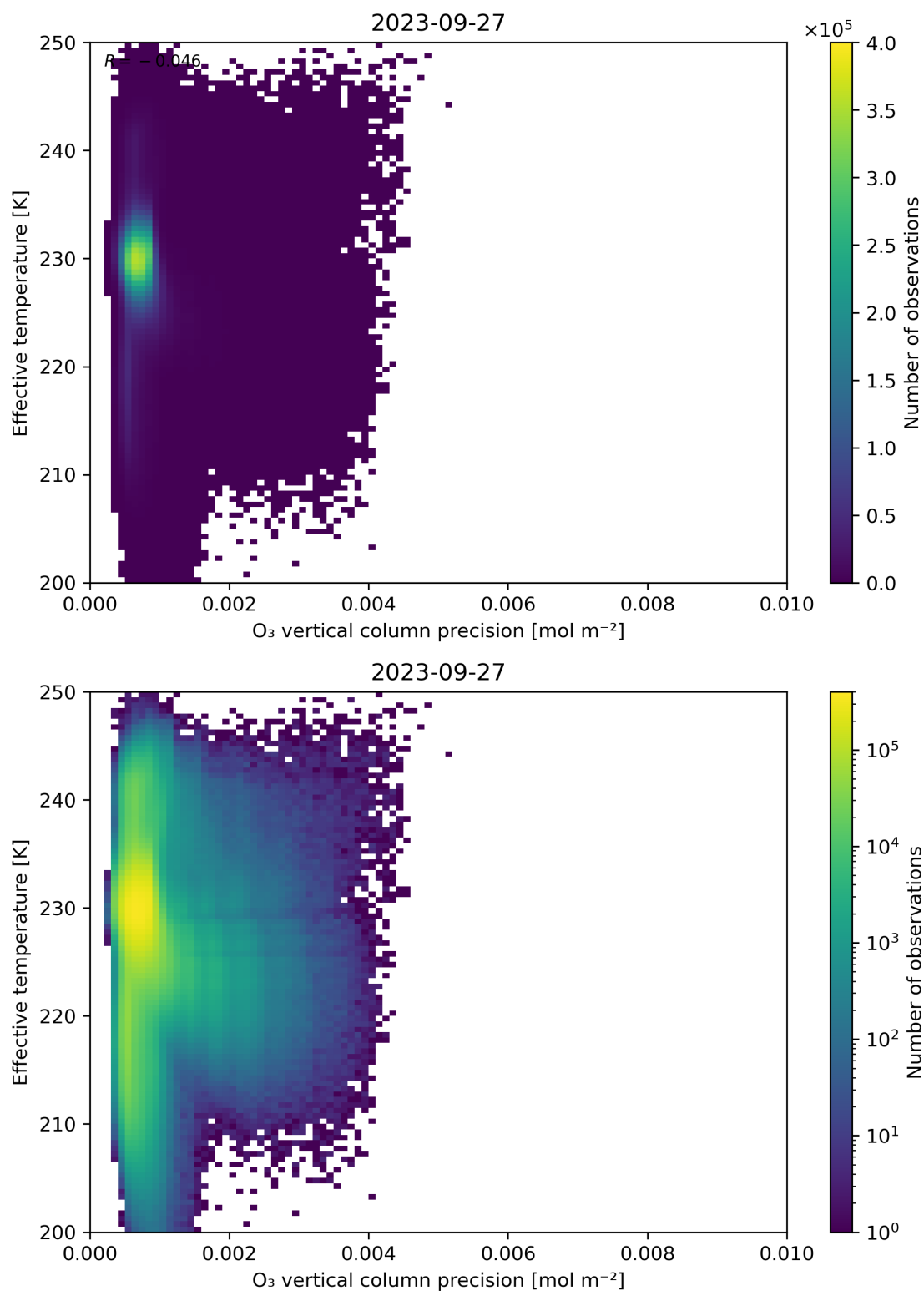
Figure 42: Scatter density plot of “O 3 vertical column precision” against “Effective temperature” for 2023-09-26 to 2023-09-28.
