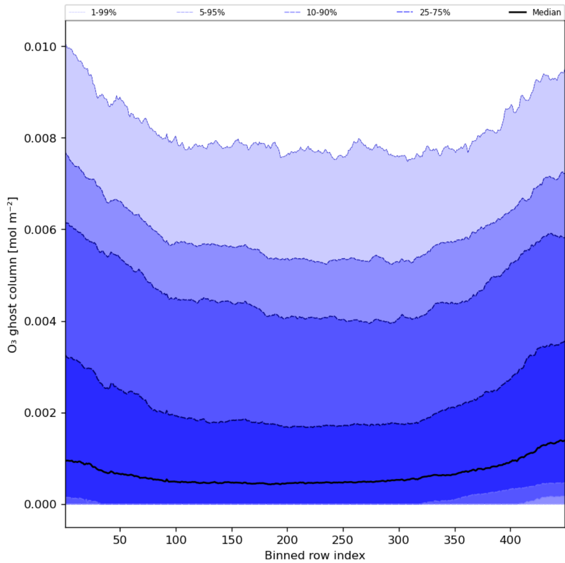
Figure 32: Along track statistics of “O 3 ghost column” for 2023-09-26 to 2023-09-28
