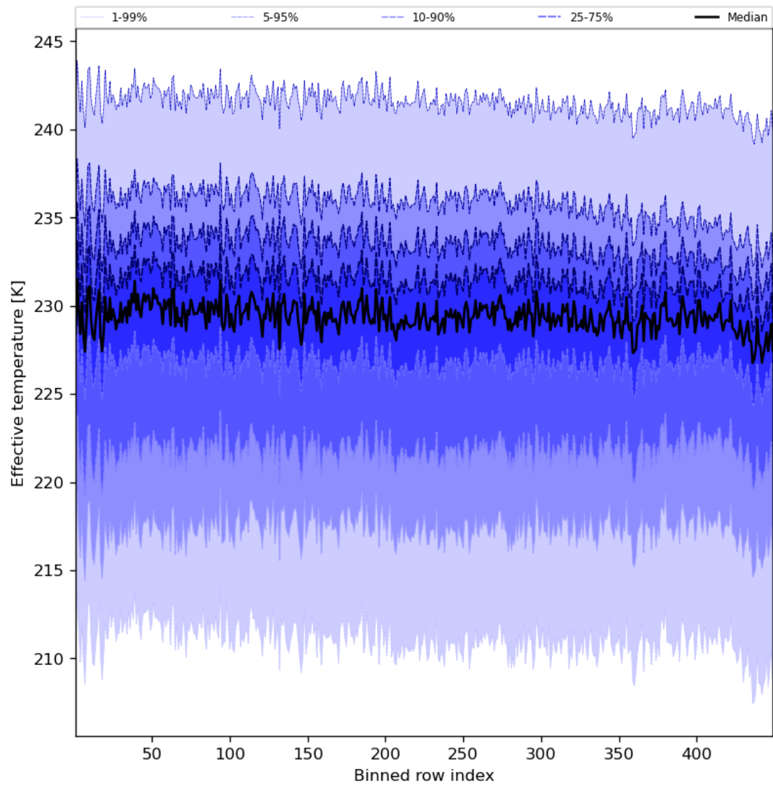
Figure 31: Along track statistics of “Effective temperature” for 2023-09-26 to 2023-09-28
