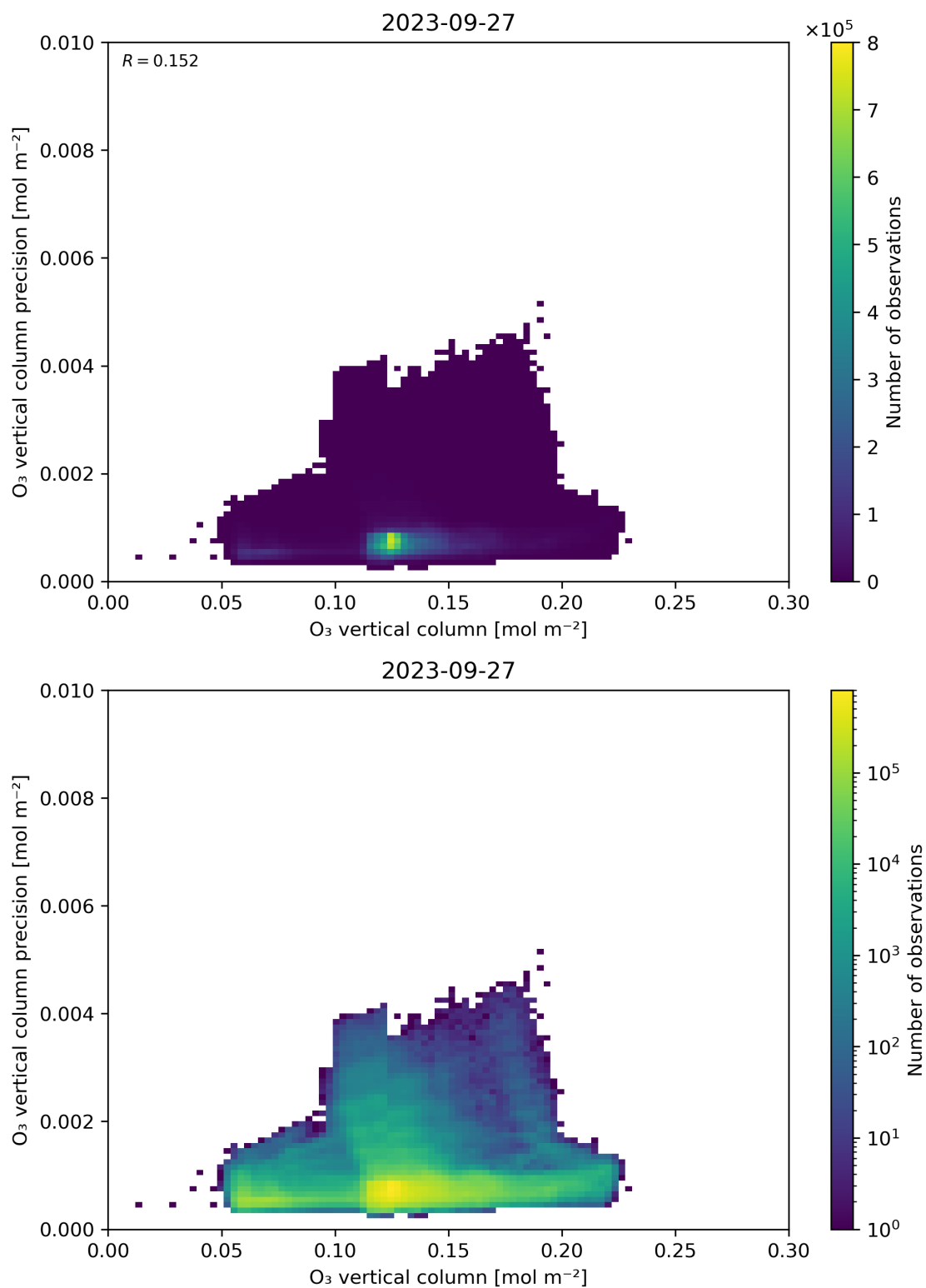
Figure 41: Scatter density plot of “O 3 vertical column” against “O 3 vertical column precision” for 2023-09-26 to 2023-09-28.
