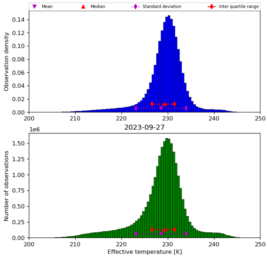
Figure 24: Histogram of “Effective temperature” for 2023-09-26 to 2023-09-28
