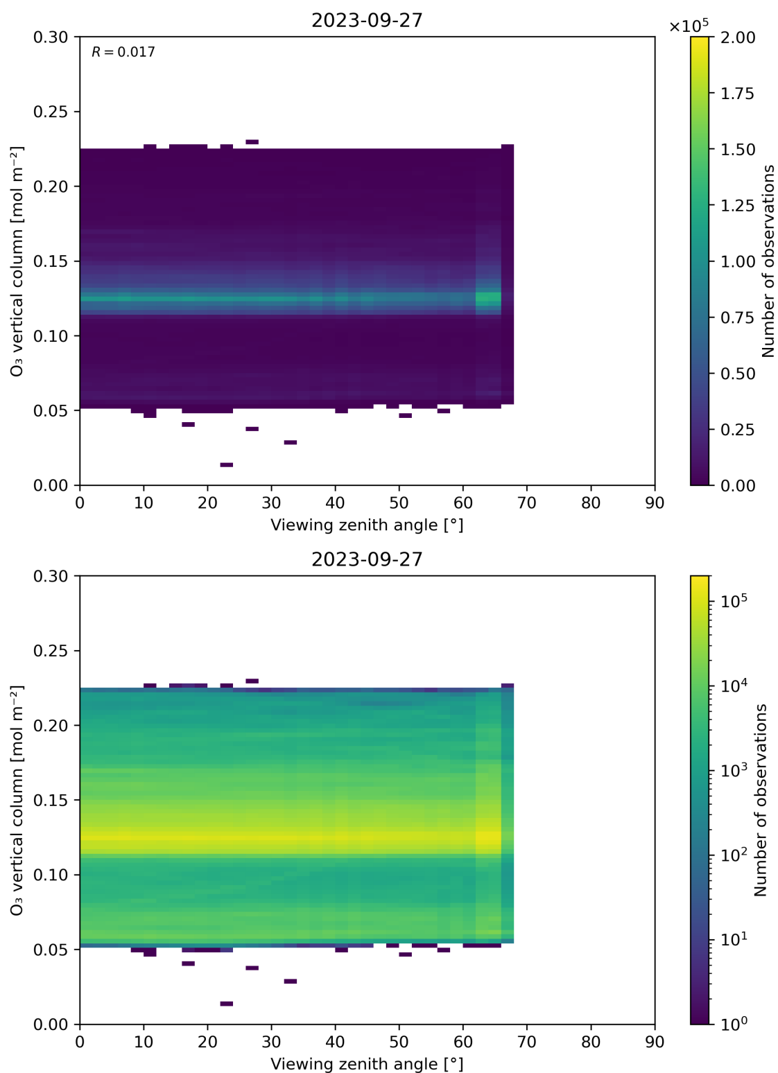
Figure 52: Scatter density plot of “Viewing zenith angle” against “O 3 vertical column” for 2023-09-26 to 2023-09-28.
