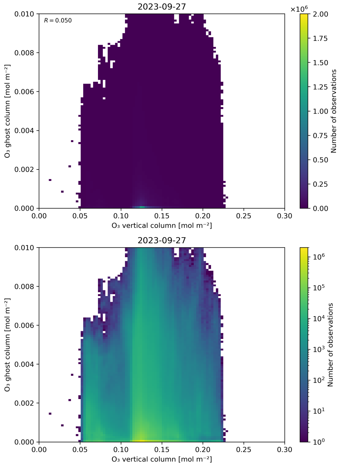
Figure 40: Scatter density plot of “O 3 vertical column” against “O 3 ghost column” for 2023-09-26 to 2023-09-28.
