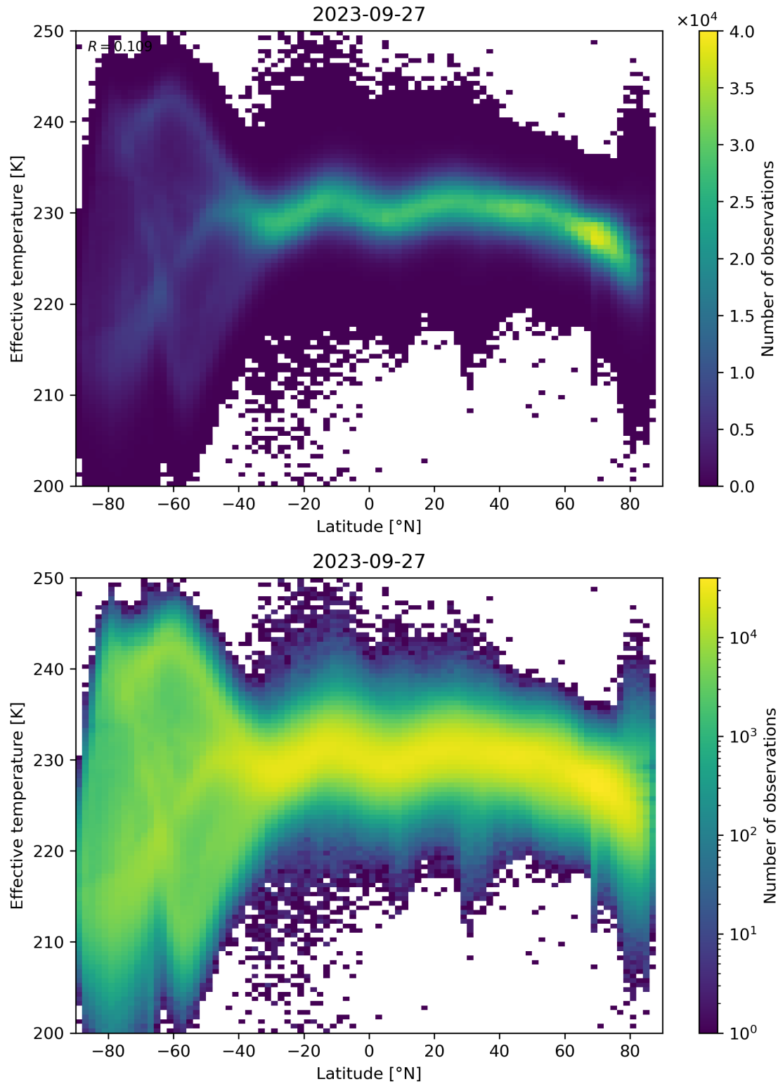
Figure 34: Scatter density plot of “Latitude” against “Effective temperature” for 2023-09-26 to 2023-09-28.
