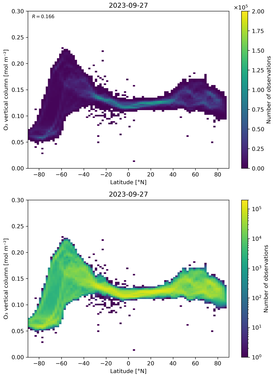
Figure 36: Scatter density plot of “Latitude” against “O 3 vertical column” for 2023-09-26 to 2023-09-28.
