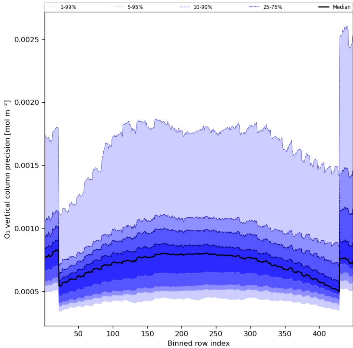
Figure 29: Along track statistics of “O 3 vertical column precision” for 2023-09-26 to 2023-09-28
