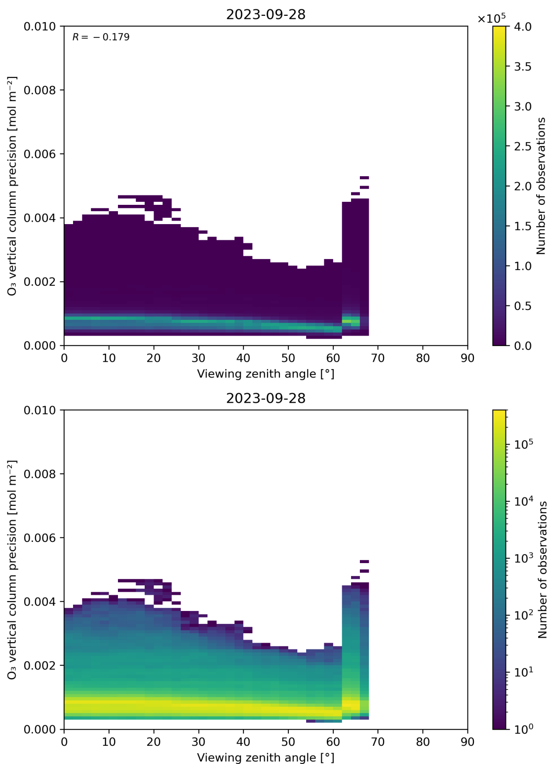
Figure 53: Scatter density plot of “Viewing zenith angle” against “O 3 vertical column precision” for 2023-09-27 to 2023-09-29.
