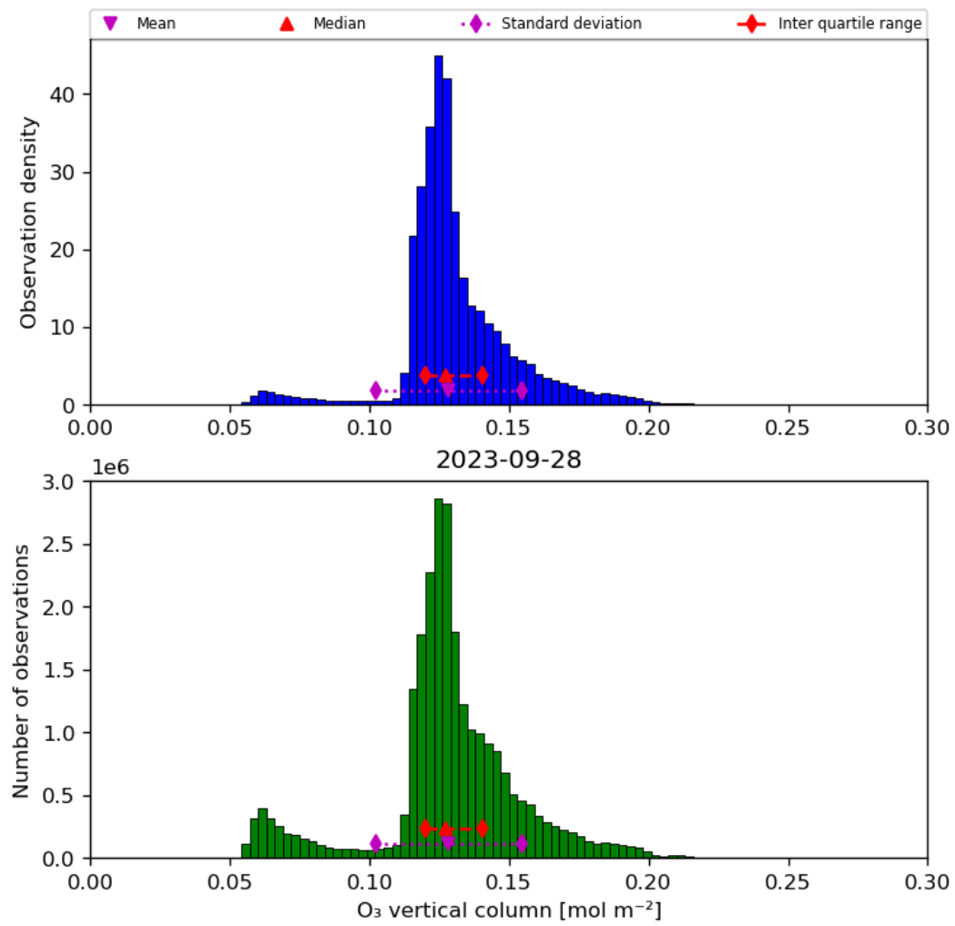
Figure 21: Histogram of “O 3 vertical column” for 2023-09-27 to 2023-09-29
