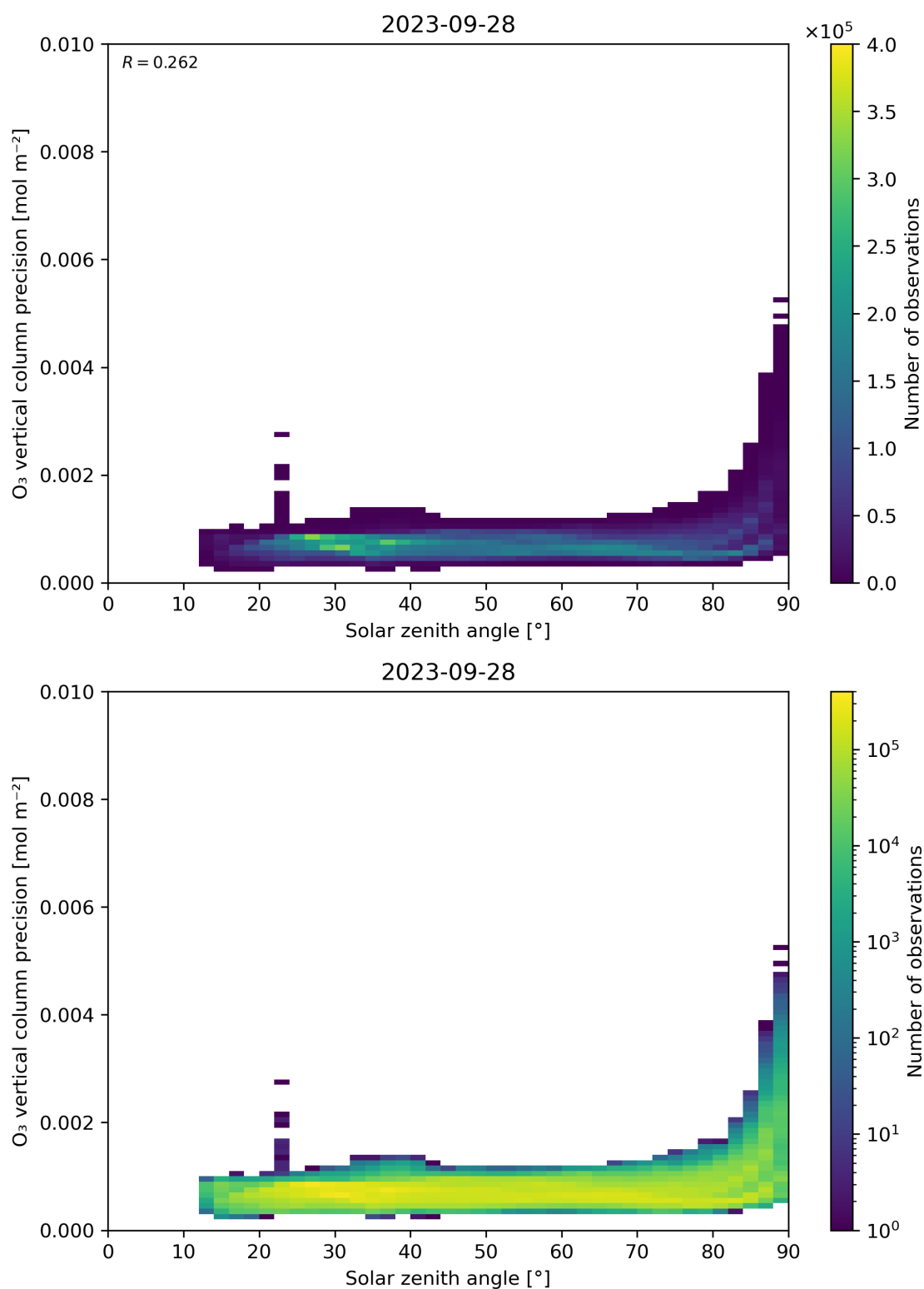
Figure 48: Scatter density plot of “Solar zenith angle” against “O 3 vertical column precision” for 2023-09-27 to 2023-09-29.
