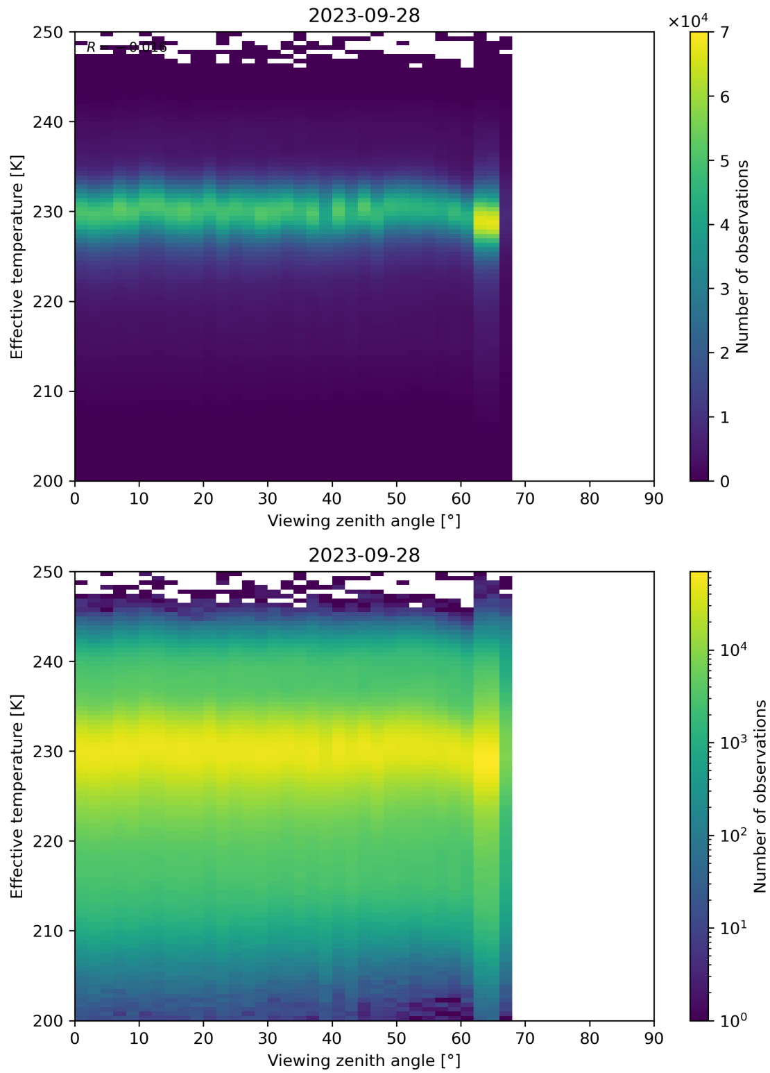
Figure 50: Scatter density plot of “Viewing zenith angle” against “Effective temperature” for 2023-09-27 to 2023-09-29.
