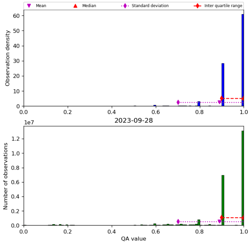
Figure 20: Histogram of “QA value” for 2023-09-27 to 2023-09-29
