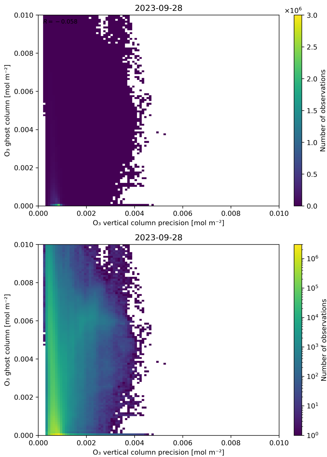
Figure 43: Scatter density plot of “ \text{O}_3 vertical column precision” against “ \text{O}_3 ghost column” for 2023-09-27 to 2023-09-29.
