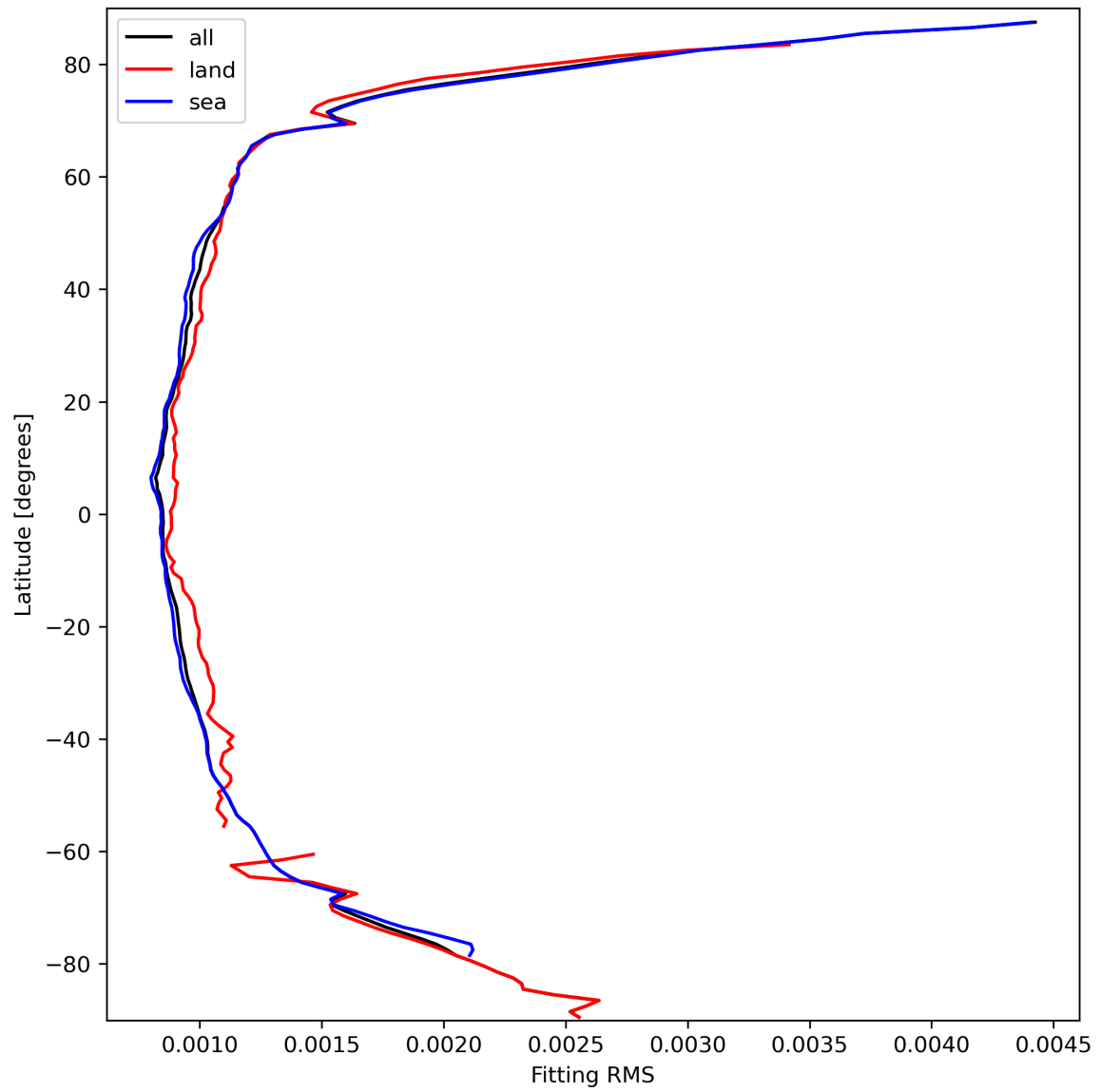
Figure 16: Zonal average of “Fitting RMS” for 2023-09-27 to 2023-09-29.
