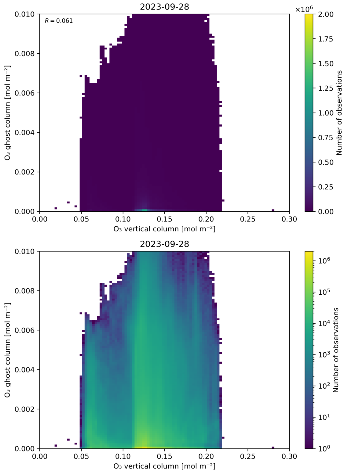
Figure 40: Scatter density plot of “O 3 vertical column” against “O 3 ghost column” for 2023-09-27 to 2023-09-29.
