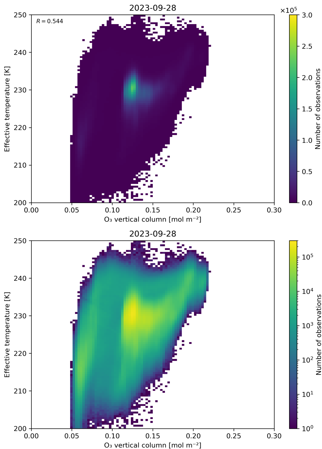
Figure 39: Scatter density plot of “O 3 vertical column” against “Effective temperature” for 2023-09-27 to 2023-09-29.
