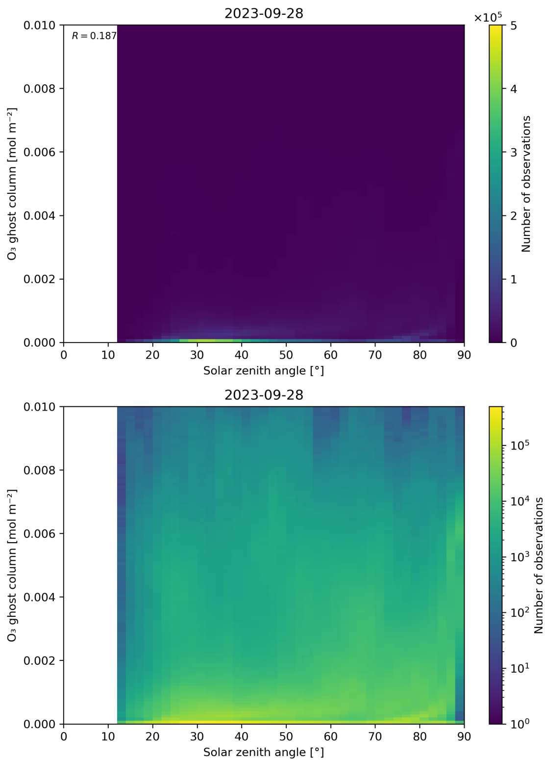
Figure 46: Scatter density plot of “Solar zenith angle” against “O 3 ghost column” for 2023-09-27 to 2023-09-29.
