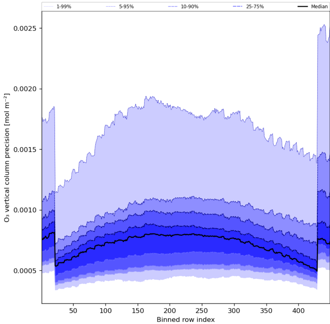
Figure 29: Along track statistics of “O 3 vertical column precision” for 2023-09-27 to 2023-09-29
