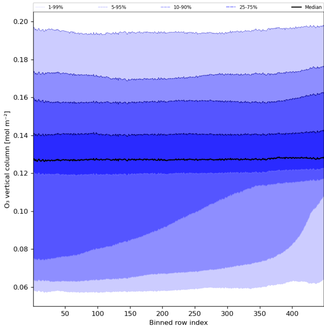
Figure 28: Along track statistics of “O 3 vertical column” for 2023-09-27 to 2023-09-29
