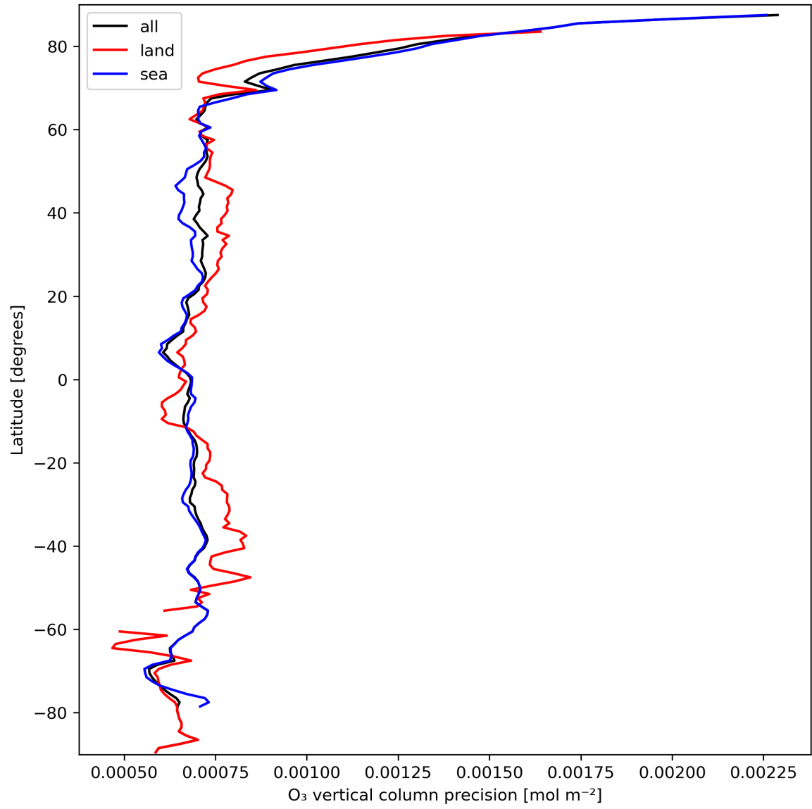
Figure 15: Zonal average of “O 3 vertical column precision” for 2023-09-27 to 2023-09-29.
