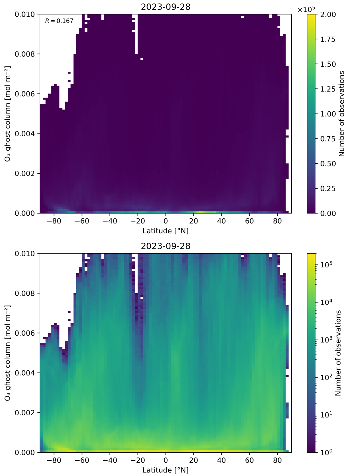
Figure 35: Scatter density plot of “Latitude” against “O 3 ghost column” for 2023-09-27 to 2023-09-29.
