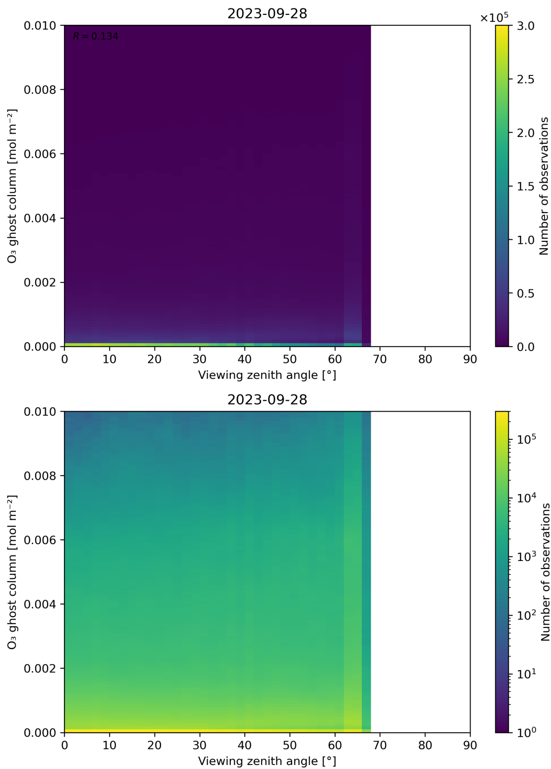
Figure 51: Scatter density plot of “Viewing zenith angle” against “O 3 ghost column” for 2023-09-27 to 2023-09-29.
