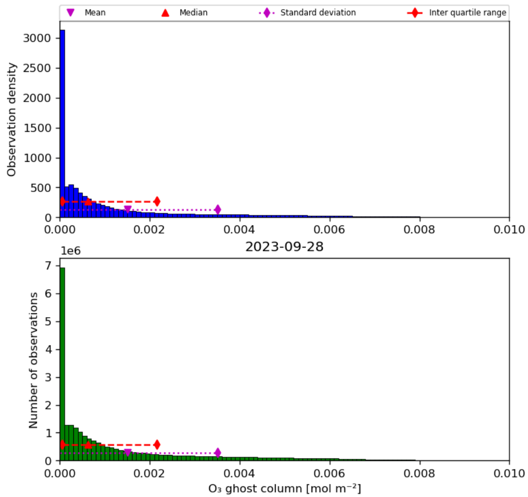
Figure 25: Histogram of "O 3 ghost column" for 2023-09-27 to 2023-09-29
