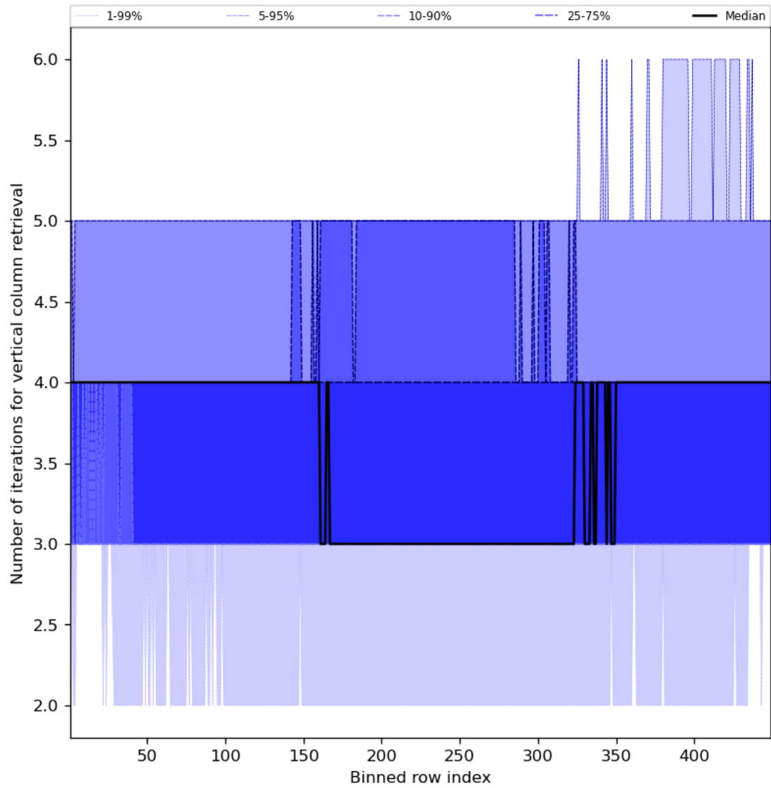
Figure 33: Along track statistics of “Number of iterations for vertical column retrieval” for 2023-09-27 to 2023-09-29
