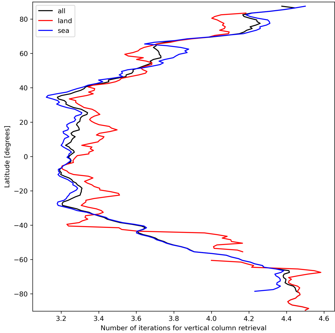
Figure 19: Zonal average of “Number of iterations for vertical column retrieval” for 2023-09-27 to 2023-09-29.
