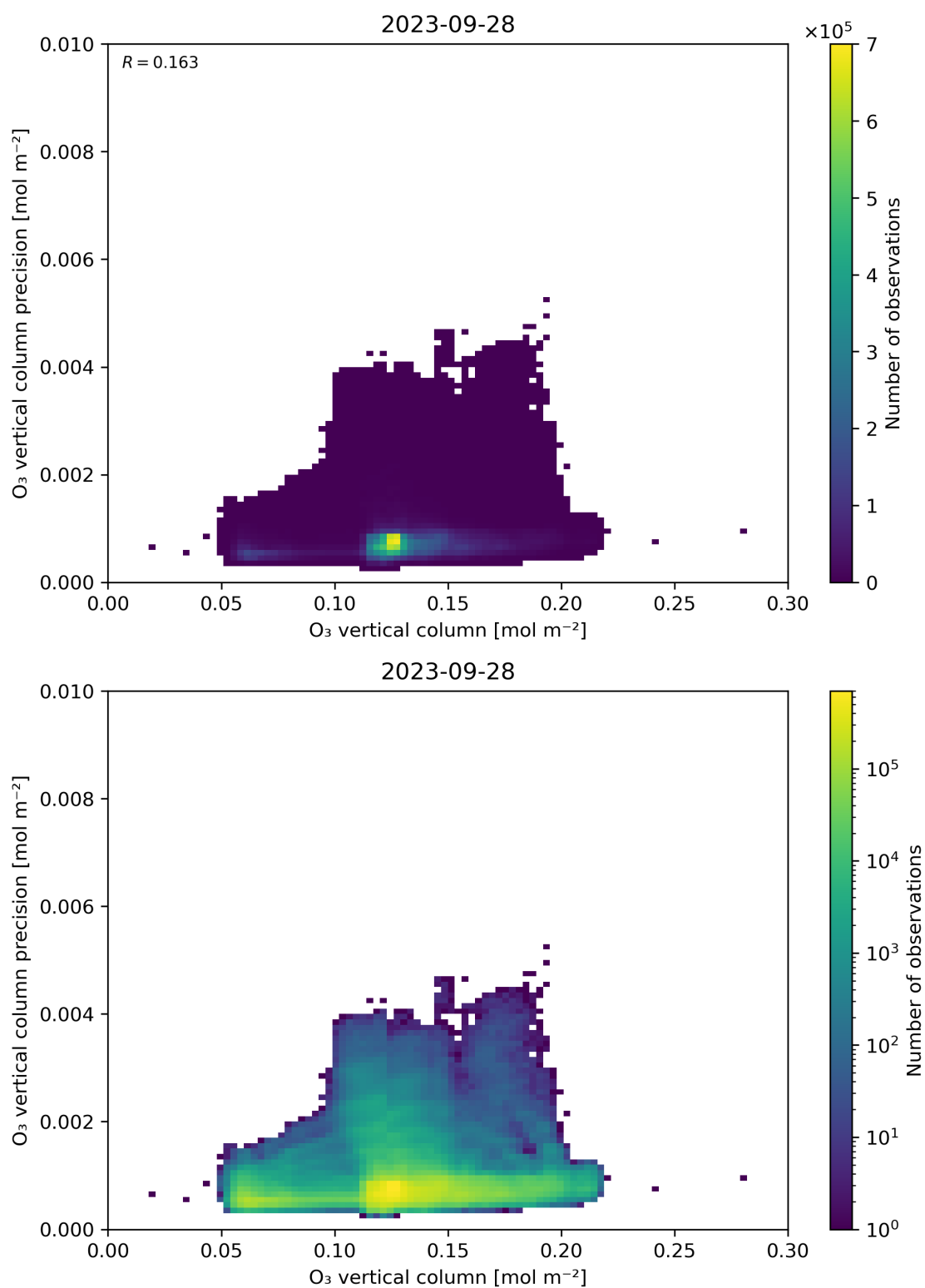
Figure 41: Scatter density plot of “O 3 vertical column” against “O 3 vertical column precision” for 2023-09-27 to 2023-09-29.
