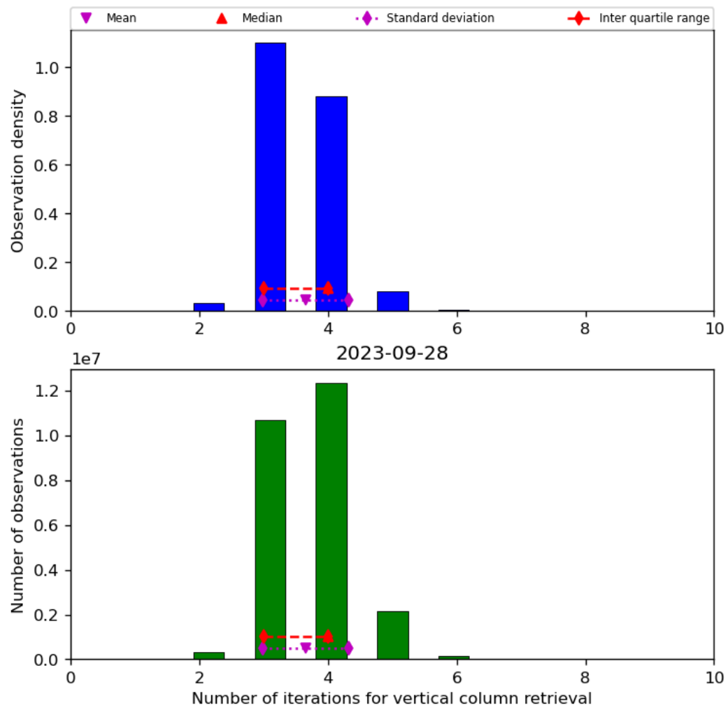
Figure 26: Histogram of “Number of iterations for vertical column retrieval” for 2023-09-27 to 2023-09-29
