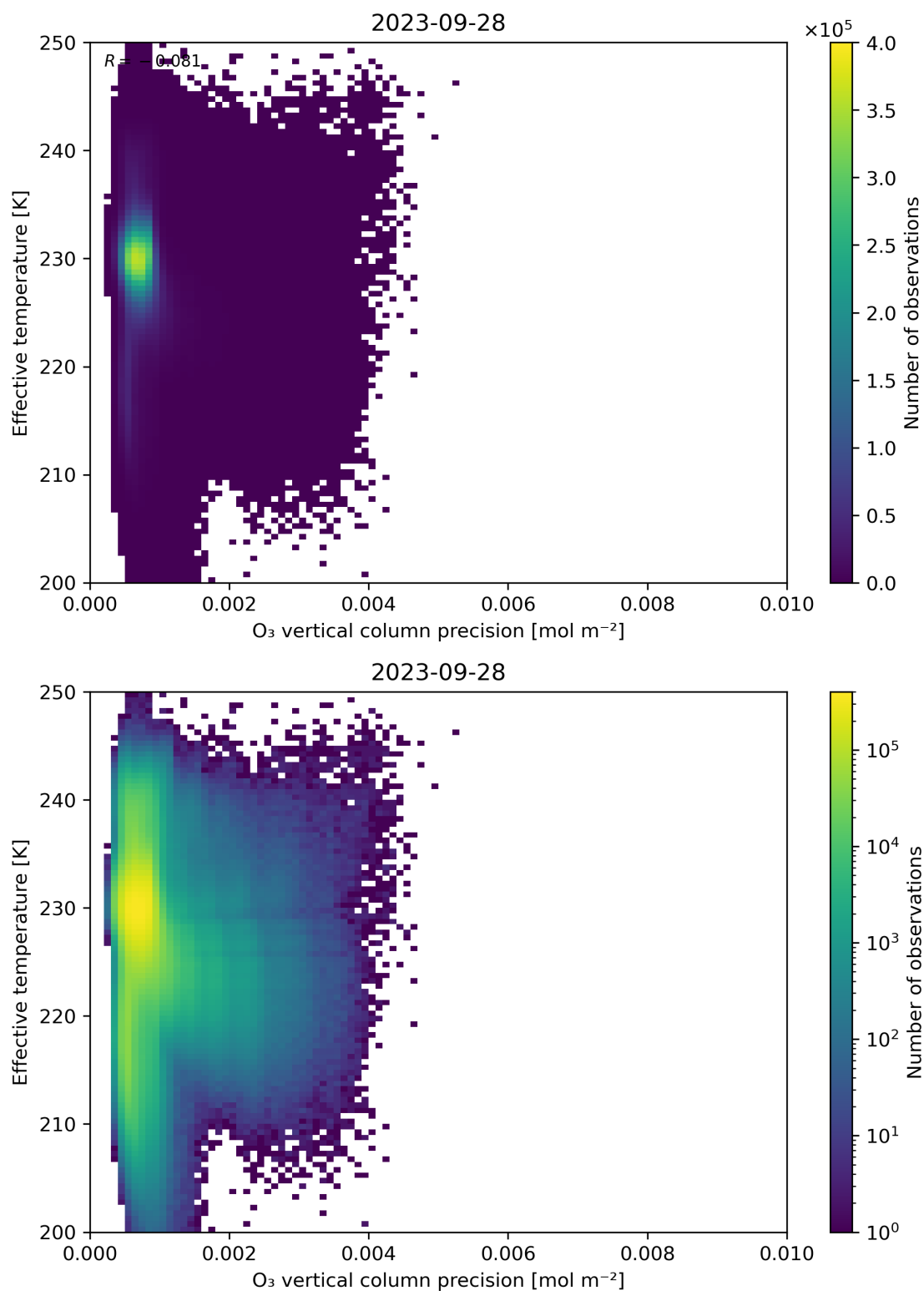
Figure 42: Scatter density plot of “O 3 vertical column precision” against “Effective temperature” for 2023-09-27 to 2023-09-29.
