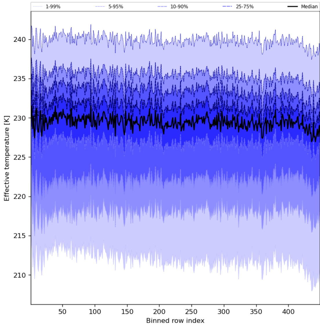
Figure 31: Along track statistics of “Effective temperature” for 2023-09-27 to 2023-09-29
