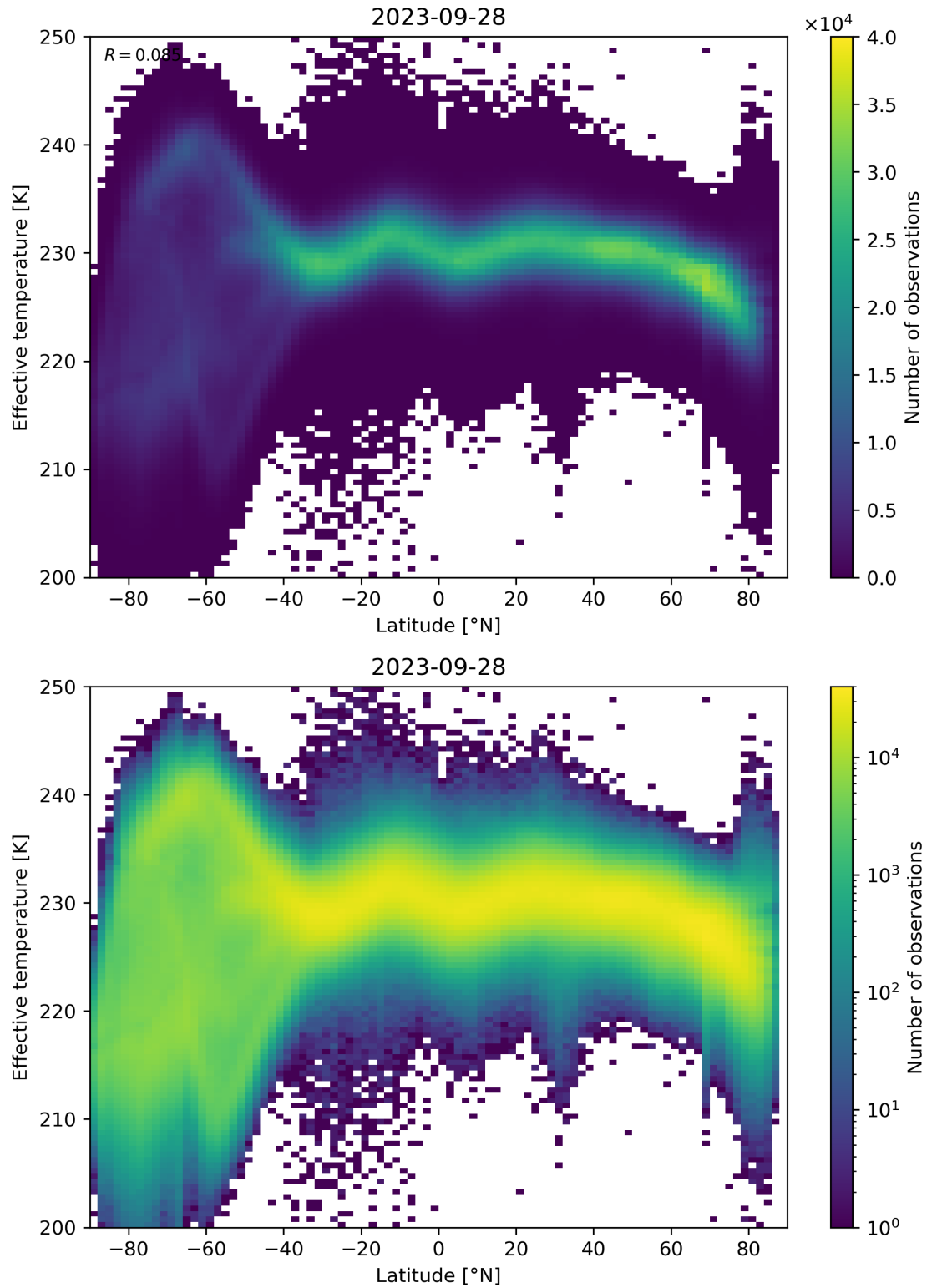
Figure 34: Scatter density plot of “Latitude” against “Effective temperature” for 2023-09-27 to 2023-09-29.
