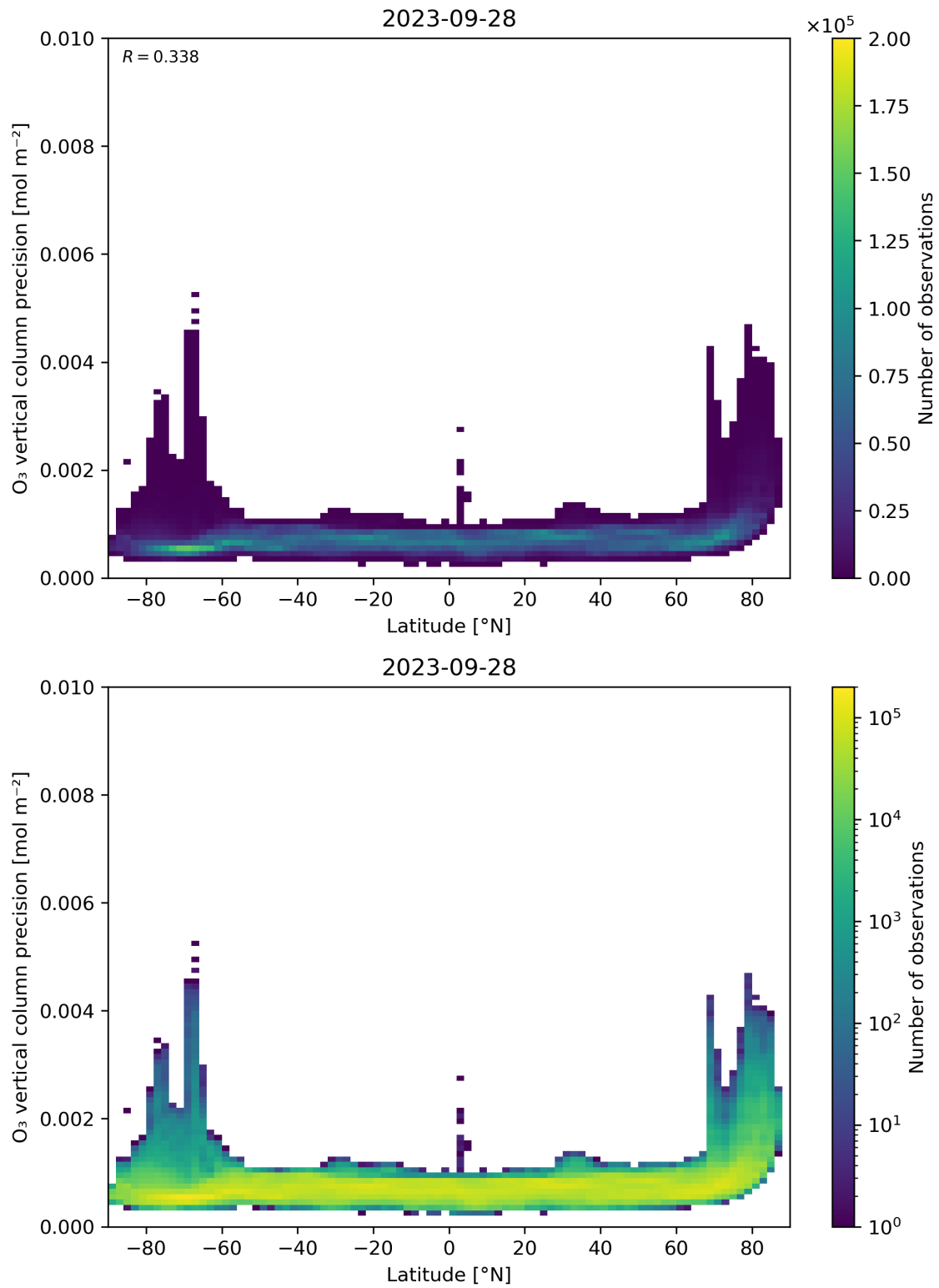
Figure 37: Scatter density plot of “Latitude” against “O 3 vertical column precision” for 2023-09-27 to 2023-09-29.
