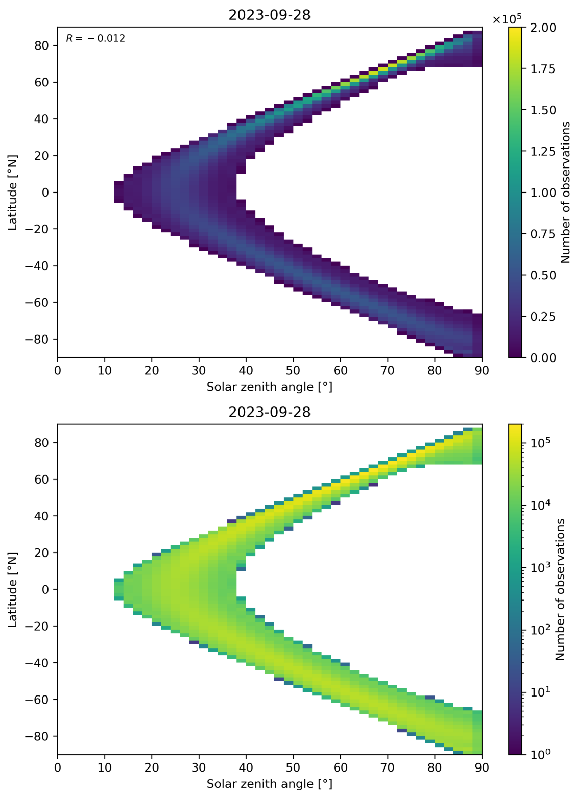
Figure 44: Scatter density plot of “Solar zenith angle” against “Latitude” for 2023-09-27 to 2023-09-29.
