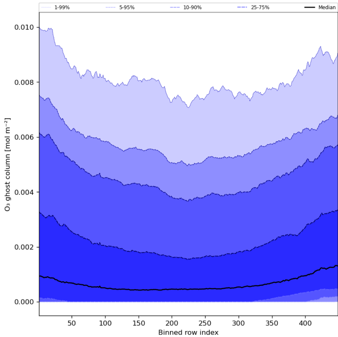
Figure 32: Along track statistics of “O 3 ghost column” for 2023-09-27 to 2023-09-29
