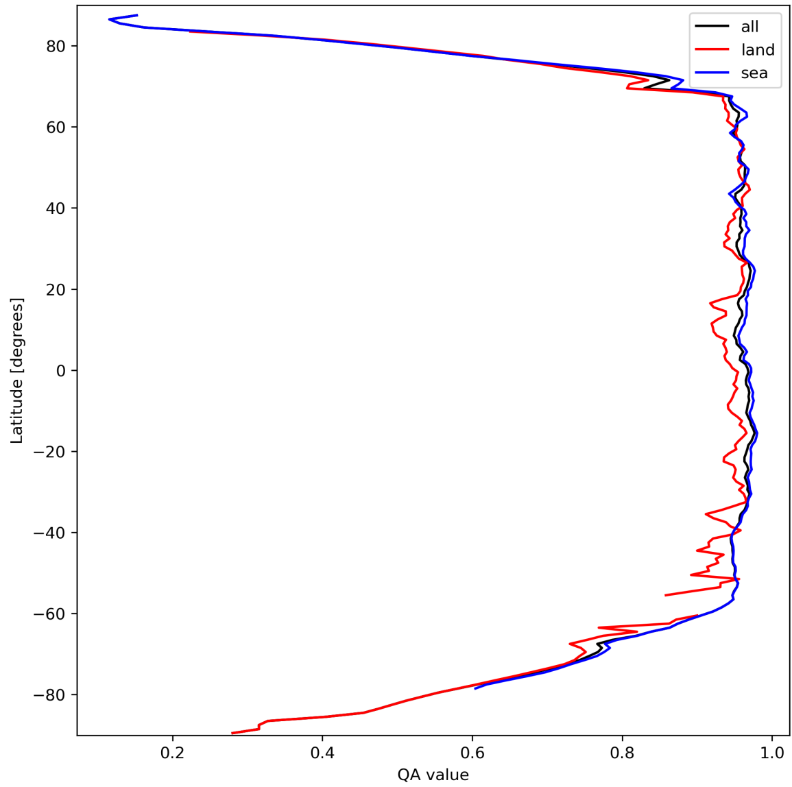
Figure 13: Zonal average of “QA value” for 2023-09-27 to 2023-09-29.
