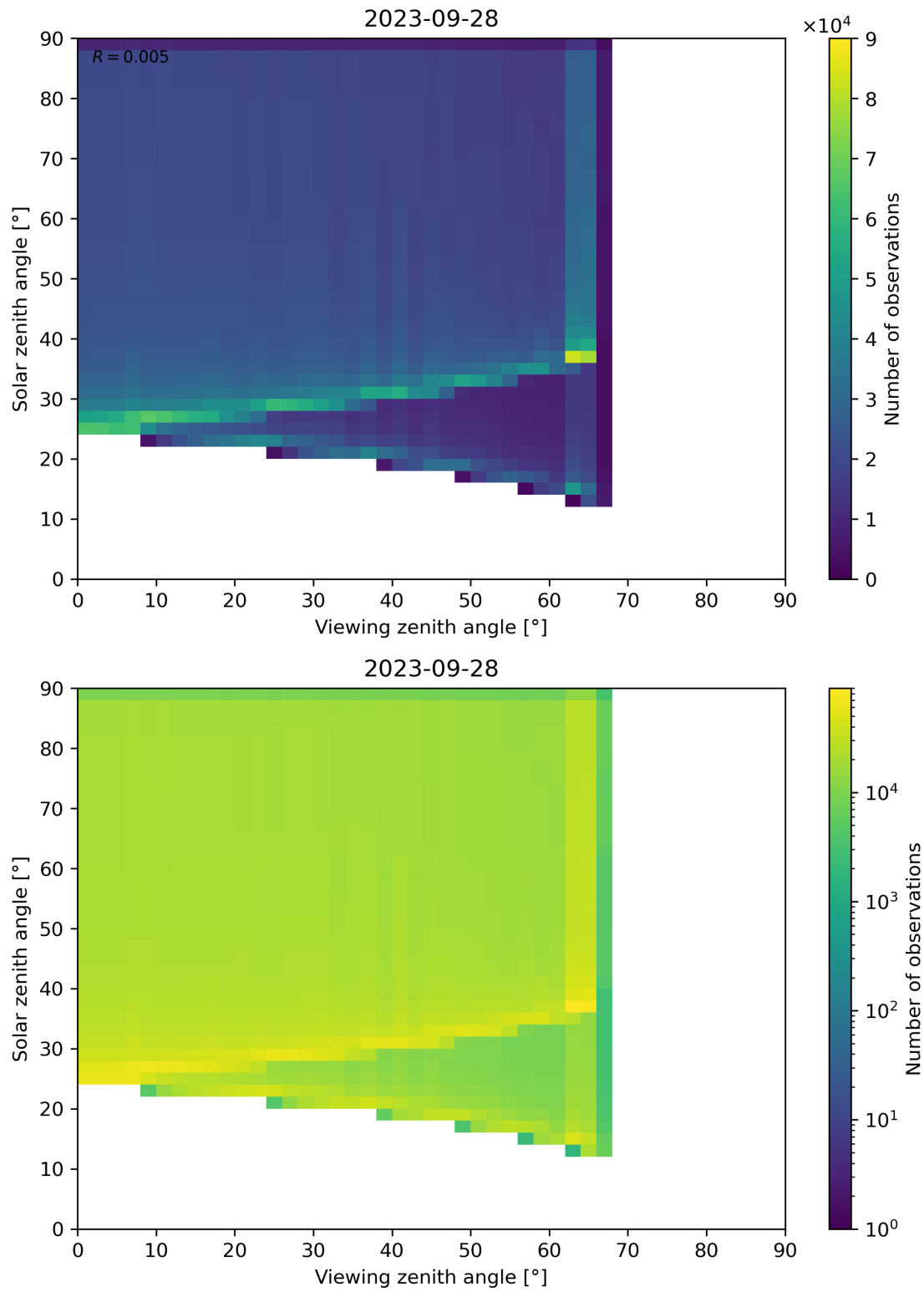
Figure 54: Scatter density plot of “Viewing zenith angle” against “Solar zenith angle” for 2023-09-27 to 2023-09-29.
