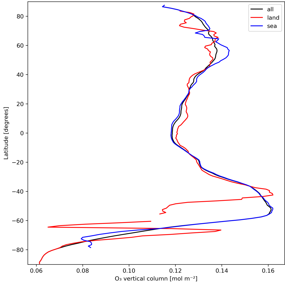
Figure 14: Zonal average of “O 3 vertical column” for 2023-09-27 to 2023-09-29.
