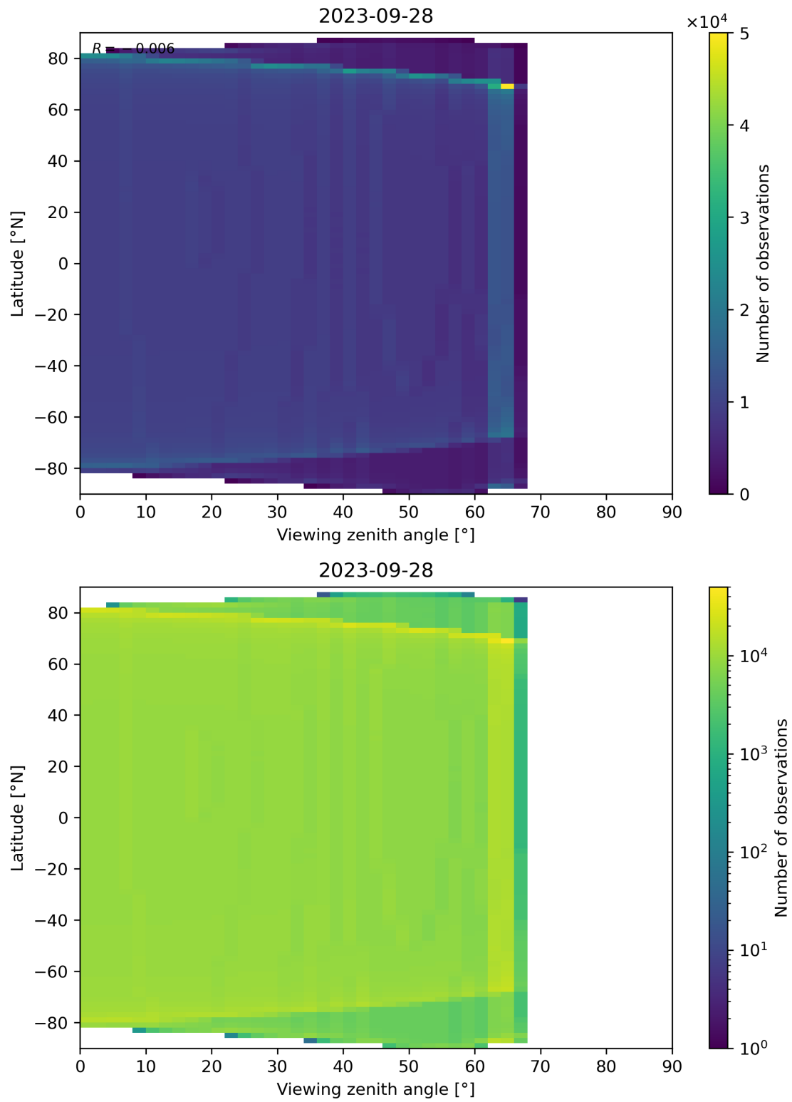
Figure 49: Scatter density plot of “Viewing zenith angle” against “Latitude” for 2023-09-27 to 2023-09-29.
