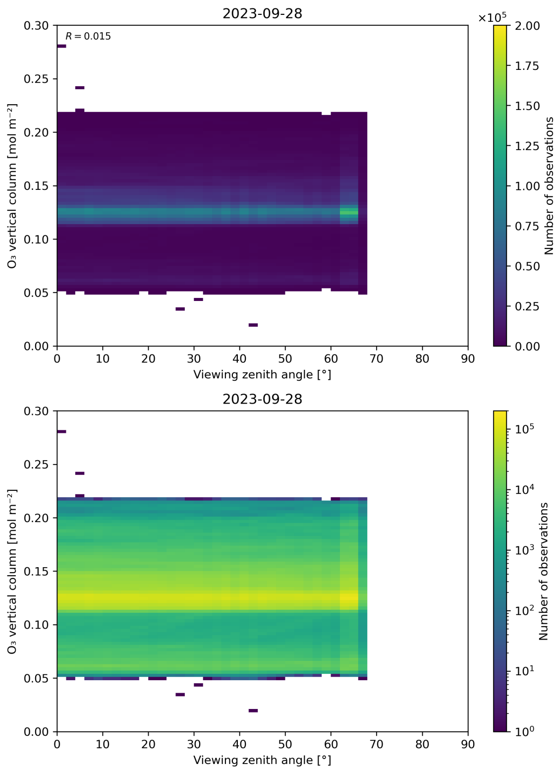
Figure 52: Scatter density plot of “Viewing zenith angle” against “O 3 vertical column” for 2023-09-27 to 2023-09-29.
