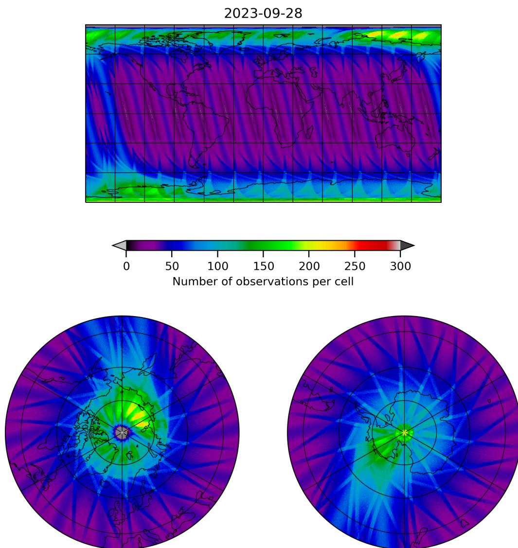
Figure 12: Map of the number of observations for 2023-09-27 to 2023-09-29
