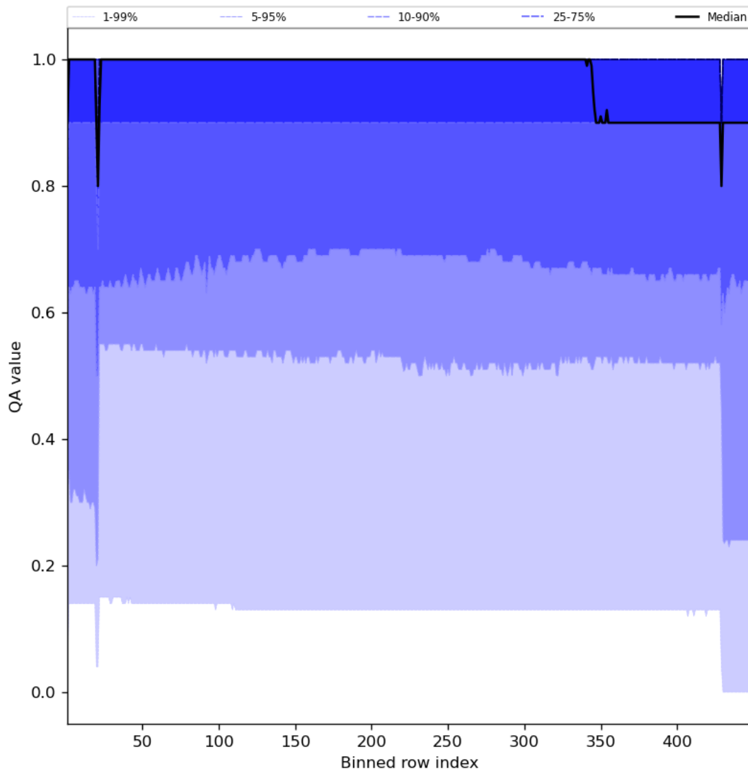
Figure 27: Along track statistics of “QA value” for 2023-09-27 to 2023-09-29
