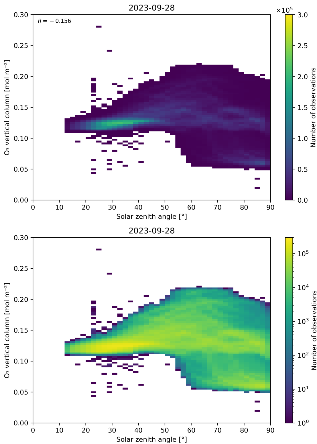
Figure 47: Scatter density plot of “Solar zenith angle” against “O 3 vertical column” for 2023-09-27 to 2023-09-29.
