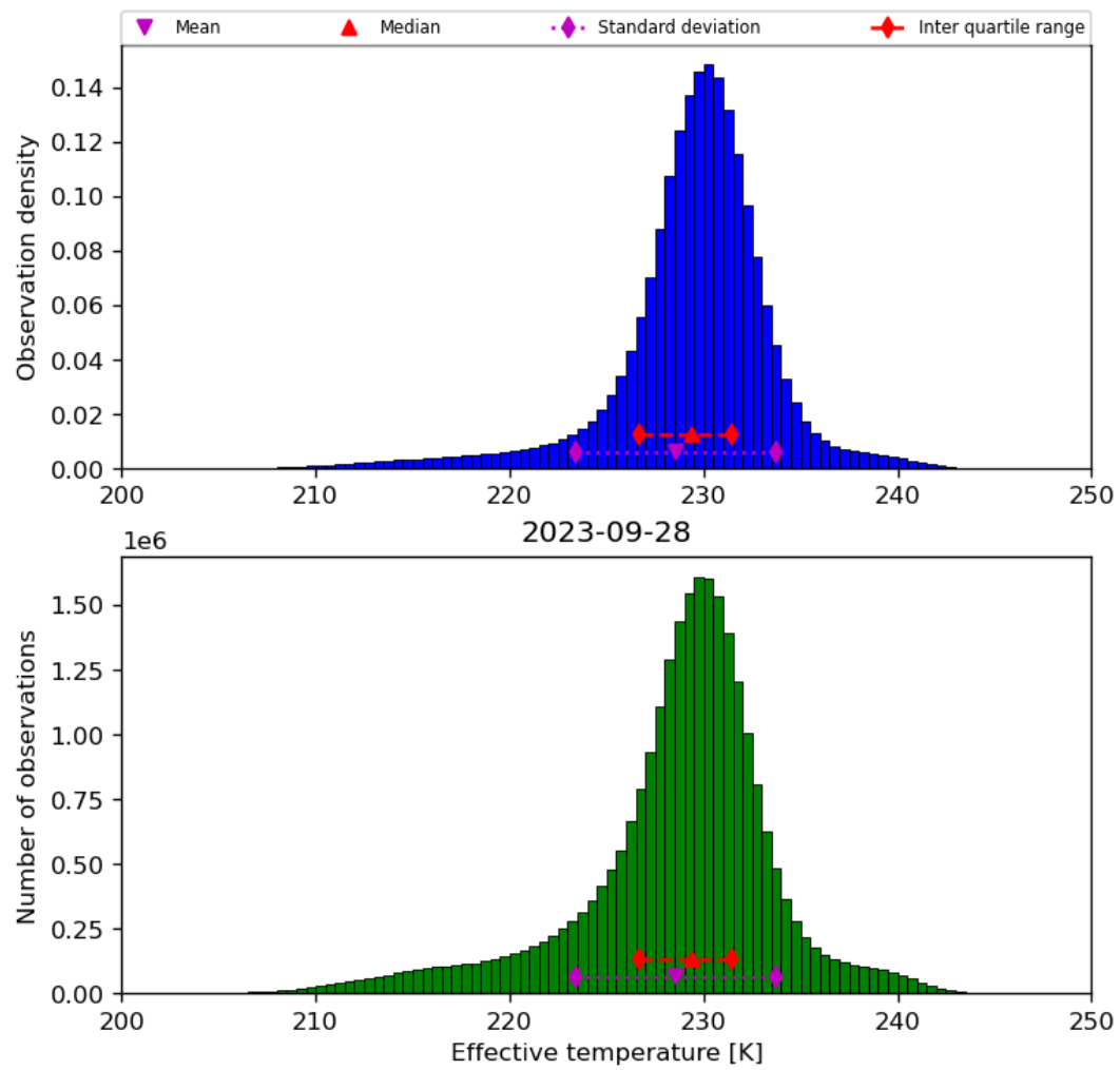
Figure 24: Histogram of “Effective temperature” for 2023-09-27 to 2023-09-29
