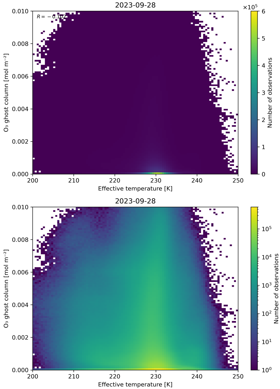
Figure 38: Scatter density plot of “Effective temperature” against “O 3 ghost column” for 2023-09-27 to 2023-09-29.
