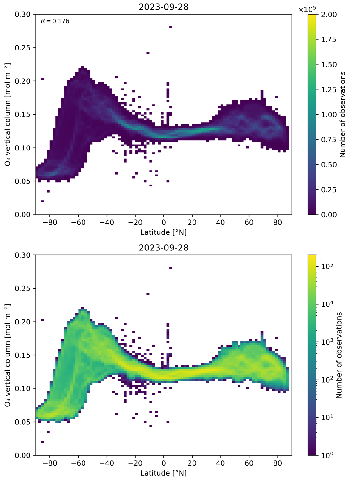
Figure 36: Scatter density plot of “Latitude” against “O 3 vertical column” for 2023-09-27 to 2023-09-29.
