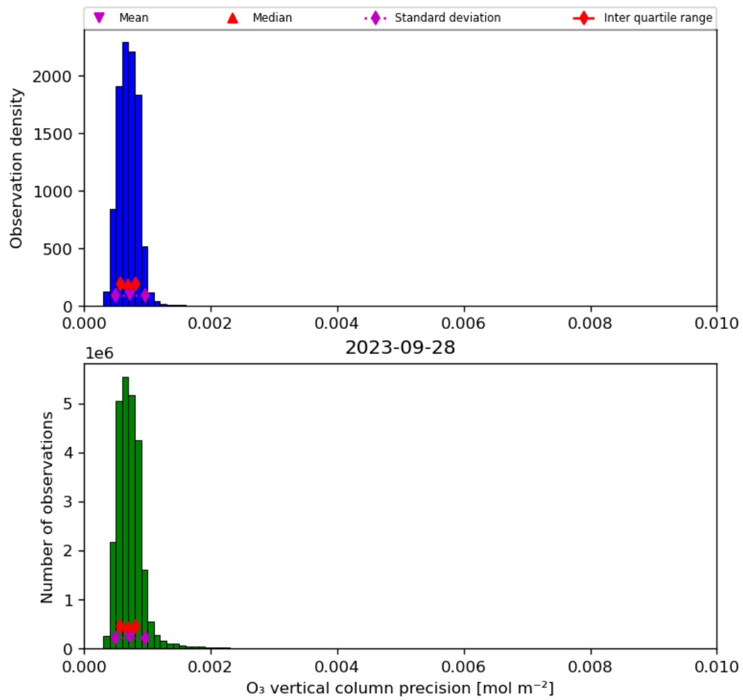
Figure 22: Histogram of “O 3 vertical column precision” for 2023-09-27 to 2023-09-29
