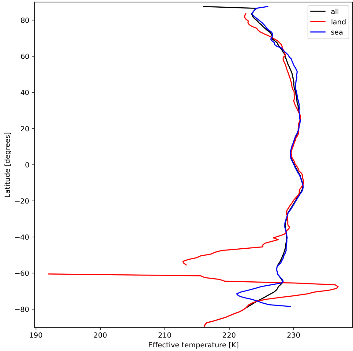
Figure 17: Zonal average of "Effective temperature" for 2023-09-27 to 2023-09-29.
