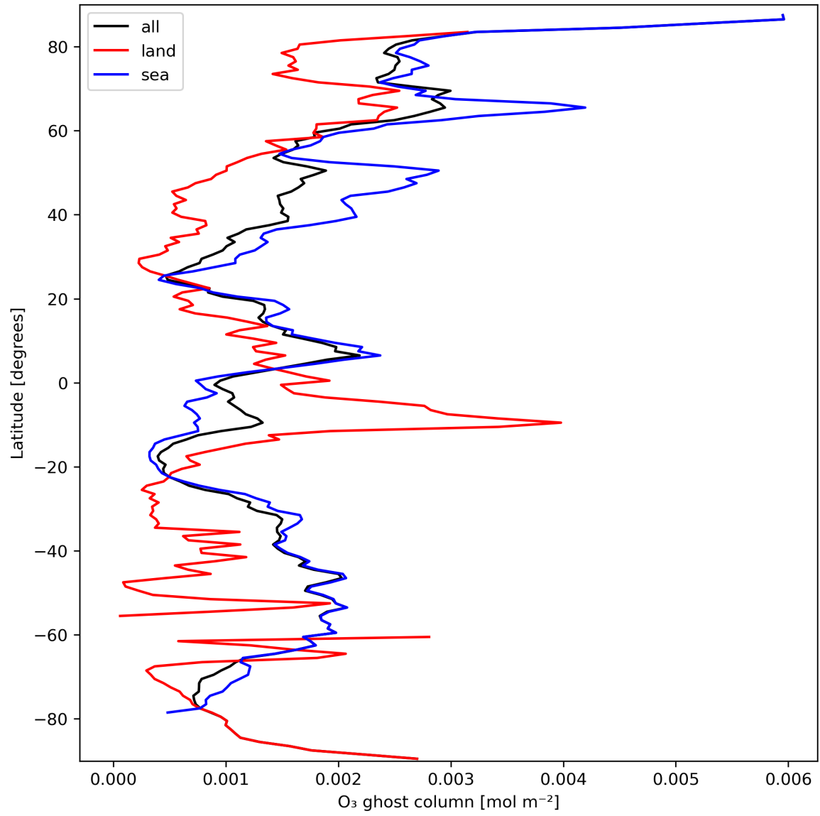
Figure 18: Zonal average of "O 3 ghost column" for 2023-09-27 to 2023-09-29.
