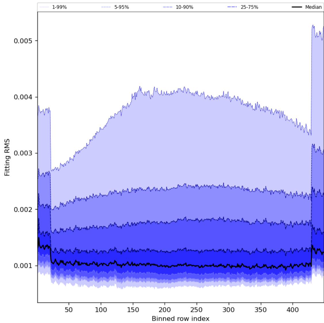
Figure 30: Along track statistics of “Fitting RMS” for 2023-09-27 to 2023-09-29
