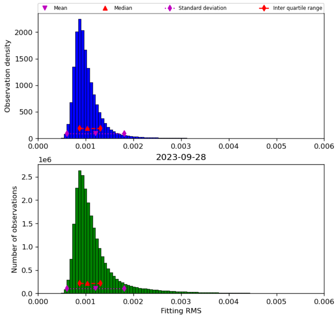
Figure 23: Histogram of “Fitting RMS” for 2023-09-27 to 2023-09-29
