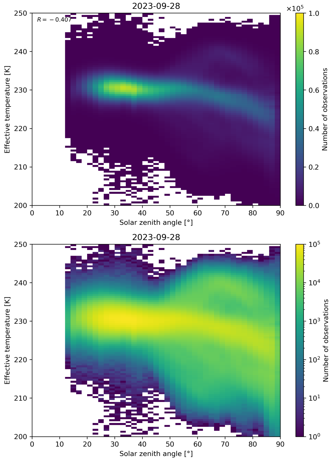
Figure 45: Scatter density plot of “Solar zenith angle” against “Effective temperature” for 2023-09-27 to 2023-09-29.
