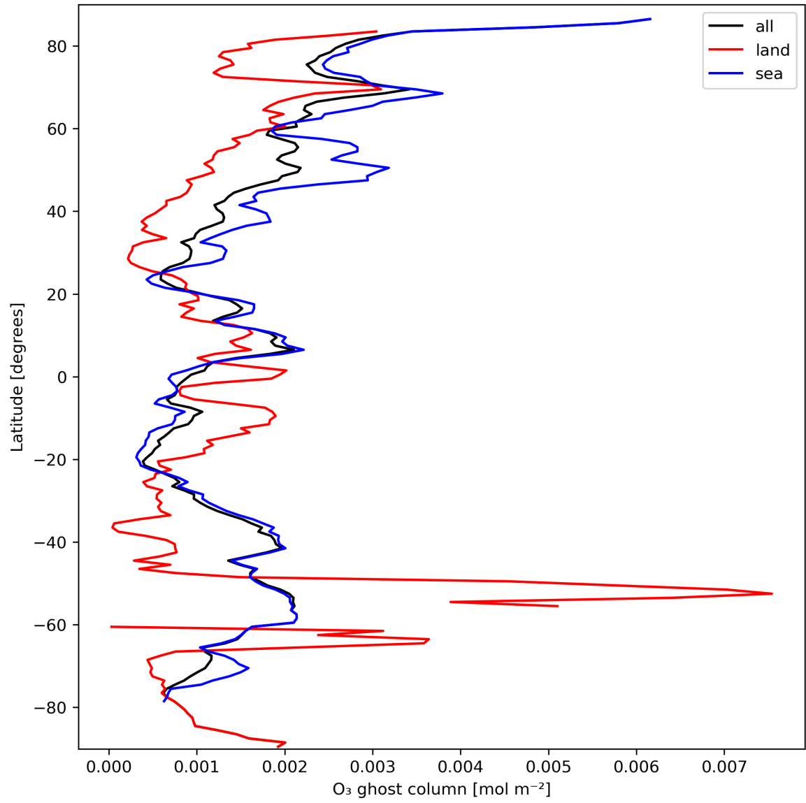
Figure 18: Zonal average of “O 3 ghost column” for 2023-09-28 to 2023-09-30.
