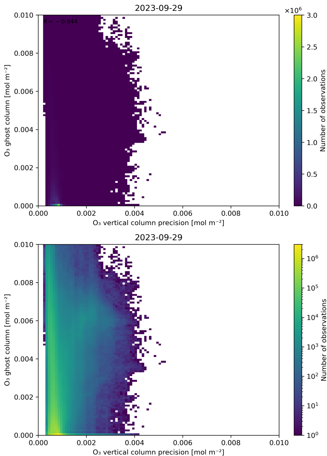
Figure 43: Scatter density plot of “ \text{O}_3 vertical column precision” against “ \text{O}_3 ghost column” for 2023-09-28 to 2023-09-30.
