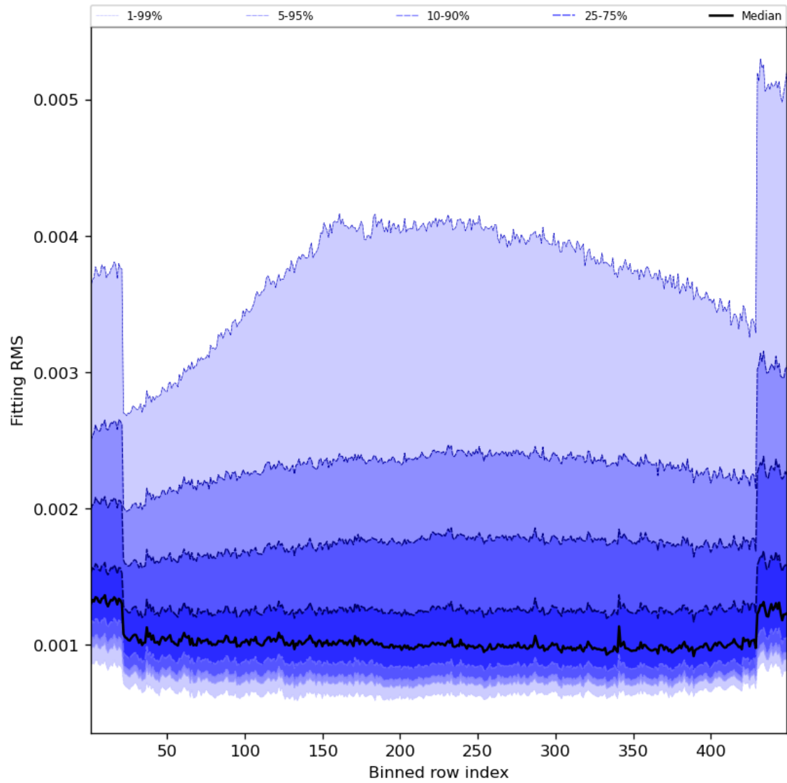
Figure 30: Along track statistics of “Fitting RMS” for 2023-09-28 to 2023-09-30
