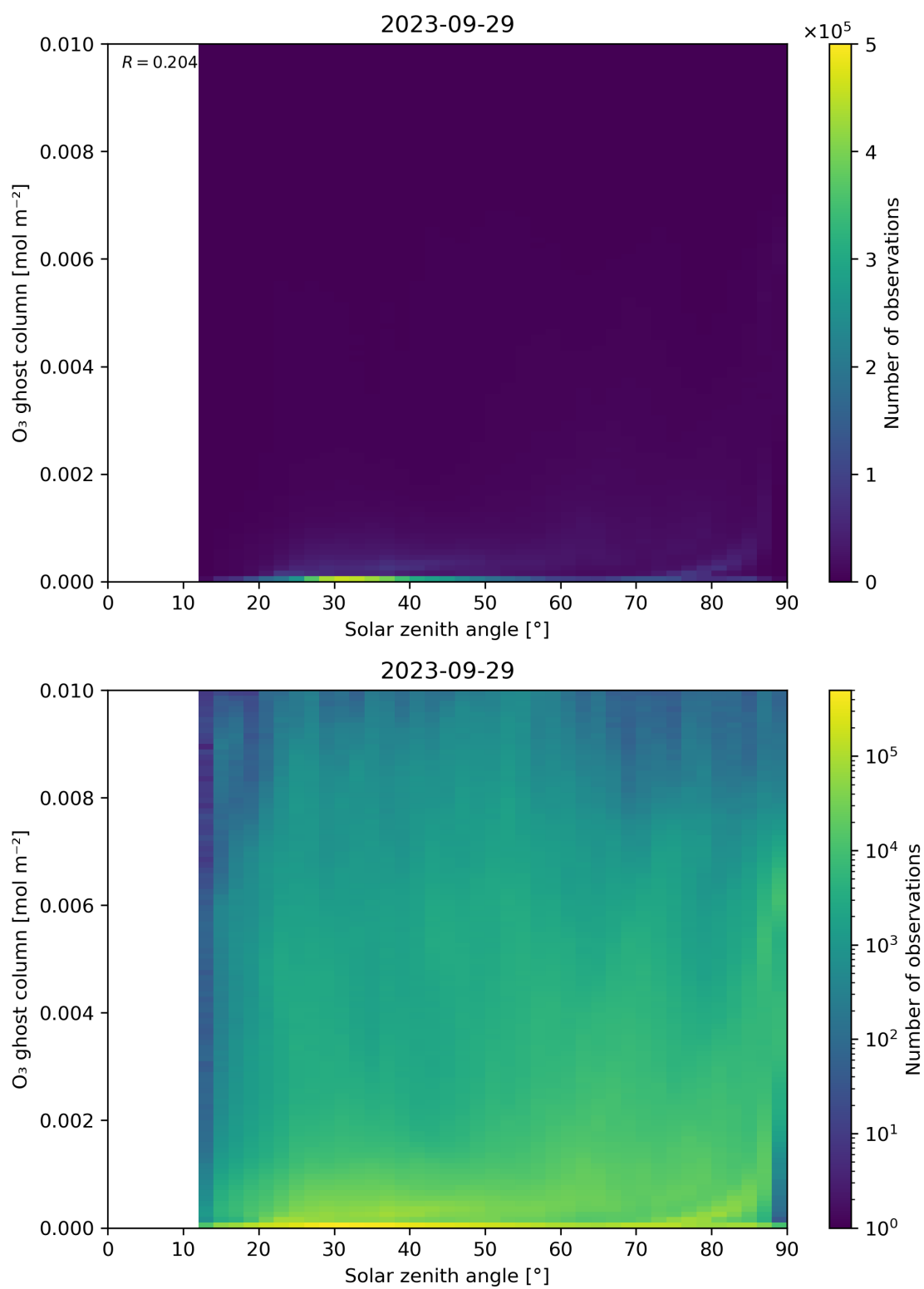
Figure 46: Scatter density plot of “Solar zenith angle” against “O 3 ghost column” for 2023-09-28 to 2023-09-30.
