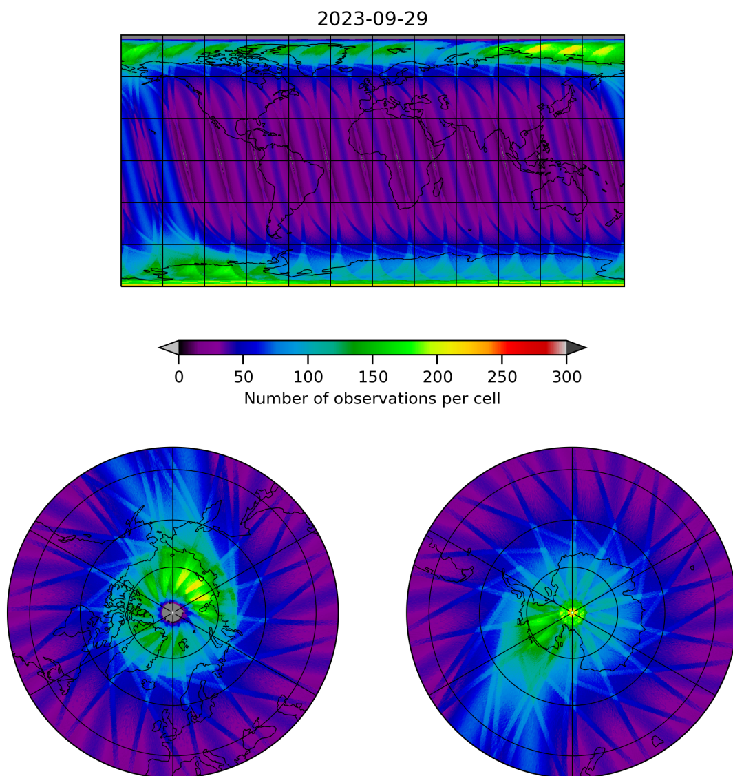
Figure 12: Map of the number of observations for 2023-09-28 to 2023-09-30
