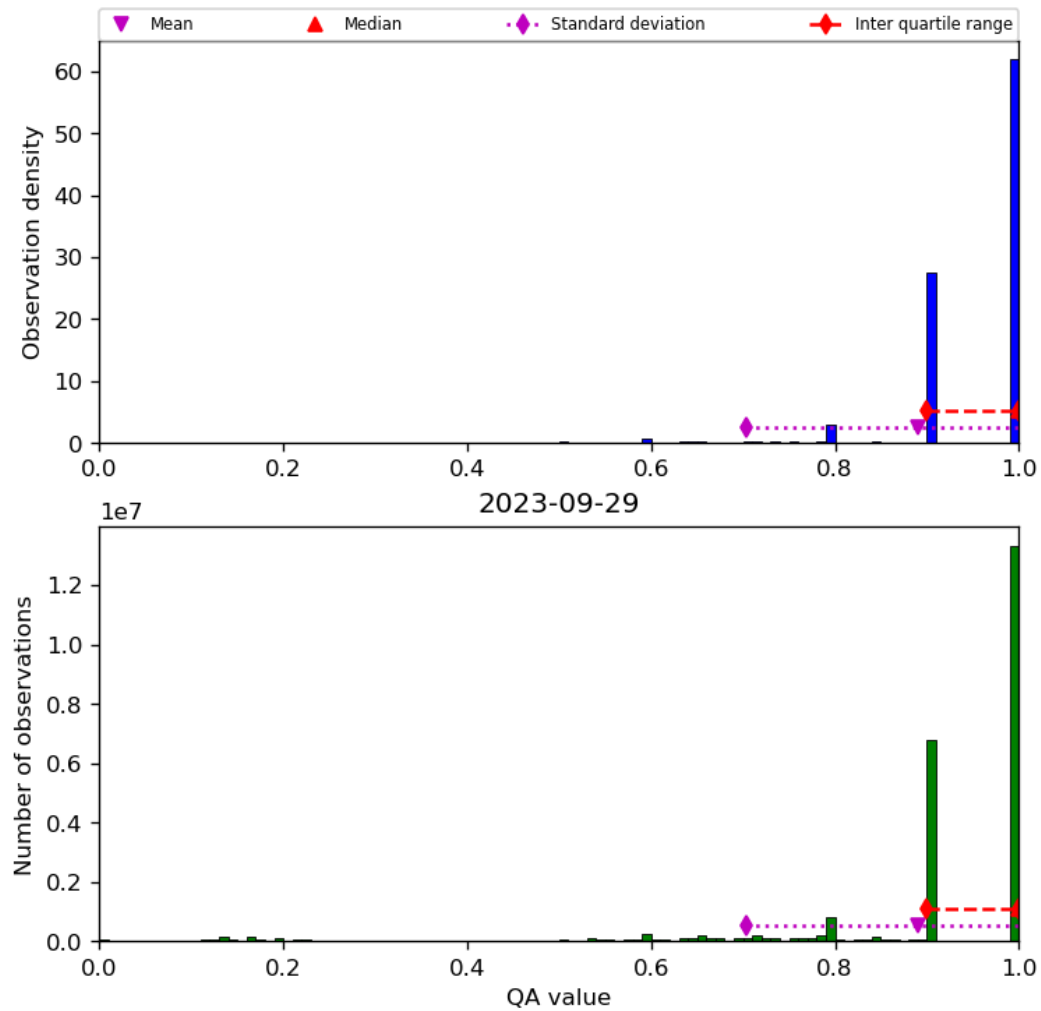
Figure 20: Histogram of “QA value” for 2023-09-28 to 2023-09-30
