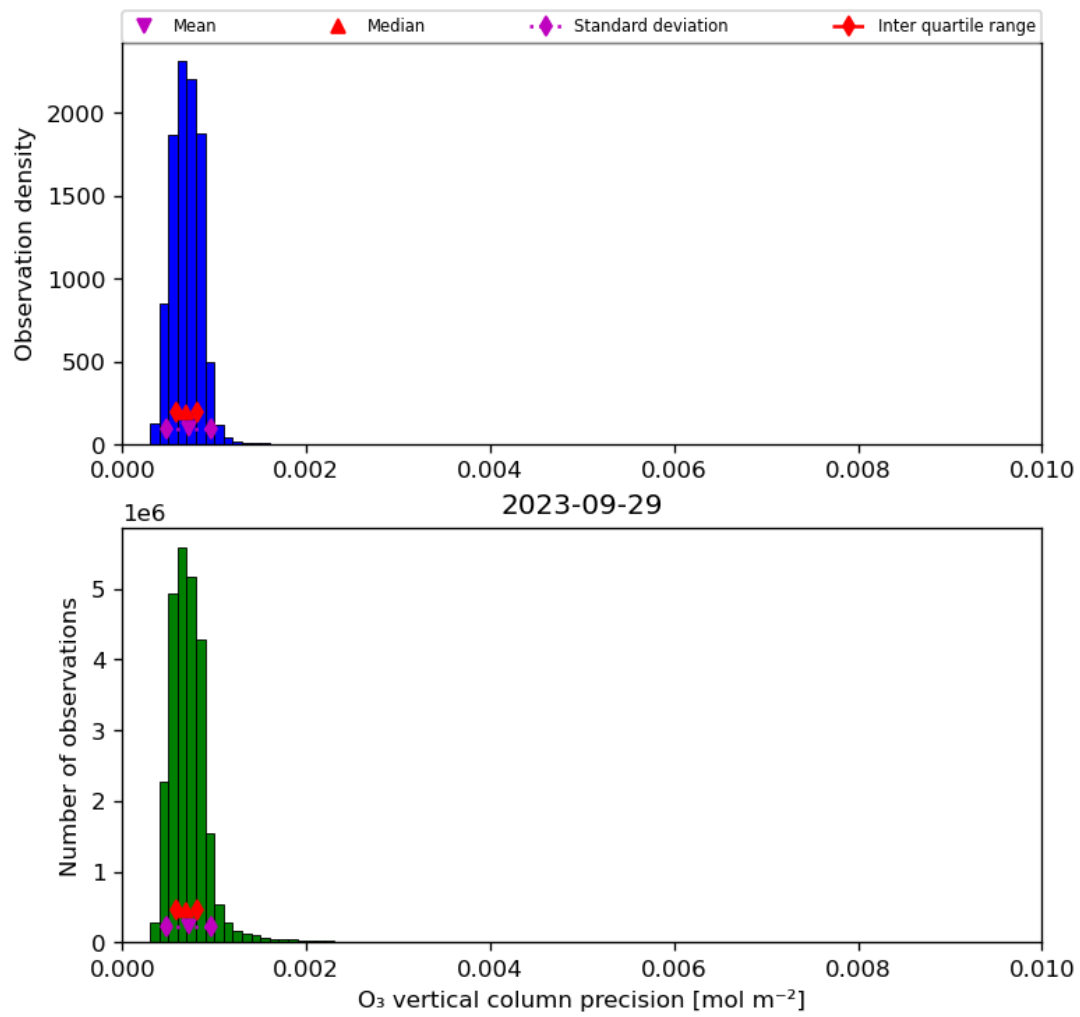
Figure 22: Histogram of “O 3 vertical column precision” for 2023-09-28 to 2023-09-30
