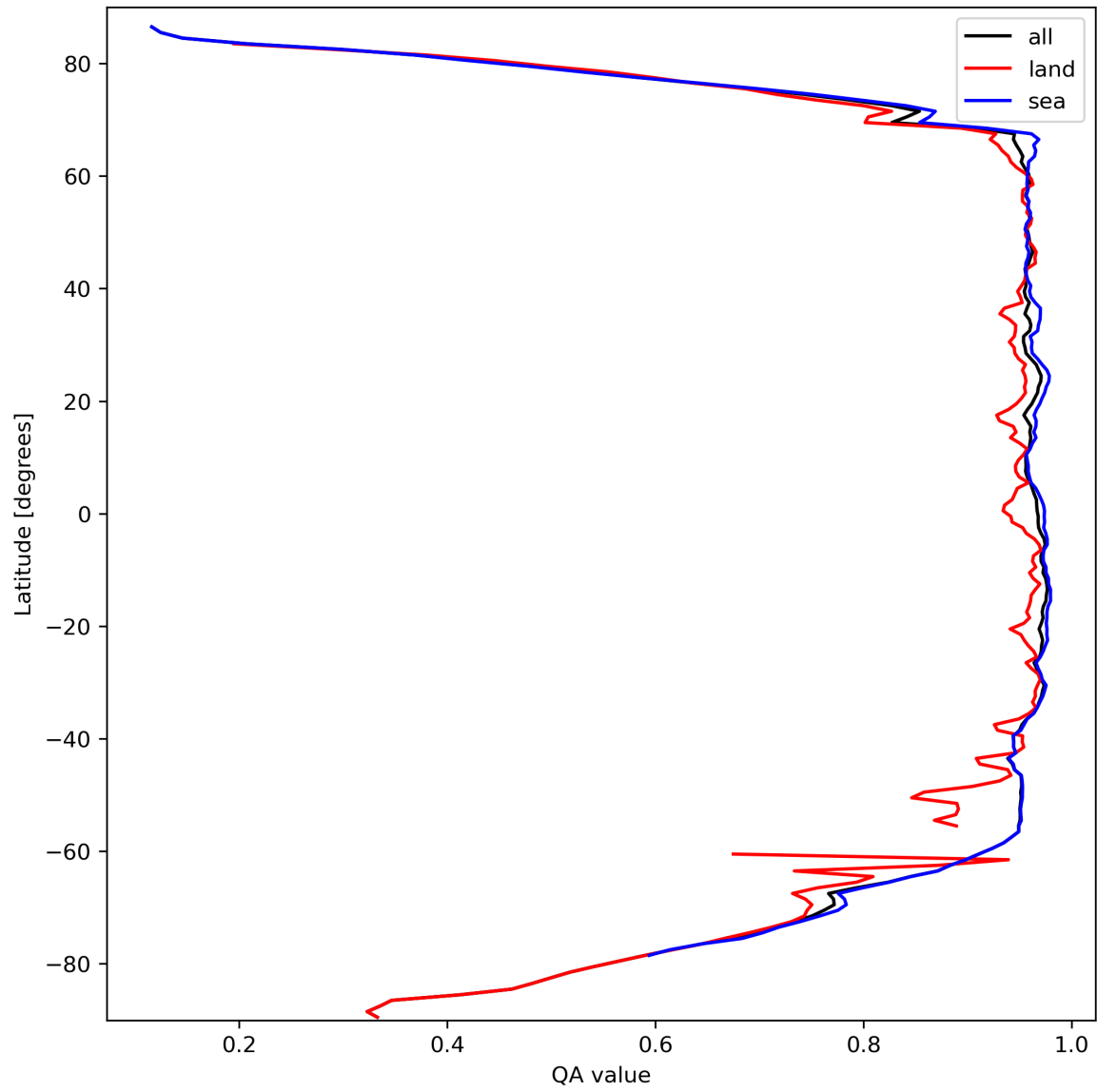
Figure 13: Zonal average of “QA value” for 2023-09-28 to 2023-09-30.
