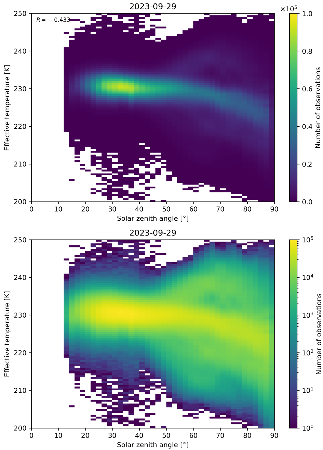
Figure 45: Scatter density plot of “Solar zenith angle” against “Effective temperature” for 2023-09-28 to 2023-09-30.
