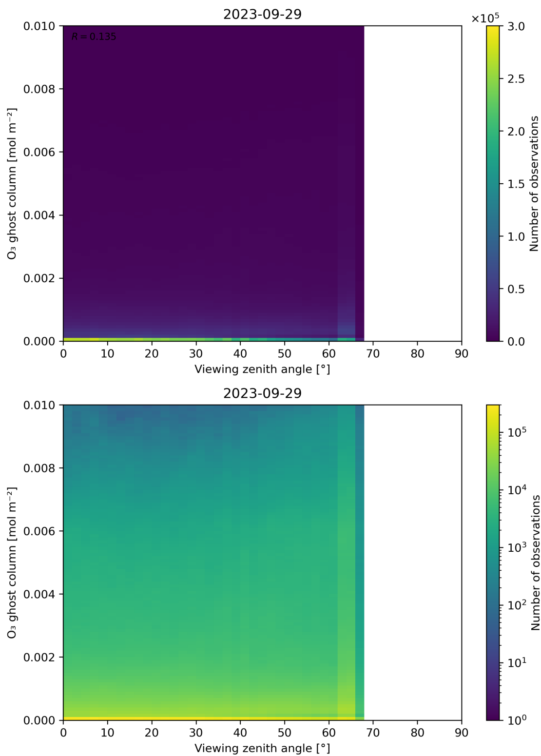
Figure 51: Scatter density plot of “Viewing zenith angle” against “O 3 ghost column” for 2023-09-28 to 2023-09-30.
