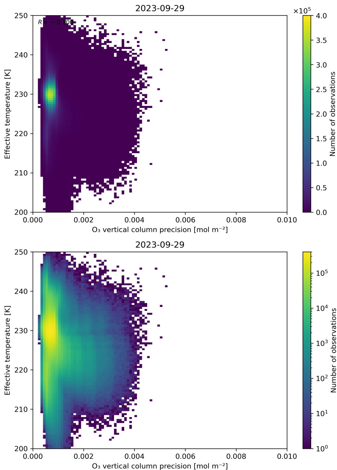
Figure 42: Scatter density plot of “ O_3 vertical column precision” against “Effective temperature” for 2023-09-28 to 2023-09-30.
