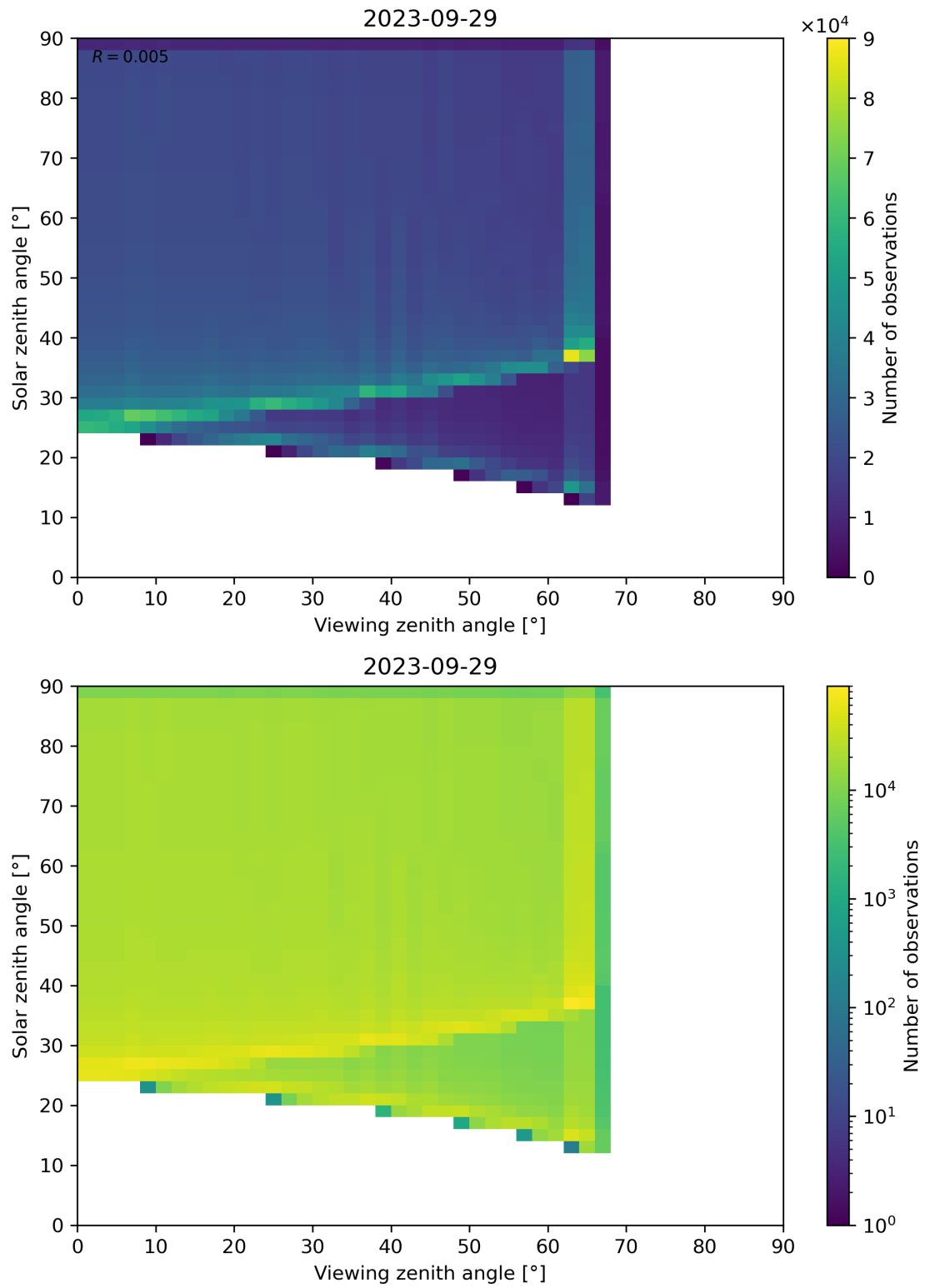
Figure 54: Scatter density plot of “Viewing zenith angle” against “Solar zenith angle” for 2023-09-28 to 2023-09-30.
