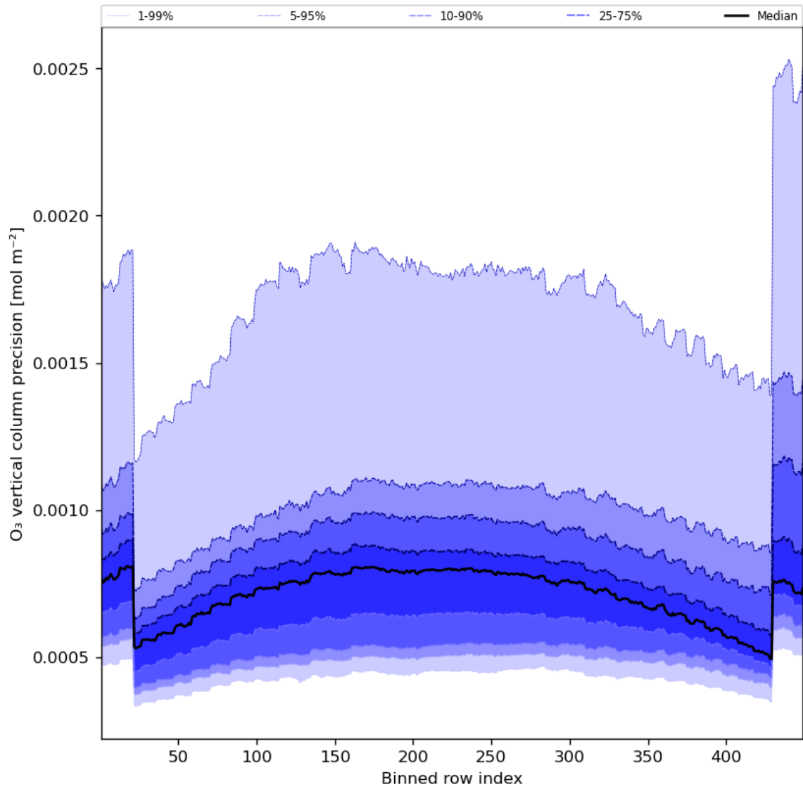
Figure 29: Along track statistics of “O 3 vertical column precision” for 2023-09-28 to 2023-09-30
