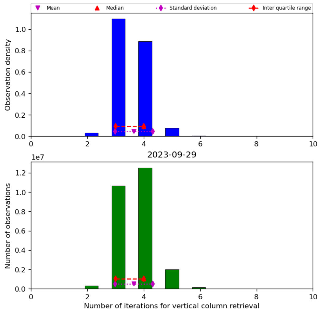
Figure 26: Histogram of “Number of iterations for vertical column retrieval” for 2023-09-28 to 2023-09-30
