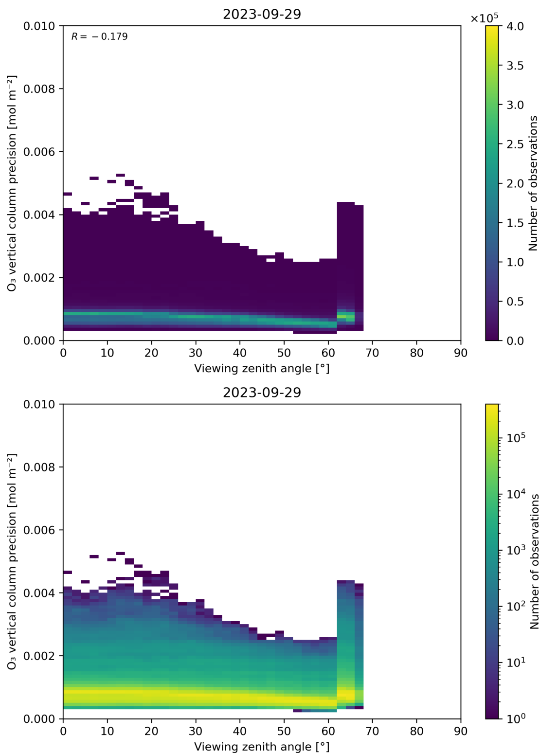
Figure 53: Scatter density plot of “Viewing zenith angle” against “O 3 vertical column precision” for 2023-09-28 to 2023-09-30.
