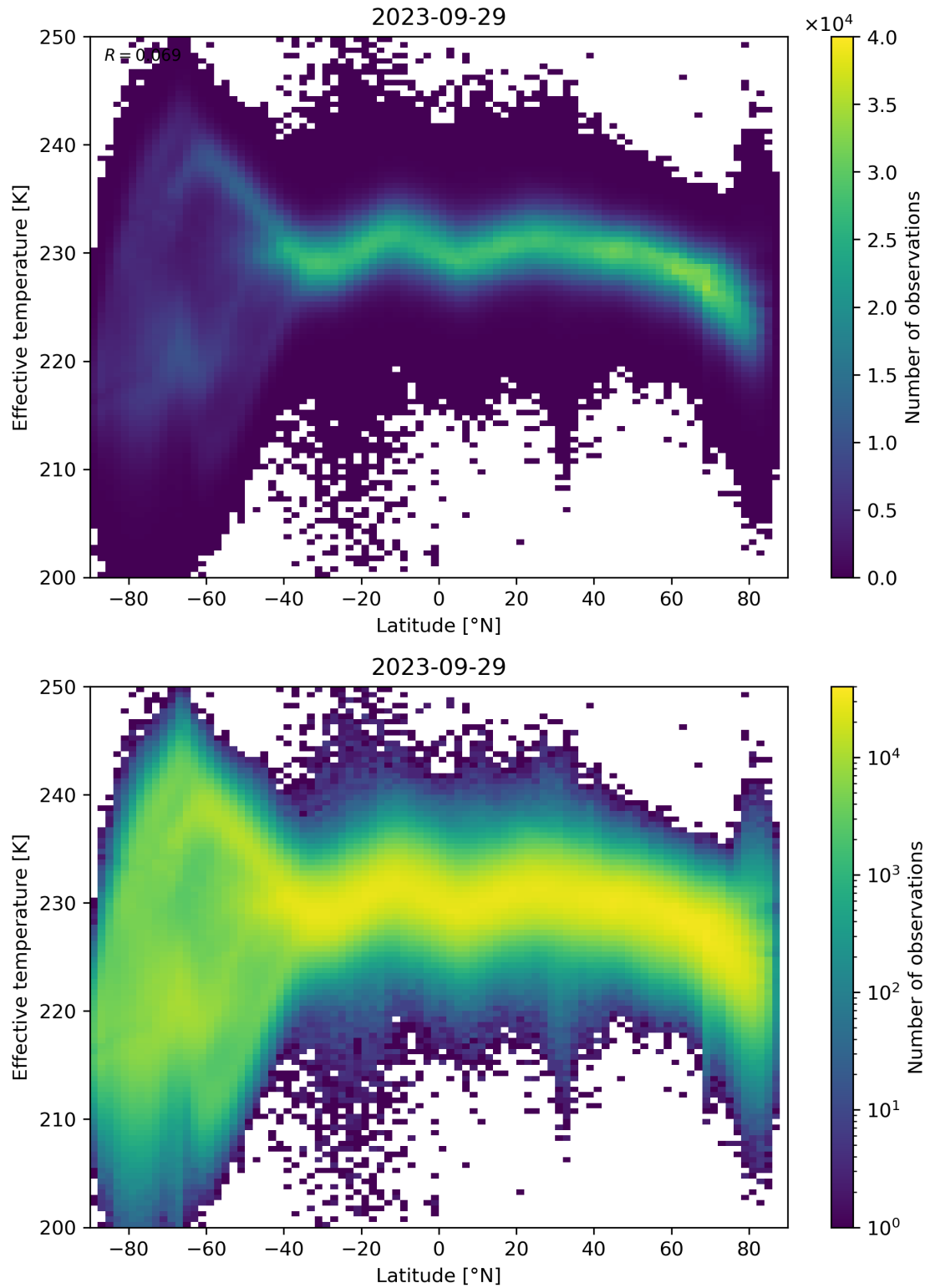
Figure 34: Scatter density plot of “Latitude” against “Effective temperature” for 2023-09-28 to 2023-09-30.
