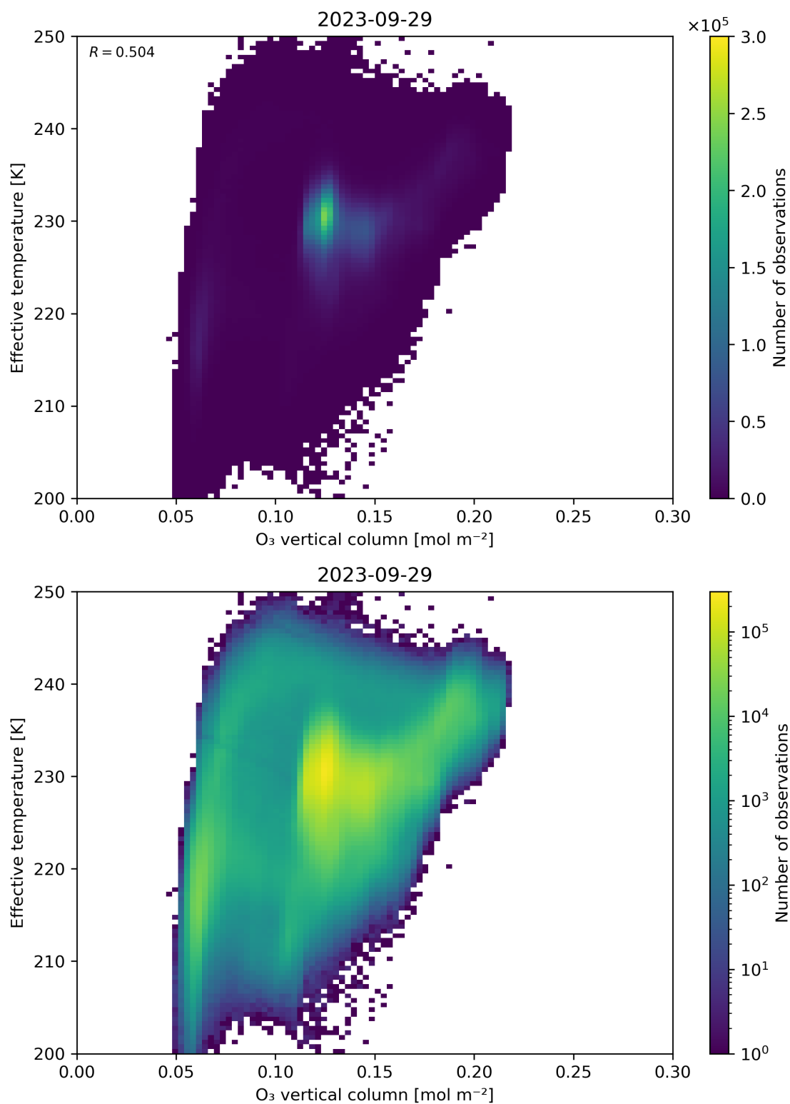
Figure 39: Scatter density plot of “O 3 vertical column” against “Effective temperature” for 2023-09-28 to 2023-09-30.
