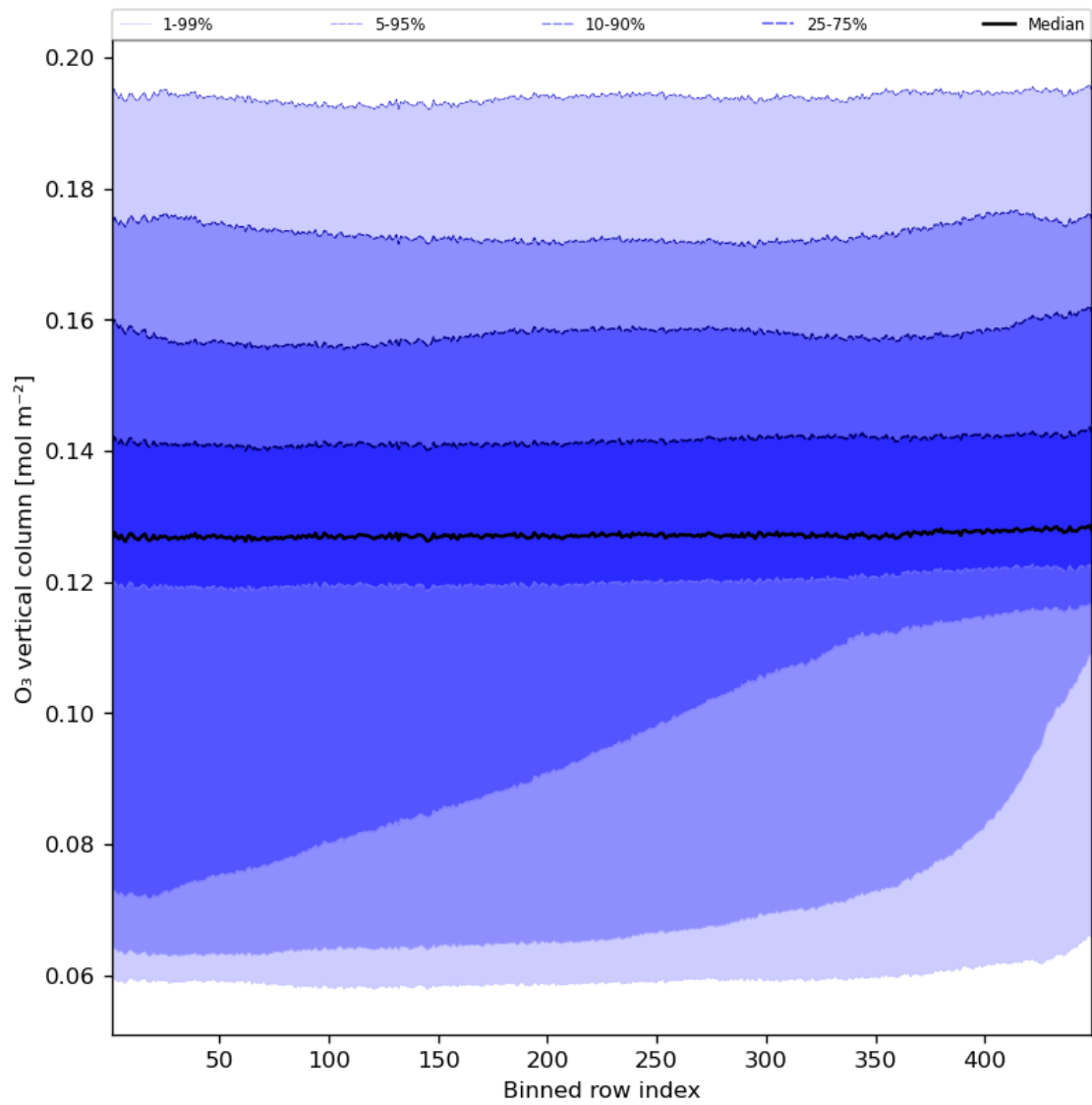
Figure 28: Along track statistics of “O 3 vertical column” for 2023-09-28 to 2023-09-30
