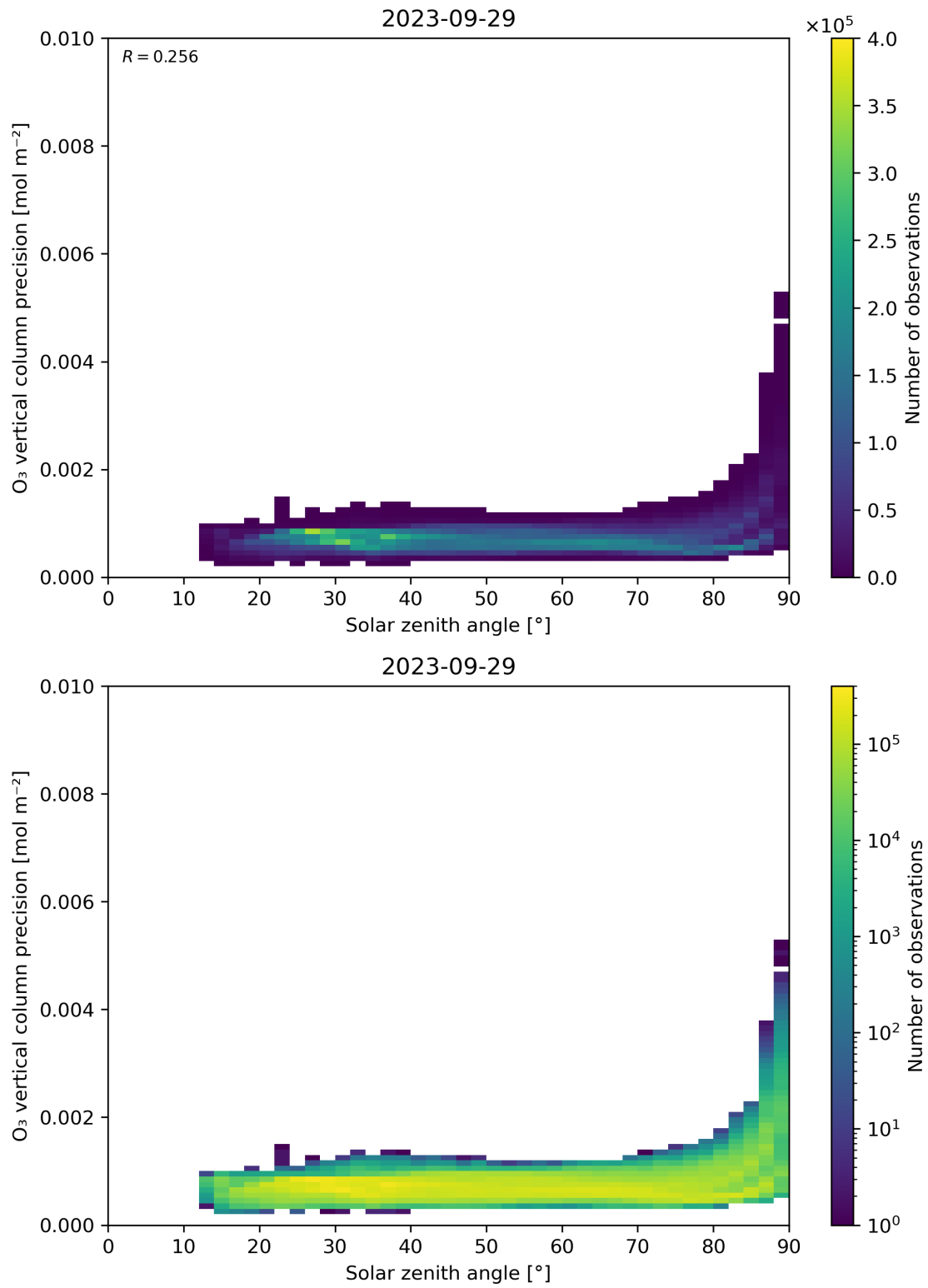
Figure 48: Scatter density plot of “Solar zenith angle” against “O 3 vertical column precision” for 2023-09-28 to 2023-09-30.
