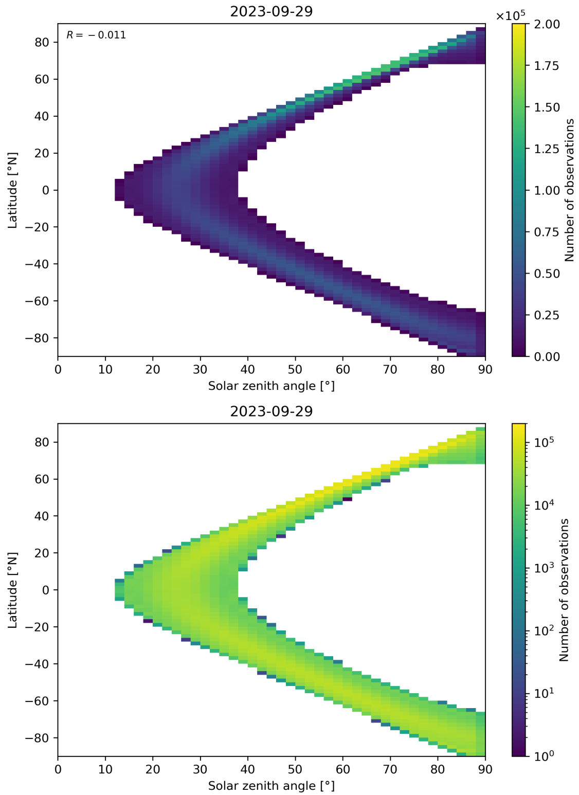
Figure 44: Scatter density plot of “Solar zenith angle” against “Latitude” for 2023-09-28 to 2023-09-30.
