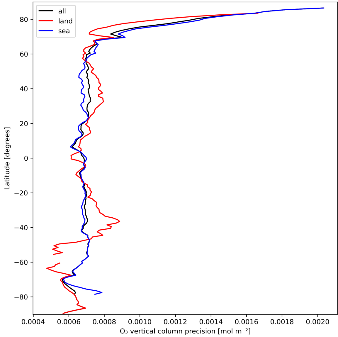
Figure 15: Zonal average of “O 3 vertical column precision” for 2023-09-28 to 2023-09-30.
