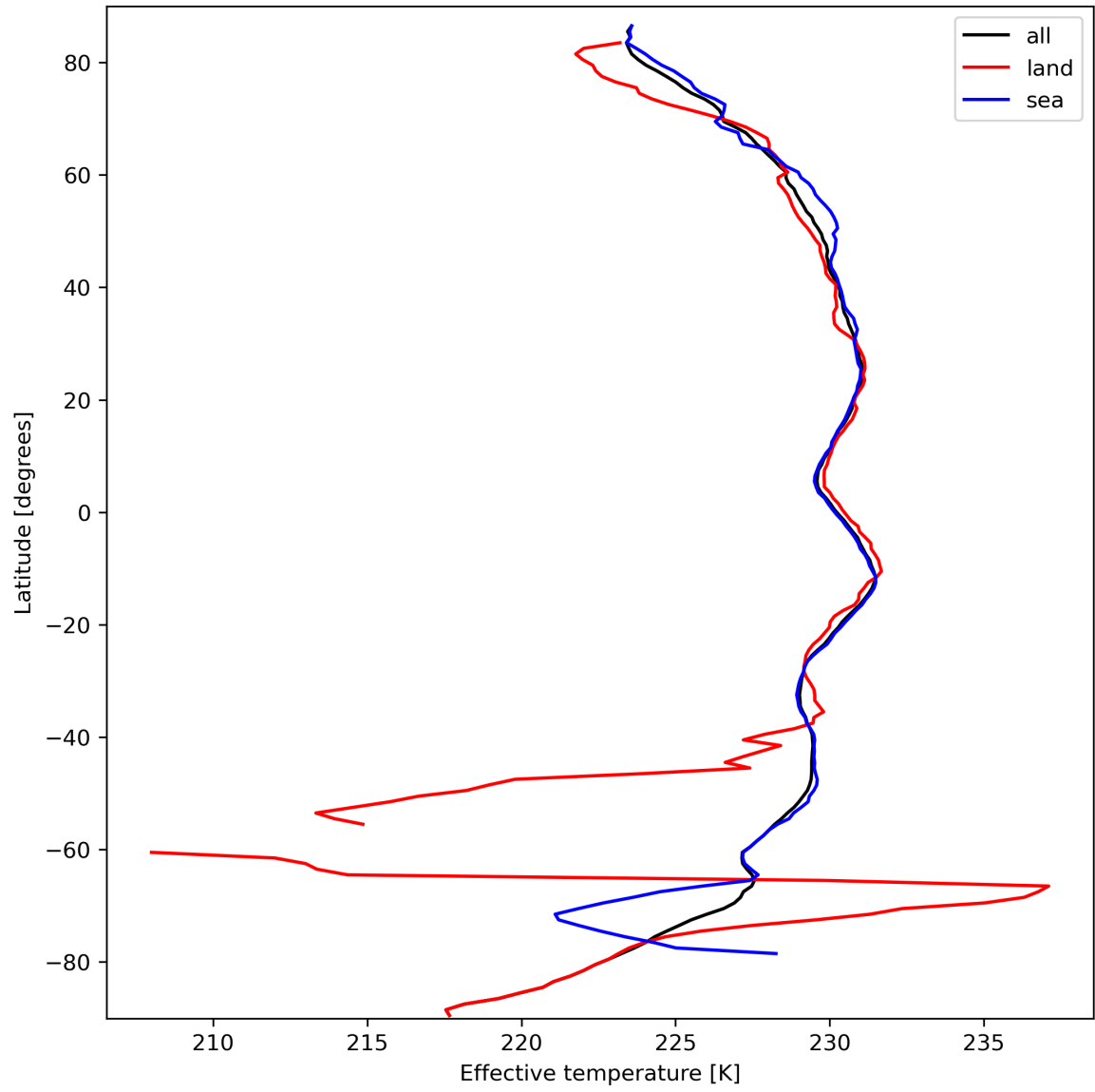
Figure 17: Zonal average of “Effective temperature” for 2023-09-28 to 2023-09-30.
