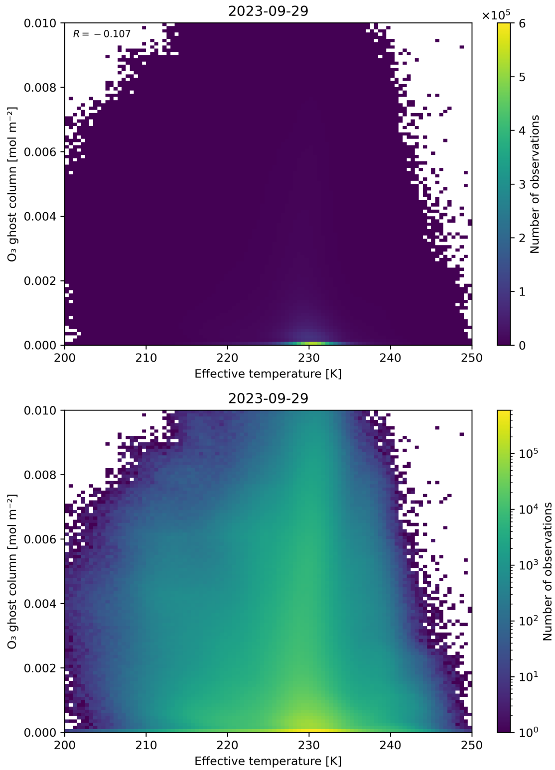
Figure 38: Scatter density plot of “Effective temperature” against “O 3 ghost column” for 2023-09-28 to 2023-09-30.
