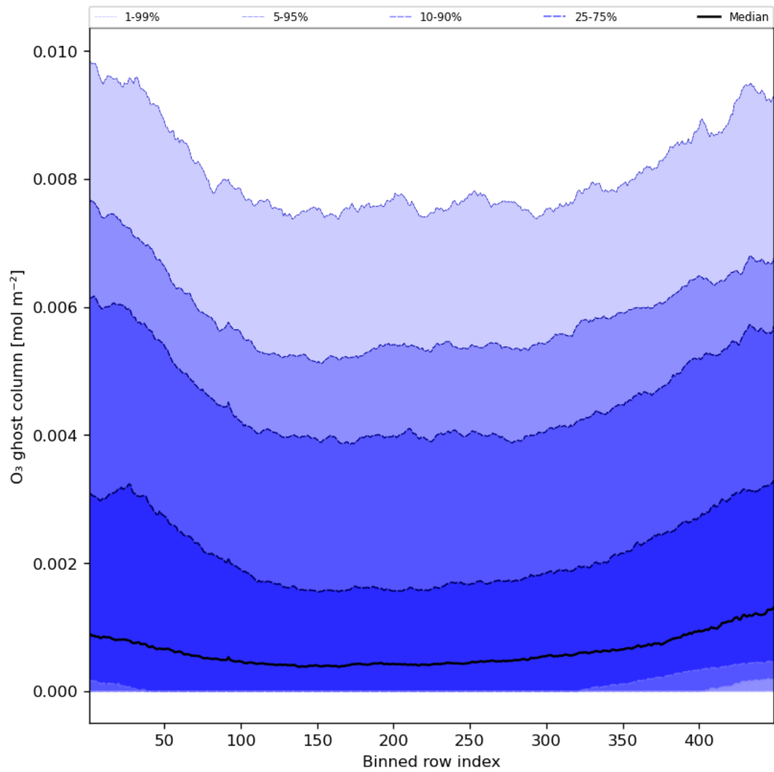
Figure 32: Along track statistics of “O 3 ghost column” for 2023-09-28 to 2023-09-30
