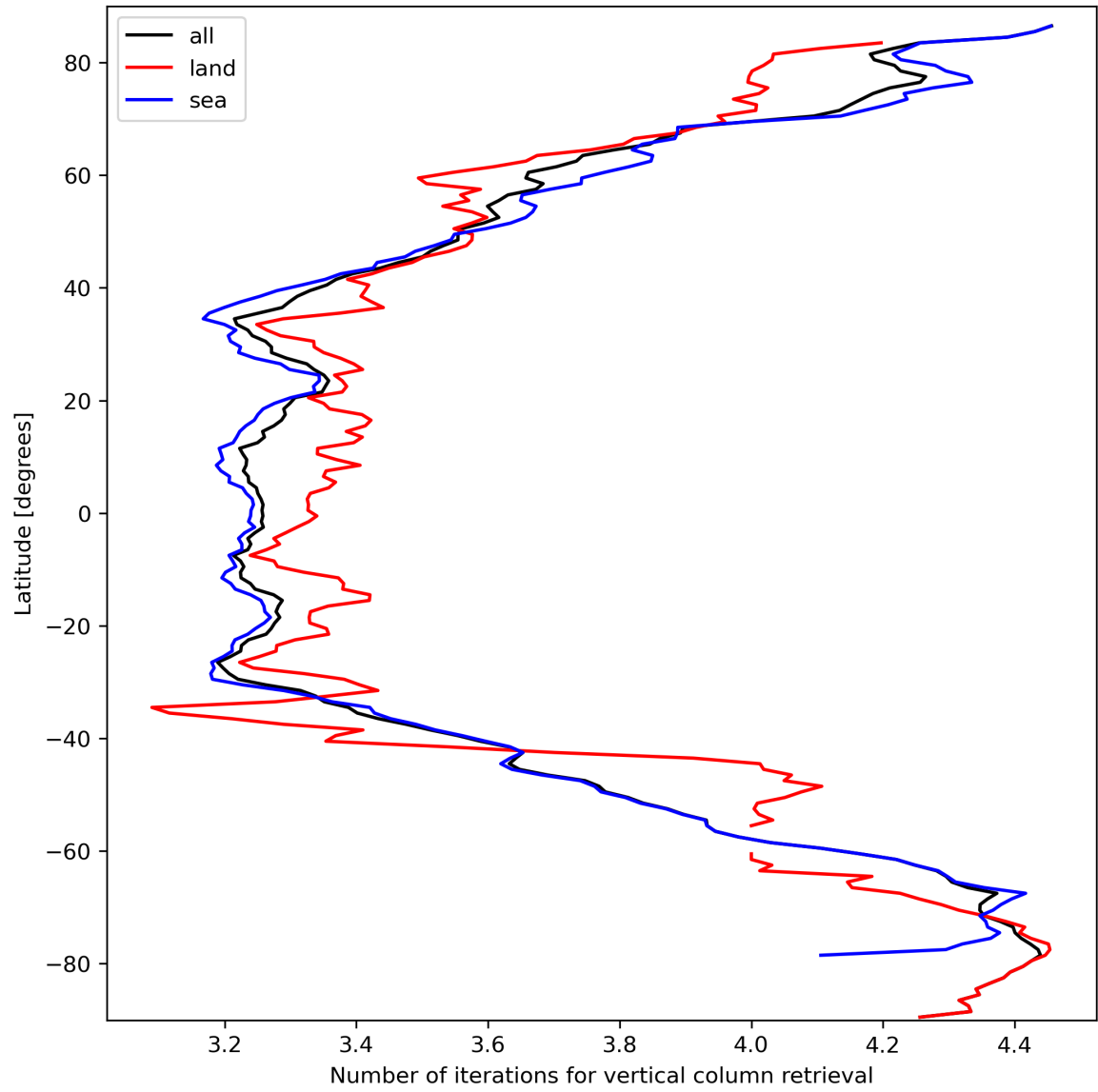
Figure 19: Zonal average of “Number of iterations for vertical column retrieval” for 2023-09-28 to 2023-09-30.
