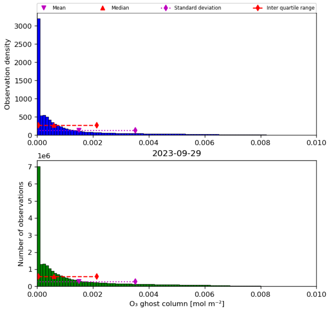
Figure 25: Histogram of “O 3 ghost column” for 2023-09-28 to 2023-09-30
