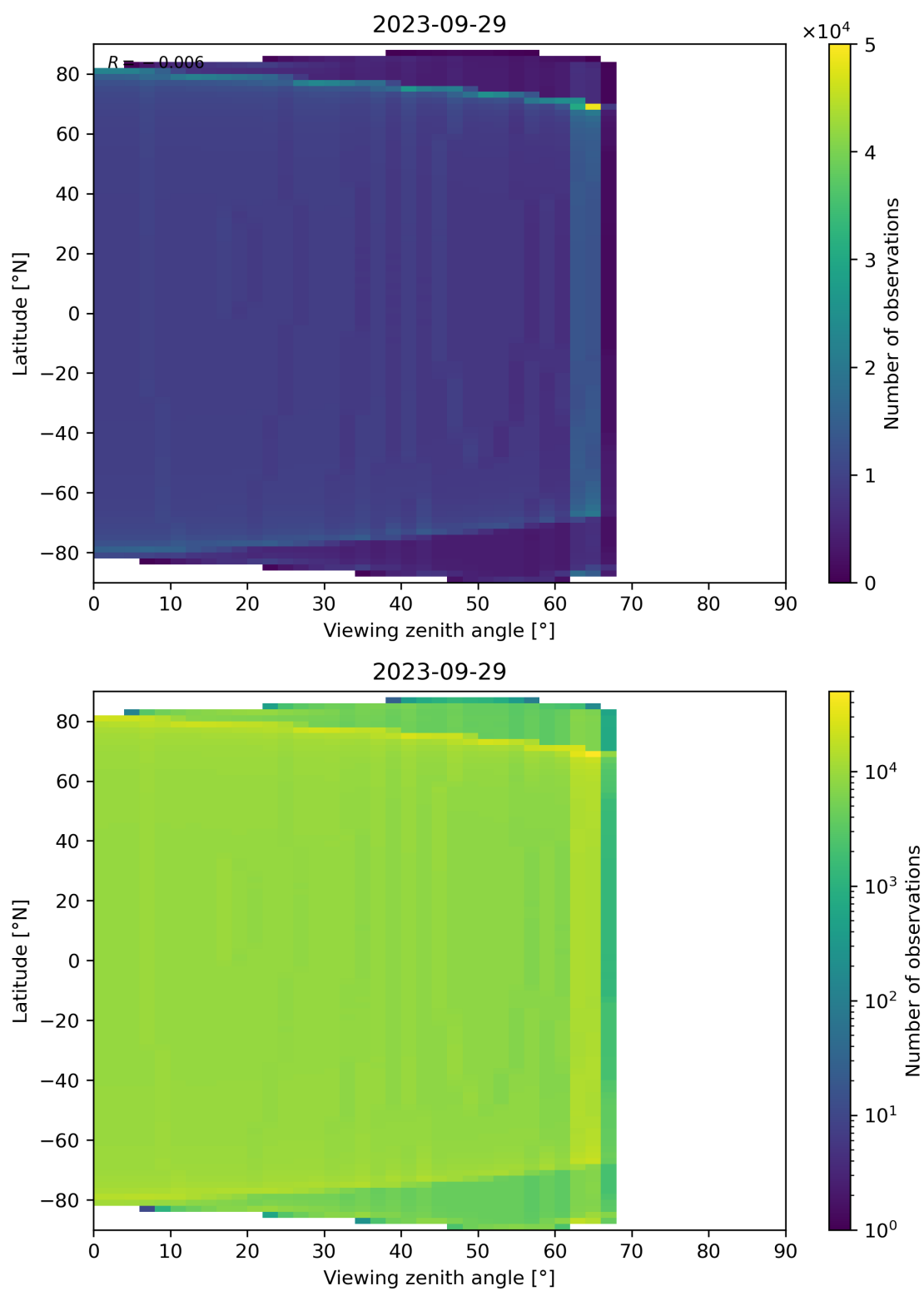
Figure 49: Scatter density plot of “Viewing zenith angle” against “Latitude” for 2023-09-28 to 2023-09-30.
