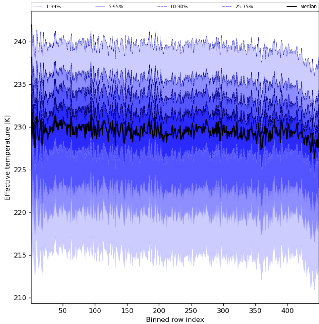
Figure 31: Along track statistics of “Effective temperature” for 2023-09-29 to 2023-10-01
