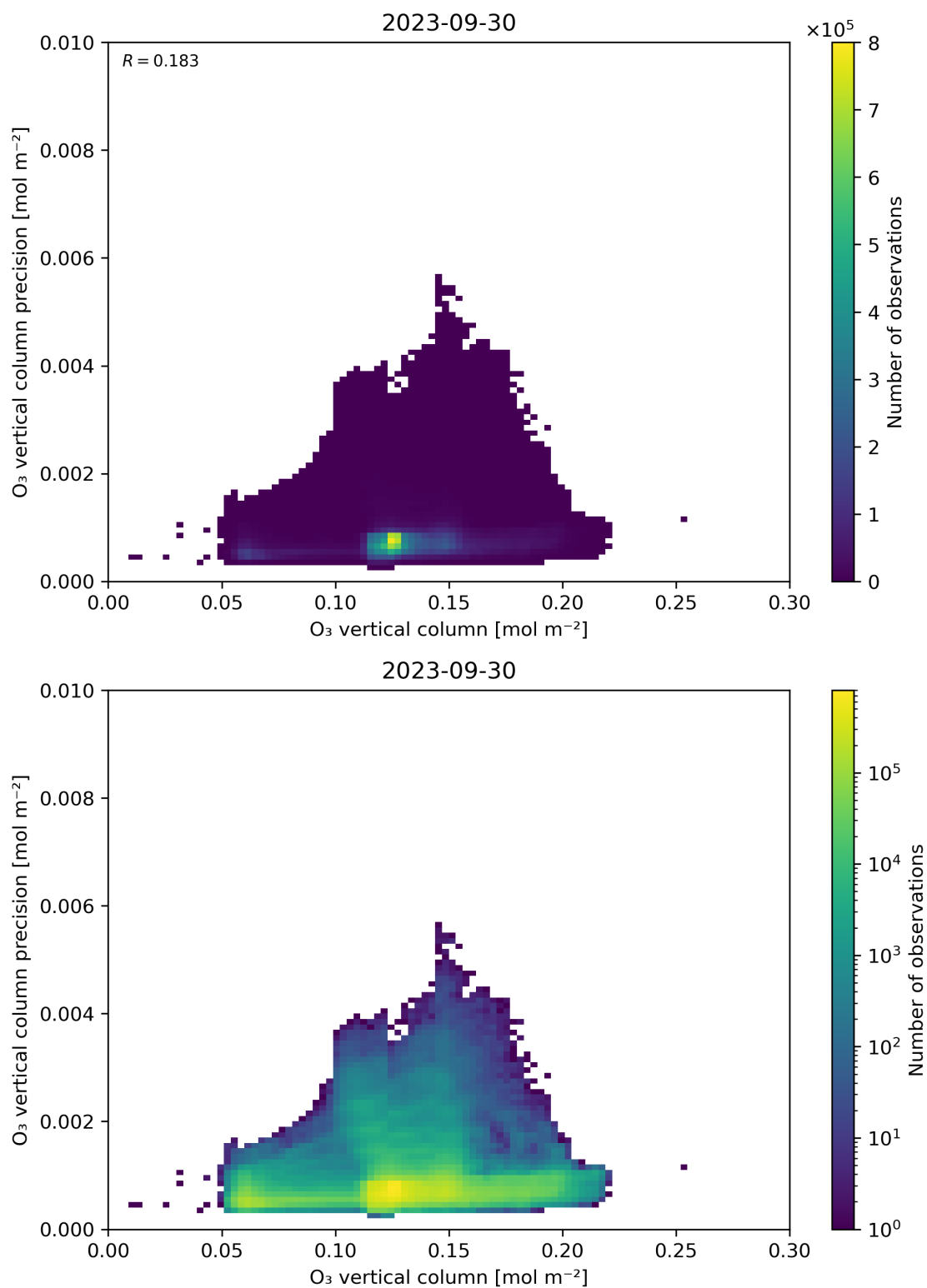
Figure 41: Scatter density plot of “O 3 vertical column” against “O 3 vertical column precision” for 2023-09-29 to 2023-10-01.
