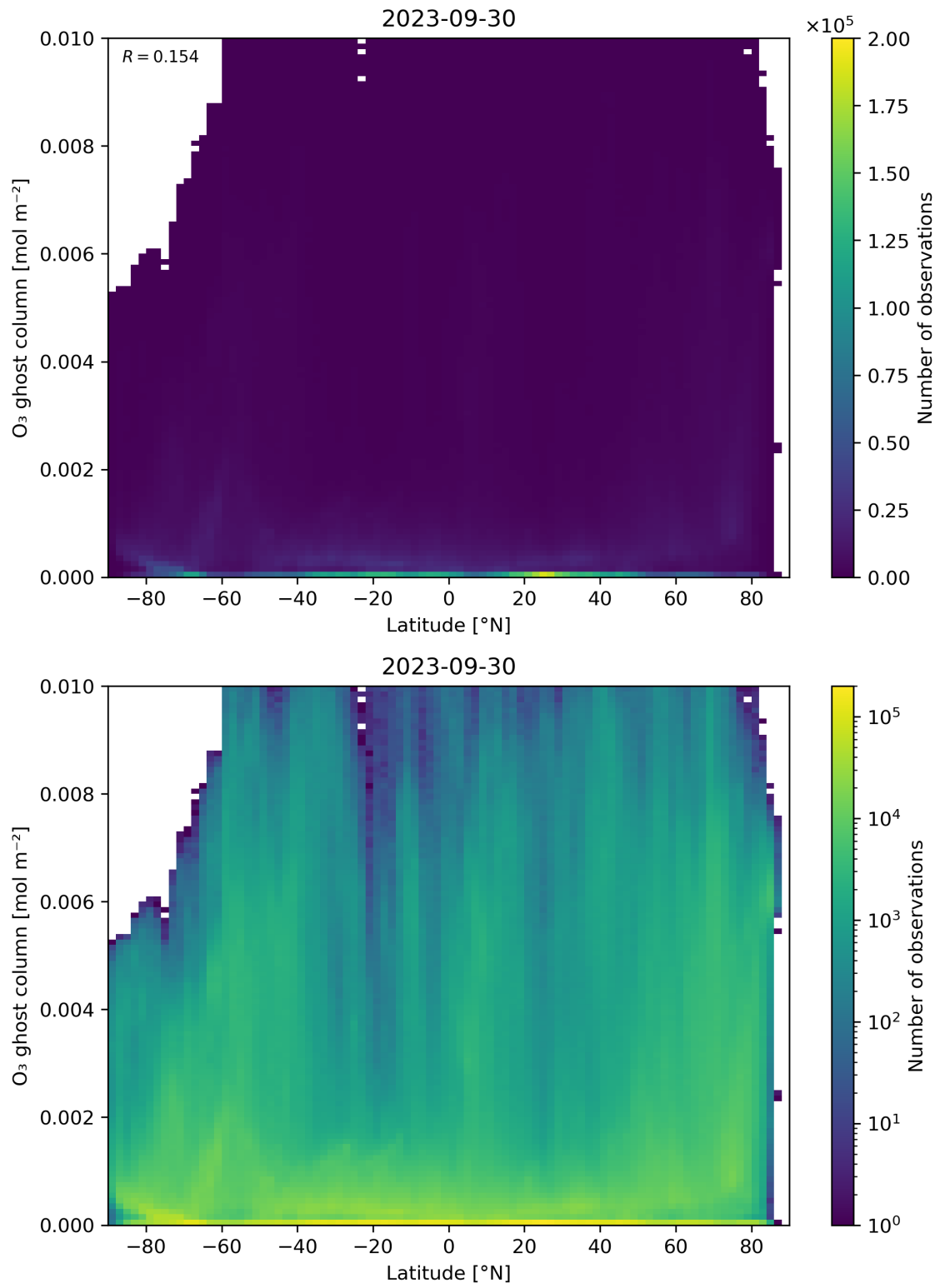
Figure 35: Scatter density plot of “Latitude” against “O 3 ghost column” for 2023-09-29 to 2023-10-01.
