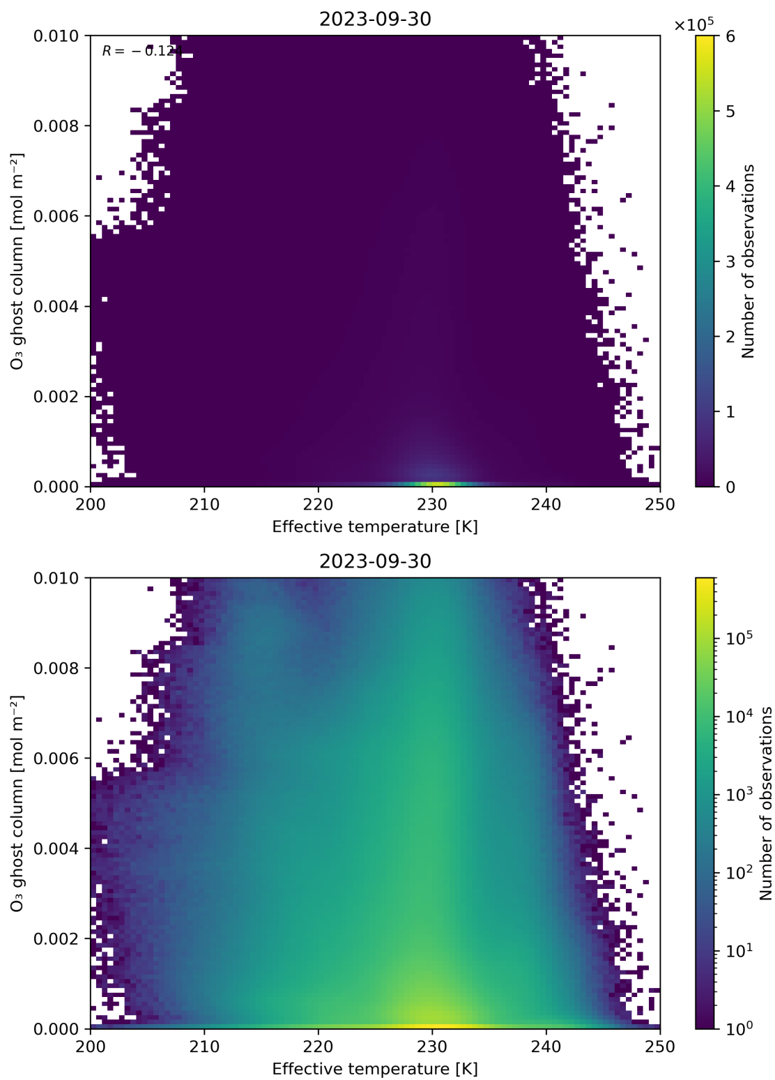
Figure 38: Scatter density plot of “Effective temperature” against “O 3 ghost column” for 2023-09-29 to 2023-10-01.
