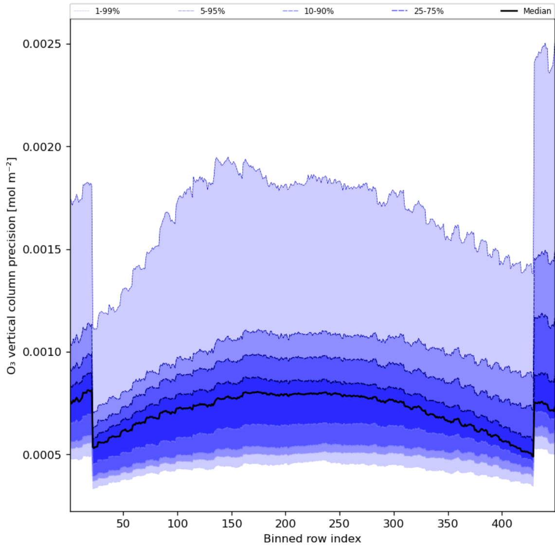
Figure 29: Along track statistics of “O 3 vertical column precision” for 2023-09-29 to 2023-10-01
