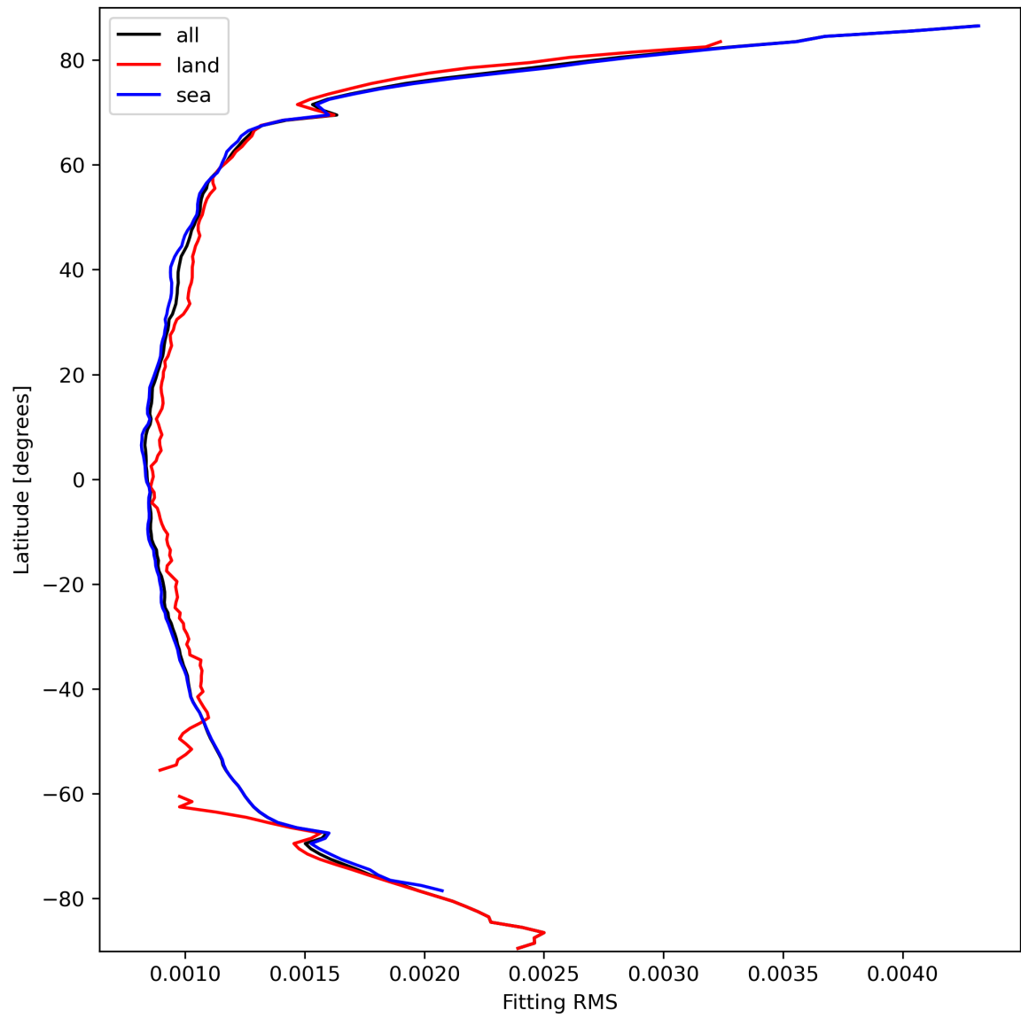
Figure 16: Zonal average of “Fitting RMS” for 2023-09-29 to 2023-10-01.
