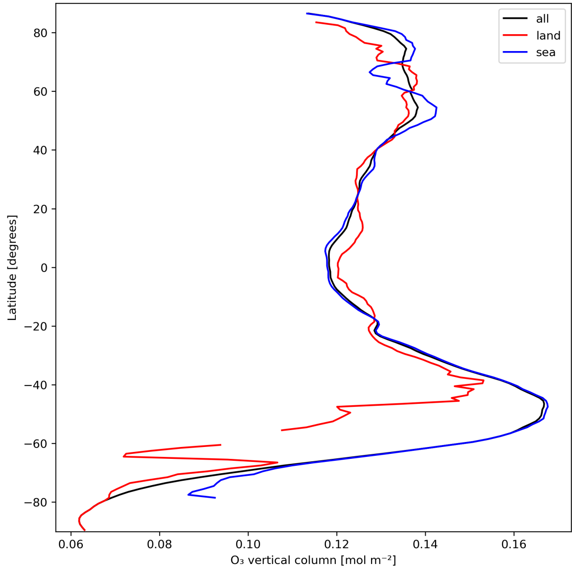
Figure 14: Zonal average of “O 3 vertical column” for 2023-09-29 to 2023-10-01.
