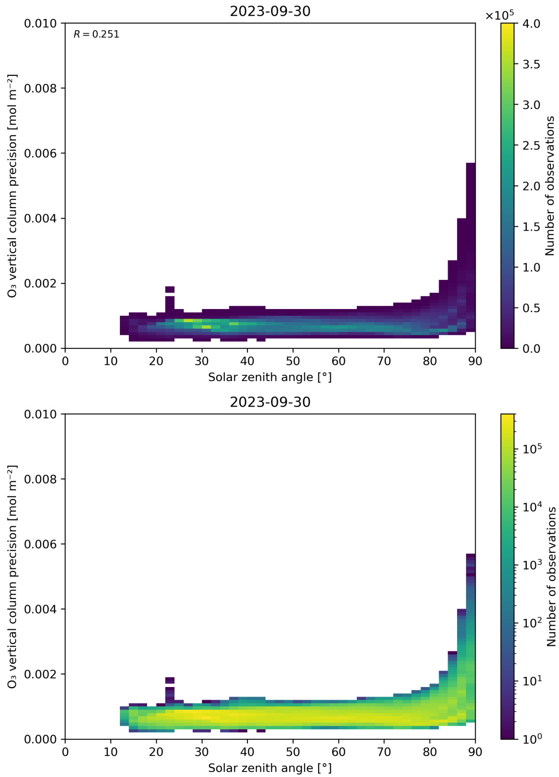
Figure 48: Scatter density plot of “Solar zenith angle” against “O 3 vertical column precision” for 2023-09-29 to 2023-10-01.
