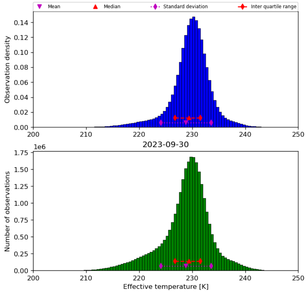
Figure 24: Histogram of “Effective temperature” for 2023-09-29 to 2023-10-01
