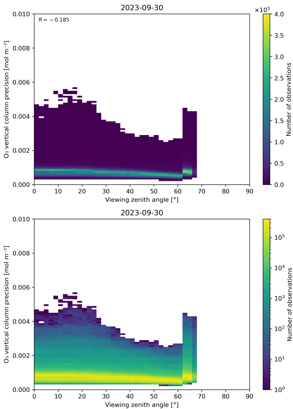
Figure 53: Scatter density plot of “Viewing zenith angle” against “O 3 vertical column precision” for 2023-09-29 to 2023-10-01.
