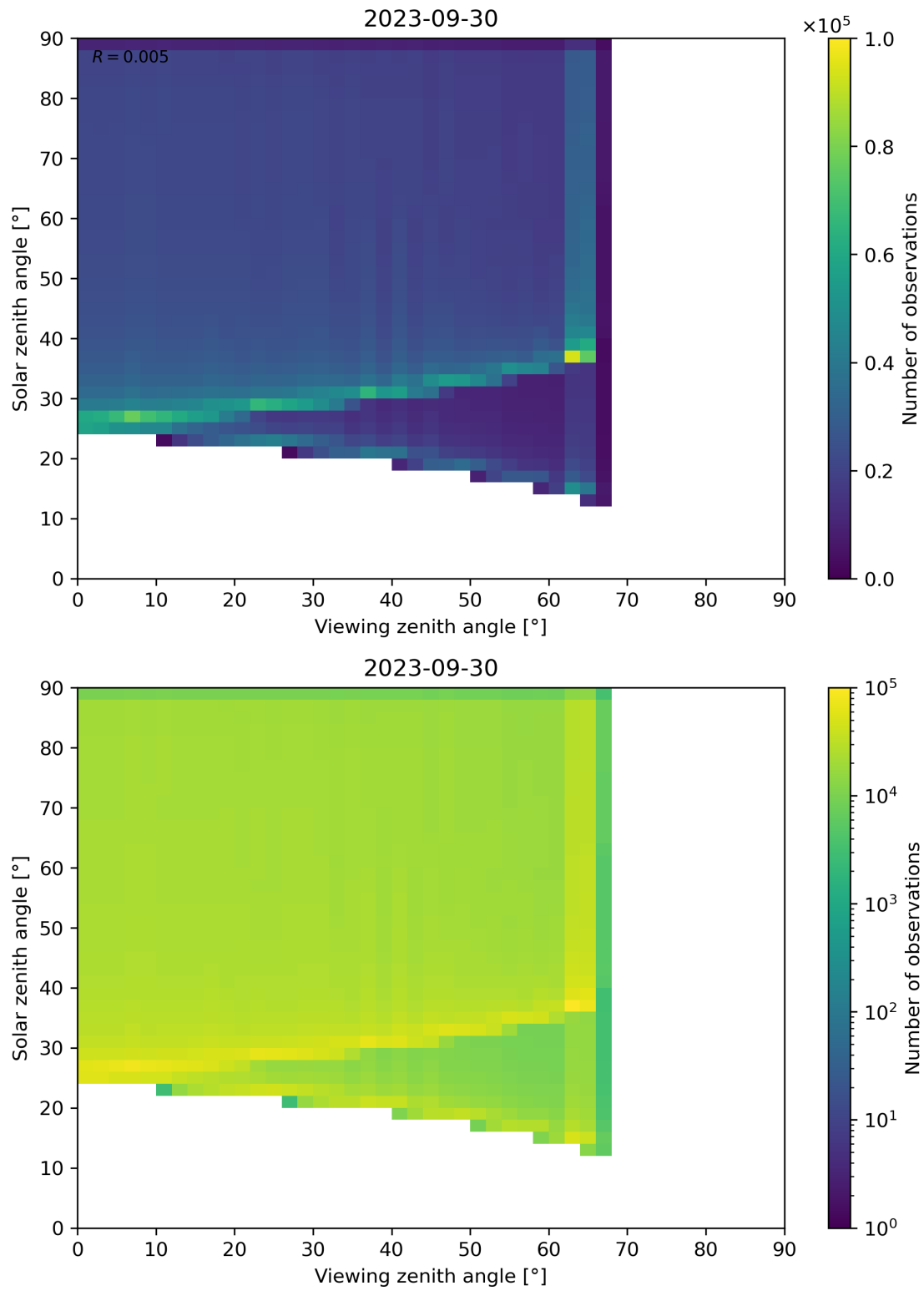
Figure 54: Scatter density plot of “Viewing zenith angle” against “Solar zenith angle” for 2023-09-29 to 2023-10-01.
