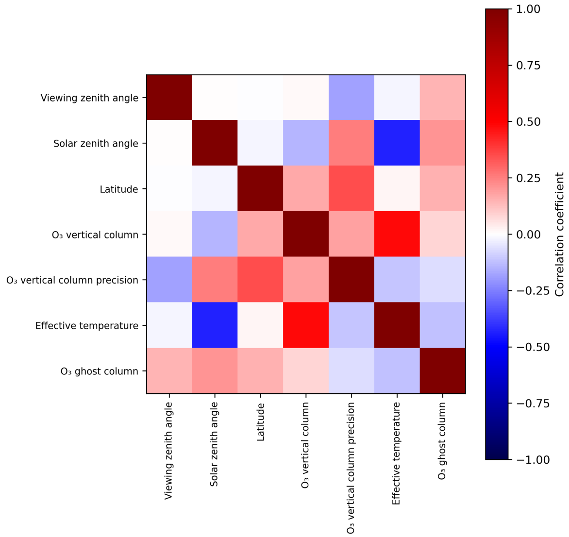
Figure 2: Map of correlation matrix for 2023-09-29 to 2023-10-01.
