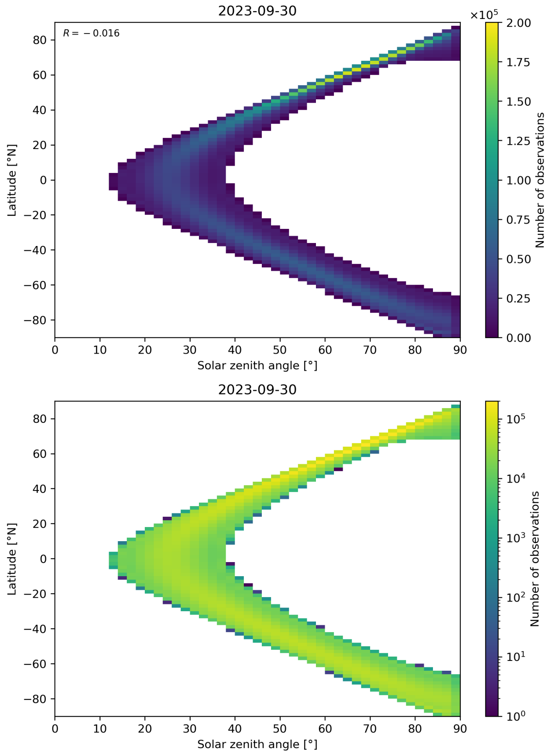
Figure 44: Scatter density plot of “Solar zenith angle” against “Latitude” for 2023-09-29 to 2023-10-01.
