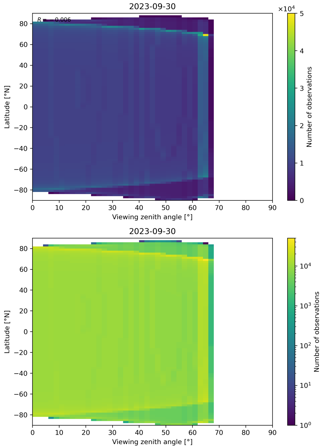
Figure 49: Scatter density plot of “Viewing zenith angle” against “Latitude” for 2023-09-29 to 2023-10-01.
