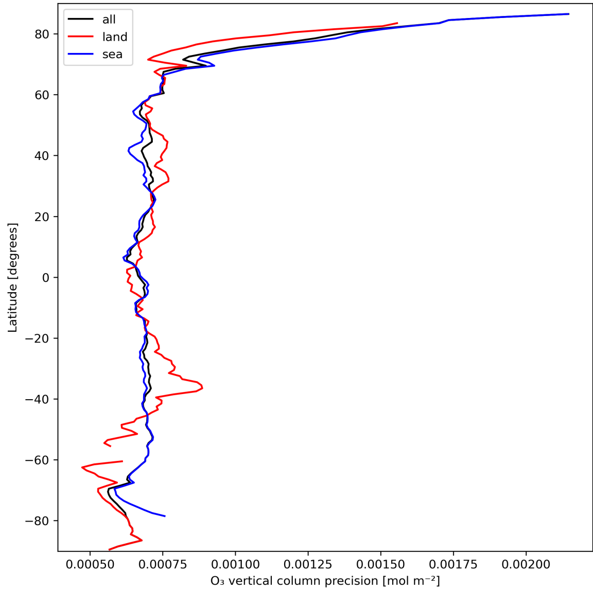
Figure 15: Zonal average of “O 3 vertical column precision” for 2023-09-29 to 2023-10-01.
