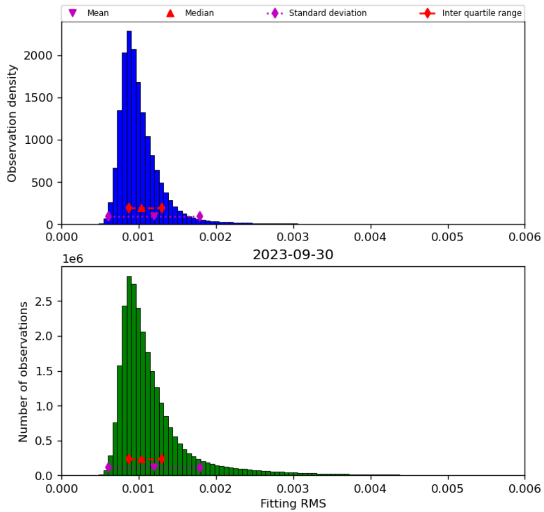
Figure 23: Histogram of “Fitting RMS” for 2023-09-29 to 2023-10-01
