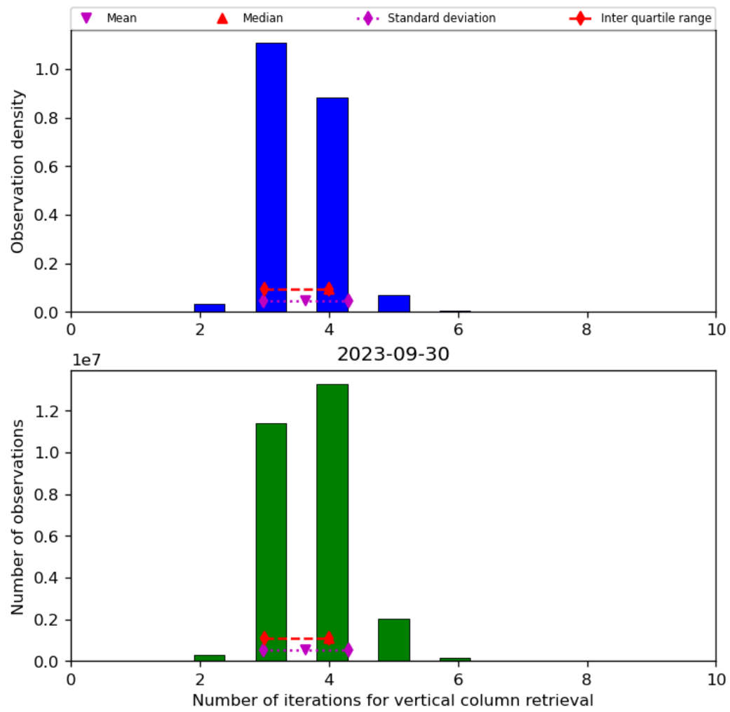
Figure 26: Histogram of “Number of iterations for vertical column retrieval” for 2023-09-29 to 2023-10-01
