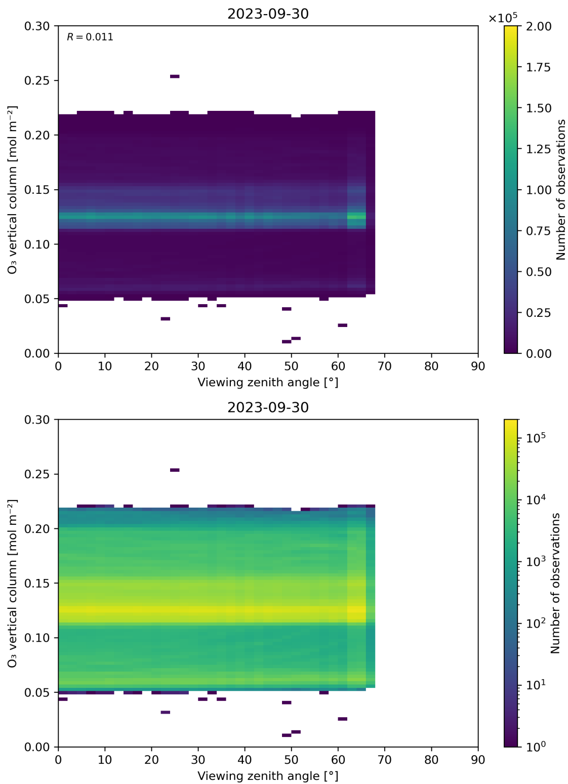
Figure 52: Scatter density plot of “Viewing zenith angle” against “O 3 vertical column” for 2023-09-29 to 2023-10-01.
