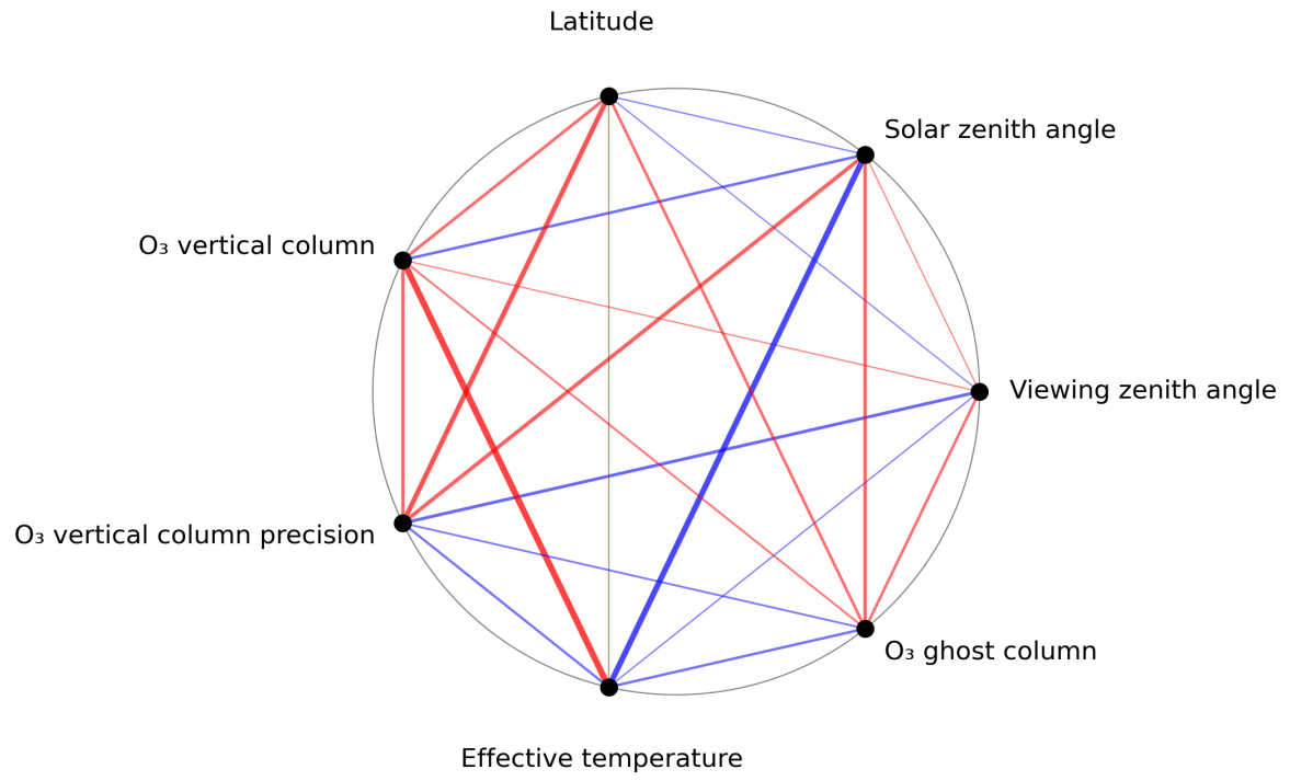
Figure 1: Map of correlation graph for 2023-09-29 to 2023-10-01.
