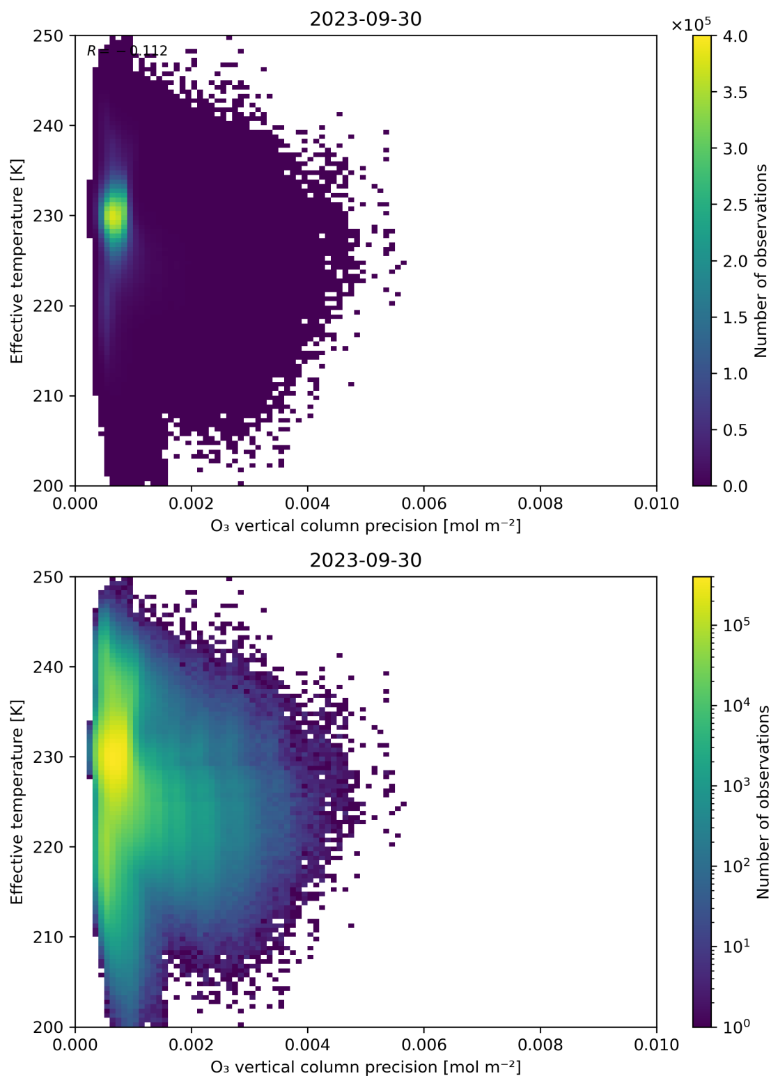
Figure 42: Scatter density plot of “O 3 vertical column precision” against “Effective temperature” for 2023-09-29 to 2023-10-01.
