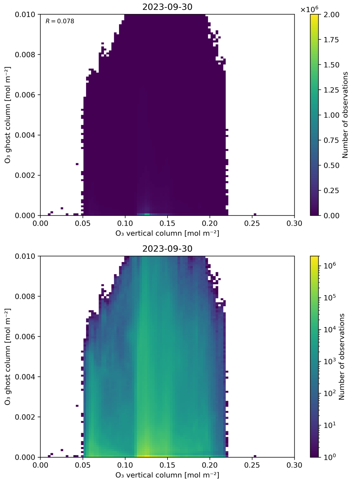
Figure 40: Scatter density plot of “O 3 vertical column” against “O 3 ghost column” for 2023-09-29 to 2023-10-01.
