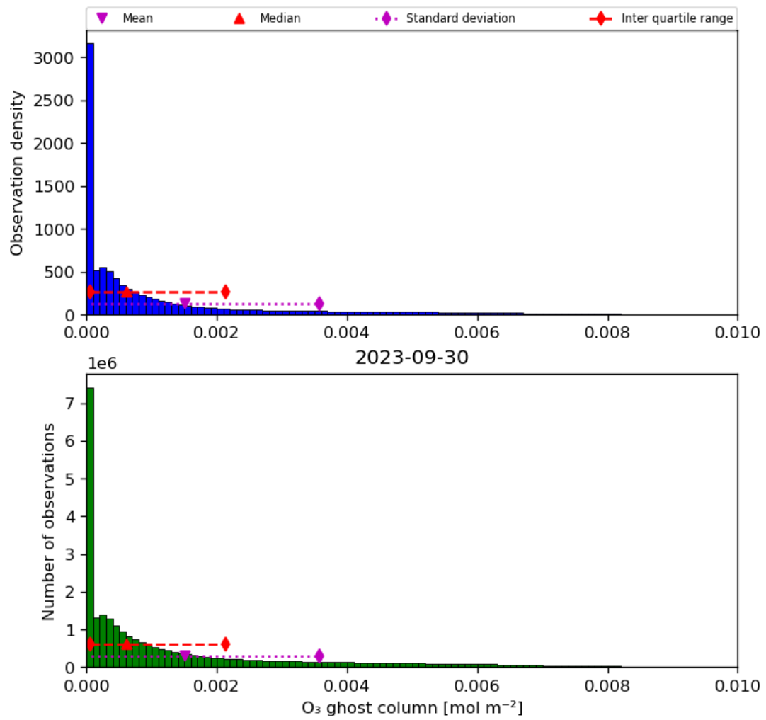
Figure 25: Histogram of “O 3 ghost column” for 2023-09-29 to 2023-10-01
