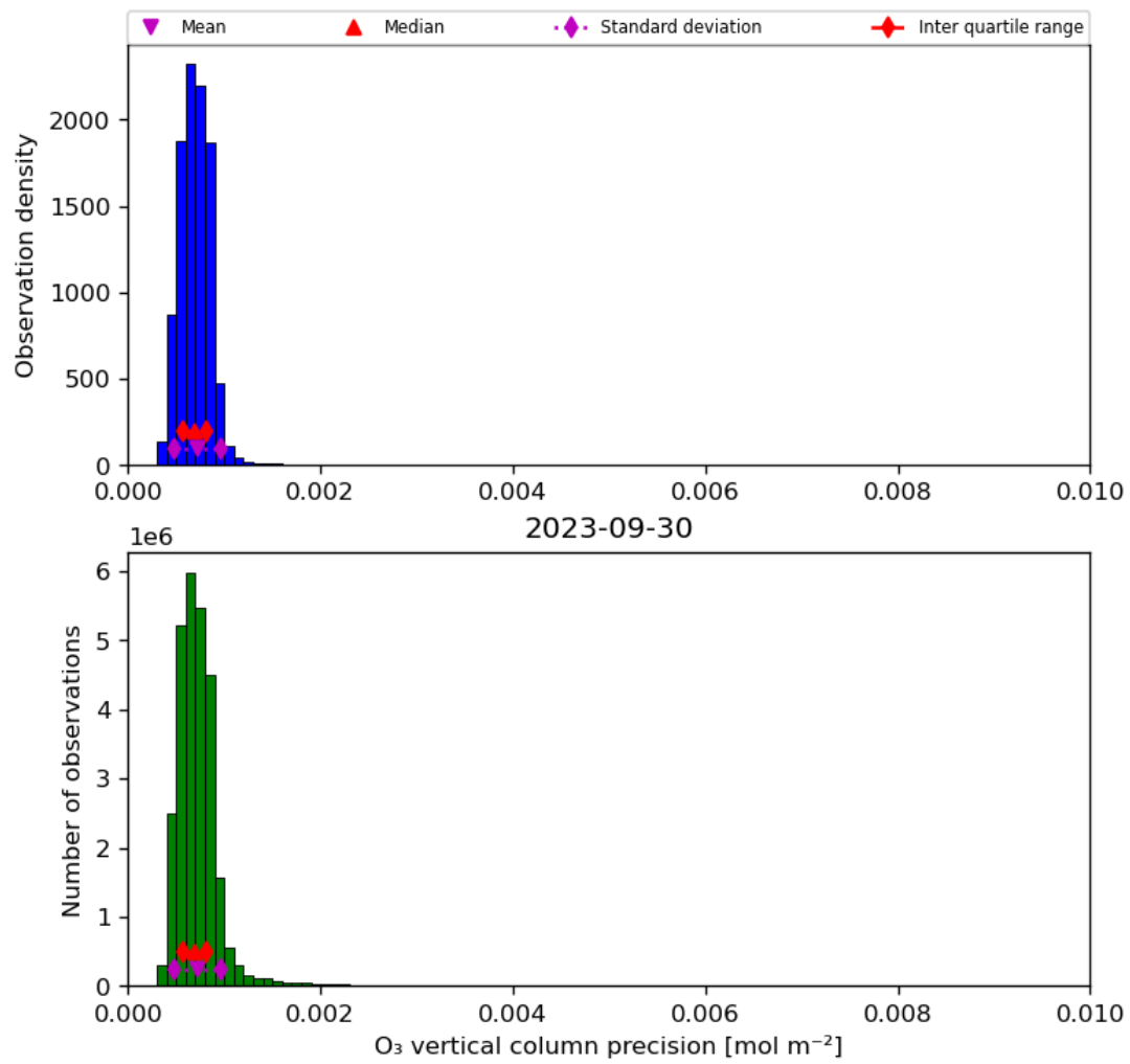
Figure 22: Histogram of “O 3 vertical column precision” for 2023-09-29 to 2023-10-01
