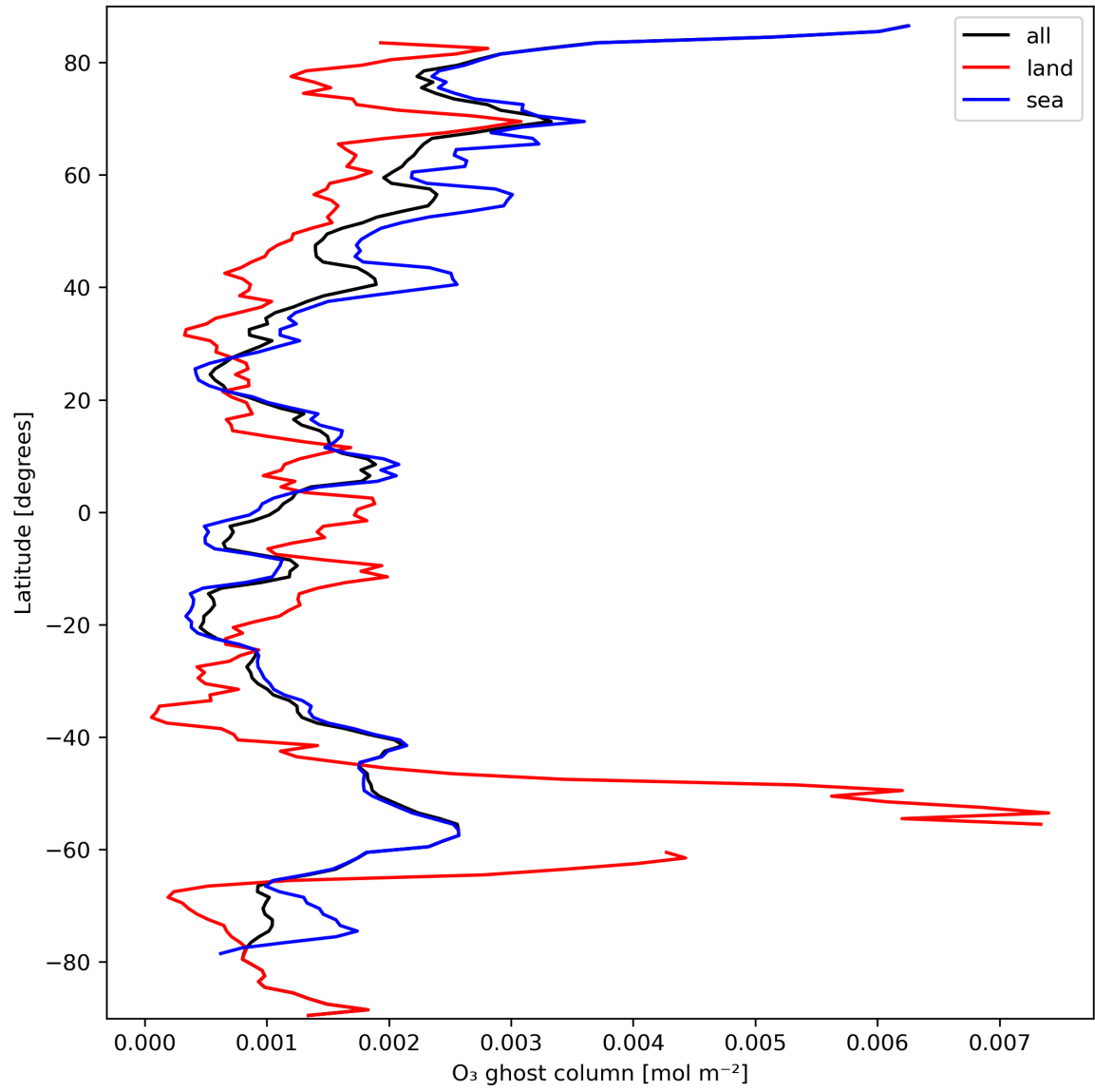
Figure 18: Zonal average of “O 3 ghost column” for 2023-09-29 to 2023-10-01.
