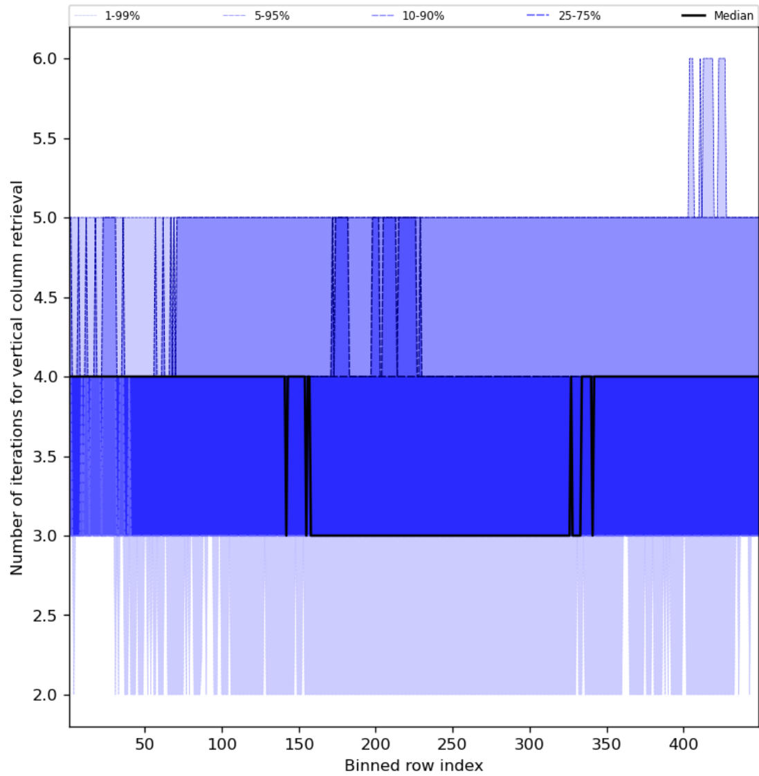
Figure 33: Along track statistics of “Number of iterations for vertical column retrieval” for 2023-09-29 to 2023-10-01
