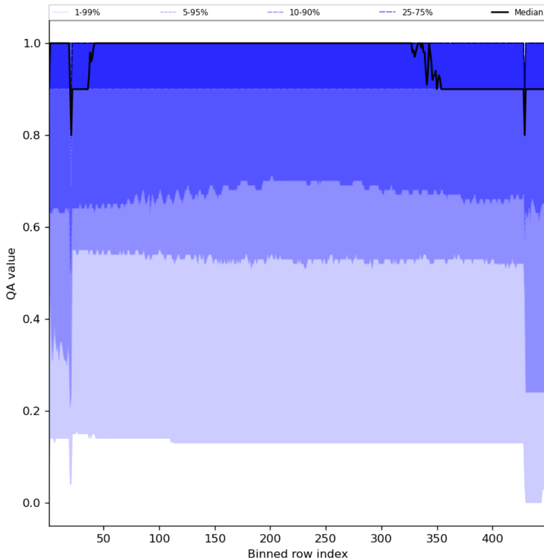
Figure 27: Along track statistics of “QA value” for 2023-09-29 to 2023-10-01
