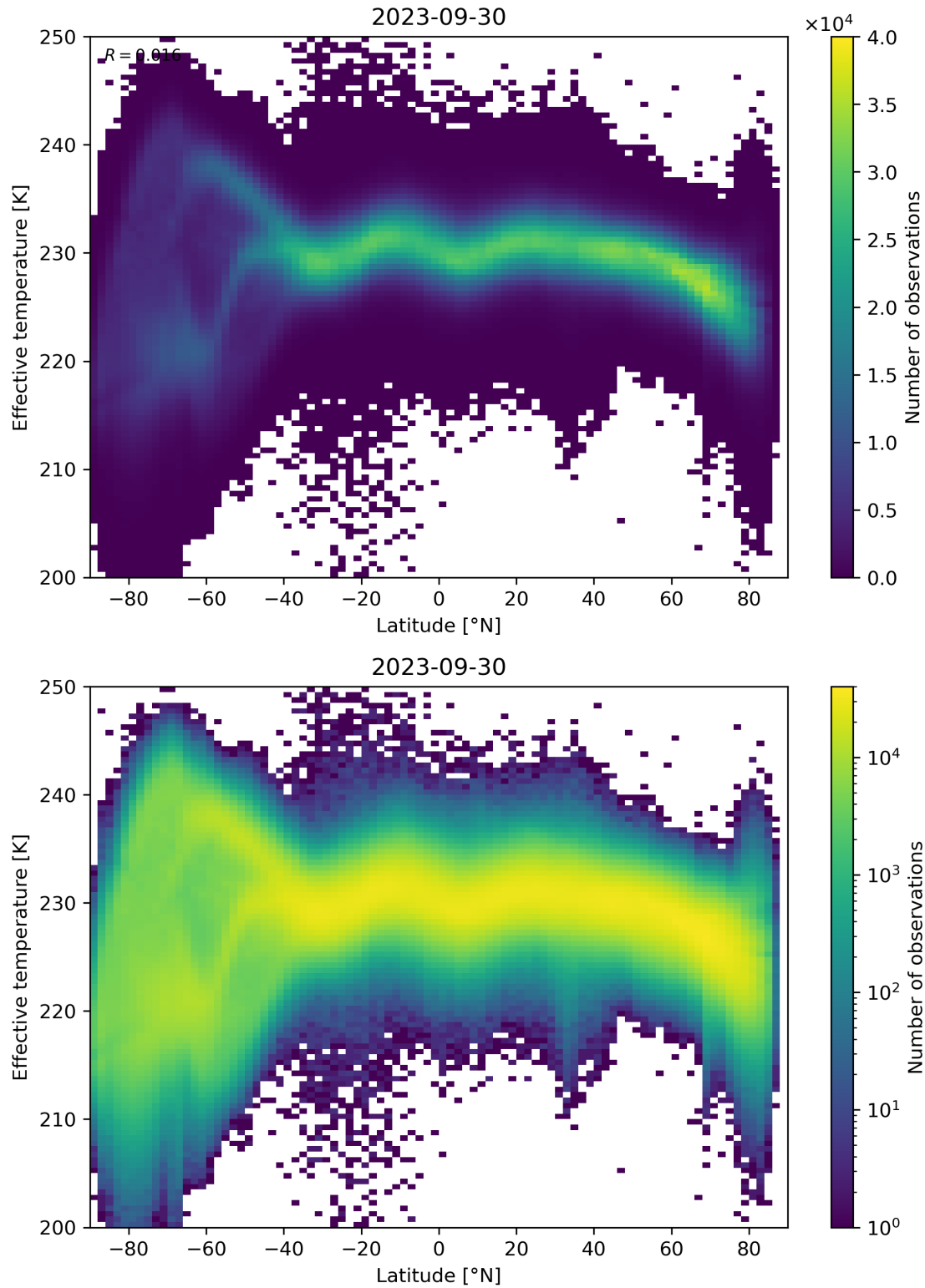
Figure 34: Scatter density plot of “Latitude” against “Effective temperature” for 2023-09-29 to 2023-10-01.
