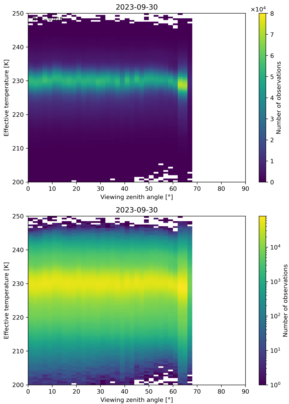
Figure 50: Scatter density plot of “Viewing zenith angle” against “Effective temperature” for 2023-09-29 to 2023-10-01.
