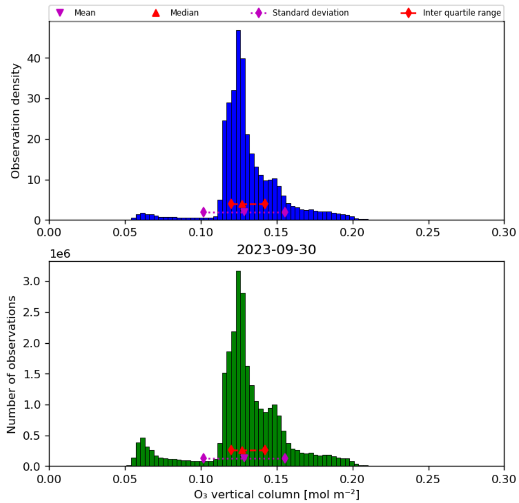
Figure 21: Histogram of “O 3 vertical column” for 2023-09-29 to 2023-10-01
