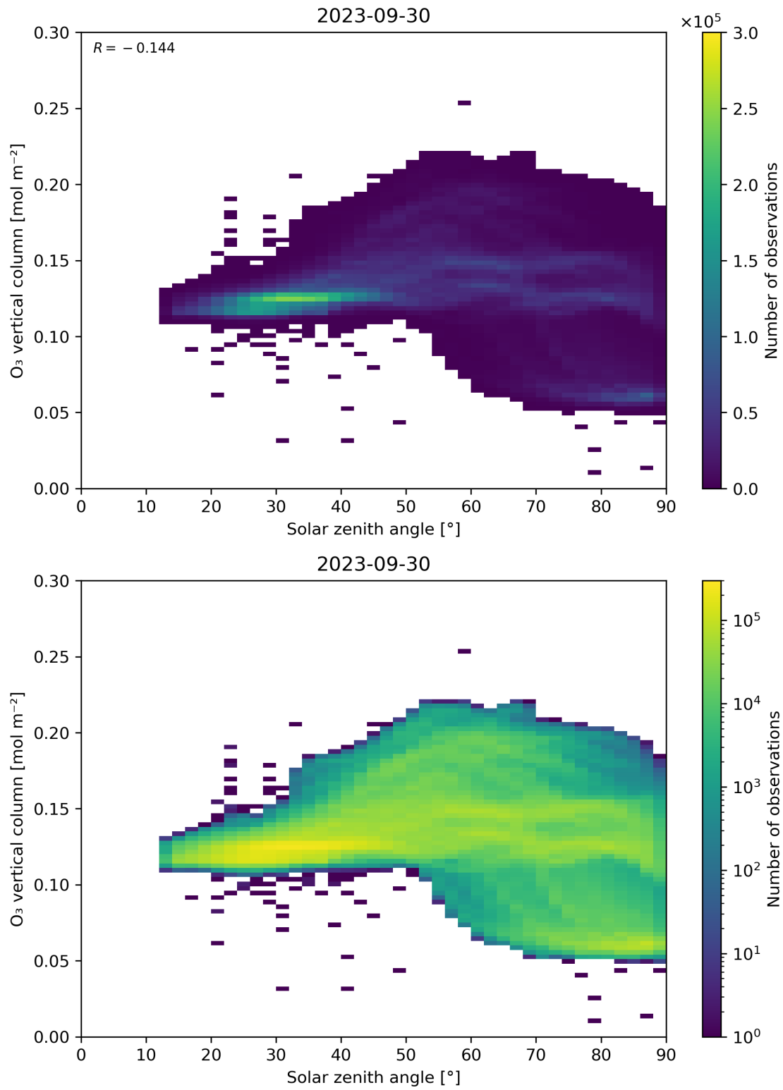
Figure 47: Scatter density plot of “Solar zenith angle” against “O 3 vertical column” for 2023-09-29 to 2023-10-01.
