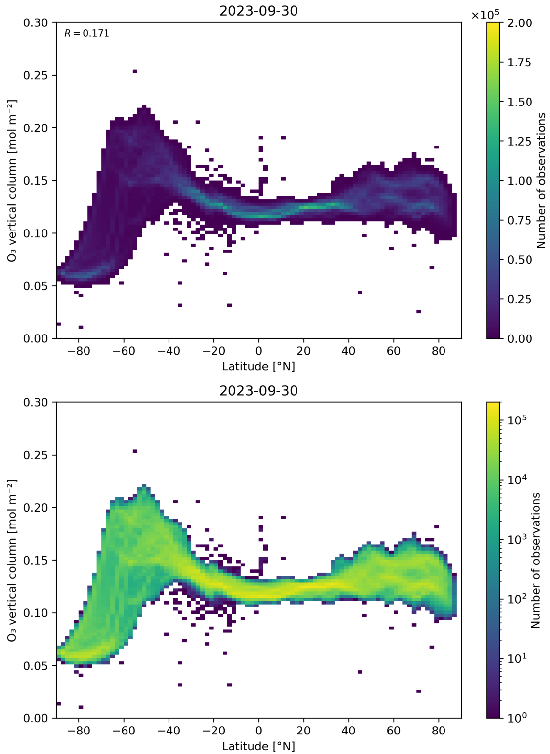
Figure 36: Scatter density plot of “Latitude” against “O 3 vertical column” for 2023-09-29 to 2023-10-01.
