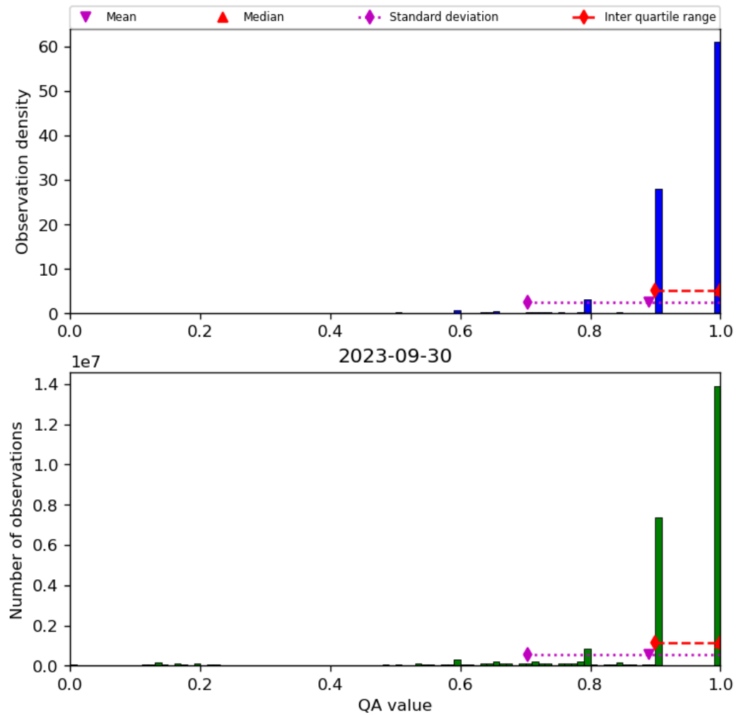
Figure 20: Histogram of “QA value” for 2023-09-29 to 2023-10-01
