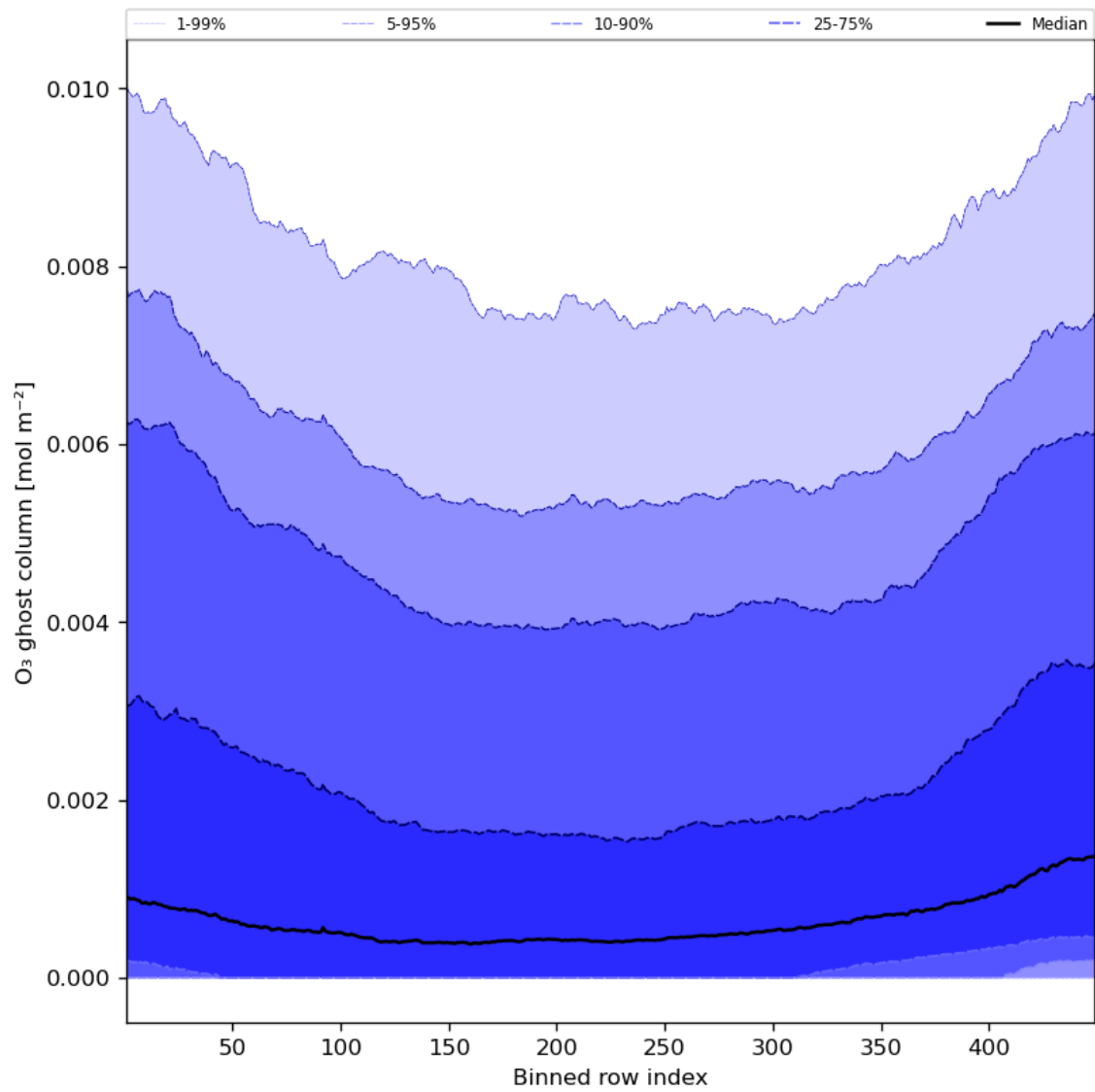
Figure 32: Along track statistics of “O 3 ghost column” for 2023-09-29 to 2023-10-01
