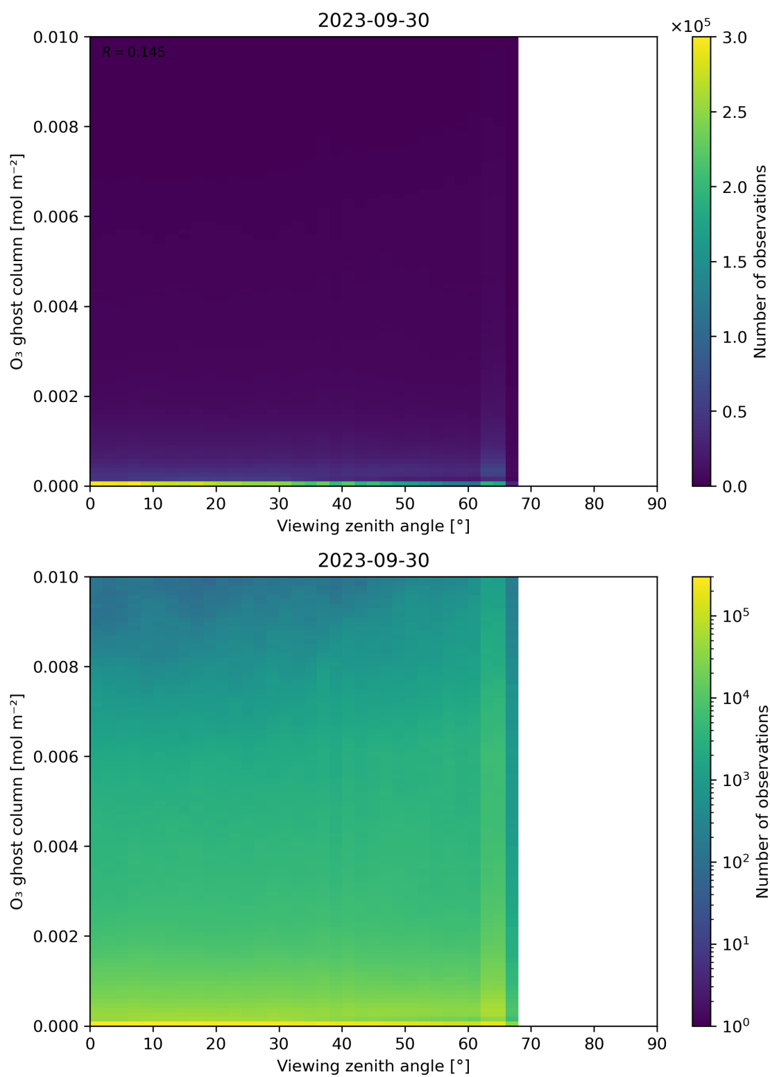
Figure 51: Scatter density plot of “Viewing zenith angle” against “O 3 ghost column” for 2023-09-29 to 2023-10-01.
