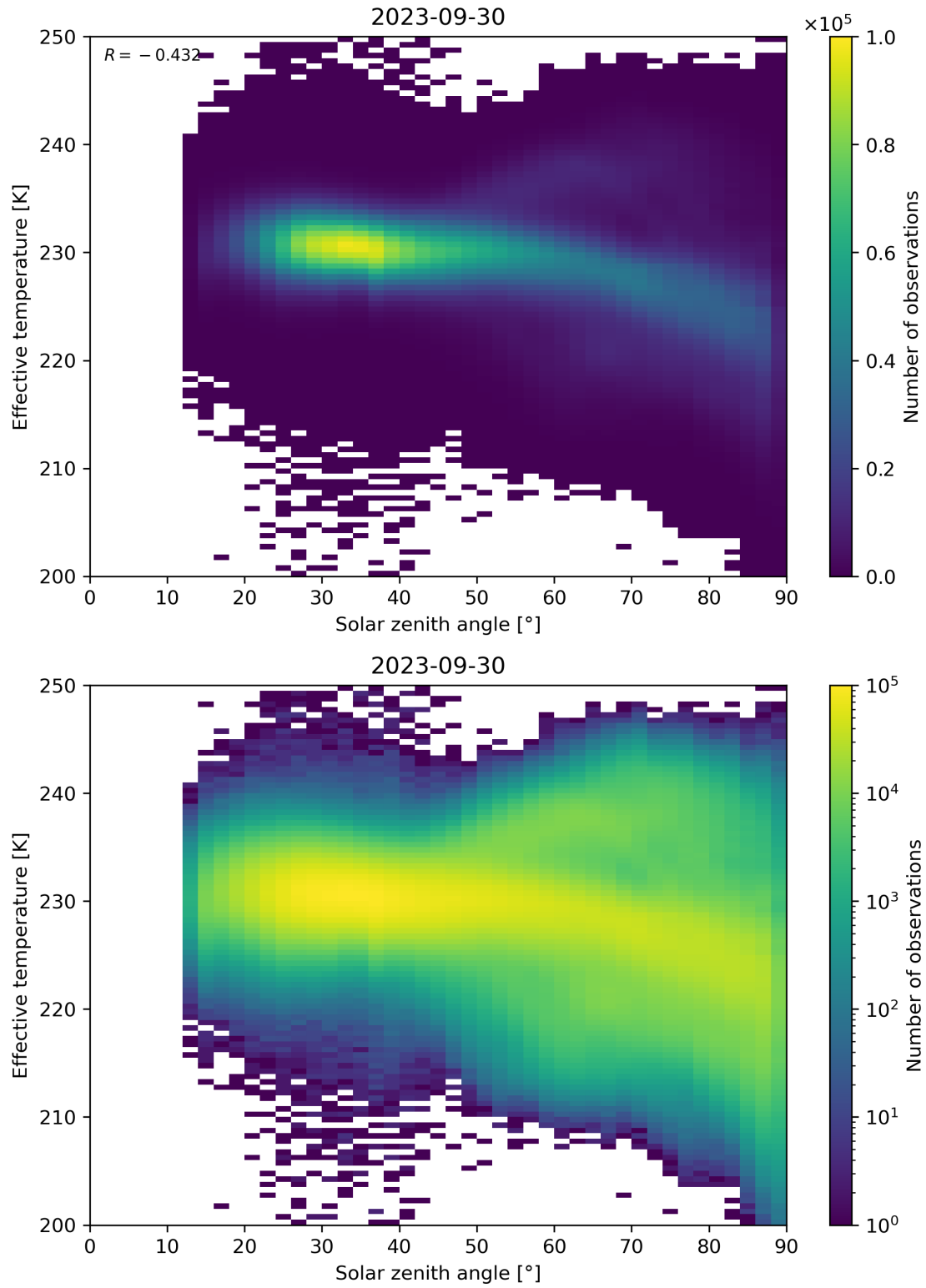
Figure 45: Scatter density plot of “Solar zenith angle” against “Effective temperature” for 2023-09-29 to 2023-10-01.
