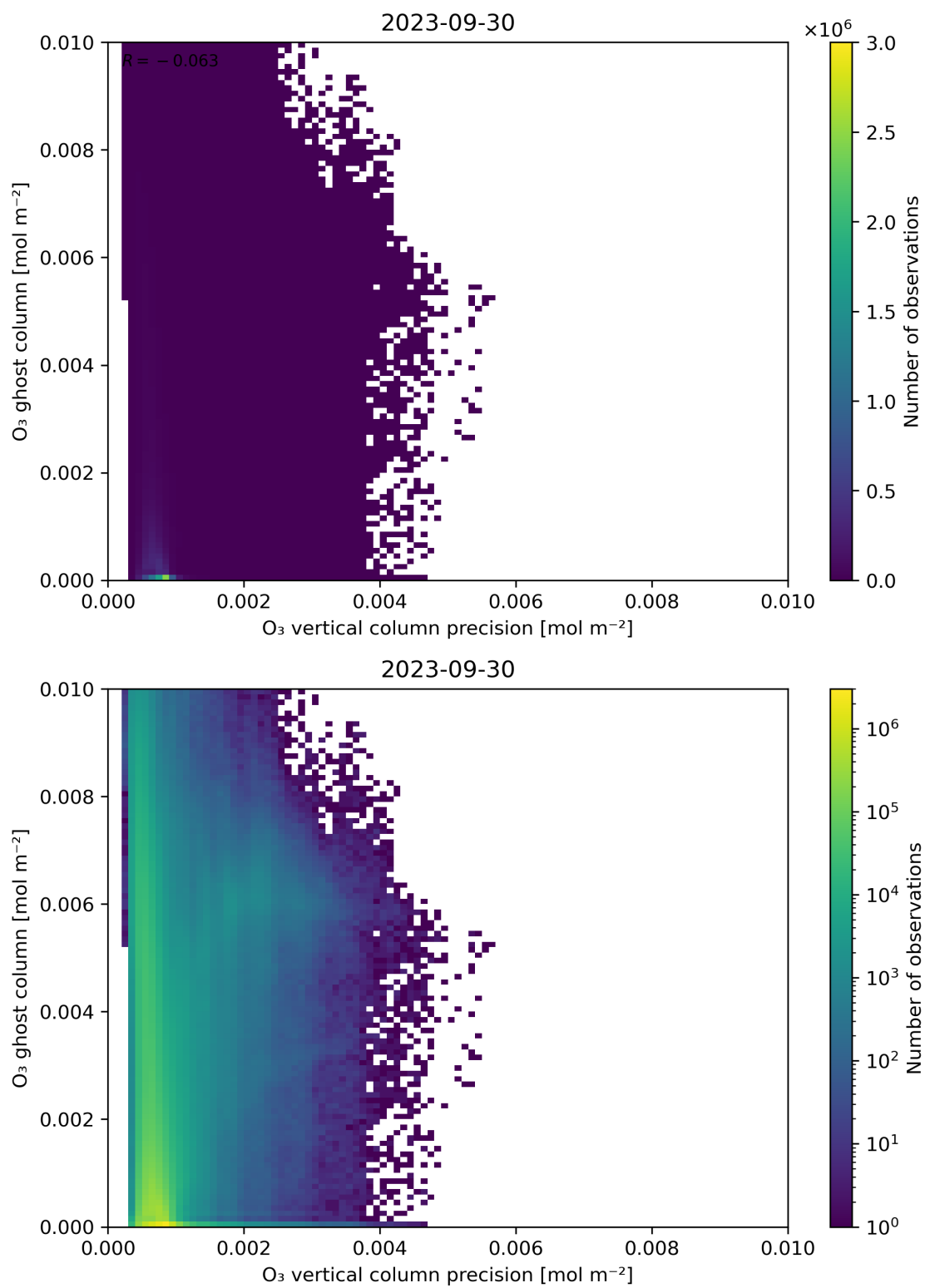
Figure 43: Scatter density plot of “ \text{O}_3 vertical column precision” against “ \text{O}_3 ghost column” for 2023-09-29 to 2023-10-01.
