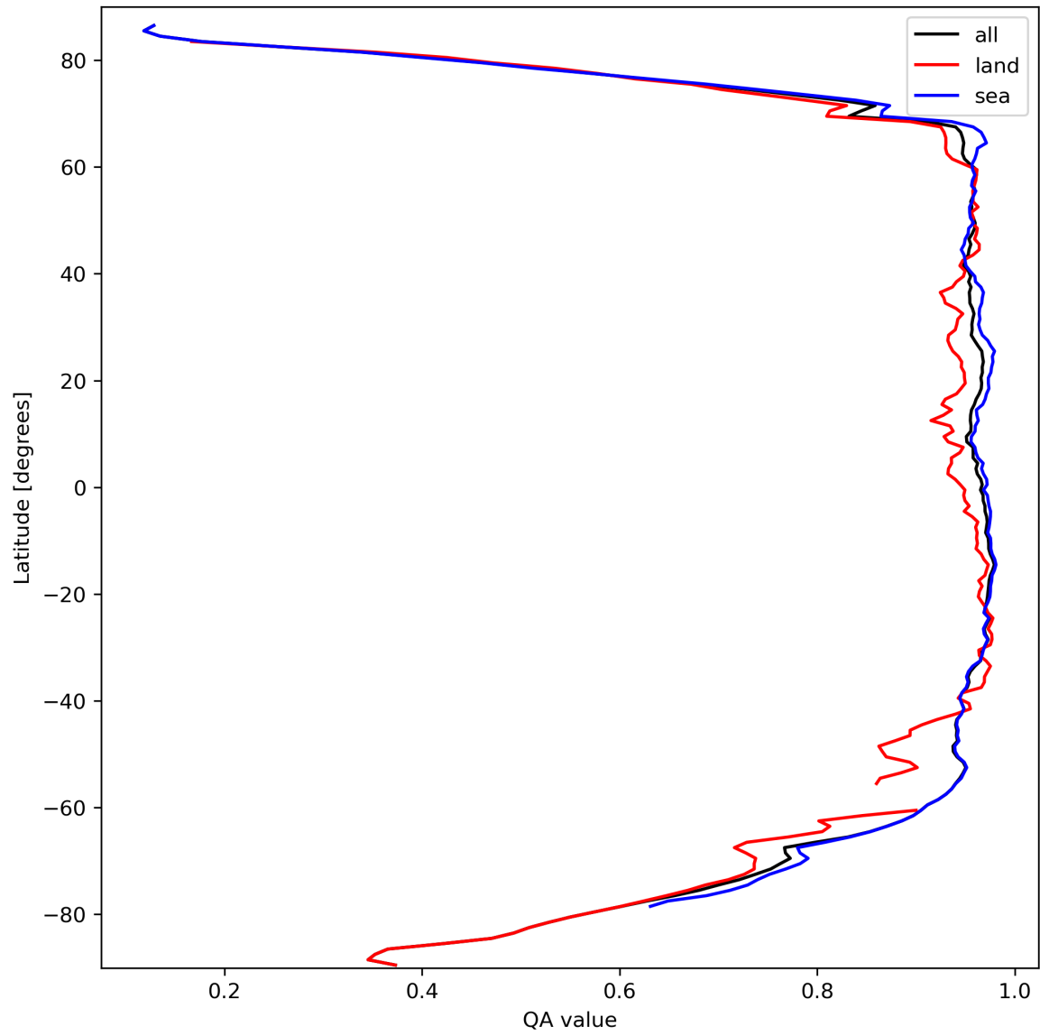
Figure 13: Zonal average of “QA value” for 2023-09-29 to 2023-10-01.
