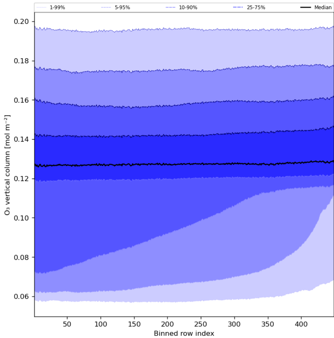
Figure 28: Along track statistics of “O 3 vertical column” for 2023-09-29 to 2023-10-01
