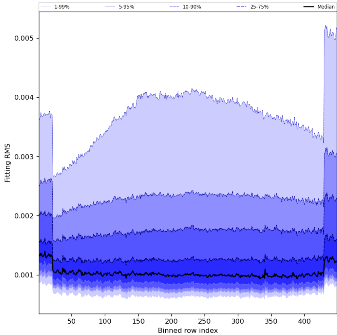
Figure 30: Along track statistics of “Fitting RMS” for 2023-09-29 to 2023-10-01
