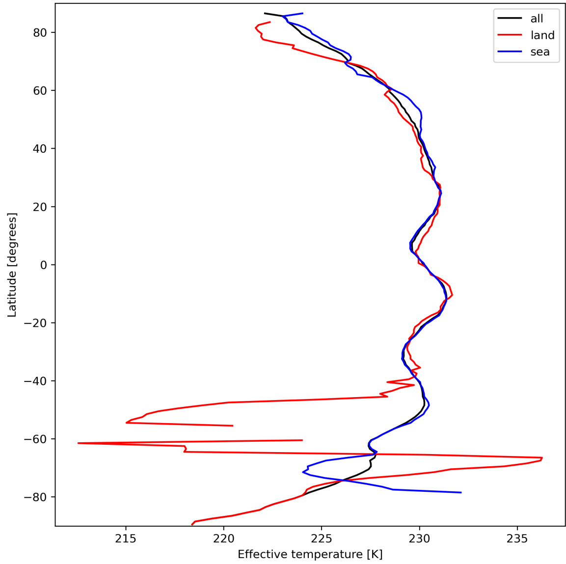
Figure 17: Zonal average of “Effective temperature” for 2023-09-29 to 2023-10-01.
