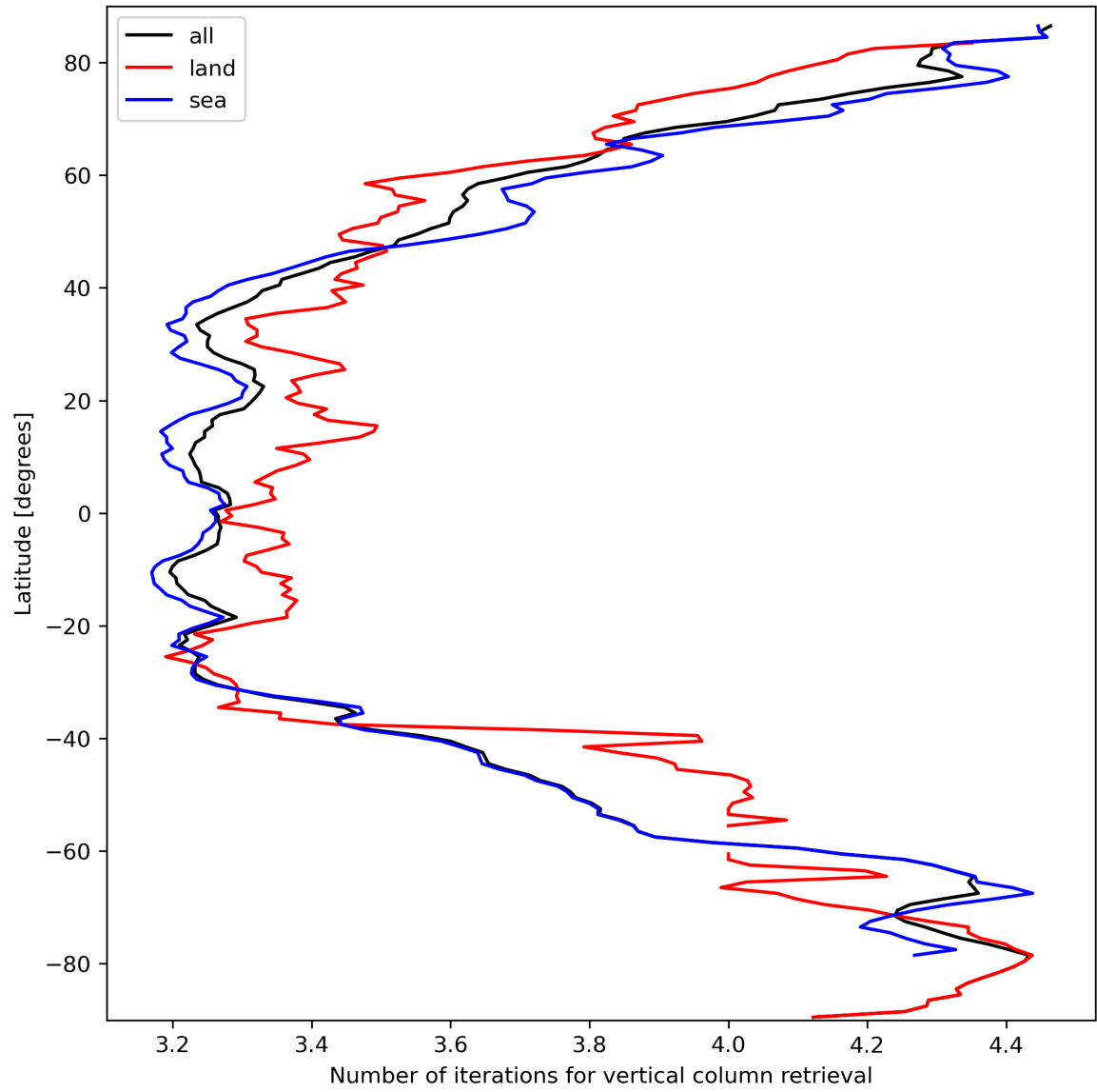
Figure 19: Zonal average of “Number of iterations for vertical column retrieval” for 2023-09-29 to 2023-10-01.
