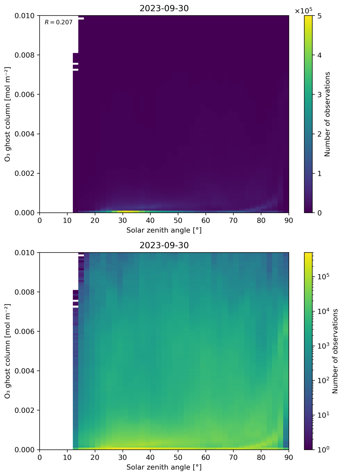
Figure 46: Scatter density plot of “Solar zenith angle” against “O 3 ghost column” for 2023-09-29 to 2023-10-01.
