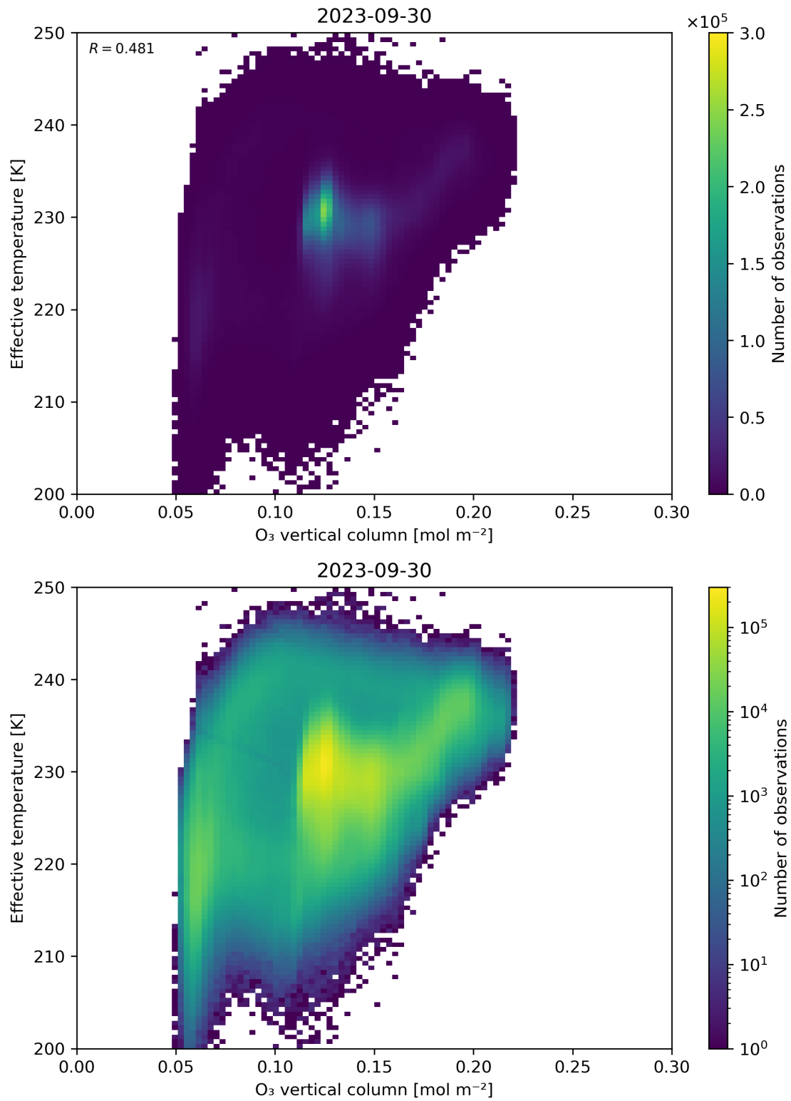
Figure 39: Scatter density plot of “O 3 vertical column” against “Effective temperature” for 2023-09-29 to 2023-10-01.
