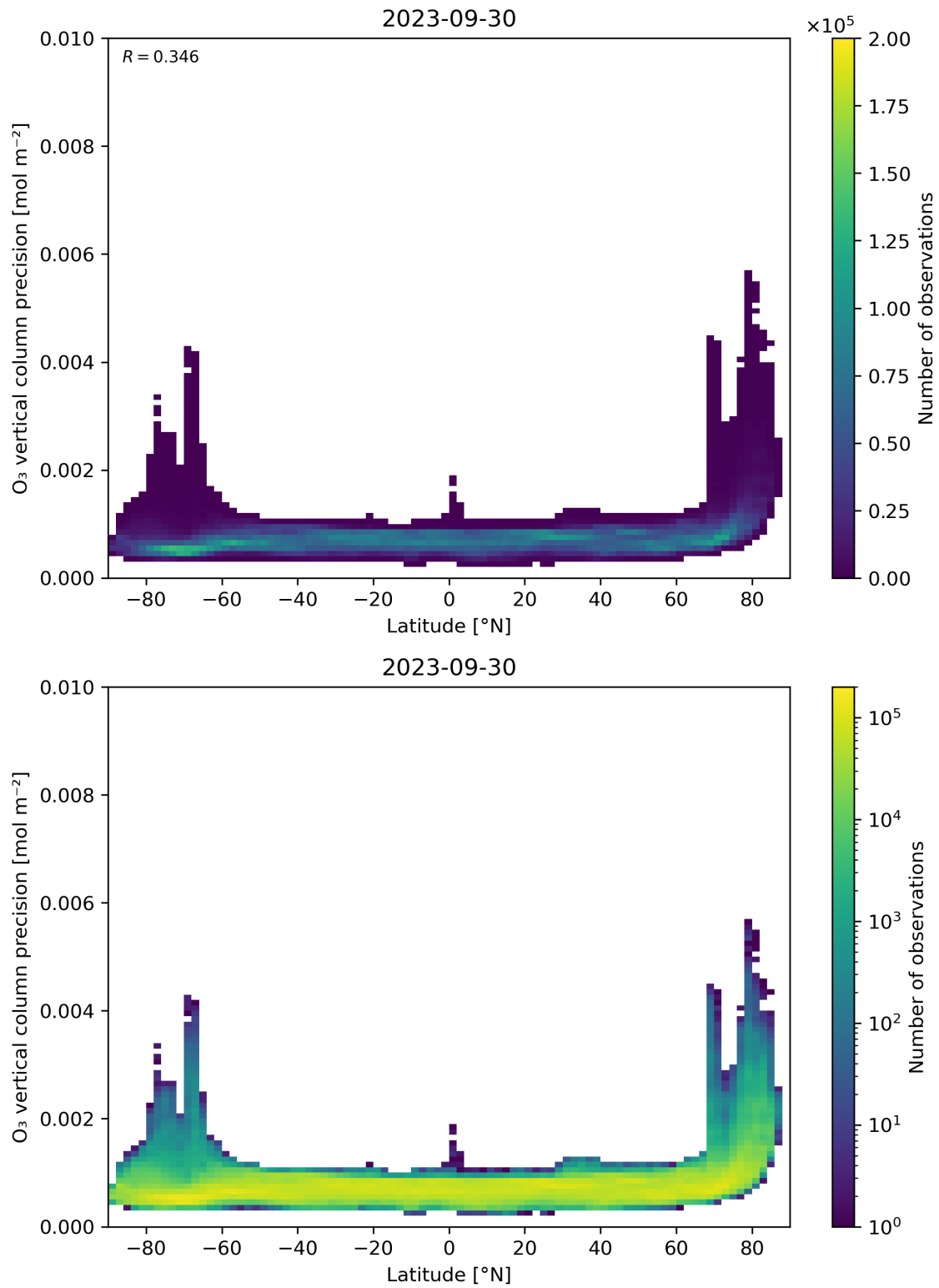
Figure 37: Scatter density plot of “Latitude” against “O 3 vertical column precision” for 2023-09-29 to 2023-10-01.
