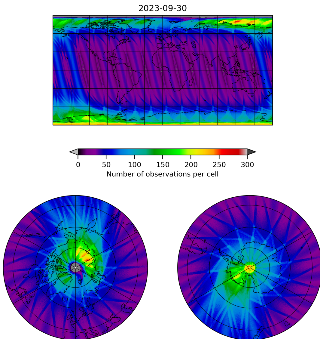
Figure 12: Map of the number of observations for 2023-09-29 to 2023-10-01
