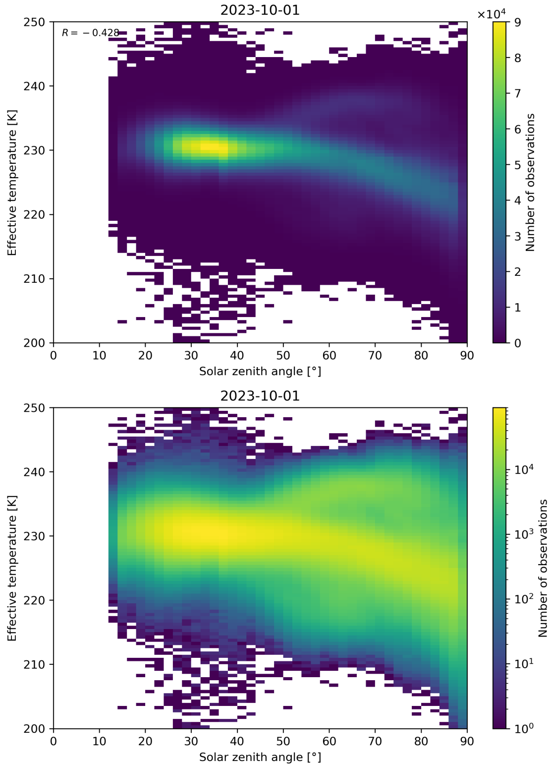
Figure 45: Scatter density plot of “Solar zenith angle” against “Effective temperature” for 2023-10-01 to 2023-10-02.
