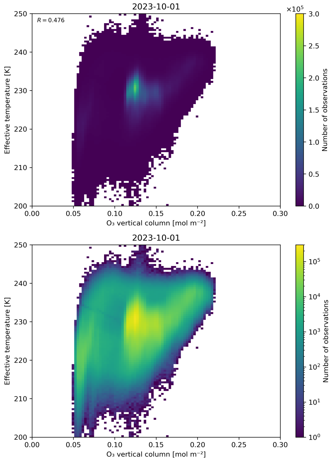
Figure 39: Scatter density plot of “O 3 vertical column” against “Effective temperature” for 2023-10-01 to 2023-10-02.
