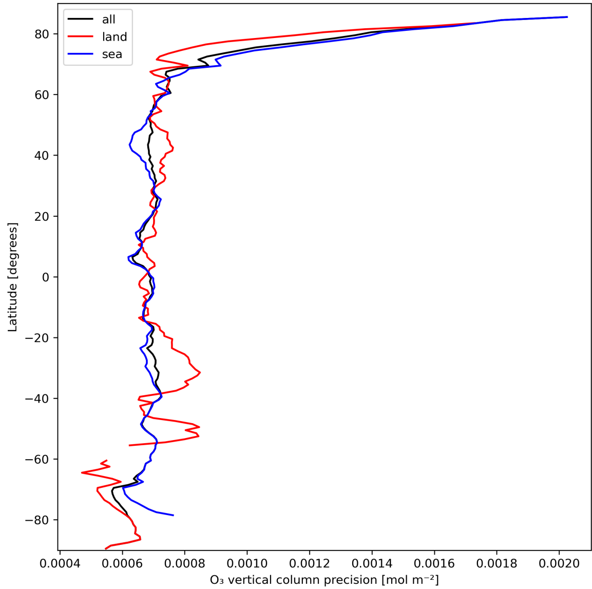
Figure 15: Zonal average of “O 3 vertical column precision” for 2023-10-01 to 2023-10-02.
