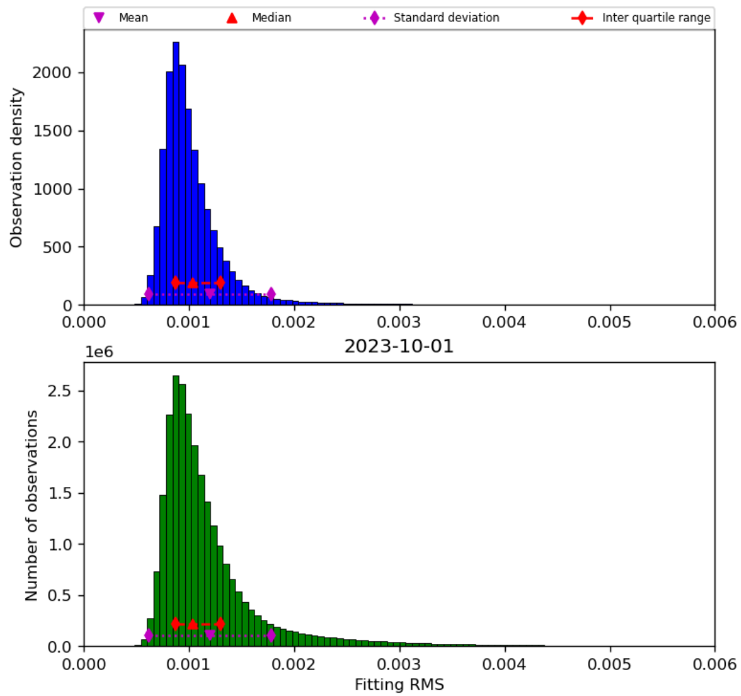
Figure 23: Histogram of “Fitting RMS” for 2023-10-01 to 2023-10-02
