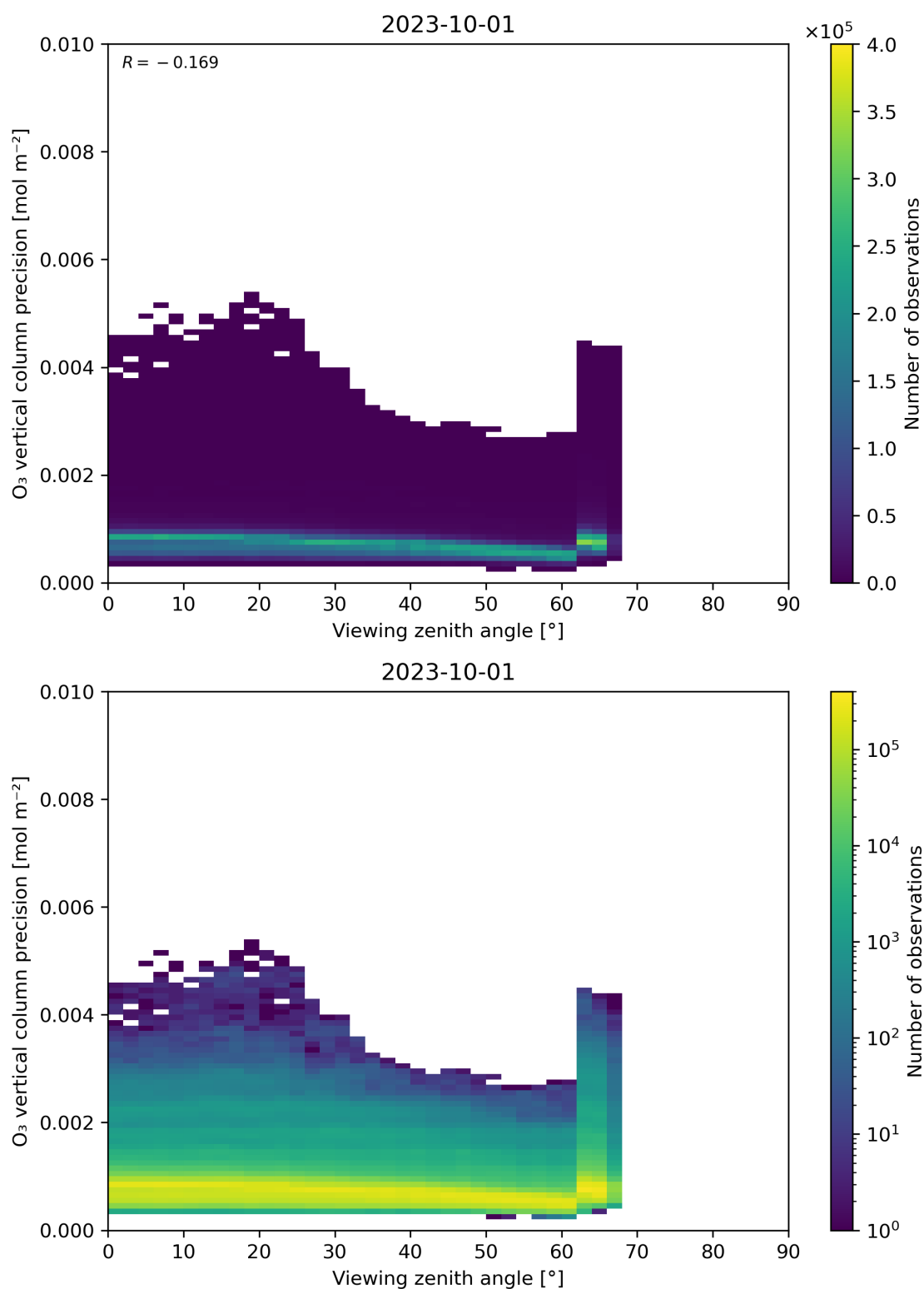
Figure 53: Scatter density plot of “Viewing zenith angle” against “O 3 vertical column precision” for 2023-10-01 to 2023-10-02.
