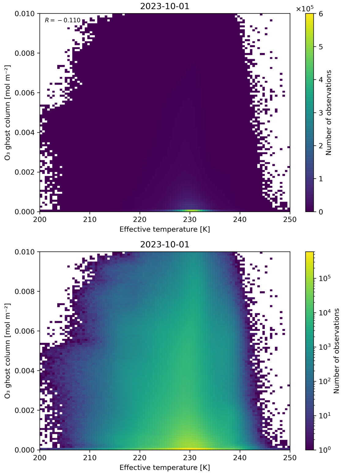
Figure 38: Scatter density plot of “Effective temperature” against “O 3 ghost column” for 2023-10-01 to 2023-10-02.
