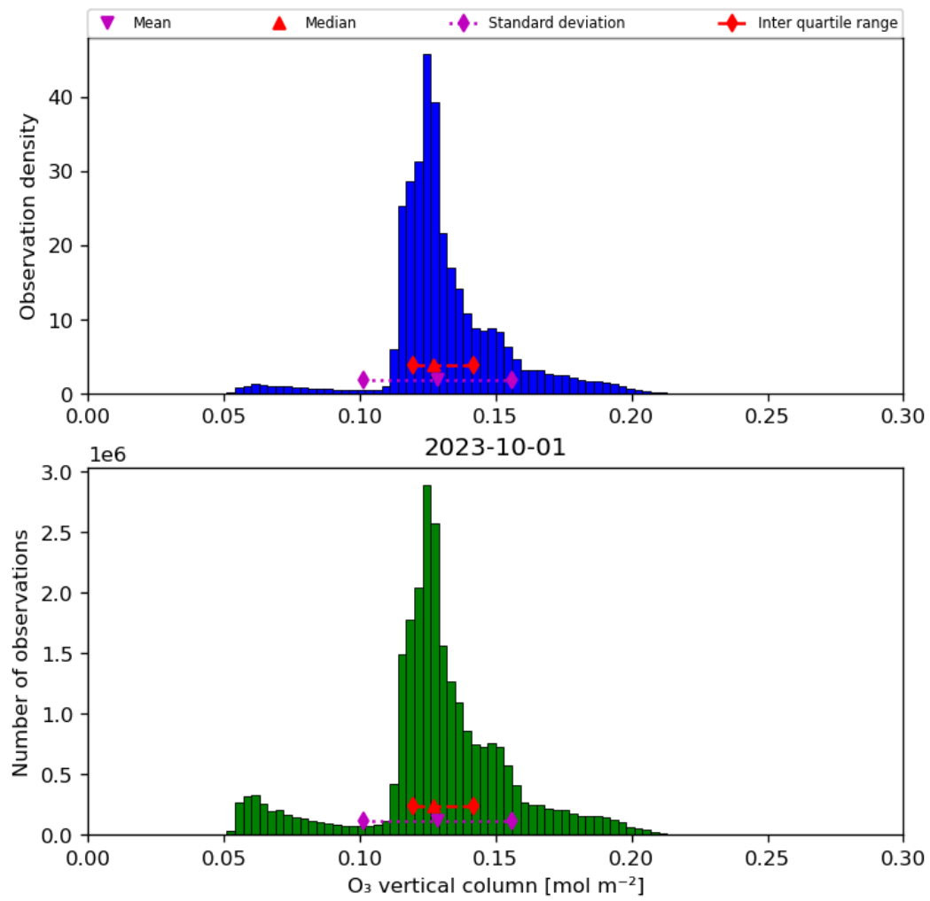
Figure 21: Histogram of “O 3 vertical column” for 2023-10-01 to 2023-10-02
