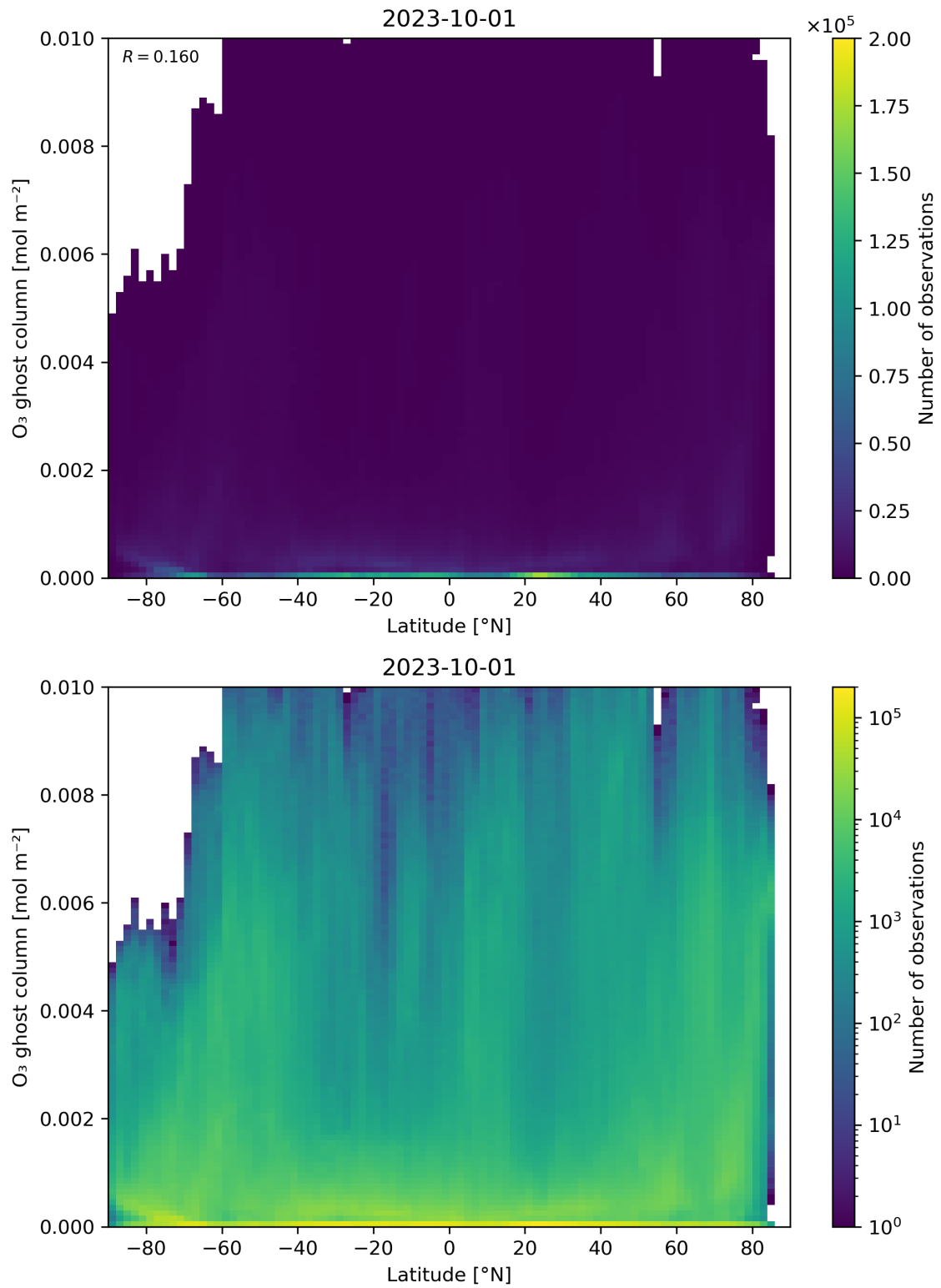
Figure 35: Scatter density plot of “Latitude” against “O 3 ghost column” for 2023-10-01 to 2023-10-02.
