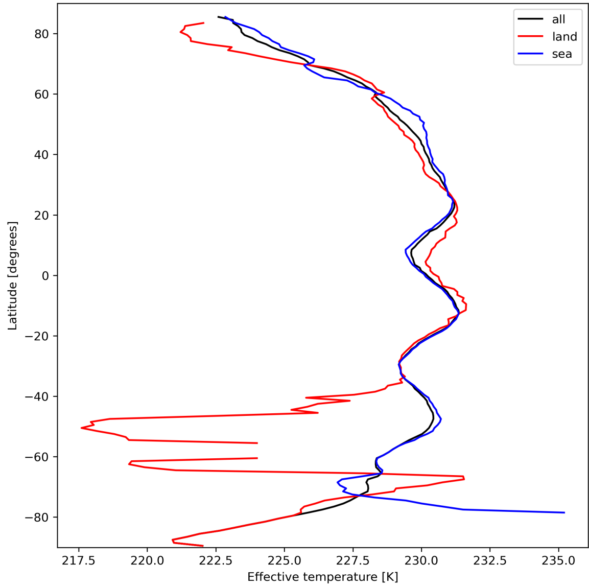
Figure 17: Zonal average of “Effective temperature” for 2023-10-01 to 2023-10-02.
