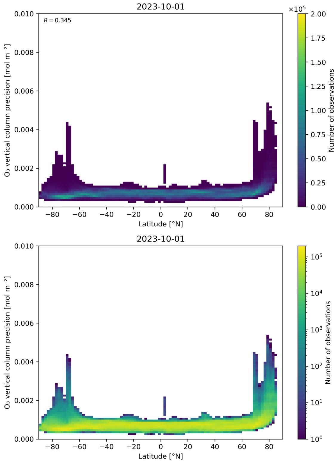
Figure 37: Scatter density plot of “Latitude” against “O 3 vertical column precision” for 2023-10-01 to 2023-10-02.
