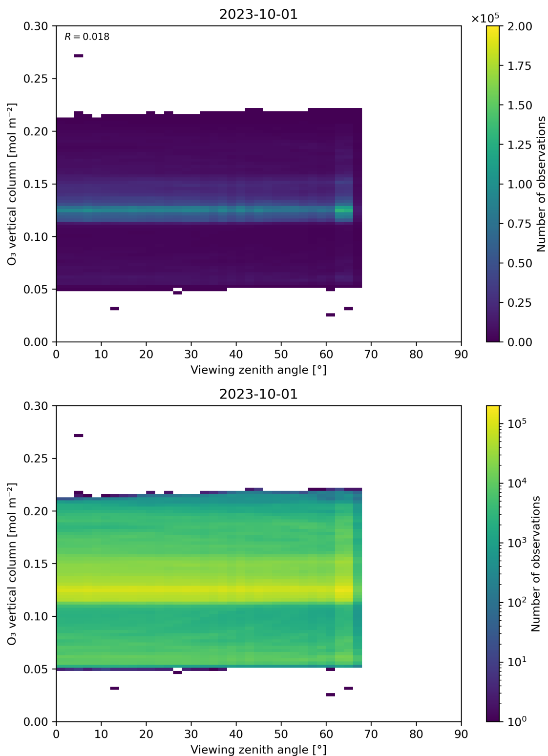
Figure 52: Scatter density plot of “Viewing zenith angle” against “O 3 vertical column” for 2023-10-01 to 2023-10-02.
