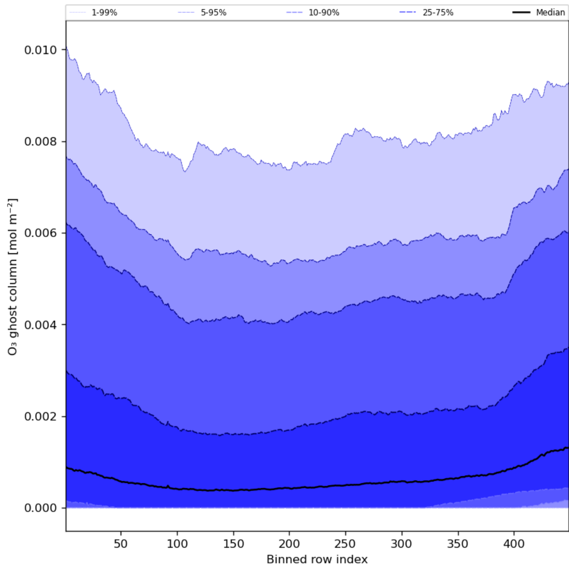
Figure 32: Along track statistics of “O 3 ghost column” for 2023-10-01 to 2023-10-02
