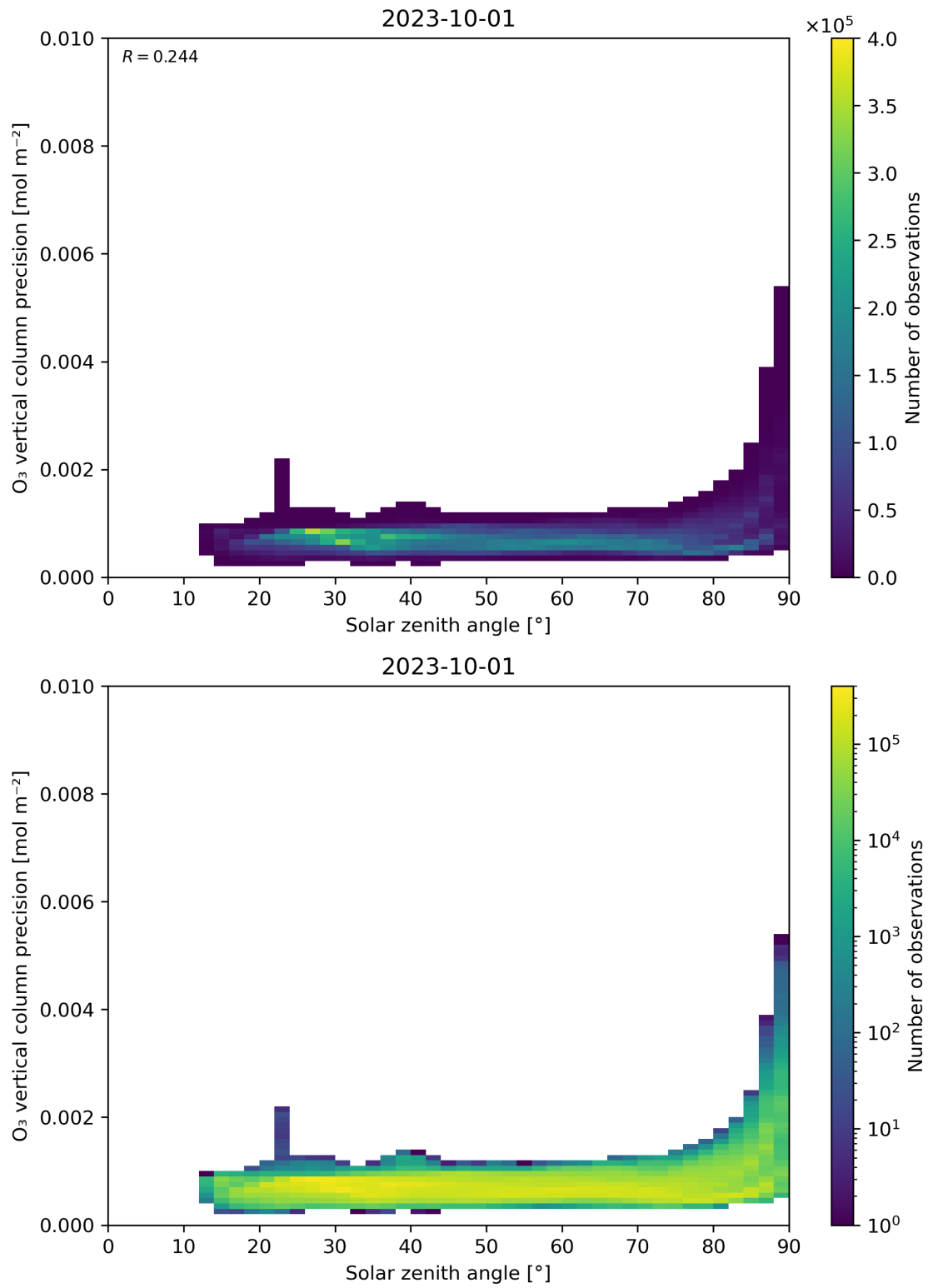
Figure 48: Scatter density plot of “Solar zenith angle” against “O 3 vertical column precision” for 2023-10-01 to 2023-10-02.
