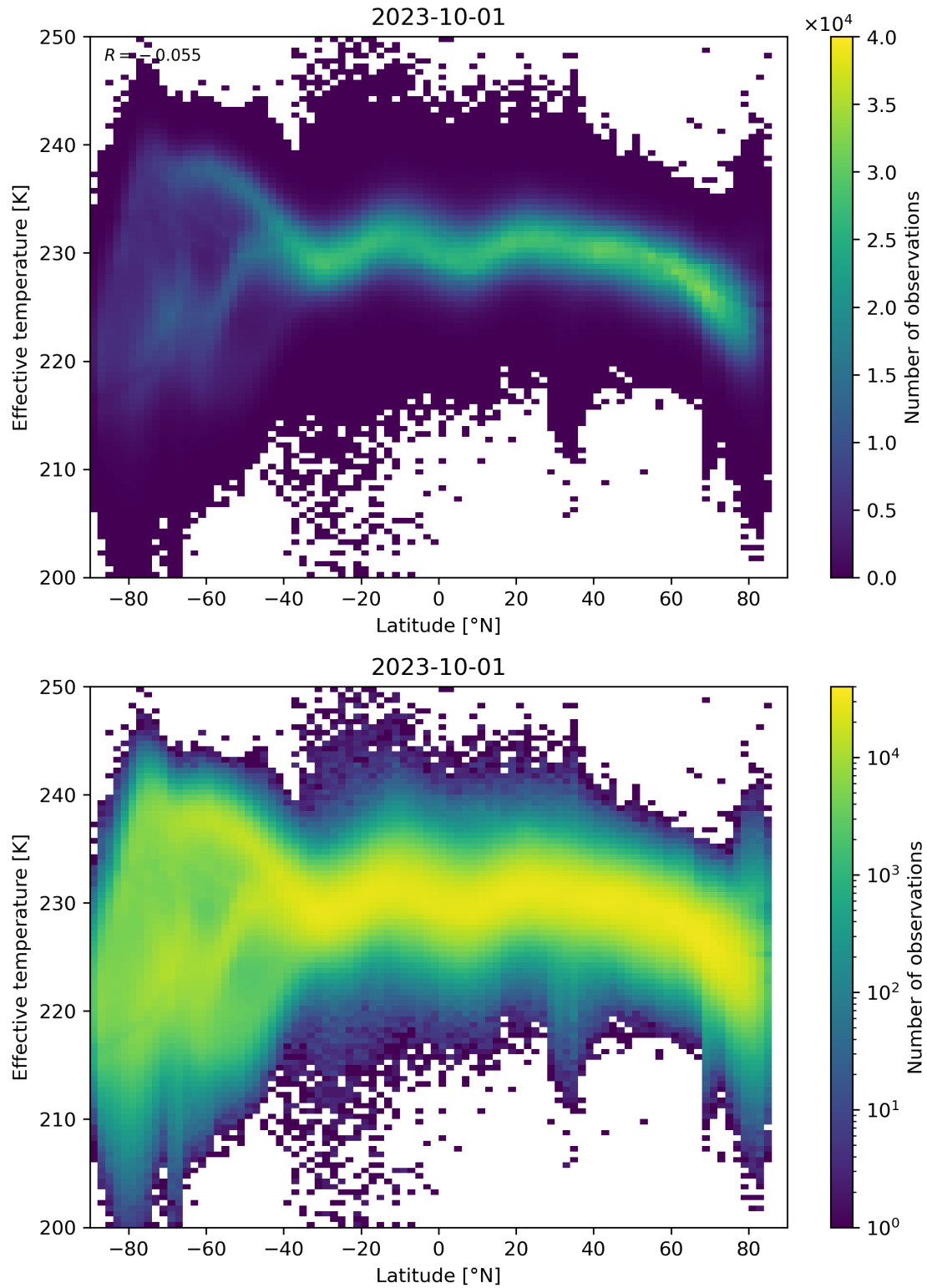
Figure 34: Scatter density plot of “Latitude” against “Effective temperature” for 2023-10-01 to 2023-10-02.
