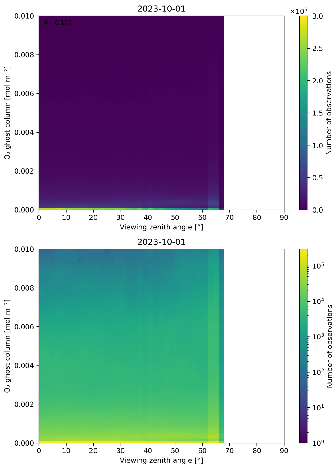
Figure 51: Scatter density plot of “Viewing zenith angle” against “O 3 ghost column” for 2023-10-01 to 2023-10-02.
