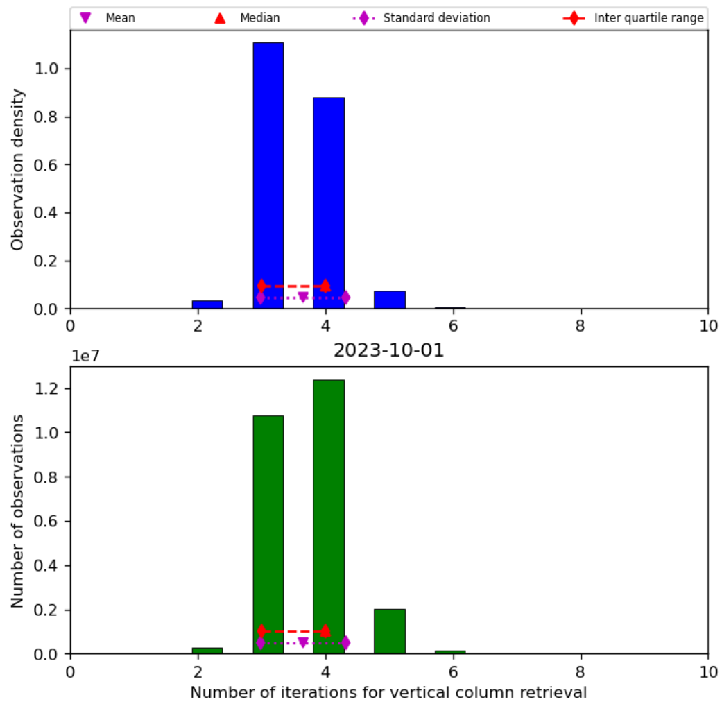
Figure 26: Histogram of “Number of iterations for vertical column retrieval” for 2023-10-01 to 2023-10-02
