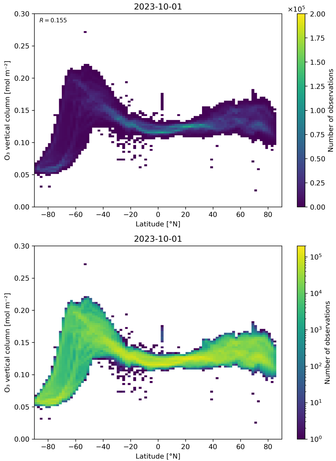
Figure 36: Scatter density plot of “Latitude” against “O 3 vertical column” for 2023-10-01 to 2023-10-02.
