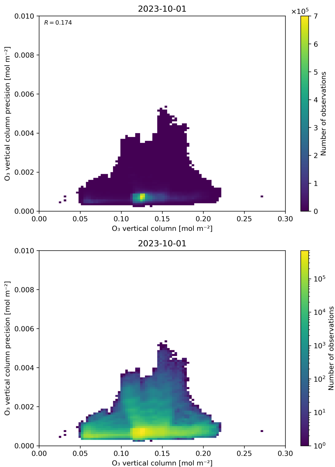
Figure 41: Scatter density plot of “O 3 vertical column” against “O 3 vertical column precision” for 2023-10-01 to 2023-10-02.
