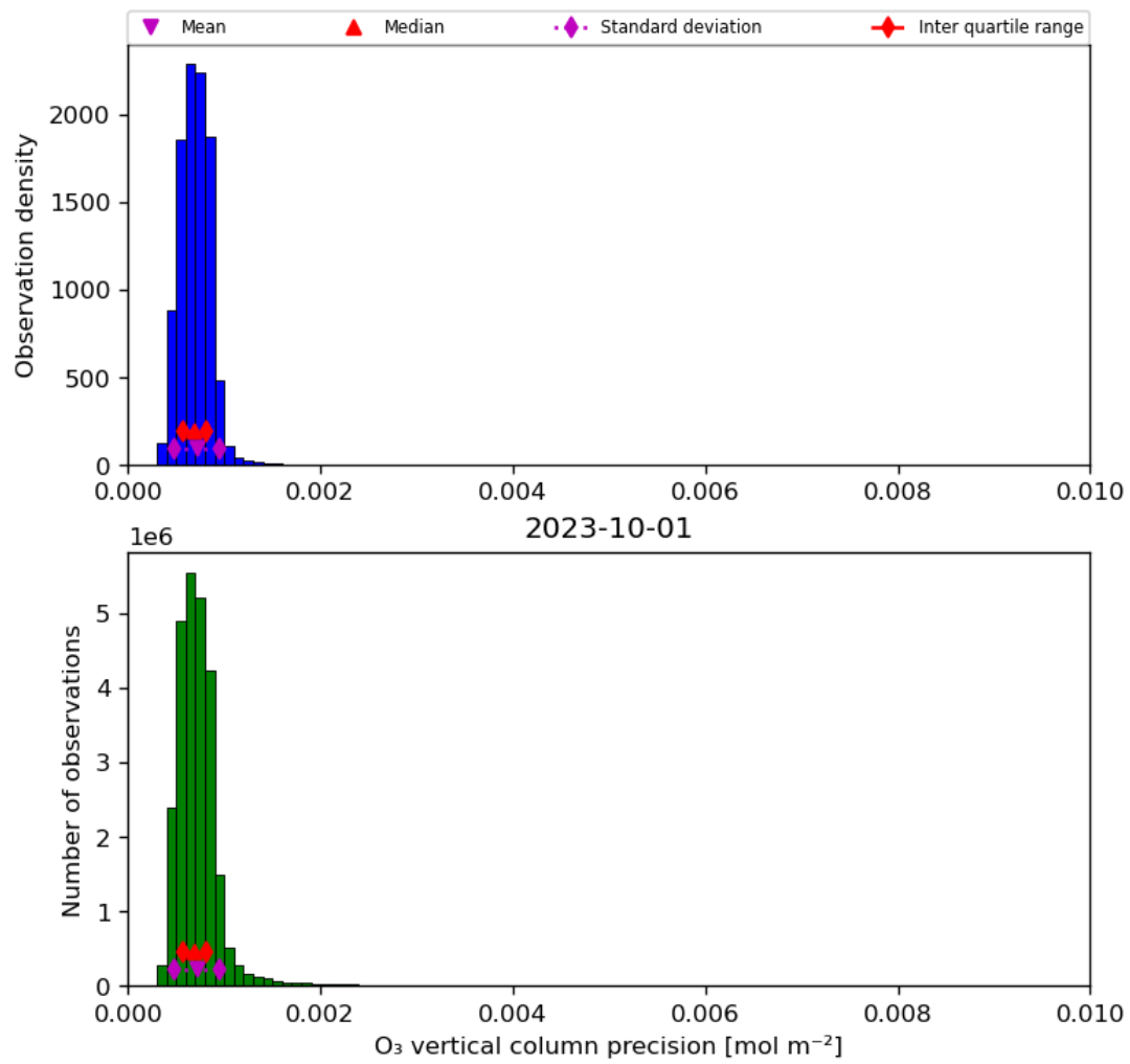
Figure 22: Histogram of “O 3 vertical column precision” for 2023-10-01 to 2023-10-02
