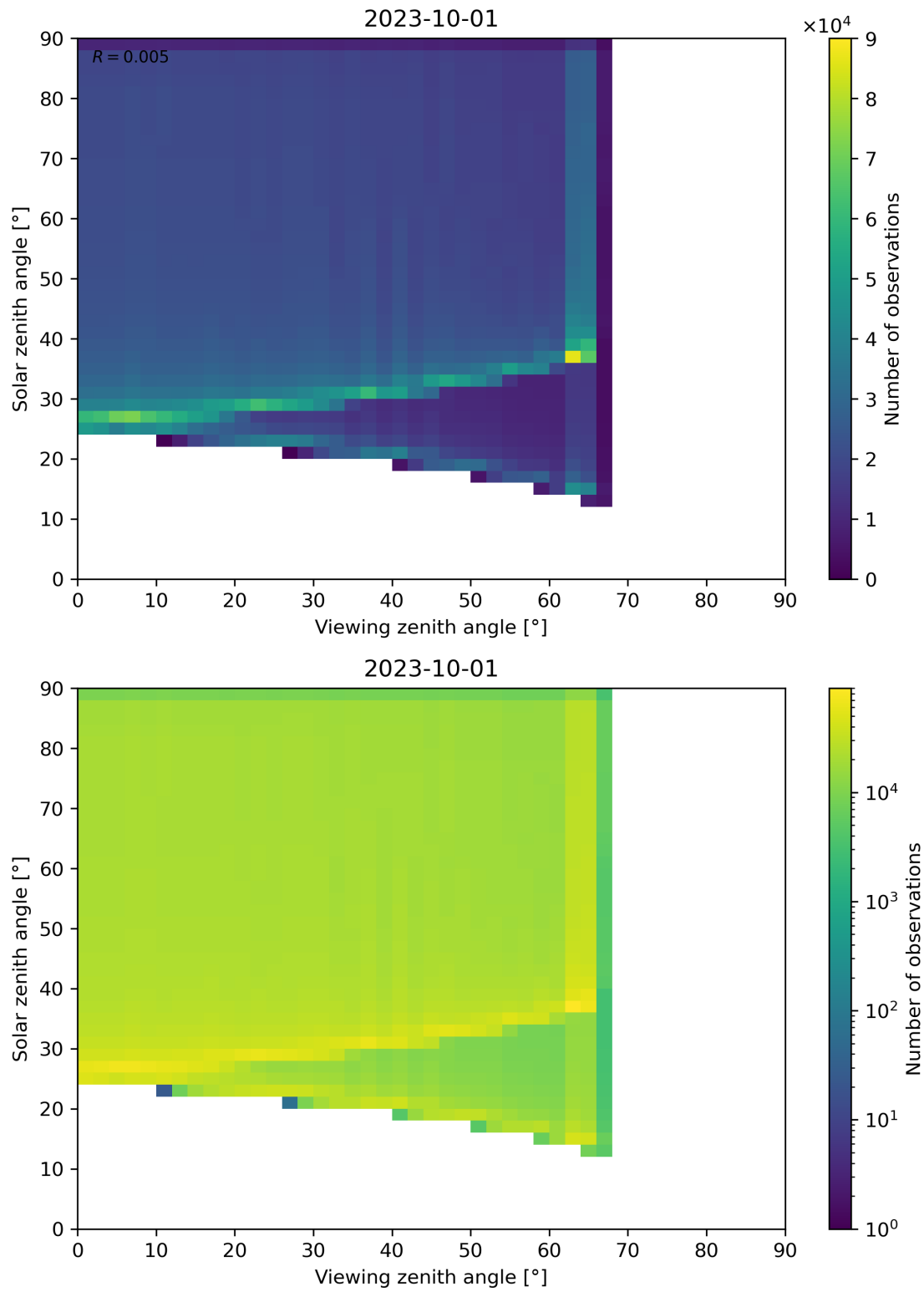
Figure 54: Scatter density plot of “Viewing zenith angle” against “Solar zenith angle” for 2023-10-01 to 2023-10-02.
