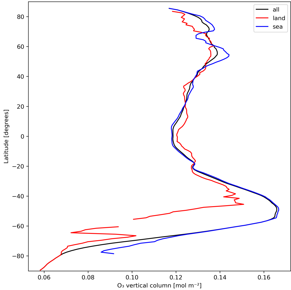
Figure 14: Zonal average of “O 3 vertical column” for 2023-10-01 to 2023-10-02.
