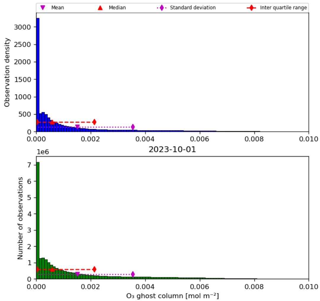
Figure 25: Histogram of “O 3 ghost column” for 2023-10-01 to 2023-10-02
