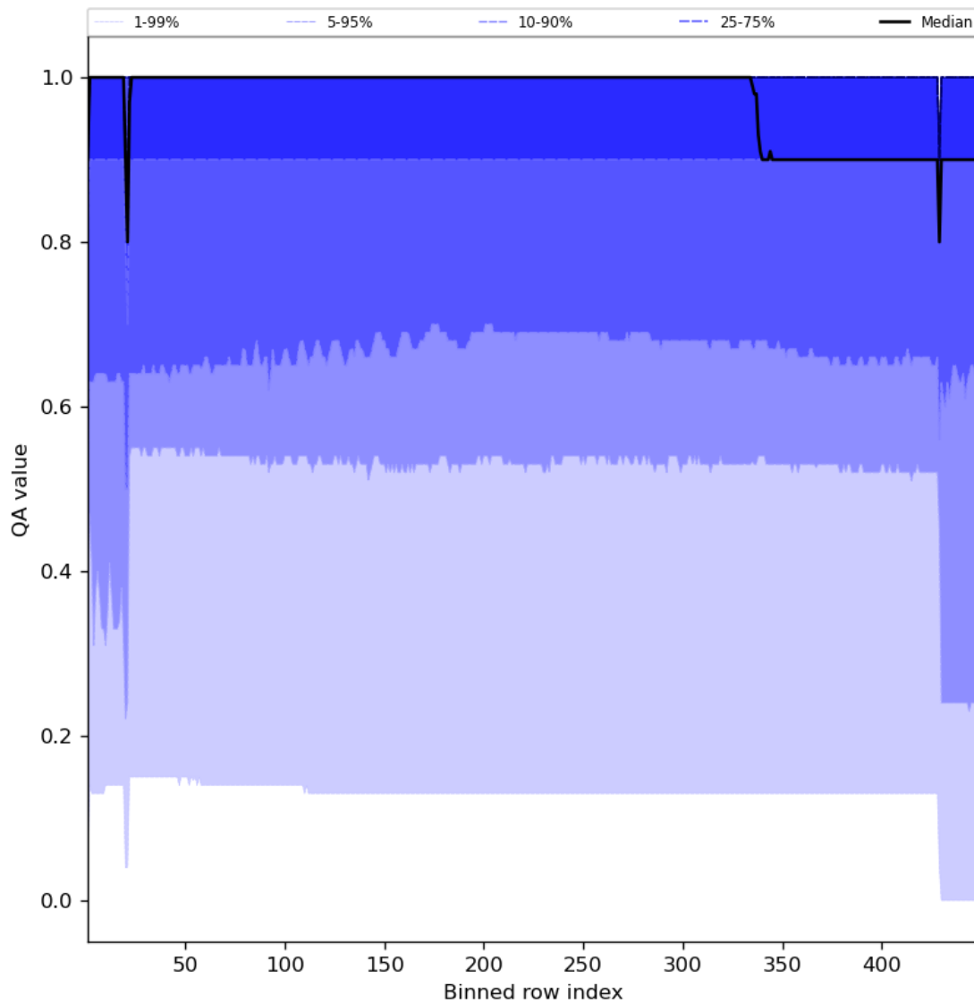
Figure 27: Along track statistics of “QA value” for 2023-10-01 to 2023-10-02
