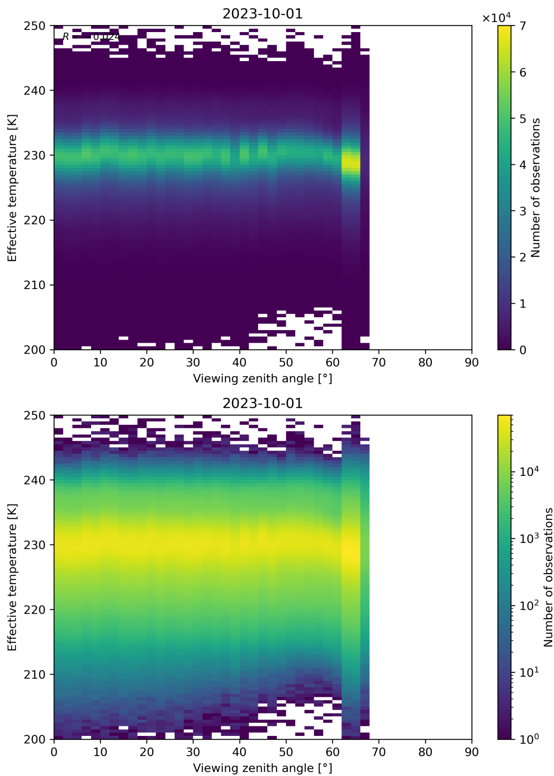
Figure 50: Scatter density plot of “Viewing zenith angle” against “Effective temperature” for 2023-10-01 to 2023-10-02.
