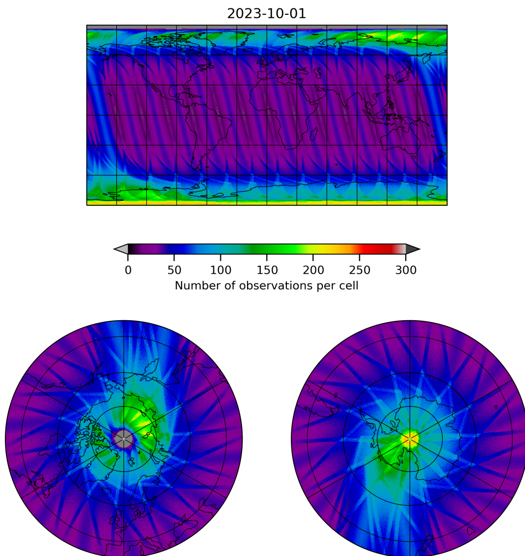
Figure 12: Map of the number of observations for 2023-10-01 to 2023-10-02
