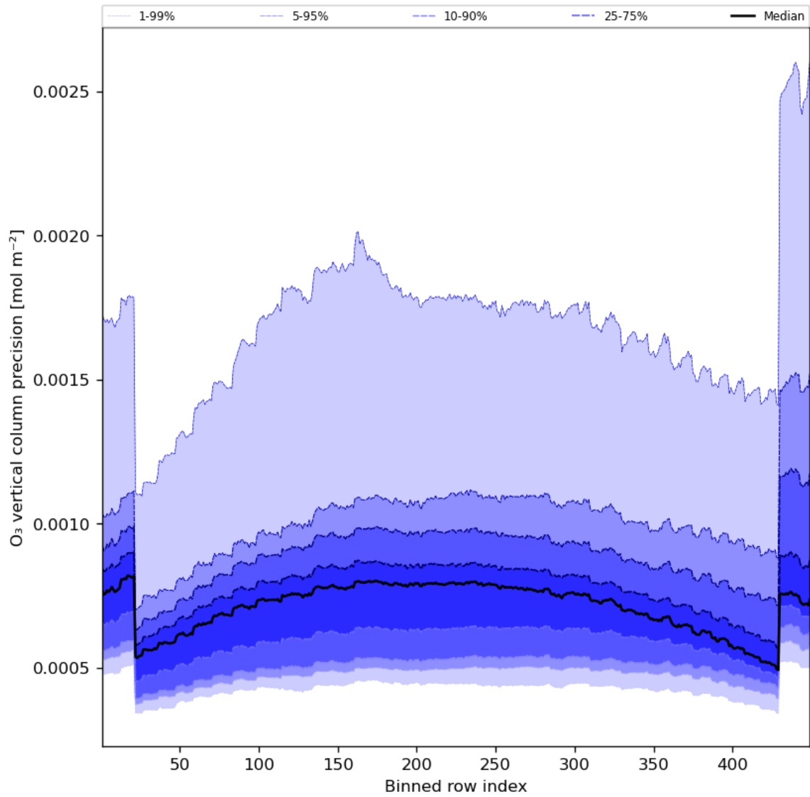
Figure 29: Along track statistics of “O 3 vertical column precision” for 2023-10-01 to 2023-10-02
