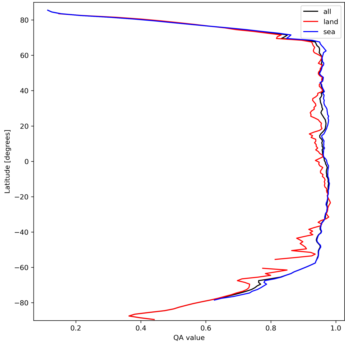
Figure 13: Zonal average of “QA value” for 2023-10-01 to 2023-10-02.
