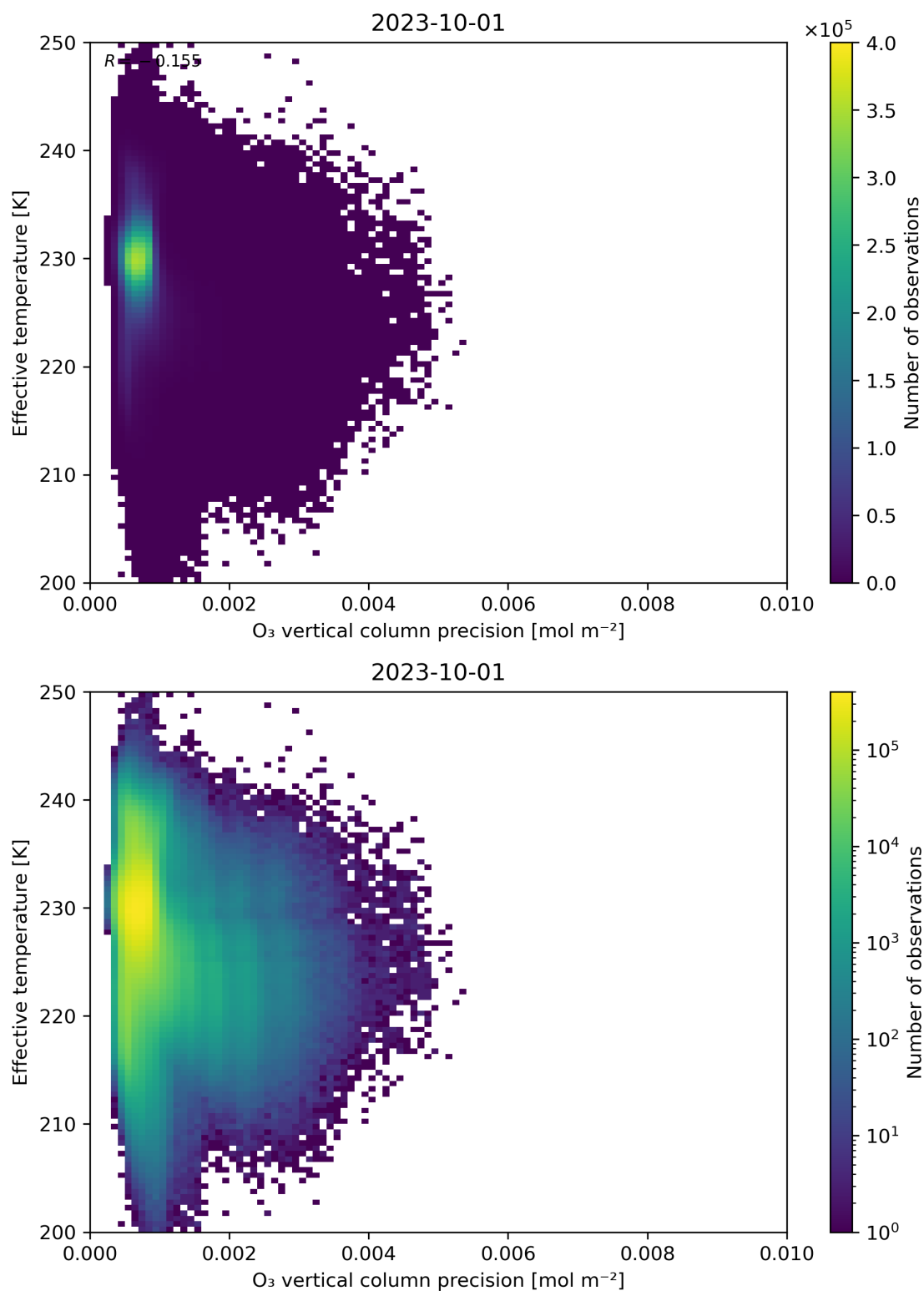
Figure 42: Scatter density plot of “O 3 vertical column precision” against “Effective temperature” for 2023-10-01 to 2023-10-02.
