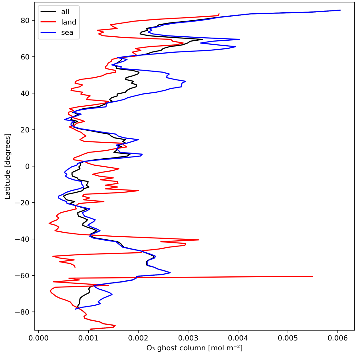
Figure 18: Zonal average of "O 3 ghost column" for 2023-10-01 to 2023-10-02.
