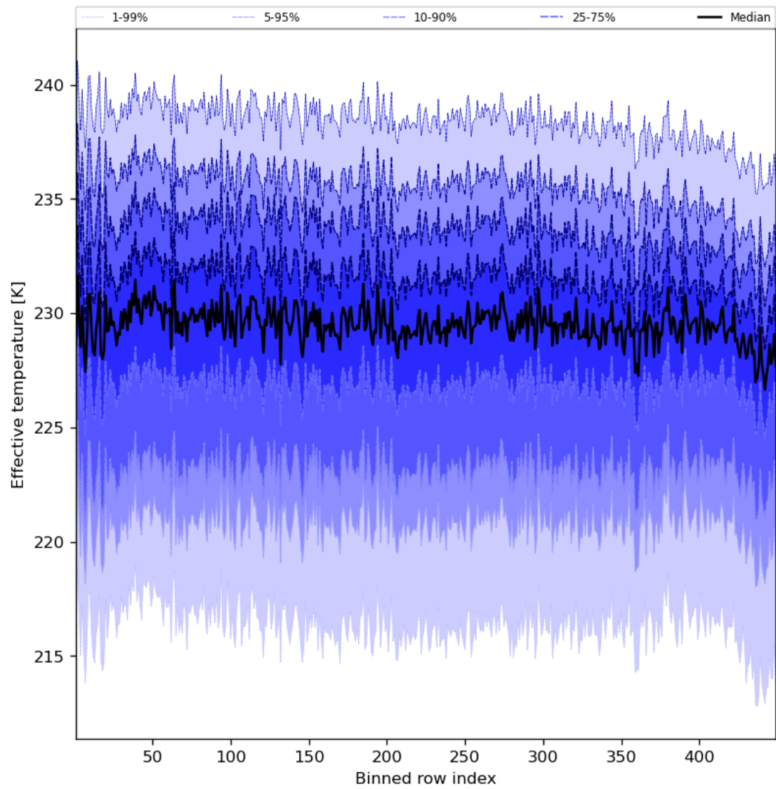
Figure 31: Along track statistics of “Effective temperature” for 2023-10-01 to 2023-10-02
