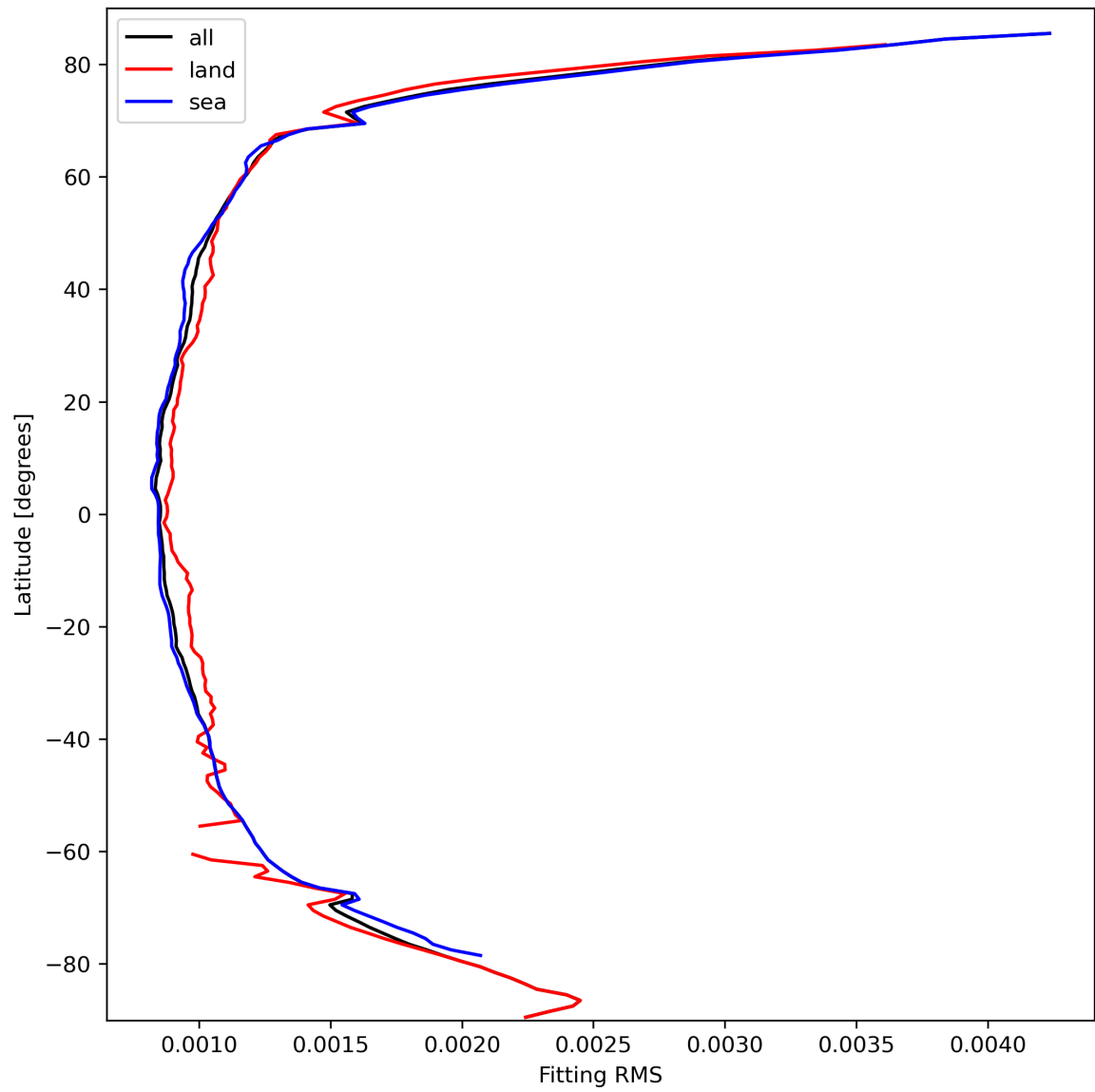
Figure 16: Zonal average of “Fitting RMS” for 2023-10-01 to 2023-10-02.
