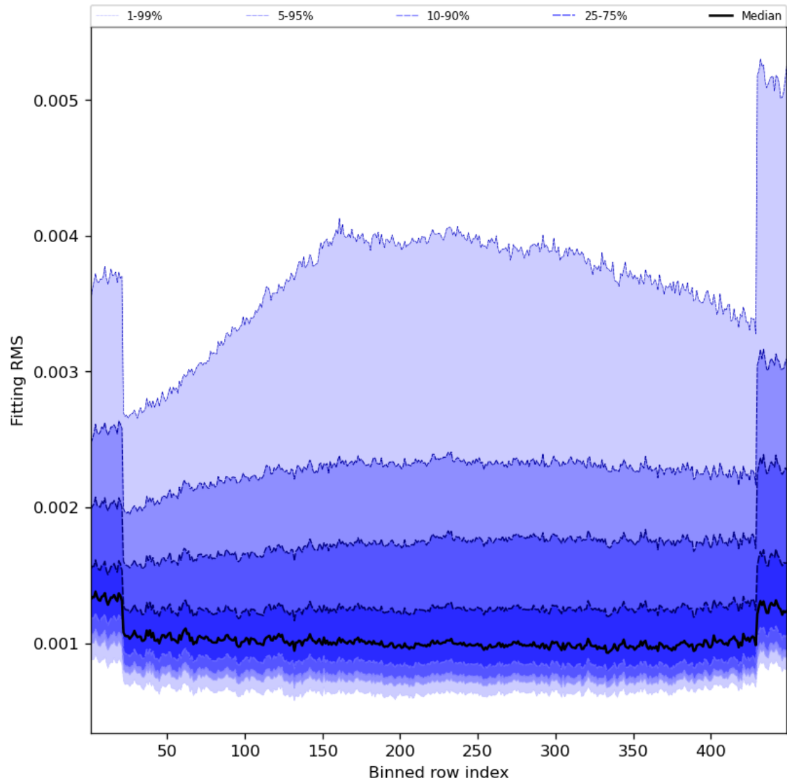
Figure 30: Along track statistics of “Fitting RMS” for 2023-10-01 to 2023-10-02
