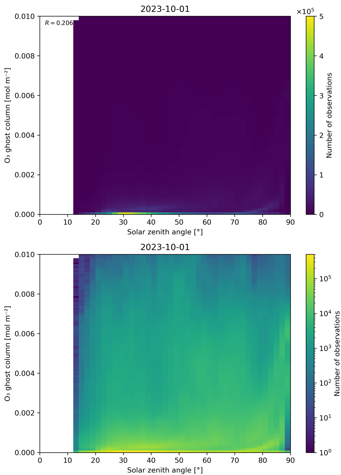
Figure 46: Scatter density plot of “Solar zenith angle” against “O 3 ghost column” for 2023-10-01 to 2023-10-02.
