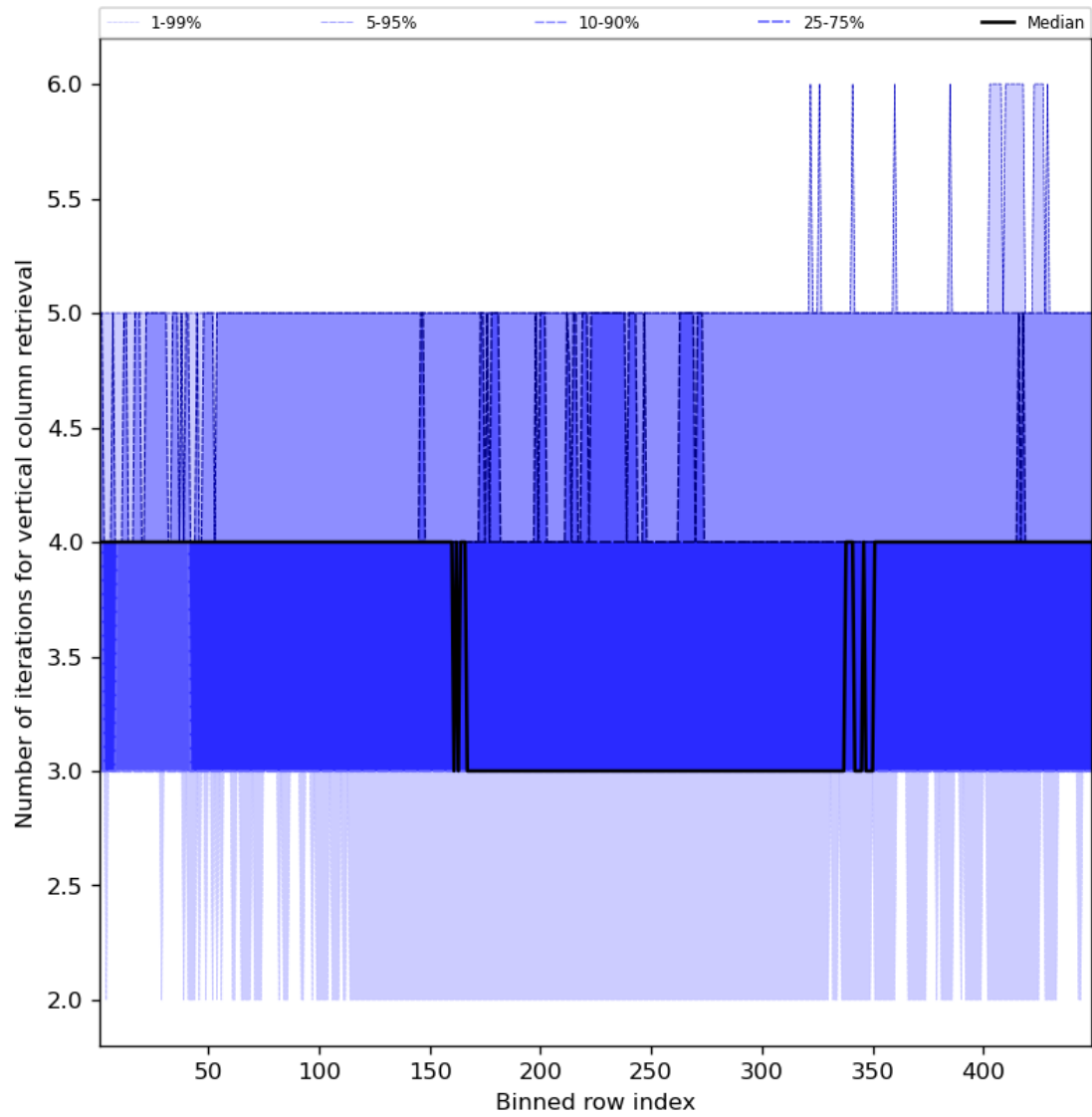
Figure 33: Along track statistics of “Number of iterations for vertical column retrieval” for 2023-10-01 to 2023-10-02
