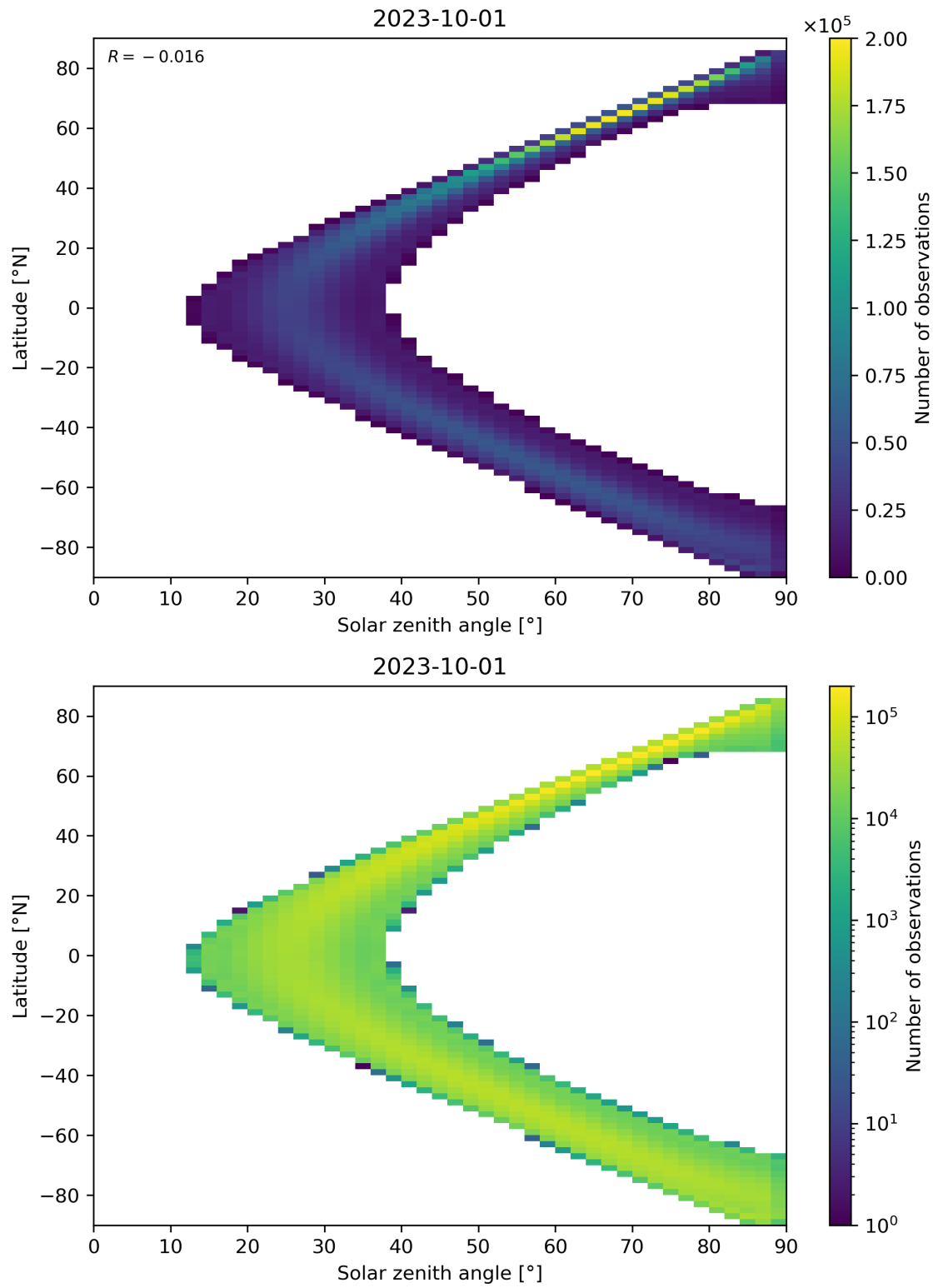
Figure 44: Scatter density plot of “Solar zenith angle” against “Latitude” for 2023-10-01 to 2023-10-02.
