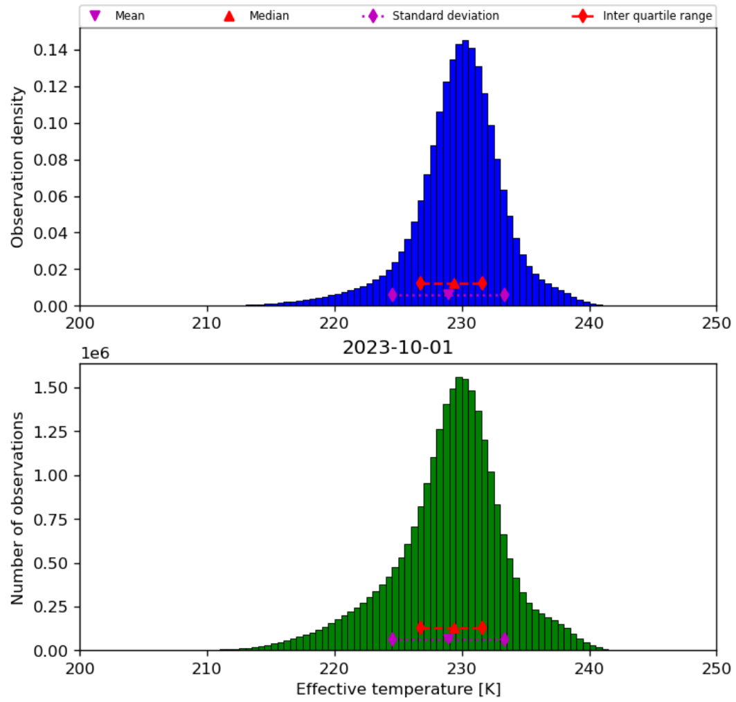
Figure 24: Histogram of “Effective temperature” for 2023-10-01 to 2023-10-02
