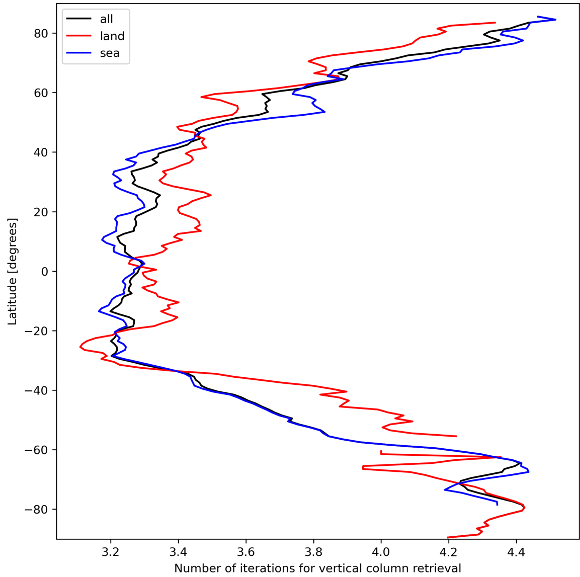
Figure 19: Zonal average of “Number of iterations for vertical column retrieval” for 2023-10-01 to 2023-10-02.
