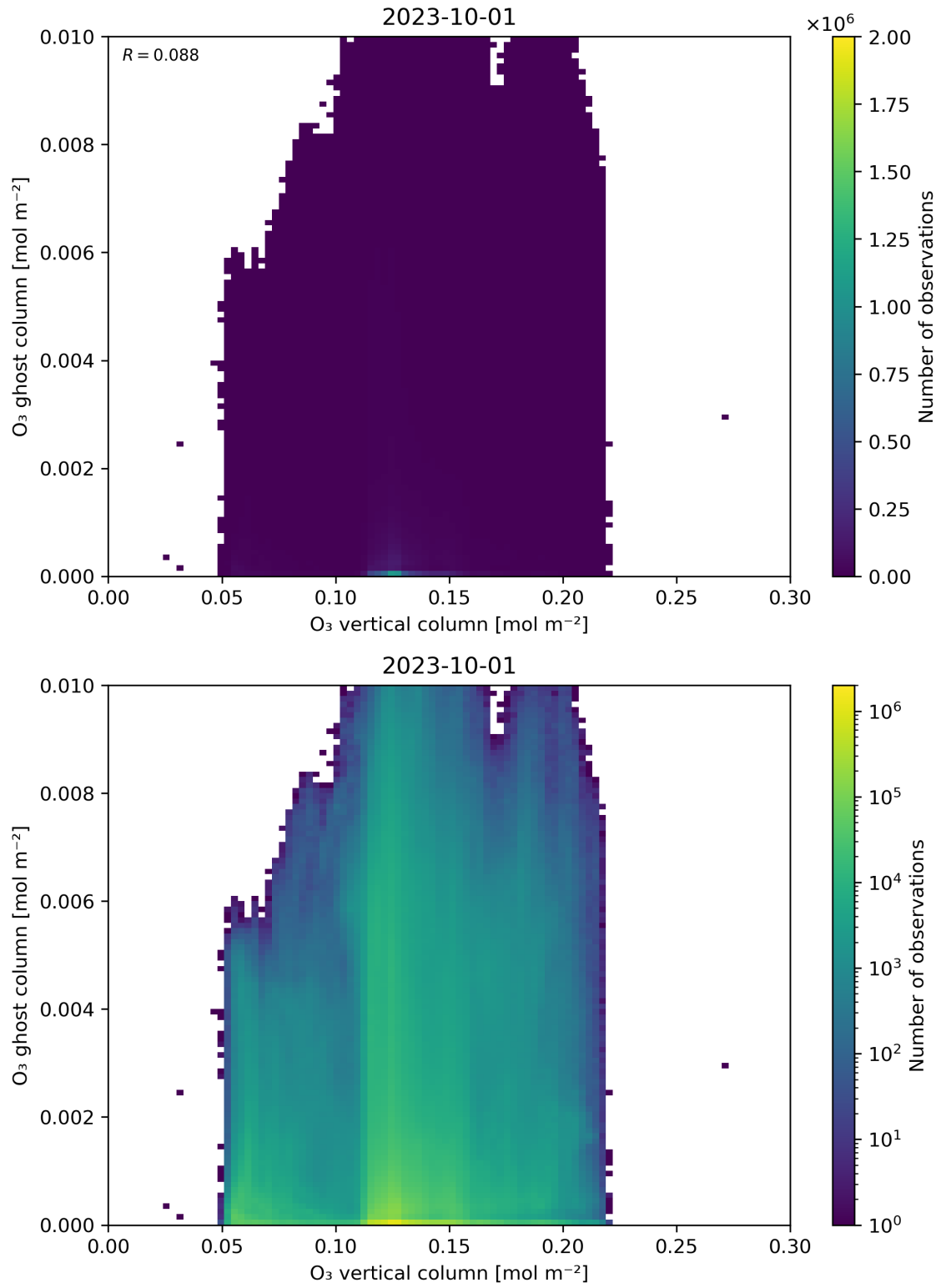
Figure 40: Scatter density plot of “O 3 vertical column” against “O 3 ghost column” for 2023-10-01 to 2023-10-02.
