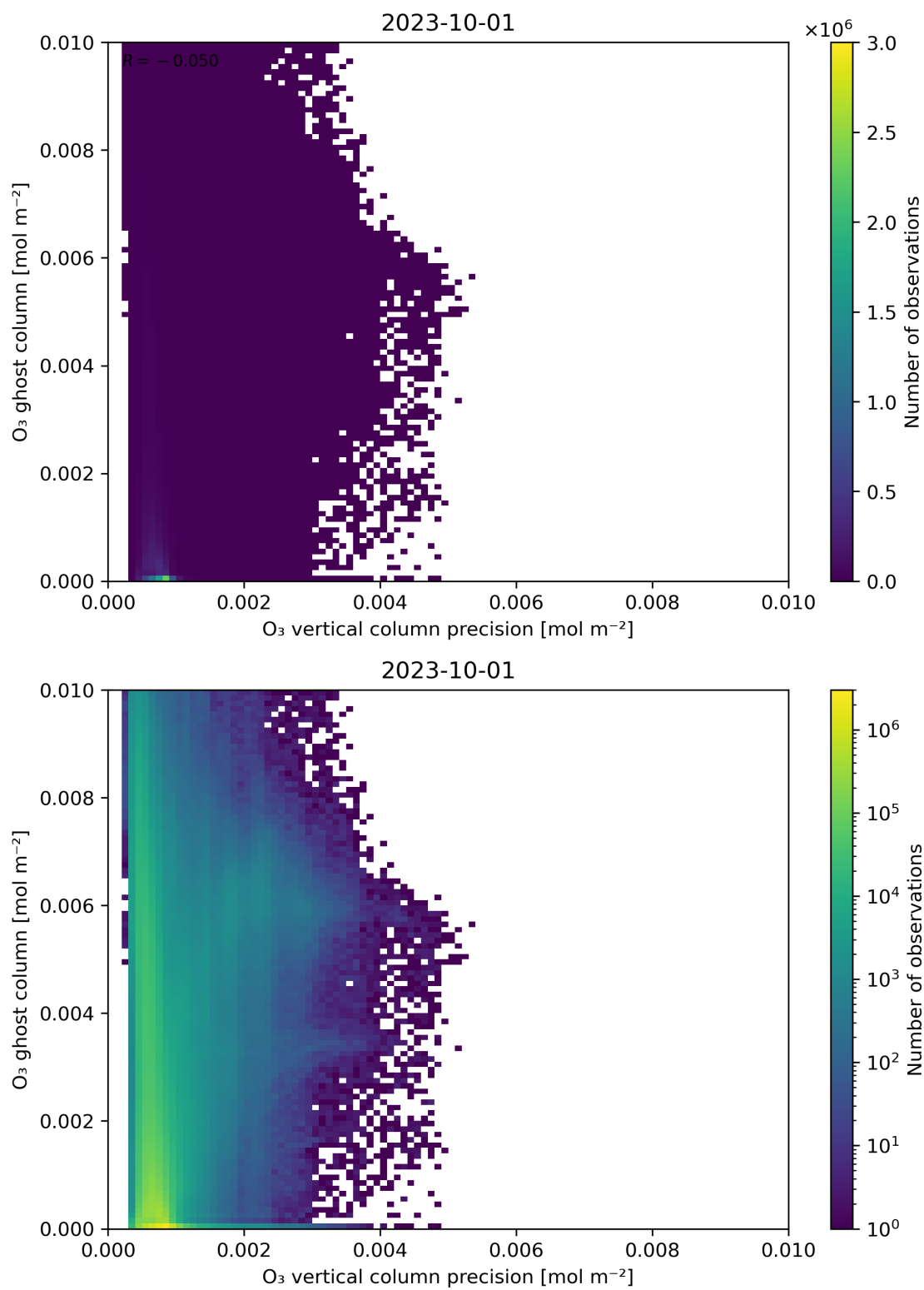
Figure 43: Scatter density plot of “ \text{O}_3 vertical column precision” against “ \text{O}_3 ghost column” for 2023-10-01 to 2023-10-02.
