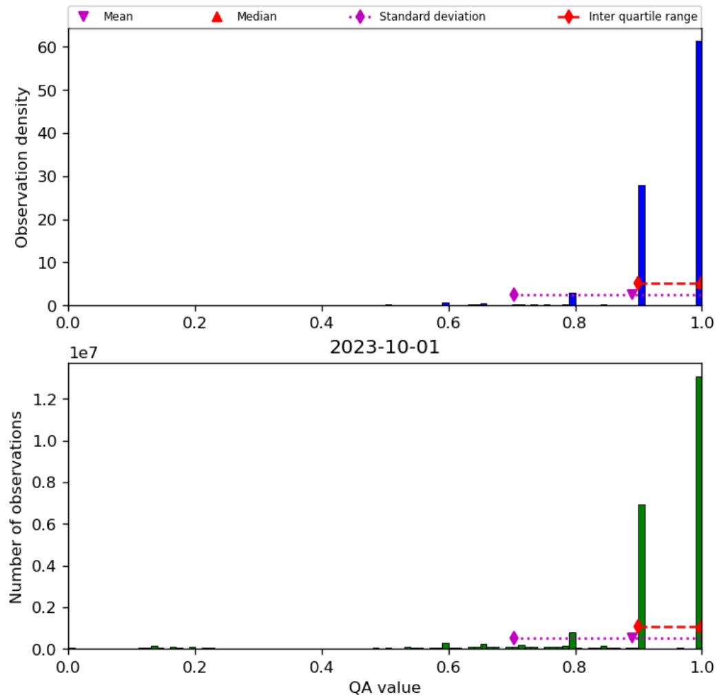
Figure 20: Histogram of “QA value” for 2023-10-01 to 2023-10-02
