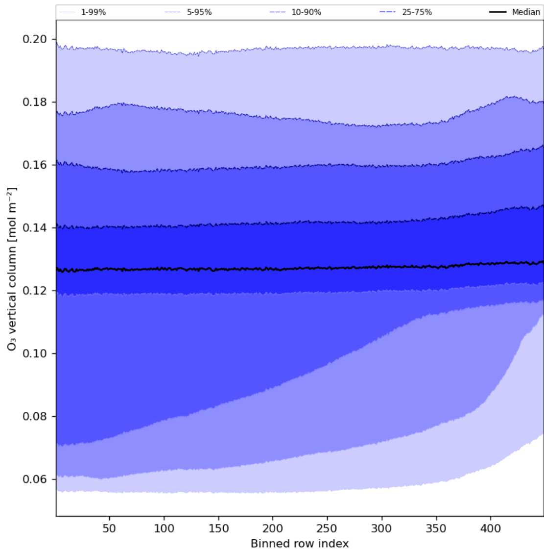
Figure 28: Along track statistics of “O 3 vertical column” for 2023-10-01 to 2023-10-02
