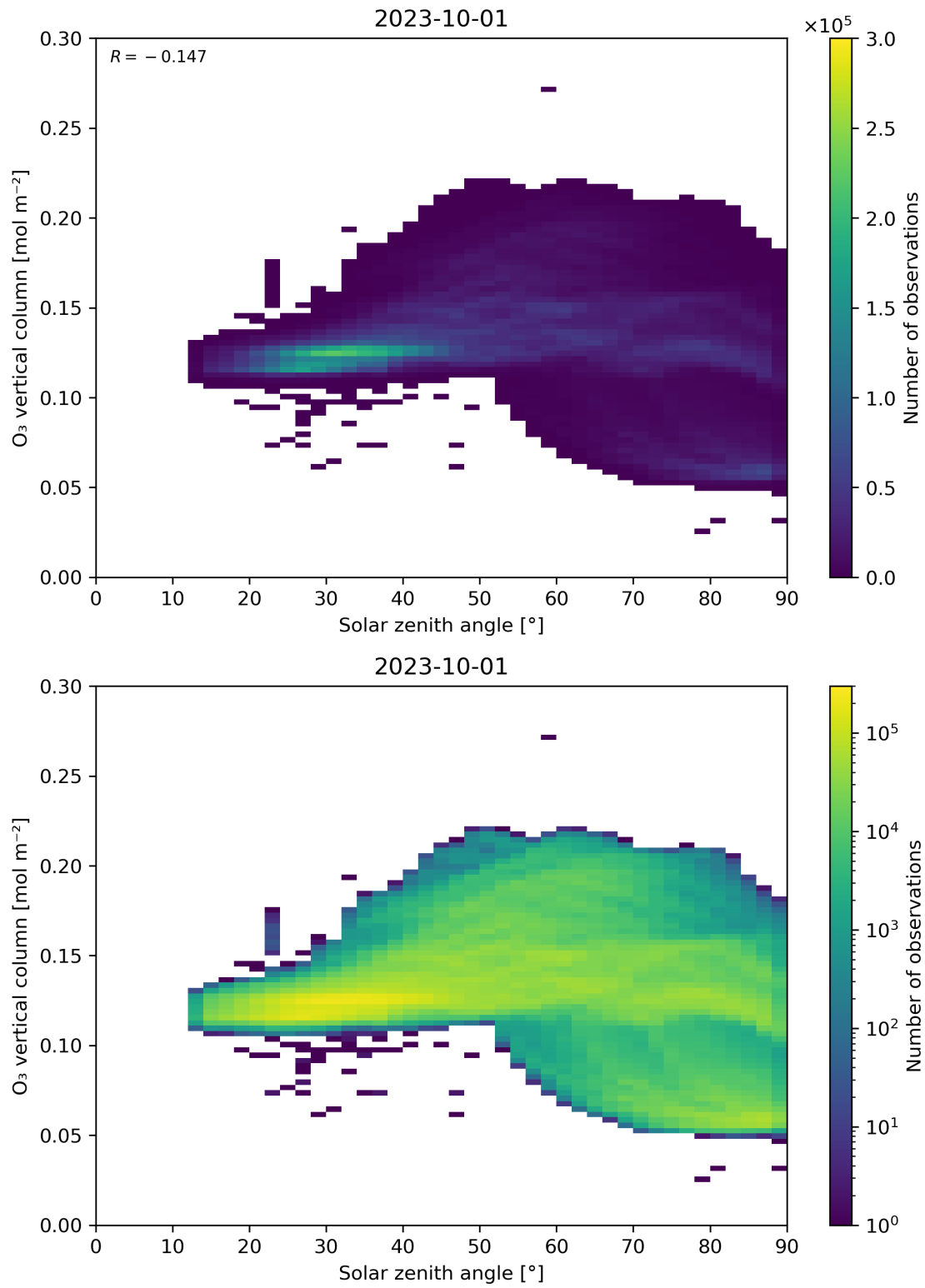
Figure 47: Scatter density plot of “Solar zenith angle” against “O 3 vertical column” for 2023-10-01 to 2023-10-02.
