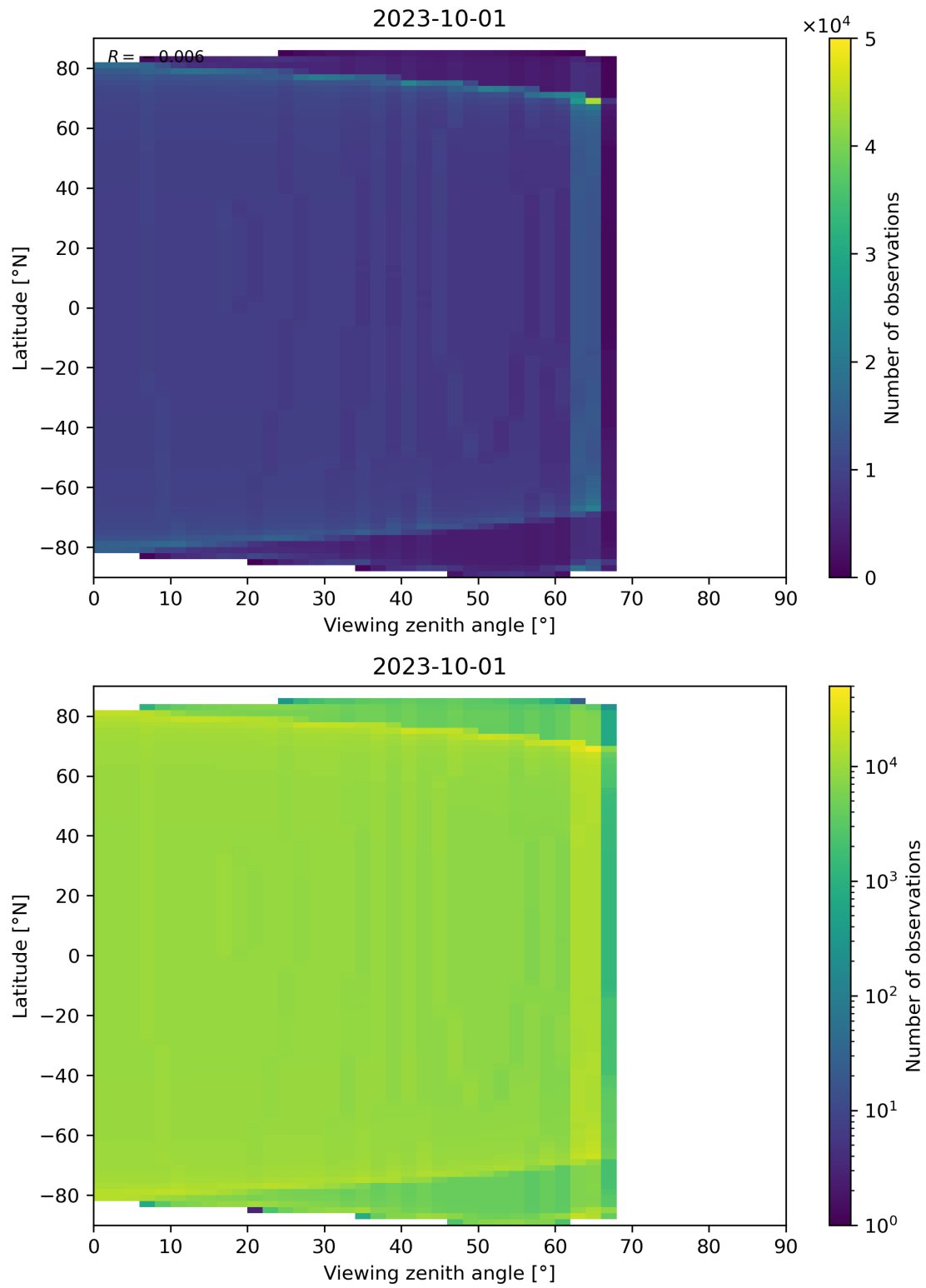
Figure 49: Scatter density plot of “Viewing zenith angle” against “Latitude” for 2023-10-01 to 2023-10-02.
