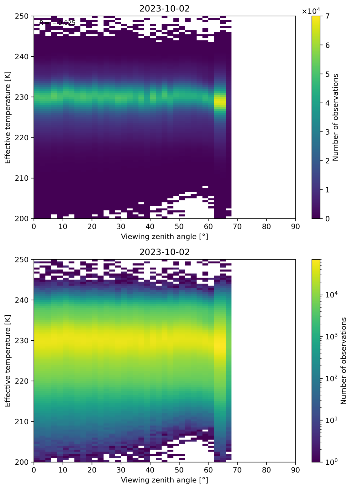
Figure 50: Scatter density plot of “Viewing zenith angle” against “Effective temperature” for 2023-10-01 to 2023-10-03.
