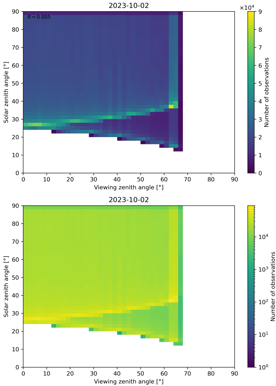
Figure 54: Scatter density plot of “Viewing zenith angle” against “Solar zenith angle” for 2023-10-01 to 2023-10-03.
