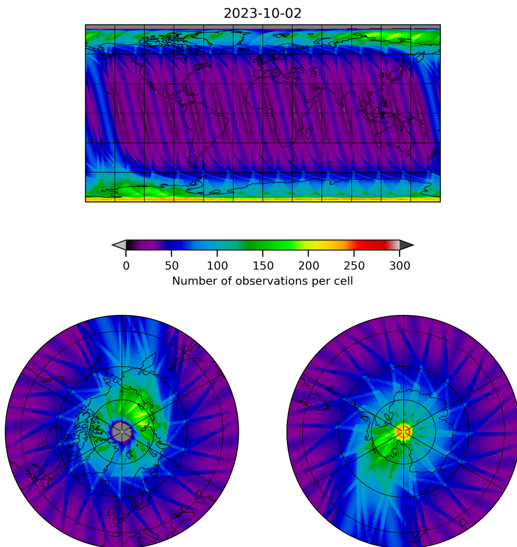
Figure 12: Map of the number of observations for 2023-10-01 to 2023-10-03
