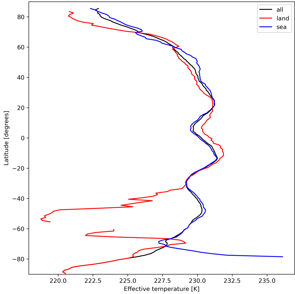
Figure 17: Zonal average of “Effective temperature” for 2023-10-01 to 2023-10-03.
