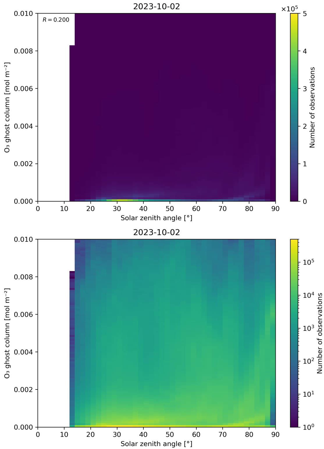
Figure 46: Scatter density plot of “Solar zenith angle” against “O 3 ghost column” for 2023-10-01 to 2023-10-03.
