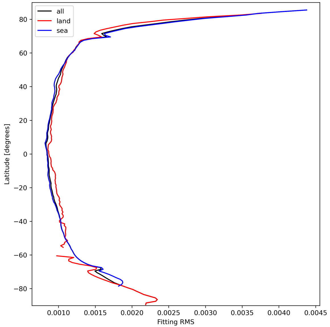
Figure 16: Zonal average of “Fitting RMS” for 2023-10-01 to 2023-10-03.
