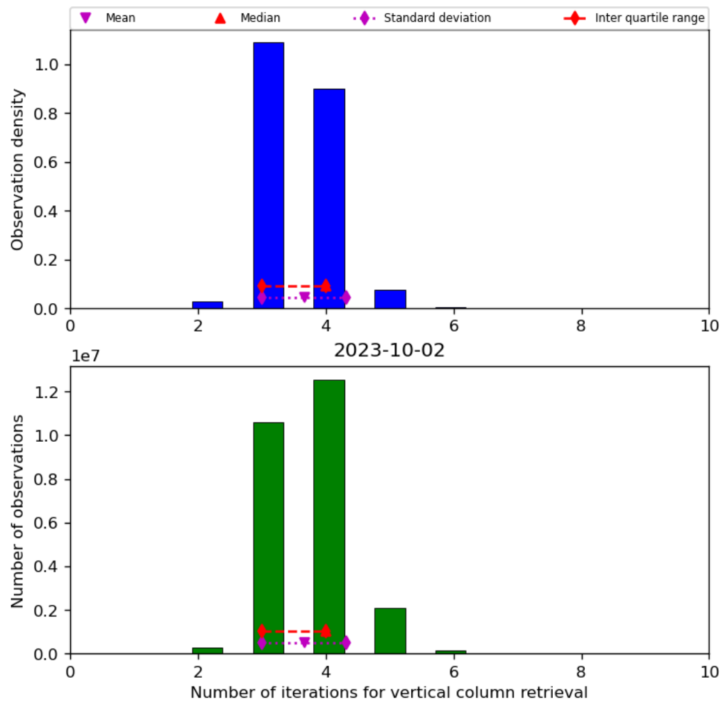
Figure 26: Histogram of “Number of iterations for vertical column retrieval” for 2023-10-01 to 2023-10-03
