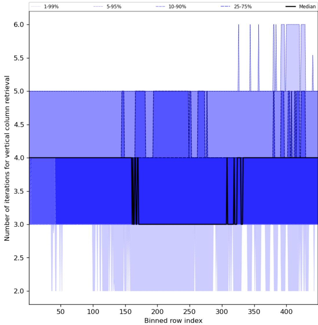
Figure 33: Along track statistics of “Number of iterations for vertical column retrieval” for 2023-10-01 to 2023-10-03
