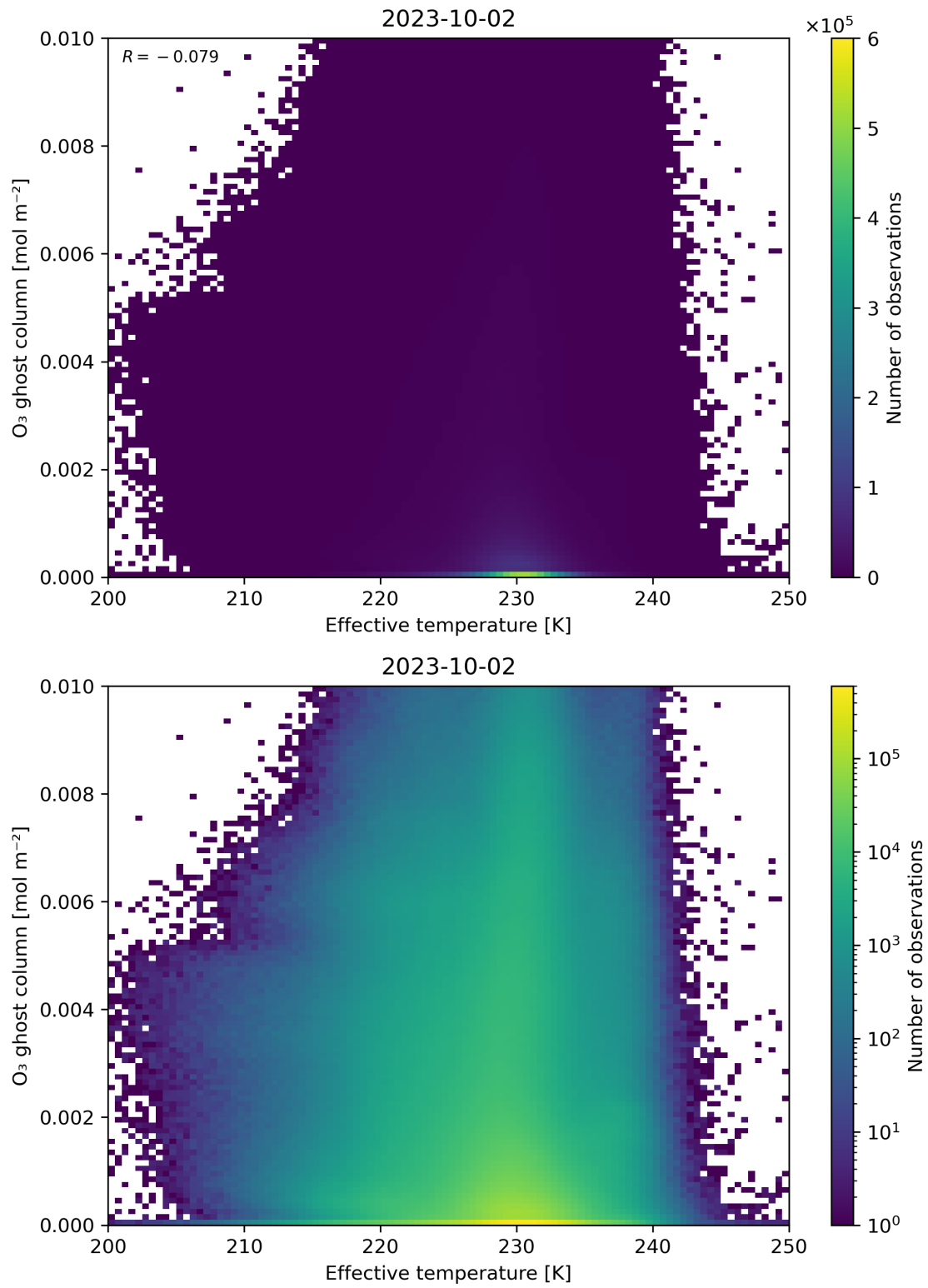
Figure 38: Scatter density plot of “Effective temperature” against “O 3 ghost column” for 2023-10-01 to 2023-10-03.
