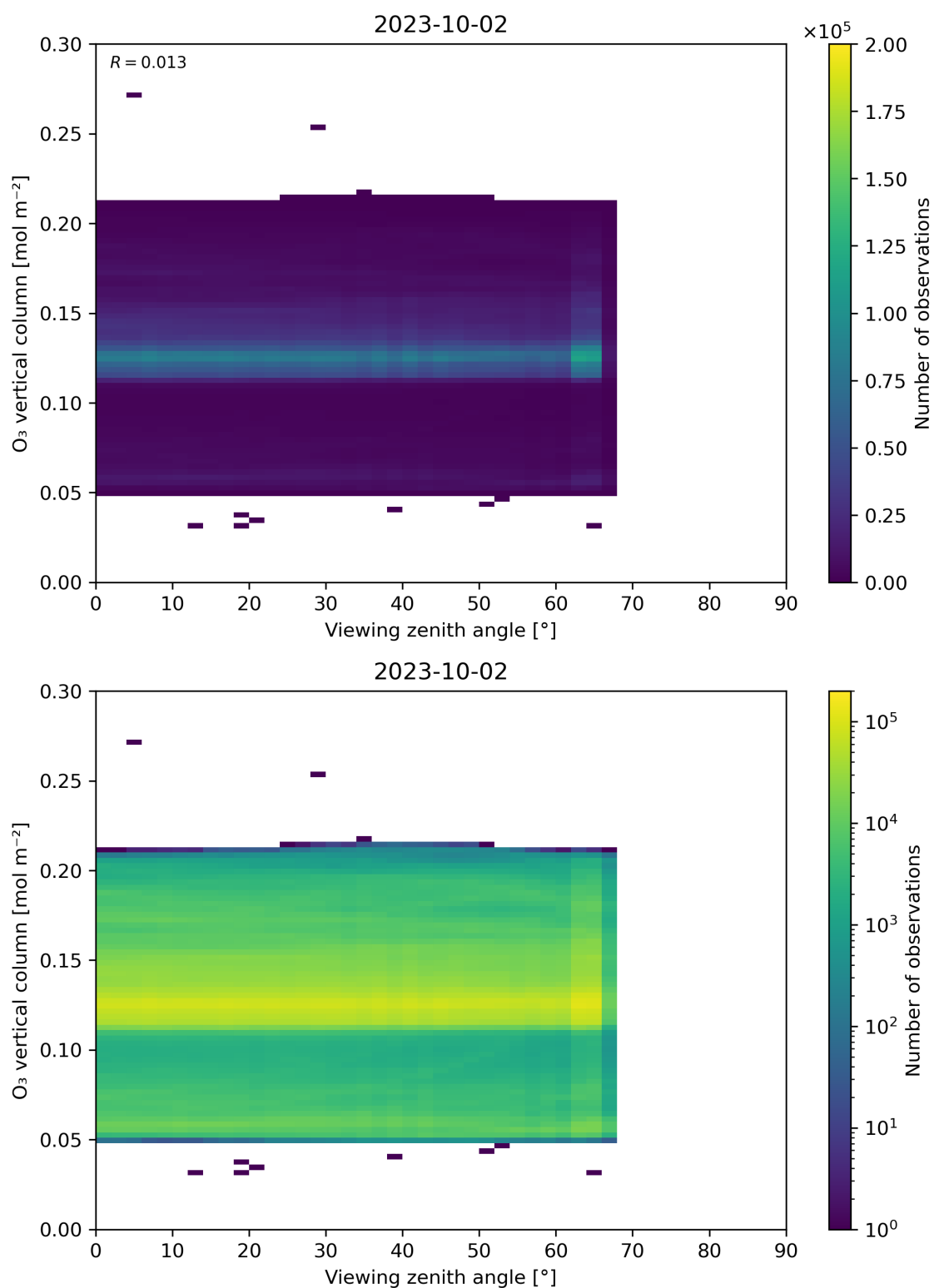
Figure 52: Scatter density plot of “Viewing zenith angle” against “O 3 vertical column” for 2023-10-01 to 2023-10-03.
