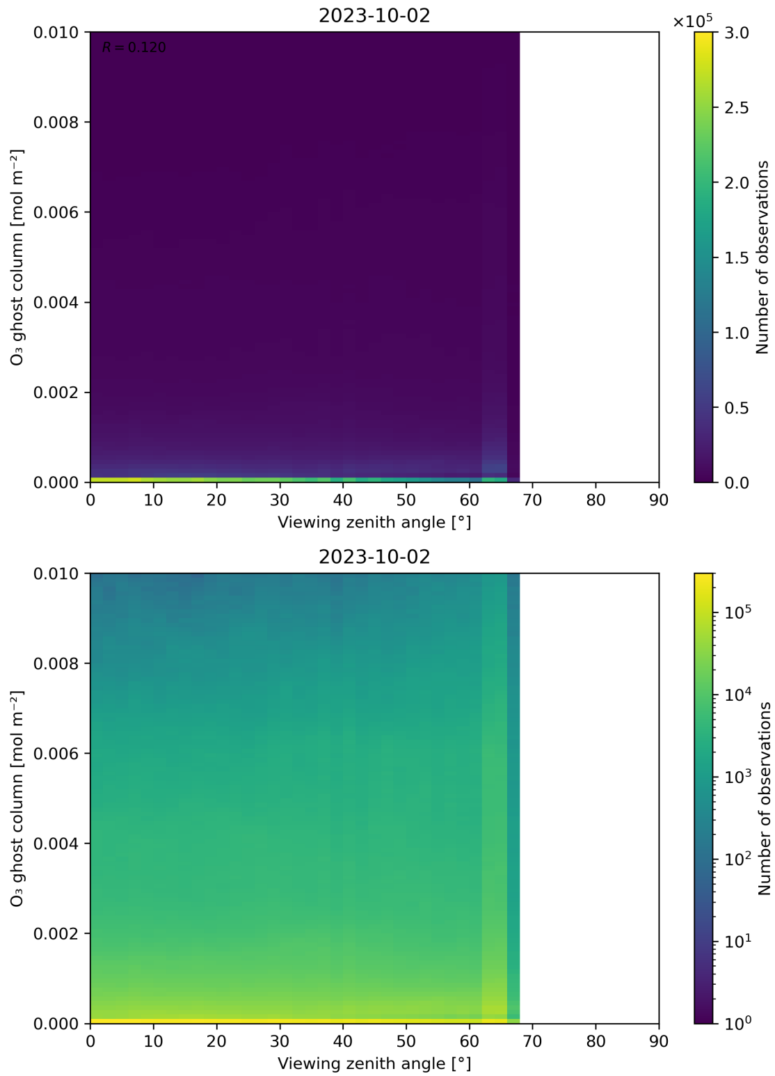
Figure 51: Scatter density plot of “Viewing zenith angle” against “O 3 ghost column” for 2023-10-01 to 2023-10-03.
