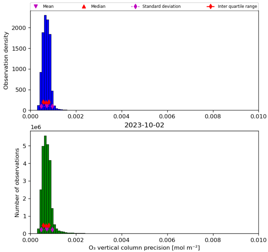
Figure 22: Histogram of “O 3 vertical column precision” for 2023-10-01 to 2023-10-03
