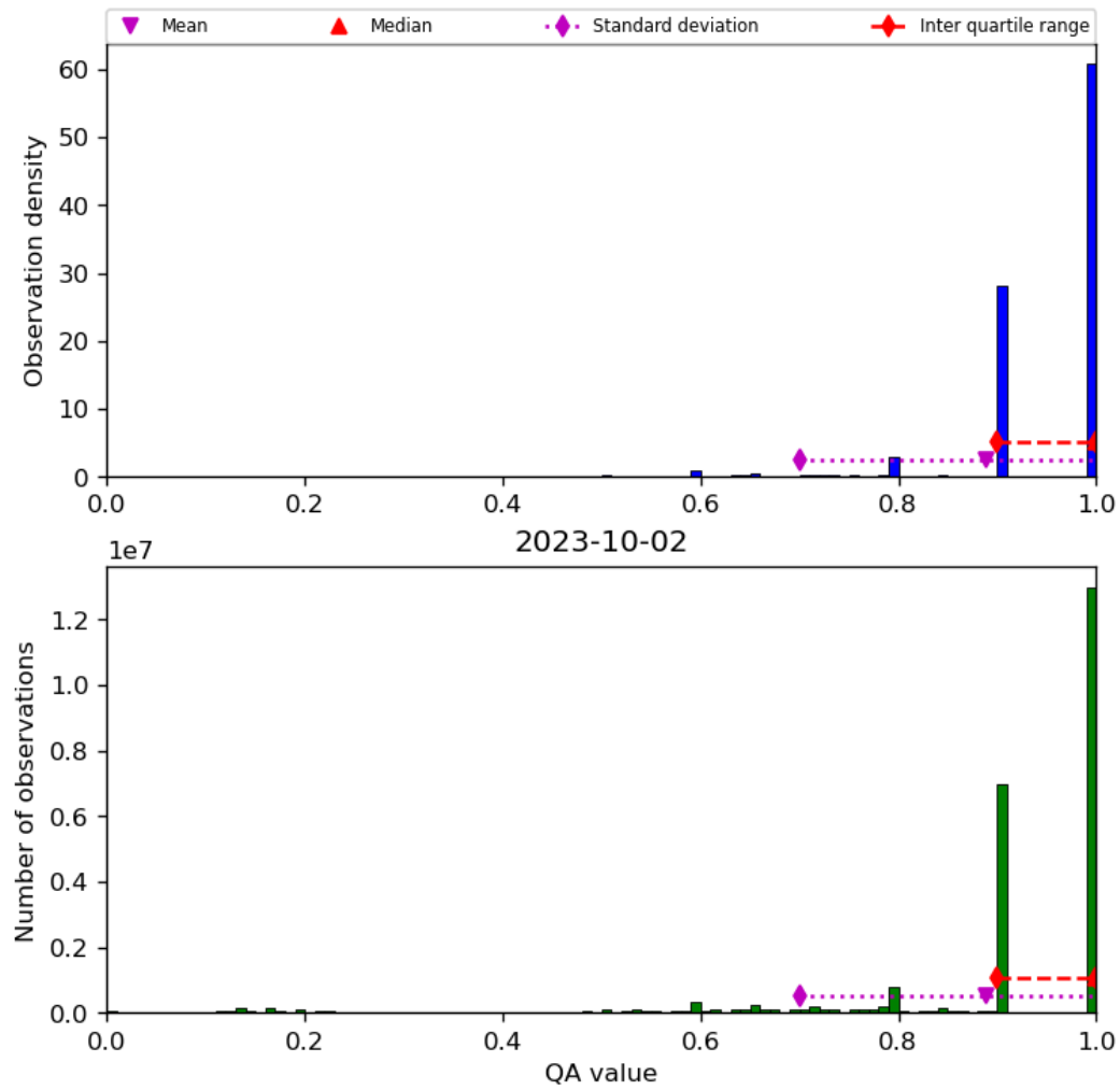
Figure 20: Histogram of “QA value” for 2023-10-01 to 2023-10-03
