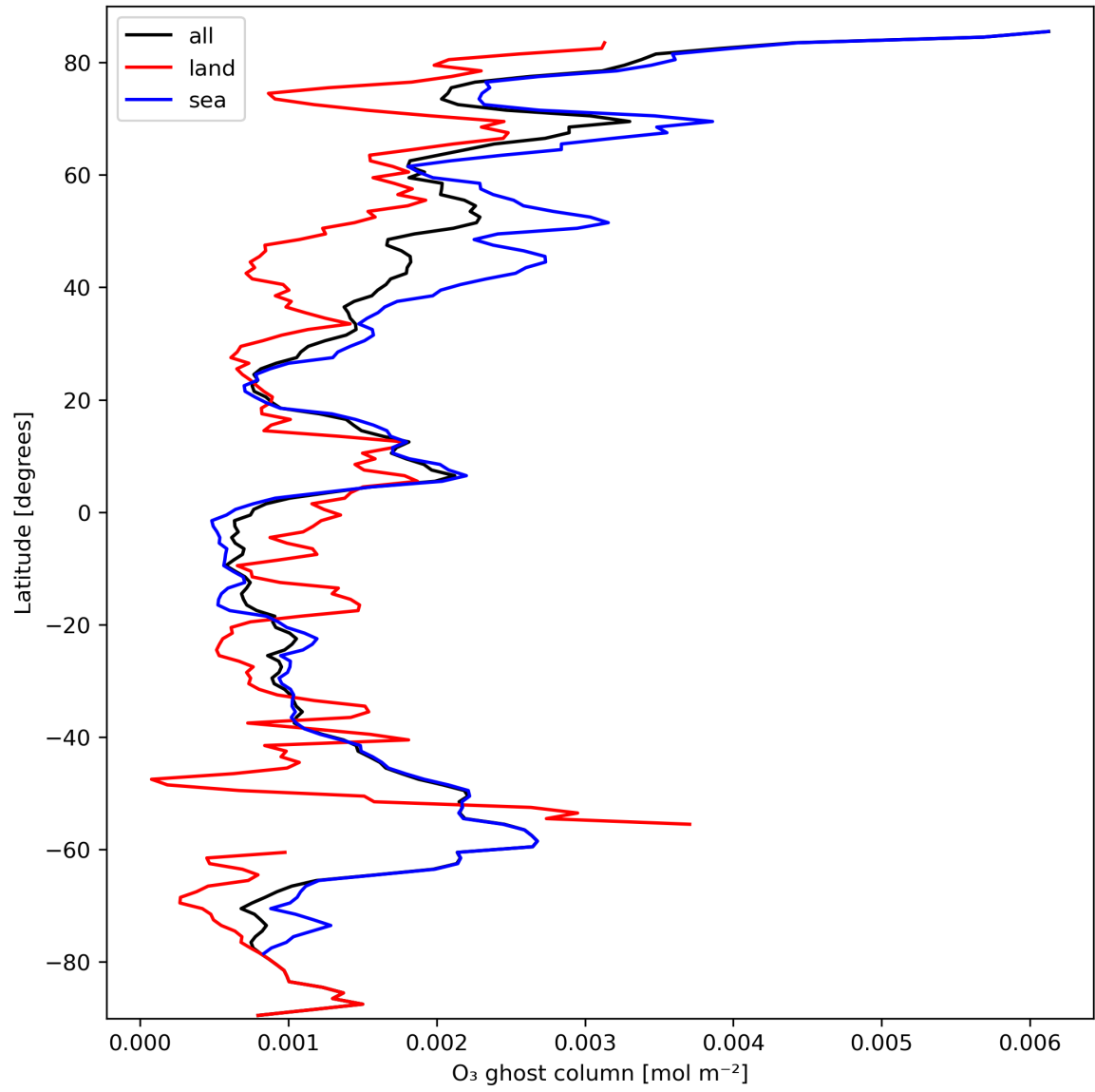
Figure 18: Zonal average of "O 3 ghost column" for 2023-10-01 to 2023-10-03.
