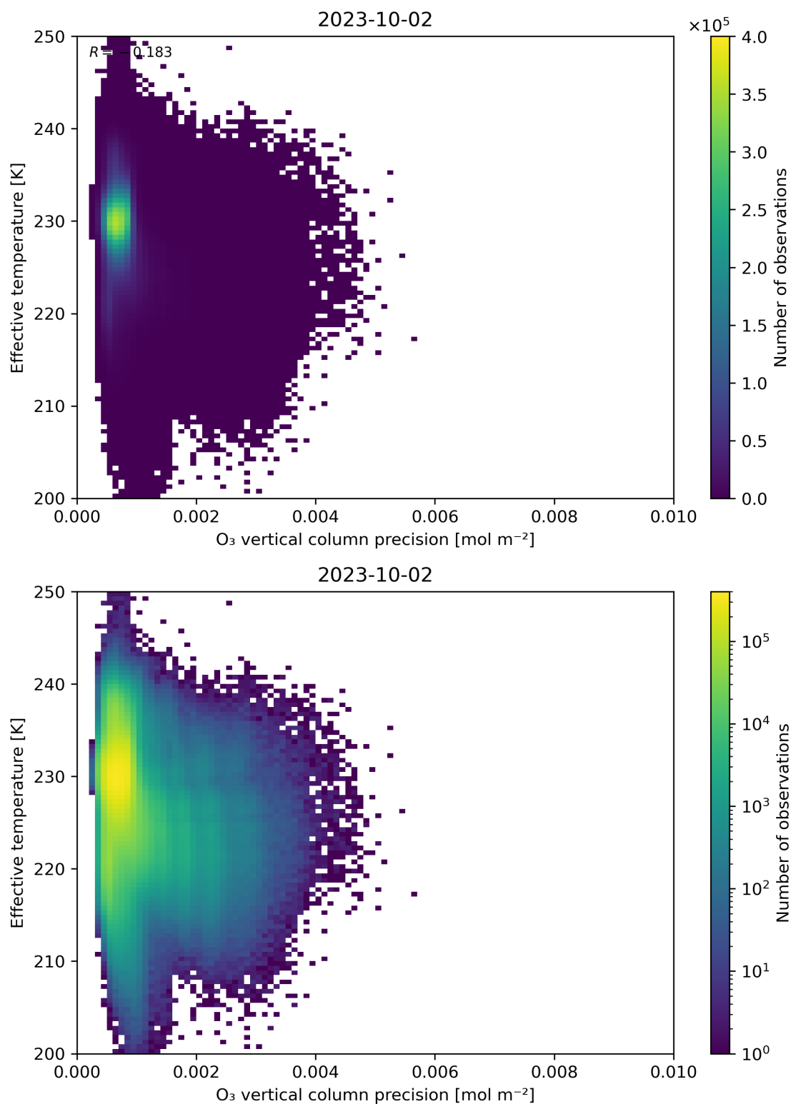
Figure 42: Scatter density plot of “O 3 vertical column precision” against “Effective temperature” for 2023-10-01 to 2023-10-03.
