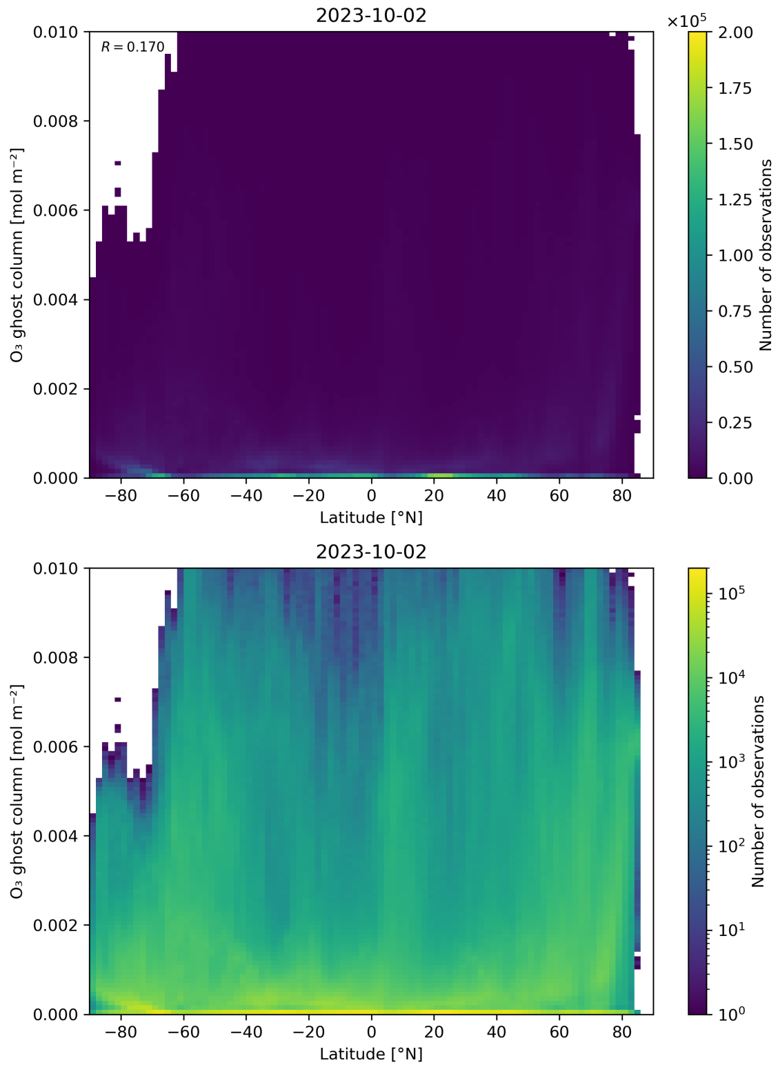
Figure 35: Scatter density plot of “Latitude” against “O 3 ghost column” for 2023-10-01 to 2023-10-03.
