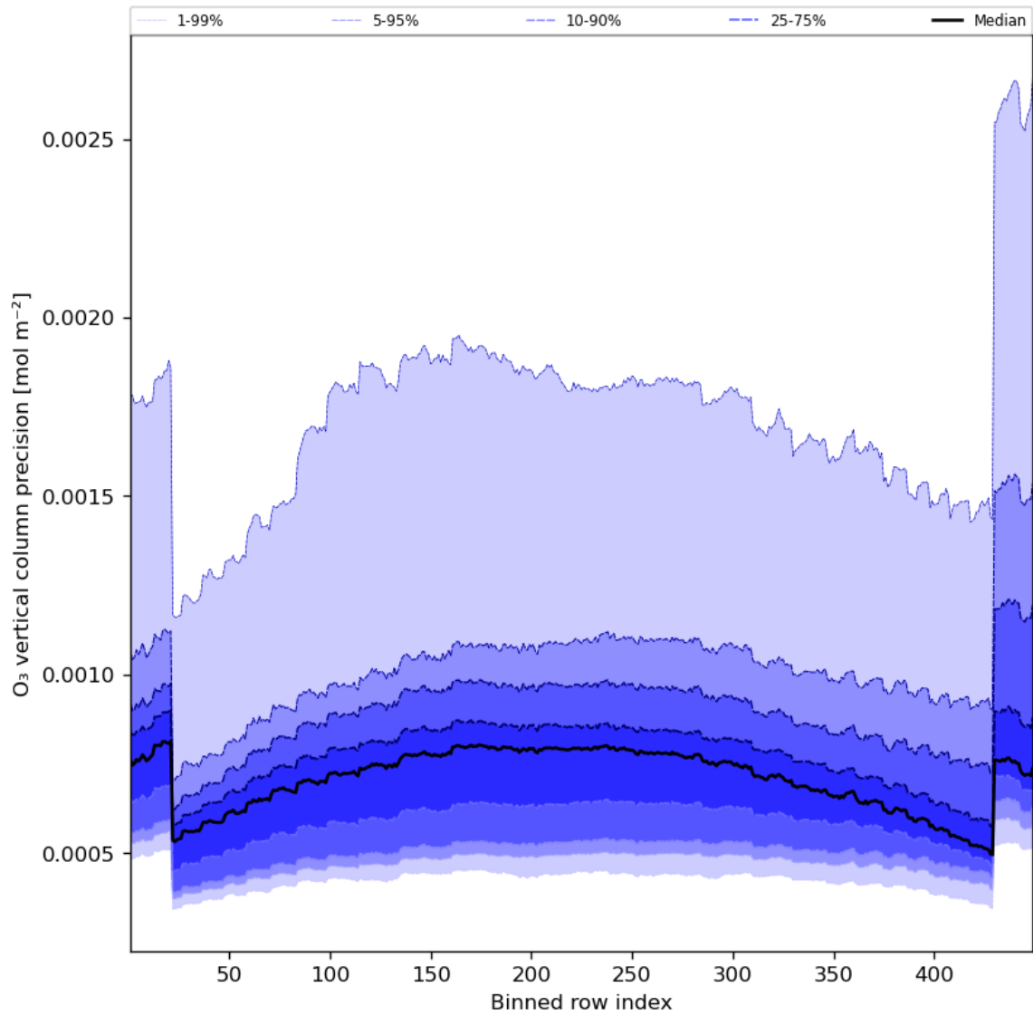
Figure 29: Along track statistics of “O 3 vertical column precision” for 2023-10-01 to 2023-10-03
