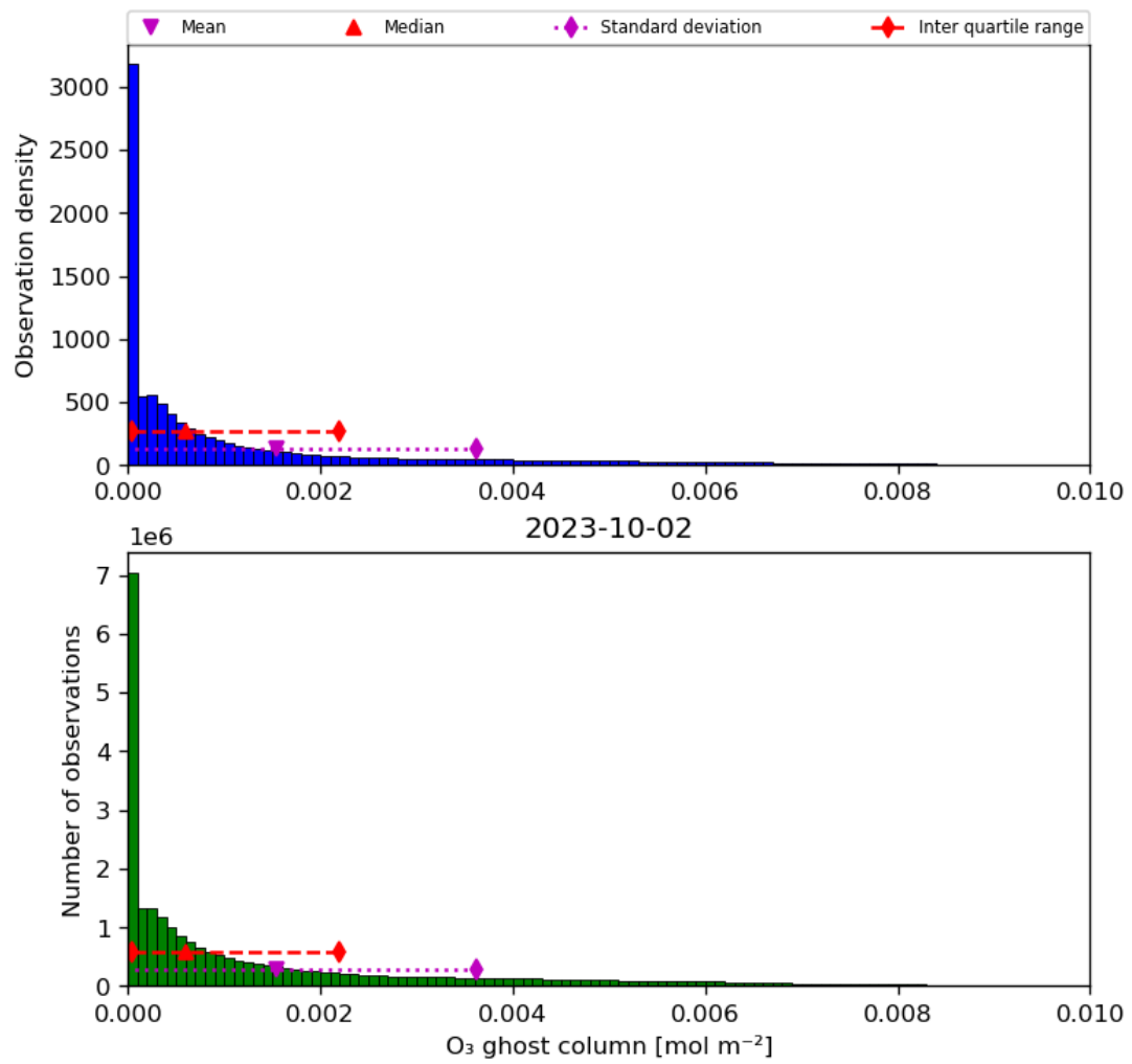
Figure 25: Histogram of “O 3 ghost column” for 2023-10-01 to 2023-10-03
