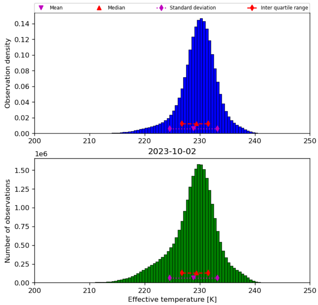
Figure 24: Histogram of “Effective temperature” for 2023-10-01 to 2023-10-03
