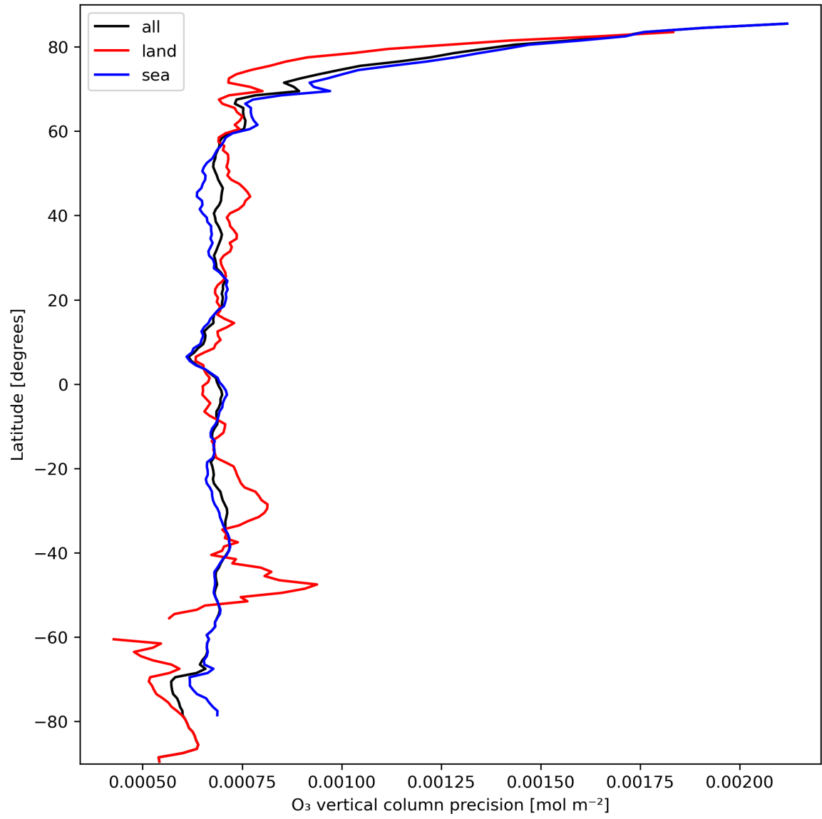
Figure 15: Zonal average of “O 3 vertical column precision” for 2023-10-01 to 2023-10-03.
