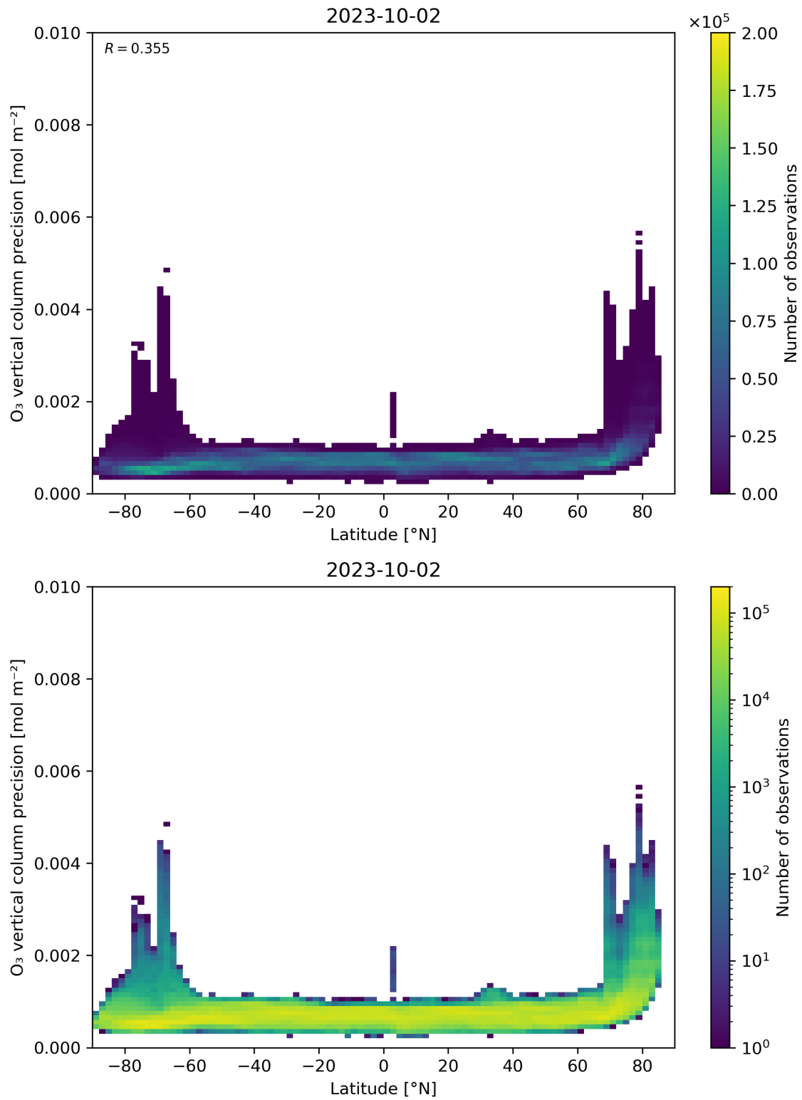
Figure 37: Scatter density plot of “Latitude” against “O 3 vertical column precision” for 2023-10-01 to 2023-10-03.
