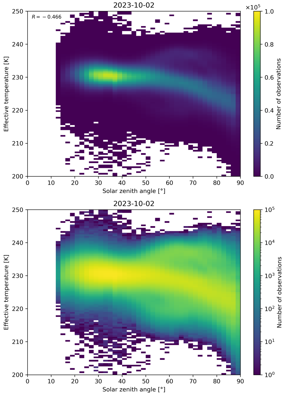
Figure 45: Scatter density plot of “Solar zenith angle” against “Effective temperature” for 2023-10-01 to 2023-10-03.
