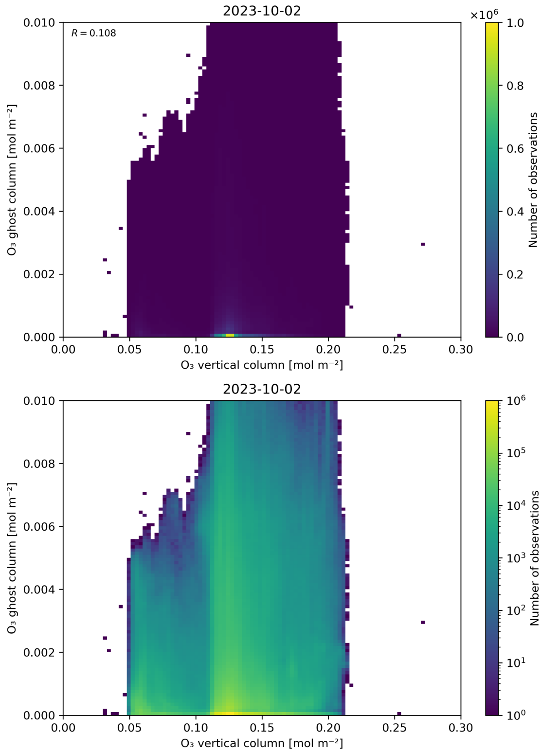
Figure 40: Scatter density plot of “O 3 vertical column” against “O 3 ghost column” for 2023-10-01 to 2023-10-03.
