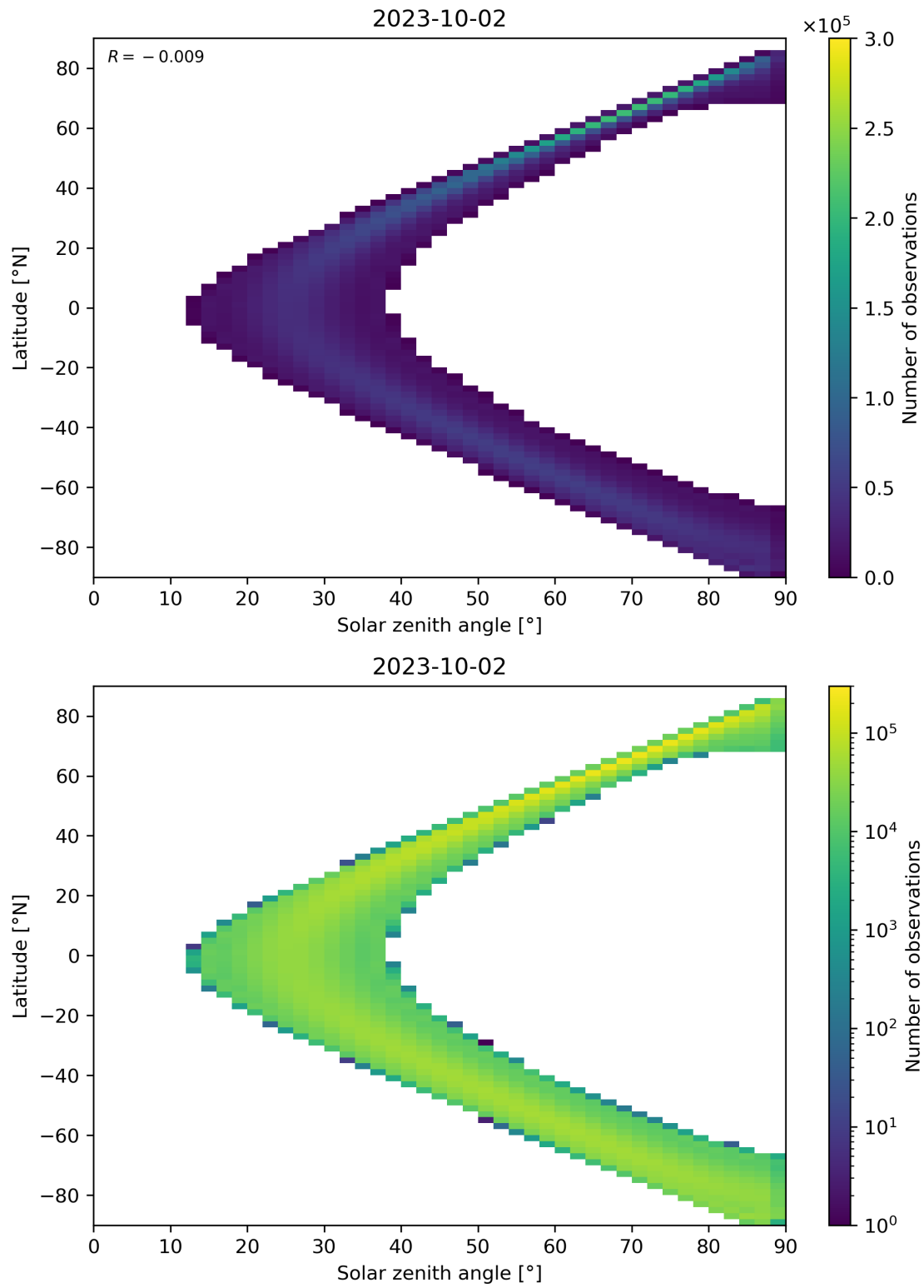
Figure 44: Scatter density plot of “Solar zenith angle” against “Latitude” for 2023-10-01 to 2023-10-03.
