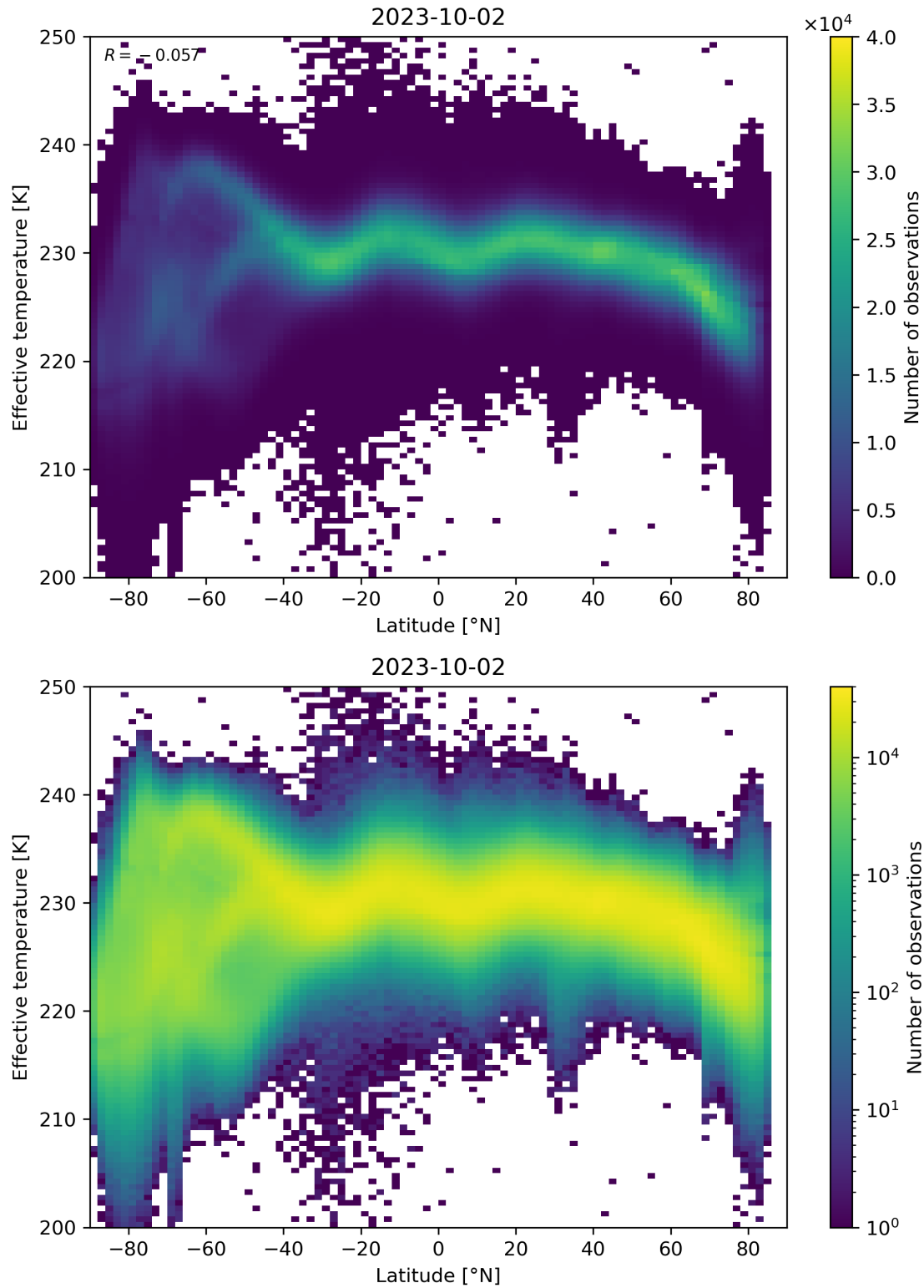
Figure 34: Scatter density plot of “Latitude” against “Effective temperature” for 2023-10-01 to 2023-10-03.
