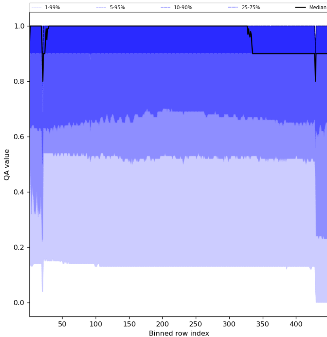
Figure 27: Along track statistics of “QA value” for 2023-10-01 to 2023-10-03
