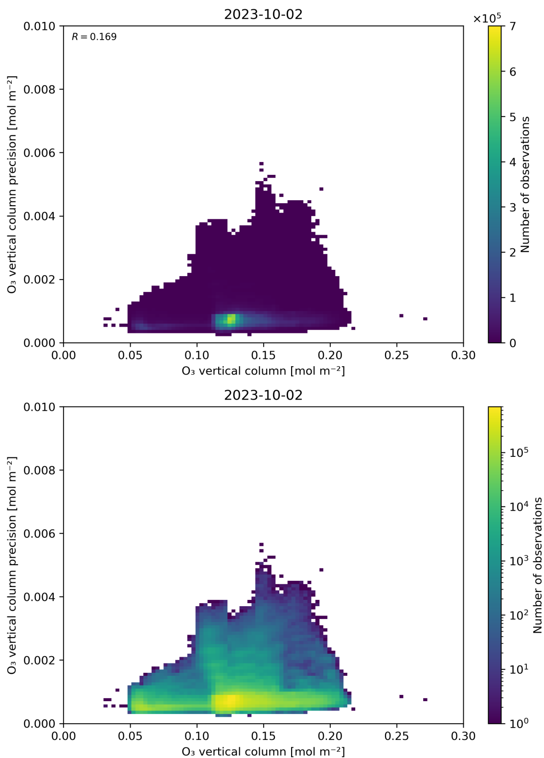
Figure 41: Scatter density plot of “O 3 vertical column” against “O 3 vertical column precision” for 2023-10-01 to 2023-10-03.
