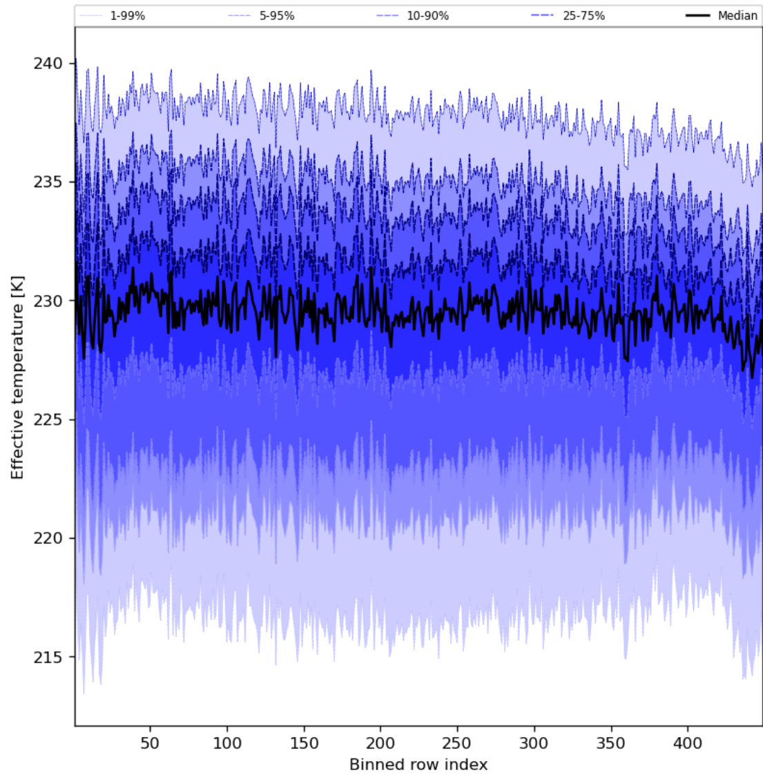
Figure 31: Along track statistics of “Effective temperature” for 2023-10-01 to 2023-10-03
