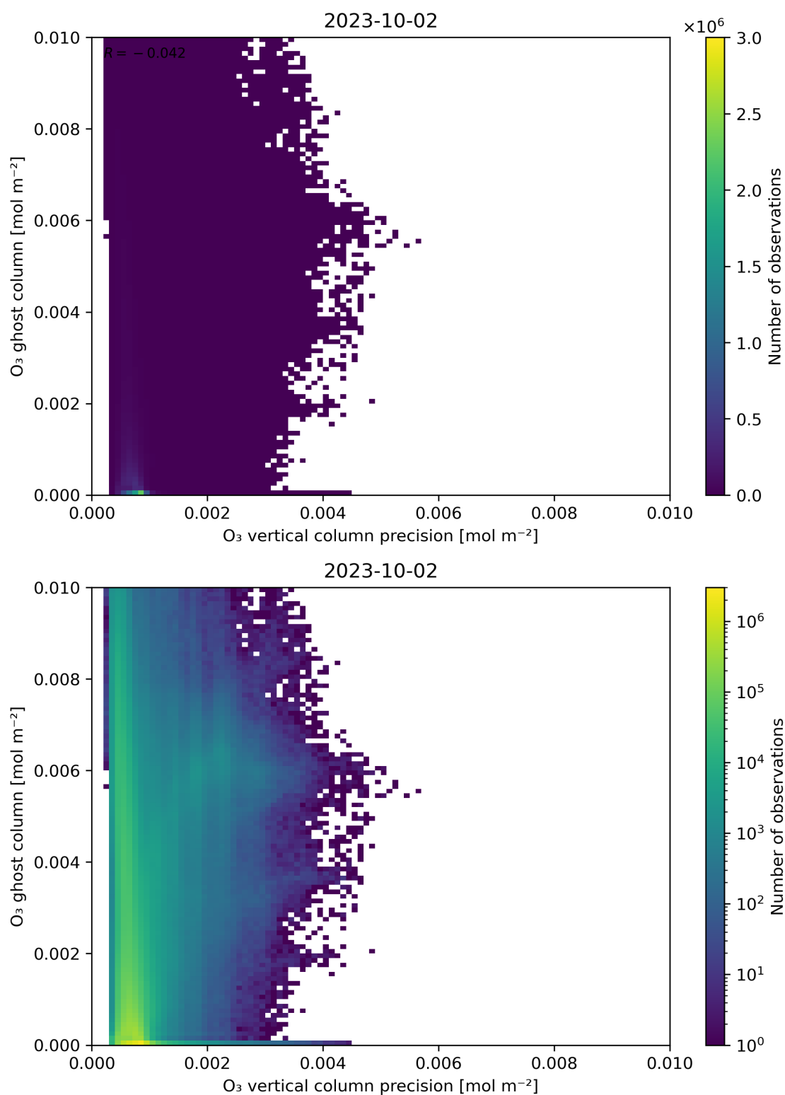
Figure 43: Scatter density plot of “O 3 vertical column precision” against “O 3 ghost column” for 2023-10-01 to 2023-10-03.
