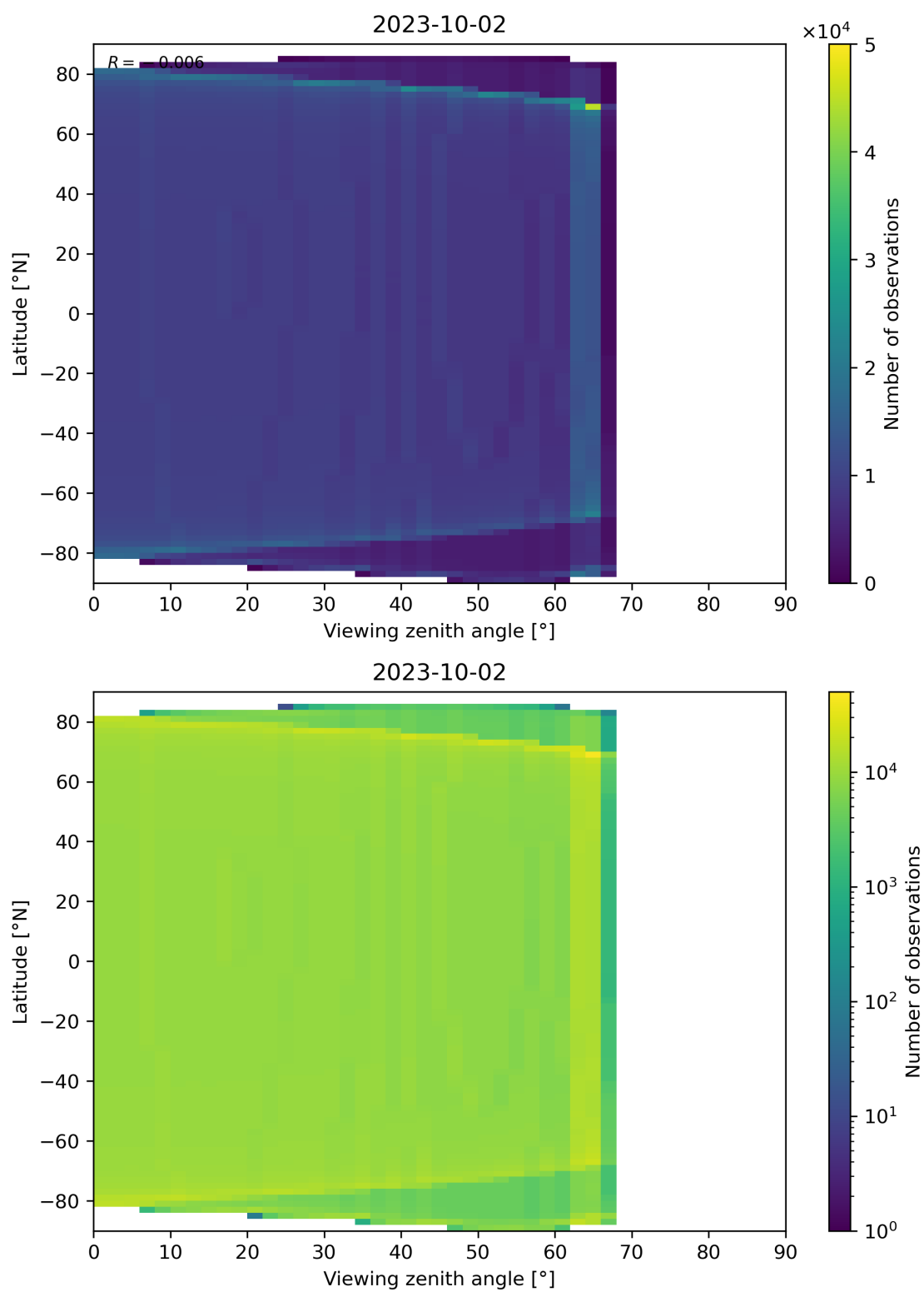
Figure 49: Scatter density plot of “Viewing zenith angle” against “Latitude” for 2023-10-01 to 2023-10-03.
