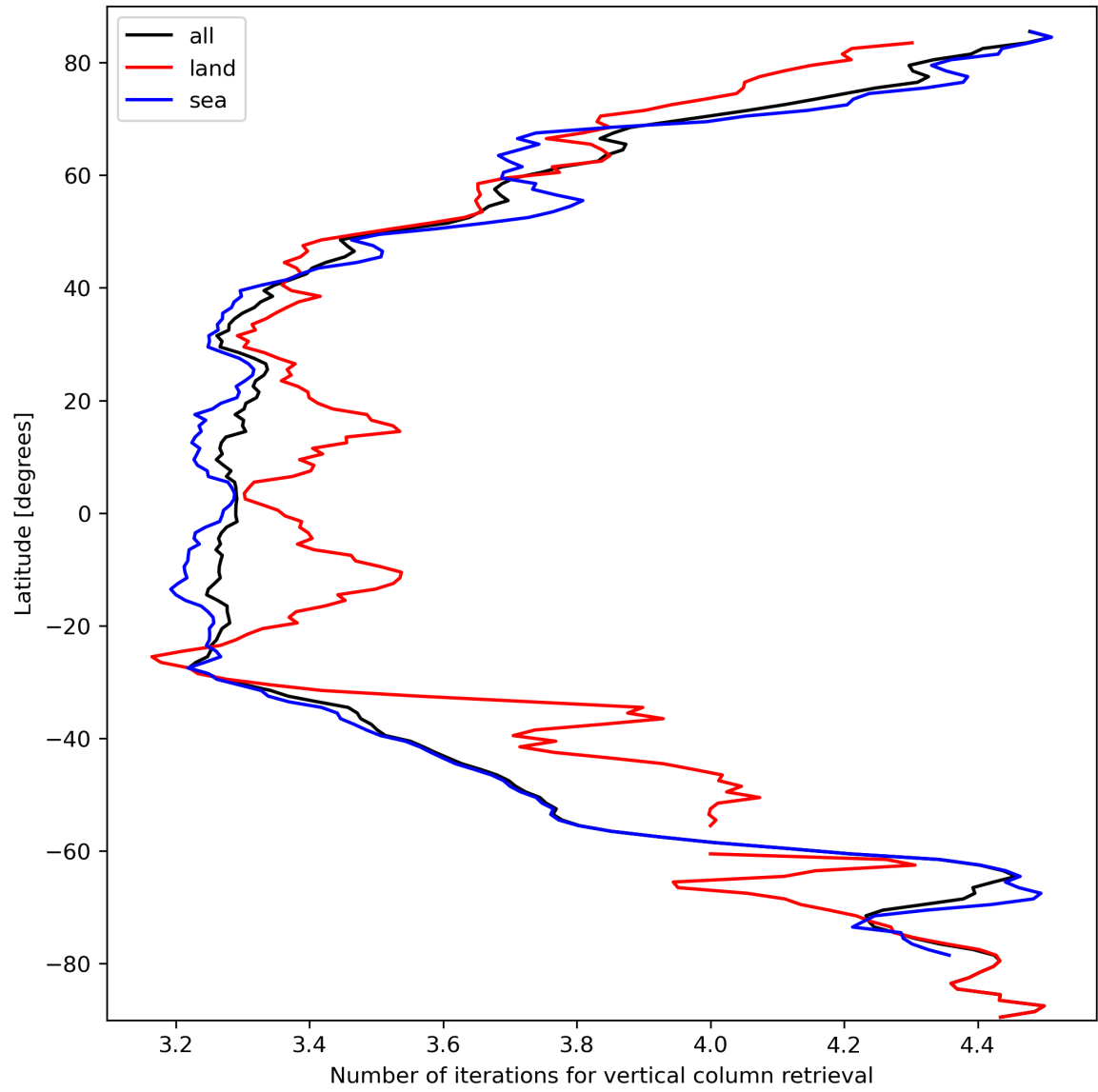
Figure 19: Zonal average of “Number of iterations for vertical column retrieval” for 2023-10-01 to 2023-10-03.
