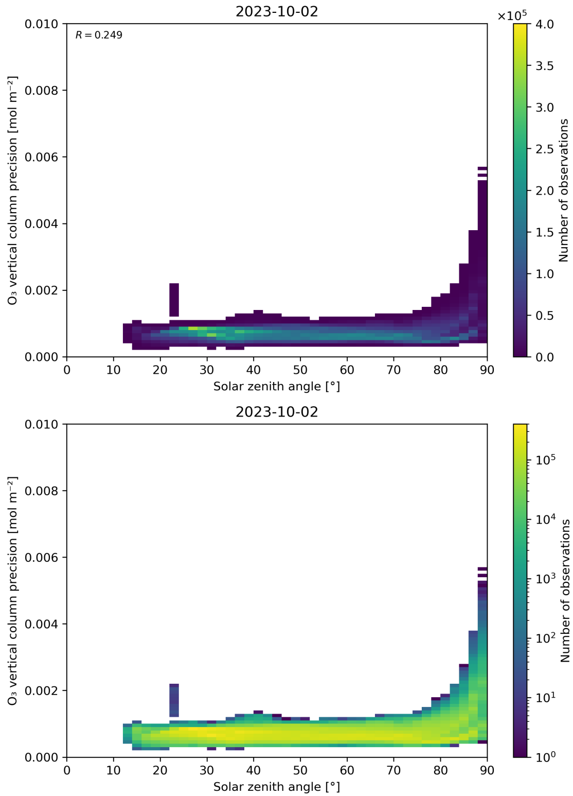
Figure 48: Scatter density plot of “Solar zenith angle” against “O 3 vertical column precision” for 2023-10-01 to 2023-10-03.
