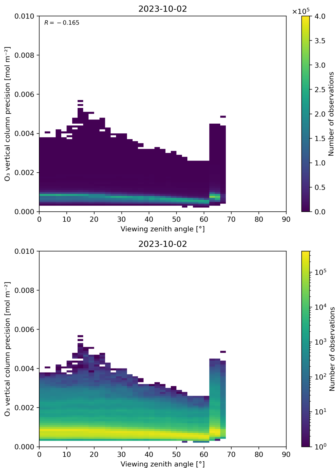
Figure 53: Scatter density plot of “Viewing zenith angle” against “O 3 vertical column precision” for 2023-10-01 to 2023-10-03.
