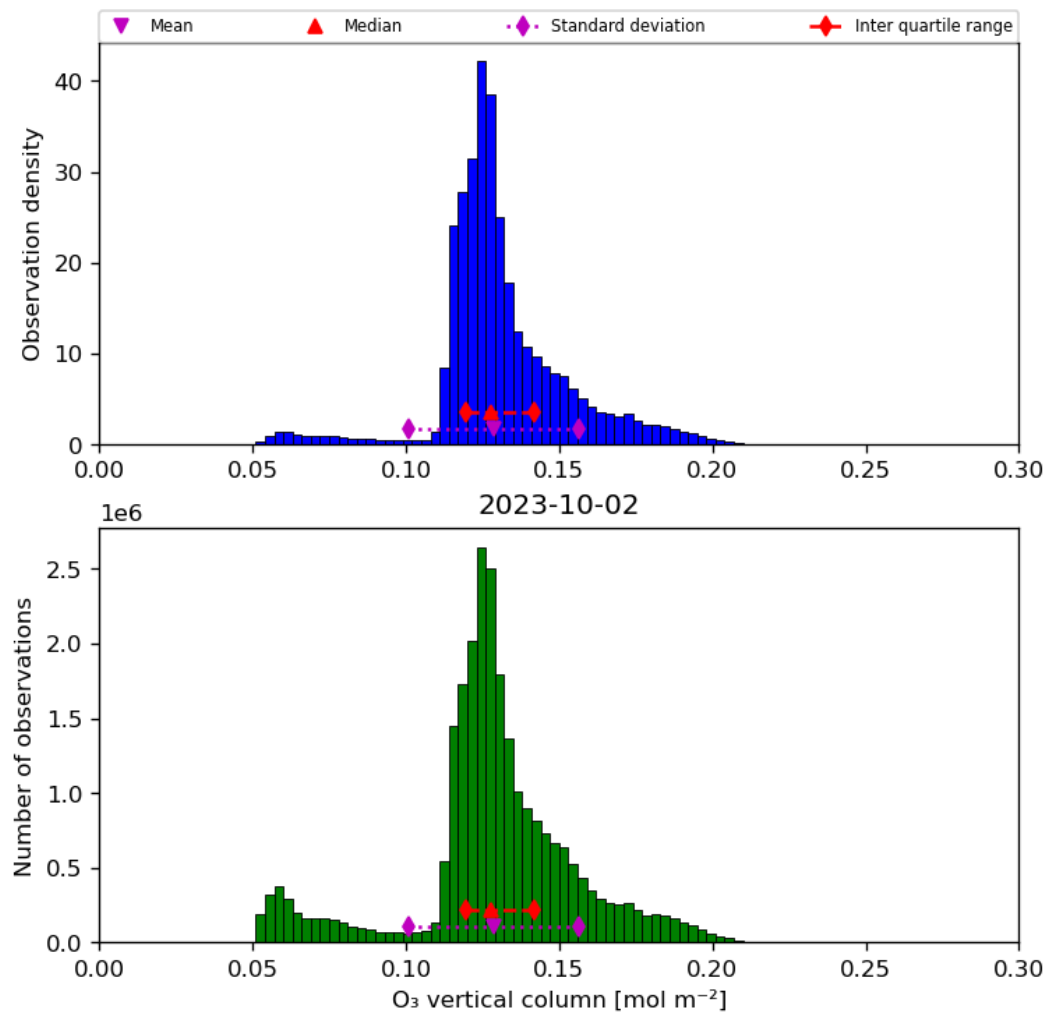
Figure 21: Histogram of “O 3 vertical column” for 2023-10-01 to 2023-10-03
