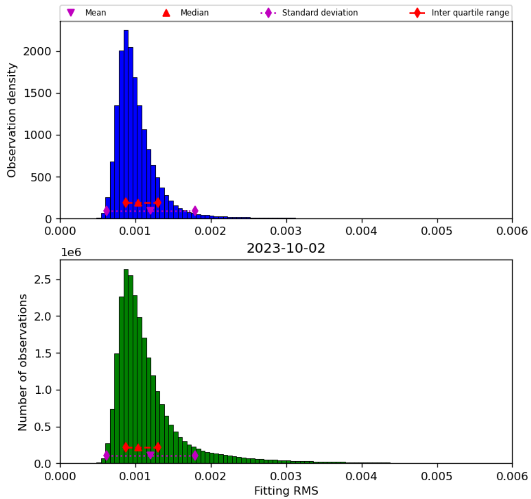
Figure 23: Histogram of “Fitting RMS” for 2023-10-01 to 2023-10-03
