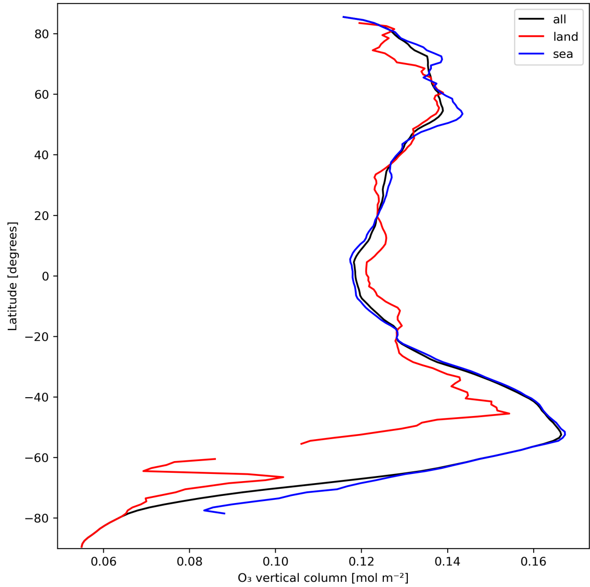
Figure 14: Zonal average of “O 3 vertical column” for 2023-10-01 to 2023-10-03.
