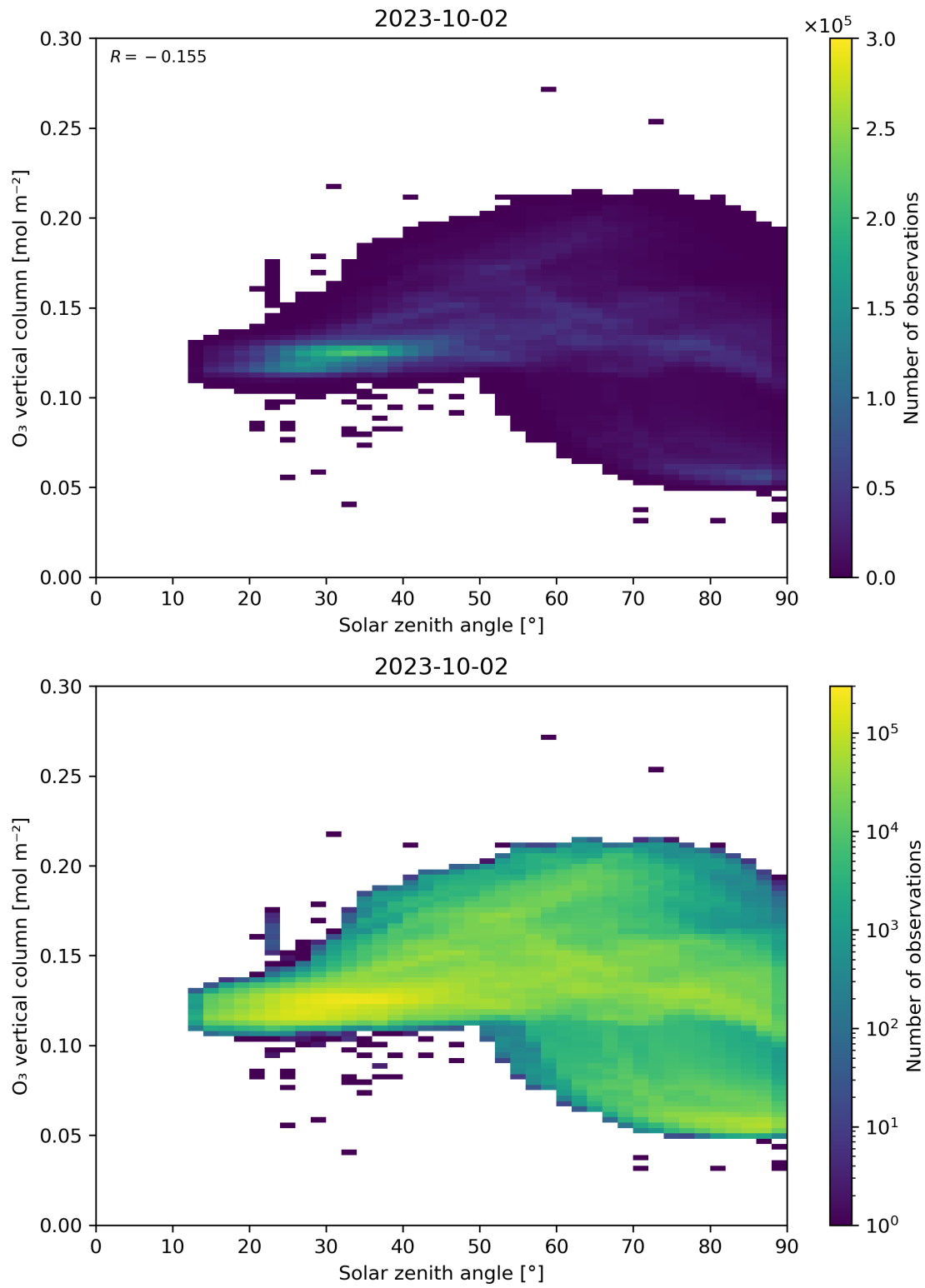
Figure 47: Scatter density plot of “Solar zenith angle” against “O 3 vertical column” for 2023-10-01 to 2023-10-03.
