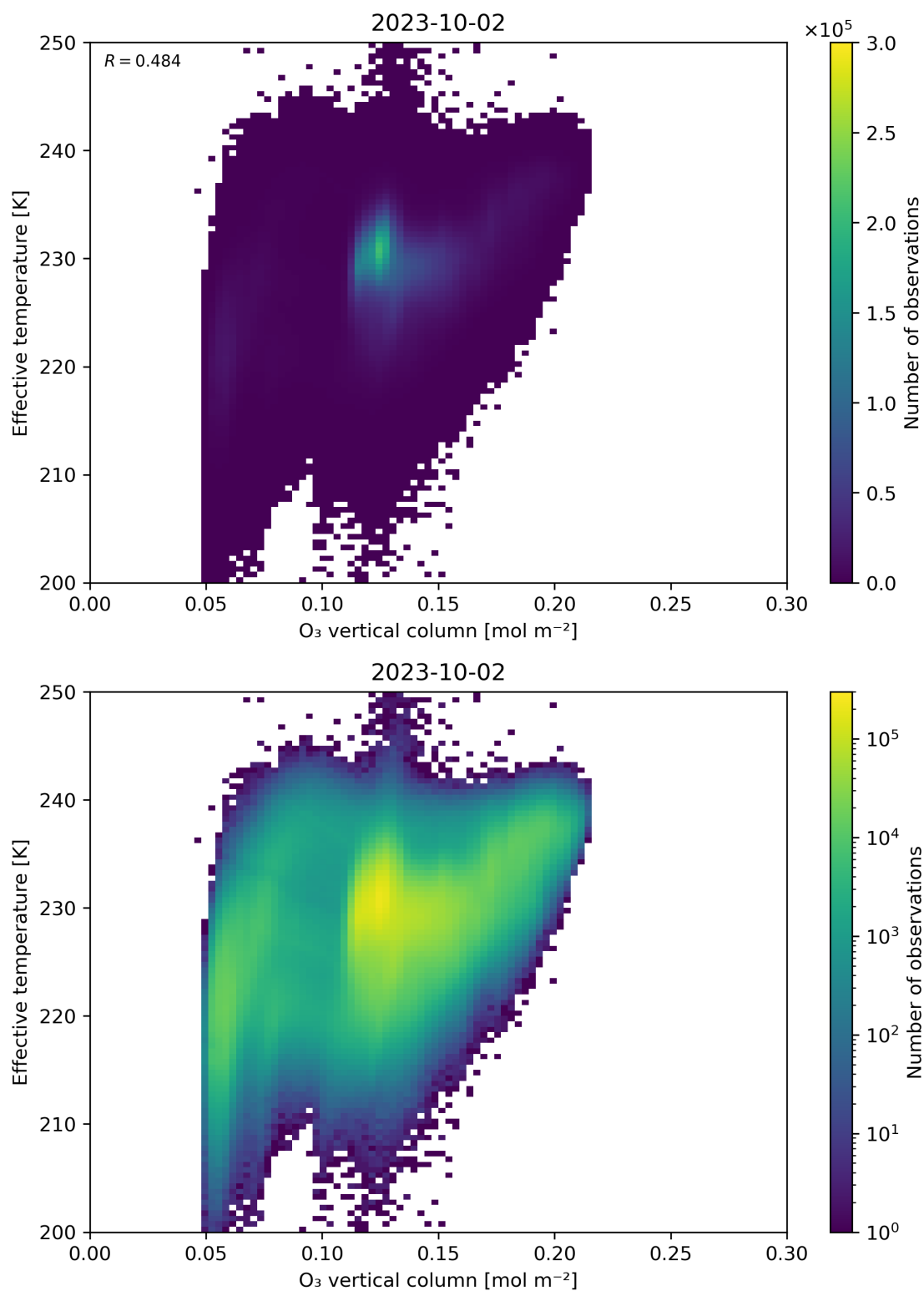
Figure 39: Scatter density plot of “O 3 vertical column” against “Effective temperature” for 2023-10-01 to 2023-10-03.
