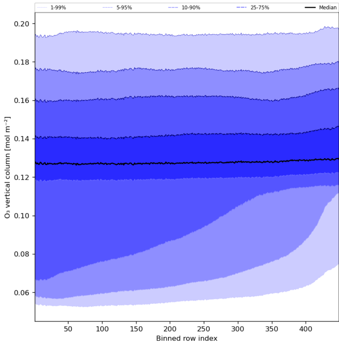
Figure 28: Along track statistics of “O 3 vertical column” for 2023-10-01 to 2023-10-03
