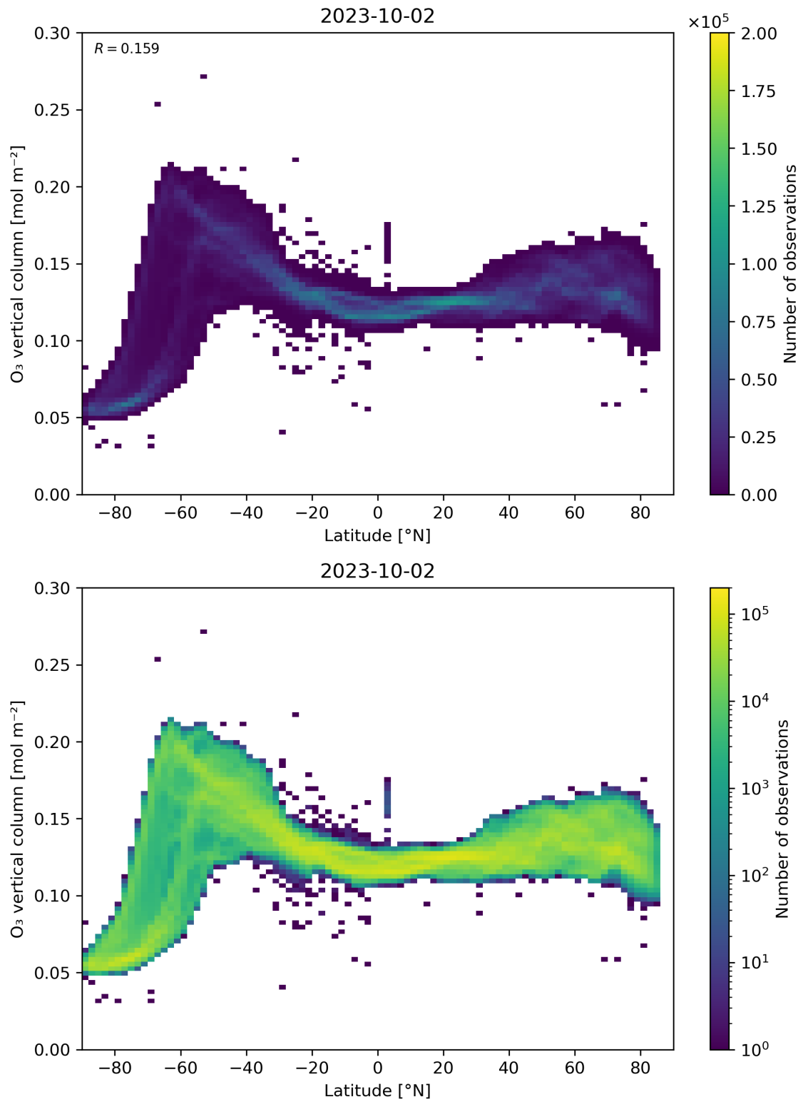
Figure 36: Scatter density plot of “Latitude” against “O 3 vertical column” for 2023-10-01 to 2023-10-03.
