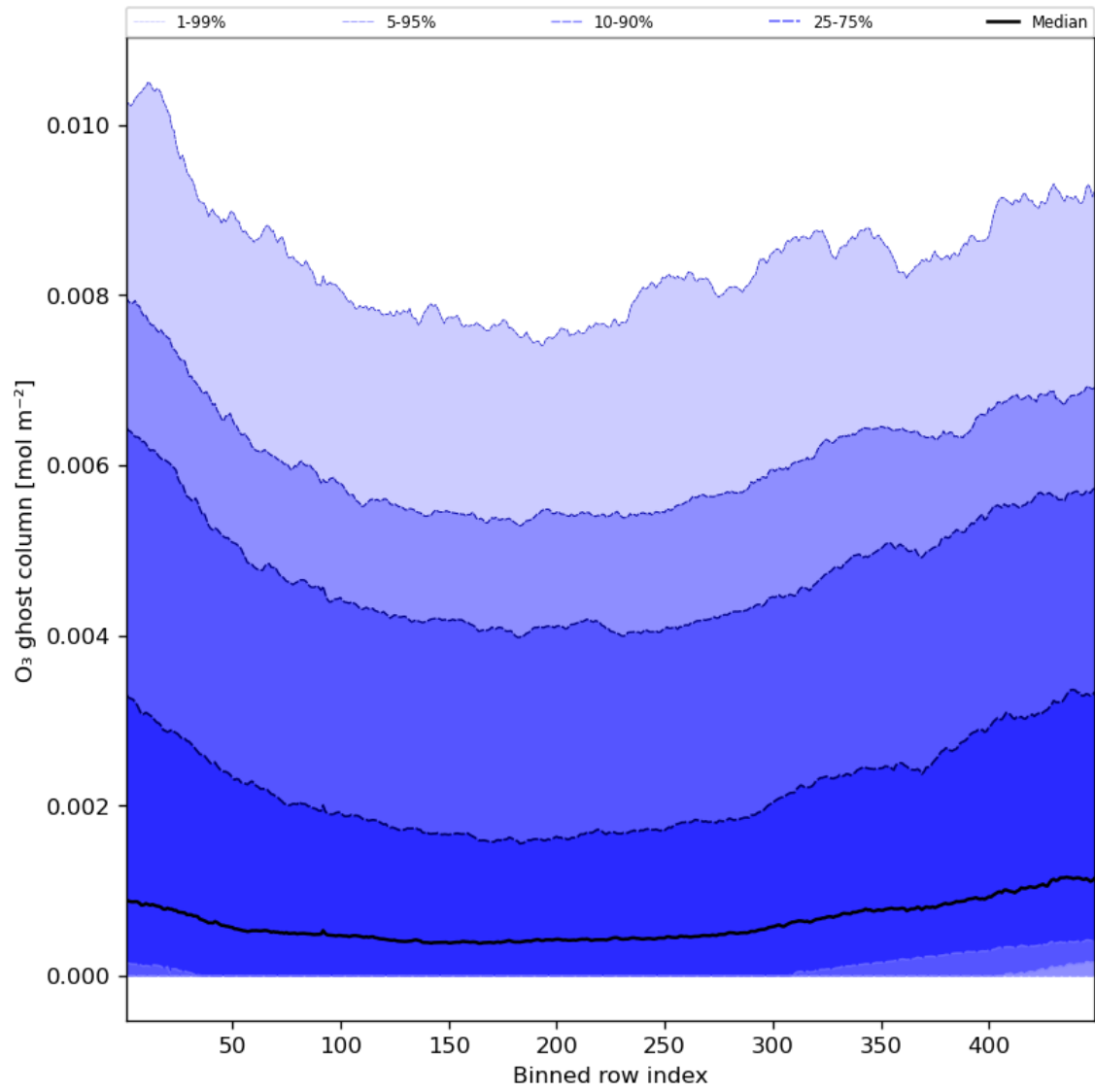
Figure 32: Along track statistics of “O 3 ghost column” for 2023-10-01 to 2023-10-03
