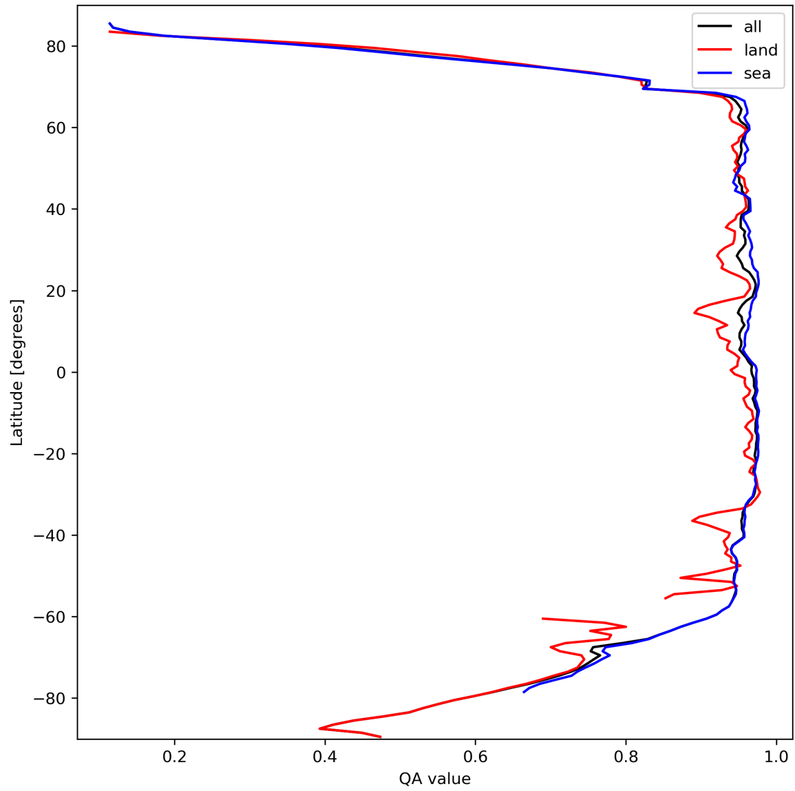
Figure 13: Zonal average of “QA value” for 2023-10-01 to 2023-10-03.
