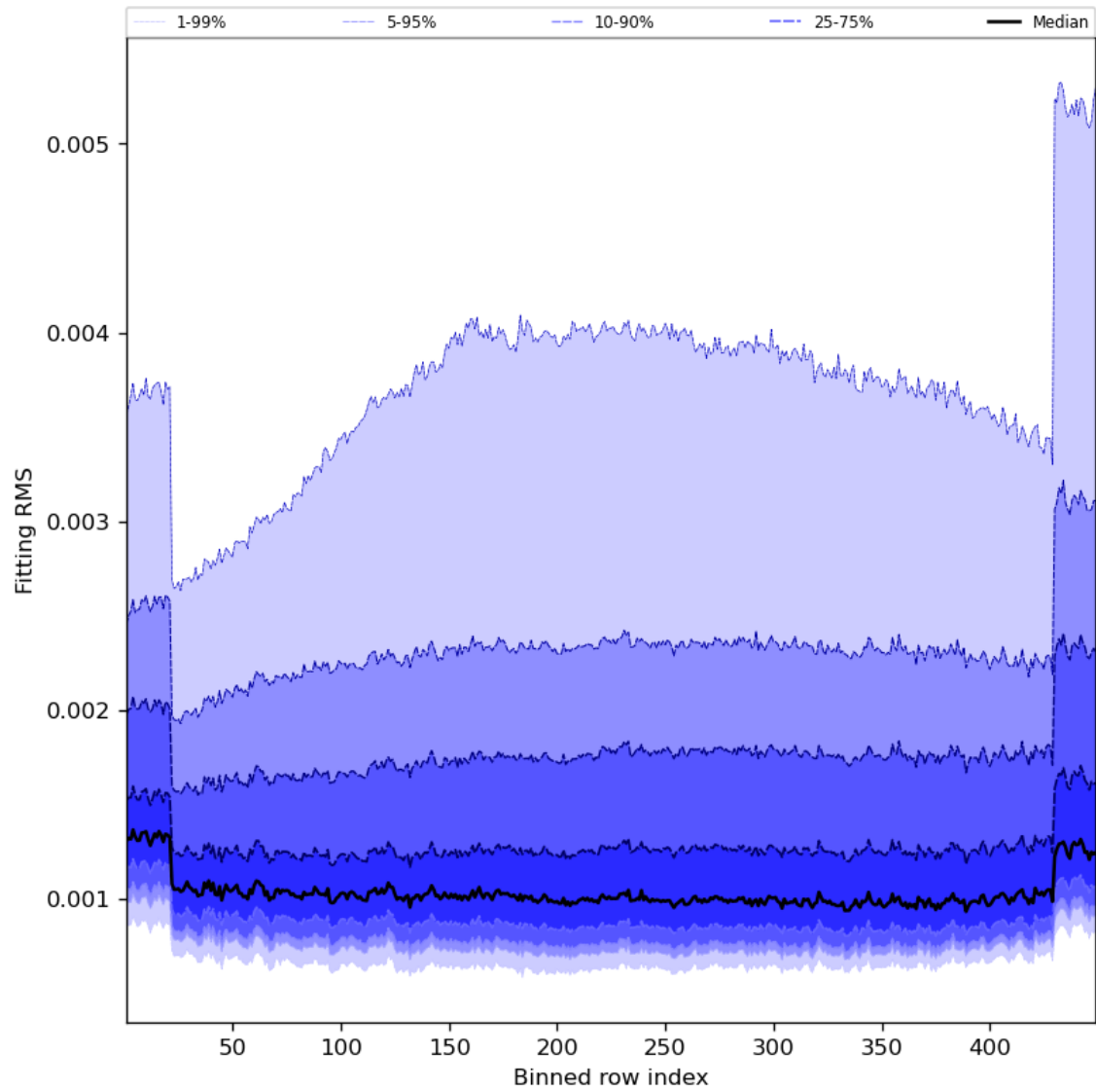
Figure 30: Along track statistics of “Fitting RMS” for 2023-10-01 to 2023-10-03
