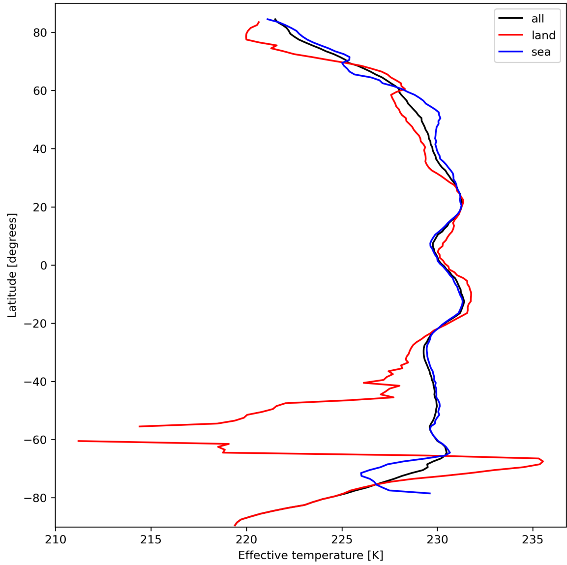
Figure 17: Zonal average of “Effective temperature” for 2023-10-04 to 2023-10-06.
