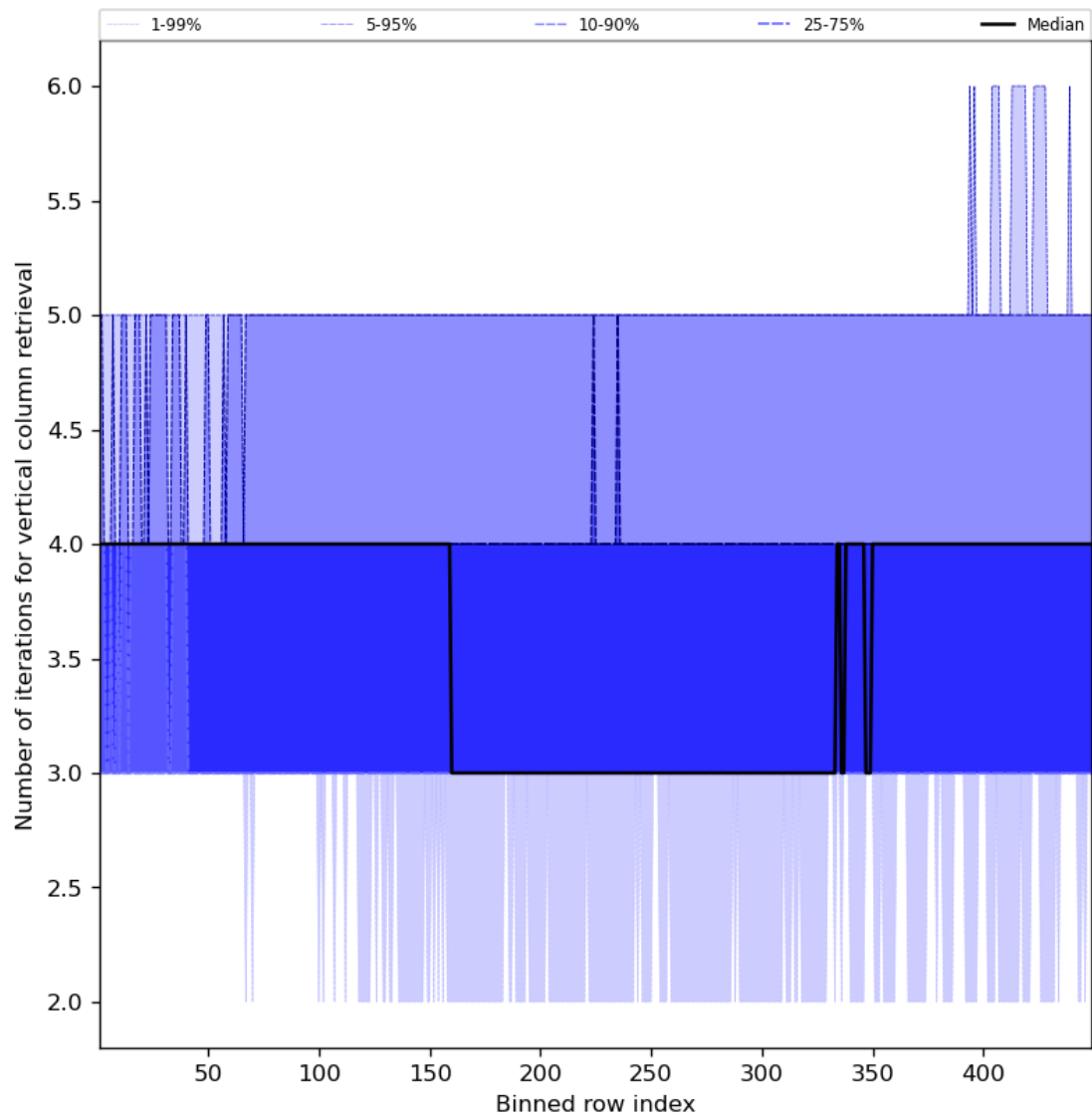
Figure 33: Along track statistics of “Number of iterations for vertical column retrieval” for 2023-10-04 to 2023-10-06
