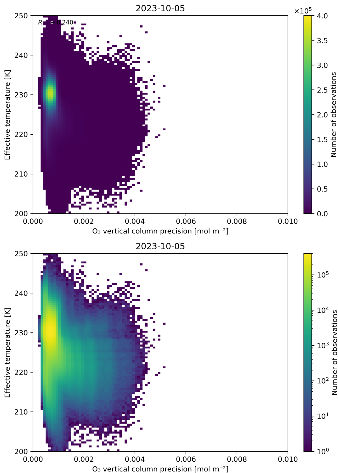
Figure 42: Scatter density plot of “O 3 vertical column precision” against “Effective temperature” for 2023-10-04 to 2023-10-06.
