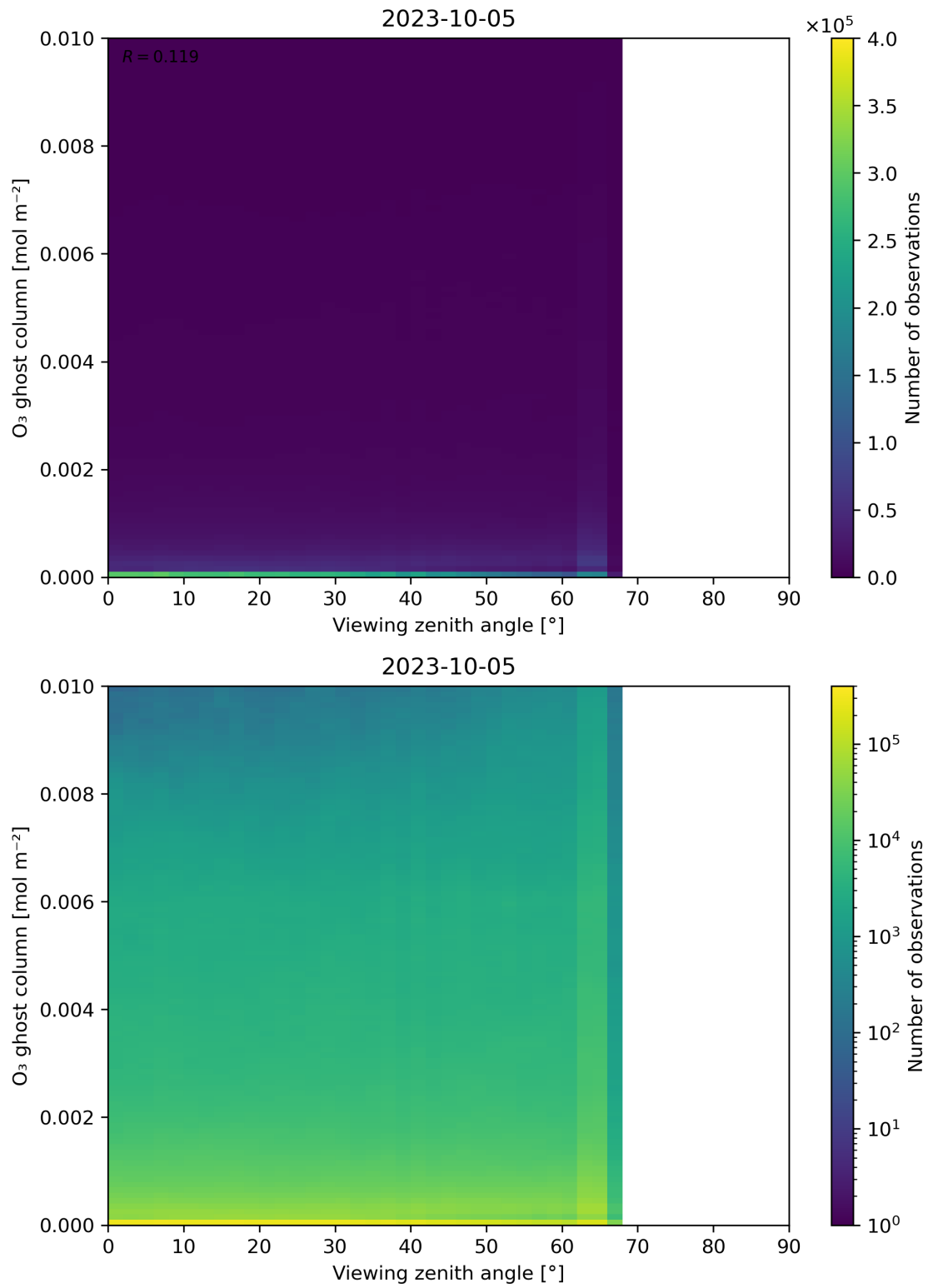
Figure 51: Scatter density plot of “Viewing zenith angle” against “O 3 ghost column” for 2023-10-04 to 2023-10-06.
