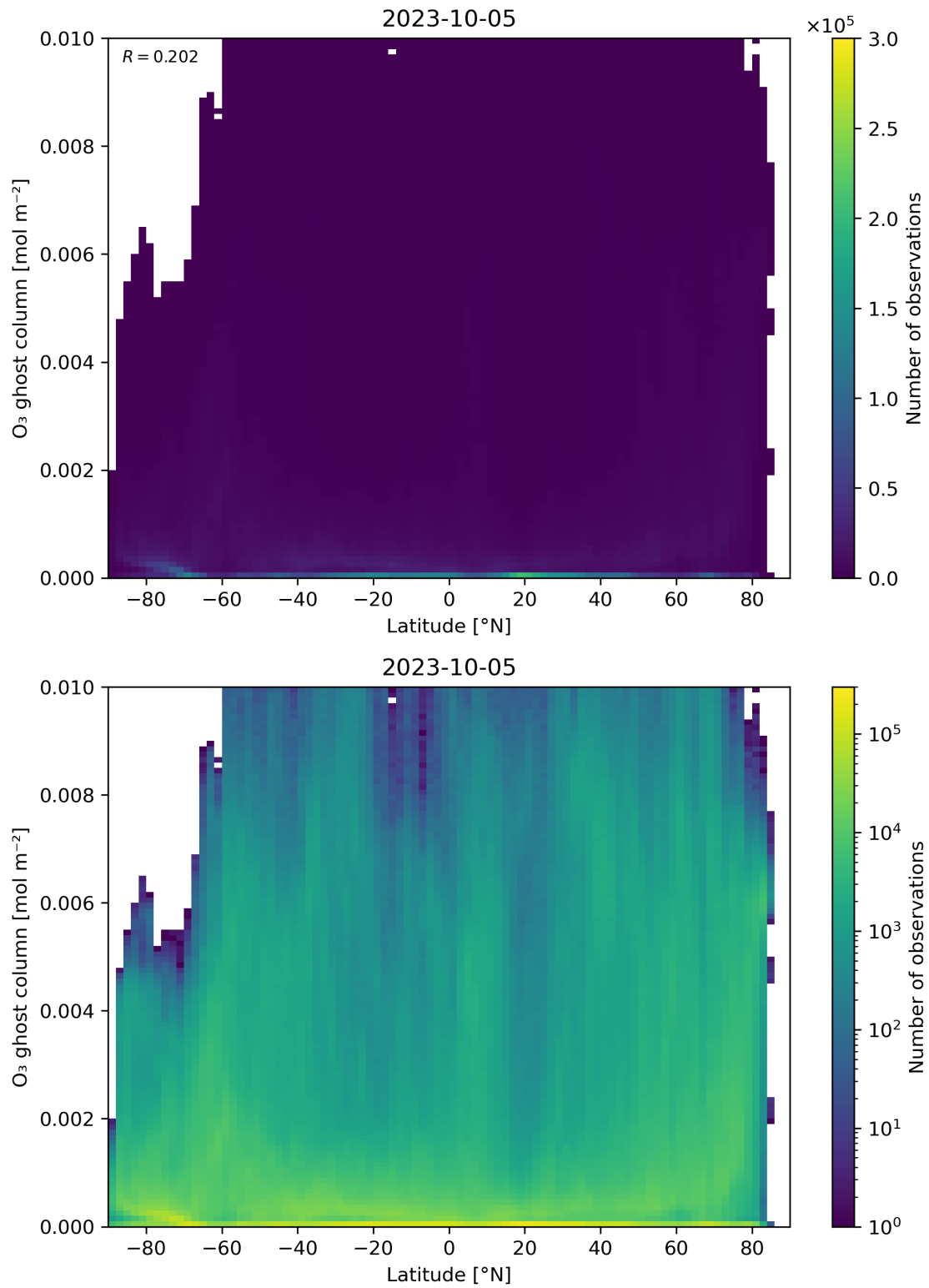
Figure 35: Scatter density plot of “Latitude” against “O 3 ghost column” for 2023-10-04 to 2023-10-06.
