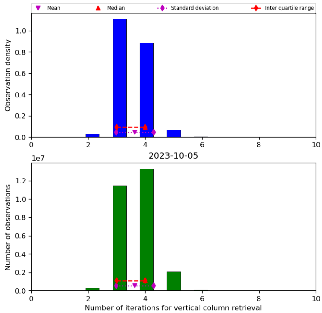
Figure 26: Histogram of “Number of iterations for vertical column retrieval” for 2023-10-04 to 2023-10-06
