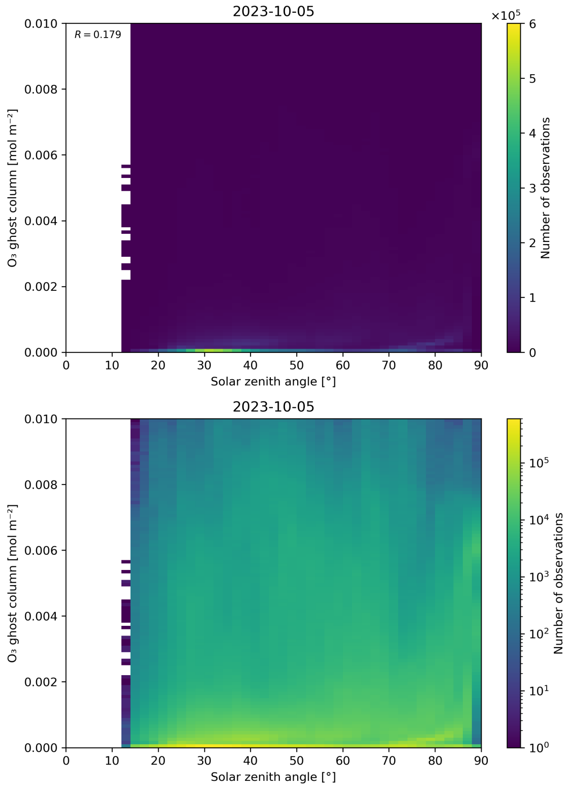
Figure 46: Scatter density plot of “Solar zenith angle” against “O 3 ghost column” for 2023-10-04 to 2023-10-06.
