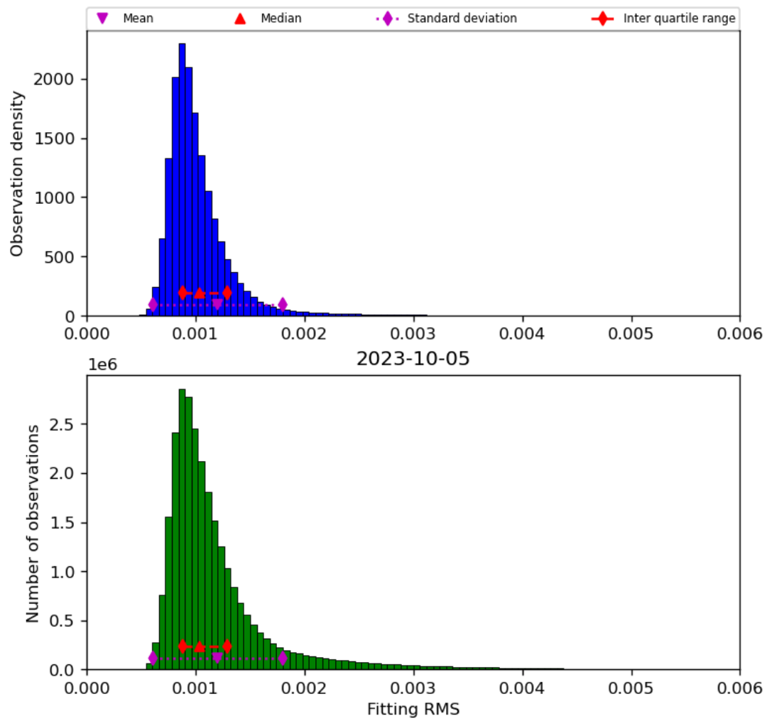
Figure 23: Histogram of “Fitting RMS” for 2023-10-04 to 2023-10-06
