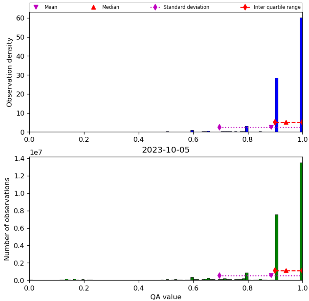
Figure 20: Histogram of “QA value” for 2023-10-04 to 2023-10-06
