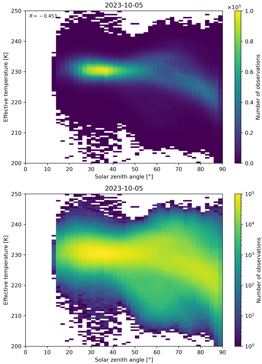
Figure 45: Scatter density plot of “Solar zenith angle” against “Effective temperature” for 2023-10-04 to 2023-10-06.
