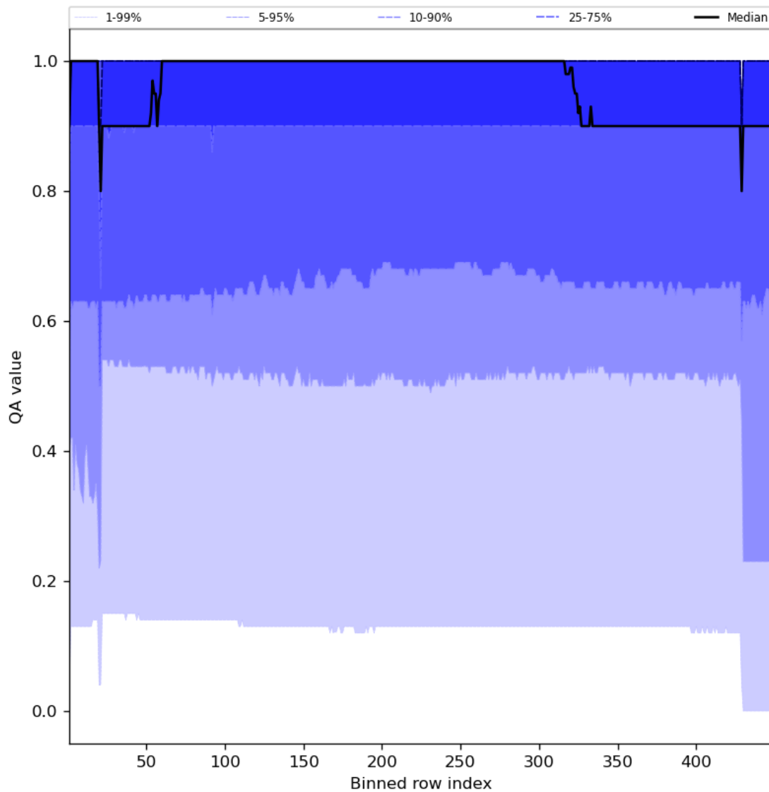
Figure 27: Along track statistics of “QA value” for 2023-10-04 to 2023-10-06
