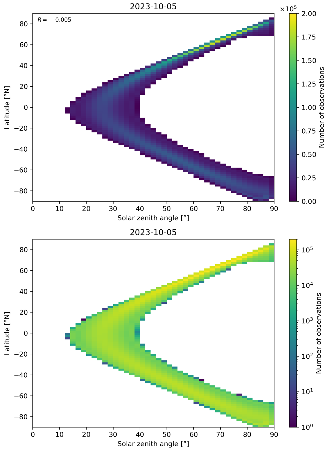
Figure 44: Scatter density plot of “Solar zenith angle” against “Latitude” for 2023-10-04 to 2023-10-06.
