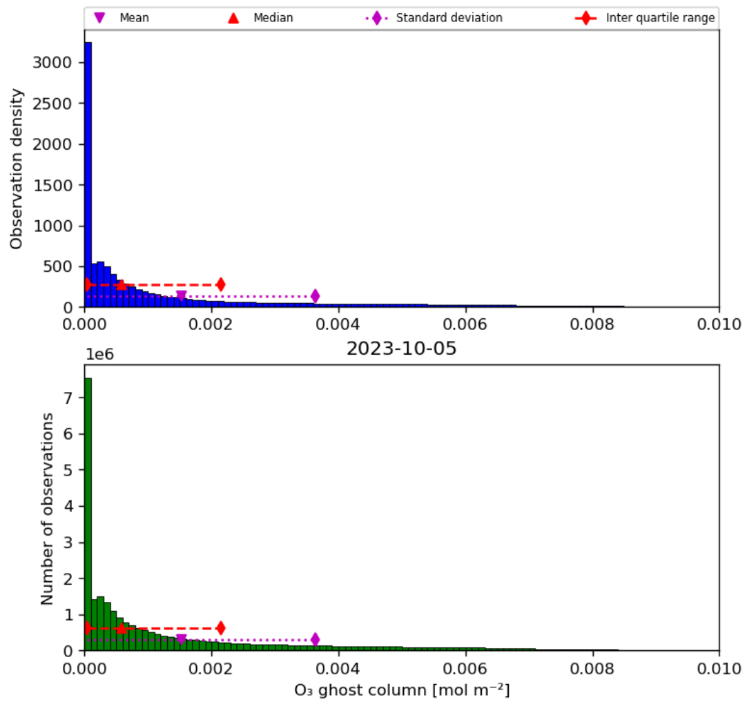
Figure 25: Histogram of “O 3 ghost column” for 2023-10-04 to 2023-10-06
