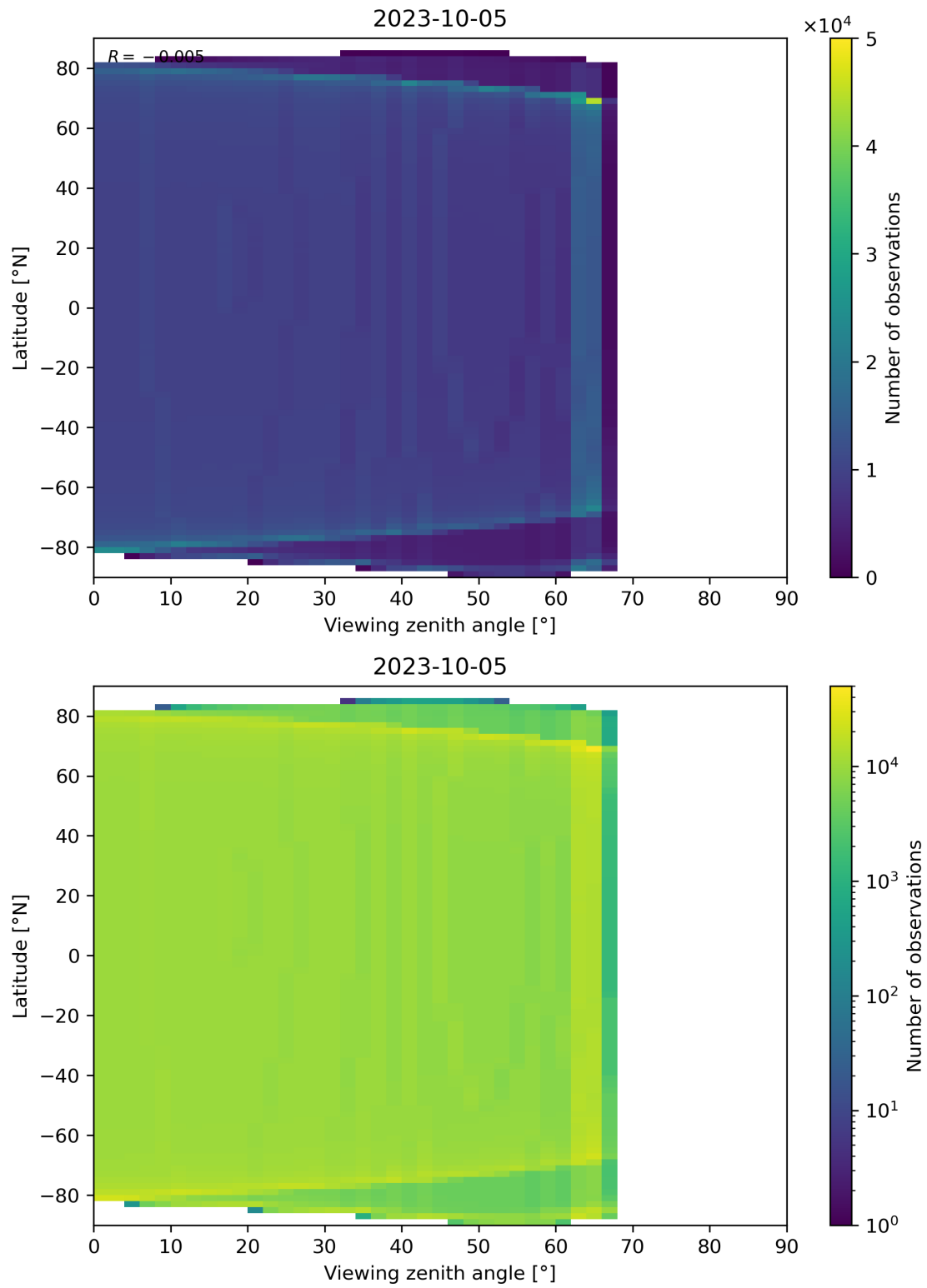
Figure 49: Scatter density plot of “Viewing zenith angle” against “Latitude” for 2023-10-04 to 2023-10-06.
