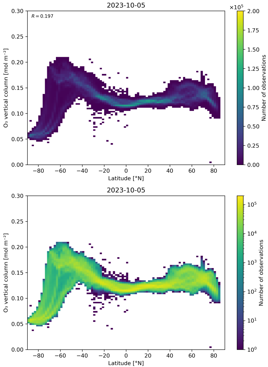
Figure 36: Scatter density plot of “Latitude” against “O 3 vertical column” for 2023-10-04 to 2023-10-06.
