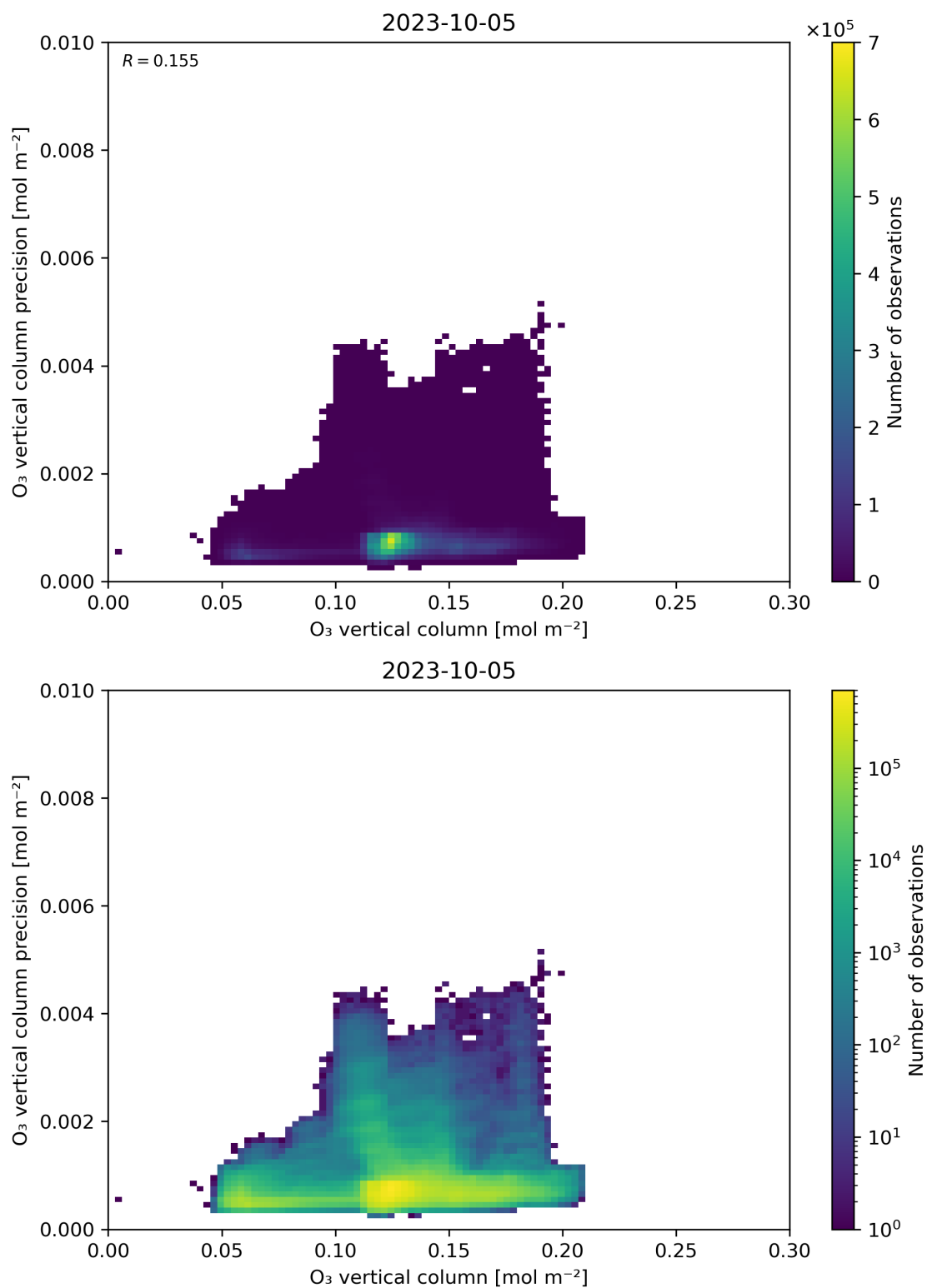
Figure 41: Scatter density plot of “O 3 vertical column” against “O 3 vertical column precision” for 2023-10-04 to 2023-10-06.
