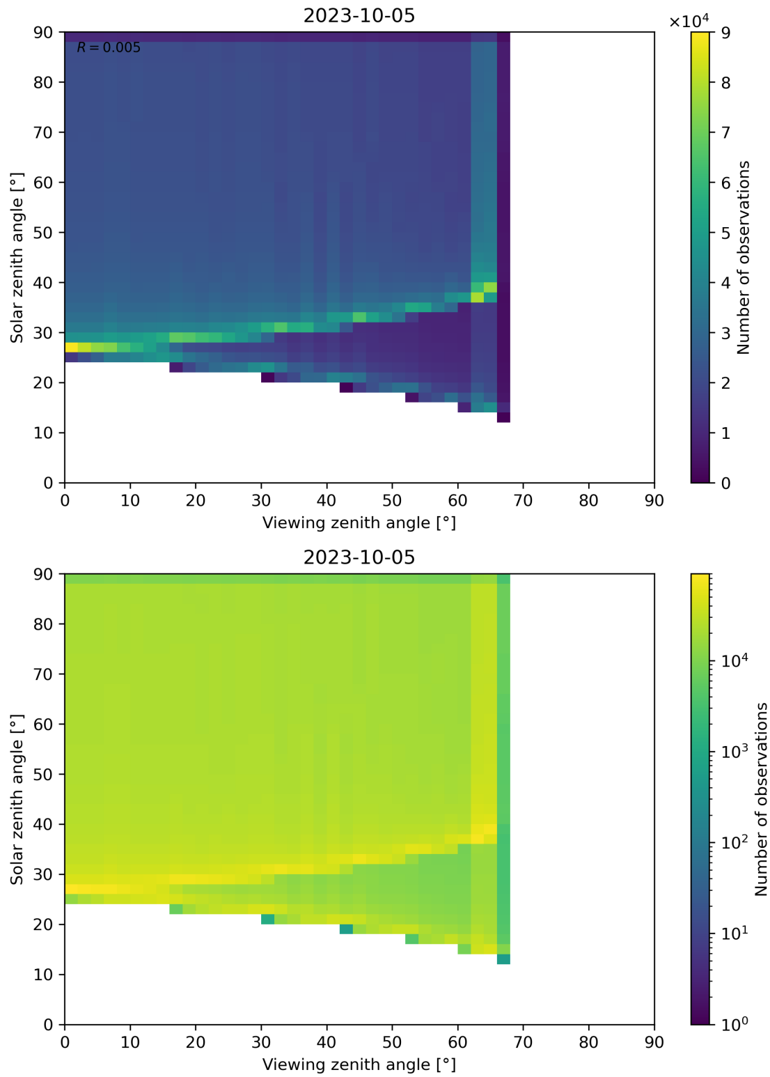
Figure 54: Scatter density plot of “Viewing zenith angle” against “Solar zenith angle” for 2023-10-04 to 2023-10-06.
