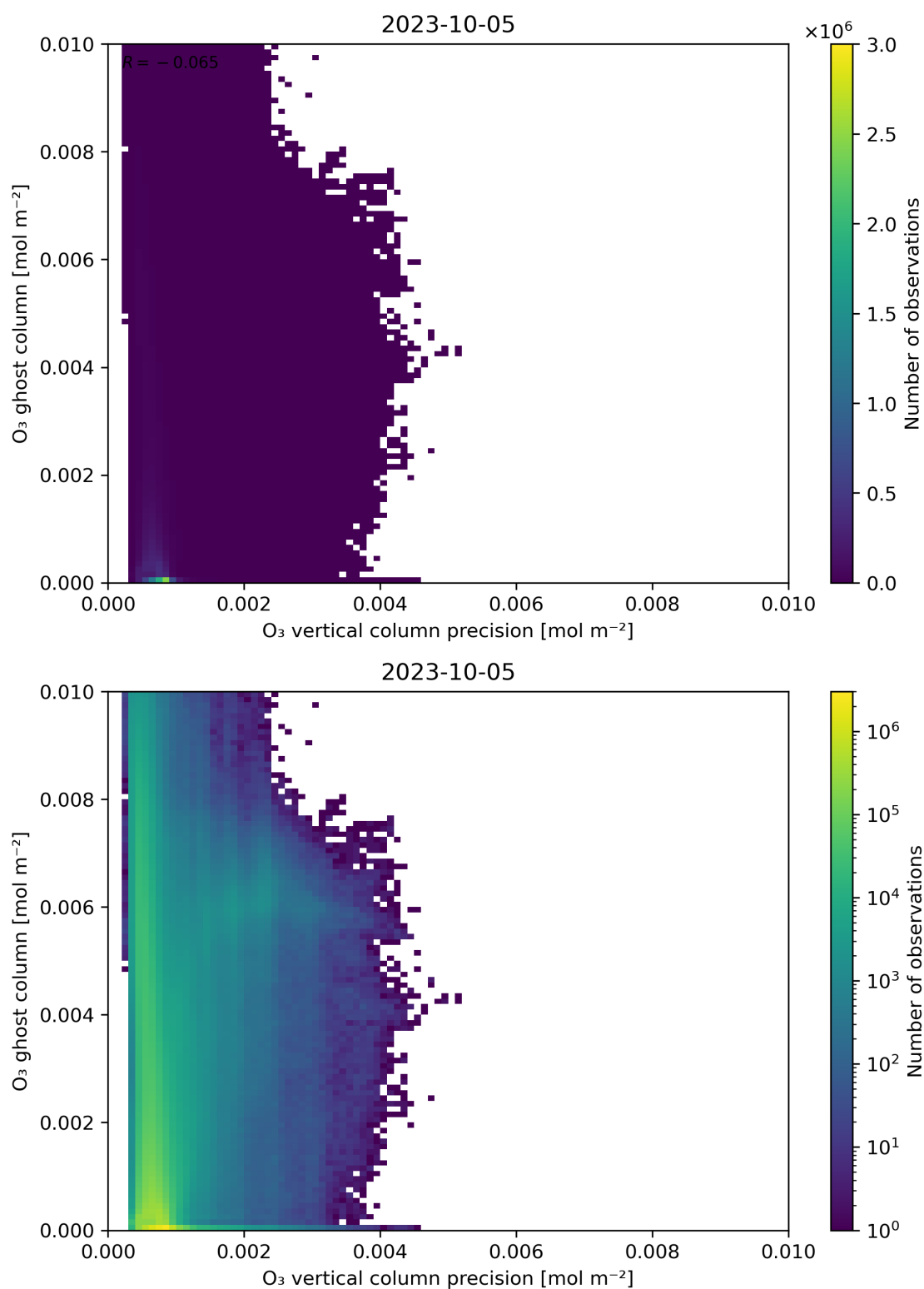
Figure 43: Scatter density plot of “ \text{O}_3 vertical column precision” against “ \text{O}_3 ghost column” for 2023-10-04 to 2023-10-06.
