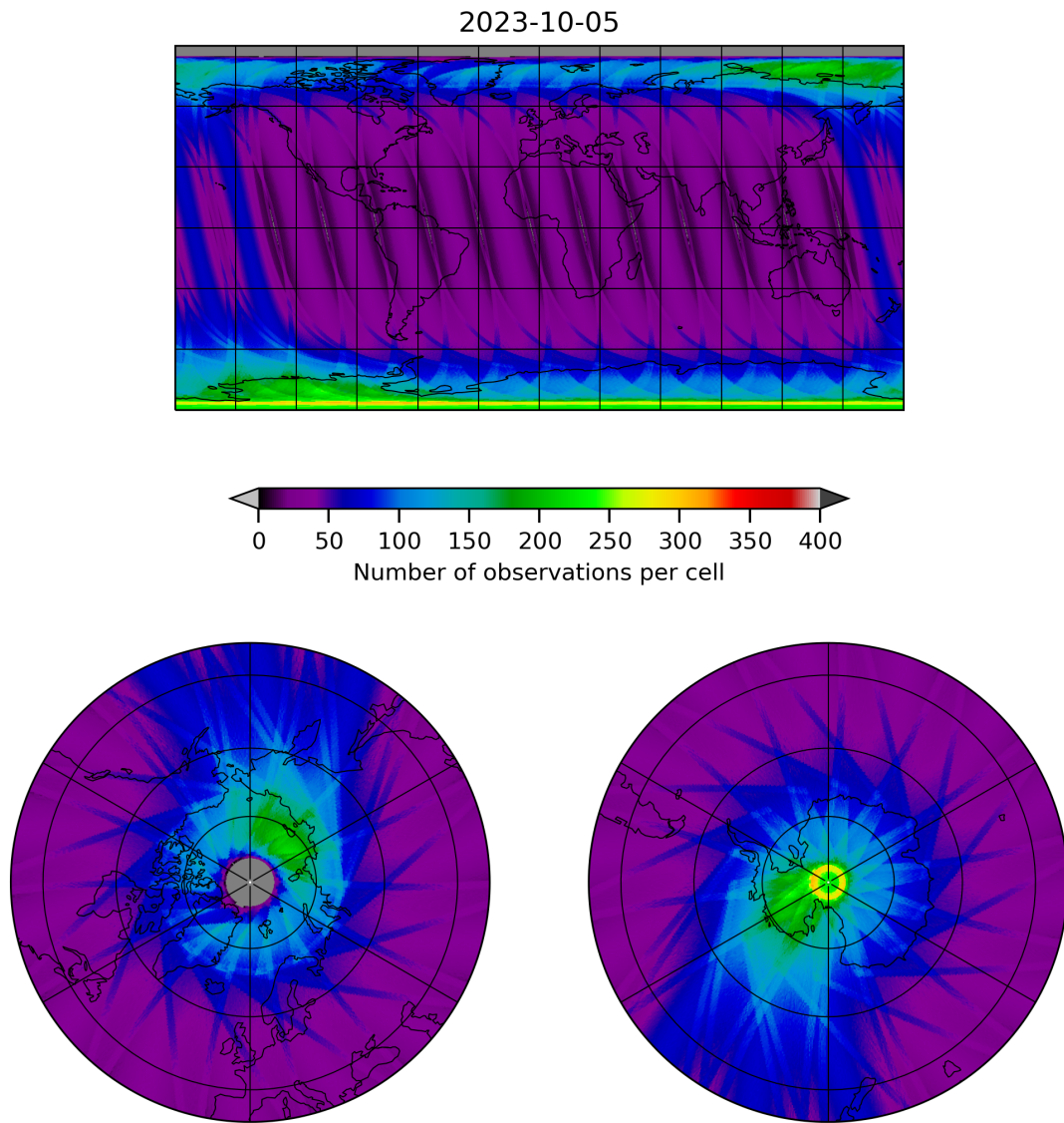
Figure 12: Map of the number of observations for 2023-10-04 to 2023-10-06
