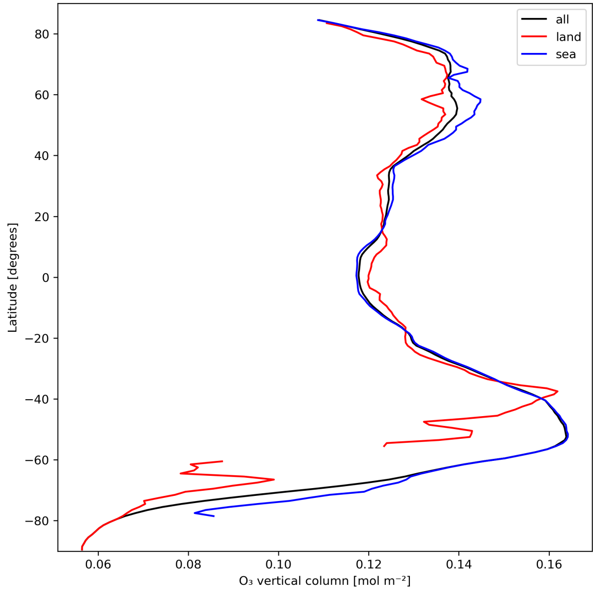
Figure 14: Zonal average of “O 3 vertical column” for 2023-10-04 to 2023-10-06.
