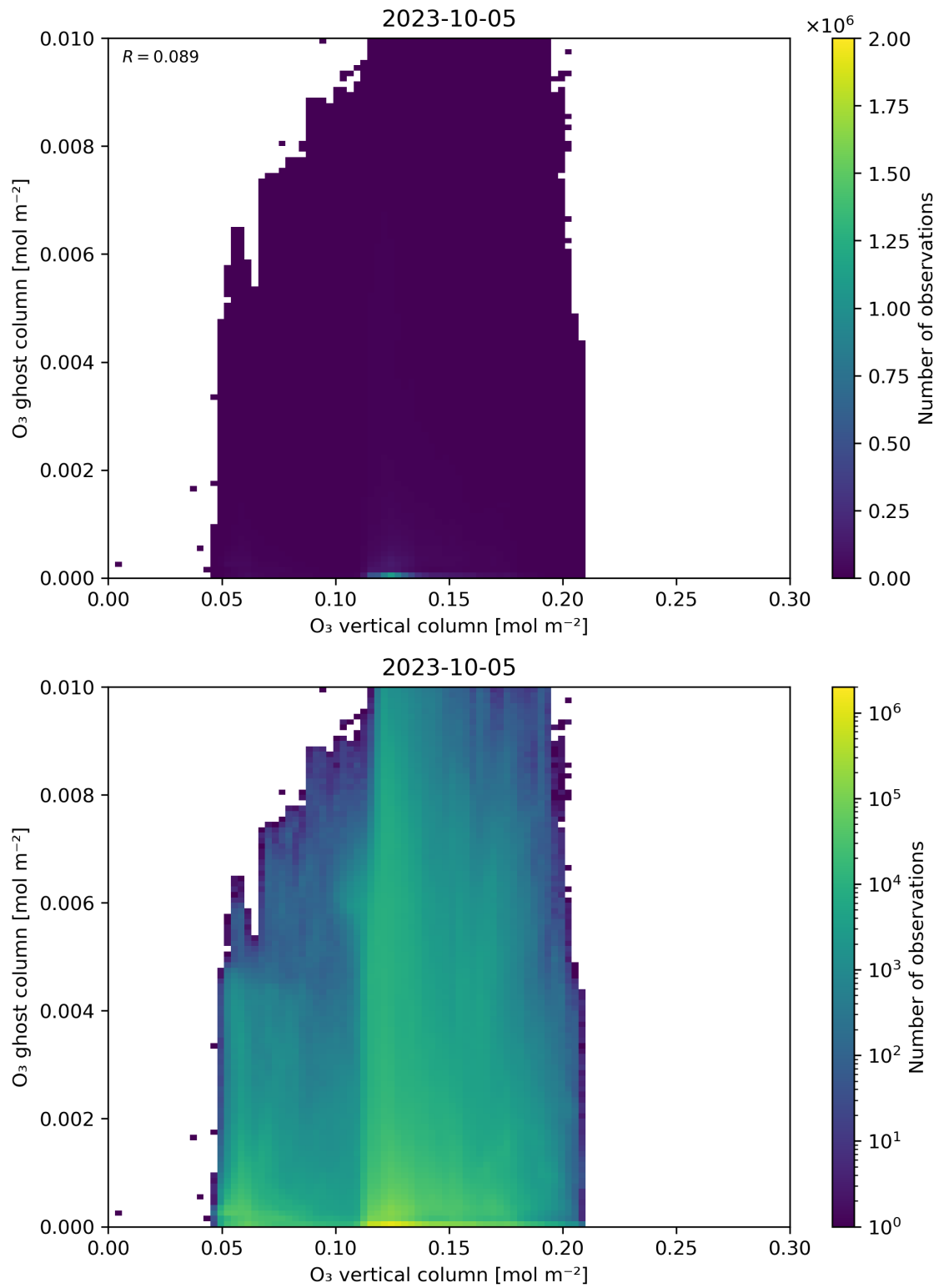
Figure 40: Scatter density plot of “O 3 vertical column” against “O 3 ghost column” for 2023-10-04 to 2023-10-06.
