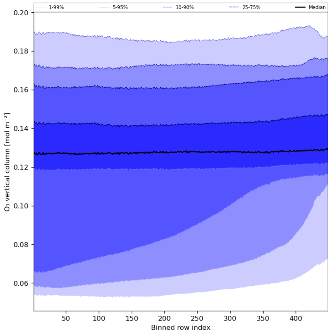
Figure 28: Along track statistics of “O 3 vertical column” for 2023-10-04 to 2023-10-06
