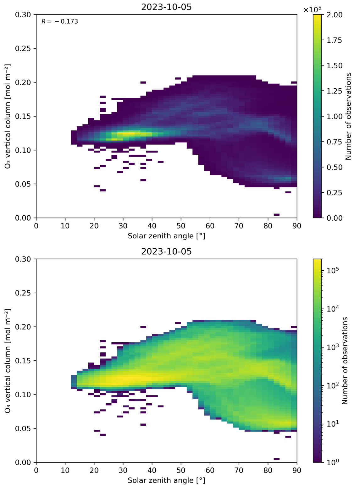
Figure 47: Scatter density plot of “Solar zenith angle” against “O 3 vertical column” for 2023-10-04 to 2023-10-06.
