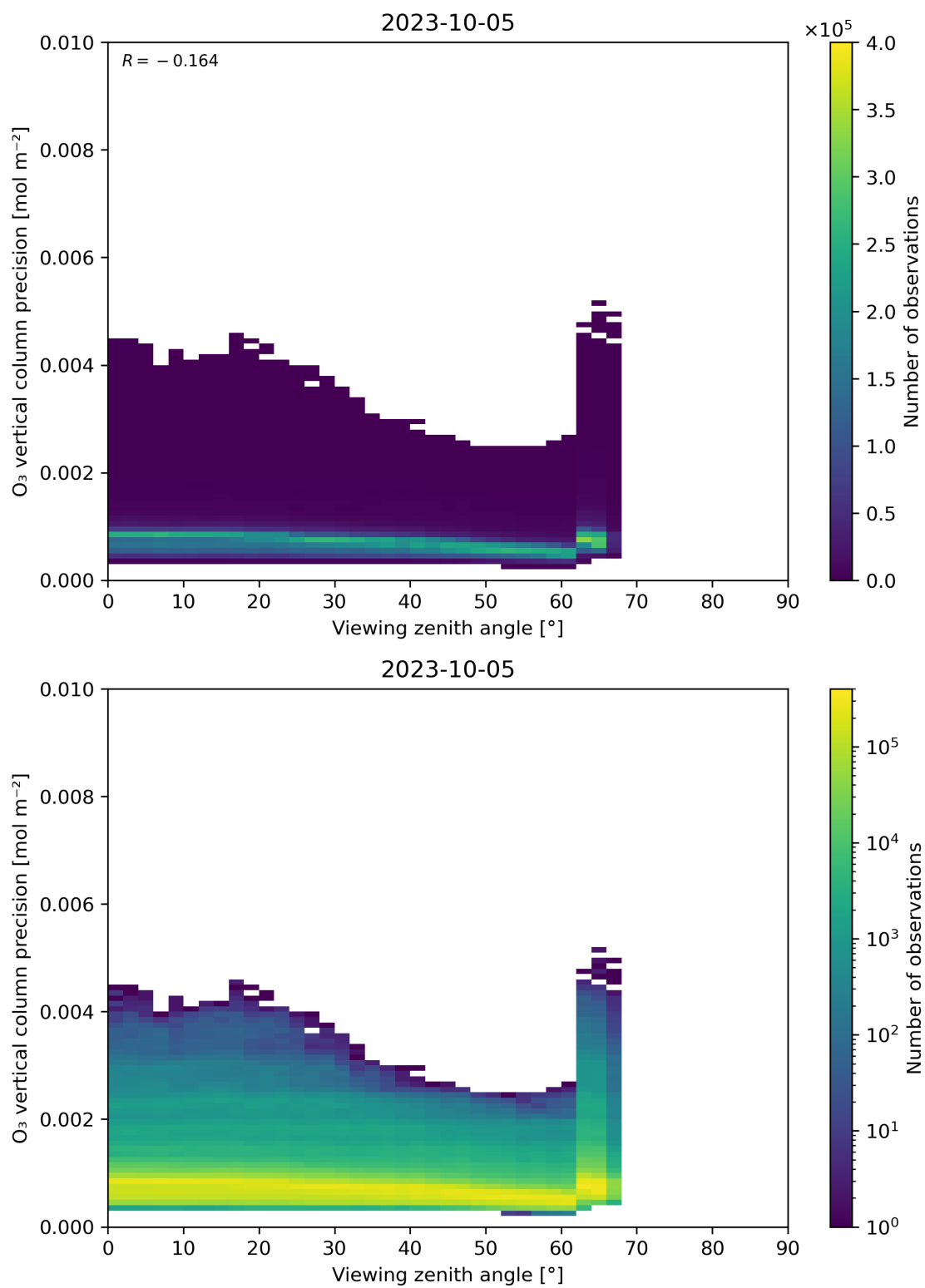
Figure 53: Scatter density plot of “Viewing zenith angle” against “O 3 vertical column precision” for 2023-10-04 to 2023-10-06.
