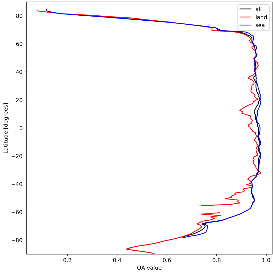
Figure 13: Zonal average of “QA value” for 2023-10-04 to 2023-10-06.
