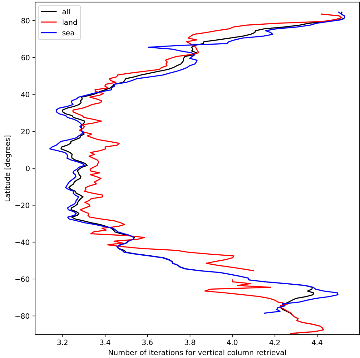
Figure 19: Zonal average of “Number of iterations for vertical column retrieval” for 2023-10-04 to 2023-10-06.
