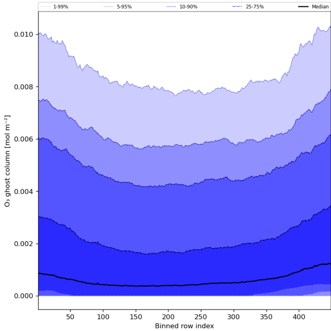
Figure 32: Along track statistics of “O 3 ghost column” for 2023-10-04 to 2023-10-06
