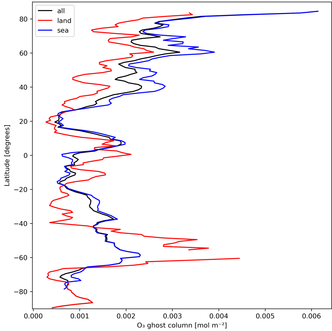
Figure 18: Zonal average of “O 3 ghost column” for 2023-10-04 to 2023-10-06.
