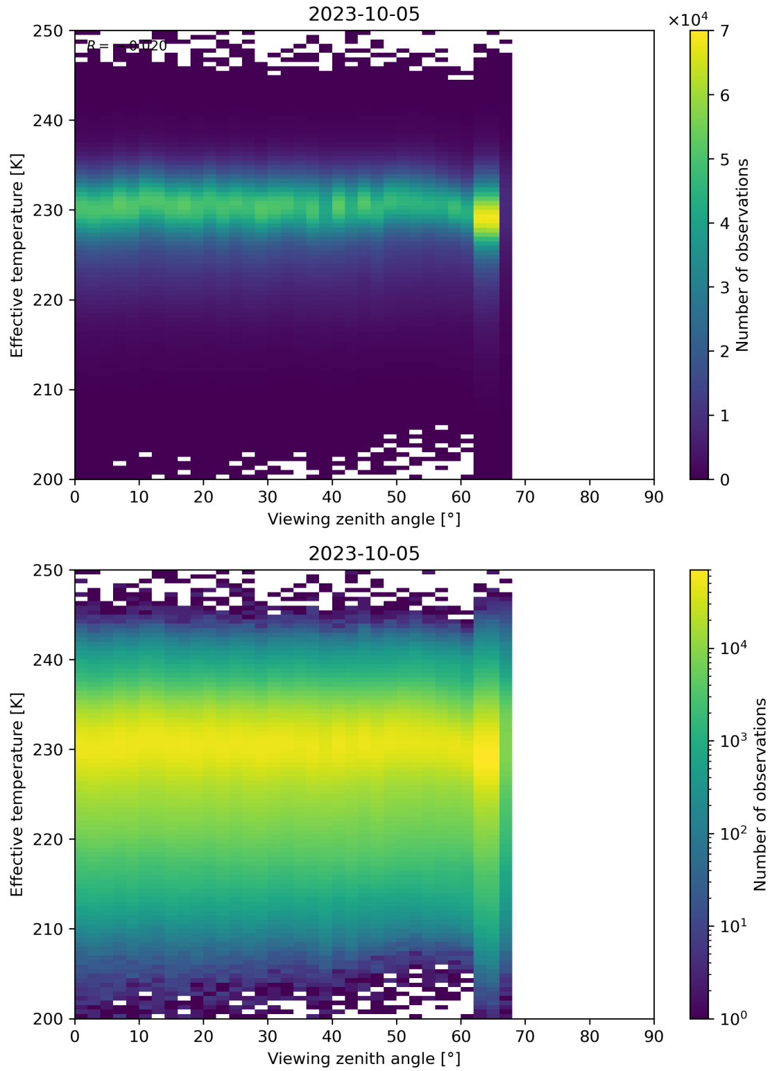
Figure 50: Scatter density plot of “Viewing zenith angle” against “Effective temperature” for 2023-10-04 to 2023-10-06.
