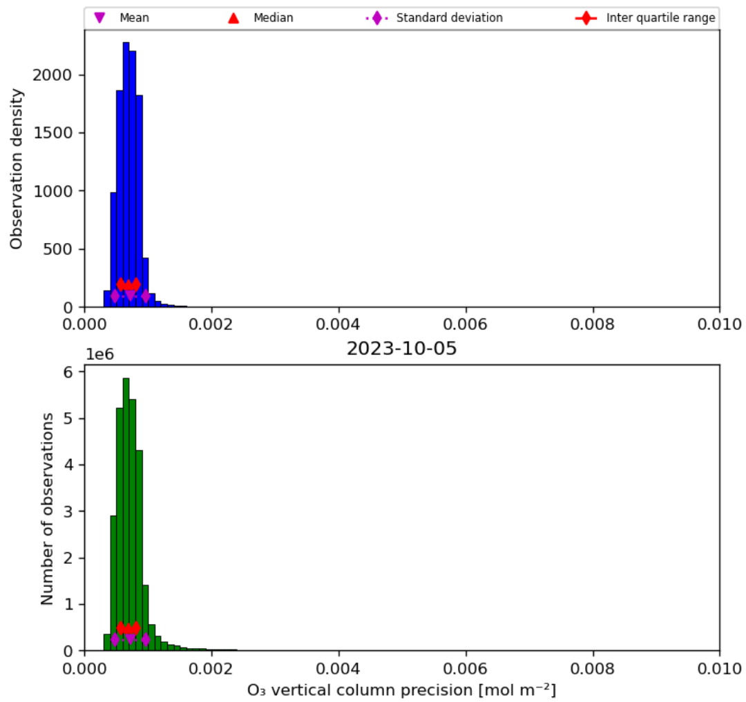
Figure 22: Histogram of “O 3 vertical column precision” for 2023-10-04 to 2023-10-06
