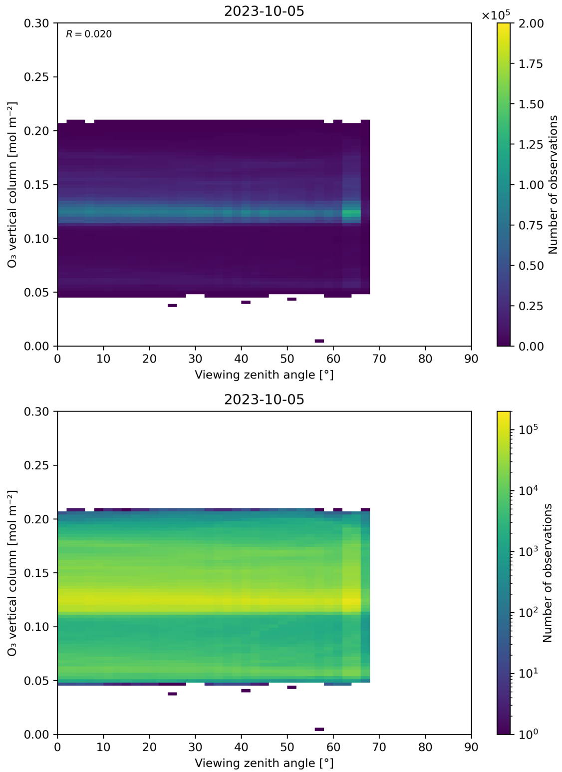
Figure 52: Scatter density plot of “Viewing zenith angle” against “O 3 vertical column” for 2023-10-04 to 2023-10-06.
