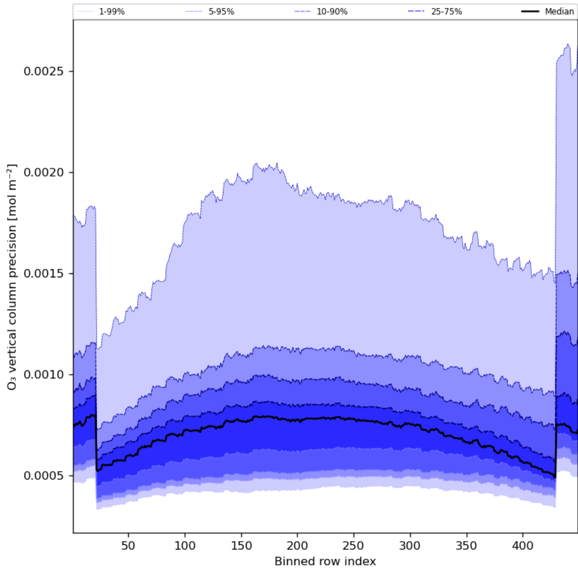
Figure 29: Along track statistics of “O 3 vertical column precision” for 2023-10-04 to 2023-10-06
