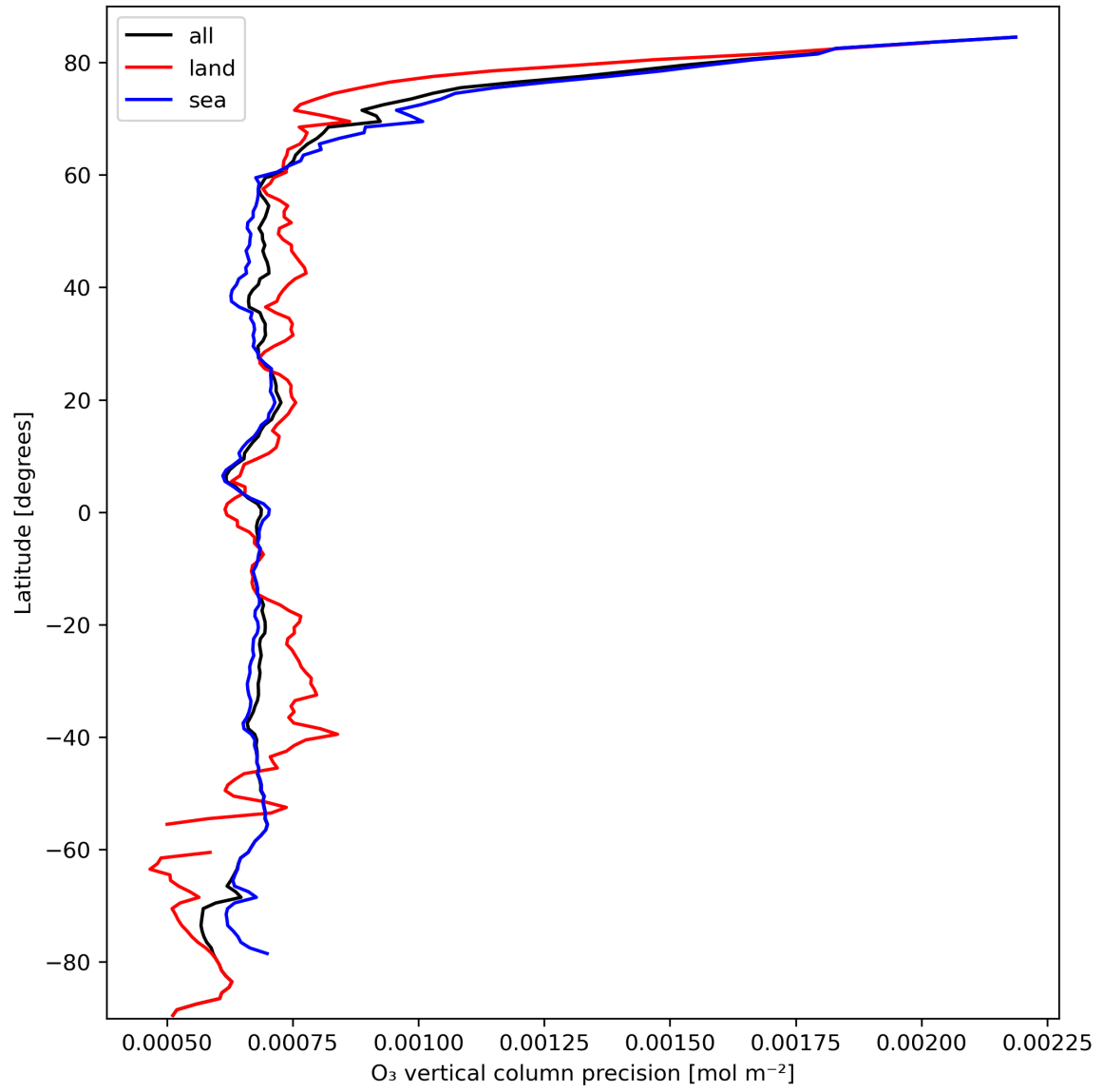
Figure 15: Zonal average of “O 3 vertical column precision” for 2023-10-04 to 2023-10-06.
