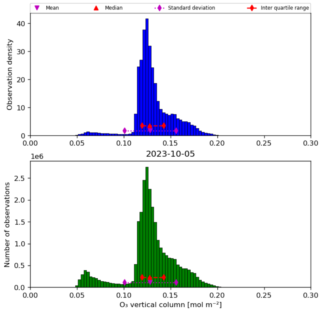
Figure 21: Histogram of “O 3 vertical column” for 2023-10-04 to 2023-10-06
