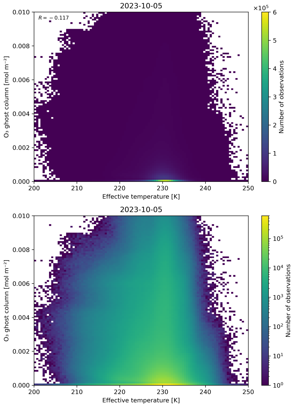
Figure 38: Scatter density plot of “Effective temperature” against “O 3 ghost column” for 2023-10-04 to 2023-10-06.
