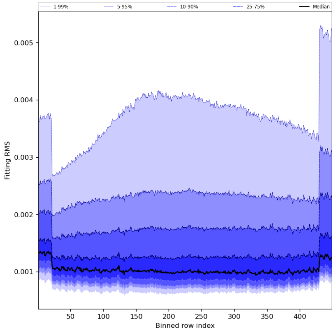
Figure 30: Along track statistics of “Fitting RMS” for 2023-10-04 to 2023-10-06
