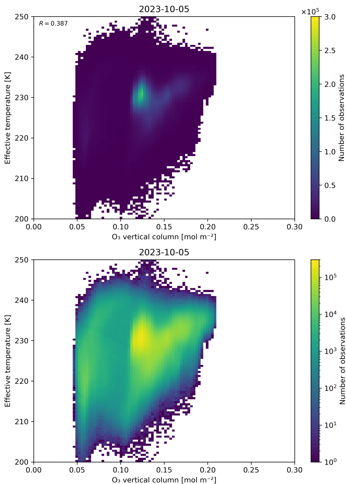
Figure 39: Scatter density plot of “O 3 vertical column” against “Effective temperature” for 2023-10-04 to 2023-10-06.
