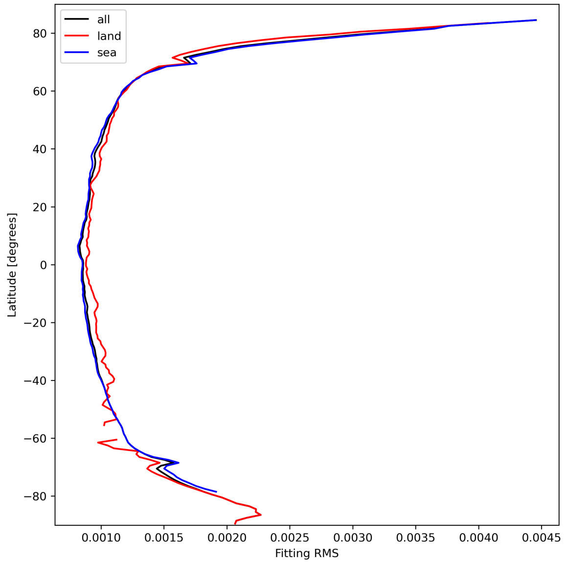
Figure 16: Zonal average of “Fitting RMS” for 2023-10-04 to 2023-10-06.
