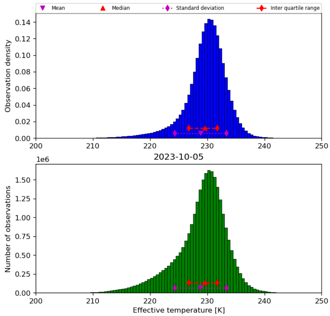
Figure 24: Histogram of “Effective temperature” for 2023-10-04 to 2023-10-06
