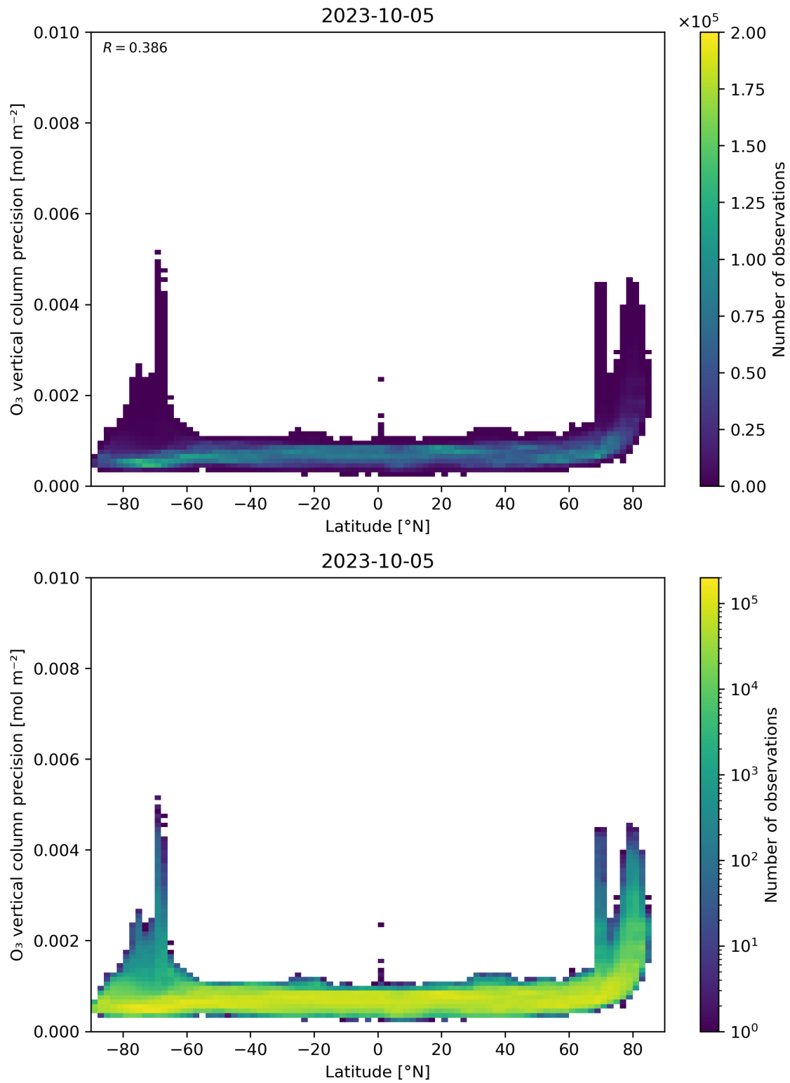
Figure 37: Scatter density plot of “Latitude” against “O 3 vertical column precision” for 2023-10-04 to 2023-10-06.
