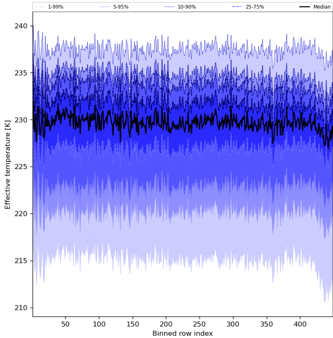
Figure 31: Along track statistics of “Effective temperature” for 2023-10-04 to 2023-10-06
