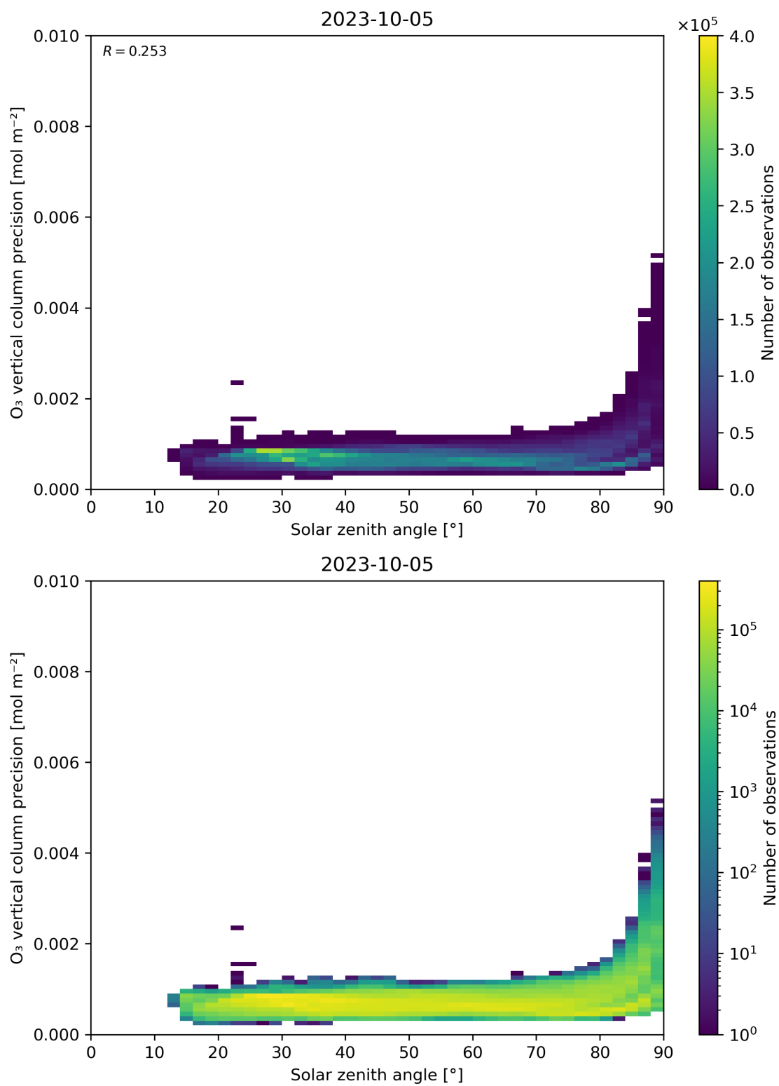
Figure 48: Scatter density plot of “Solar zenith angle” against “O 3 vertical column precision” for 2023-10-04 to 2023-10-06.
