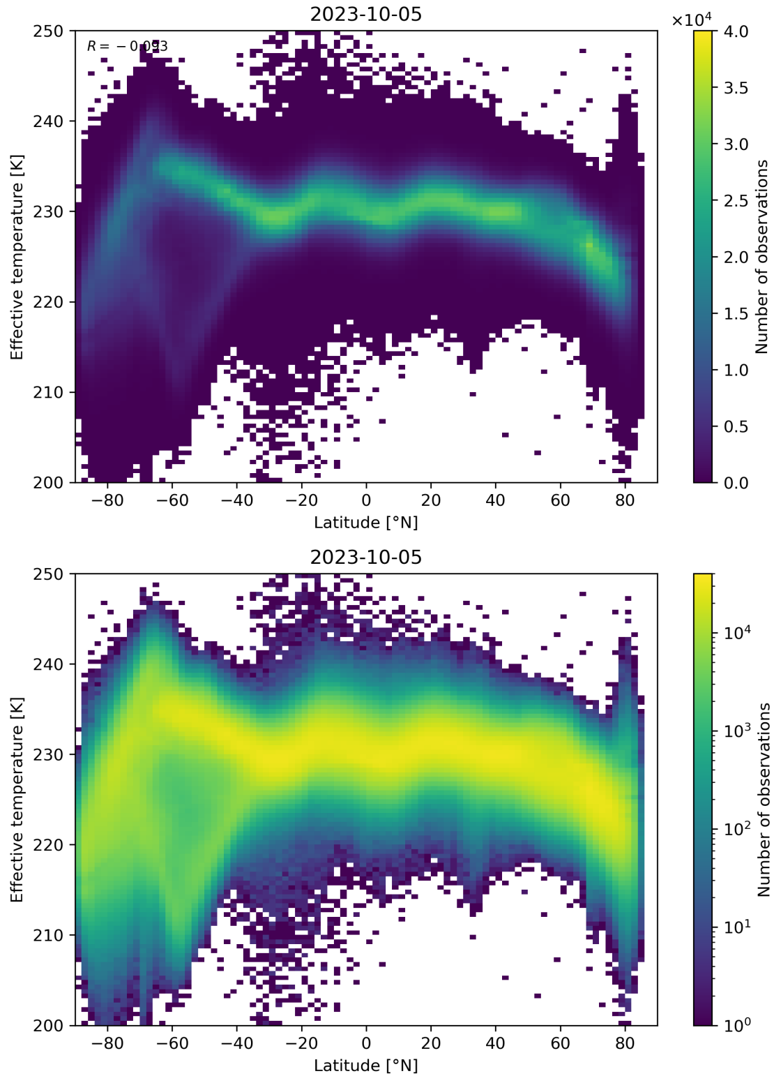
Figure 34: Scatter density plot of “Latitude” against “Effective temperature” for 2023-10-04 to 2023-10-06.
