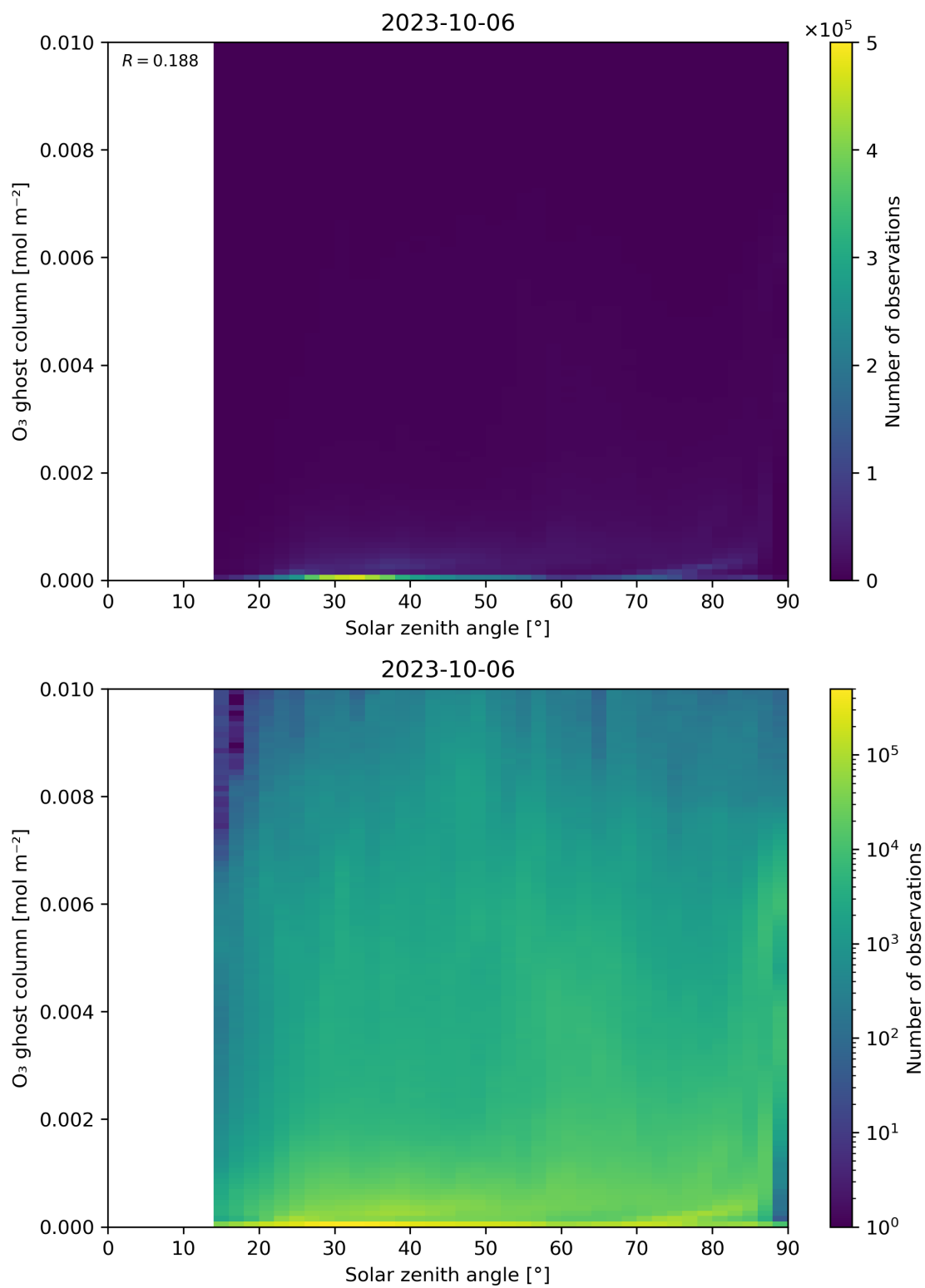
Figure 46: Scatter density plot of “Solar zenith angle” against “O 3 ghost column” for 2023-10-06 to 2023-10-07.
