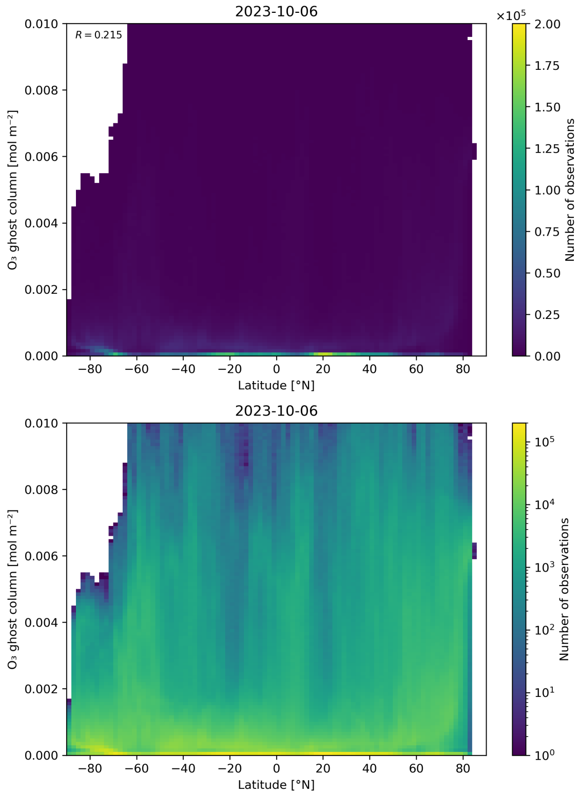
Figure 35: Scatter density plot of “Latitude” against “O 3 ghost column” for 2023-10-06 to 2023-10-07.
