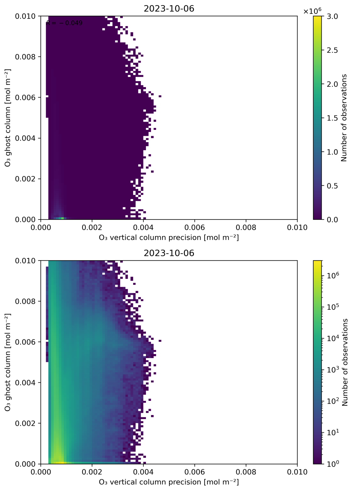
Figure 43: Scatter density plot of “ \text{O}_3 vertical column precision” against “ \text{O}_3 ghost column” for 2023-10-06 to 2023-10-07.
