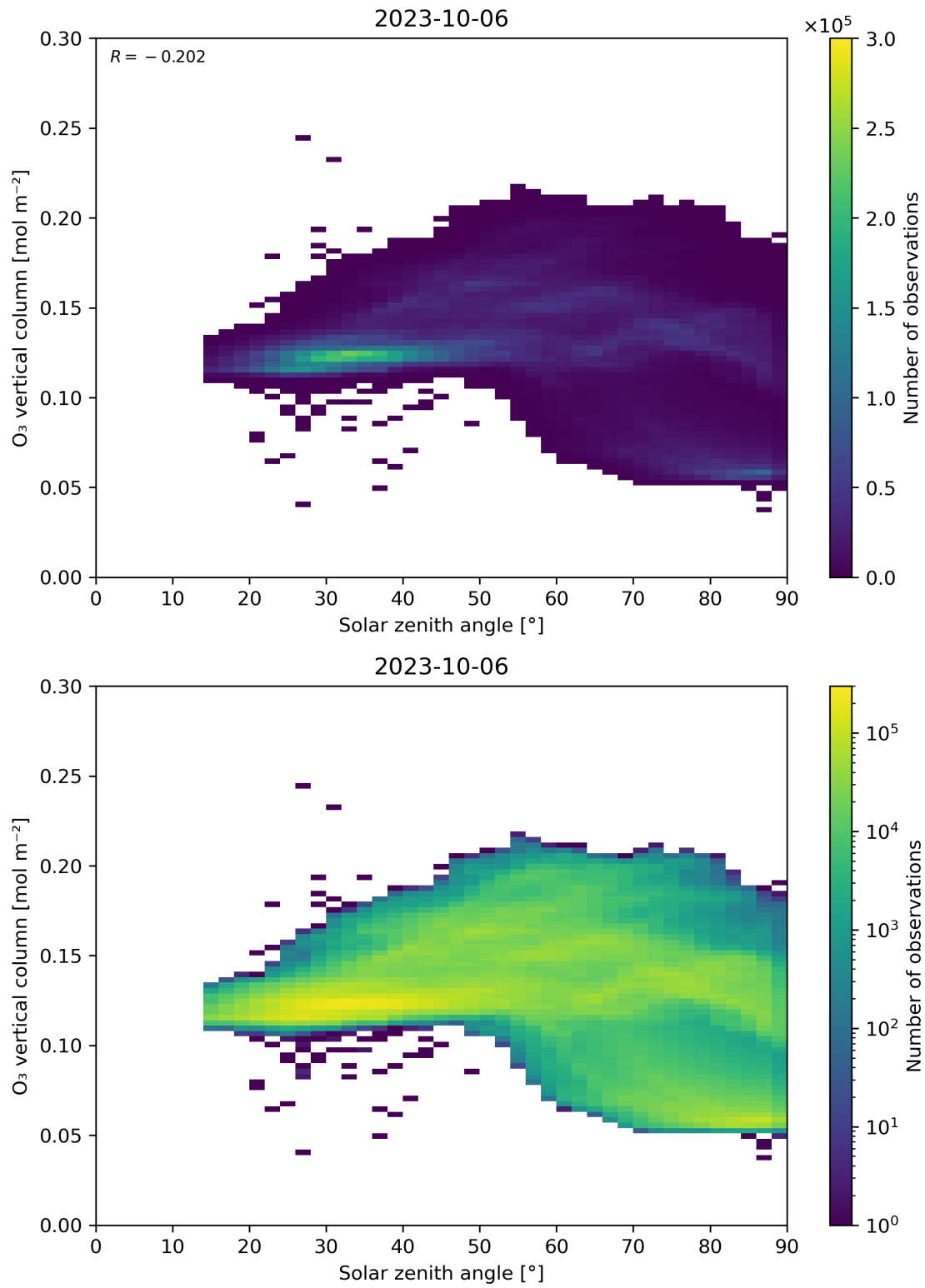
Figure 47: Scatter density plot of “Solar zenith angle” against “O 3 vertical column” for 2023-10-06 to 2023-10-07.
