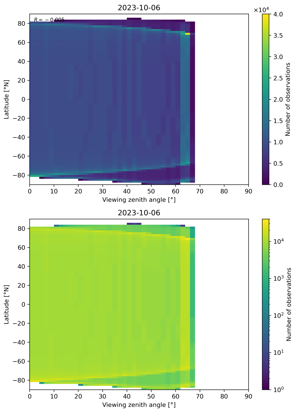
Figure 49: Scatter density plot of “Viewing zenith angle” against “Latitude” for 2023-10-06 to 2023-10-07.
