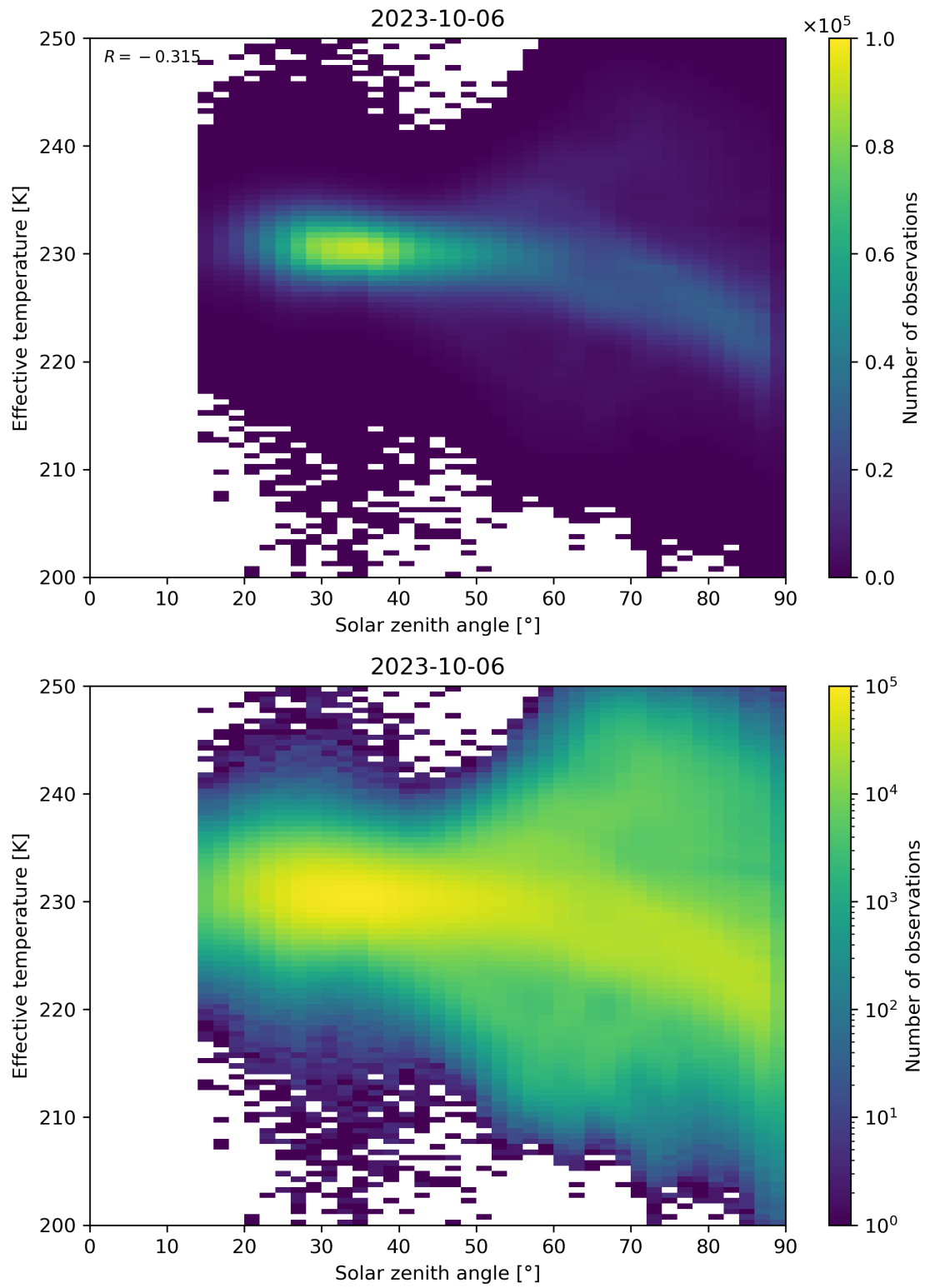
Figure 45: Scatter density plot of “Solar zenith angle” against “Effective temperature” for 2023-10-06 to 2023-10-07.
