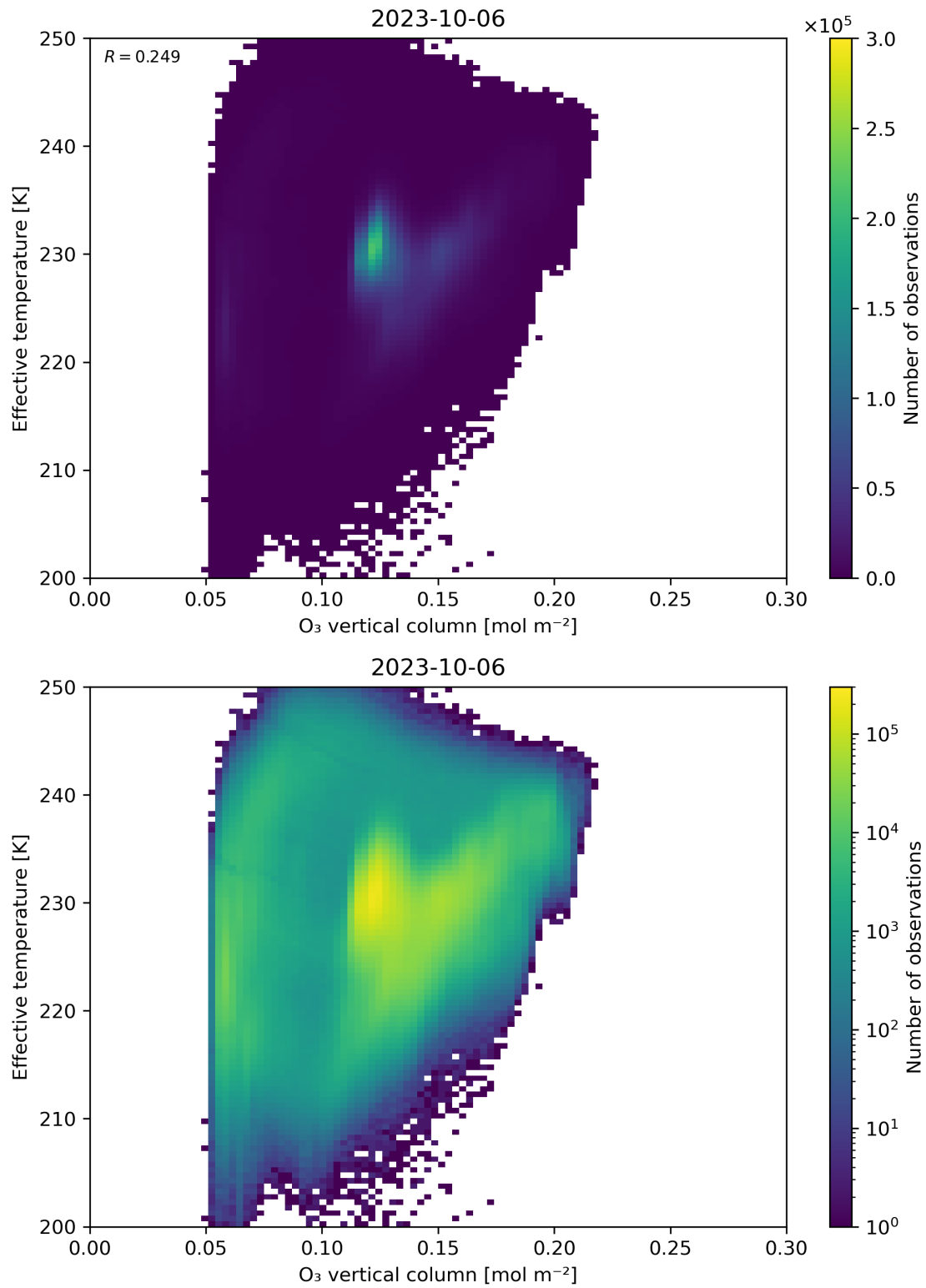
Figure 39: Scatter density plot of “O 3 vertical column” against “Effective temperature” for 2023-10-06 to 2023-10-07.
