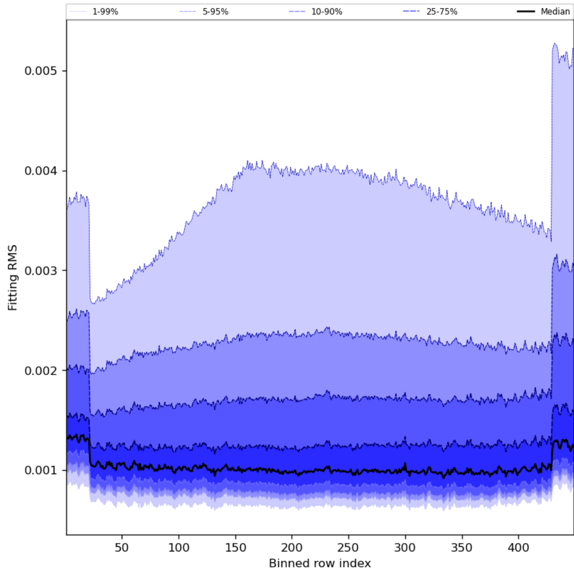
Figure 30: Along track statistics of “Fitting RMS” for 2023-10-06 to 2023-10-07
