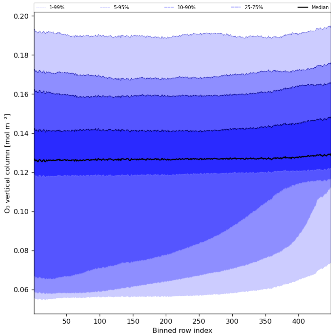
Figure 28: Along track statistics of “O 3 vertical column” for 2023-10-06 to 2023-10-07
