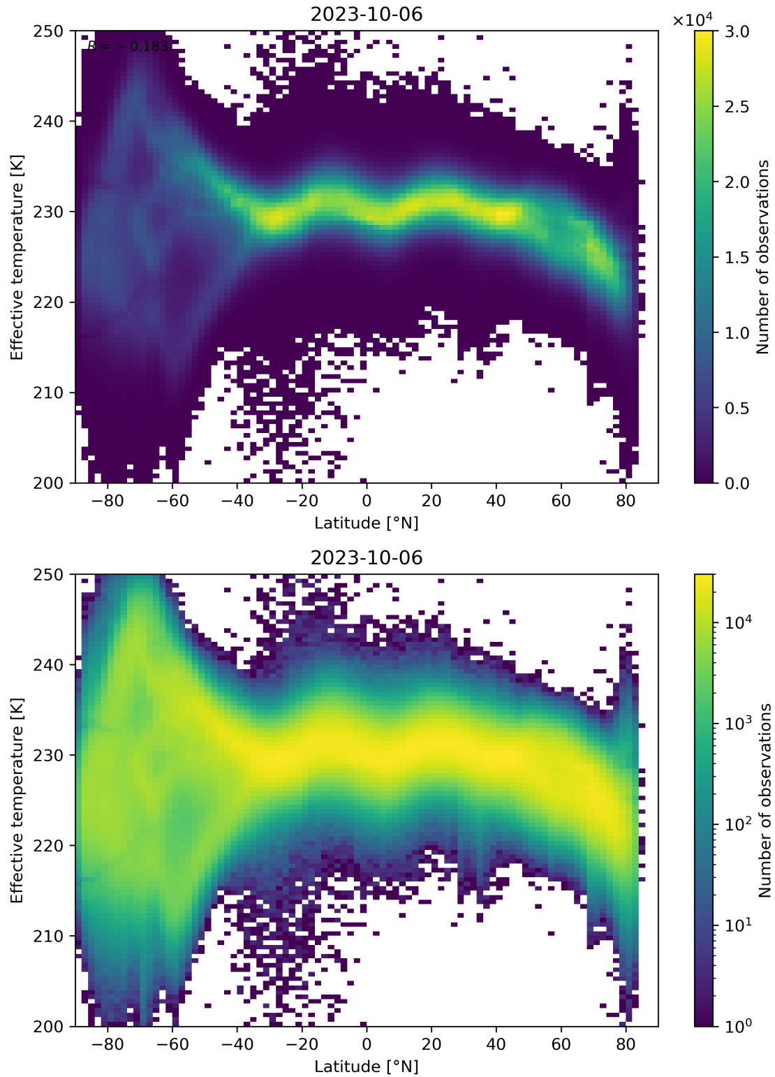
Figure 34: Scatter density plot of “Latitude” against “Effective temperature” for 2023-10-06 to 2023-10-07.
