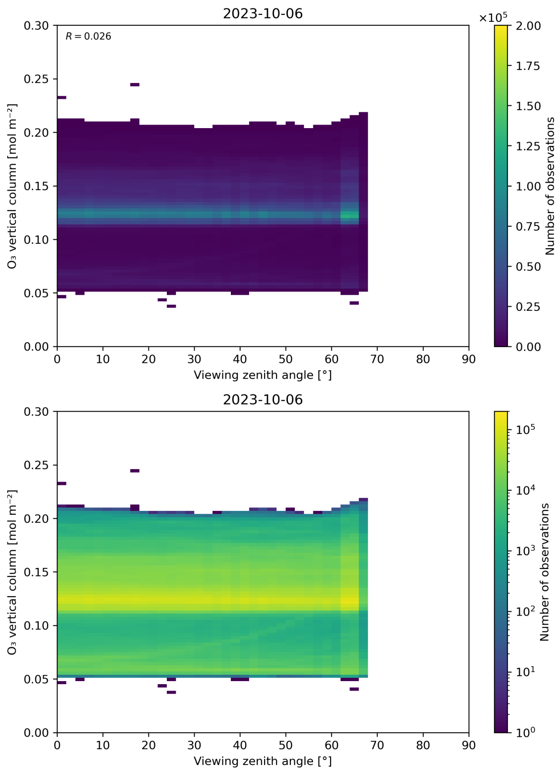
Figure 52: Scatter density plot of “Viewing zenith angle” against “O 3 vertical column” for 2023-10-06 to 2023-10-07.
