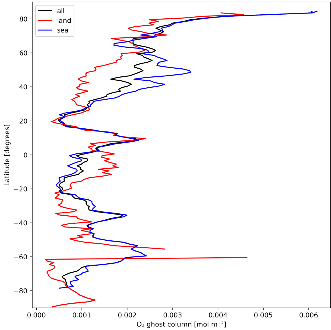
Figure 18: Zonal average of “O 3 ghost column” for 2023-10-06 to 2023-10-07.
