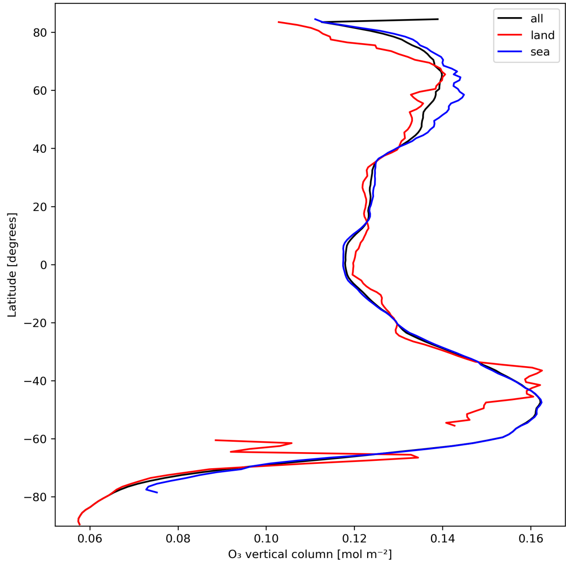
Figure 14: Zonal average of “O 3 vertical column” for 2023-10-06 to 2023-10-07.
