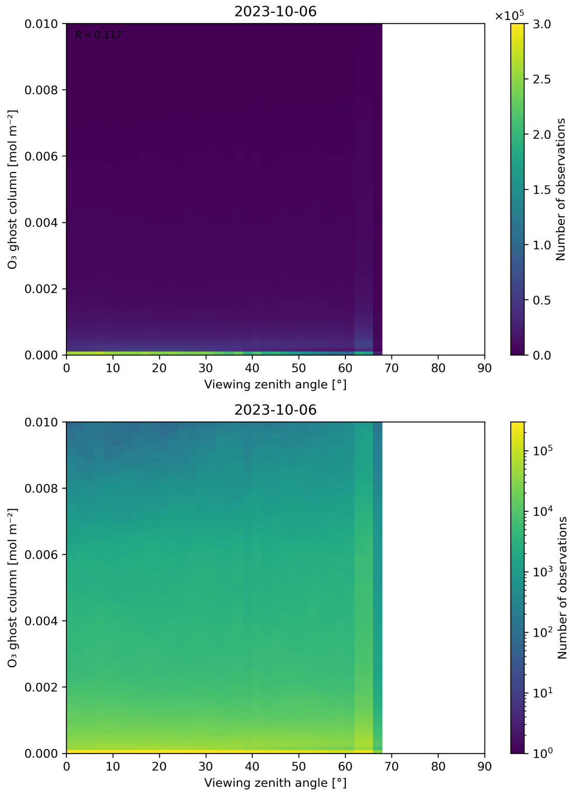
Figure 51: Scatter density plot of “Viewing zenith angle” against “O 3 ghost column” for 2023-10-06 to 2023-10-07.
