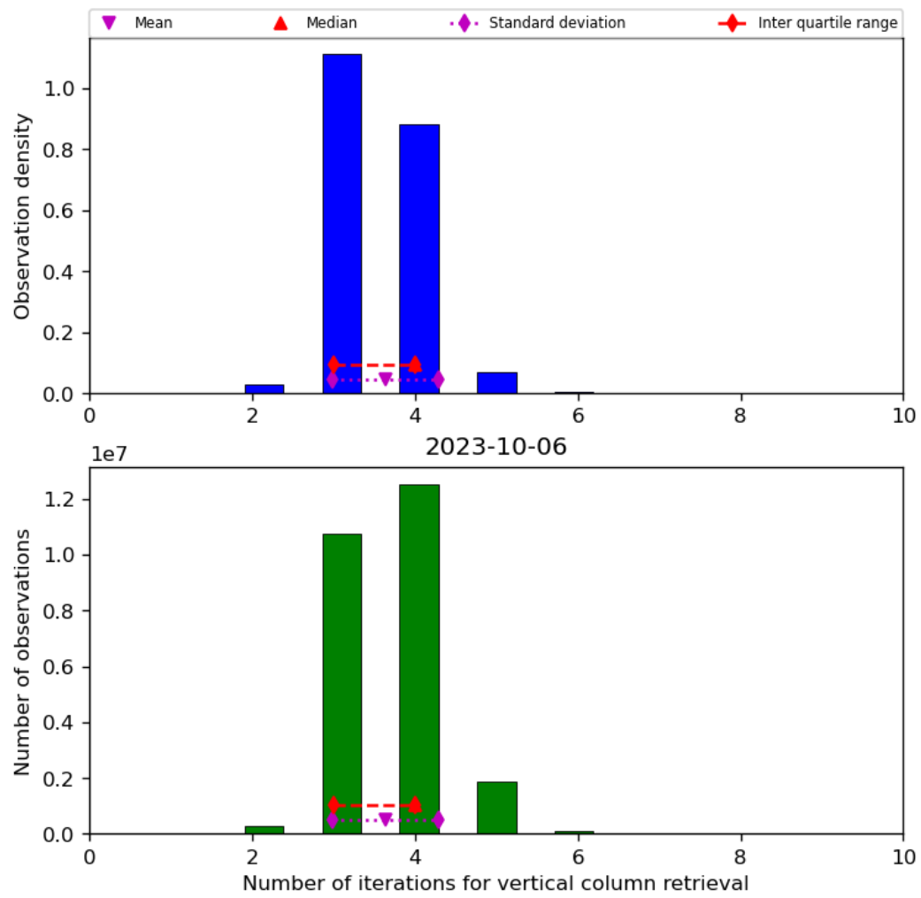
Figure 26: Histogram of “Number of iterations for vertical column retrieval” for 2023-10-06 to 2023-10-07
