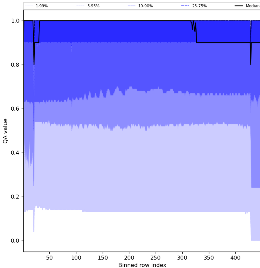
Figure 27: Along track statistics of “QA value” for 2023-10-06 to 2023-10-07
