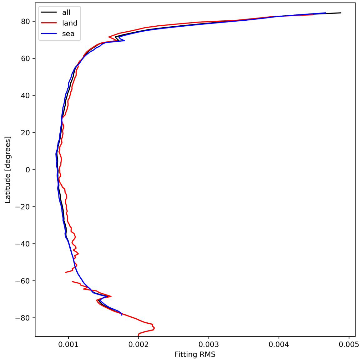
Figure 16: Zonal average of “Fitting RMS” for 2023-10-06 to 2023-10-07.
