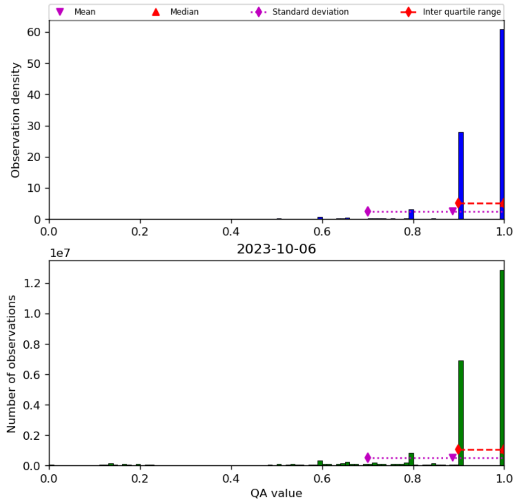
Figure 20: Histogram of “QA value” for 2023-10-06 to 2023-10-07
