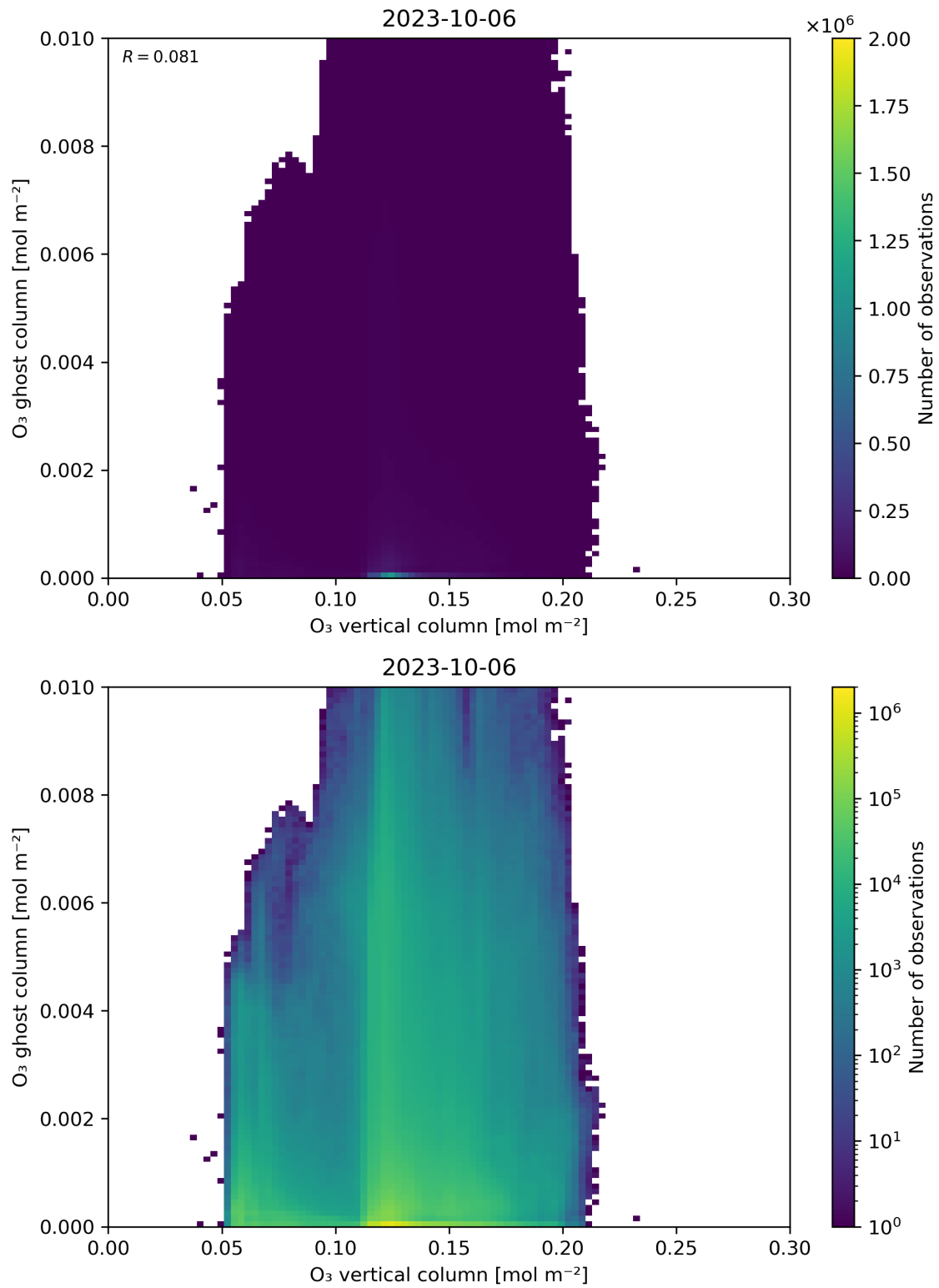
Figure 40: Scatter density plot of “O 3 vertical column” against “O 3 ghost column” for 2023-10-06 to 2023-10-07.
