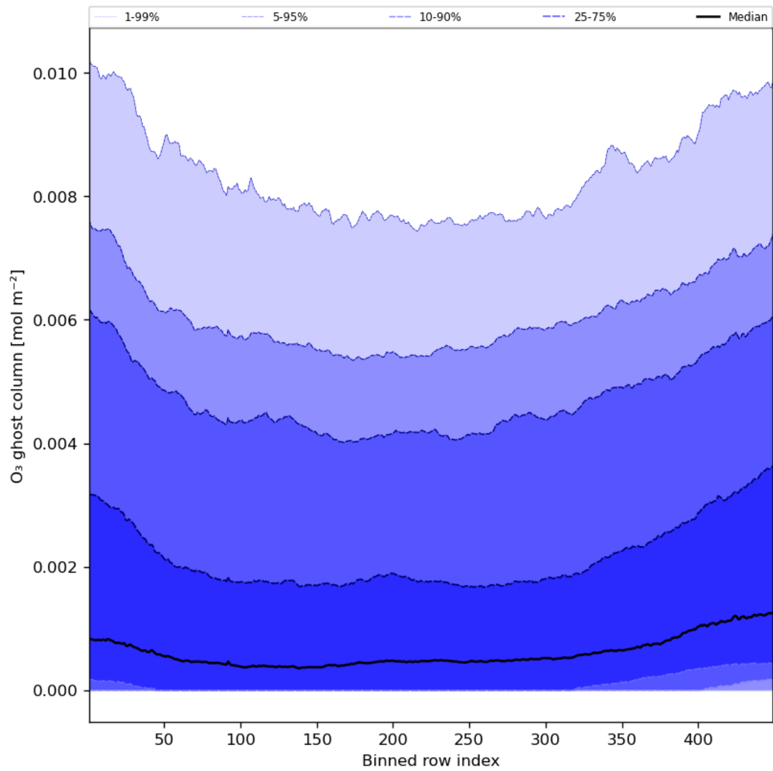
Figure 32: Along track statistics of “O 3 ghost column” for 2023-10-06 to 2023-10-07
