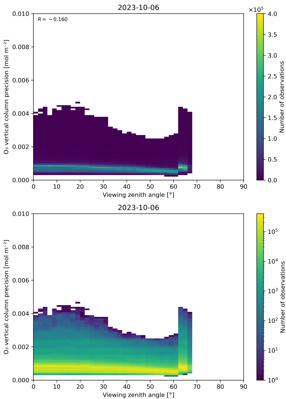
Figure 53: Scatter density plot of “Viewing zenith angle” against “O 3 vertical column precision” for 2023-10-06 to 2023-10-07.
