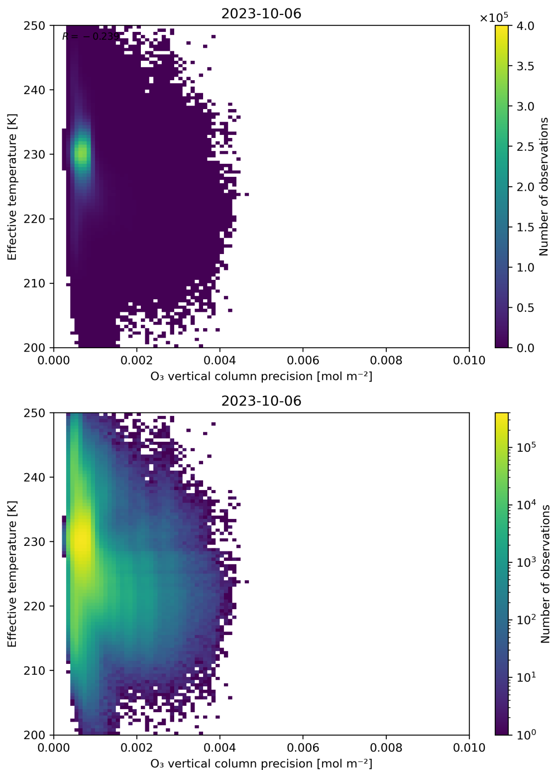
Figure 42: Scatter density plot of “O 3 vertical column precision” against “Effective temperature” for 2023-10-06 to 2023-10-07.
