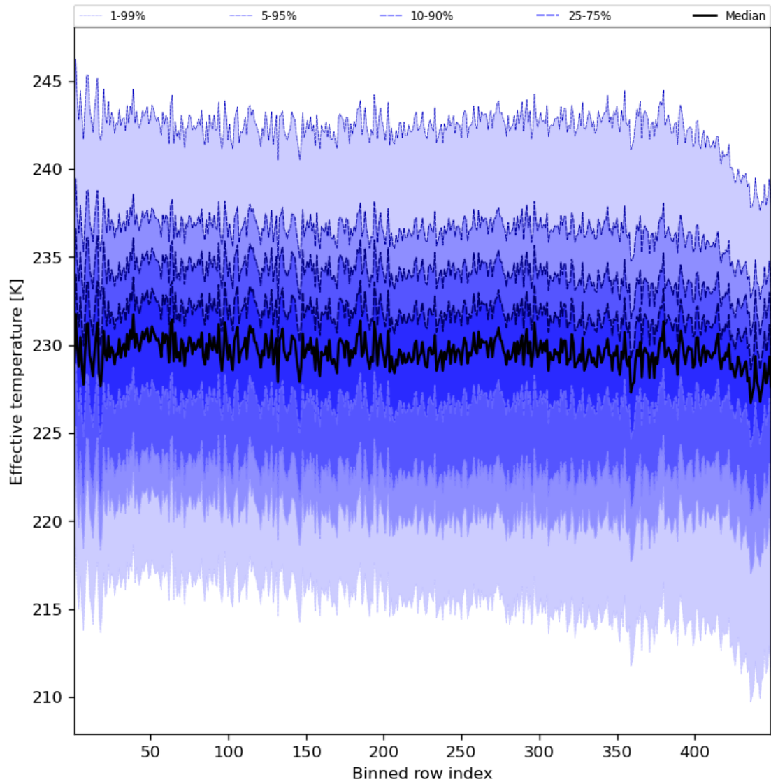
Figure 31: Along track statistics of “Effective temperature” for 2023-10-06 to 2023-10-07
