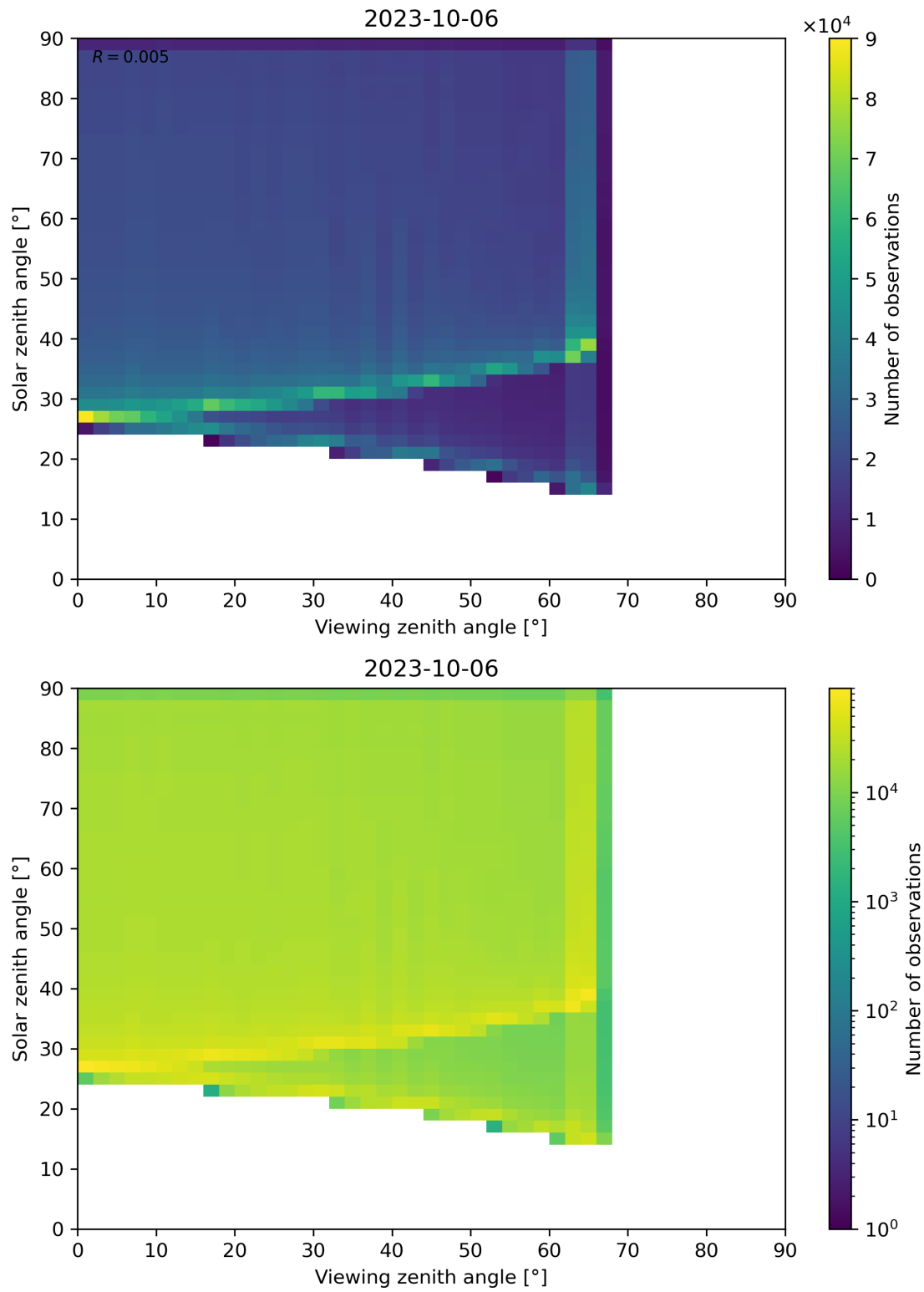
Figure 54: Scatter density plot of “Viewing zenith angle” against “Solar zenith angle” for 2023-10-06 to 2023-10-07.
