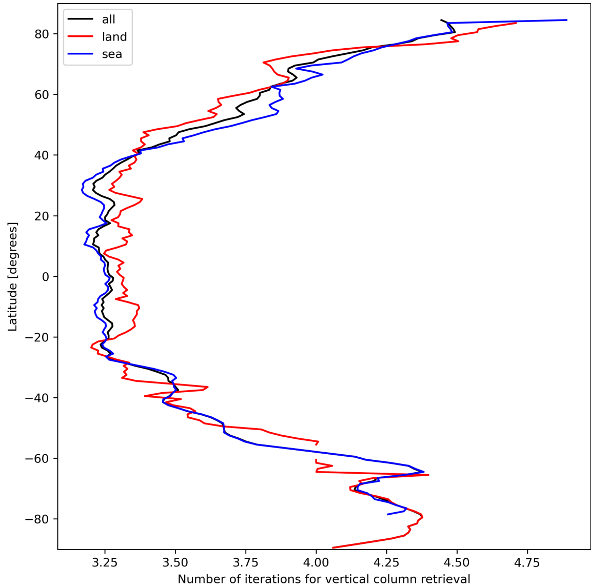
Figure 19: Zonal average of “Number of iterations for vertical column retrieval” for 2023-10-06 to 2023-10-07.
