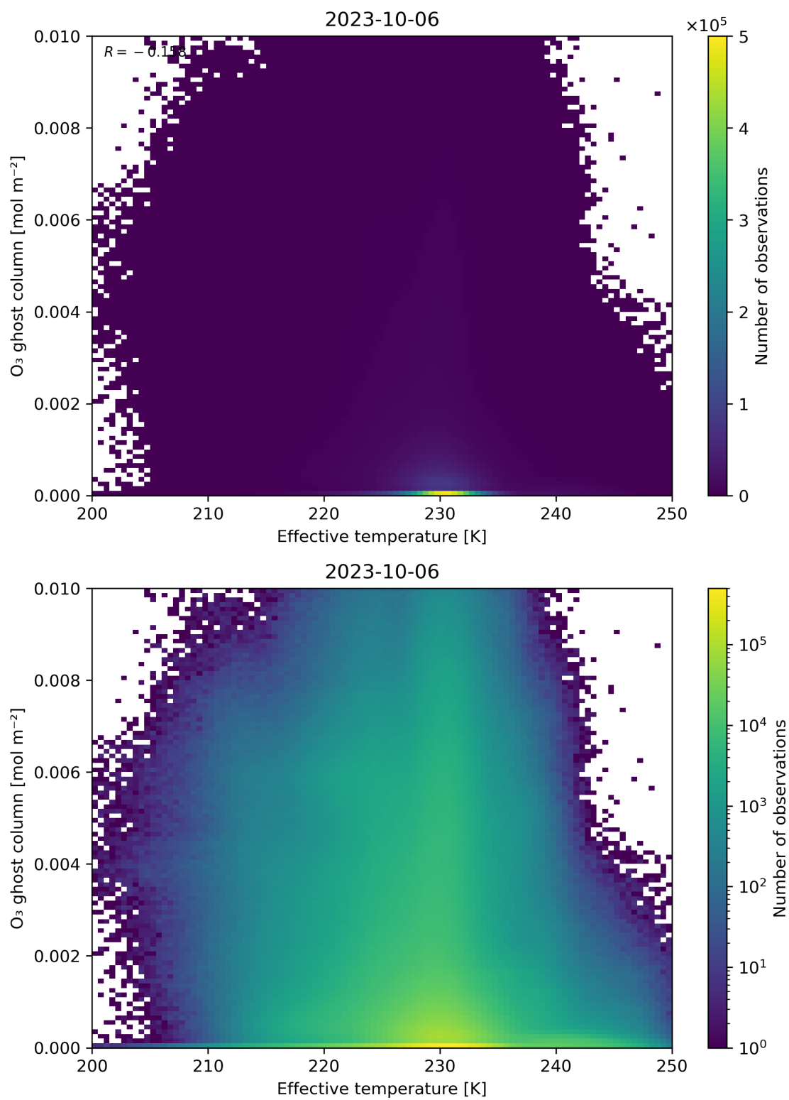
Figure 38: Scatter density plot of “Effective temperature” against “O 3 ghost column” for 2023-10-06 to 2023-10-07.
