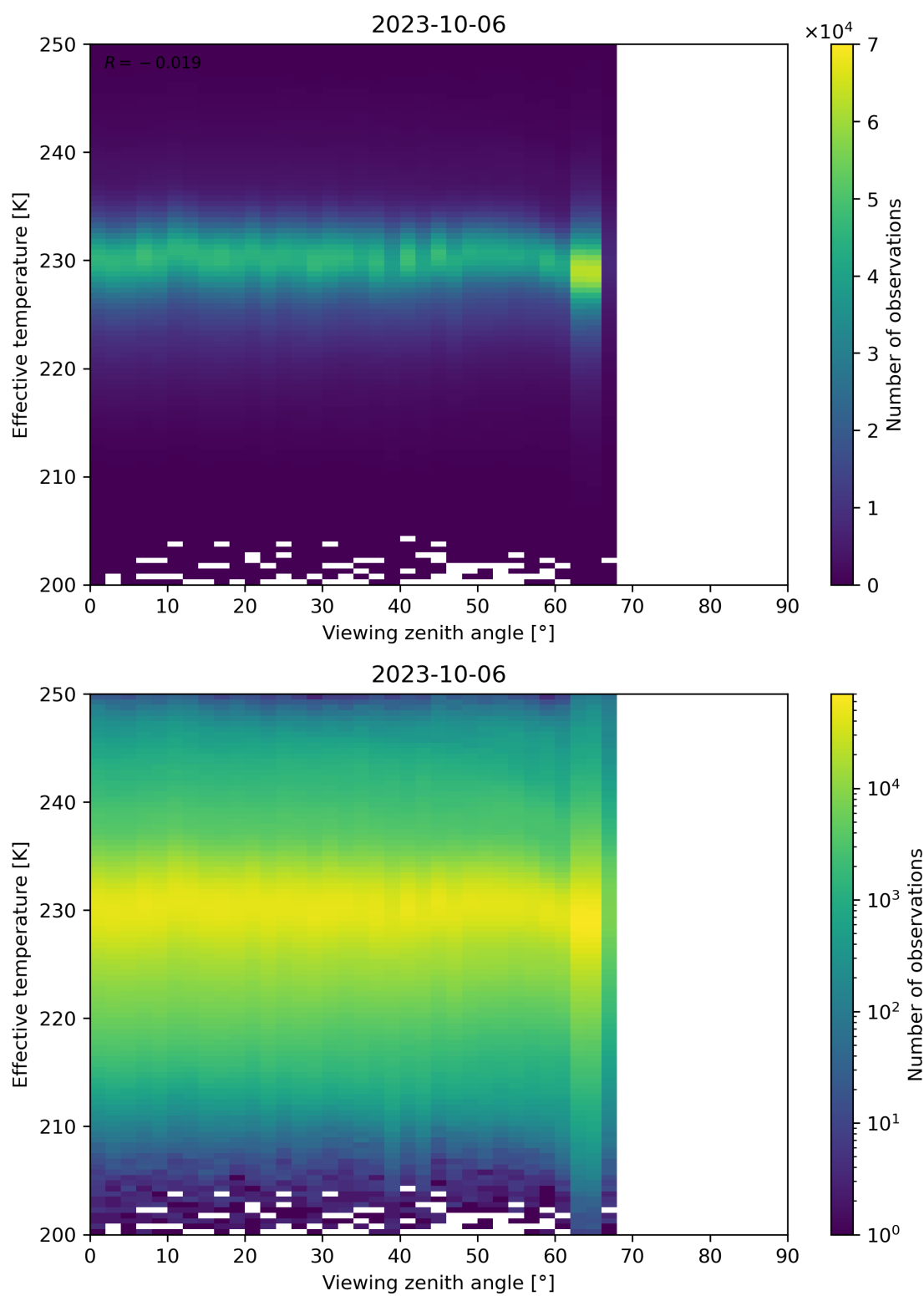
Figure 50: Scatter density plot of “Viewing zenith angle” against “Effective temperature” for 2023-10-06 to 2023-10-07.
