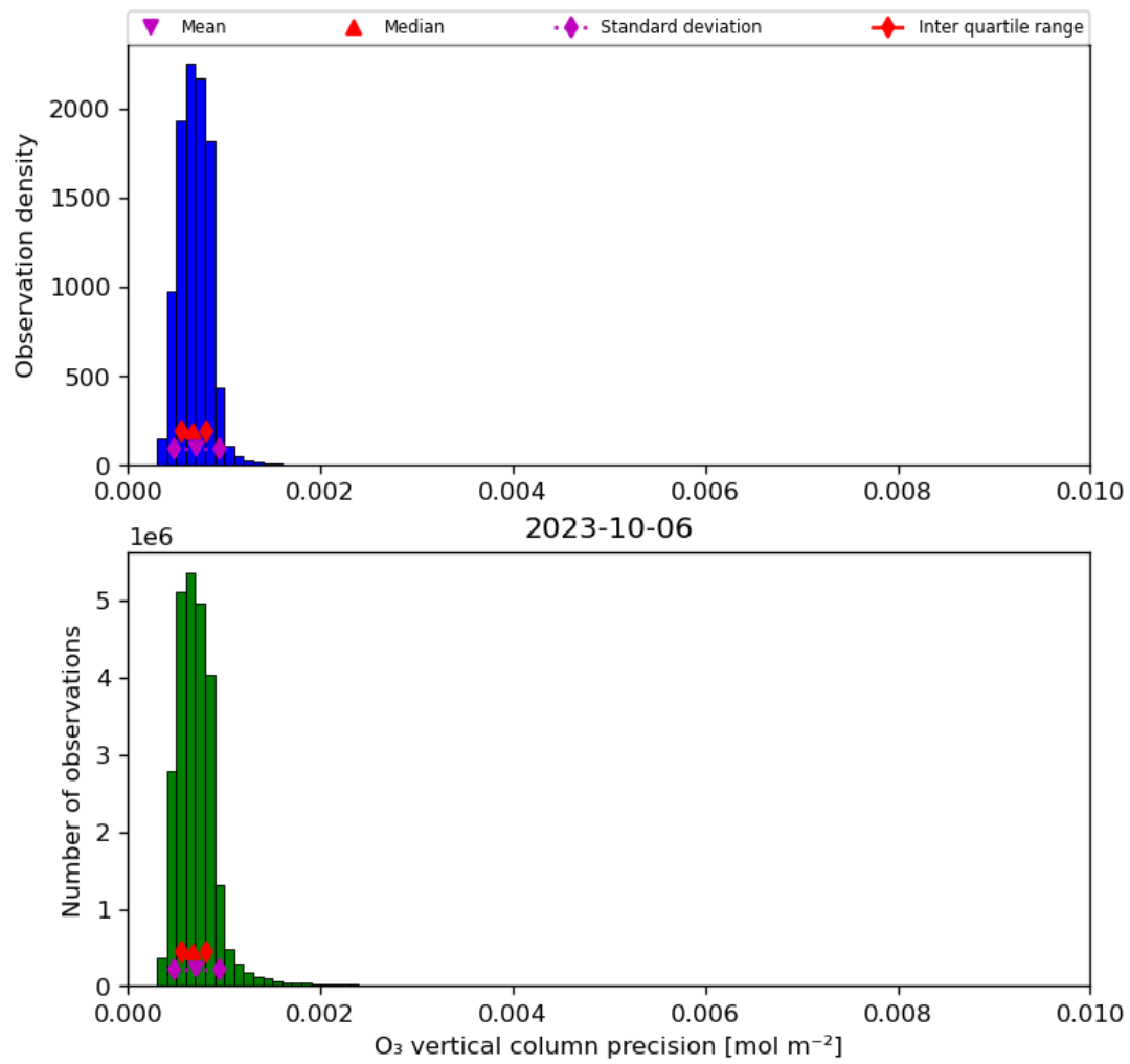
Figure 22: Histogram of “O 3 vertical column precision” for 2023-10-06 to 2023-10-07
