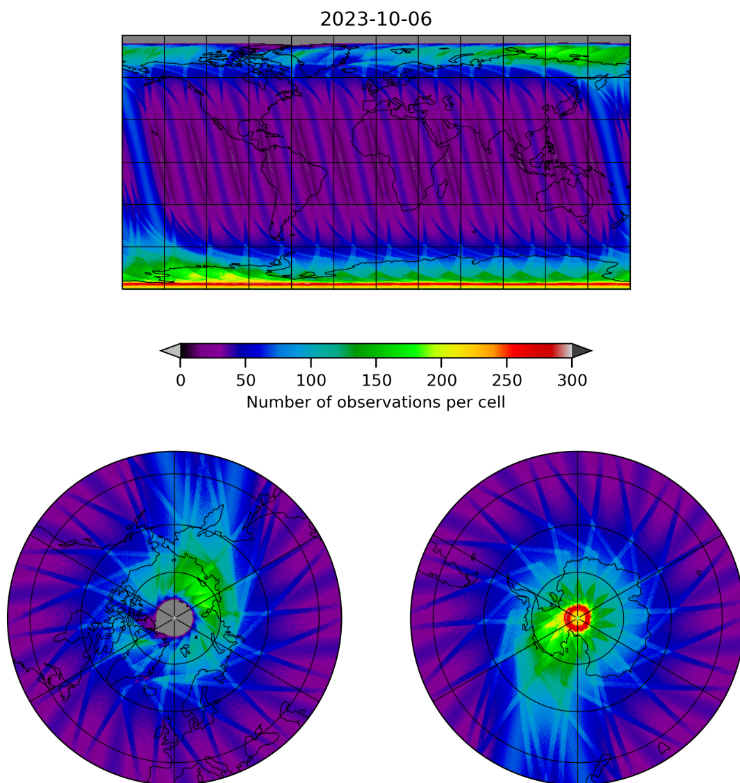
Figure 12: Map of the number of observations for 2023-10-06 to 2023-10-07
