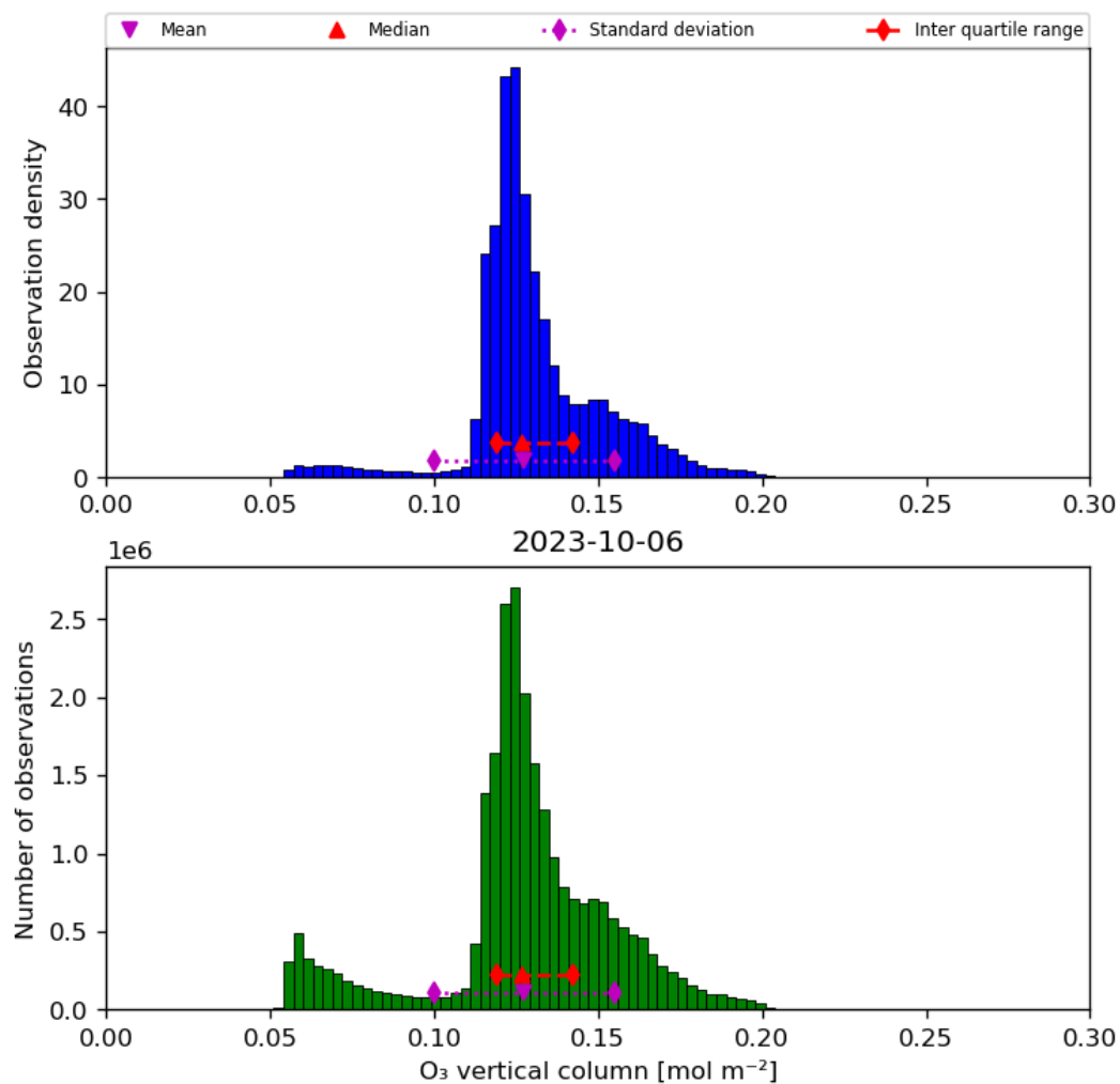
Figure 21: Histogram of “O 3 vertical column” for 2023-10-06 to 2023-10-07
