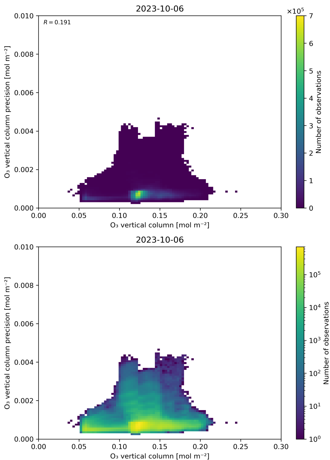
Figure 41: Scatter density plot of “O 3 vertical column” against “O 3 vertical column precision” for 2023-10-06 to 2023-10-07.
