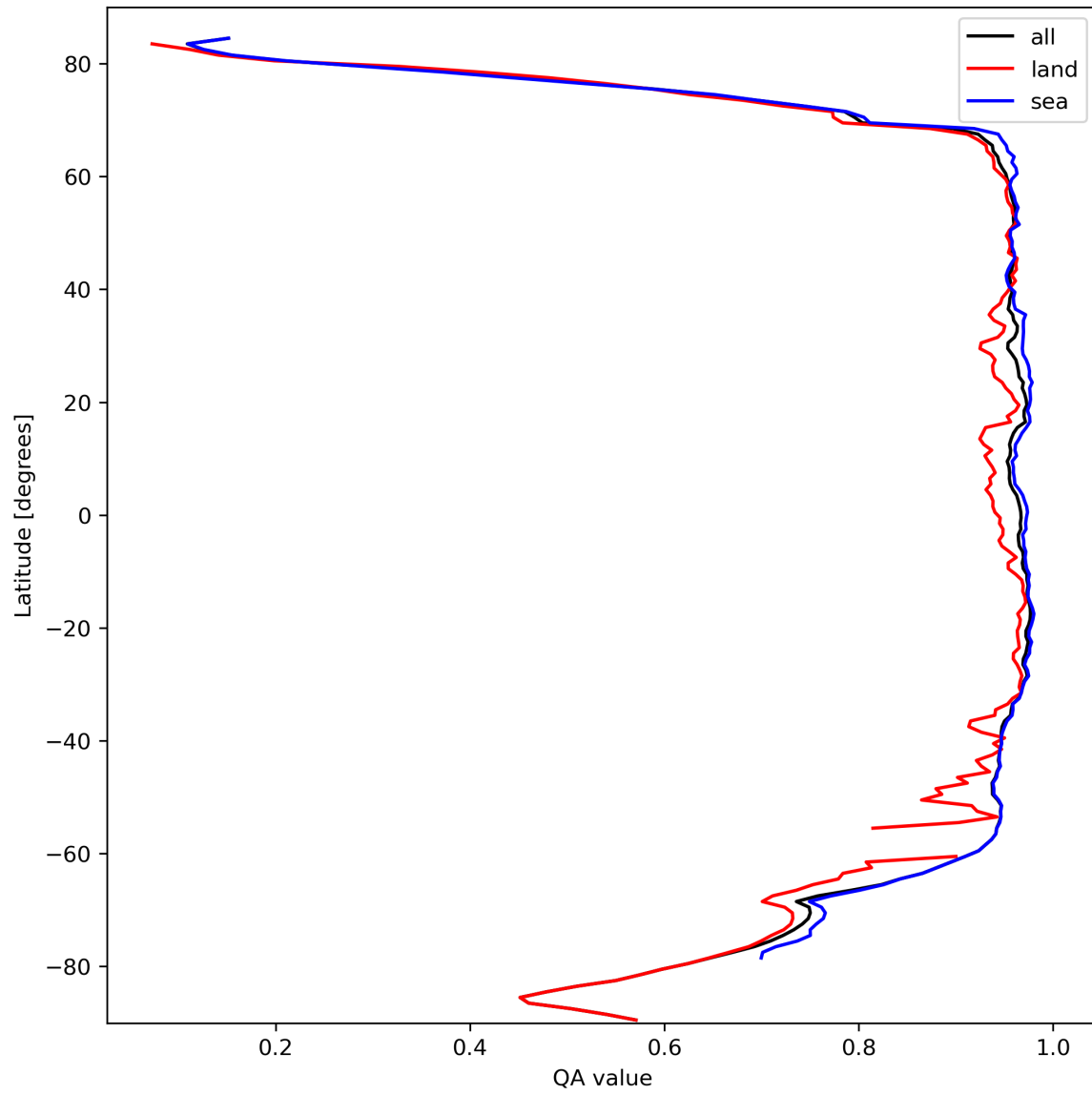
Figure 13: Zonal average of “QA value” for 2023-10-06 to 2023-10-07.
