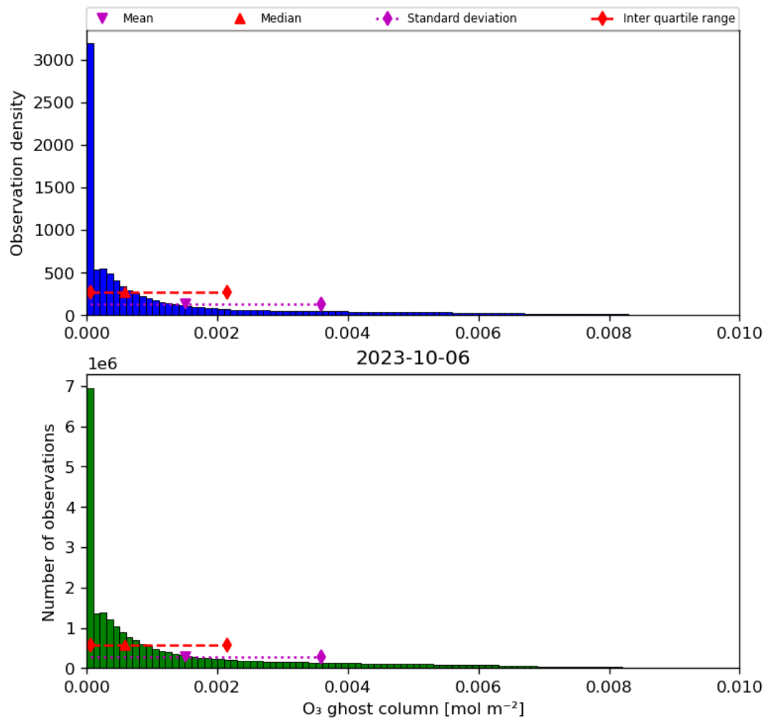
Figure 25: Histogram of “O 3 ghost column” for 2023-10-06 to 2023-10-07
