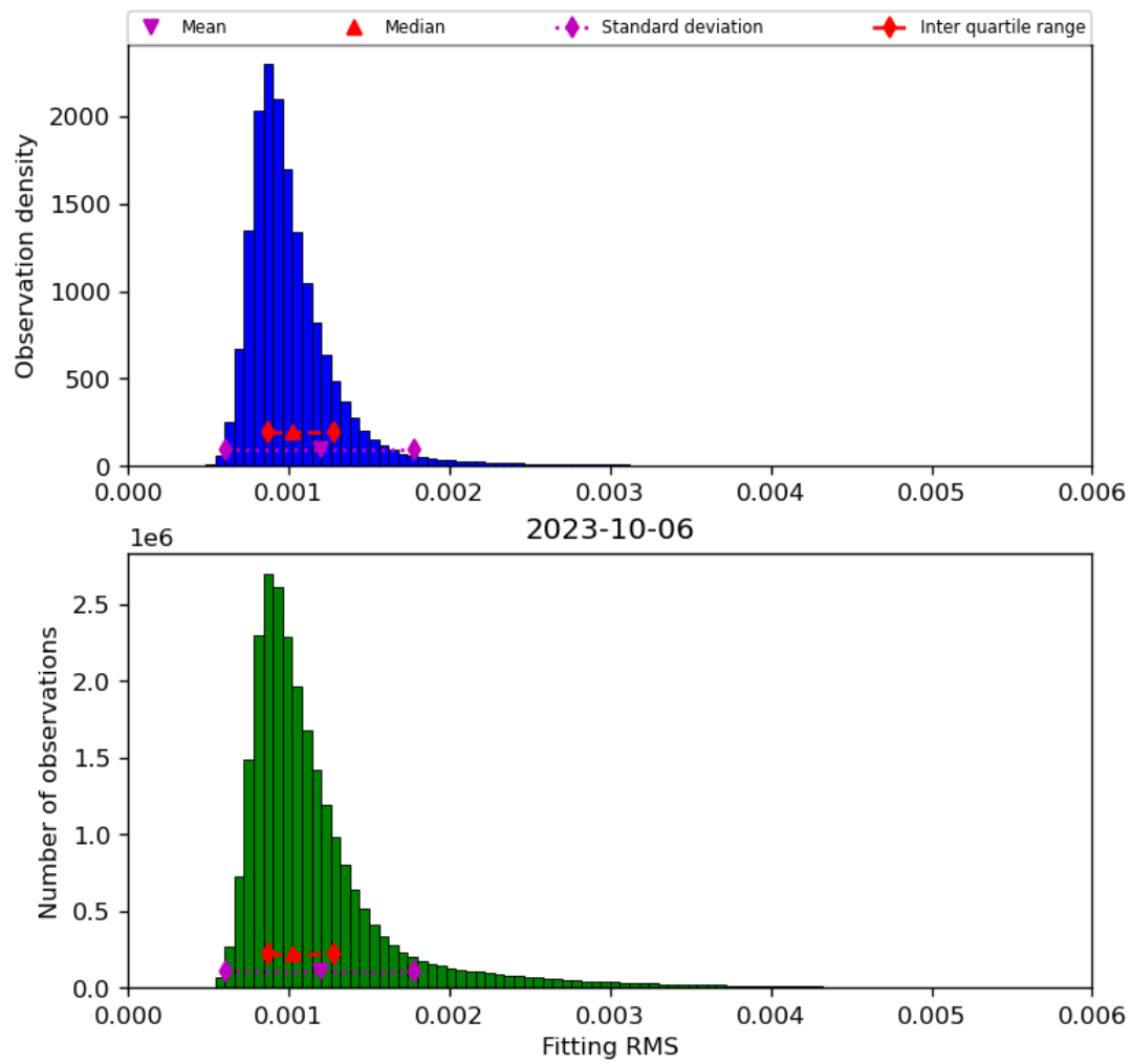
Figure 23: Histogram of “Fitting RMS” for 2023-10-06 to 2023-10-07
