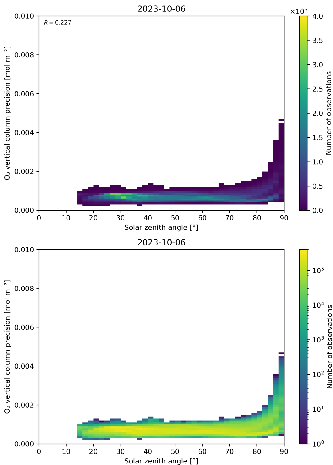
Figure 48: Scatter density plot of “Solar zenith angle” against “O 3 vertical column precision” for 2023-10-06 to 2023-10-07.
