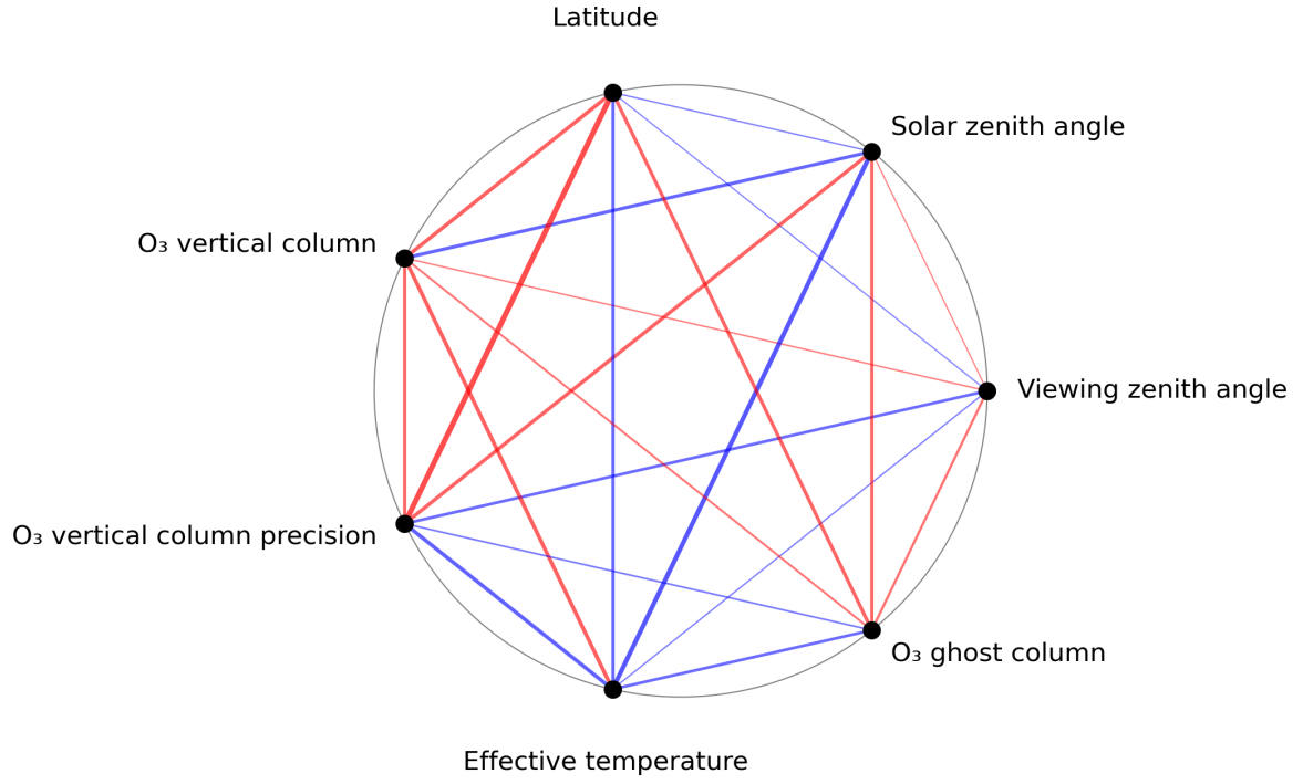
Figure 1: Map of correlation graph for 2023-10-06 to 2023-10-07.
