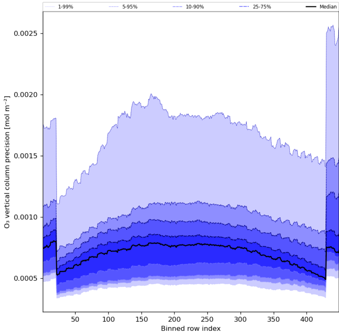
Figure 29: Along track statistics of “O 3 vertical column precision” for 2023-10-06 to 2023-10-07
