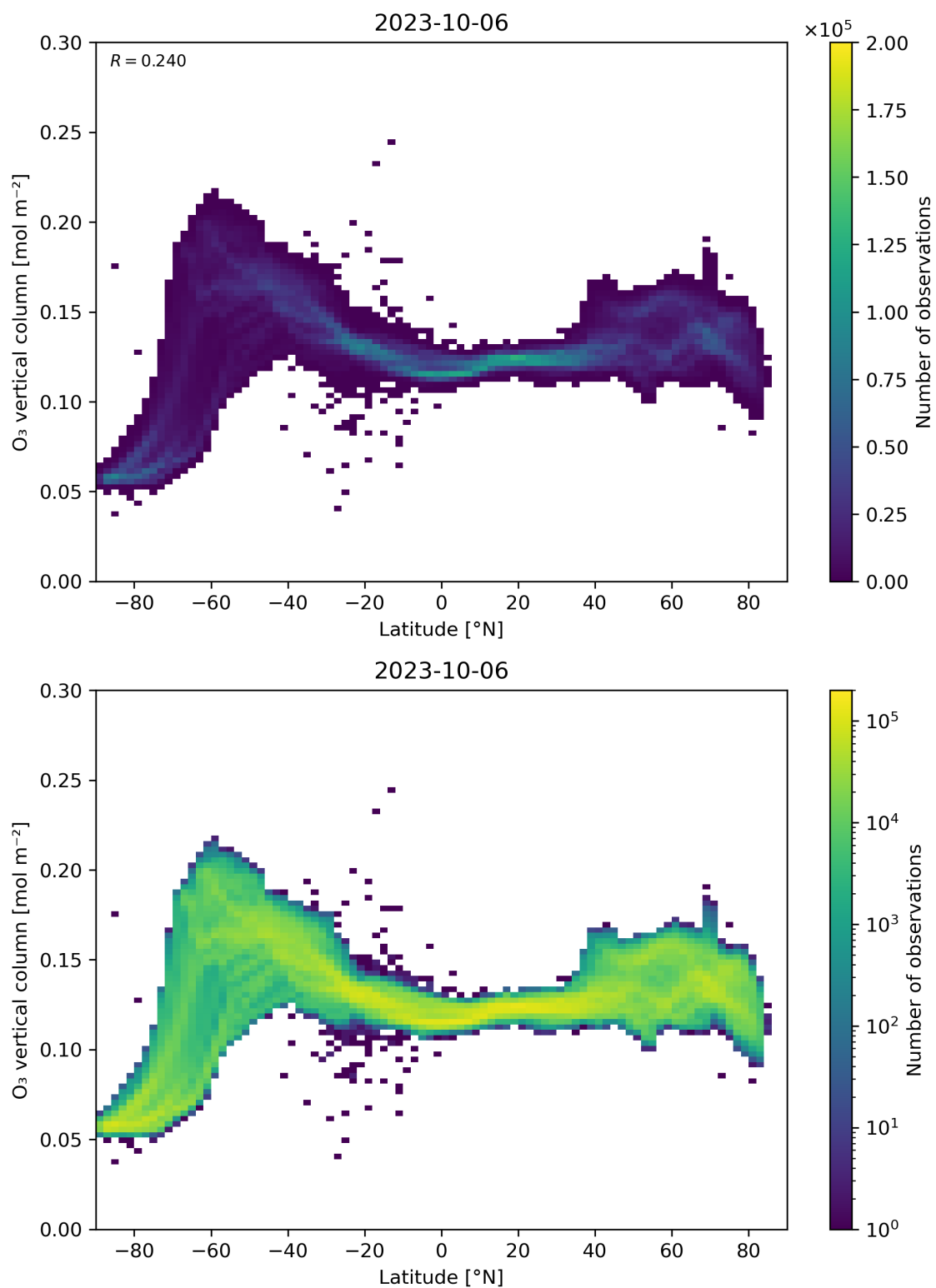
Figure 36: Scatter density plot of “Latitude” against “O 3 vertical column” for 2023-10-06 to 2023-10-07.
