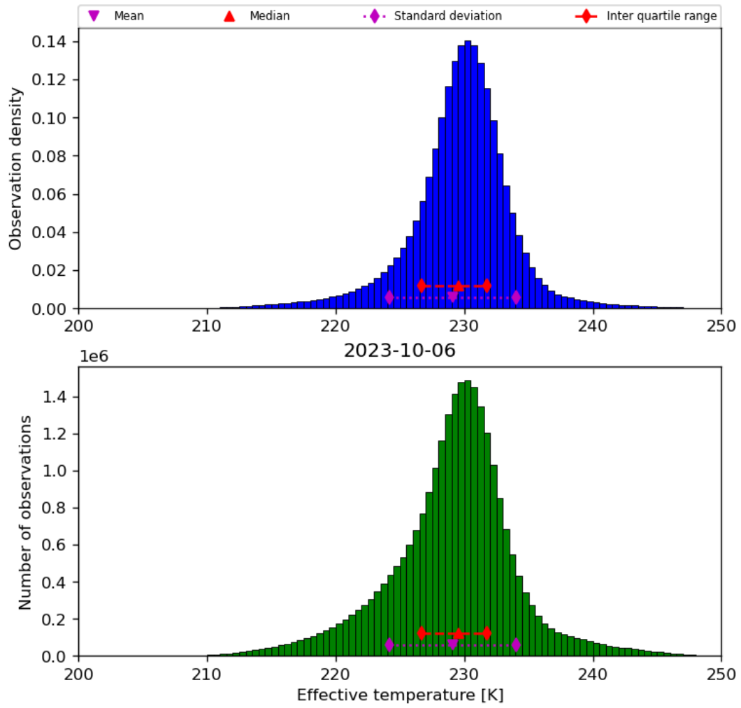
Figure 24: Histogram of “Effective temperature” for 2023-10-06 to 2023-10-07
