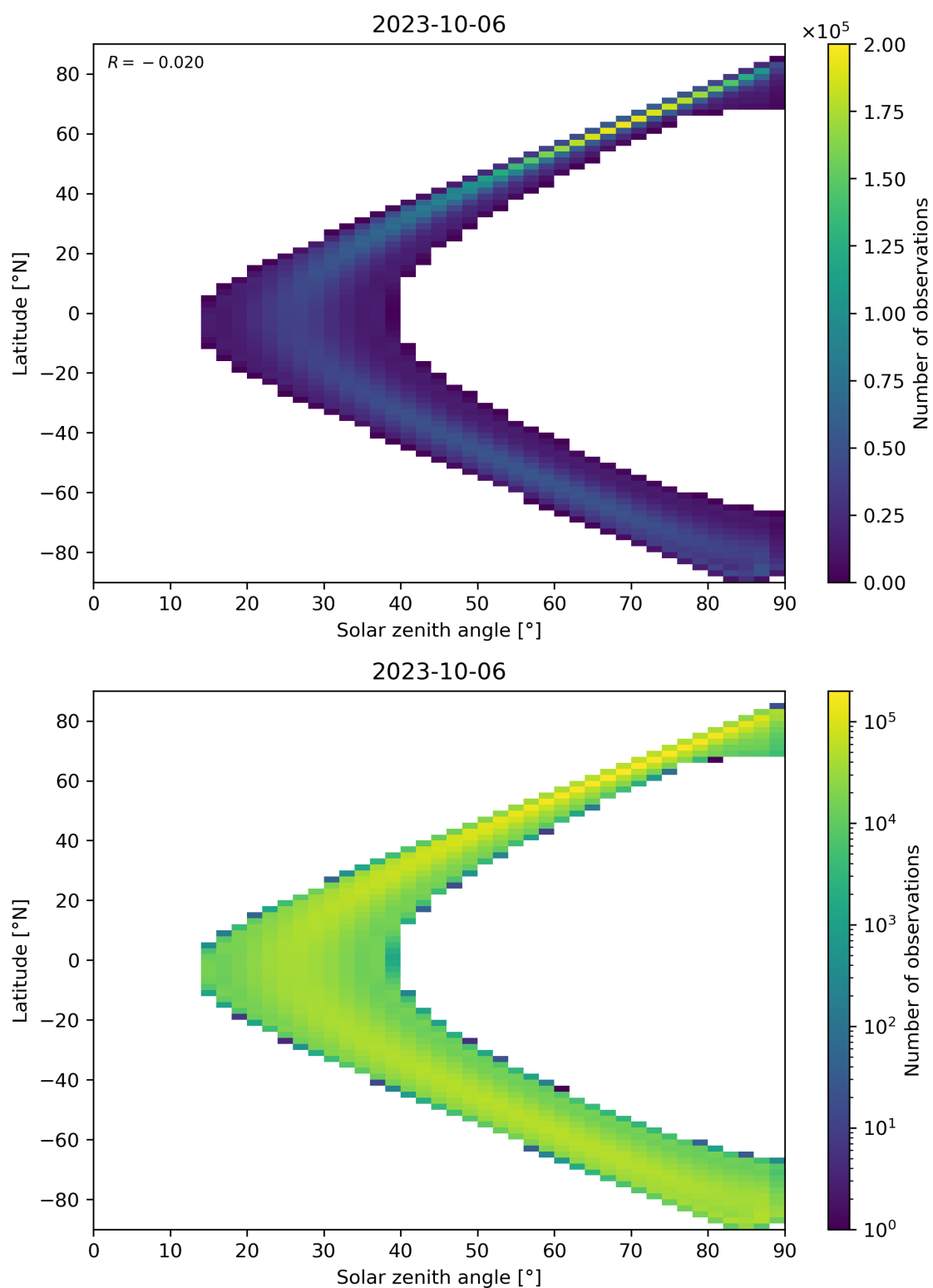
Figure 44: Scatter density plot of “Solar zenith angle” against “Latitude” for 2023-10-06 to 2023-10-07.
