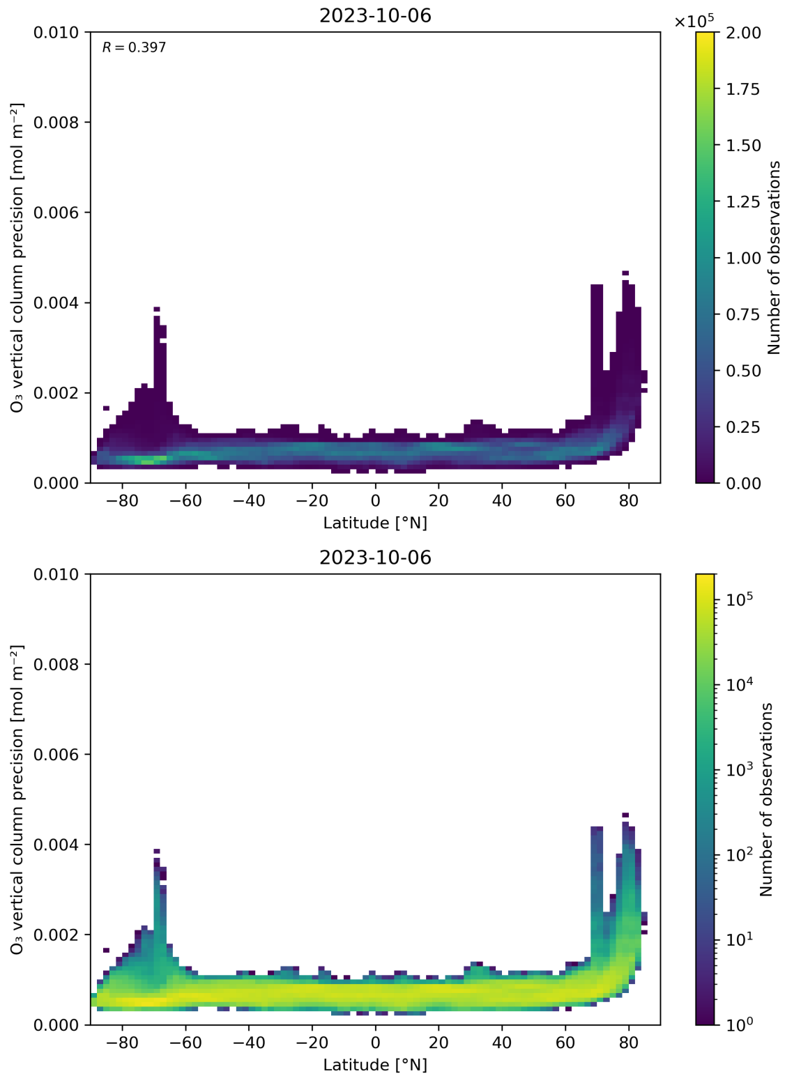
Figure 37: Scatter density plot of “Latitude” against “O 3 vertical column precision” for 2023-10-06 to 2023-10-07.
