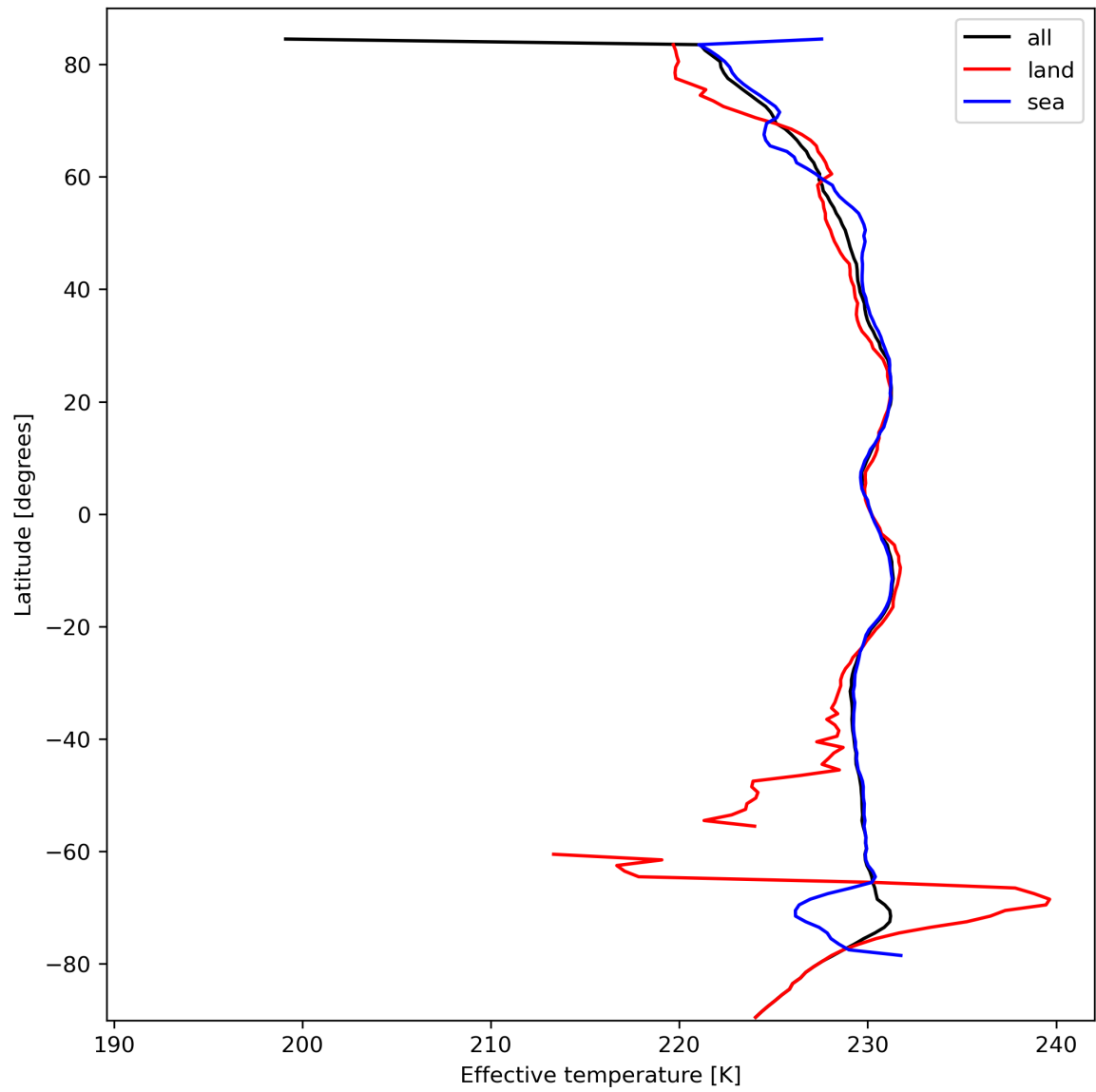
Figure 17: Zonal average of “Effective temperature” for 2023-10-06 to 2023-10-07.
