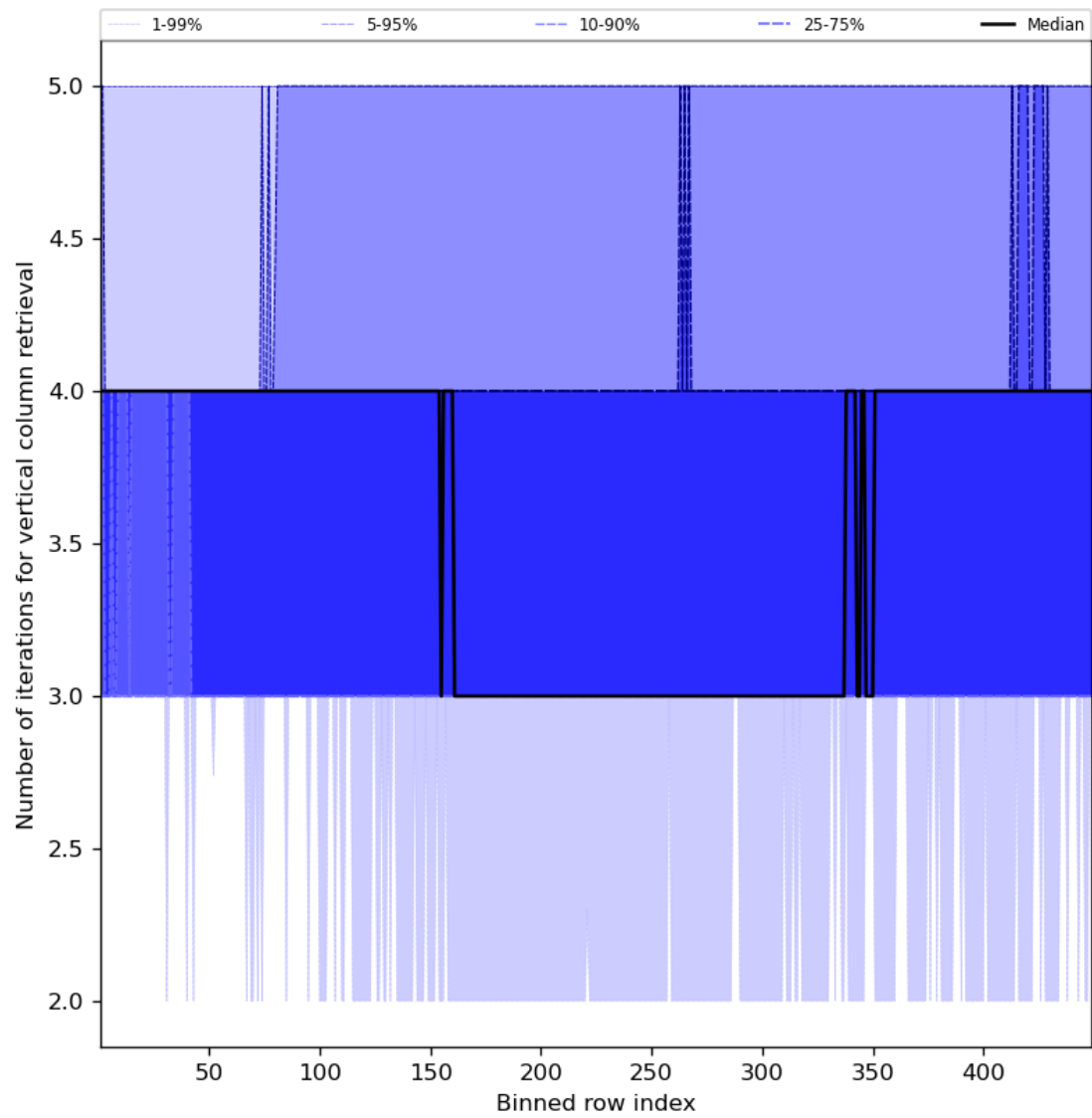
Figure 33: Along track statistics of “Number of iterations for vertical column retrieval” for 2023-10-06 to 2023-10-07
