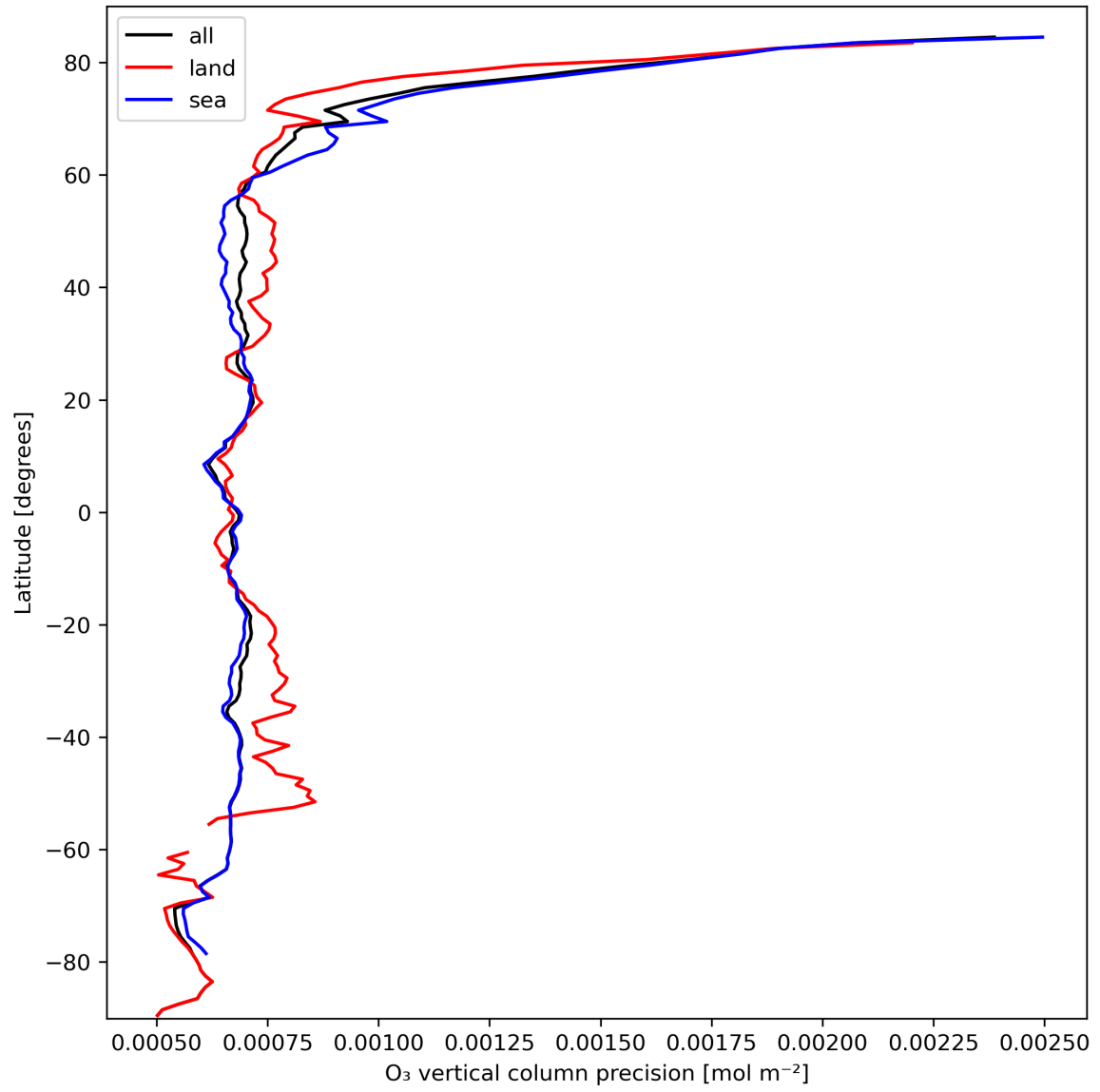
Figure 15: Zonal average of “O 3 vertical column precision” for 2023-10-06 to 2023-10-07.
