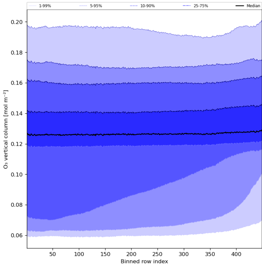
Figure 28: Along track statistics of “O 3 vertical column” for 2023-10-06 to 2023-10-08
