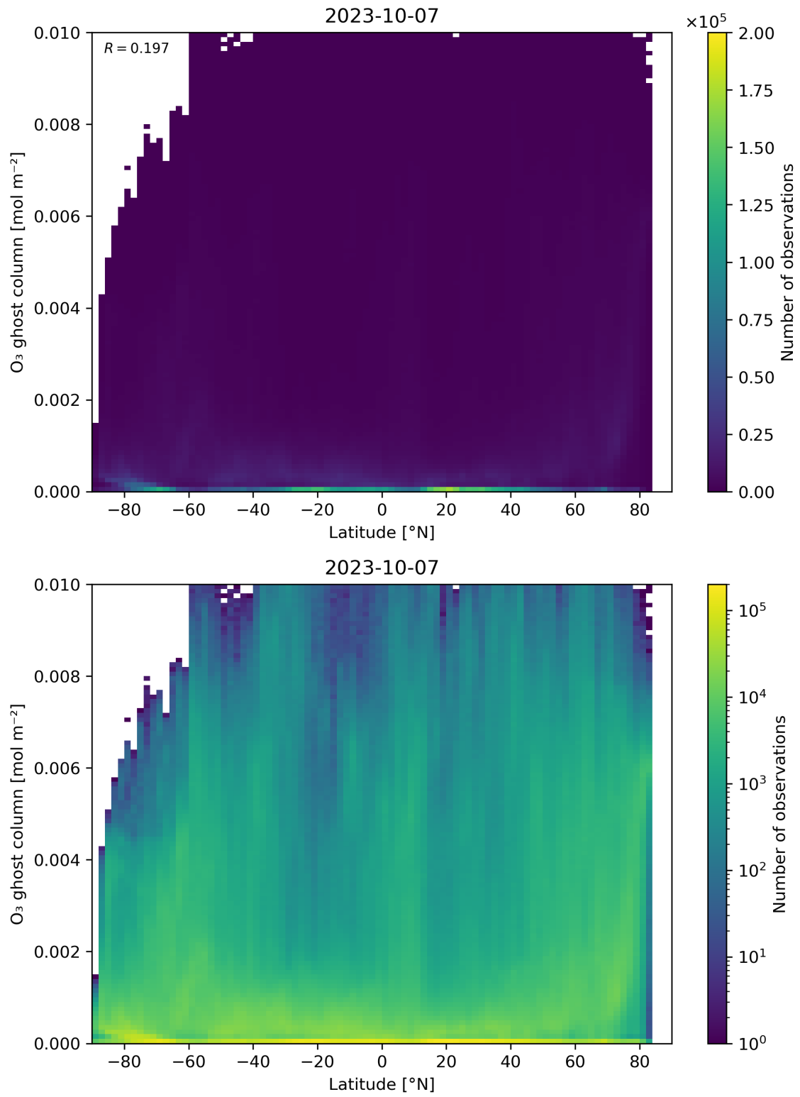
Figure 35: Scatter density plot of “Latitude” against “O 3 ghost column” for 2023-10-06 to 2023-10-08.
