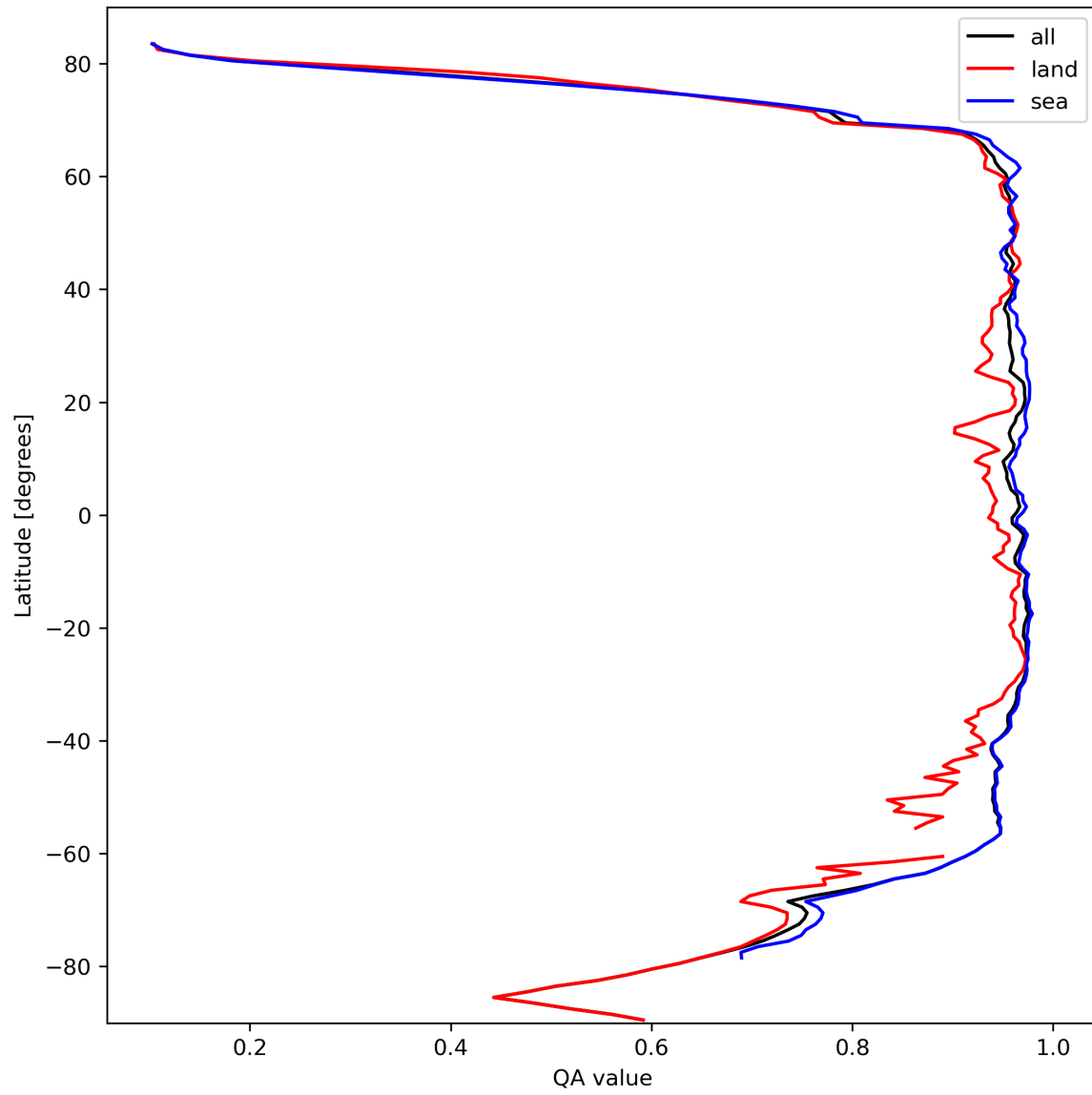
Figure 13: Zonal average of “QA value” for 2023-10-06 to 2023-10-08.
