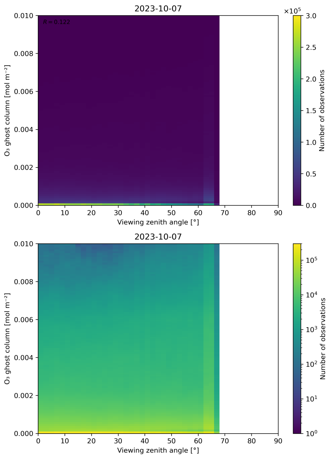
Figure 51: Scatter density plot of “Viewing zenith angle” against “O 3 ghost column” for 2023-10-06 to 2023-10-08.
