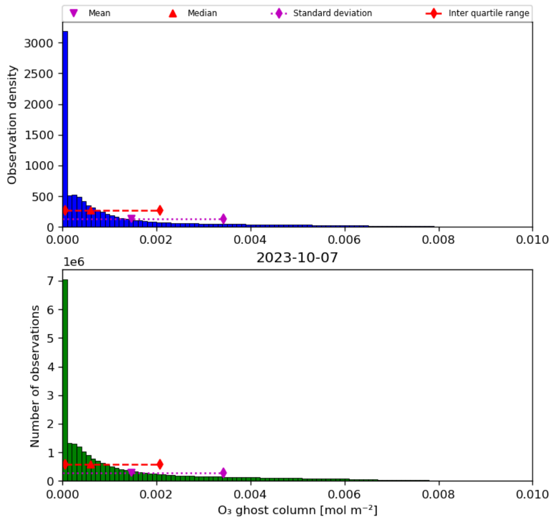
Figure 25: Histogram of “O 3 ghost column” for 2023-10-06 to 2023-10-08
