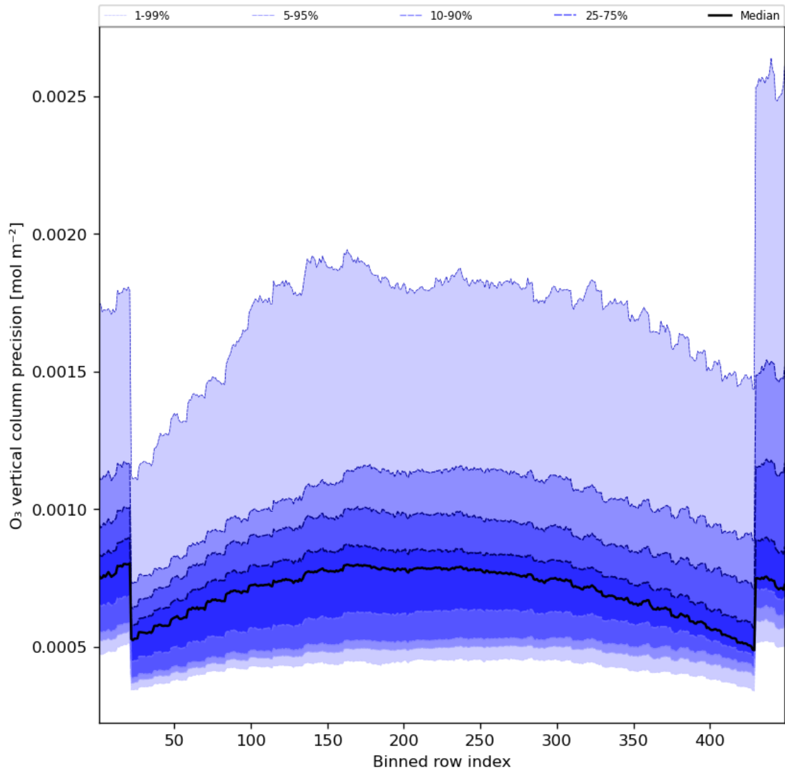
Figure 29: Along track statistics of “O 3 vertical column precision” for 2023-10-06 to 2023-10-08
