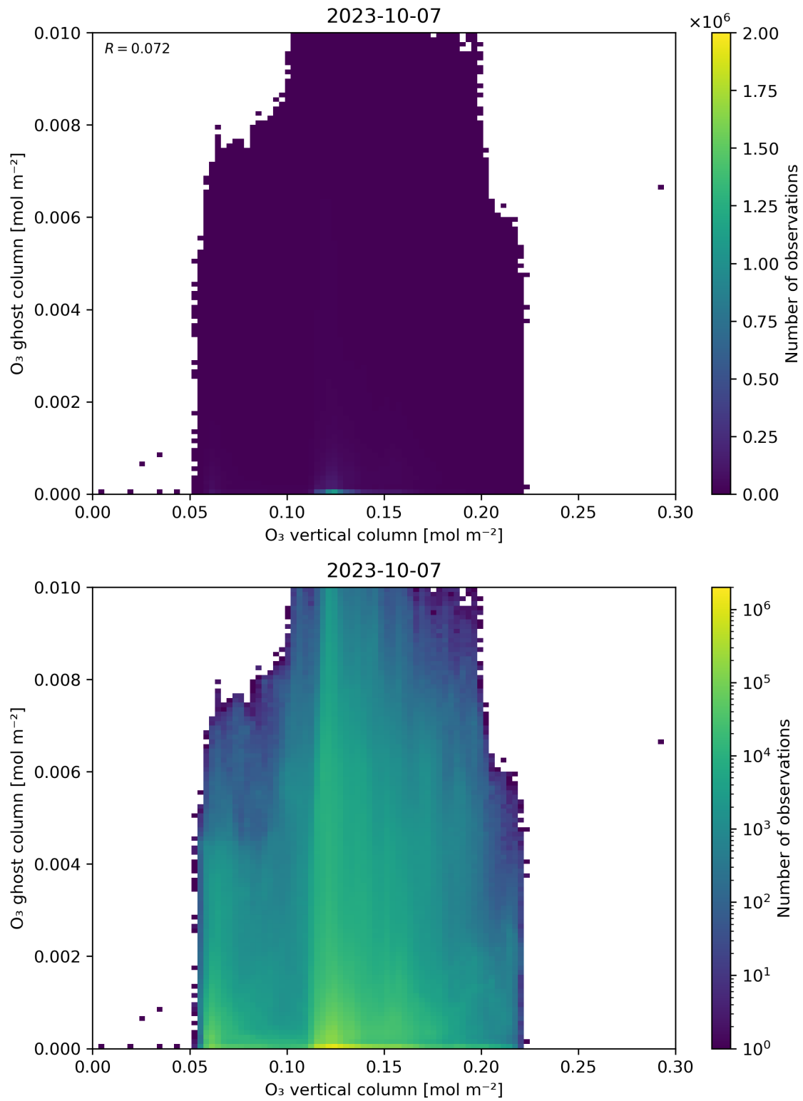
Figure 40: Scatter density plot of “O 3 vertical column” against “O 3 ghost column” for 2023-10-06 to 2023-10-08.
