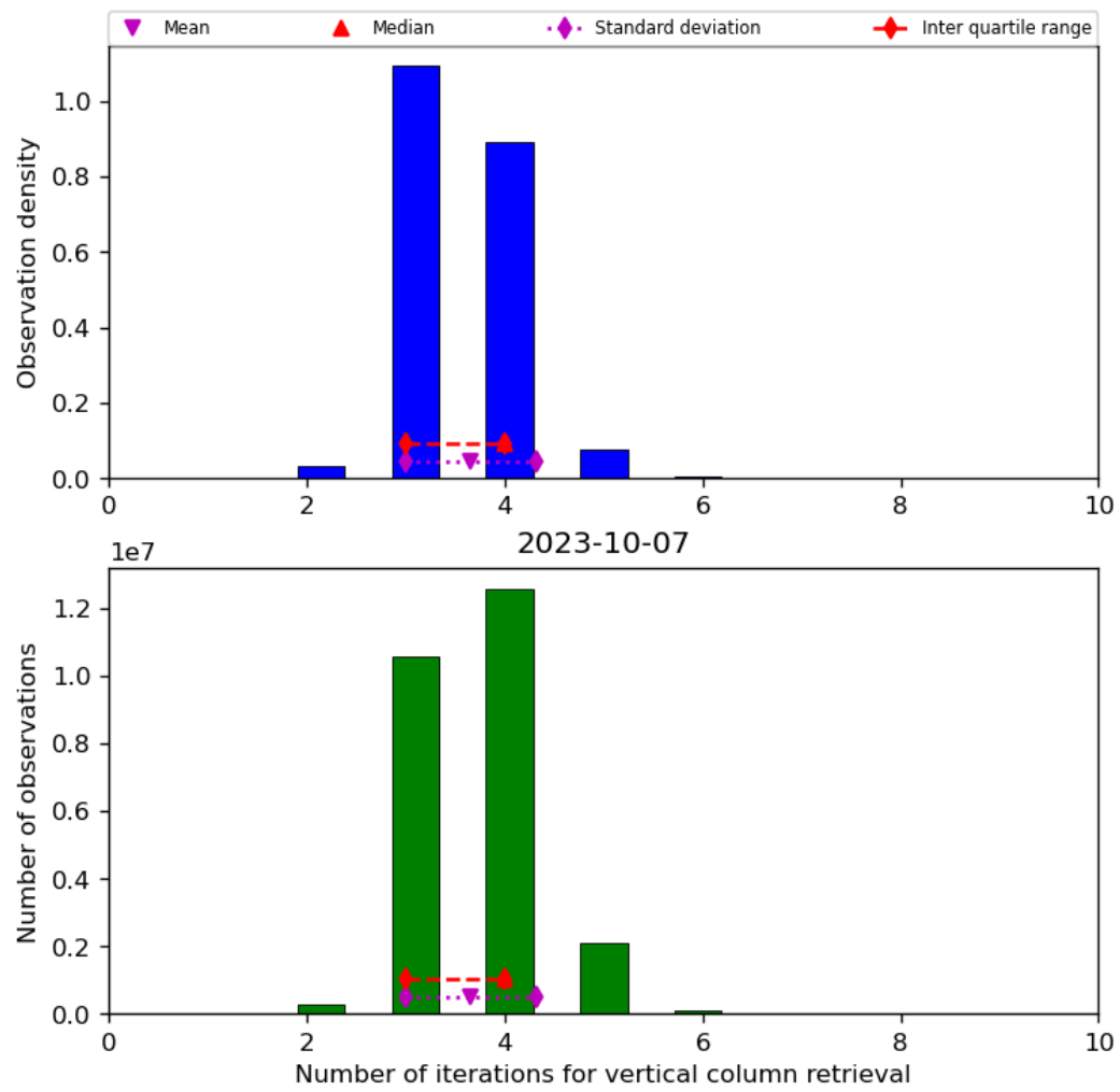
Figure 26: Histogram of “Number of iterations for vertical column retrieval” for 2023-10-06 to 2023-10-08
