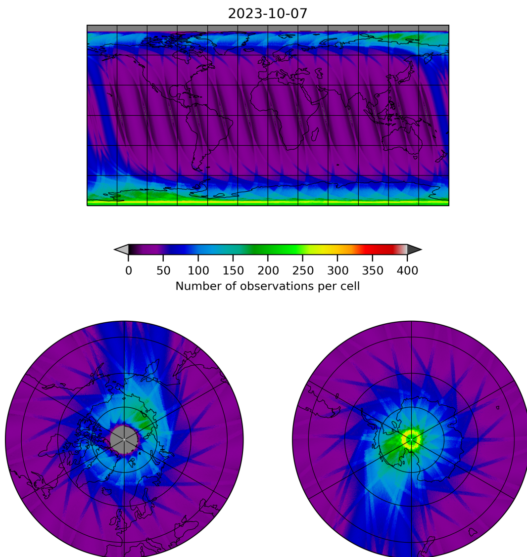
Figure 12: Map of the number of observations for 2023-10-06 to 2023-10-08
