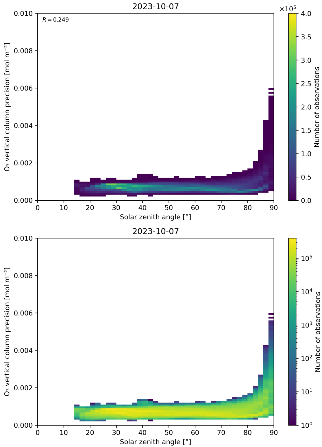
Figure 48: Scatter density plot of “Solar zenith angle” against “O 3 vertical column precision” for 2023-10-06 to 2023-10-08.
