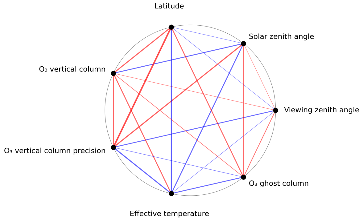
Figure 1: Map of correlation graph for 2023-10-06 to 2023-10-08.
