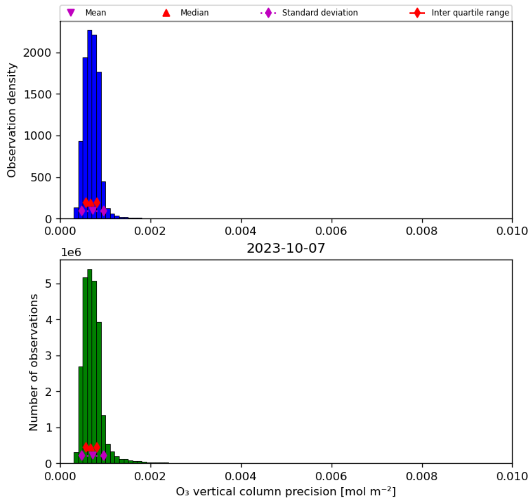
Figure 22: Histogram of “O 3 vertical column precision” for 2023-10-06 to 2023-10-08
