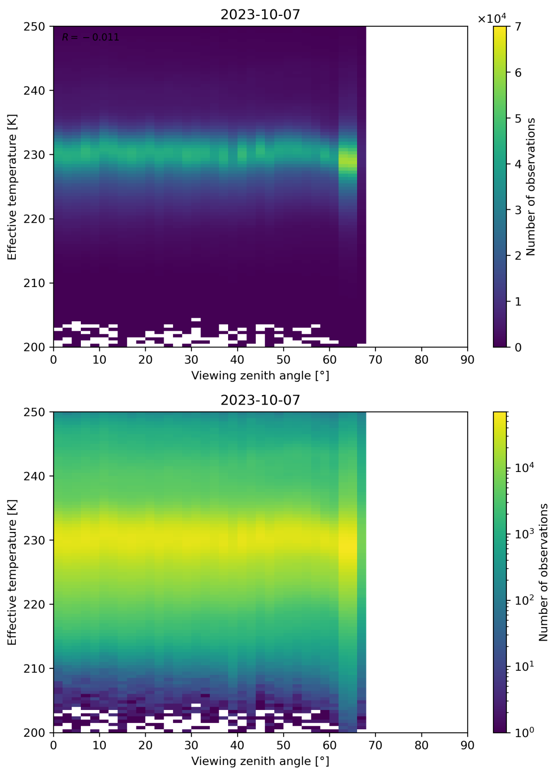
Figure 50: Scatter density plot of “Viewing zenith angle” against “Effective temperature” for 2023-10-06 to 2023-10-08.
