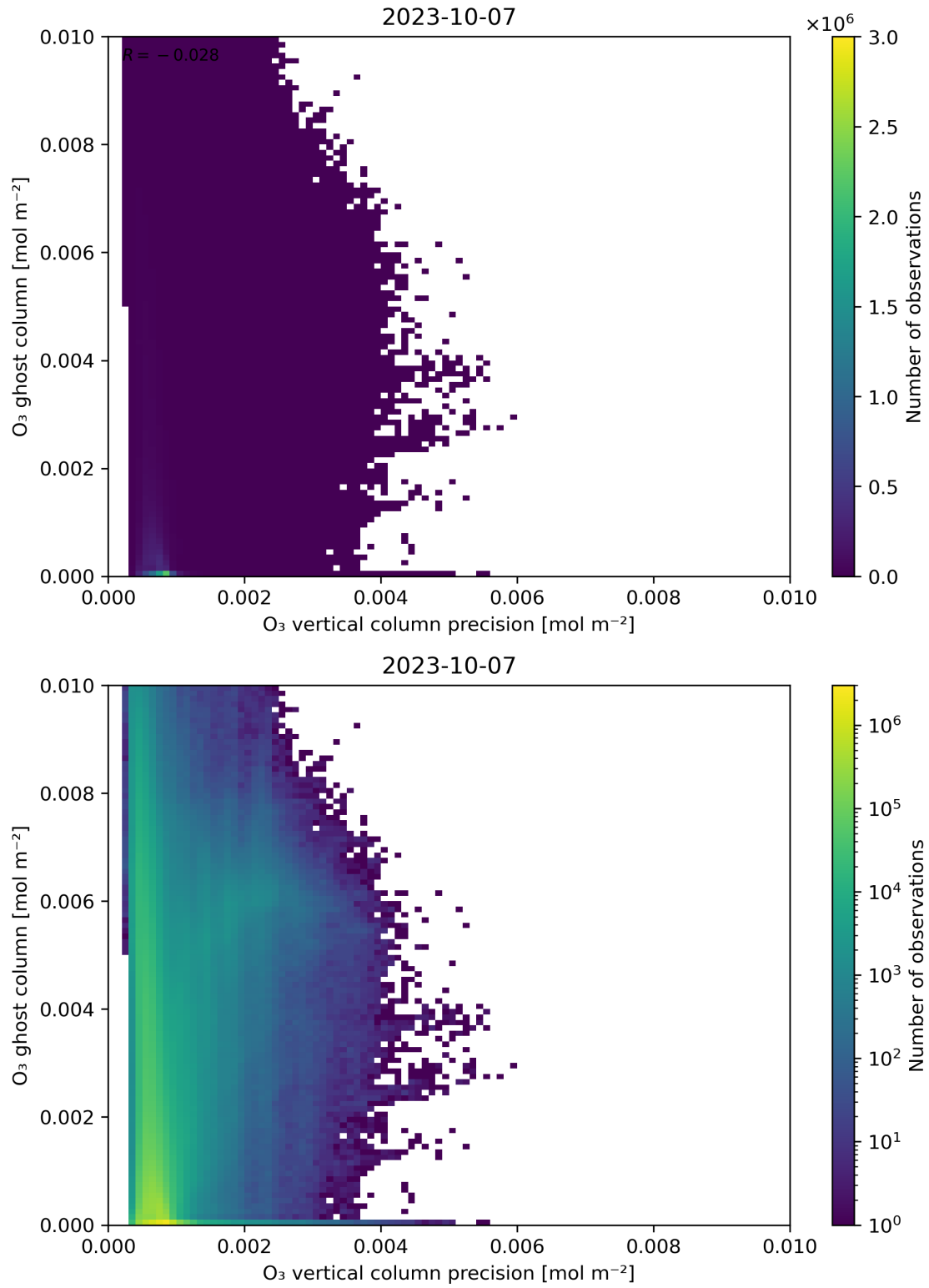
Figure 43: Scatter density plot of “ \text{O}_3 vertical column precision” against “ \text{O}_3 ghost column” for 2023-10-06 to 2023-10-08.
