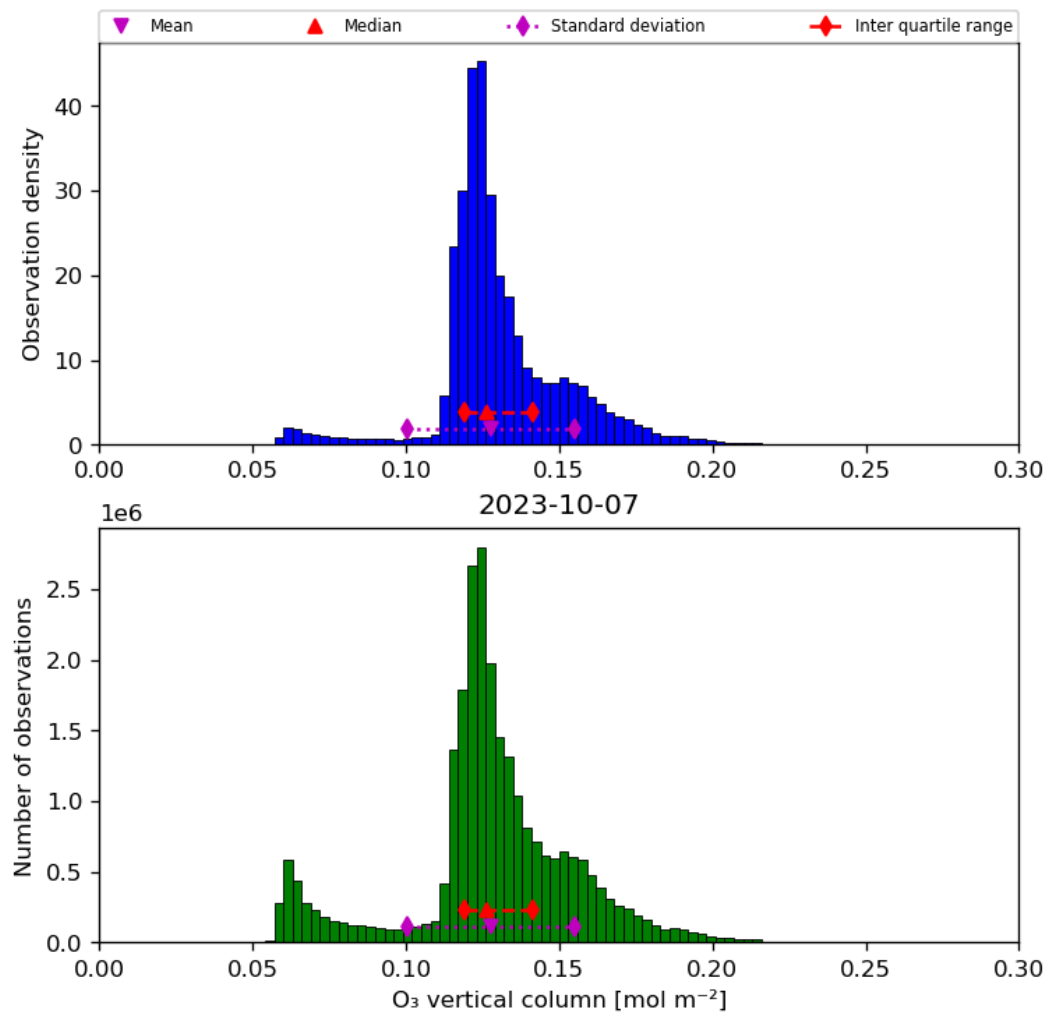
Figure 21: Histogram of “O 3 vertical column” for 2023-10-06 to 2023-10-08
