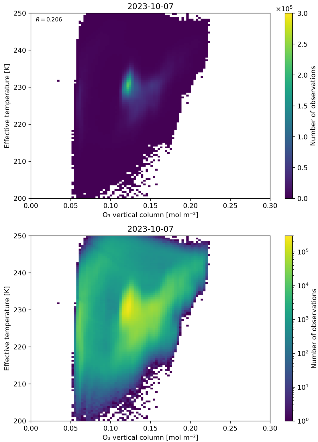
Figure 39: Scatter density plot of “O 3 vertical column” against “Effective temperature” for 2023-10-06 to 2023-10-08.
