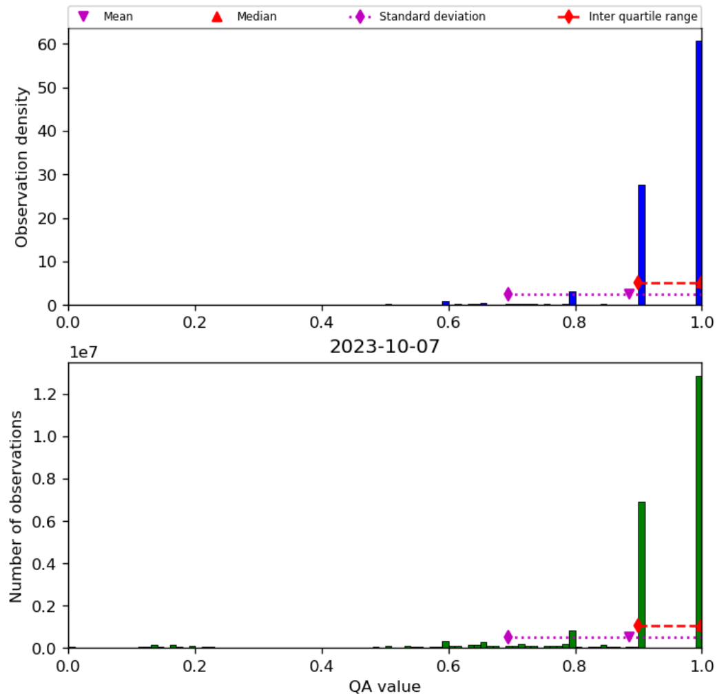
Figure 20: Histogram of “QA value” for 2023-10-06 to 2023-10-08
