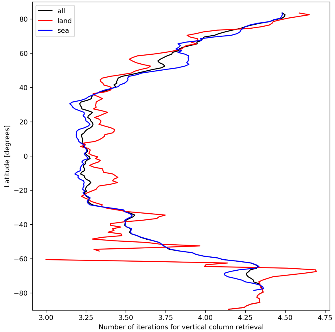
Figure 19: Zonal average of “Number of iterations for vertical column retrieval” for 2023-10-06 to 2023-10-08.
