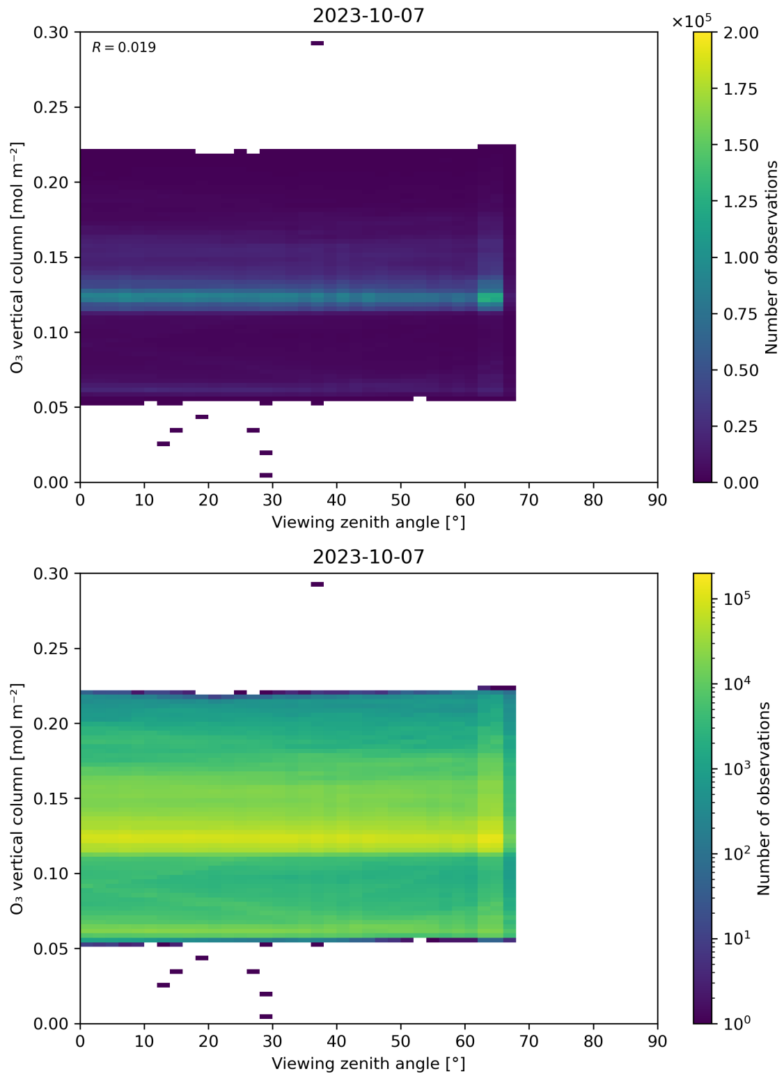
Figure 52: Scatter density plot of “Viewing zenith angle” against “O 3 vertical column” for 2023-10-06 to 2023-10-08.
