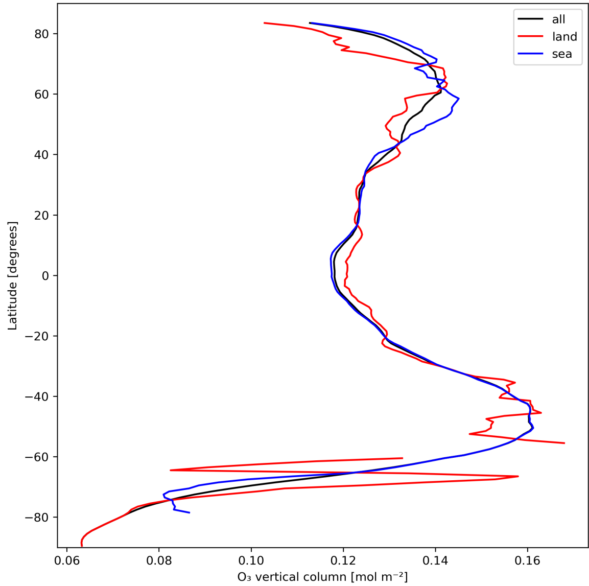
Figure 14: Zonal average of “O 3 vertical column” for 2023-10-06 to 2023-10-08.
