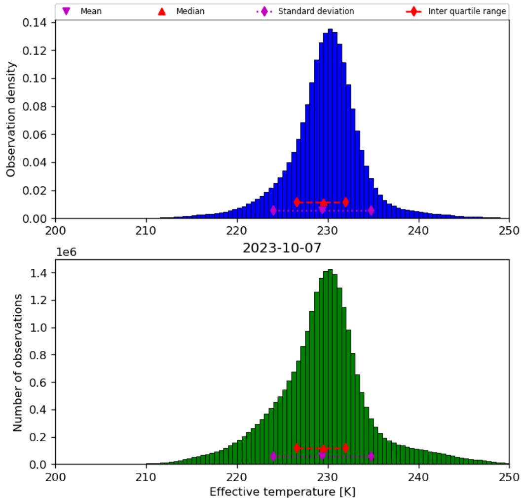
Figure 24: Histogram of “Effective temperature” for 2023-10-06 to 2023-10-08
