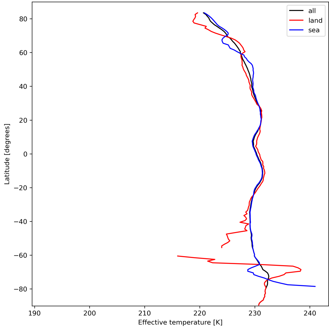
Figure 17: Zonal average of "Effective temperature" for 2023-10-06 to 2023-10-08.
