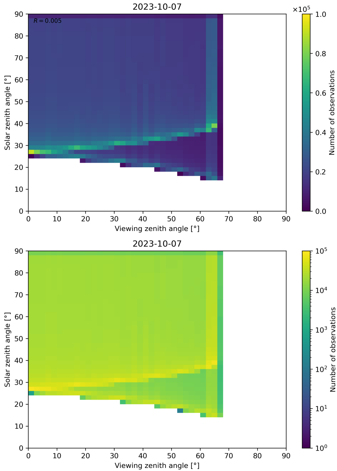
Figure 54: Scatter density plot of “Viewing zenith angle” against “Solar zenith angle” for 2023-10-06 to 2023-10-08.
