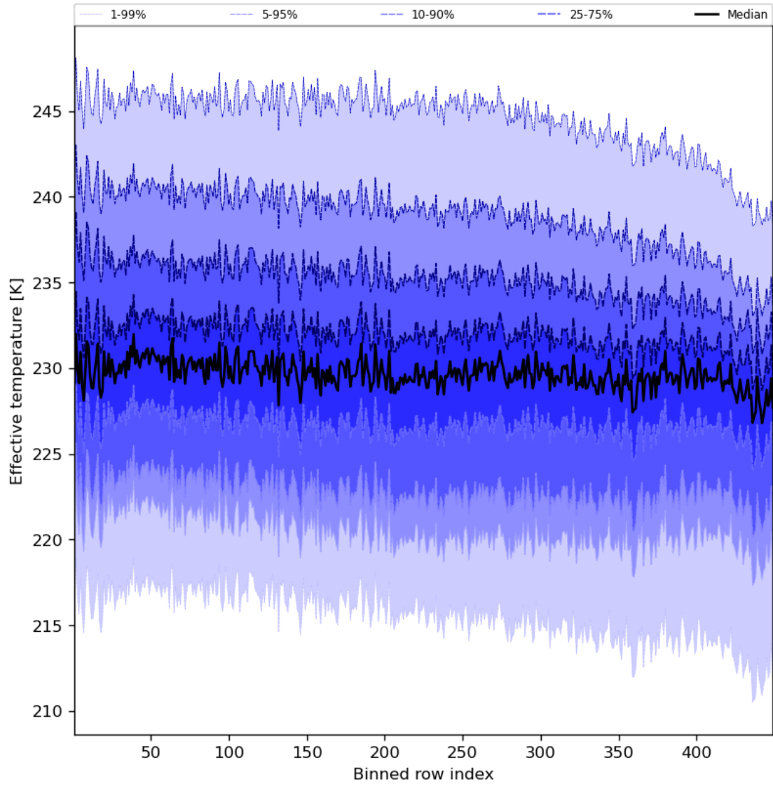
Figure 31: Along track statistics of “Effective temperature” for 2023-10-06 to 2023-10-08
