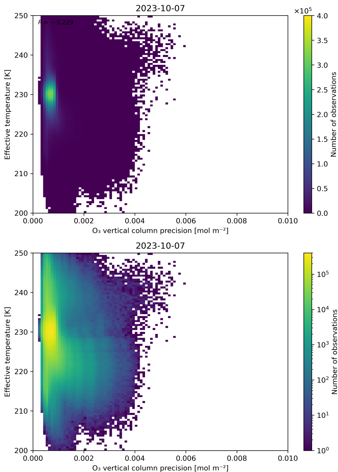
Figure 42: Scatter density plot of “O 3 vertical column precision” against “Effective temperature” for 2023-10-06 to 2023-10-08.
