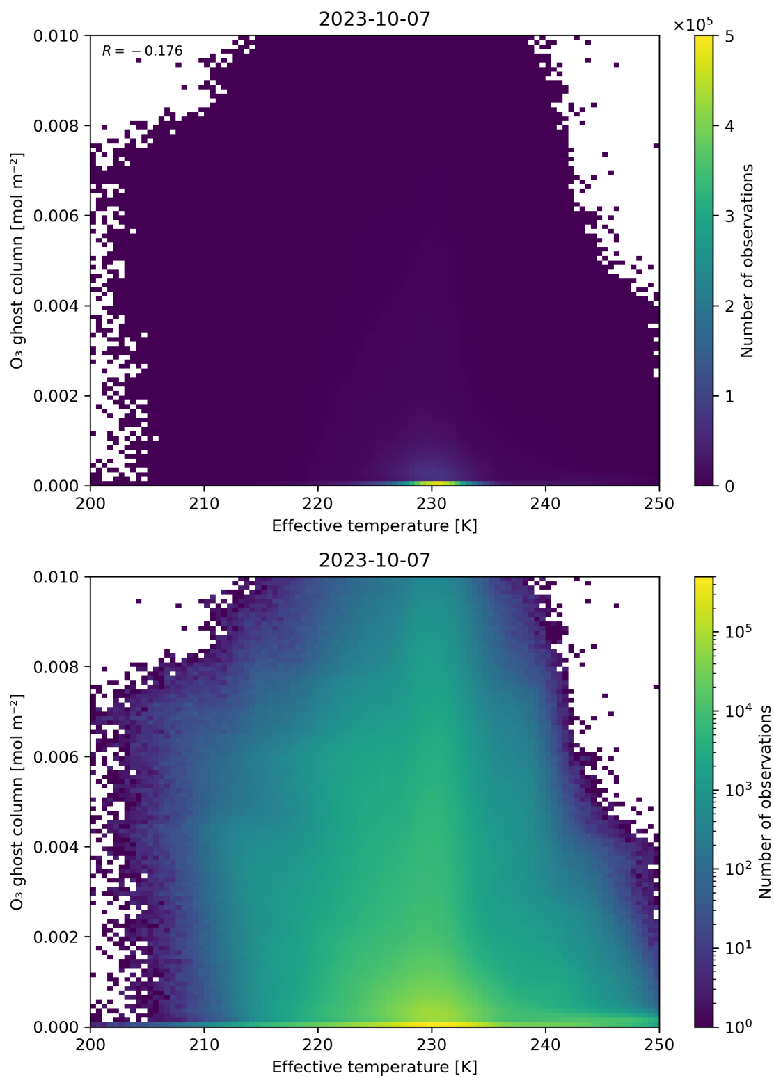
Figure 38: Scatter density plot of “Effective temperature” against “O 3 ghost column” for 2023-10-06 to 2023-10-08.
