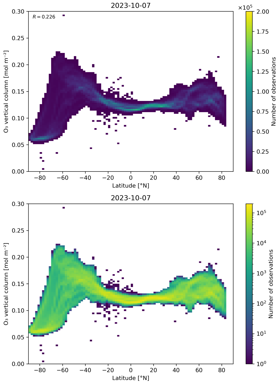
Figure 36: Scatter density plot of “Latitude” against “O 3 vertical column” for 2023-10-06 to 2023-10-08.
