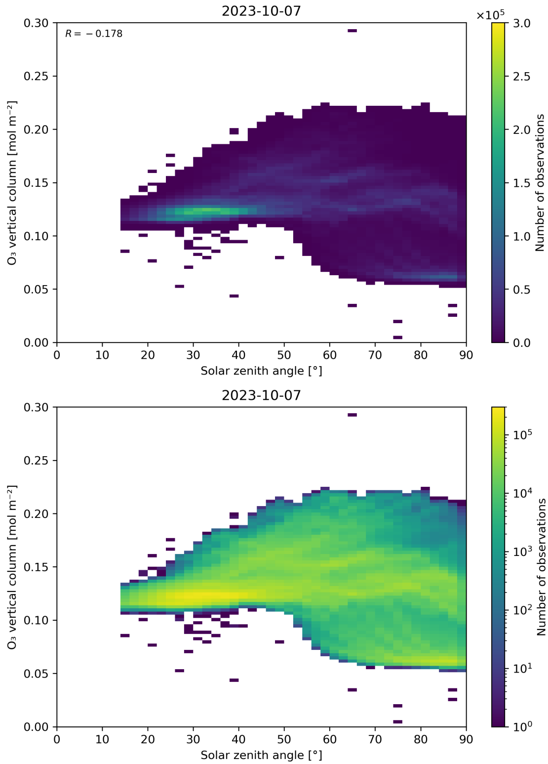
Figure 47: Scatter density plot of “Solar zenith angle” against “O 3 vertical column” for 2023-10-06 to 2023-10-08.
