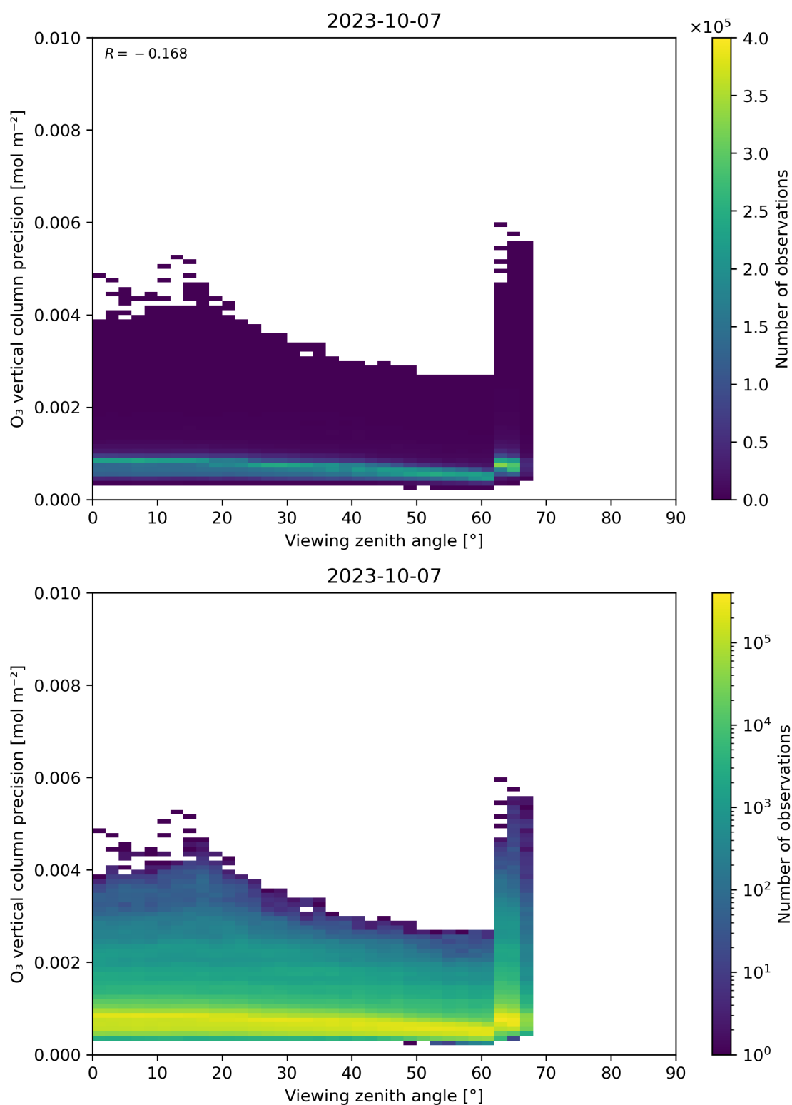
Figure 53: Scatter density plot of “Viewing zenith angle” against “O 3 vertical column precision” for 2023-10-06 to 2023-10-08.
