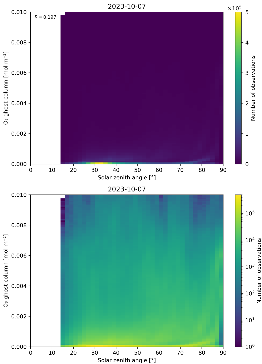
Figure 46: Scatter density plot of “Solar zenith angle” against “O 3 ghost column” for 2023-10-06 to 2023-10-08.
