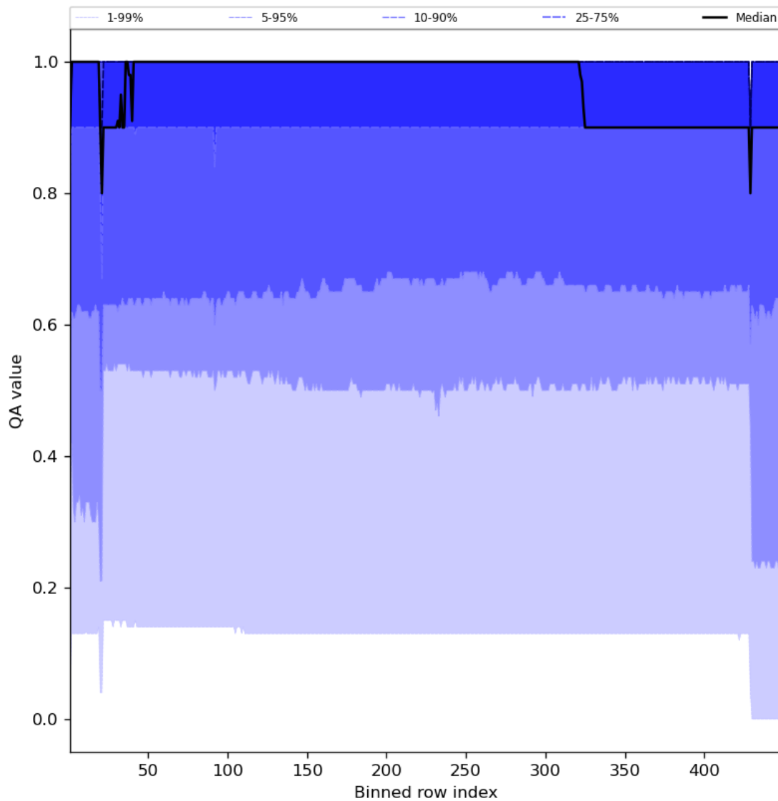
Figure 27: Along track statistics of “QA value” for 2023-10-06 to 2023-10-08
