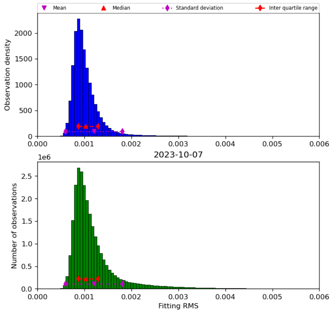
Figure 23: Histogram of “Fitting RMS” for 2023-10-06 to 2023-10-08
