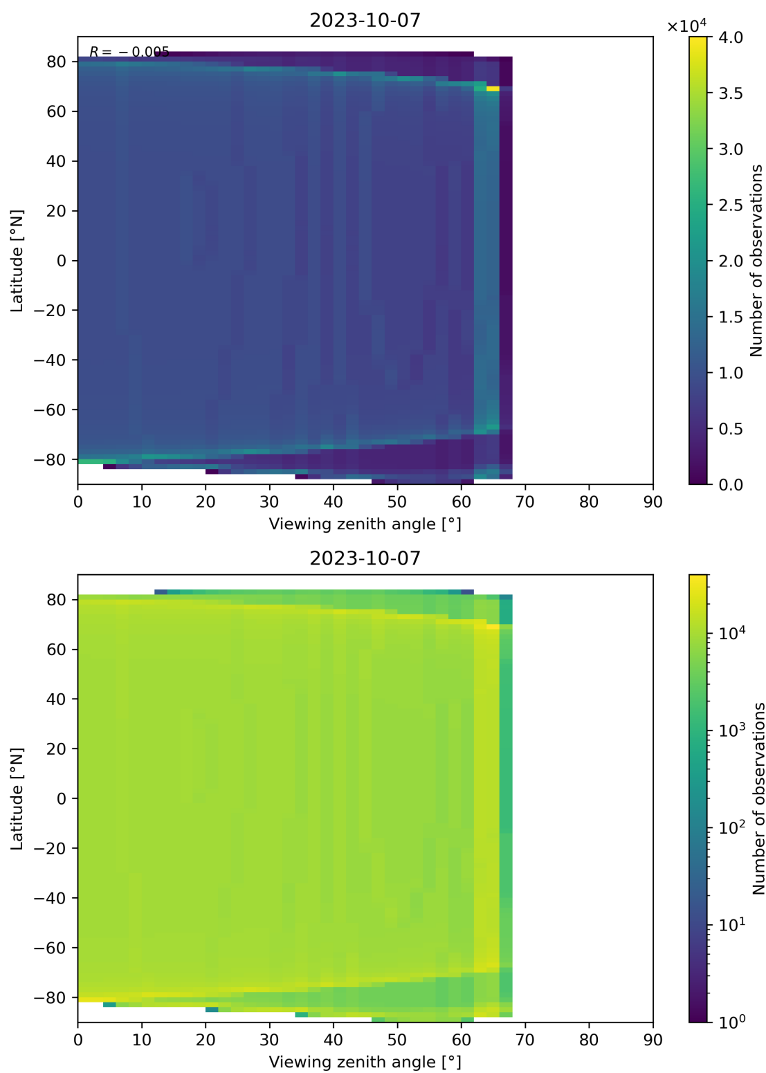
Figure 49: Scatter density plot of “Viewing zenith angle” against “Latitude” for 2023-10-06 to 2023-10-08.
