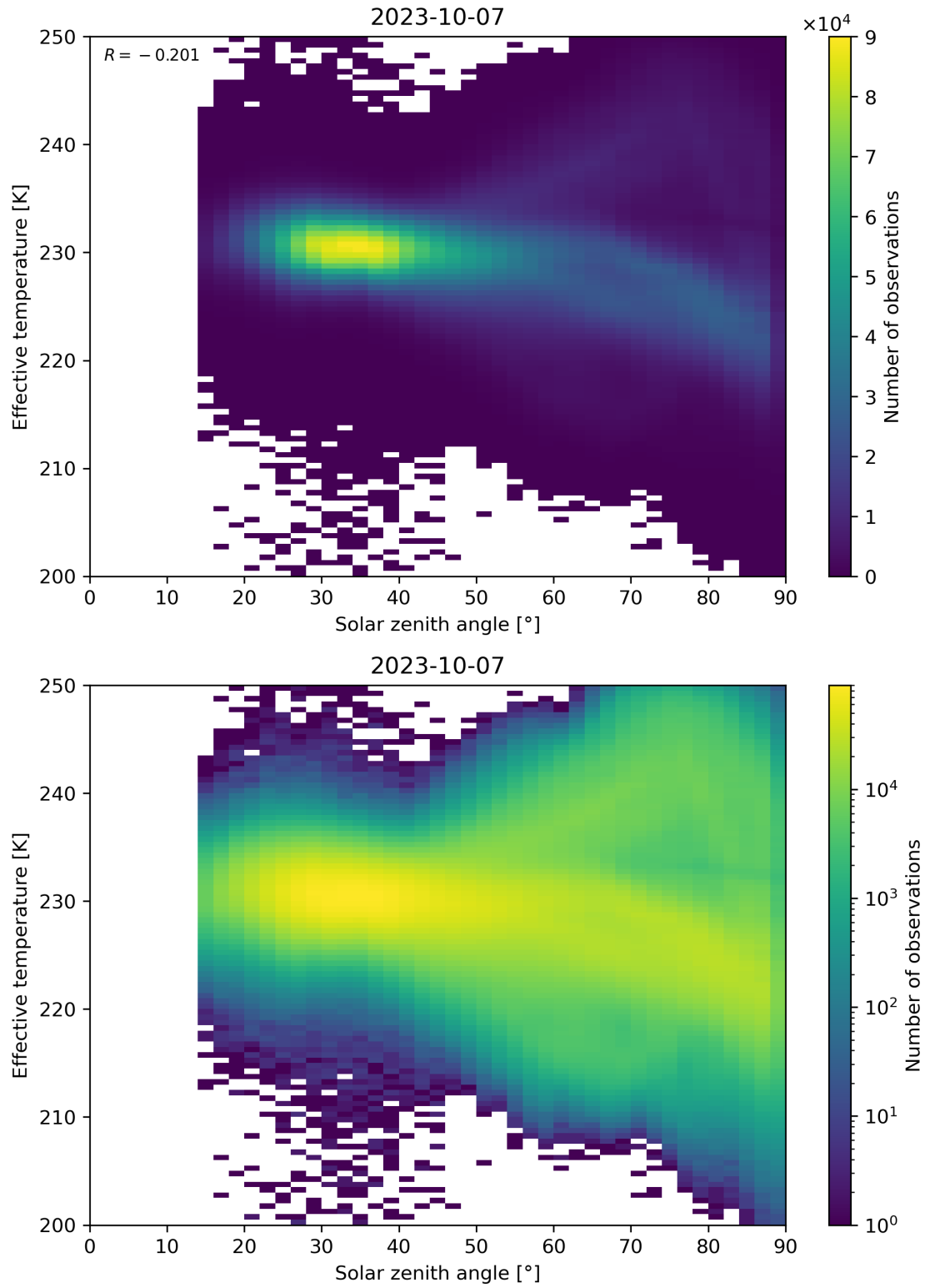
Figure 45: Scatter density plot of “Solar zenith angle” against “Effective temperature” for 2023-10-06 to 2023-10-08.
