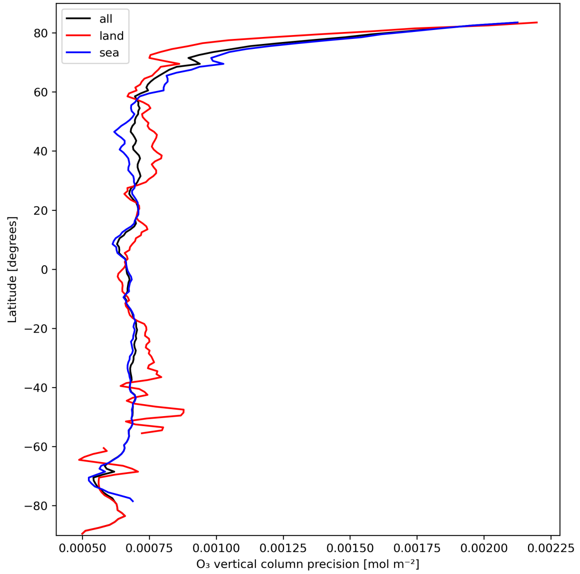
Figure 15: Zonal average of “O 3 vertical column precision” for 2023-10-06 to 2023-10-08.
