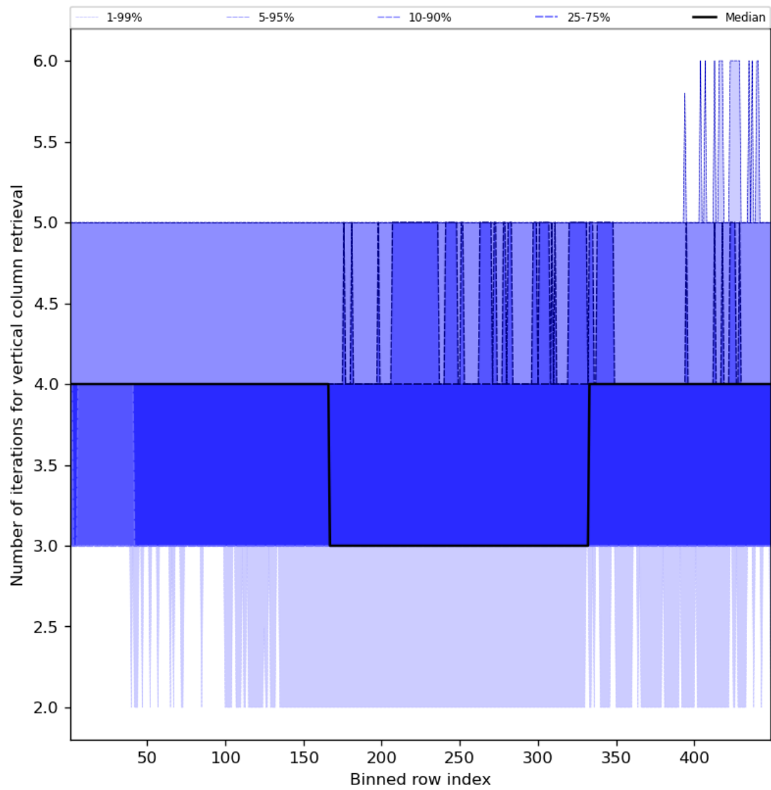
Figure 33: Along track statistics of “Number of iterations for vertical column retrieval” for 2023-10-06 to 2023-10-08
