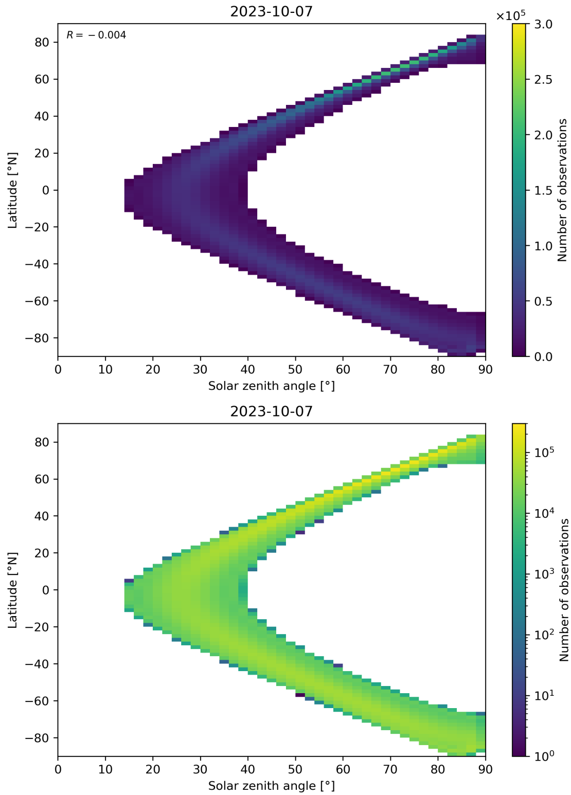
Figure 44: Scatter density plot of “Solar zenith angle” against “Latitude” for 2023-10-06 to 2023-10-08.
