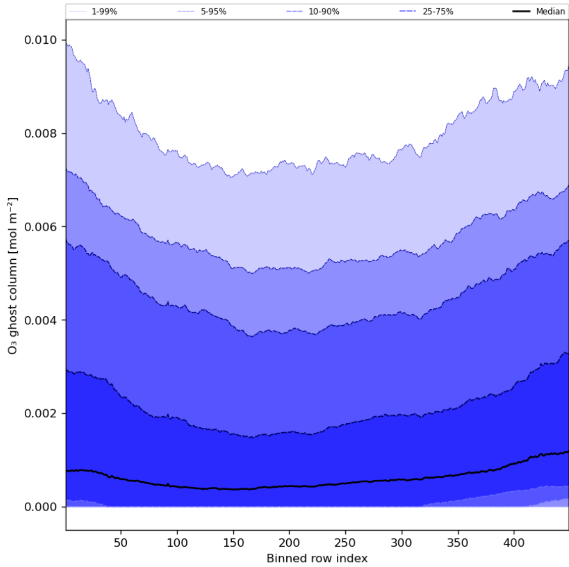
Figure 32: Along track statistics of “O 3 ghost column” for 2023-10-06 to 2023-10-08
