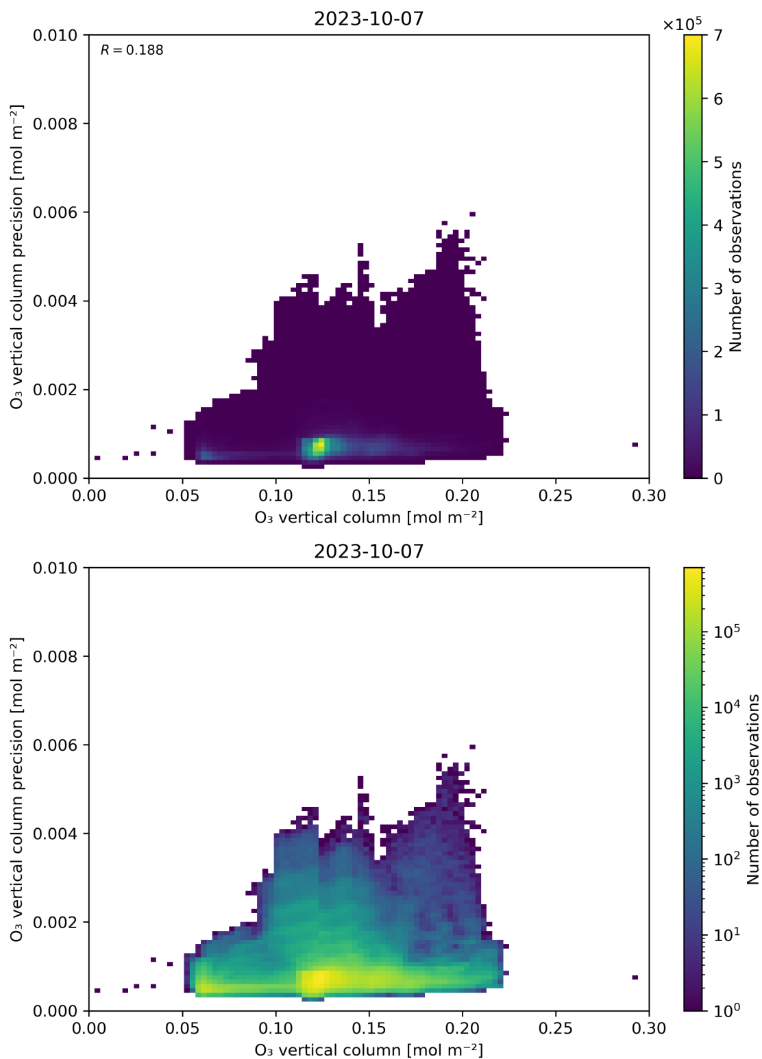
Figure 41: Scatter density plot of “O 3 vertical column” against “O 3 vertical column precision” for 2023-10-06 to 2023-10-08.
