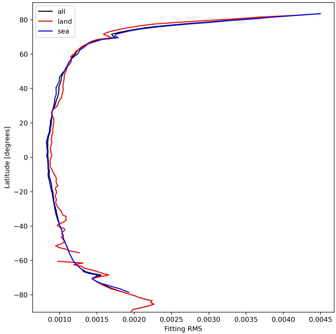
Figure 16: Zonal average of “Fitting RMS” for 2023-10-06 to 2023-10-08.
