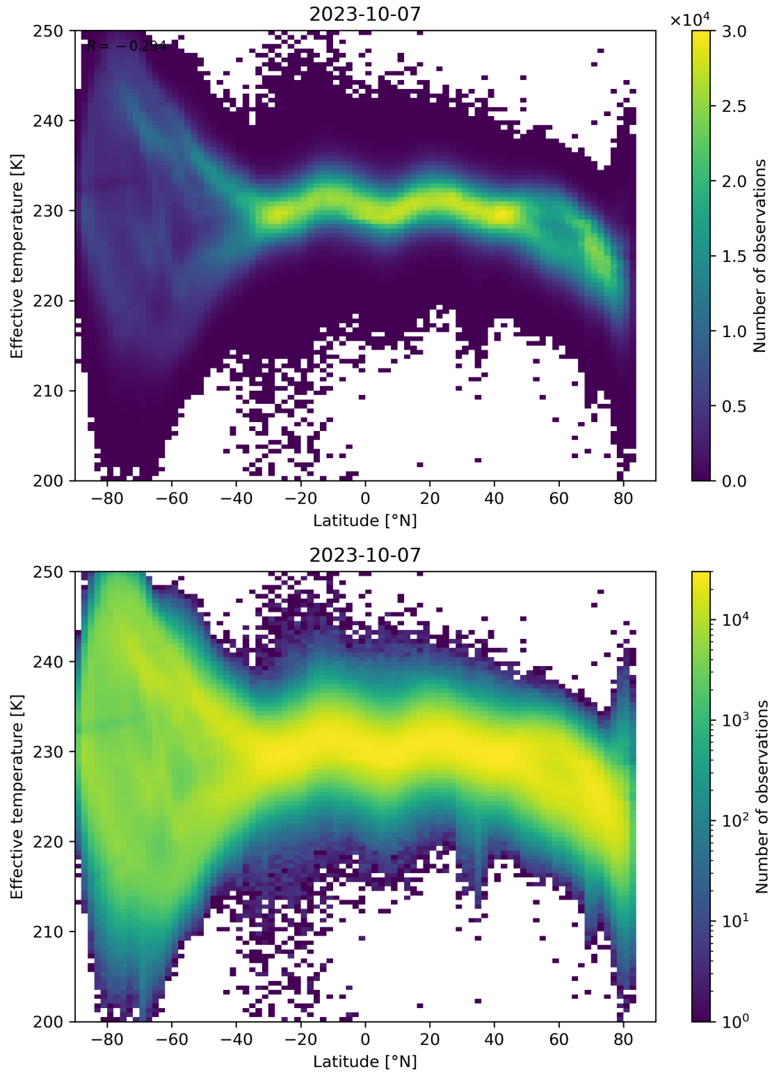
Figure 34: Scatter density plot of “Latitude” against “Effective temperature” for 2023-10-06 to 2023-10-08.
