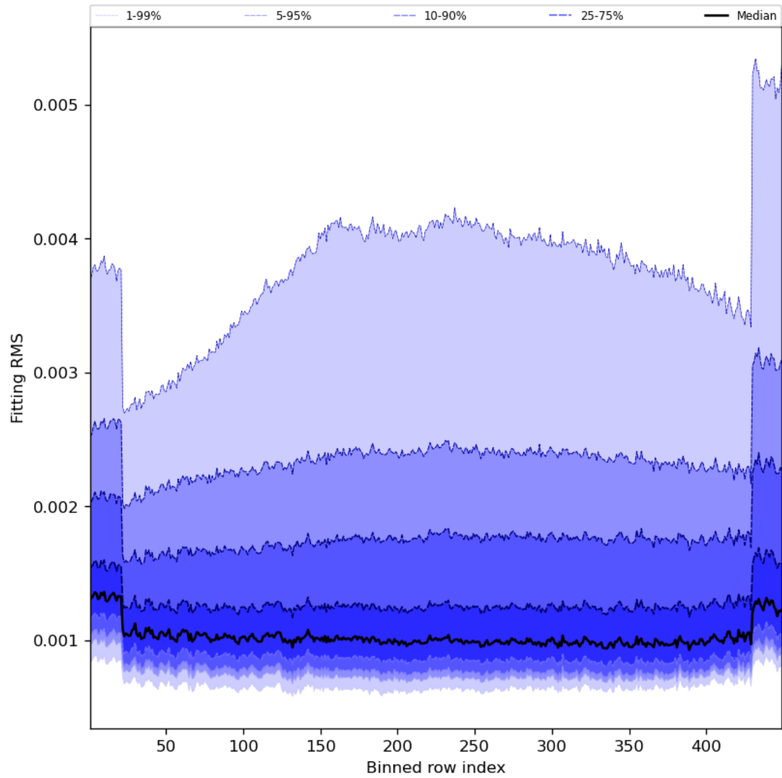
Figure 30: Along track statistics of “Fitting RMS” for 2023-10-06 to 2023-10-08
