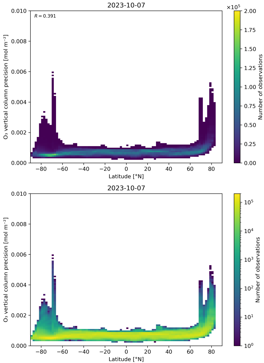
Figure 37: Scatter density plot of “Latitude” against “O 3 vertical column precision” for 2023-10-06 to 2023-10-08.
