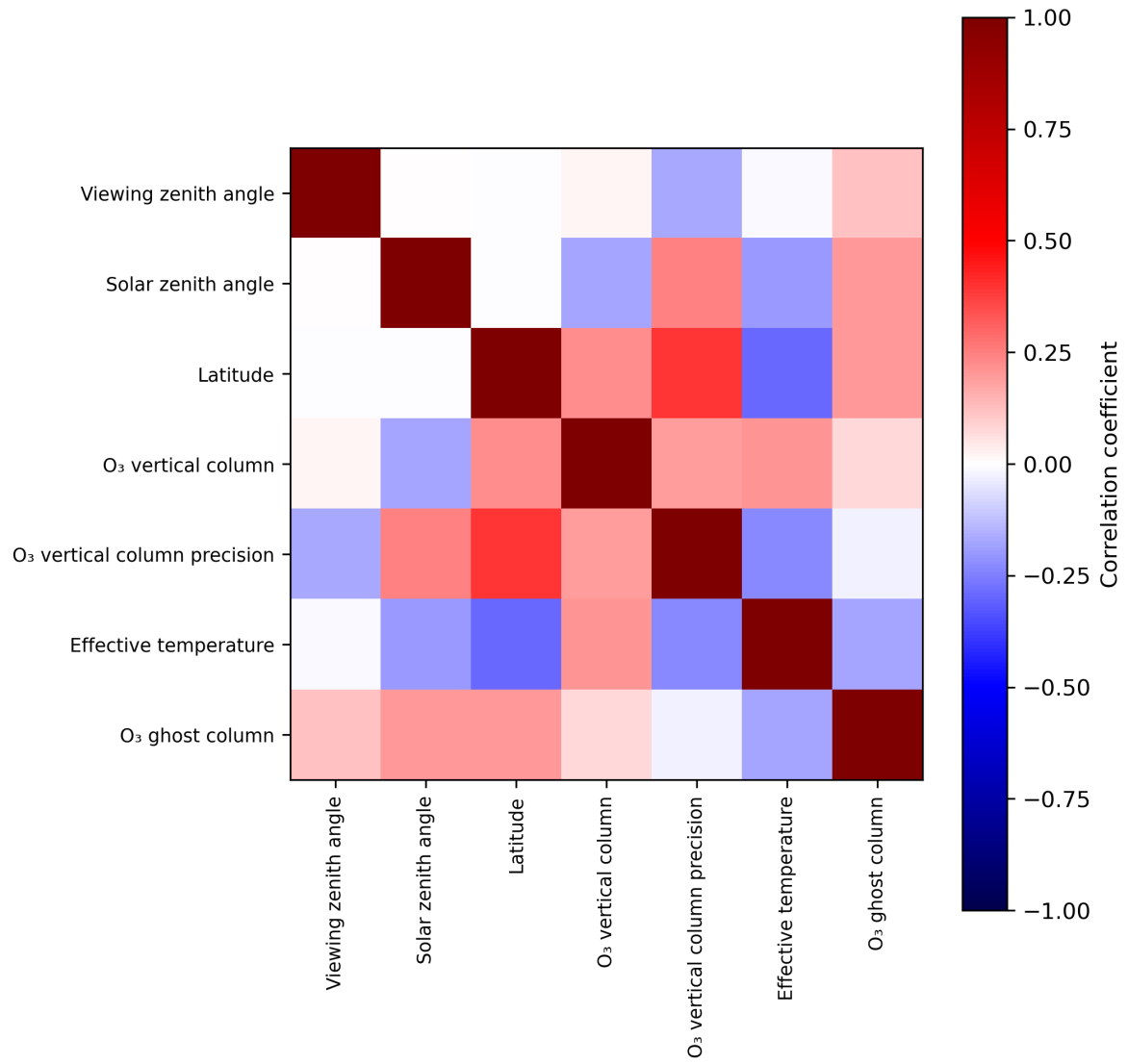
Figure 2: Map of correlation matrix for 2023-10-06 to 2023-10-08.
