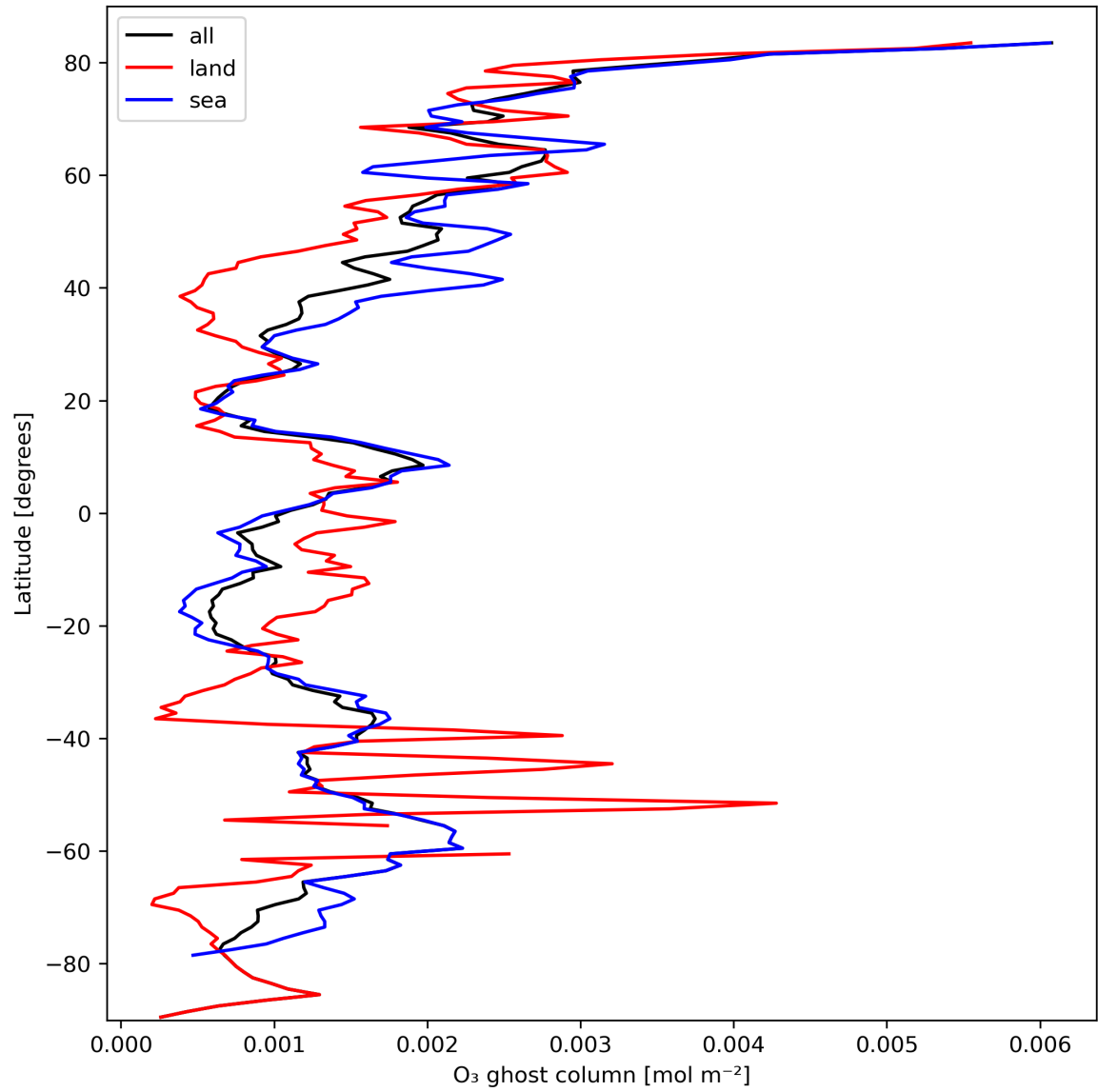
Figure 18: Zonal average of “O 3 ghost column” for 2023-10-06 to 2023-10-08.
