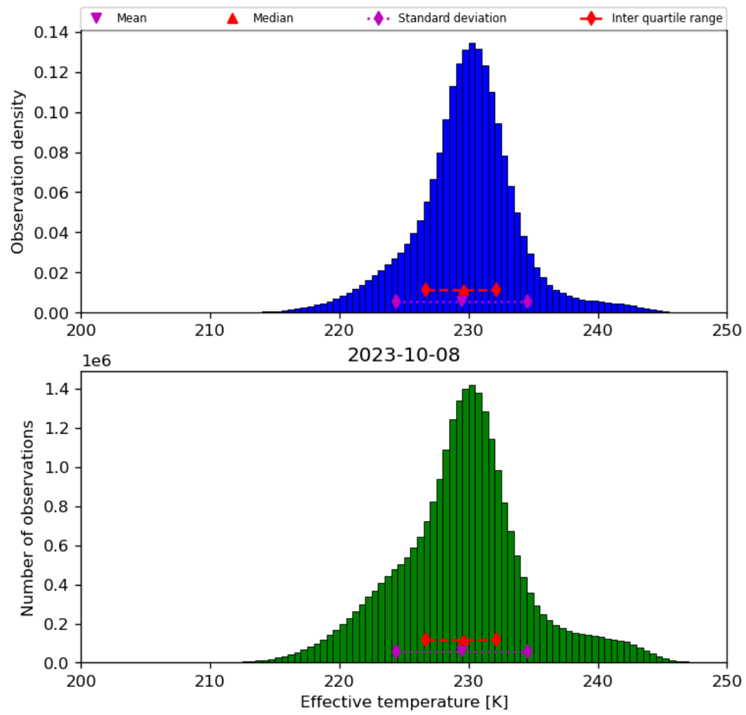
Figure 24: Histogram of “Effective temperature” for 2023-10-07 to 2023-10-09
