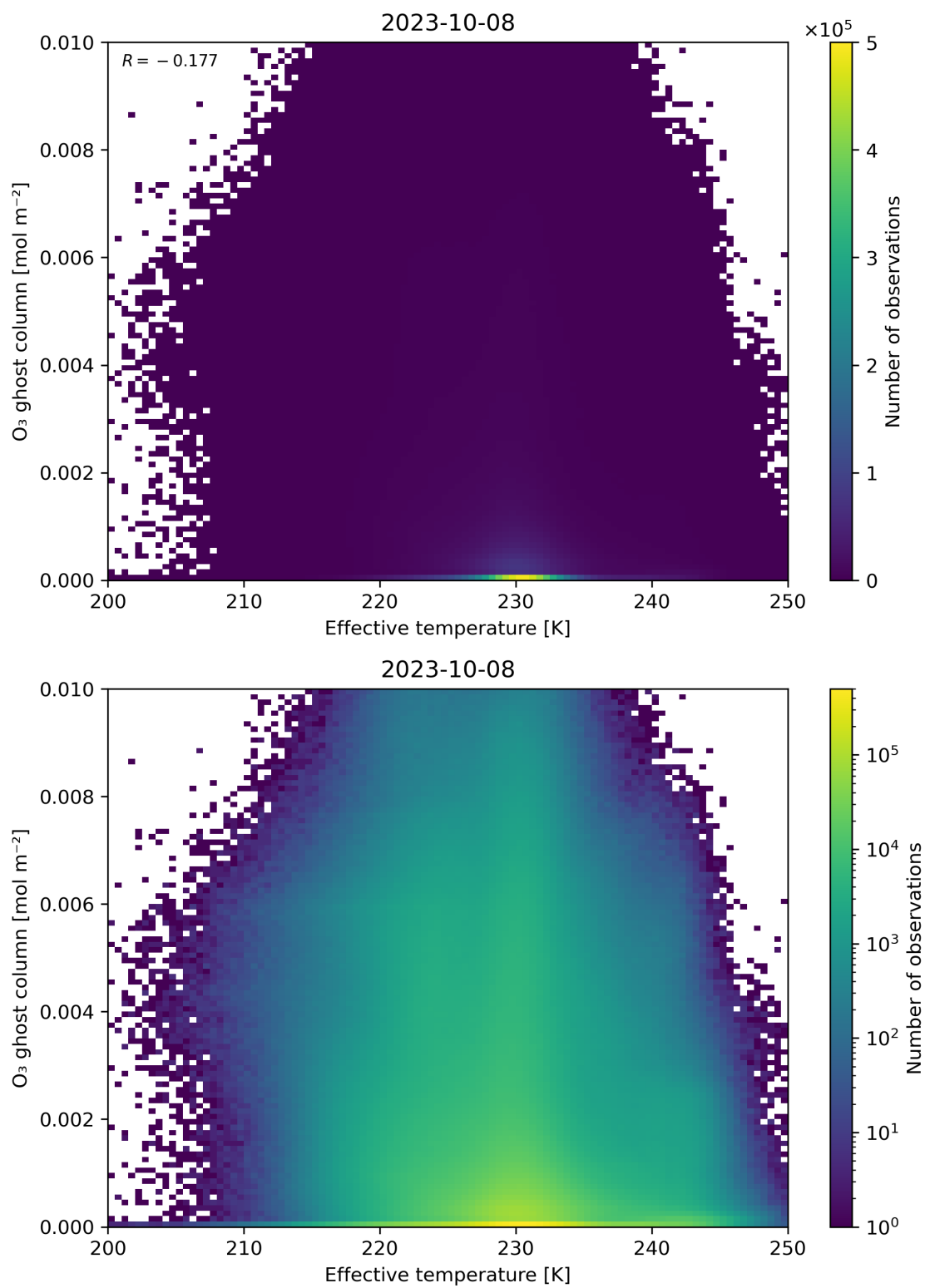
Figure 38: Scatter density plot of “Effective temperature” against “O 3 ghost column” for 2023-10-07 to 2023-10-09.
