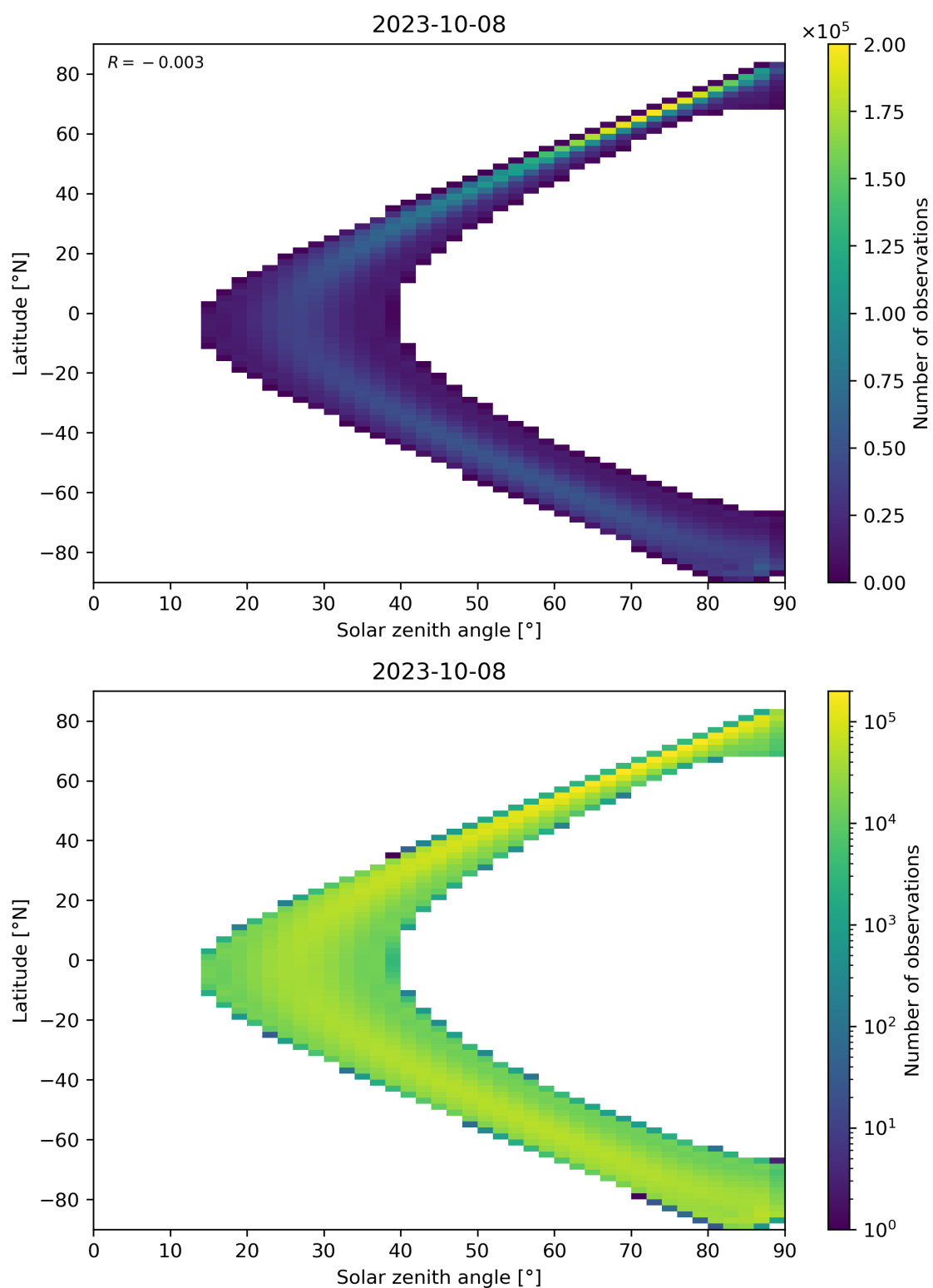
Figure 44: Scatter density plot of “Solar zenith angle” against “Latitude” for 2023-10-07 to 2023-10-09.
