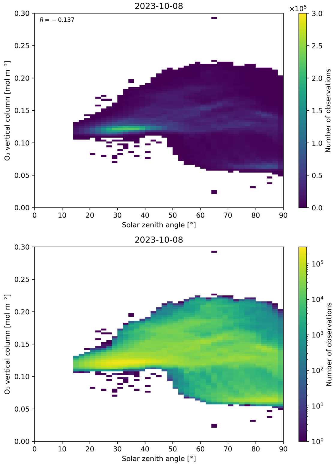
Figure 47: Scatter density plot of “Solar zenith angle” against “O 3 vertical column” for 2023-10-07 to 2023-10-09.
