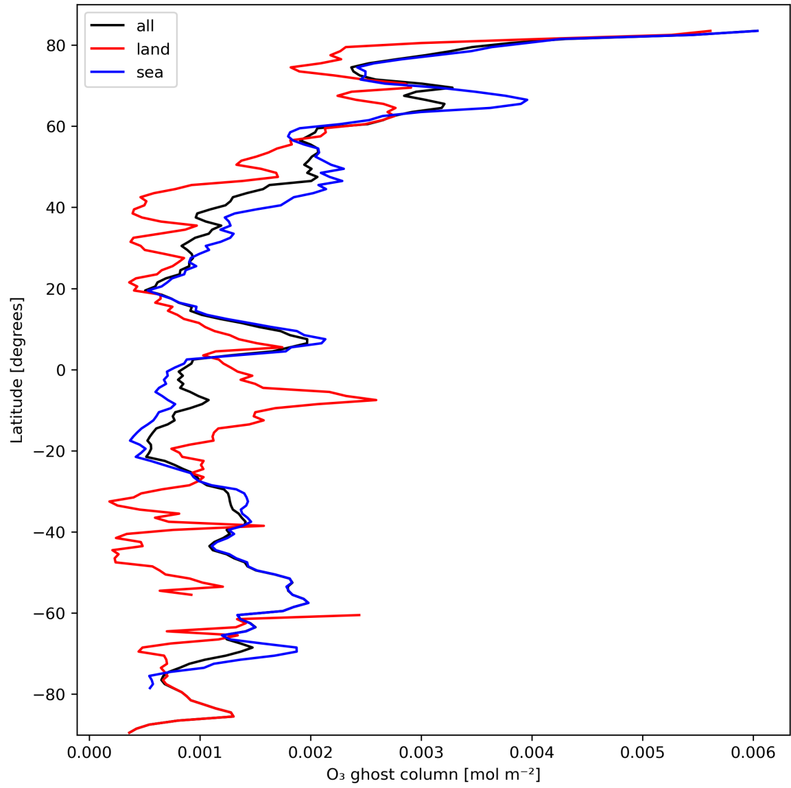
Figure 18: Zonal average of "O 3 ghost column" for 2023-10-07 to 2023-10-09.
