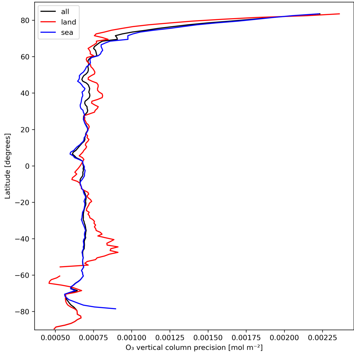
Figure 15: Zonal average of “O 3 vertical column precision” for 2023-10-07 to 2023-10-09.
