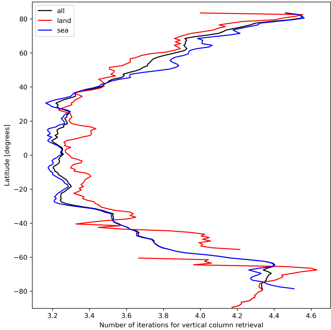
Figure 19: Zonal average of “Number of iterations for vertical column retrieval” for 2023-10-07 to 2023-10-09.
