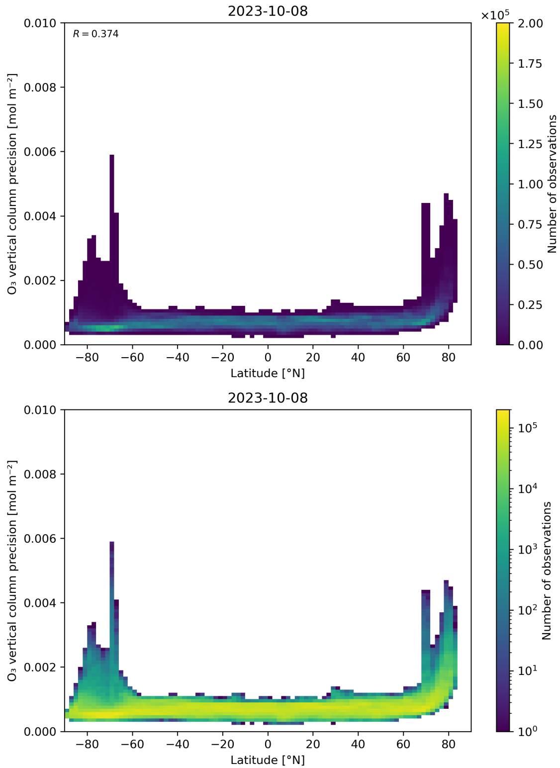
Figure 37: Scatter density plot of “Latitude” against “O 3 vertical column precision” for 2023-10-07 to 2023-10-09.
