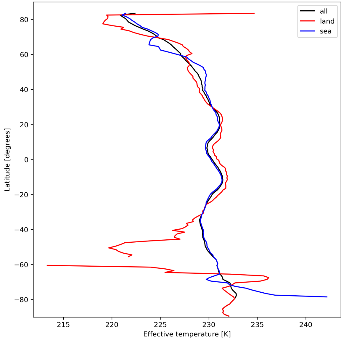
Figure 17: Zonal average of “Effective temperature” for 2023-10-07 to 2023-10-09.
