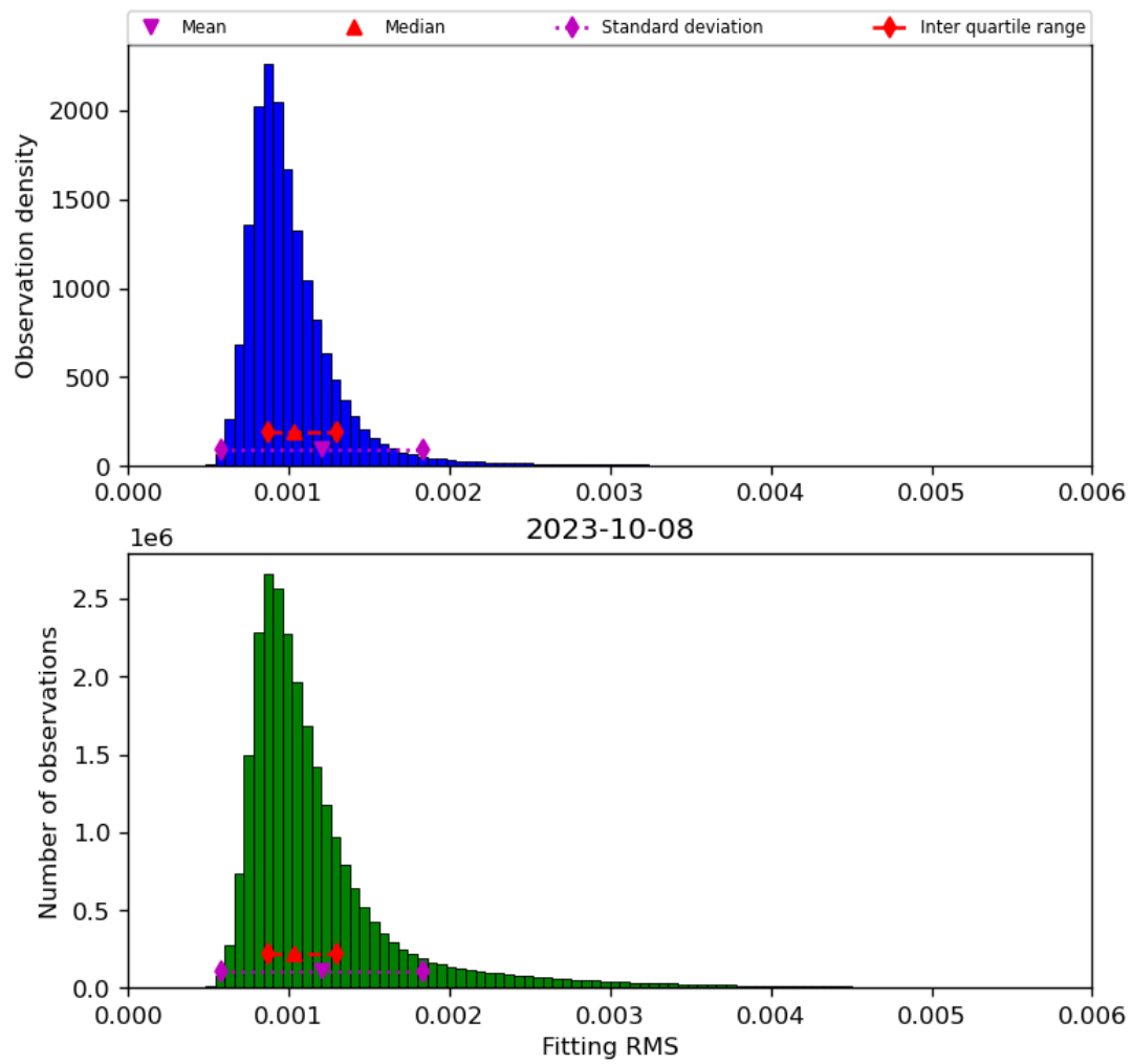
Figure 23: Histogram of “Fitting RMS” for 2023-10-07 to 2023-10-09
