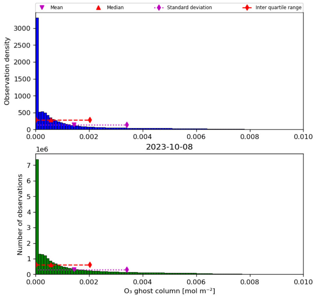
Figure 25: Histogram of “O 3 ghost column” for 2023-10-07 to 2023-10-09
