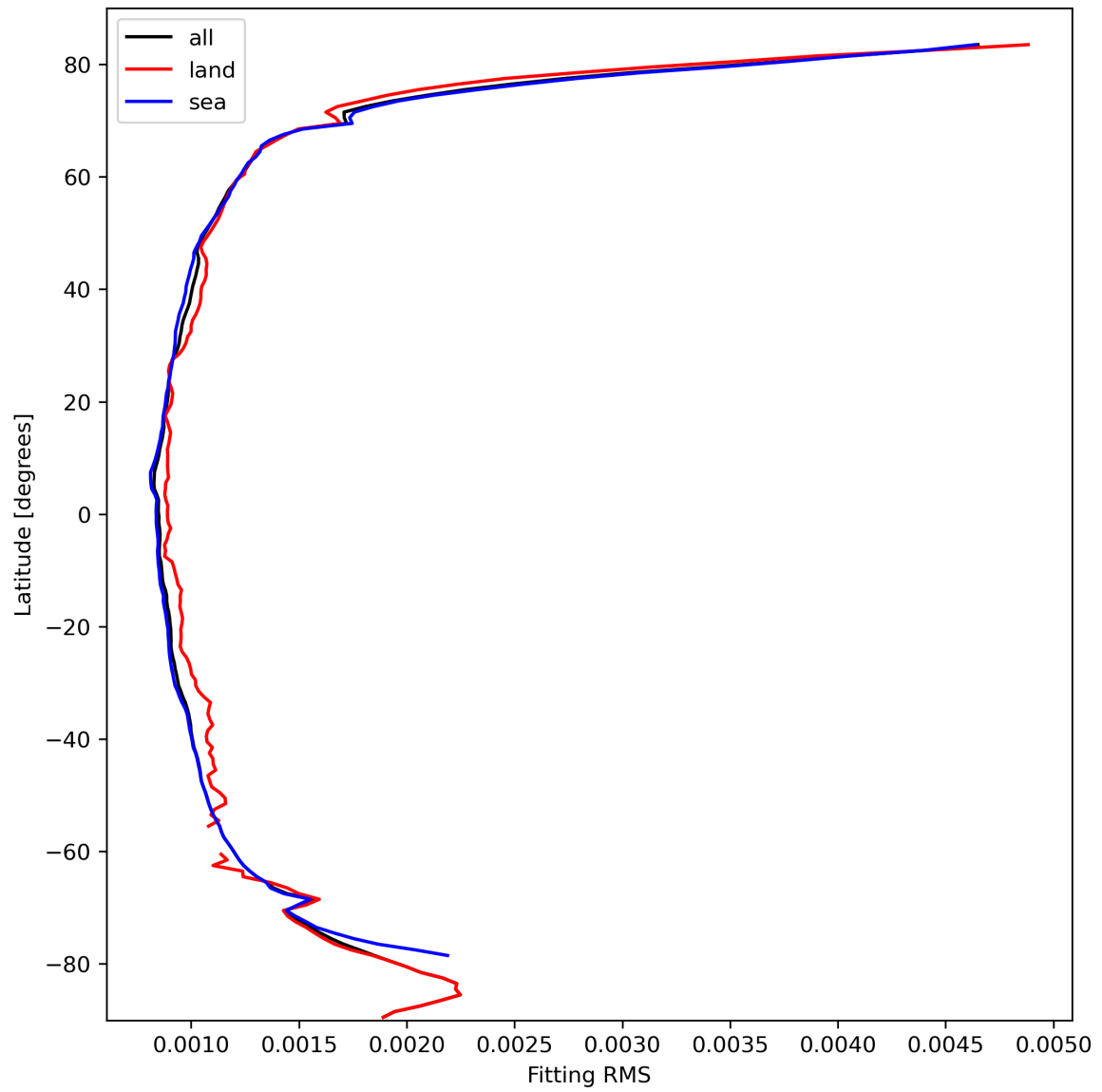
Figure 16: Zonal average of “Fitting RMS” for 2023-10-07 to 2023-10-09.
