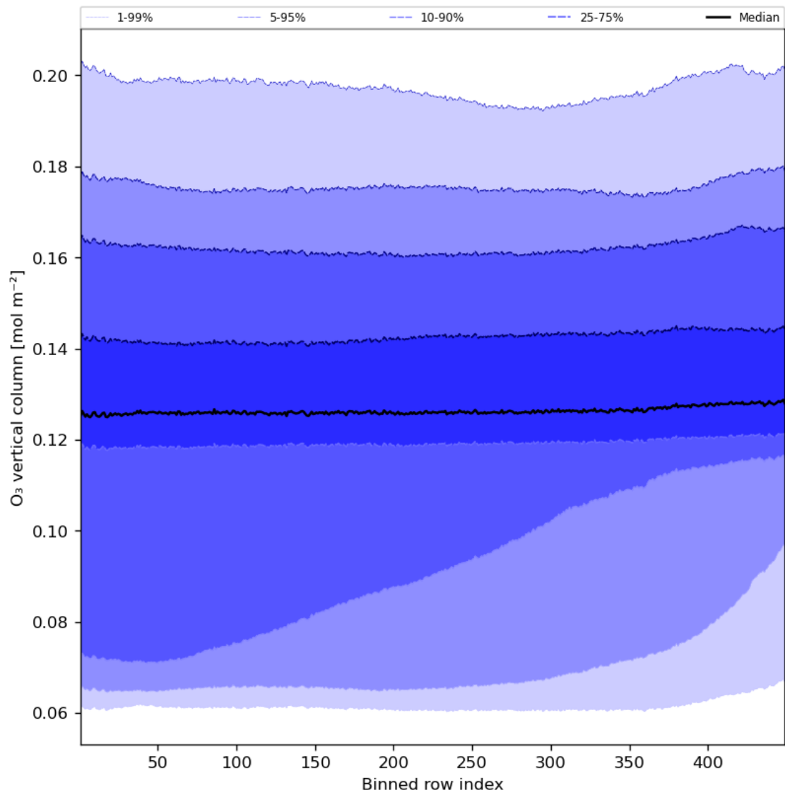
Figure 28: Along track statistics of “O 3 vertical column” for 2023-10-07 to 2023-10-09
