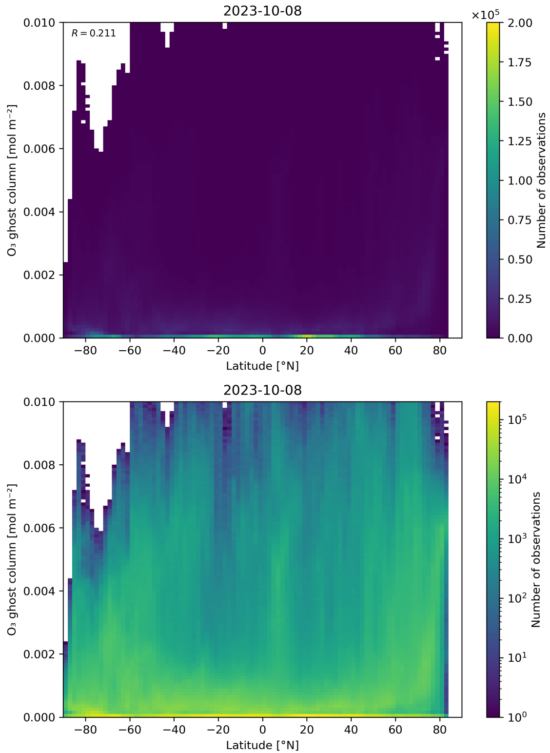
Figure 35: Scatter density plot of “Latitude” against “O 3 ghost column” for 2023-10-07 to 2023-10-09.
