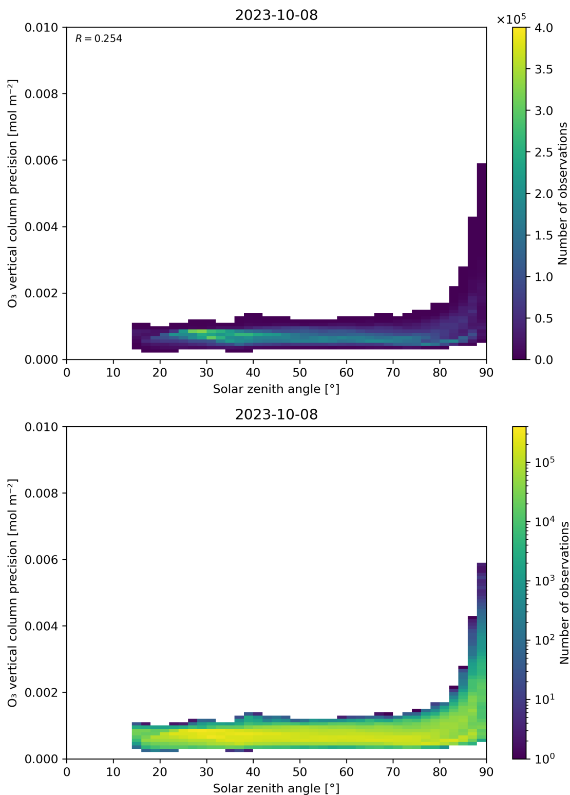
Figure 48: Scatter density plot of “Solar zenith angle” against “O 3 vertical column precision” for 2023-10-07 to 2023-10-09.
