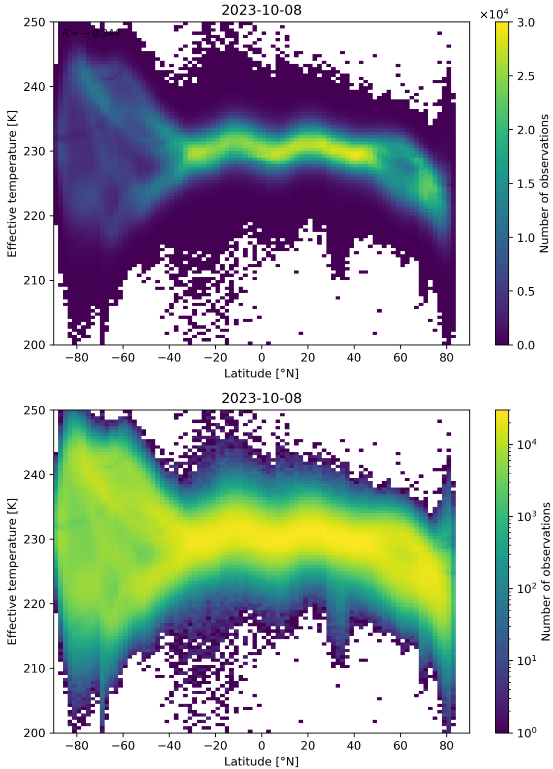
Figure 34: Scatter density plot of “Latitude” against “Effective temperature” for 2023-10-07 to 2023-10-09.
