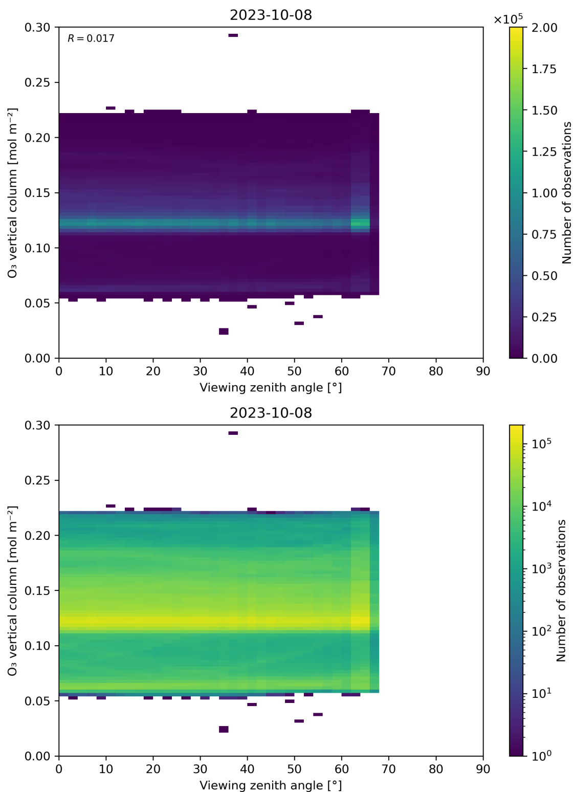
Figure 52: Scatter density plot of “Viewing zenith angle” against “O 3 vertical column” for 2023-10-07 to 2023-10-09.
