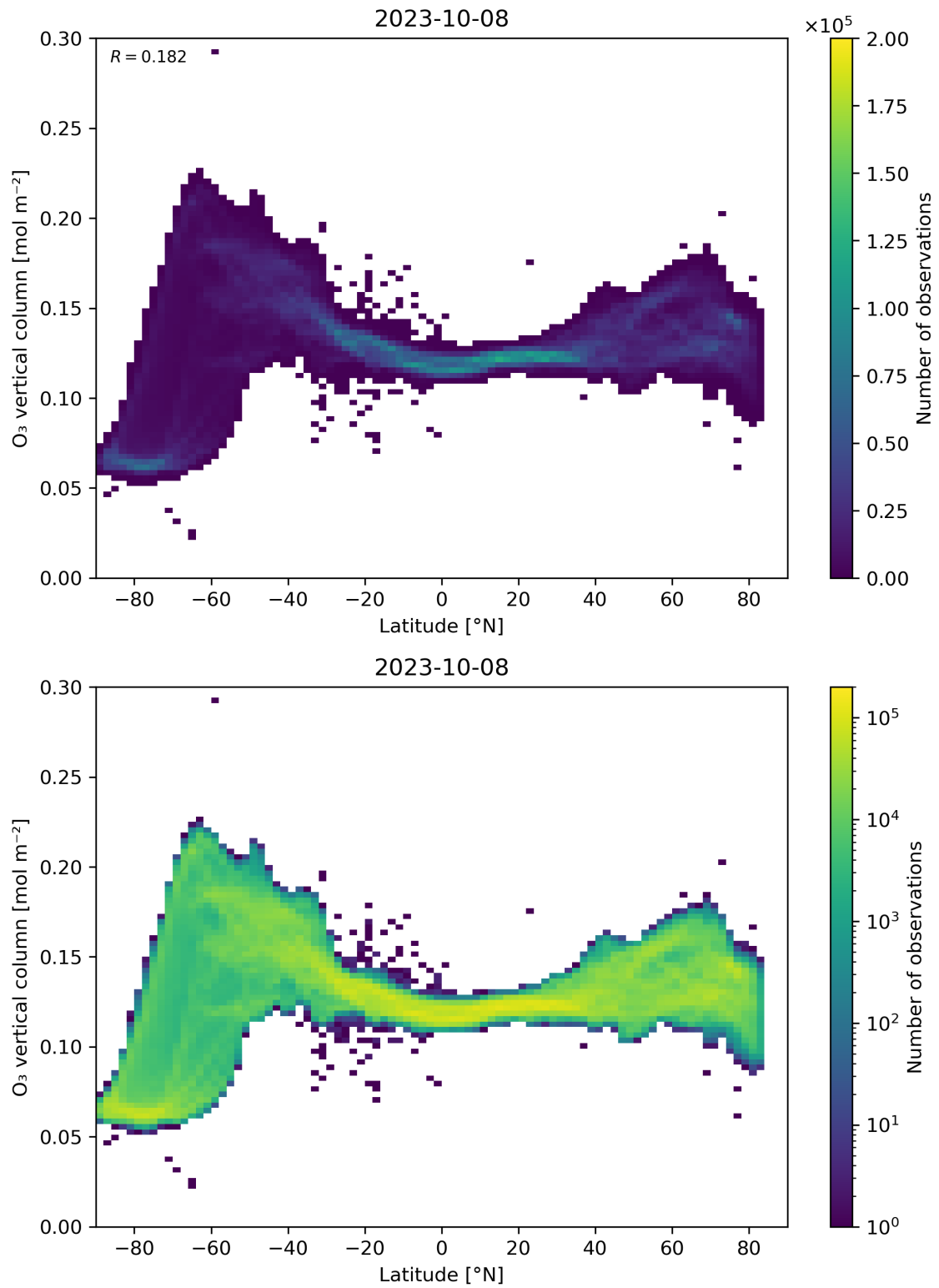
Figure 36: Scatter density plot of “Latitude” against “O 3 vertical column” for 2023-10-07 to 2023-10-09.
