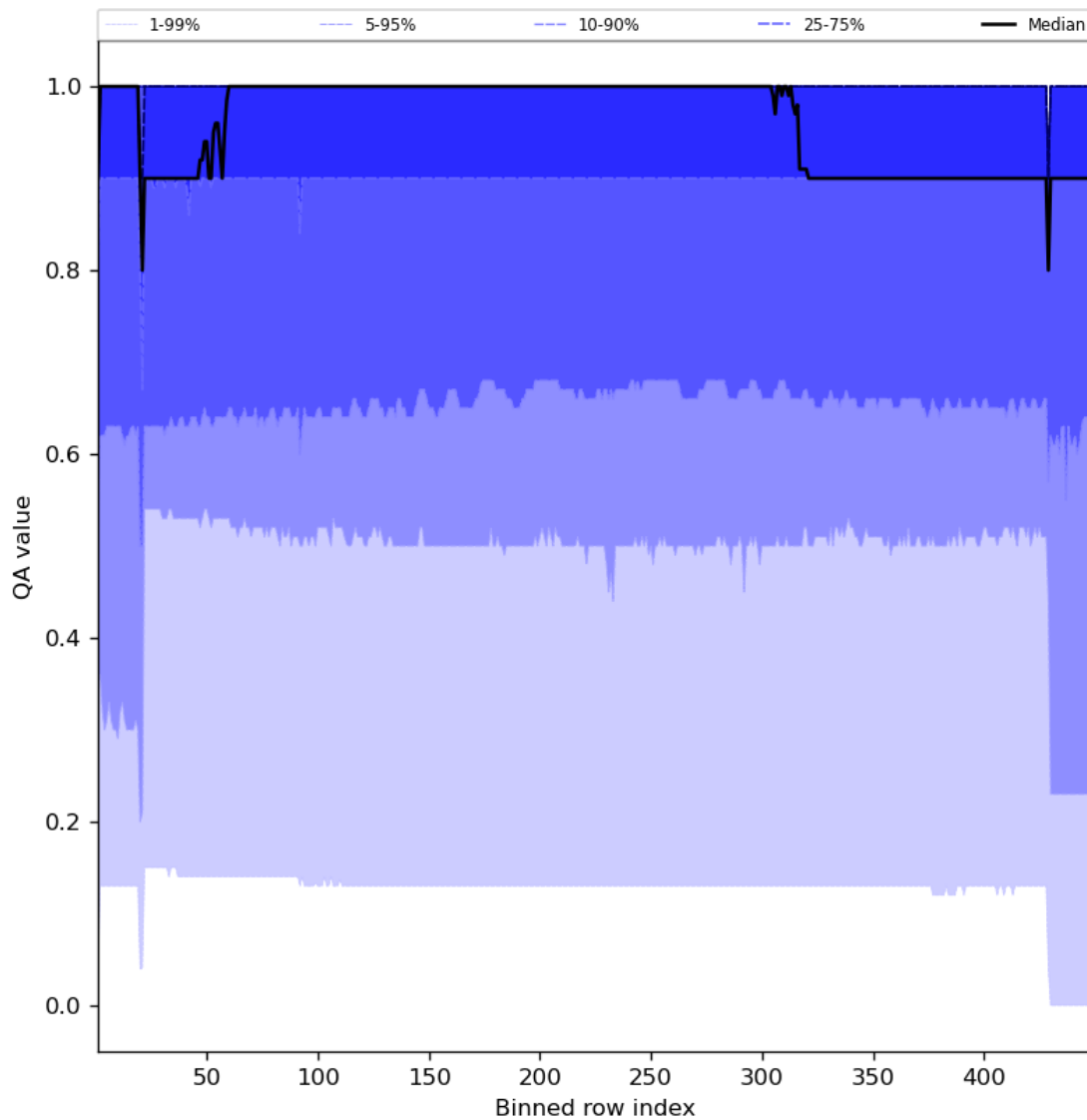
Figure 27: Along track statistics of “QA value” for 2023-10-07 to 2023-10-09
