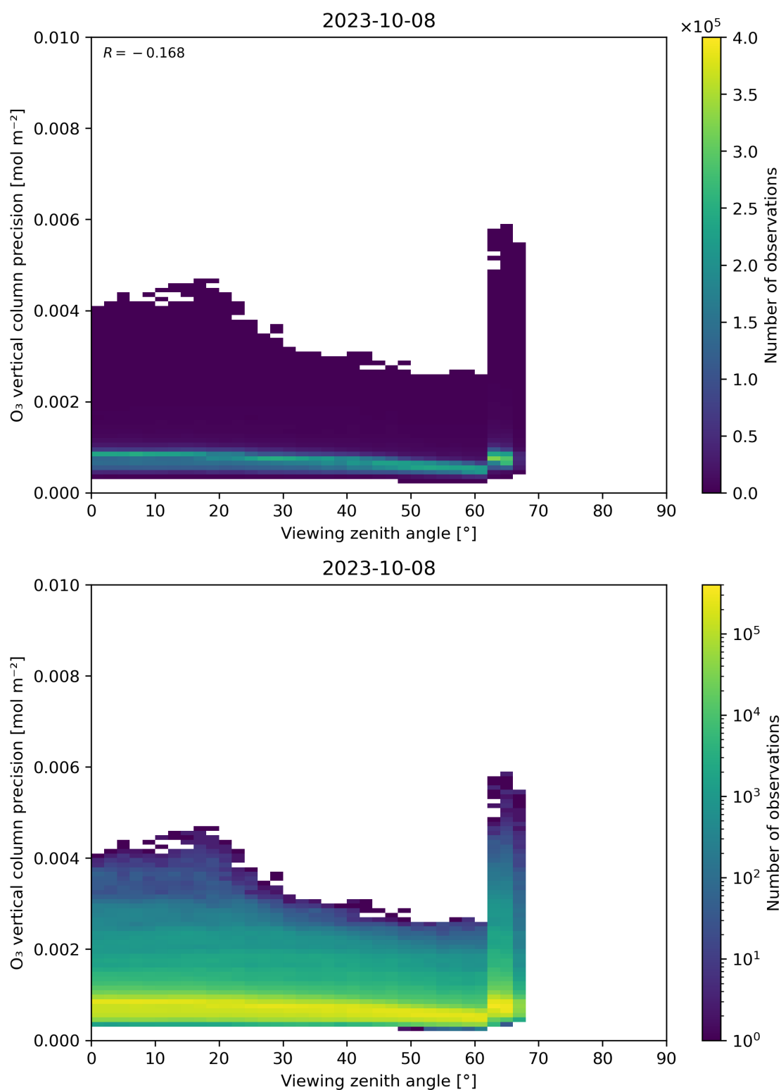
Figure 53: Scatter density plot of “Viewing zenith angle” against “O 3 vertical column precision” for 2023-10-07 to 2023-10-09.
