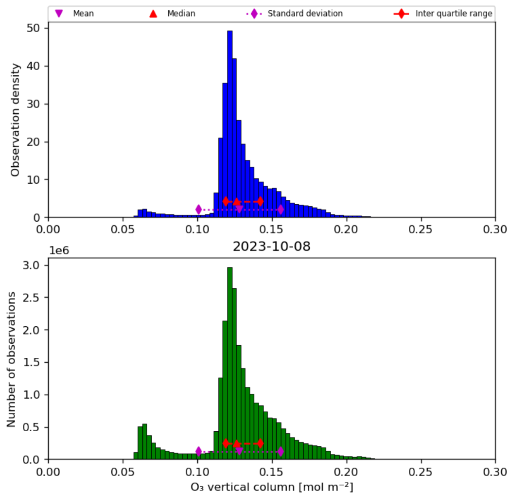
Figure 21: Histogram of “O 3 vertical column” for 2023-10-07 to 2023-10-09
