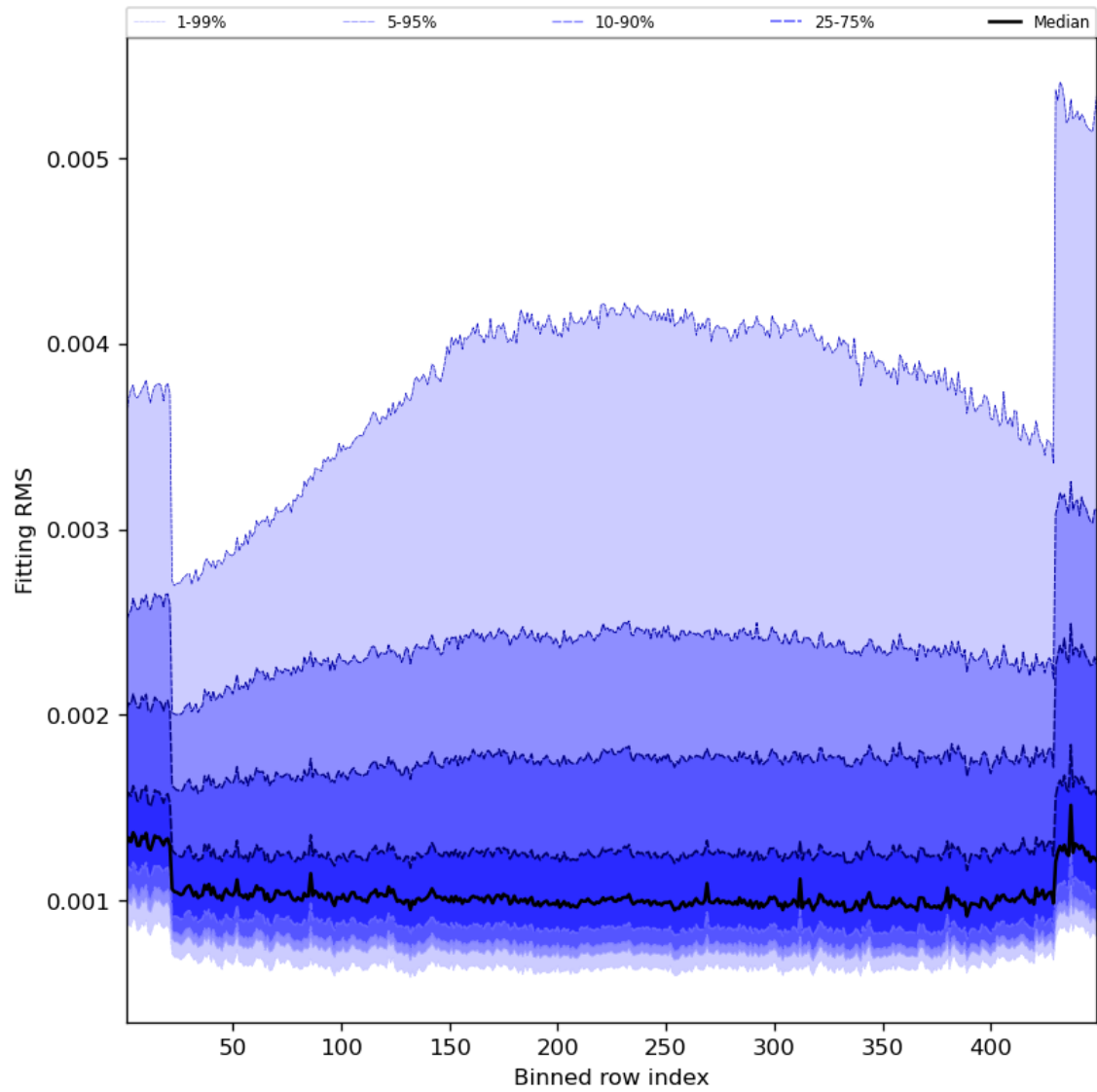
Figure 30: Along track statistics of “Fitting RMS” for 2023-10-07 to 2023-10-09
