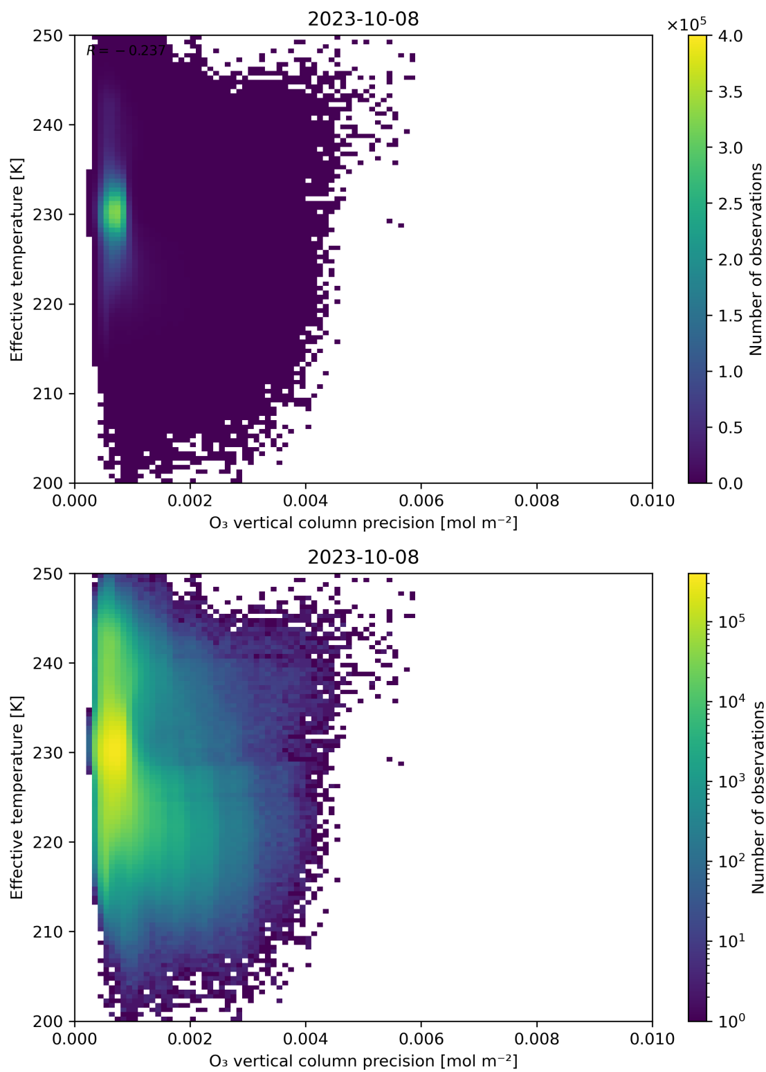
Figure 42: Scatter density plot of “O 3 vertical column precision” against “Effective temperature” for 2023-10-07 to 2023-10-09.
