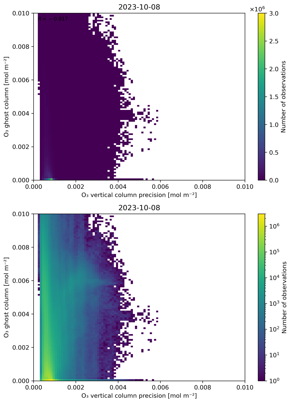
Figure 43: Scatter density plot of “O 3 vertical column precision” against “O 3 ghost column” for 2023-10-07 to 2023-10-09.
