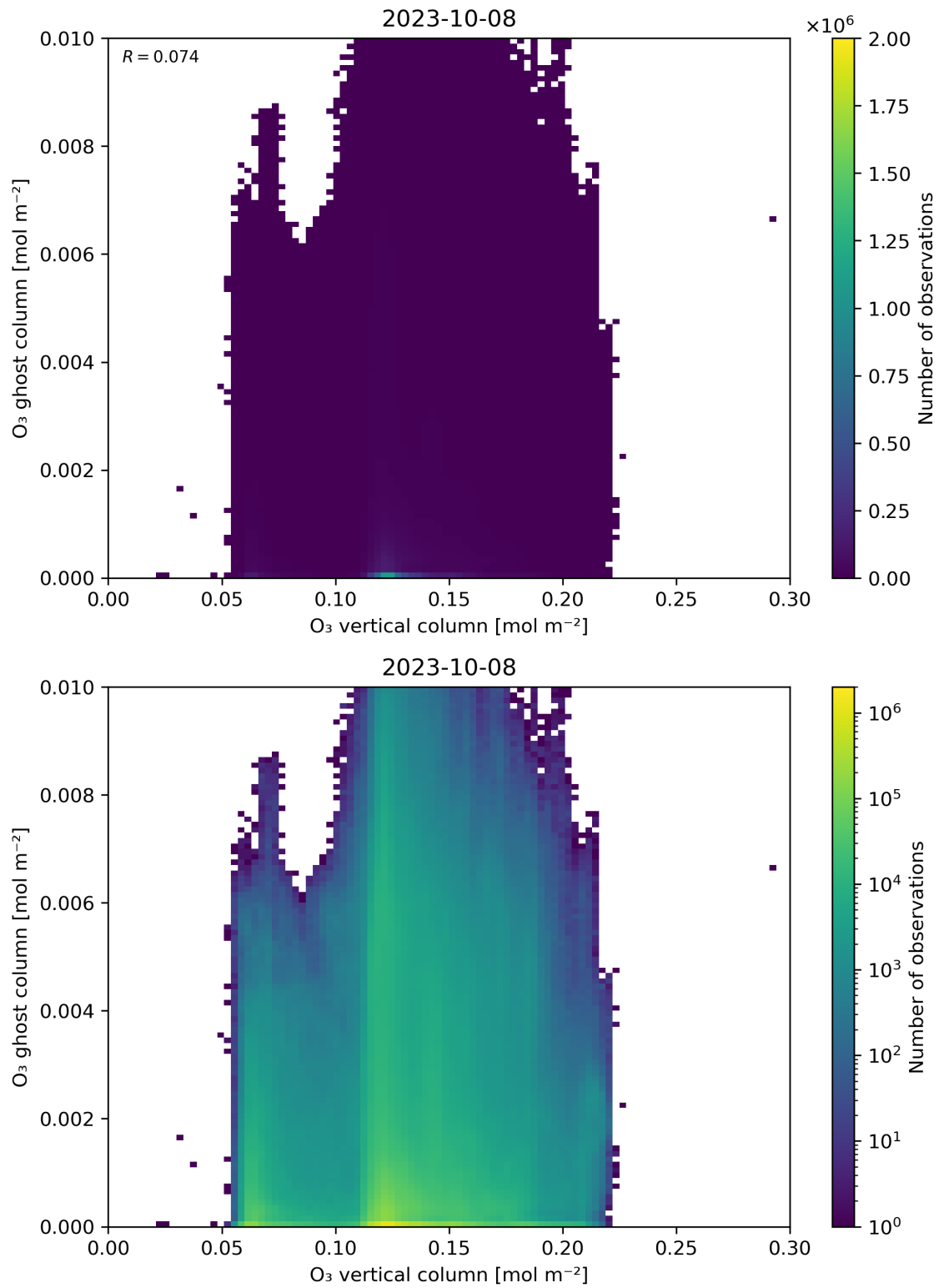
Figure 40: Scatter density plot of “O 3 vertical column” against “O 3 ghost column” for 2023-10-07 to 2023-10-09.
