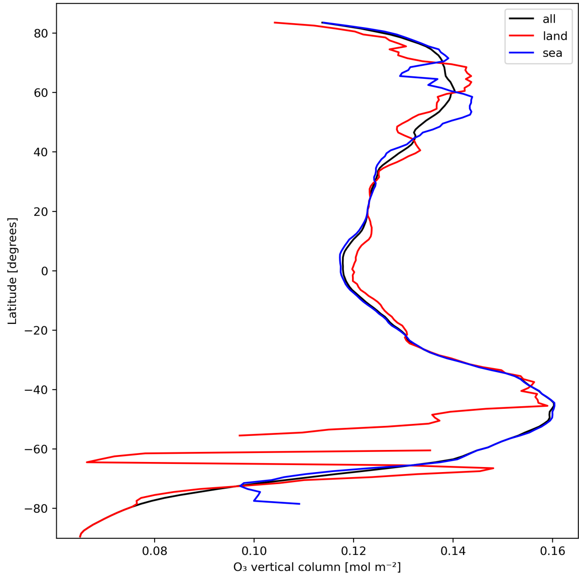
Figure 14: Zonal average of “O 3 vertical column” for 2023-10-07 to 2023-10-09.
