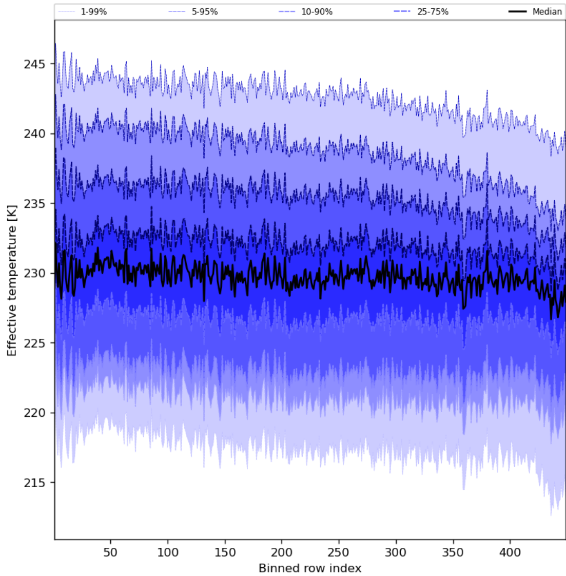
Figure 31: Along track statistics of “Effective temperature” for 2023-10-07 to 2023-10-09
