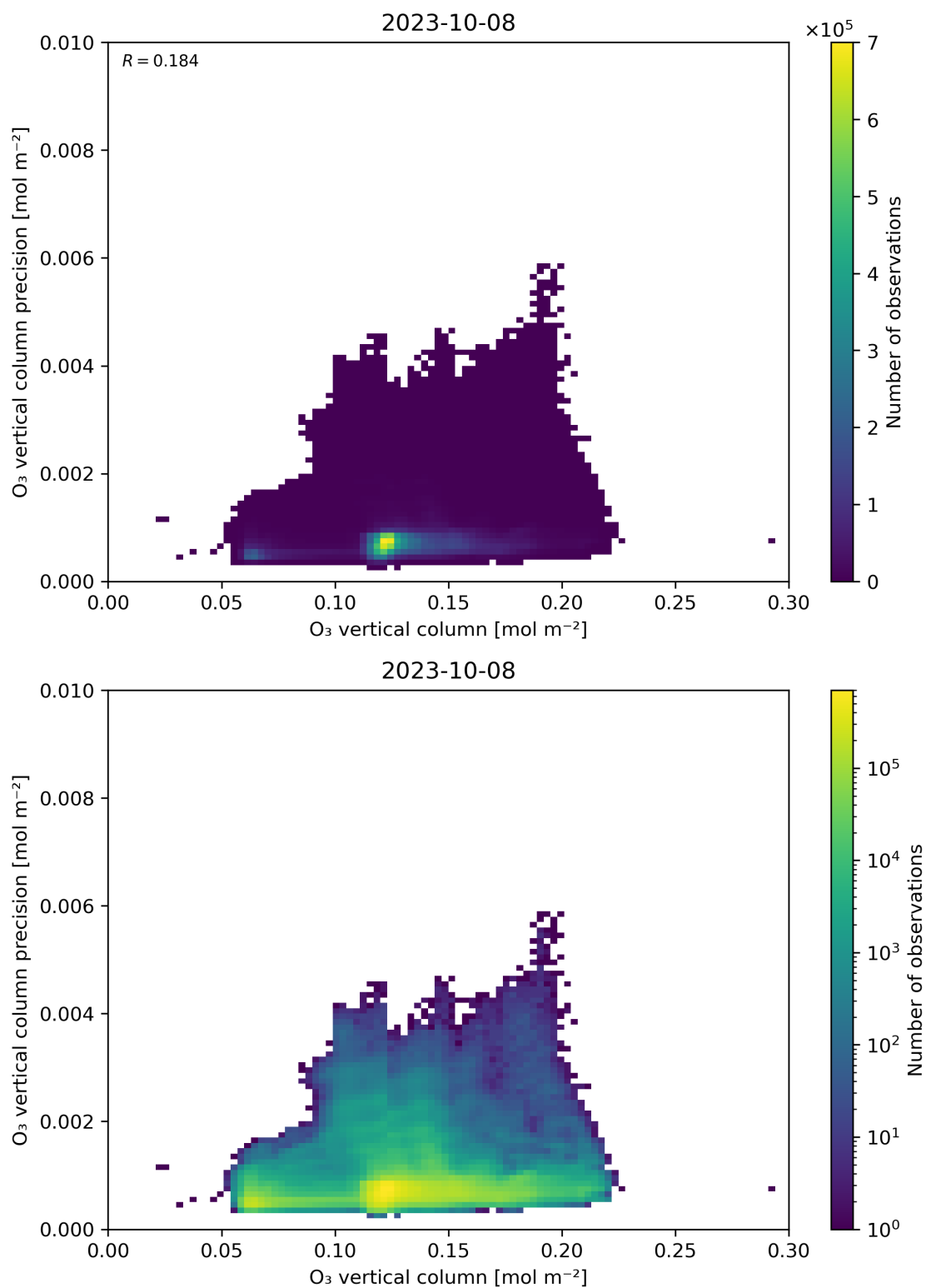
Figure 41: Scatter density plot of “O 3 vertical column” against “O 3 vertical column precision” for 2023-10-07 to 2023-10-09.
