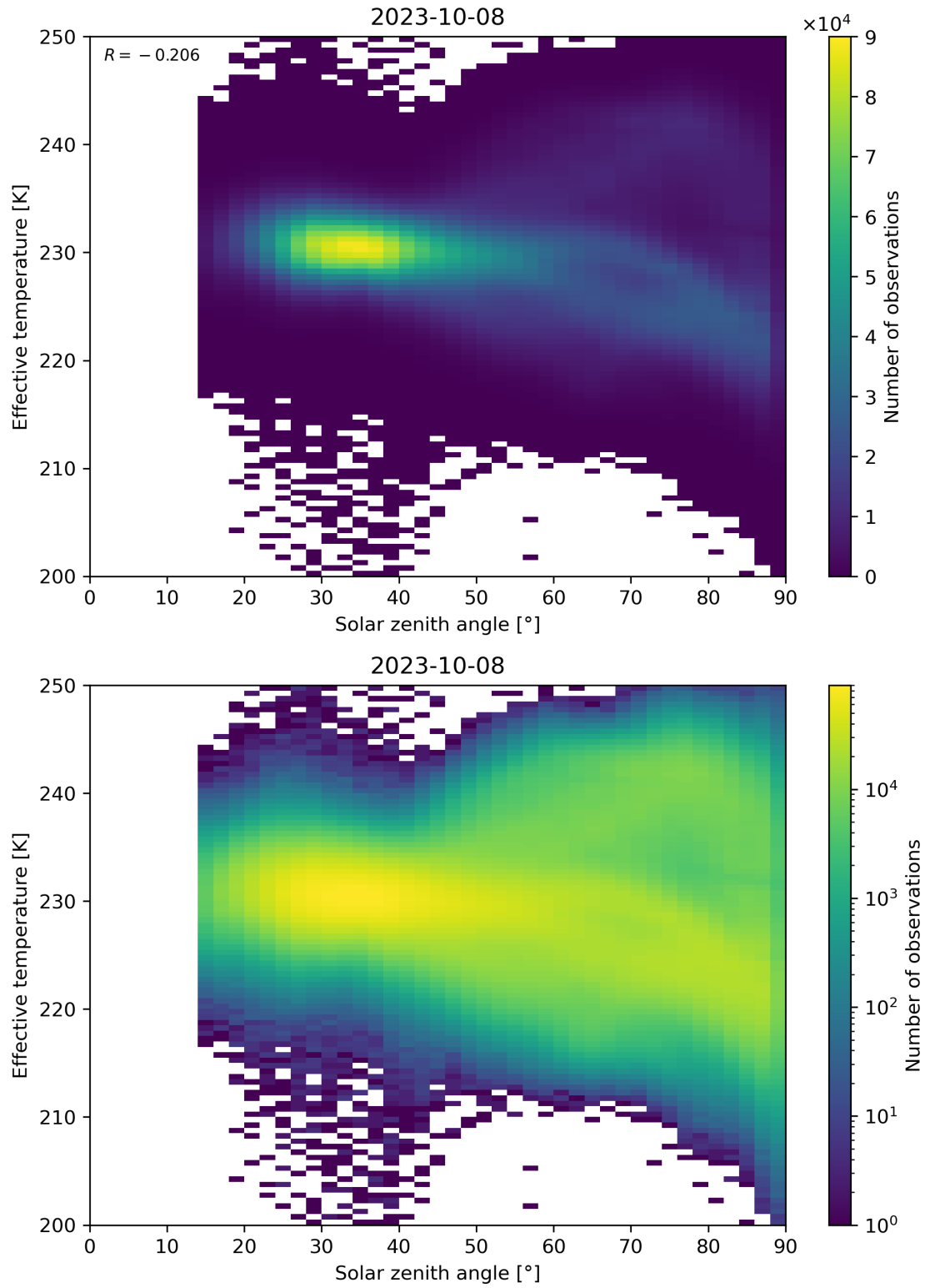
Figure 45: Scatter density plot of “Solar zenith angle” against “Effective temperature” for 2023-10-07 to 2023-10-09.
