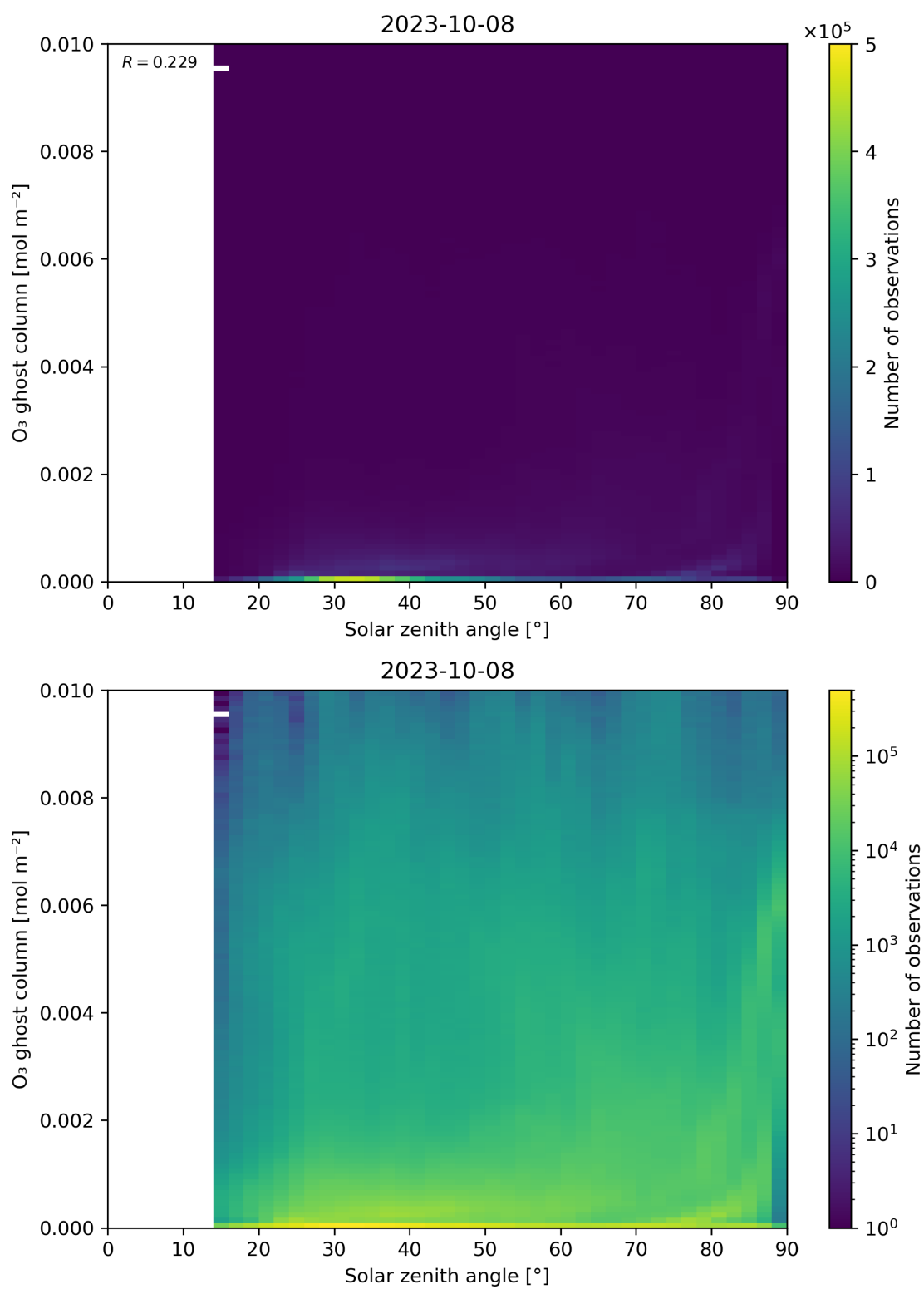
Figure 46: Scatter density plot of “Solar zenith angle” against “O 3 ghost column” for 2023-10-07 to 2023-10-09.
