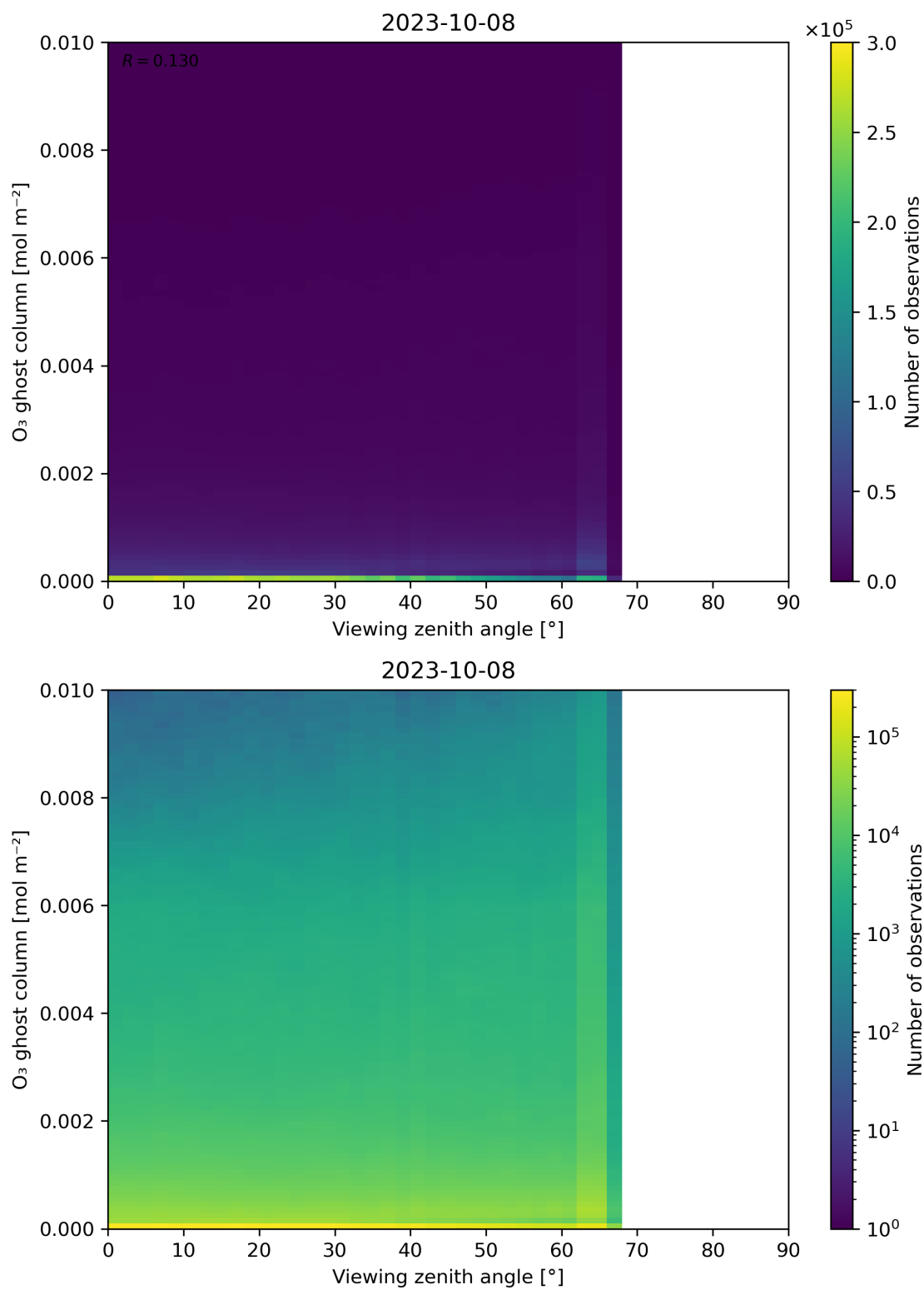
Figure 51: Scatter density plot of “Viewing zenith angle” against “O 3 ghost column” for 2023-10-07 to 2023-10-09.
