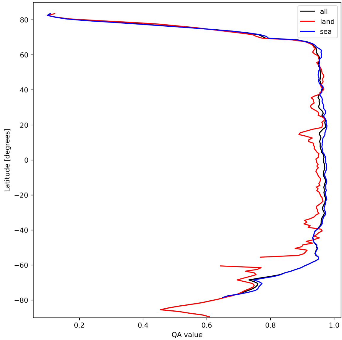
Figure 13: Zonal average of “QA value” for 2023-10-07 to 2023-10-09.
