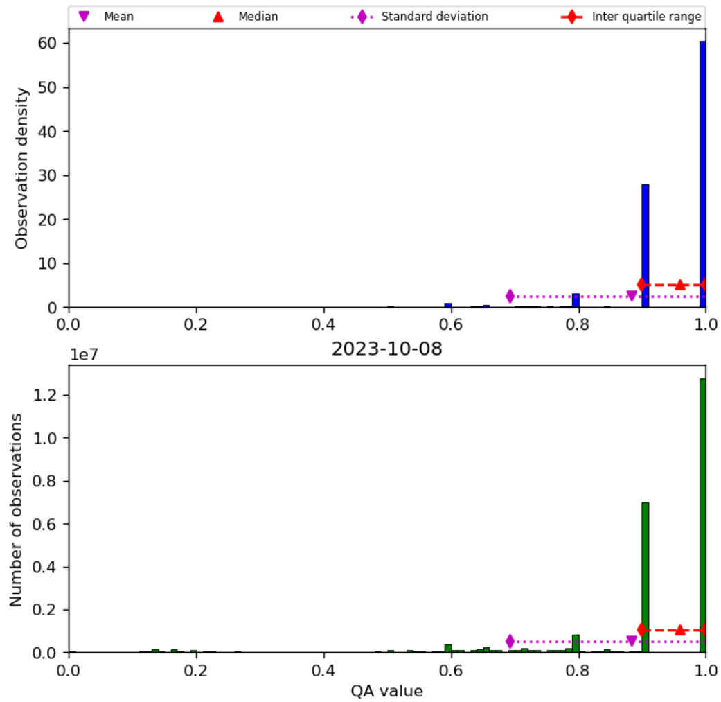
Figure 20: Histogram of “QA value” for 2023-10-07 to 2023-10-09
