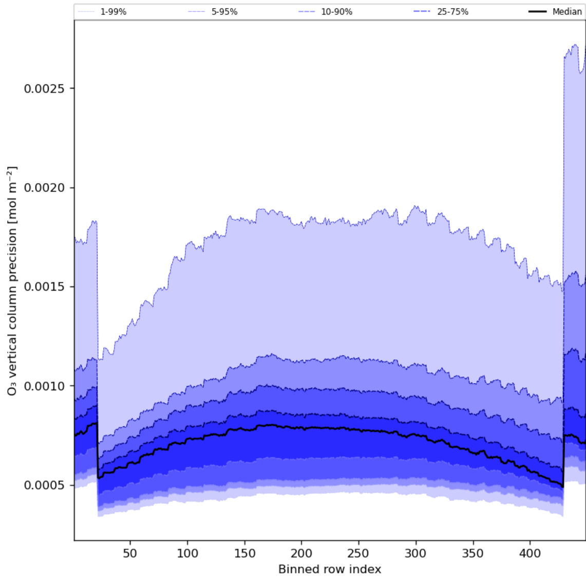
Figure 29: Along track statistics of “O 3 vertical column precision” for 2023-10-07 to 2023-10-09
