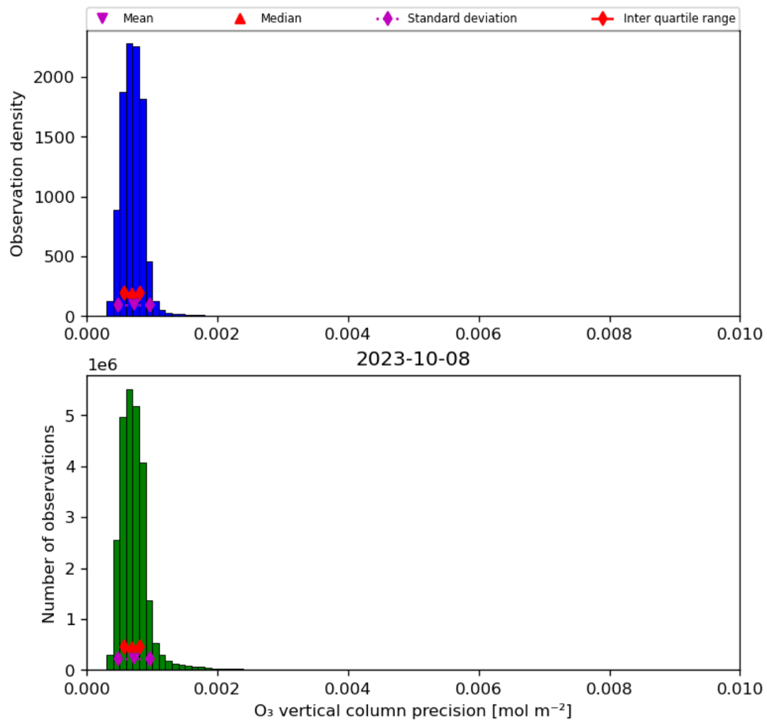
Figure 22: Histogram of “O 3 vertical column precision” for 2023-10-07 to 2023-10-09
