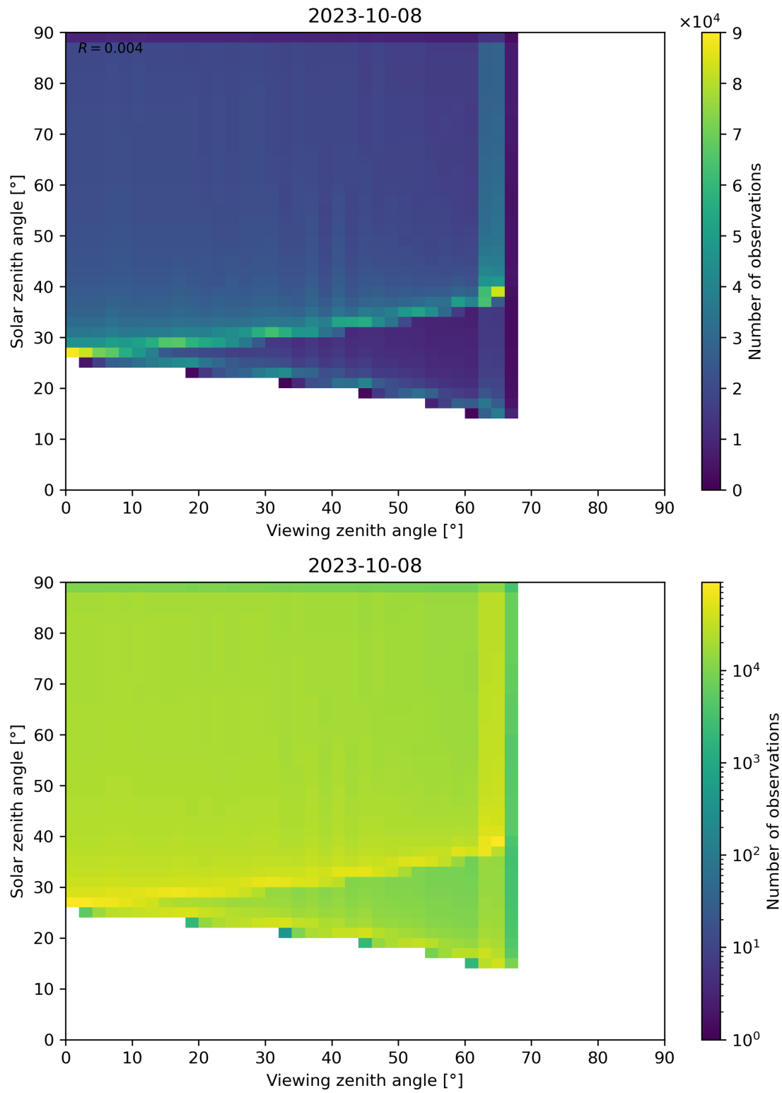
Figure 54: Scatter density plot of “Viewing zenith angle” against “Solar zenith angle” for 2023-10-07 to 2023-10-09.
