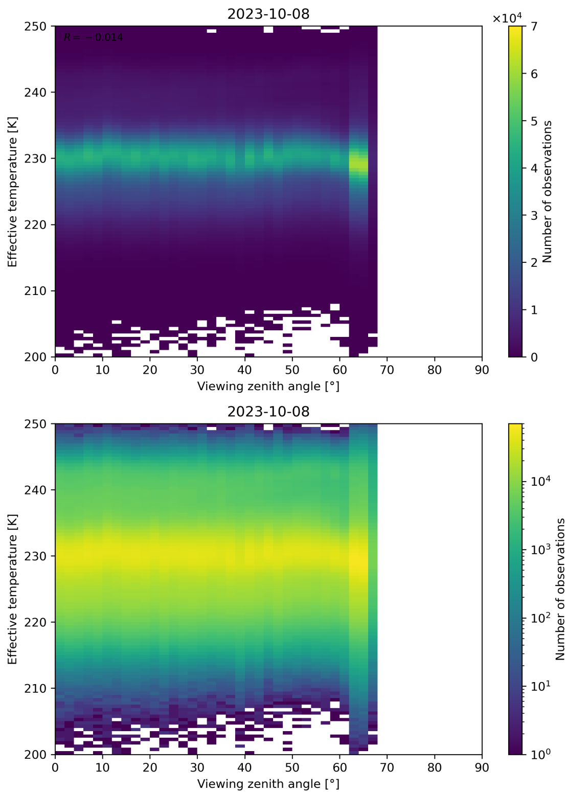
Figure 50: Scatter density plot of “Viewing zenith angle” against “Effective temperature” for 2023-10-07 to 2023-10-09.
