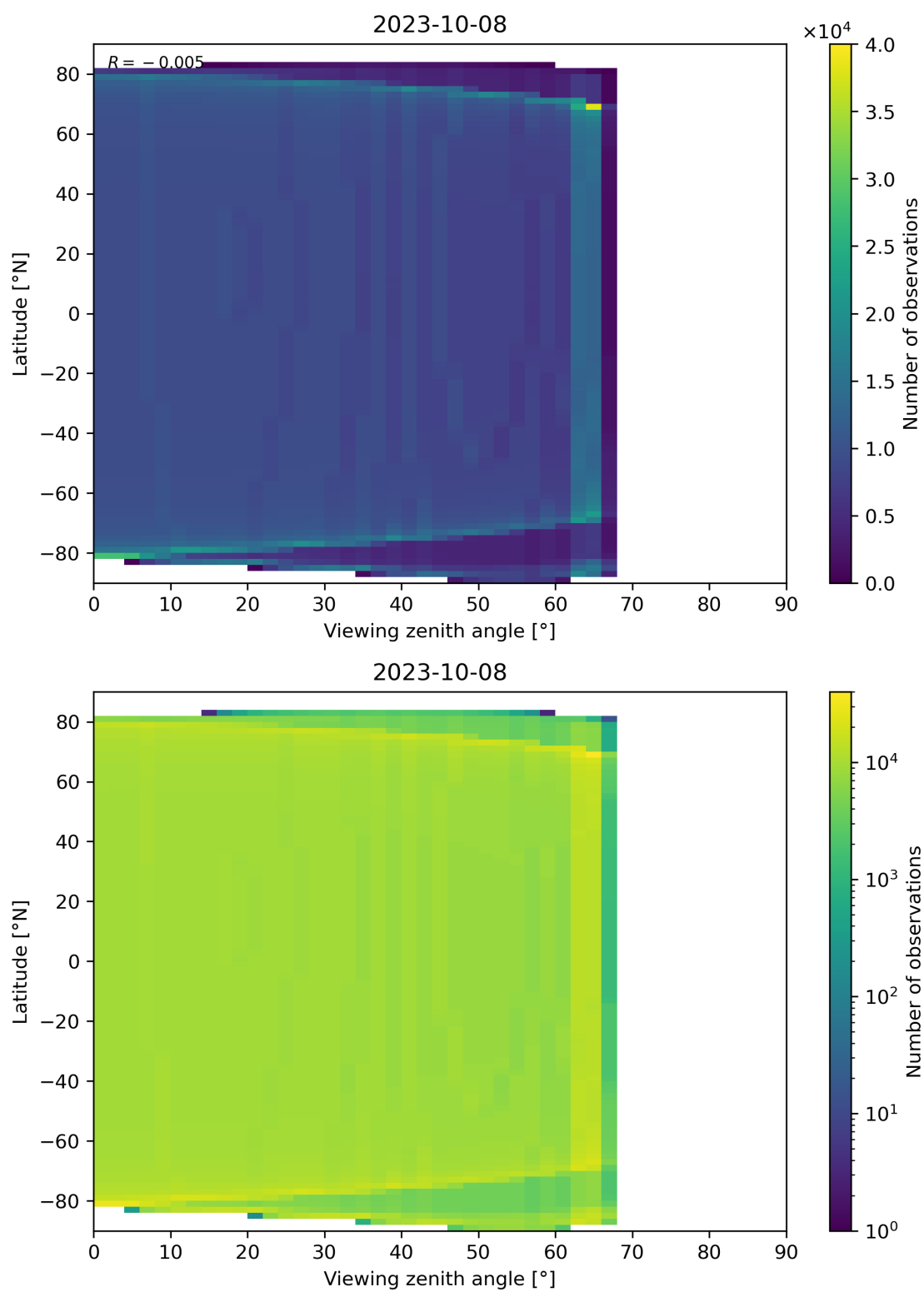
Figure 49: Scatter density plot of “Viewing zenith angle” against “Latitude” for 2023-10-07 to 2023-10-09.
