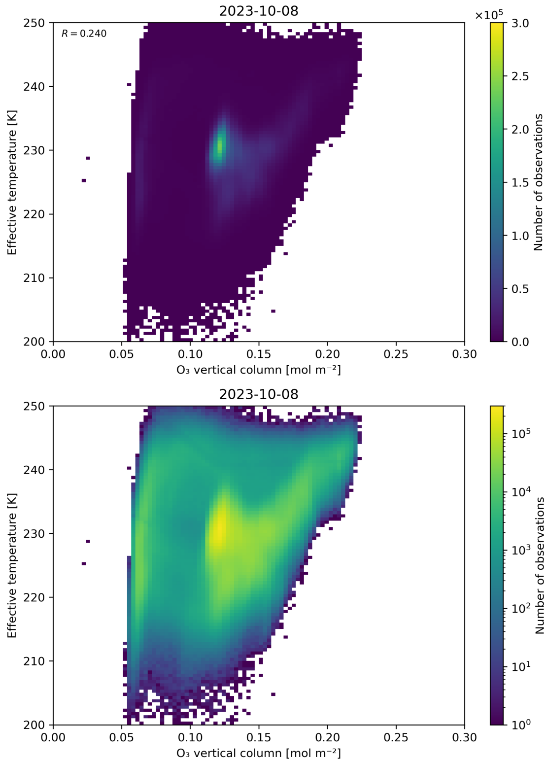
Figure 39: Scatter density plot of “O 3 vertical column” against “Effective temperature” for 2023-10-07 to 2023-10-09.
