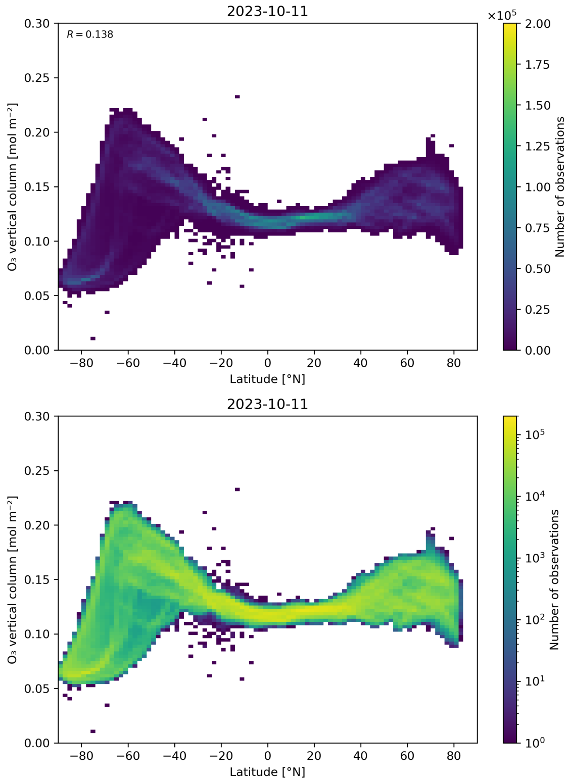
Figure 36: Scatter density plot of “Latitude” against “O 3 vertical column” for 2023-10-10 to 2023-10-12.
