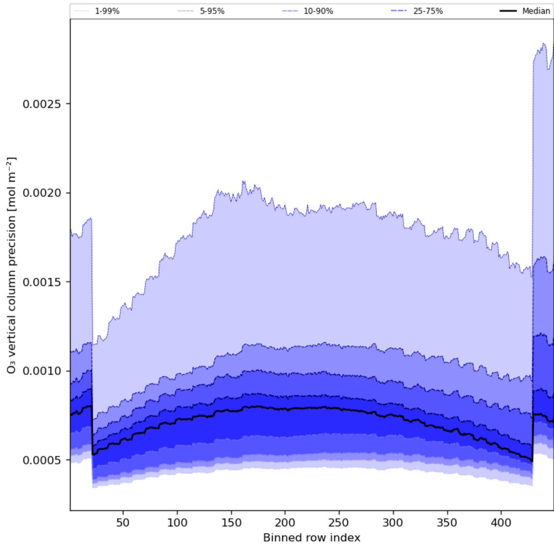
Figure 29: Along track statistics of “O 3 vertical column precision” for 2023-10-10 to 2023-10-12
