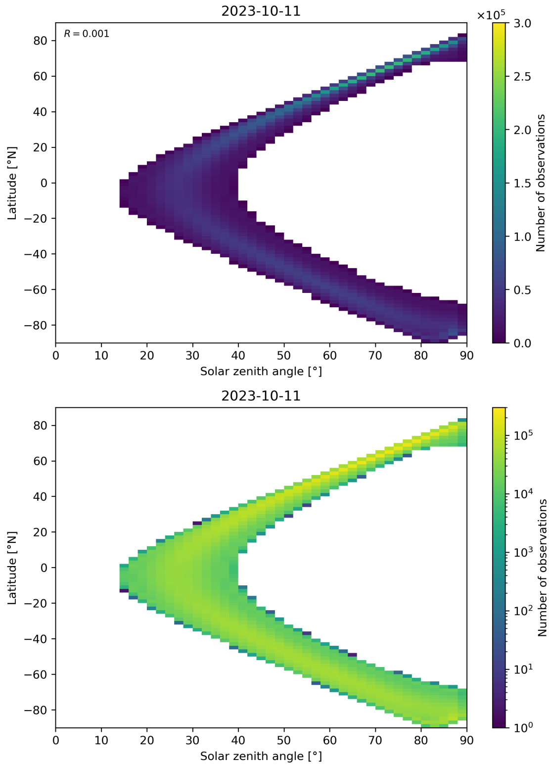
Figure 44: Scatter density plot of “Solar zenith angle” against “Latitude” for 2023-10-10 to 2023-10-12.
