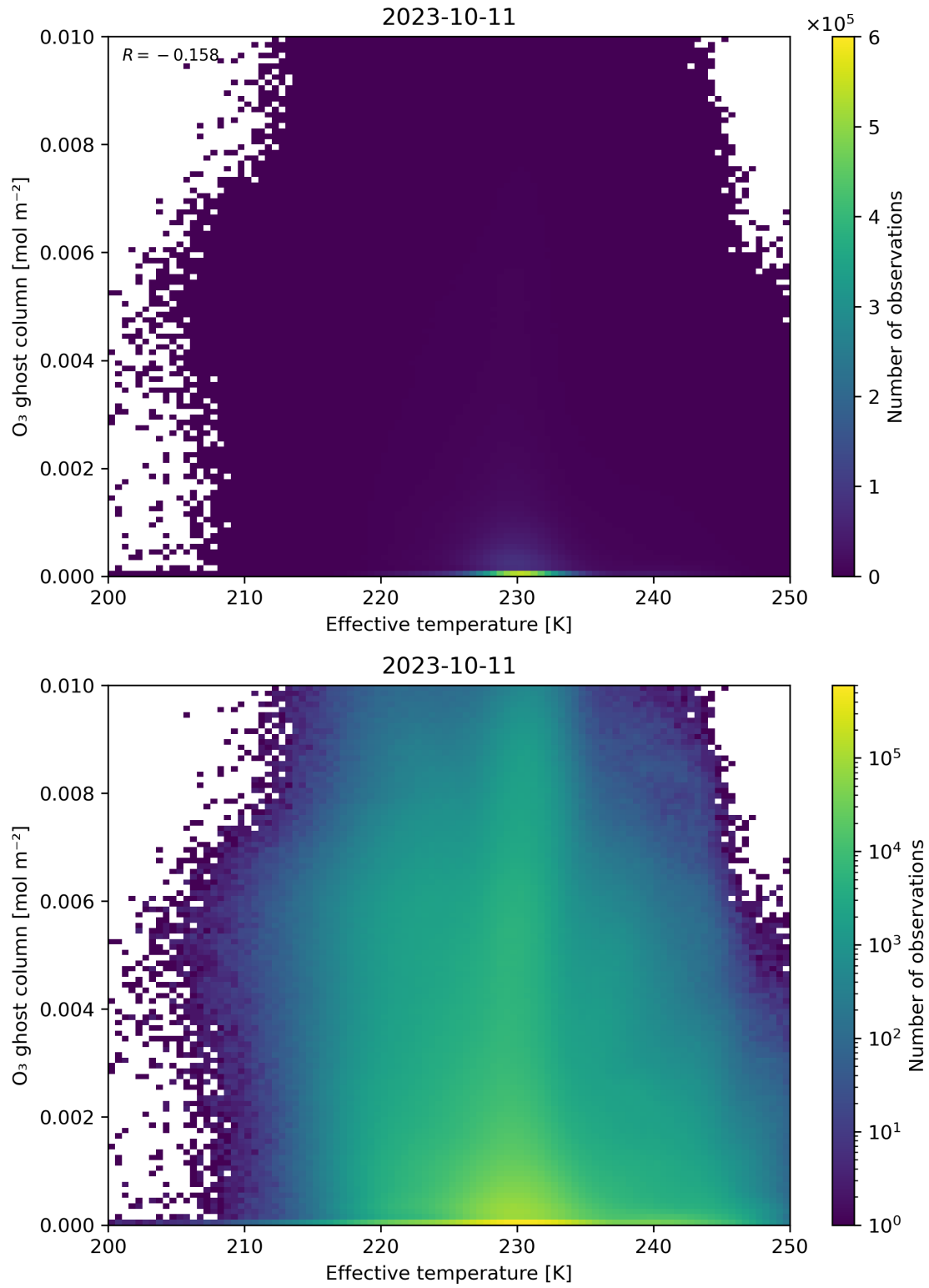
Figure 38: Scatter density plot of “Effective temperature” against “O 3 ghost column” for 2023-10-10 to 2023-10-12.
