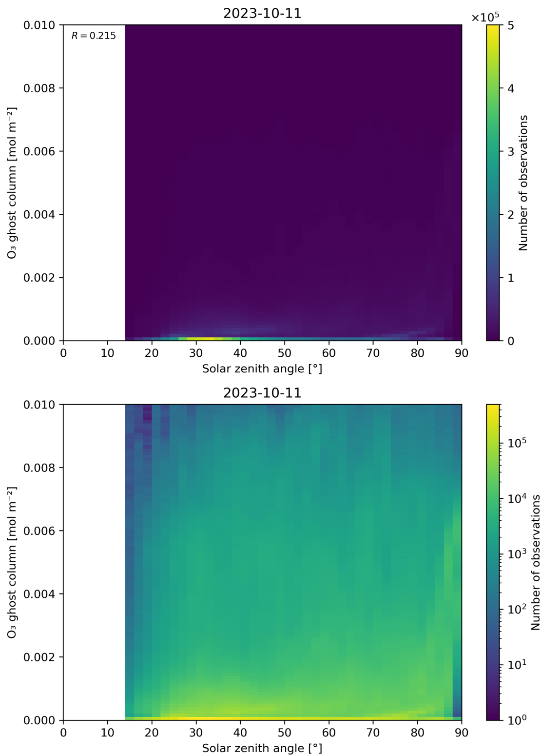
Figure 46: Scatter density plot of “Solar zenith angle” against “O 3 ghost column” for 2023-10-10 to 2023-10-12.
