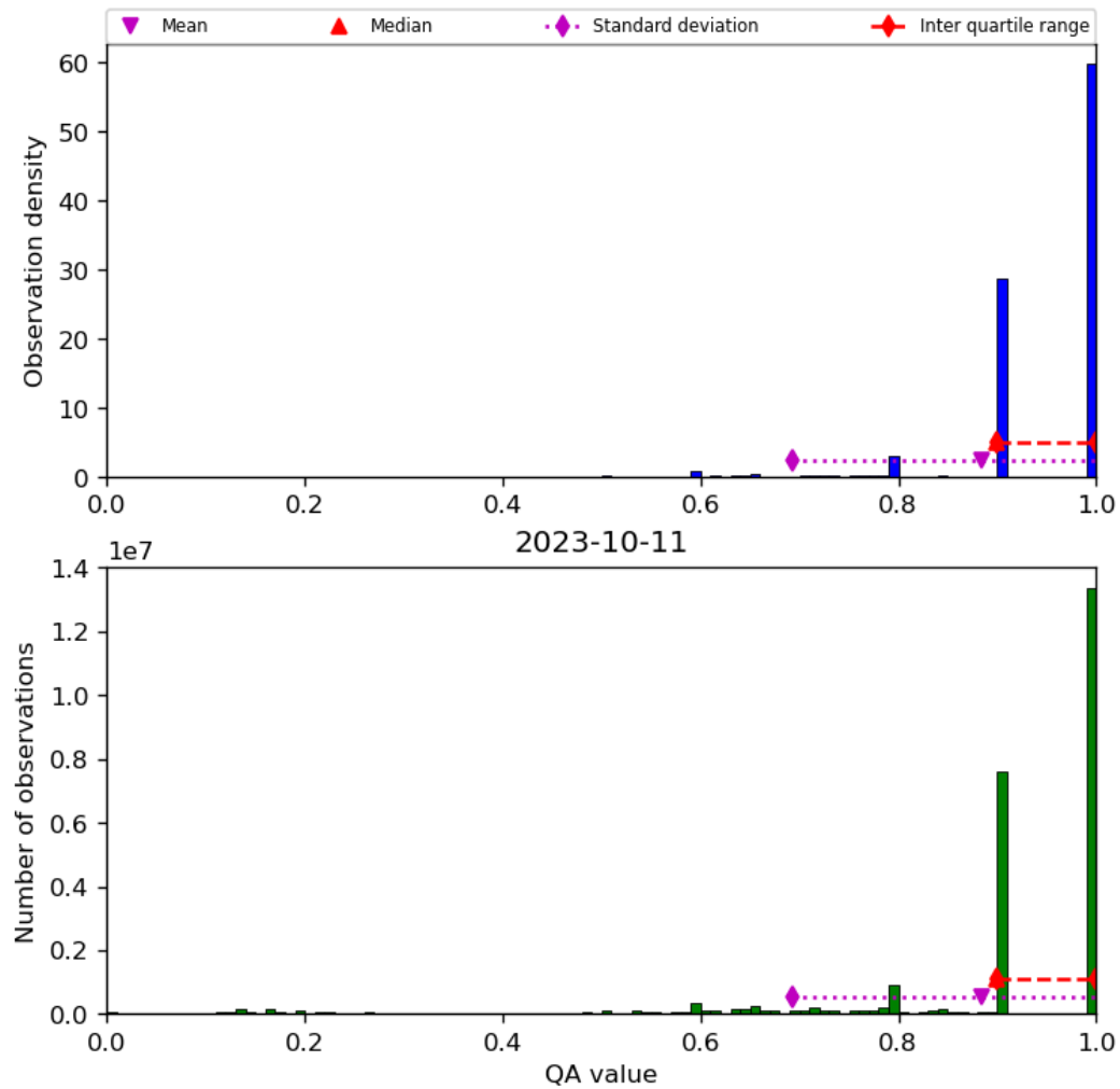
Figure 20: Histogram of “QA value” for 2023-10-10 to 2023-10-12
