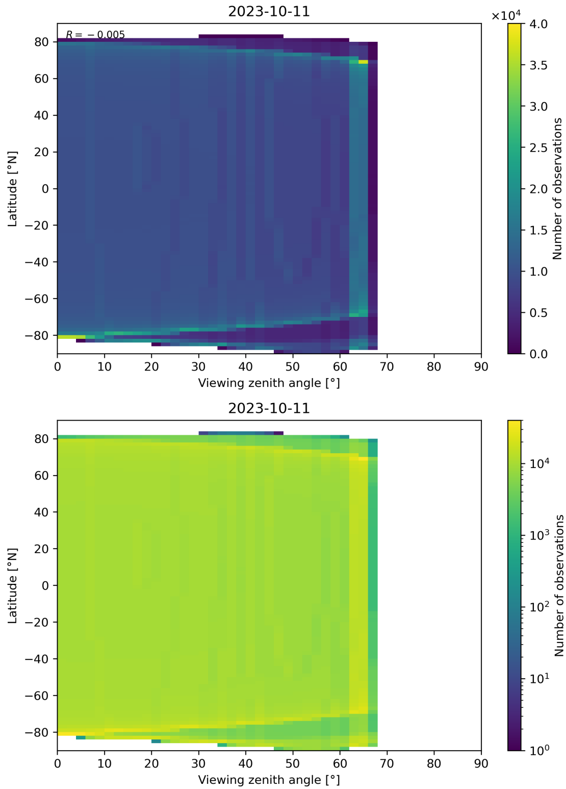
Figure 49: Scatter density plot of “Viewing zenith angle” against “Latitude” for 2023-10-10 to 2023-10-12.
