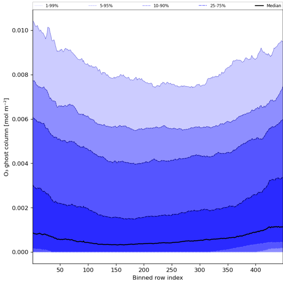
Figure 32: Along track statistics of “O 3 ghost column” for 2023-10-10 to 2023-10-12
