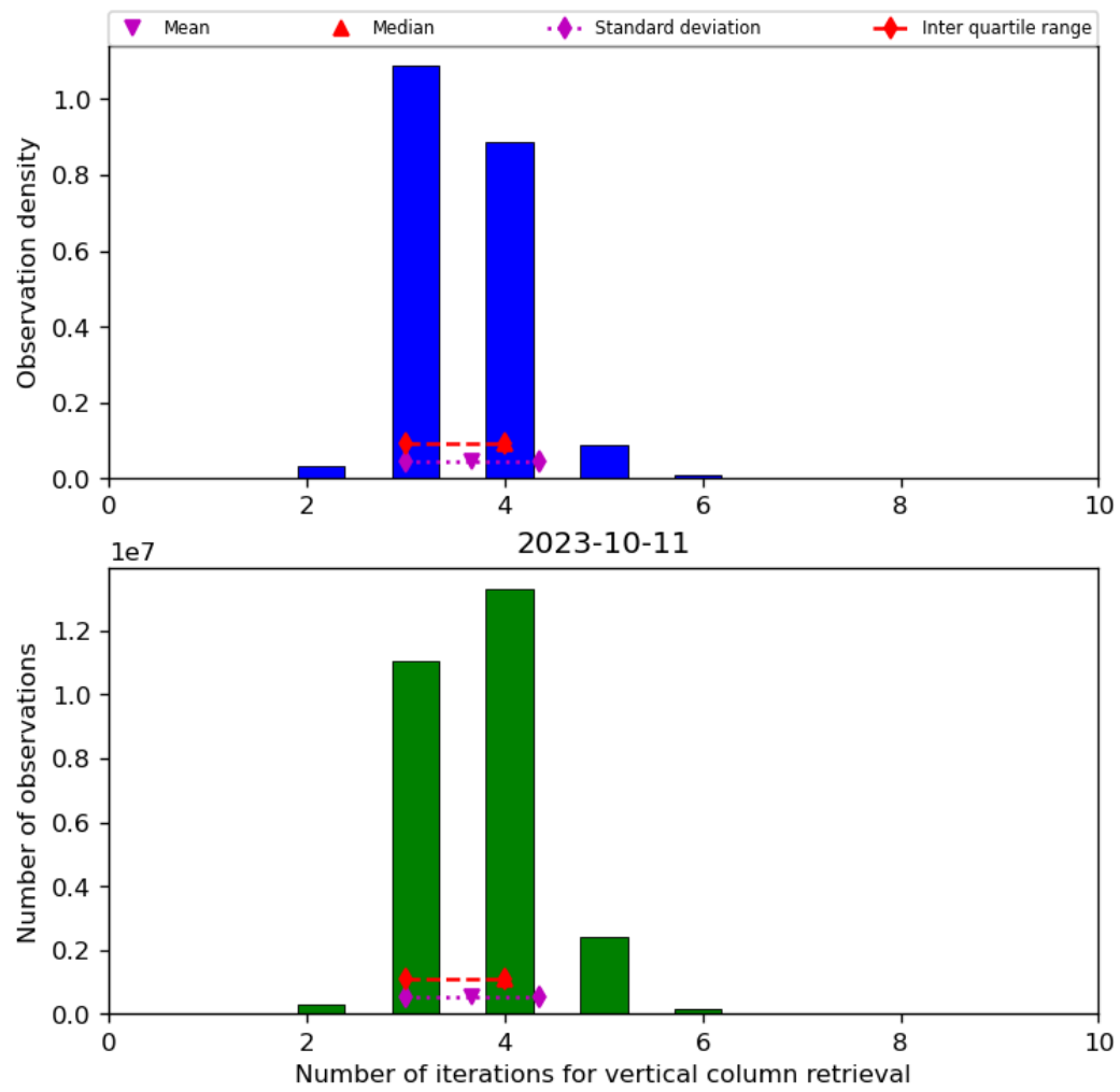
Figure 26: Histogram of “Number of iterations for vertical column retrieval” for 2023-10-10 to 2023-10-12
