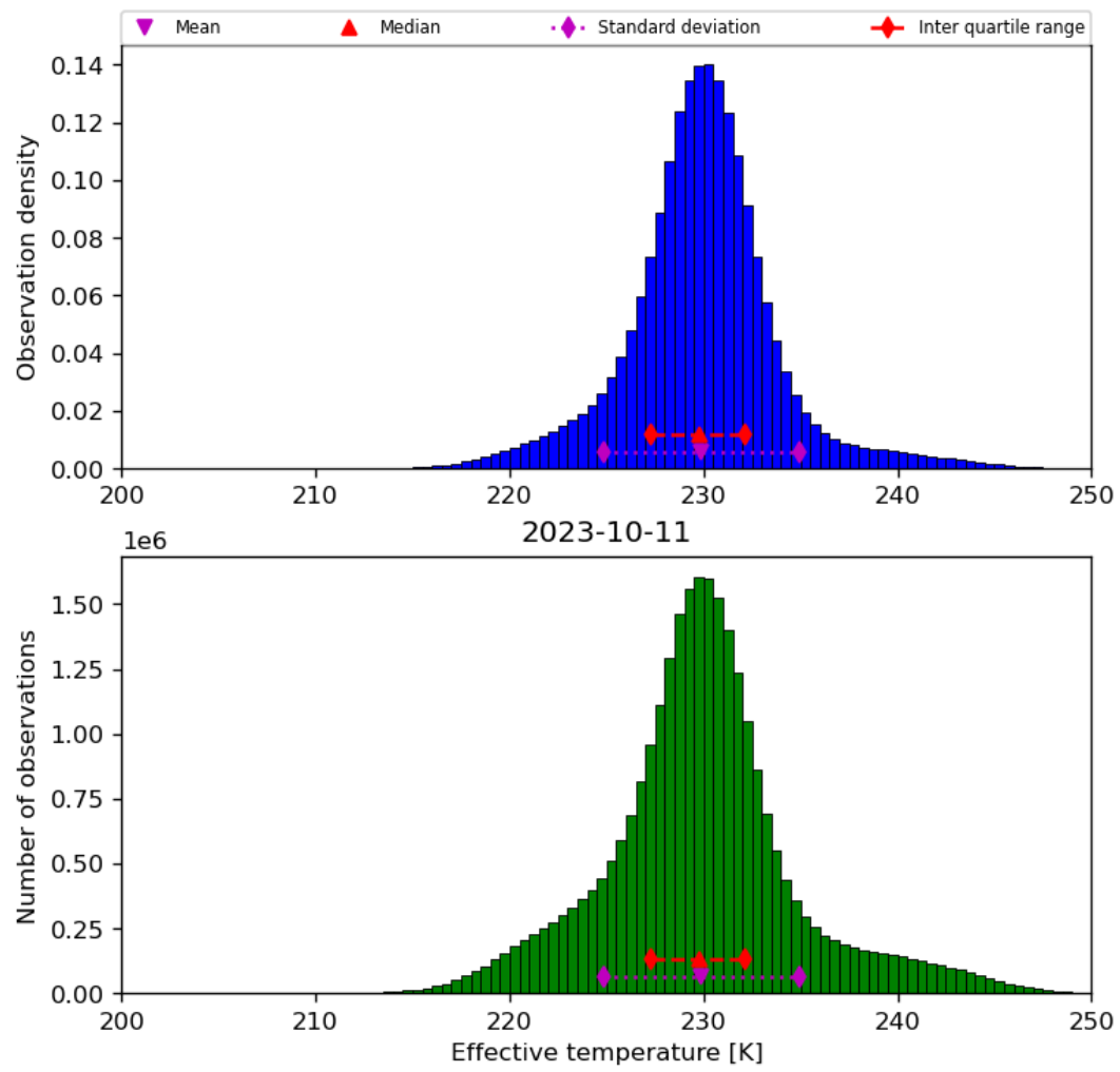
Figure 24: Histogram of “Effective temperature” for 2023-10-10 to 2023-10-12
