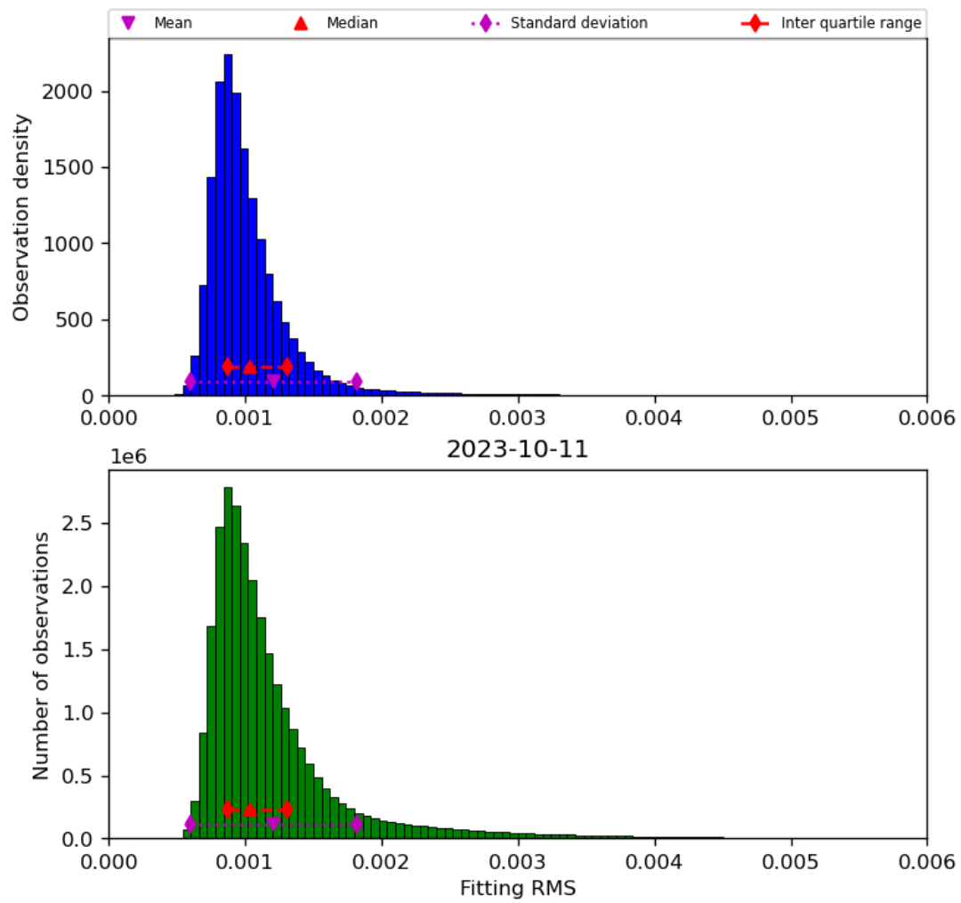
Figure 23: Histogram of “Fitting RMS” for 2023-10-10 to 2023-10-12
