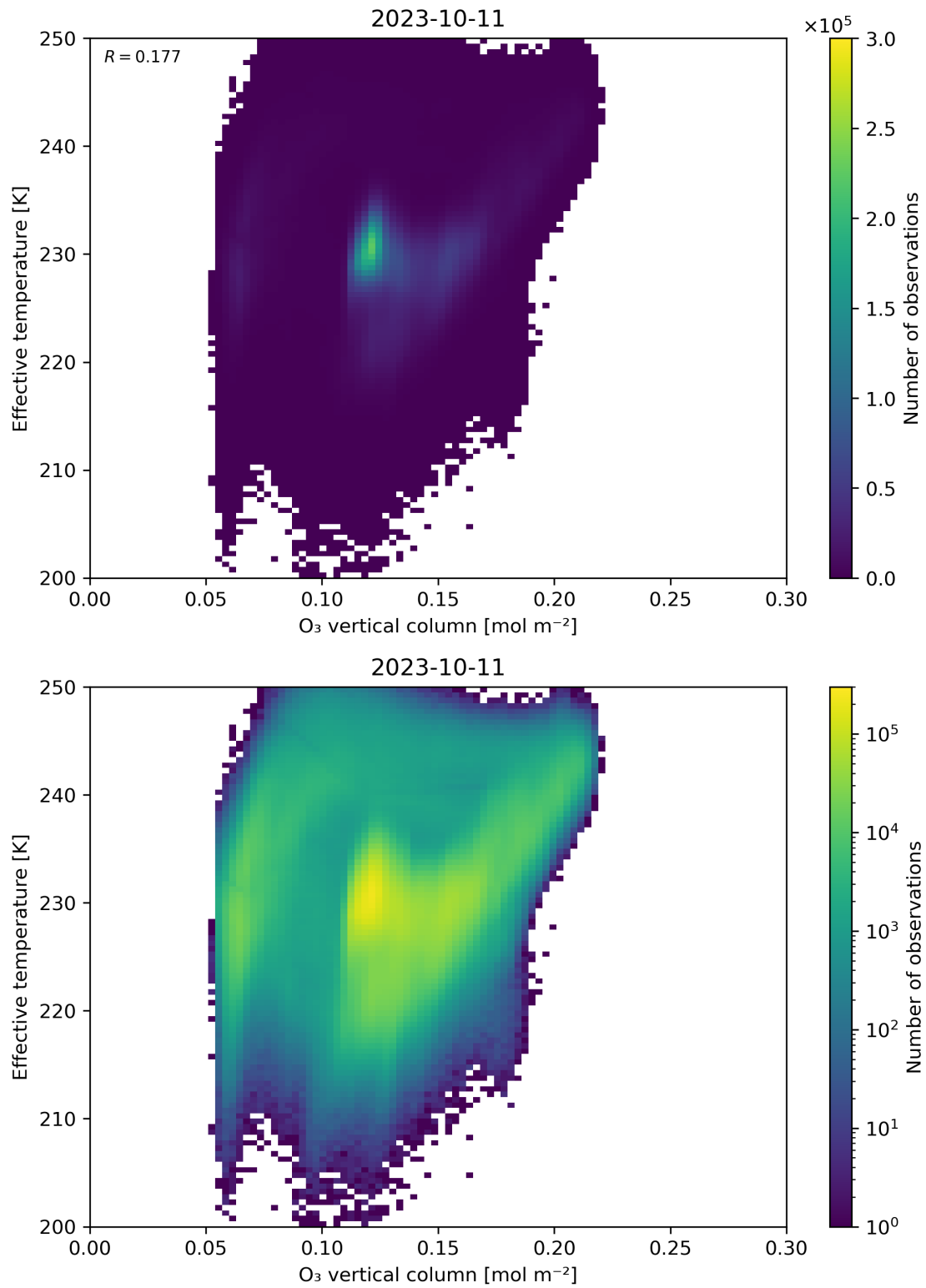
Figure 39: Scatter density plot of “O 3 vertical column” against “Effective temperature” for 2023-10-10 to 2023-10-12.
