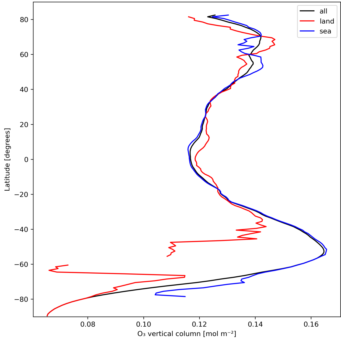
Figure 14: Zonal average of “O 3 vertical column” for 2023-10-10 to 2023-10-12.
