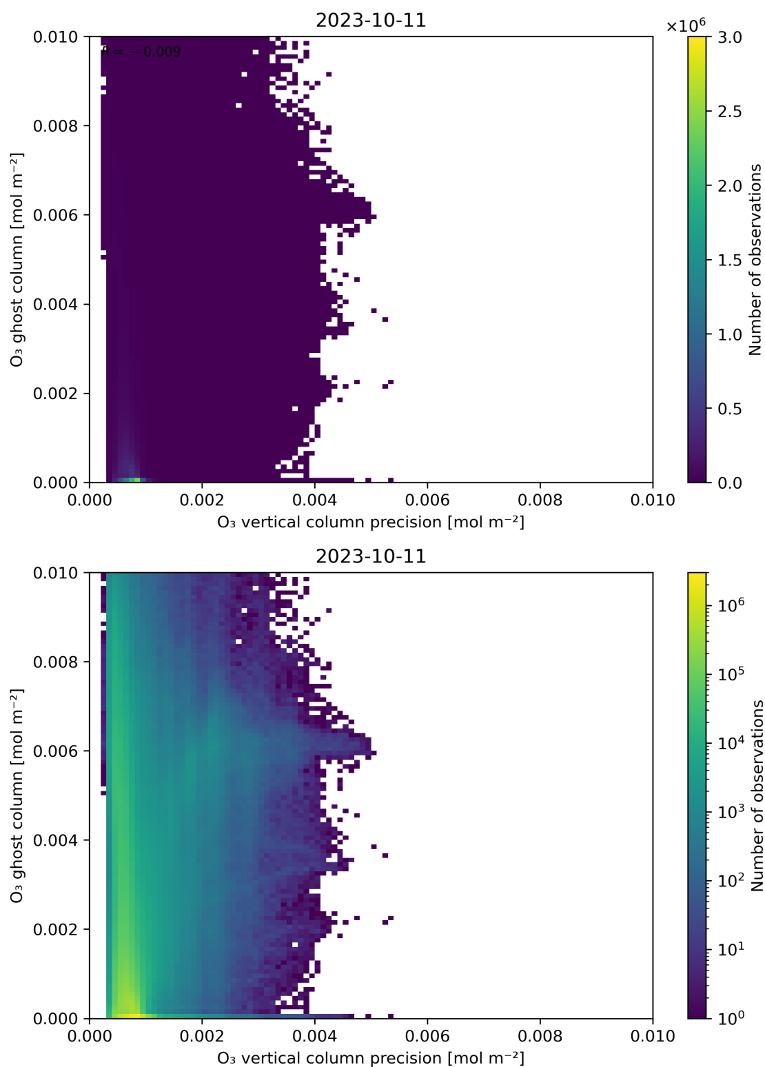
Figure 43: Scatter density plot of “O 3 vertical column precision” against “O 3 ghost column” for 2023-10-10 to 2023-10-12.
