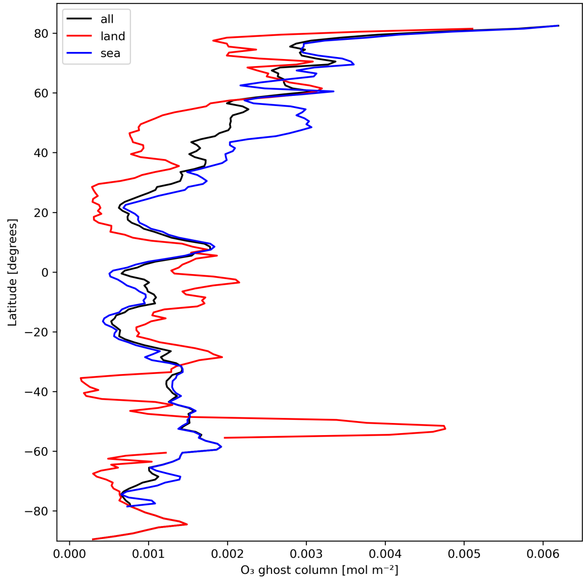
Figure 18: Zonal average of “O 3 ghost column” for 2023-10-10 to 2023-10-12.
