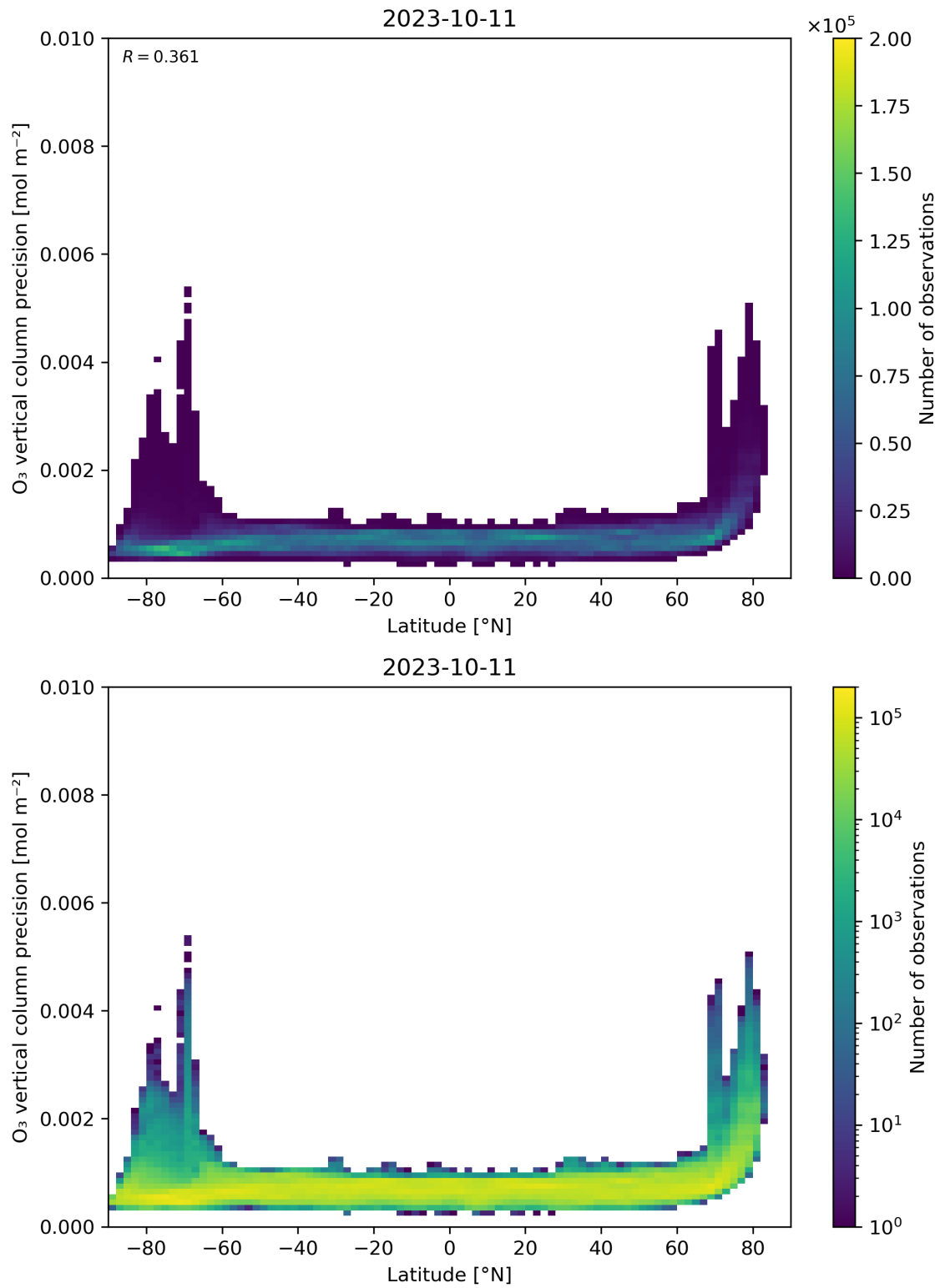
Figure 37: Scatter density plot of “Latitude” against “O 3 vertical column precision” for 2023-10-10 to 2023-10-12.
