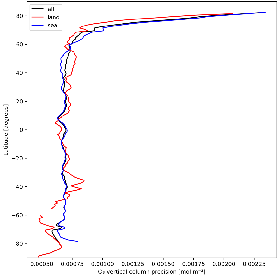
Figure 15: Zonal average of “O 3 vertical column precision” for 2023-10-10 to 2023-10-12.
