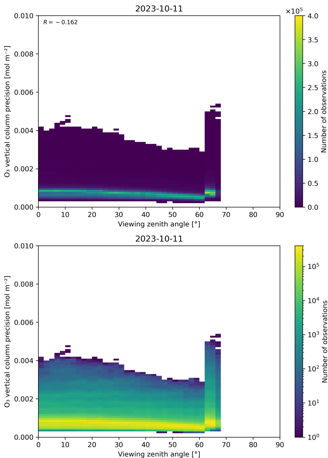
Figure 53: Scatter density plot of “Viewing zenith angle” against “O 3 vertical column precision” for 2023-10-10 to 2023-10-12.
