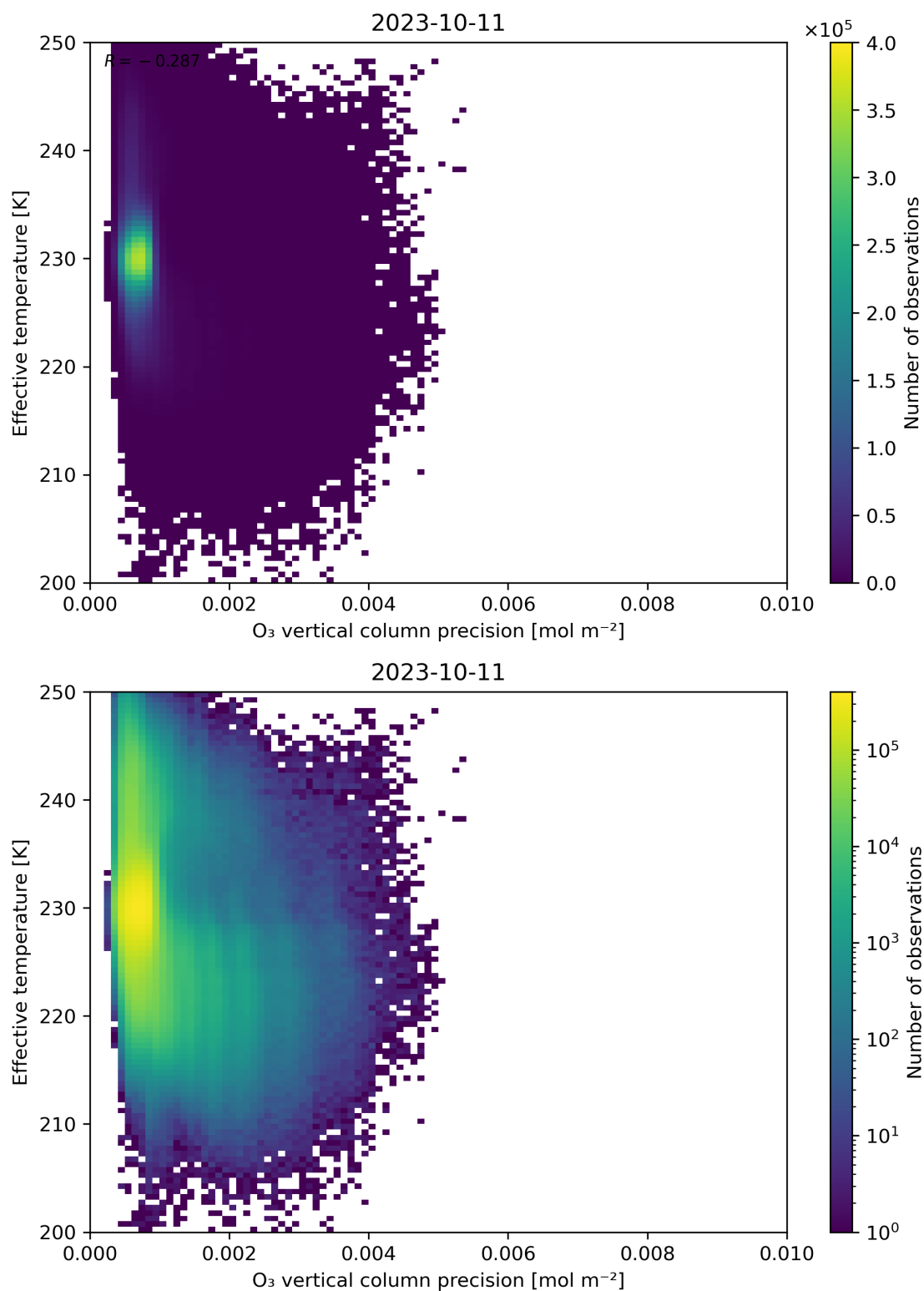
Figure 42: Scatter density plot of “O 3 vertical column precision” against “Effective temperature” for 2023-10-10 to 2023-10-12.
