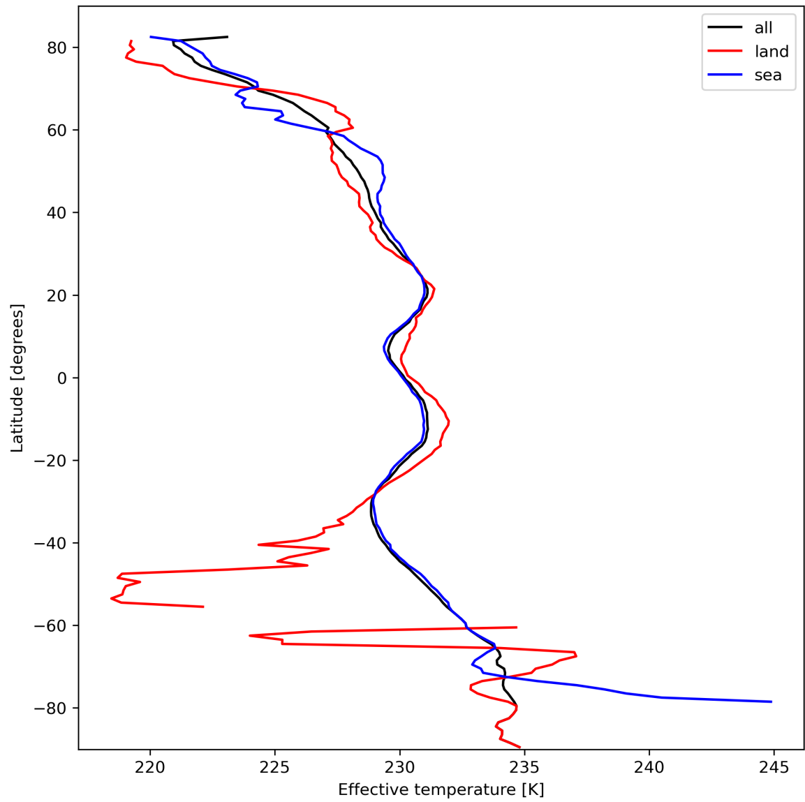
Figure 17: Zonal average of “Effective temperature” for 2023-10-10 to 2023-10-12.
