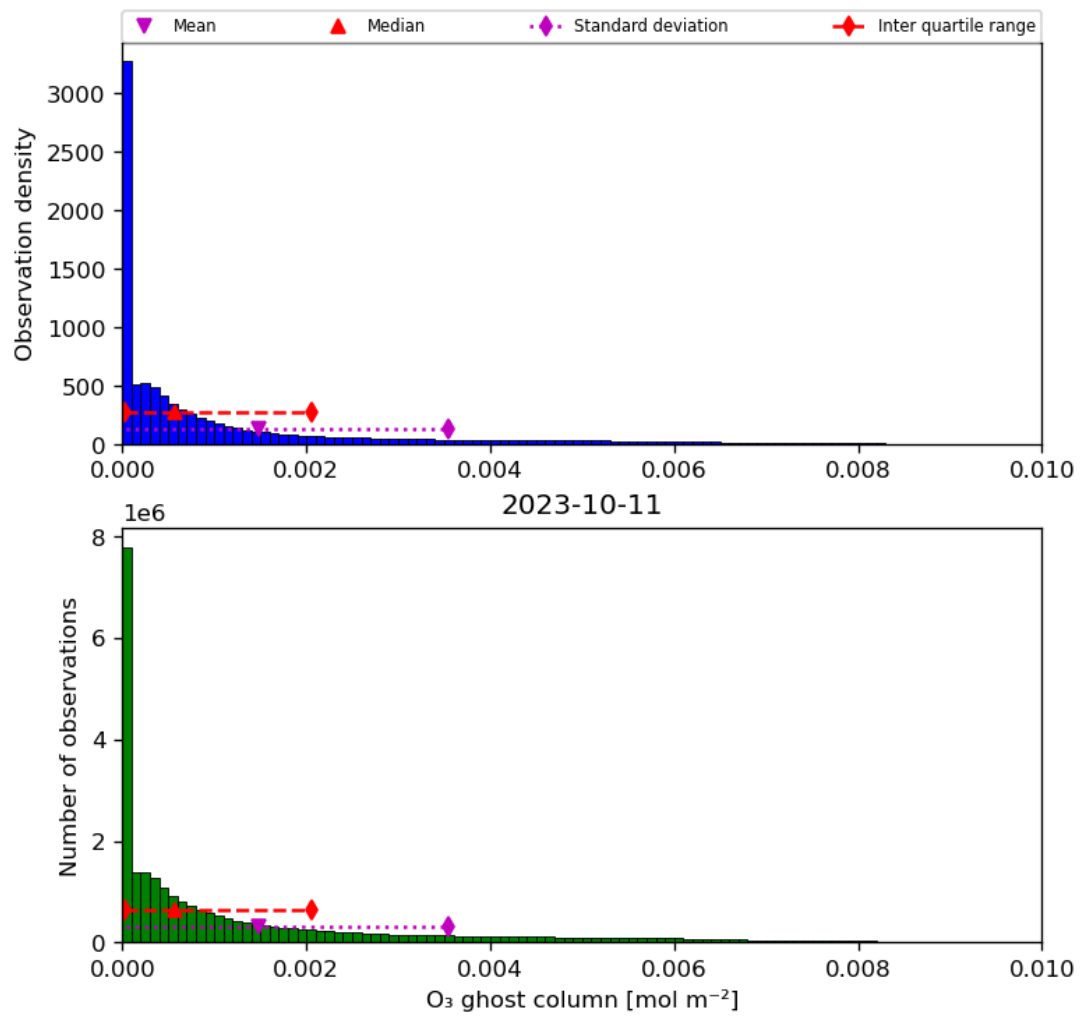
Figure 25: Histogram of “O 3 ghost column” for 2023-10-10 to 2023-10-12
