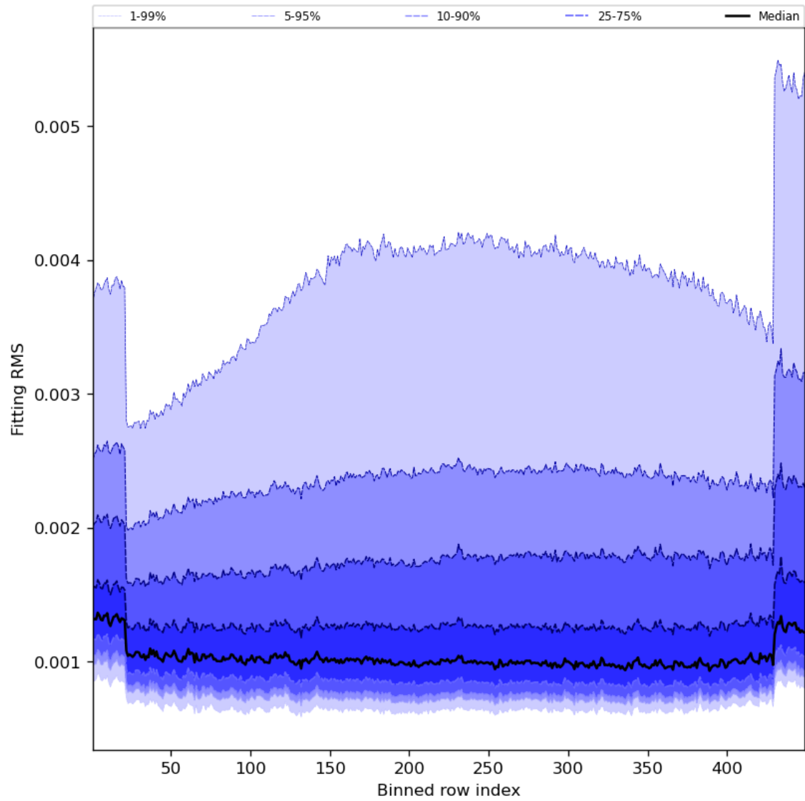
Figure 30: Along track statistics of “Fitting RMS” for 2023-10-10 to 2023-10-12
