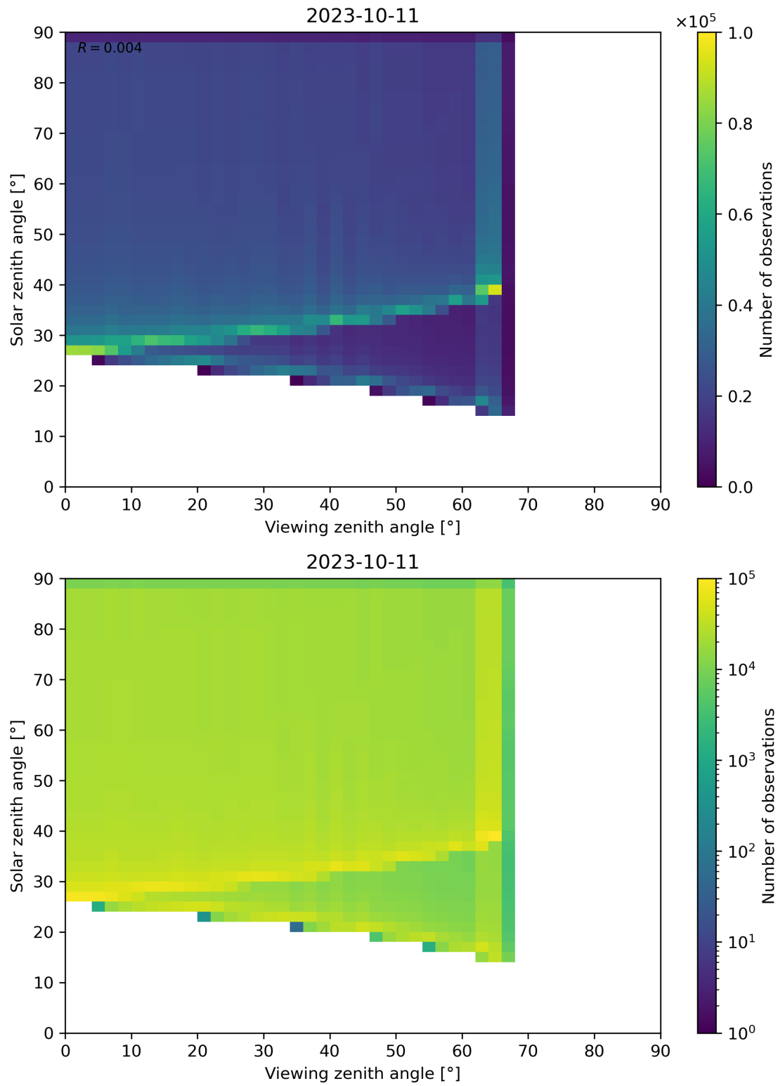
Figure 54: Scatter density plot of “Viewing zenith angle” against “Solar zenith angle” for 2023-10-10 to 2023-10-12.
