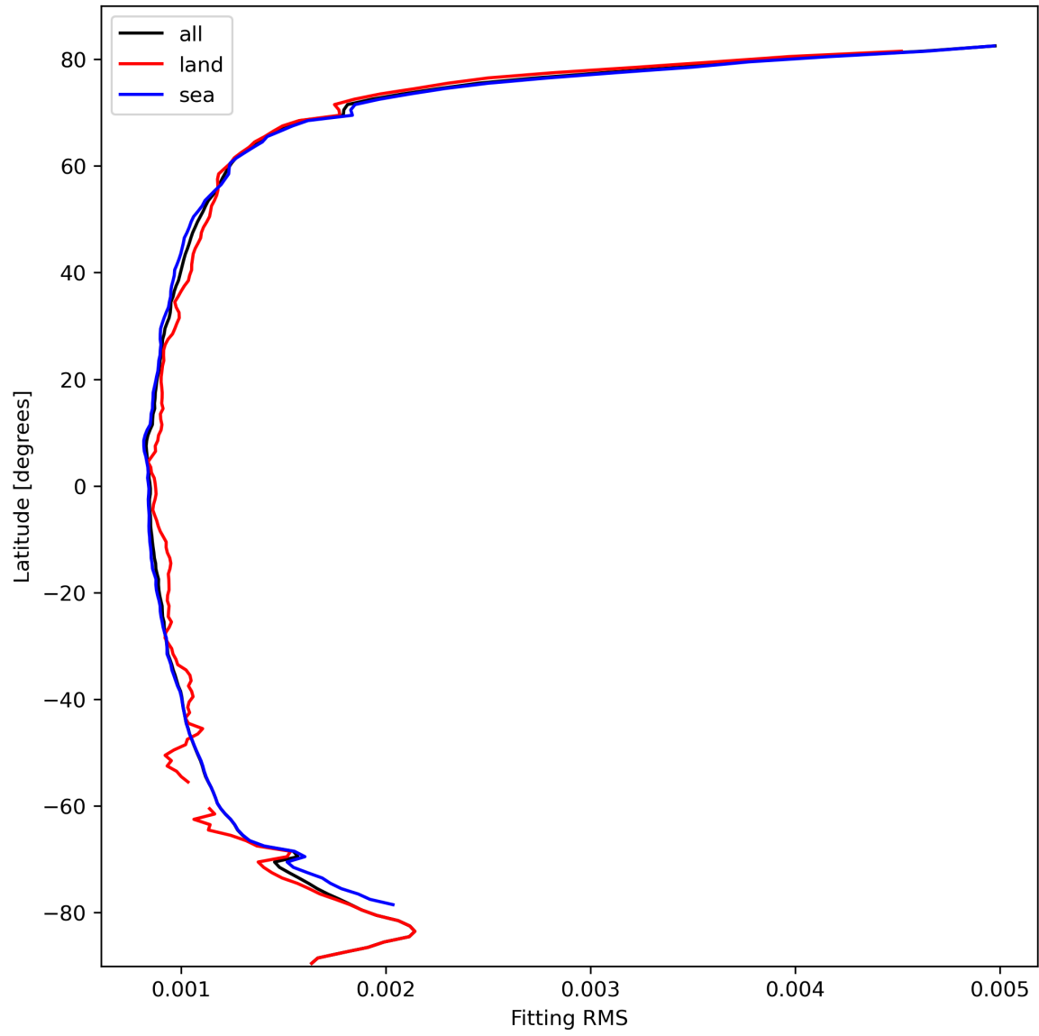
Figure 16: Zonal average of “Fitting RMS” for 2023-10-10 to 2023-10-12.
