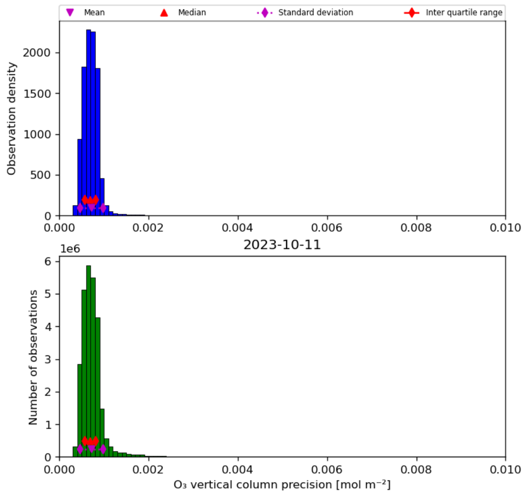
Figure 22: Histogram of “O 3 vertical column precision” for 2023-10-10 to 2023-10-12
