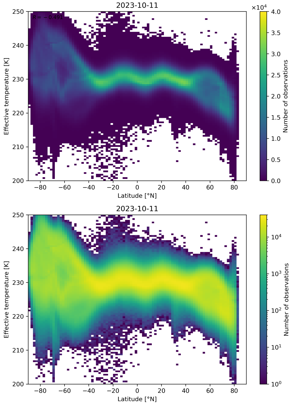
Figure 34: Scatter density plot of “Latitude” against “Effective temperature” for 2023-10-10 to 2023-10-12.
