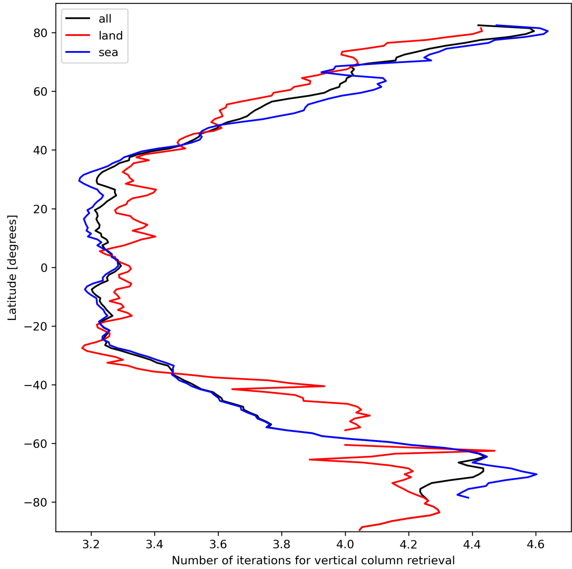
Figure 19: Zonal average of “Number of iterations for vertical column retrieval” for 2023-10-10 to 2023-10-12.
