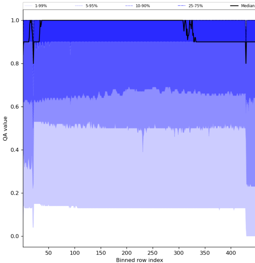
Figure 27: Along track statistics of “QA value” for 2023-10-10 to 2023-10-12
