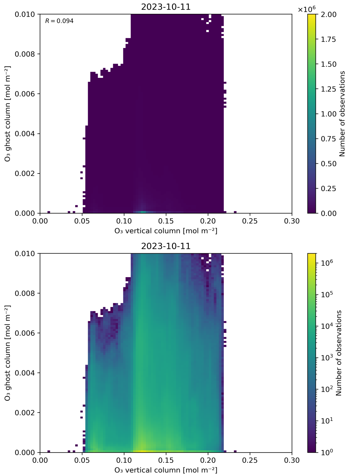
Figure 40: Scatter density plot of “O 3 vertical column” against “O 3 ghost column” for 2023-10-10 to 2023-10-12.
