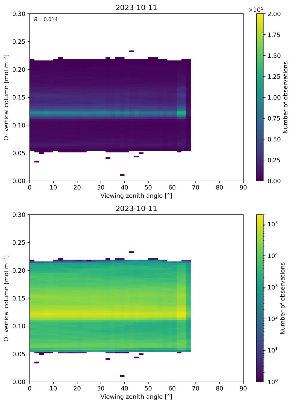
Figure 52: Scatter density plot of “Viewing zenith angle” against “O 3 vertical column” for 2023-10-10 to 2023-10-12.
