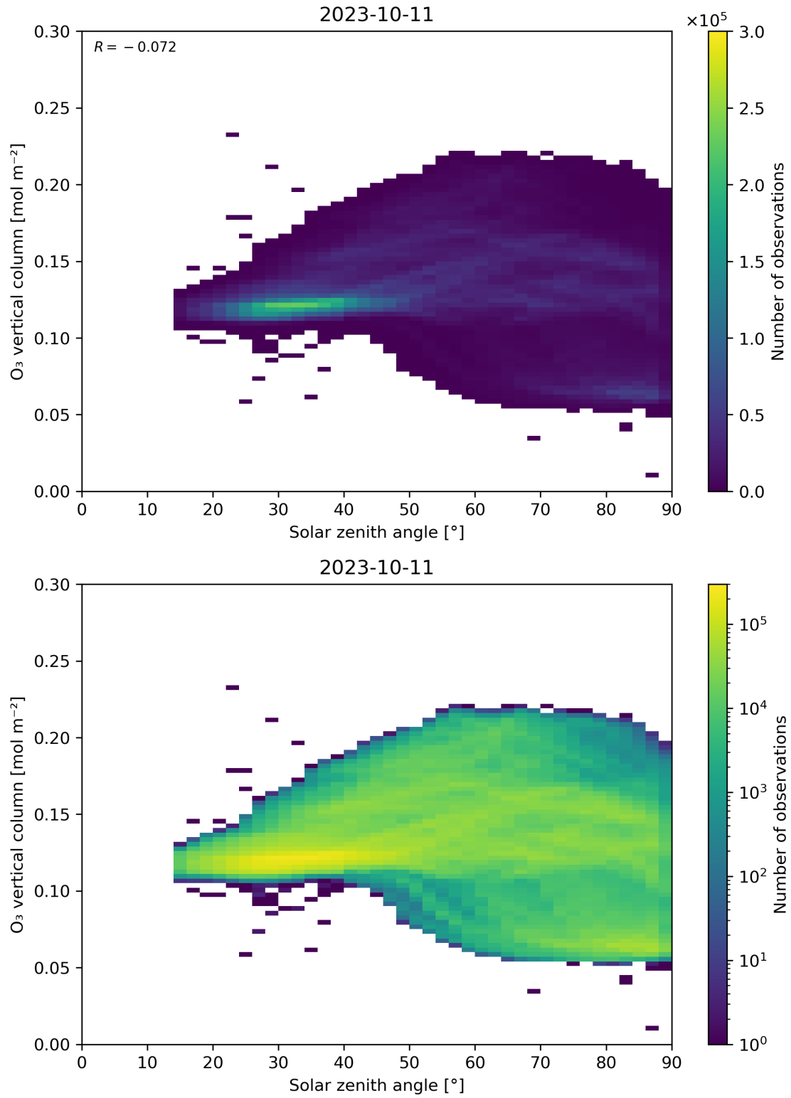
Figure 47: Scatter density plot of “Solar zenith angle” against “O 3 vertical column” for 2023-10-10 to 2023-10-12.
