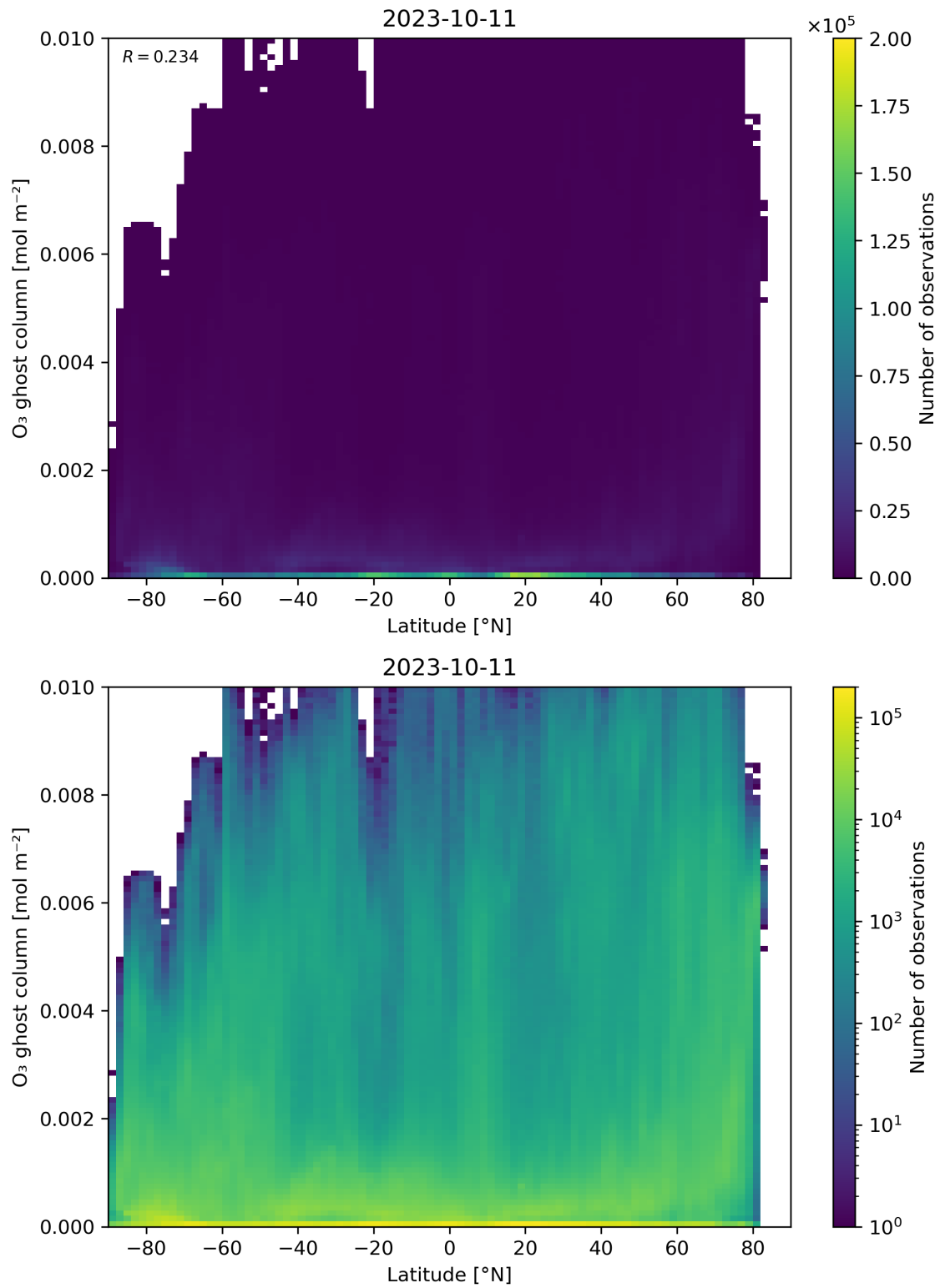
Figure 35: Scatter density plot of “Latitude” against “O 3 ghost column” for 2023-10-10 to 2023-10-12.
