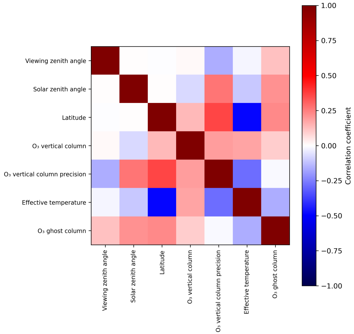
Figure 2: Map of correlation matrix for 2023-10-10 to 2023-10-12.
