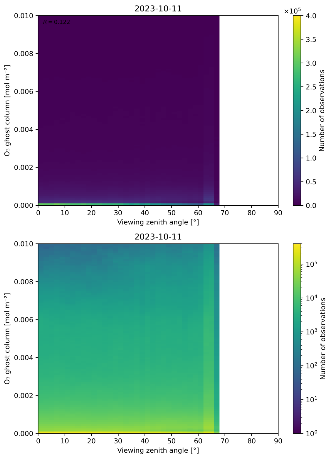
Figure 51: Scatter density plot of “Viewing zenith angle” against “O 3 ghost column” for 2023-10-10 to 2023-10-12.
