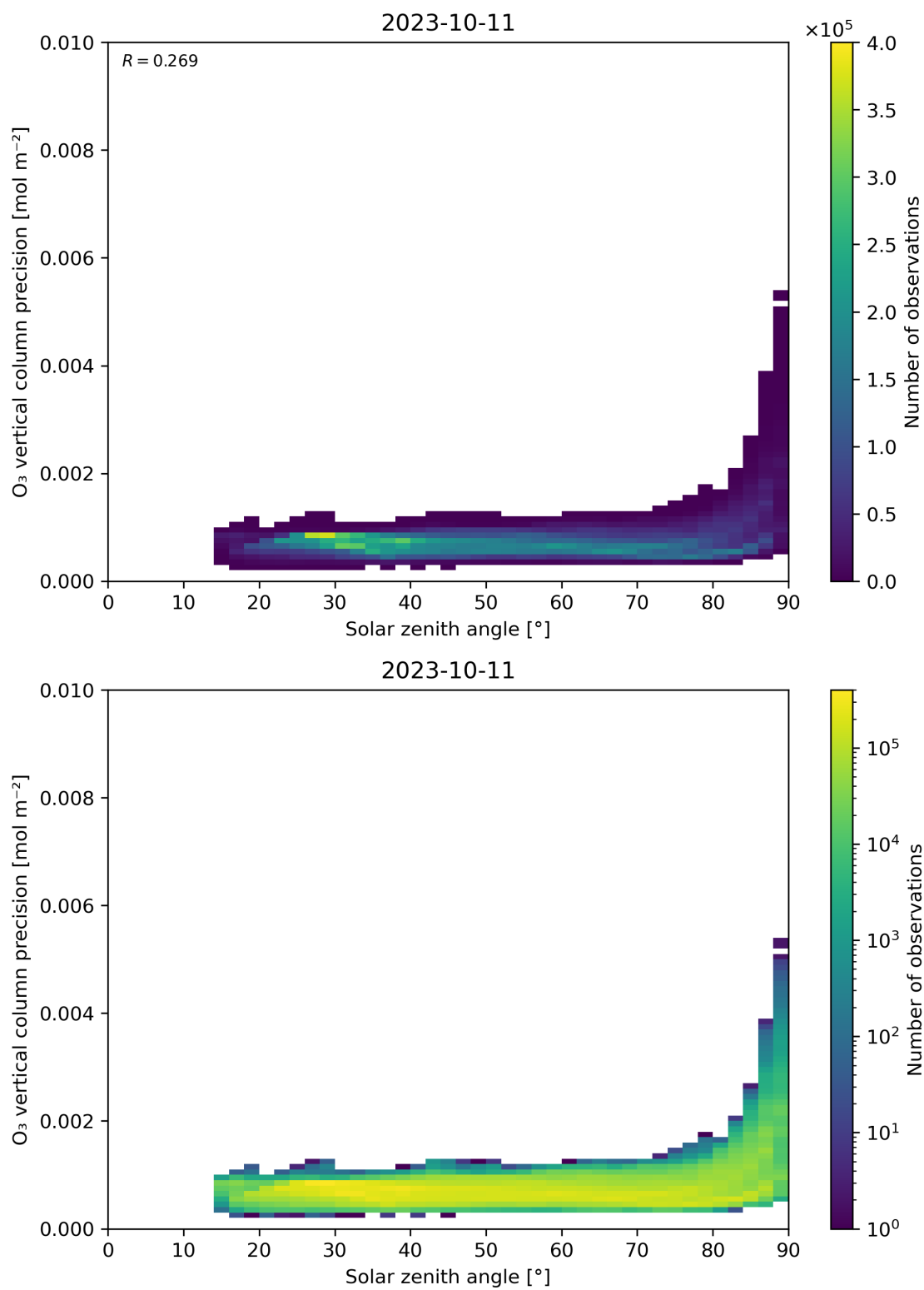
Figure 48: Scatter density plot of “Solar zenith angle” against “O 3 vertical column precision” for 2023-10-10 to 2023-10-12.
