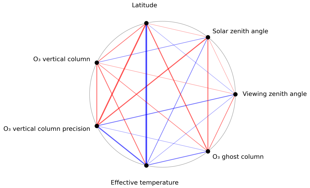
Figure 1: Map of correlation graph for 2023-10-10 to 2023-10-12.
