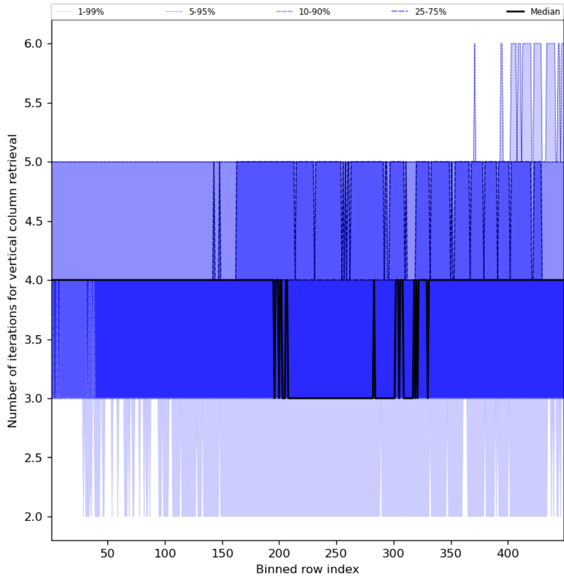
Figure 33: Along track statistics of “Number of iterations for vertical column retrieval” for 2023-10-10 to 2023-10-12
