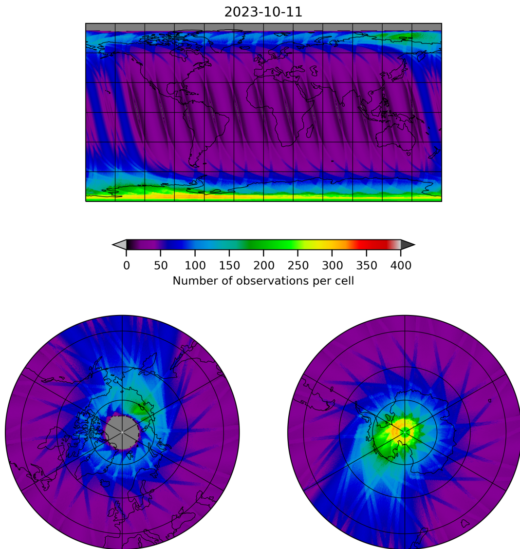
Figure 12: Map of the number of observations for 2023-10-10 to 2023-10-12
