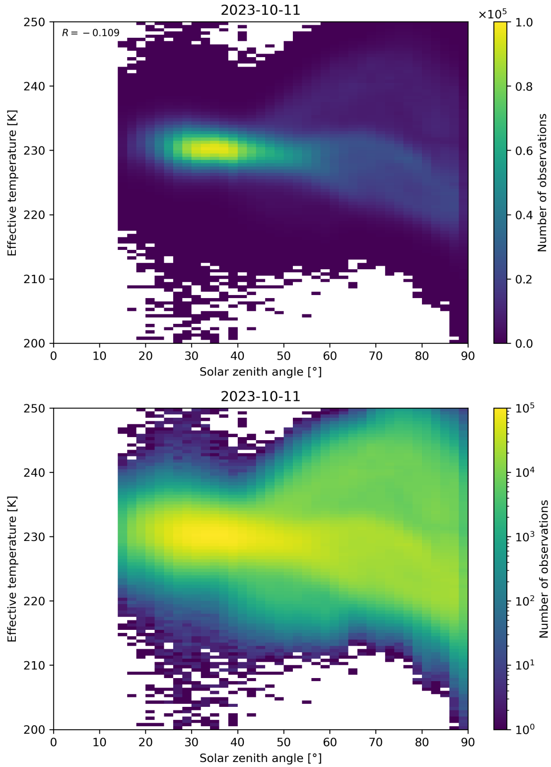
Figure 45: Scatter density plot of “Solar zenith angle” against “Effective temperature” for 2023-10-10 to 2023-10-12.
