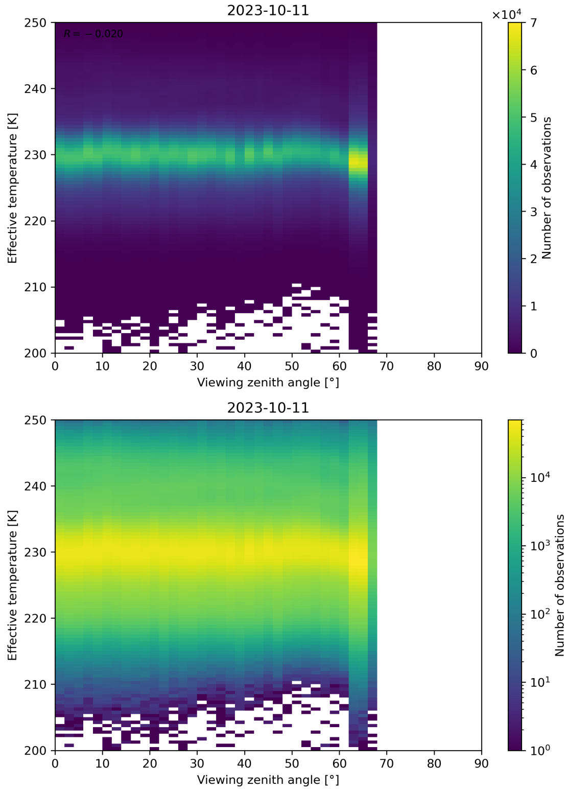
Figure 50: Scatter density plot of “Viewing zenith angle” against “Effective temperature” for 2023-10-10 to 2023-10-12.
