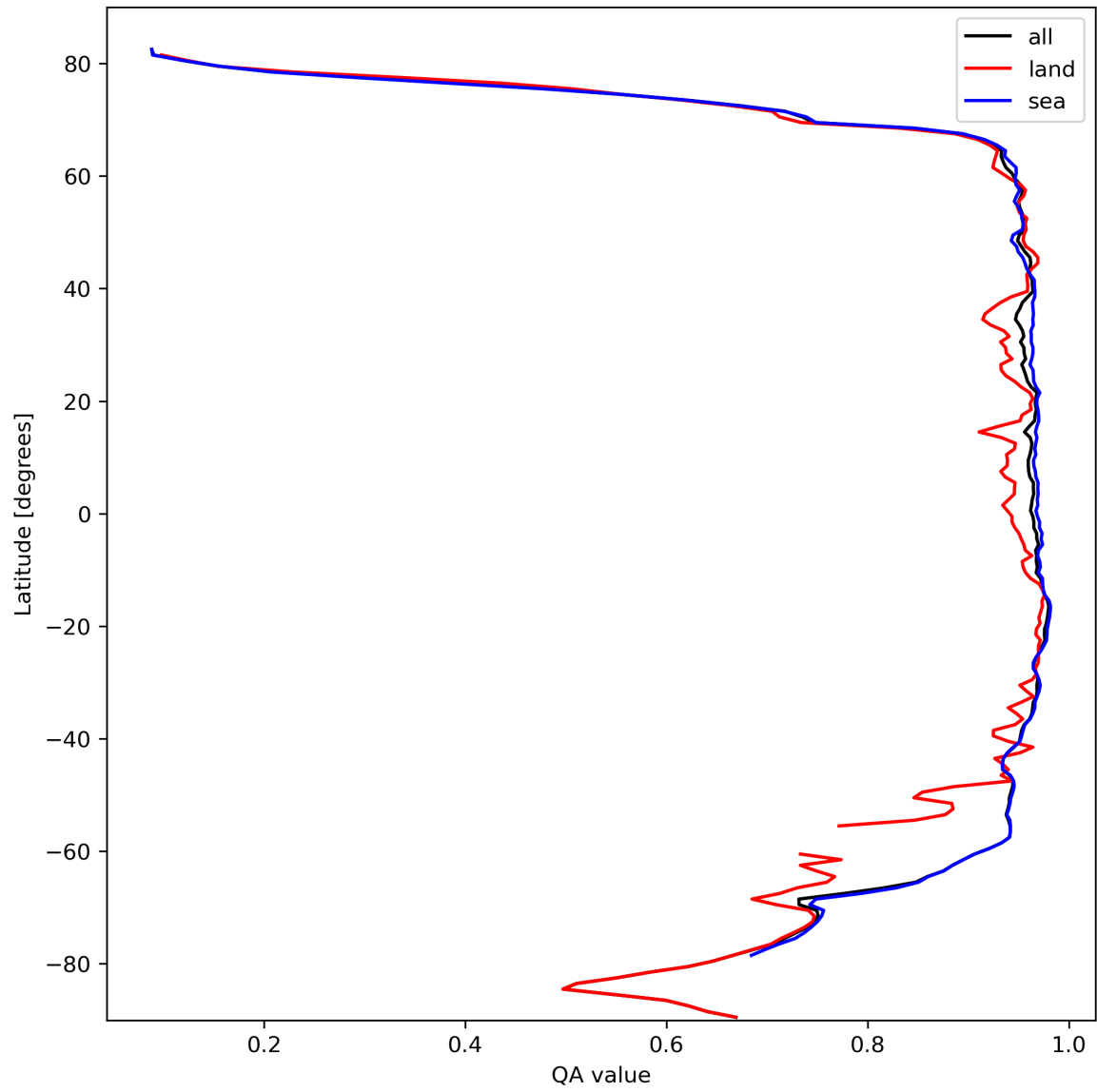
Figure 13: Zonal average of “QA value” for 2023-10-10 to 2023-10-12.
