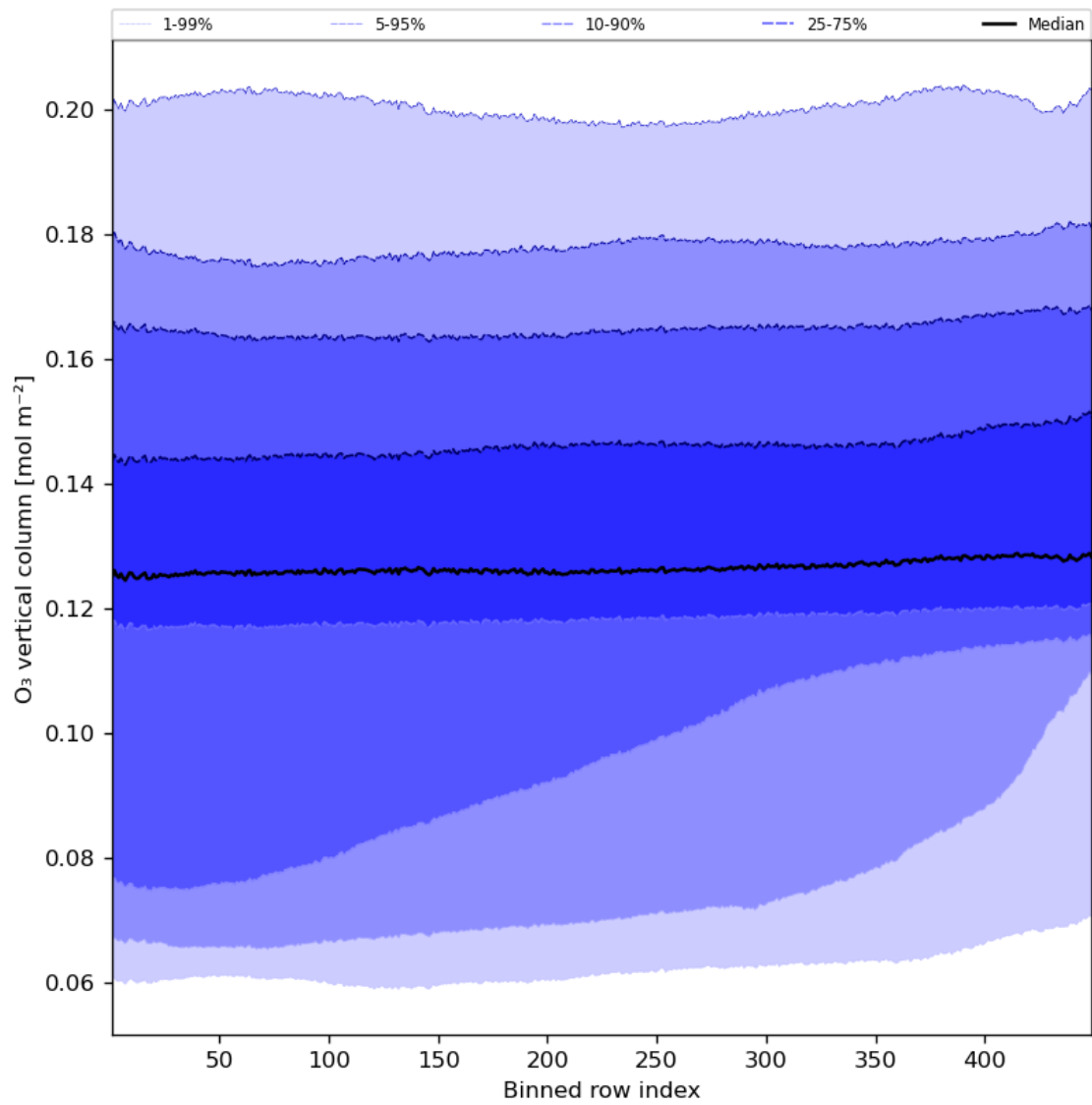
Figure 28: Along track statistics of “O 3 vertical column” for 2023-10-10 to 2023-10-12
