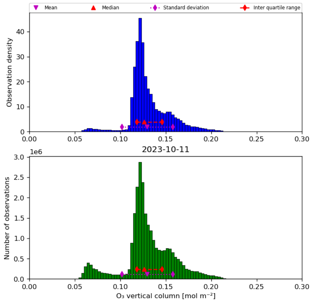
Figure 21: Histogram of “O 3 vertical column” for 2023-10-10 to 2023-10-12
