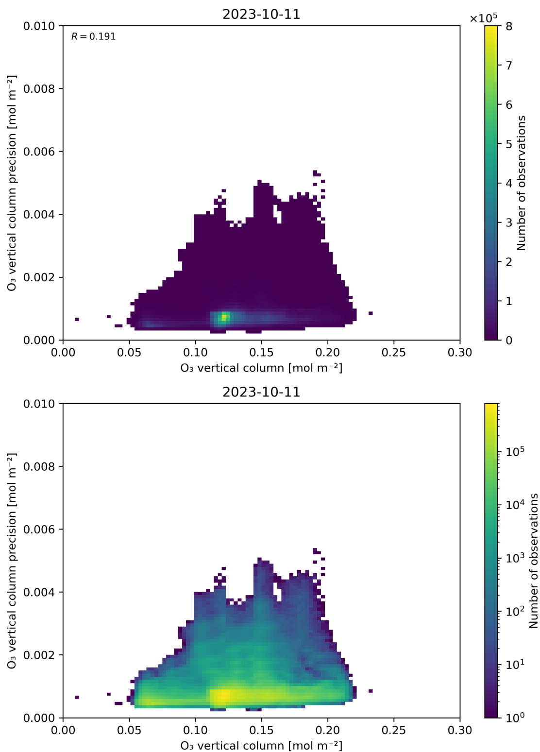
Figure 41: Scatter density plot of “O 3 vertical column” against “O 3 vertical column precision” for 2023-10-10 to 2023-10-12.
