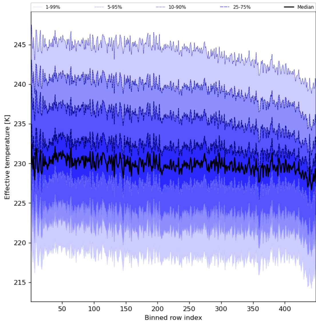
Figure 31: Along track statistics of “Effective temperature” for 2023-10-10 to 2023-10-12
